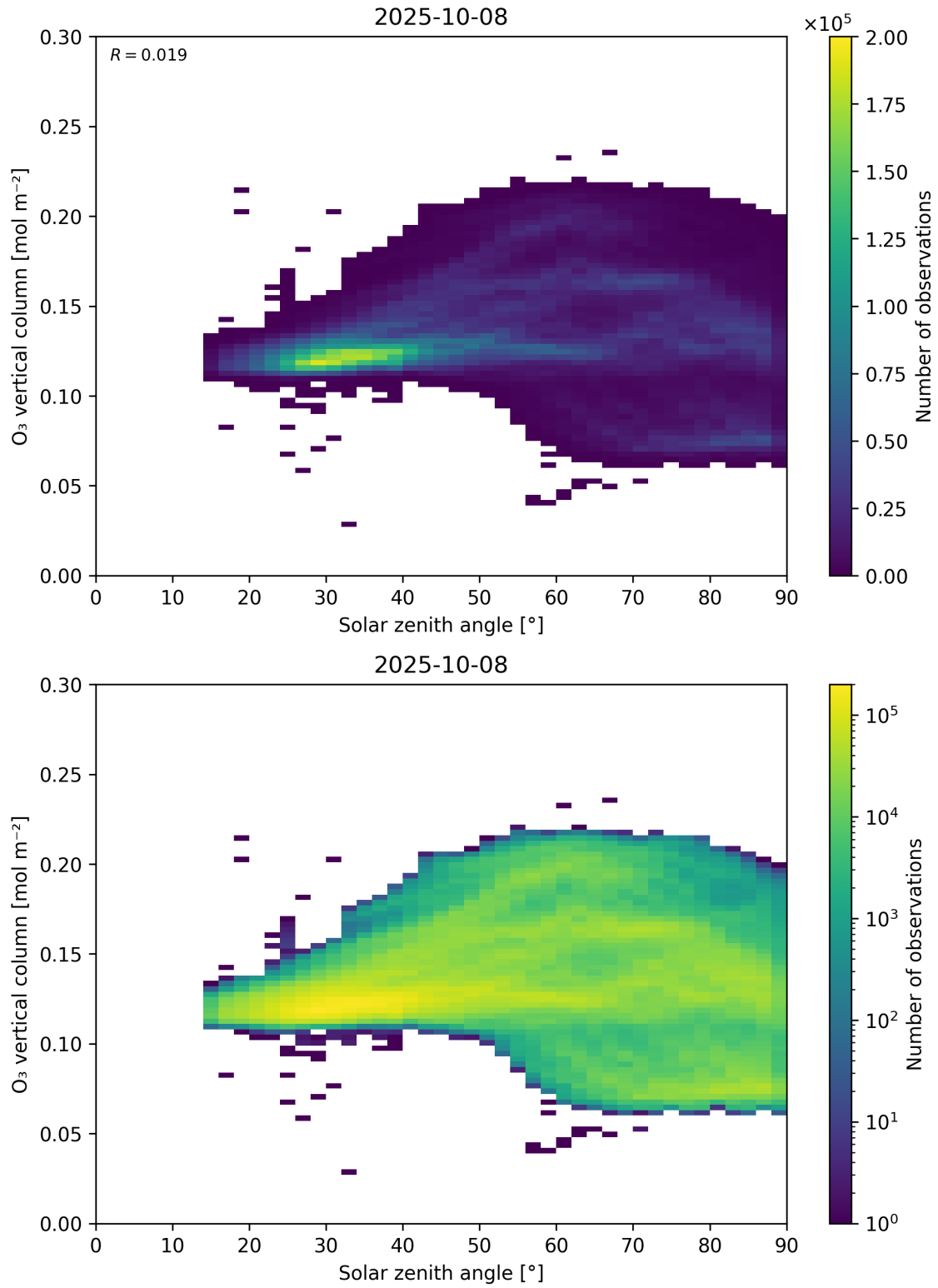
Figure 47: Scatter density plot of “Solar zenith angle” against “O 3 vertical column” for 2025-10-07 to 2025-10-09.
