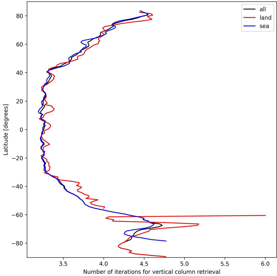
Figure 19: Zonal average of “Number of iterations for vertical column retrieval” for 2025-10-07 to 2025-10-09.
