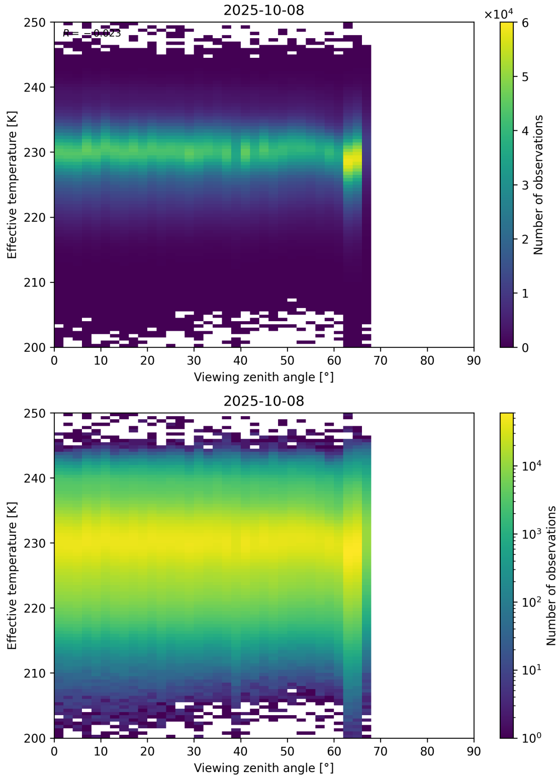
Figure 50: Scatter density plot of “Viewing zenith angle” against “Effective temperature” for 2025-10-07 to 2025-10-09.
