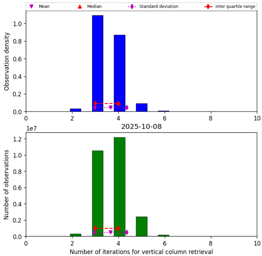
Figure 26: Histogram of “Number of iterations for vertical column retrieval” for 2025-10-07 to 2025-10-09
