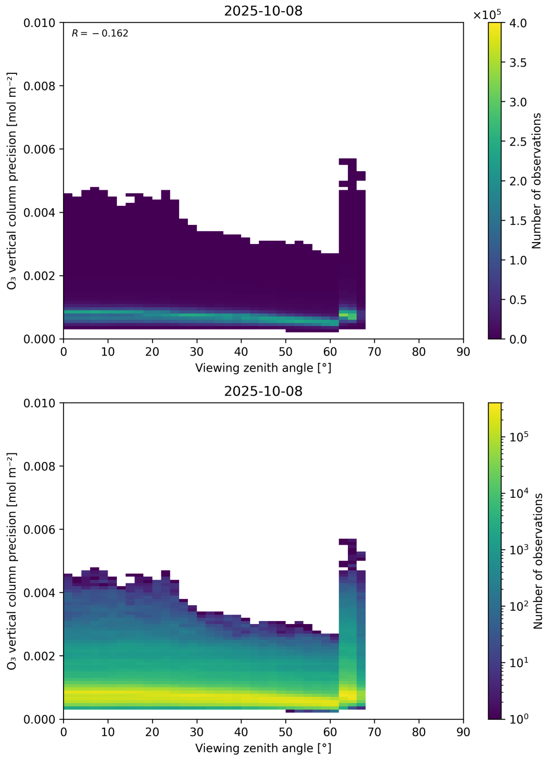
Figure 53: Scatter density plot of “Viewing zenith angle” against “O 3 vertical column precision” for 2025-10-07 to 2025-10-09.
