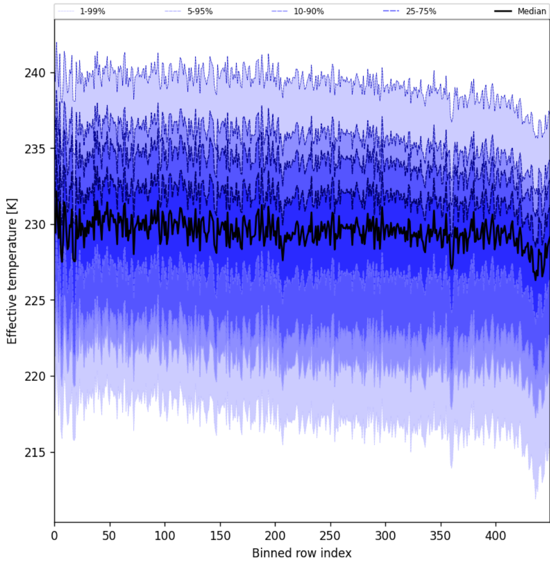
Figure 31: Along track statistics of “Effective temperature” for 2025-10-07 to 2025-10-09
