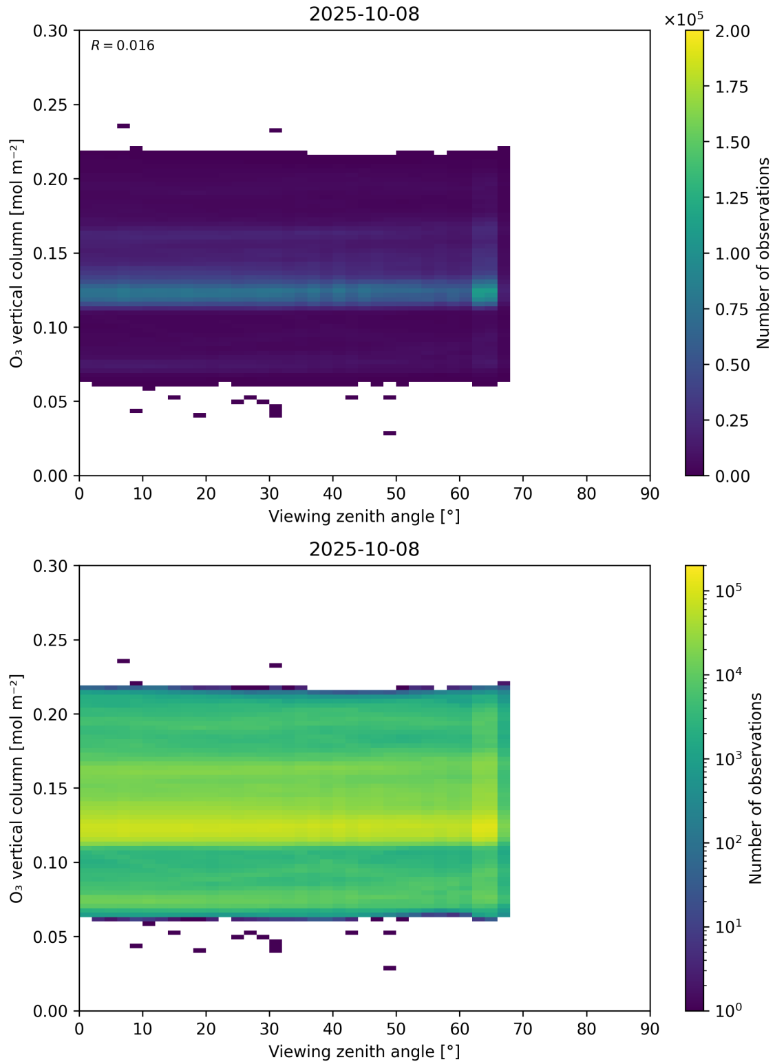
Figure 52: Scatter density plot of “Viewing zenith angle” against “O 3 vertical column” for 2025-10-07 to 2025-10-09.
