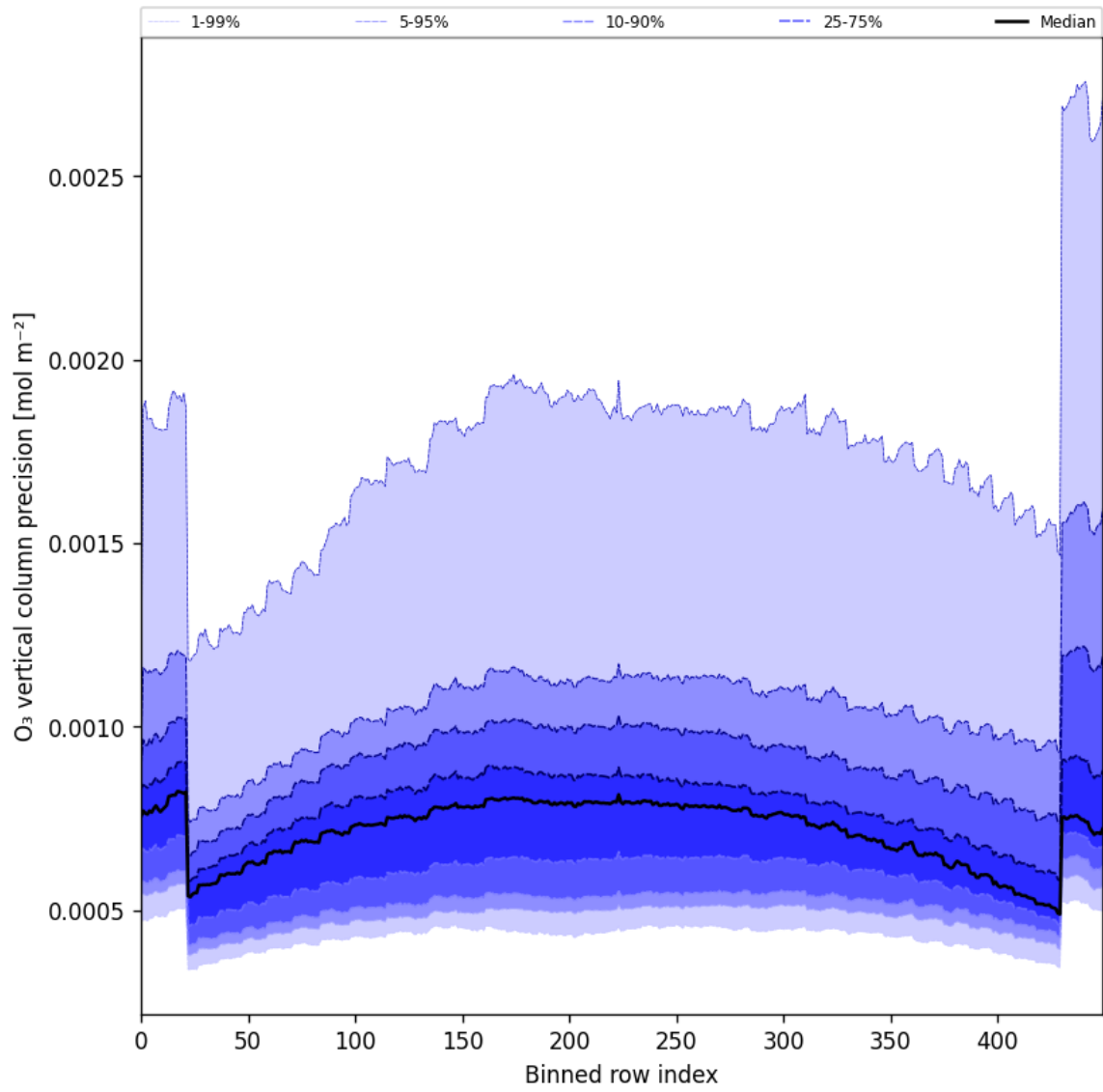
Figure 29: Along track statistics of “O 3 vertical column precision” for 2025-10-07 to 2025-10-09
