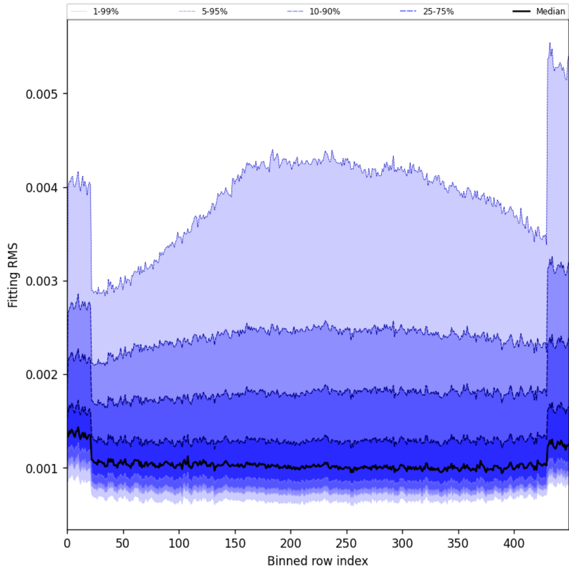
Figure 30: Along track statistics of “Fitting RMS” for 2025-10-07 to 2025-10-09
