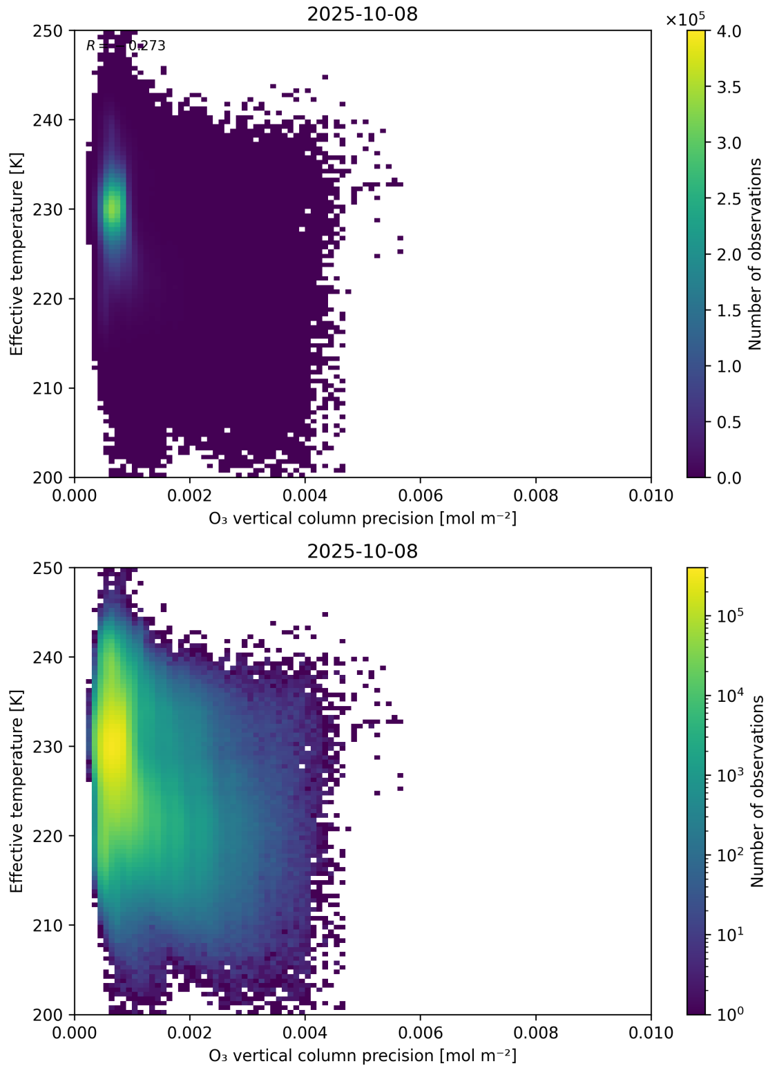
Figure 42: Scatter density plot of “O 3 vertical column precision” against “Effective temperature” for 2025-10-07 to 2025-10-09.
