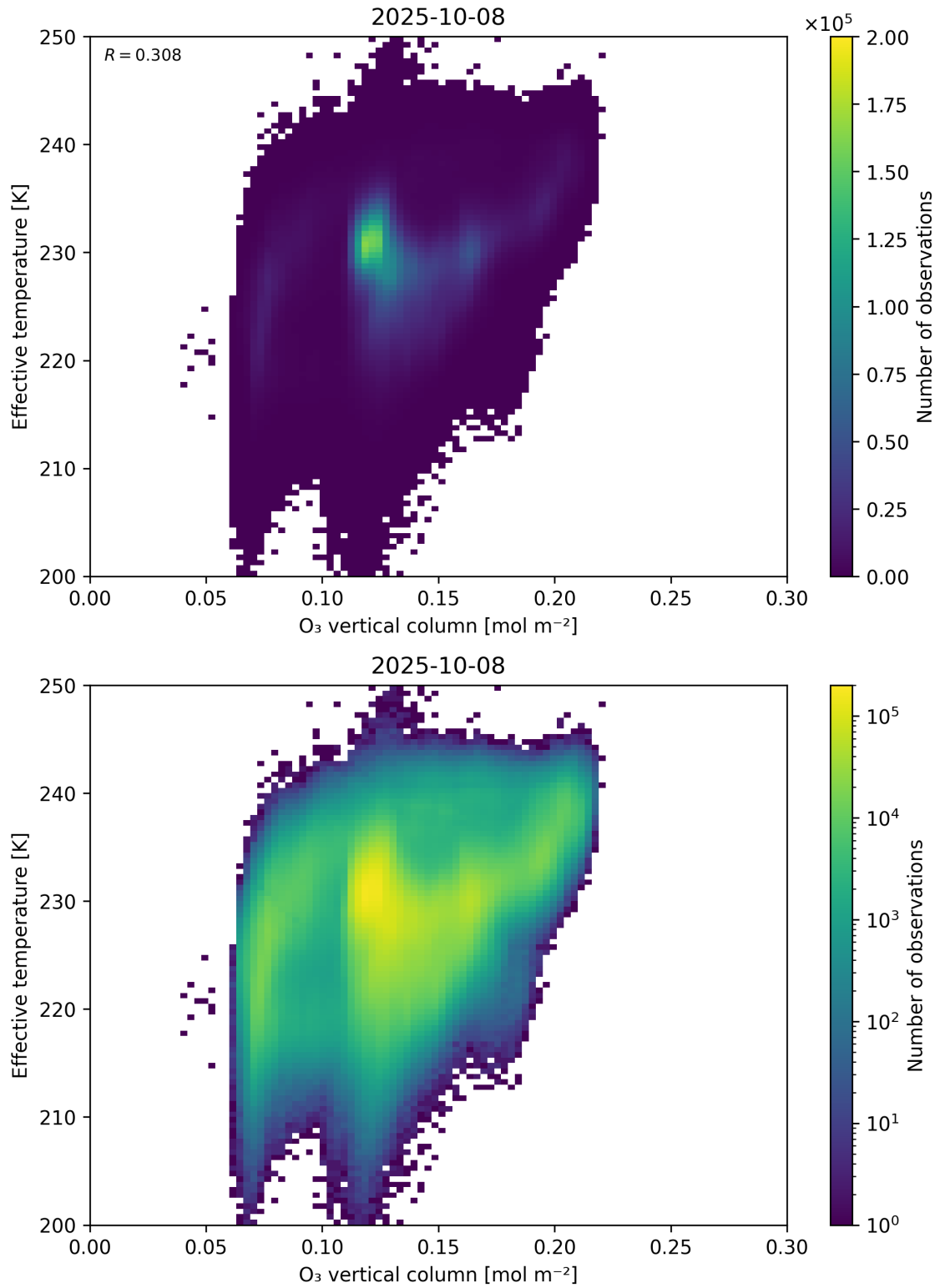
Figure 39: Scatter density plot of “O 3 vertical column” against “Effective temperature” for 2025-10-07 to 2025-10-09.
