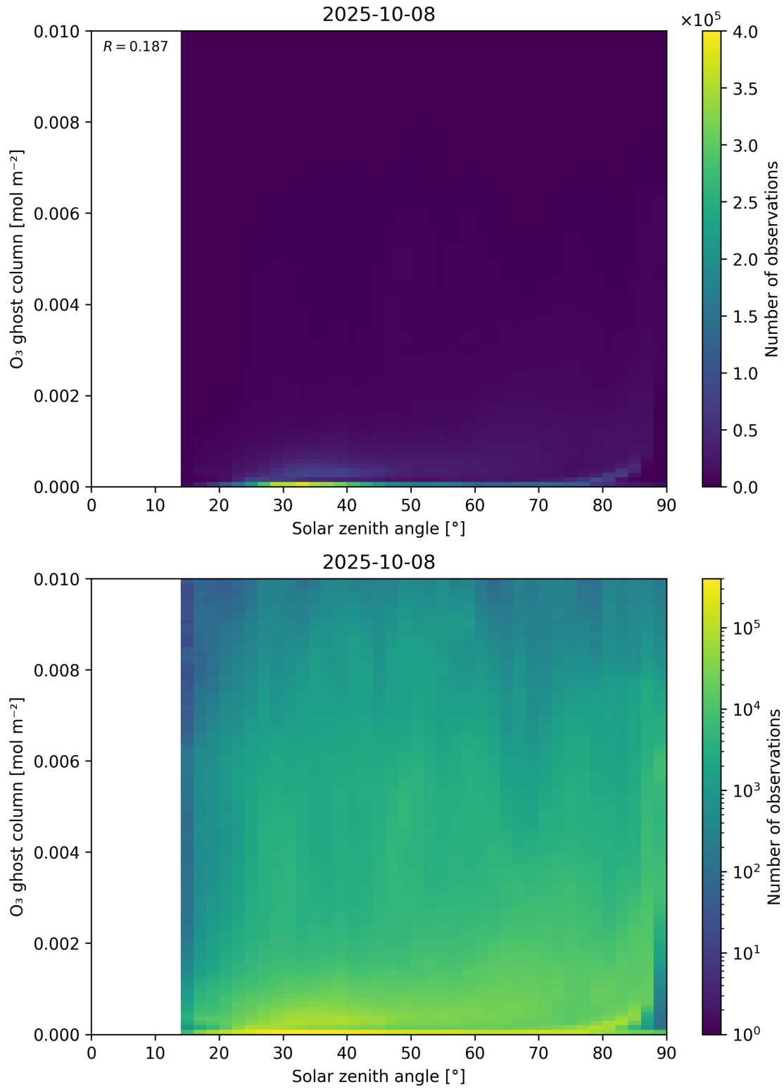
Figure 46: Scatter density plot of “Solar zenith angle” against “O 3 ghost column” for 2025-10-07 to 2025-10-09.
