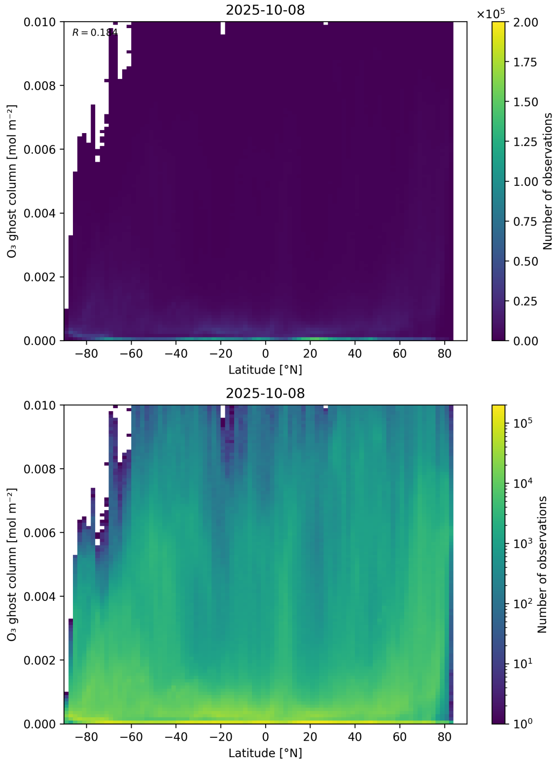
Figure 35: Scatter density plot of “Latitude” against “O 3 ghost column” for 2025-10-07 to 2025-10-09.
