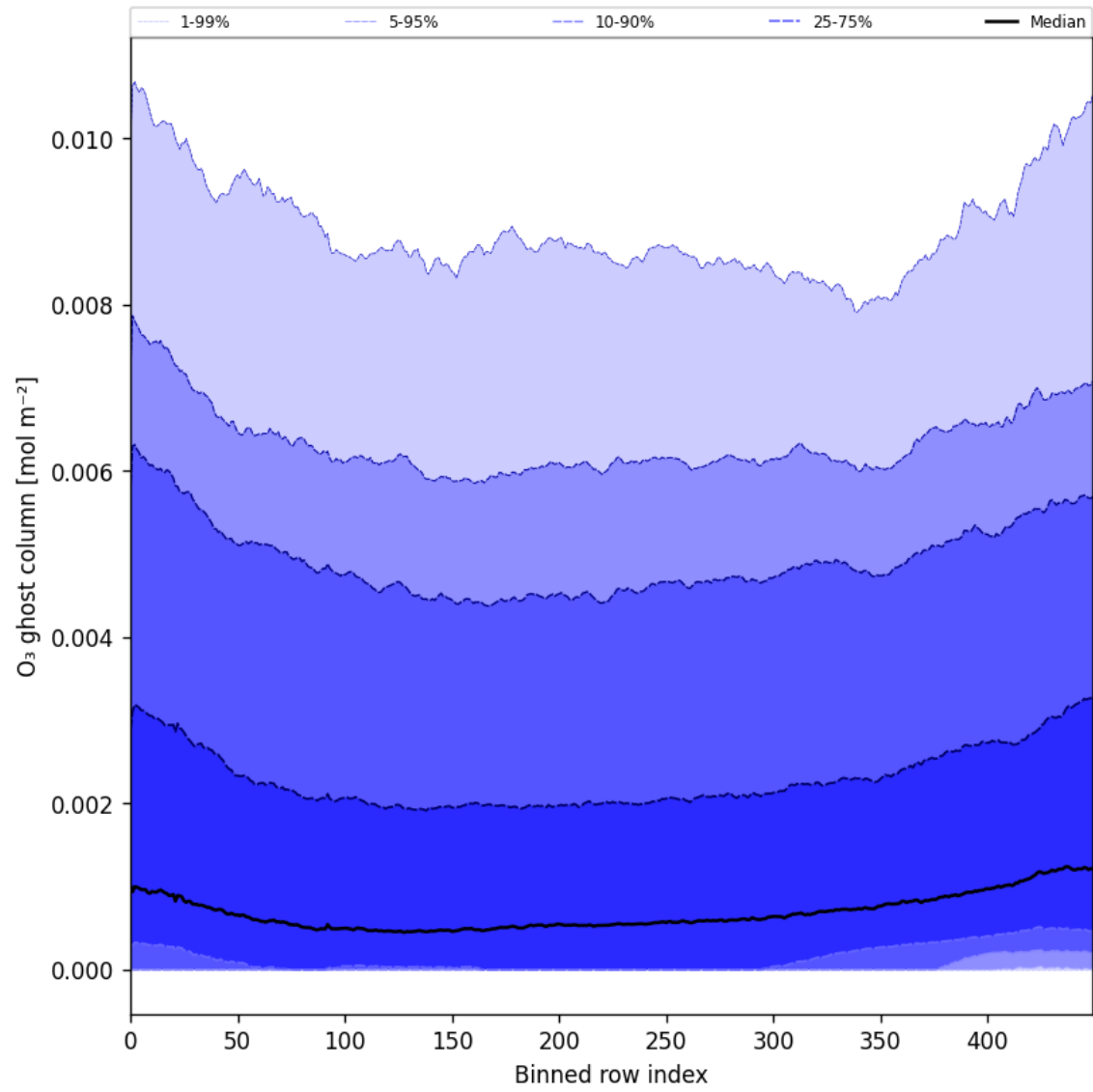
Figure 32: Along track statistics of “O 3 ghost column” for 2025-10-07 to 2025-10-09
