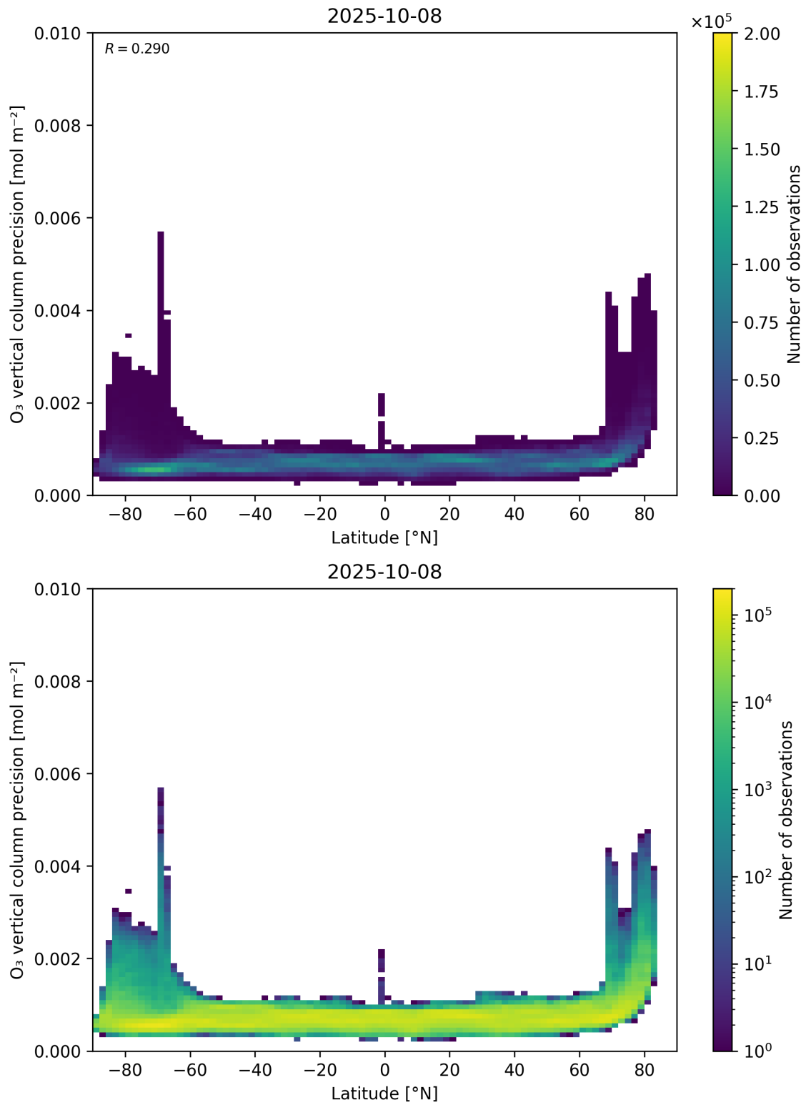
Figure 37: Scatter density plot of “Latitude” against “O 3 vertical column precision” for 2025-10-07 to 2025-10-09.
