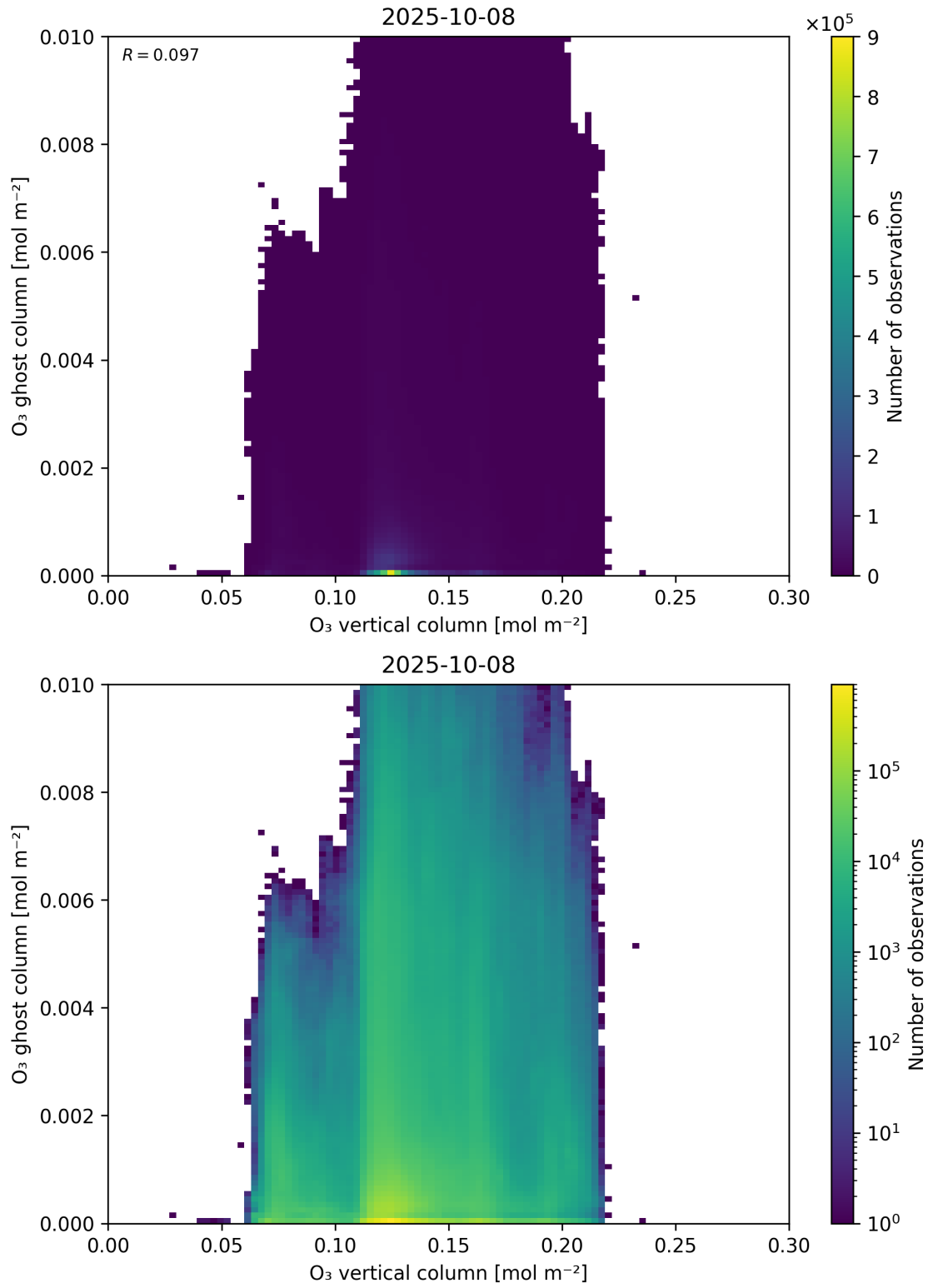
Figure 40: Scatter density plot of “O 3 vertical column” against “O 3 ghost column” for 2025-10-07 to 2025-10-09.
