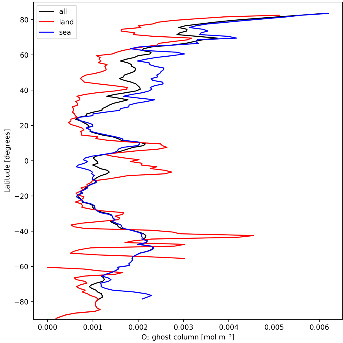
Figure 18: Zonal average of "O 3 ghost column" for 2025-10-07 to 2025-10-09.
