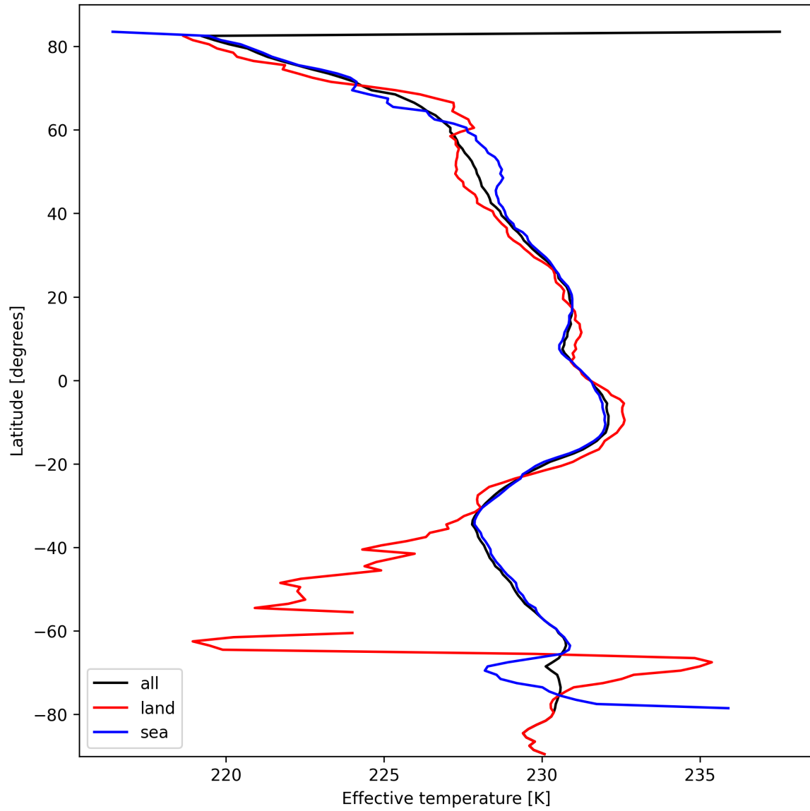
Figure 17: Zonal average of “Effective temperature” for 2025-10-07 to 2025-10-09.
