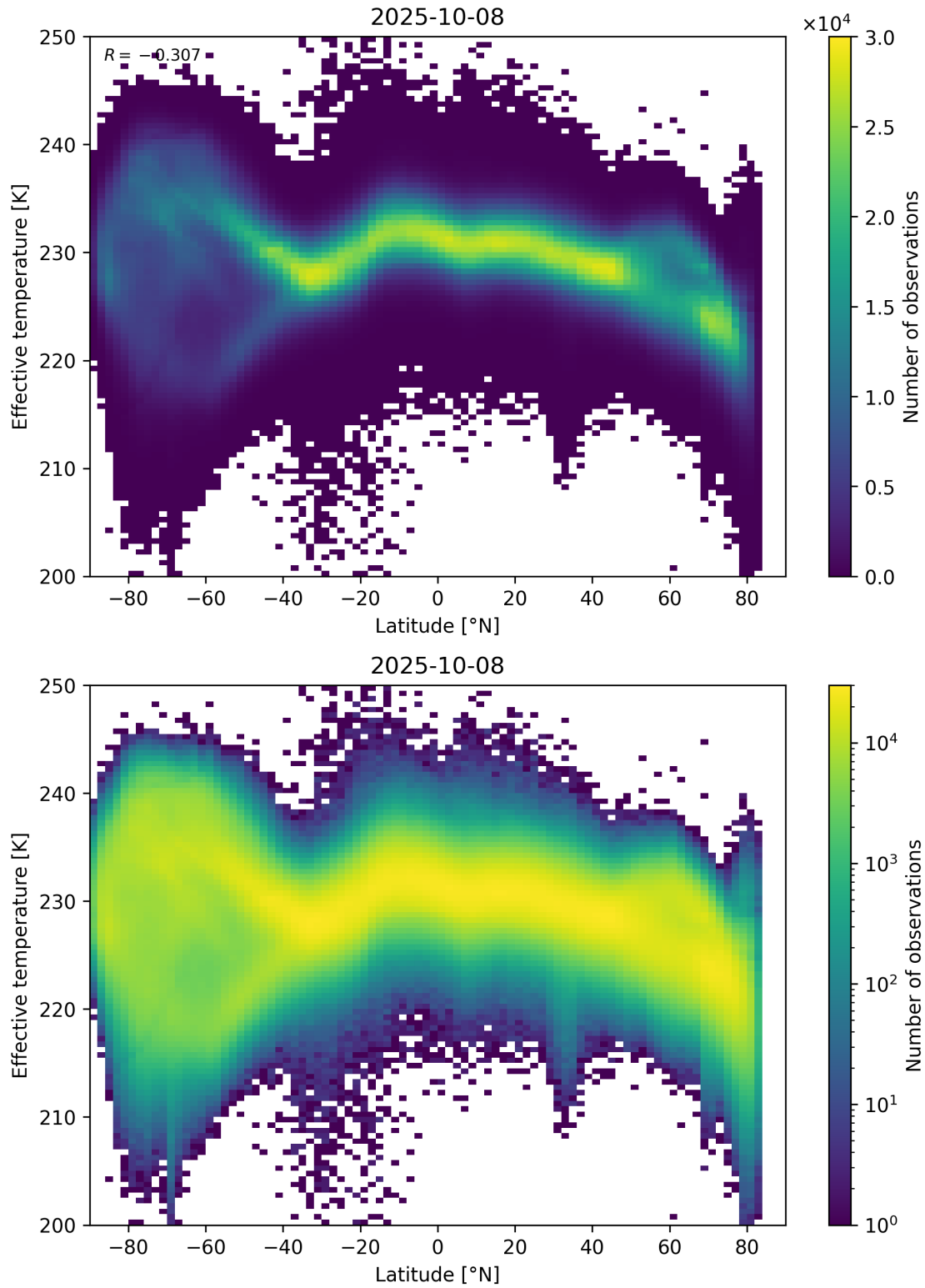
Figure 34: Scatter density plot of “Latitude” against “Effective temperature” for 2025-10-07 to 2025-10-09.
