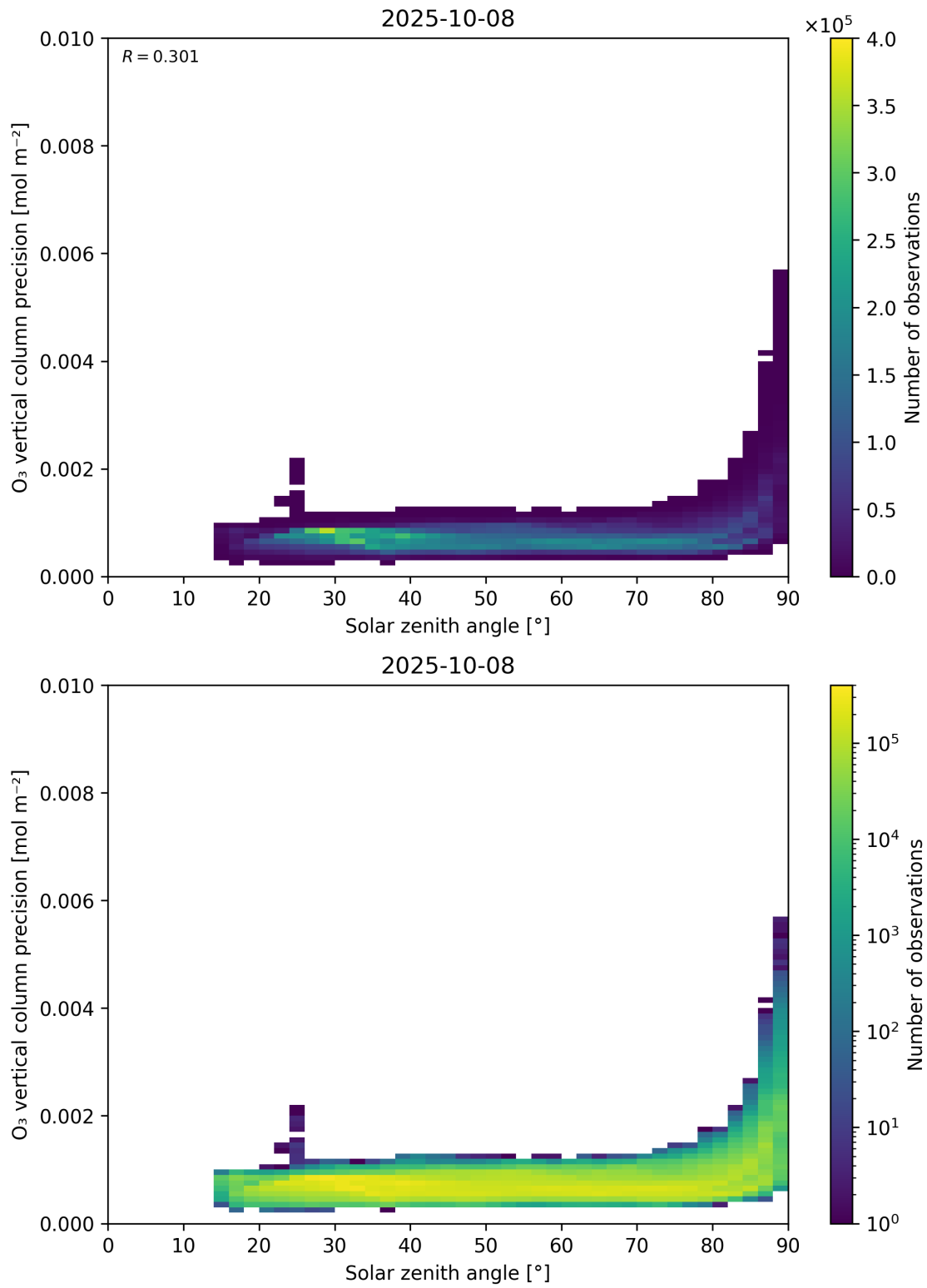
Figure 48: Scatter density plot of “Solar zenith angle” against “O 3 vertical column precision” for 2025-10-07 to 2025-10-09.
