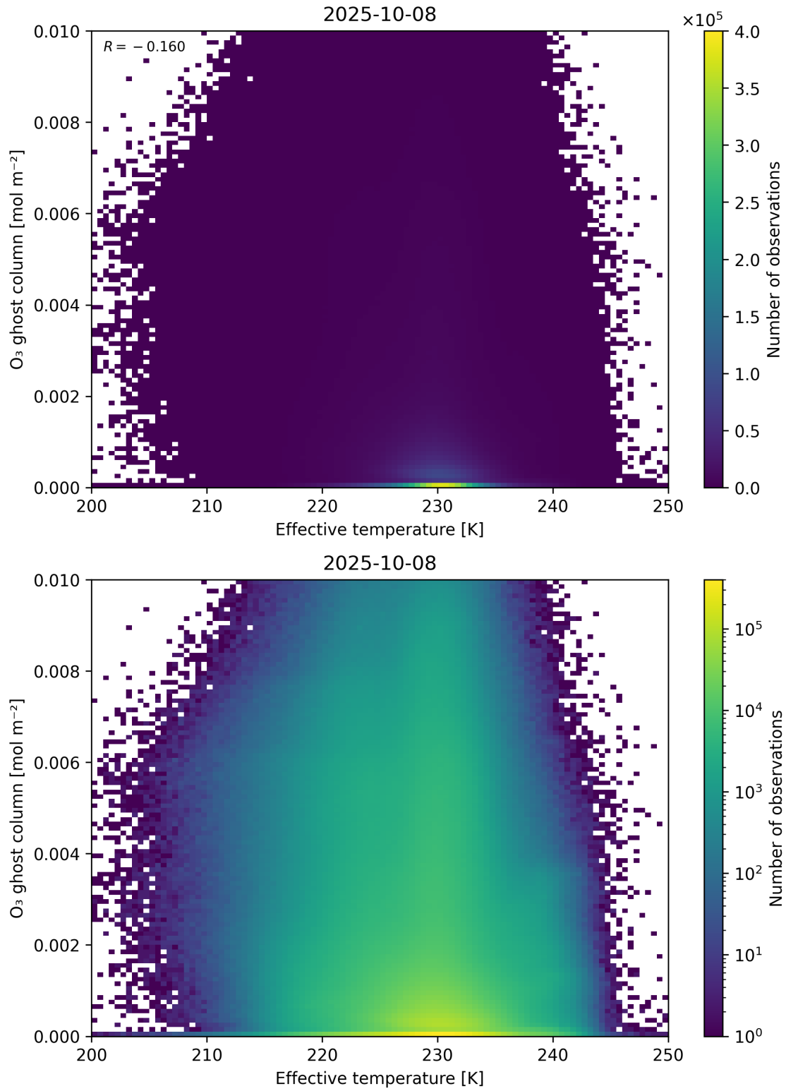
Figure 38: Scatter density plot of “Effective temperature” against “O 3 ghost column” for 2025-10-07 to 2025-10-09.
