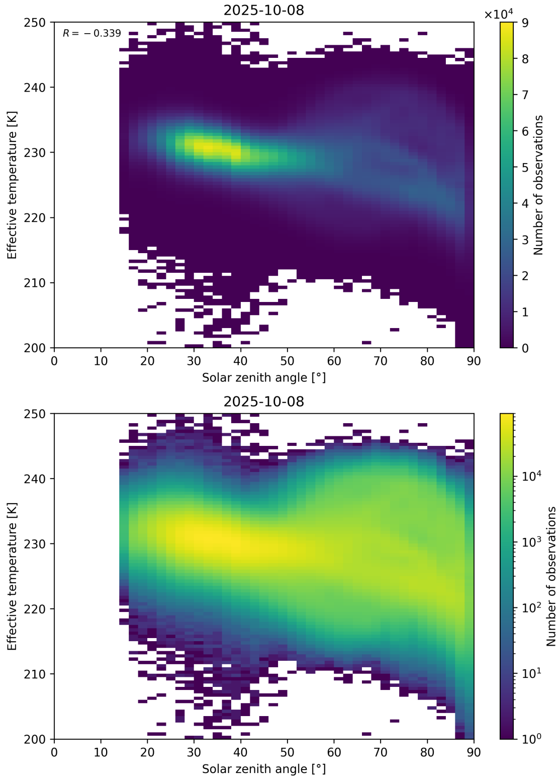
Figure 45: Scatter density plot of “Solar zenith angle” against “Effective temperature” for 2025-10-07 to 2025-10-09.
