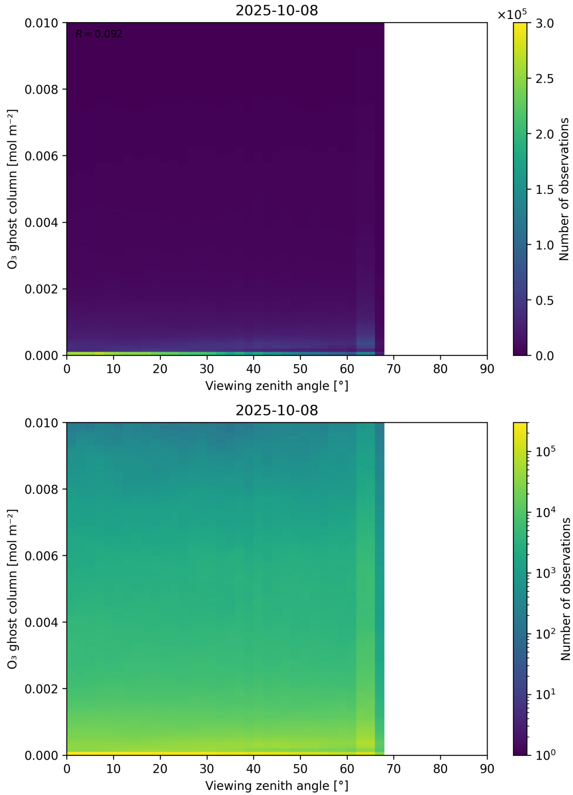
Figure 51: Scatter density plot of “Viewing zenith angle” against “O 3 ghost column” for 2025-10-07 to 2025-10-09.
