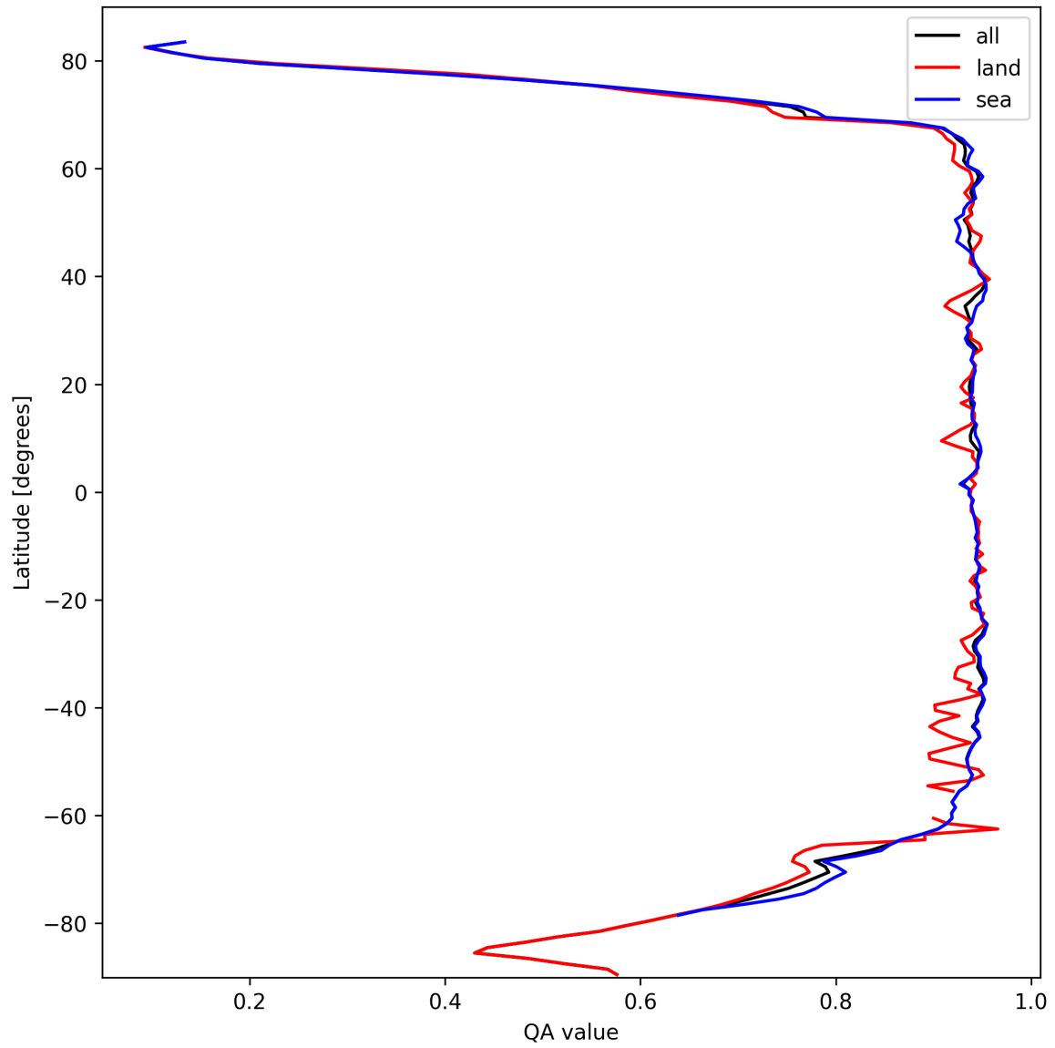
Figure 13: Zonal average of “QA value” for 2025-10-07 to 2025-10-09.
