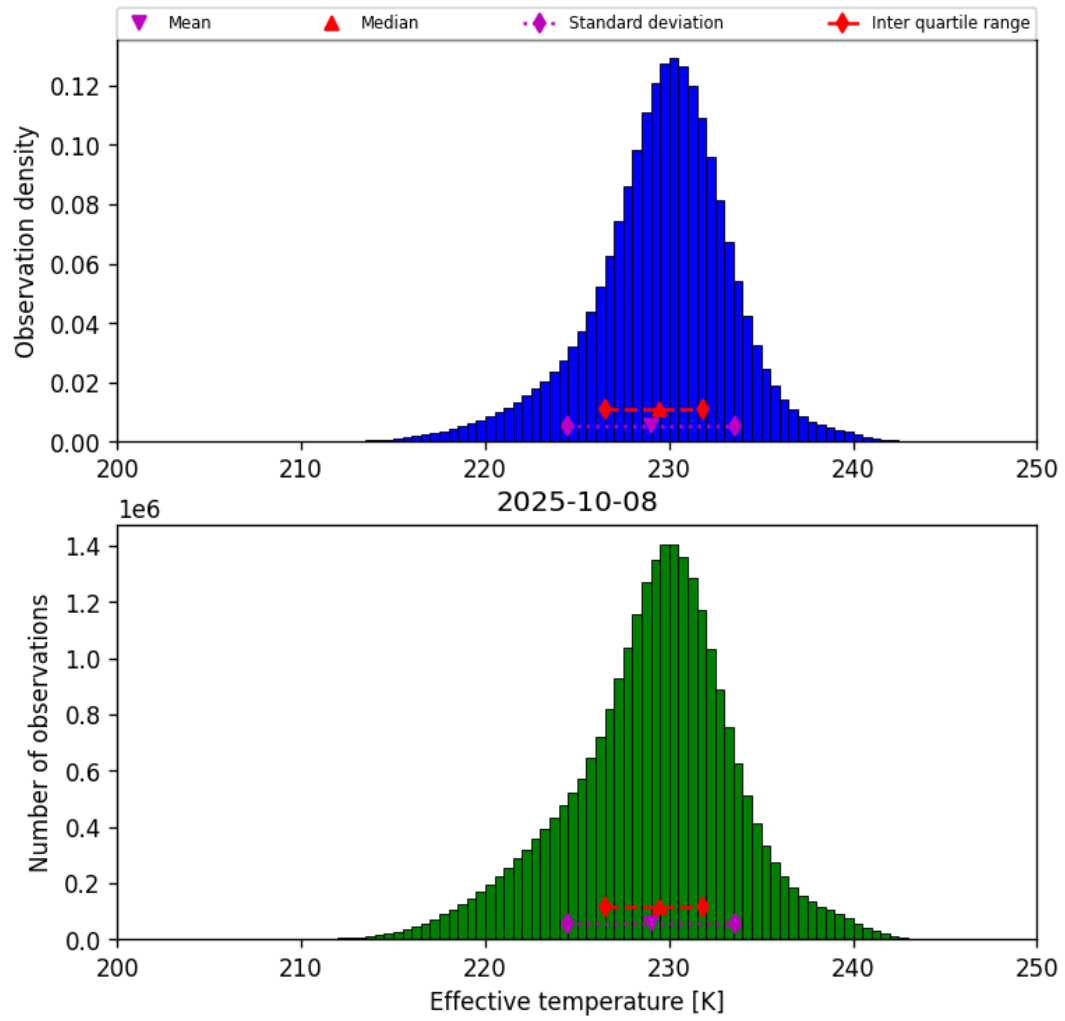
Figure 24: Histogram of “Effective temperature” for 2025-10-07 to 2025-10-09
