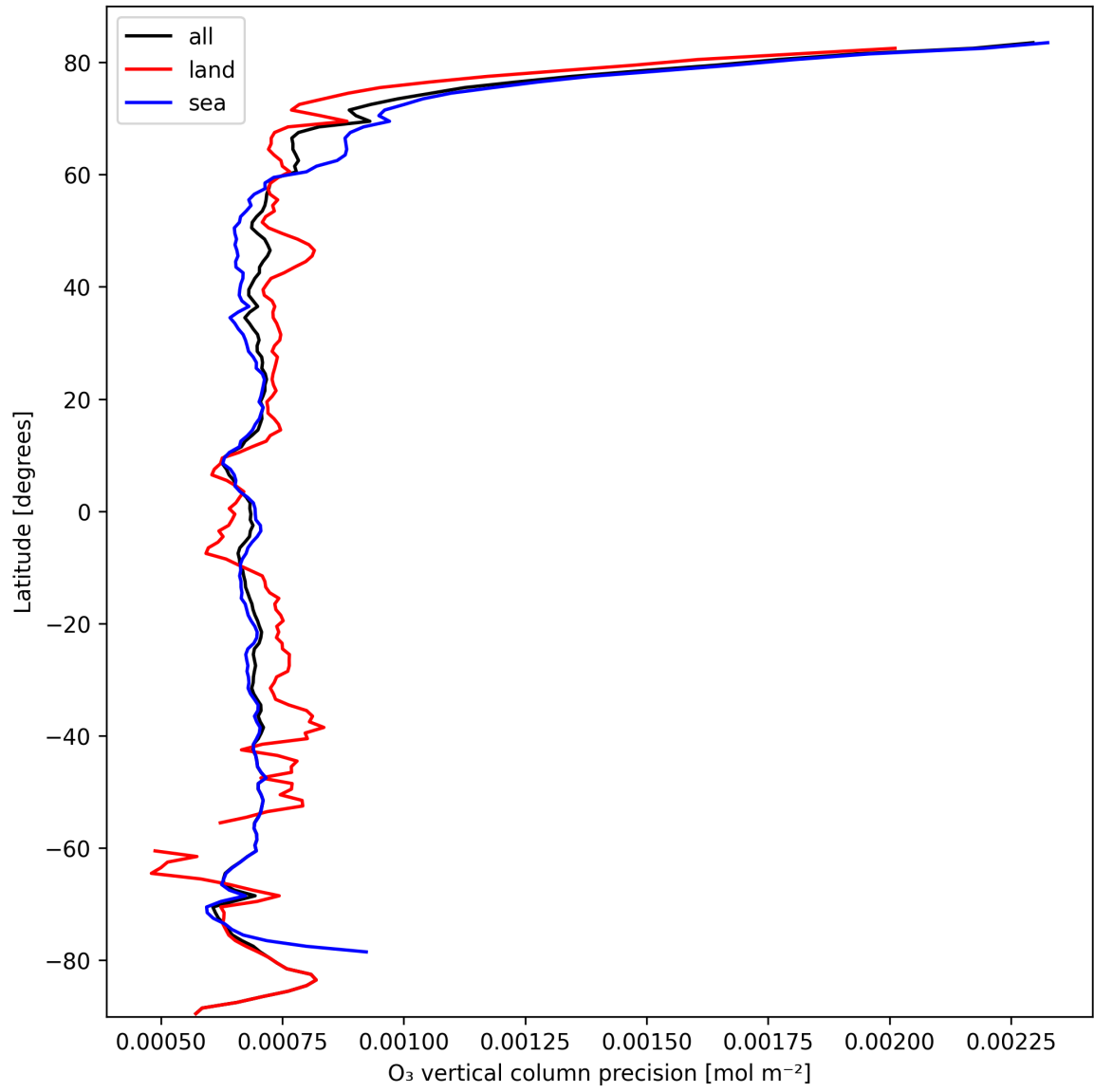
Figure 15: Zonal average of “O 3 vertical column precision” for 2025-10-07 to 2025-10-09.
