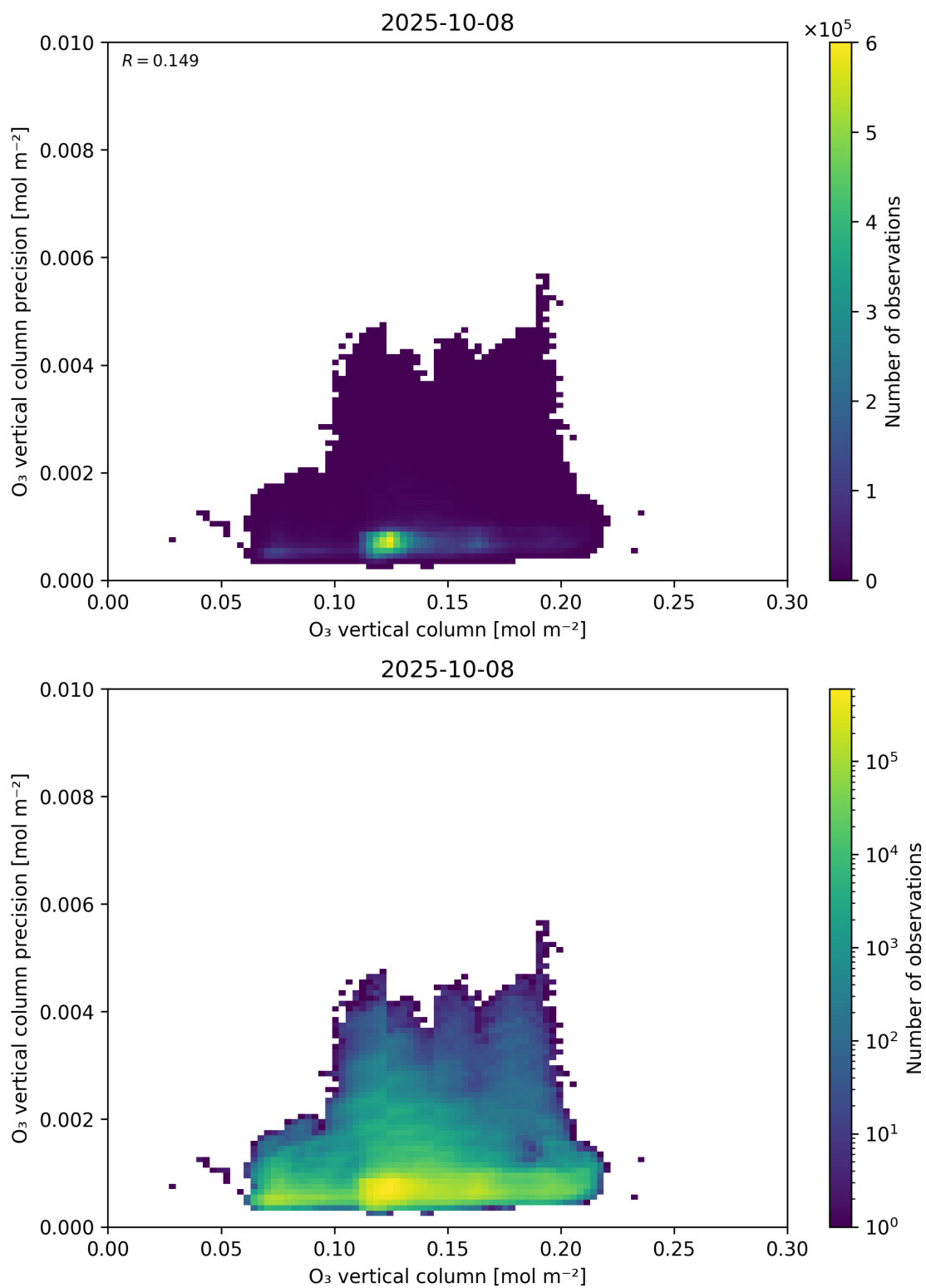
Figure 41: Scatter density plot of “O 3 vertical column” against “O 3 vertical column precision” for 2025-10-07 to 2025-10-09.
