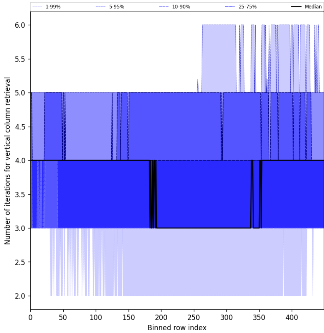
Figure 33: Along track statistics of “Number of iterations for vertical column retrieval” for 2025-10-07 to 2025-10-09
