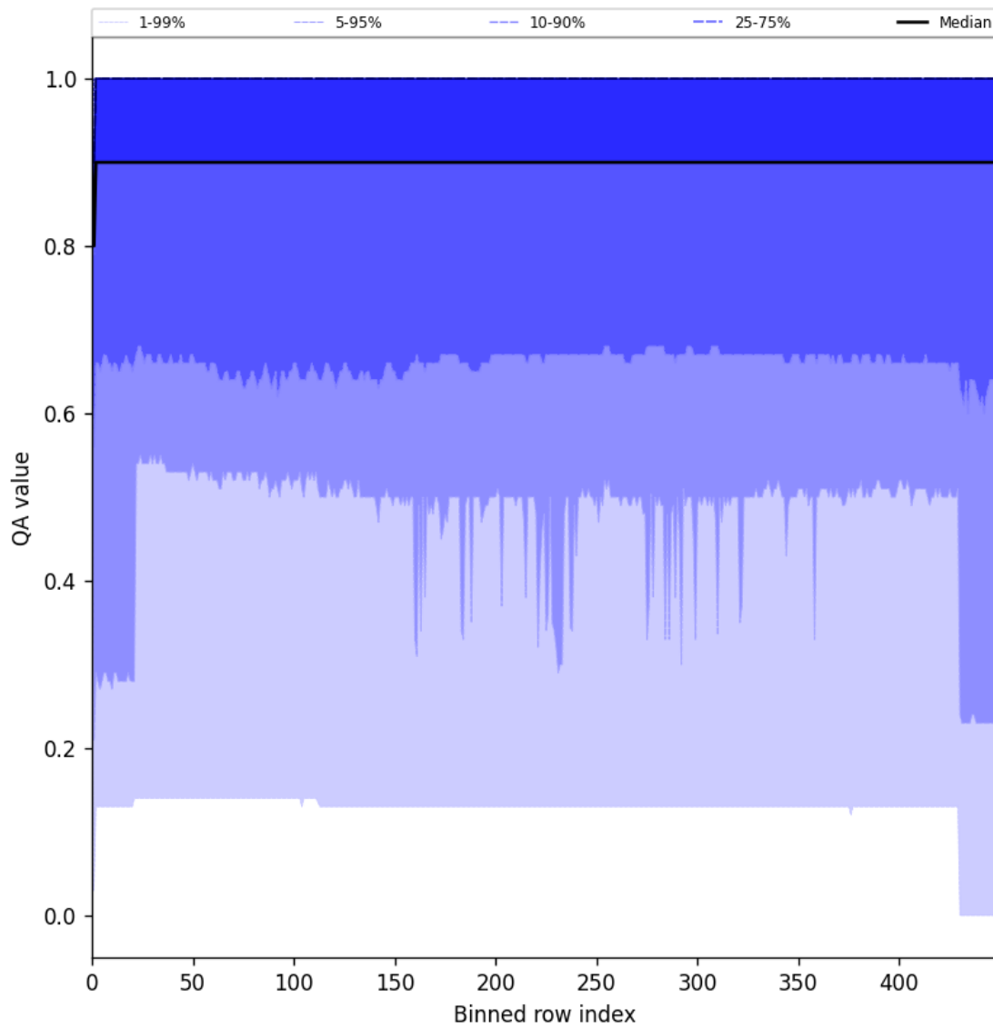
Figure 27: Along track statistics of “QA value” for 2025-10-07 to 2025-10-09
