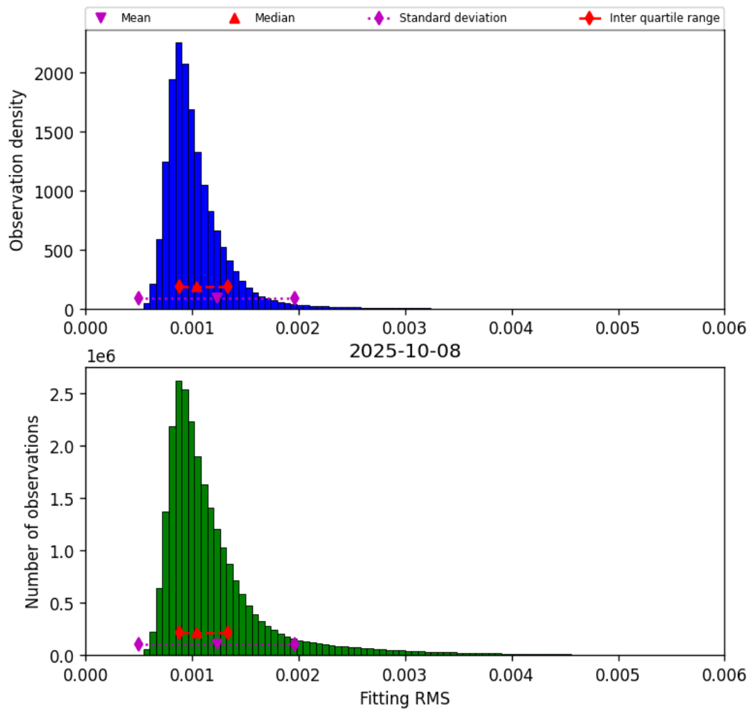
Figure 23: Histogram of “Fitting RMS” for 2025-10-07 to 2025-10-09
