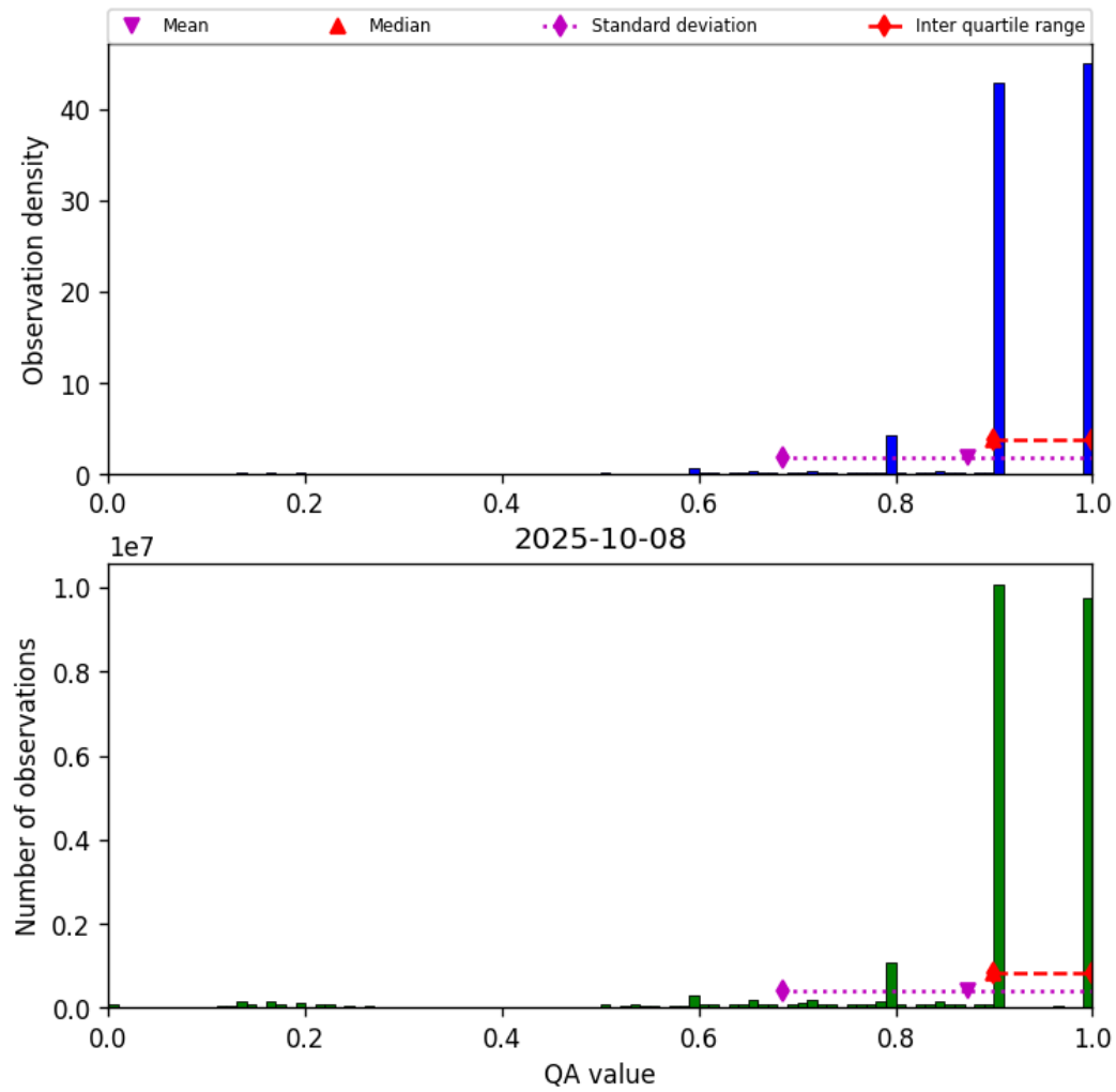
Figure 20: Histogram of “QA value” for 2025-10-07 to 2025-10-09
