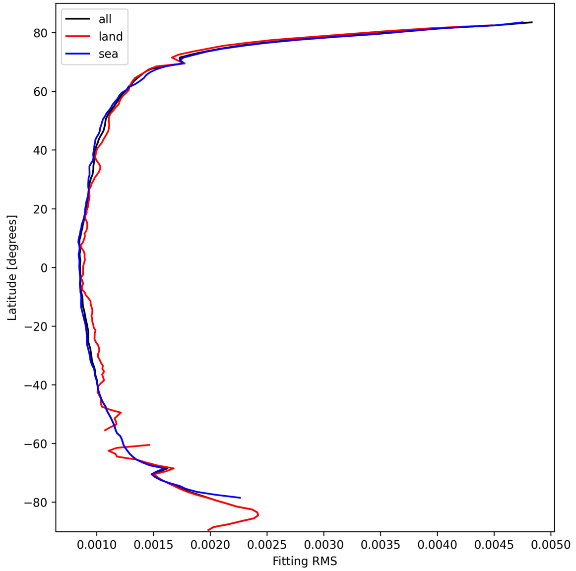
Figure 16: Zonal average of “Fitting RMS” for 2025-10-07 to 2025-10-09.
