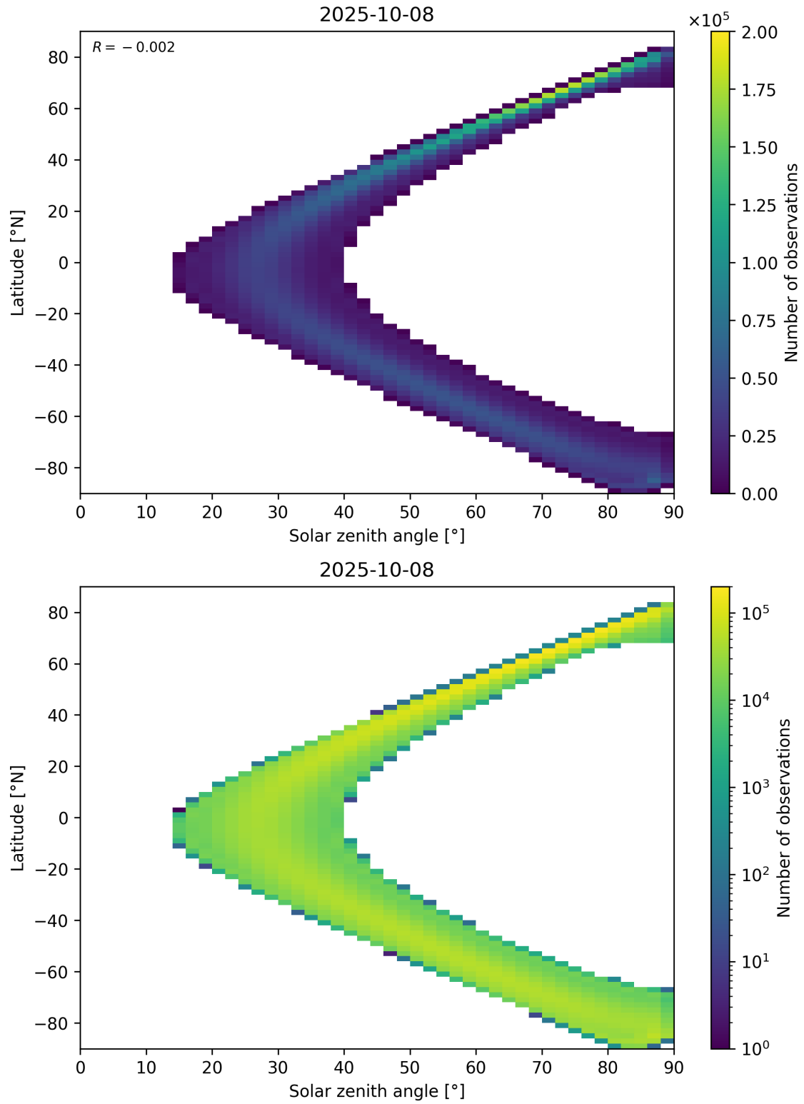
Figure 44: Scatter density plot of “Solar zenith angle” against “Latitude” for 2025-10-07 to 2025-10-09.
