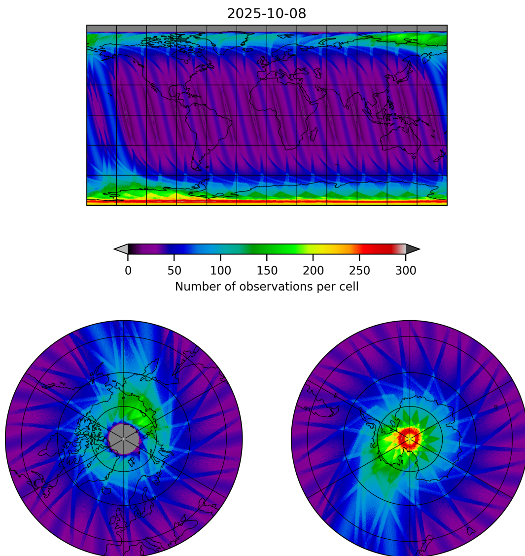
Figure 12: Map of the number of observations for 2025-10-07 to 2025-10-09
