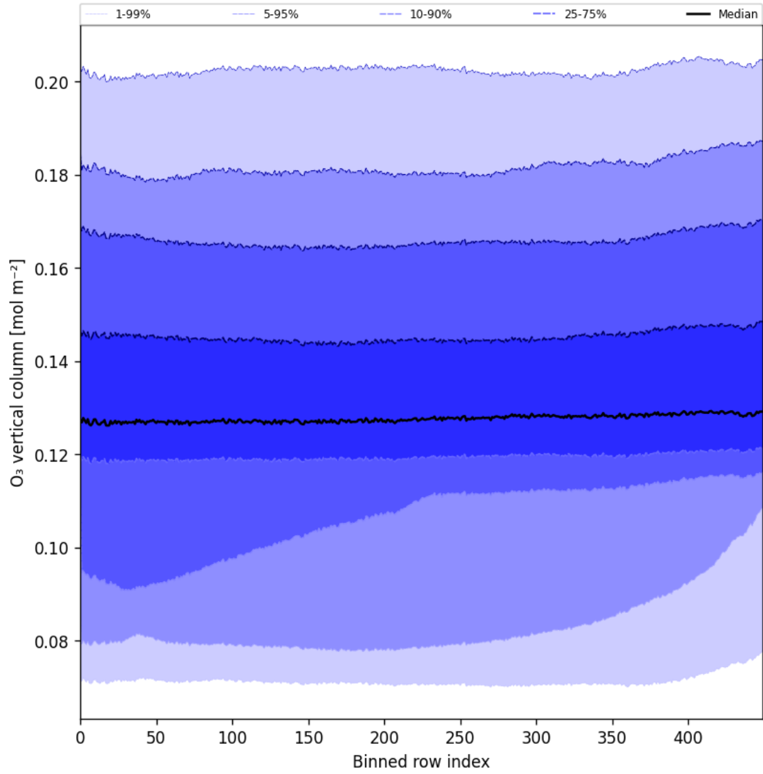
Figure 28: Along track statistics of “O 3 vertical column” for 2025-10-07 to 2025-10-09
