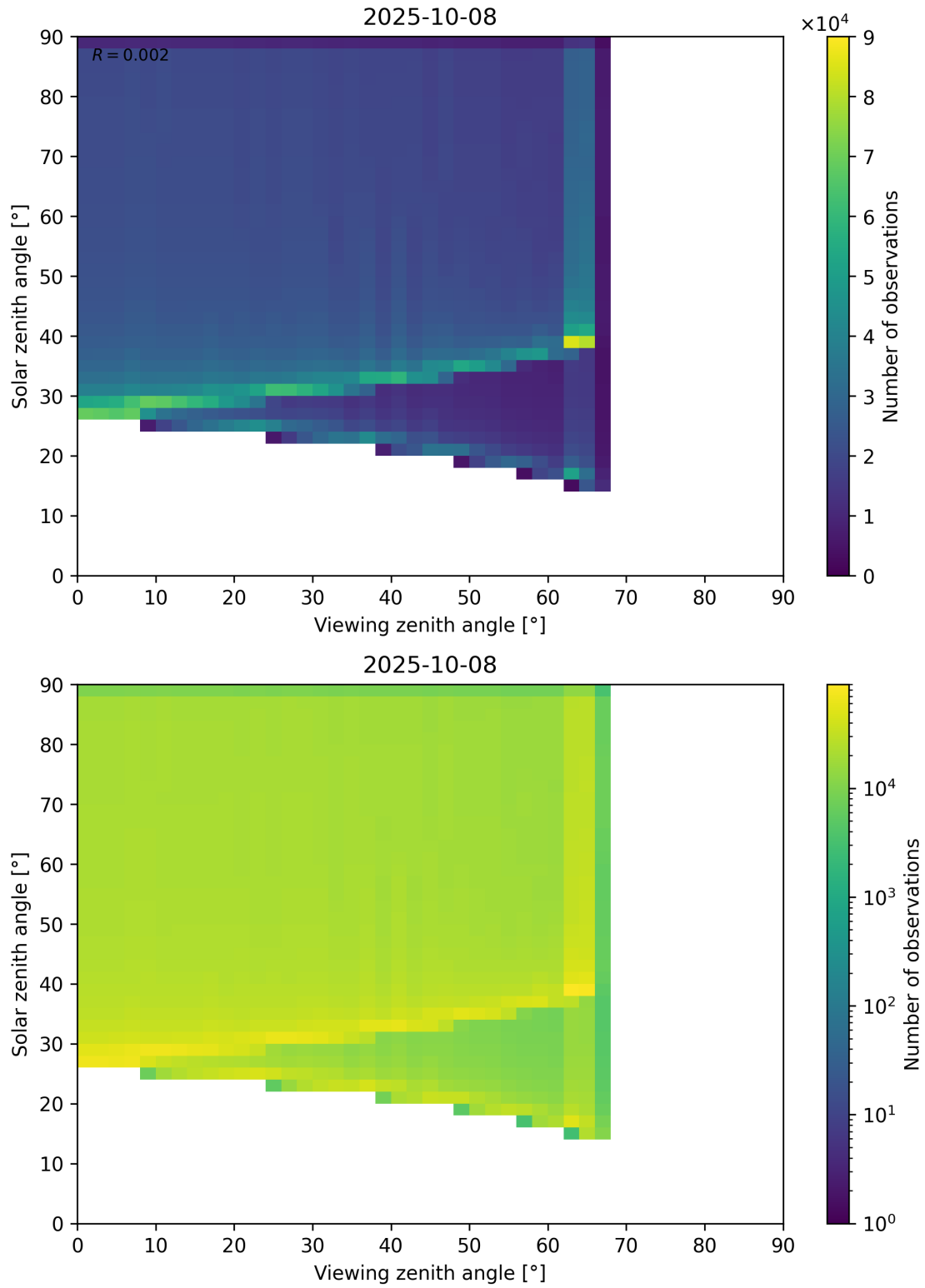
Figure 54: Scatter density plot of “Viewing zenith angle” against “Solar zenith angle” for 2025-10-07 to 2025-10-09.
