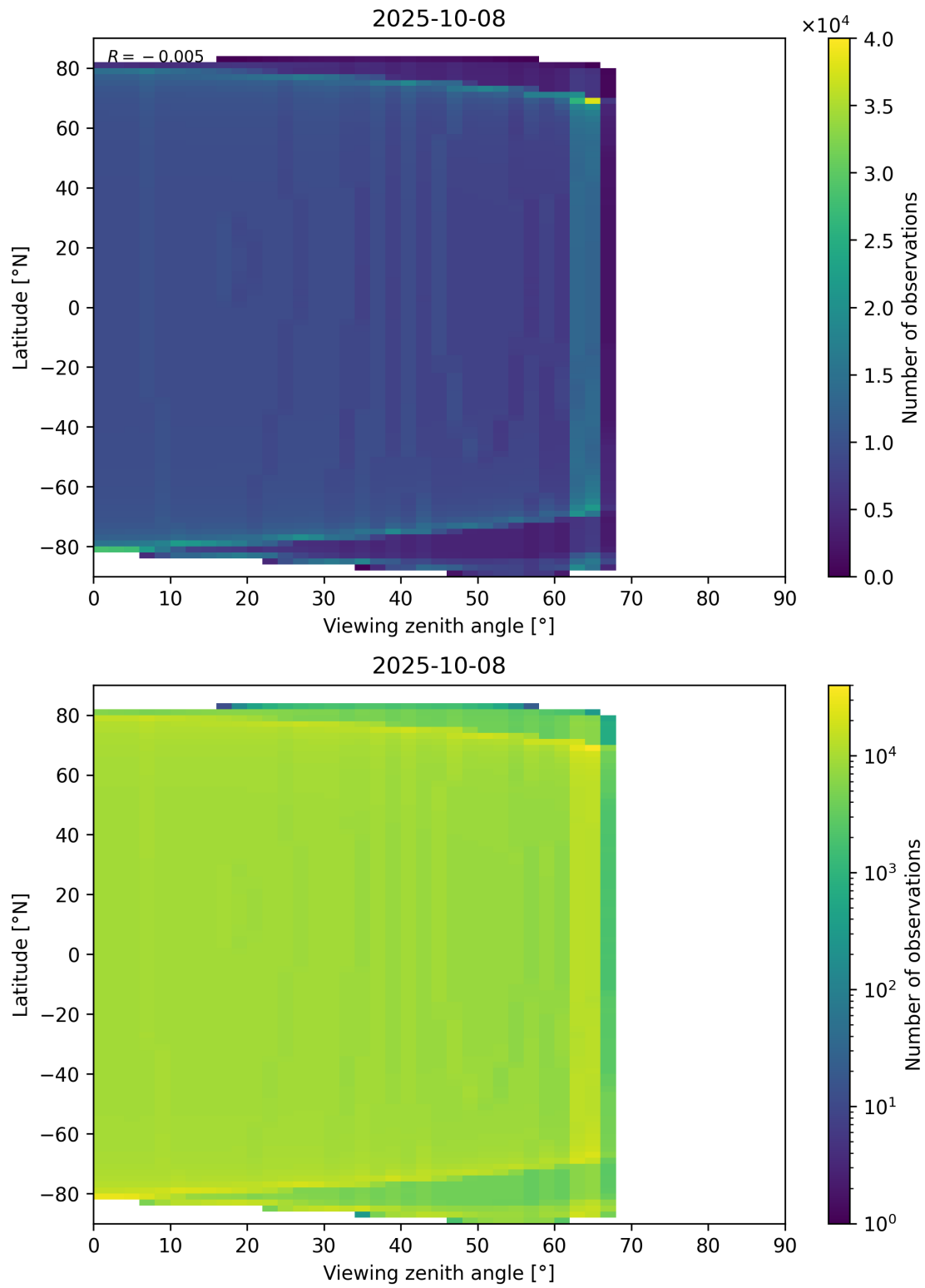
Figure 49: Scatter density plot of “Viewing zenith angle” against “Latitude” for 2025-10-07 to 2025-10-09.
