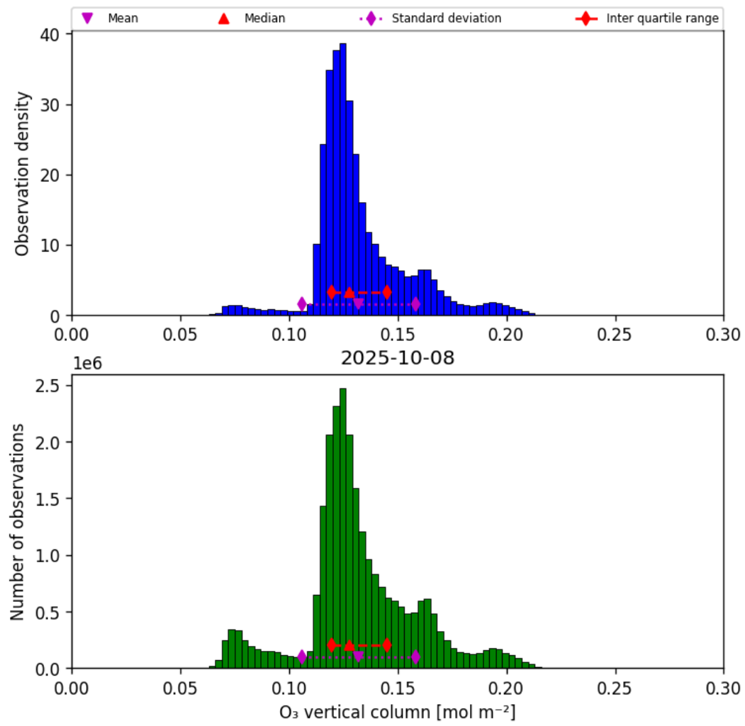
Figure 21: Histogram of “O 3 vertical column” for 2025-10-07 to 2025-10-09
