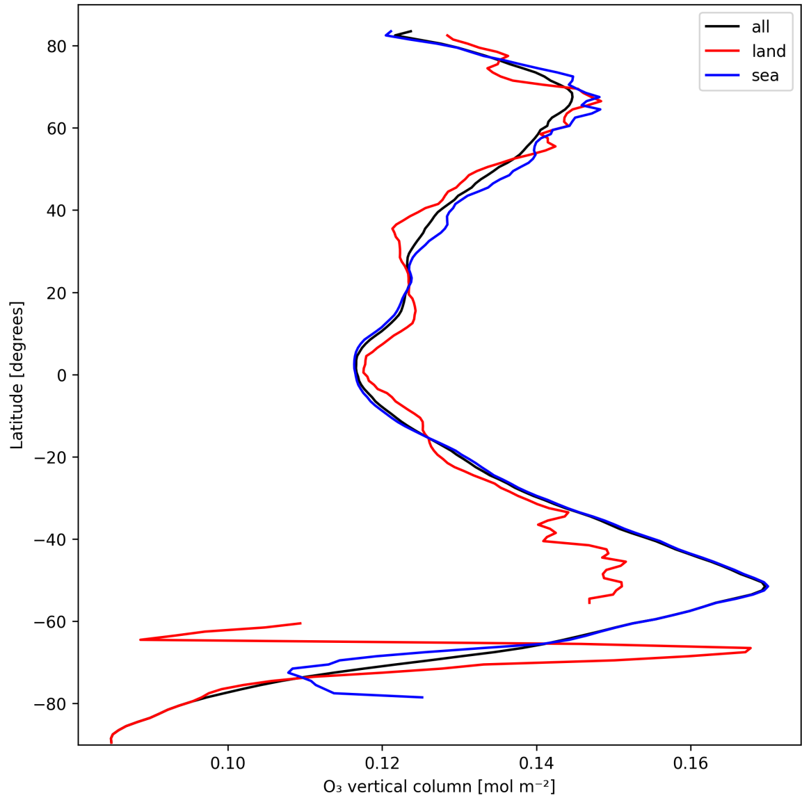
Figure 14: Zonal average of “O 3 vertical column” for 2025-10-07 to 2025-10-09.
