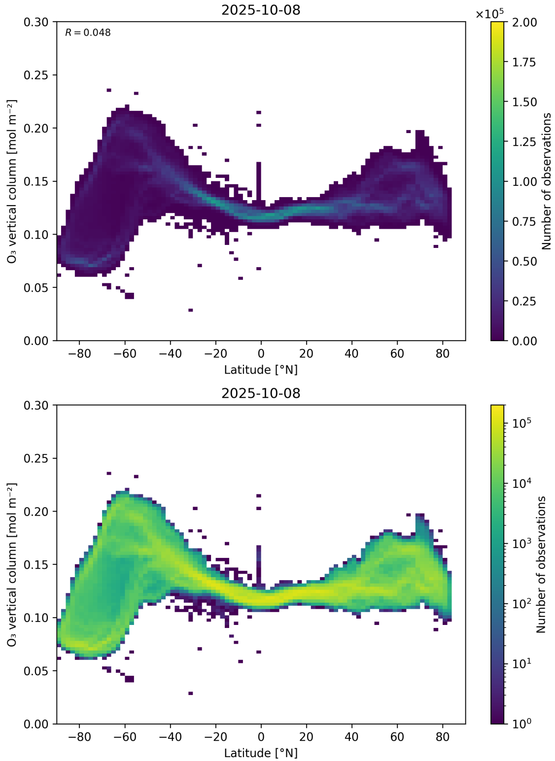
Figure 36: Scatter density plot of “Latitude” against “O 3 vertical column” for 2025-10-07 to 2025-10-09.
