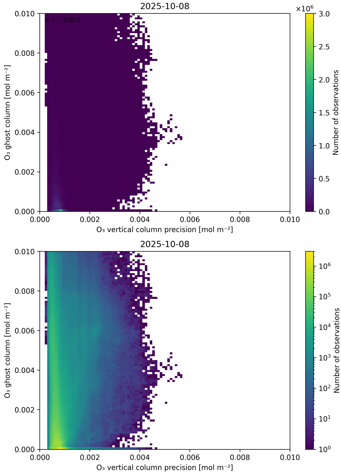
Figure 43: Scatter density plot of “O 3 vertical column precision” against “O 3 ghost column” for 2025-10-07 to 2025-10-09.
