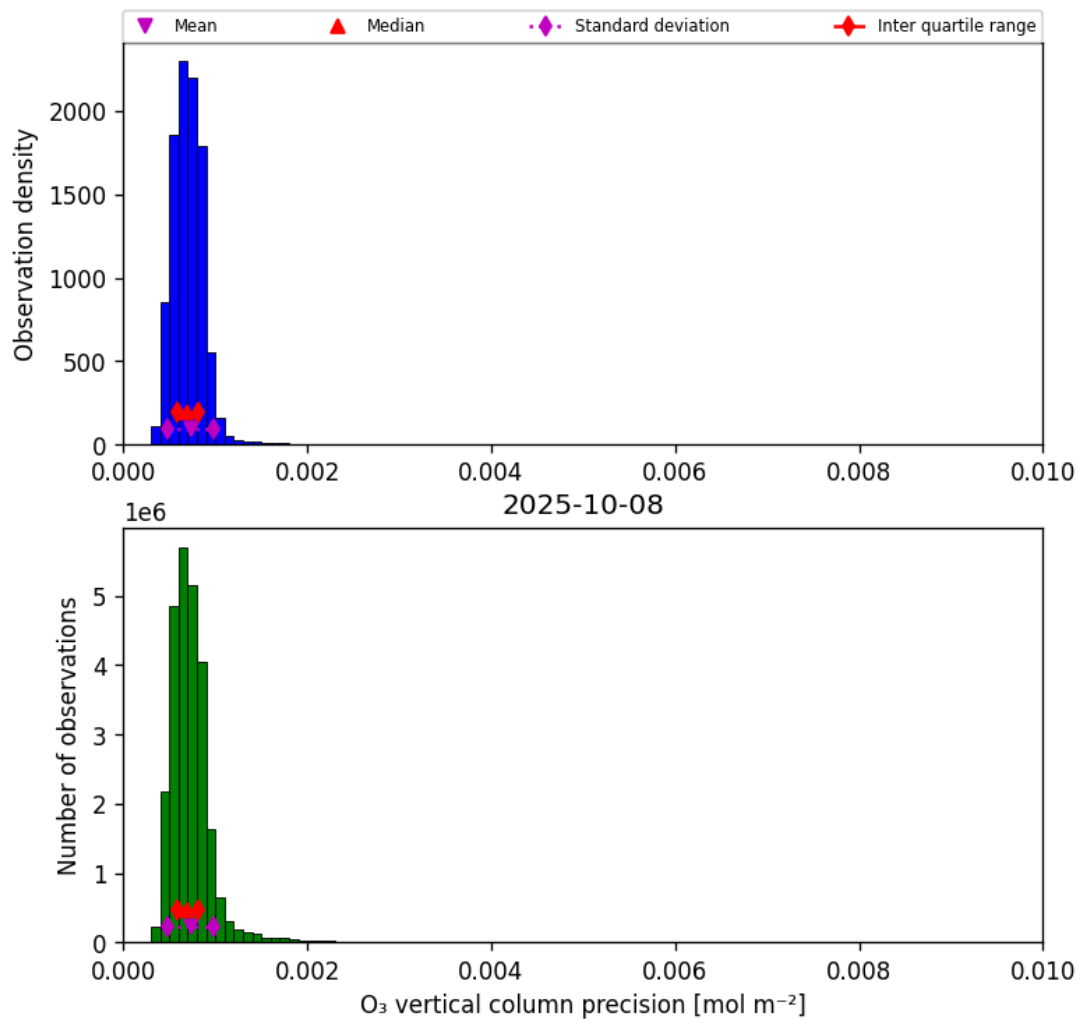
Figure 22: Histogram of “O 3 vertical column precision” for 2025-10-07 to 2025-10-09
