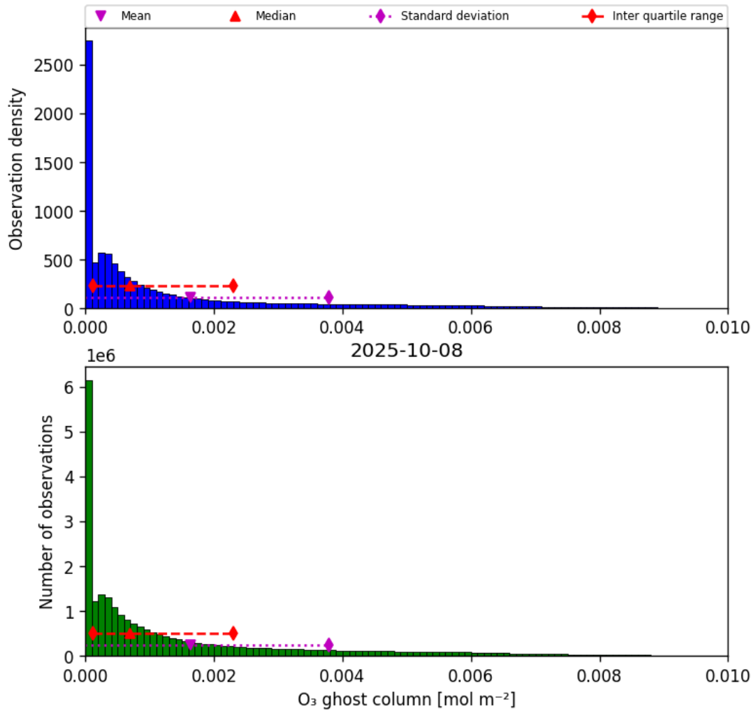
Figure 25: Histogram of “O 3 ghost column” for 2025-10-07 to 2025-10-09
