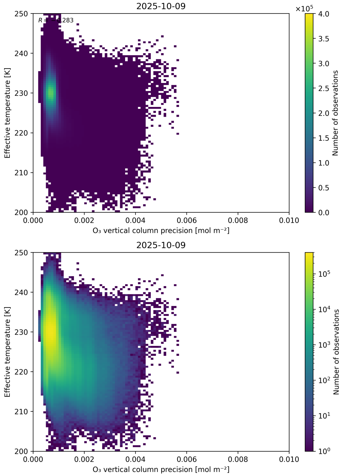
Figure 42: Scatter density plot of “O 3 vertical column precision” against “Effective temperature” for 2025-10-08 to 2025-10-10.
