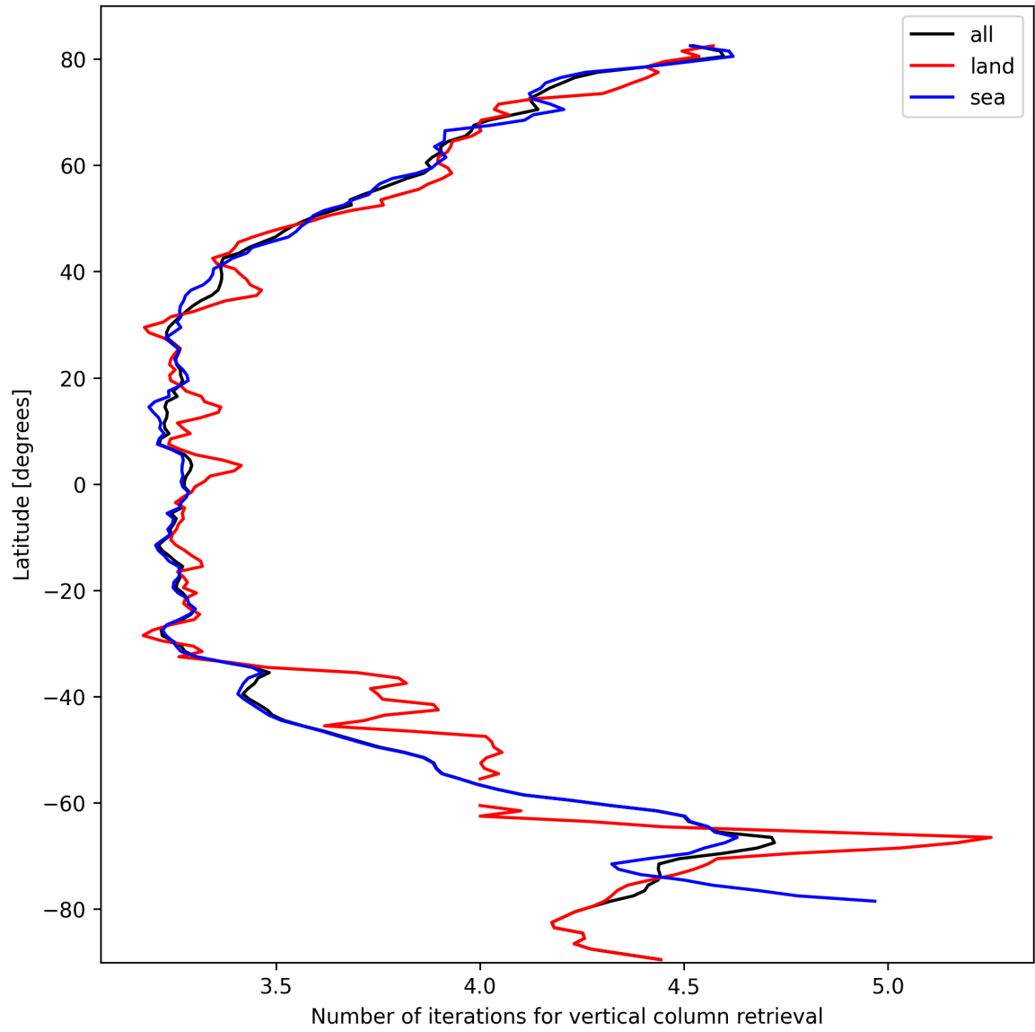
Figure 19: Zonal average of “Number of iterations for vertical column retrieval” for 2025-10-08 to 2025-10-10.
