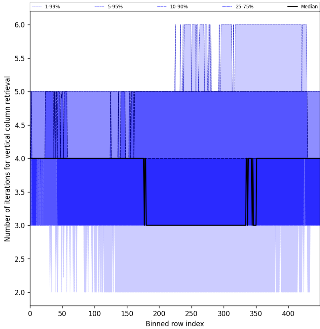
Figure 33: Along track statistics of “Number of iterations for vertical column retrieval” for 2025-10-08 to 2025-10-10
