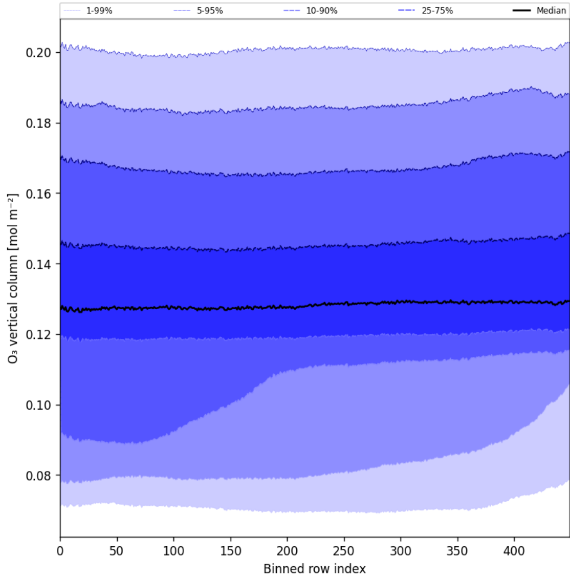
Figure 28: Along track statistics of “O 3 vertical column” for 2025-10-08 to 2025-10-10
