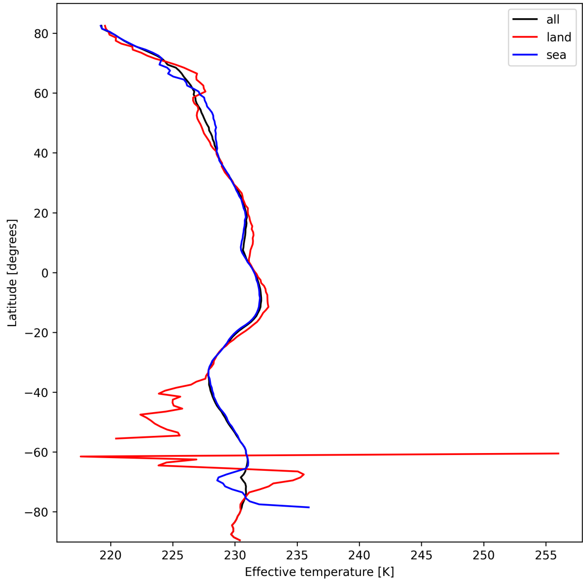
Figure 17: Zonal average of "Effective temperature" for 2025-10-08 to 2025-10-10.
