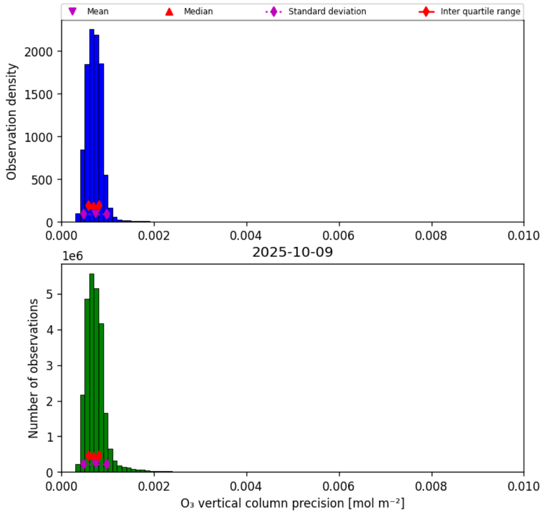
Figure 22: Histogram of “O 3 vertical column precision” for 2025-10-08 to 2025-10-10
