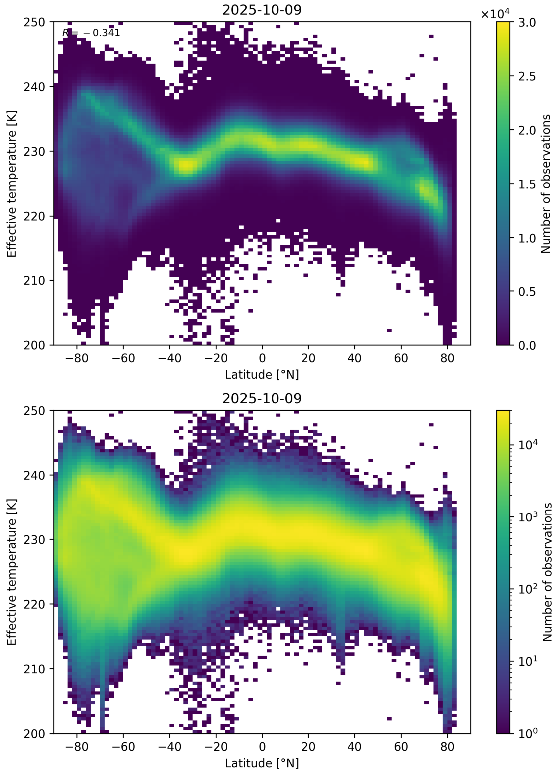
Figure 34: Scatter density plot of “Latitude” against “Effective temperature” for 2025-10-08 to 2025-10-10.
