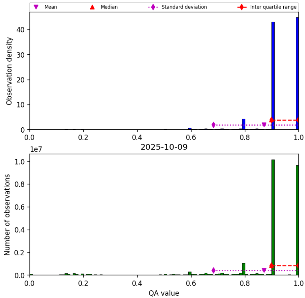
Figure 20: Histogram of “QA value” for 2025-10-08 to 2025-10-10
