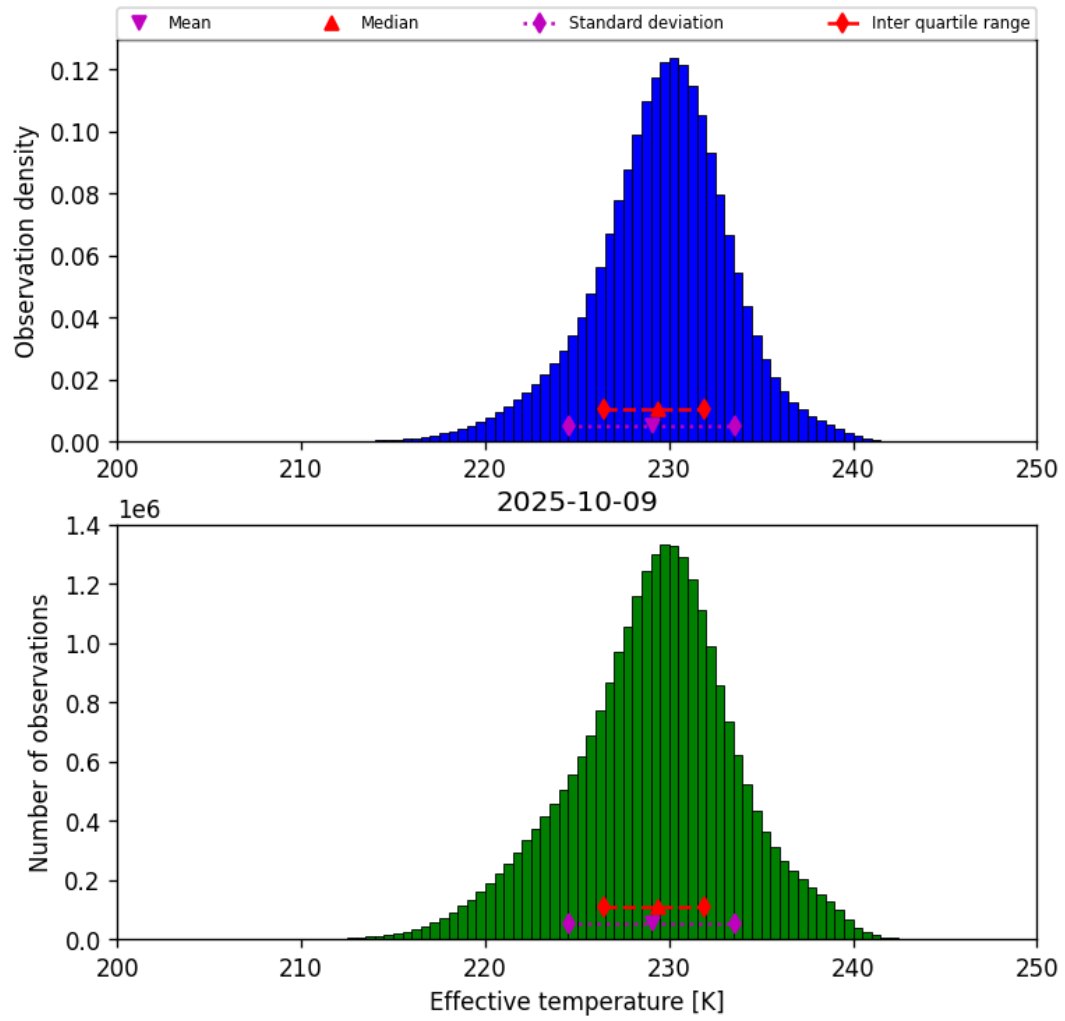
Figure 24: Histogram of “Effective temperature” for 2025-10-08 to 2025-10-10
