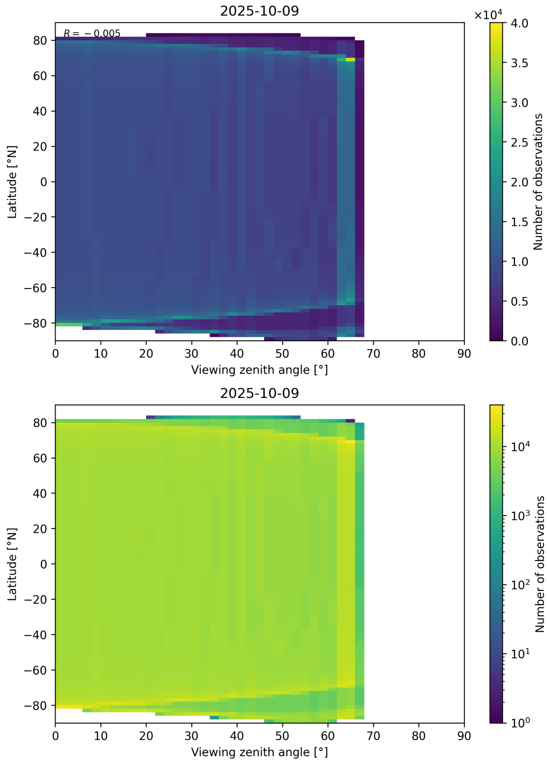
Figure 49: Scatter density plot of “Viewing zenith angle” against “Latitude” for 2025-10-08 to 2025-10-10.
