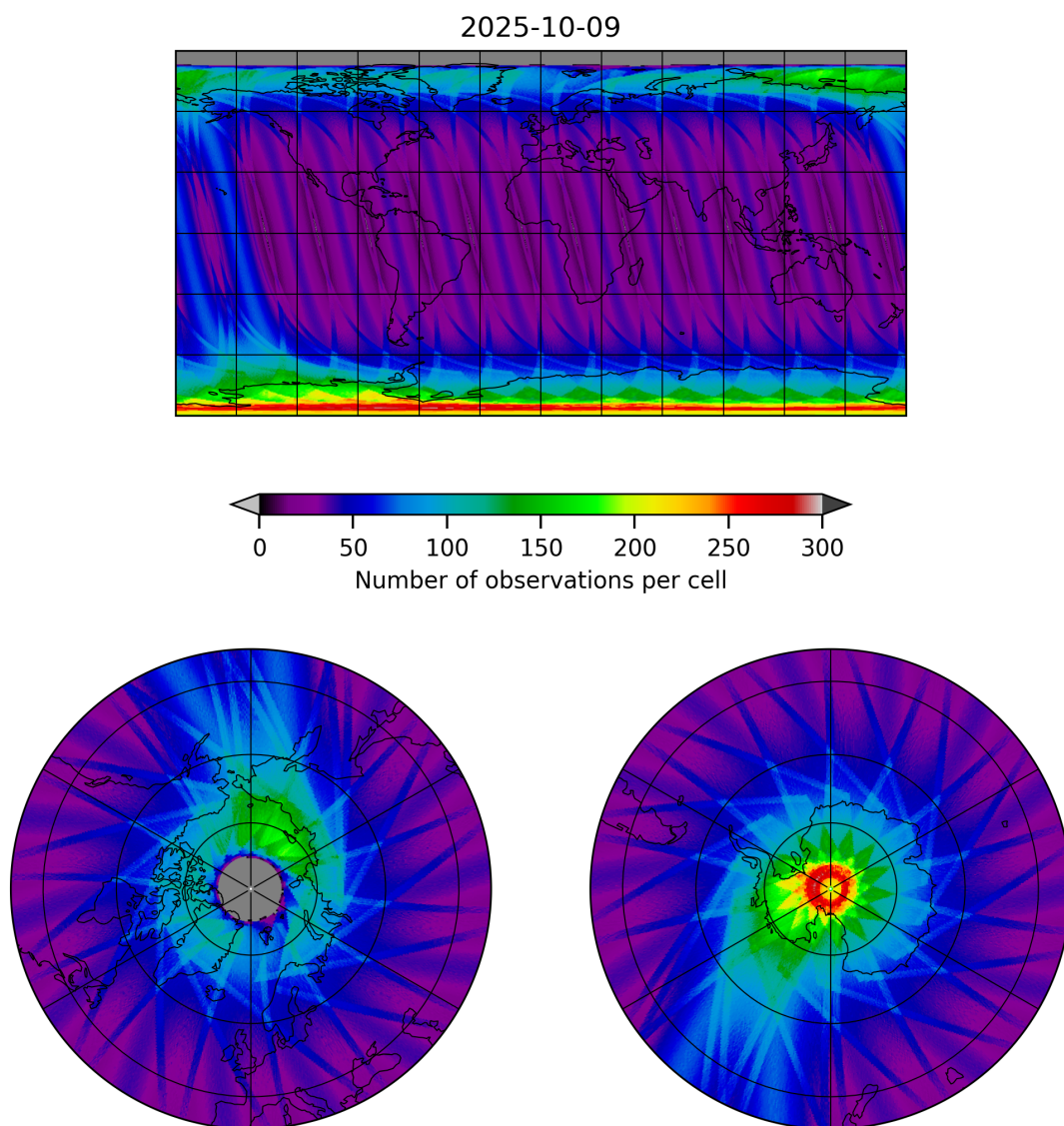
Figure 12: Map of the number of observations for 2025-10-08 to 2025-10-10
