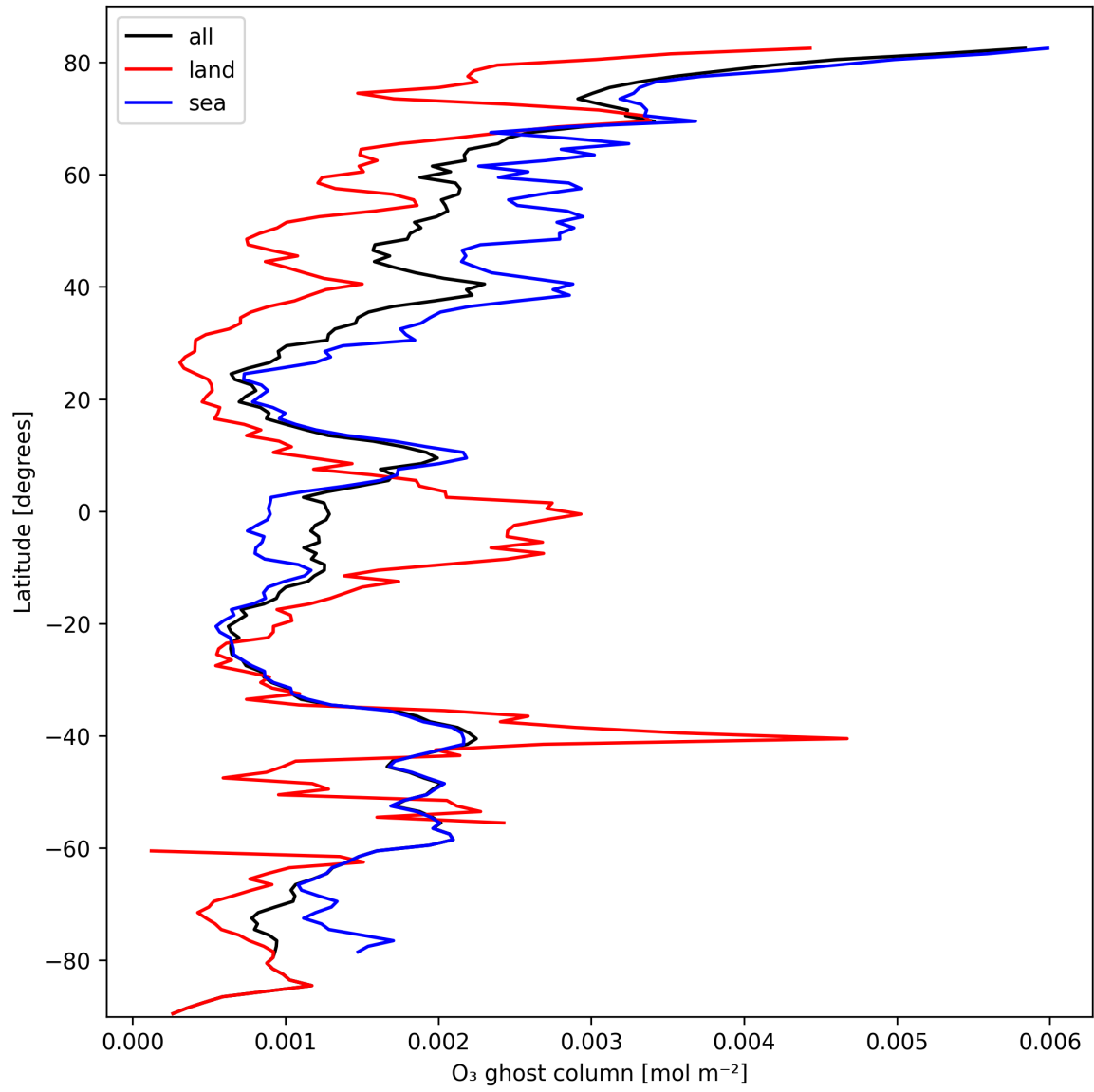
Figure 18: Zonal average of “O 3 ghost column” for 2025-10-08 to 2025-10-10.
