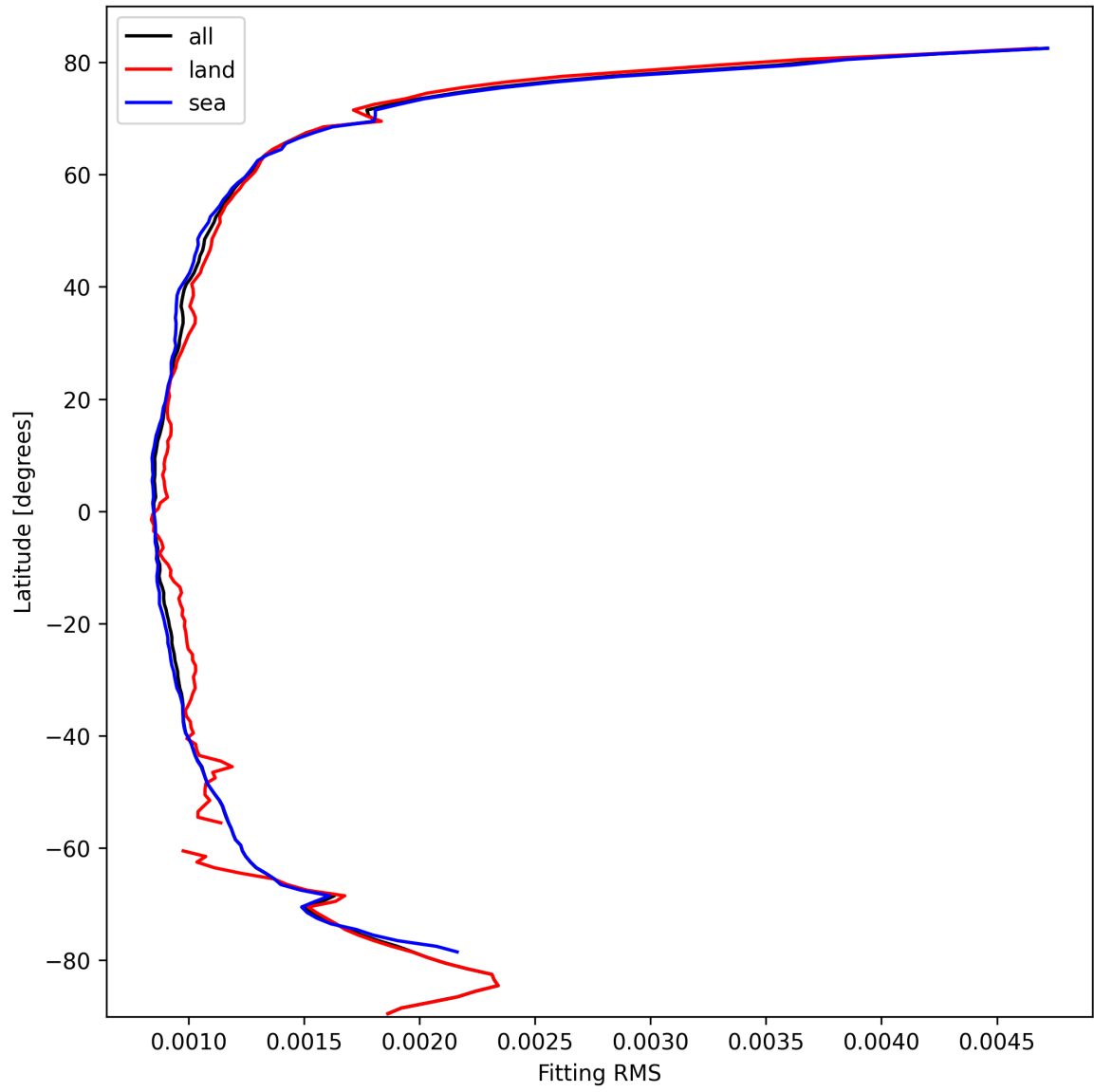
Figure 16: Zonal average of “Fitting RMS” for 2025-10-08 to 2025-10-10.
