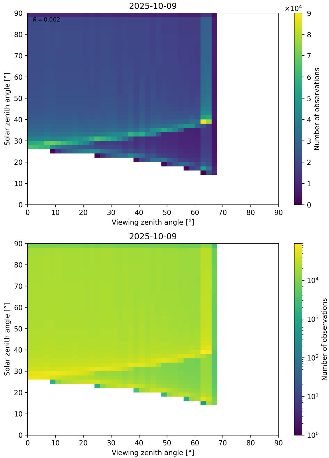
Figure 54: Scatter density plot of “Viewing zenith angle” against “Solar zenith angle” for 2025-10-08 to 2025-10-10.
