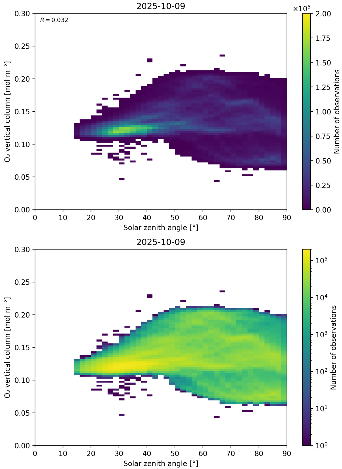
Figure 47: Scatter density plot of “Solar zenith angle” against “O 3 vertical column” for 2025-10-08 to 2025-10-10.
