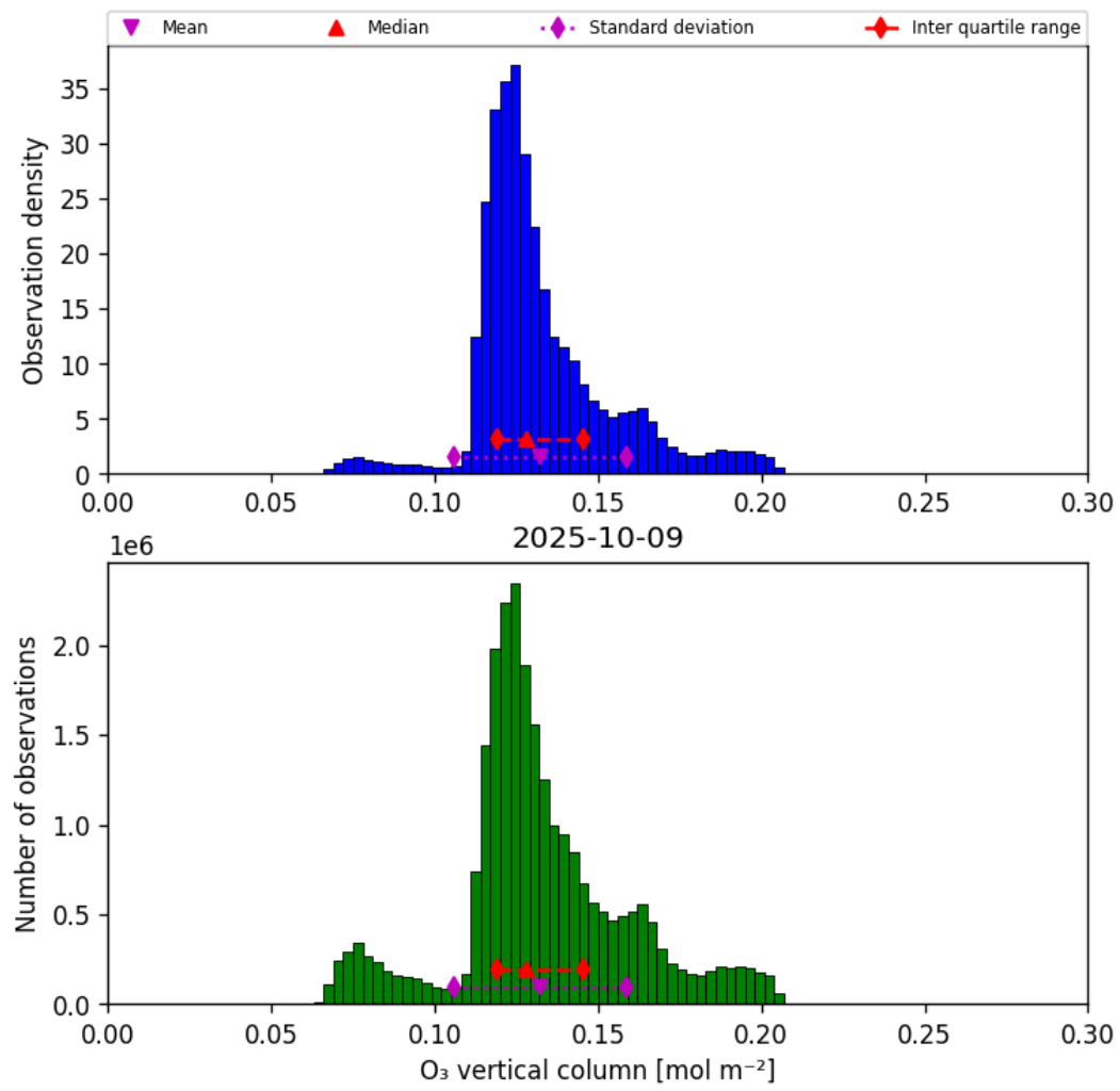
Figure 21: Histogram of “O 3 vertical column” for 2025-10-08 to 2025-10-10
