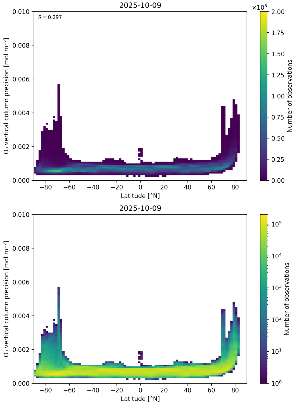
Figure 37: Scatter density plot of “Latitude” against “O 3 vertical column precision” for 2025-10-08 to 2025-10-10.
