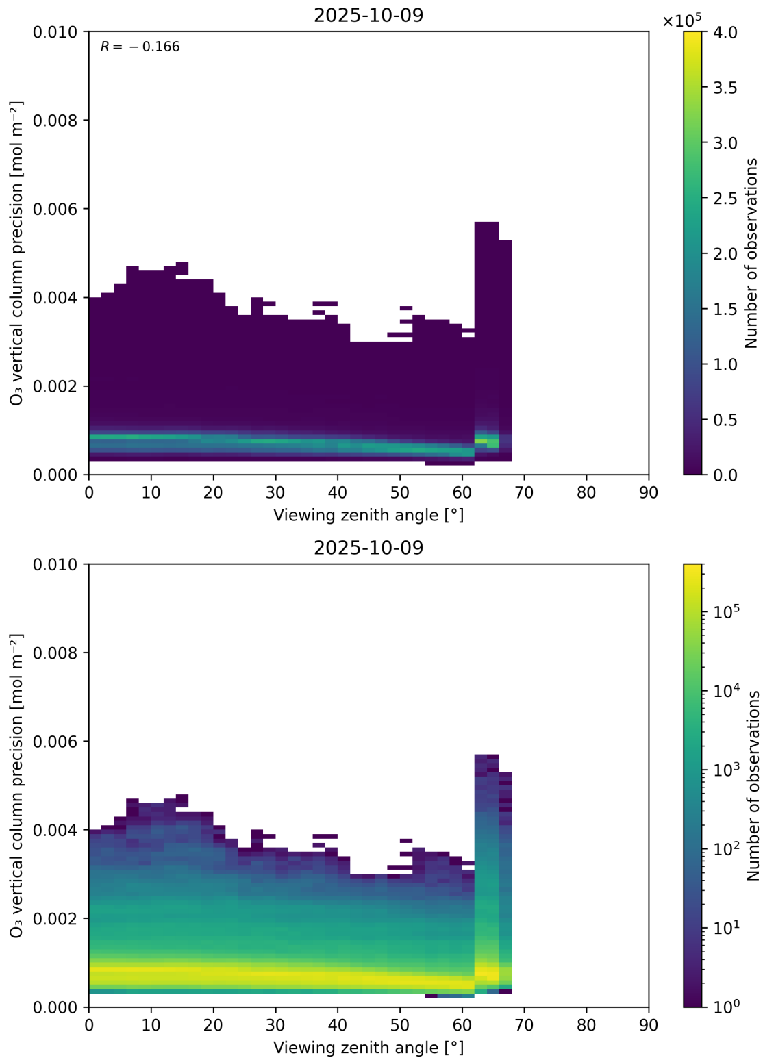
Figure 53: Scatter density plot of “Viewing zenith angle” against “O 3 vertical column precision” for 2025-10-08 to 2025-10-10.
