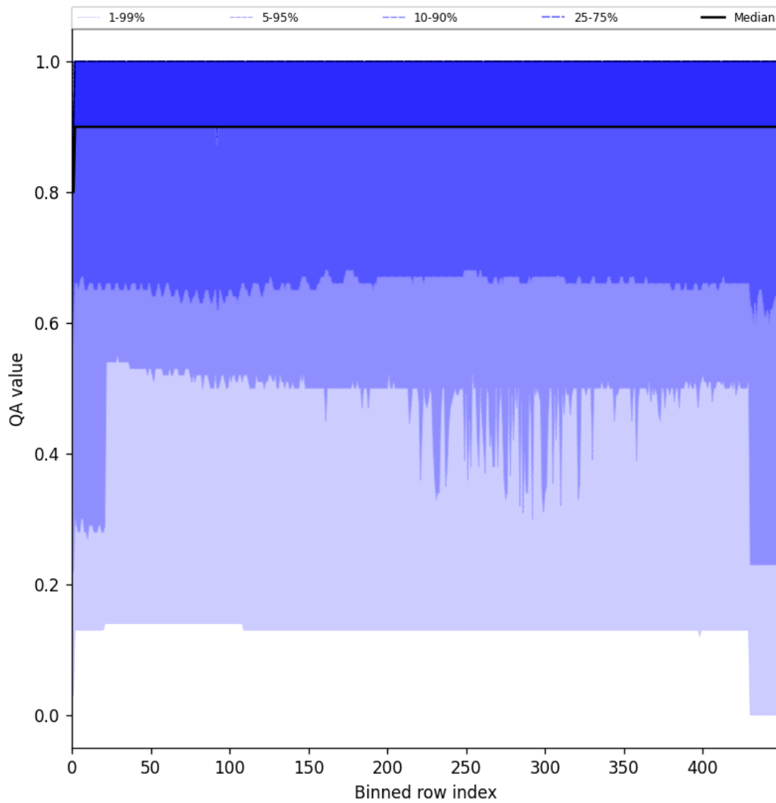
Figure 27: Along track statistics of “QA value” for 2025-10-08 to 2025-10-10
