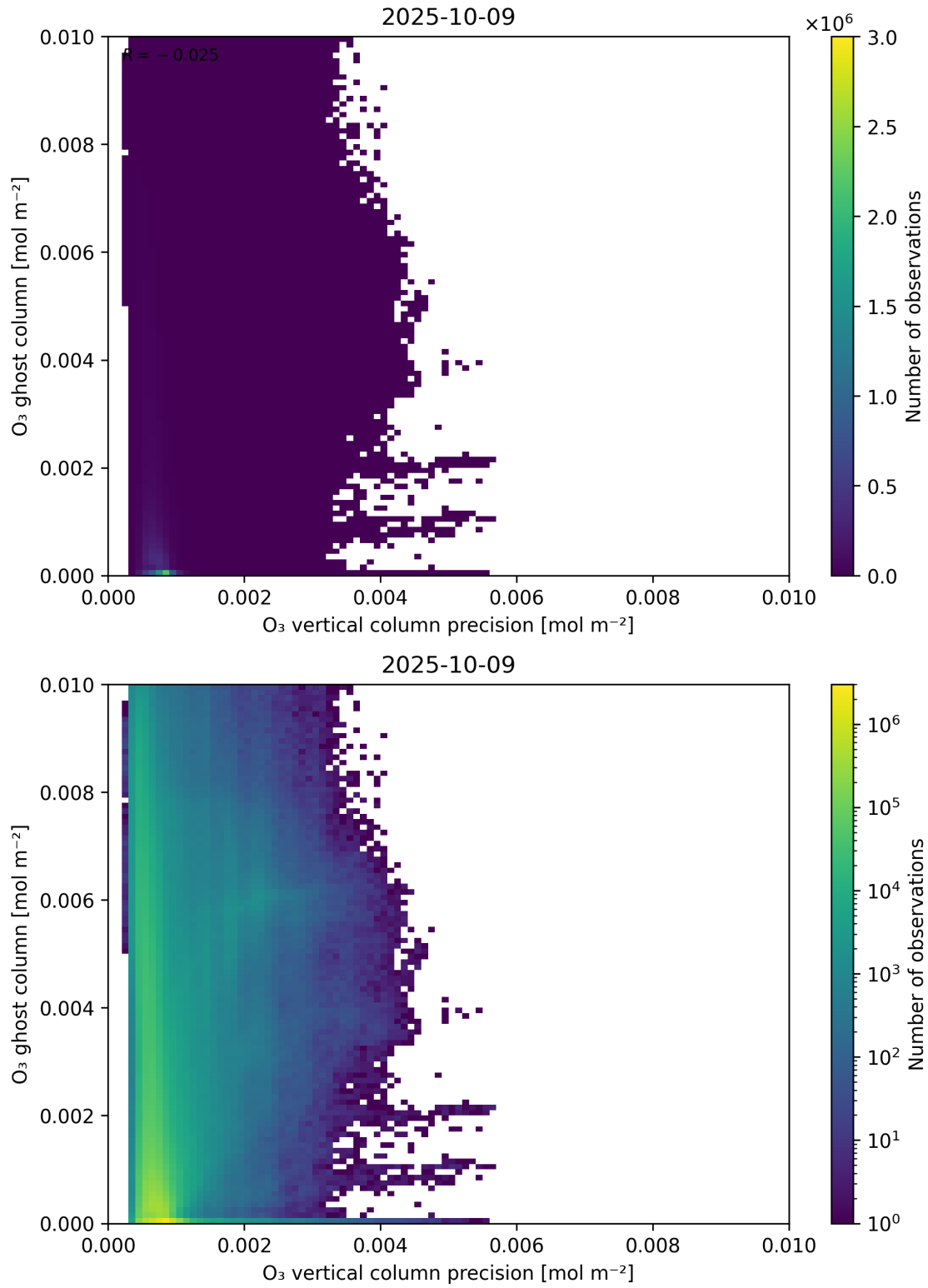
Figure 43: Scatter density plot of “ O_3 vertical column precision” against “ O_3 ghost column” for 2025-10-08 to 2025-10-10.
