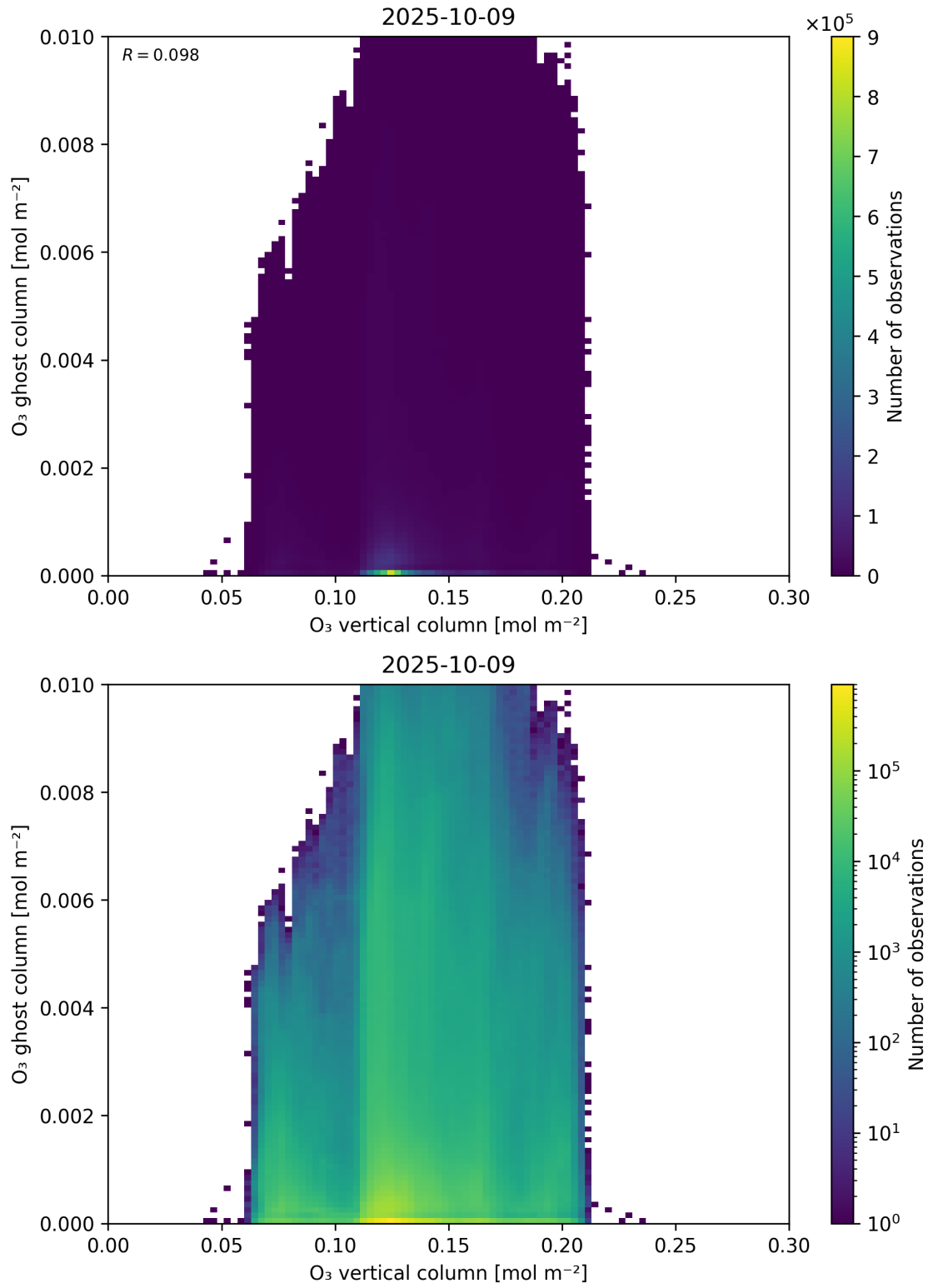
Figure 40: Scatter density plot of “O 3 vertical column” against “O 3 ghost column” for 2025-10-08 to 2025-10-10.
