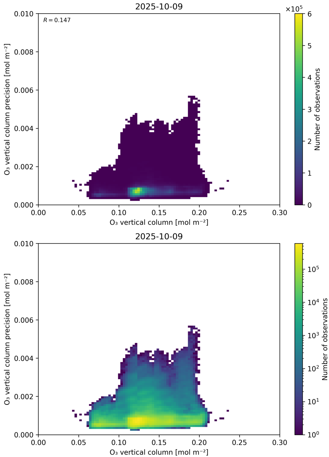
Figure 41: Scatter density plot of “O 3 vertical column” against “O 3 vertical column precision” for 2025-10-08 to 2025-10-10.
