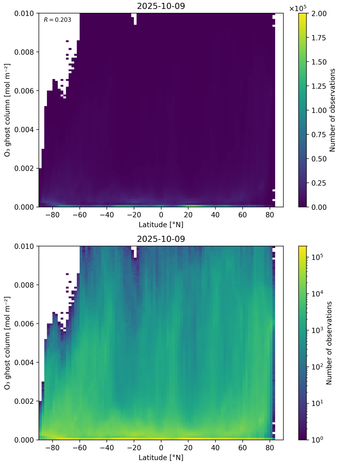
Figure 35: Scatter density plot of “Latitude” against “O 3 ghost column” for 2025-10-08 to 2025-10-10.
