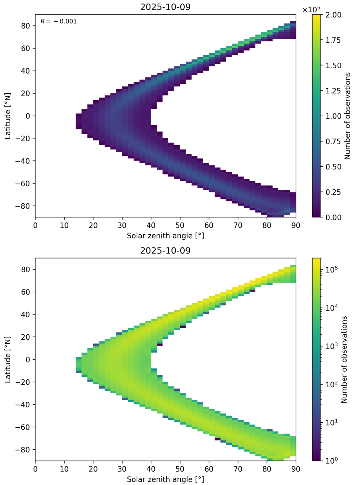
Figure 44: Scatter density plot of “Solar zenith angle” against “Latitude” for 2025-10-08 to 2025-10-10.
