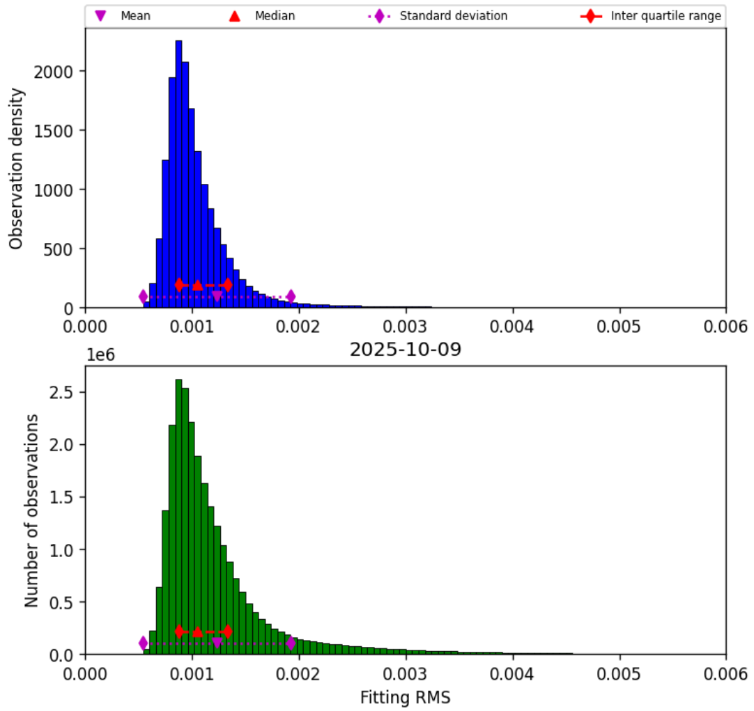
Figure 23: Histogram of “Fitting RMS” for 2025-10-08 to 2025-10-10
