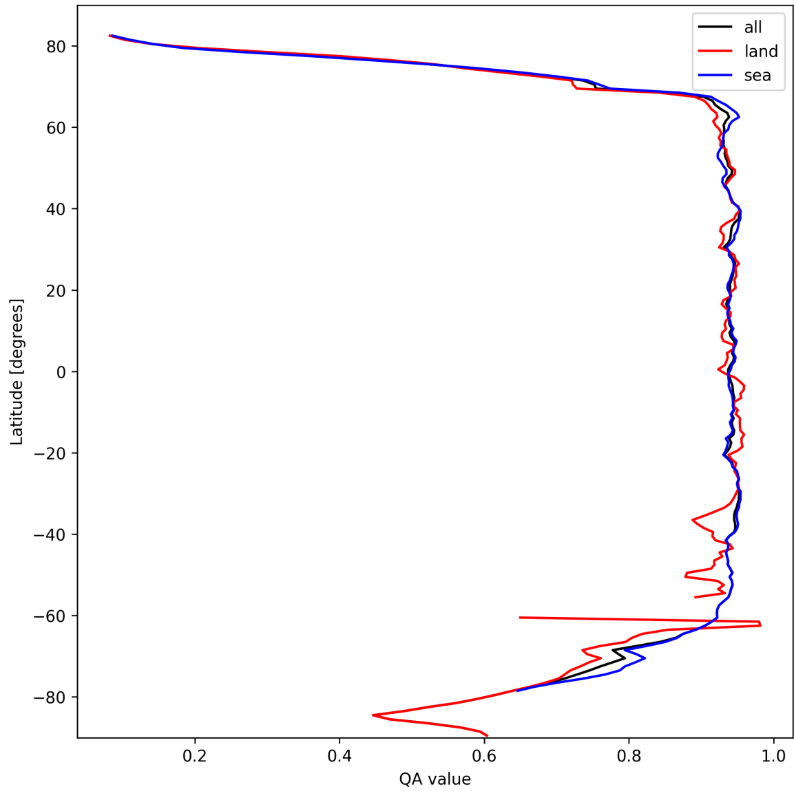
Figure 13: Zonal average of “QA value” for 2025-10-08 to 2025-10-10.
