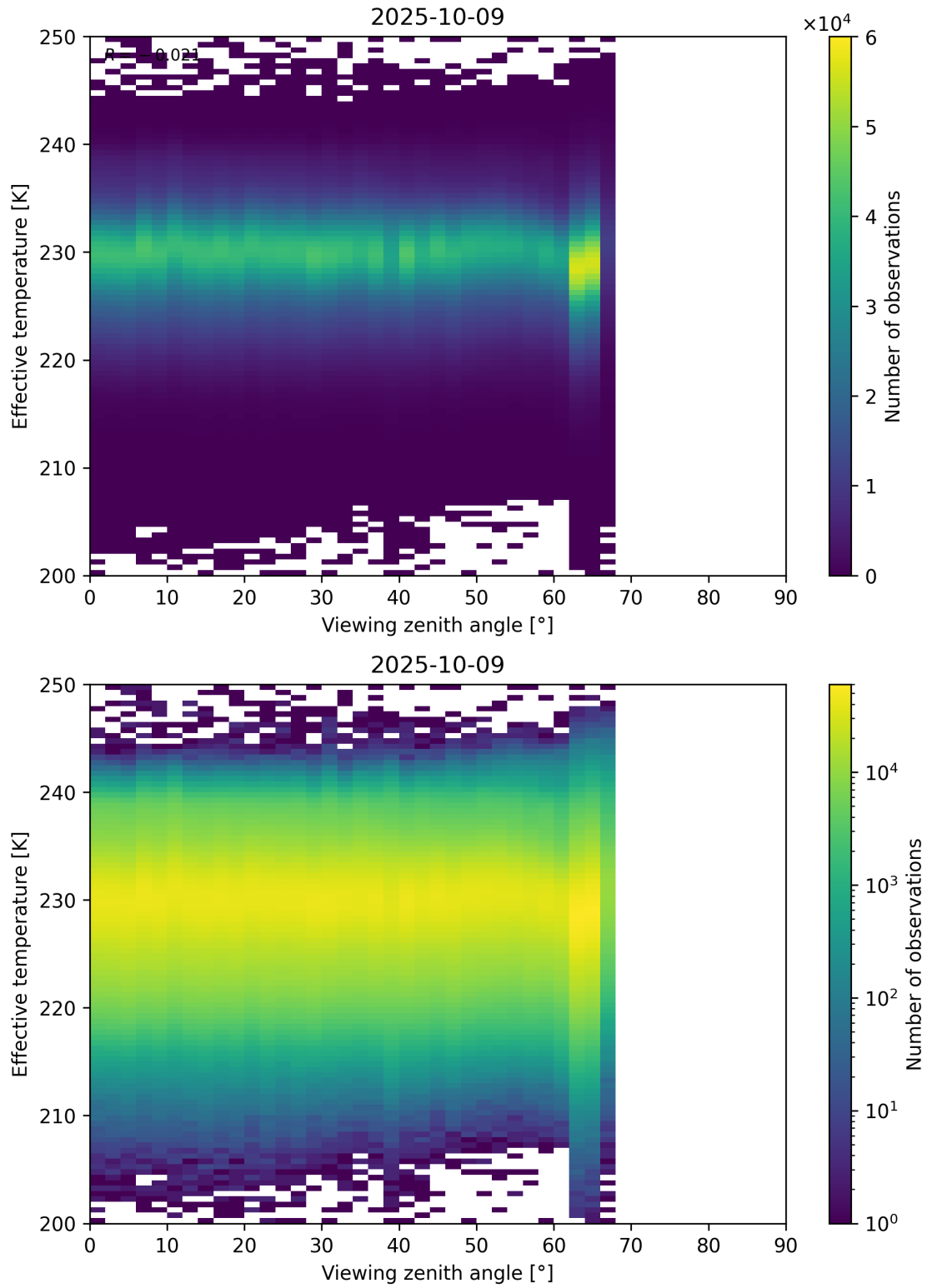
Figure 50: Scatter density plot of “Viewing zenith angle” against “Effective temperature” for 2025-10-08 to 2025-10-10.
