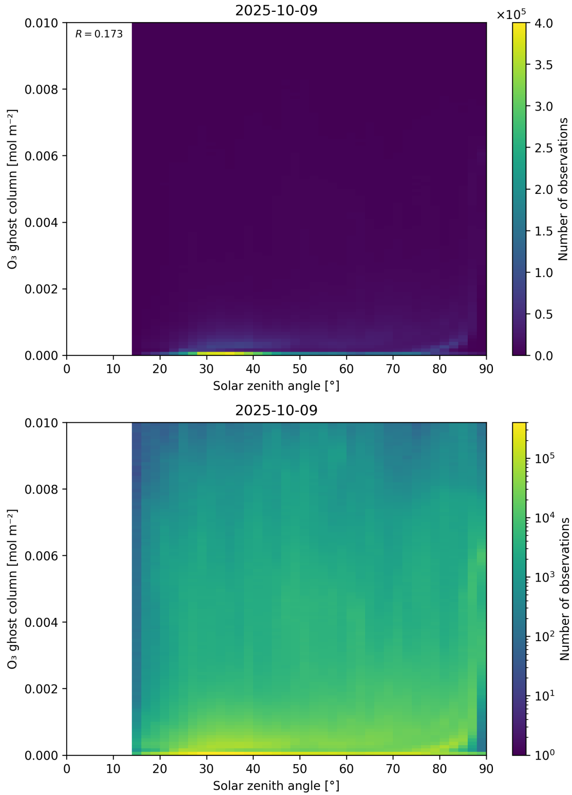
Figure 46: Scatter density plot of “Solar zenith angle” against “O 3 ghost column” for 2025-10-08 to 2025-10-10.
