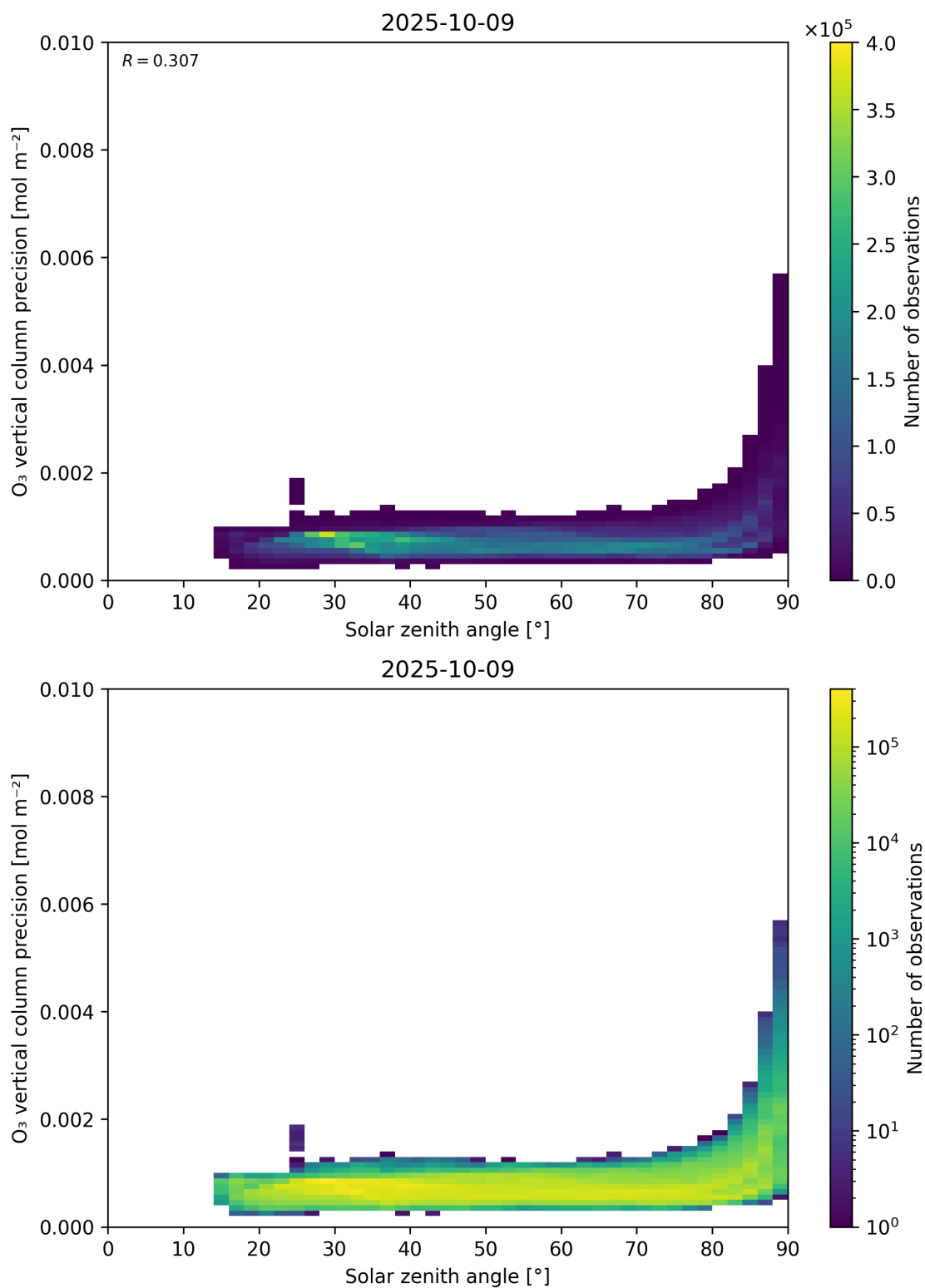
Figure 48: Scatter density plot of “Solar zenith angle” against “O 3 vertical column precision” for 2025-10-08 to 2025-10-10.
