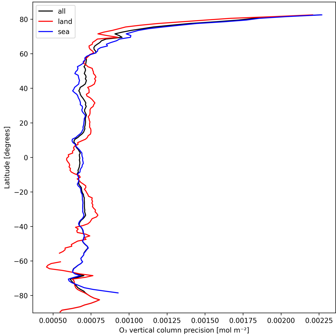
Figure 15: Zonal average of “O 3 vertical column precision” for 2025-10-08 to 2025-10-10.
