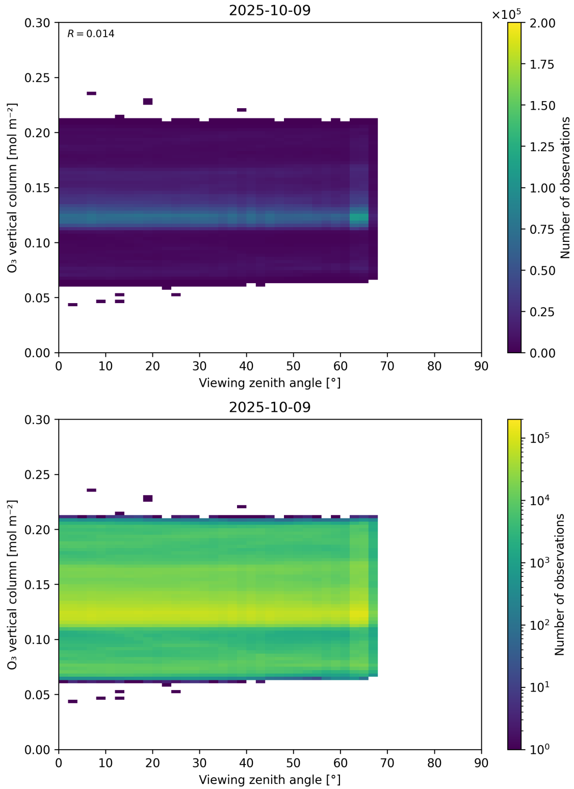
Figure 52: Scatter density plot of “Viewing zenith angle” against “O 3 vertical column” for 2025-10-08 to 2025-10-10.
