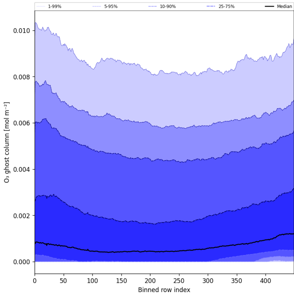
Figure 32: Along track statistics of “O 3 ghost column” for 2025-10-08 to 2025-10-10
