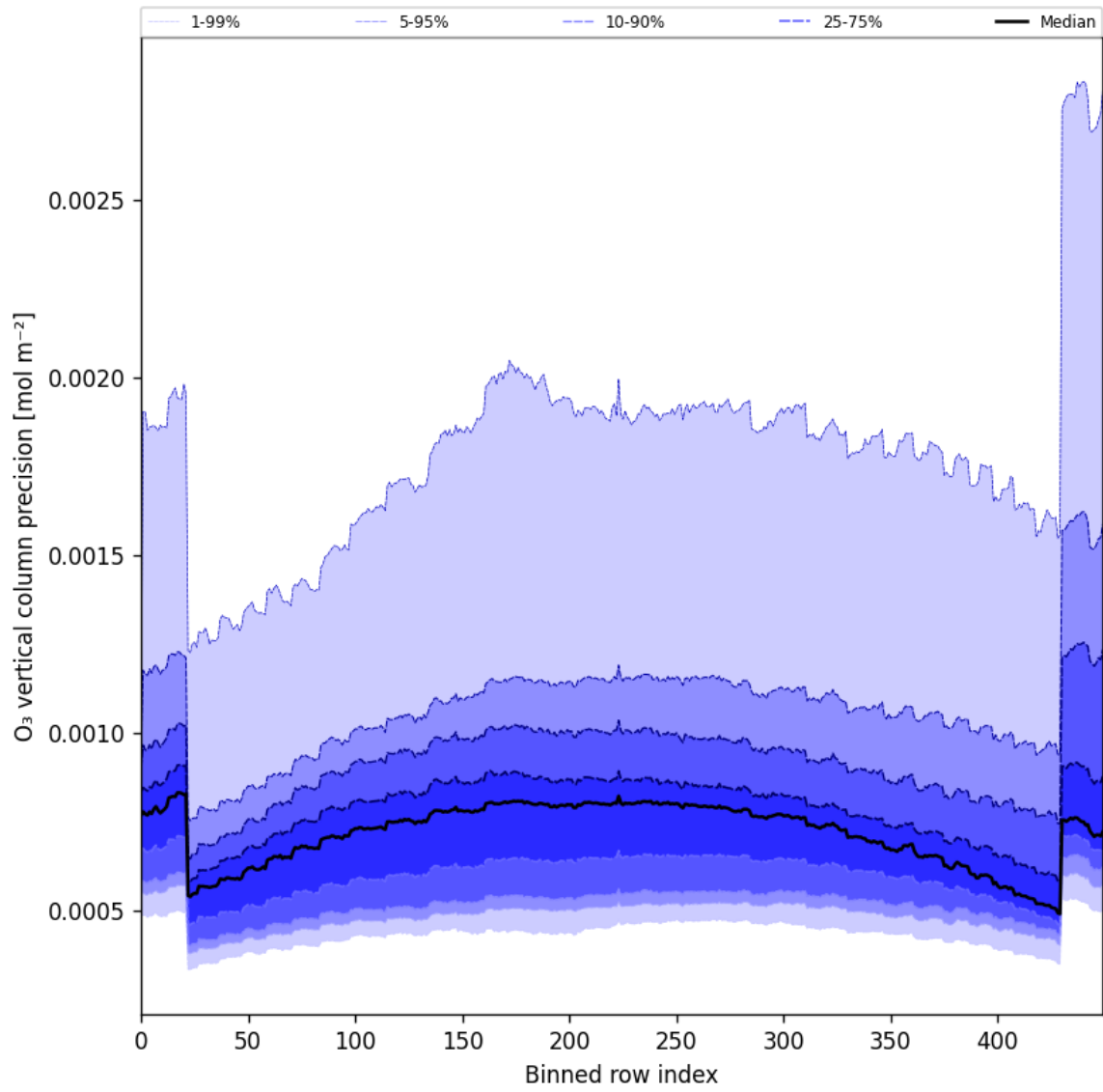
Figure 29: Along track statistics of “O 3 vertical column precision” for 2025-10-08 to 2025-10-10
