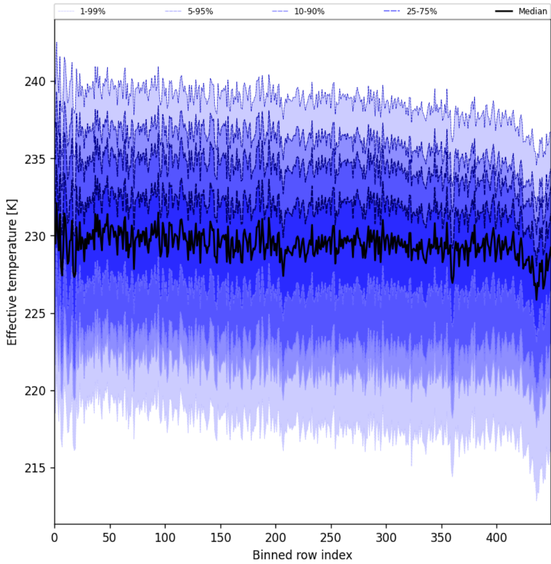
Figure 31: Along track statistics of “Effective temperature” for 2025-10-08 to 2025-10-10
