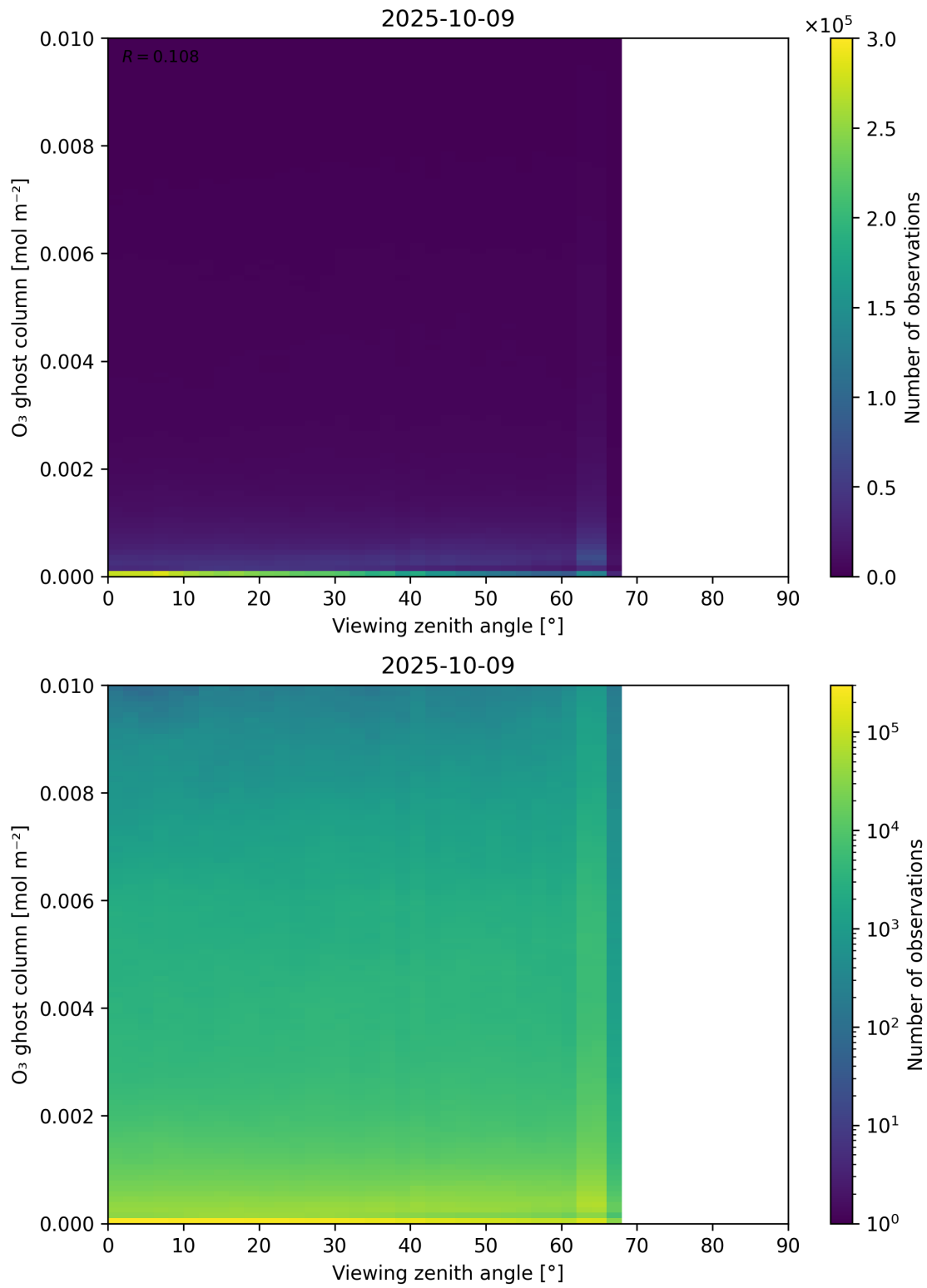
Figure 51: Scatter density plot of “Viewing zenith angle” against “O 3 ghost column” for 2025-10-08 to 2025-10-10.
