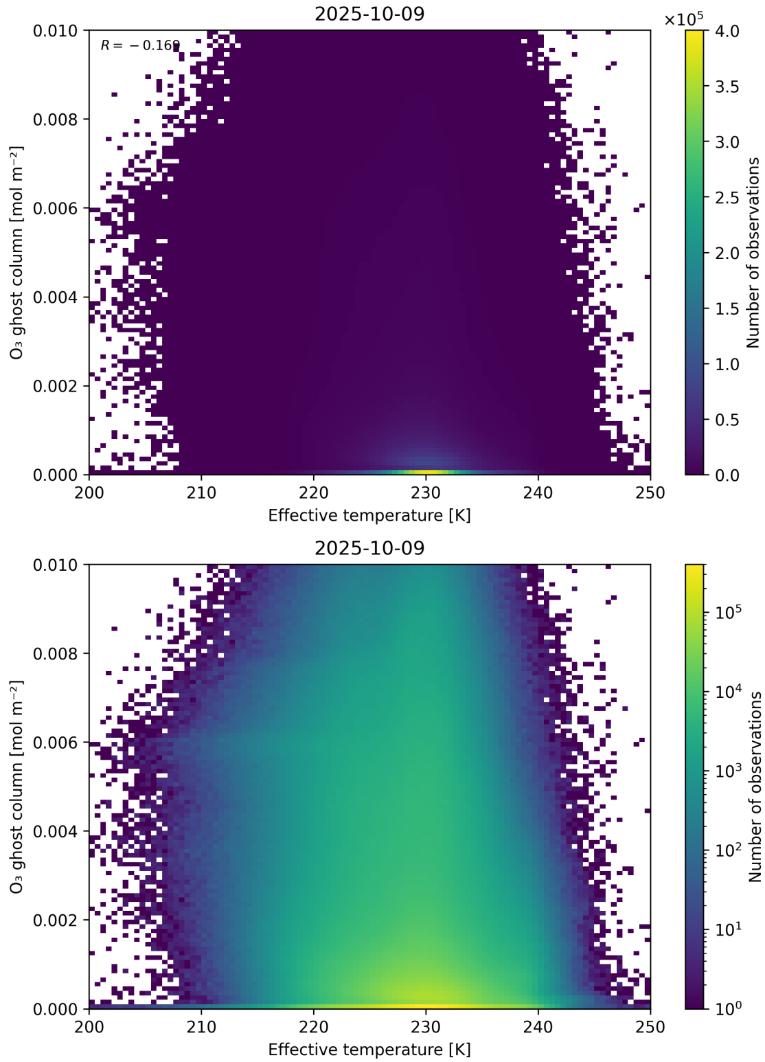
Figure 38: Scatter density plot of “Effective temperature” against “O 3 ghost column” for 2025-10-08 to 2025-10-10.
