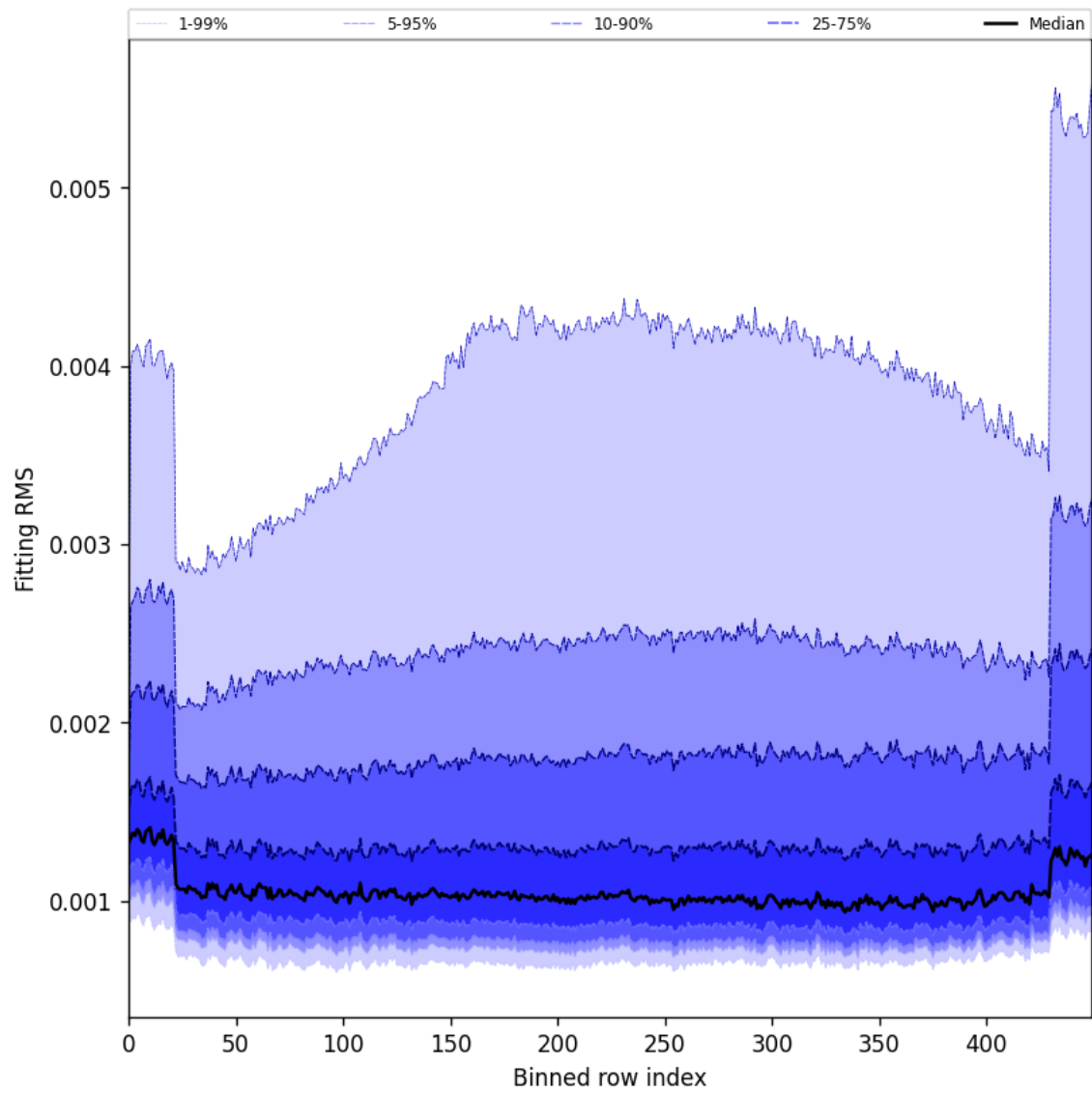
Figure 30: Along track statistics of “Fitting RMS” for 2025-10-08 to 2025-10-10
