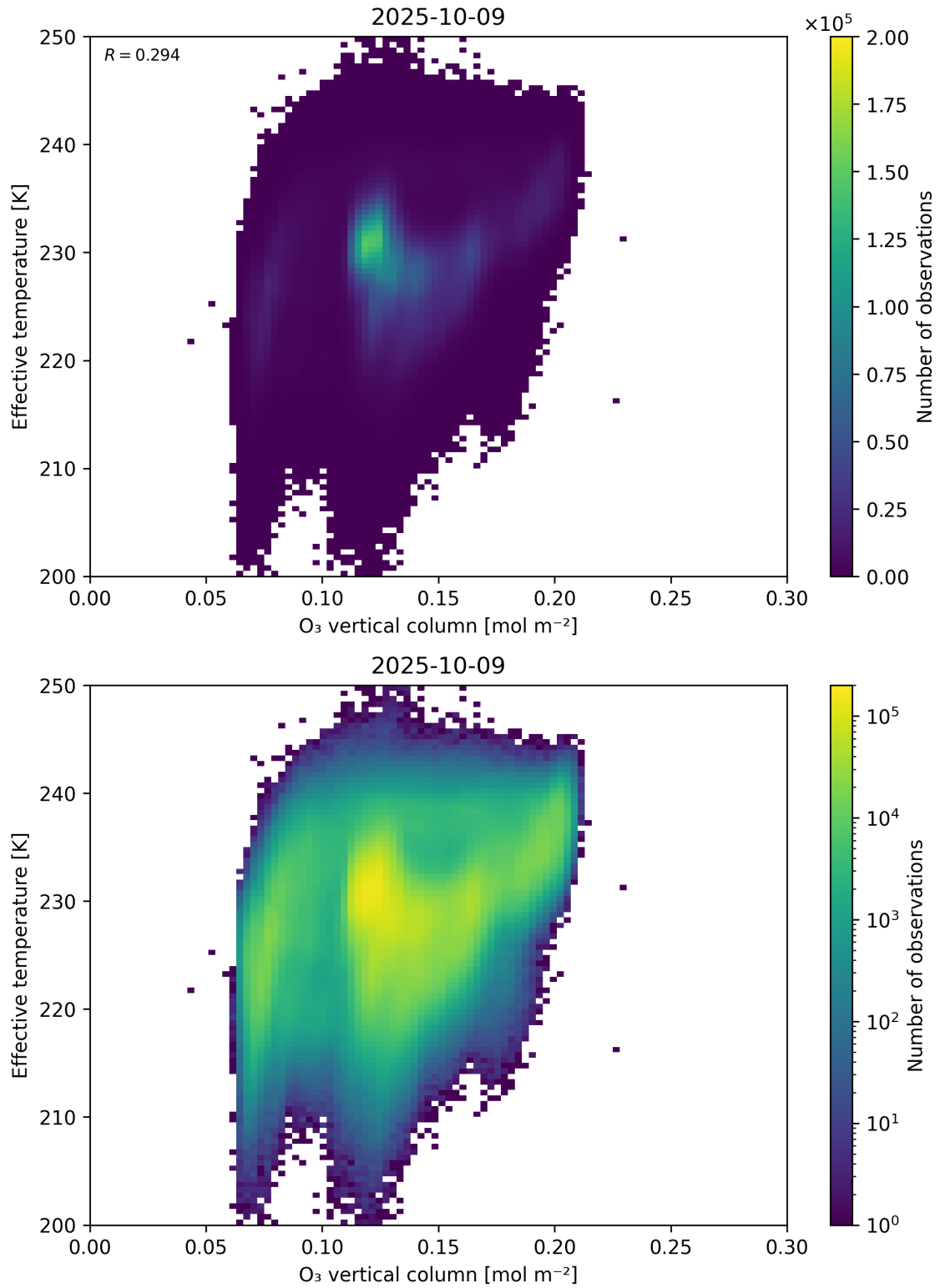
Figure 39: Scatter density plot of “O 3 vertical column” against “Effective temperature” for 2025-10-08 to 2025-10-10.
