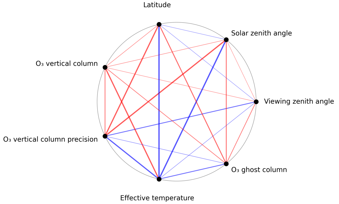
Figure 1: Map of correlation graph for 2025-10-08 to 2025-10-10.
