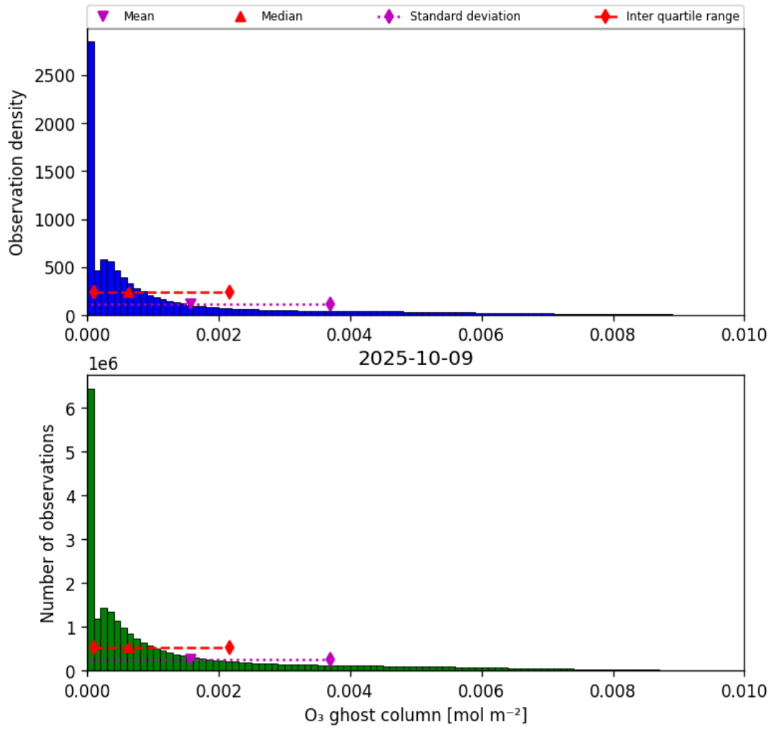
Figure 25: Histogram of “O 3 ghost column” for 2025-10-08 to 2025-10-10
