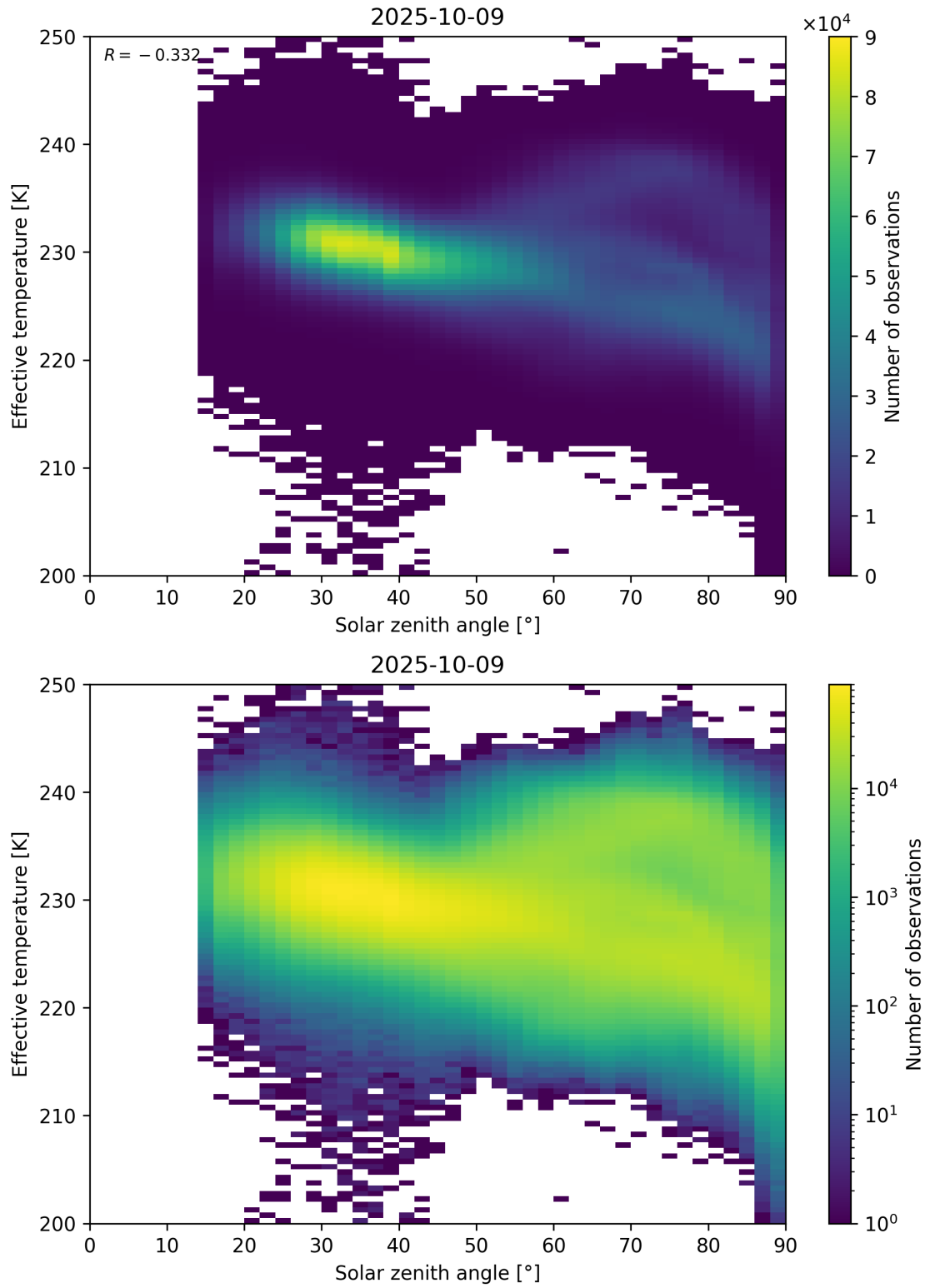
Figure 45: Scatter density plot of “Solar zenith angle” against “Effective temperature” for 2025-10-08 to 2025-10-10.
