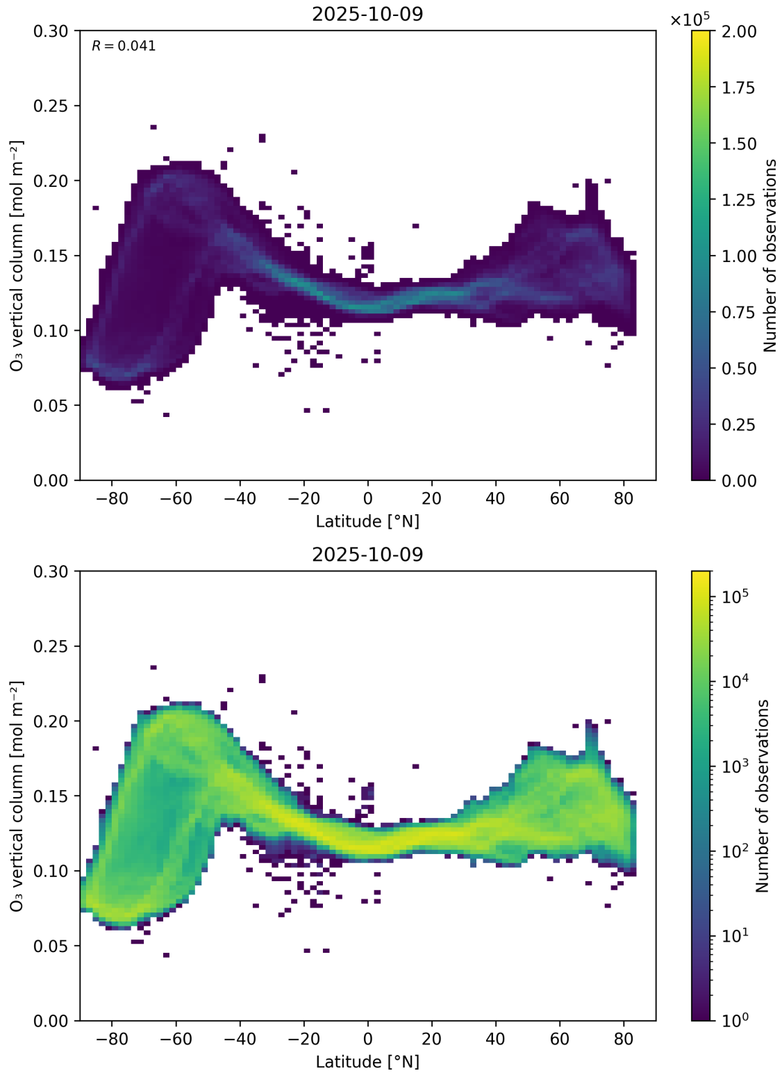
Figure 36: Scatter density plot of “Latitude” against “O 3 vertical column” for 2025-10-08 to 2025-10-10.
