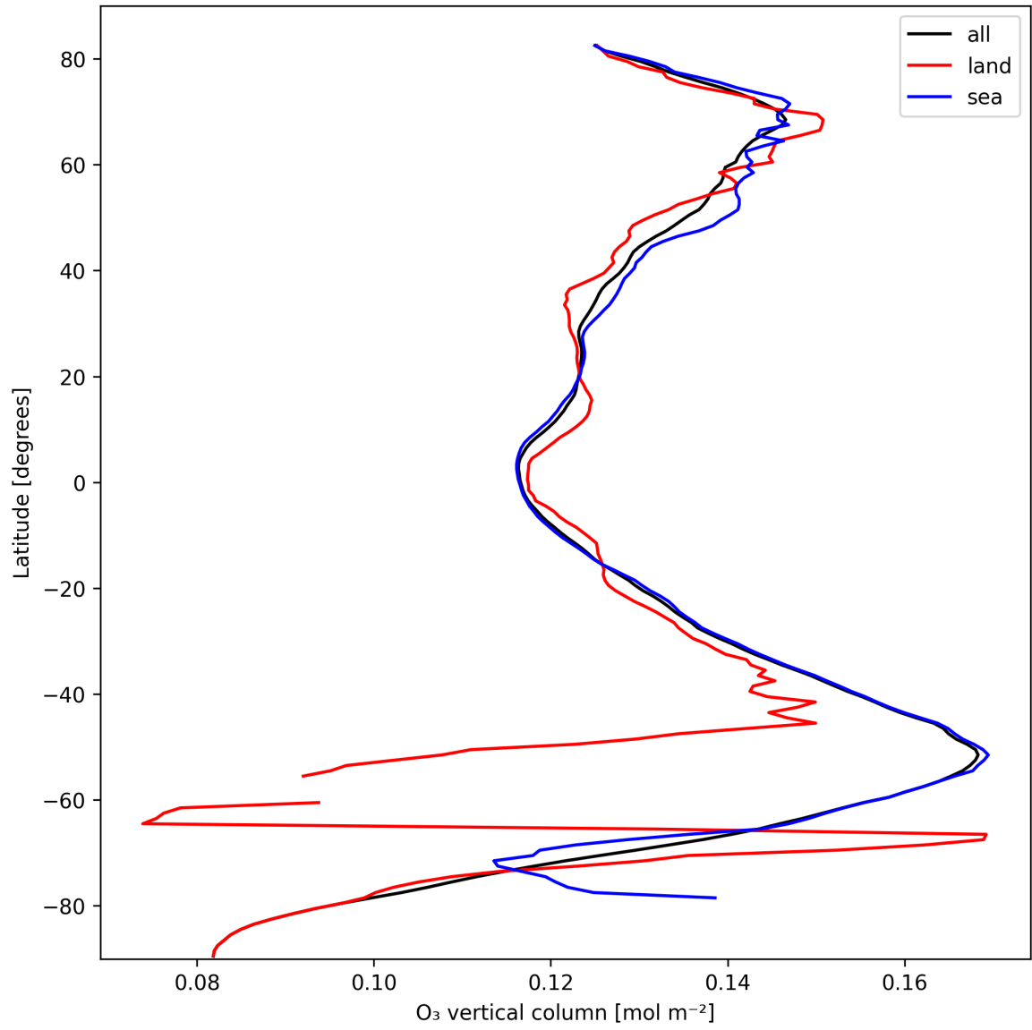
Figure 14: Zonal average of “O 3 vertical column” for 2025-10-08 to 2025-10-10.
