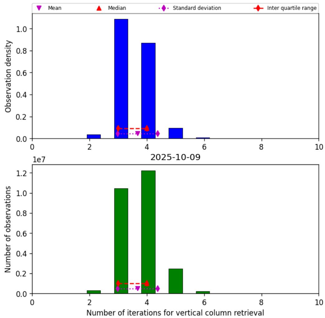
Figure 26: Histogram of “Number of iterations for vertical column retrieval” for 2025-10-08 to 2025-10-10
