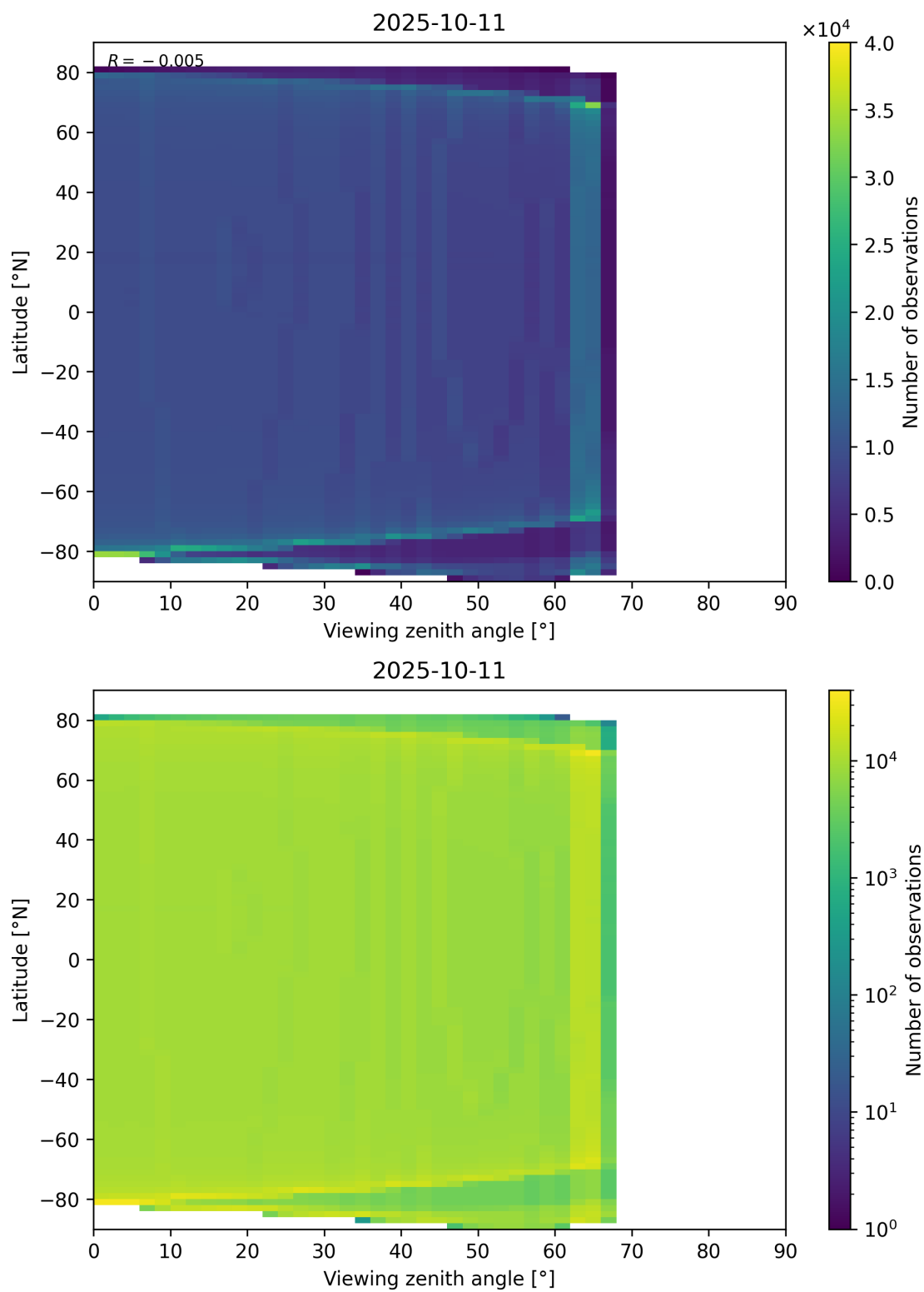
Figure 49: Scatter density plot of “Viewing zenith angle” against “Latitude” for 2025-10-11 to 2025-10-12.
