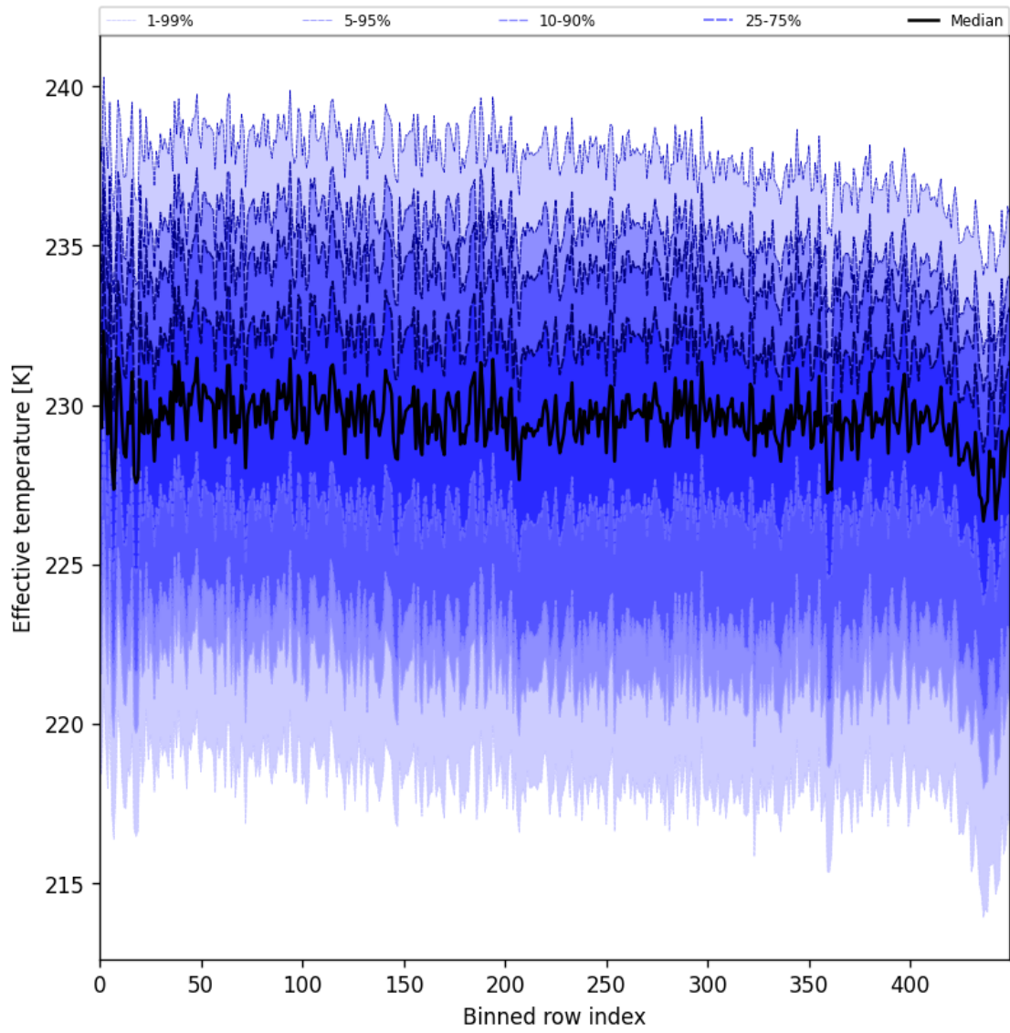
Figure 31: Along track statistics of “Effective temperature” for 2025-10-11 to 2025-10-12
