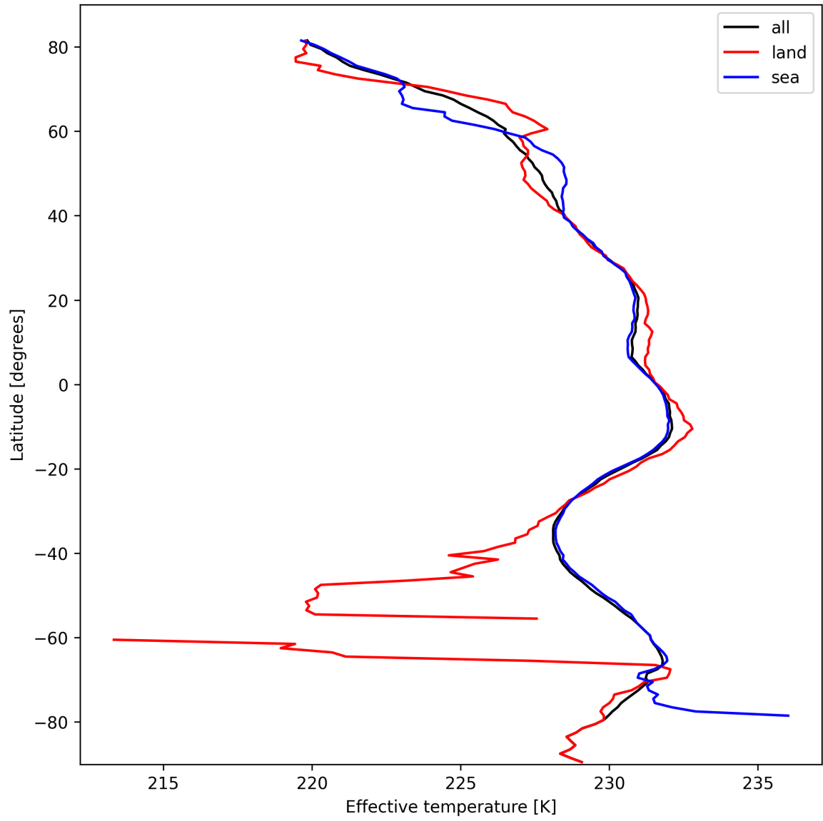
Figure 17: Zonal average of "Effective temperature" for 2025-10-11 to 2025-10-12.
