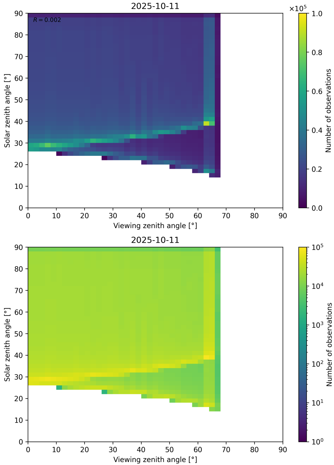
Figure 54: Scatter density plot of “Viewing zenith angle” against “Solar zenith angle” for 2025-10-11 to 2025-10-12.
