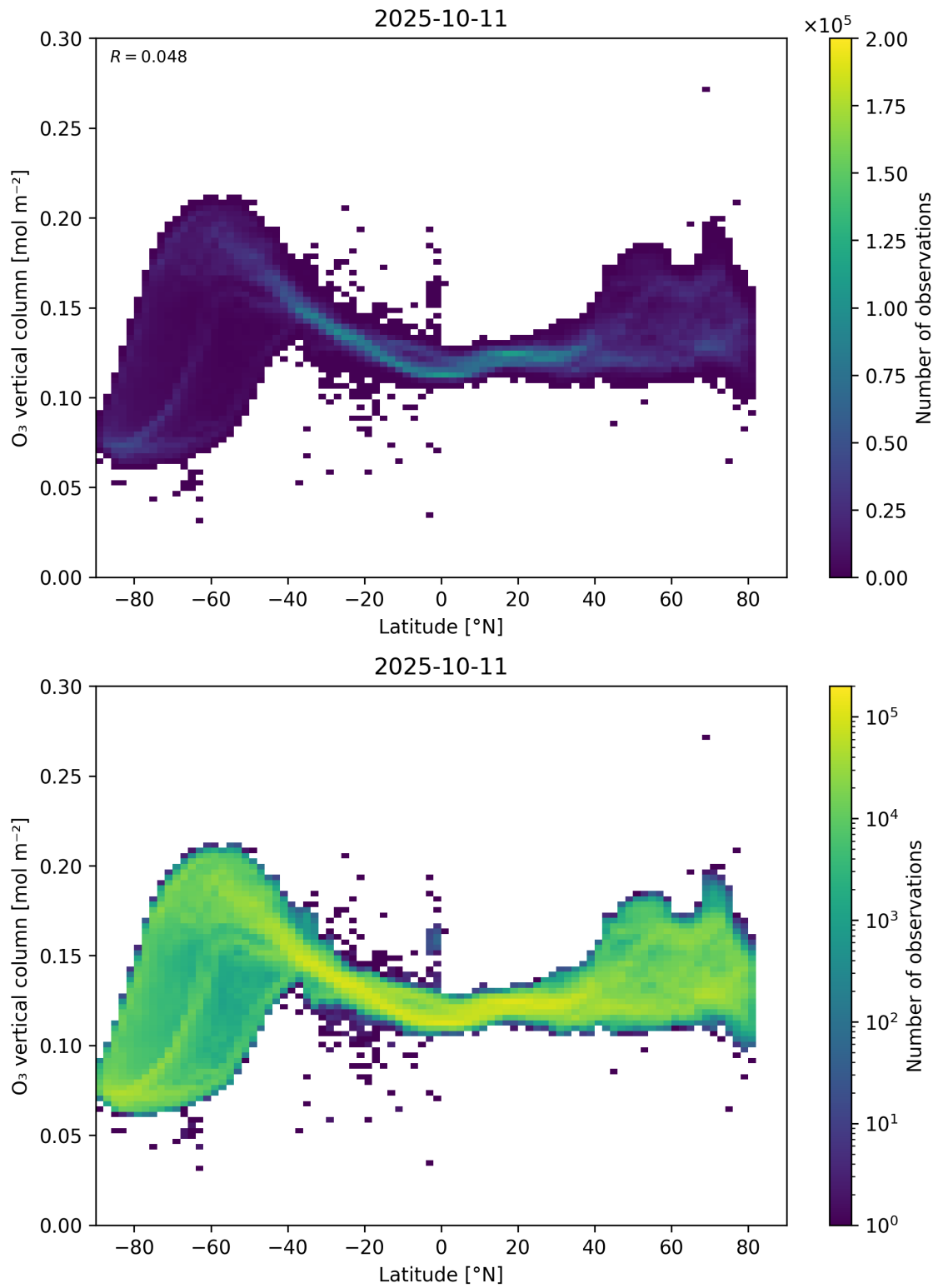
Figure 36: Scatter density plot of “Latitude” against “O 3 vertical column” for 2025-10-11 to 2025-10-12.
