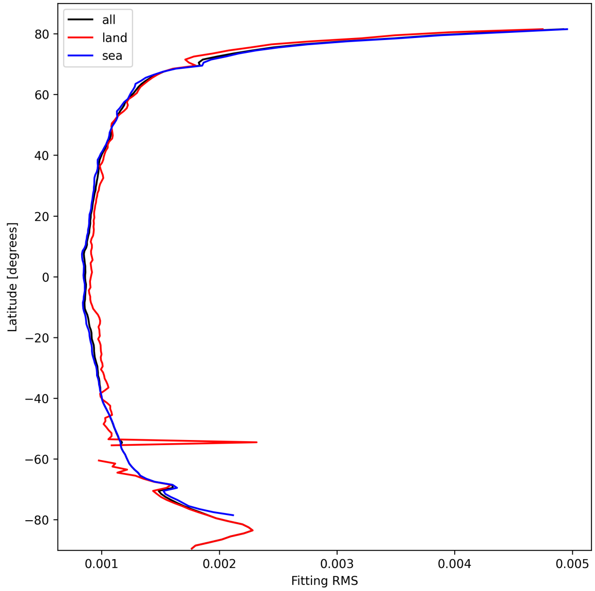
Figure 16: Zonal average of “Fitting RMS” for 2025-10-11 to 2025-10-12.
