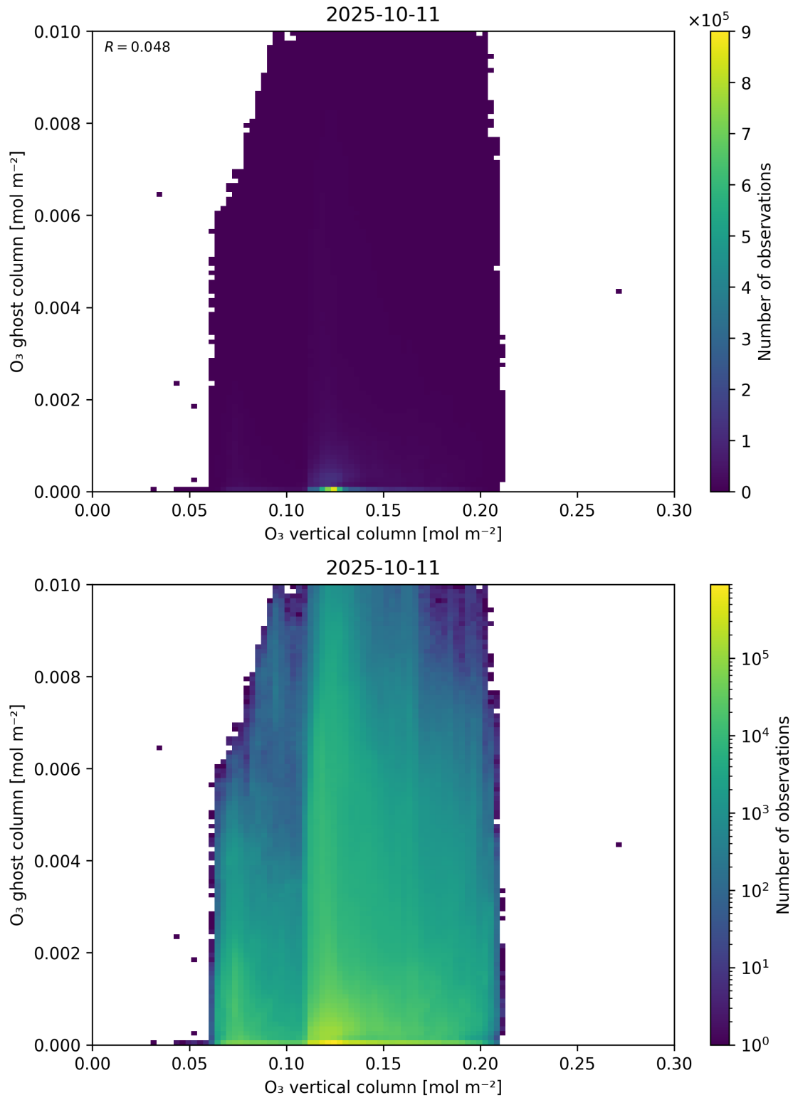
Figure 40: Scatter density plot of “O 3 vertical column” against “O 3 ghost column” for 2025-10-11 to 2025-10-12.
