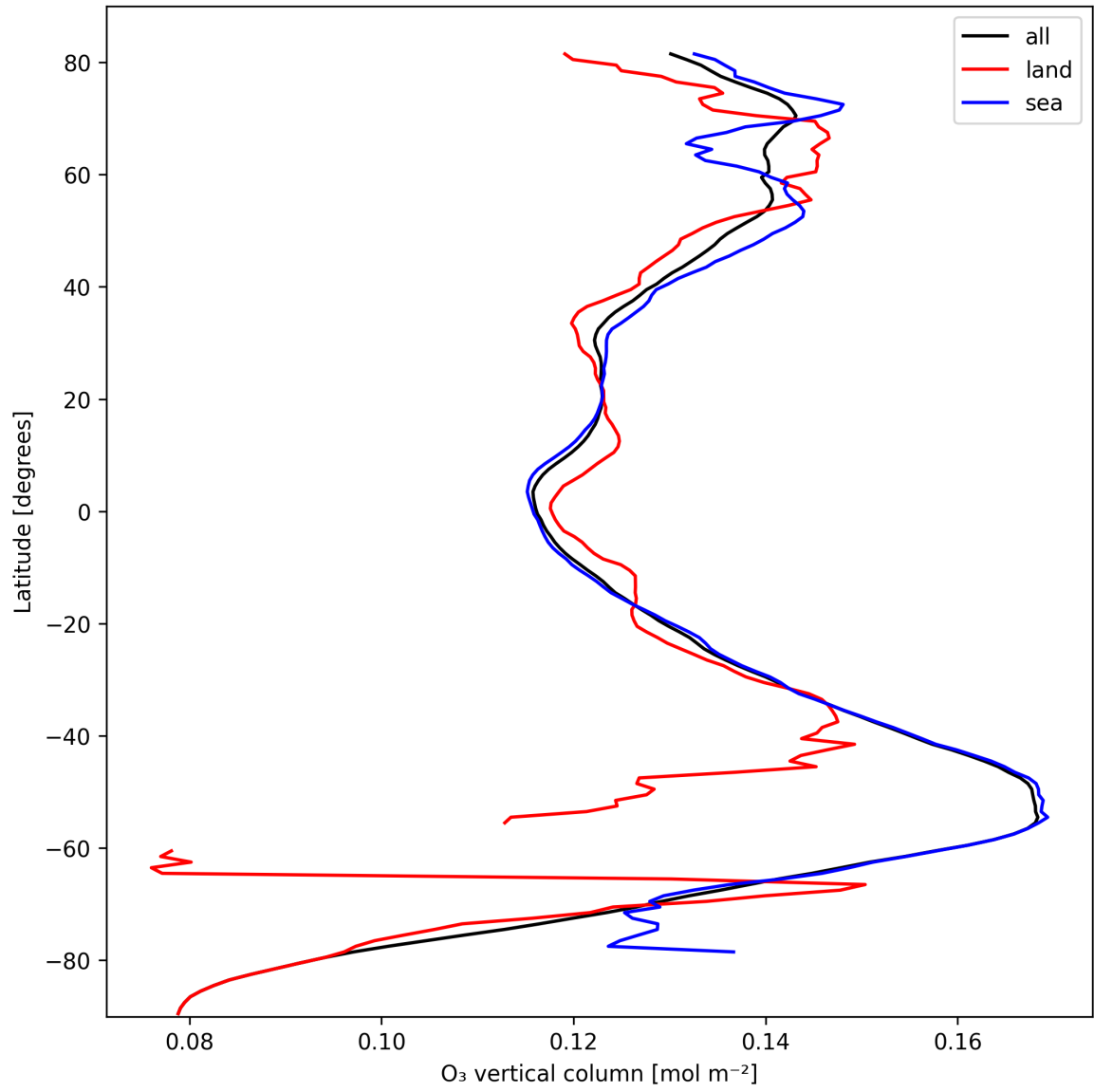
Figure 14: Zonal average of “O 3 vertical column” for 2025-10-11 to 2025-10-12.
