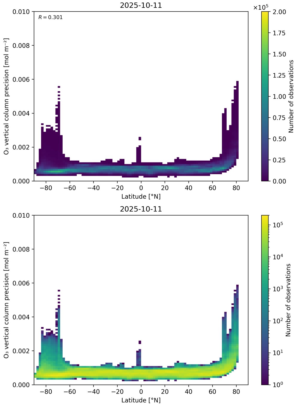
Figure 37: Scatter density plot of “Latitude” against “O 3 vertical column precision” for 2025-10-11 to 2025-10-12.
