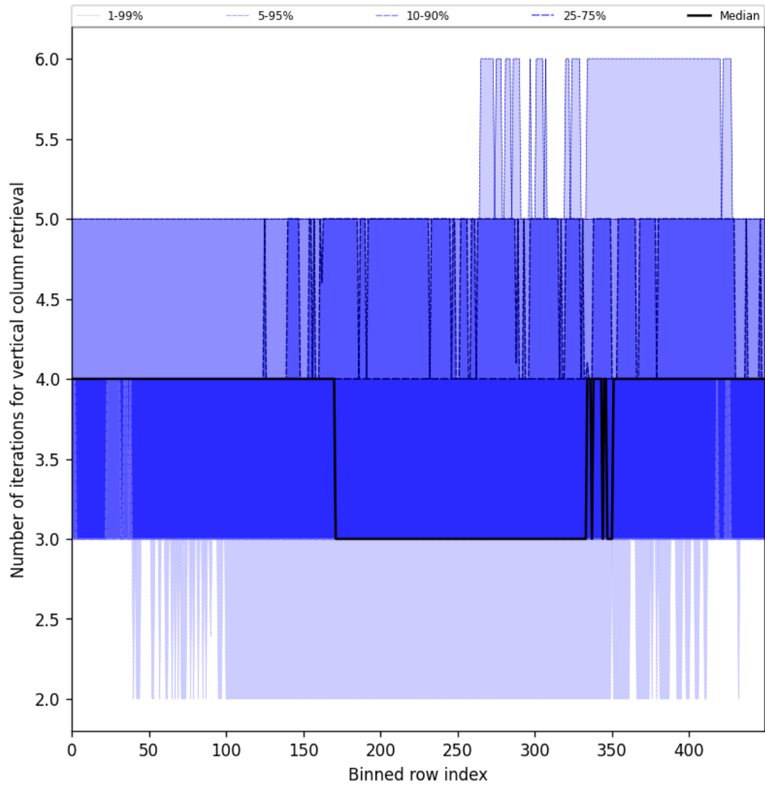
Figure 33: Along track statistics of “Number of iterations for vertical column retrieval” for 2025-10-11 to 2025-10-12
