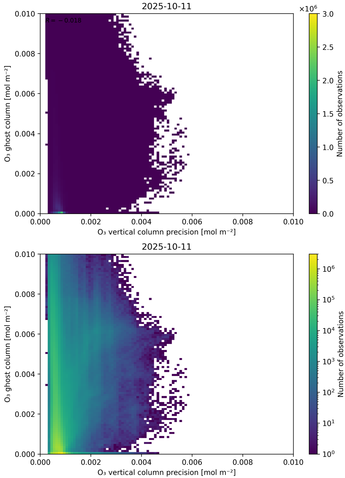
Figure 43: Scatter density plot of “ O_3 vertical column precision” against “ O_3 ghost column” for 2025-10-11 to 2025-10-12.
