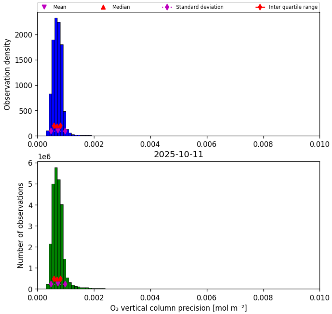
Figure 22: Histogram of “O 3 vertical column precision” for 2025-10-11 to 2025-10-12
