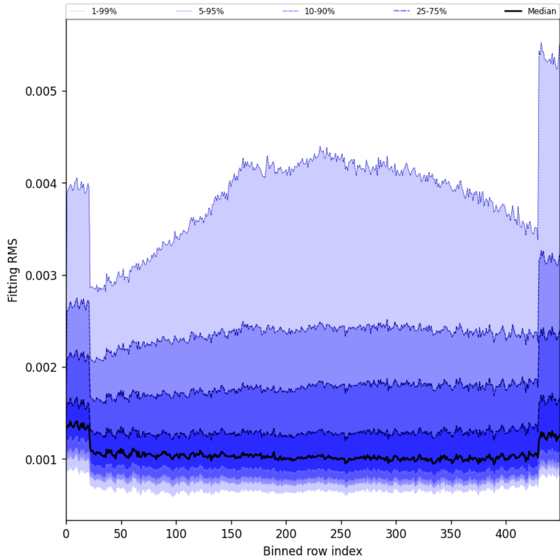
Figure 30: Along track statistics of “Fitting RMS” for 2025-10-11 to 2025-10-12
