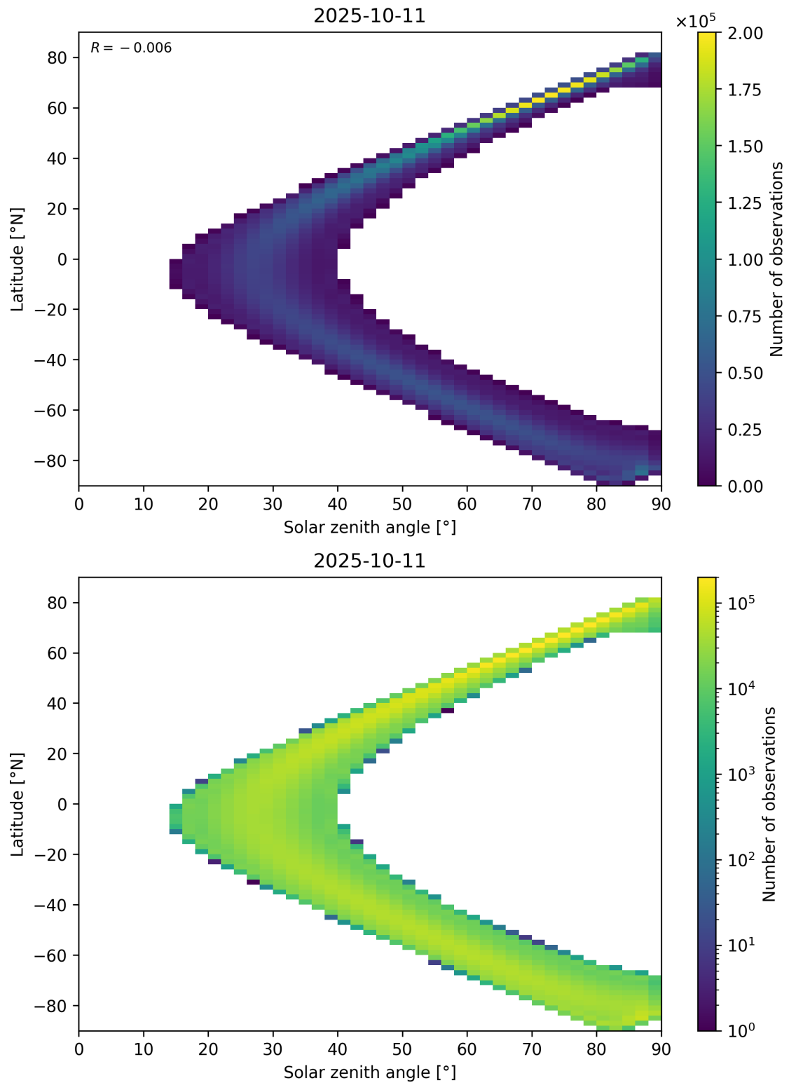
Figure 44: Scatter density plot of “Solar zenith angle” against “Latitude” for 2025-10-11 to 2025-10-12.
