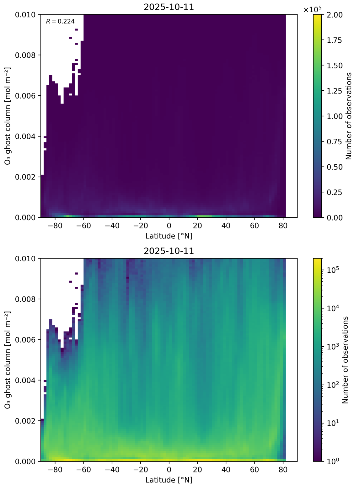
Figure 35: Scatter density plot of “Latitude” against “O 3 ghost column” for 2025-10-11 to 2025-10-12.
