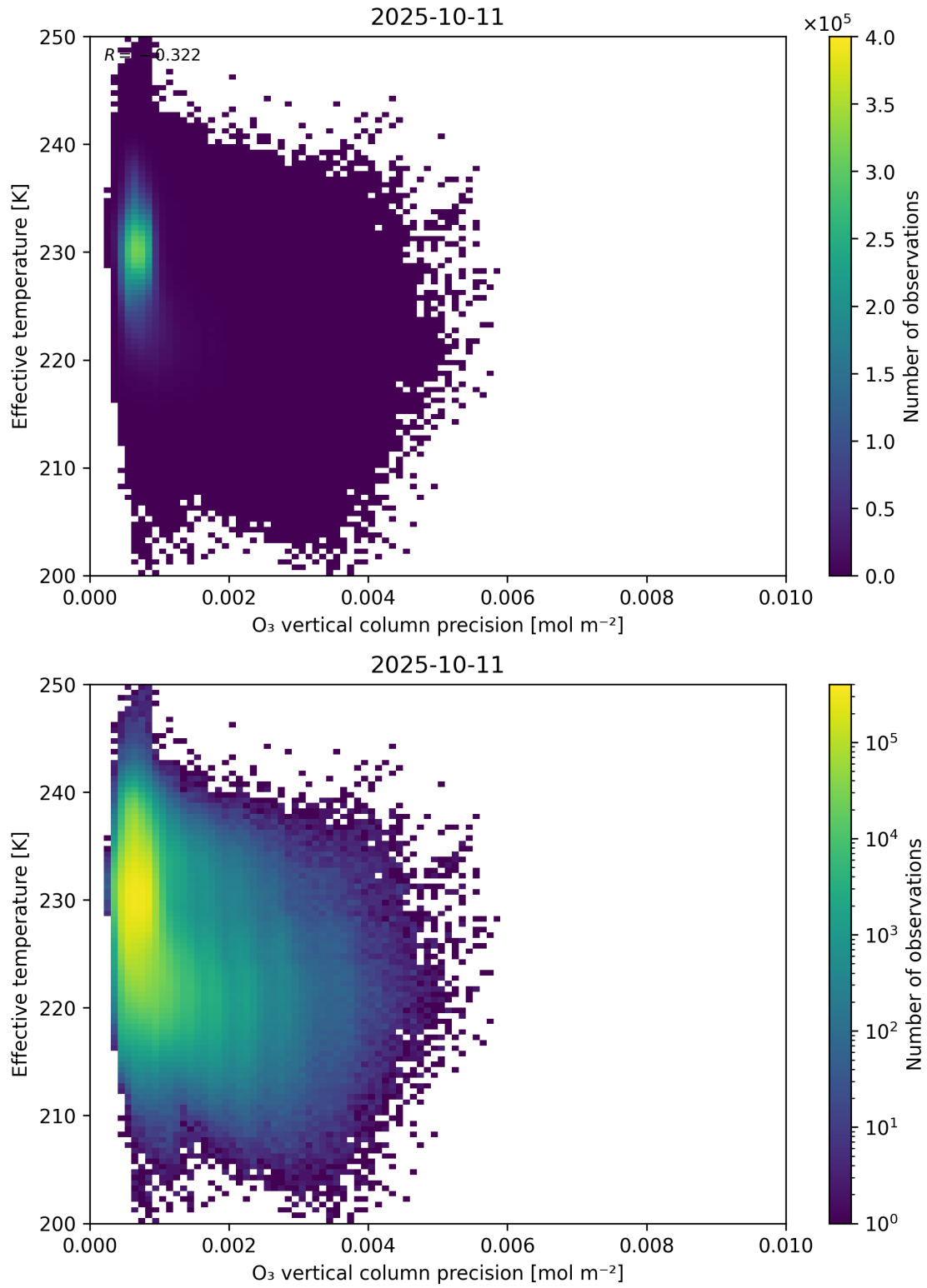
Figure 42: Scatter density plot of “O 3 vertical column precision” against “Effective temperature” for 2025-10-11 to 2025-10-12.
