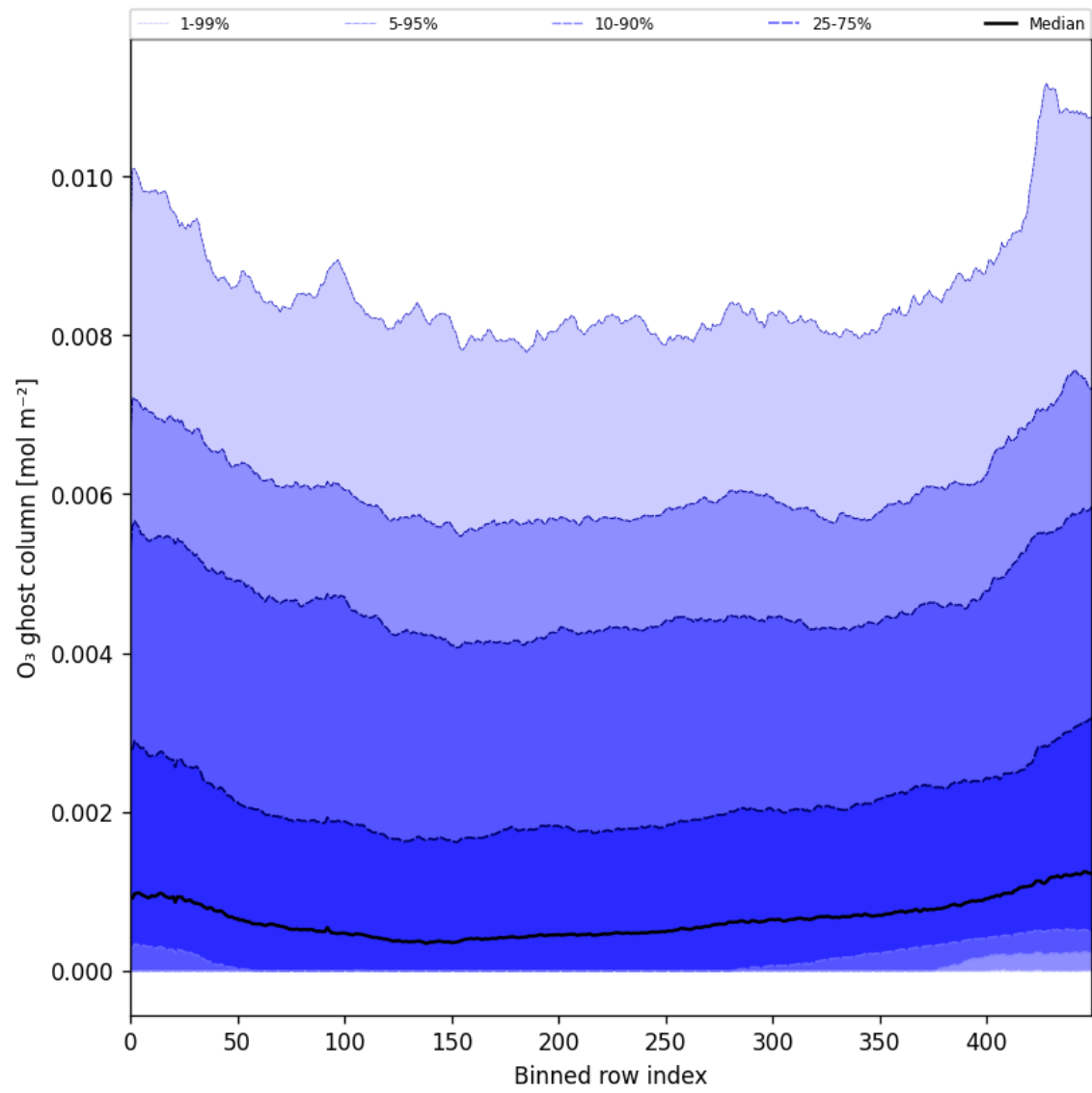
Figure 32: Along track statistics of “O 3 ghost column” for 2025-10-11 to 2025-10-12
