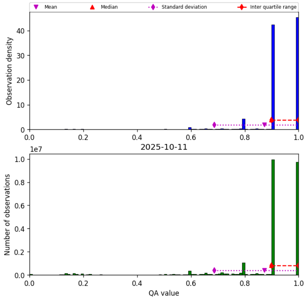
Figure 20: Histogram of “QA value” for 2025-10-11 to 2025-10-12
