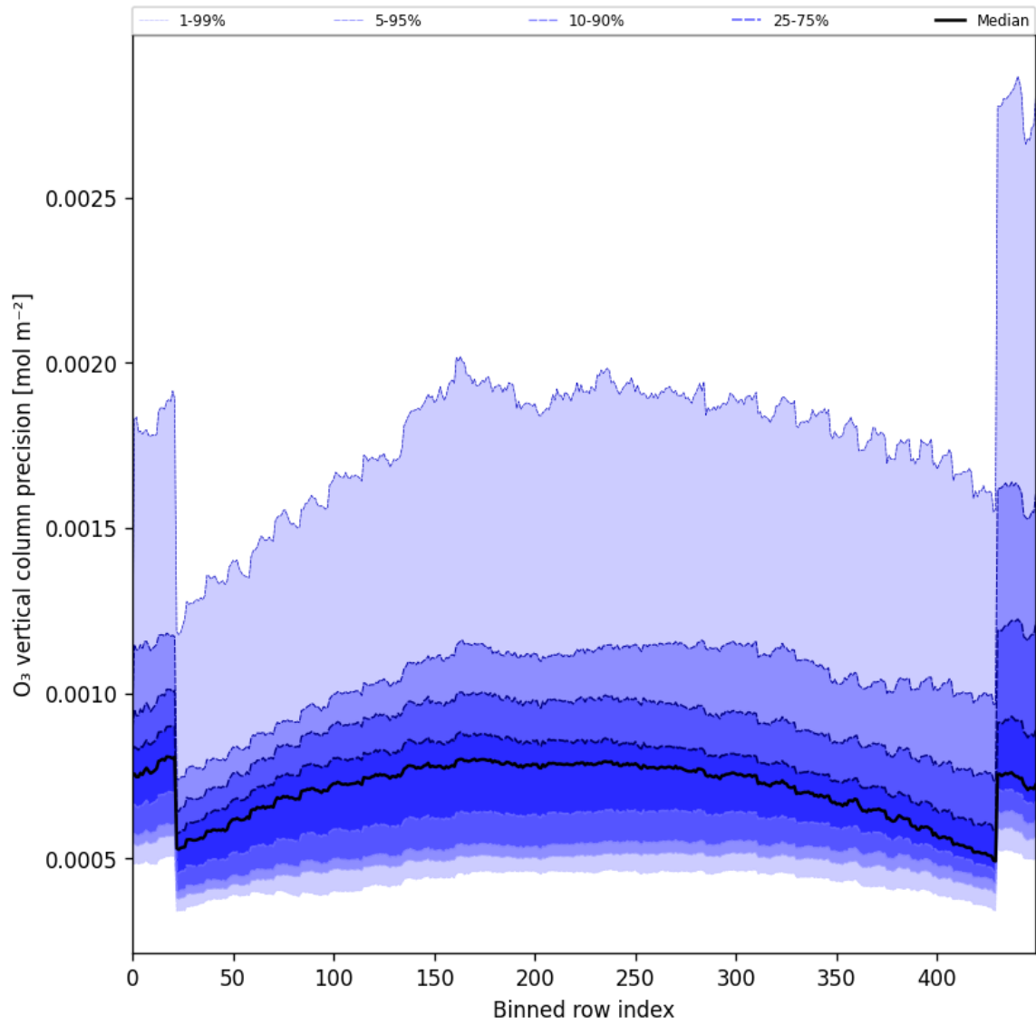
Figure 29: Along track statistics of “O 3 vertical column precision” for 2025-10-11 to 2025-10-12
