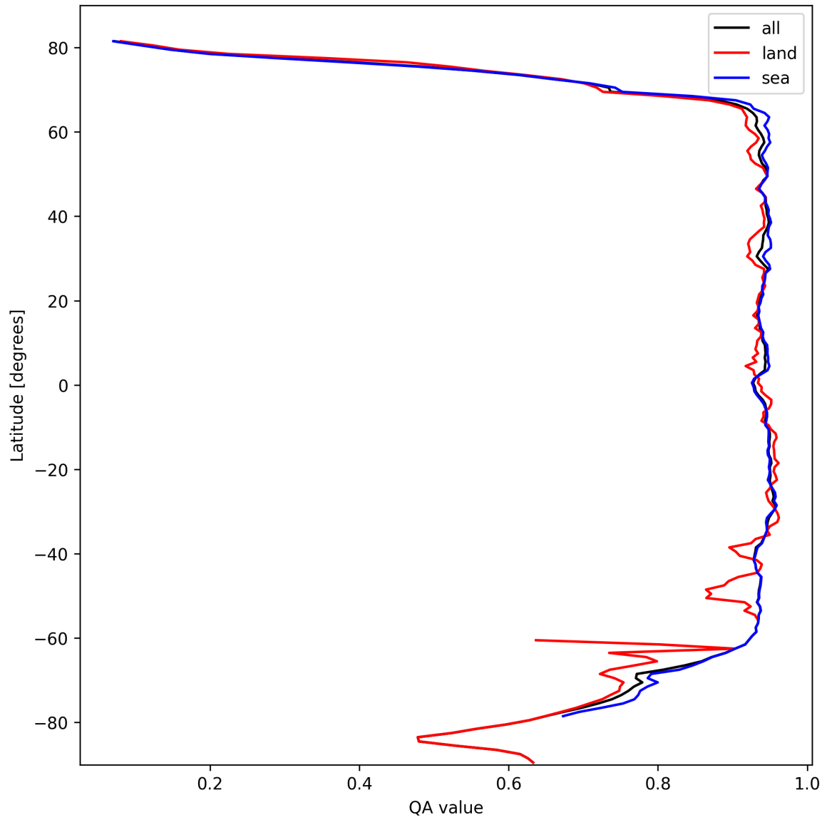
Figure 13: Zonal average of “QA value” for 2025-10-11 to 2025-10-12.
