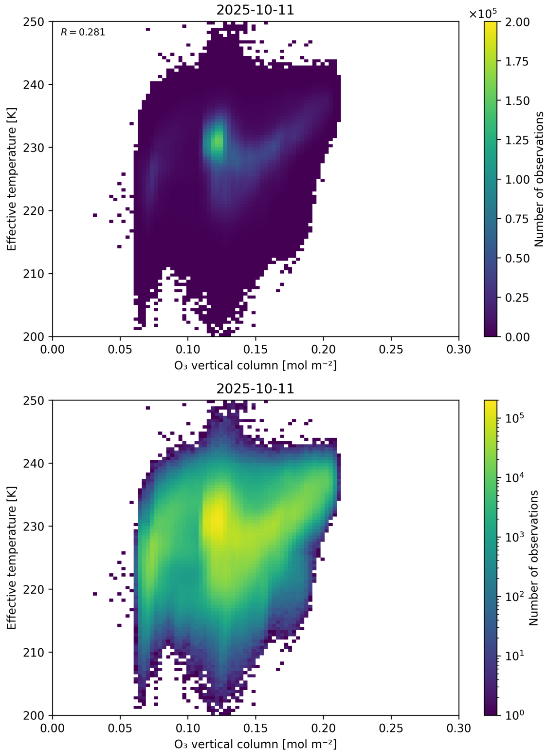
Figure 39: Scatter density plot of “O 3 vertical column” against “Effective temperature” for 2025-10-11 to 2025-10-12.
