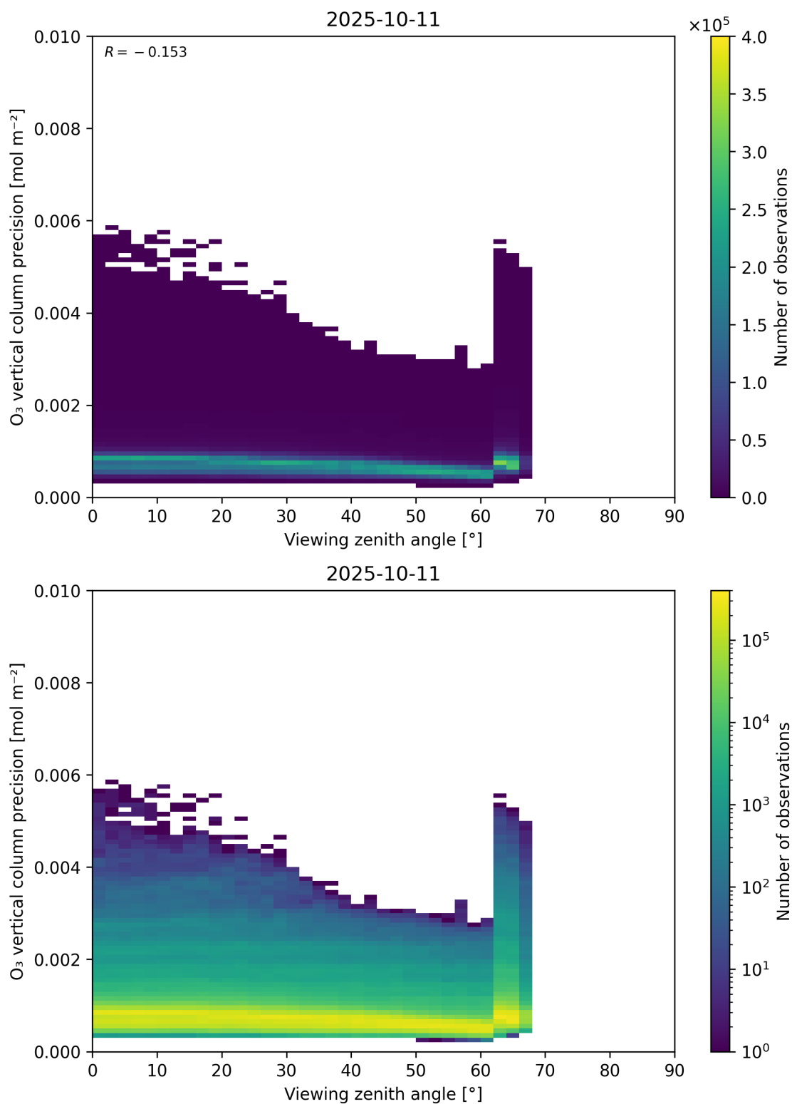
Figure 53: Scatter density plot of “Viewing zenith angle” against “O 3 vertical column precision” for 2025-10-11 to 2025-10-12.
