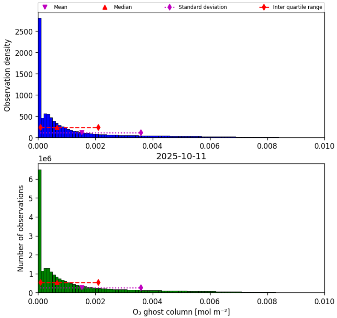
Figure 25: Histogram of “O 3 ghost column” for 2025-10-11 to 2025-10-12
