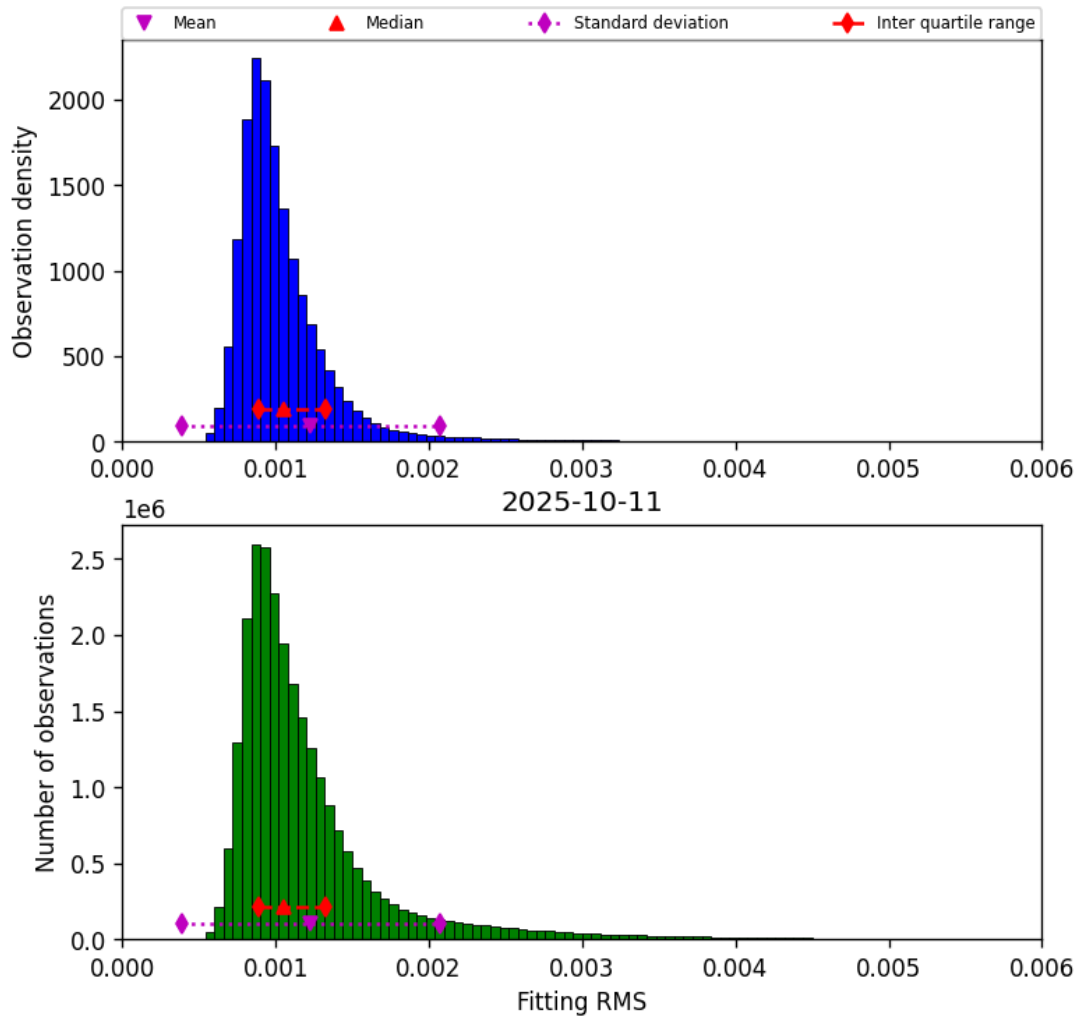
Figure 23: Histogram of “Fitting RMS” for 2025-10-11 to 2025-10-12
