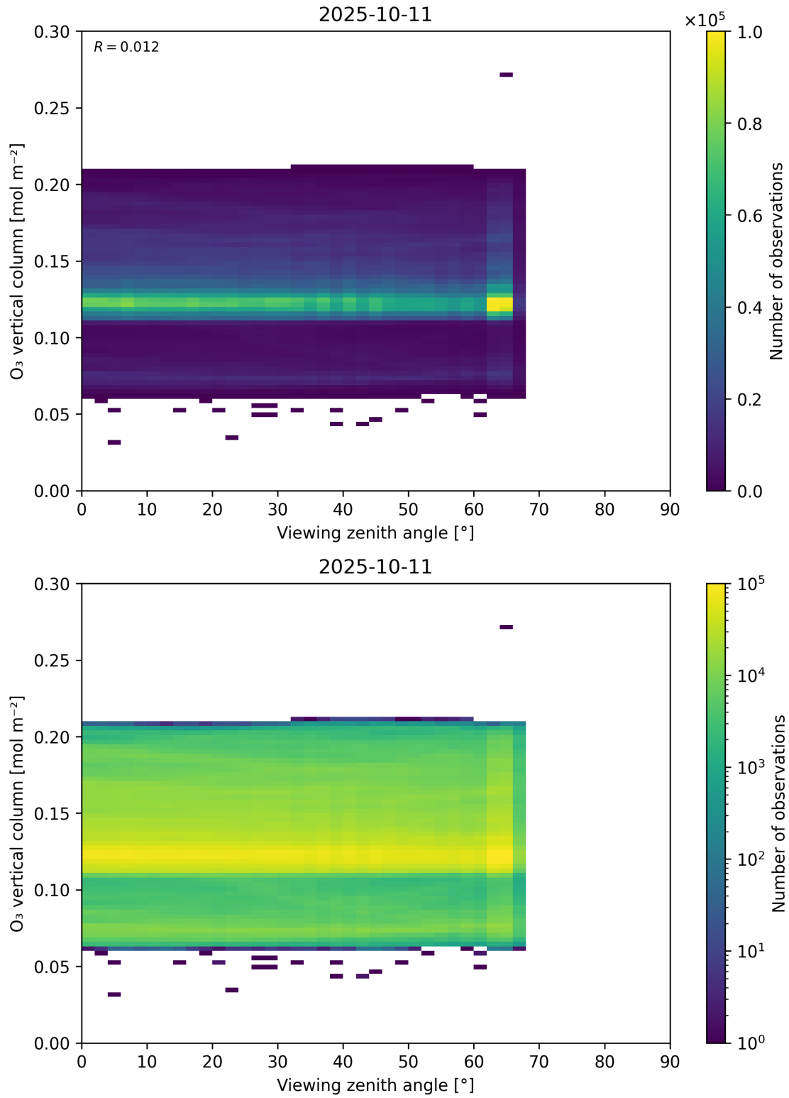
Figure 52: Scatter density plot of “Viewing zenith angle” against “O 3 vertical column” for 2025-10-11 to 2025-10-12.
