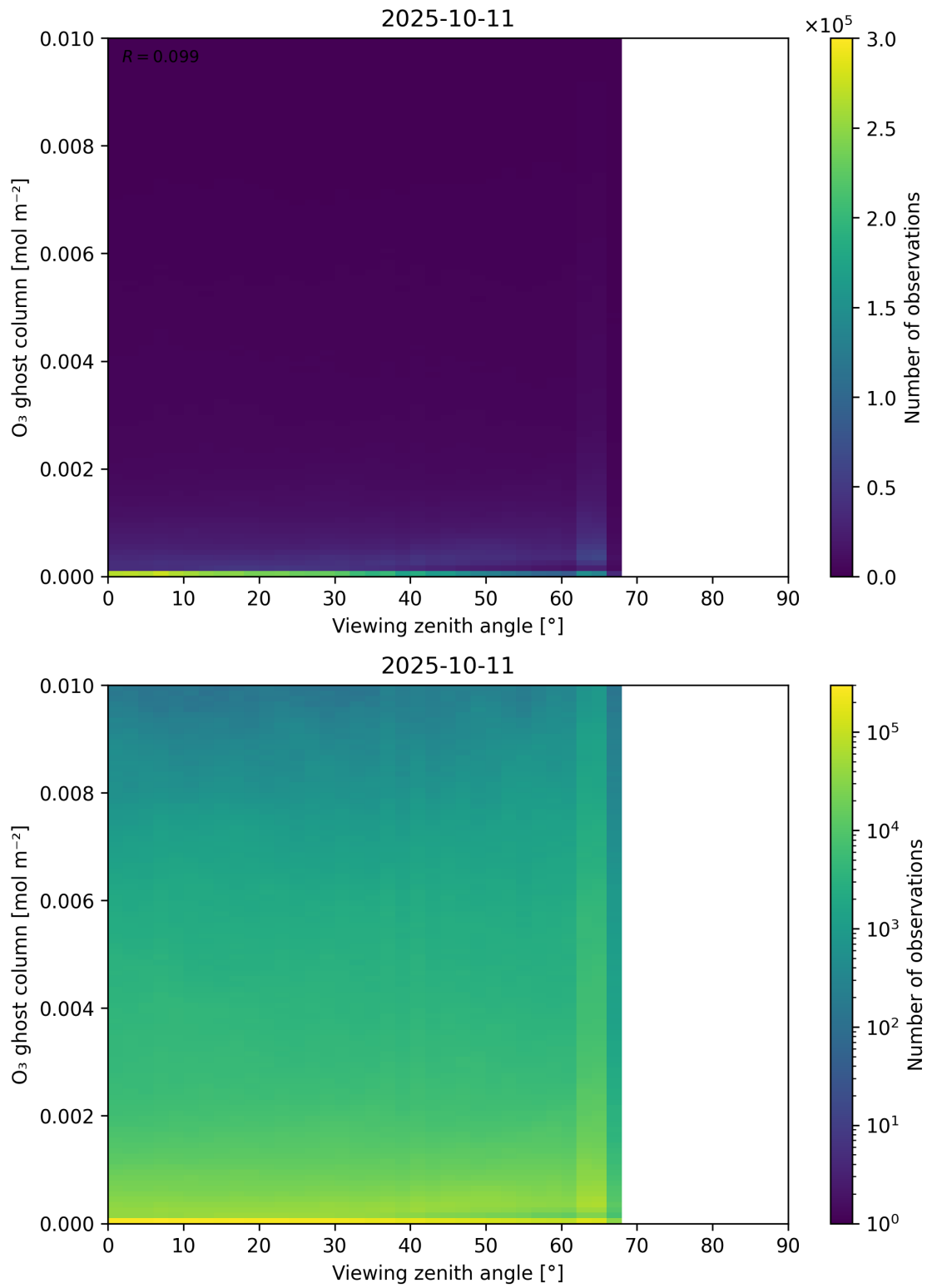
Figure 51: Scatter density plot of “Viewing zenith angle” against “O 3 ghost column” for 2025-10-11 to 2025-10-12.
