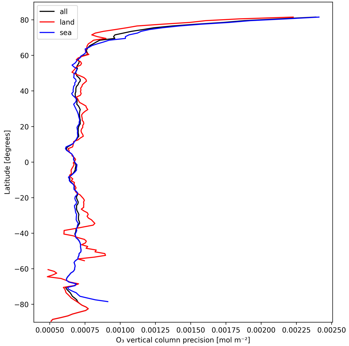
Figure 15: Zonal average of “O 3 vertical column precision” for 2025-10-11 to 2025-10-12.
