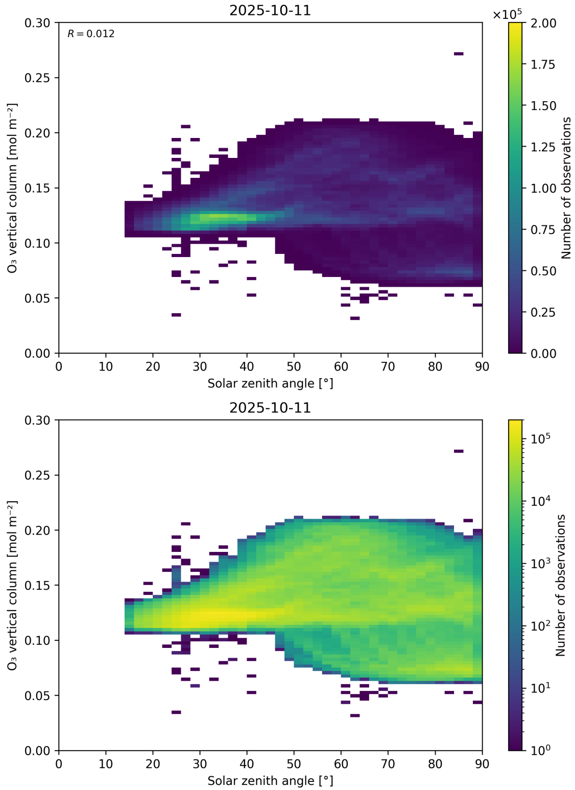
Figure 47: Scatter density plot of “Solar zenith angle” against “O 3 vertical column” for 2025-10-11 to 2025-10-12.
