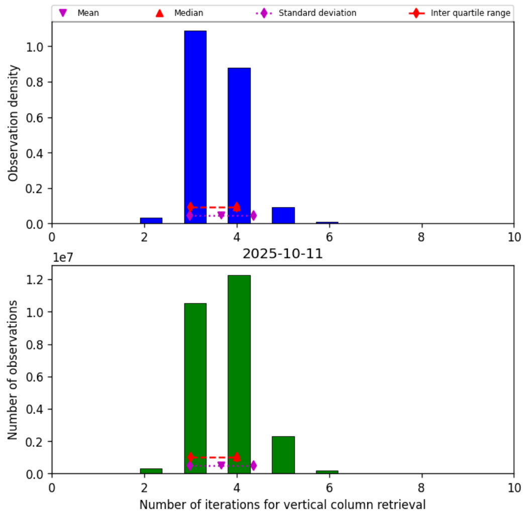
Figure 26: Histogram of “Number of iterations for vertical column retrieval” for 2025-10-11 to 2025-10-12
