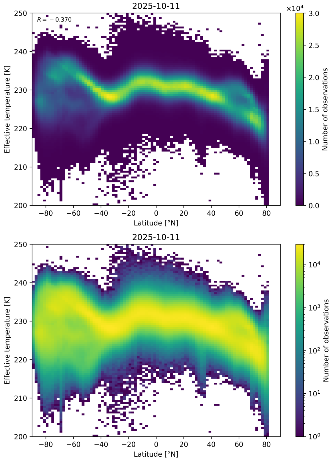
Figure 34: Scatter density plot of “Latitude” against “Effective temperature” for 2025-10-11 to 2025-10-12.
