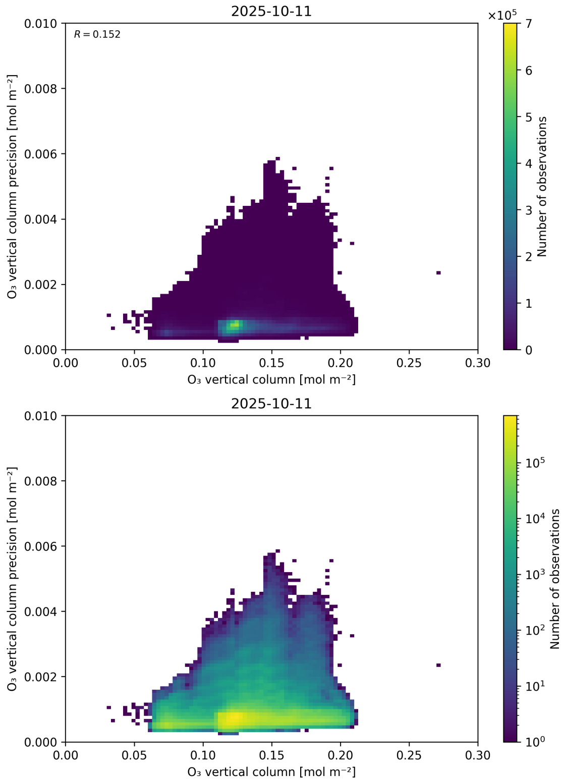
Figure 41: Scatter density plot of “O 3 vertical column” against “O 3 vertical column precision” for 2025-10-11 to 2025-10-12.
