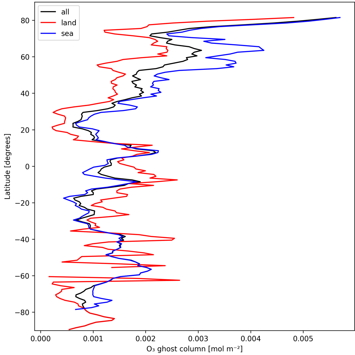
Figure 18: Zonal average of "O 3 ghost column" for 2025-10-11 to 2025-10-12.
