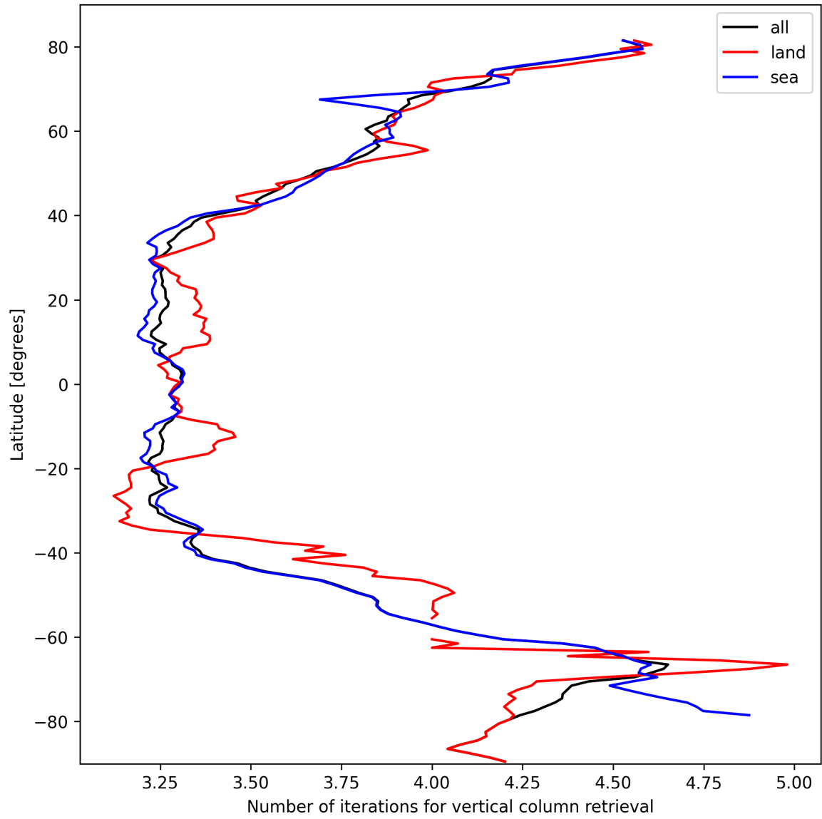
Figure 19: Zonal average of “Number of iterations for vertical column retrieval” for 2025-10-11 to 2025-10-12.
