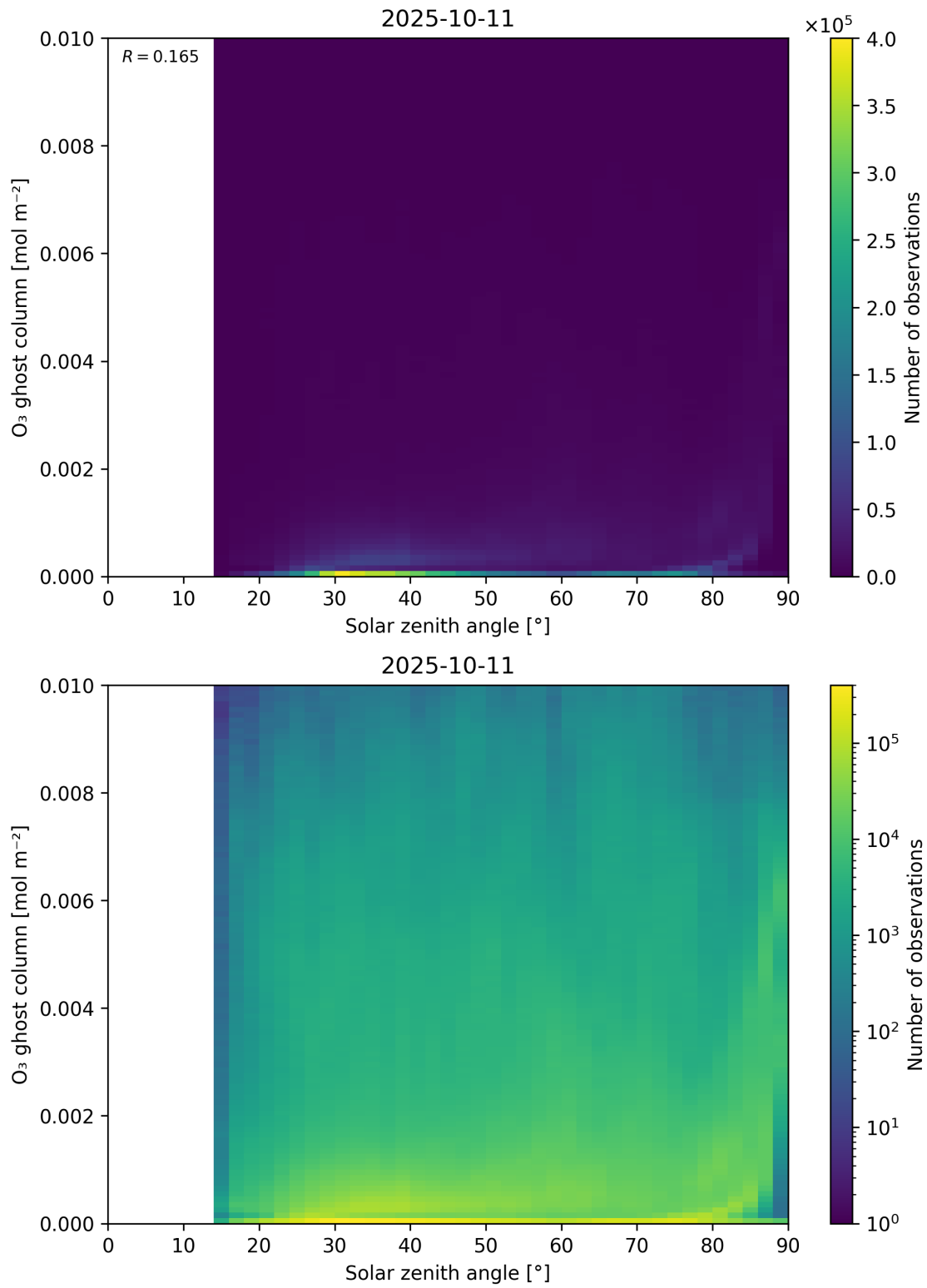
Figure 46: Scatter density plot of “Solar zenith angle” against “O 3 ghost column” for 2025-10-11 to 2025-10-12.
