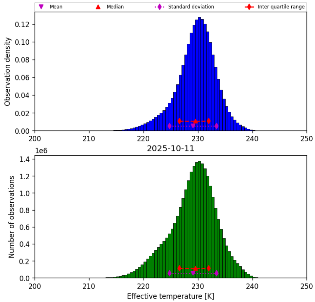
Figure 24: Histogram of “Effective temperature” for 2025-10-11 to 2025-10-12
