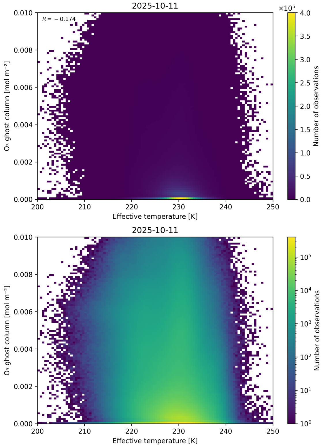
Figure 38: Scatter density plot of “Effective temperature” against “O 3 ghost column” for 2025-10-11 to 2025-10-12.
