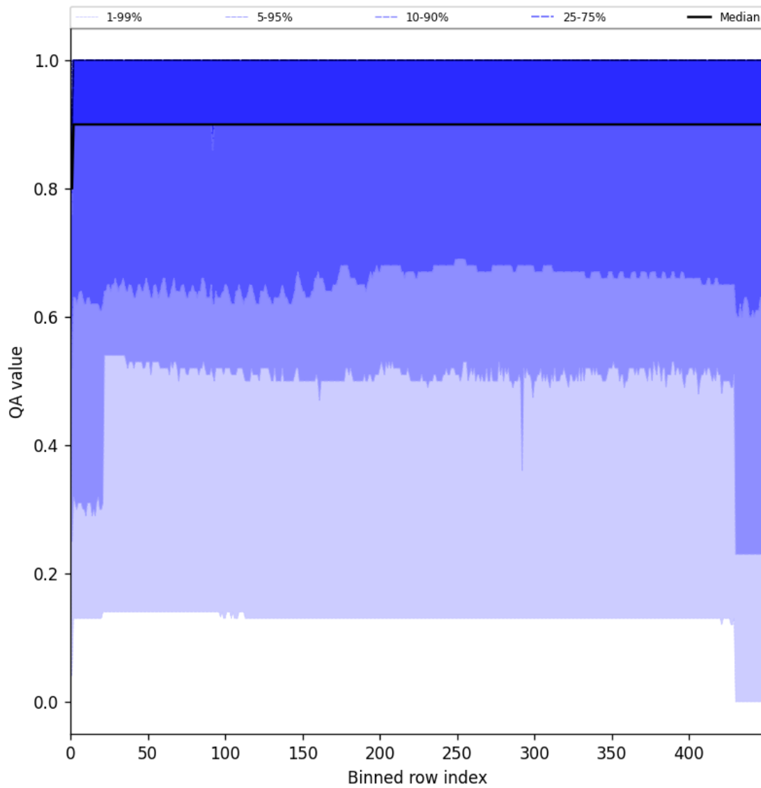
Figure 27: Along track statistics of “QA value” for 2025-10-11 to 2025-10-12
