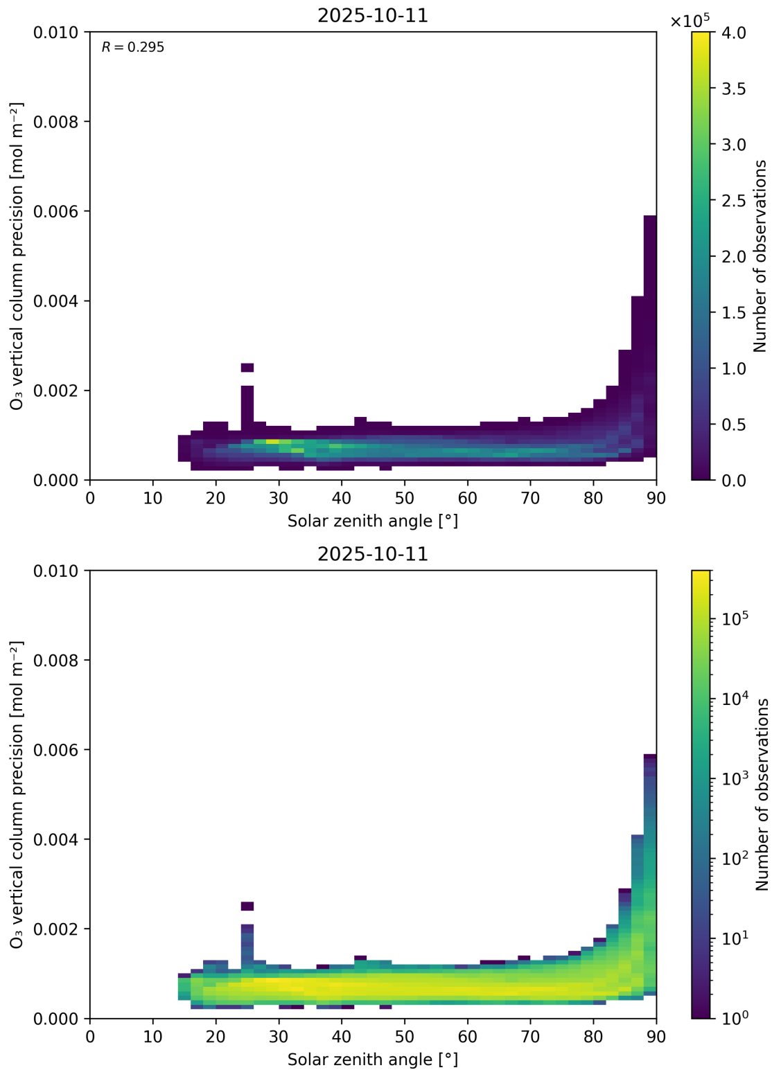
Figure 48: Scatter density plot of “Solar zenith angle” against “O 3 vertical column precision” for 2025-10-11 to 2025-10-12.
