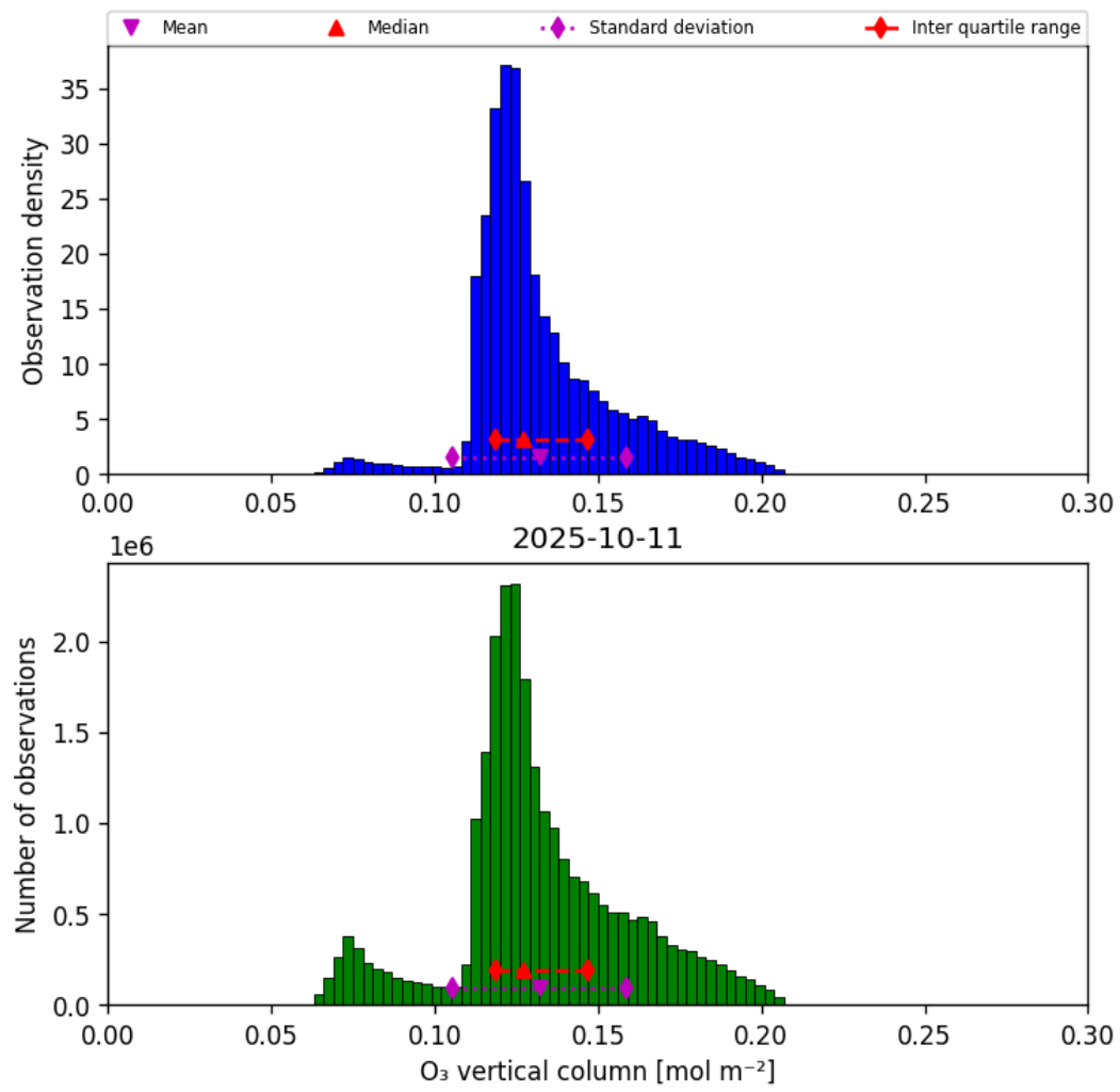
Figure 21: Histogram of “O 3 vertical column” for 2025-10-11 to 2025-10-12
