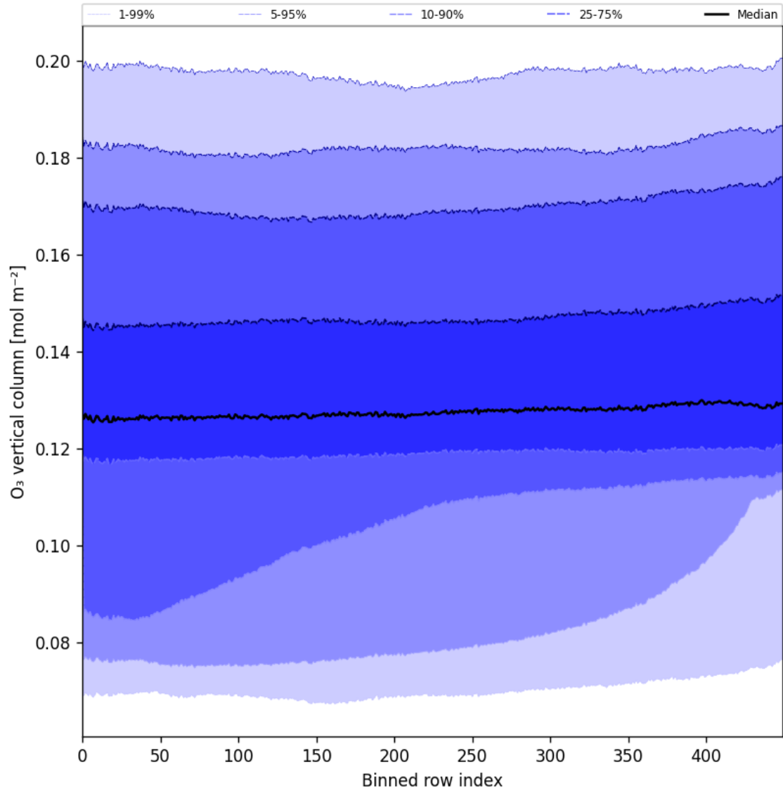
Figure 28: Along track statistics of “O 3 vertical column” for 2025-10-11 to 2025-10-12
