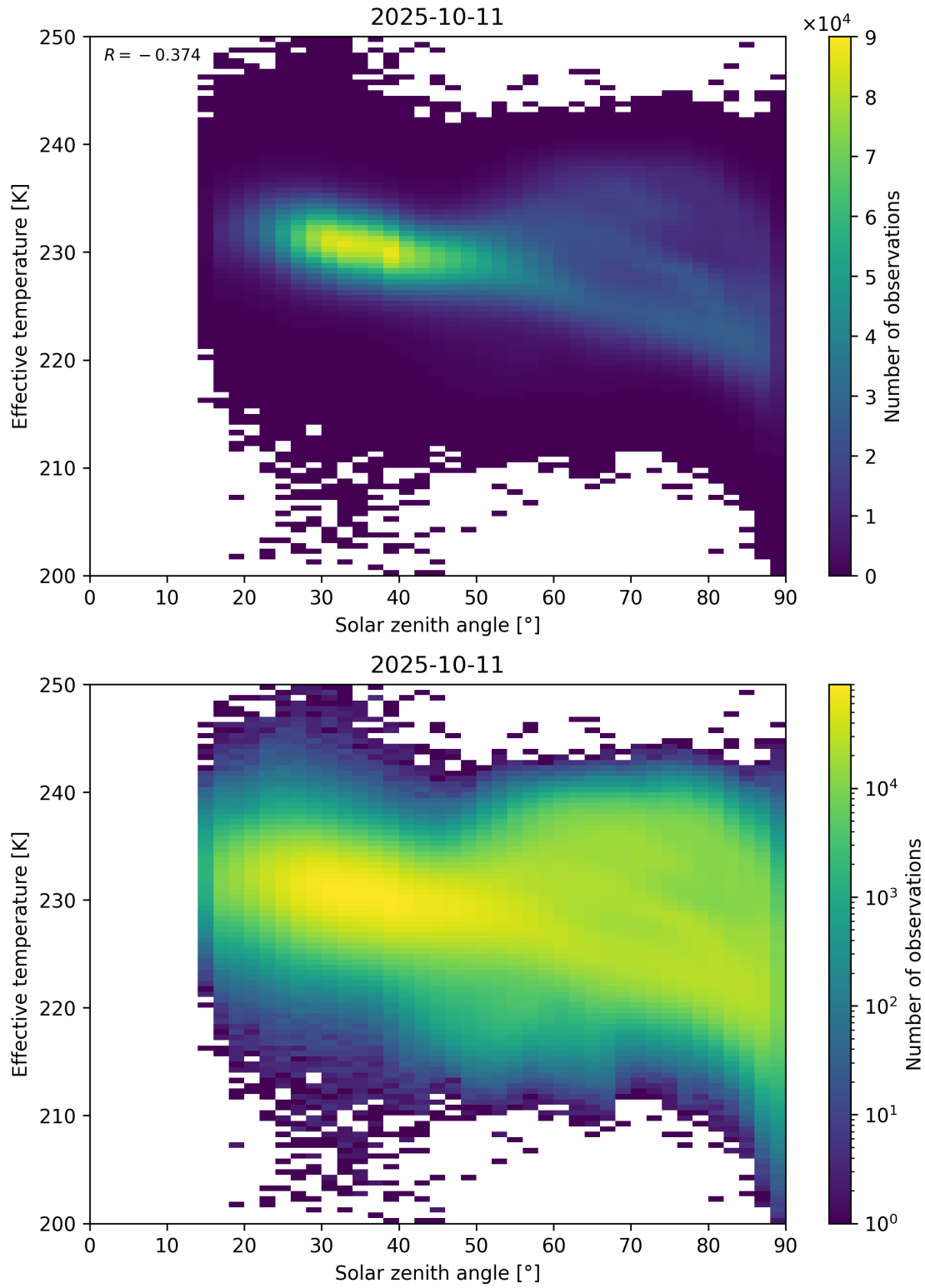
Figure 45: Scatter density plot of “Solar zenith angle” against “Effective temperature” for 2025-10-11 to 2025-10-12.
