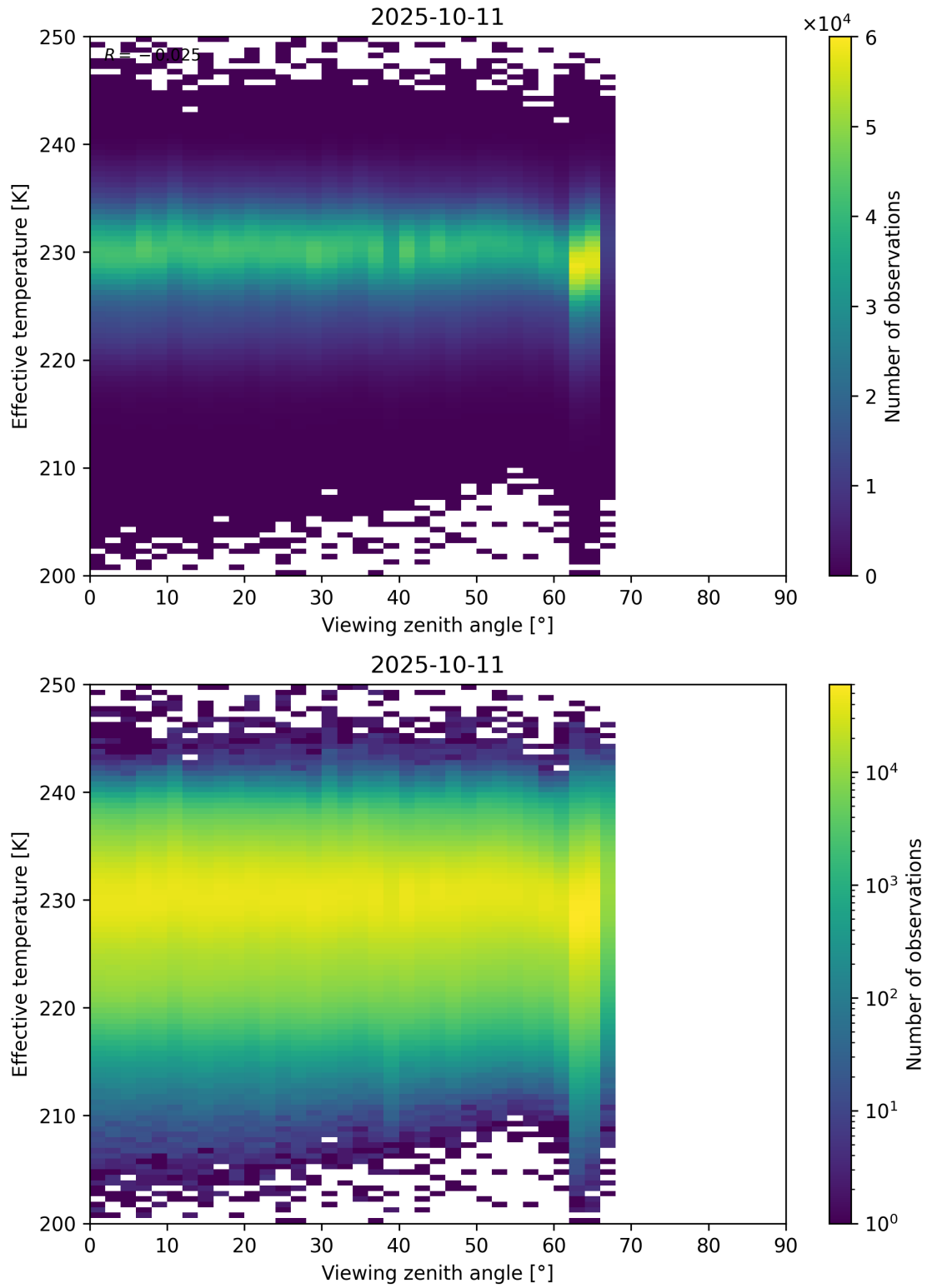
Figure 50: Scatter density plot of “Viewing zenith angle” against “Effective temperature” for 2025-10-11 to 2025-10-12.
