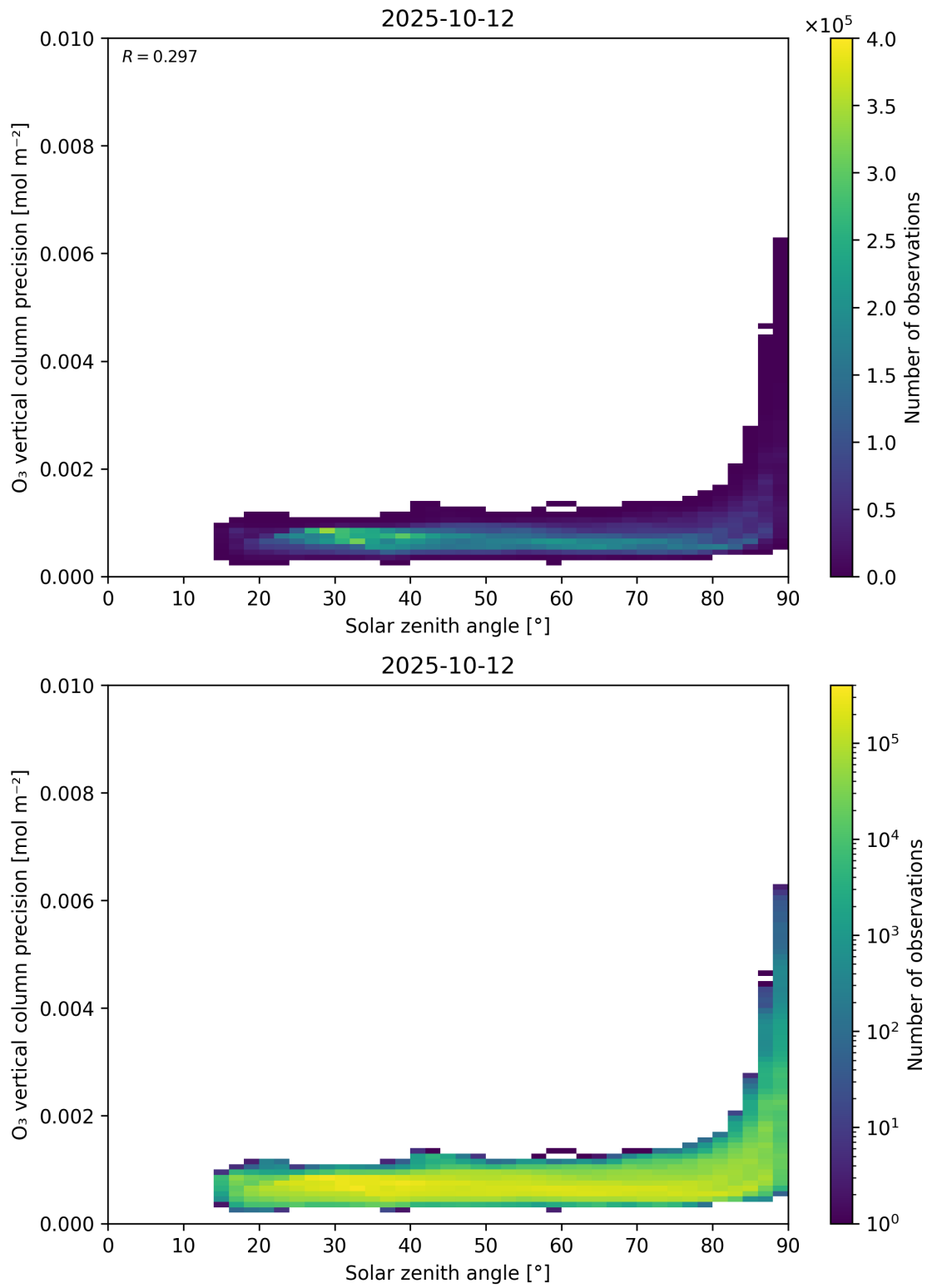
Figure 48: Scatter density plot of “Solar zenith angle” against “O 3 vertical column precision” for 2025-10-11 to 2025-10-13.
