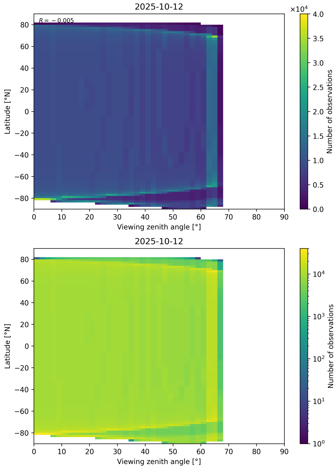
Figure 49: Scatter density plot of “Viewing zenith angle” against “Latitude” for 2025-10-11 to 2025-10-13.
