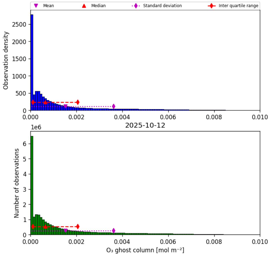
Figure 25: Histogram of “O 3 ghost column” for 2025-10-11 to 2025-10-13
