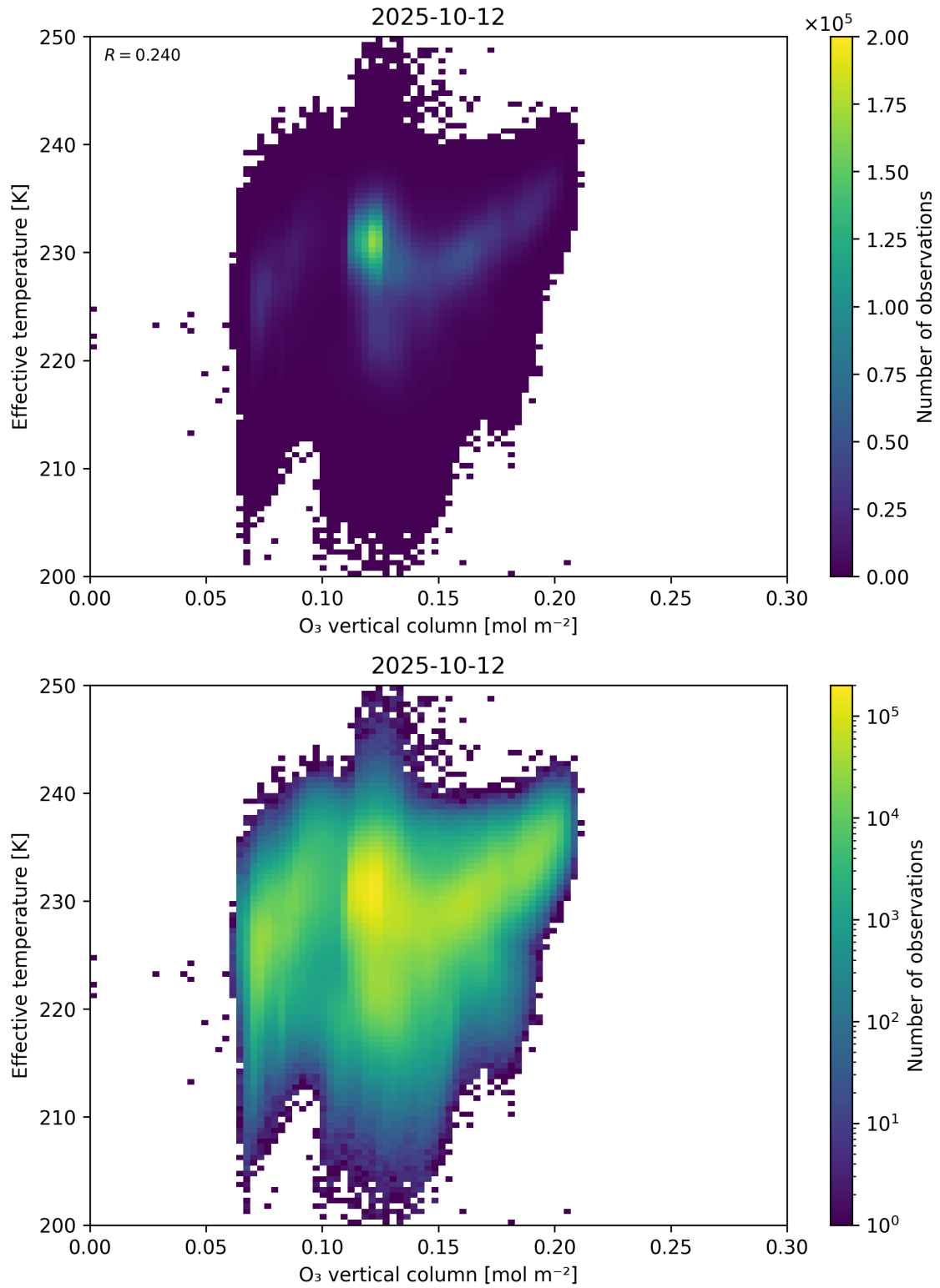
Figure 39: Scatter density plot of “O 3 vertical column” against “Effective temperature” for 2025-10-11 to 2025-10-13.
