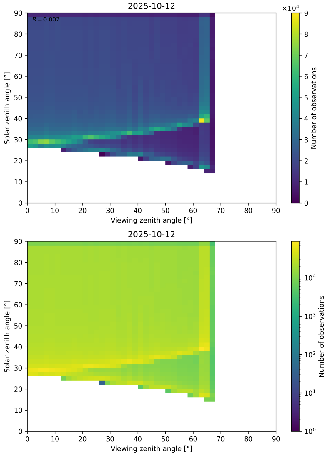
Figure 54: Scatter density plot of “Viewing zenith angle” against “Solar zenith angle” for 2025-10-11 to 2025-10-13.
