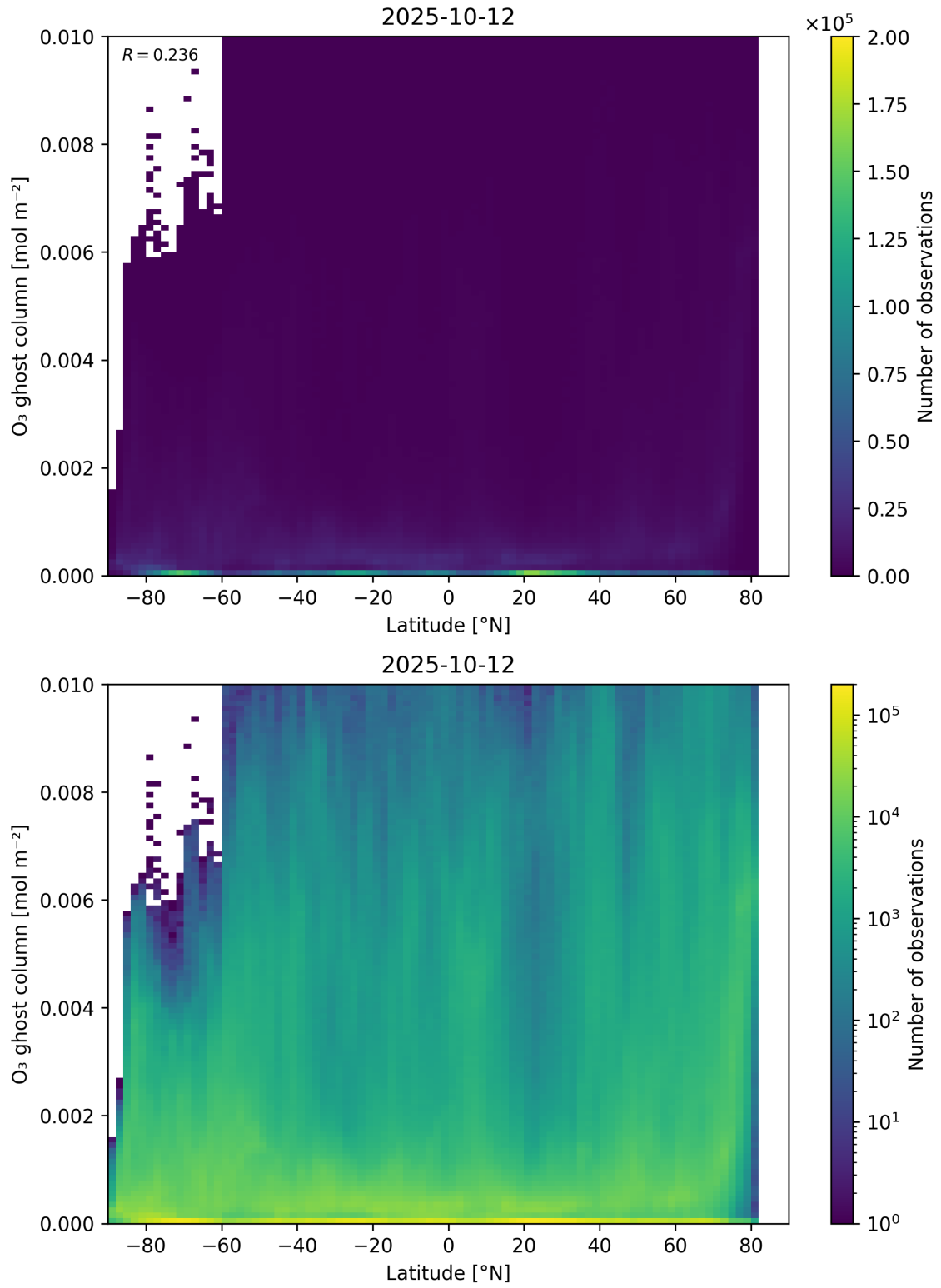
Figure 35: Scatter density plot of “Latitude” against “O 3 ghost column” for 2025-10-11 to 2025-10-13.
