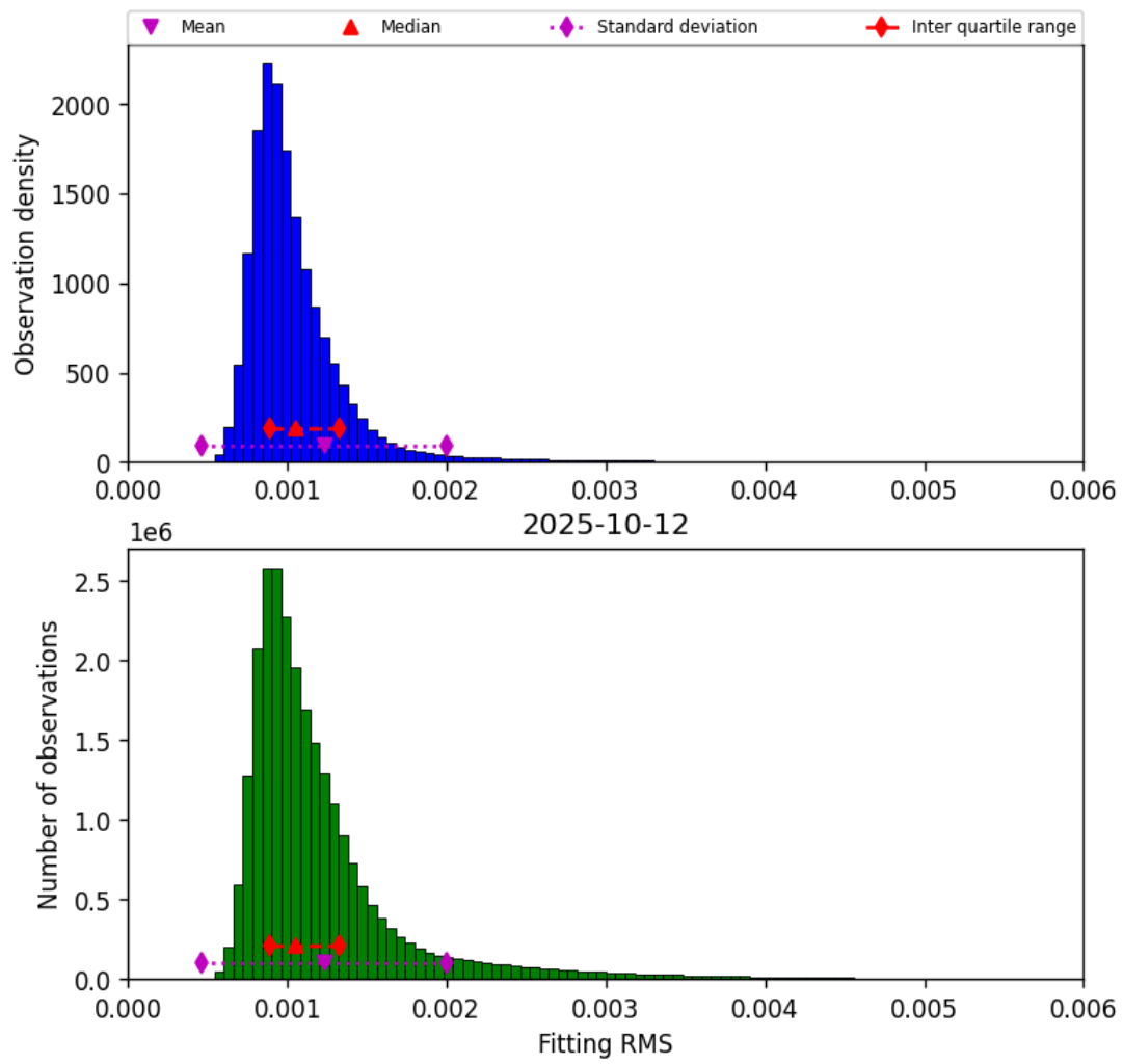
Figure 23: Histogram of “Fitting RMS” for 2025-10-11 to 2025-10-13
