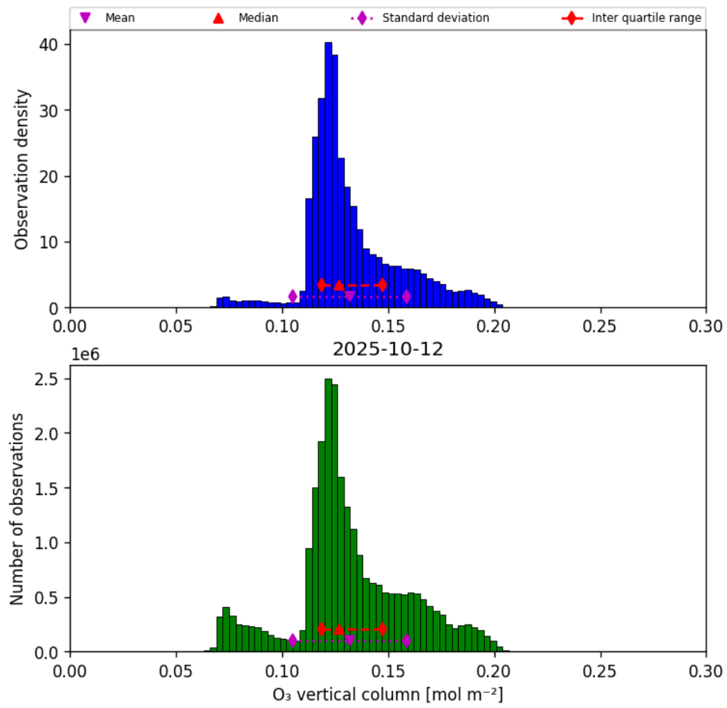
Figure 21: Histogram of “O 3 vertical column” for 2025-10-11 to 2025-10-13
