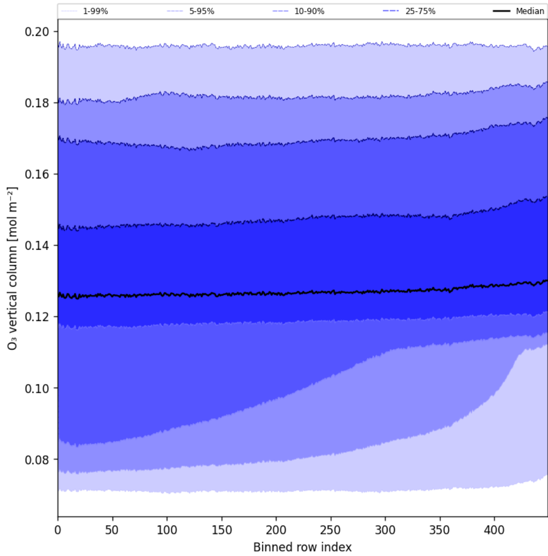
Figure 28: Along track statistics of “O 3 vertical column” for 2025-10-11 to 2025-10-13
