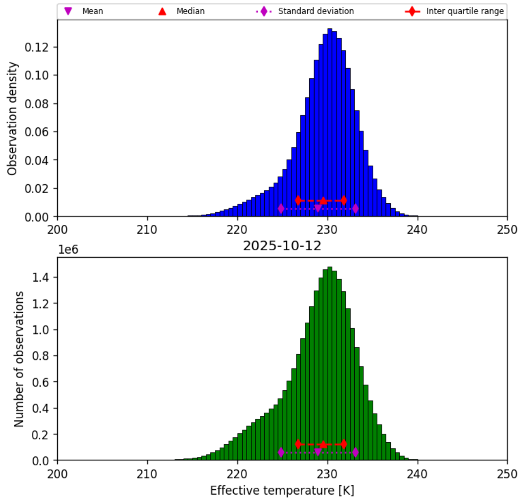
Figure 24: Histogram of “Effective temperature” for 2025-10-11 to 2025-10-13
