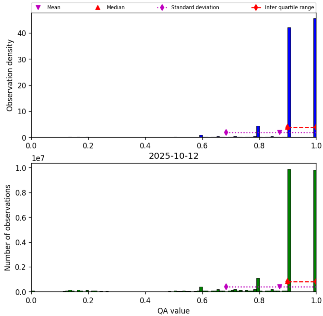
Figure 20: Histogram of “QA value” for 2025-10-11 to 2025-10-13
