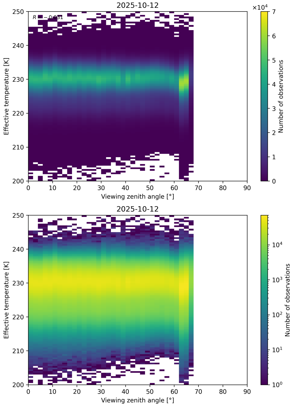
Figure 50: Scatter density plot of “Viewing zenith angle” against “Effective temperature” for 2025-10-11 to 2025-10-13.
