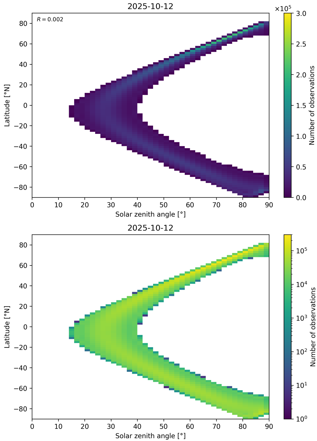
Figure 44: Scatter density plot of “Solar zenith angle” against “Latitude” for 2025-10-11 to 2025-10-13.
