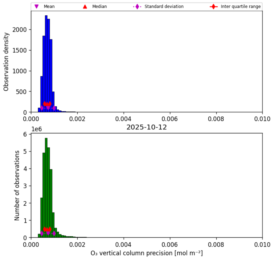
Figure 22: Histogram of “O 3 vertical column precision” for 2025-10-11 to 2025-10-13
