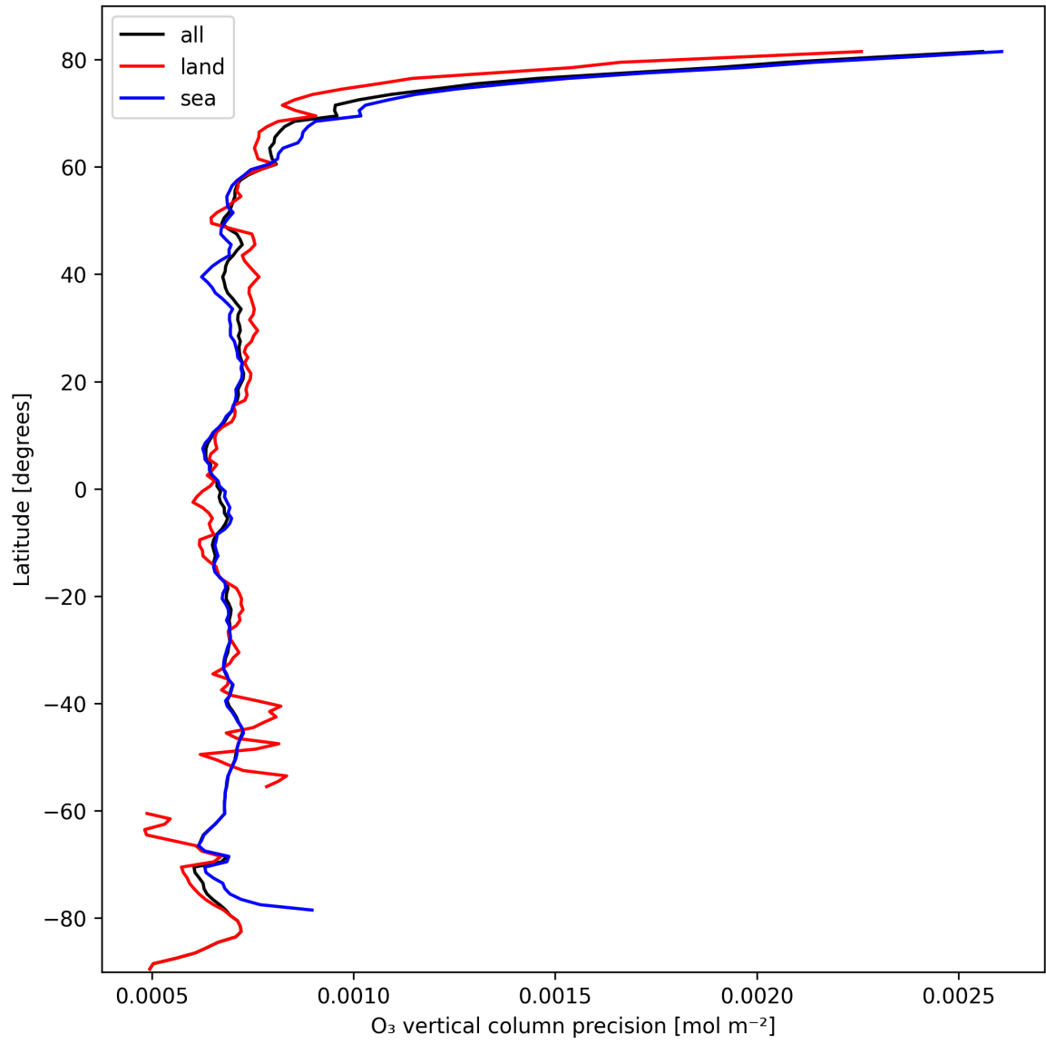
Figure 15: Zonal average of “O 3 vertical column precision” for 2025-10-11 to 2025-10-13.
