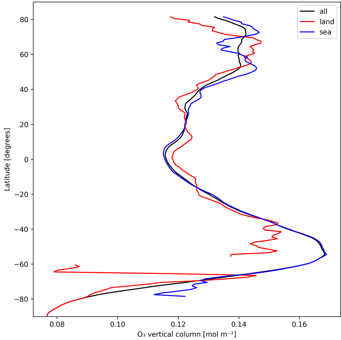
Figure 14: Zonal average of “O 3 vertical column” for 2025-10-11 to 2025-10-13.
