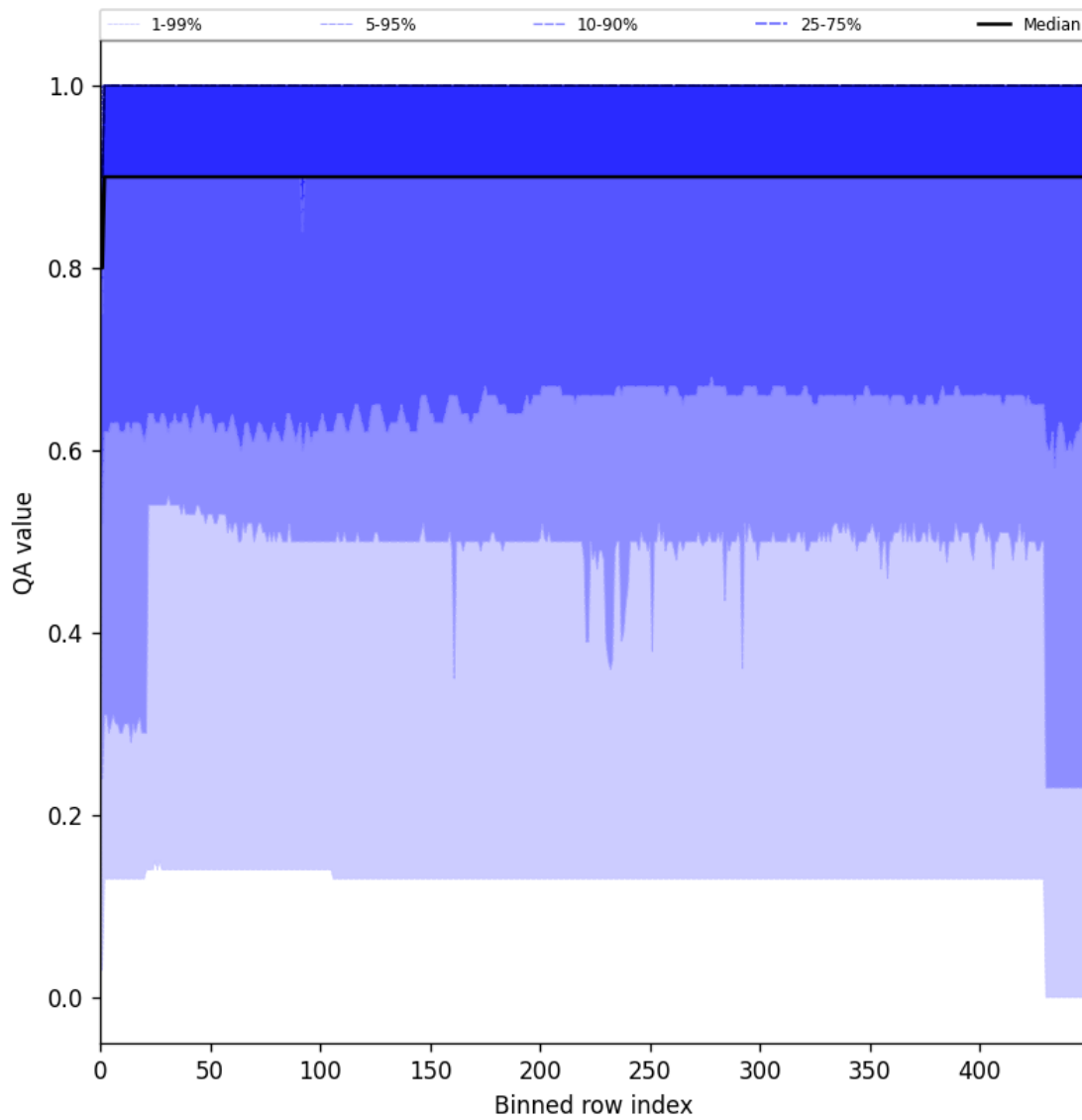
Figure 27: Along track statistics of “QA value” for 2025-10-11 to 2025-10-13
