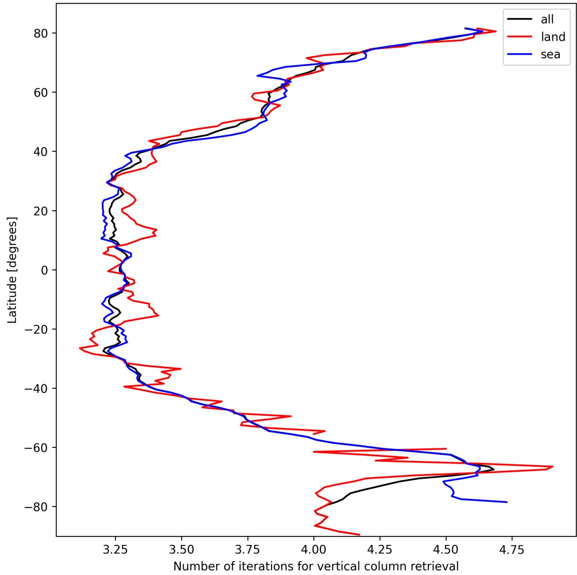
Figure 19: Zonal average of “Number of iterations for vertical column retrieval” for 2025-10-11 to 2025-10-13.
