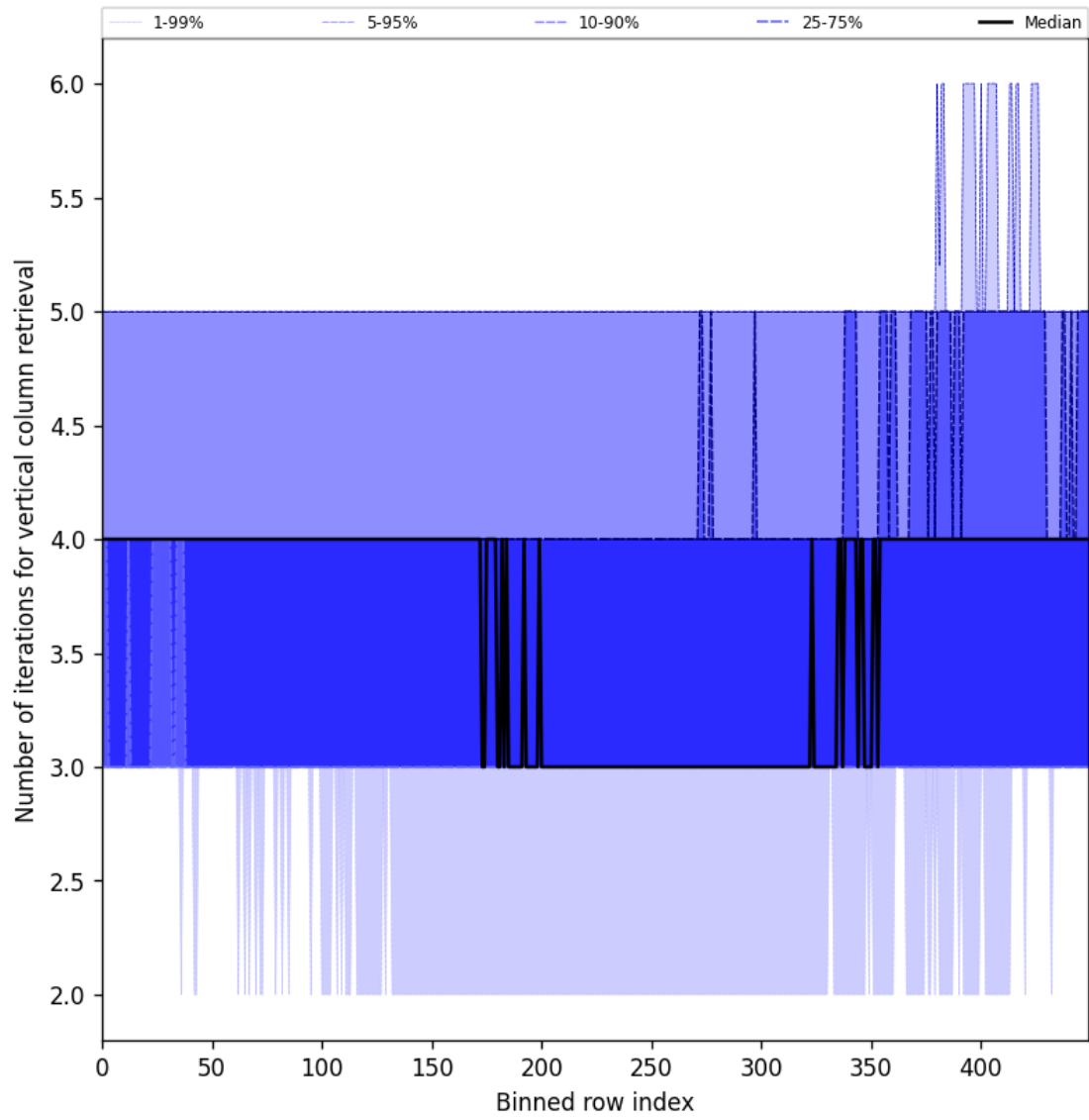
Figure 33: Along track statistics of “Number of iterations for vertical column retrieval” for 2025-10-11 to 2025-10-13
