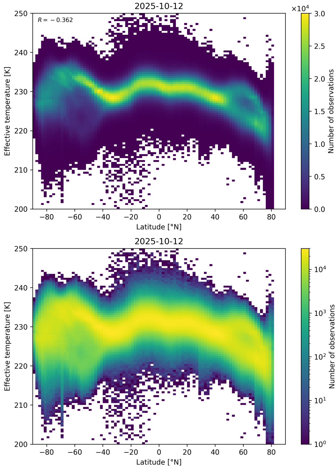
Figure 34: Scatter density plot of “Latitude” against “Effective temperature” for 2025-10-11 to 2025-10-13.
