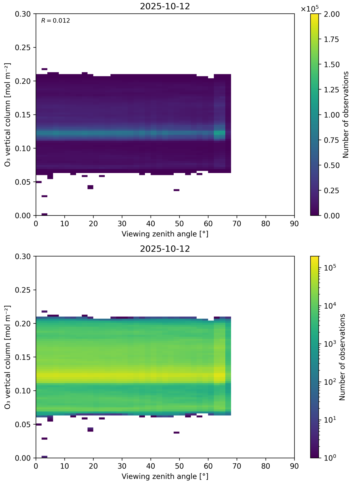
Figure 52: Scatter density plot of “Viewing zenith angle” against “O 3 vertical column” for 2025-10-11 to 2025-10-13.
