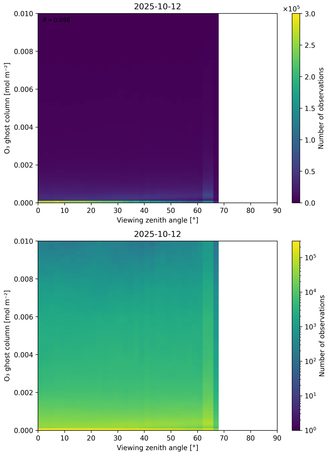
Figure 51: Scatter density plot of “Viewing zenith angle” against “O 3 ghost column” for 2025-10-11 to 2025-10-13.
