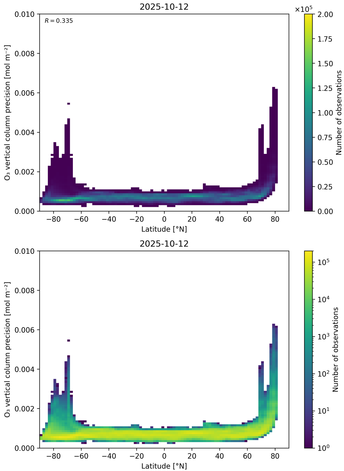
Figure 37: Scatter density plot of “Latitude” against “O 3 vertical column precision” for 2025-10-11 to 2025-10-13.
