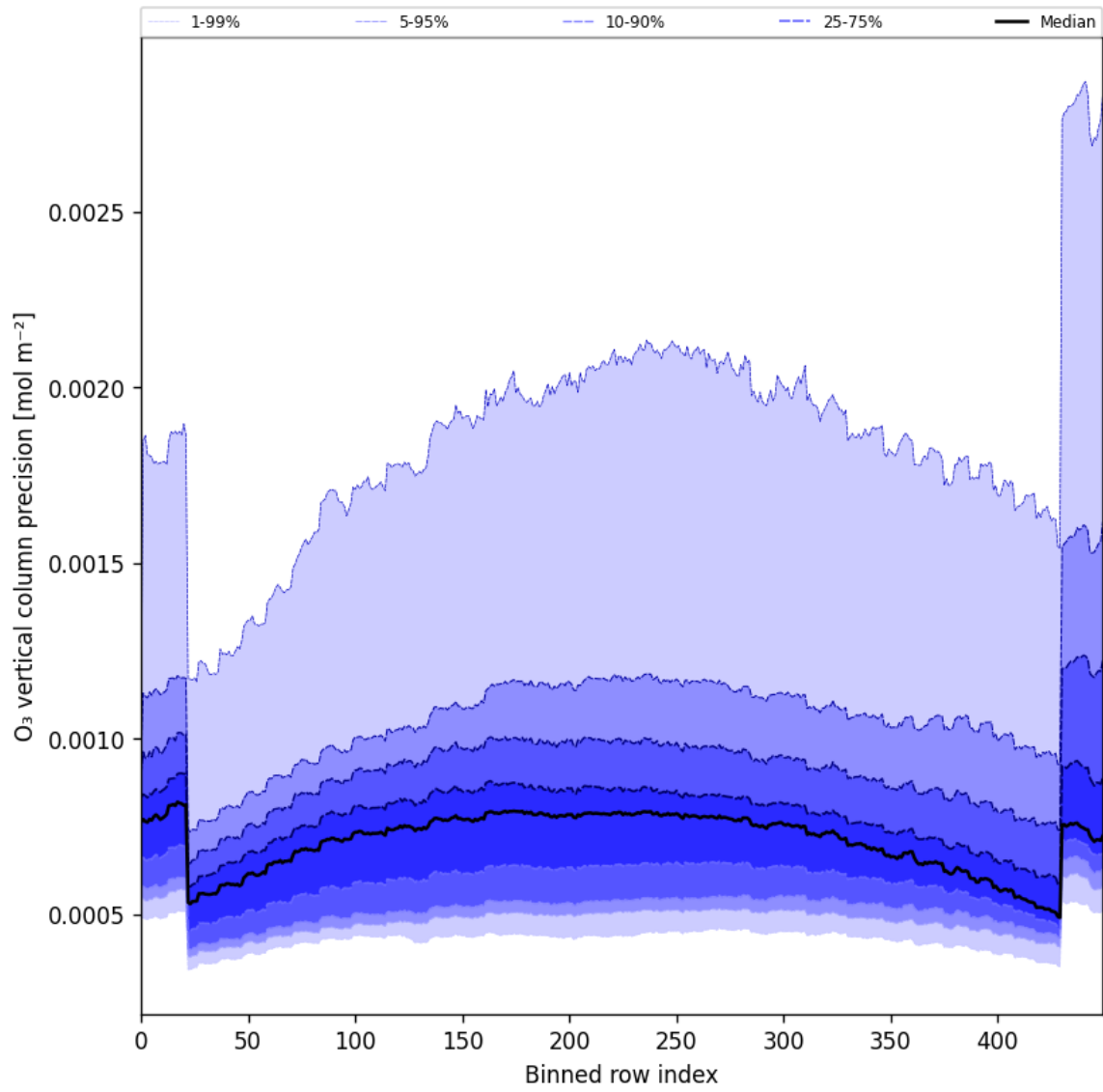
Figure 29: Along track statistics of “O 3 vertical column precision” for 2025-10-11 to 2025-10-13
