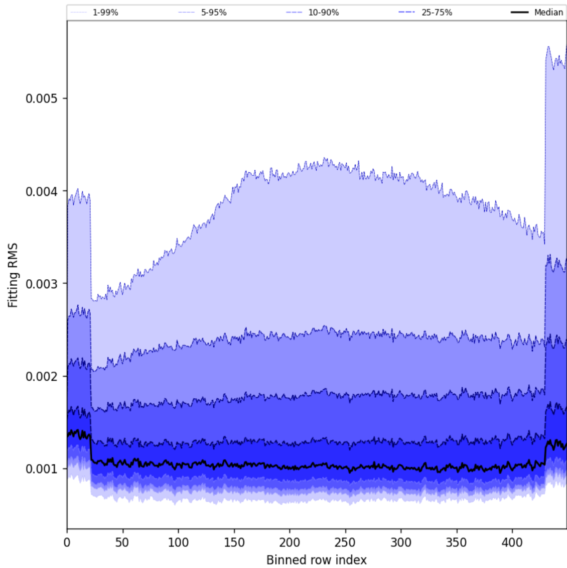
Figure 30: Along track statistics of “Fitting RMS” for 2025-10-11 to 2025-10-13
