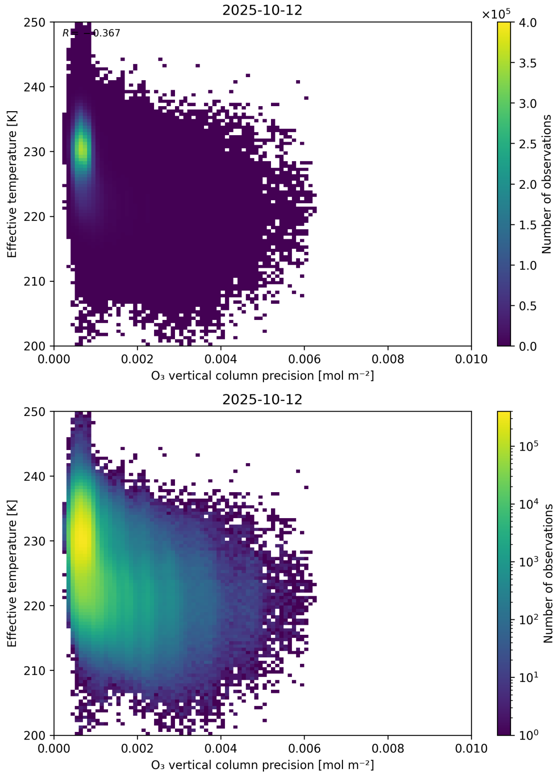
Figure 42: Scatter density plot of “O 3 vertical column precision” against “Effective temperature” for 2025-10-11 to 2025-10-13.
