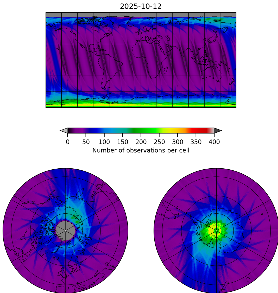
Figure 12: Map of the number of observations for 2025-10-11 to 2025-10-13
