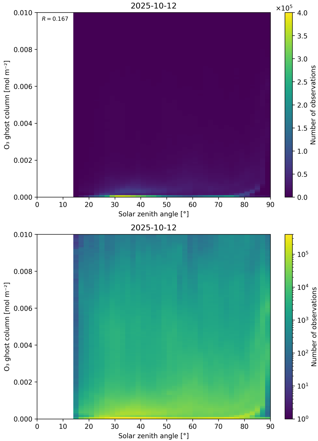
Figure 46: Scatter density plot of “Solar zenith angle” against “O 3 ghost column” for 2025-10-11 to 2025-10-13.
