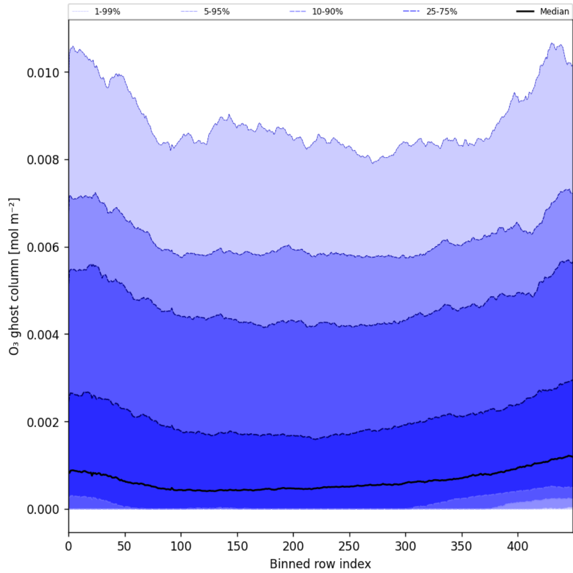
Figure 32: Along track statistics of “O 3 ghost column” for 2025-10-11 to 2025-10-13
