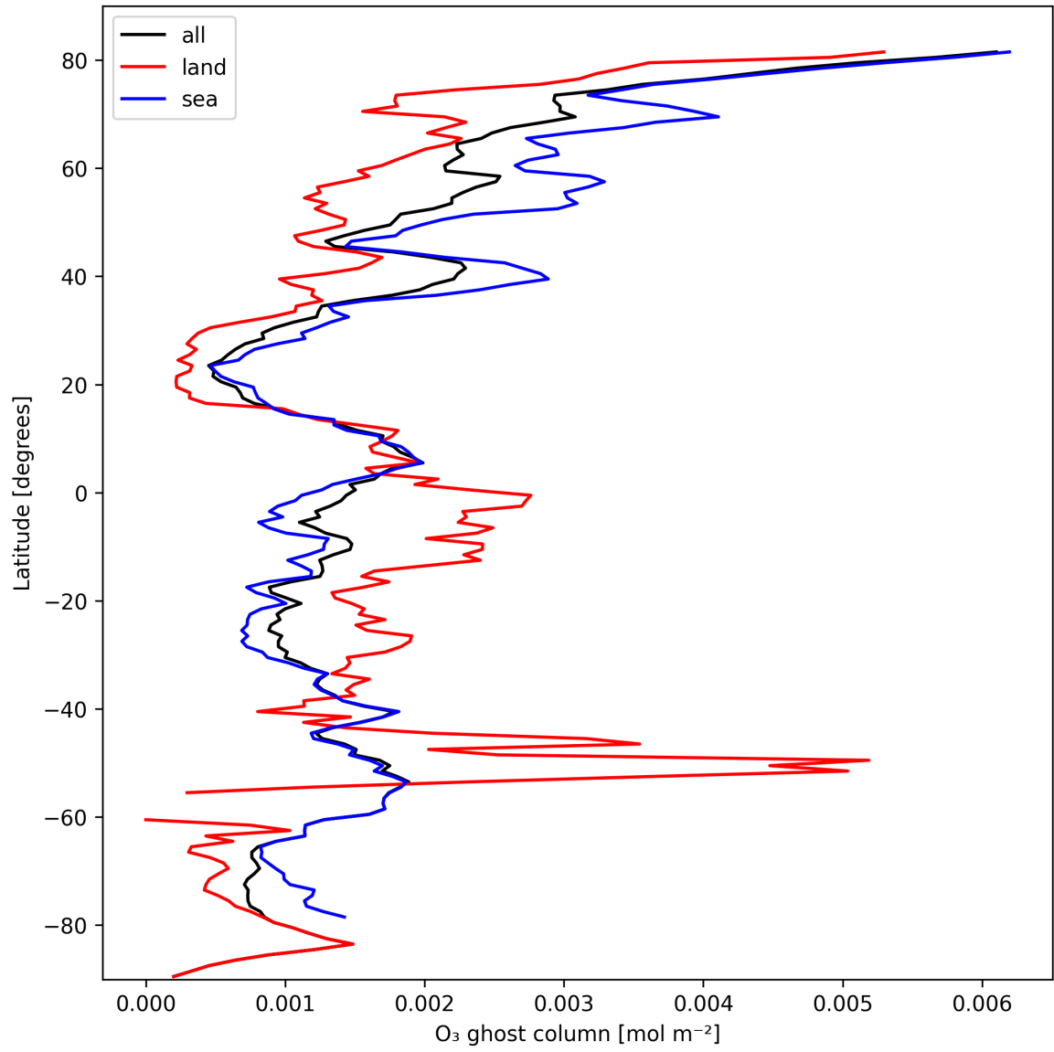
Figure 18: Zonal average of “O 3 ghost column” for 2025-10-11 to 2025-10-13.
