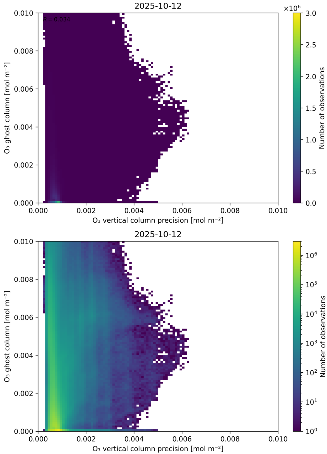
Figure 43: Scatter density plot of “O 3 vertical column precision” against “O 3 ghost column” for 2025-10-11 to 2025-10-13.
