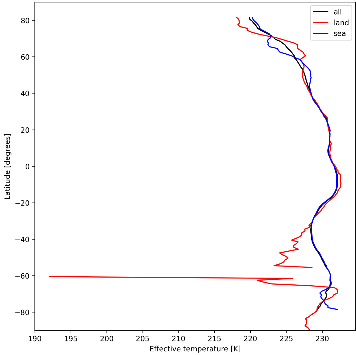
Figure 17: Zonal average of "Effective temperature" for 2025-10-11 to 2025-10-13.
