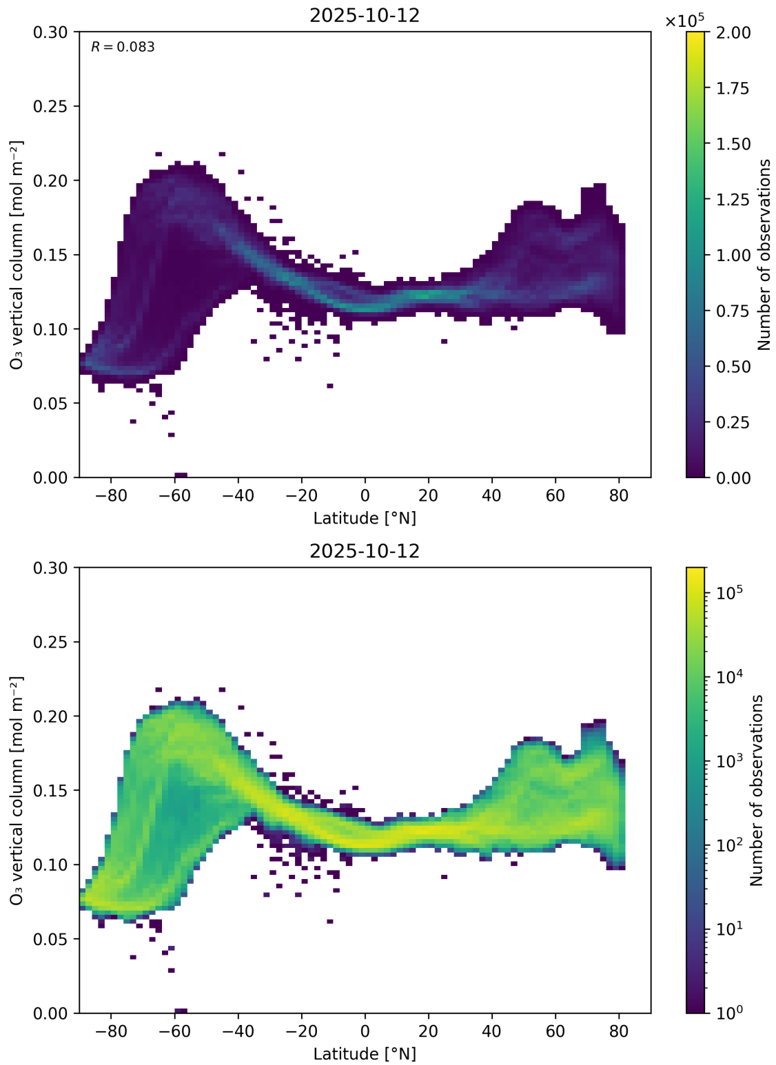
Figure 36: Scatter density plot of “Latitude” against “O 3 vertical column” for 2025-10-11 to 2025-10-13.
