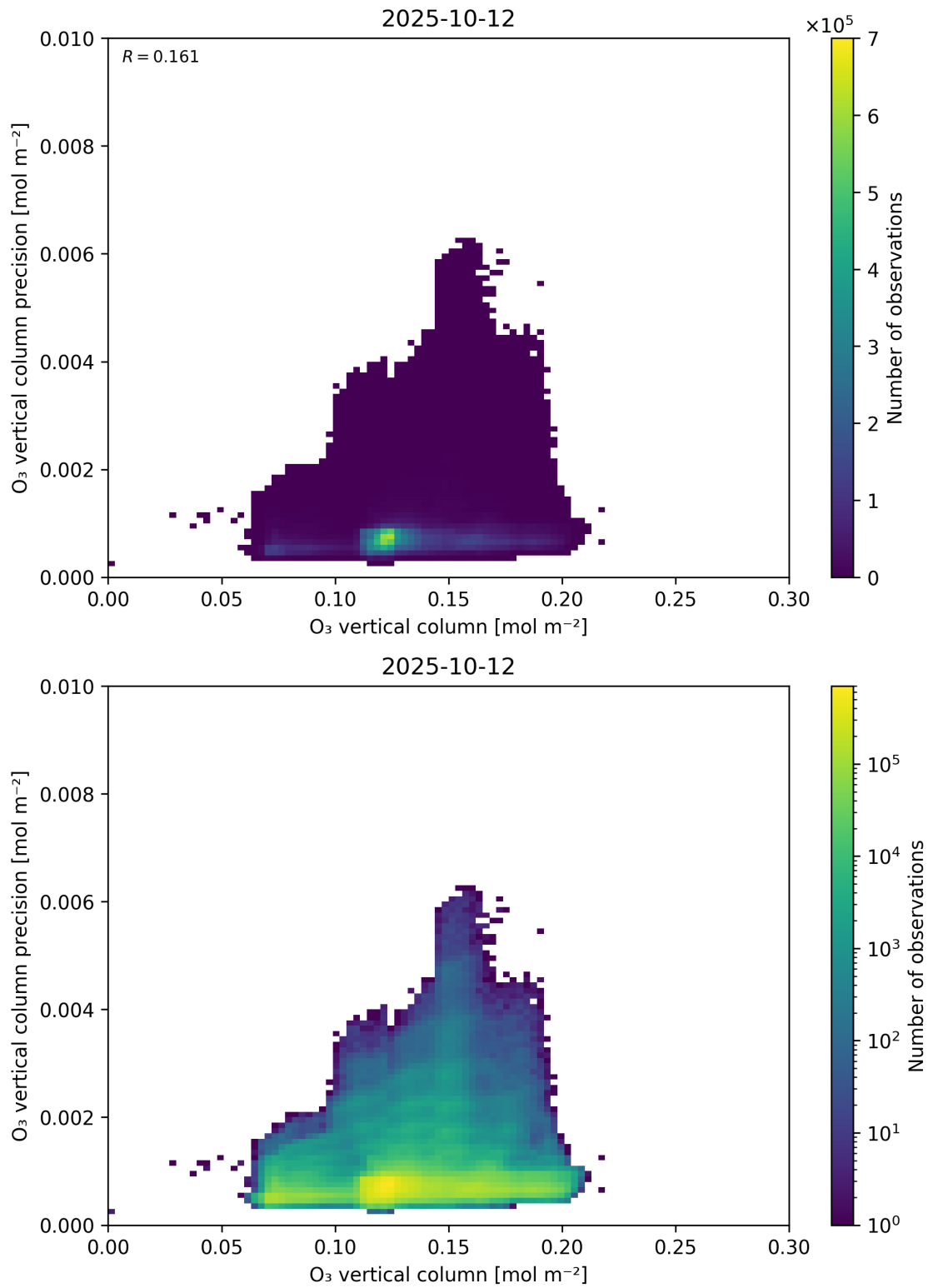
Figure 41: Scatter density plot of “O 3 vertical column” against “O 3 vertical column precision” for 2025-10-11 to 2025-10-13.
