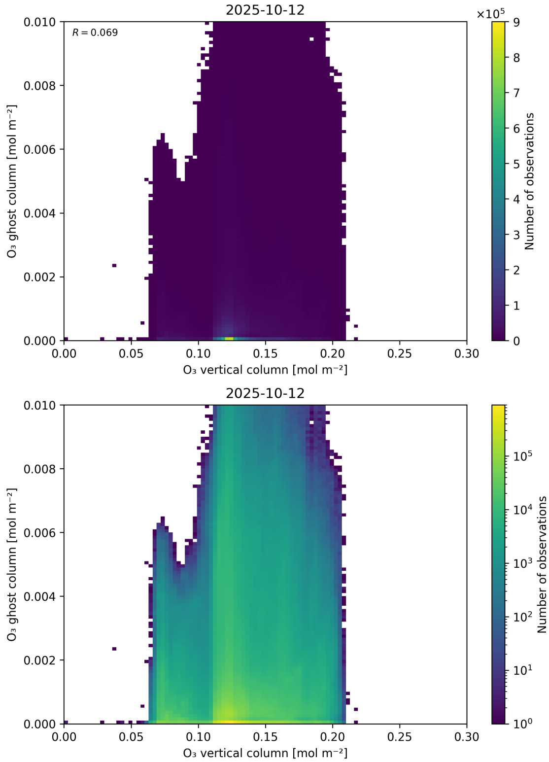
Figure 40: Scatter density plot of “O 3 vertical column” against “O 3 ghost column” for 2025-10-11 to 2025-10-13.
