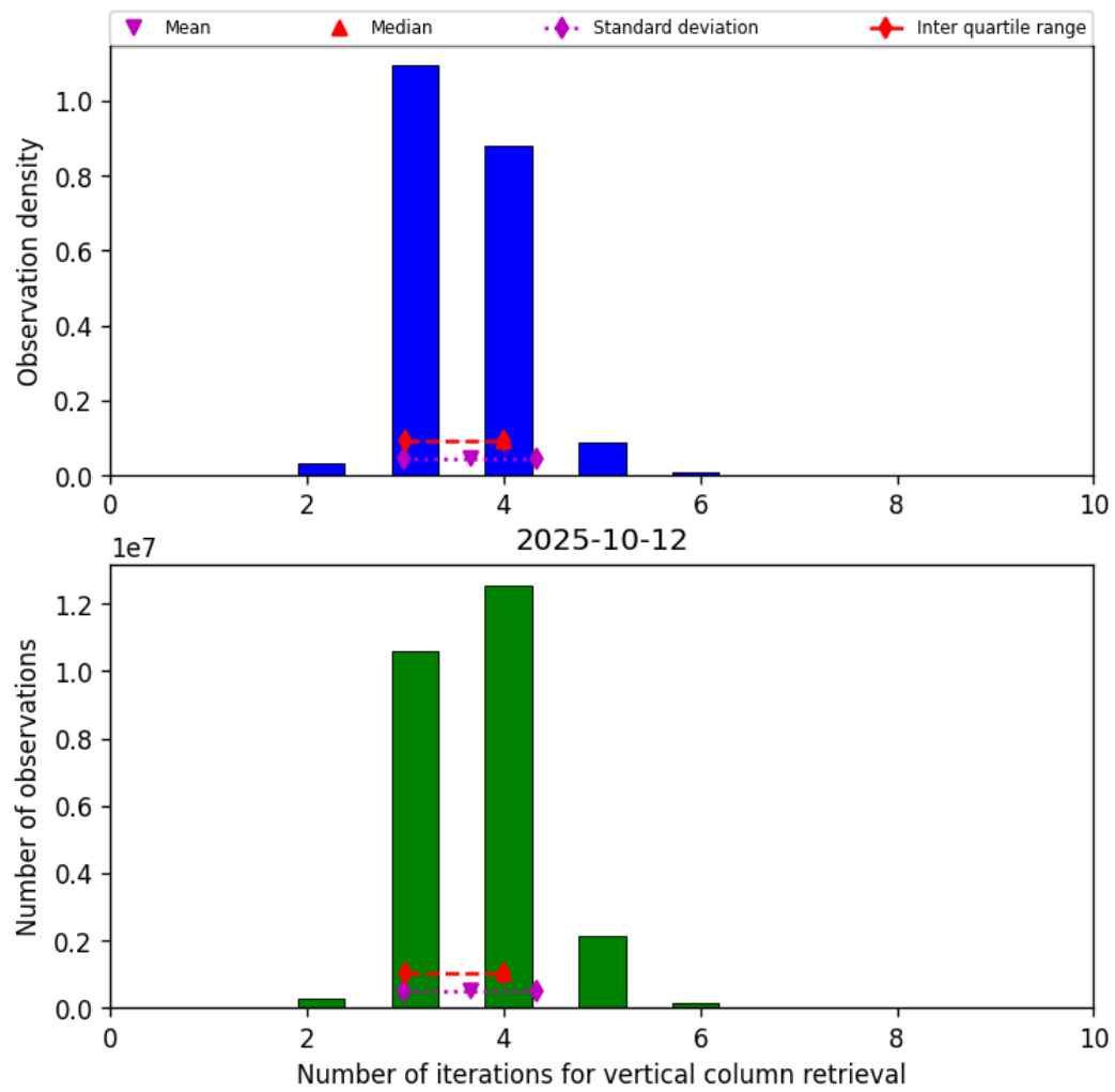
Figure 26: Histogram of “Number of iterations for vertical column retrieval” for 2025-10-11 to 2025-10-13
