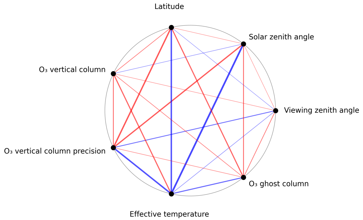
Figure 1: Map of correlation graph for 2025-10-11 to 2025-10-13.
