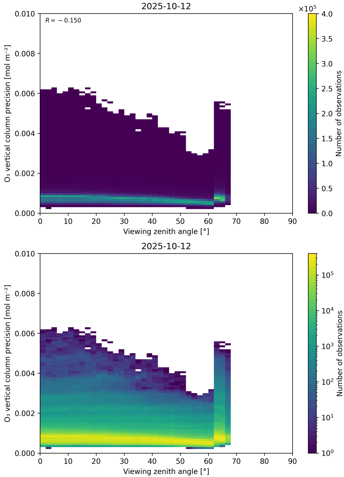
Figure 53: Scatter density plot of “Viewing zenith angle” against “O 3 vertical column precision” for 2025-10-11 to 2025-10-13.
