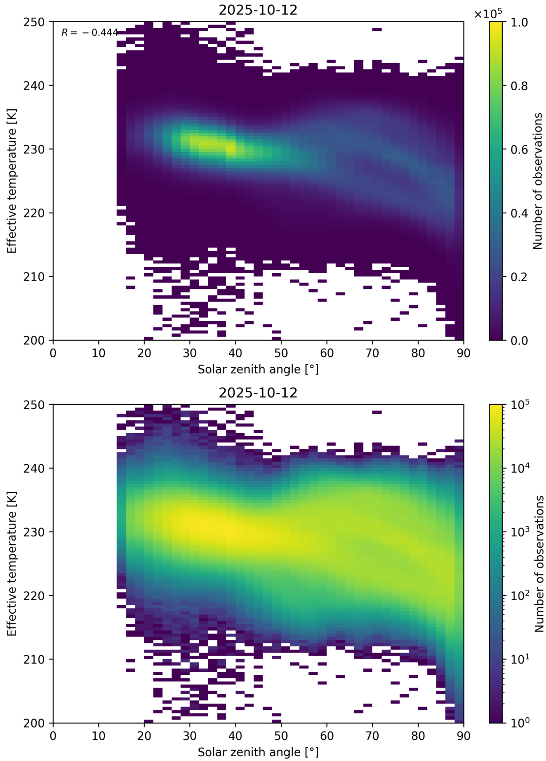
Figure 45: Scatter density plot of “Solar zenith angle” against “Effective temperature” for 2025-10-11 to 2025-10-13.
