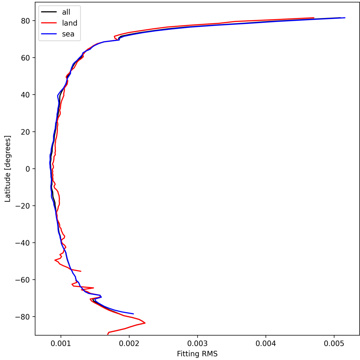
Figure 16: Zonal average of “Fitting RMS” for 2025-10-11 to 2025-10-13.
