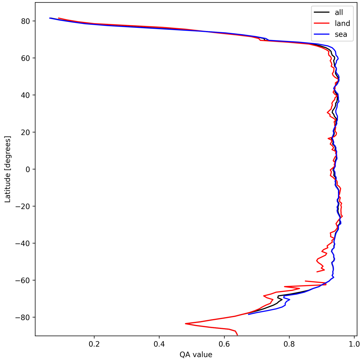
Figure 13: Zonal average of “QA value” for 2025-10-11 to 2025-10-13.
