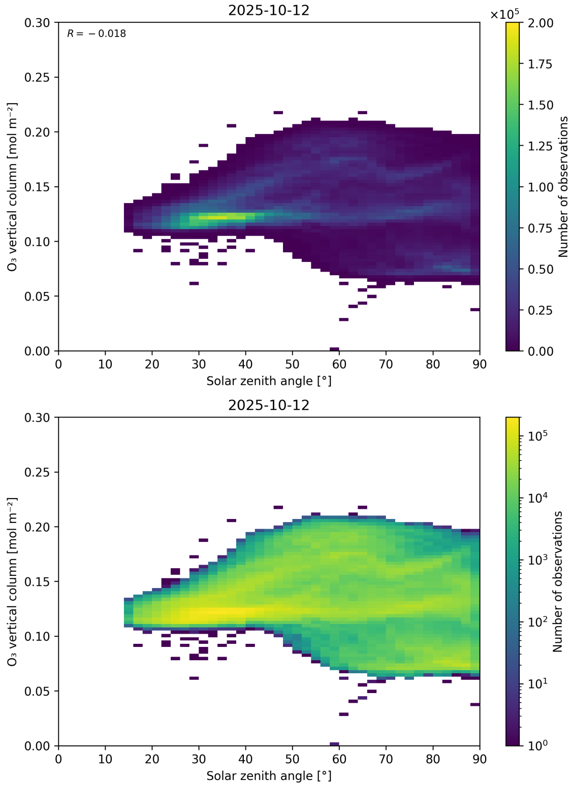
Figure 47: Scatter density plot of “Solar zenith angle” against “O 3 vertical column” for 2025-10-11 to 2025-10-13.
