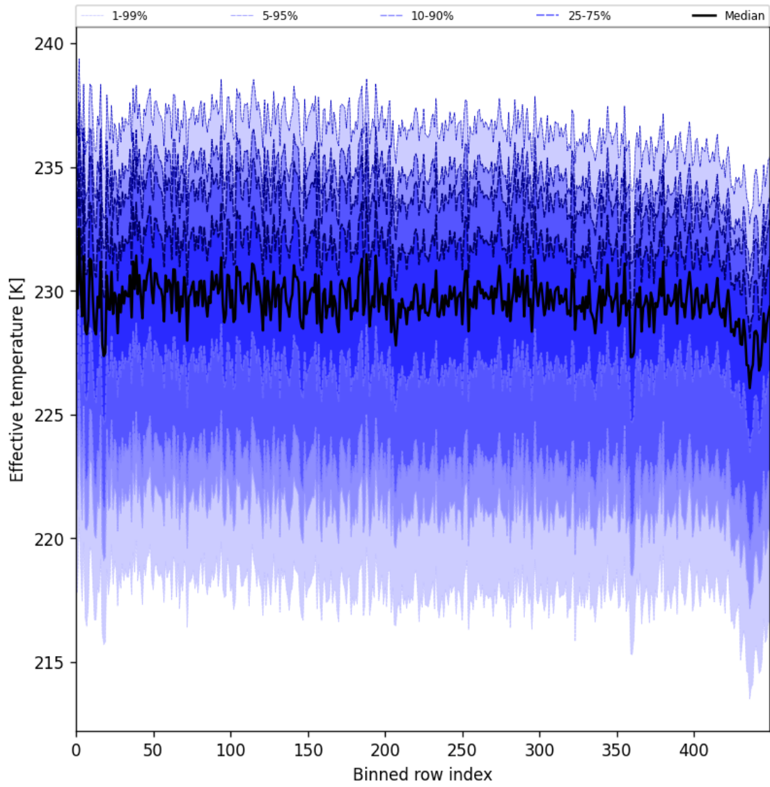
Figure 31: Along track statistics of “Effective temperature” for 2025-10-11 to 2025-10-13
