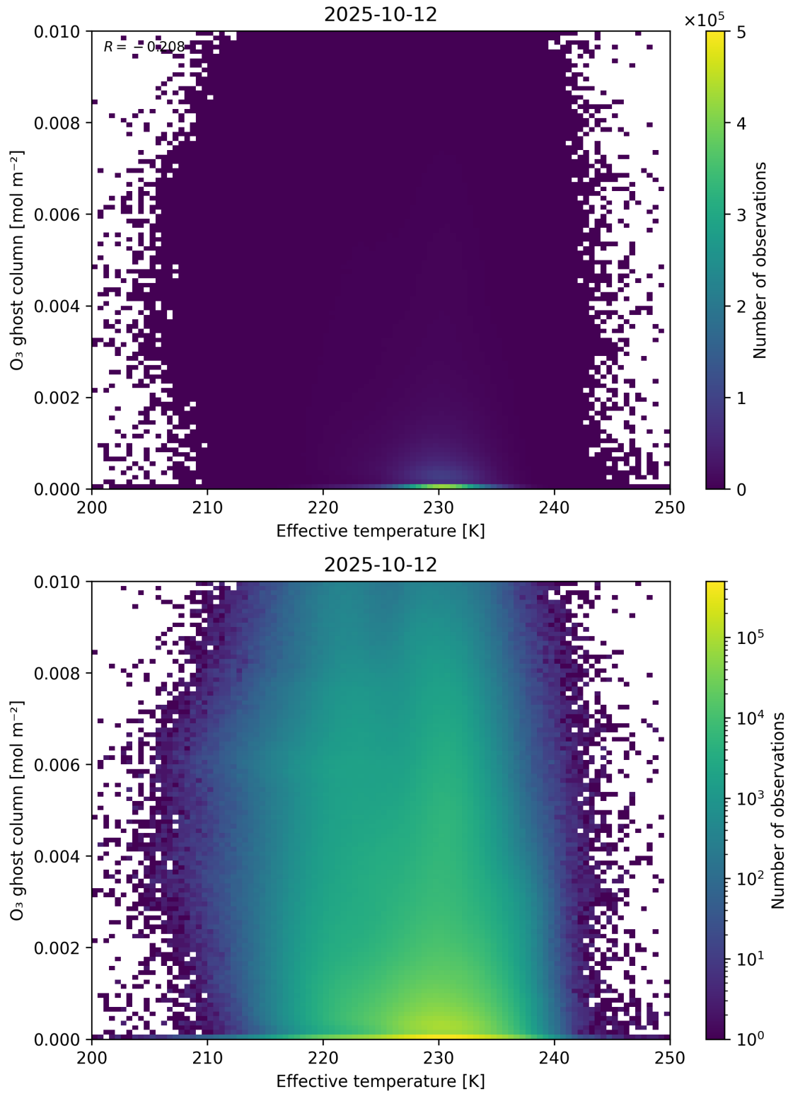
Figure 38: Scatter density plot of “Effective temperature” against “O 3 ghost column” for 2025-10-11 to 2025-10-13.
