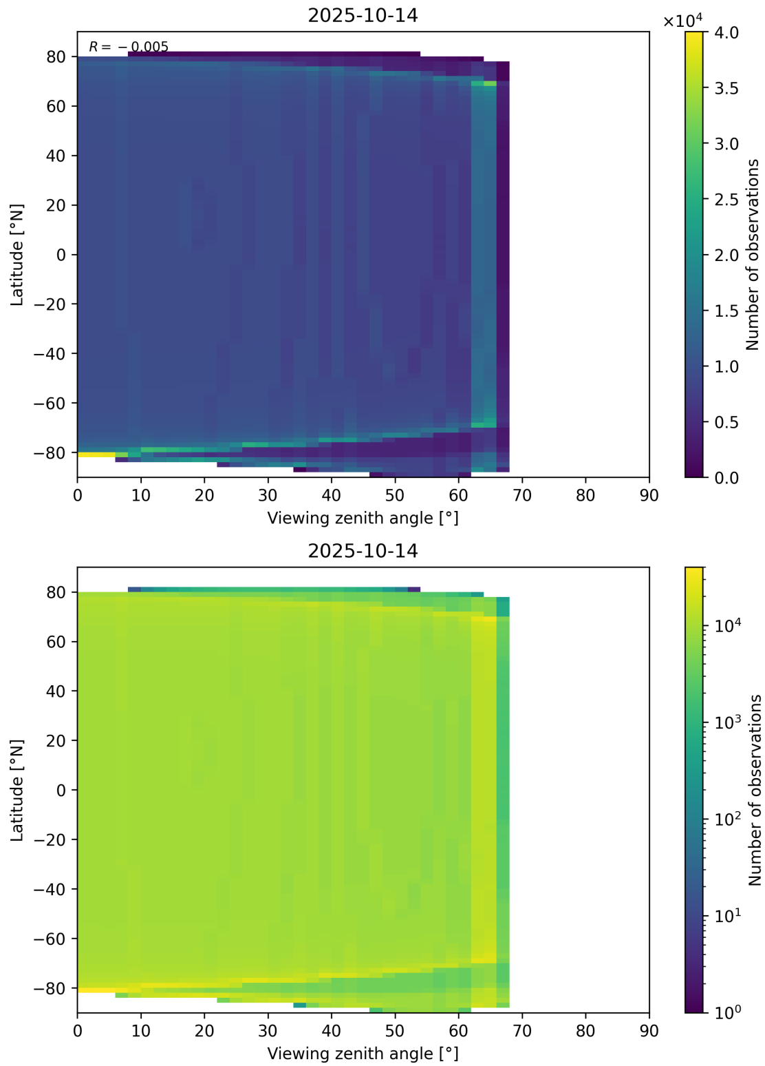
Figure 49: Scatter density plot of “Viewing zenith angle” against “Latitude” for 2025-10-13 to 2025-10-15.
