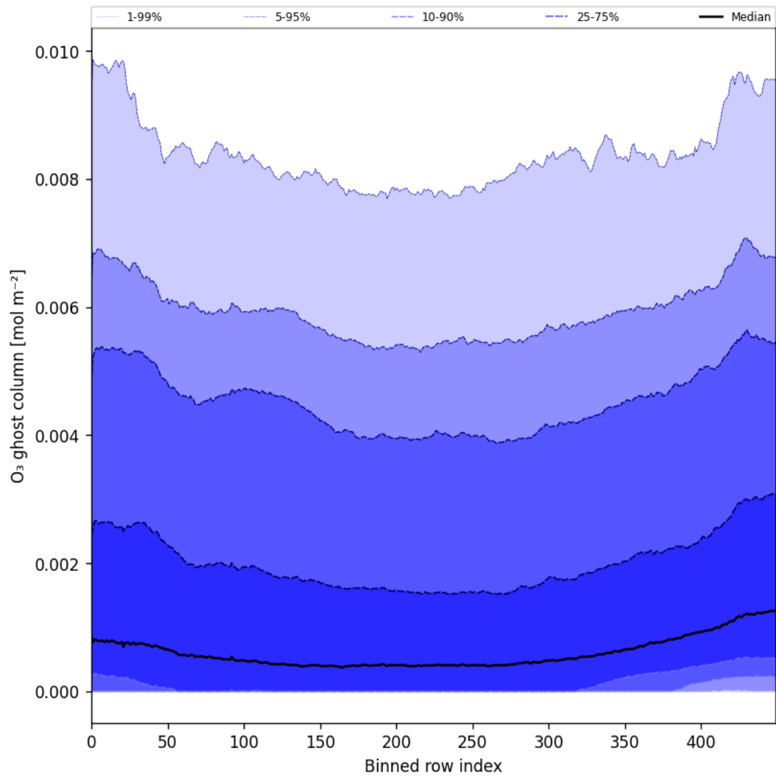
Figure 32: Along track statistics of “O 3 ghost column” for 2025-10-13 to 2025-10-15
