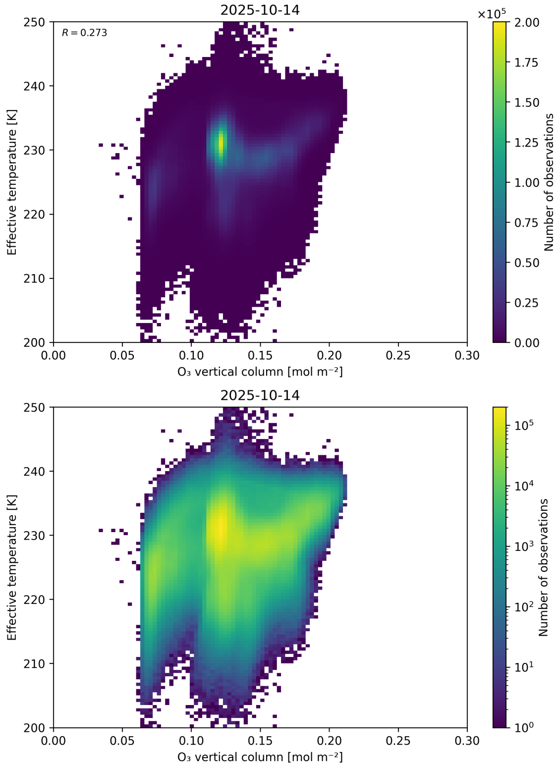
Figure 39: Scatter density plot of “O 3 vertical column” against “Effective temperature” for 2025-10-13 to 2025-10-15.
