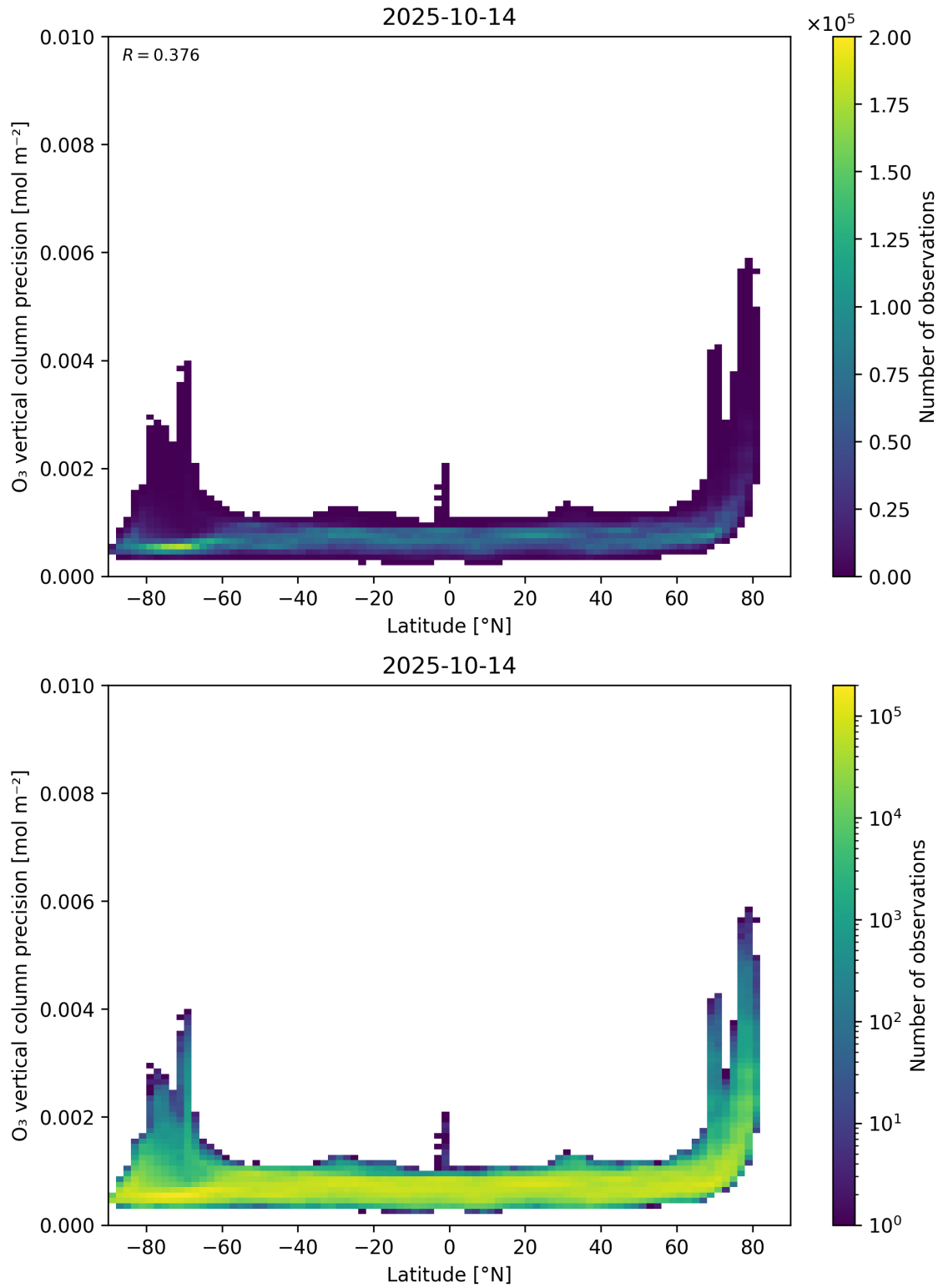
Figure 37: Scatter density plot of “Latitude” against “O 3 vertical column precision” for 2025-10-13 to 2025-10-15.
