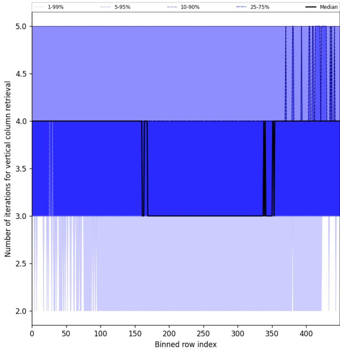
Figure 33: Along track statistics of “Number of iterations for vertical column retrieval” for 2025-10-13 to 2025-10-15
