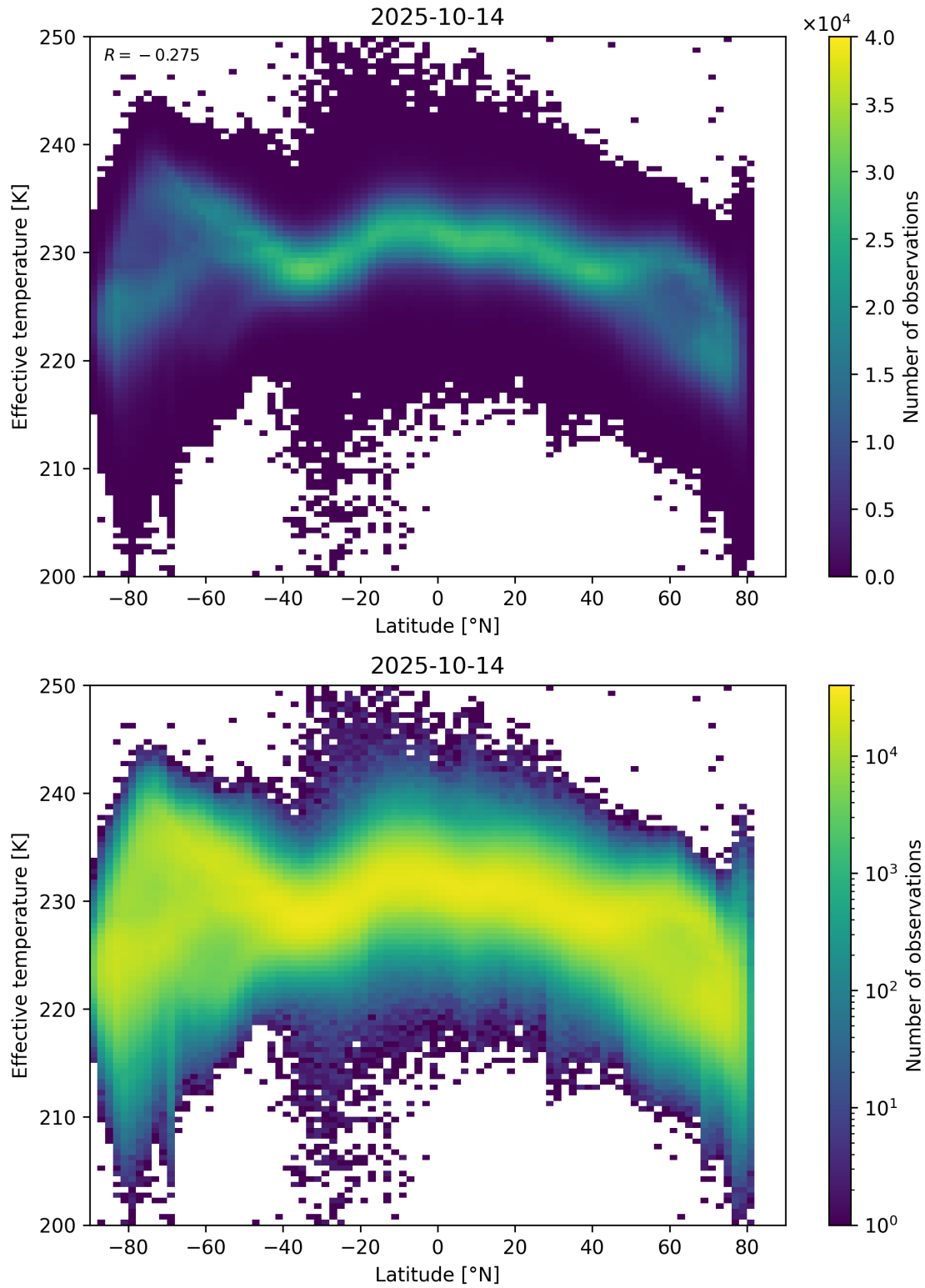
Figure 34: Scatter density plot of “Latitude” against “Effective temperature” for 2025-10-13 to 2025-10-15.
