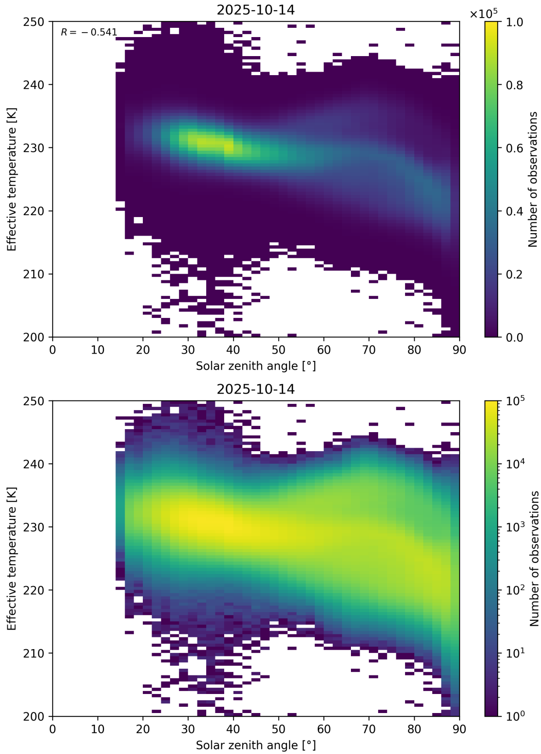
Figure 45: Scatter density plot of “Solar zenith angle” against “Effective temperature” for 2025-10-13 to 2025-10-15.
