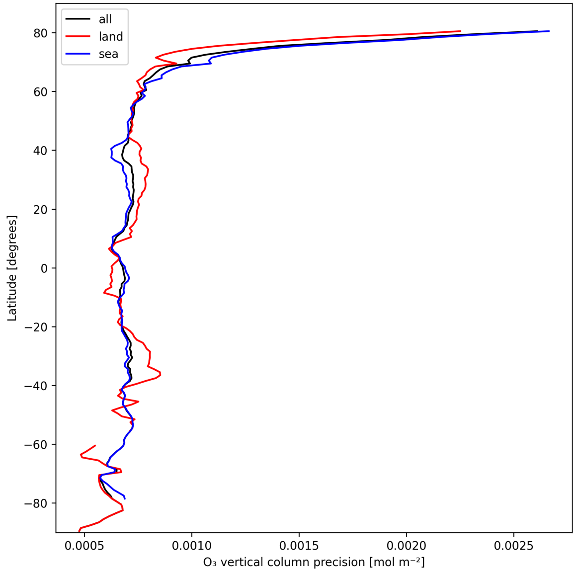
Figure 15: Zonal average of “O 3 vertical column precision” for 2025-10-13 to 2025-10-15.
