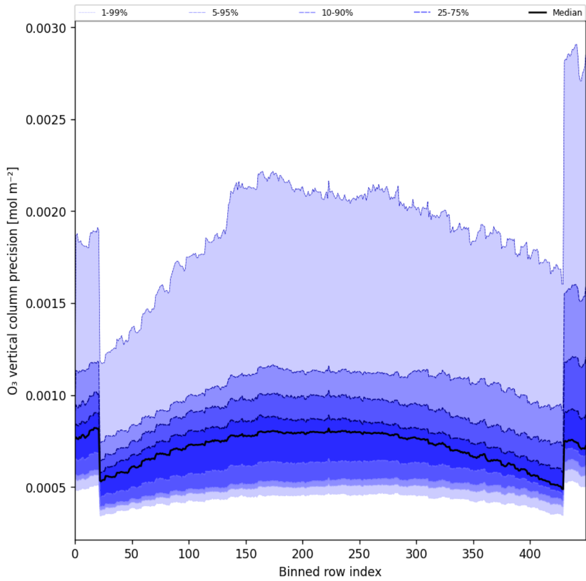
Figure 29: Along track statistics of “O 3 vertical column precision” for 2025-10-13 to 2025-10-15
