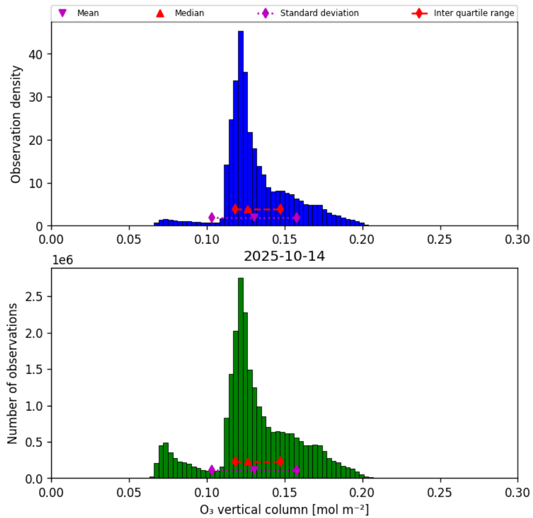
Figure 21: Histogram of “O 3 vertical column” for 2025-10-13 to 2025-10-15
