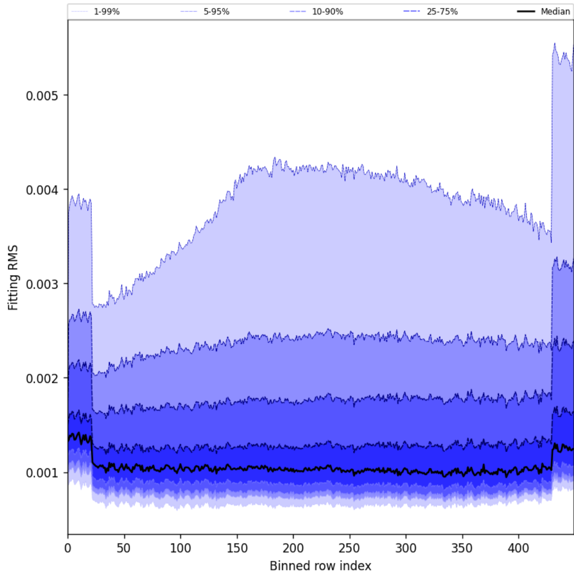
Figure 30: Along track statistics of “Fitting RMS” for 2025-10-13 to 2025-10-15
