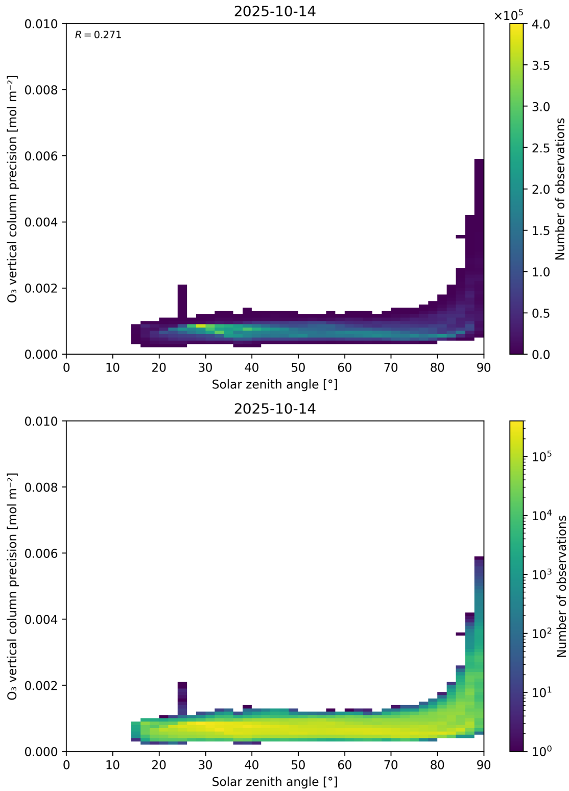
Figure 48: Scatter density plot of “Solar zenith angle” against “O 3 vertical column precision” for 2025-10-13 to 2025-10-15.
