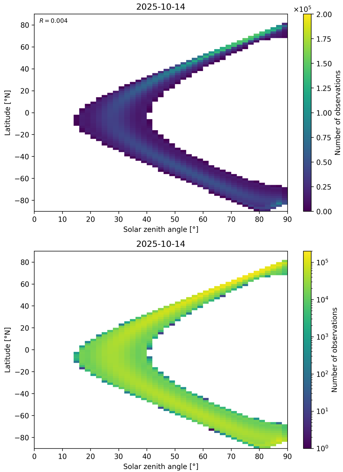
Figure 44: Scatter density plot of “Solar zenith angle” against “Latitude” for 2025-10-13 to 2025-10-15.
