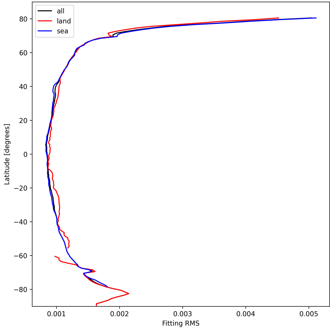
Figure 16: Zonal average of “Fitting RMS” for 2025-10-13 to 2025-10-15.
