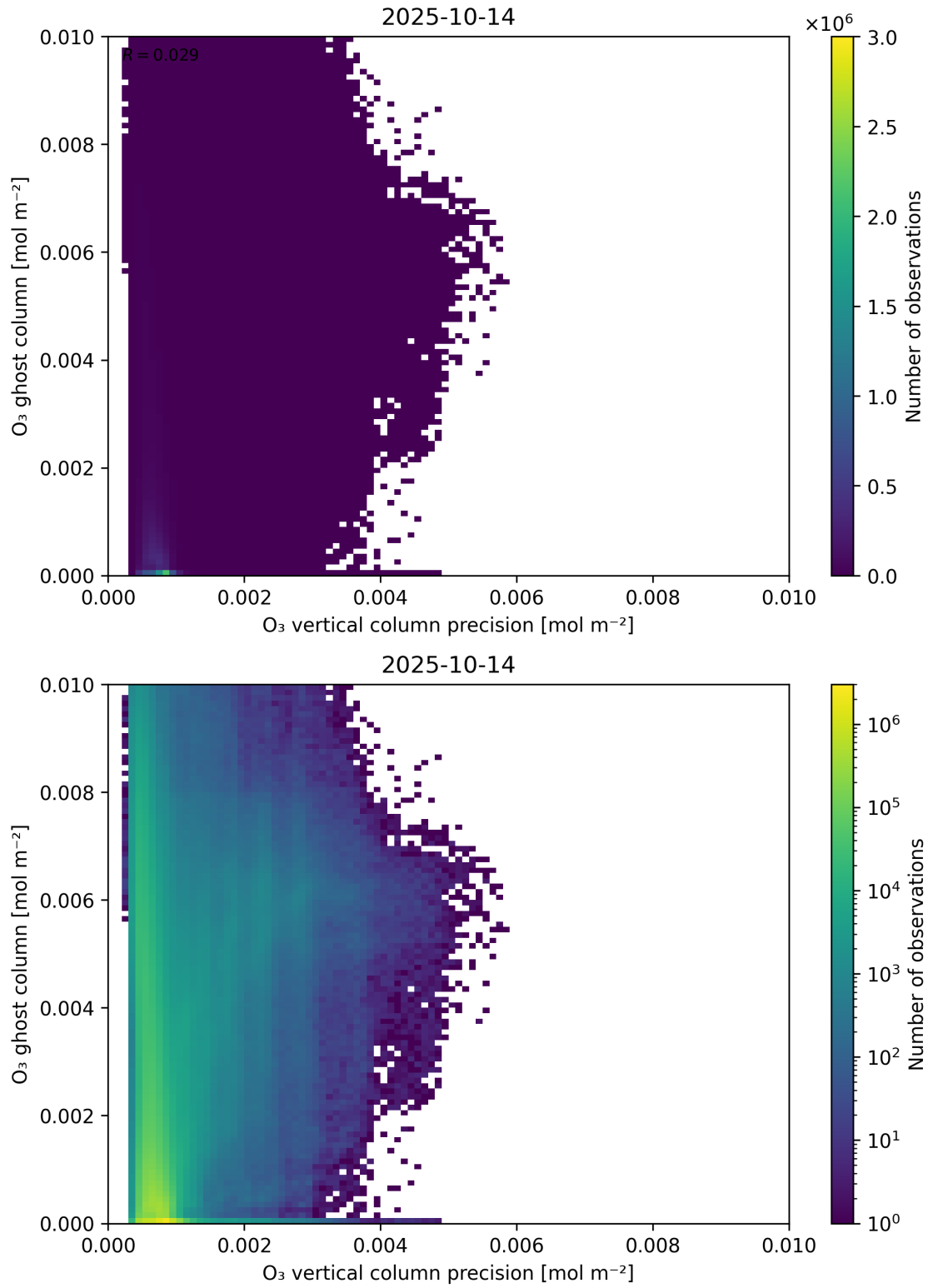
Figure 43: Scatter density plot of “ O_3 vertical column precision” against “ O_3 ghost column” for 2025-10-13 to 2025-10-15.
