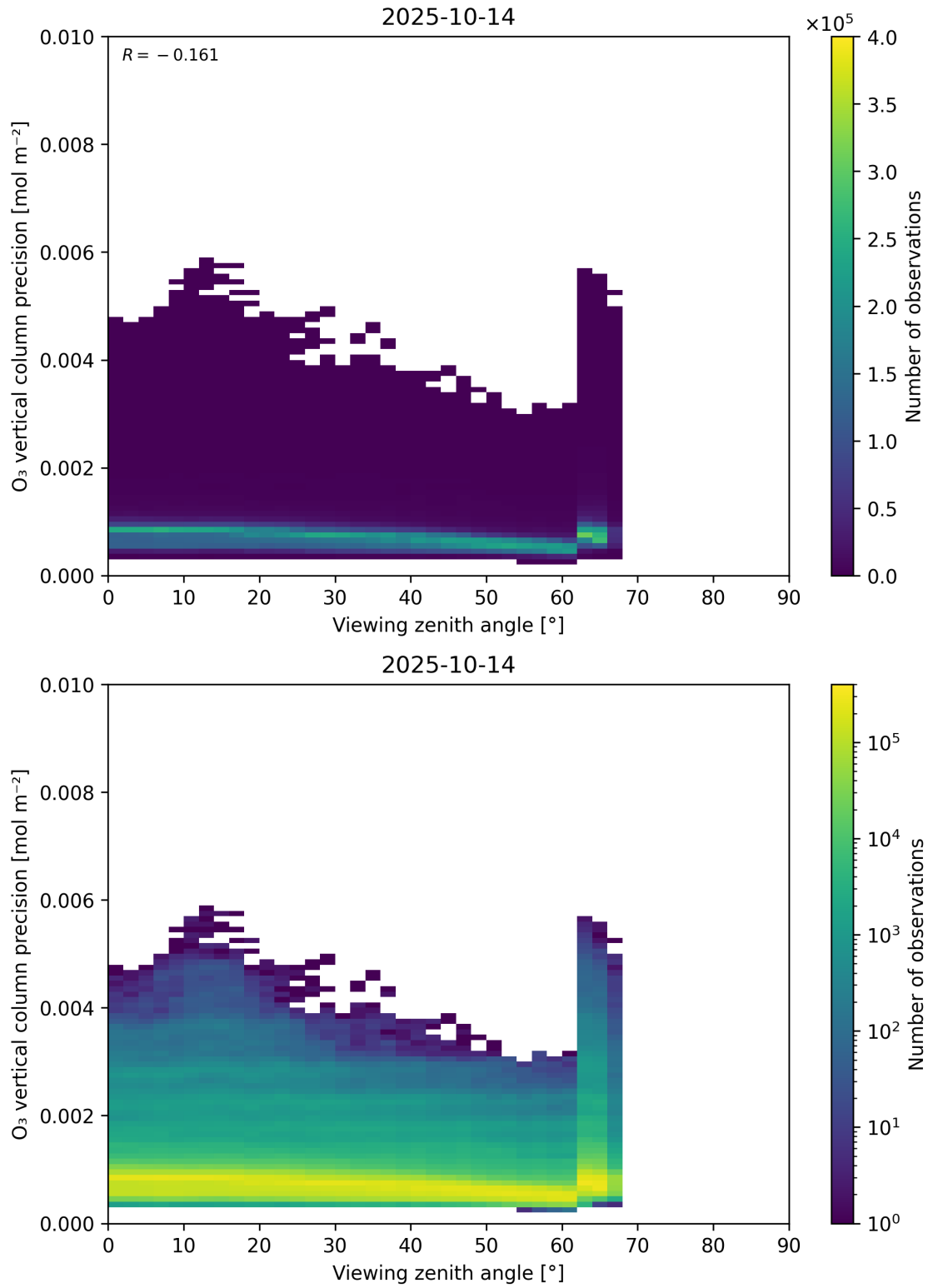
Figure 53: Scatter density plot of “Viewing zenith angle” against “O 3 vertical column precision” for 2025-10-13 to 2025-10-15.
