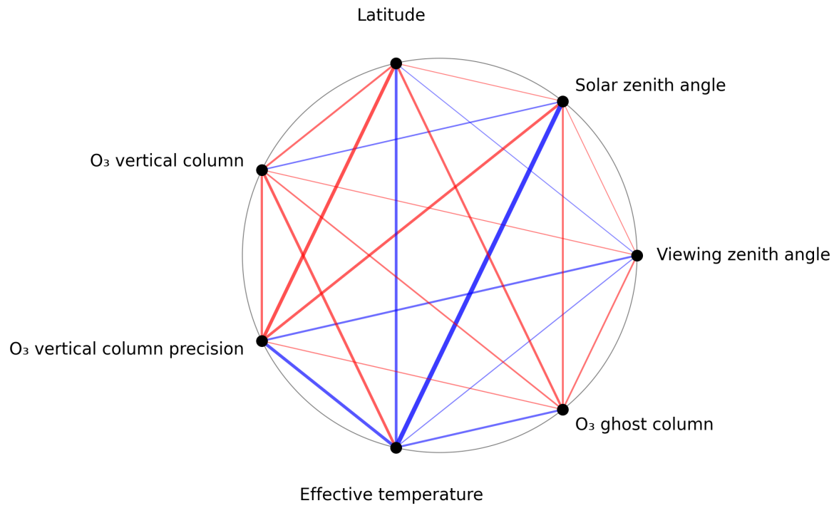
Figure 1: Map of correlation graph for 2025-10-13 to 2025-10-15.
