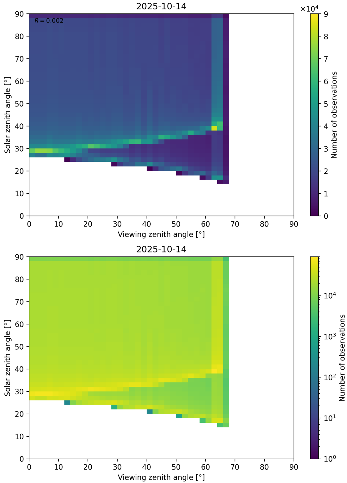
Figure 54: Scatter density plot of “Viewing zenith angle” against “Solar zenith angle” for 2025-10-13 to 2025-10-15.
