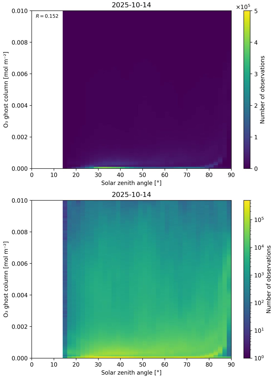
Figure 46: Scatter density plot of “Solar zenith angle” against “O 3 ghost column” for 2025-10-13 to 2025-10-15.
