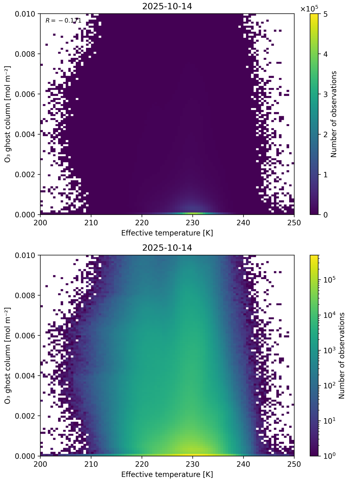
Figure 38: Scatter density plot of “Effective temperature” against “O 3 ghost column” for 2025-10-13 to 2025-10-15.
