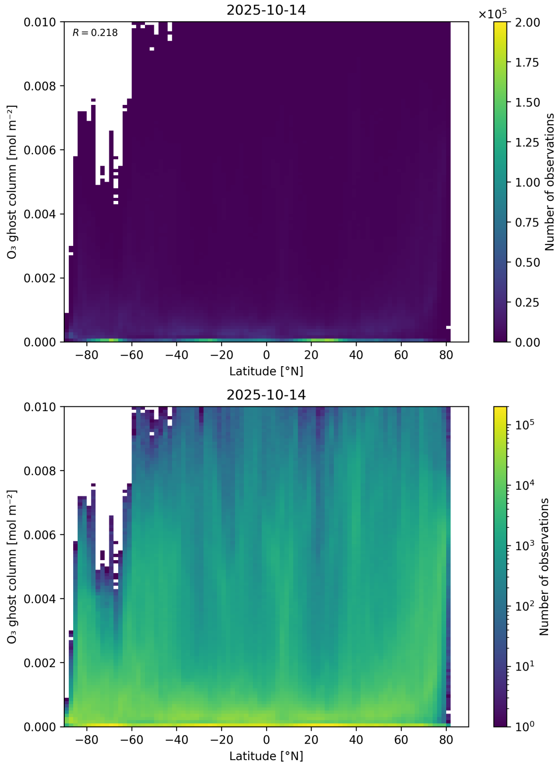
Figure 35: Scatter density plot of “Latitude” against “O 3 ghost column” for 2025-10-13 to 2025-10-15.
