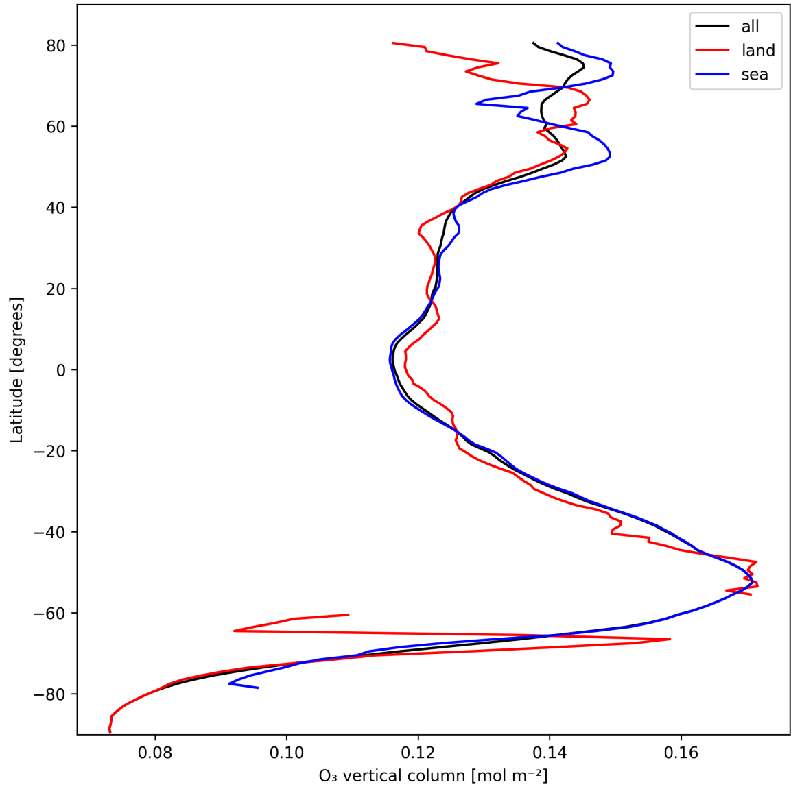
Figure 14: Zonal average of “O 3 vertical column” for 2025-10-13 to 2025-10-15.
