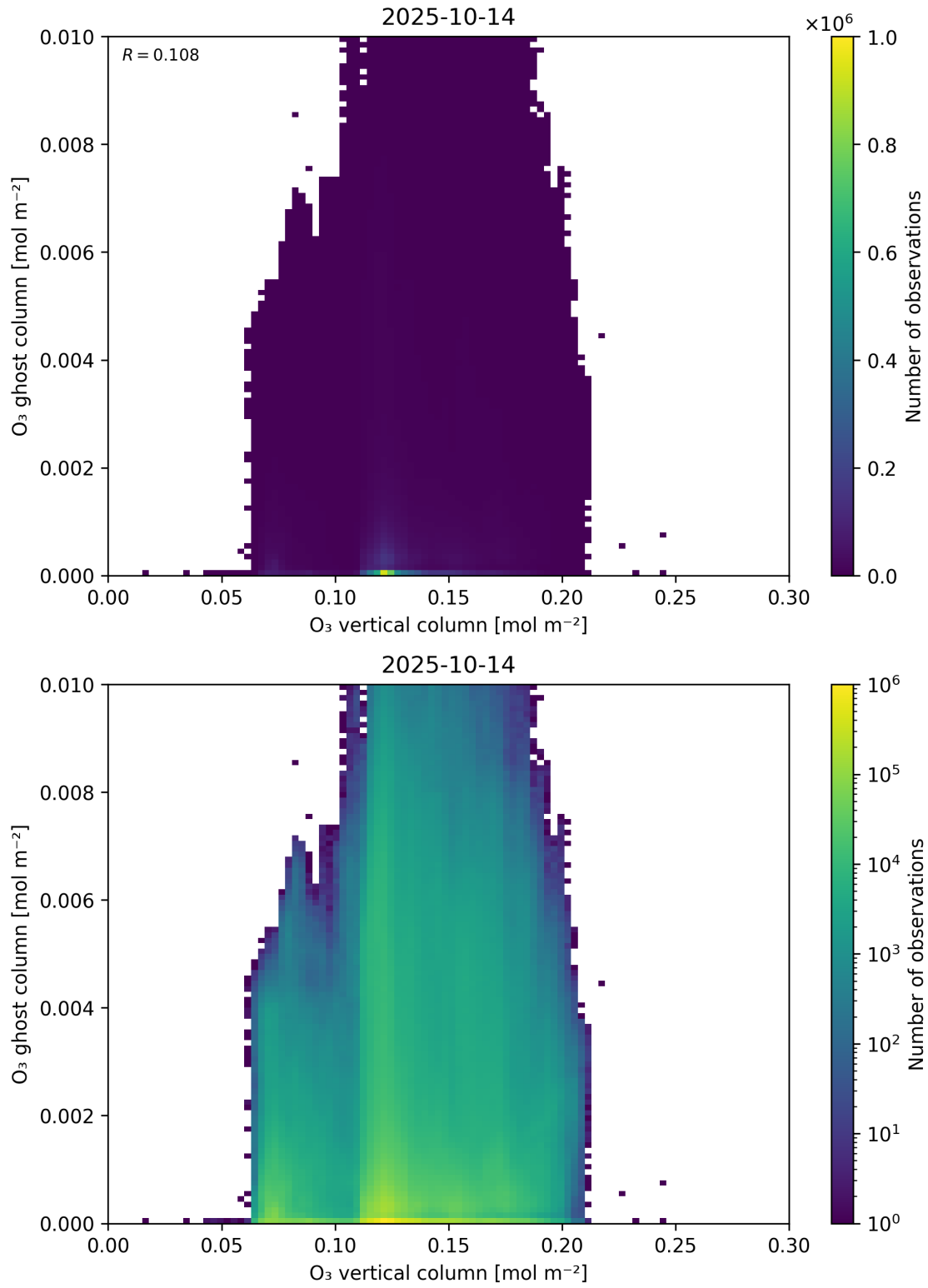
Figure 40: Scatter density plot of “O 3 vertical column” against “O 3 ghost column” for 2025-10-13 to 2025-10-15.
