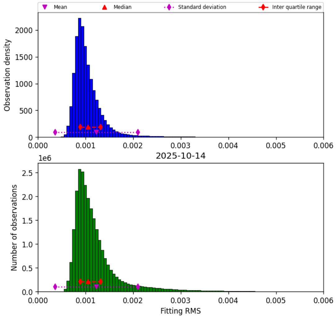
Figure 23: Histogram of “Fitting RMS” for 2025-10-13 to 2025-10-15
