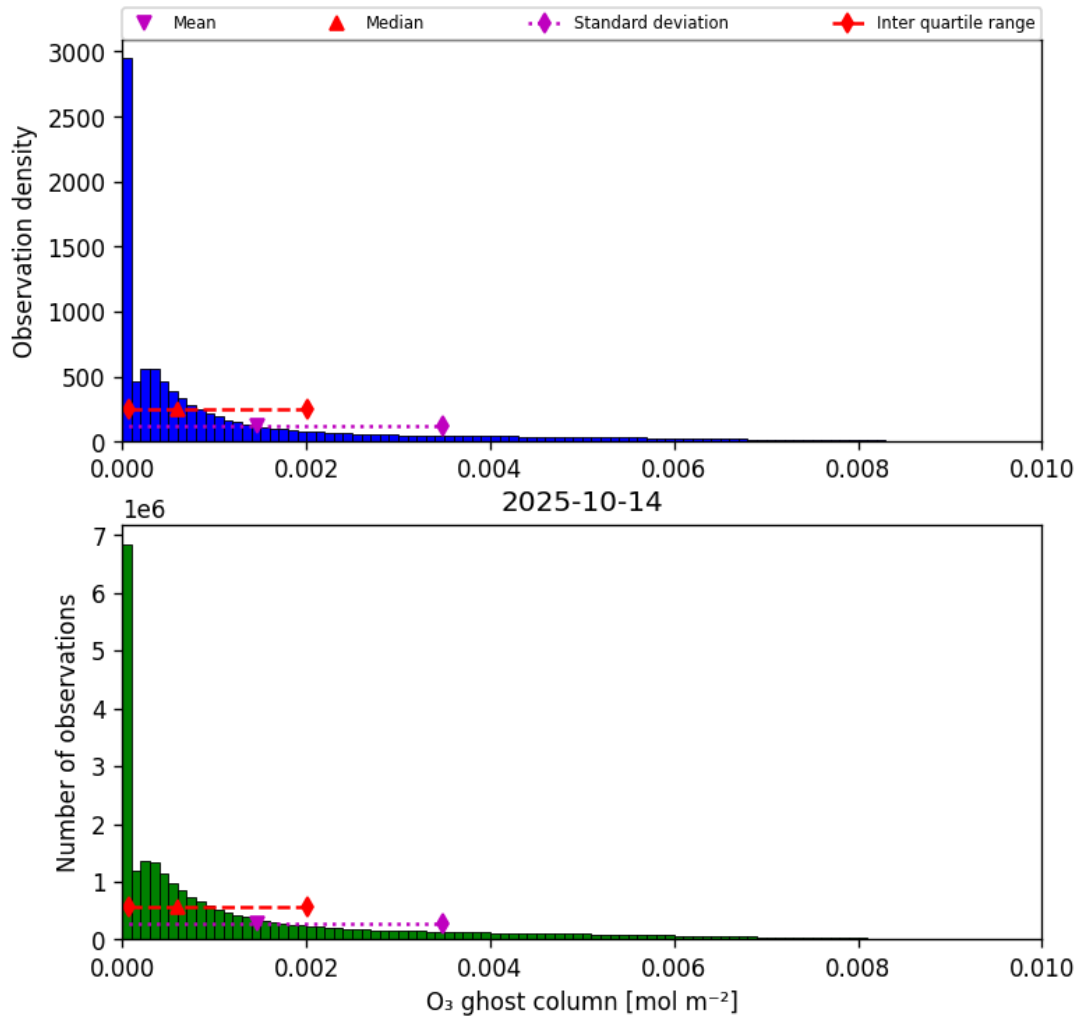
Figure 25: Histogram of “O 3 ghost column” for 2025-10-13 to 2025-10-15
