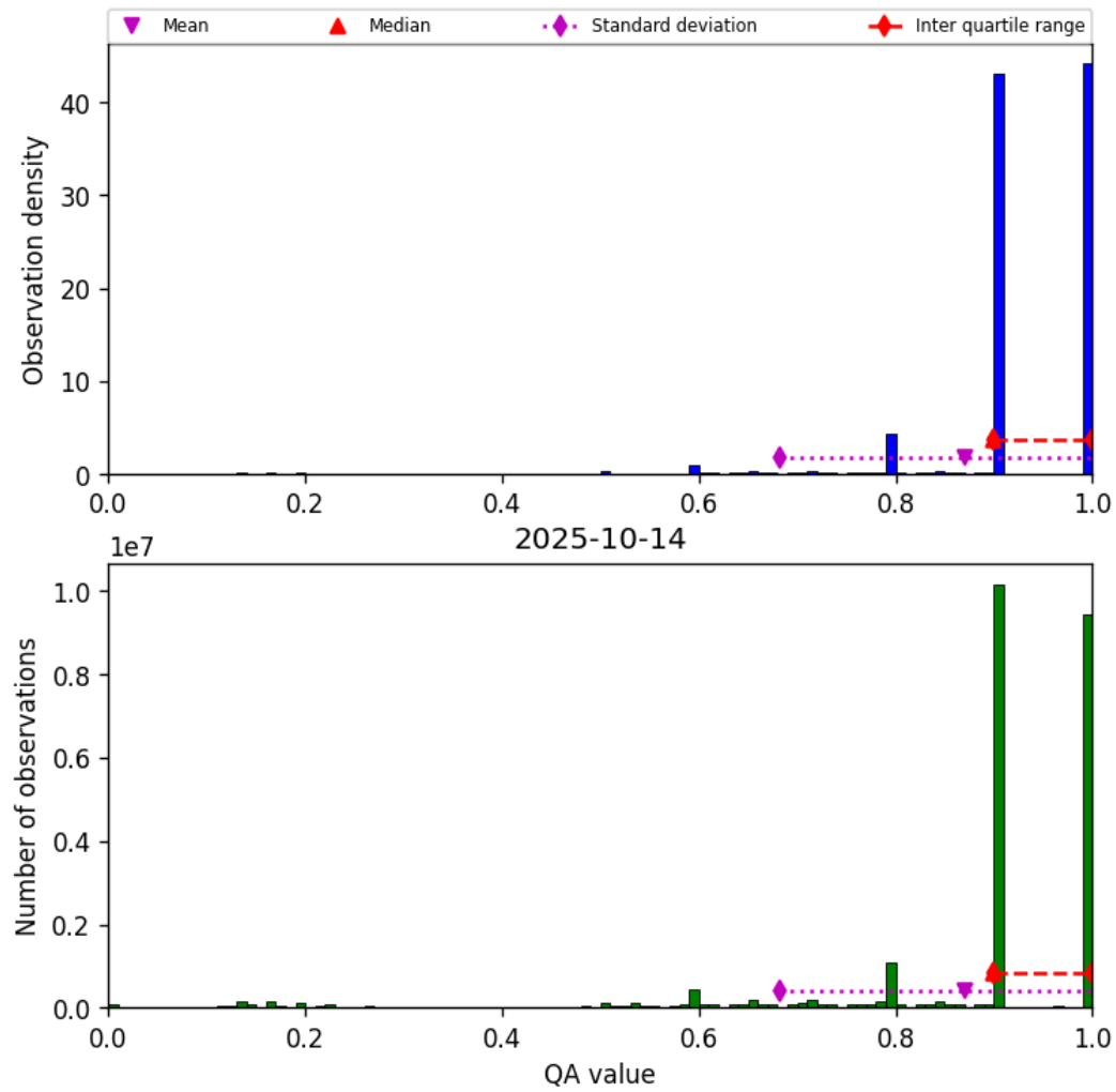
Figure 20: Histogram of “QA value” for 2025-10-13 to 2025-10-15
