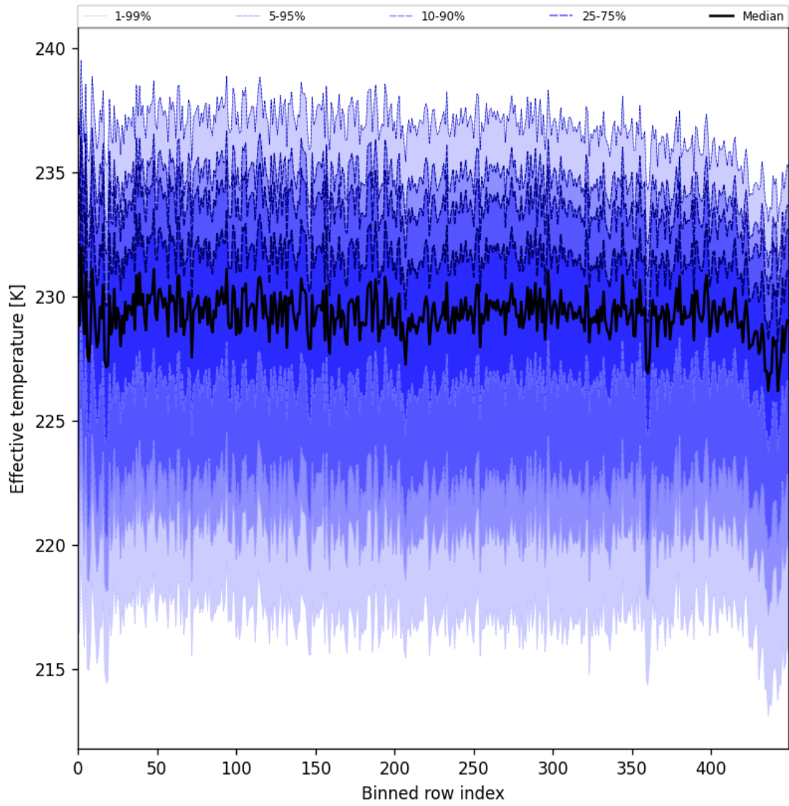
Figure 31: Along track statistics of “Effective temperature” for 2025-10-13 to 2025-10-15
