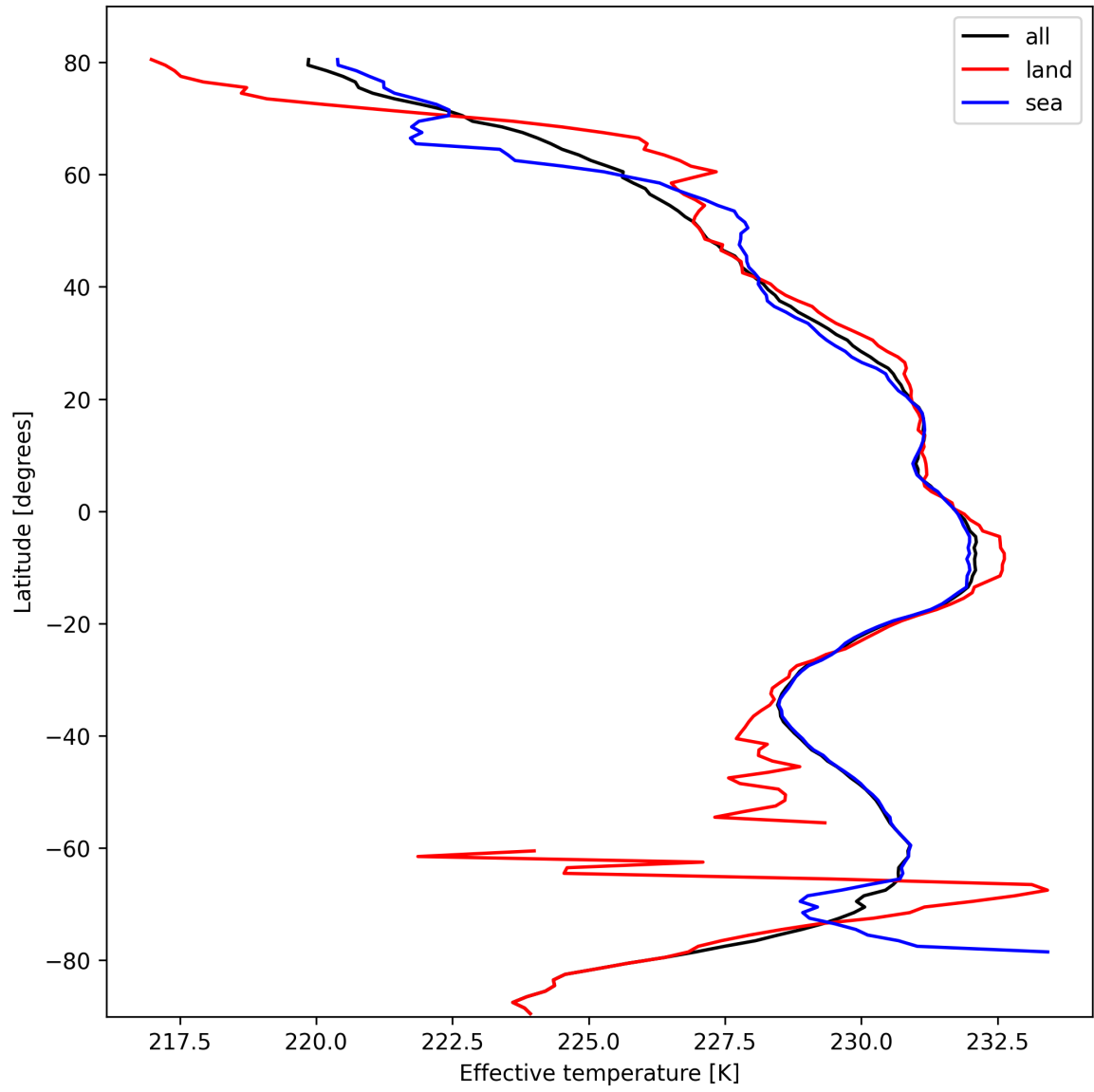
Figure 17: Zonal average of “Effective temperature” for 2025-10-13 to 2025-10-15.
