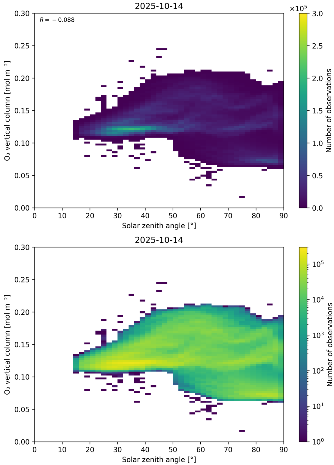
Figure 47: Scatter density plot of “Solar zenith angle” against “O 3 vertical column” for 2025-10-13 to 2025-10-15.
