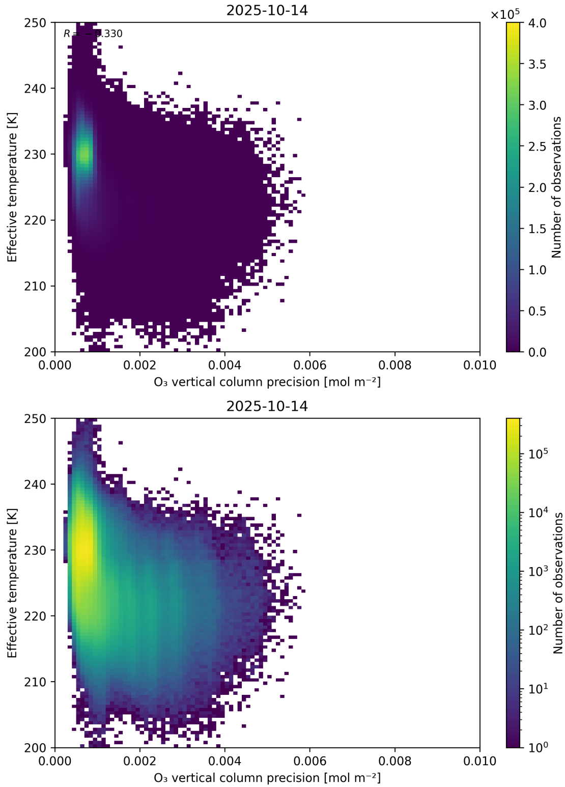
Figure 42: Scatter density plot of “O 3 vertical column precision” against “Effective temperature” for 2025-10-13 to 2025-10-15.
