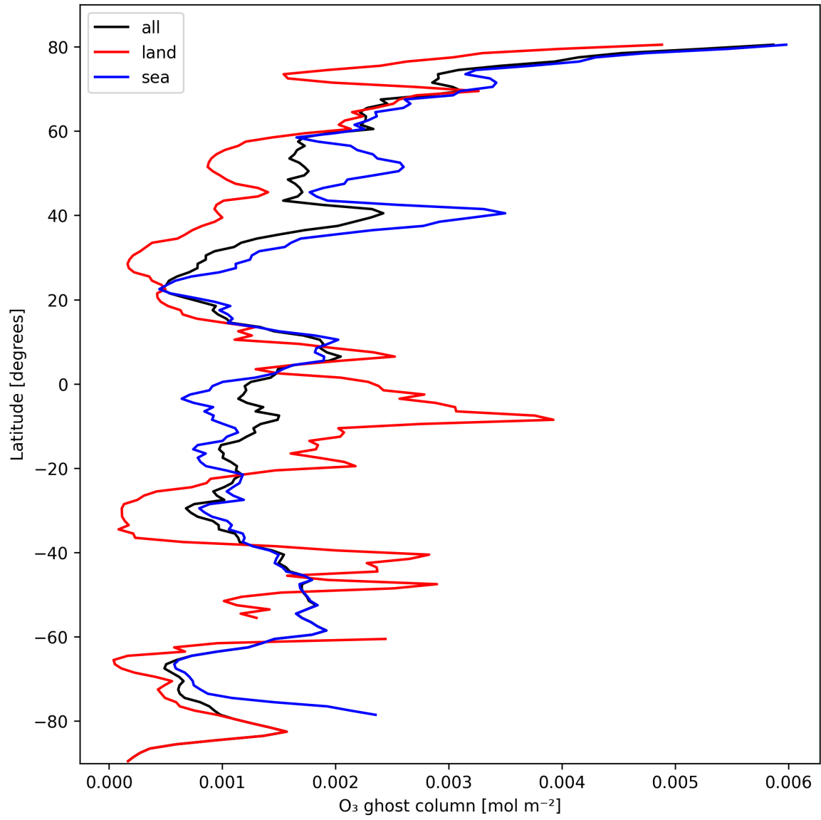
Figure 18: Zonal average of "O 3 ghost column" for 2025-10-13 to 2025-10-15.
