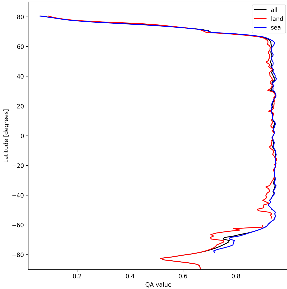
Figure 13: Zonal average of “QA value” for 2025-10-13 to 2025-10-15.
