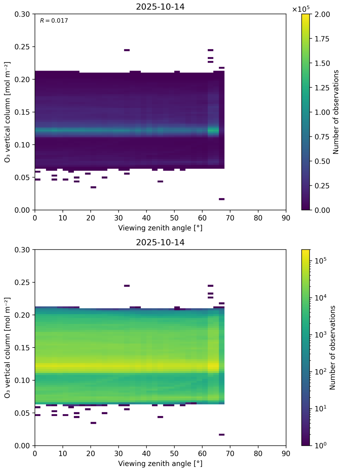
Figure 52: Scatter density plot of “Viewing zenith angle” against “O 3 vertical column” for 2025-10-13 to 2025-10-15.
