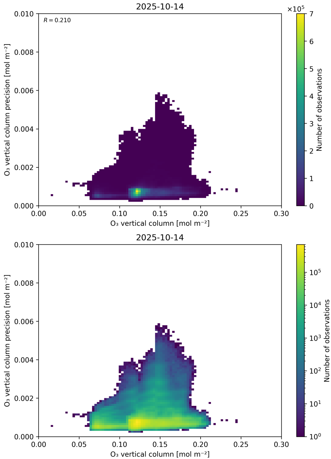
Figure 41: Scatter density plot of “O 3 vertical column” against “O 3 vertical column precision” for 2025-10-13 to 2025-10-15.
