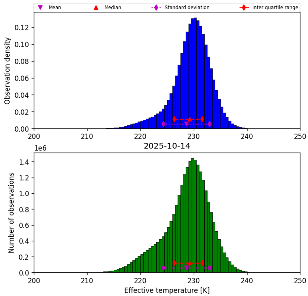
Figure 24: Histogram of “Effective temperature” for 2025-10-13 to 2025-10-15
