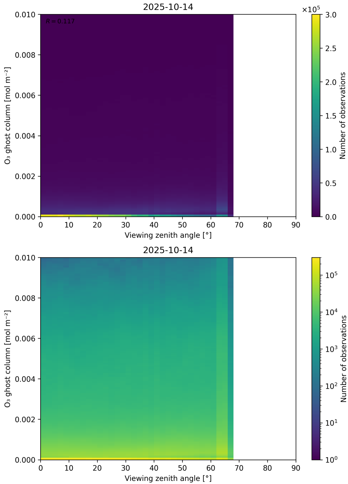
Figure 51: Scatter density plot of “Viewing zenith angle” against “O 3 ghost column” for 2025-10-13 to 2025-10-15.
