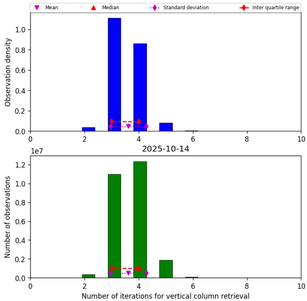
Figure 26: Histogram of “Number of iterations for vertical column retrieval” for 2025-10-13 to 2025-10-15
