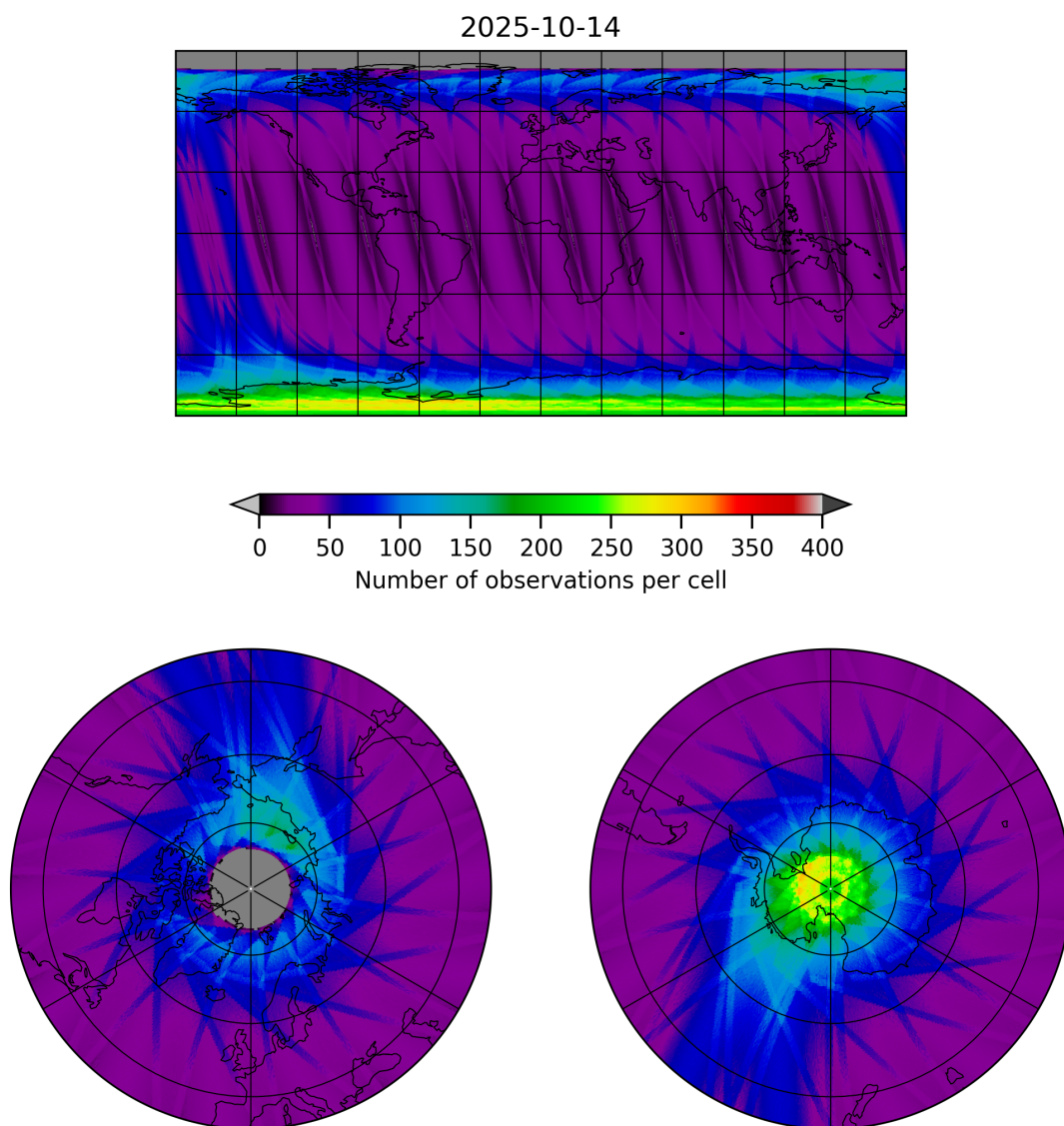
Figure 12: Map of the number of observations for 2025-10-13 to 2025-10-15
