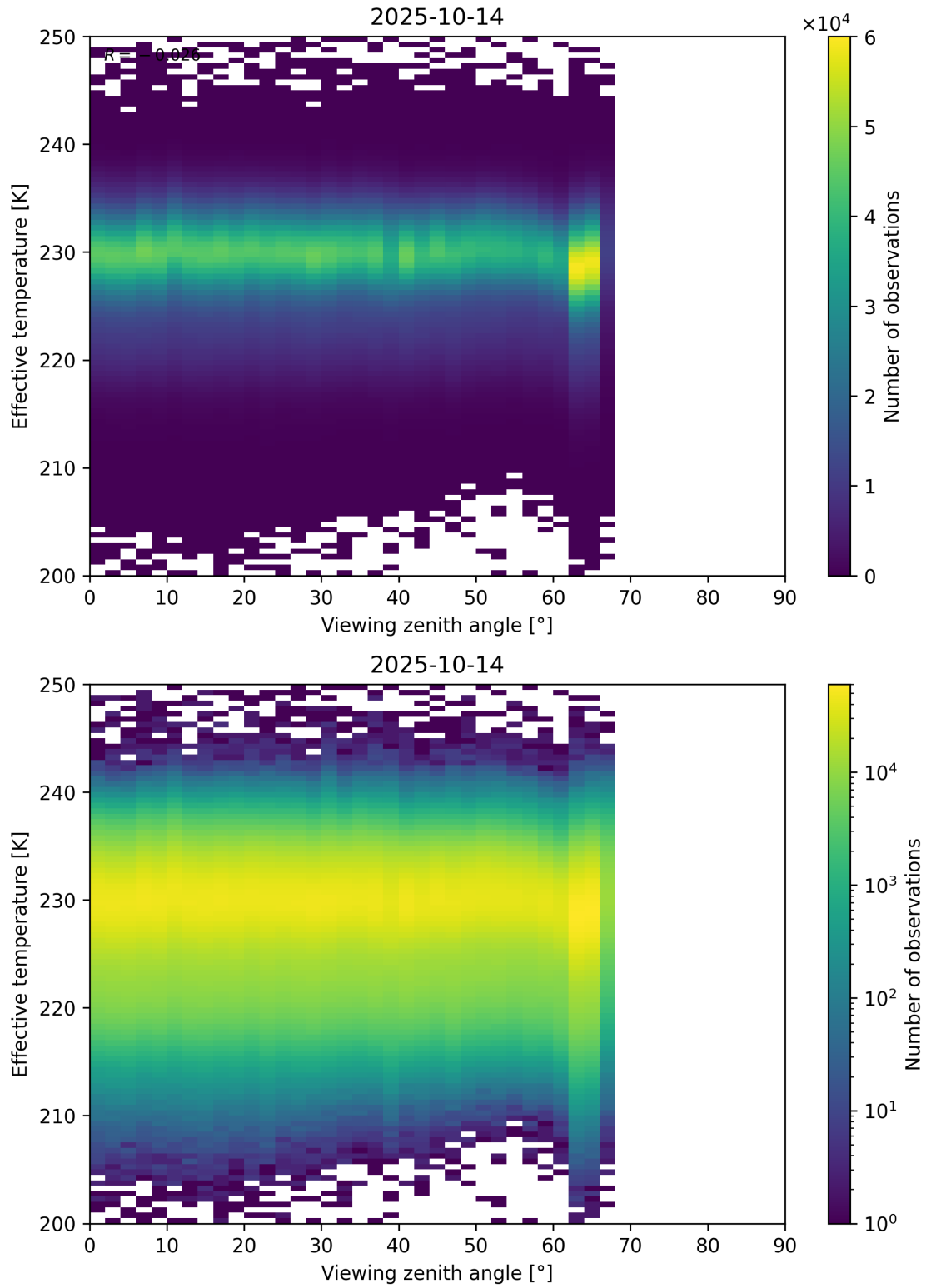
Figure 50: Scatter density plot of “Viewing zenith angle” against “Effective temperature” for 2025-10-13 to 2025-10-15.
