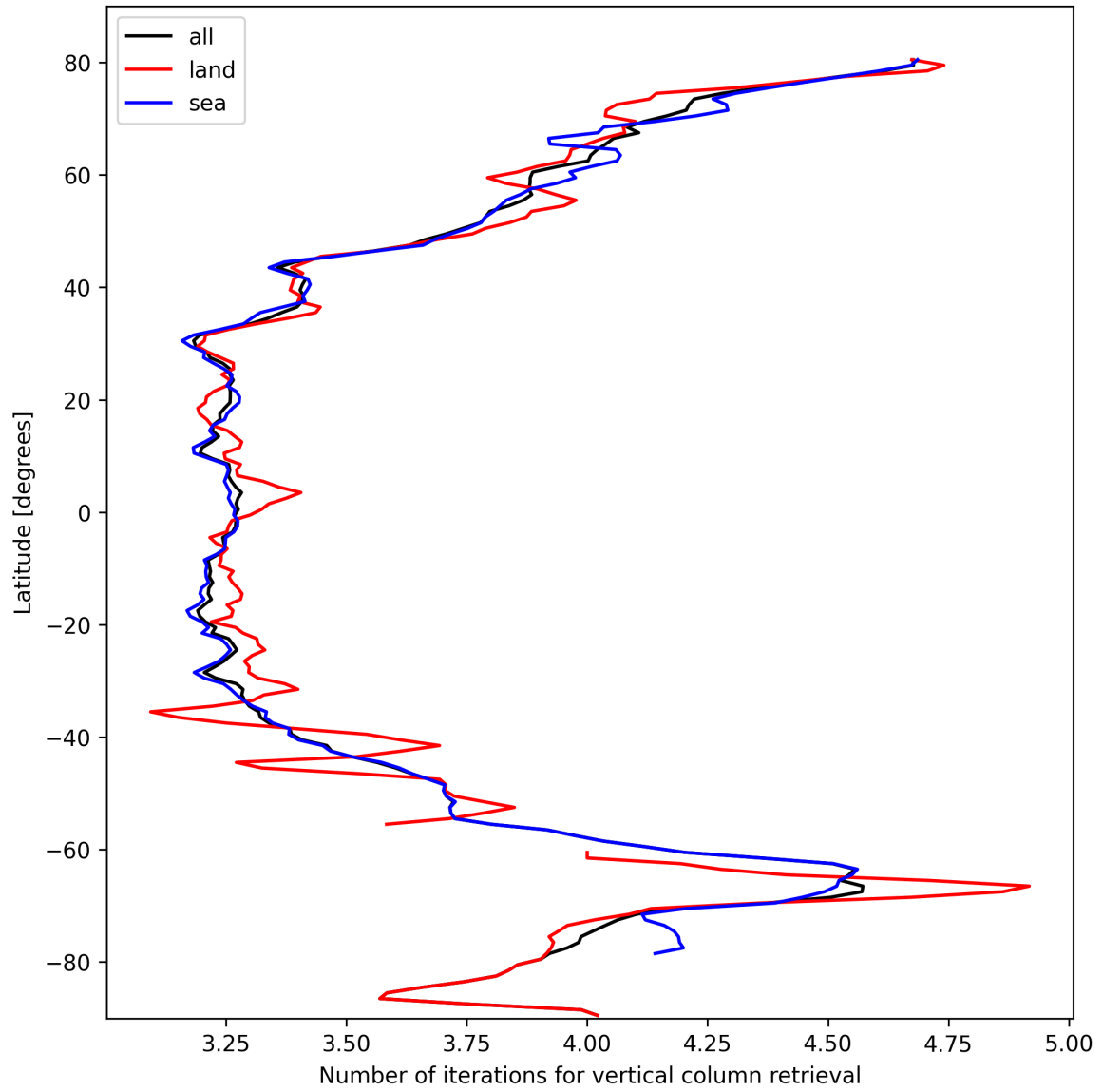
Figure 19: Zonal average of “Number of iterations for vertical column retrieval” for 2025-10-13 to 2025-10-15.
