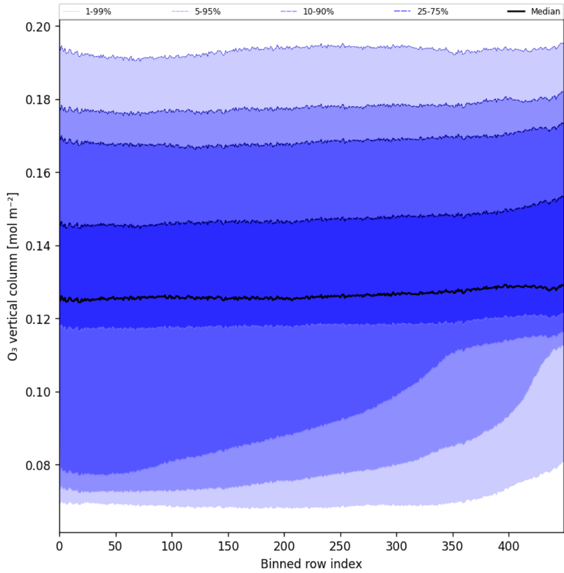
Figure 28: Along track statistics of “O 3 vertical column” for 2025-10-13 to 2025-10-15
