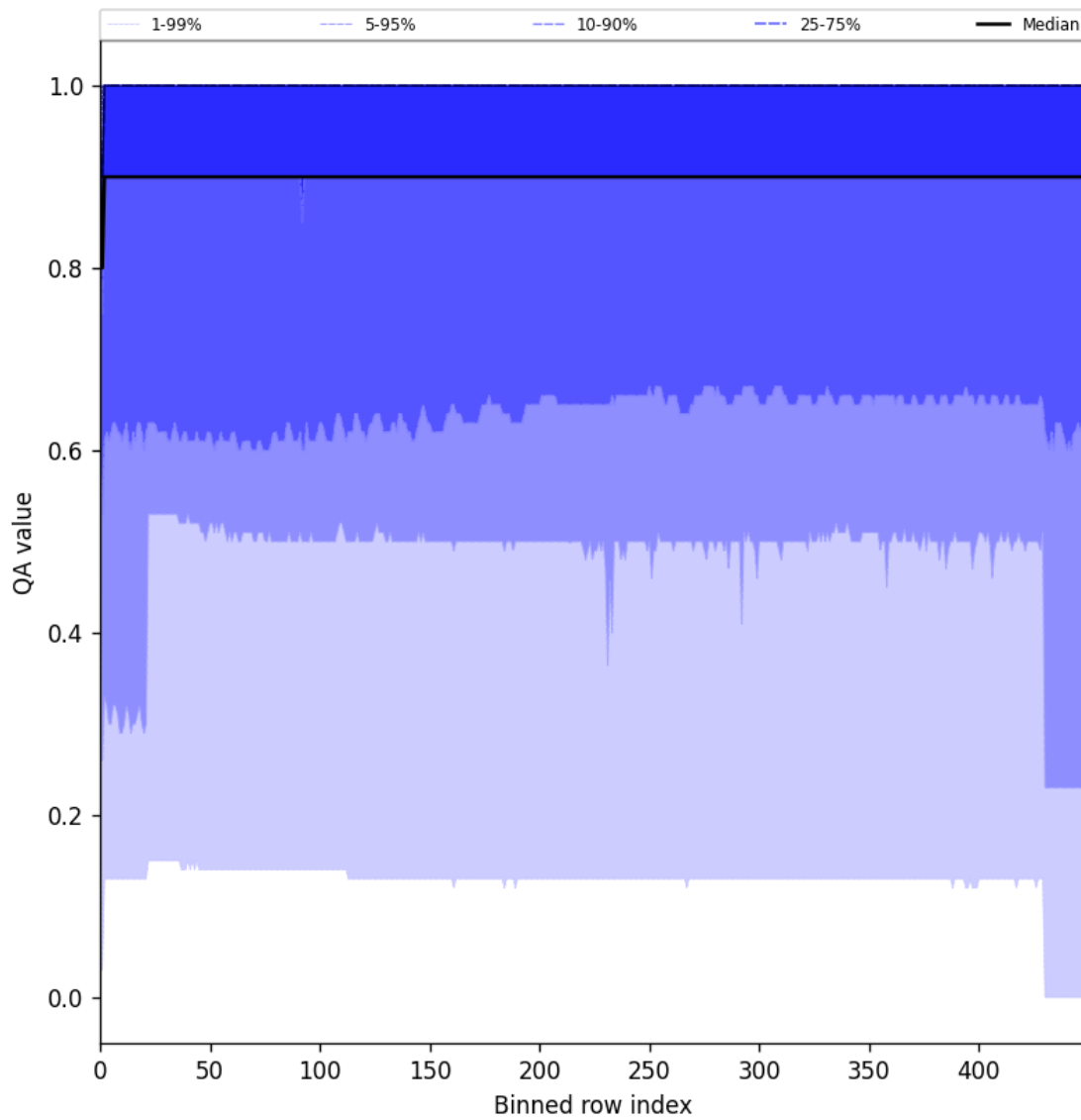
Figure 27: Along track statistics of “QA value” for 2025-10-13 to 2025-10-15
