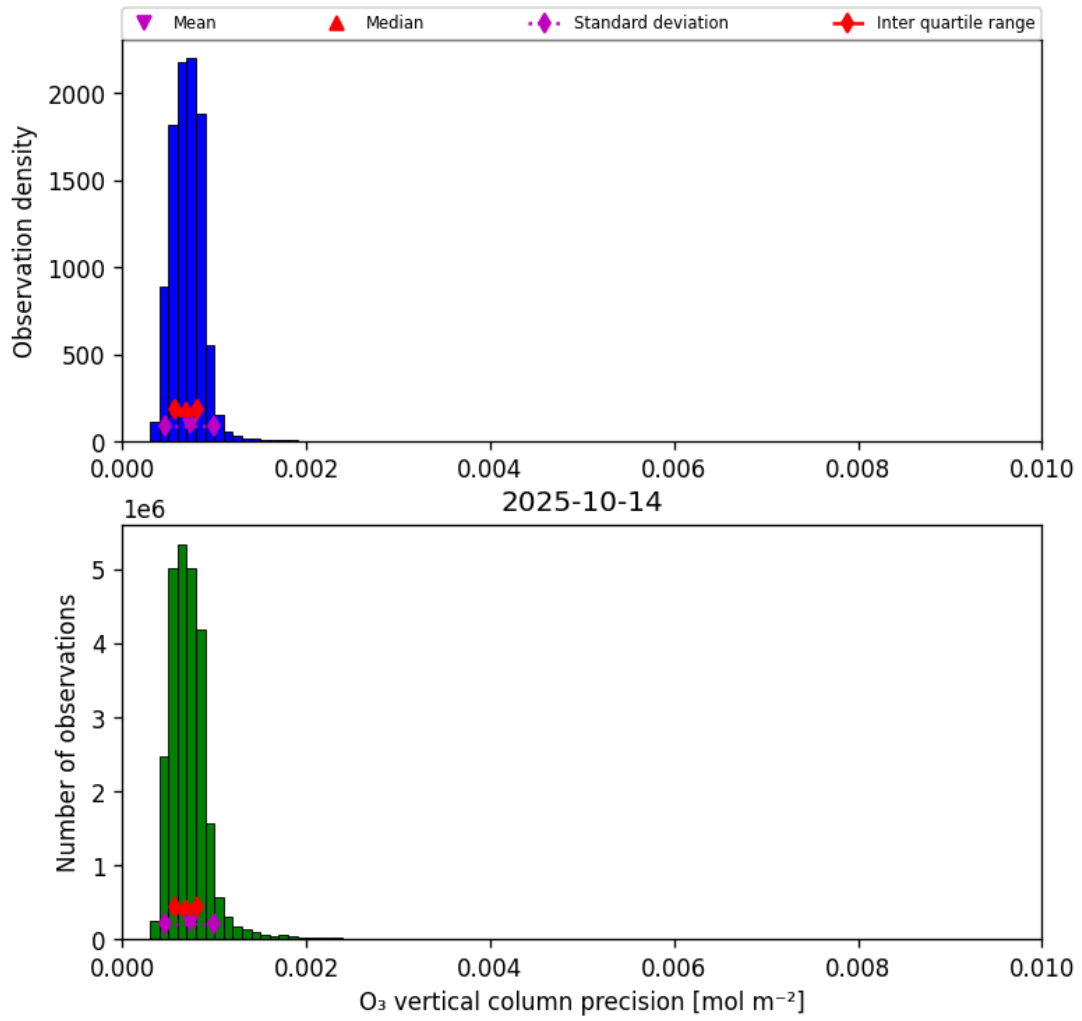
Figure 22: Histogram of “O 3 vertical column precision” for 2025-10-13 to 2025-10-15
