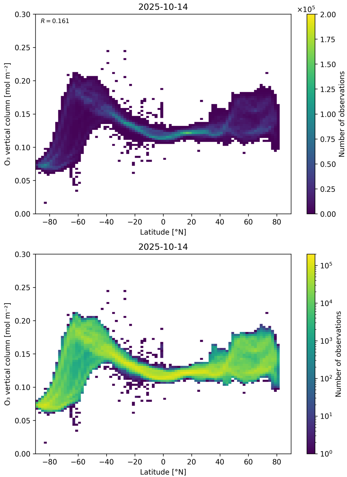
Figure 36: Scatter density plot of “Latitude” against “O 3 vertical column” for 2025-10-13 to 2025-10-15.
