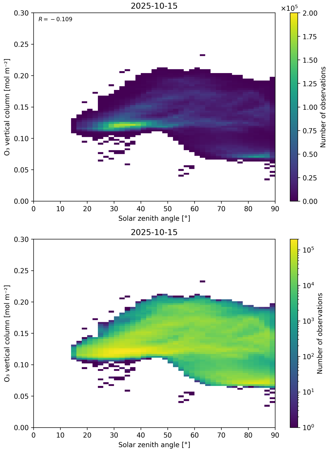
Figure 47: Scatter density plot of “Solar zenith angle” against “O 3 vertical column” for 2025-10-14 to 2025-10-16.
