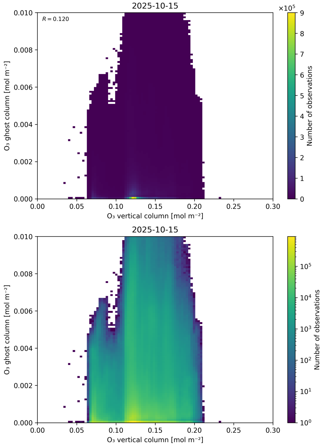
Figure 40: Scatter density plot of “O 3 vertical column” against “O 3 ghost column” for 2025-10-14 to 2025-10-16.
