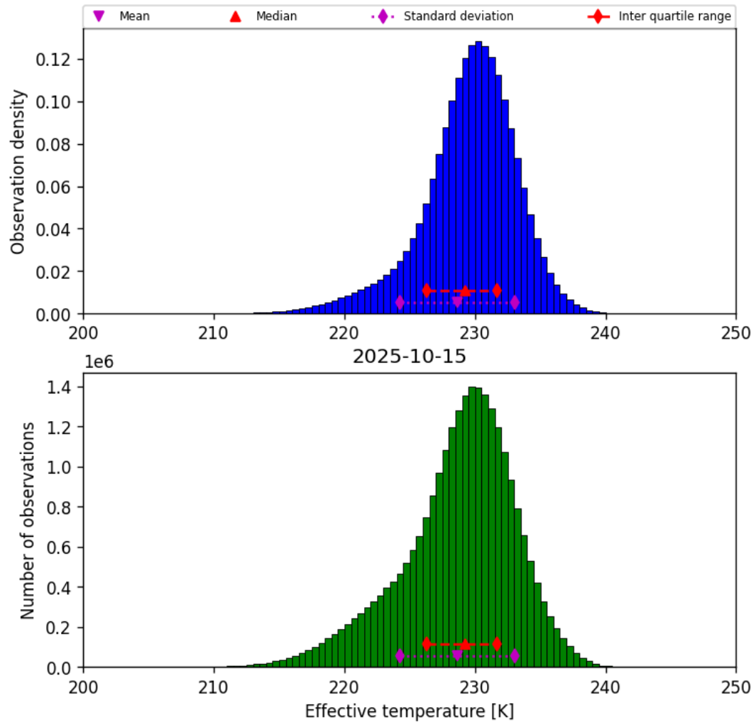
Figure 24: Histogram of “Effective temperature” for 2025-10-14 to 2025-10-16
