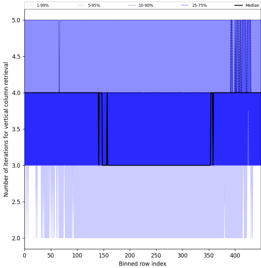
Figure 33: Along track statistics of “Number of iterations for vertical column retrieval” for 2025-10-14 to 2025-10-16
