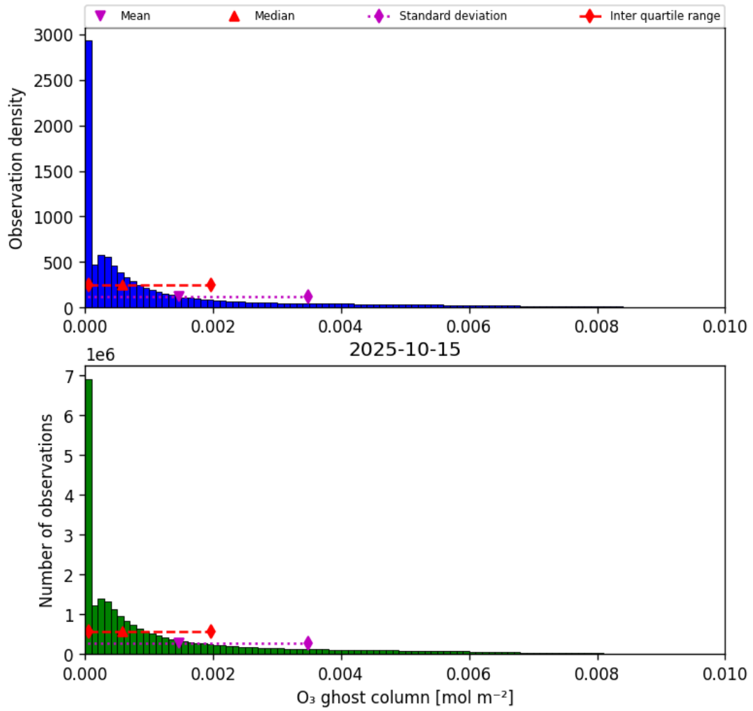
Figure 25: Histogram of “O 3 ghost column” for 2025-10-14 to 2025-10-16
