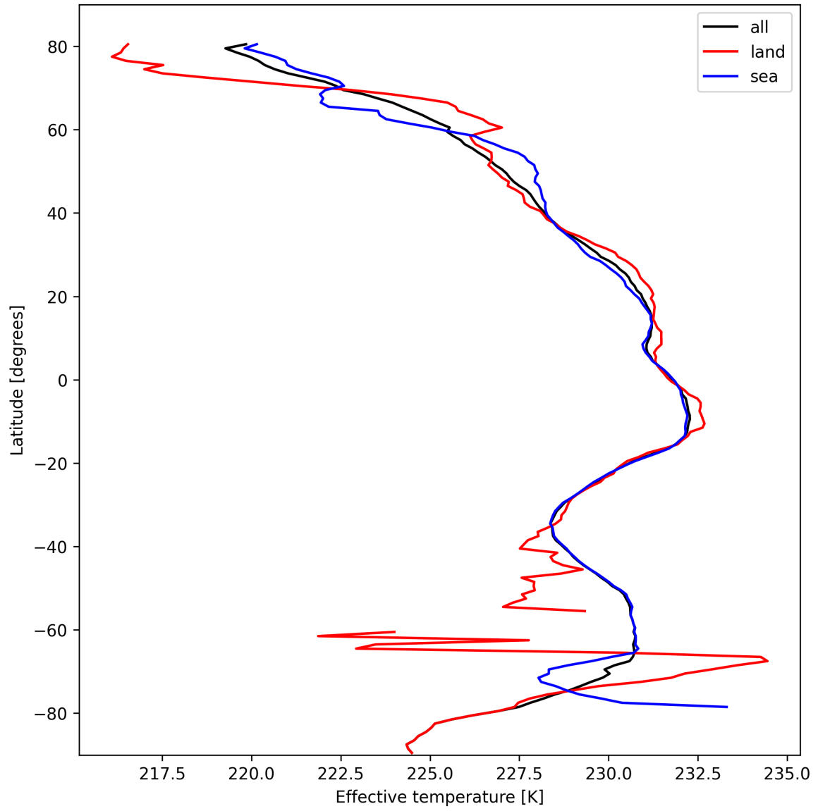
Figure 17: Zonal average of “Effective temperature” for 2025-10-14 to 2025-10-16.
