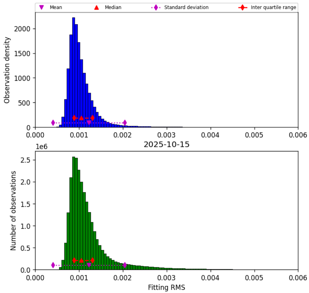
Figure 23: Histogram of “Fitting RMS” for 2025-10-14 to 2025-10-16
