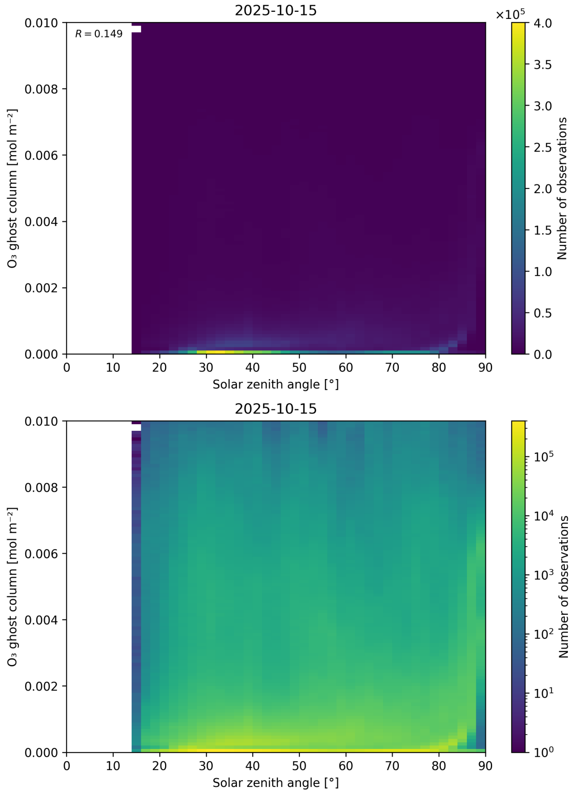
Figure 46: Scatter density plot of “Solar zenith angle” against “O 3 ghost column” for 2025-10-14 to 2025-10-16.
