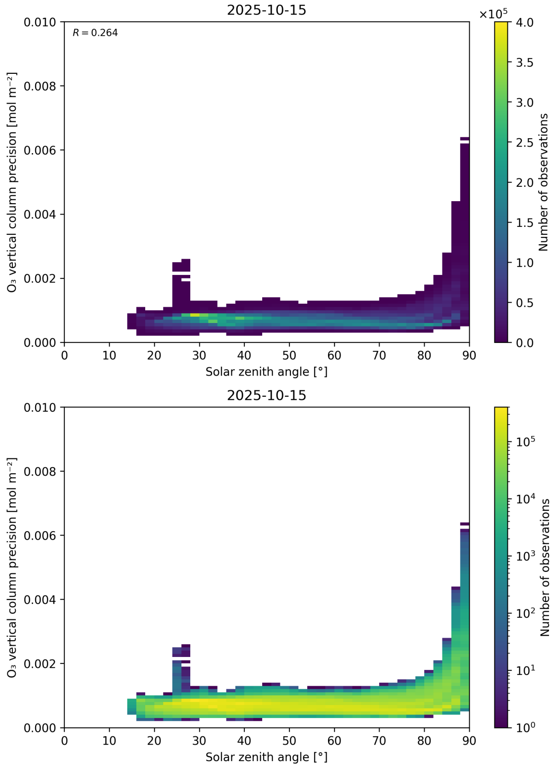
Figure 48: Scatter density plot of “Solar zenith angle” against “O 3 vertical column precision” for 2025-10-14 to 2025-10-16.
