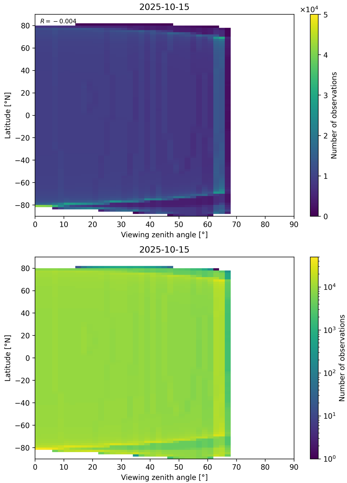
Figure 49: Scatter density plot of “Viewing zenith angle” against “Latitude” for 2025-10-14 to 2025-10-16.
