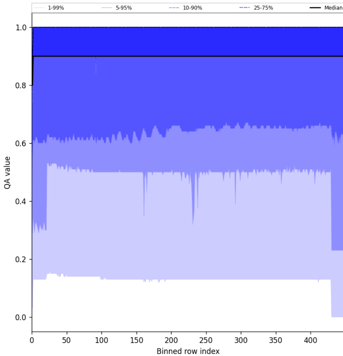
Figure 27: Along track statistics of “QA value” for 2025-10-14 to 2025-10-16
