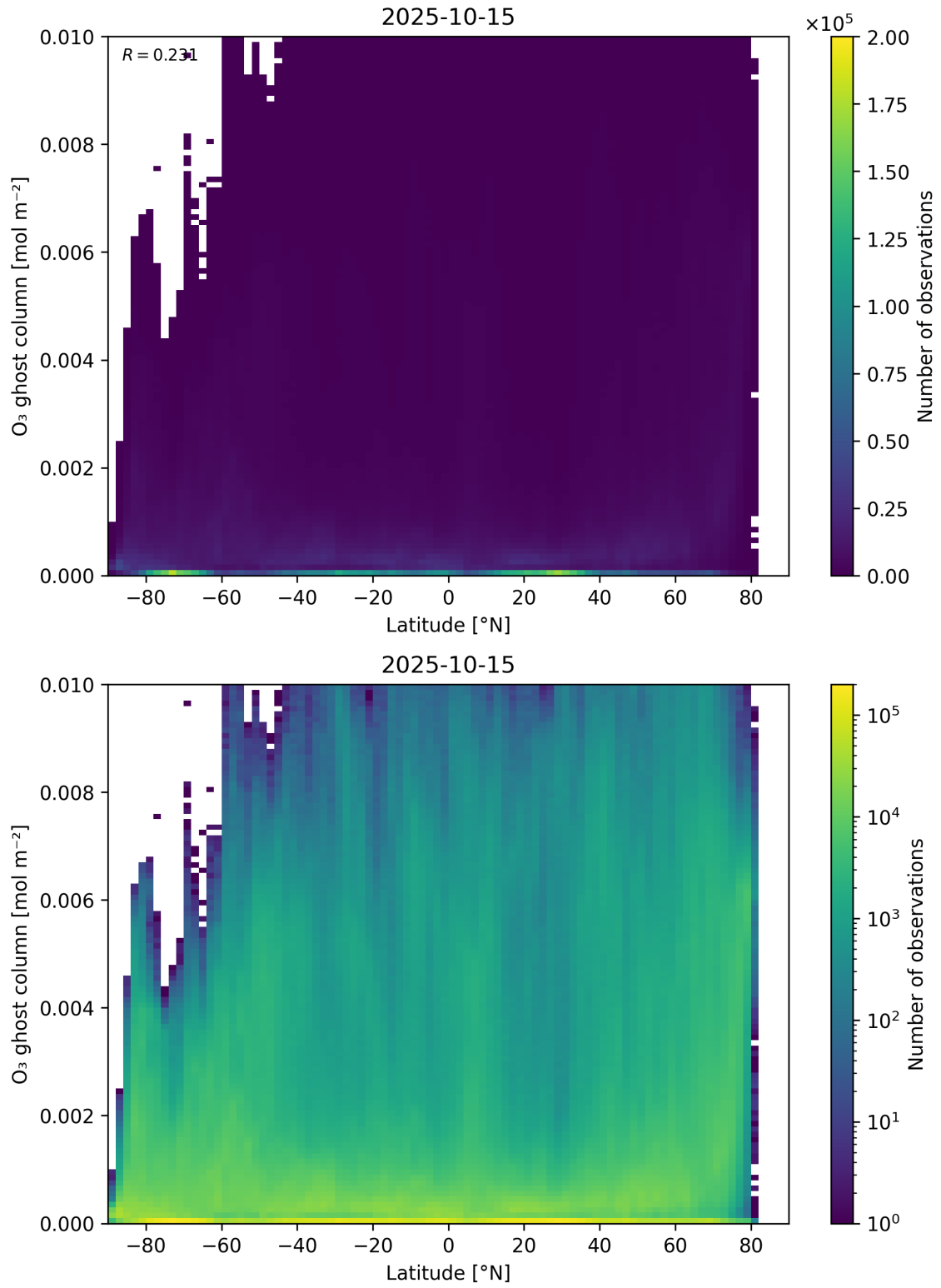
Figure 35: Scatter density plot of “Latitude” against “O 3 ghost column” for 2025-10-14 to 2025-10-16.
