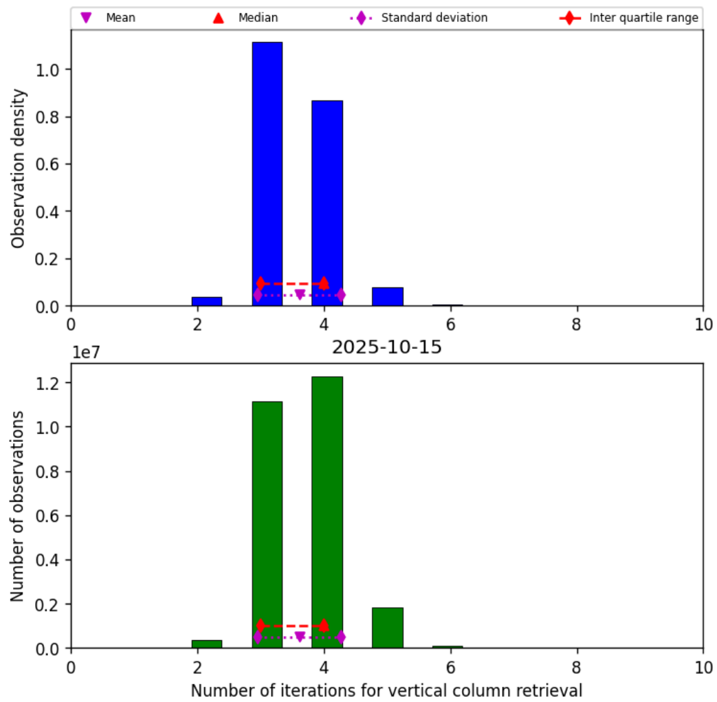
Figure 26: Histogram of “Number of iterations for vertical column retrieval” for 2025-10-14 to 2025-10-16
