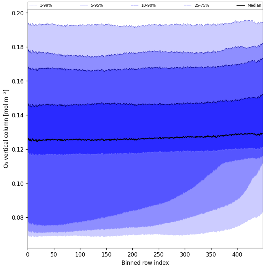
Figure 28: Along track statistics of “O 3 vertical column” for 2025-10-14 to 2025-10-16
