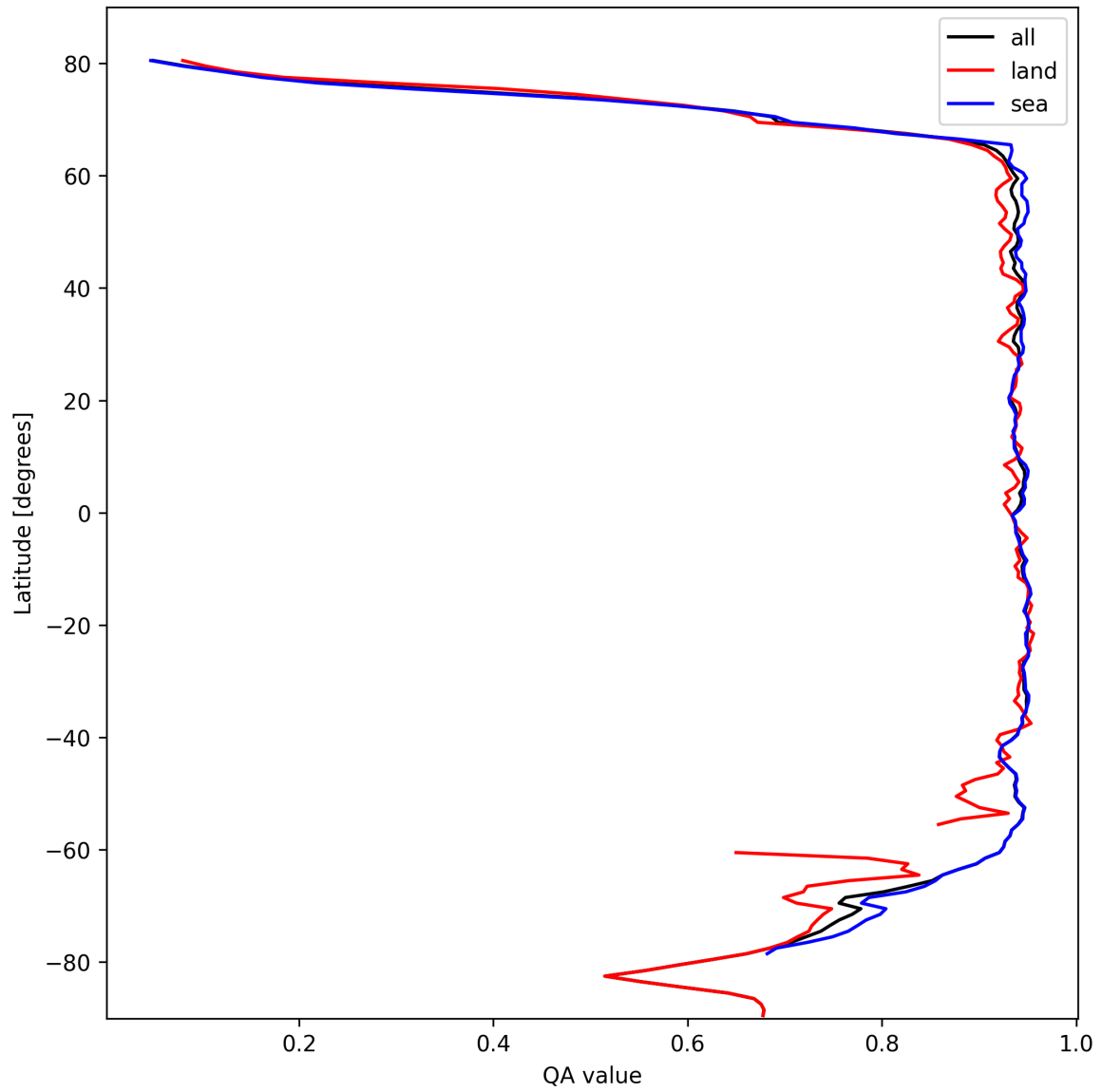
Figure 13: Zonal average of “QA value” for 2025-10-14 to 2025-10-16.
