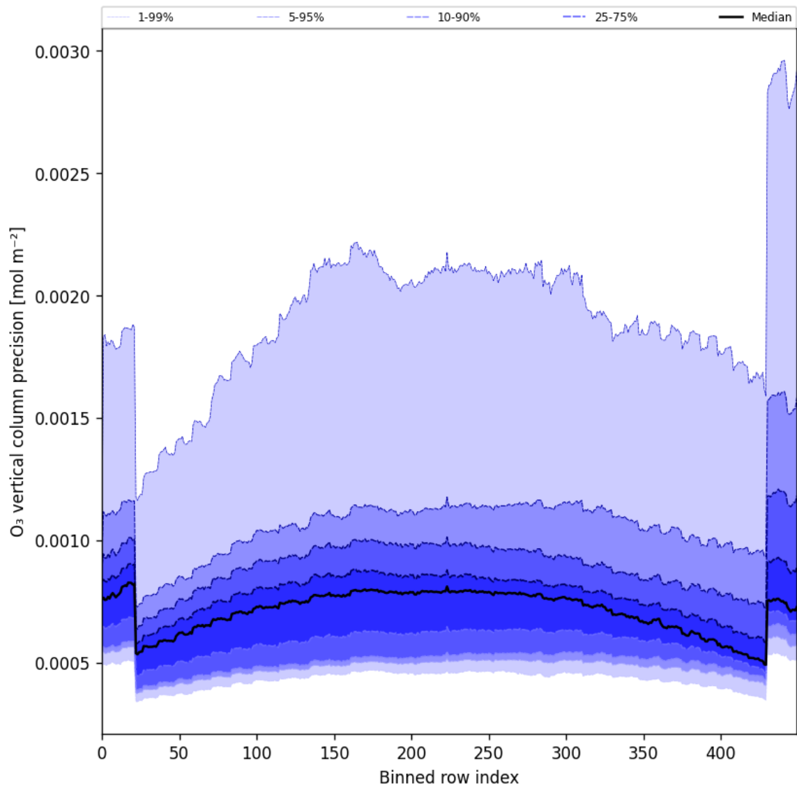
Figure 29: Along track statistics of “O 3 vertical column precision” for 2025-10-14 to 2025-10-16
