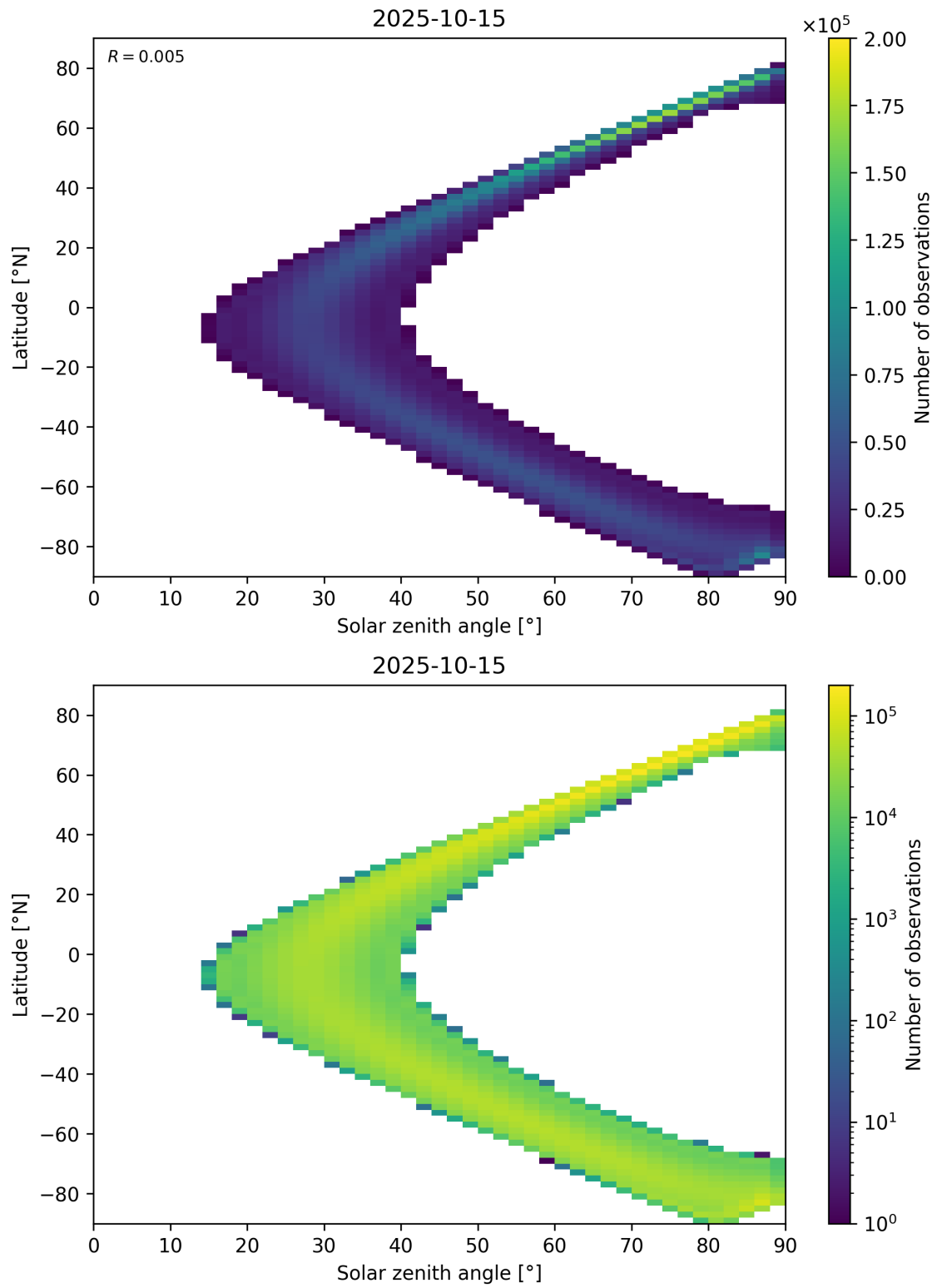
Figure 44: Scatter density plot of “Solar zenith angle” against “Latitude” for 2025-10-14 to 2025-10-16.
