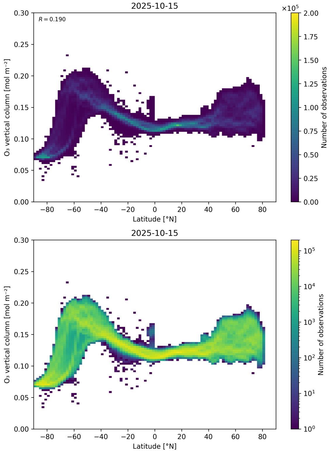
Figure 36: Scatter density plot of “Latitude” against “O 3 vertical column” for 2025-10-14 to 2025-10-16.
