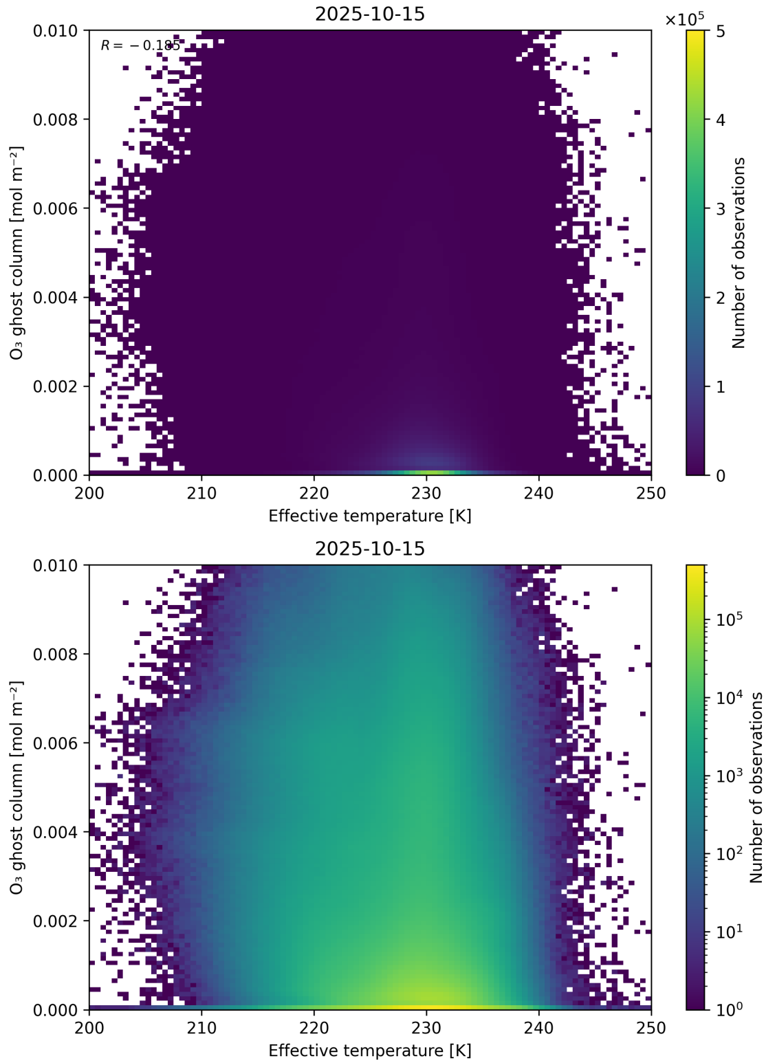
Figure 38: Scatter density plot of “Effective temperature” against “O 3 ghost column” for 2025-10-14 to 2025-10-16.
