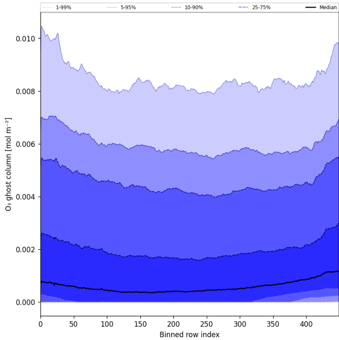
Figure 32: Along track statistics of “O 3 ghost column” for 2025-10-14 to 2025-10-16
