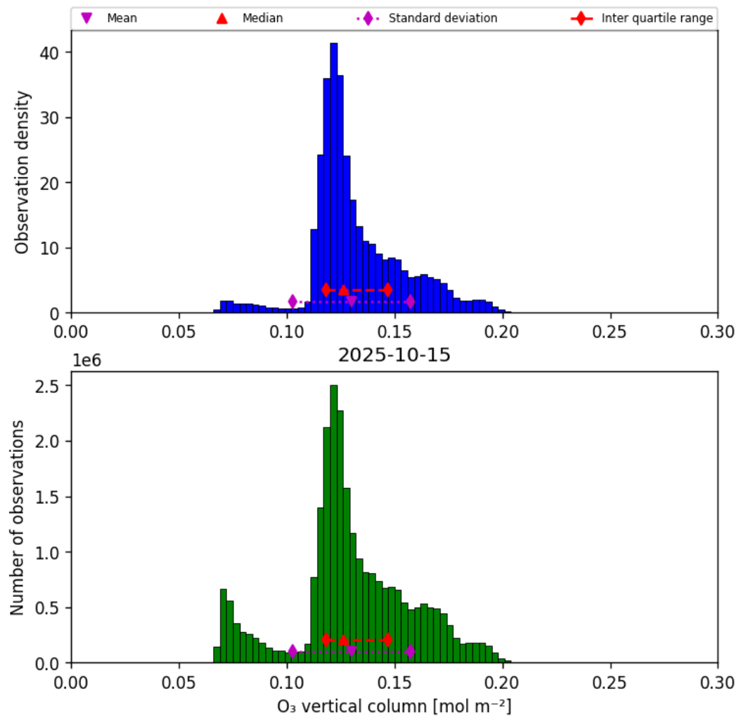
Figure 21: Histogram of “O 3 vertical column” for 2025-10-14 to 2025-10-16
