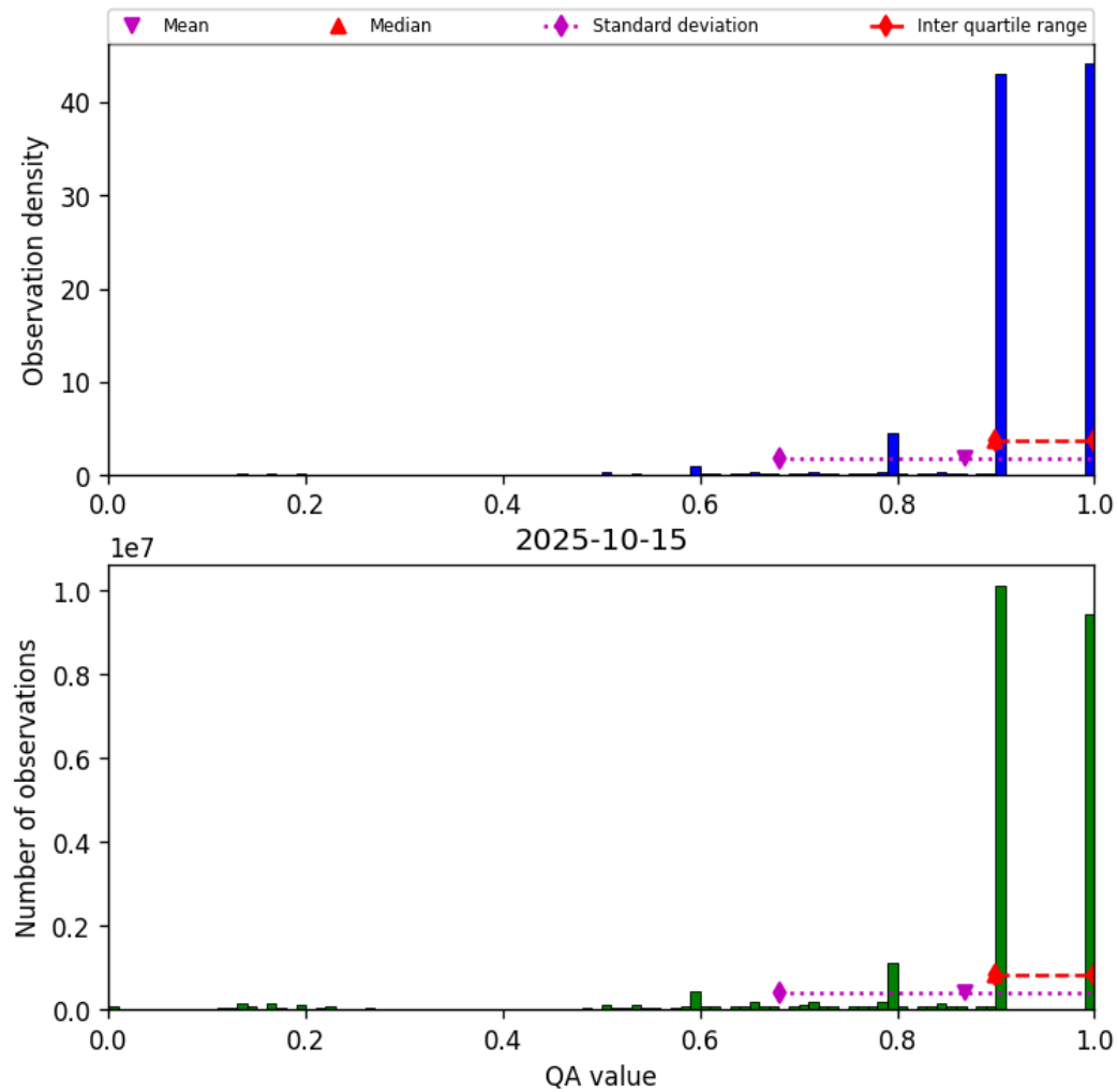
Figure 20: Histogram of “QA value” for 2025-10-14 to 2025-10-16
