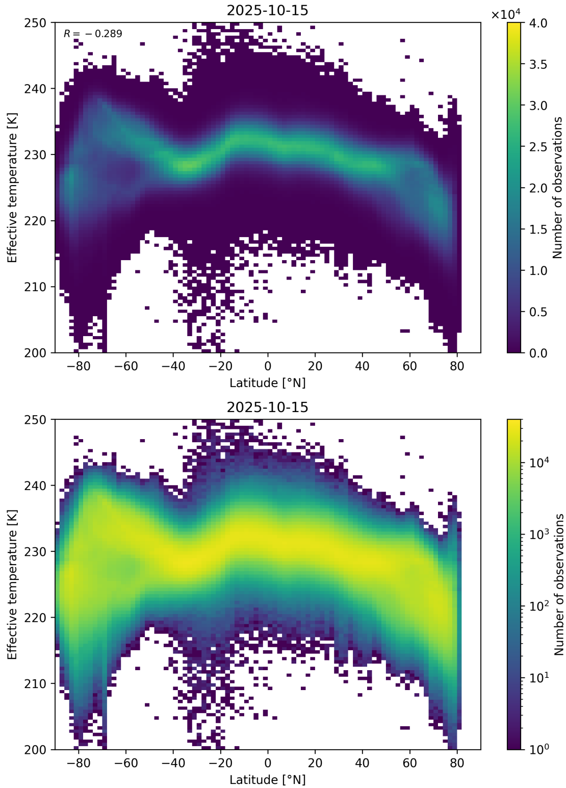
Figure 34: Scatter density plot of “Latitude” against “Effective temperature” for 2025-10-14 to 2025-10-16.
