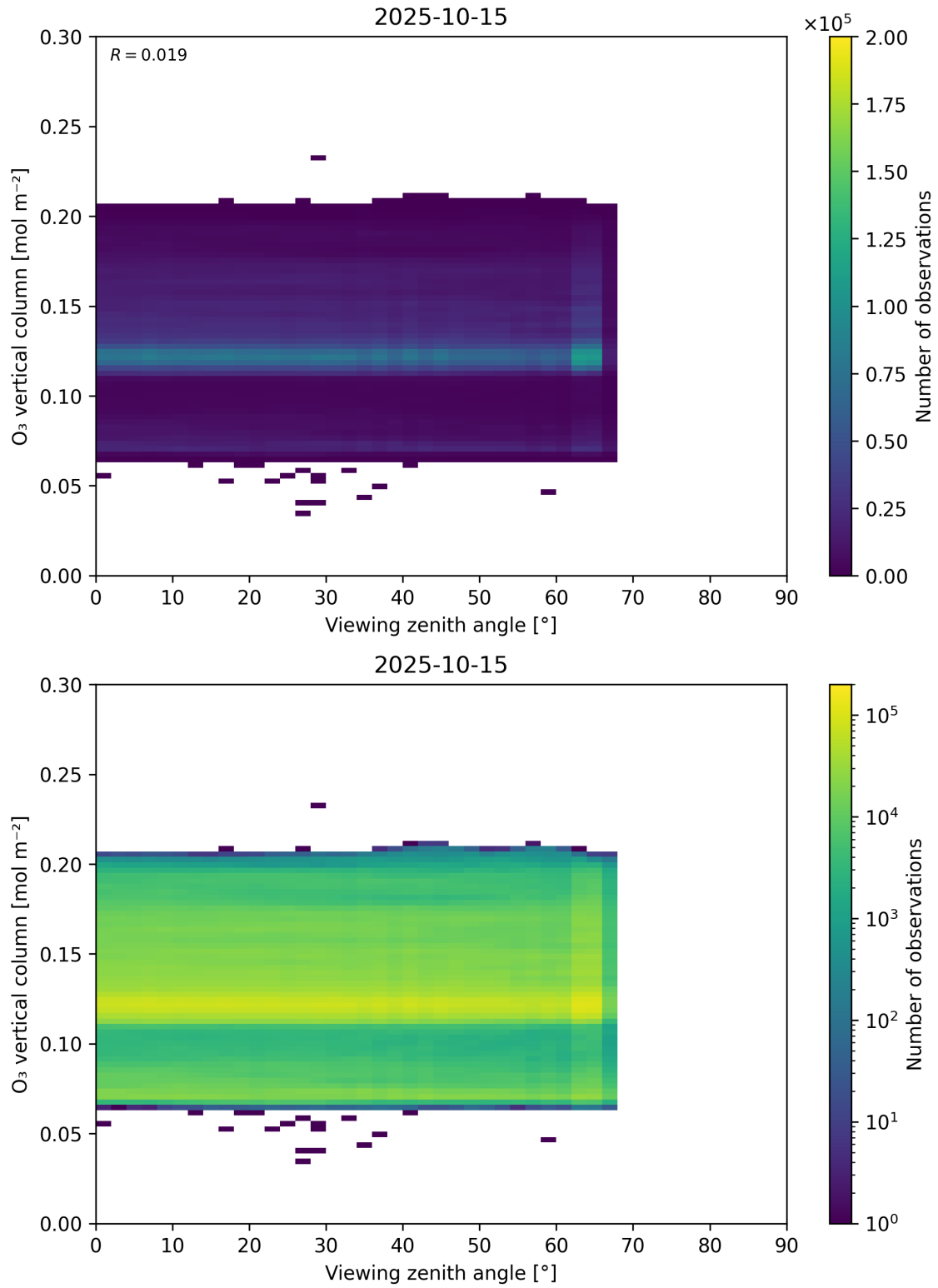
Figure 52: Scatter density plot of “Viewing zenith angle” against “O 3 vertical column” for 2025-10-14 to 2025-10-16.
