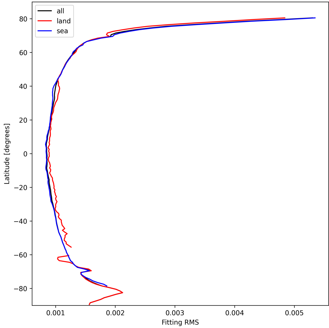
Figure 16: Zonal average of “Fitting RMS” for 2025-10-14 to 2025-10-16.
