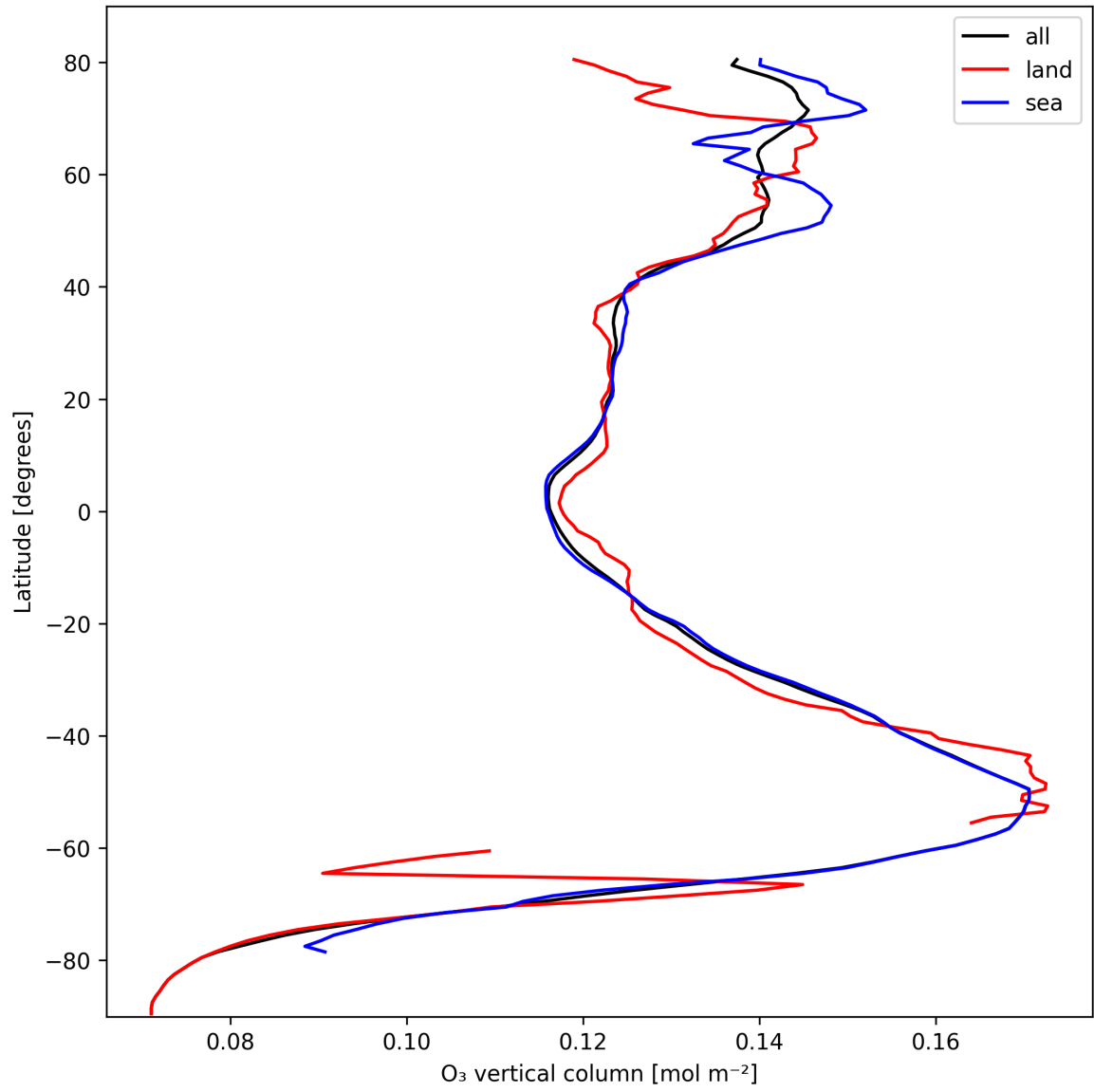
Figure 14: Zonal average of “O 3 vertical column” for 2025-10-14 to 2025-10-16.
