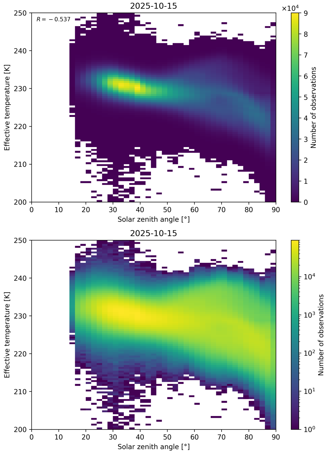
Figure 45: Scatter density plot of “Solar zenith angle” against “Effective temperature” for 2025-10-14 to 2025-10-16.
