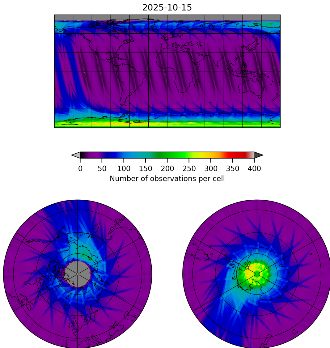
Figure 12: Map of the number of observations for 2025-10-14 to 2025-10-16
