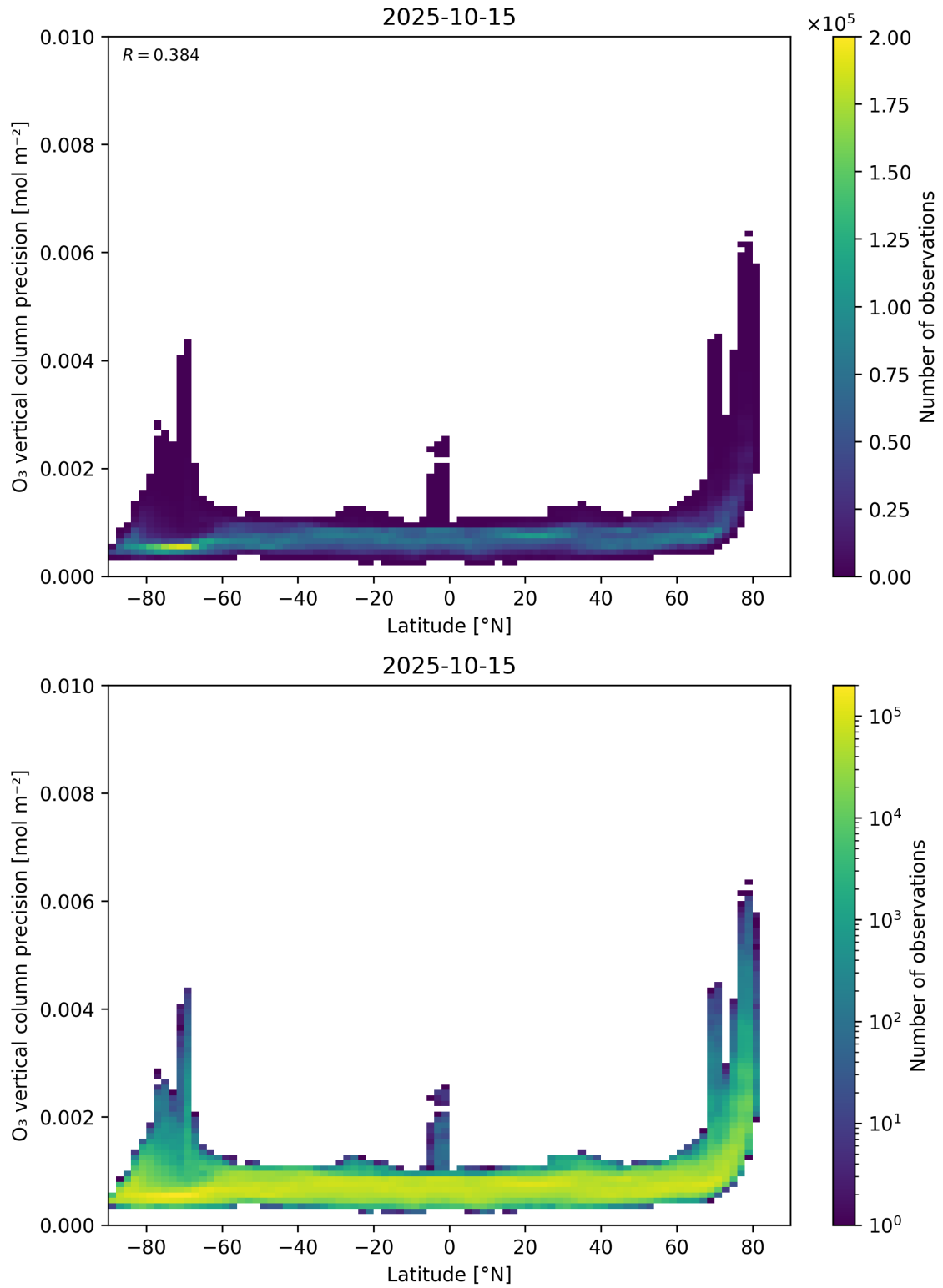
Figure 37: Scatter density plot of “Latitude” against “O 3 vertical column precision” for 2025-10-14 to 2025-10-16.
