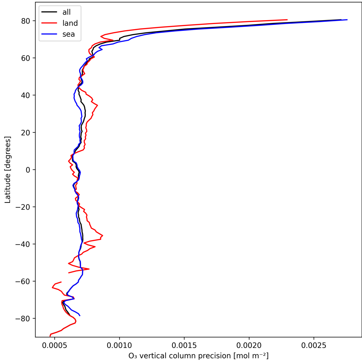
Figure 15: Zonal average of “O 3 vertical column precision” for 2025-10-14 to 2025-10-16.
