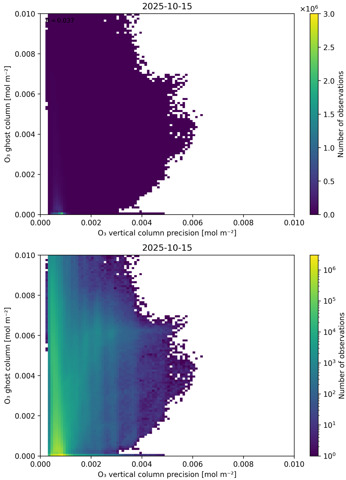
Figure 43: Scatter density plot of “O 3 vertical column precision” against “O 3 ghost column” for 2025-10-14 to 2025-10-16.
