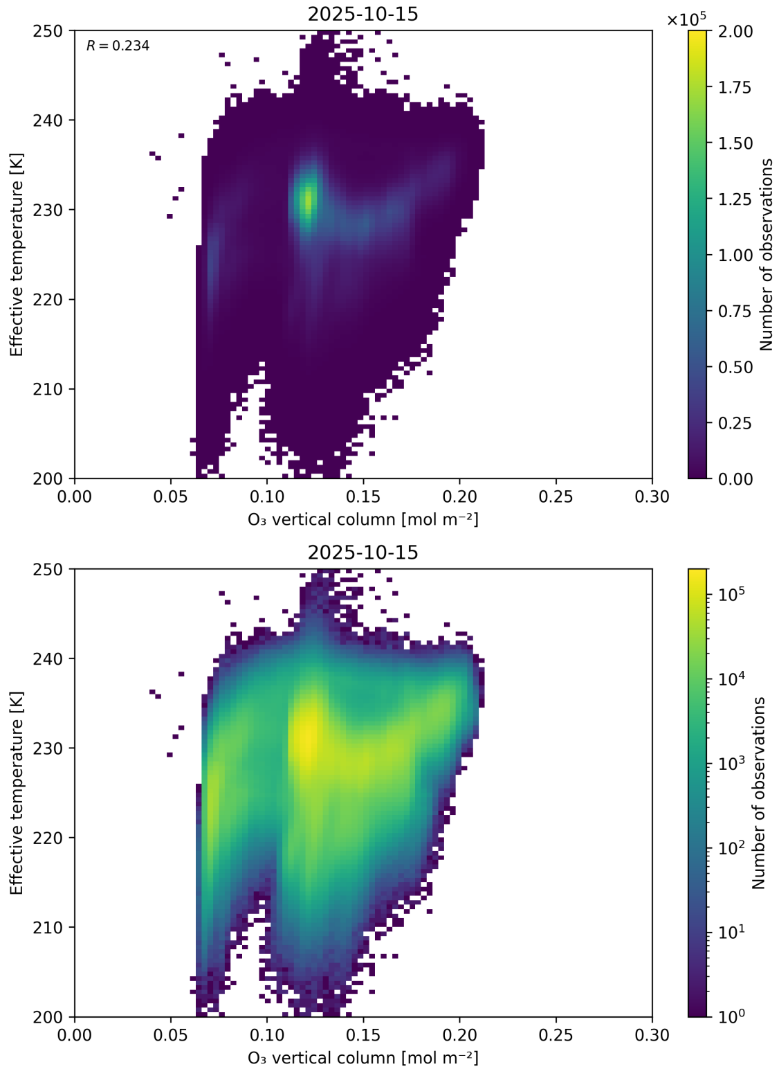
Figure 39: Scatter density plot of “O 3 vertical column” against “Effective temperature” for 2025-10-14 to 2025-10-16.
