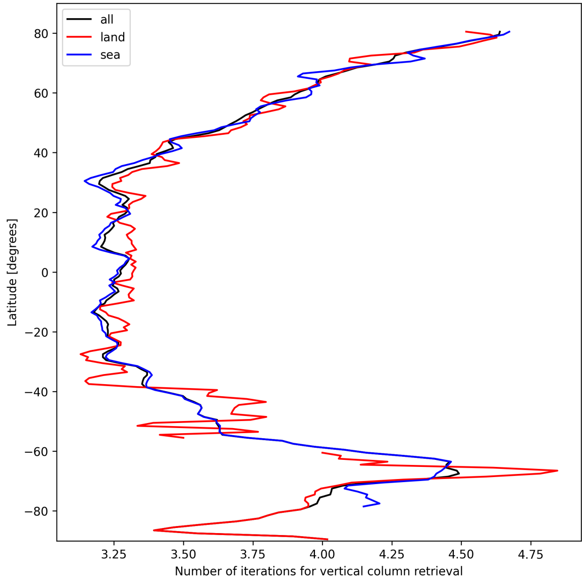
Figure 19: Zonal average of “Number of iterations for vertical column retrieval” for 2025-10-14 to 2025-10-16.
