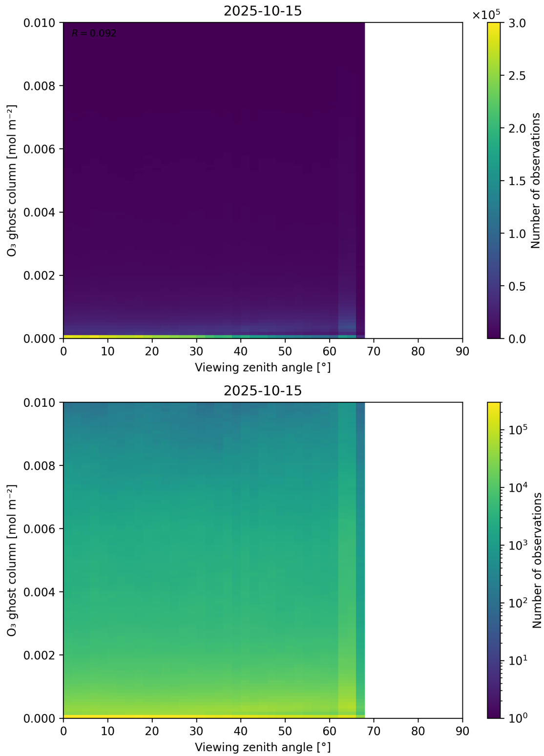
Figure 51: Scatter density plot of “Viewing zenith angle” against “O 3 ghost column” for 2025-10-14 to 2025-10-16.
