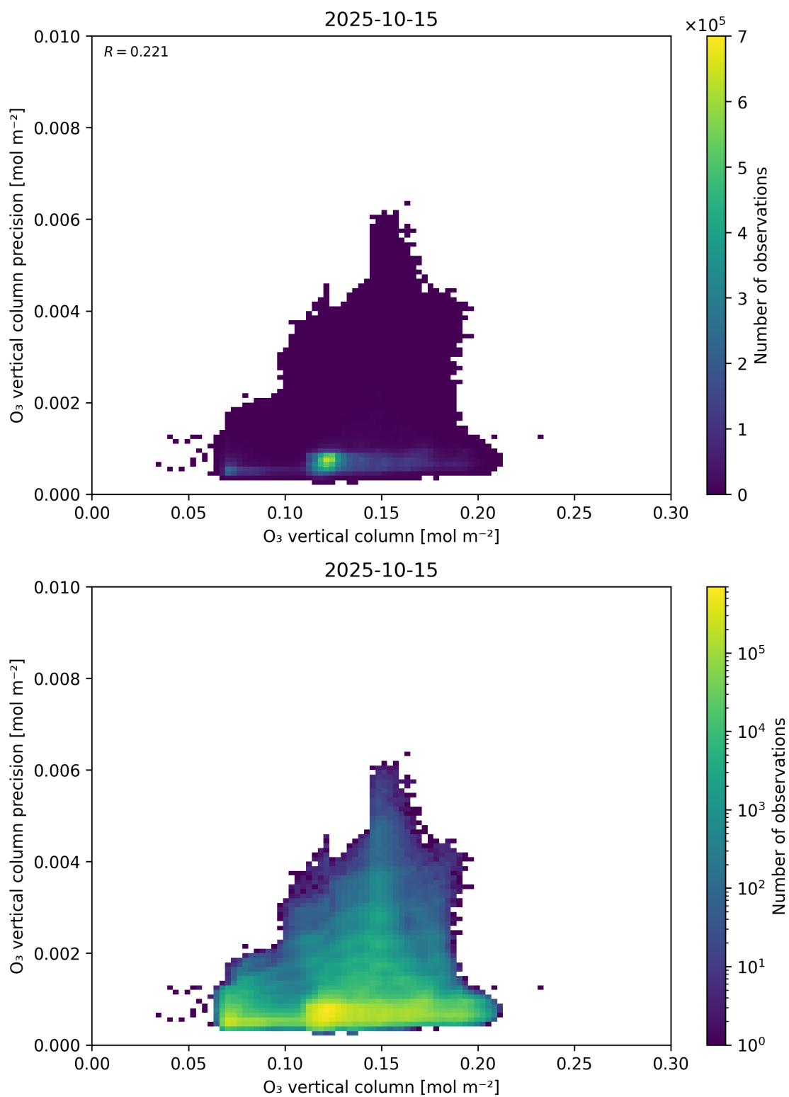
Figure 41: Scatter density plot of “O 3 vertical column” against “O 3 vertical column precision” for 2025-10-14 to 2025-10-16.
