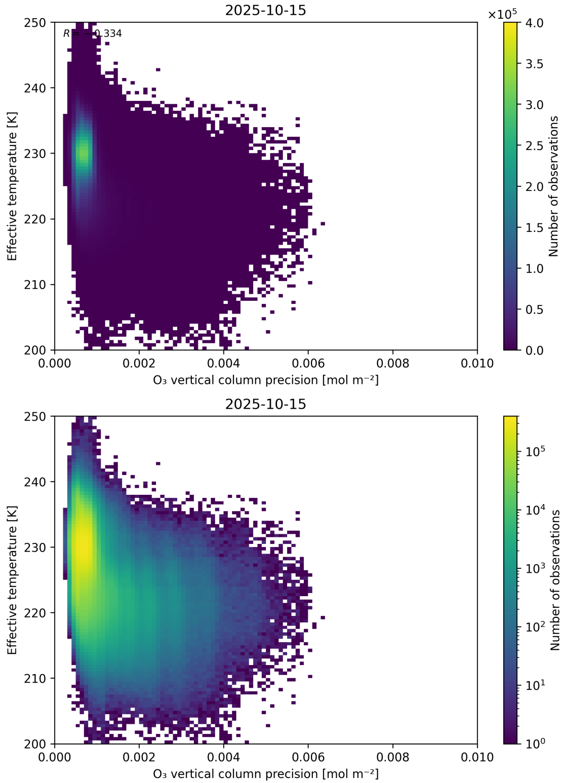
Figure 42: Scatter density plot of “O 3 vertical column precision” against “Effective temperature” for 2025-10-14 to 2025-10-16.
