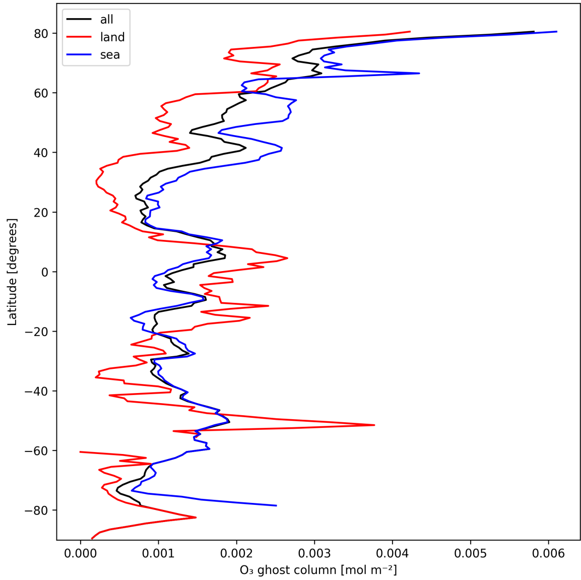
Figure 18: Zonal average of "O 3 ghost column" for 2025-10-14 to 2025-10-16.
