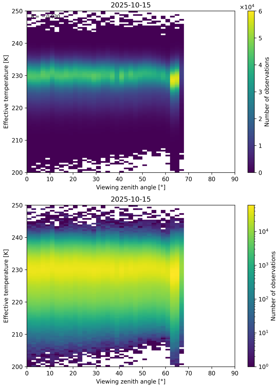
Figure 50: Scatter density plot of “Viewing zenith angle” against “Effective temperature” for 2025-10-14 to 2025-10-16.
