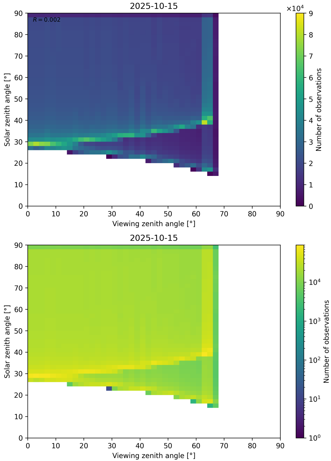
Figure 54: Scatter density plot of “Viewing zenith angle” against “Solar zenith angle” for 2025-10-14 to 2025-10-16.
