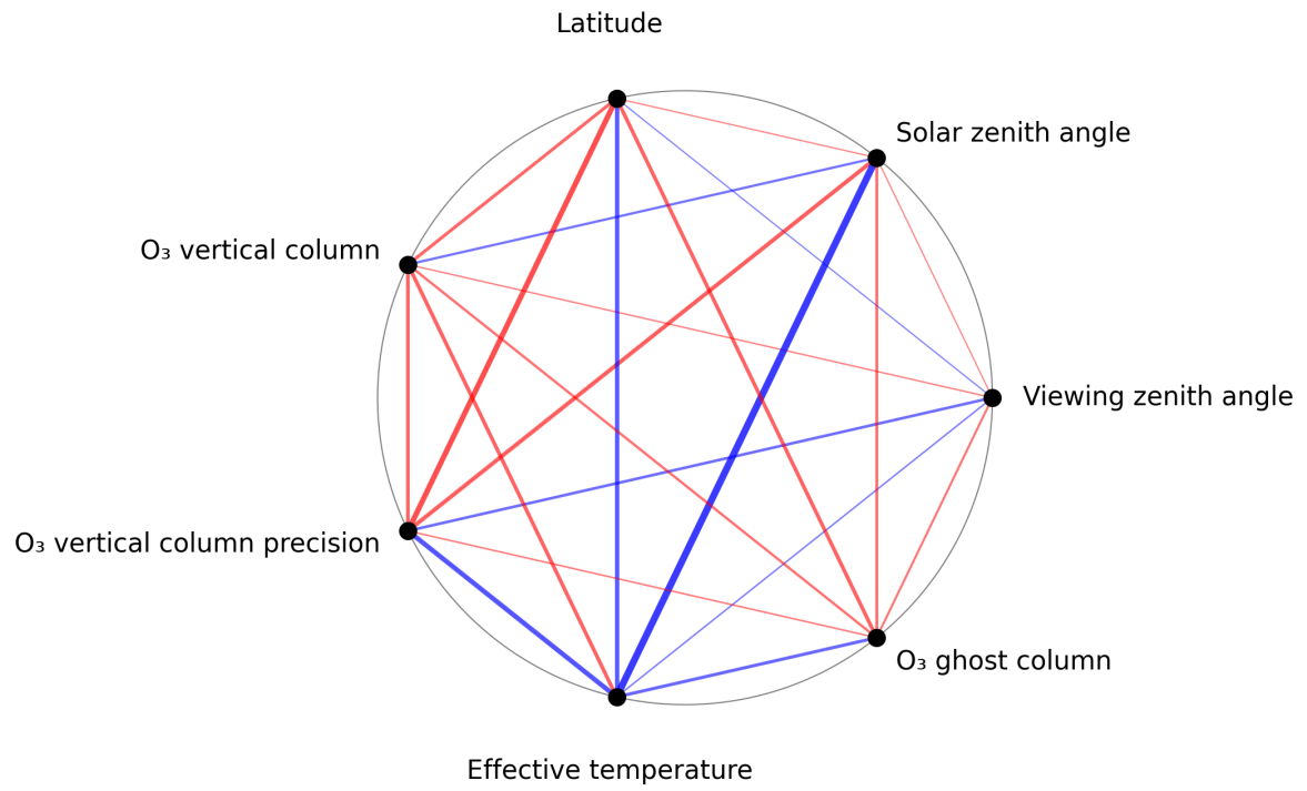
Figure 1: Map of correlation graph for 2025-10-14 to 2025-10-16.
