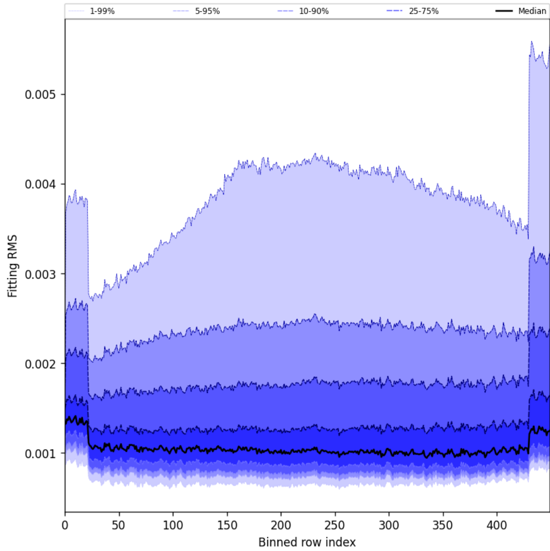
Figure 30: Along track statistics of “Fitting RMS” for 2025-10-14 to 2025-10-16
