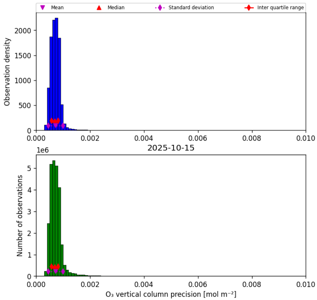
Figure 22: Histogram of “O 3 vertical column precision” for 2025-10-14 to 2025-10-16
