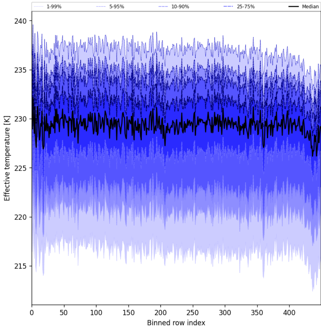
Figure 31: Along track statistics of “Effective temperature” for 2025-10-14 to 2025-10-16
