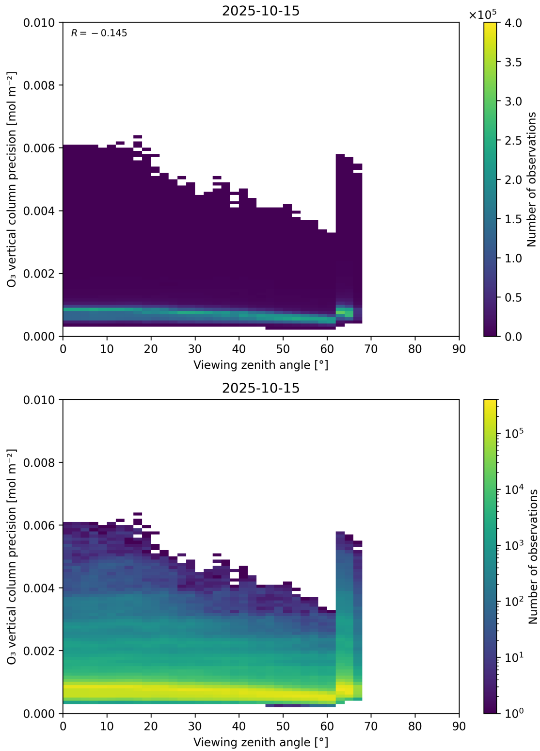
Figure 53: Scatter density plot of “Viewing zenith angle” against “O 3 vertical column precision” for 2025-10-14 to 2025-10-16.
