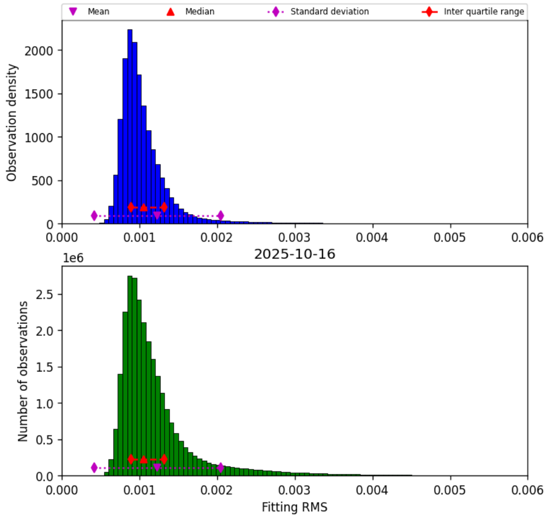
Figure 23: Histogram of “Fitting RMS” for 2025-10-15 to 2025-10-17
