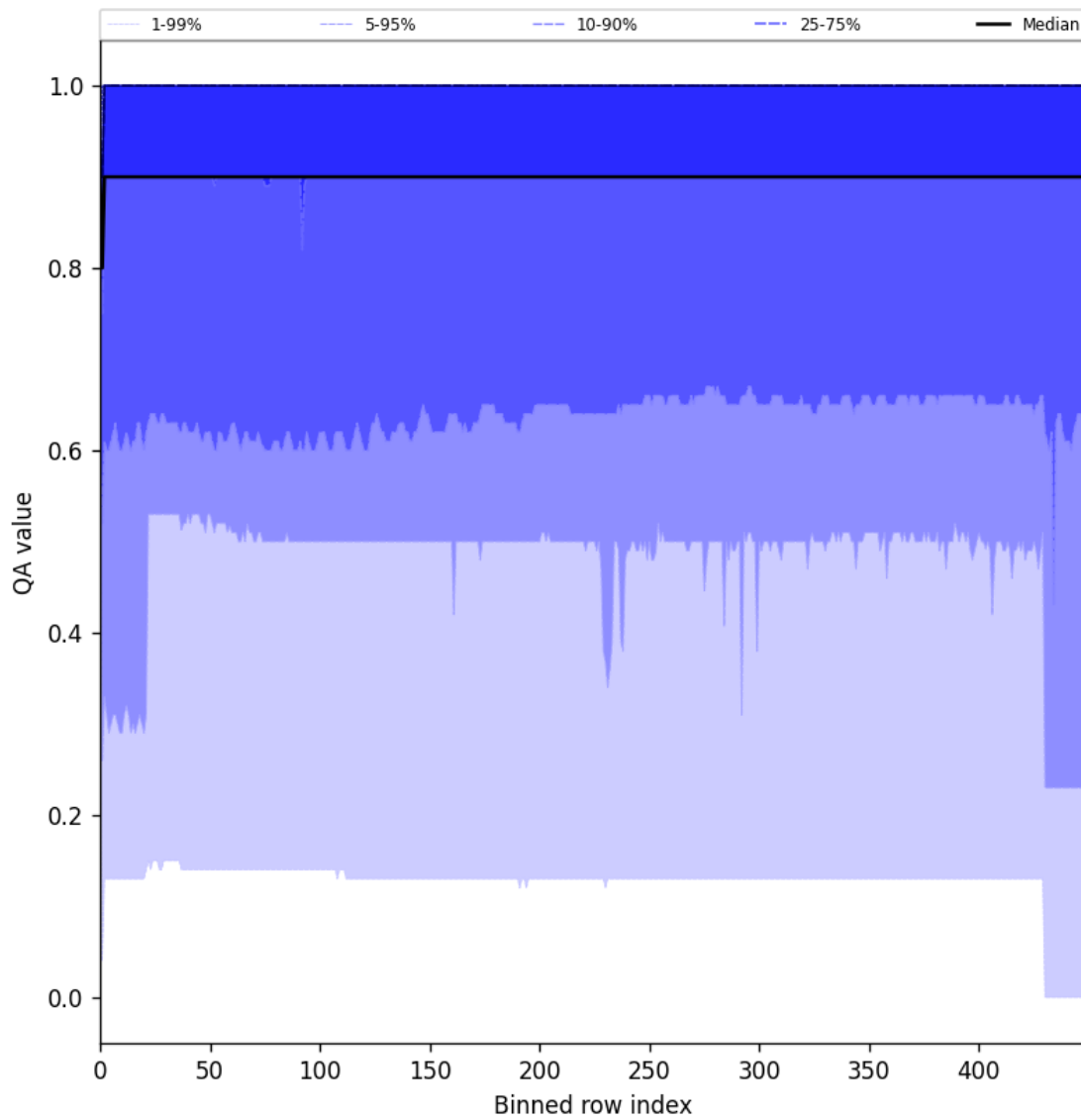
Figure 27: Along track statistics of “QA value” for 2025-10-15 to 2025-10-17
