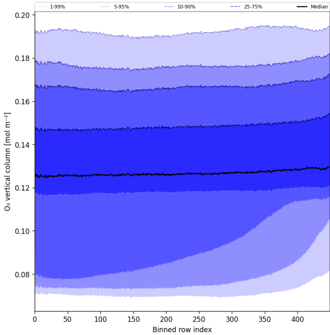
Figure 28: Along track statistics of “O 3 vertical column” for 2025-10-15 to 2025-10-17
