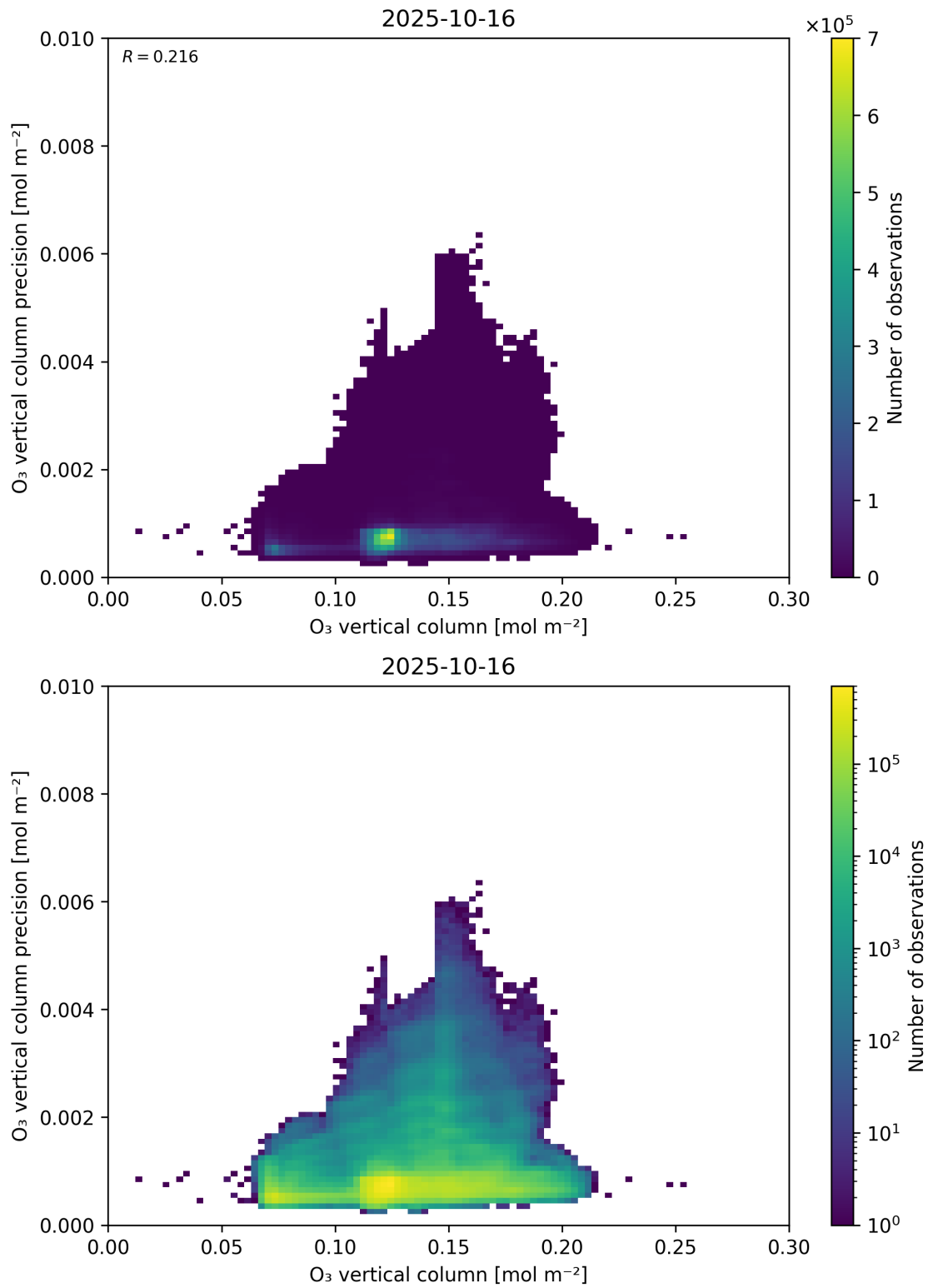
Figure 41: Scatter density plot of “O 3 vertical column” against “O 3 vertical column precision” for 2025-10-15 to 2025-10-17.
