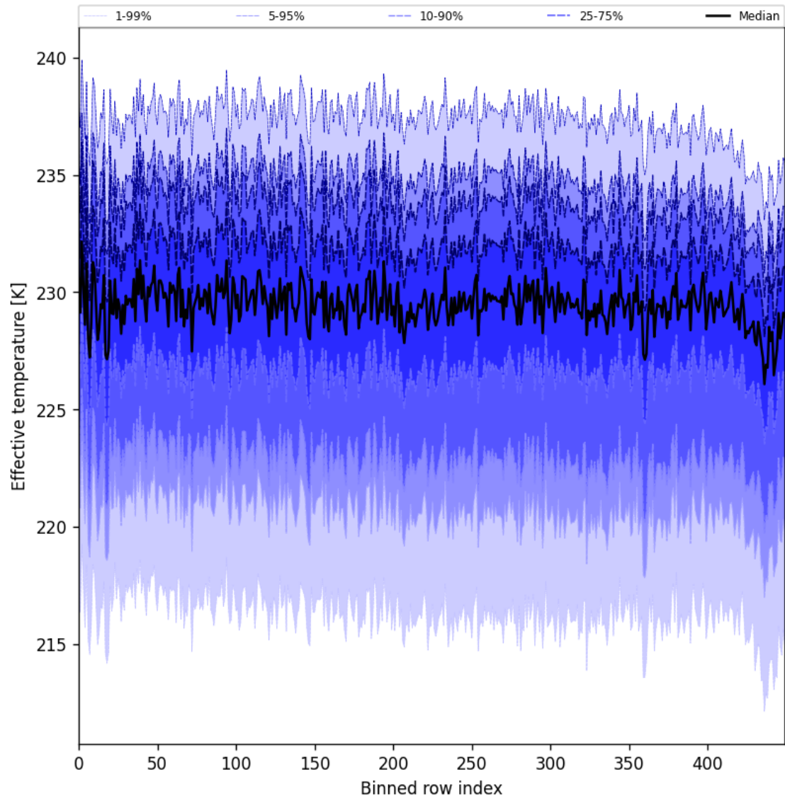
Figure 31: Along track statistics of “Effective temperature” for 2025-10-15 to 2025-10-17
