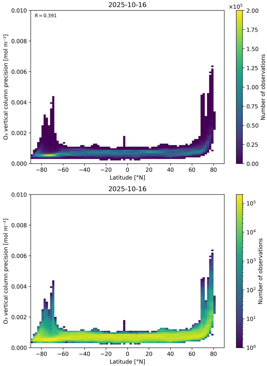
Figure 37: Scatter density plot of “Latitude” against “O 3 vertical column precision” for 2025-10-15 to 2025-10-17.
