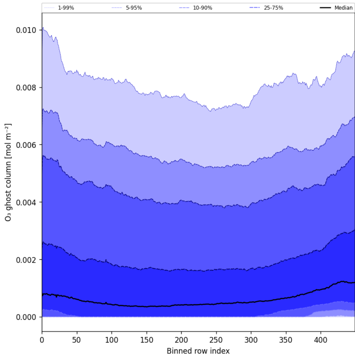
Figure 32: Along track statistics of "O 3 ghost column" for 2025-10-15 to 2025-10-17
