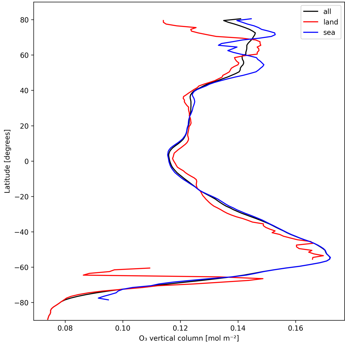
Figure 14: Zonal average of “O 3 vertical column” for 2025-10-15 to 2025-10-17.
