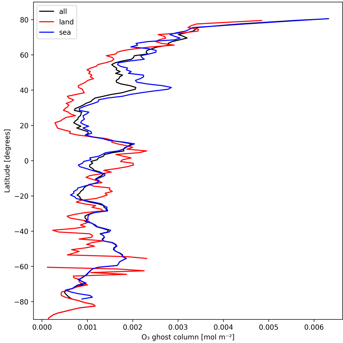
Figure 18: Zonal average of "O 3 ghost column" for 2025-10-15 to 2025-10-17.
