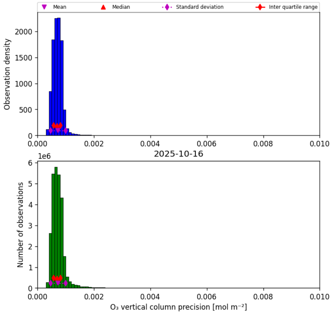
Figure 22: Histogram of “O 3 vertical column precision” for 2025-10-15 to 2025-10-17
