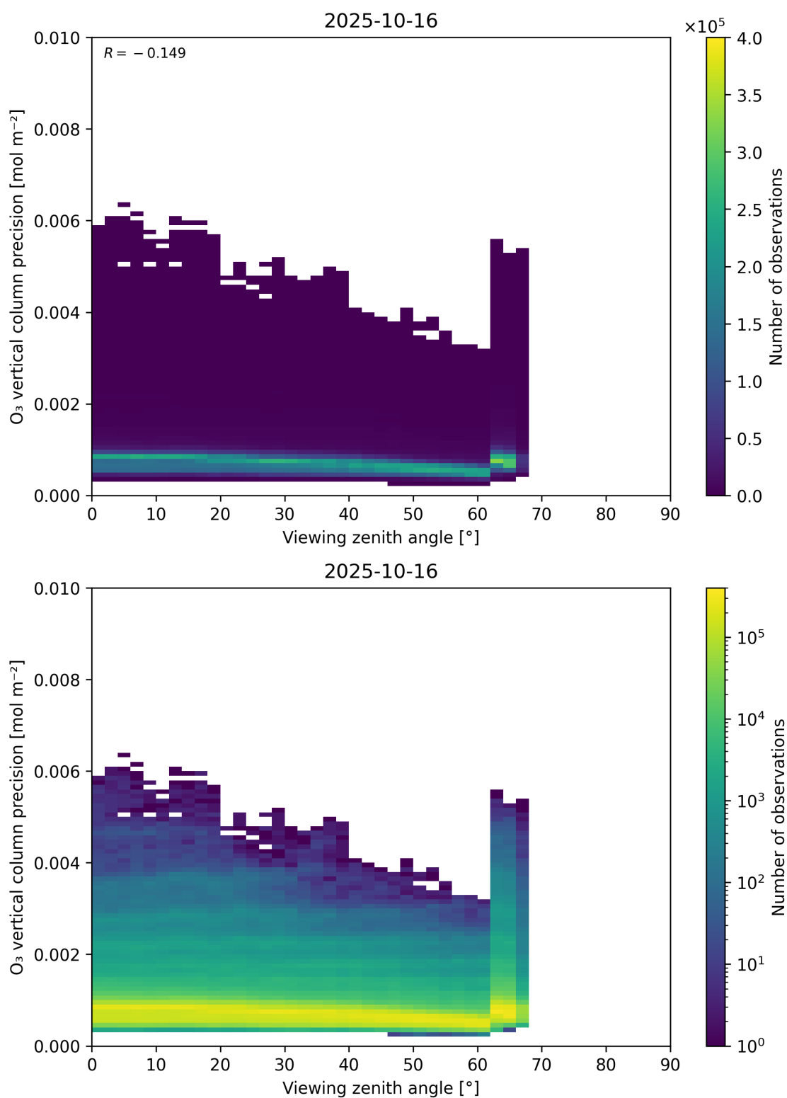
Figure 53: Scatter density plot of “Viewing zenith angle” against “O 3 vertical column precision” for 2025-10-15 to 2025-10-17.
