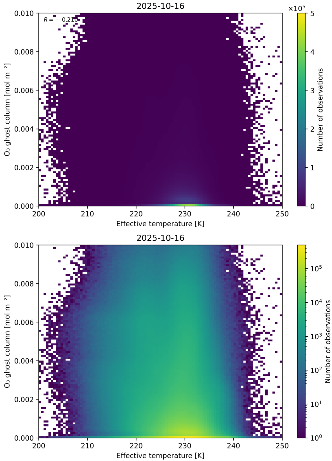
Figure 38: Scatter density plot of “Effective temperature” against “O 3 ghost column” for 2025-10-15 to 2025-10-17.
