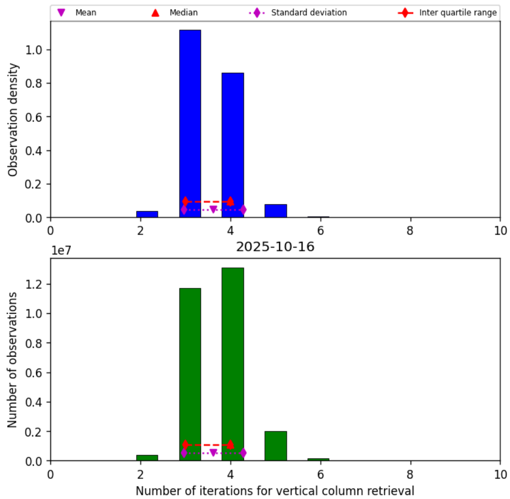
Figure 26: Histogram of “Number of iterations for vertical column retrieval” for 2025-10-15 to 2025-10-17
