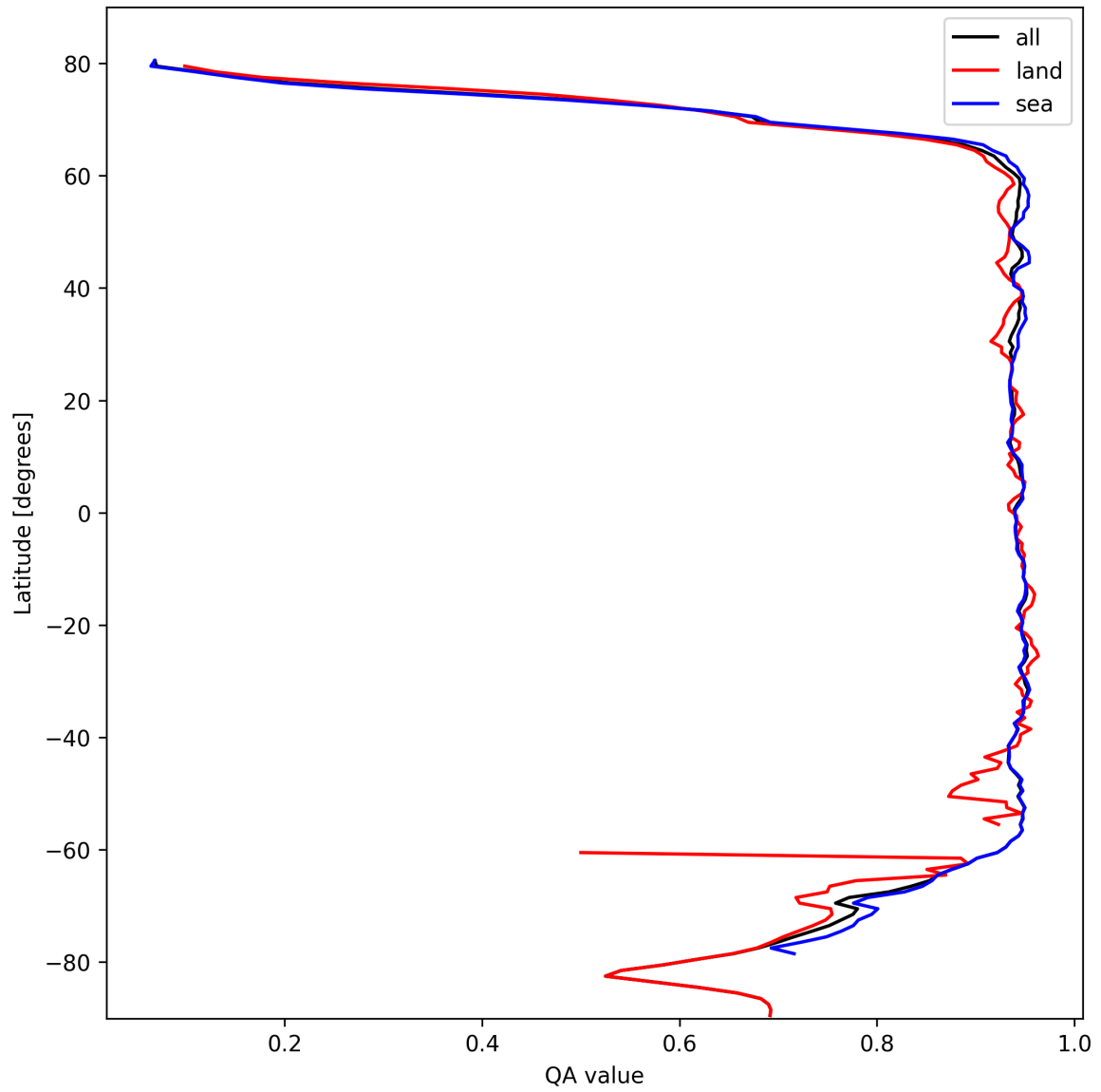
Figure 13: Zonal average of “QA value” for 2025-10-15 to 2025-10-17.
