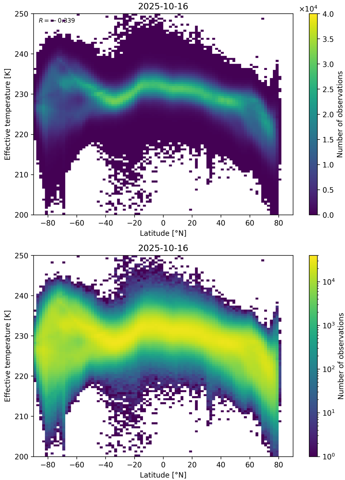
Figure 34: Scatter density plot of “Latitude” against “Effective temperature” for 2025-10-15 to 2025-10-17.
