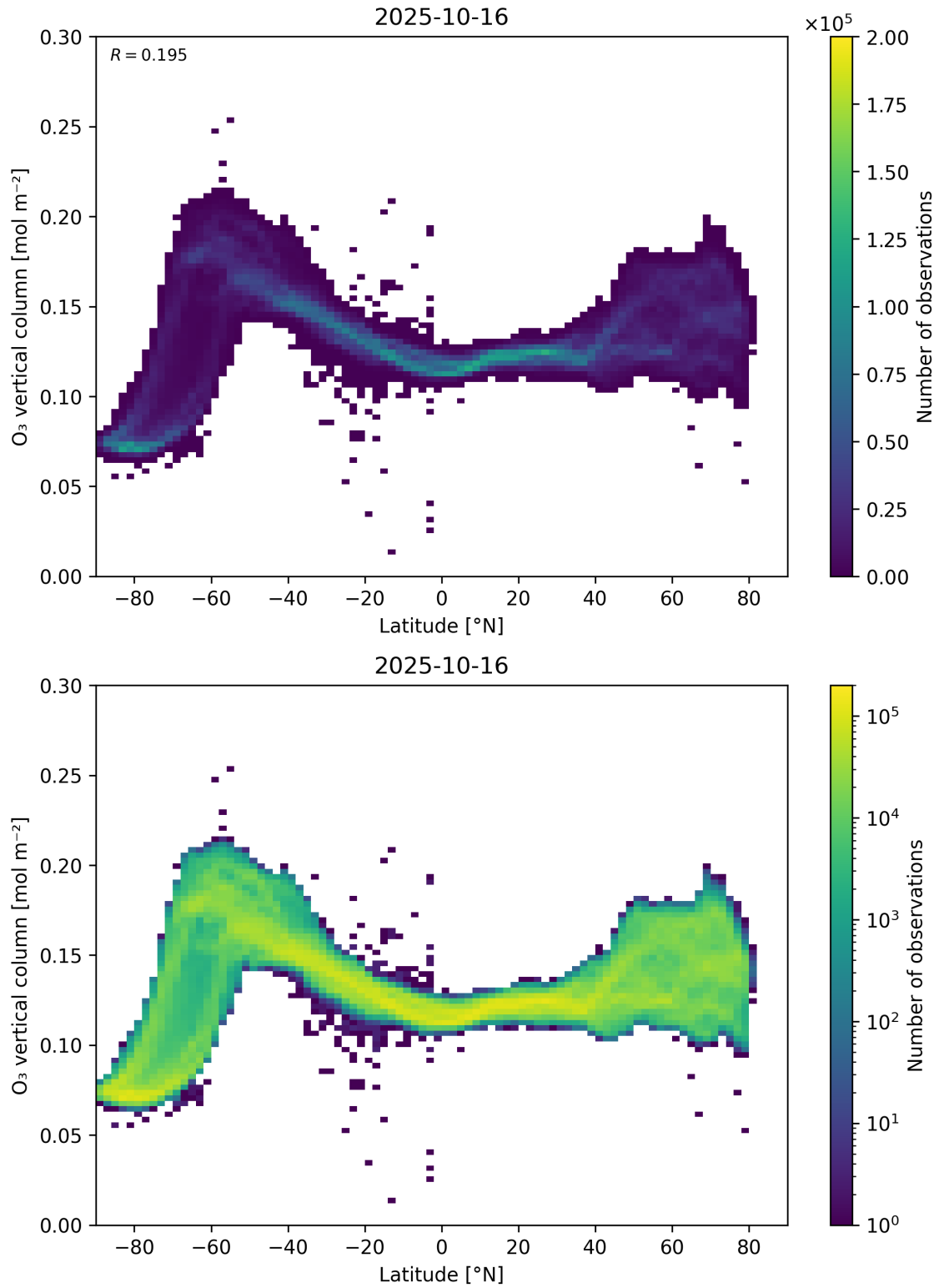
Figure 36: Scatter density plot of “Latitude” against “O 3 vertical column” for 2025-10-15 to 2025-10-17.
