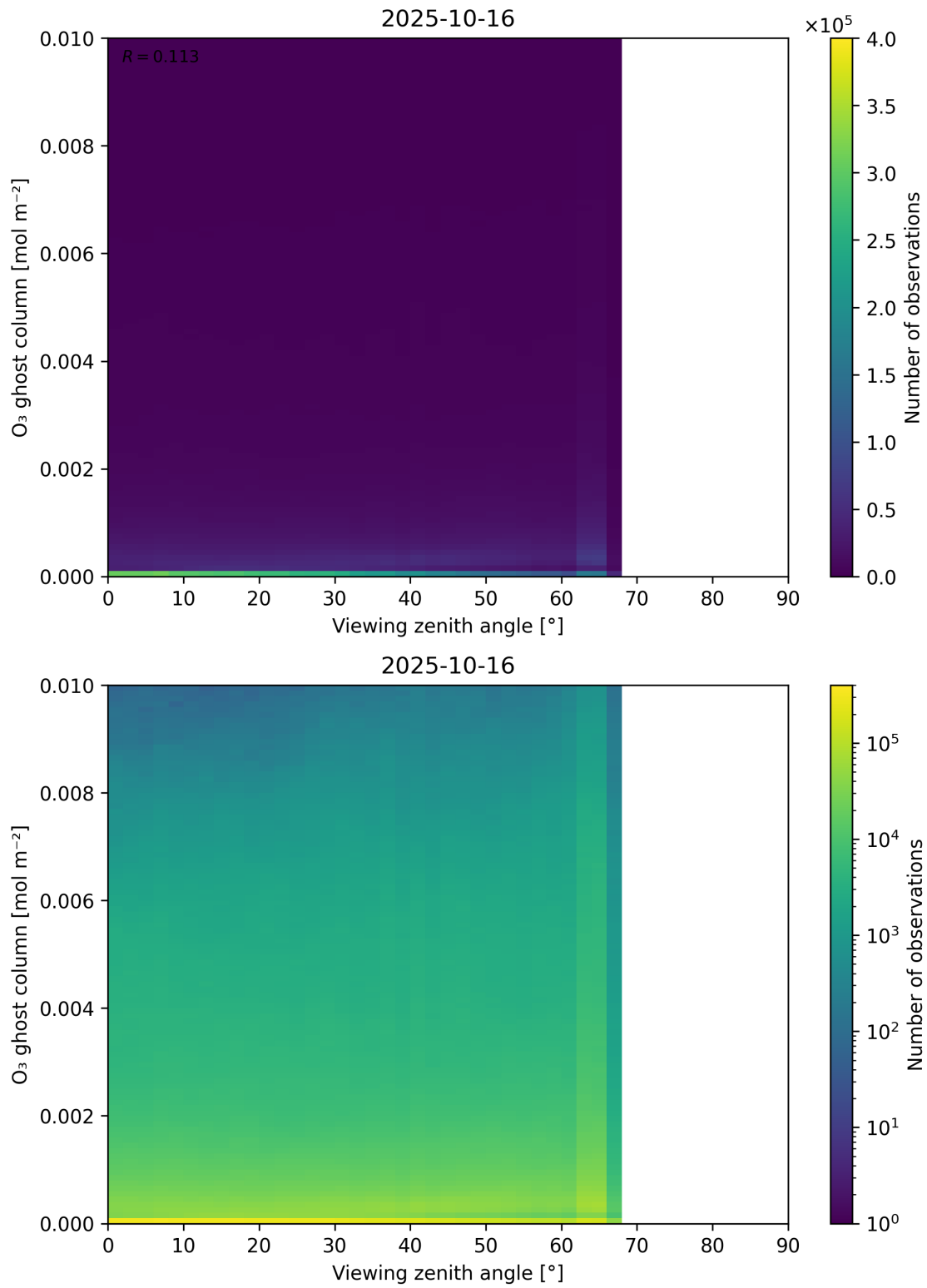
Figure 51: Scatter density plot of “Viewing zenith angle” against “O 3 ghost column” for 2025-10-15 to 2025-10-17.
