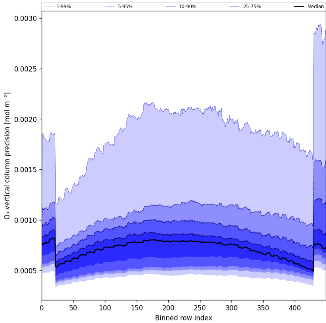
Figure 29: Along track statistics of “O 3 vertical column precision” for 2025-10-15 to 2025-10-17
