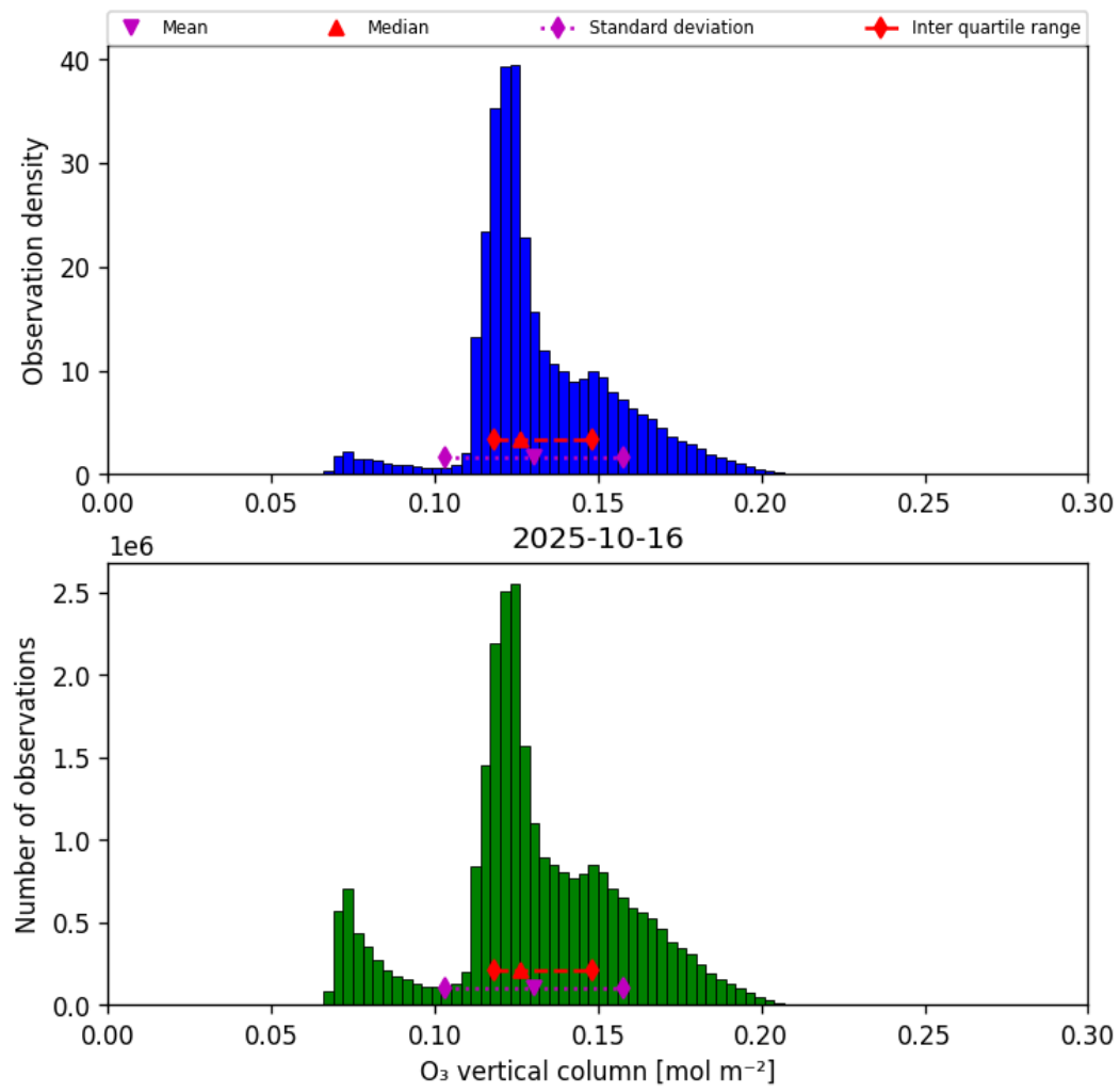
Figure 21: Histogram of “O 3 vertical column” for 2025-10-15 to 2025-10-17
