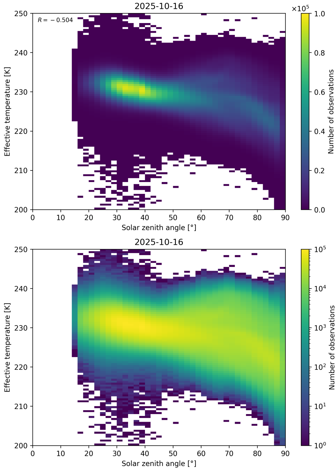
Figure 45: Scatter density plot of “Solar zenith angle” against “Effective temperature” for 2025-10-15 to 2025-10-17.
