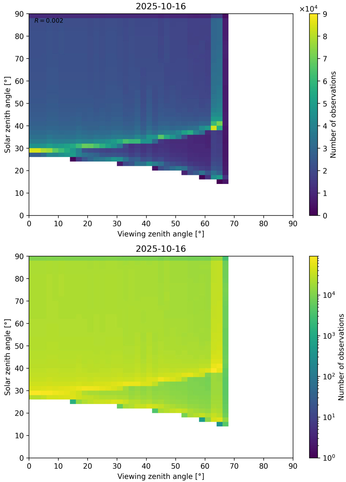
Figure 54: Scatter density plot of “Viewing zenith angle” against “Solar zenith angle” for 2025-10-15 to 2025-10-17.
