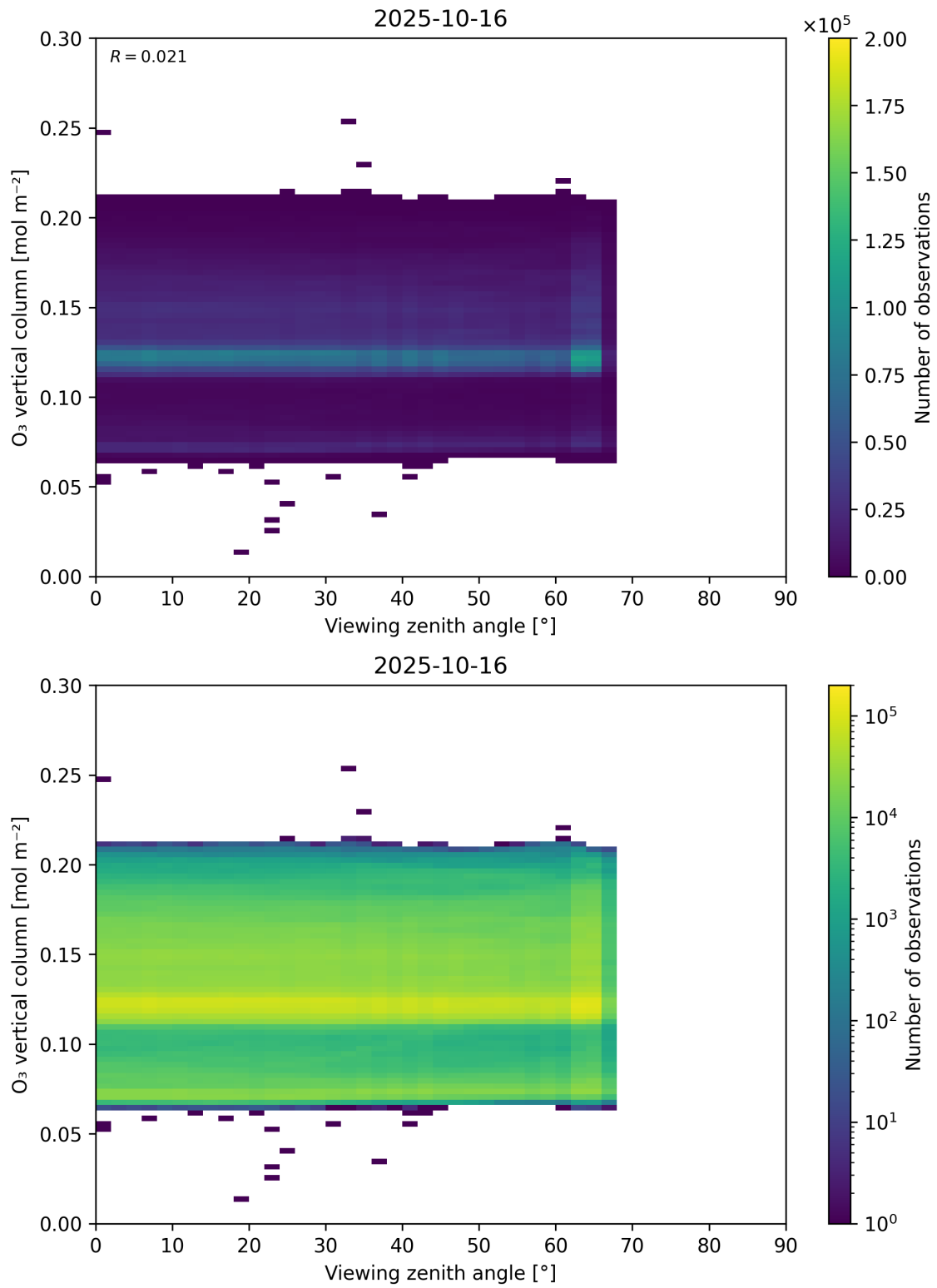
Figure 52: Scatter density plot of “Viewing zenith angle” against “O 3 vertical column” for 2025-10-15 to 2025-10-17.
