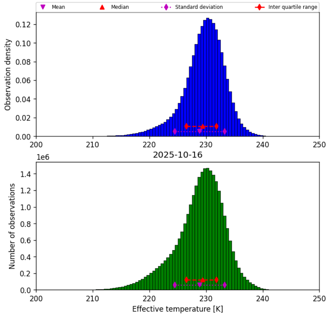
Figure 24: Histogram of “Effective temperature” for 2025-10-15 to 2025-10-17
