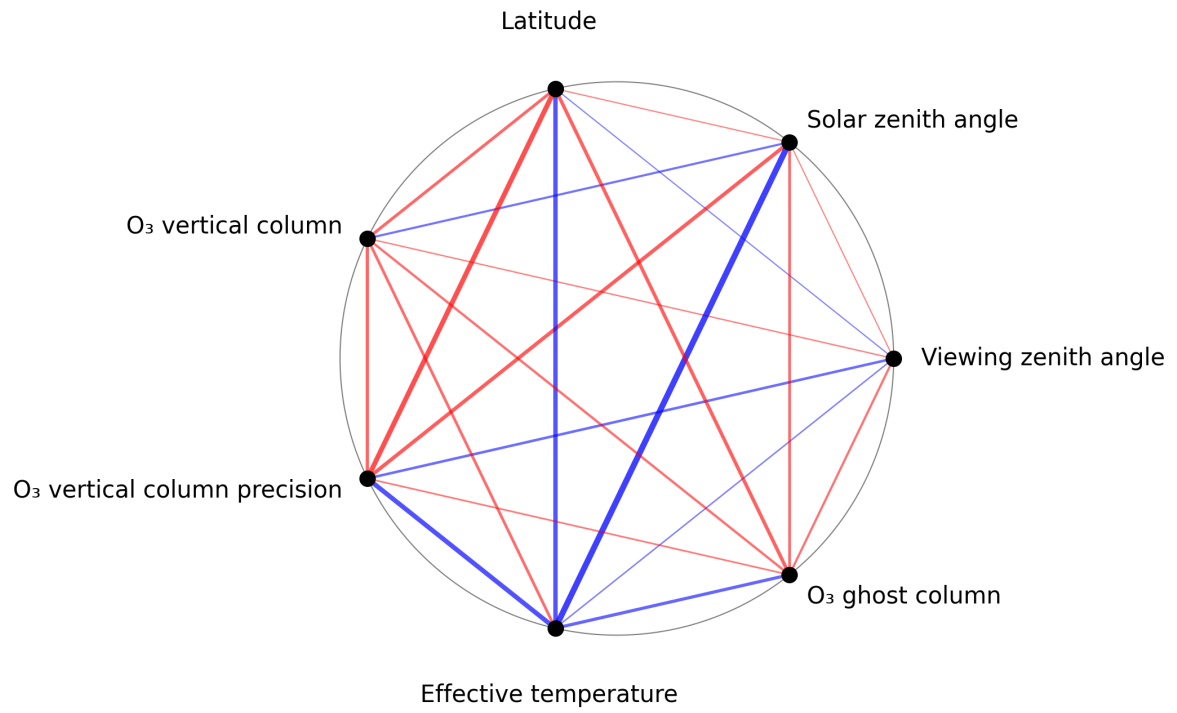
Figure 1: Map of correlation graph for 2025-10-15 to 2025-10-17.
