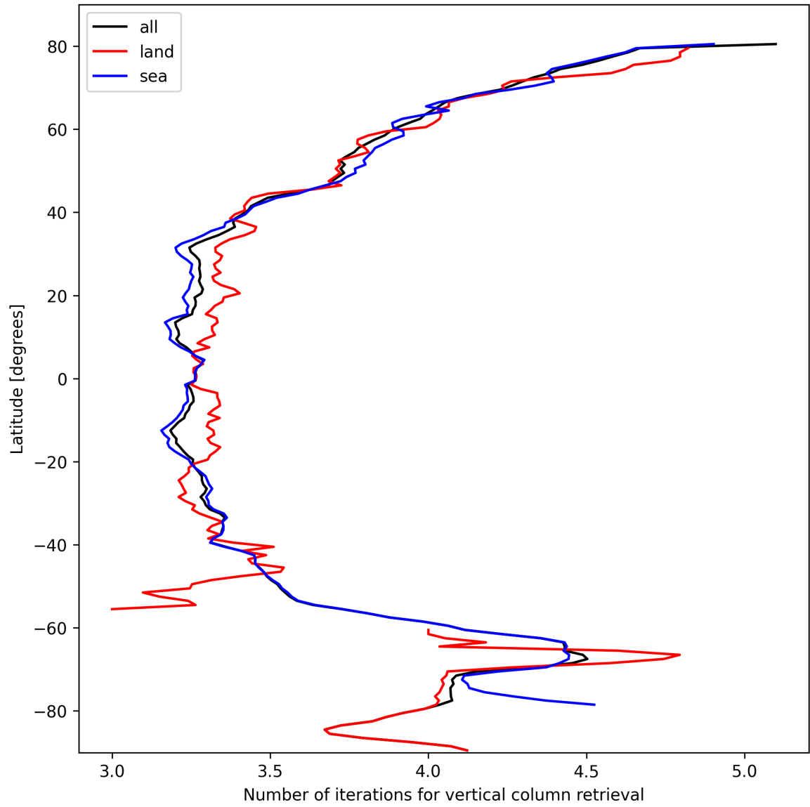
Figure 19: Zonal average of “Number of iterations for vertical column retrieval” for 2025-10-15 to 2025-10-17.
