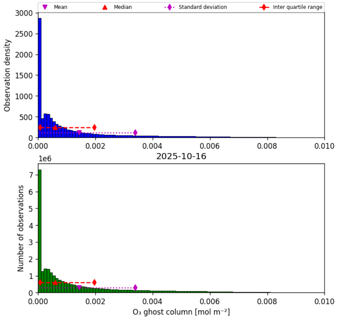
Figure 25: Histogram of “O 3 ghost column” for 2025-10-15 to 2025-10-17
