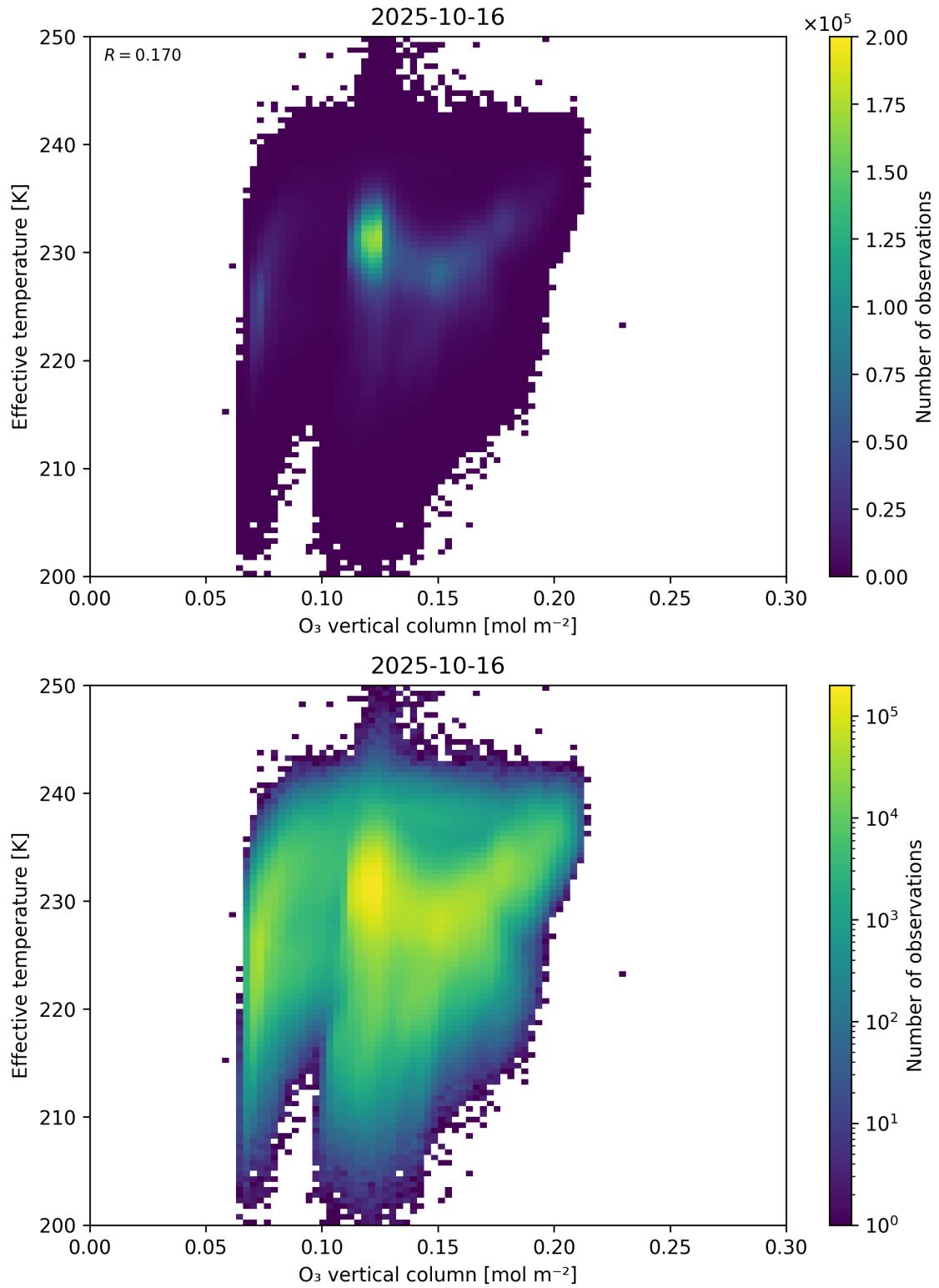
Figure 39: Scatter density plot of “O 3 vertical column” against “Effective temperature” for 2025-10-15 to 2025-10-17.
