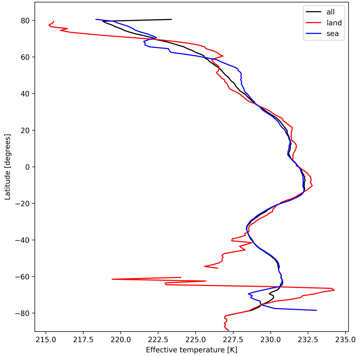
Figure 17: Zonal average of “Effective temperature” for 2025-10-15 to 2025-10-17.
