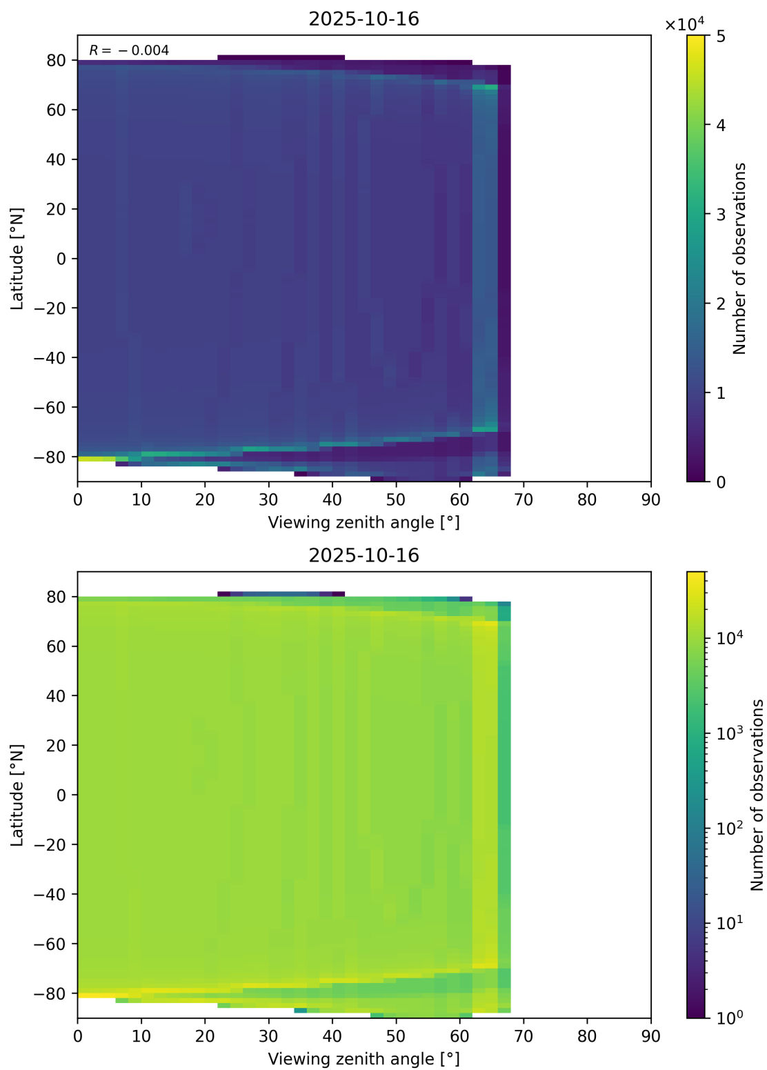
Figure 49: Scatter density plot of “Viewing zenith angle” against “Latitude” for 2025-10-15 to 2025-10-17.
