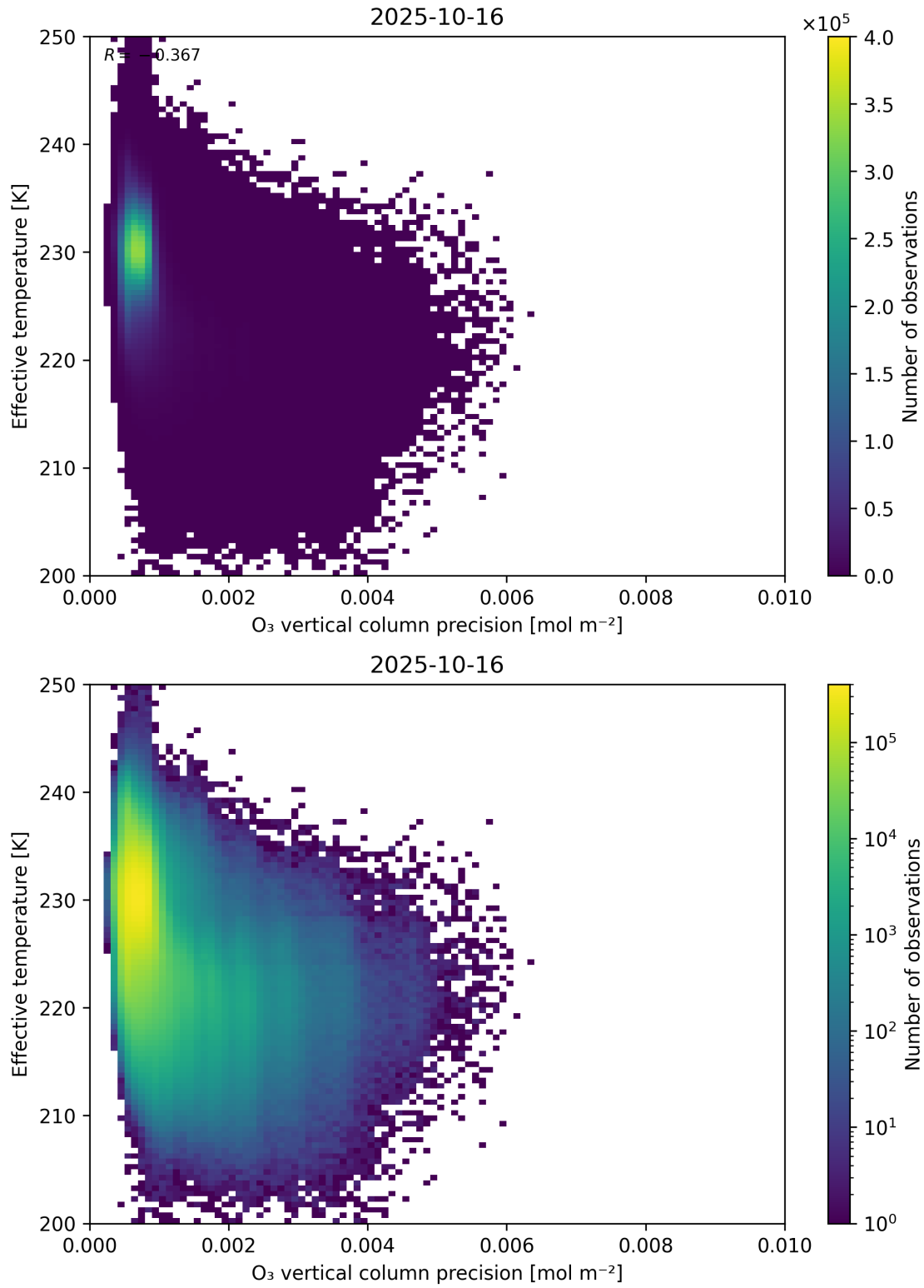
Figure 42: Scatter density plot of “ O_3 vertical column precision” against “Effective temperature” for 2025-10-15 to 2025-10-17.
