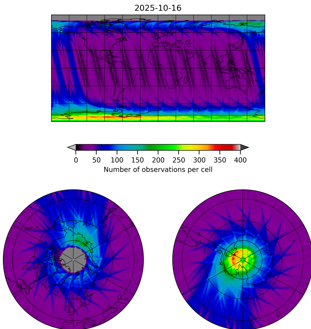
Figure 12: Map of the number of observations for 2025-10-15 to 2025-10-17
