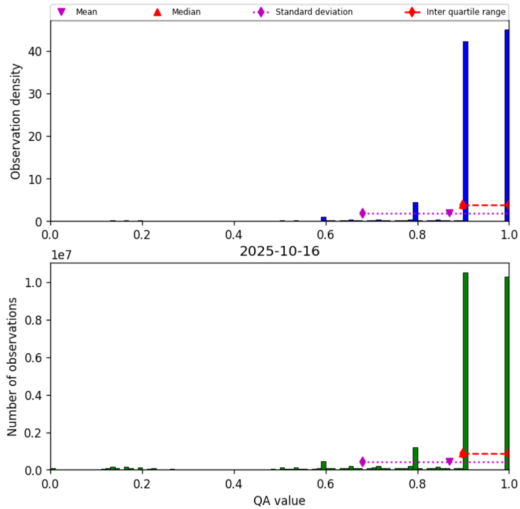
Figure 20: Histogram of “QA value” for 2025-10-15 to 2025-10-17
