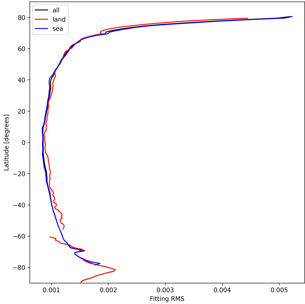
Figure 16: Zonal average of “Fitting RMS” for 2025-10-15 to 2025-10-17.
