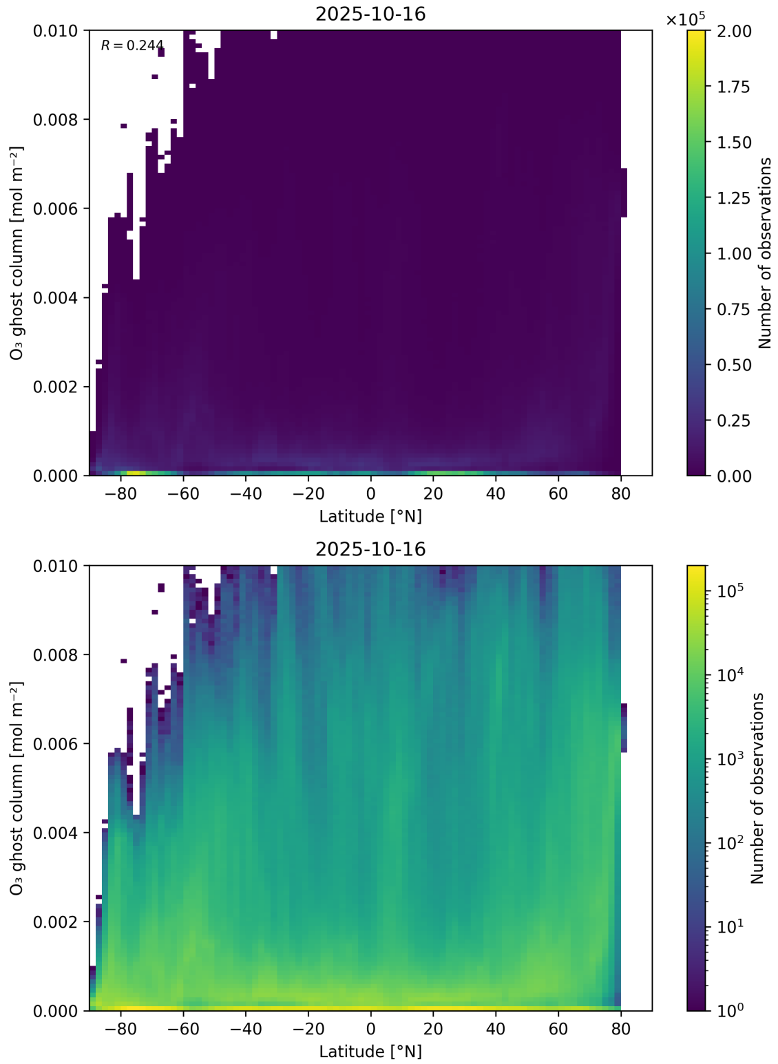
Figure 35: Scatter density plot of “Latitude” against “O 3 ghost column” for 2025-10-15 to 2025-10-17.
