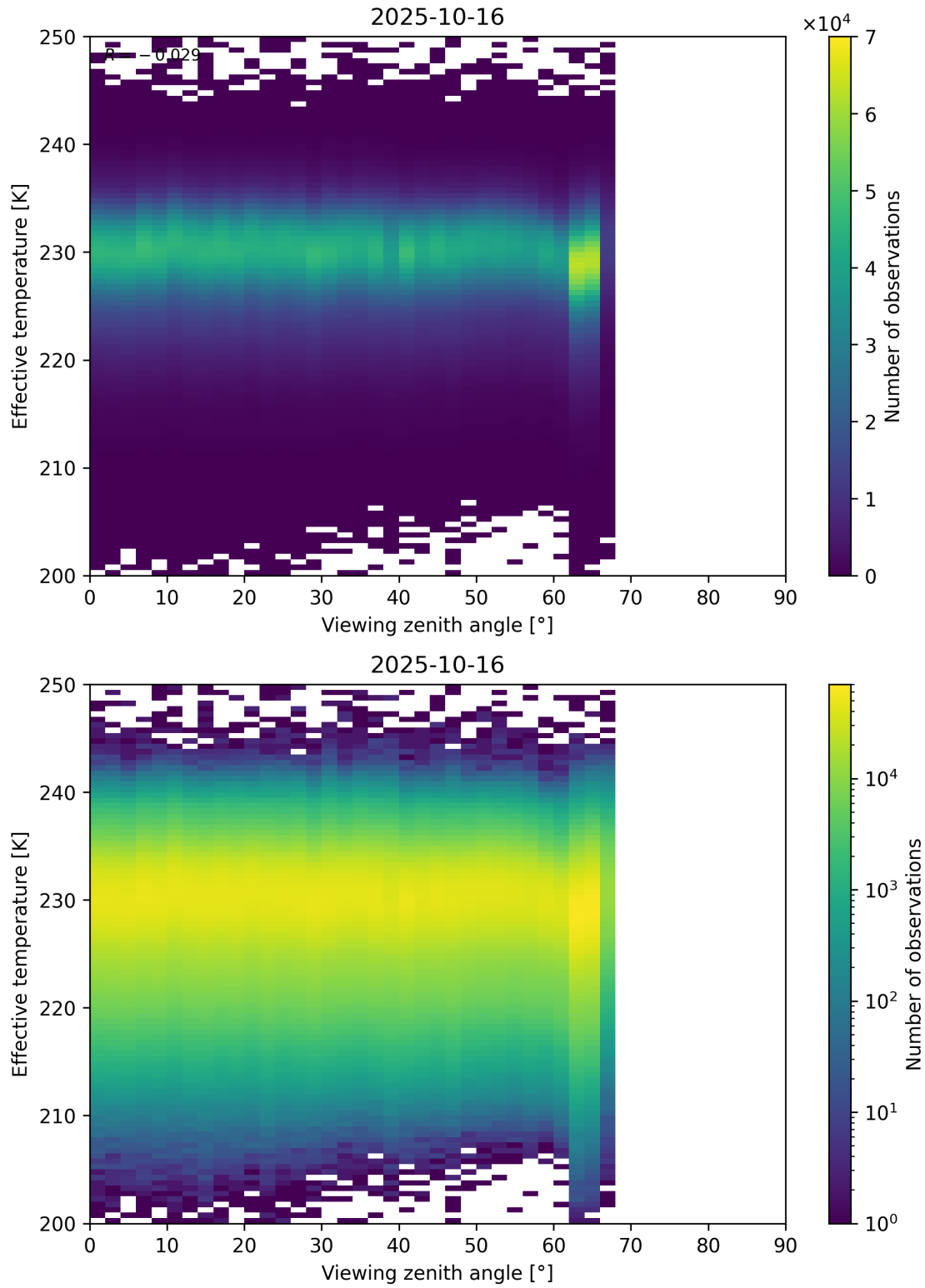
Figure 50: Scatter density plot of “Viewing zenith angle” against “Effective temperature” for 2025-10-15 to 2025-10-17.
