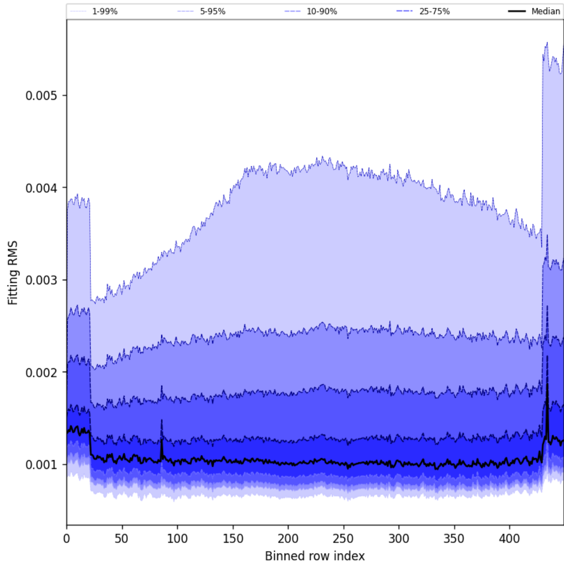
Figure 30: Along track statistics of “Fitting RMS” for 2025-10-15 to 2025-10-17
