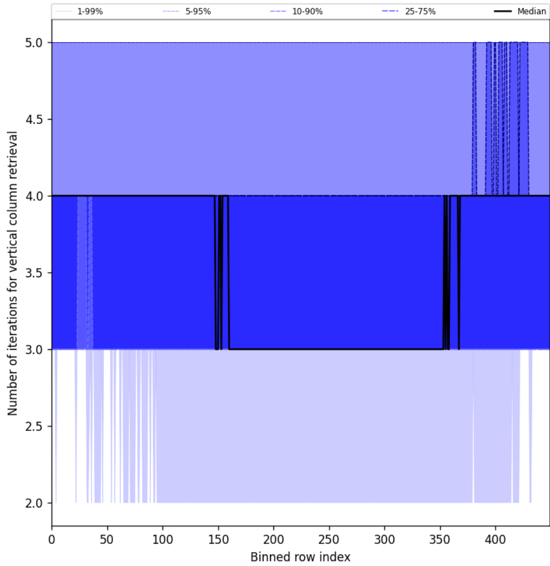
Figure 33: Along track statistics of “Number of iterations for vertical column retrieval” for 2025-10-15 to 2025-10-17
