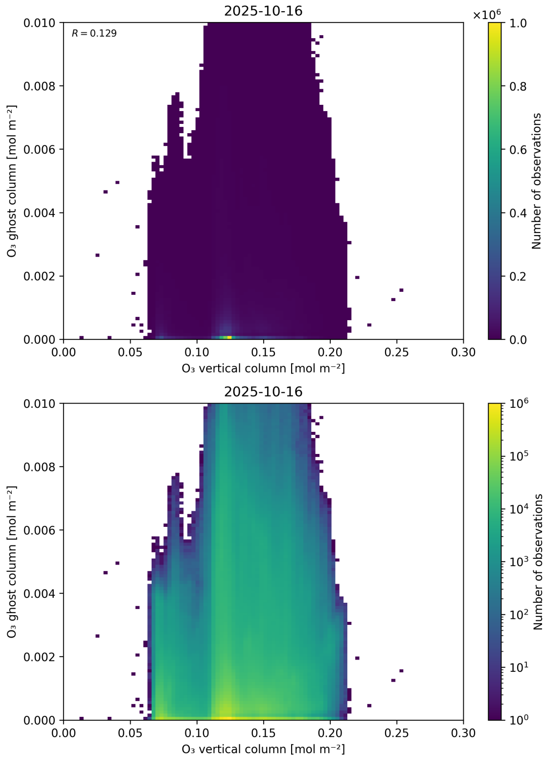
Figure 40: Scatter density plot of “O 3 vertical column” against “O 3 ghost column” for 2025-10-15 to 2025-10-17.
