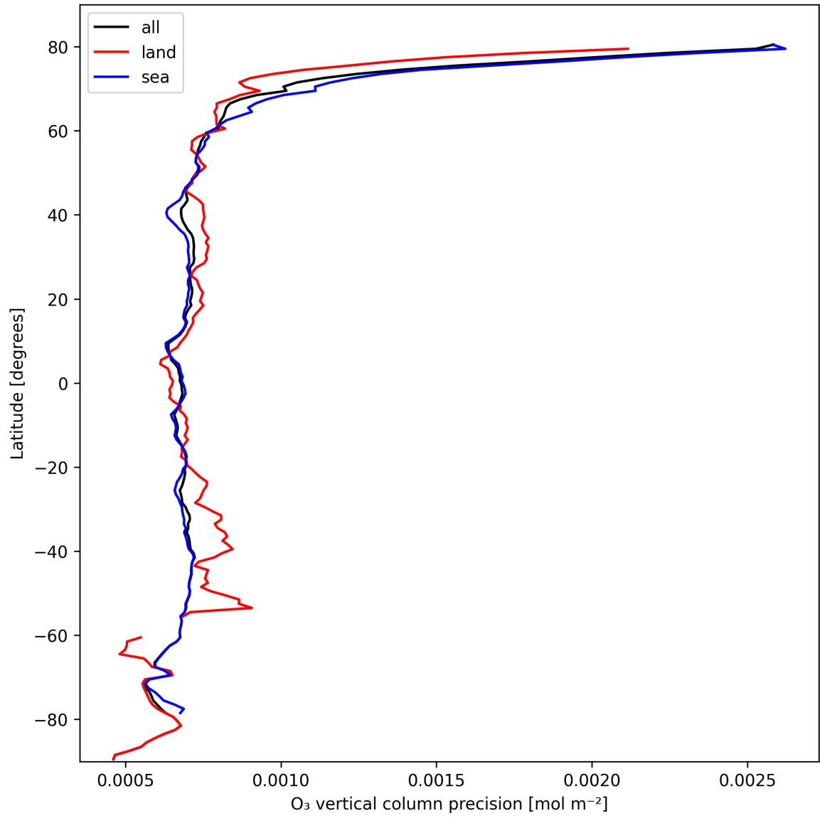
Figure 15: Zonal average of “O 3 vertical column precision” for 2025-10-15 to 2025-10-17.
