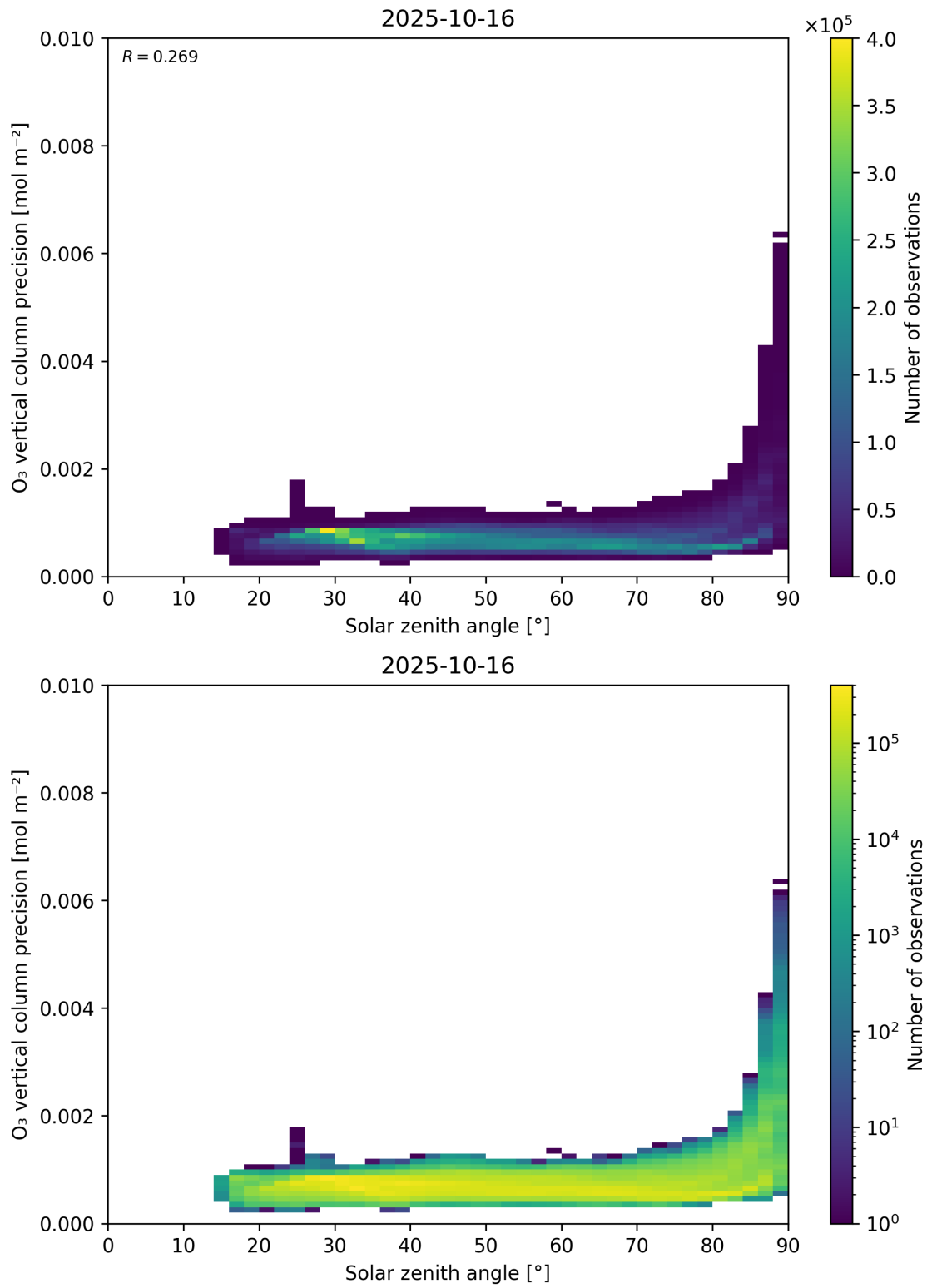
Figure 48: Scatter density plot of “Solar zenith angle” against “O 3 vertical column precision” for 2025-10-15 to 2025-10-17.
