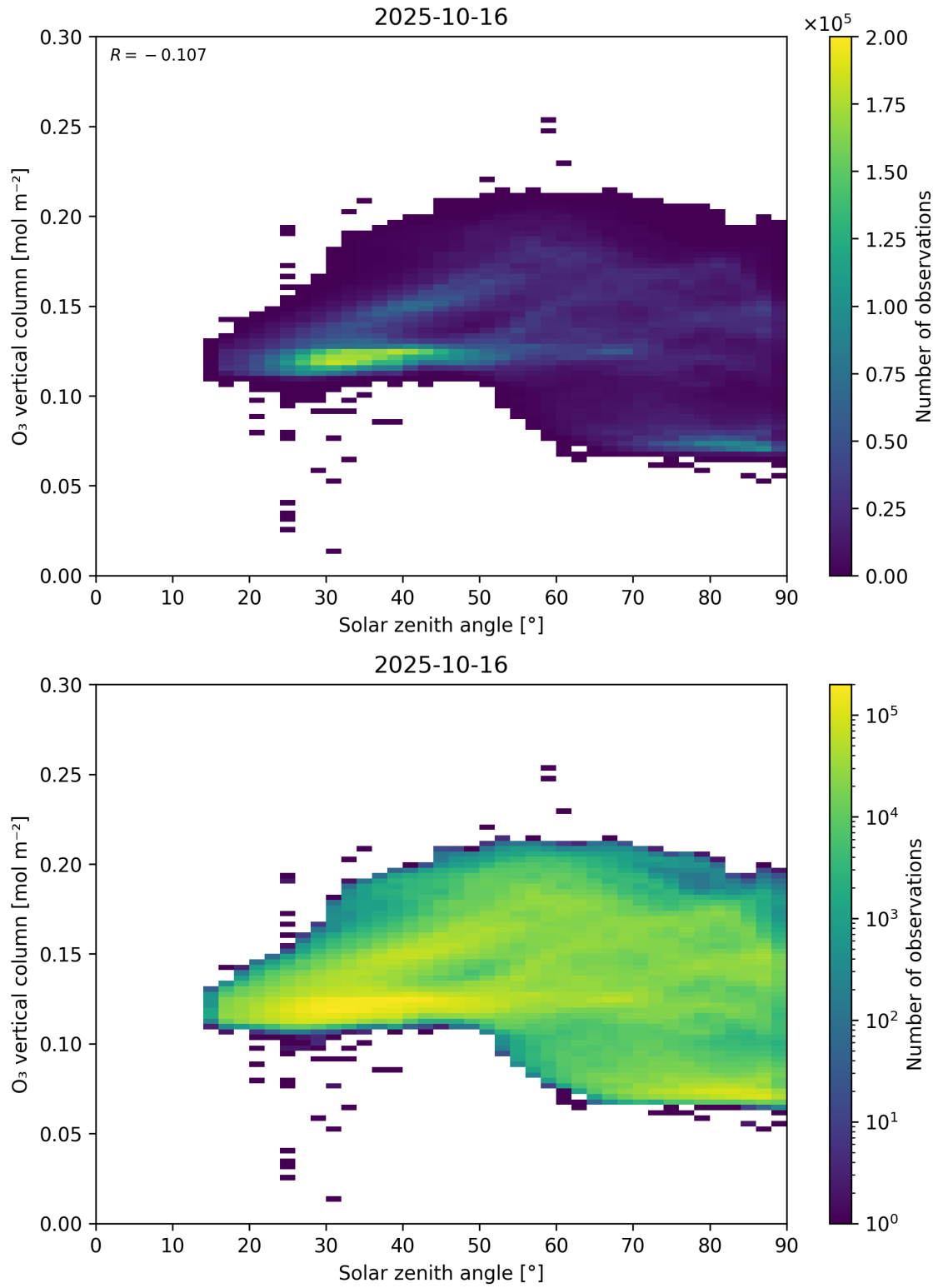
Figure 47: Scatter density plot of “Solar zenith angle” against “O 3 vertical column” for 2025-10-15 to 2025-10-17.
