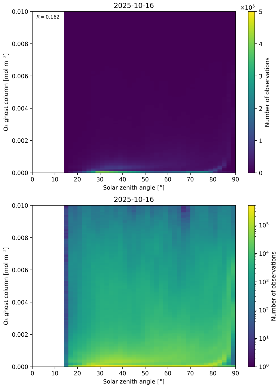
Figure 46: Scatter density plot of “Solar zenith angle” against “O 3 ghost column” for 2025-10-15 to 2025-10-17.
