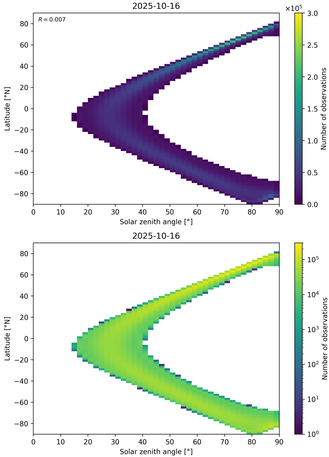
Figure 44: Scatter density plot of “Solar zenith angle” against “Latitude” for 2025-10-15 to 2025-10-17.
