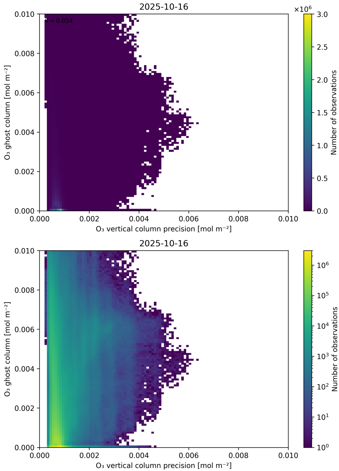
Figure 43: Scatter density plot of “O 3 vertical column precision” against “O 3 ghost column” for 2025-10-15 to 2025-10-17.
