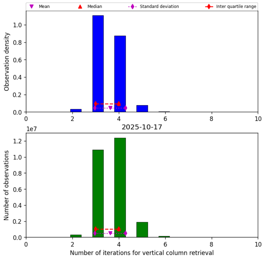
Figure 26: Histogram of “Number of iterations for vertical column retrieval” for 2025-10-17 to 2025-10-18
