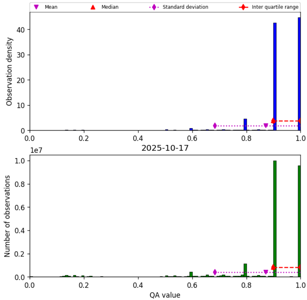
Figure 20: Histogram of “QA value” for 2025-10-17 to 2025-10-18
