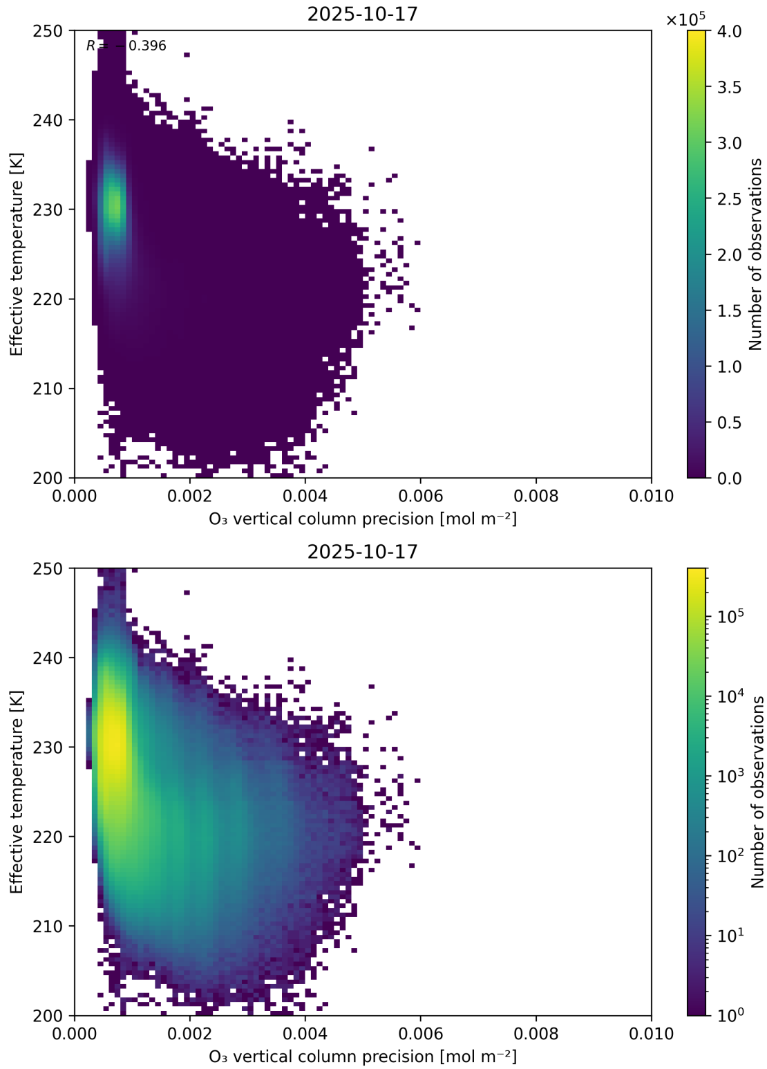
Figure 42: Scatter density plot of “ O_3 vertical column precision” against “Effective temperature” for 2025-10-17 to 2025-10-18.
