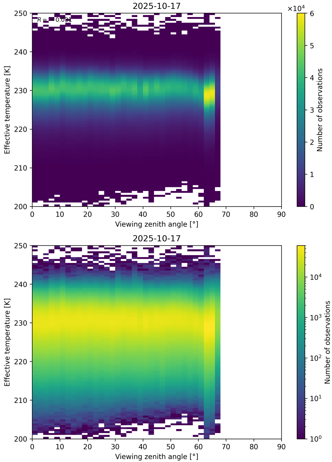
Figure 50: Scatter density plot of “Viewing zenith angle” against “Effective temperature” for 2025-10-17 to 2025-10-18.
