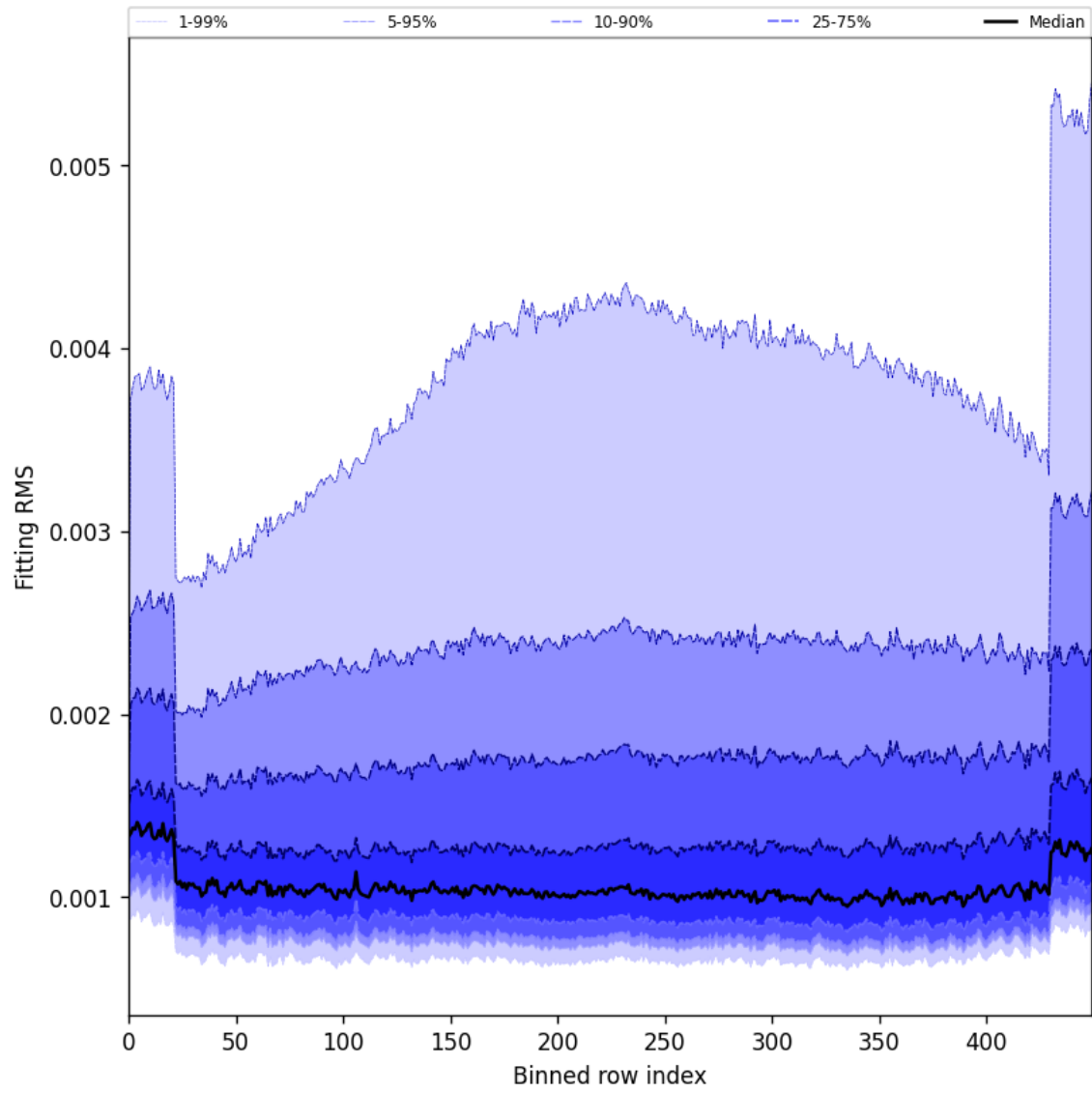
Figure 30: Along track statistics of “Fitting RMS” for 2025-10-17 to 2025-10-18
