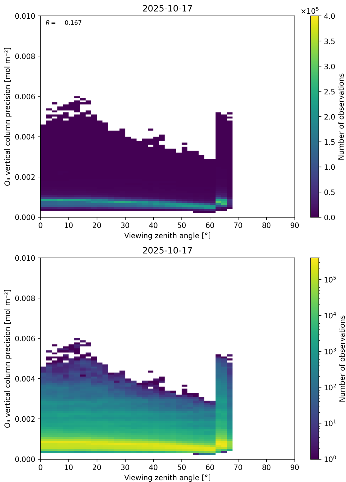
Figure 53: Scatter density plot of “Viewing zenith angle” against “O 3 vertical column precision” for 2025-10-17 to 2025-10-18.
