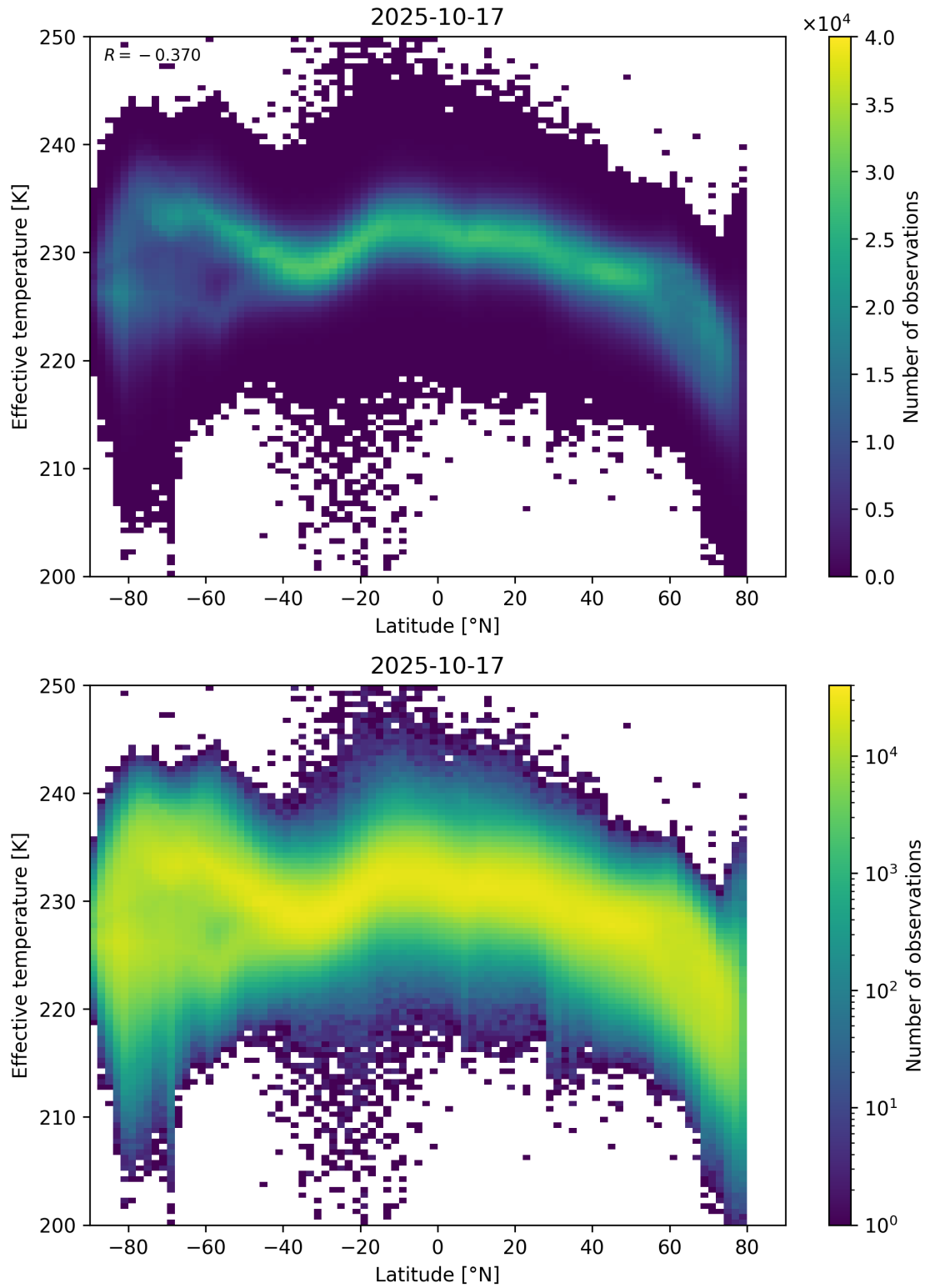
Figure 34: Scatter density plot of “Latitude” against “Effective temperature” for 2025-10-17 to 2025-10-18.
