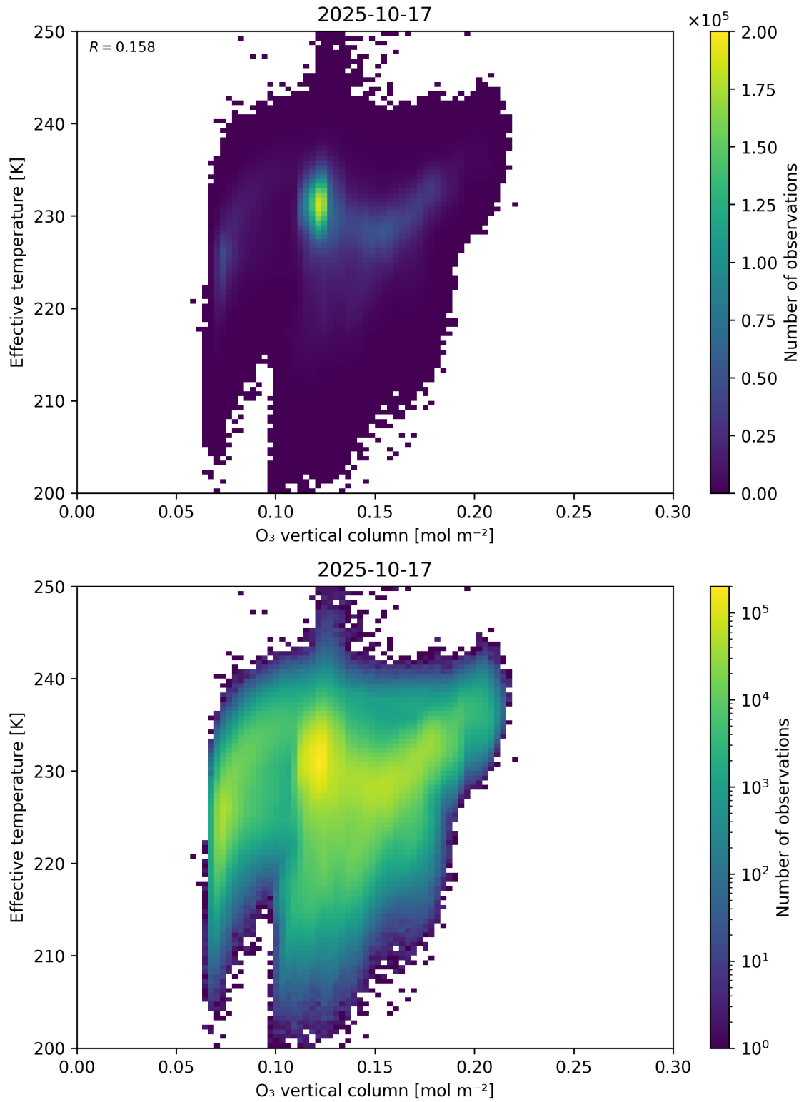
Figure 39: Scatter density plot of “O 3 vertical column” against “Effective temperature” for 2025-10-17 to 2025-10-18.
