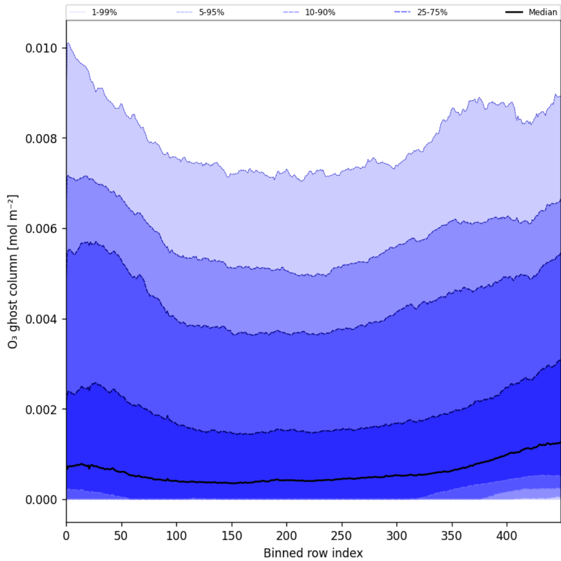
Figure 32: Along track statistics of “O 3 ghost column” for 2025-10-17 to 2025-10-18
