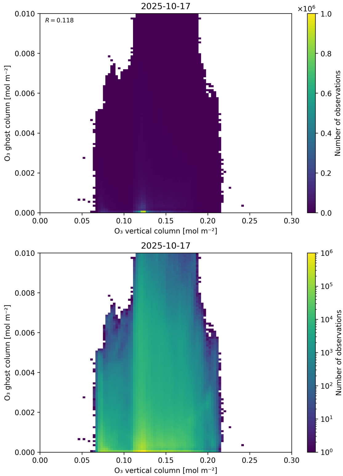
Figure 40: Scatter density plot of “O 3 vertical column” against “O 3 ghost column” for 2025-10-17 to 2025-10-18.
