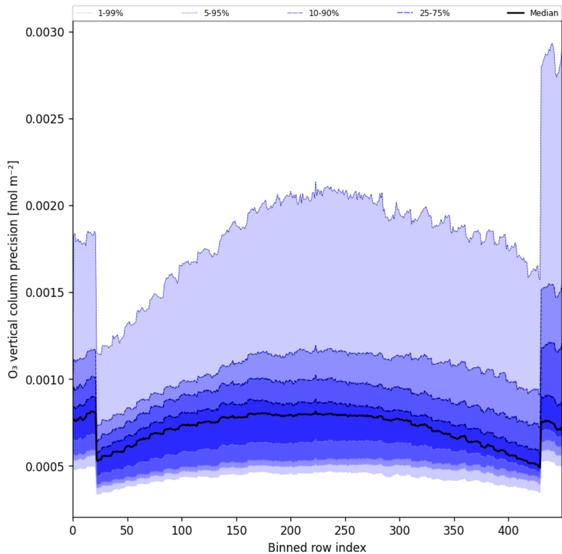
Figure 29: Along track statistics of “O 3 vertical column precision” for 2025-10-17 to 2025-10-18
