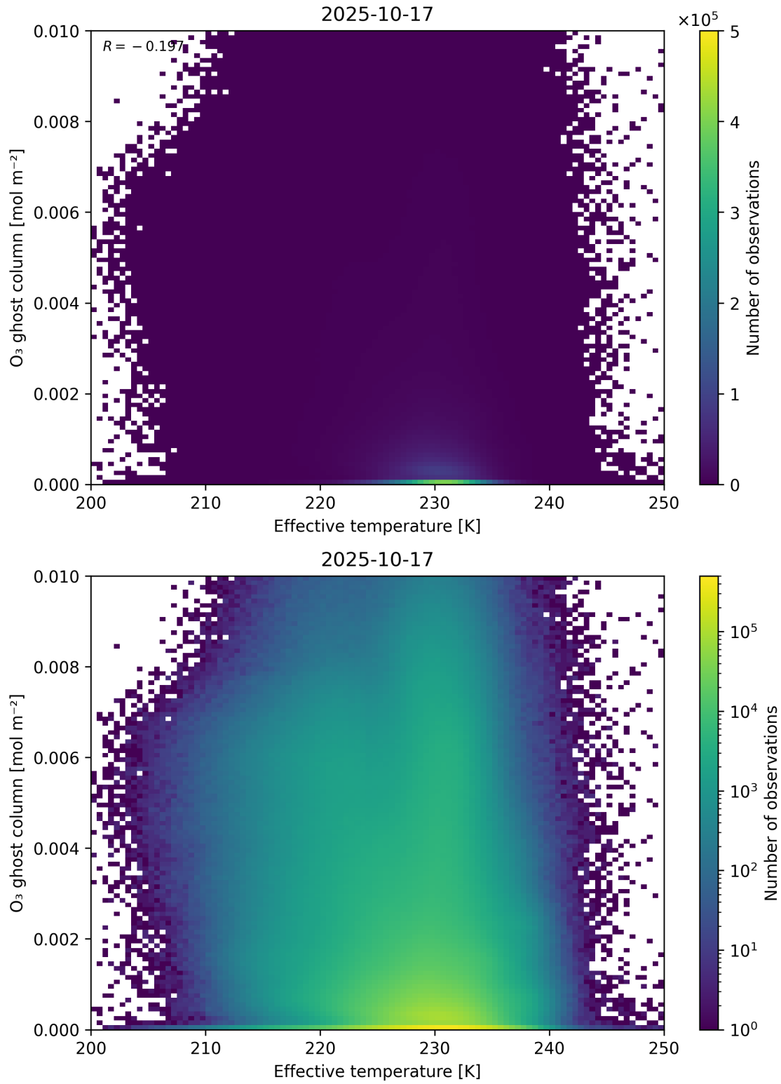
Figure 38: Scatter density plot of “Effective temperature” against “O 3 ghost column” for 2025-10-17 to 2025-10-18.
