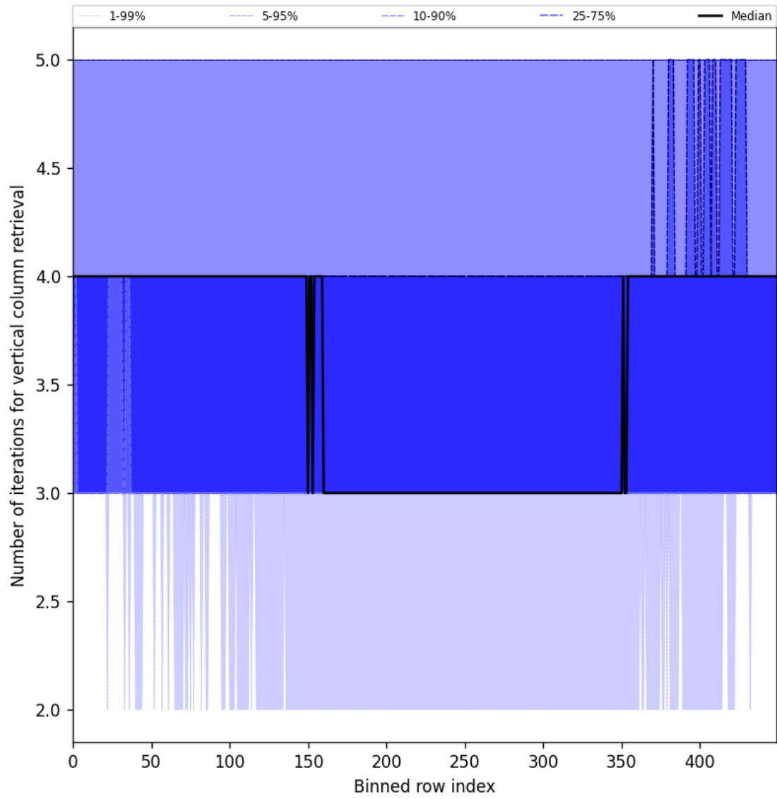
Figure 33: Along track statistics of “Number of iterations for vertical column retrieval” for 2025-10-17 to 2025-10-18
