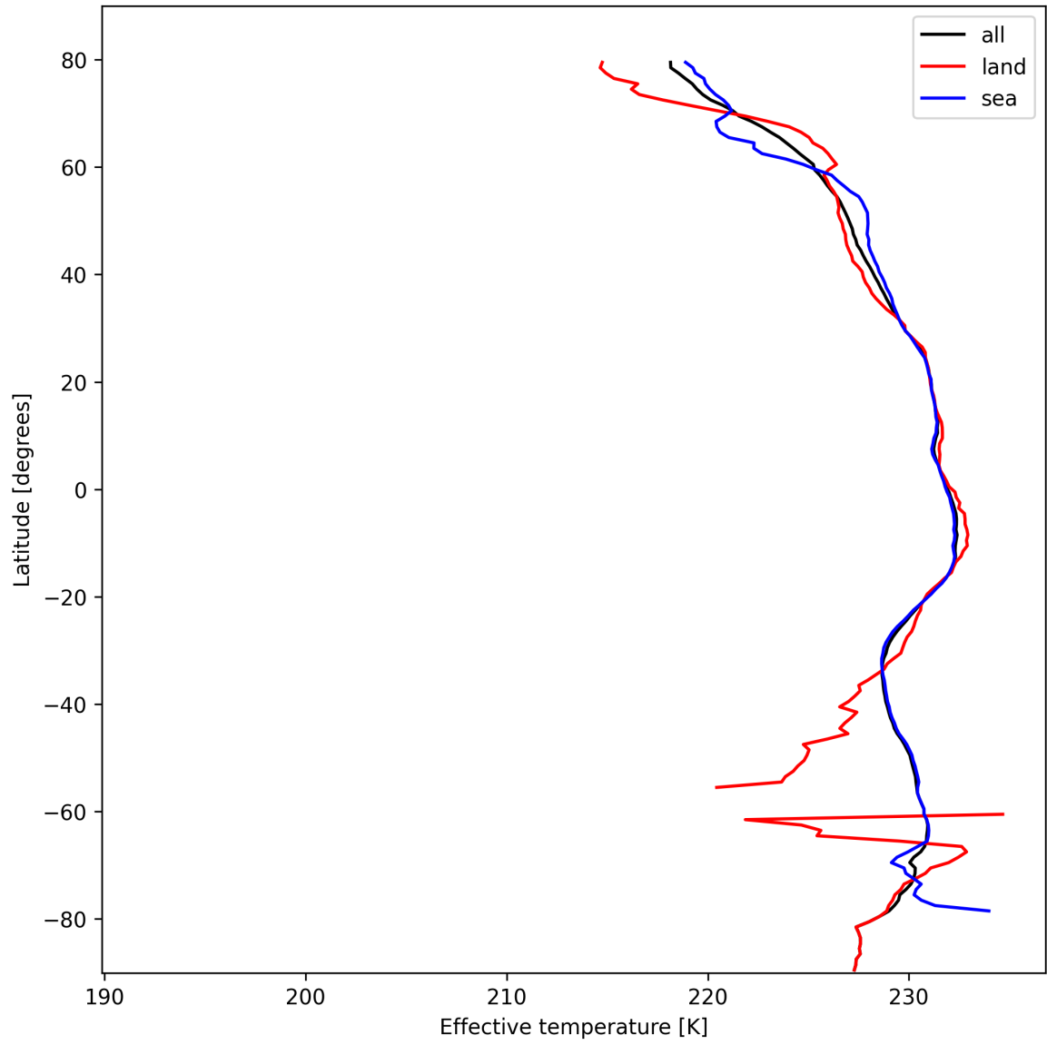
Figure 17: Zonal average of "Effective temperature" for 2025-10-17 to 2025-10-18.
