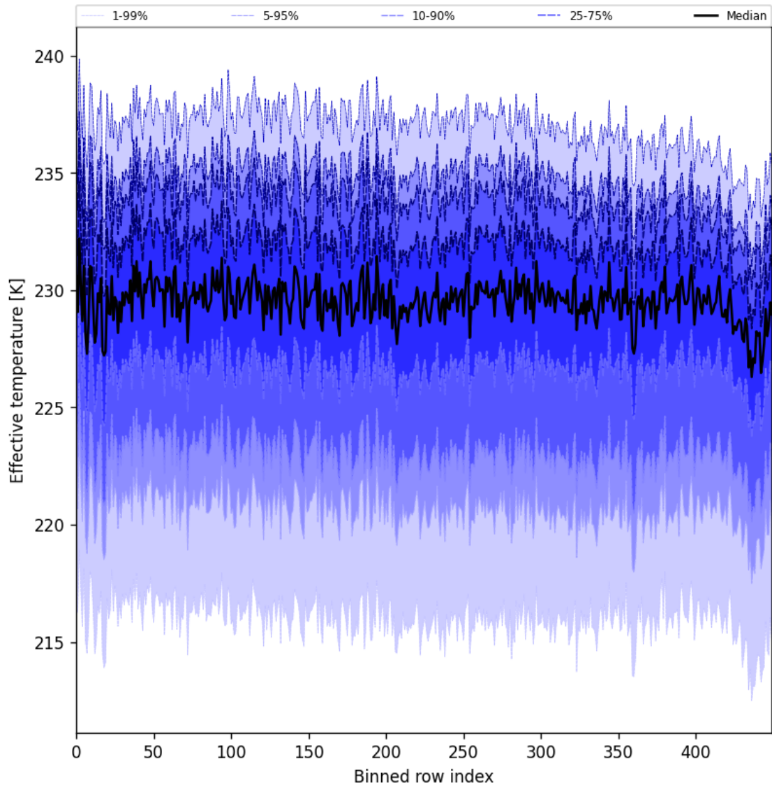
Figure 31: Along track statistics of “Effective temperature” for 2025-10-17 to 2025-10-18
