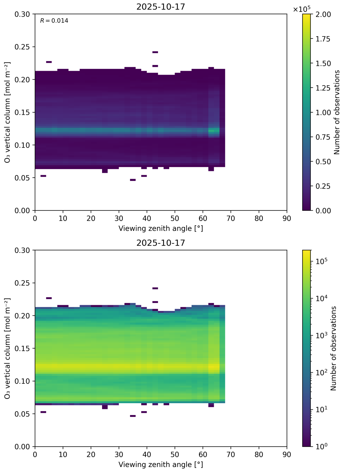
Figure 52: Scatter density plot of “Viewing zenith angle” against “O 3 vertical column” for 2025-10-17 to 2025-10-18.
