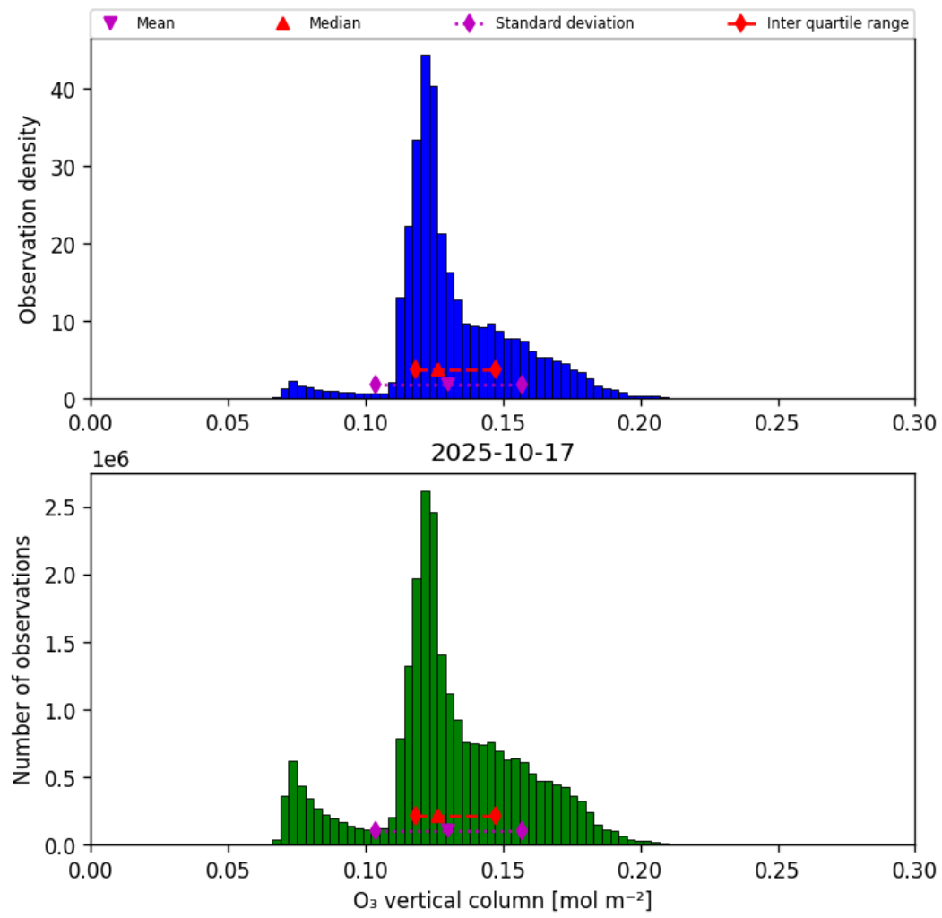
Figure 21: Histogram of “O 3 vertical column” for 2025-10-17 to 2025-10-18
