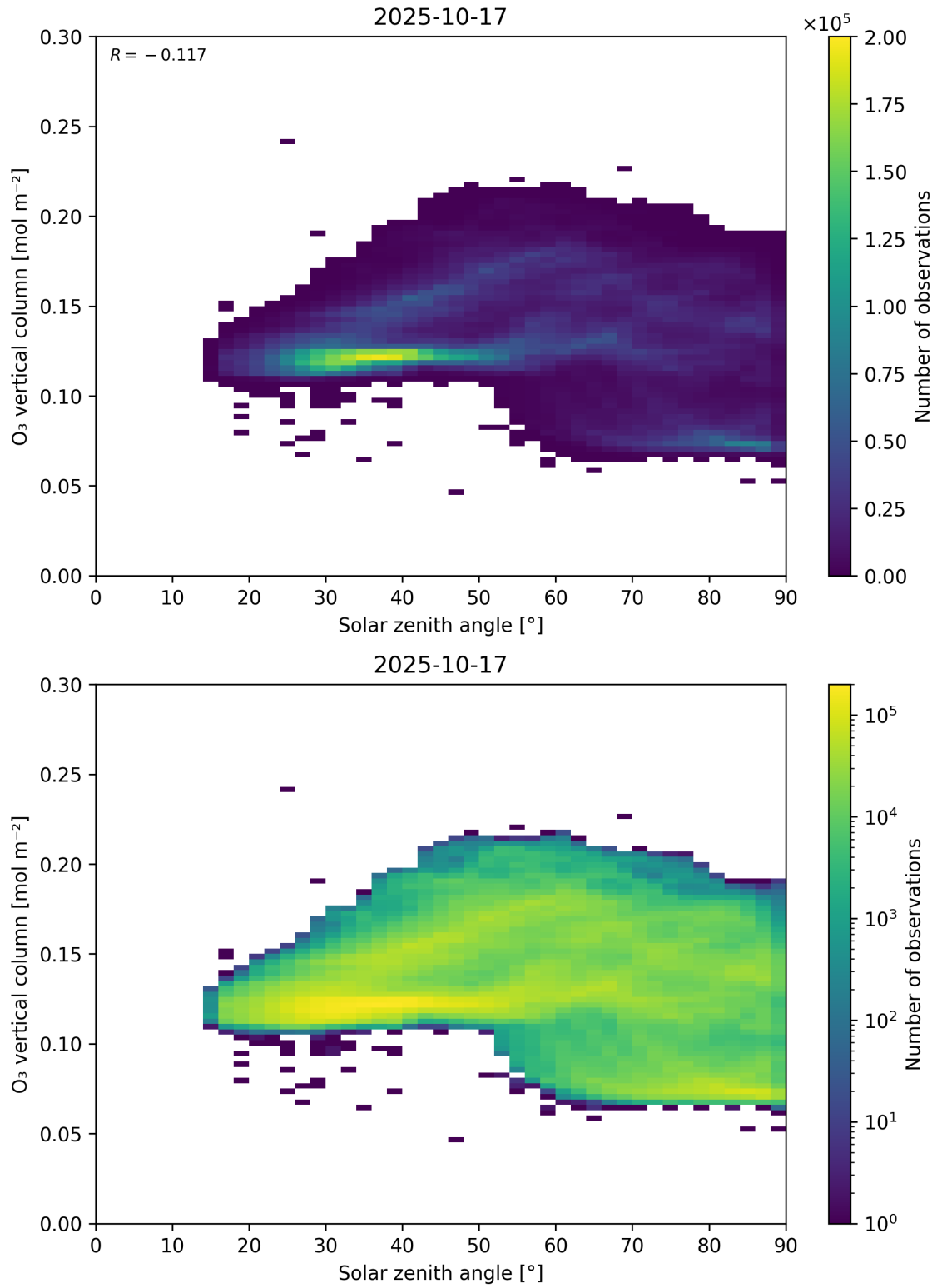
Figure 47: Scatter density plot of “Solar zenith angle” against “O 3 vertical column” for 2025-10-17 to 2025-10-18.
