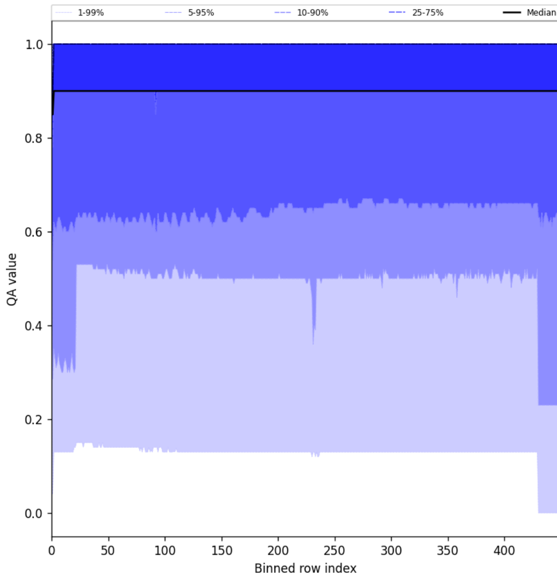
Figure 27: Along track statistics of “QA value” for 2025-10-17 to 2025-10-18
