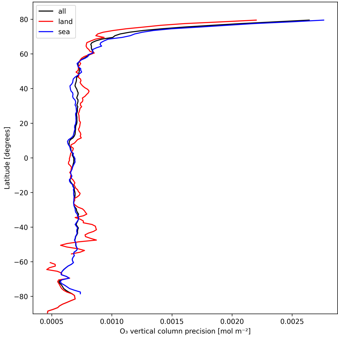
Figure 15: Zonal average of “O 3 vertical column precision” for 2025-10-17 to 2025-10-18.
