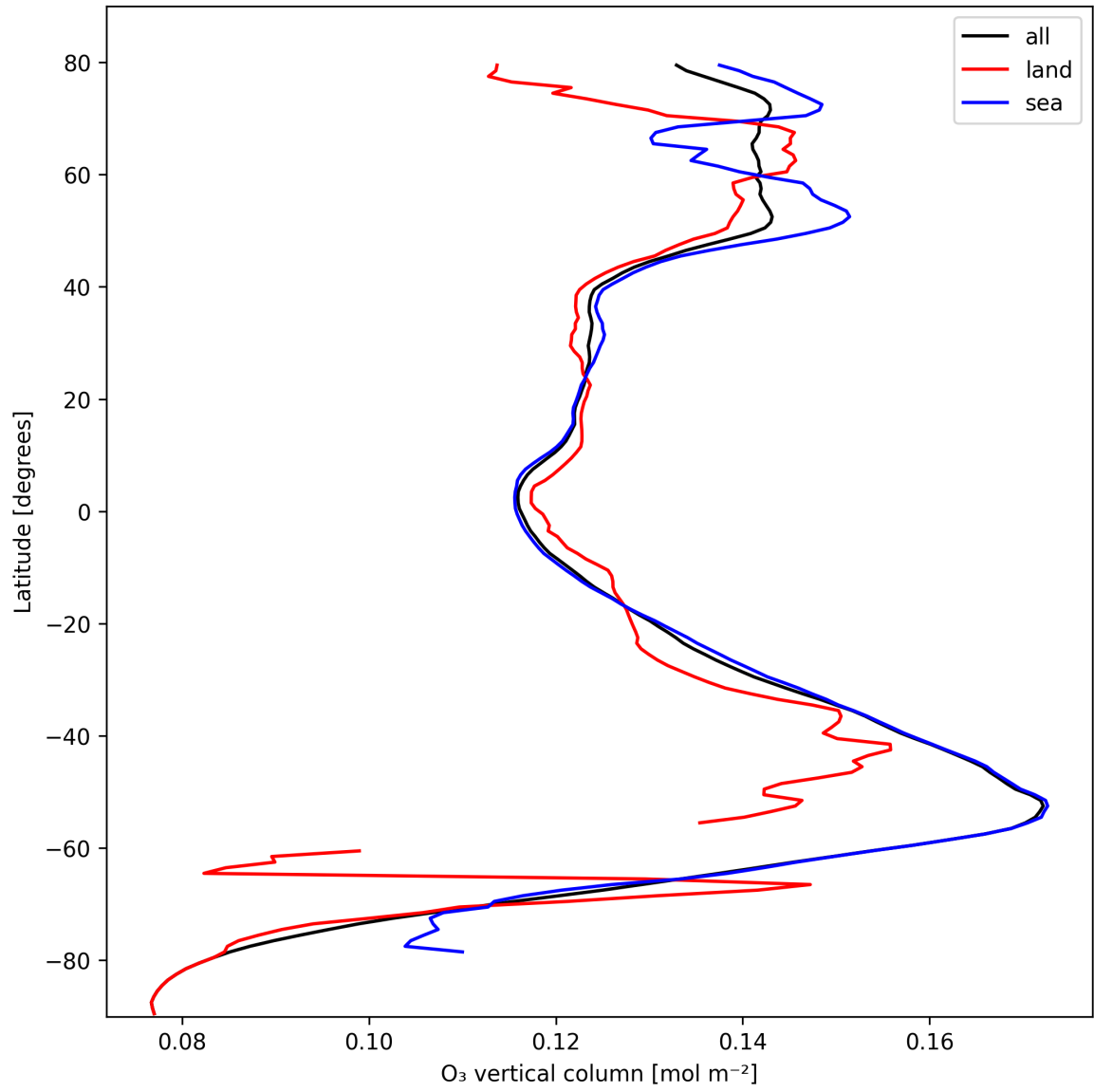
Figure 14: Zonal average of “O 3 vertical column” for 2025-10-17 to 2025-10-18.
