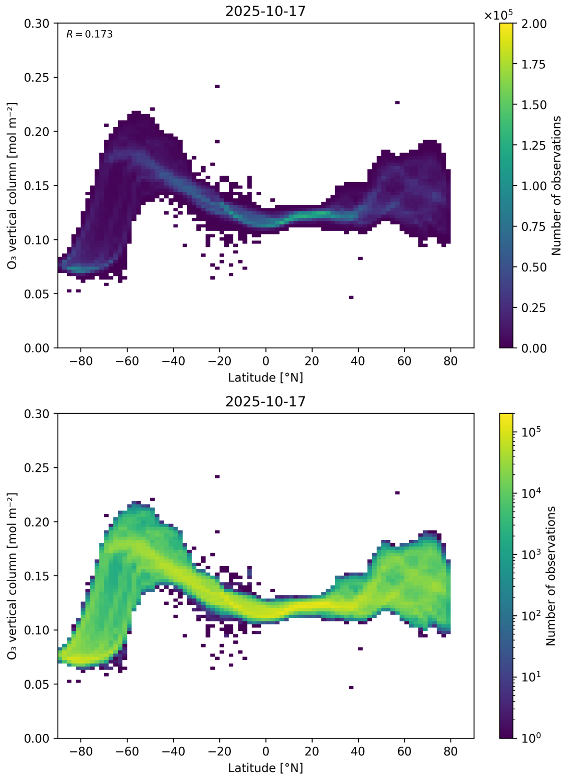
Figure 36: Scatter density plot of “Latitude” against “O 3 vertical column” for 2025-10-17 to 2025-10-18.
