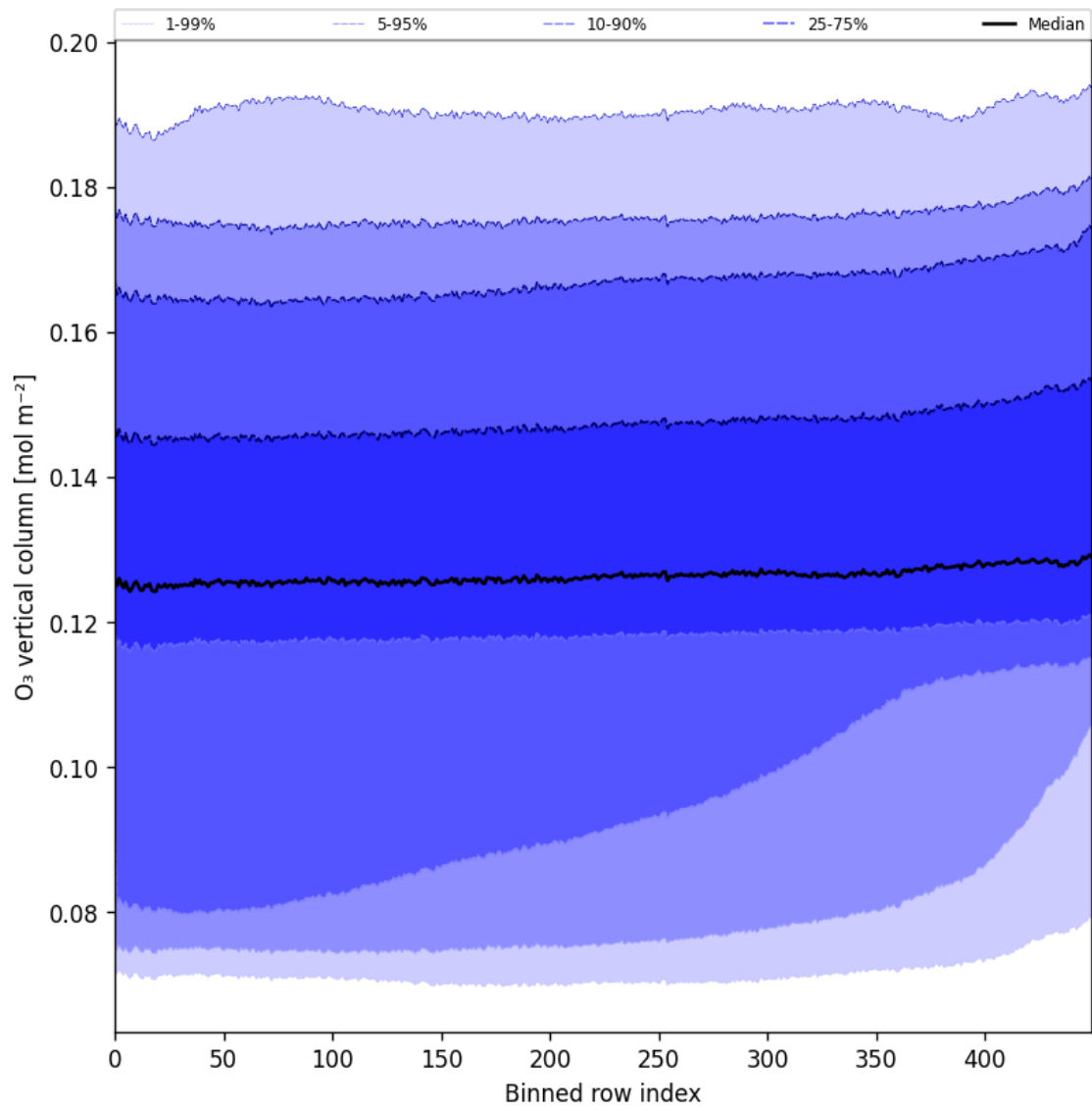
Figure 28: Along track statistics of “O 3 vertical column” for 2025-10-17 to 2025-10-18
