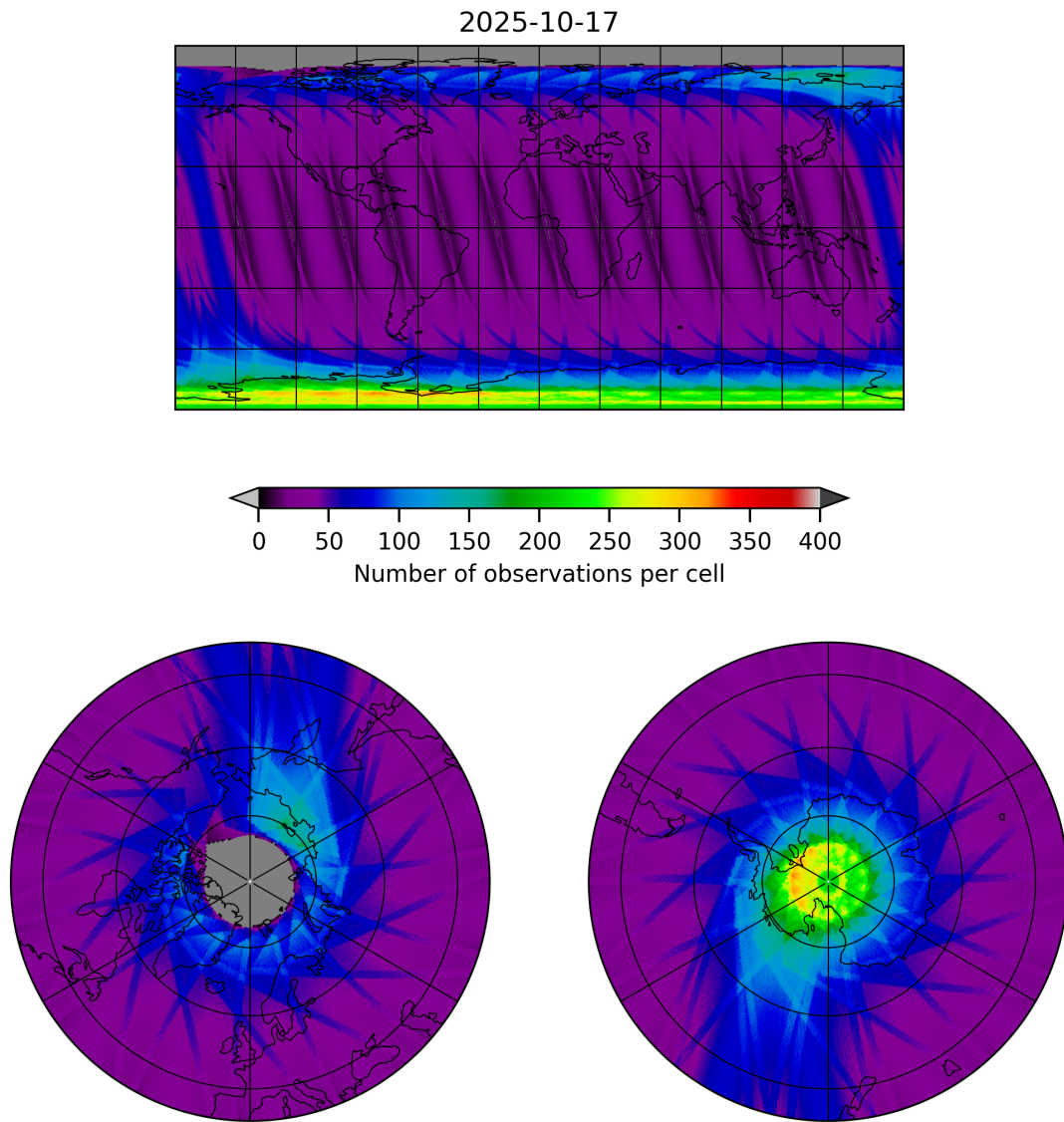
Figure 12: Map of the number of observations for 2025-10-17 to 2025-10-18
