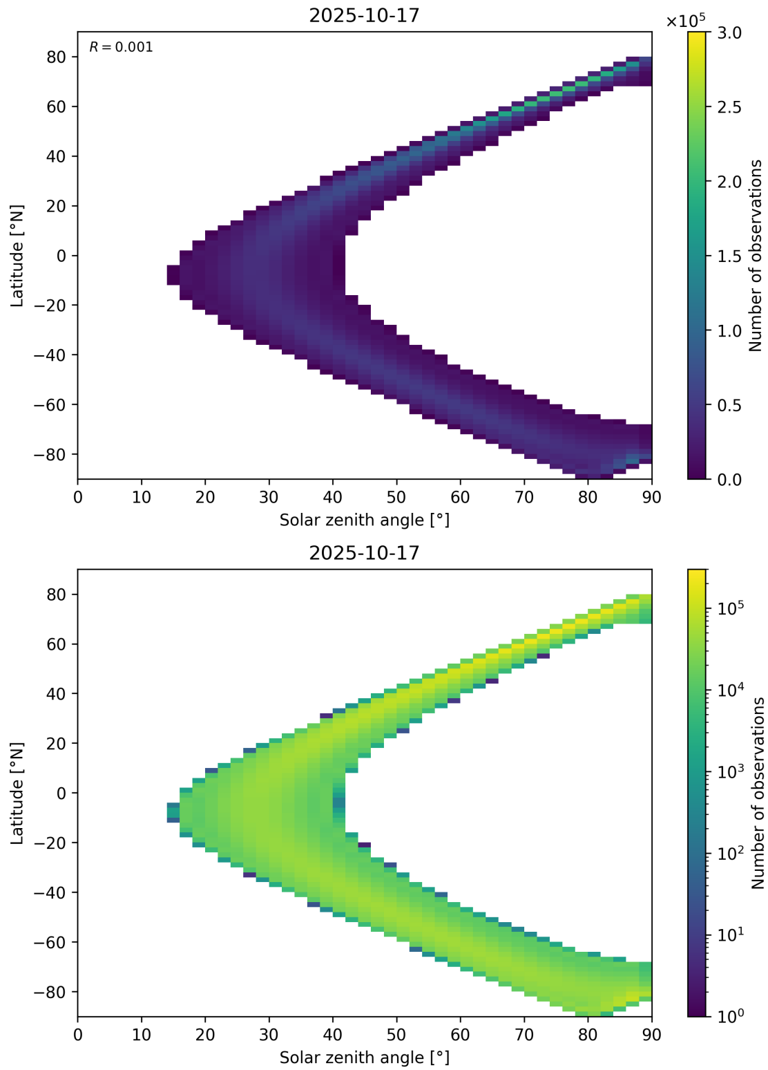
Figure 44: Scatter density plot of “Solar zenith angle” against “Latitude” for 2025-10-17 to 2025-10-18.
