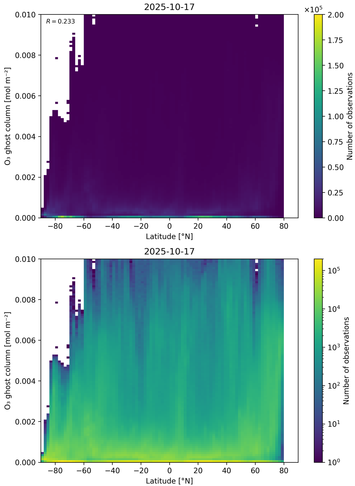
Figure 35: Scatter density plot of “Latitude” against “O 3 ghost column” for 2025-10-17 to 2025-10-18.
