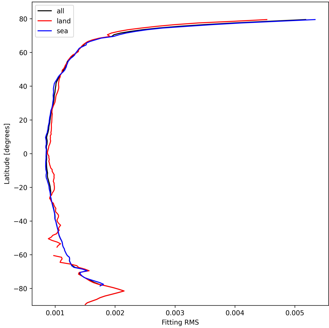
Figure 16: Zonal average of “Fitting RMS” for 2025-10-17 to 2025-10-18.
