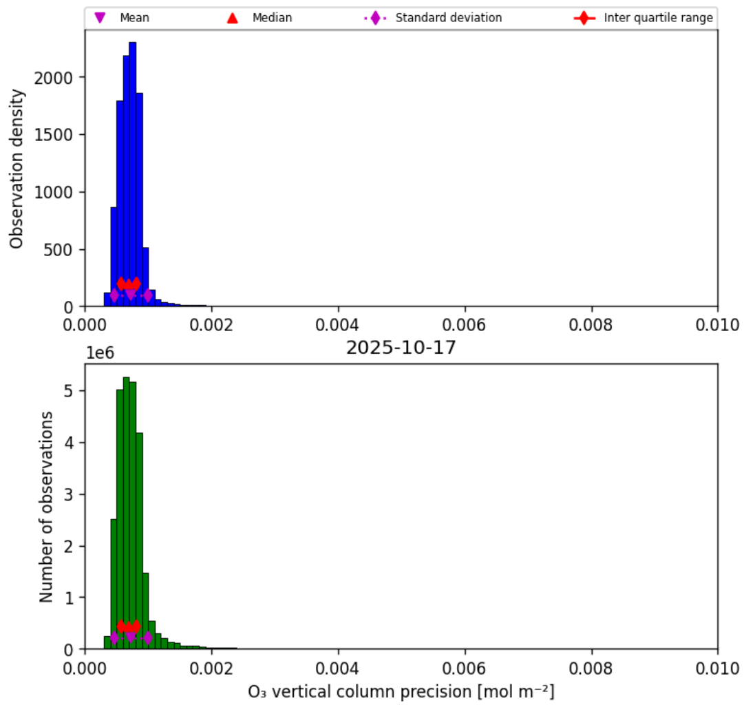
Figure 22: Histogram of “O 3 vertical column precision” for 2025-10-17 to 2025-10-18
