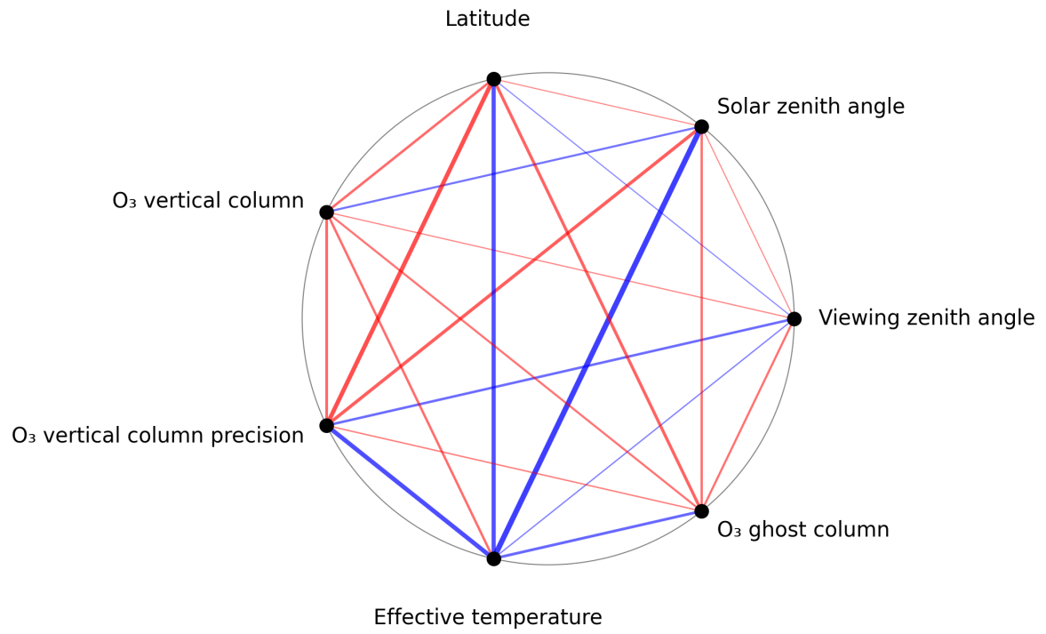
Figure 1: Map of correlation graph for 2025-10-17 to 2025-10-18.
