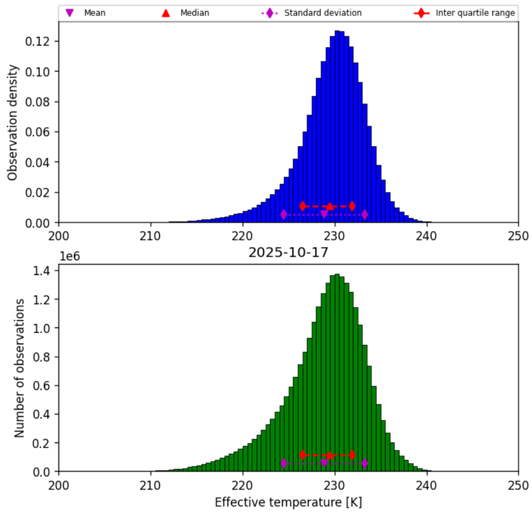
Figure 24: Histogram of “Effective temperature” for 2025-10-17 to 2025-10-18
