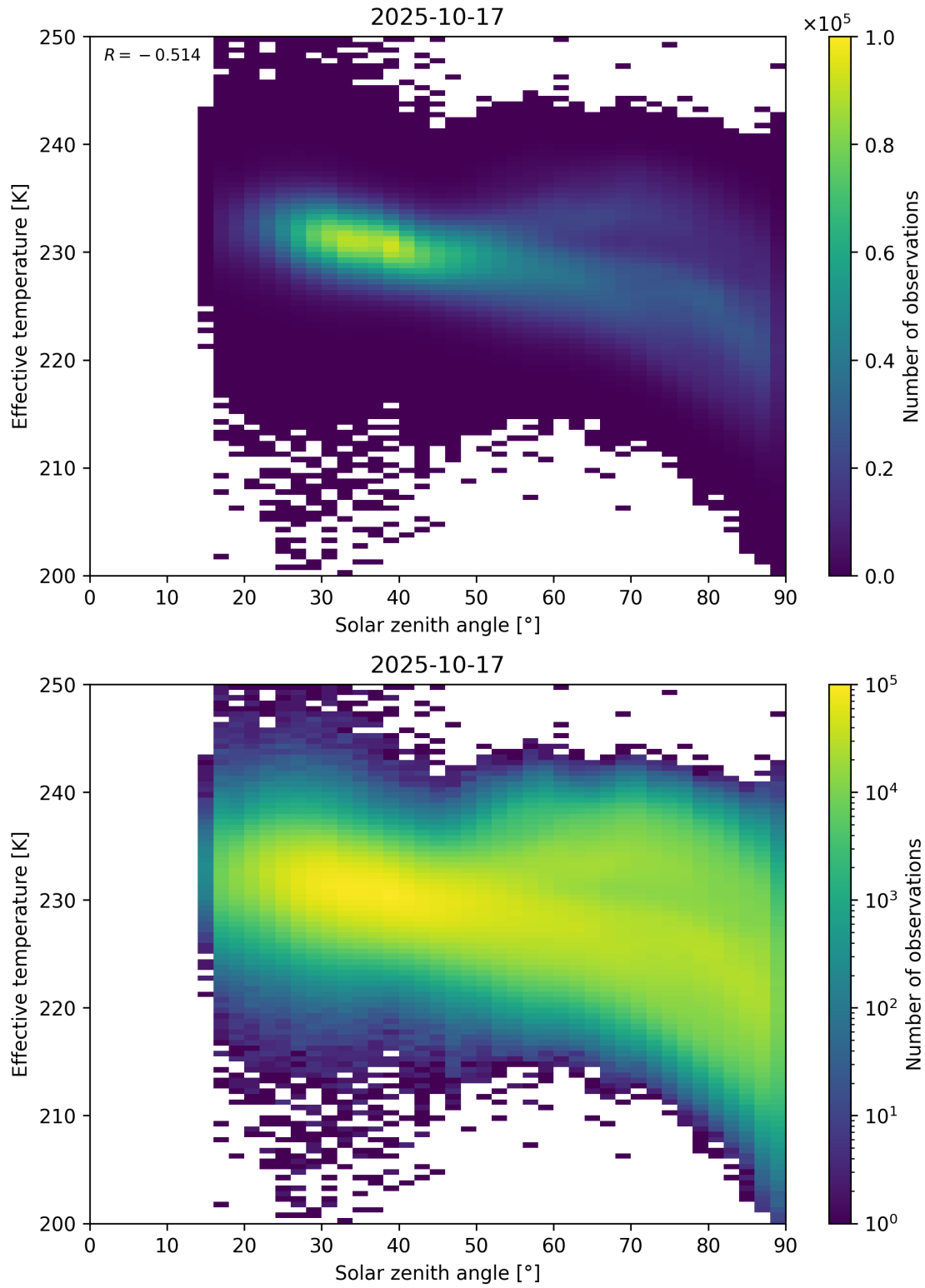
Figure 45: Scatter density plot of “Solar zenith angle” against “Effective temperature” for 2025-10-17 to 2025-10-18.
