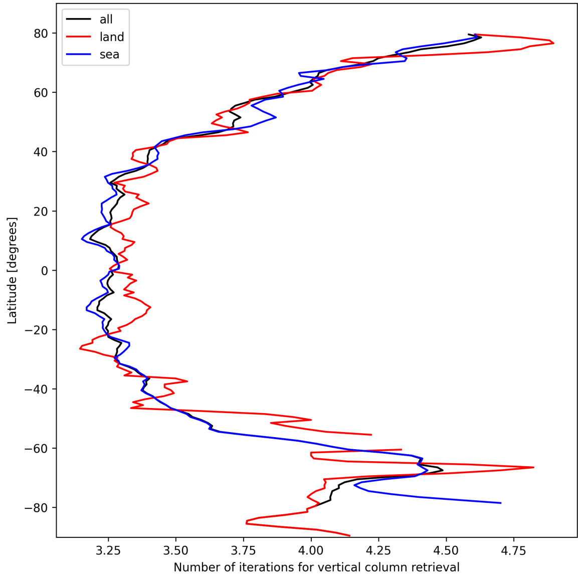
Figure 19: Zonal average of “Number of iterations for vertical column retrieval” for 2025-10-17 to 2025-10-18.
