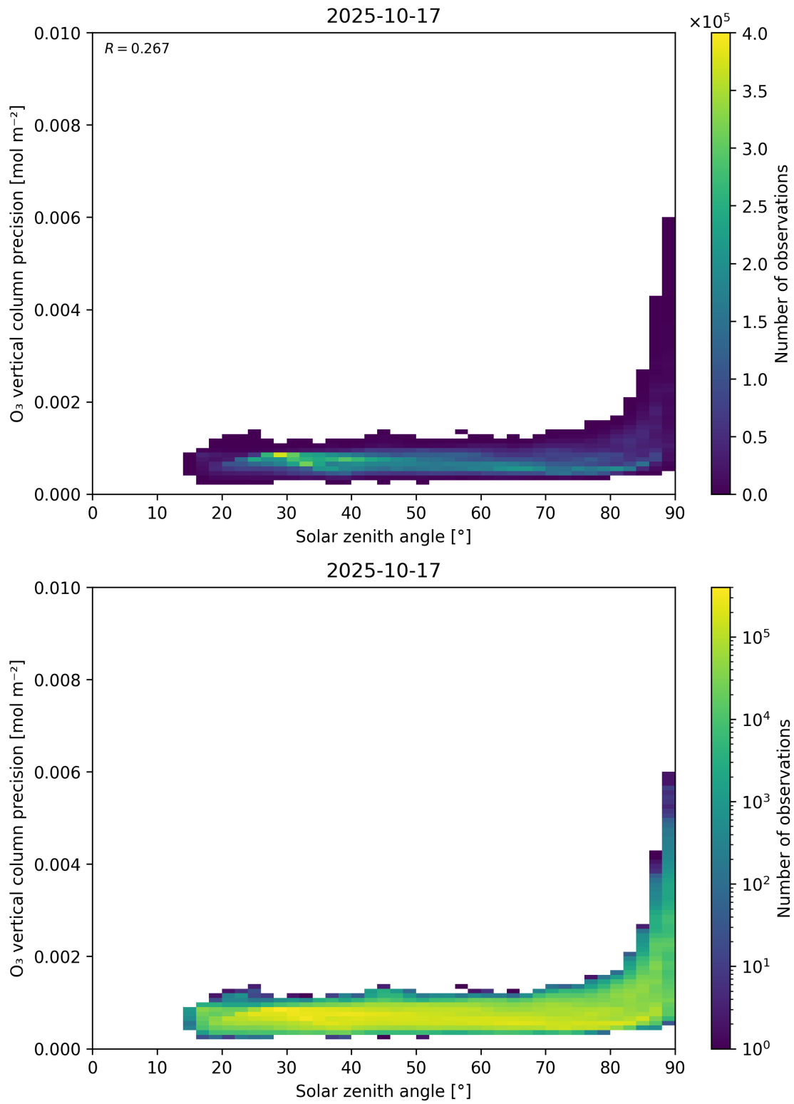
Figure 48: Scatter density plot of “Solar zenith angle” against “O 3 vertical column precision” for 2025-10-17 to 2025-10-18.
