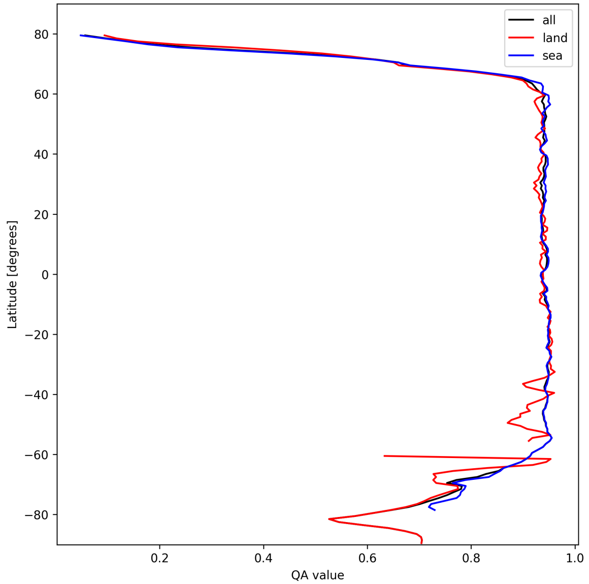
Figure 13: Zonal average of “QA value” for 2025-10-17 to 2025-10-18.
