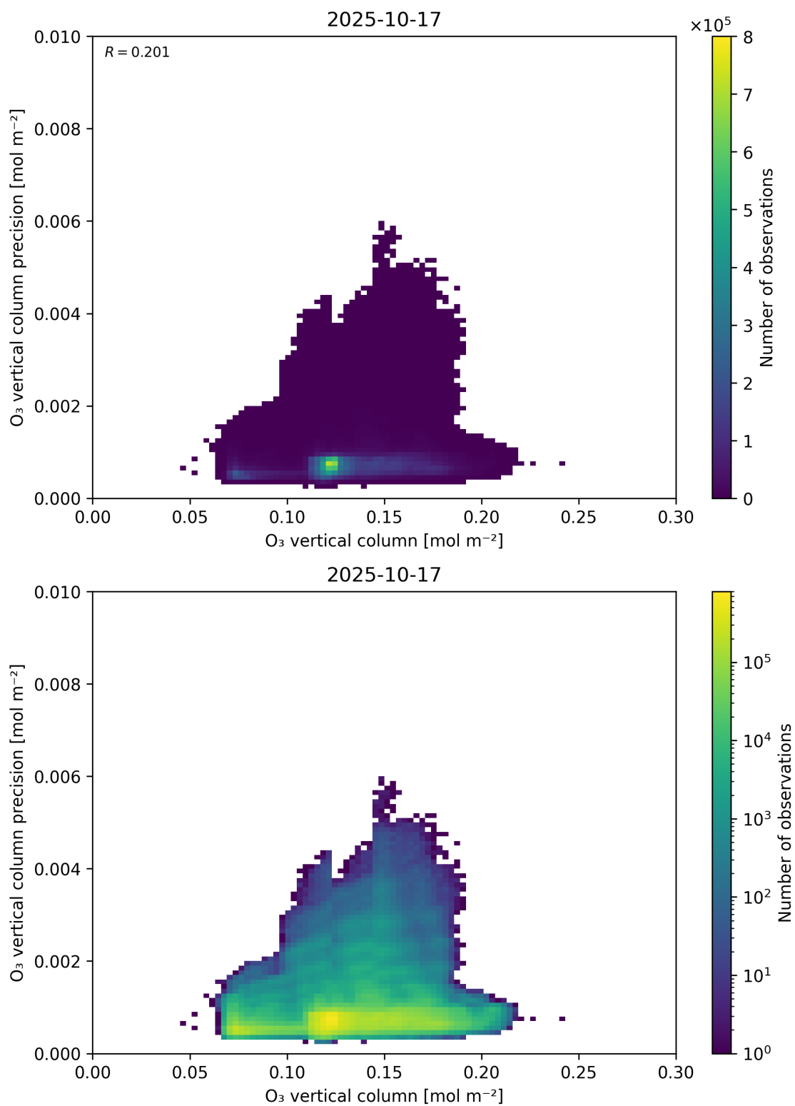
Figure 41: Scatter density plot of “O 3 vertical column” against “O 3 vertical column precision” for 2025-10-17 to 2025-10-18.
