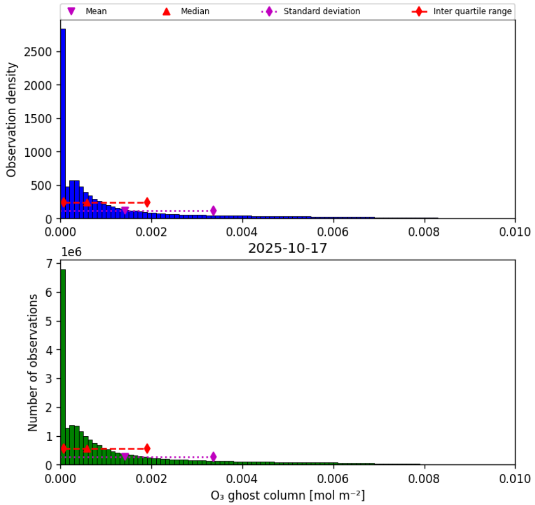
Figure 25: Histogram of “O 3 ghost column” for 2025-10-17 to 2025-10-18
