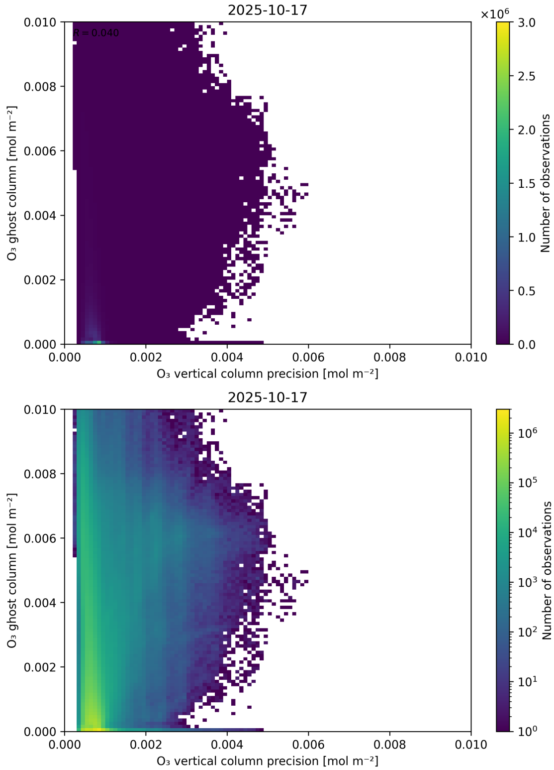
Figure 43: Scatter density plot of “O 3 vertical column precision” against “O 3 ghost column” for 2025-10-17 to 2025-10-18.
