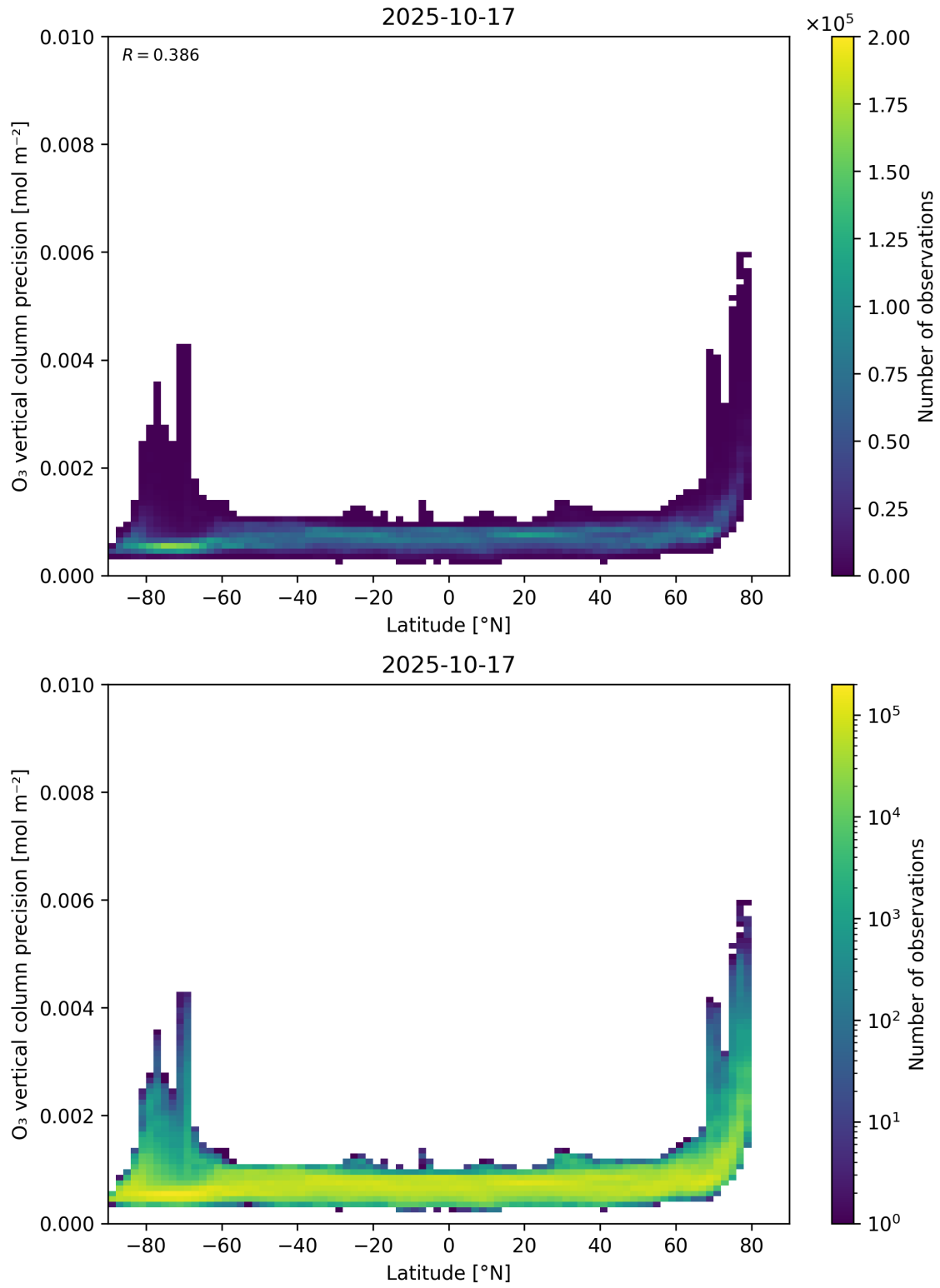
Figure 37: Scatter density plot of “Latitude” against “O 3 vertical column precision” for 2025-10-17 to 2025-10-18.
