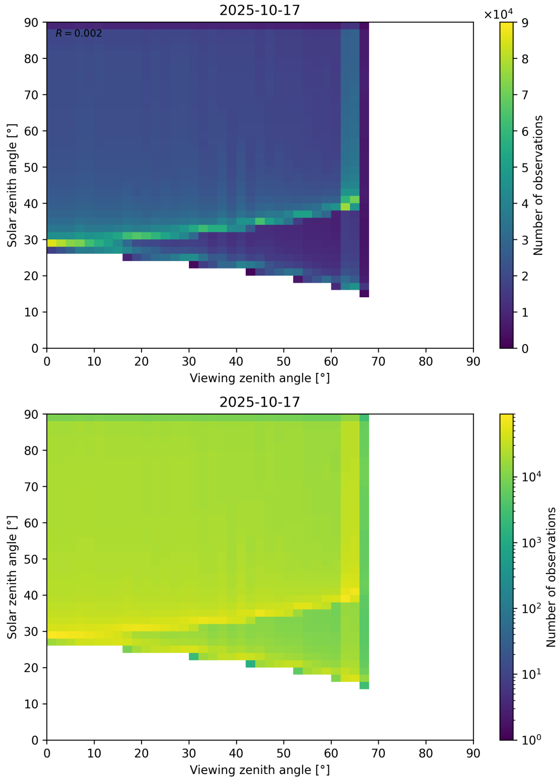
Figure 54: Scatter density plot of “Viewing zenith angle” against “Solar zenith angle” for 2025-10-17 to 2025-10-18.
