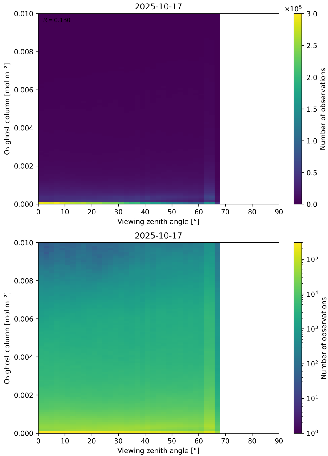
Figure 51: Scatter density plot of “Viewing zenith angle” against “O 3 ghost column” for 2025-10-17 to 2025-10-18.
