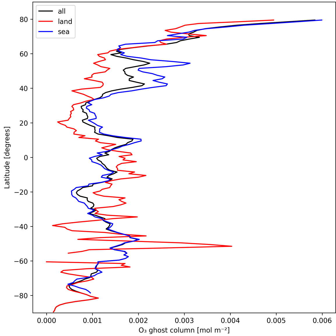
Figure 18: Zonal average of “O 3 ghost column” for 2025-10-17 to 2025-10-18.
