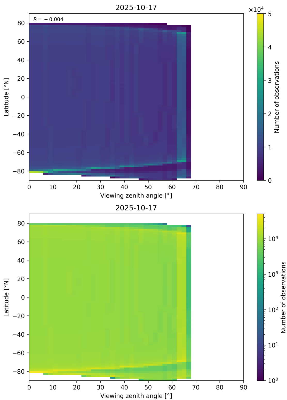
Figure 49: Scatter density plot of “Viewing zenith angle” against “Latitude” for 2025-10-17 to 2025-10-18.
