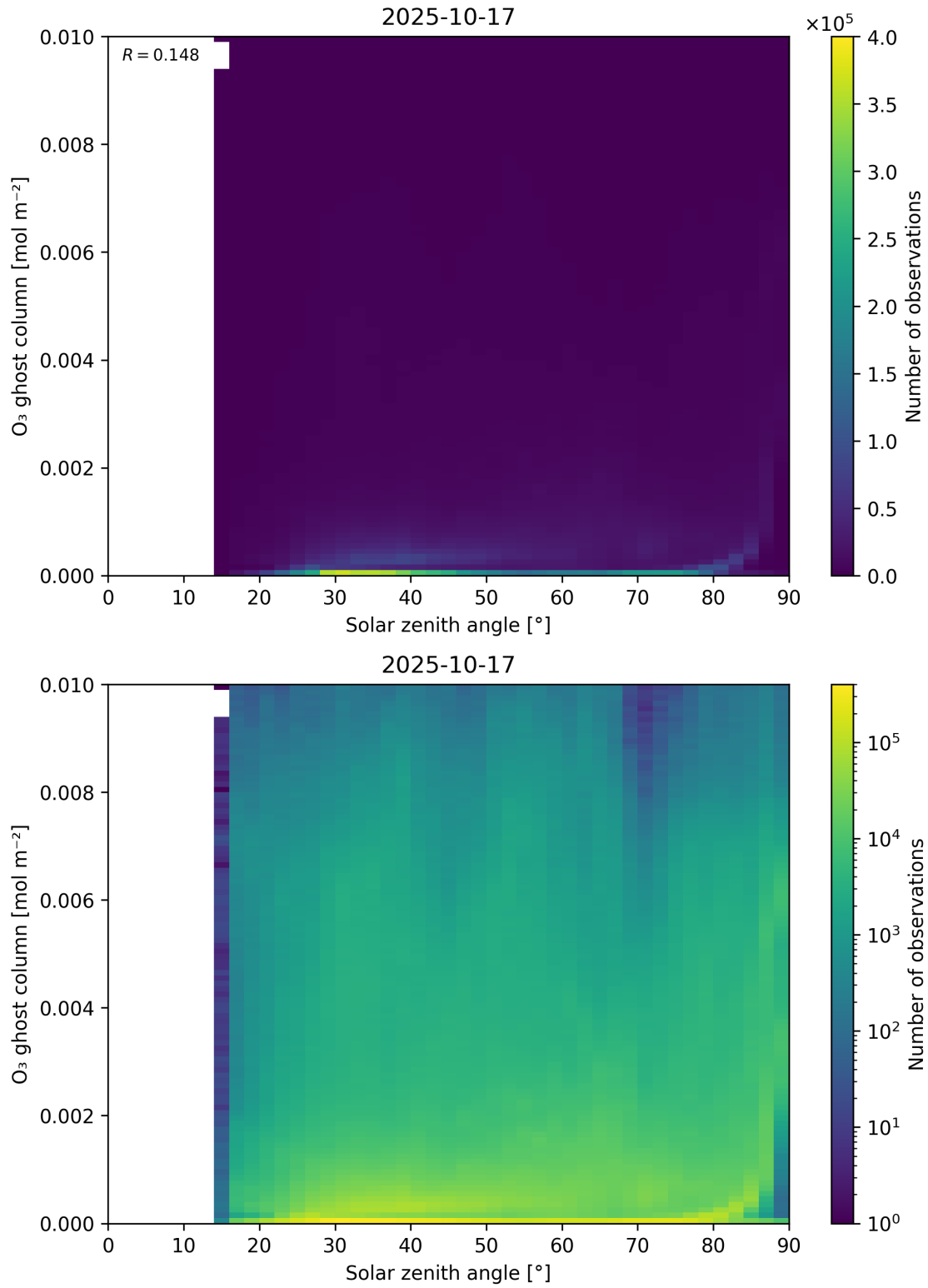
Figure 46: Scatter density plot of “Solar zenith angle” against “O 3 ghost column” for 2025-10-17 to 2025-10-18.
