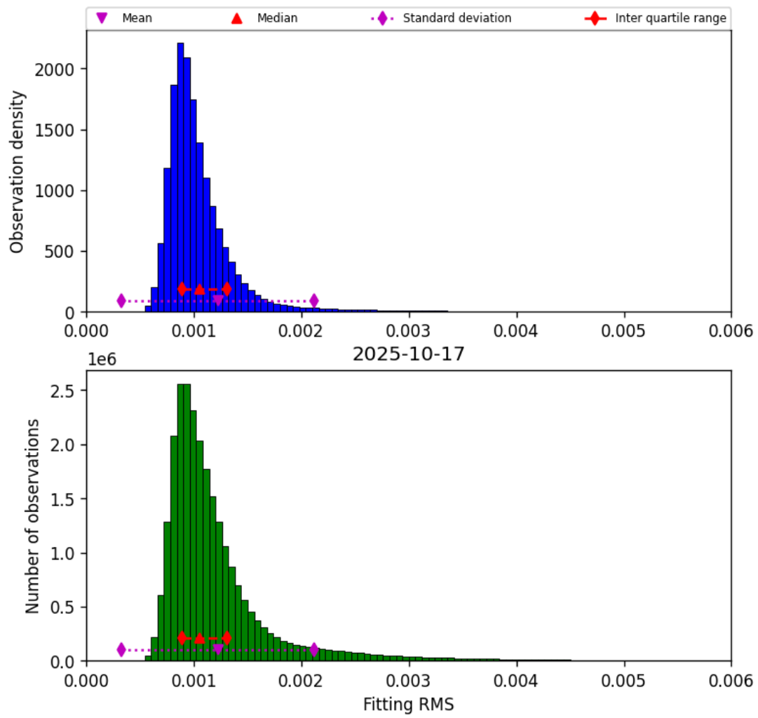
Figure 23: Histogram of “Fitting RMS” for 2025-10-17 to 2025-10-18
