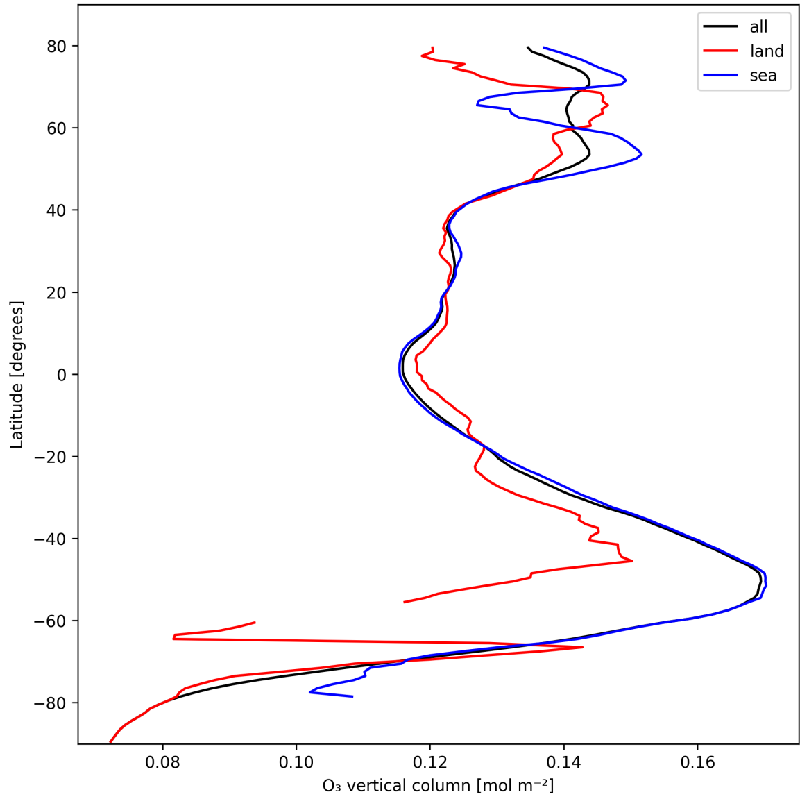
Figure 14: Zonal average of “O 3 vertical column” for 2025-10-17 to 2025-10-19.
