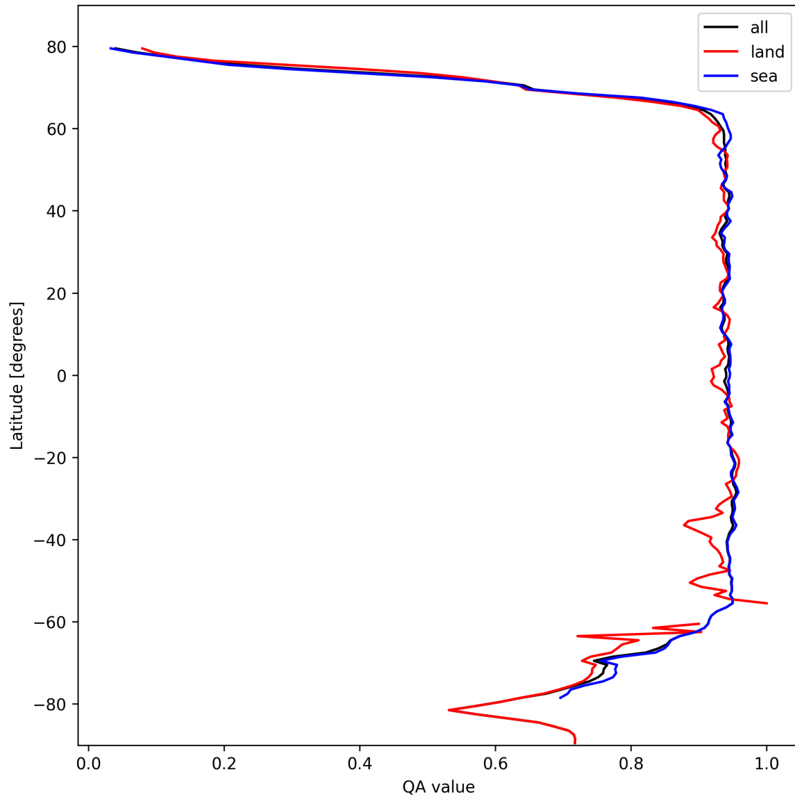
Figure 13: Zonal average of “QA value” for 2025-10-17 to 2025-10-19.
