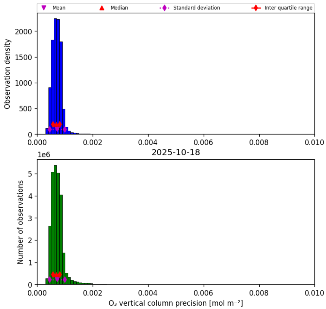
Figure 22: Histogram of “O 3 vertical column precision” for 2025-10-17 to 2025-10-19
