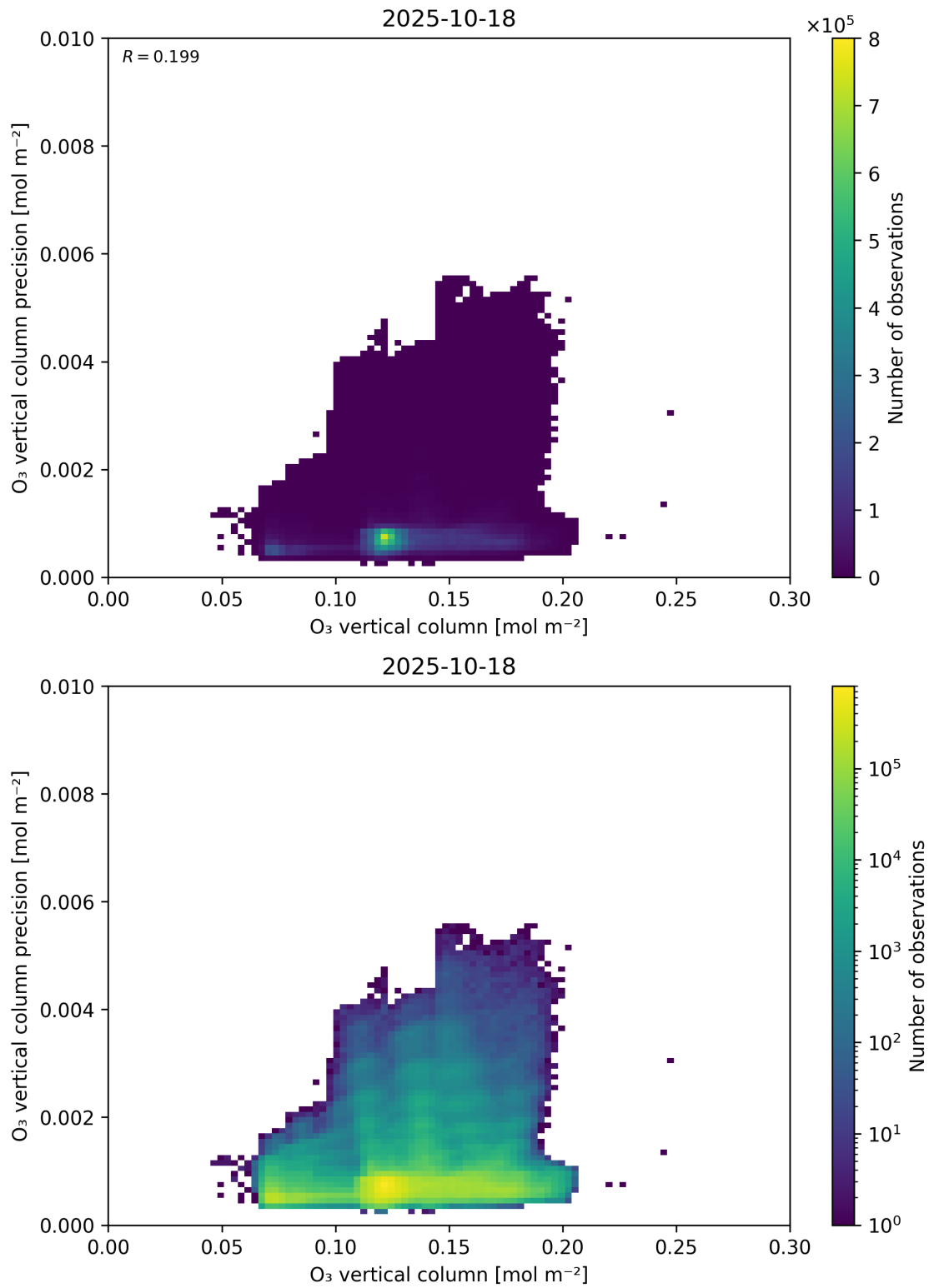
Figure 41: Scatter density plot of “O 3 vertical column” against “O 3 vertical column precision” for 2025-10-17 to 2025-10-19.
