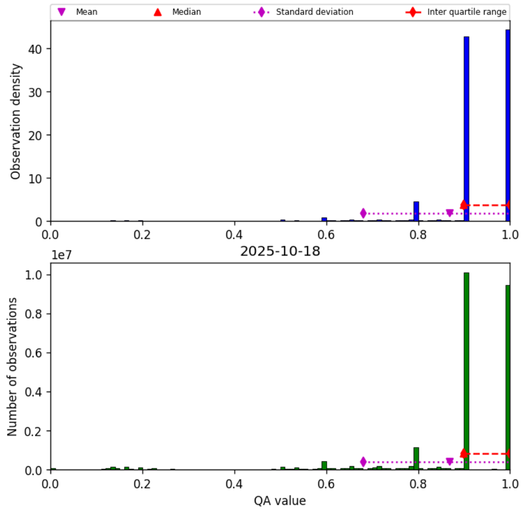
Figure 20: Histogram of “QA value” for 2025-10-17 to 2025-10-19
