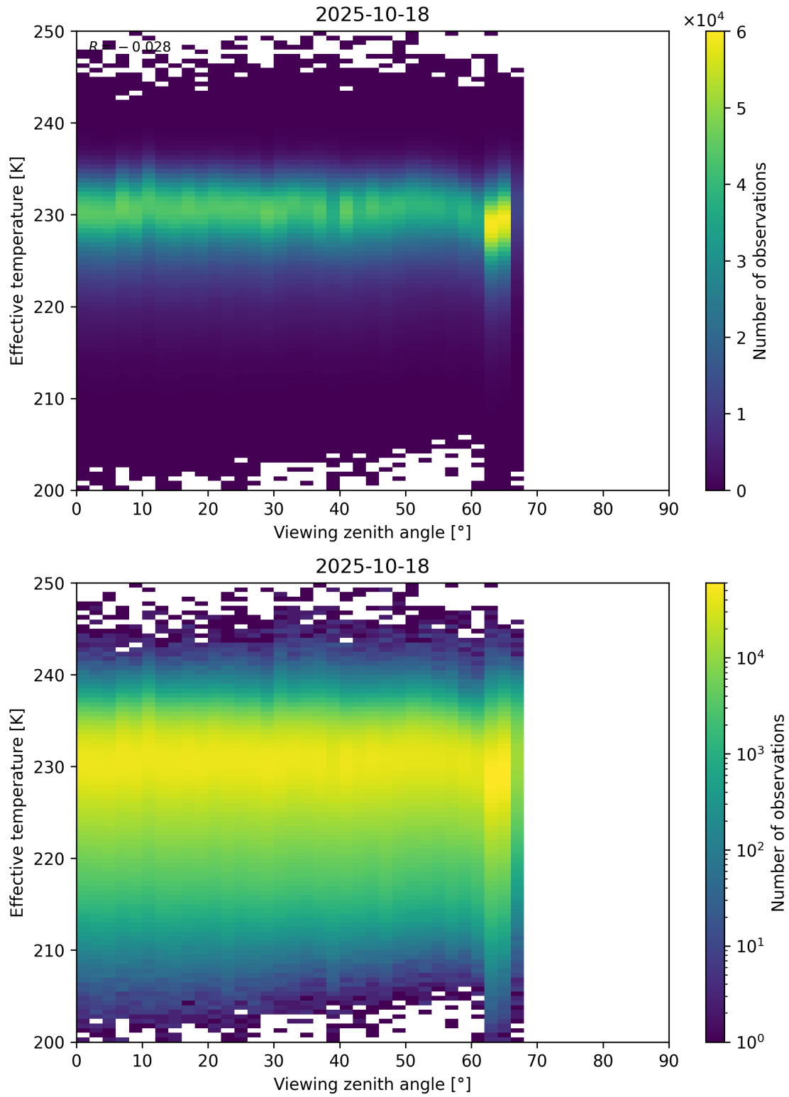
Figure 50: Scatter density plot of “Viewing zenith angle” against “Effective temperature” for 2025-10-17 to 2025-10-19.
