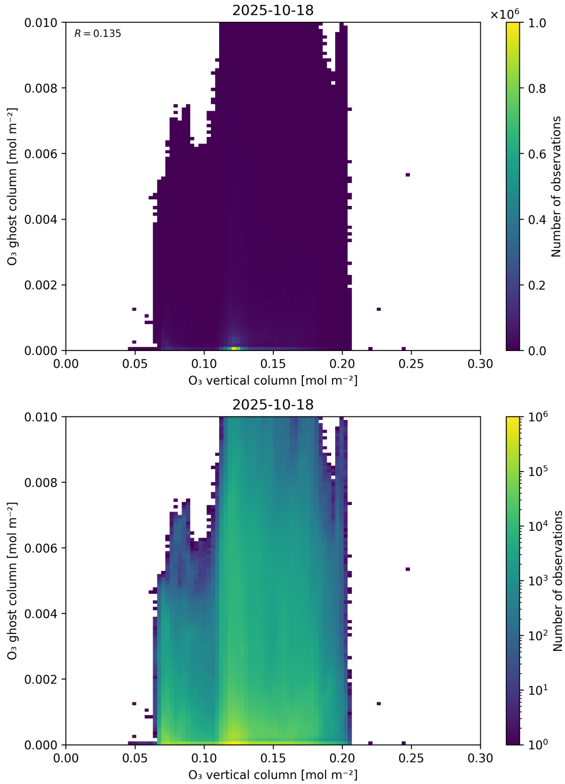
Figure 40: Scatter density plot of “O 3 vertical column” against “O 3 ghost column” for 2025-10-17 to 2025-10-19.
