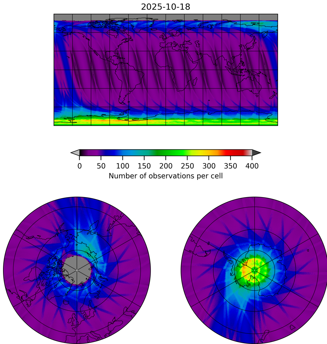
Figure 12: Map of the number of observations for 2025-10-17 to 2025-10-19
