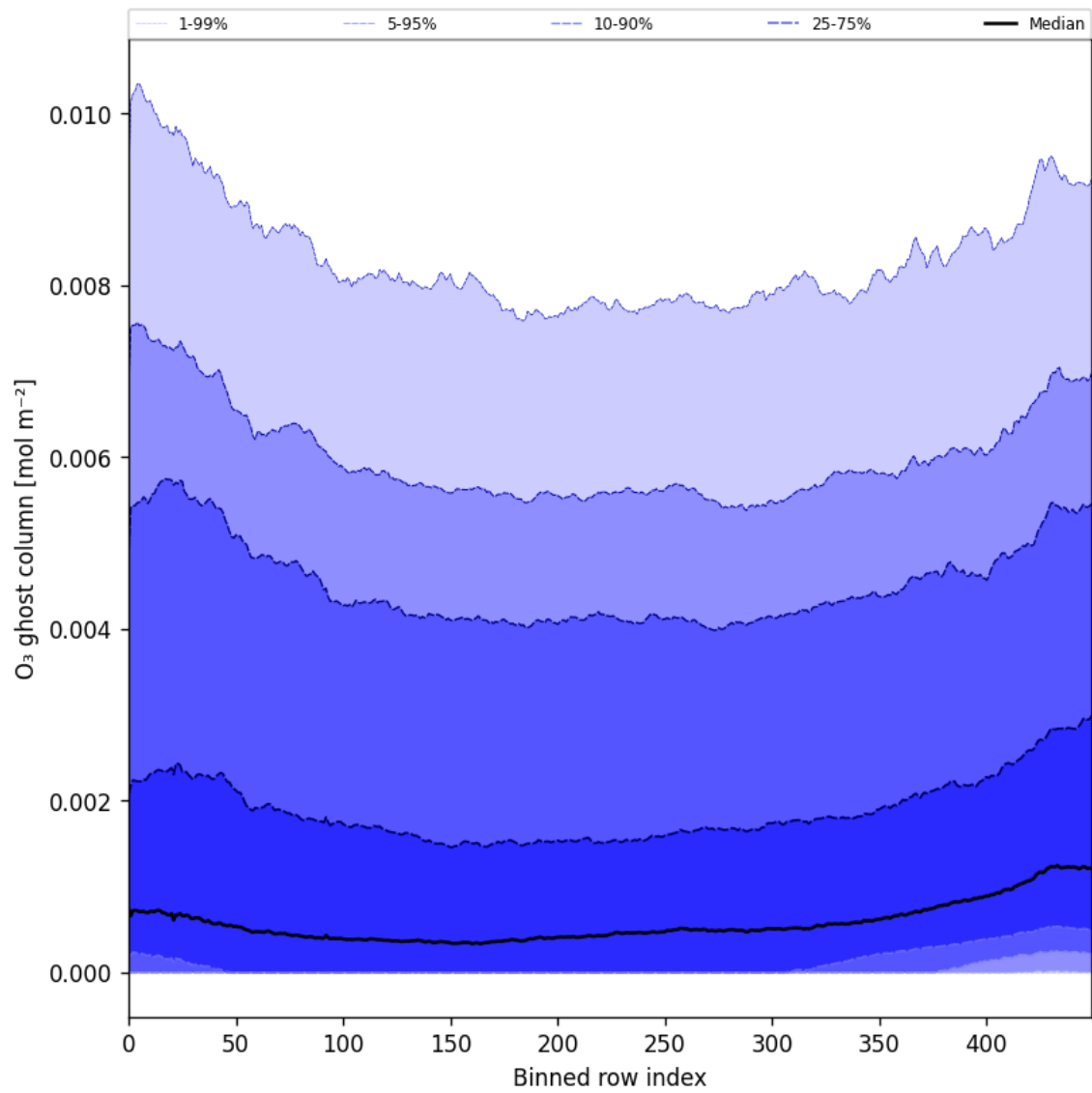
Figure 32: Along track statistics of “O 3 ghost column” for 2025-10-17 to 2025-10-19
