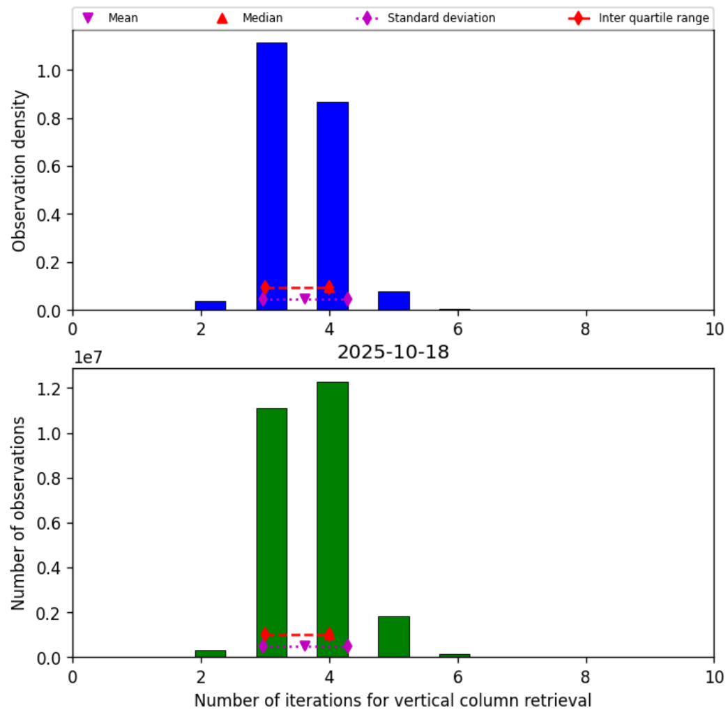
Figure 26: Histogram of “Number of iterations for vertical column retrieval” for 2025-10-17 to 2025-10-19
