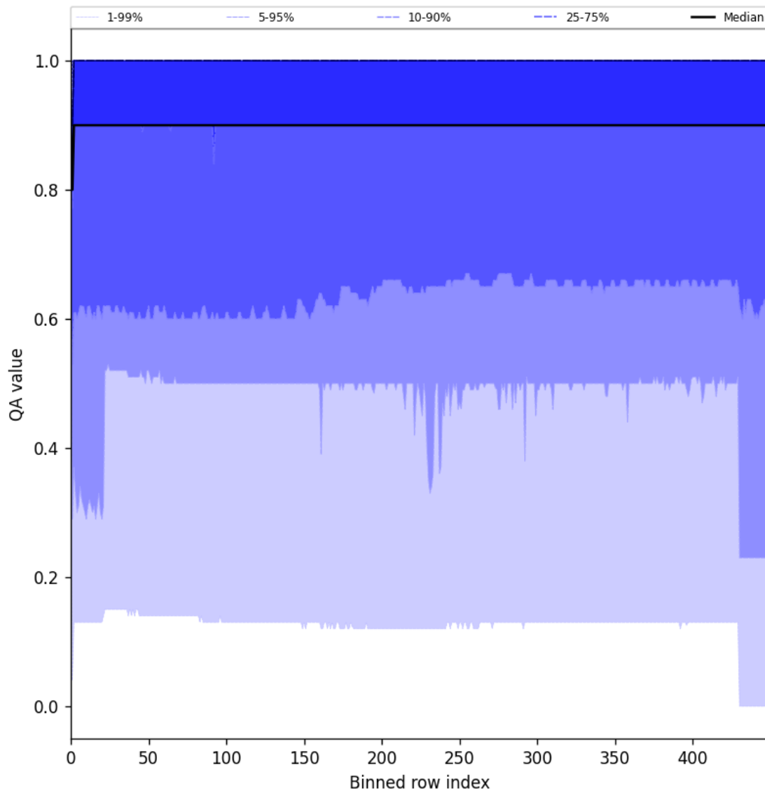
Figure 27: Along track statistics of “QA value” for 2025-10-17 to 2025-10-19
