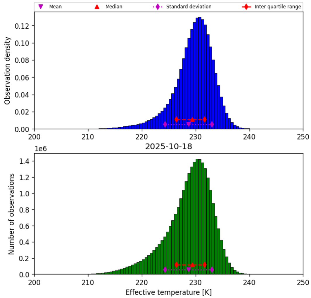
Figure 24: Histogram of “Effective temperature” for 2025-10-17 to 2025-10-19
