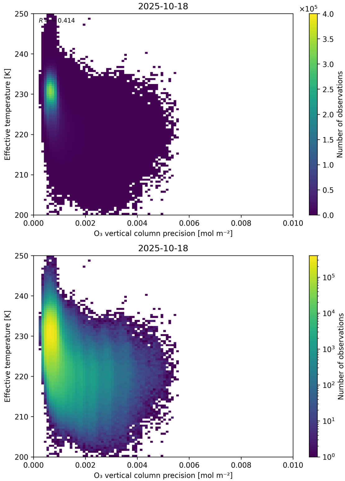
Figure 42: Scatter density plot of “ O_3 vertical column precision” against “Effective temperature” for 2025-10-17 to 2025-10-19.
