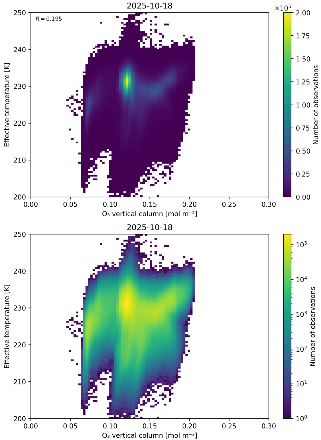
Figure 39: Scatter density plot of “O 3 vertical column” against “Effective temperature” for 2025-10-17 to 2025-10-19.
