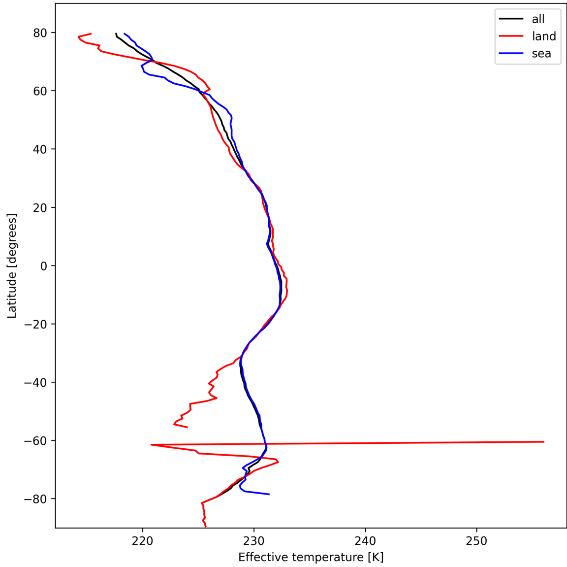
Figure 17: Zonal average of “Effective temperature” for 2025-10-17 to 2025-10-19.
