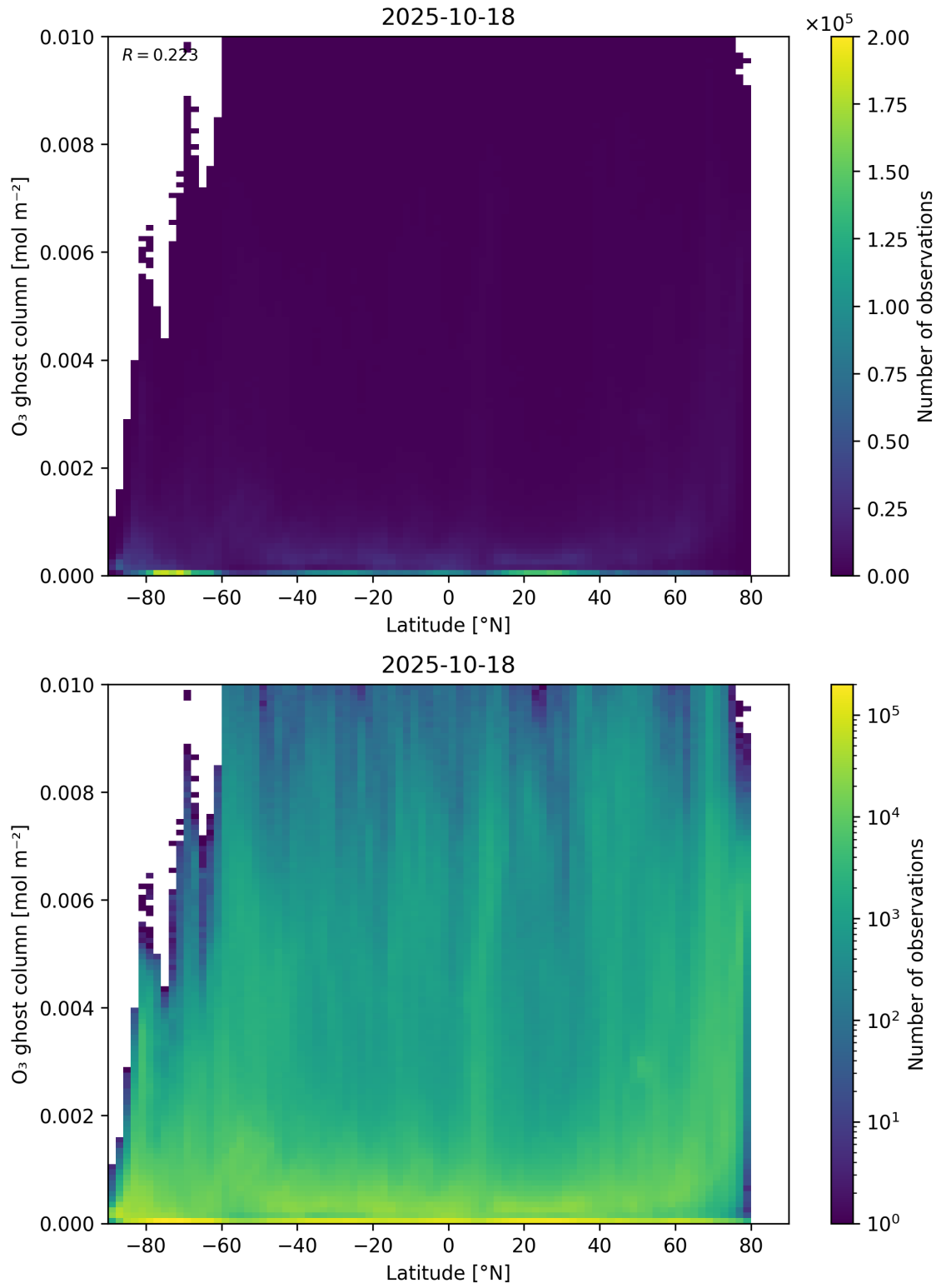
Figure 35: Scatter density plot of “Latitude” against “O 3 ghost column” for 2025-10-17 to 2025-10-19.
