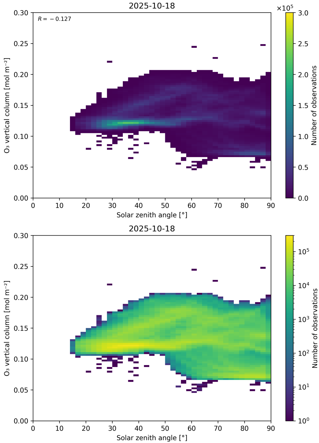
Figure 47: Scatter density plot of “Solar zenith angle” against “O 3 vertical column” for 2025-10-17 to 2025-10-19.
