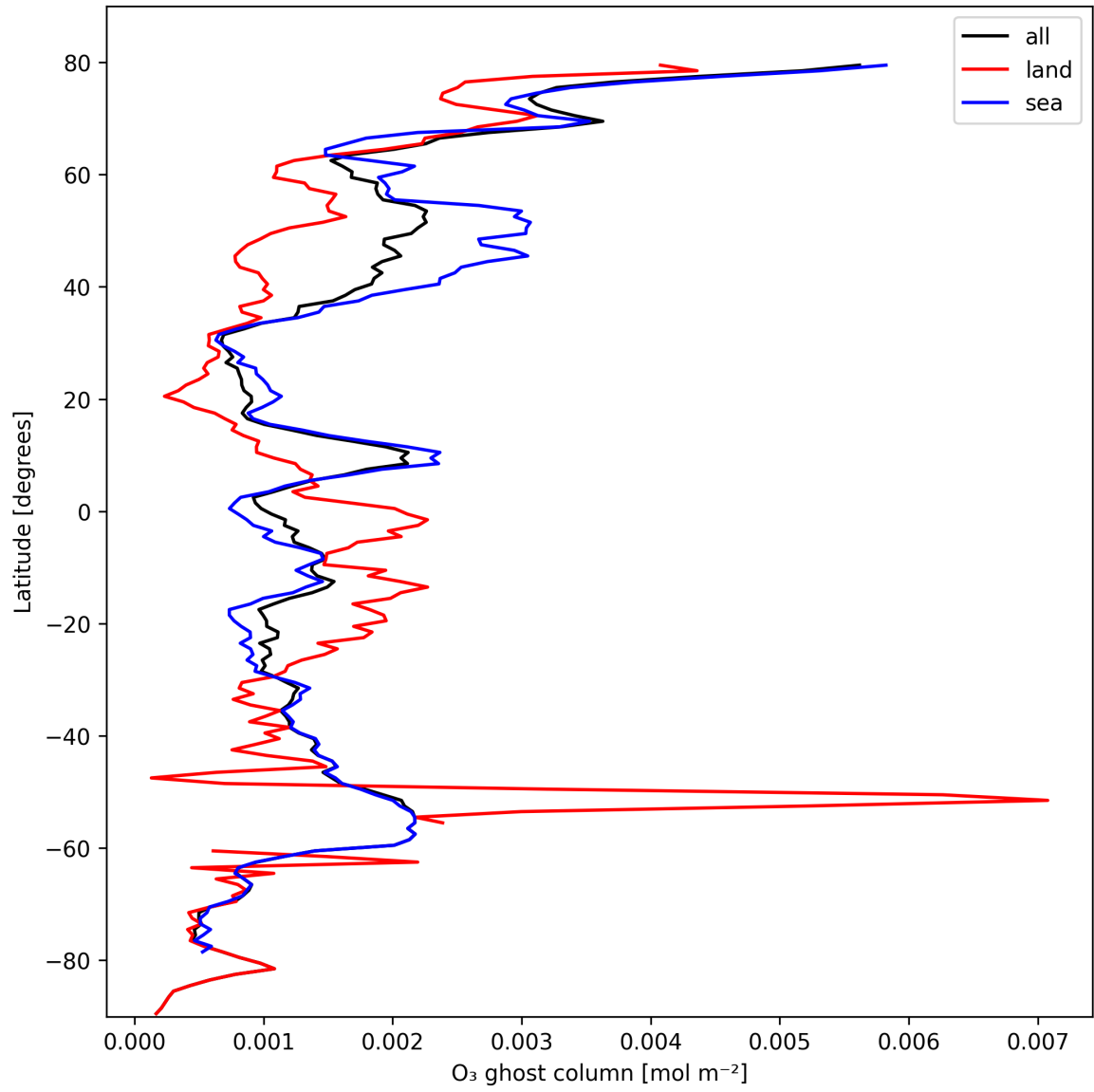
Figure 18: Zonal average of “O 3 ghost column” for 2025-10-17 to 2025-10-19.
