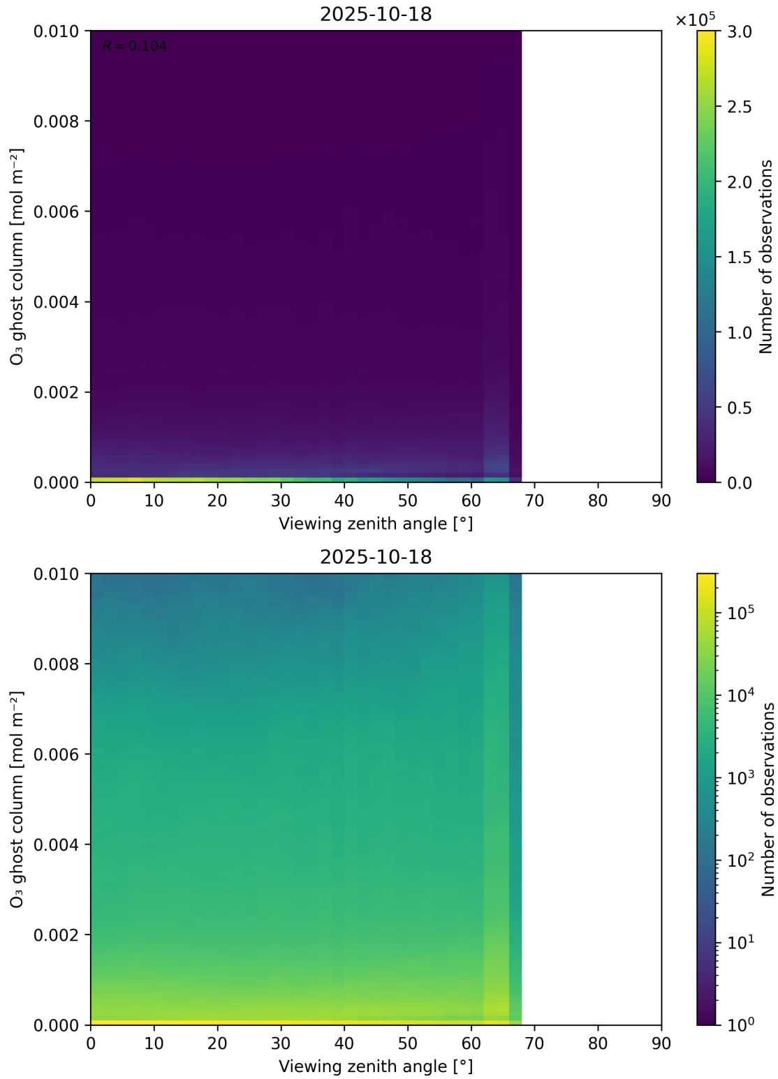
Figure 51: Scatter density plot of “Viewing zenith angle” against “O 3 ghost column” for 2025-10-17 to 2025-10-19.
