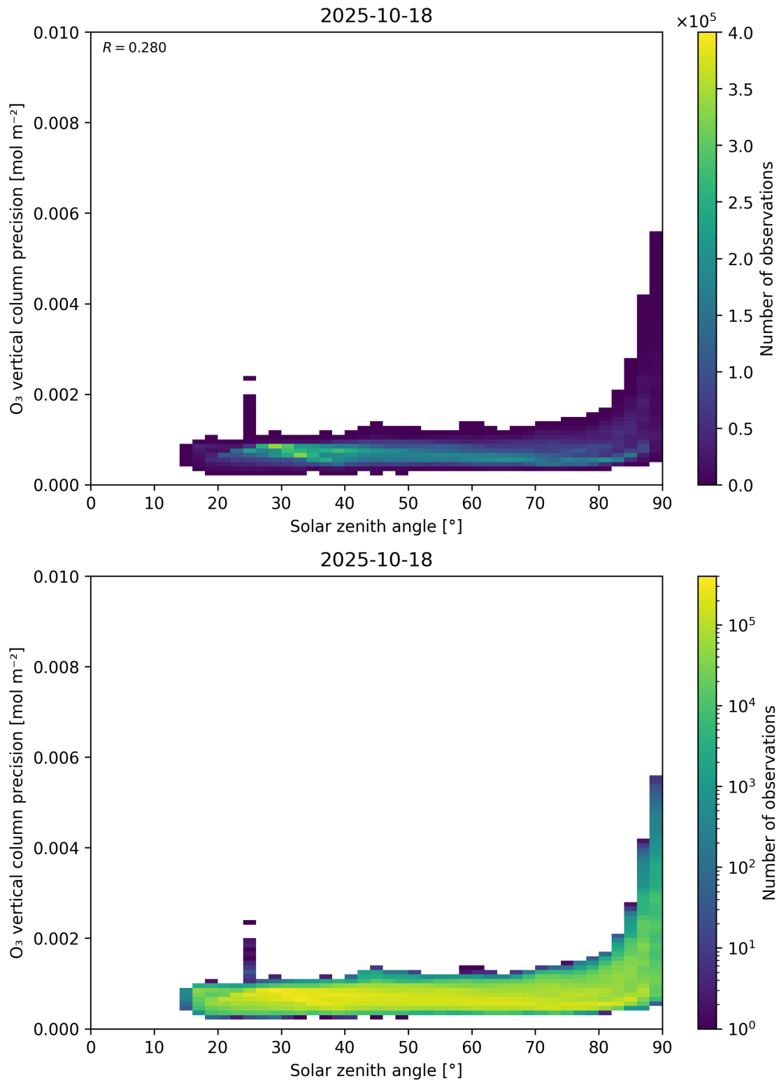
Figure 48: Scatter density plot of “Solar zenith angle” against “O 3 vertical column precision” for 2025-10-17 to 2025-10-19.
