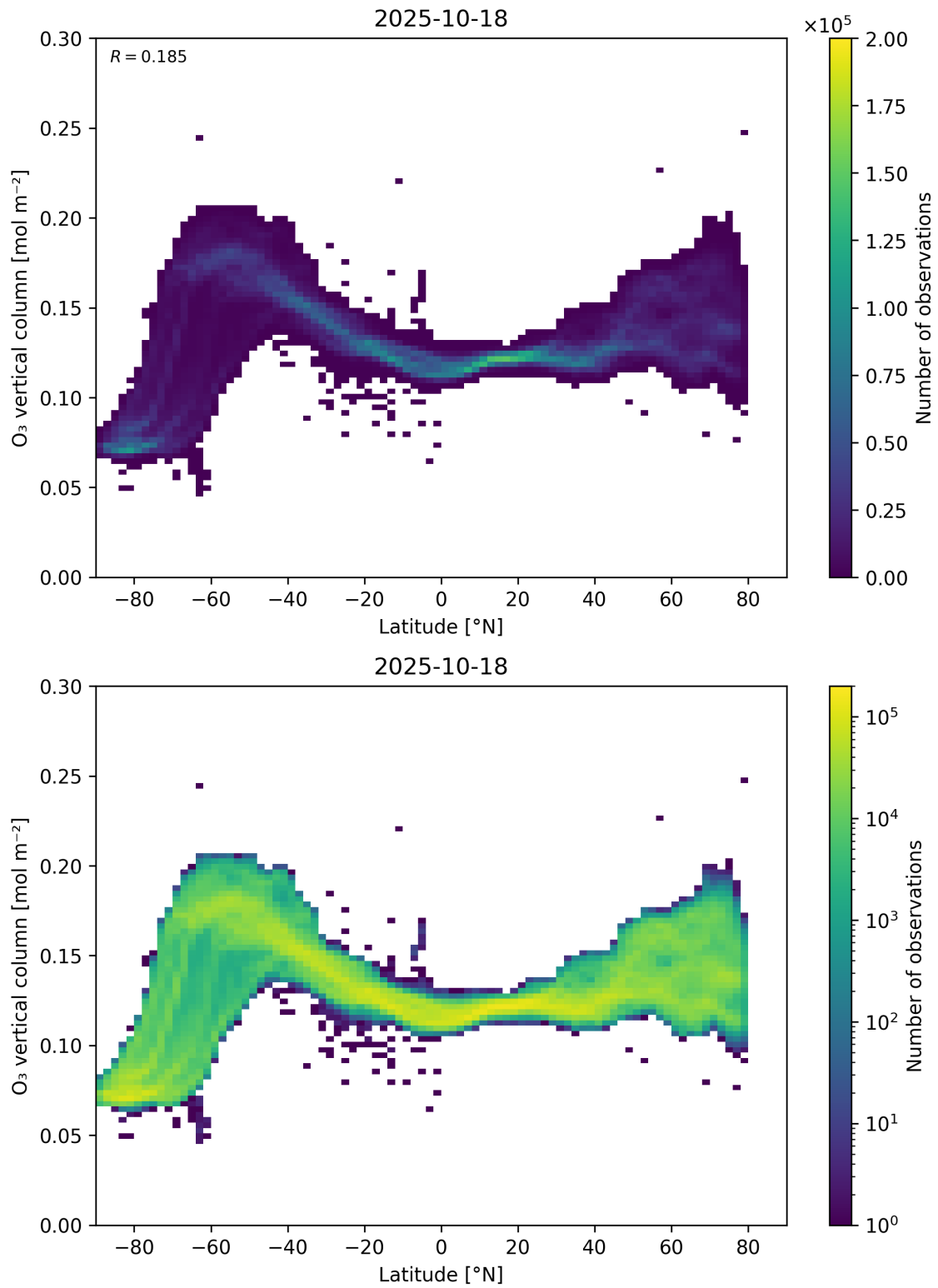
Figure 36: Scatter density plot of “Latitude” against “O 3 vertical column” for 2025-10-17 to 2025-10-19.
