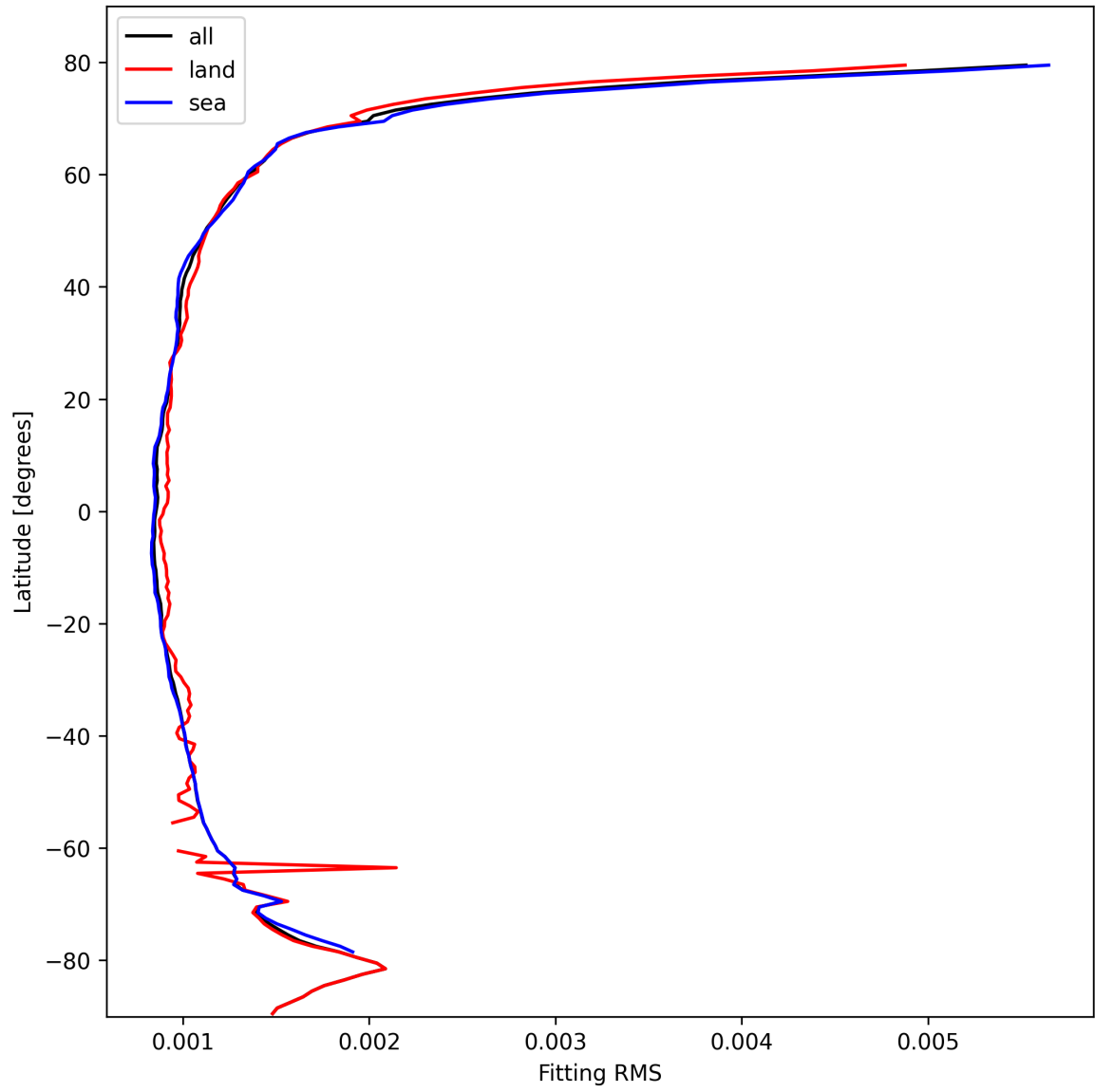
Figure 16: Zonal average of “Fitting RMS” for 2025-10-17 to 2025-10-19.
