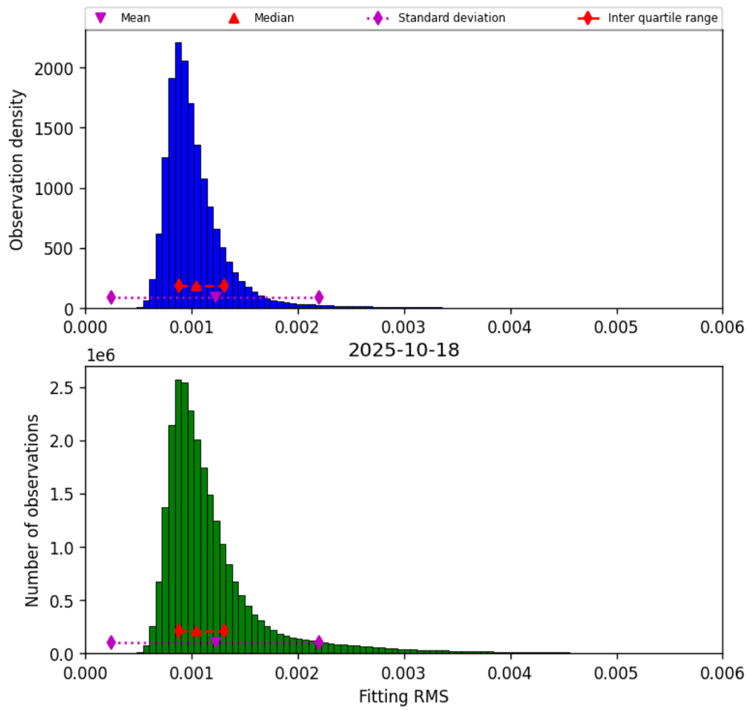
Figure 23: Histogram of “Fitting RMS” for 2025-10-17 to 2025-10-19
