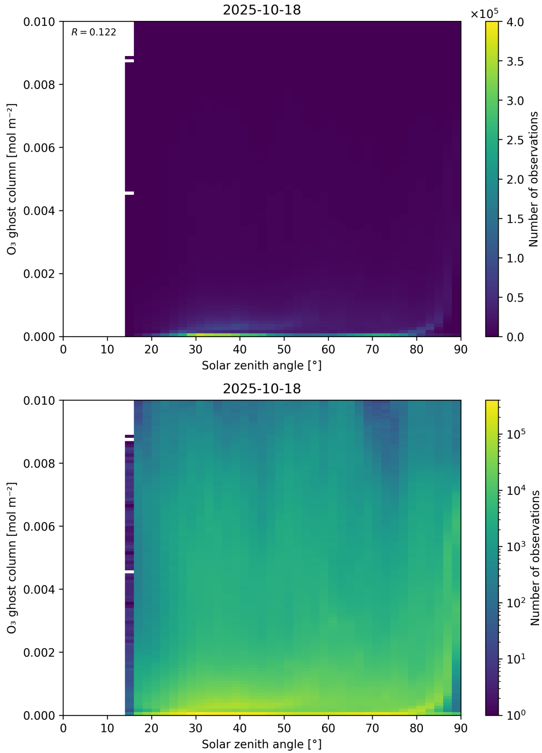
Figure 46: Scatter density plot of “Solar zenith angle” against “O 3 ghost column” for 2025-10-17 to 2025-10-19.
