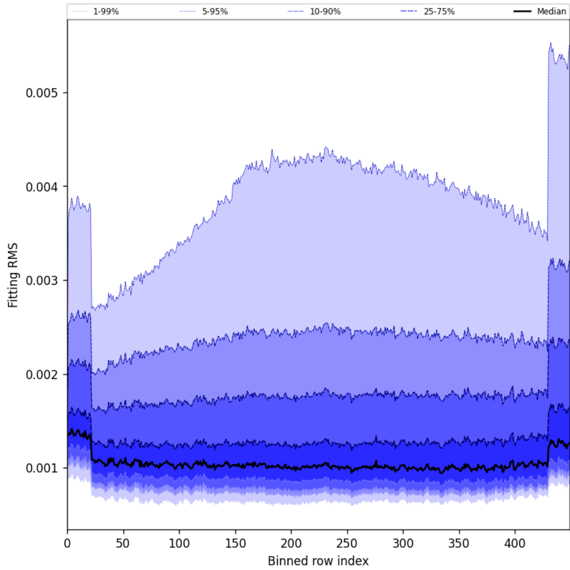
Figure 30: Along track statistics of “Fitting RMS” for 2025-10-17 to 2025-10-19
