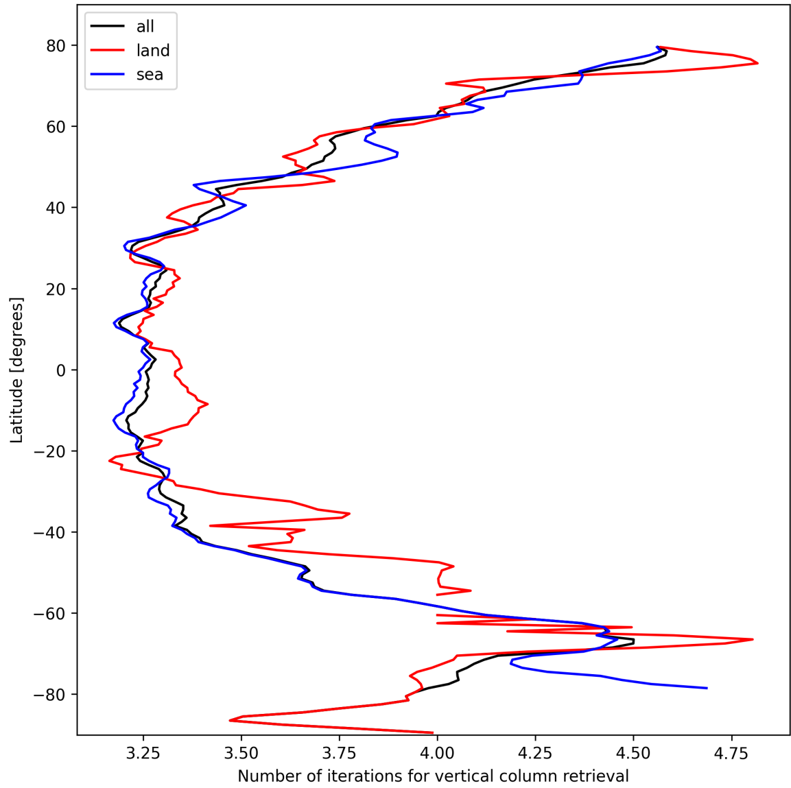
Figure 19: Zonal average of “Number of iterations for vertical column retrieval” for 2025-10-17 to 2025-10-19.
