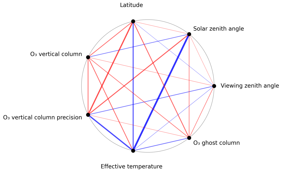
Figure 1: Map of correlation graph for 2025-10-17 to 2025-10-19.
