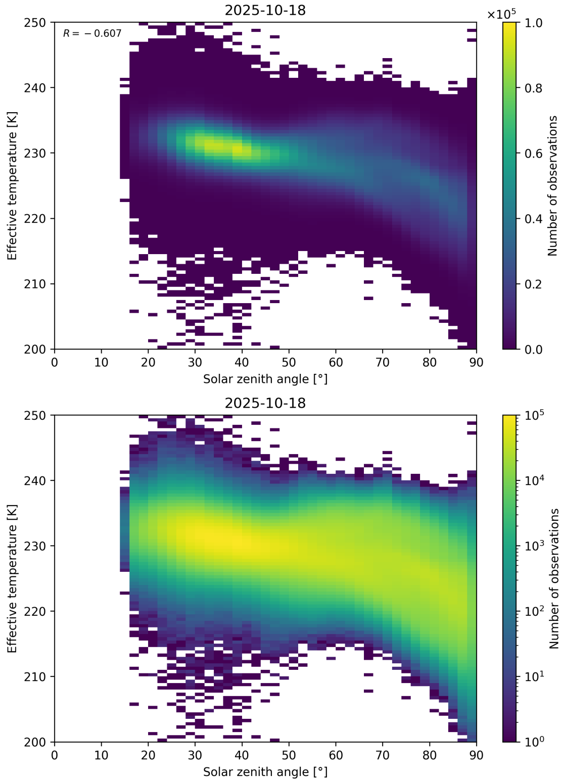
Figure 45: Scatter density plot of “Solar zenith angle” against “Effective temperature” for 2025-10-17 to 2025-10-19.
