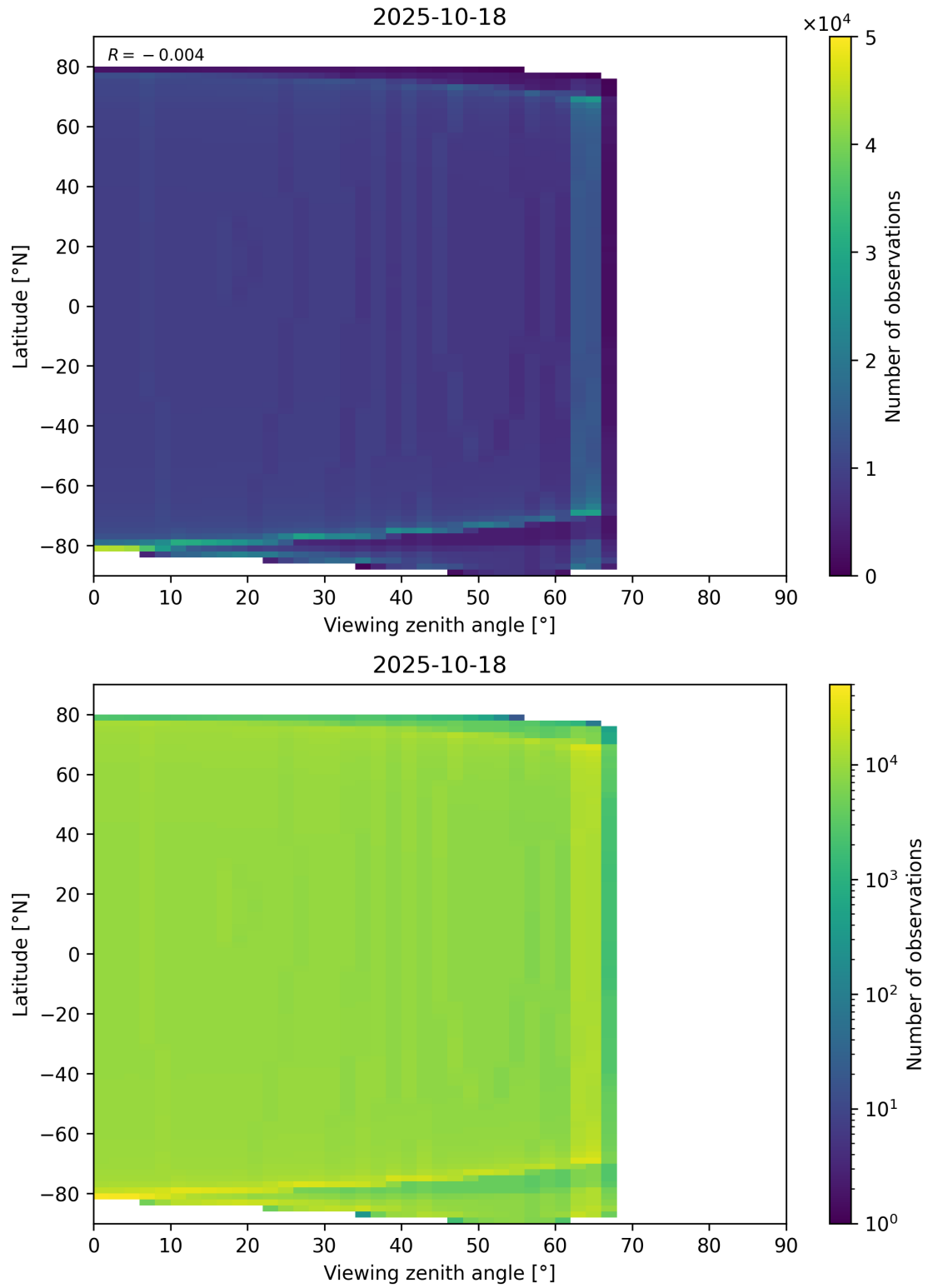
Figure 49: Scatter density plot of “Viewing zenith angle” against “Latitude” for 2025-10-17 to 2025-10-19.
