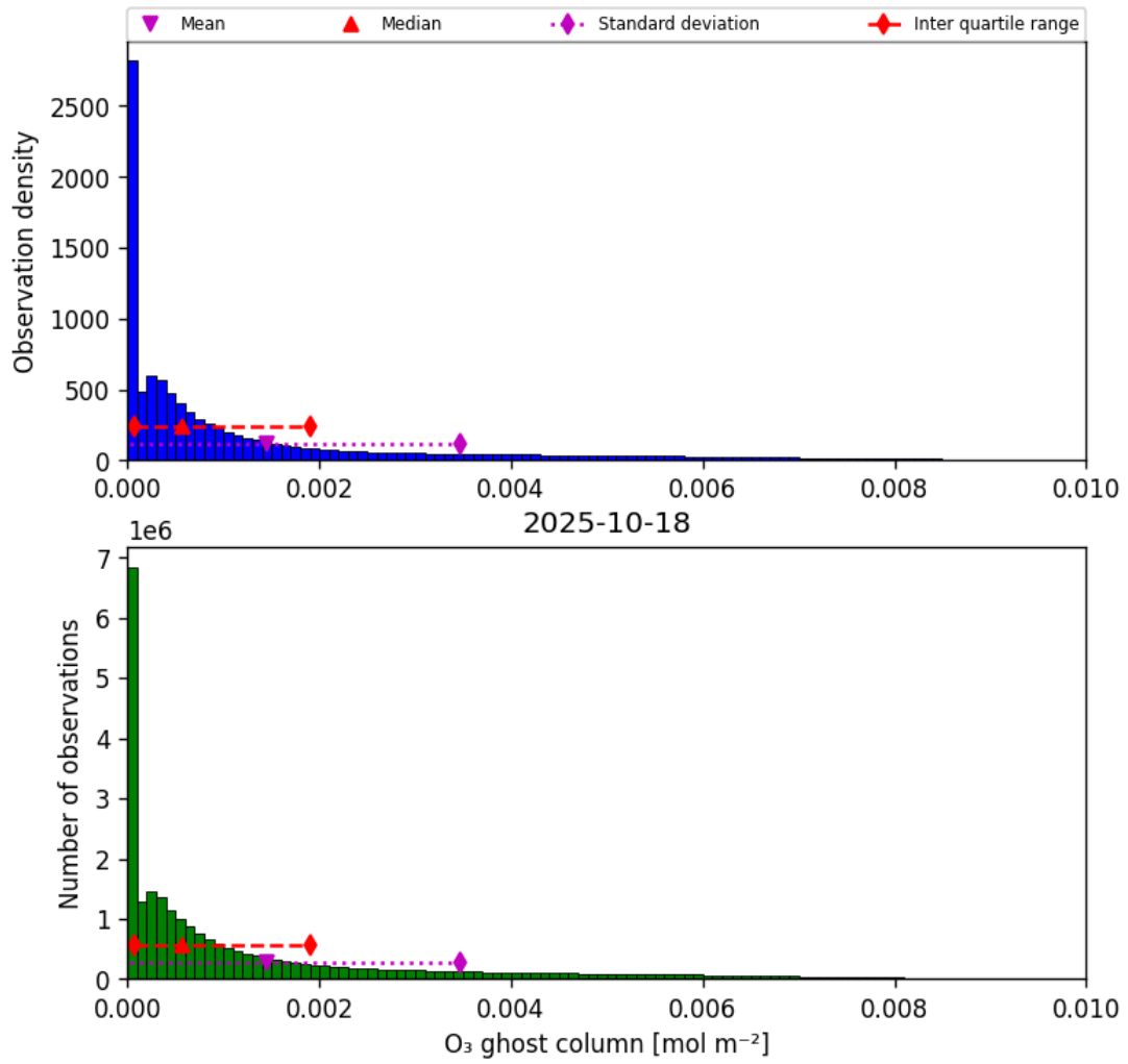
Figure 25: Histogram of “O 3 ghost column” for 2025-10-17 to 2025-10-19
