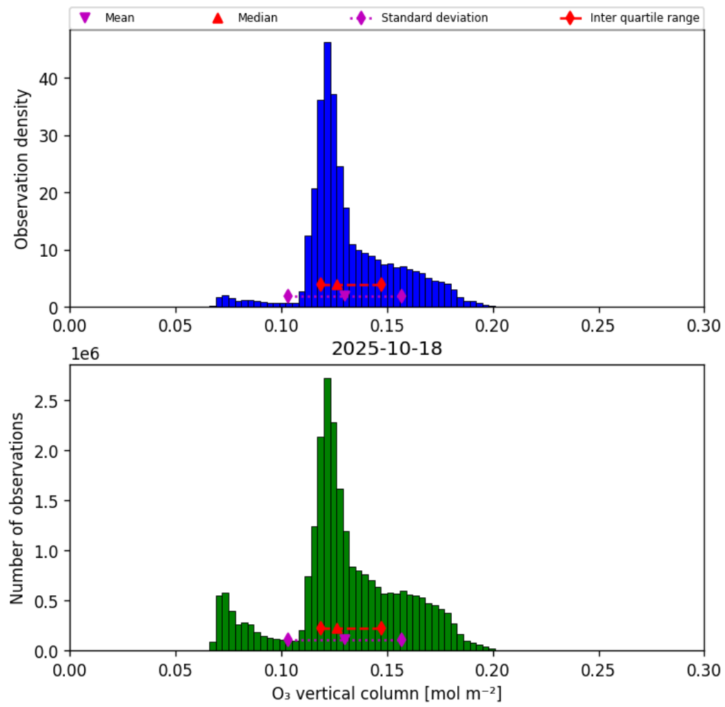
Figure 21: Histogram of “O 3 vertical column” for 2025-10-17 to 2025-10-19
