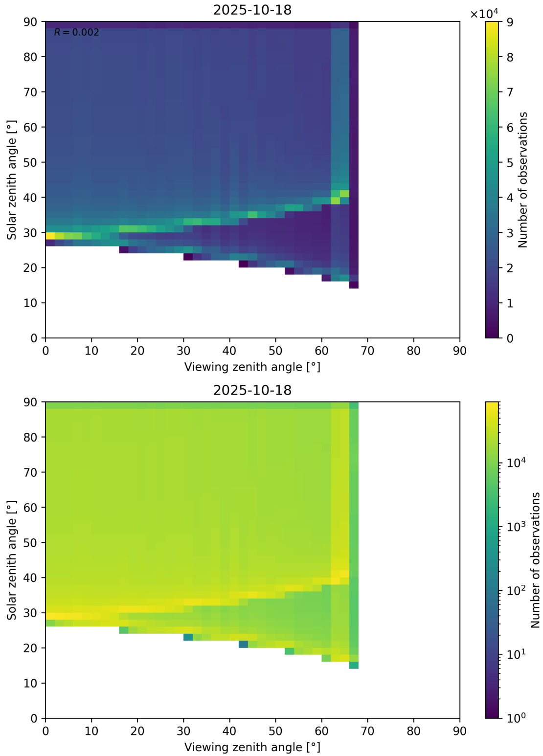
Figure 54: Scatter density plot of “Viewing zenith angle” against “Solar zenith angle” for 2025-10-17 to 2025-10-19.
