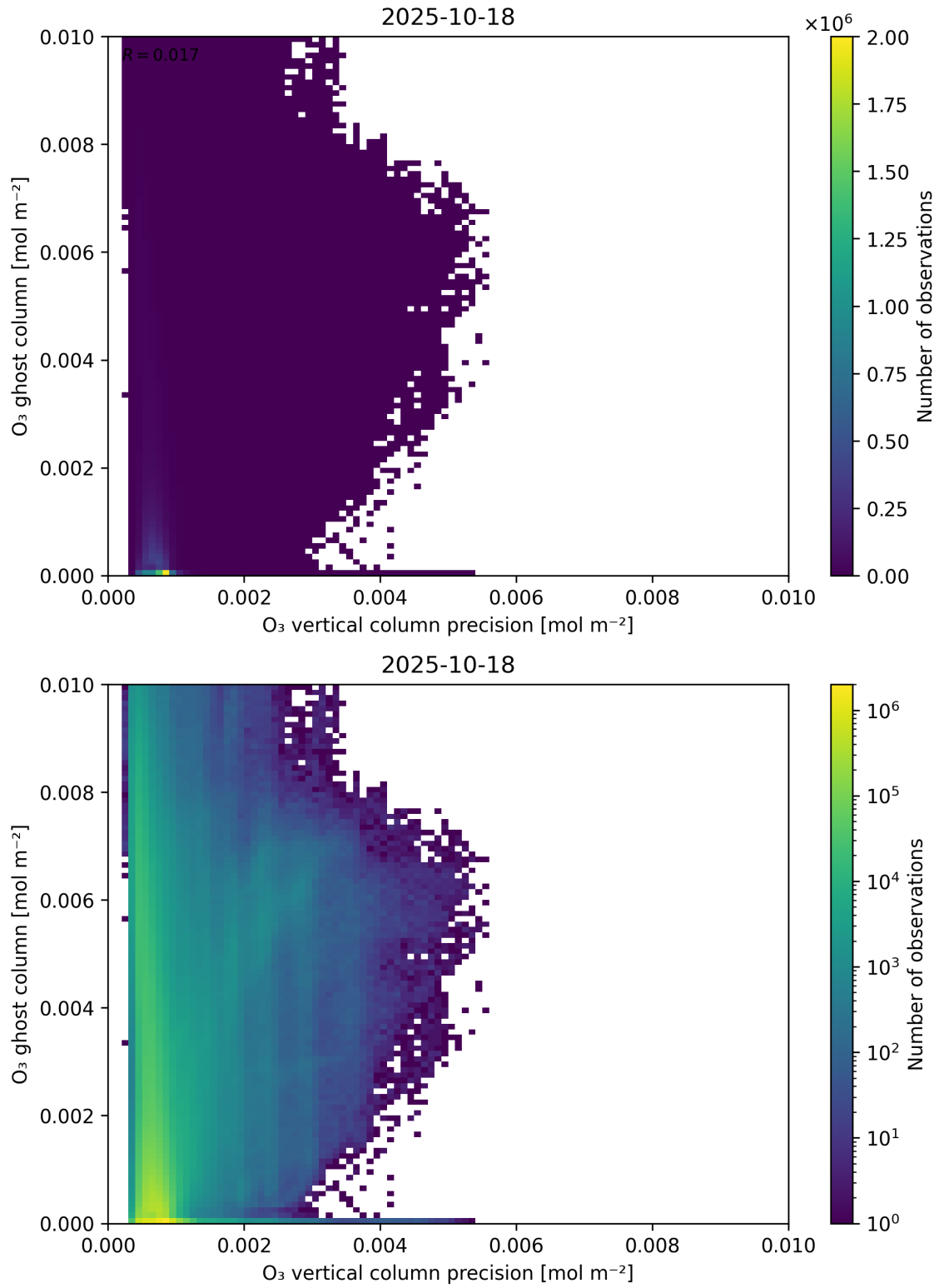
Figure 43: Scatter density plot of “O 3 vertical column precision” against “O 3 ghost column” for 2025-10-17 to 2025-10-19.
