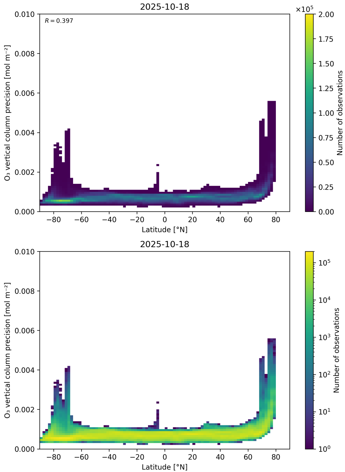
Figure 37: Scatter density plot of “Latitude” against “O 3 vertical column precision” for 2025-10-17 to 2025-10-19.
