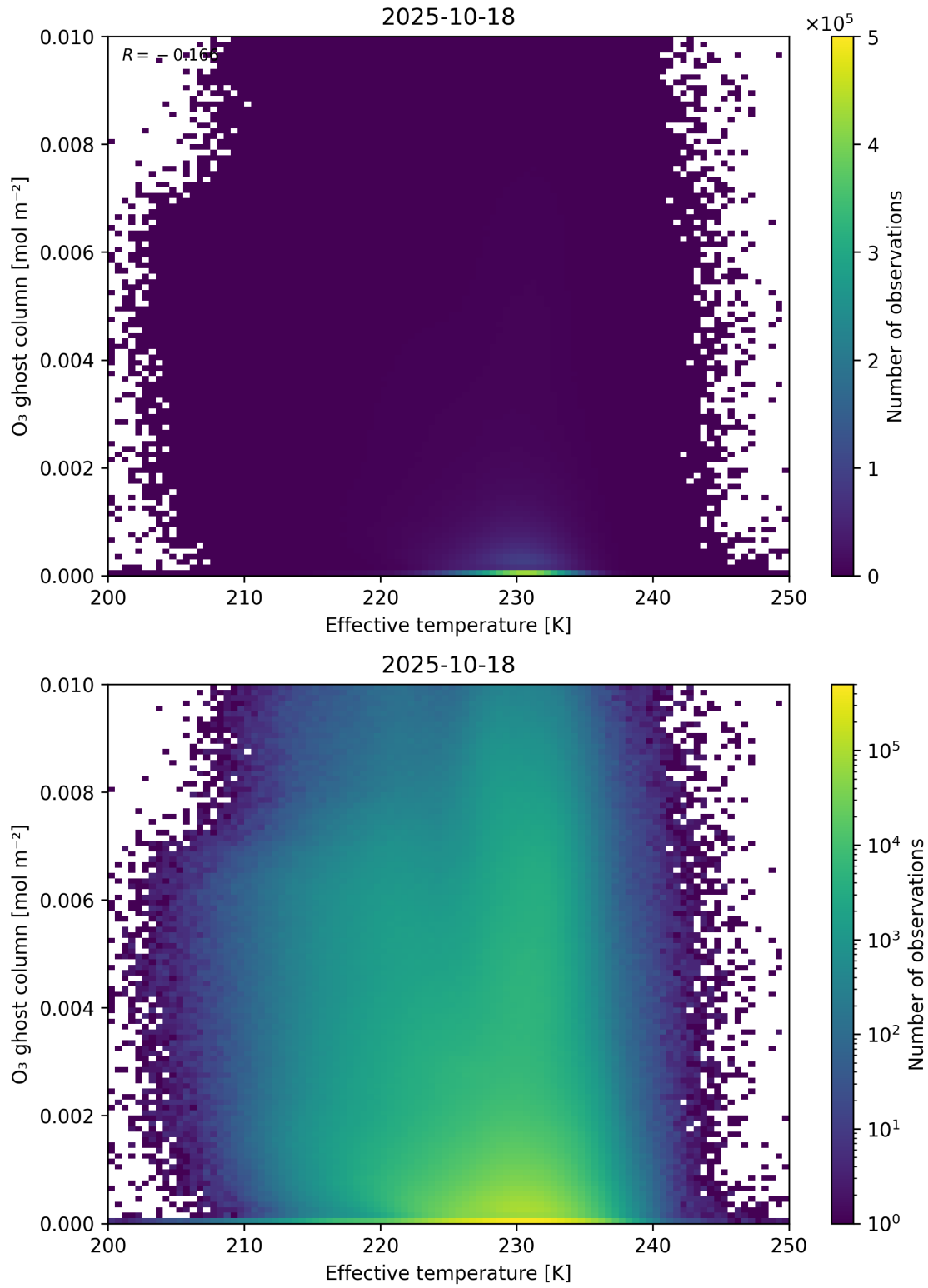
Figure 38: Scatter density plot of “Effective temperature” against “O 3 ghost column” for 2025-10-17 to 2025-10-19.
