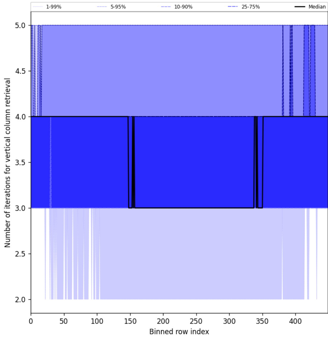
Figure 33: Along track statistics of “Number of iterations for vertical column retrieval” for 2025-10-17 to 2025-10-19
