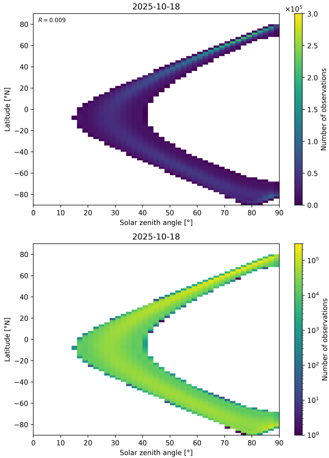
Figure 44: Scatter density plot of “Solar zenith angle” against “Latitude” for 2025-10-17 to 2025-10-19.
