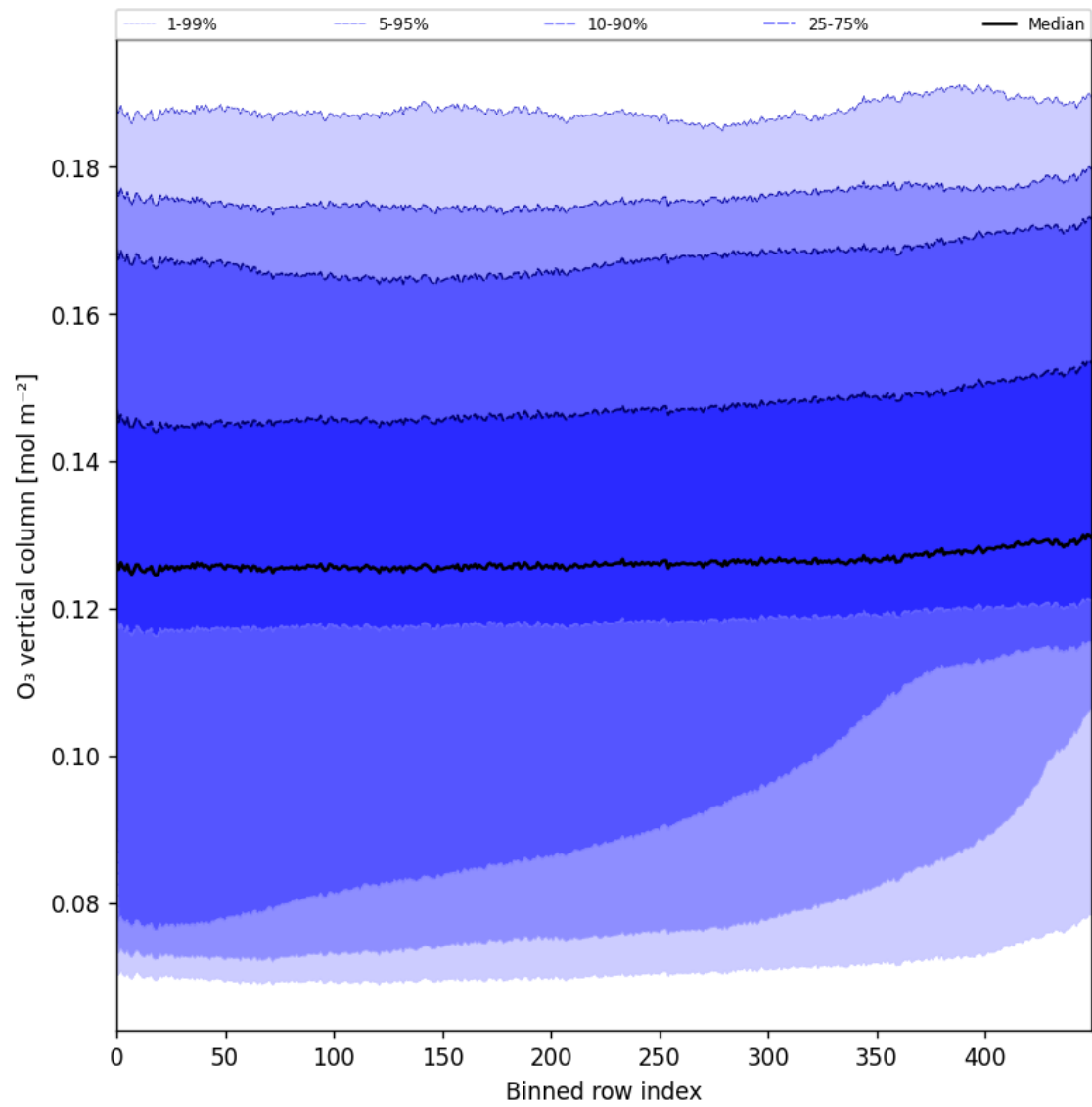
Figure 28: Along track statistics of “O 3 vertical column” for 2025-10-17 to 2025-10-19
