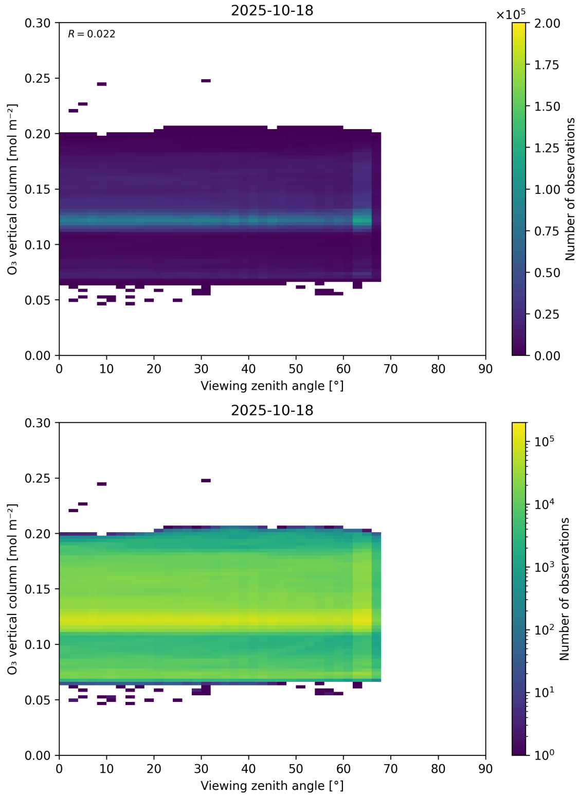
Figure 52: Scatter density plot of “Viewing zenith angle” against “O 3 vertical column” for 2025-10-17 to 2025-10-19.
