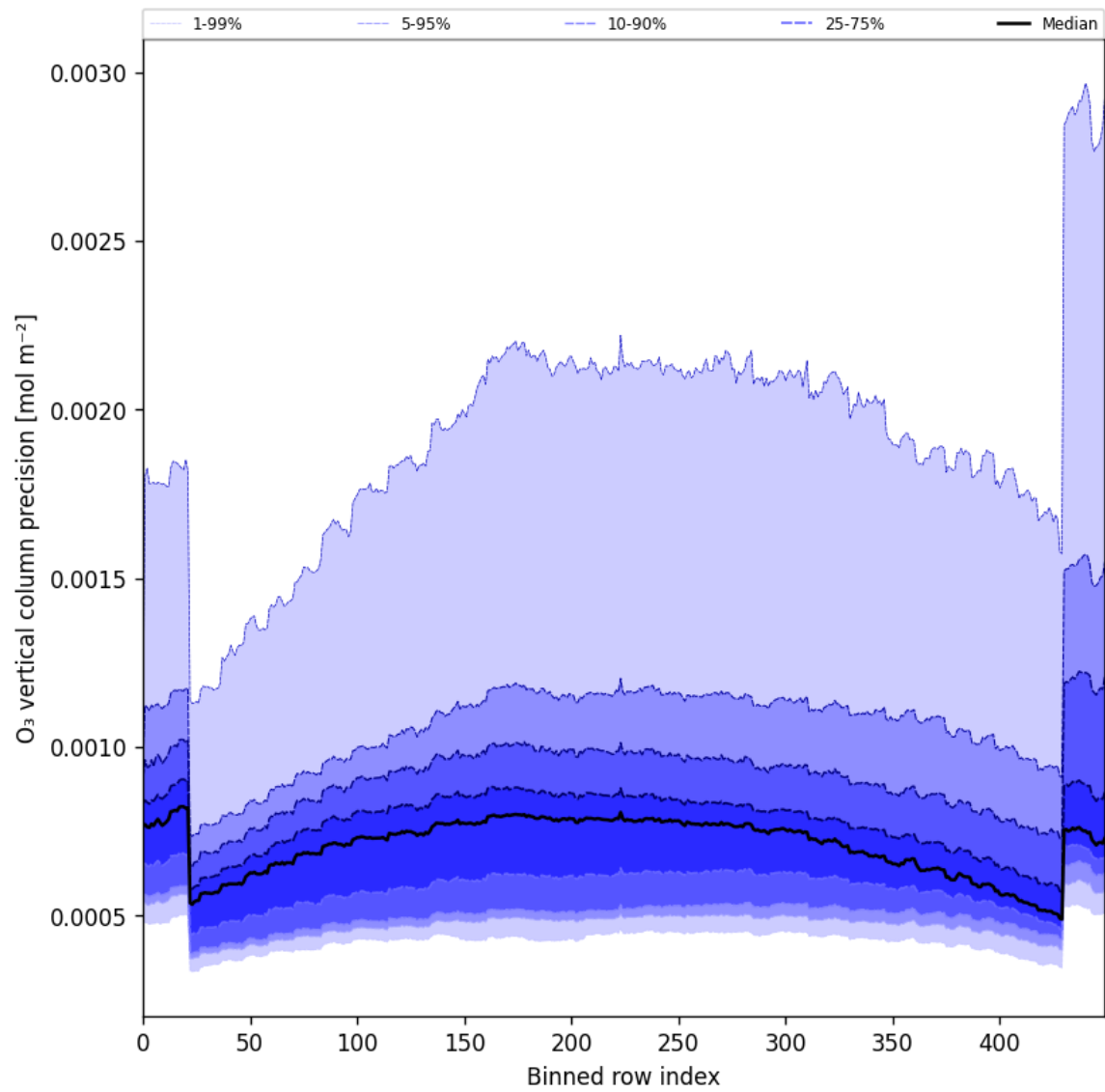
Figure 29: Along track statistics of “O 3 vertical column precision” for 2025-10-17 to 2025-10-19
