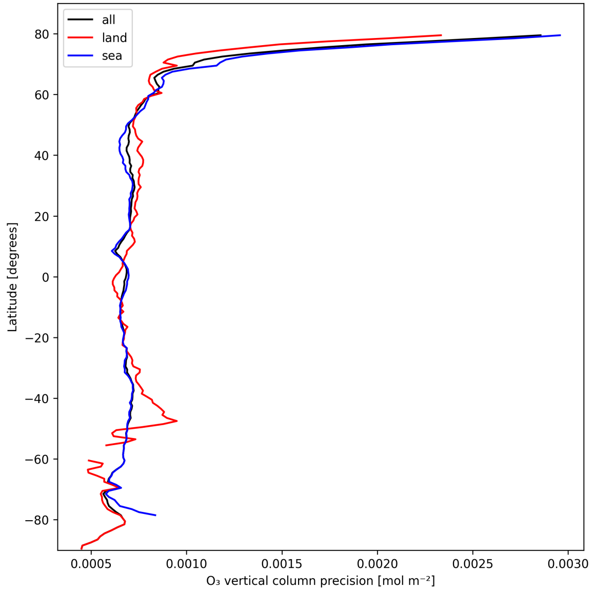
Figure 15: Zonal average of “O 3 vertical column precision” for 2025-10-17 to 2025-10-19.
