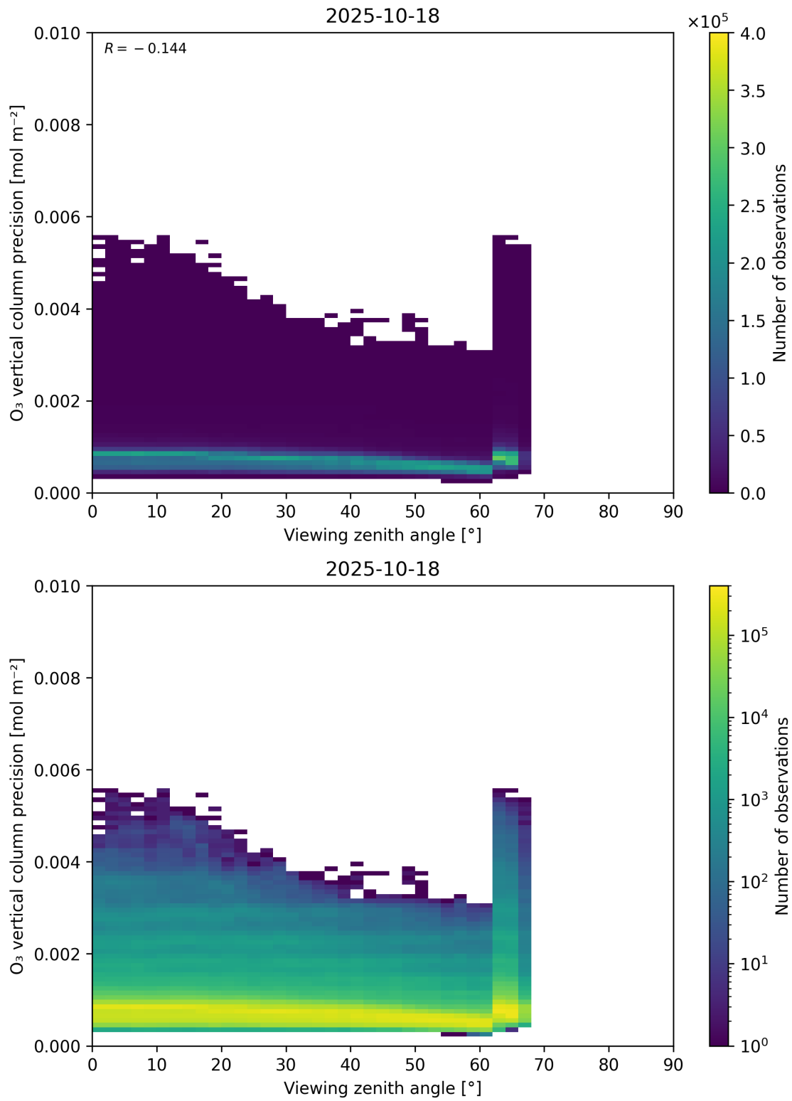
Figure 53: Scatter density plot of “Viewing zenith angle” against “O 3 vertical column precision” for 2025-10-17 to 2025-10-19.
