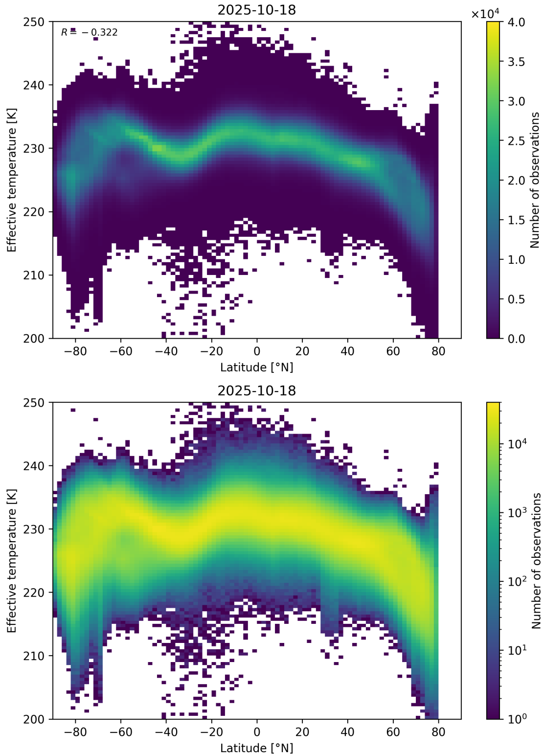
Figure 34: Scatter density plot of “Latitude” against “Effective temperature” for 2025-10-17 to 2025-10-19.
