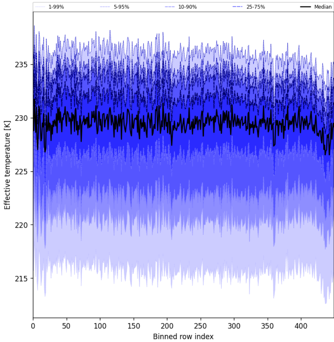
Figure 31: Along track statistics of “Effective temperature” for 2025-10-17 to 2025-10-19
