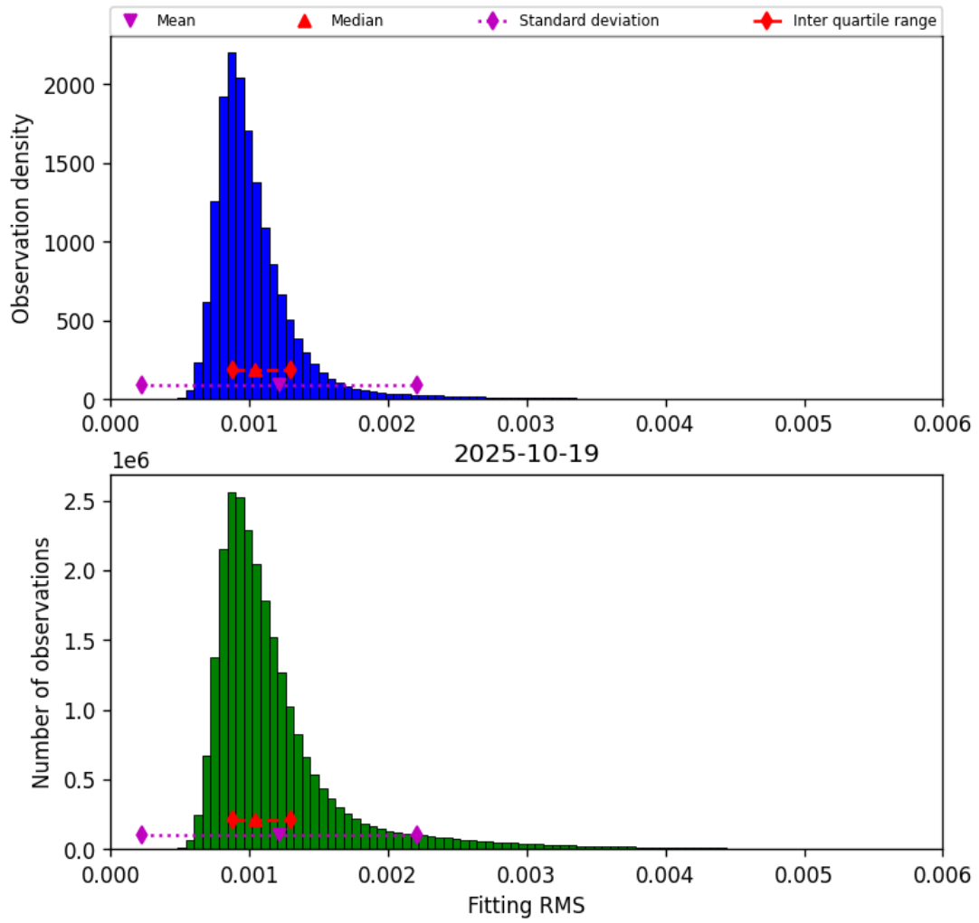
Figure 23: Histogram of “Fitting RMS” for 2025-10-18 to 2025-10-20
