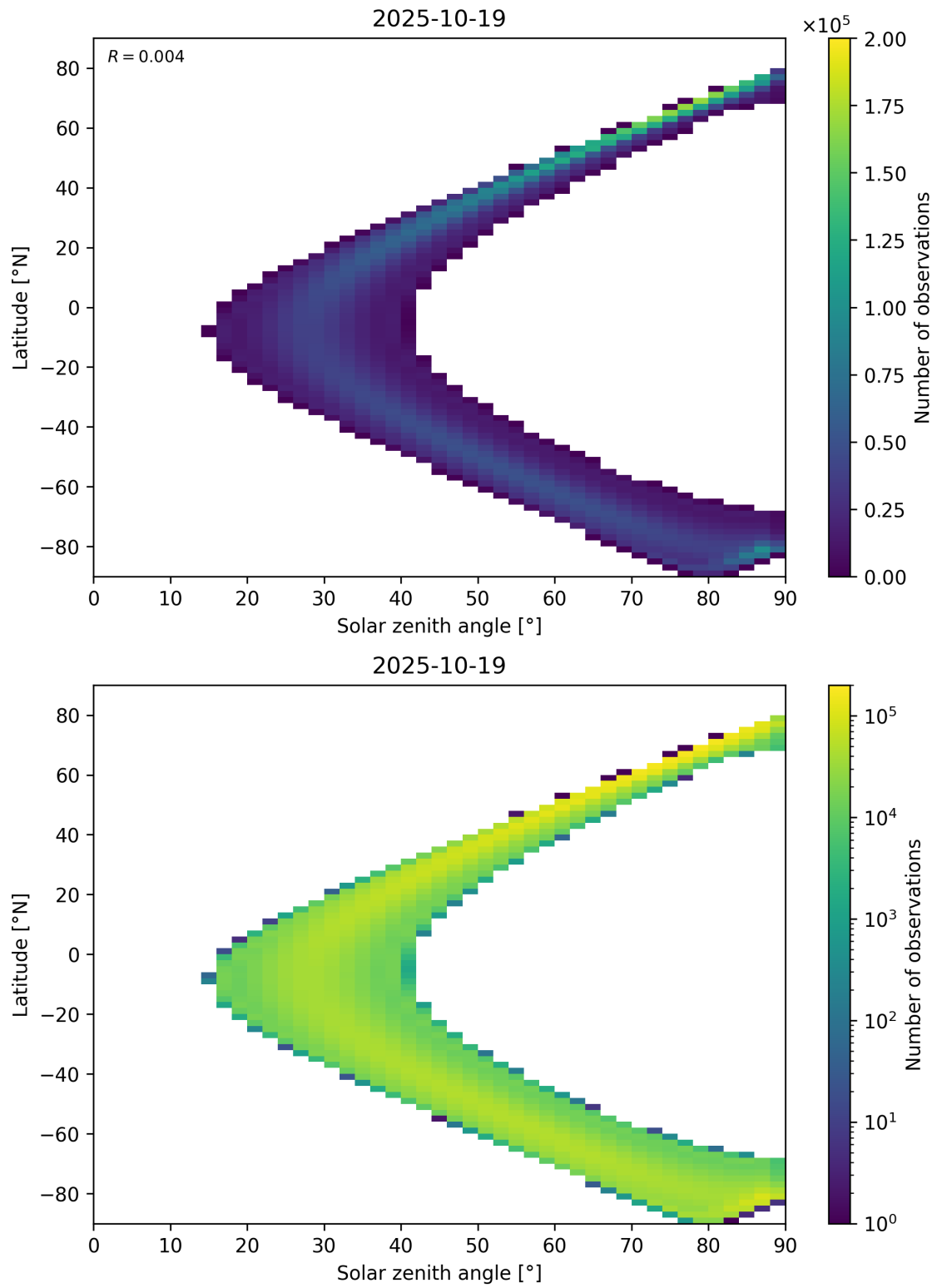
Figure 44: Scatter density plot of “Solar zenith angle” against “Latitude” for 2025-10-18 to 2025-10-20.
