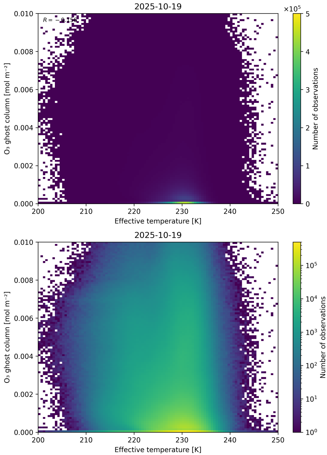
Figure 38: Scatter density plot of “Effective temperature” against “O 3 ghost column” for 2025-10-18 to 2025-10-20.
