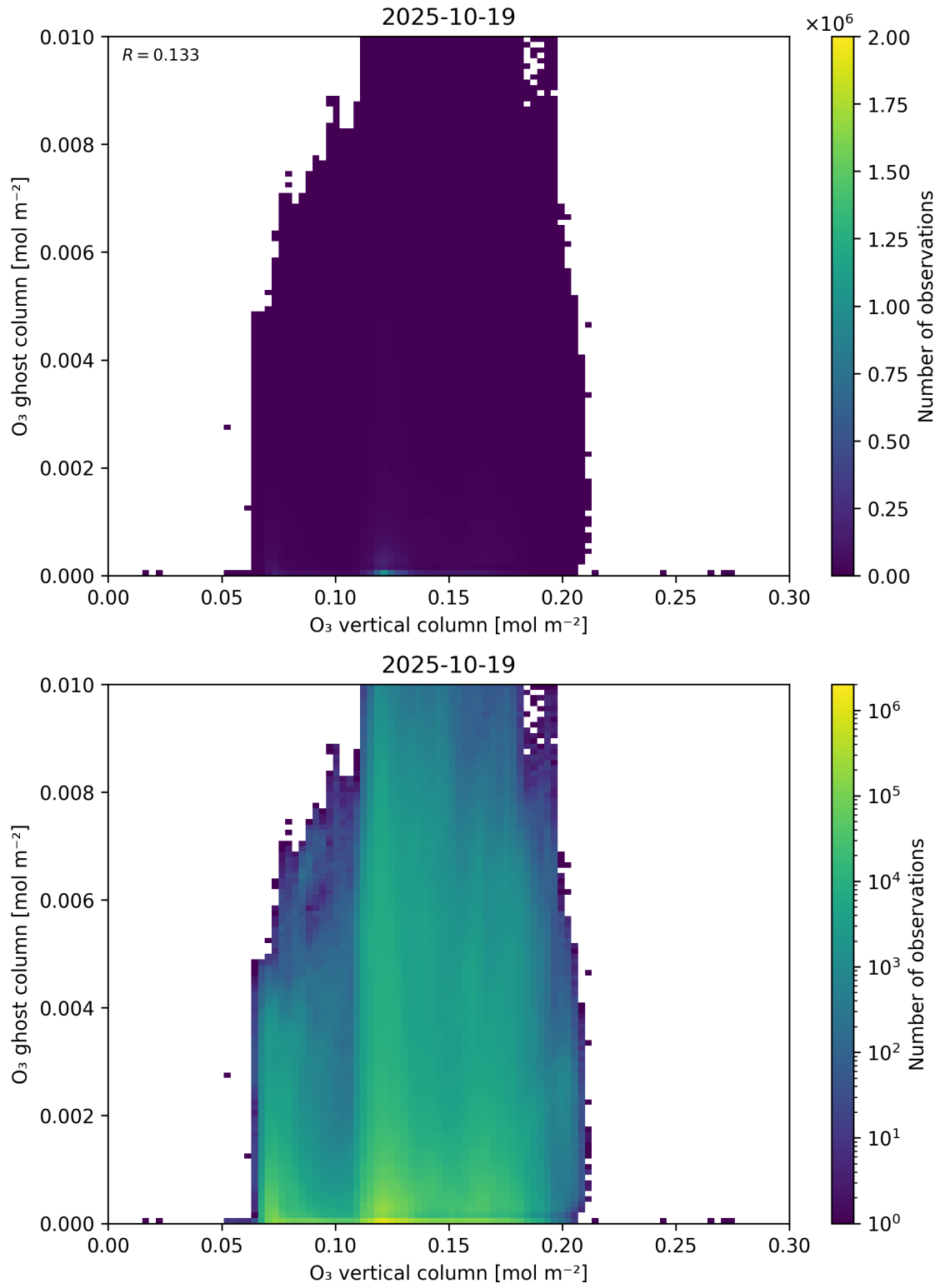
Figure 40: Scatter density plot of “O 3 vertical column” against “O 3 ghost column” for 2025-10-18 to 2025-10-20.
