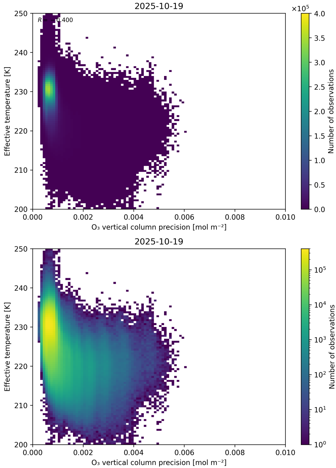
Figure 42: Scatter density plot of “ O_3 vertical column precision” against “Effective temperature” for 2025-10-18 to 2025-10-20.
