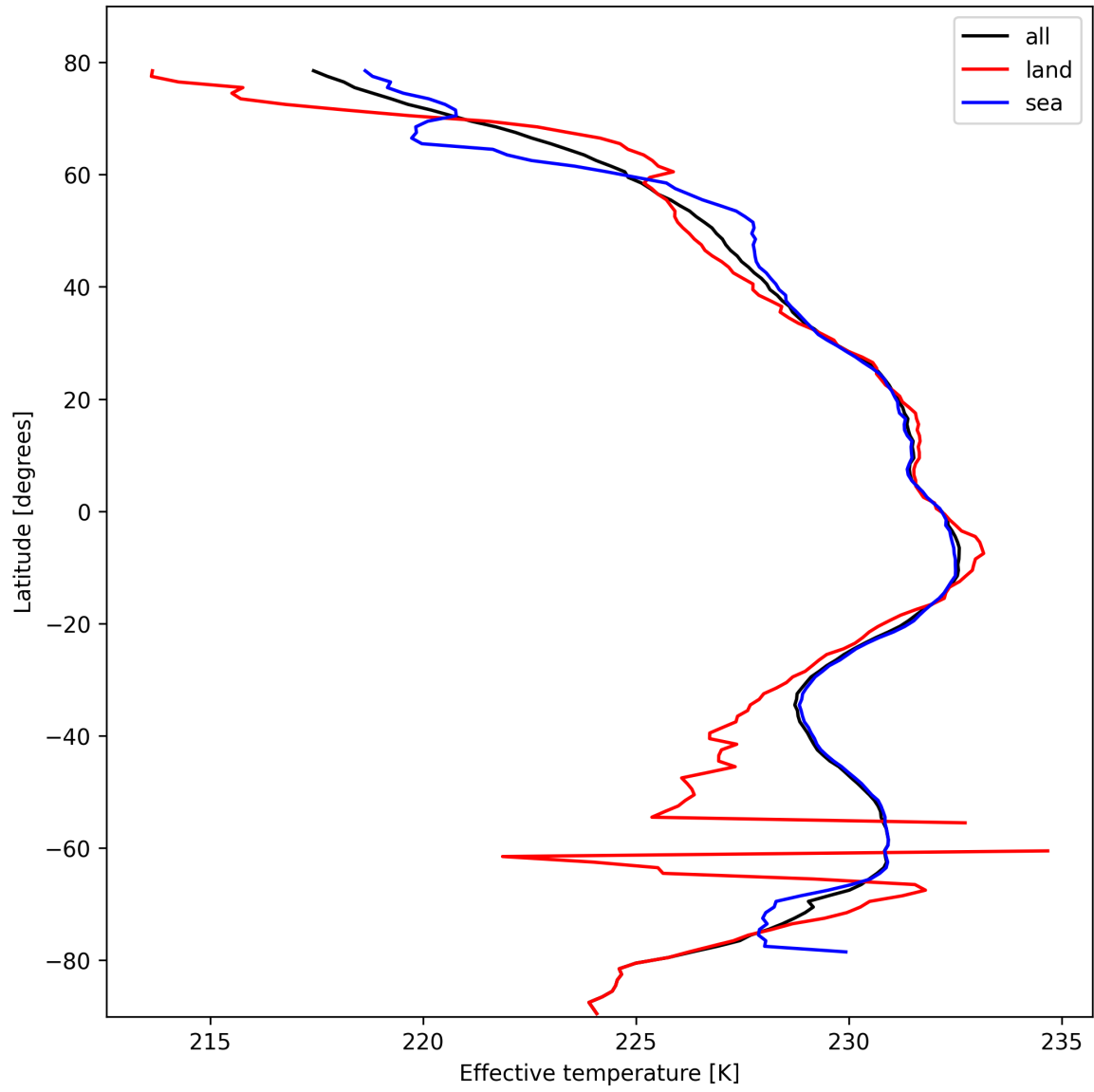
Figure 17: Zonal average of “Effective temperature” for 2025-10-18 to 2025-10-20.
