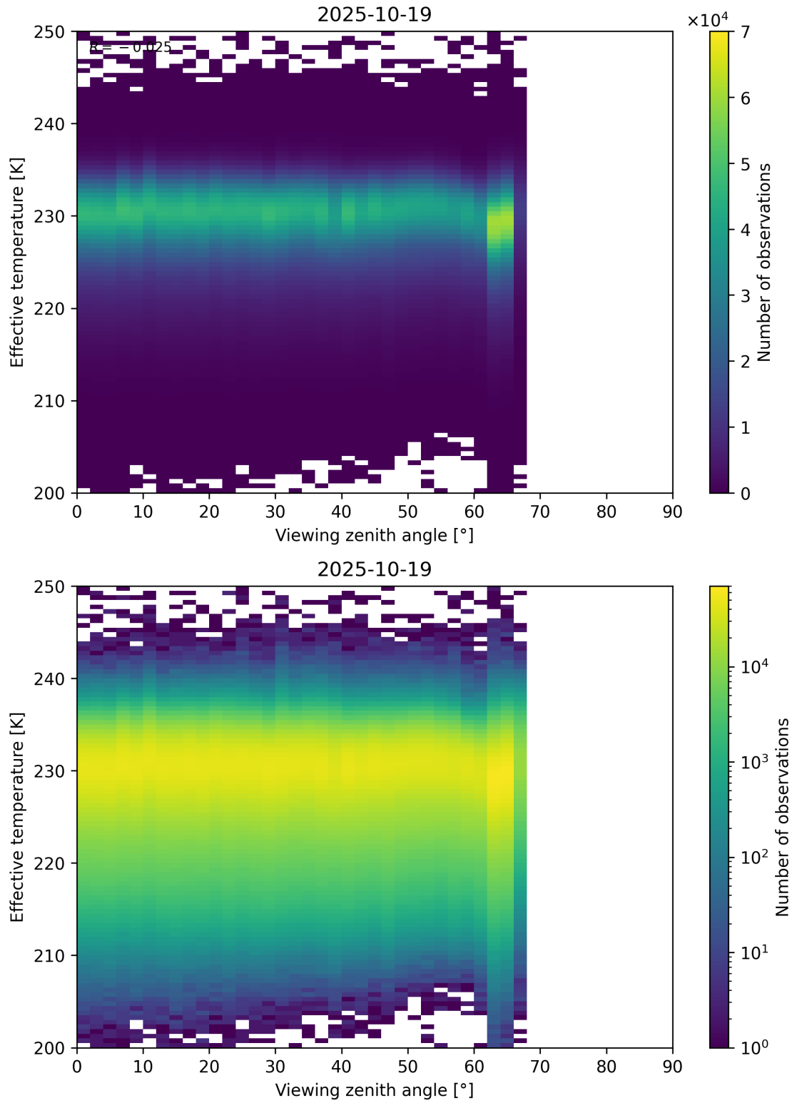
Figure 50: Scatter density plot of “Viewing zenith angle” against “Effective temperature” for 2025-10-18 to 2025-10-20.
