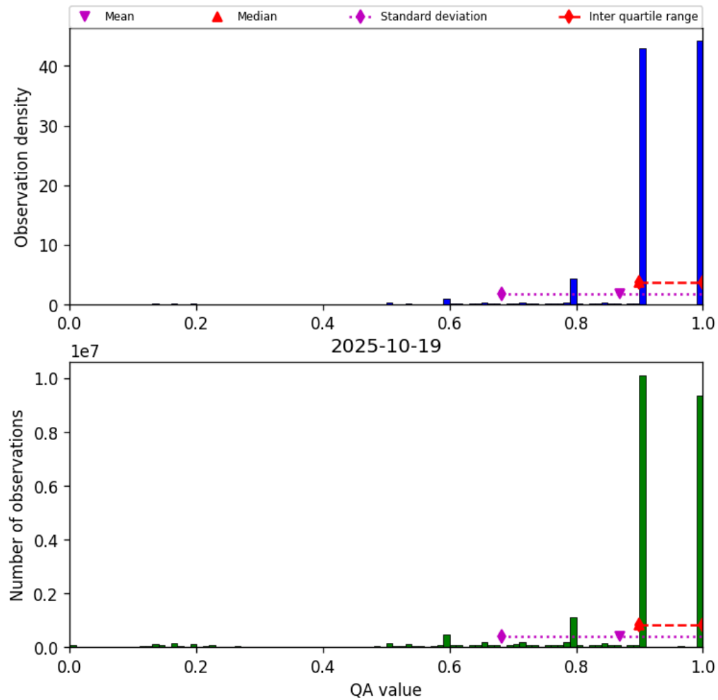
Figure 20: Histogram of “QA value” for 2025-10-18 to 2025-10-20
