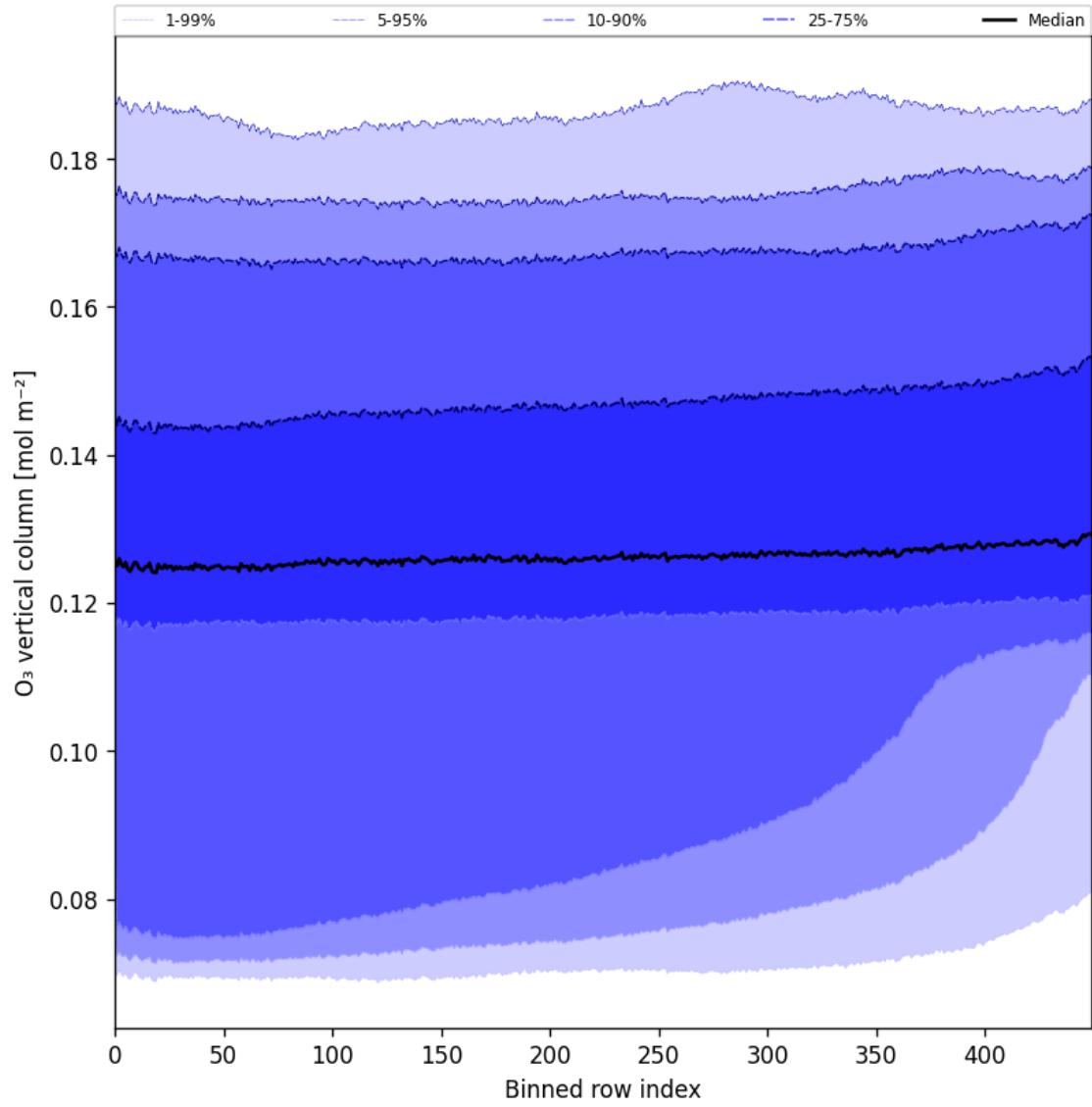
Figure 28: Along track statistics of “O 3 vertical column” for 2025-10-18 to 2025-10-20
