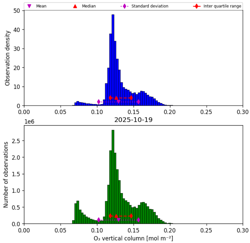
Figure 21: Histogram of “O 3 vertical column” for 2025-10-18 to 2025-10-20
