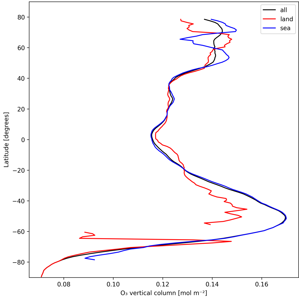
Figure 14: Zonal average of “O 3 vertical column” for 2025-10-18 to 2025-10-20.
