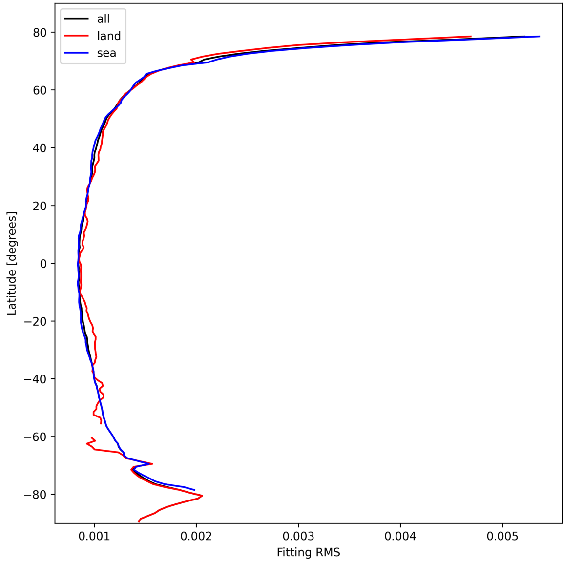
Figure 16: Zonal average of “Fitting RMS” for 2025-10-18 to 2025-10-20.
