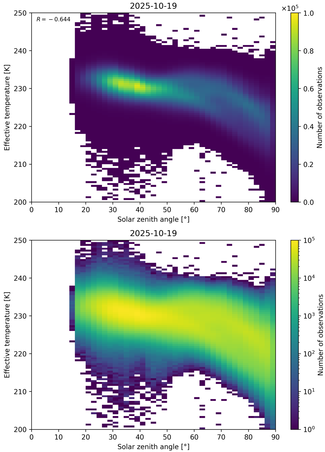
Figure 45: Scatter density plot of “Solar zenith angle” against “Effective temperature” for 2025-10-18 to 2025-10-20.
