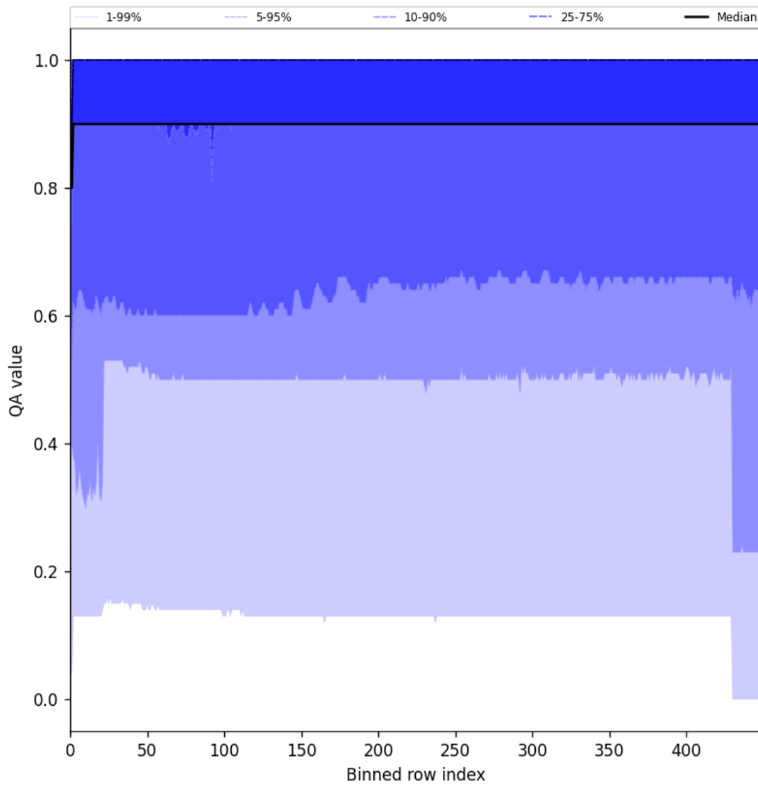
Figure 27: Along track statistics of “QA value” for 2025-10-18 to 2025-10-20
