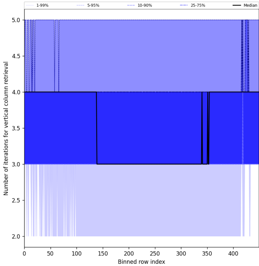
Figure 33: Along track statistics of “Number of iterations for vertical column retrieval” for 2025-10-18 to 2025-10-20
