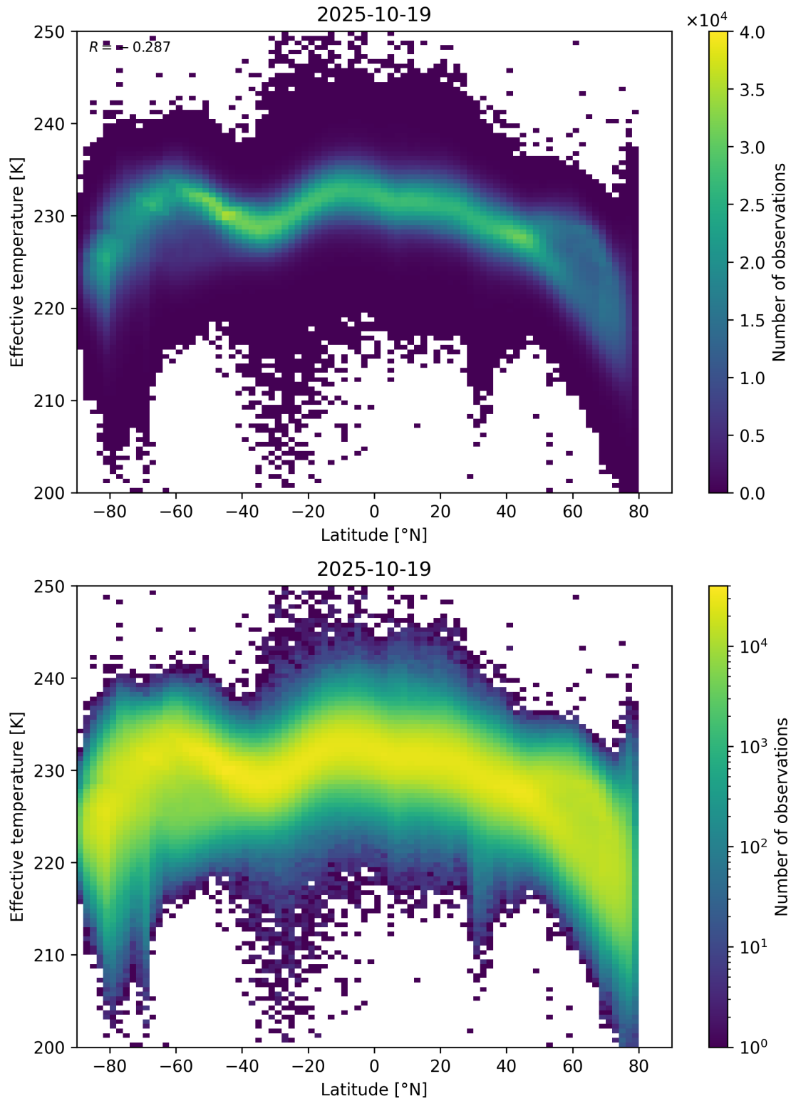
Figure 34: Scatter density plot of “Latitude” against “Effective temperature” for 2025-10-18 to 2025-10-20.
