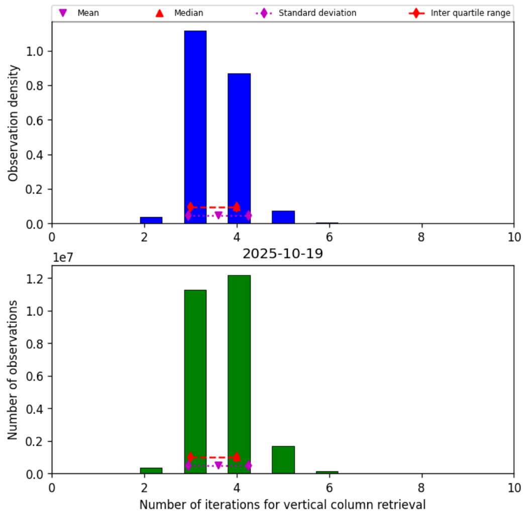
Figure 26: Histogram of “Number of iterations for vertical column retrieval” for 2025-10-18 to 2025-10-20
