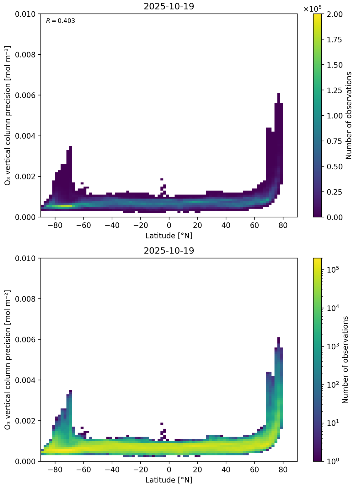
Figure 37: Scatter density plot of “Latitude” against “O 3 vertical column precision” for 2025-10-18 to 2025-10-20.
