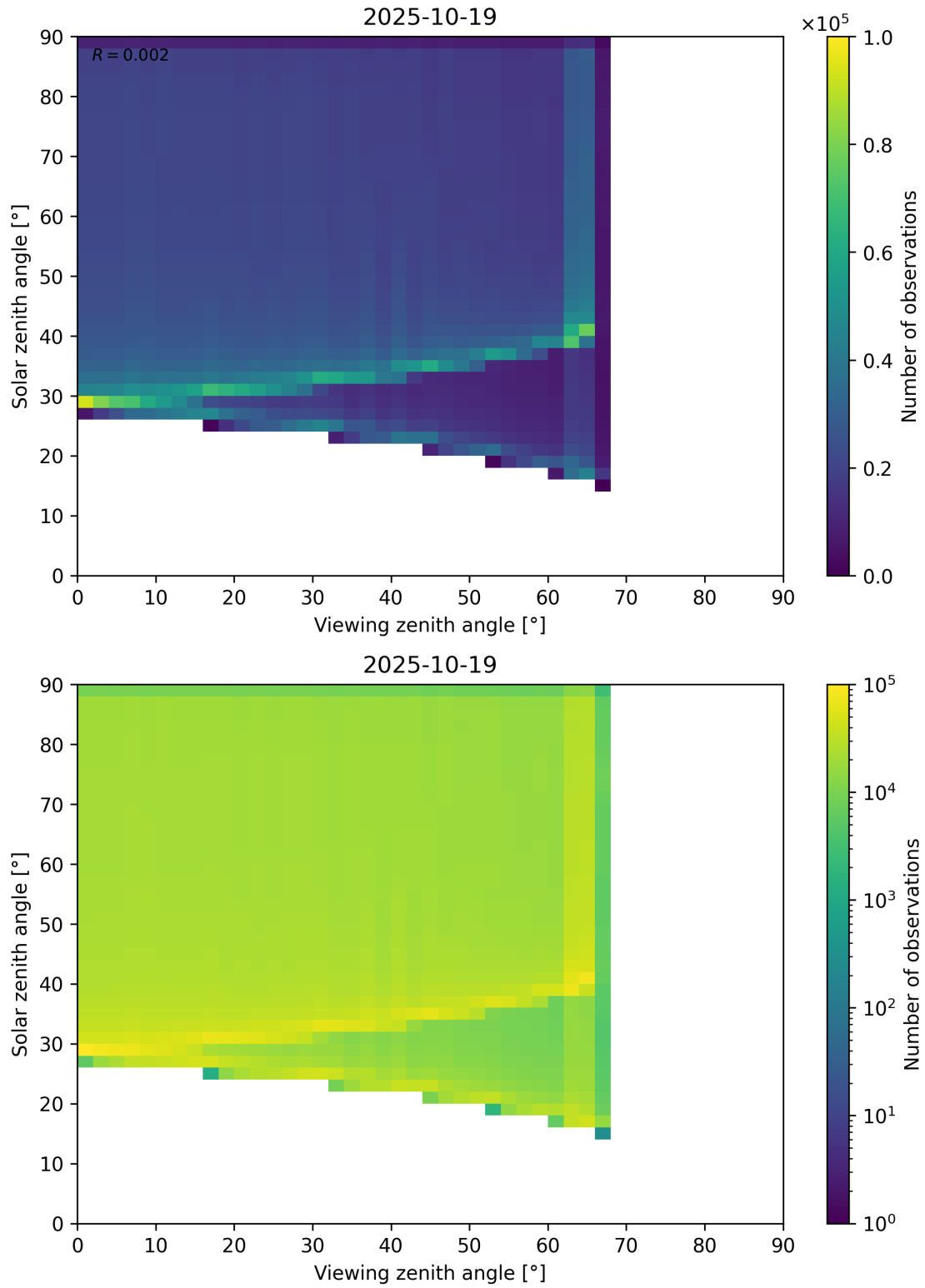
Figure 54: Scatter density plot of “Viewing zenith angle” against “Solar zenith angle” for 2025-10-18 to 2025-10-20.
