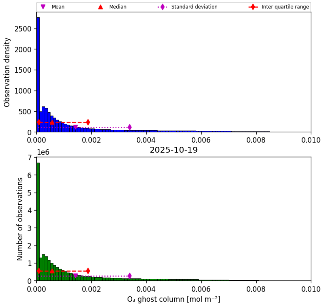
Figure 25: Histogram of "O 3 ghost column" for 2025-10-18 to 2025-10-20
