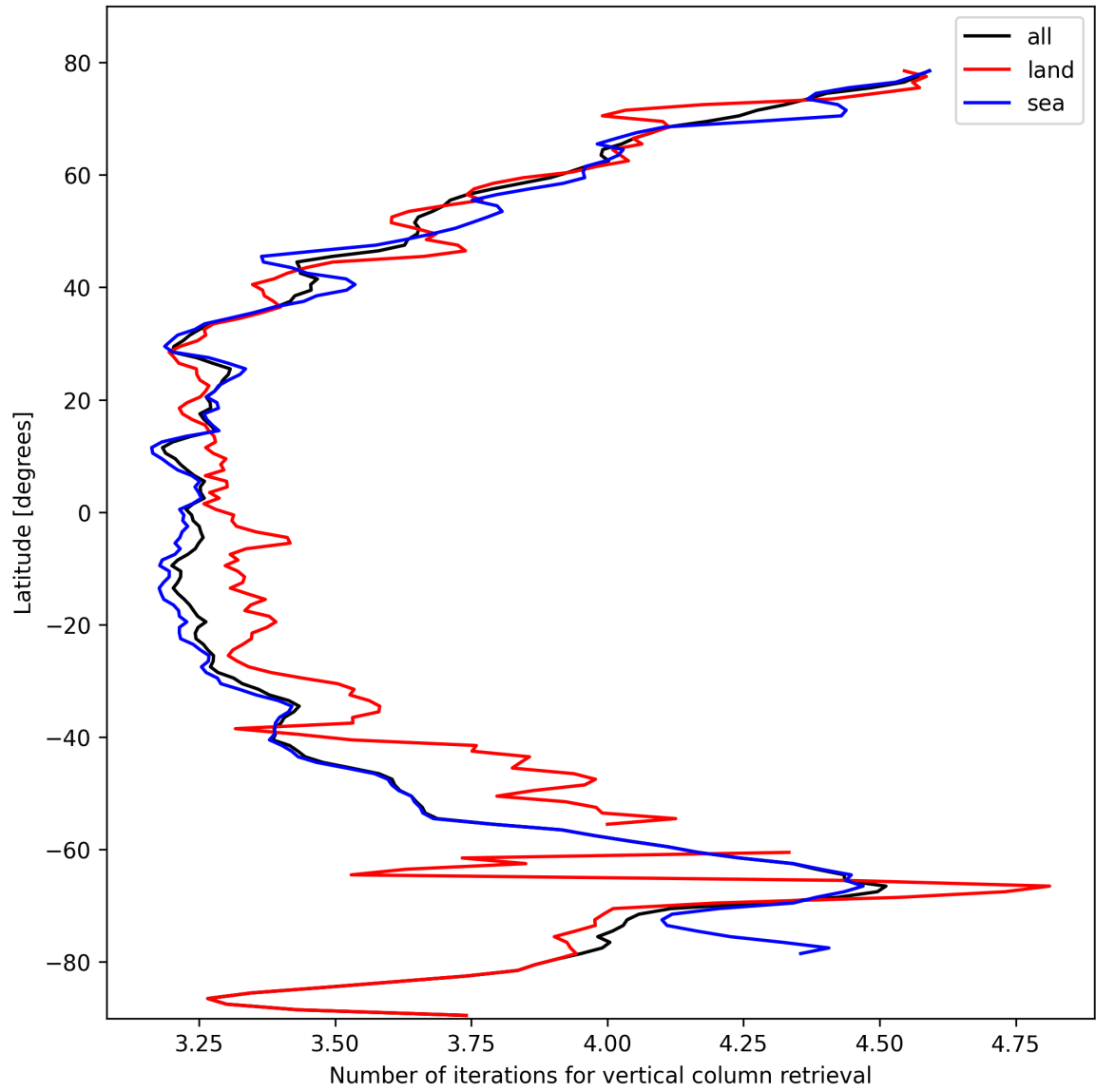
Figure 19: Zonal average of “Number of iterations for vertical column retrieval” for 2025-10-18 to 2025-10-20.
