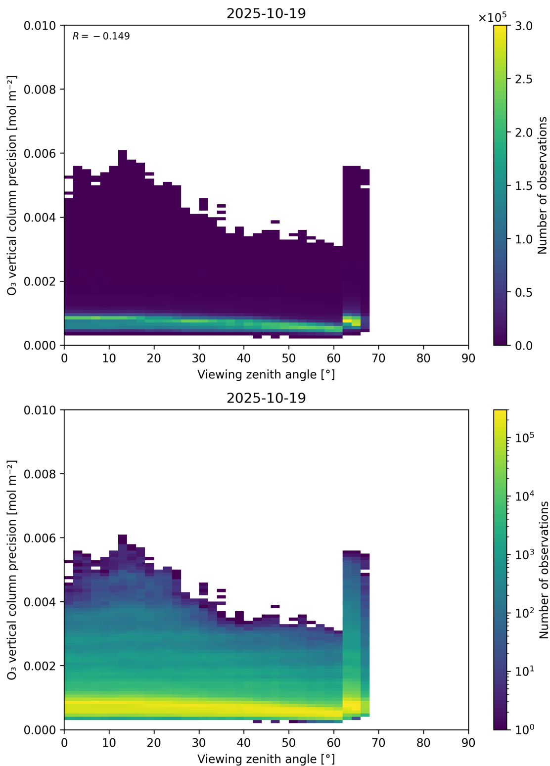
Figure 53: Scatter density plot of “Viewing zenith angle” against “O 3 vertical column precision” for 2025-10-18 to 2025-10-20.
