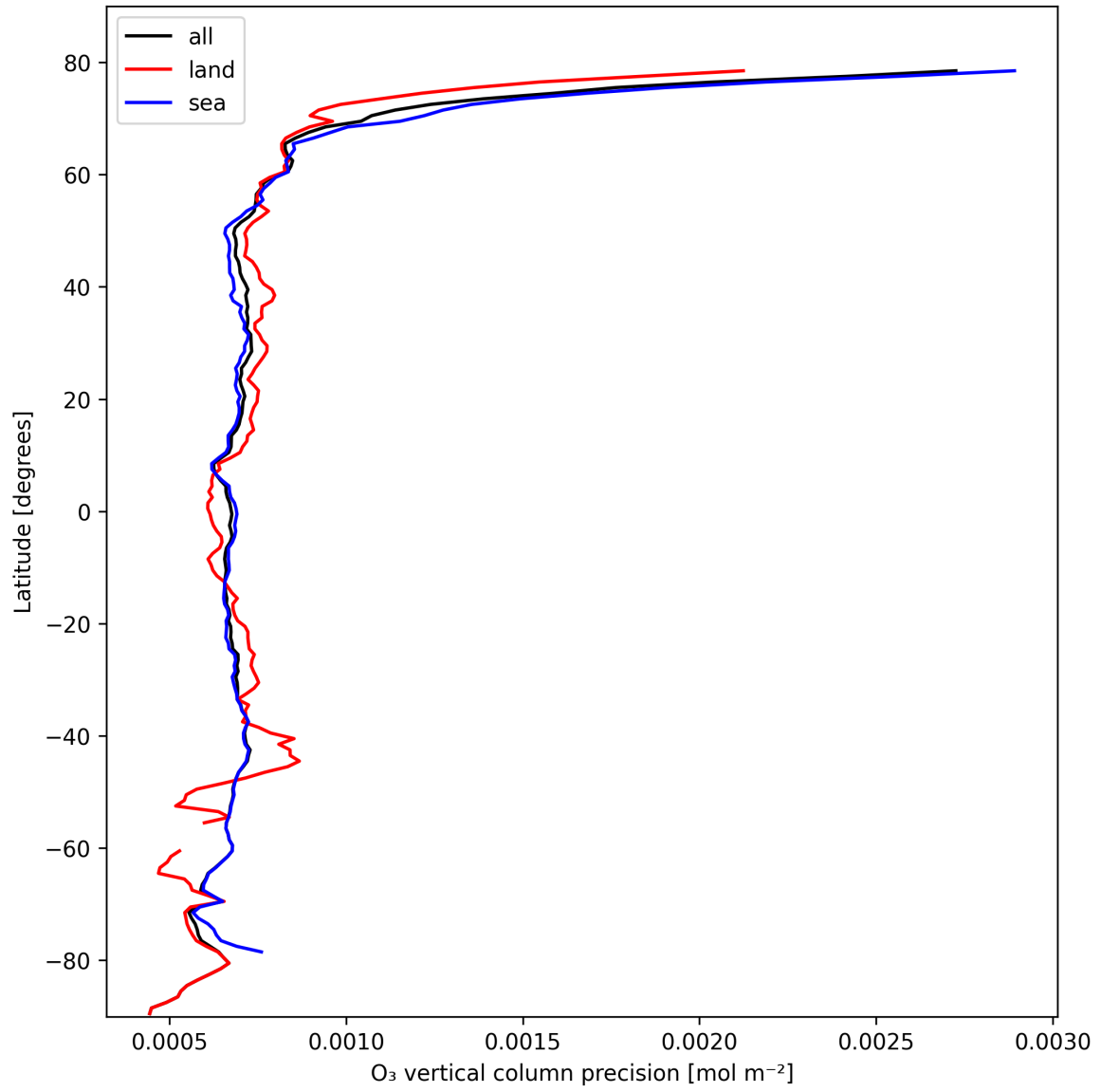
Figure 15: Zonal average of “O 3 vertical column precision” for 2025-10-18 to 2025-10-20.
