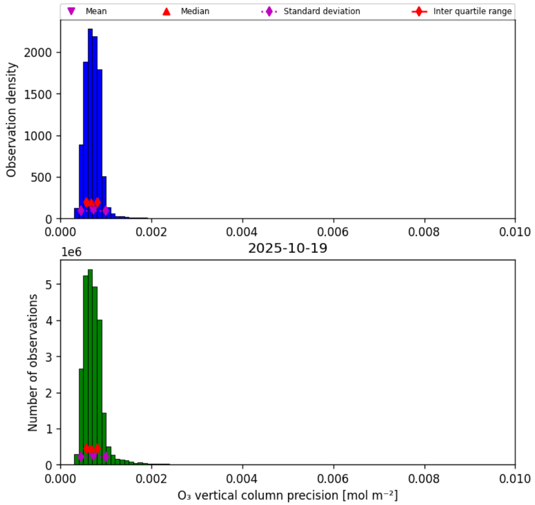
Figure 22: Histogram of “O 3 vertical column precision” for 2025-10-18 to 2025-10-20
