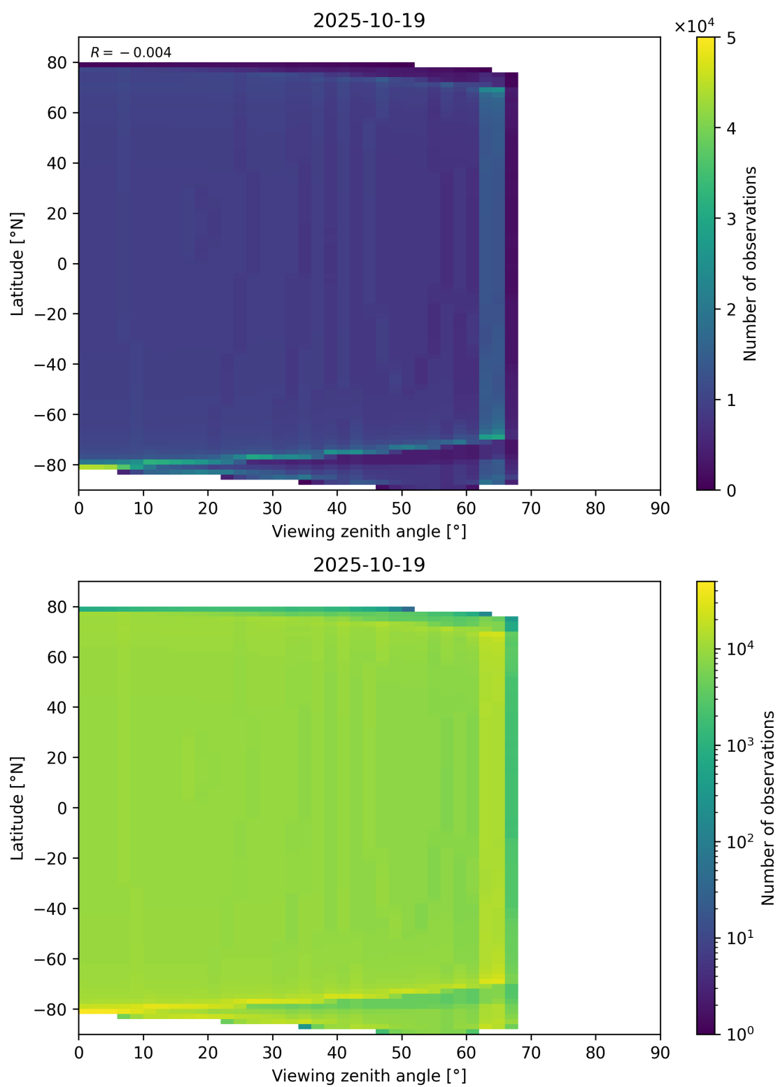
Figure 49: Scatter density plot of “Viewing zenith angle” against “Latitude” for 2025-10-18 to 2025-10-20.
