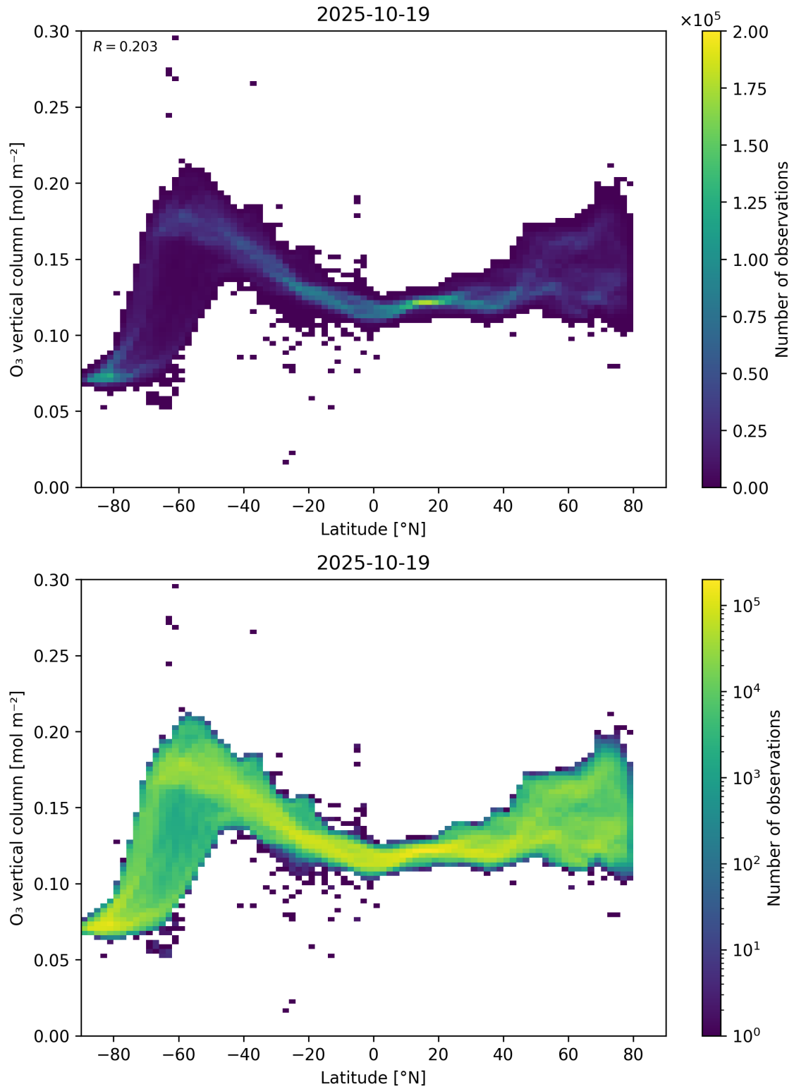
Figure 36: Scatter density plot of “Latitude” against “O 3 vertical column” for 2025-10-18 to 2025-10-20.
