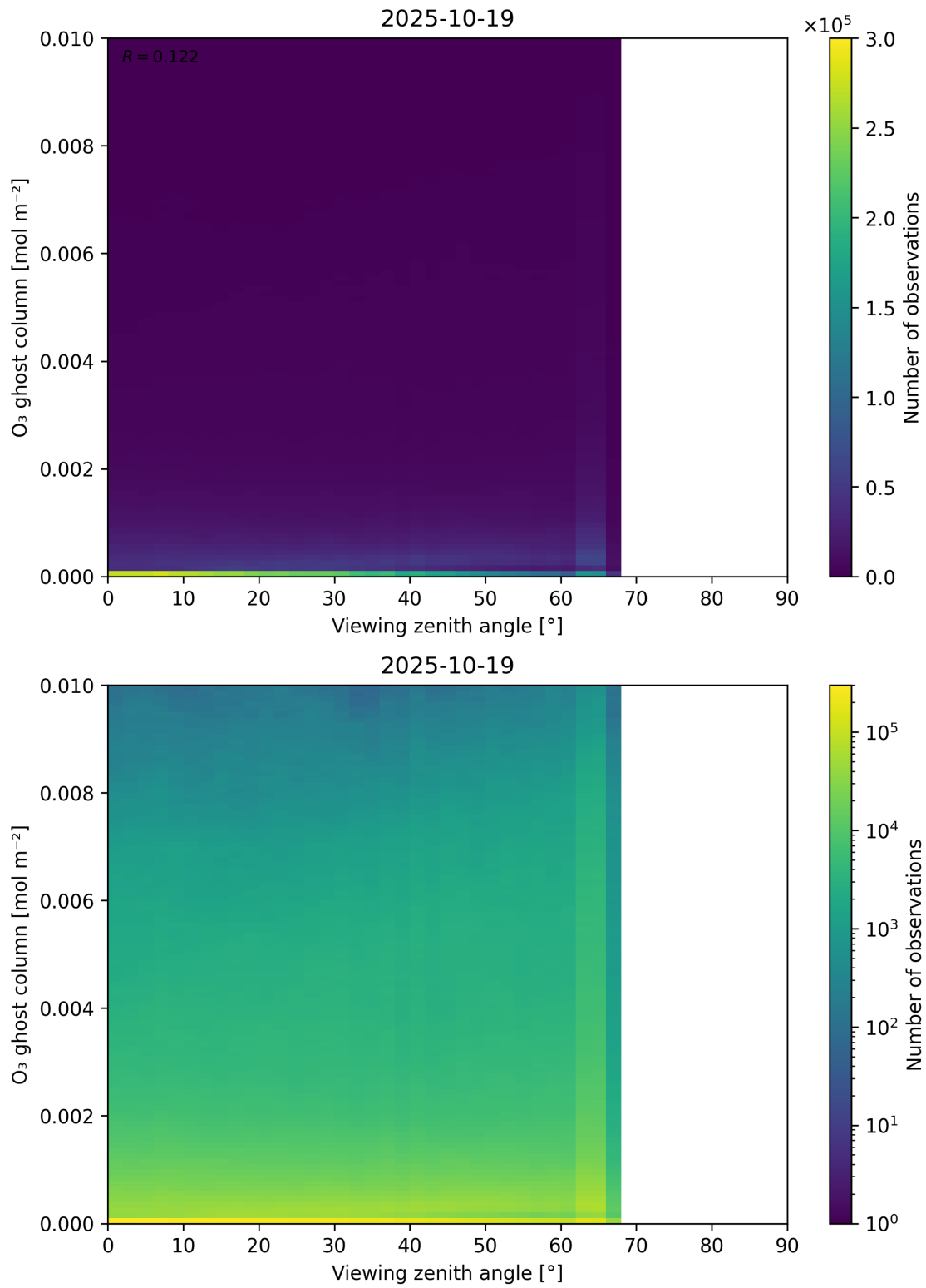
Figure 51: Scatter density plot of “Viewing zenith angle” against “O 3 ghost column” for 2025-10-18 to 2025-10-20.
