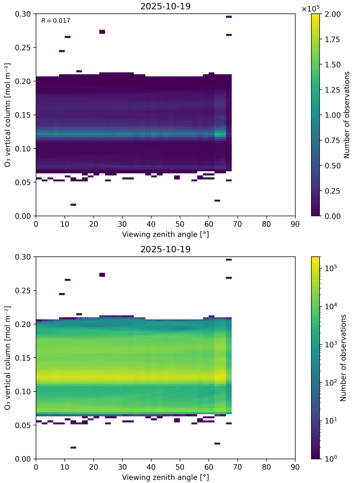
Figure 52: Scatter density plot of “Viewing zenith angle” against “O 3 vertical column” for 2025-10-18 to 2025-10-20.
