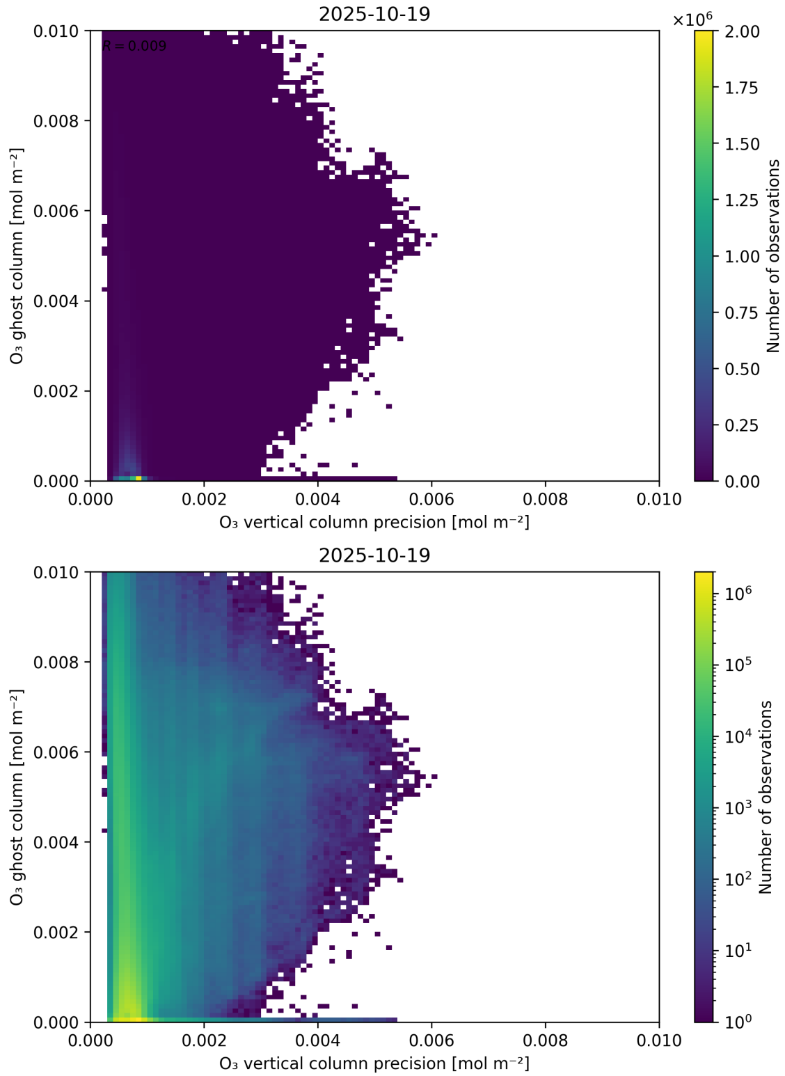
Figure 43: Scatter density plot of “O 3 vertical column precision” against “O 3 ghost column” for 2025-10-18 to 2025-10-20.
