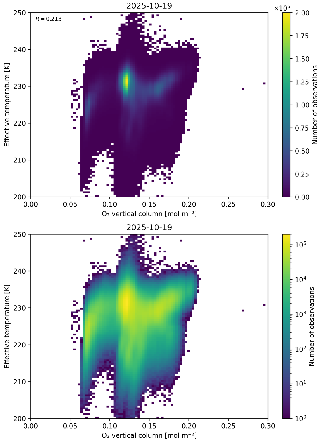
Figure 39: Scatter density plot of “O 3 vertical column” against “Effective temperature” for 2025-10-18 to 2025-10-20.
