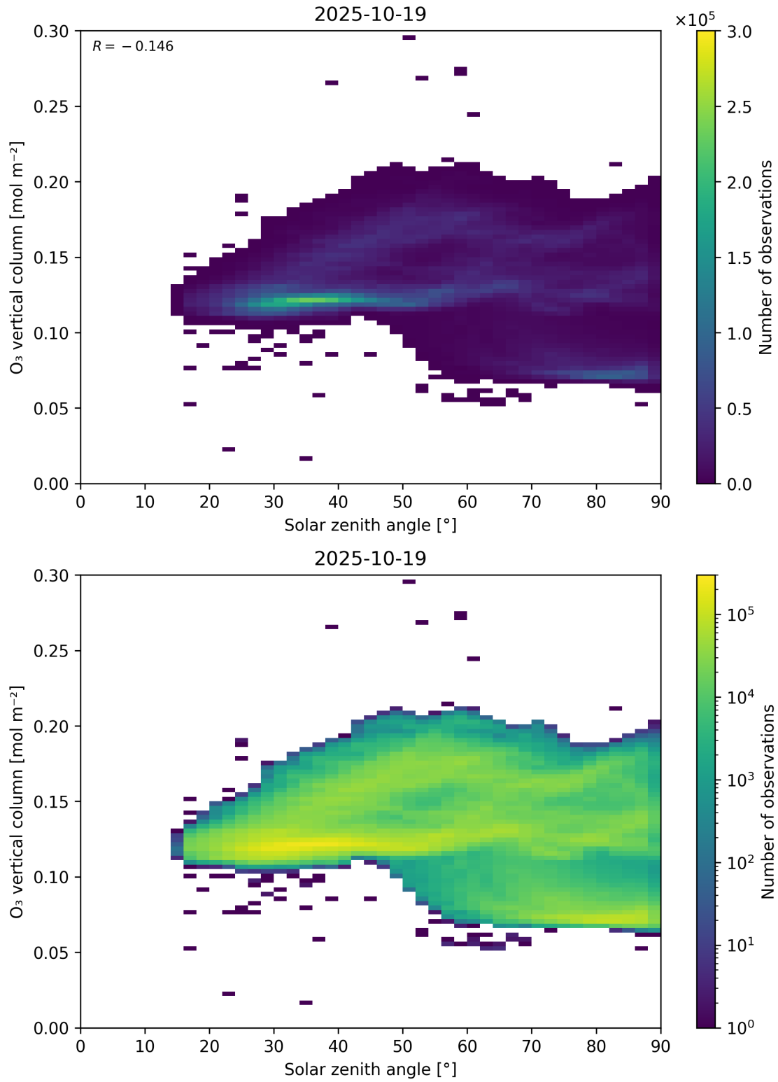
Figure 47: Scatter density plot of “Solar zenith angle” against “O 3 vertical column” for 2025-10-18 to 2025-10-20.
