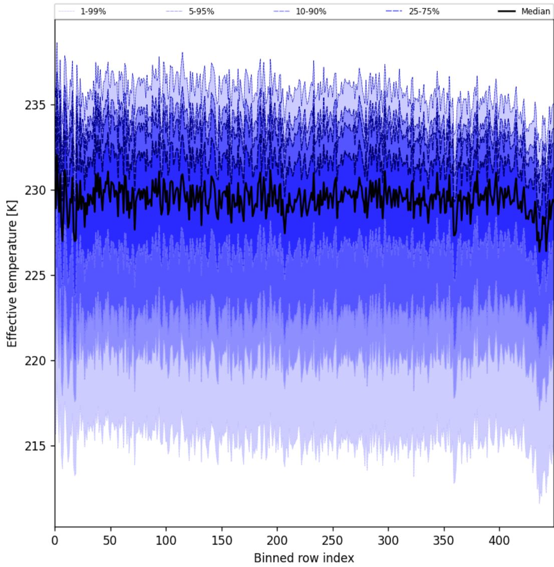
Figure 31: Along track statistics of “Effective temperature” for 2025-10-18 to 2025-10-20
