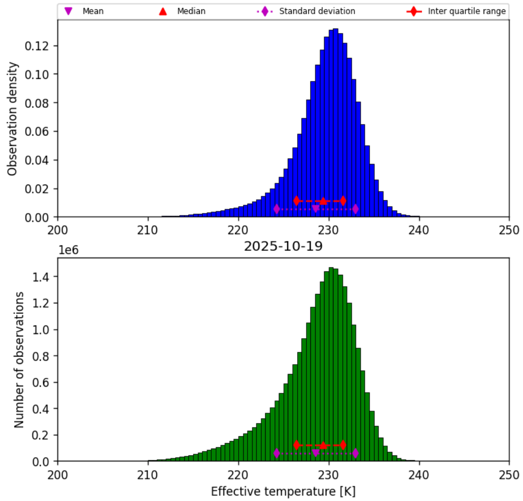
Figure 24: Histogram of “Effective temperature” for 2025-10-18 to 2025-10-20
