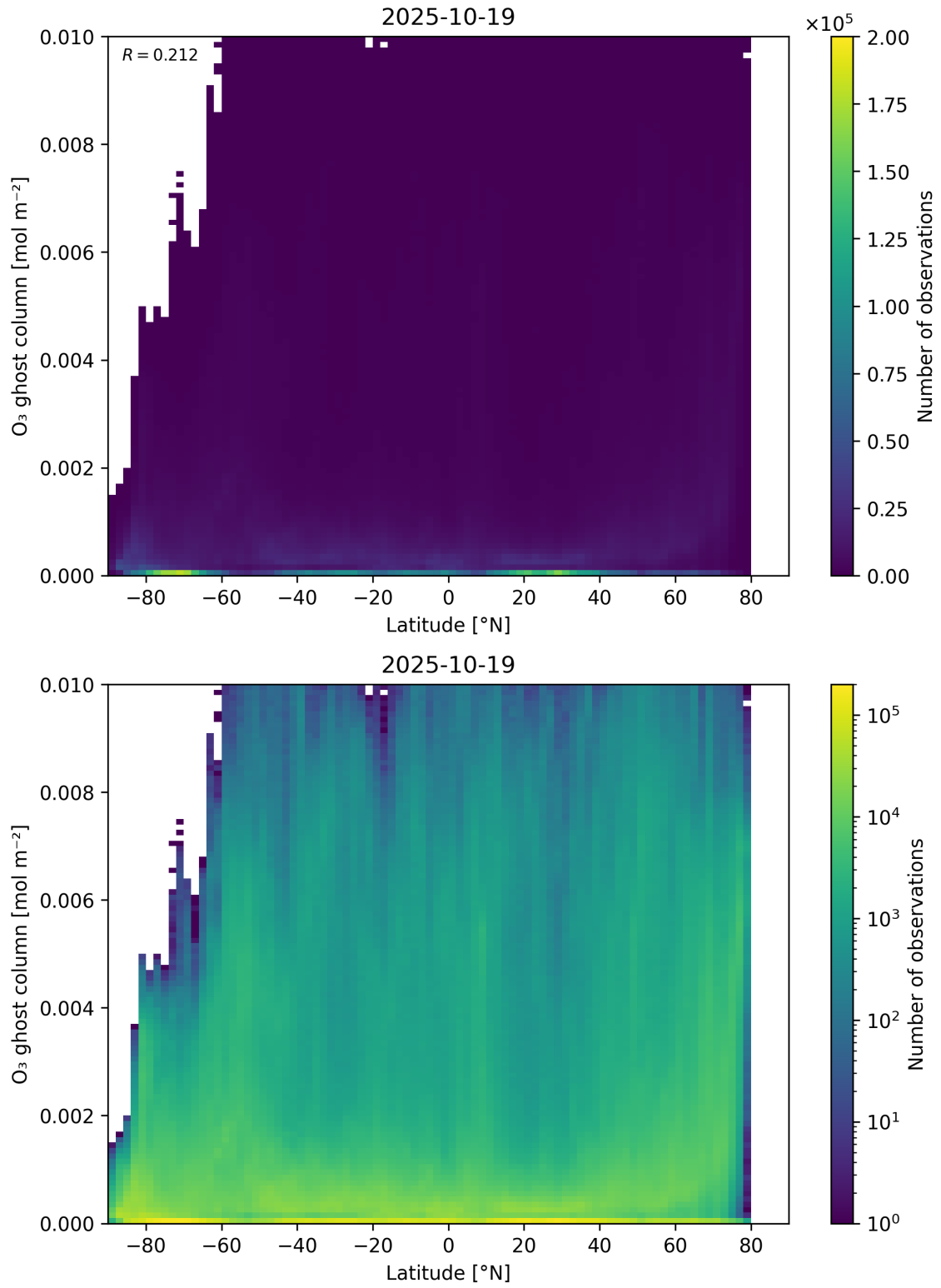
Figure 35: Scatter density plot of “Latitude” against “O 3 ghost column” for 2025-10-18 to 2025-10-20.
