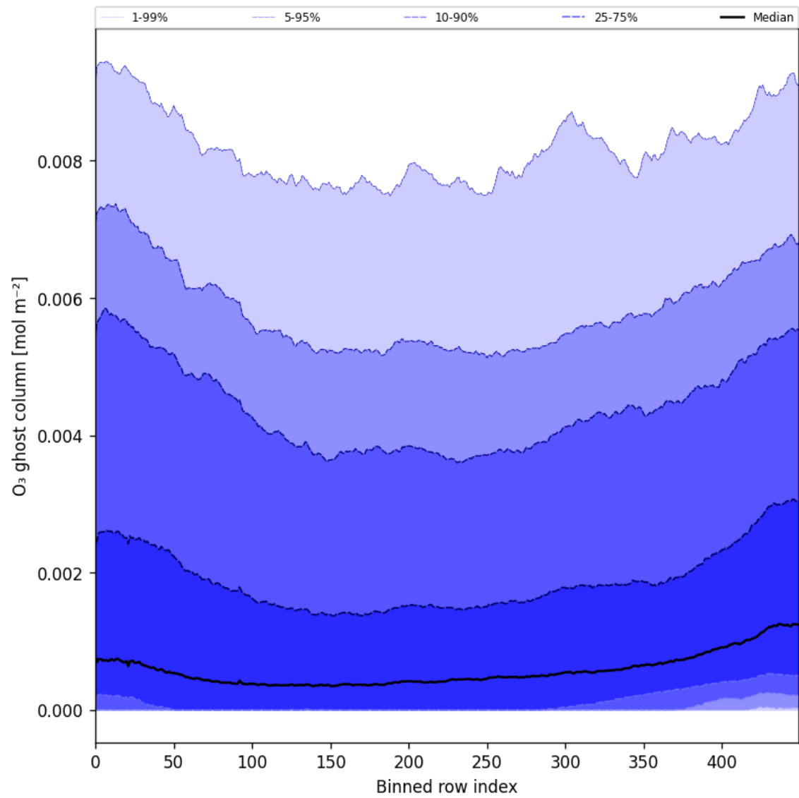
Figure 32: Along track statistics of “O 3 ghost column” for 2025-10-18 to 2025-10-20
