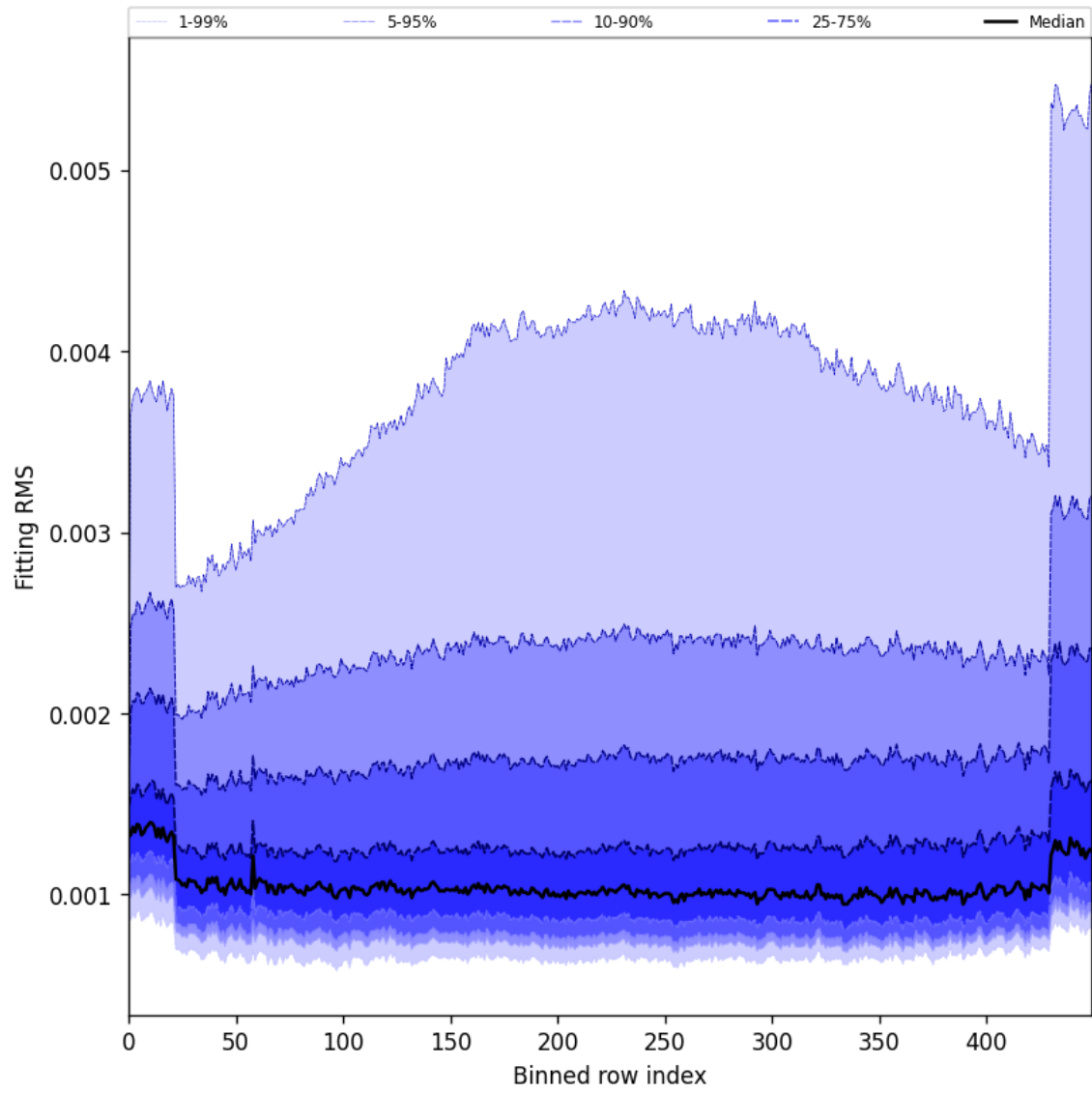
Figure 30: Along track statistics of “Fitting RMS” for 2025-10-18 to 2025-10-20
