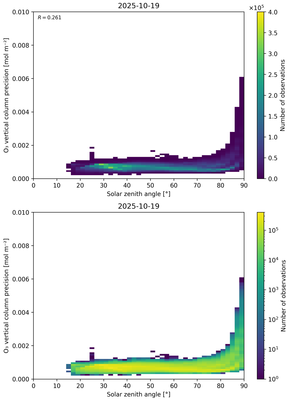
Figure 48: Scatter density plot of “Solar zenith angle” against “O 3 vertical column precision” for 2025-10-18 to 2025-10-20.
