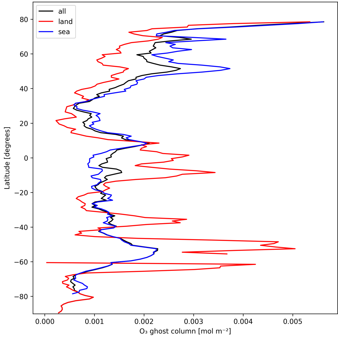
Figure 18: Zonal average of “O 3 ghost column” for 2025-10-18 to 2025-10-20.
