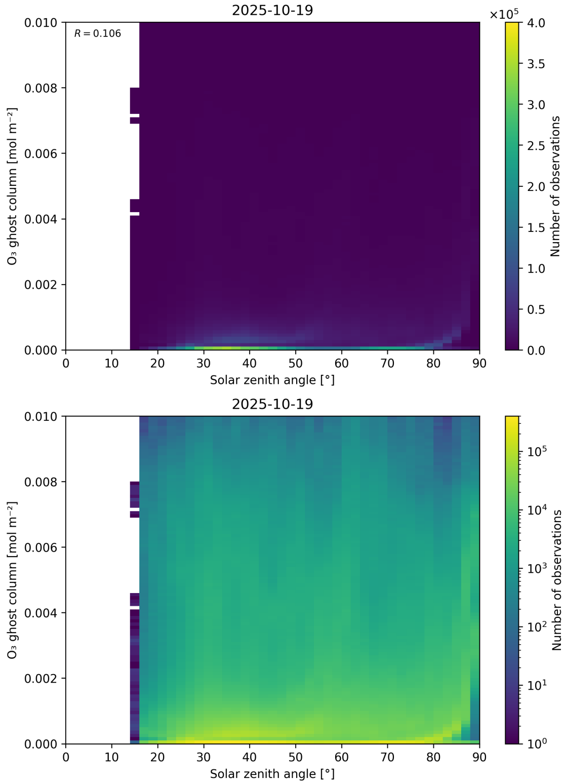
Figure 46: Scatter density plot of “Solar zenith angle” against “O 3 ghost column” for 2025-10-18 to 2025-10-20.
