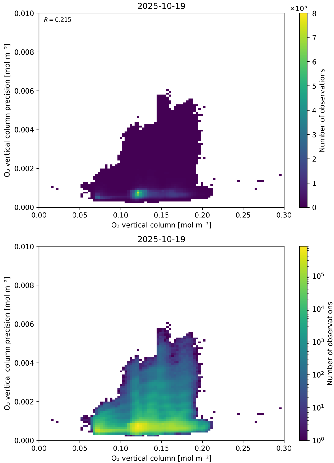
Figure 41: Scatter density plot of “O 3 vertical column” against “O 3 vertical column precision” for 2025-10-18 to 2025-10-20.
