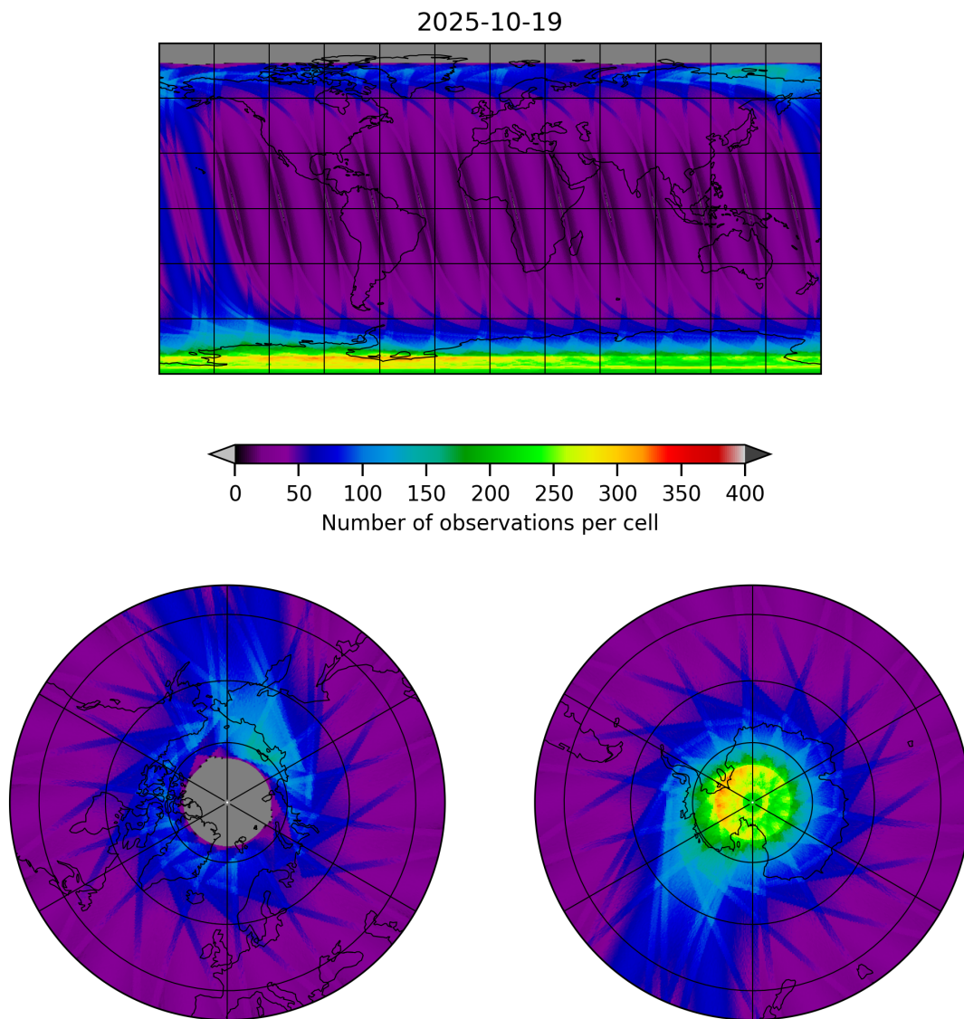
Figure 12: Map of the number of observations for 2025-10-18 to 2025-10-20
