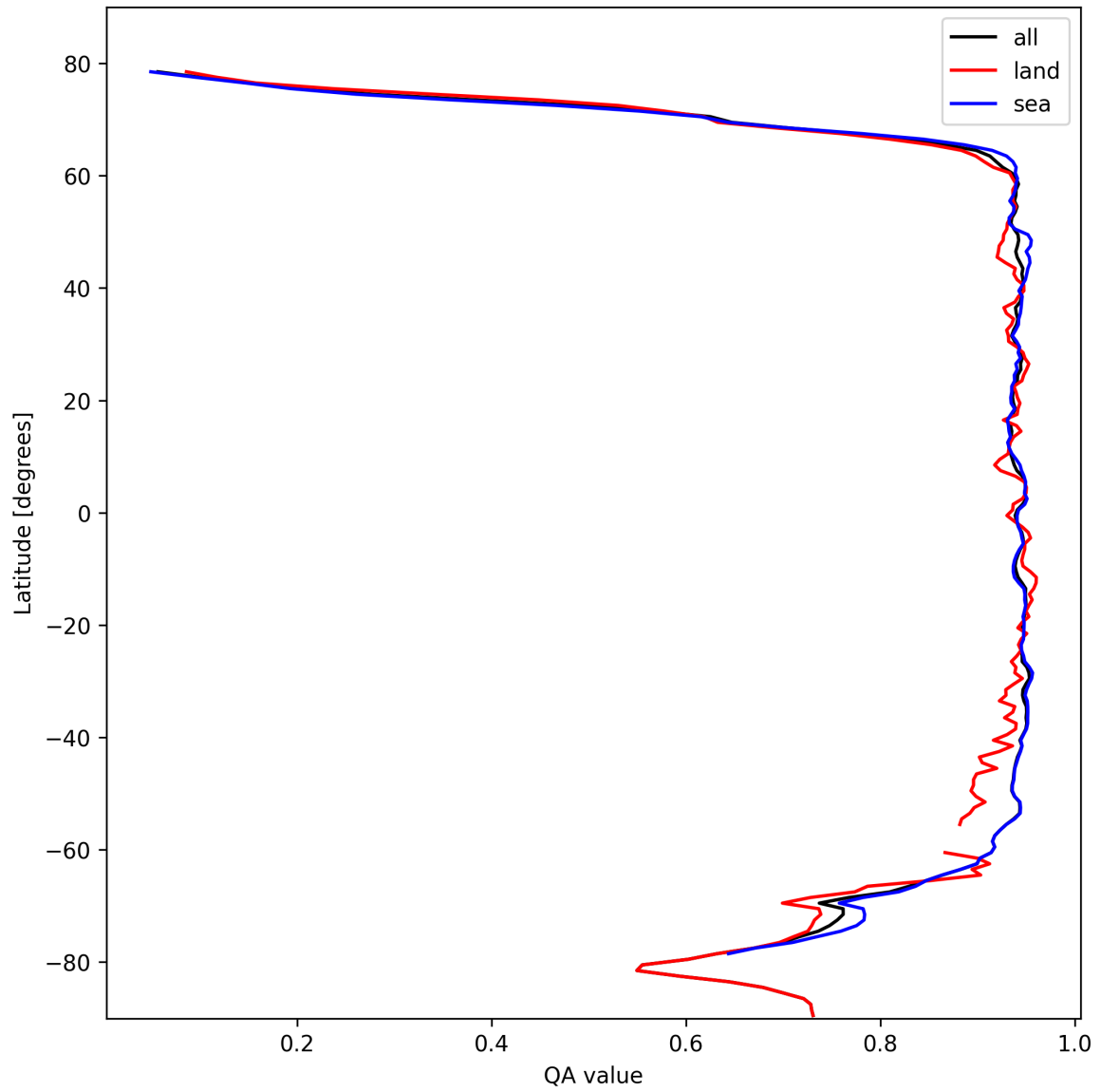
Figure 13: Zonal average of “QA value” for 2025-10-18 to 2025-10-20.
