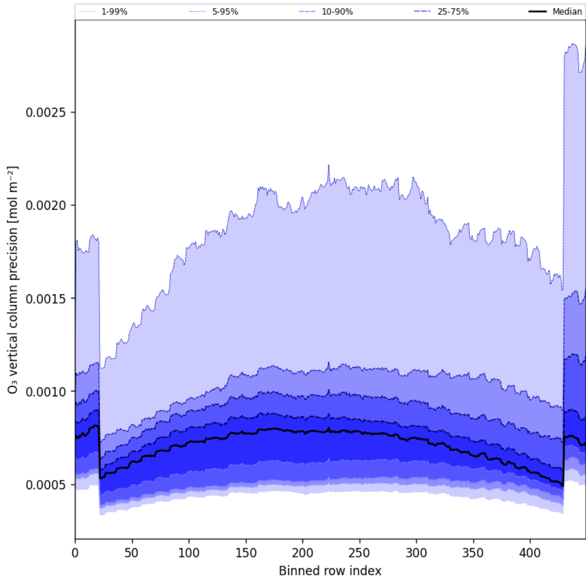
Figure 29: Along track statistics of “O 3 vertical column precision” for 2025-10-18 to 2025-10-20
