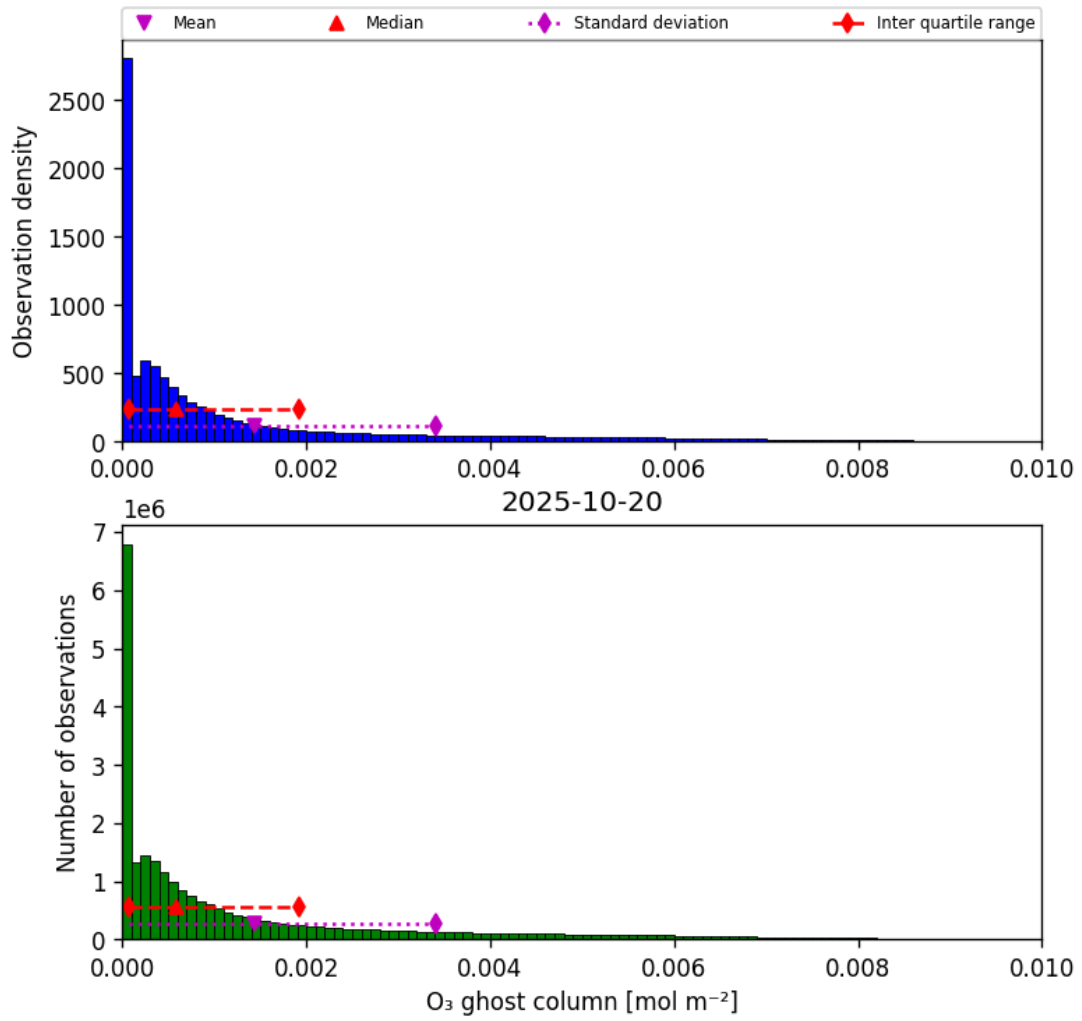
Figure 25: Histogram of "O 3 ghost column" for 2025-10-19 to 2025-10-21
