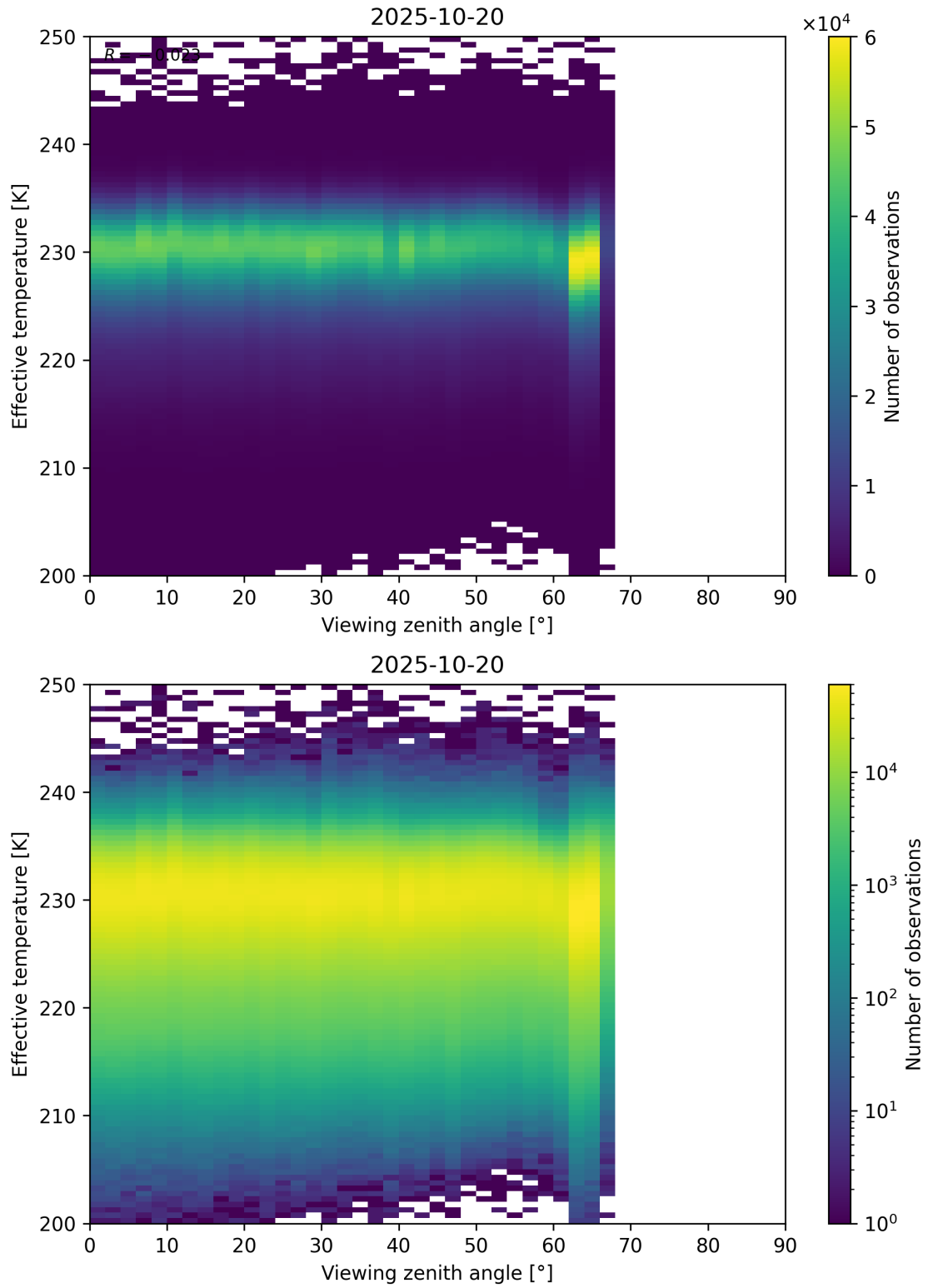
Figure 50: Scatter density plot of “Viewing zenith angle” against “Effective temperature” for 2025-10-19 to 2025-10-21.
