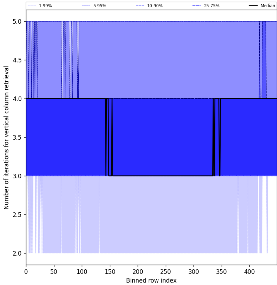
Figure 33: Along track statistics of “Number of iterations for vertical column retrieval” for 2025-10-19 to 2025-10-21
