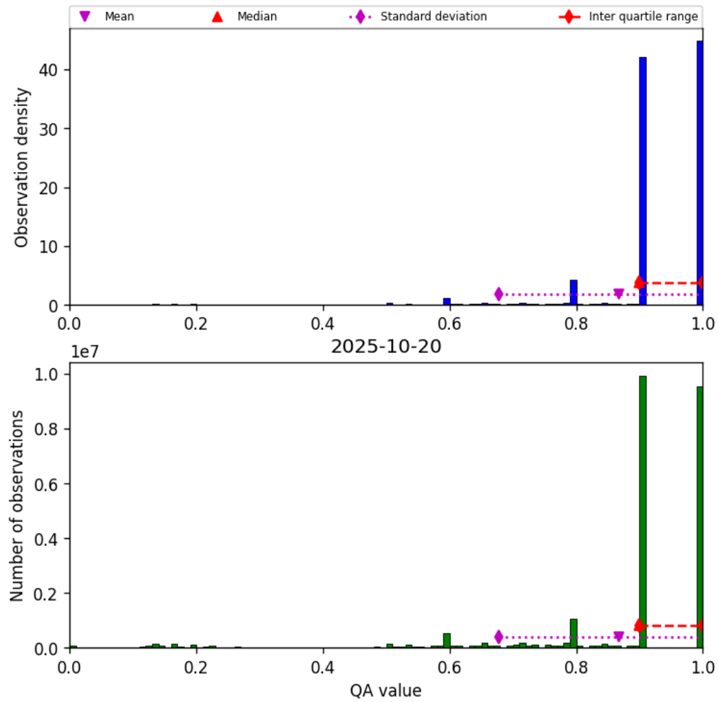
Figure 20: Histogram of “QA value” for 2025-10-19 to 2025-10-21
