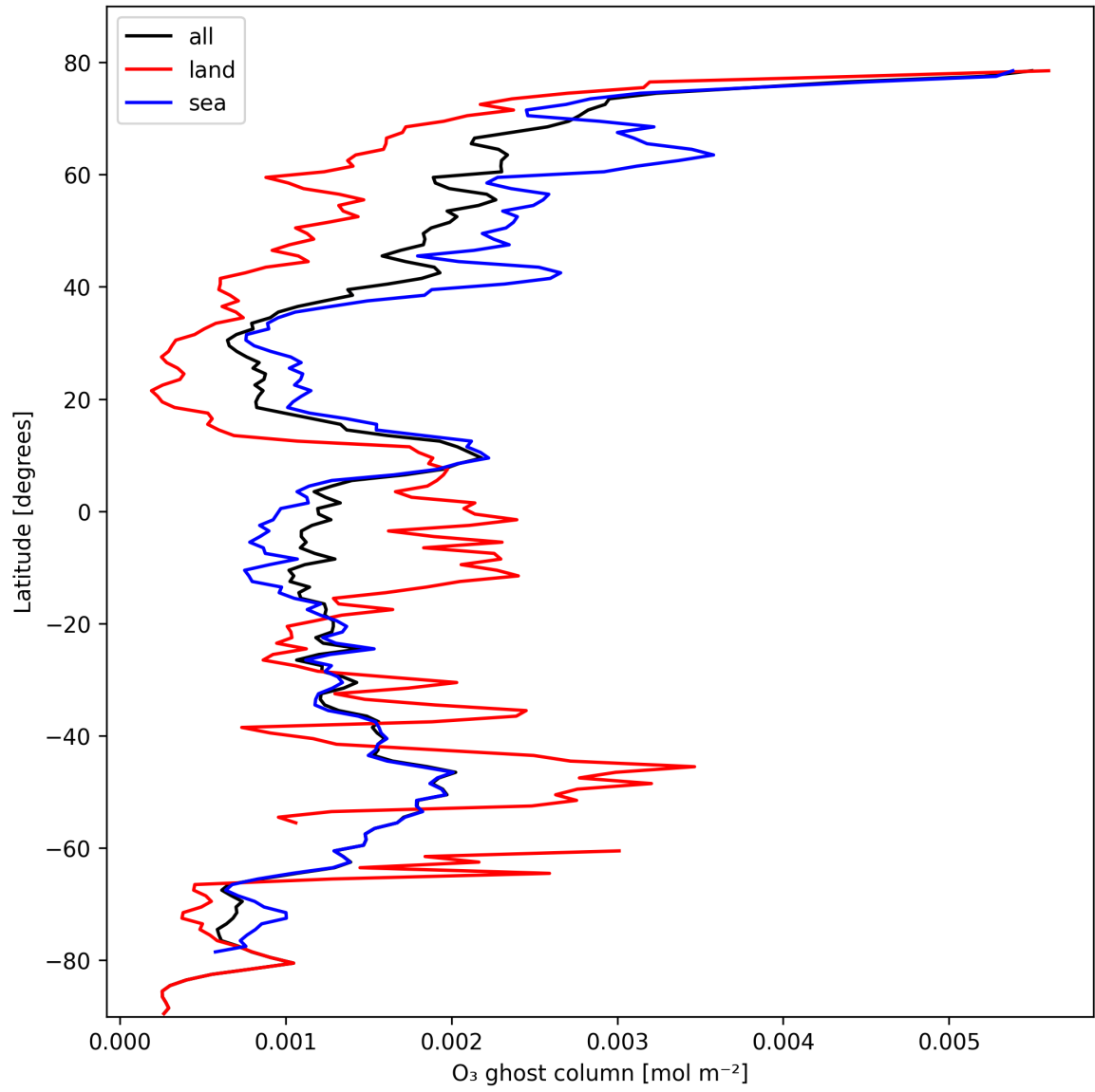
Figure 18: Zonal average of “O 3 ghost column” for 2025-10-19 to 2025-10-21.
