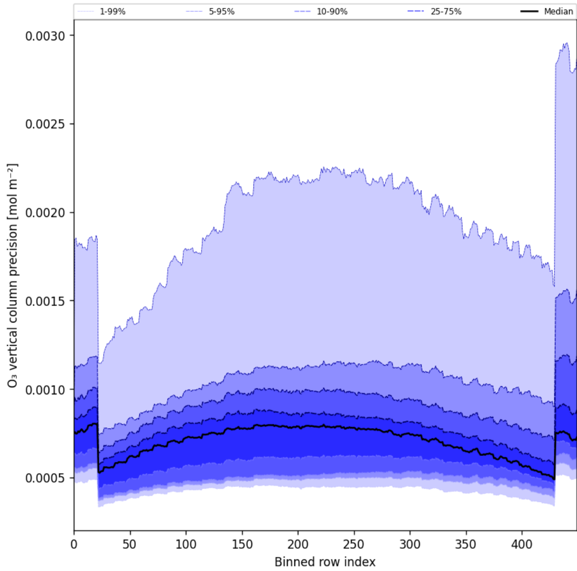
Figure 29: Along track statistics of “O 3 vertical column precision” for 2025-10-19 to 2025-10-21
