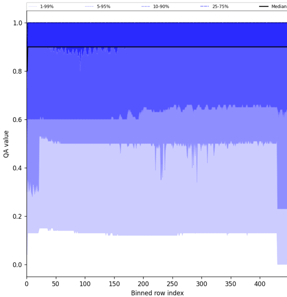
Figure 27: Along track statistics of “QA value” for 2025-10-19 to 2025-10-21
