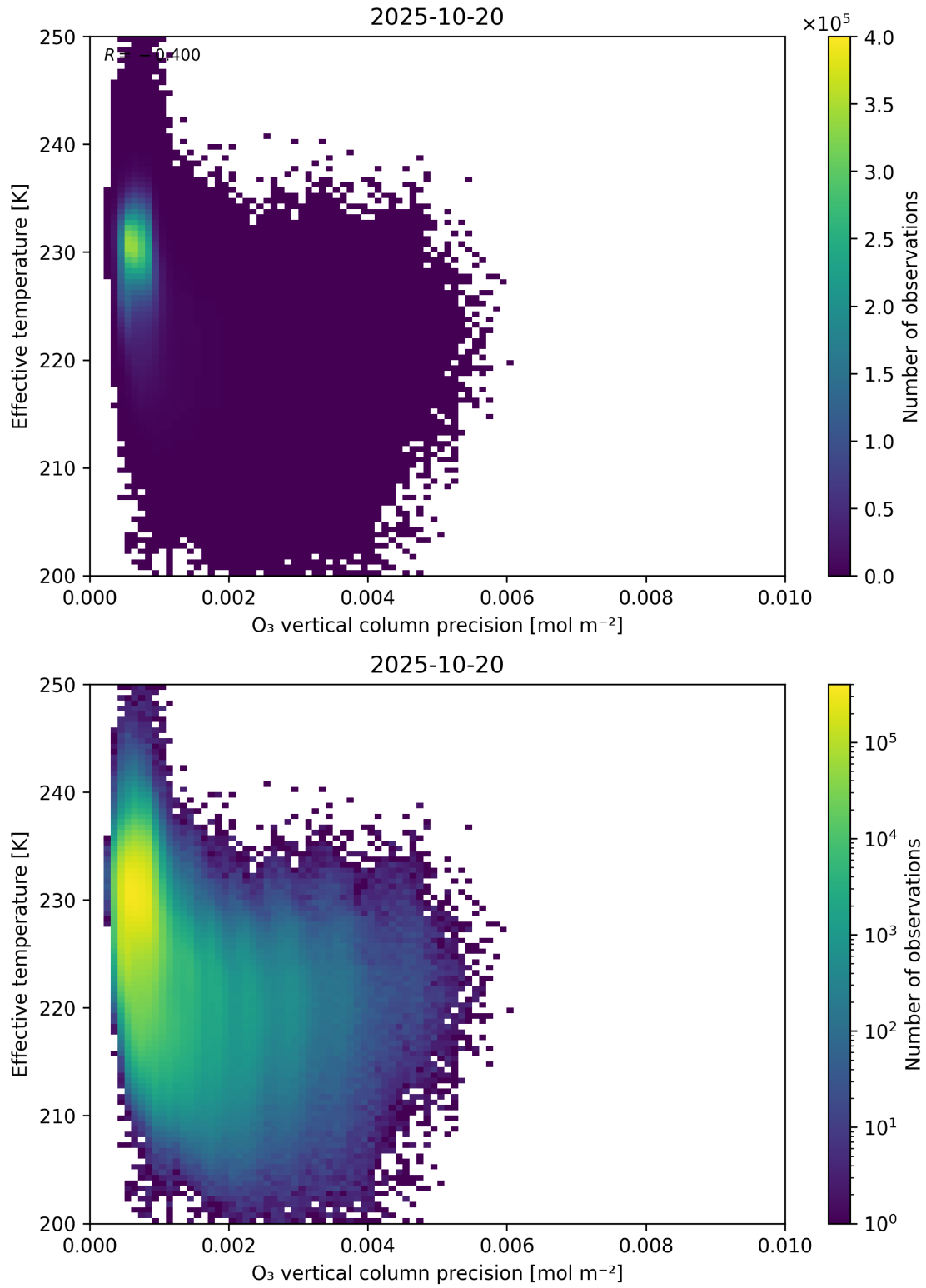
Figure 42: Scatter density plot of “ O_3 vertical column precision” against “Effective temperature” for 2025-10-19 to 2025-10-21.
