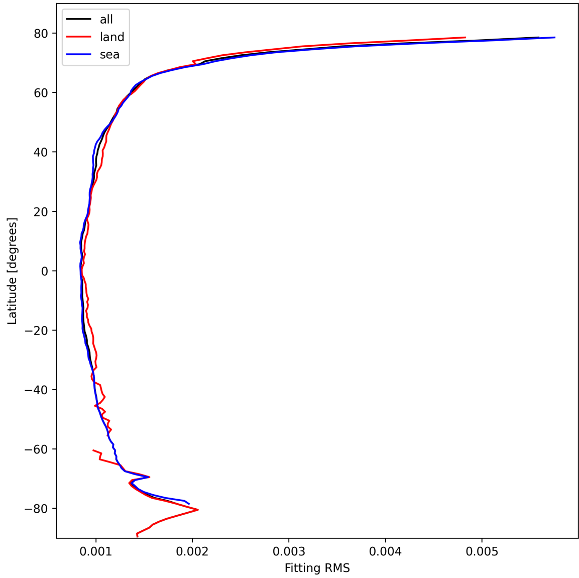
Figure 16: Zonal average of “Fitting RMS” for 2025-10-19 to 2025-10-21.
