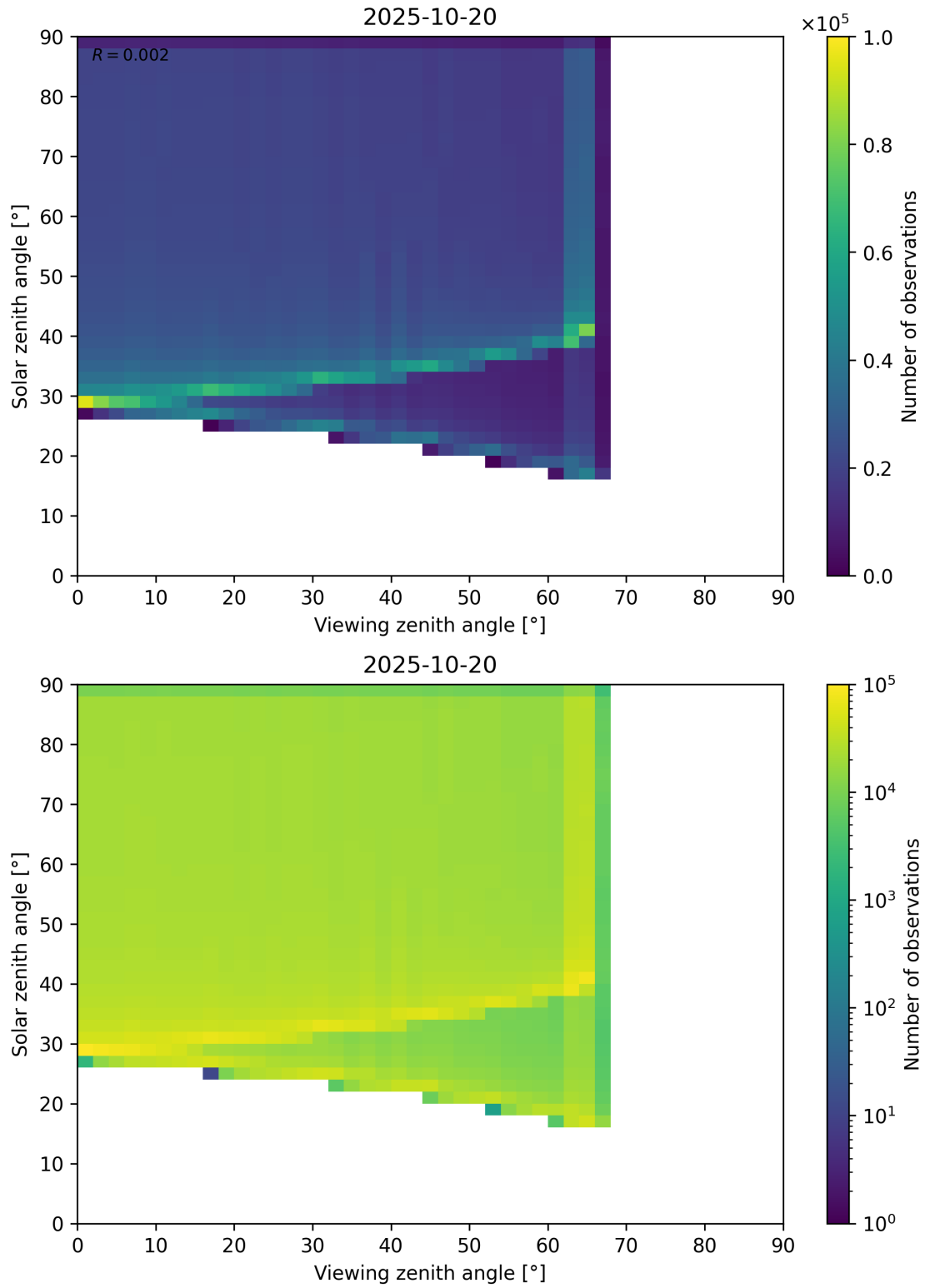
Figure 54: Scatter density plot of “Viewing zenith angle” against “Solar zenith angle” for 2025-10-19 to 2025-10-21.
