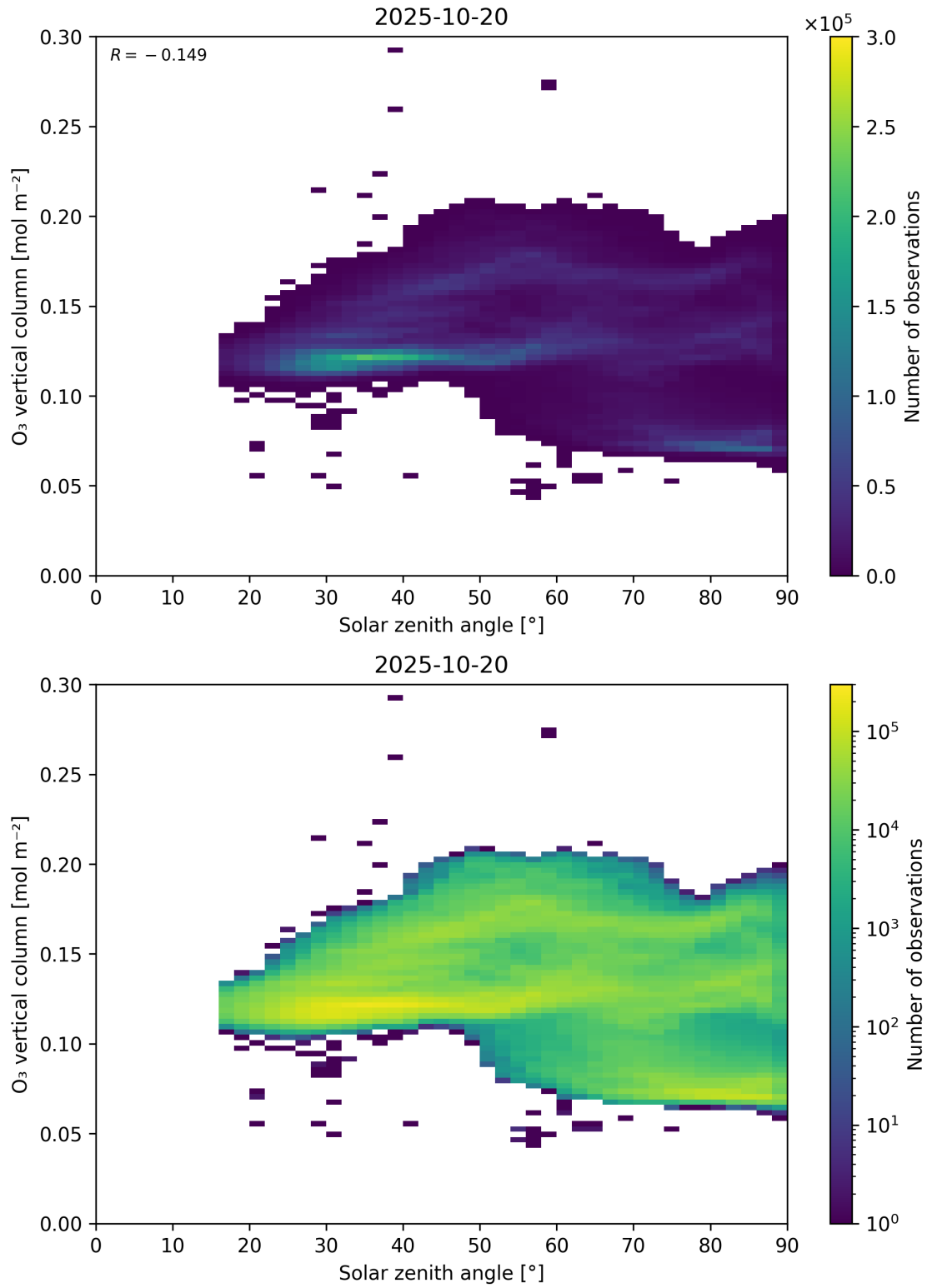
Figure 47: Scatter density plot of “Solar zenith angle” against “O 3 vertical column” for 2025-10-19 to 2025-10-21.
