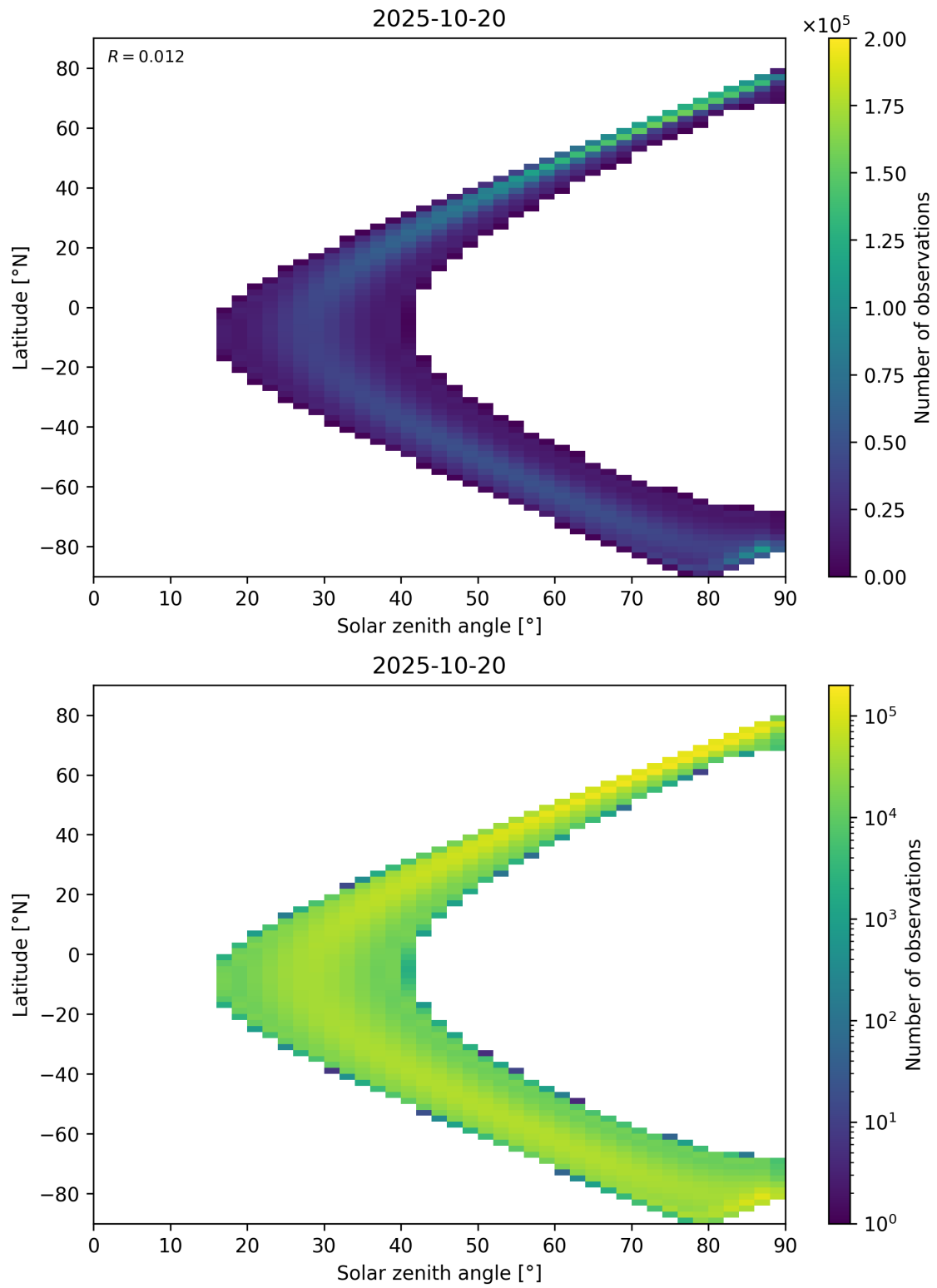
Figure 44: Scatter density plot of “Solar zenith angle” against “Latitude” for 2025-10-19 to 2025-10-21.
