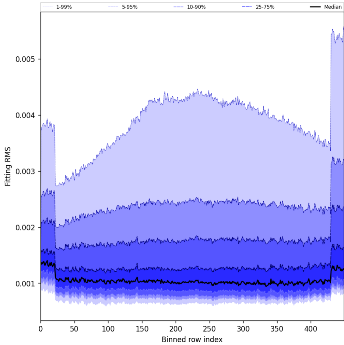
Figure 30: Along track statistics of “Fitting RMS” for 2025-10-19 to 2025-10-21
