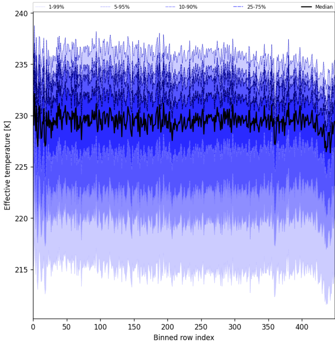
Figure 31: Along track statistics of “Effective temperature” for 2025-10-19 to 2025-10-21
