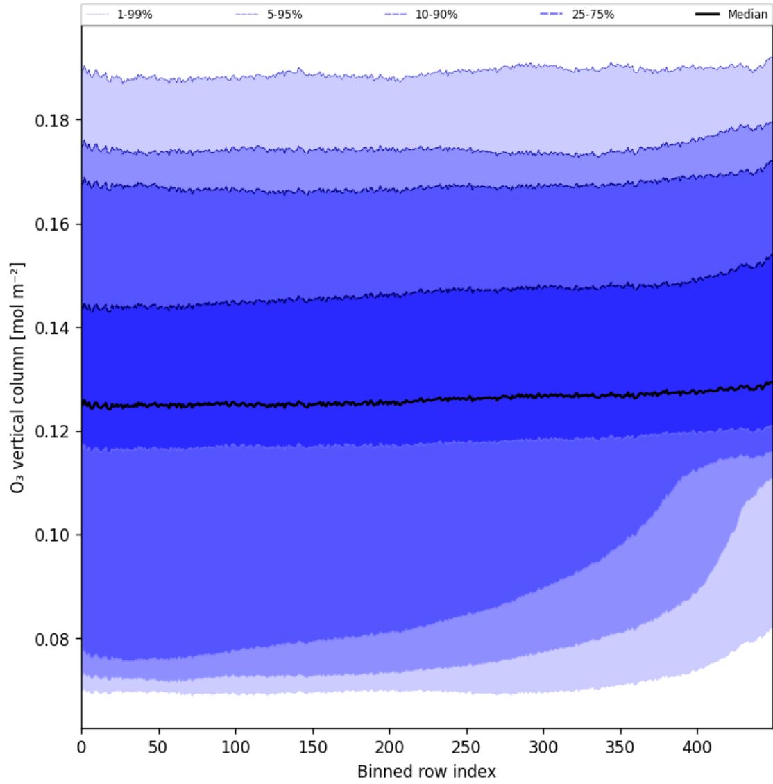
Figure 28: Along track statistics of “O 3 vertical column” for 2025-10-19 to 2025-10-21
