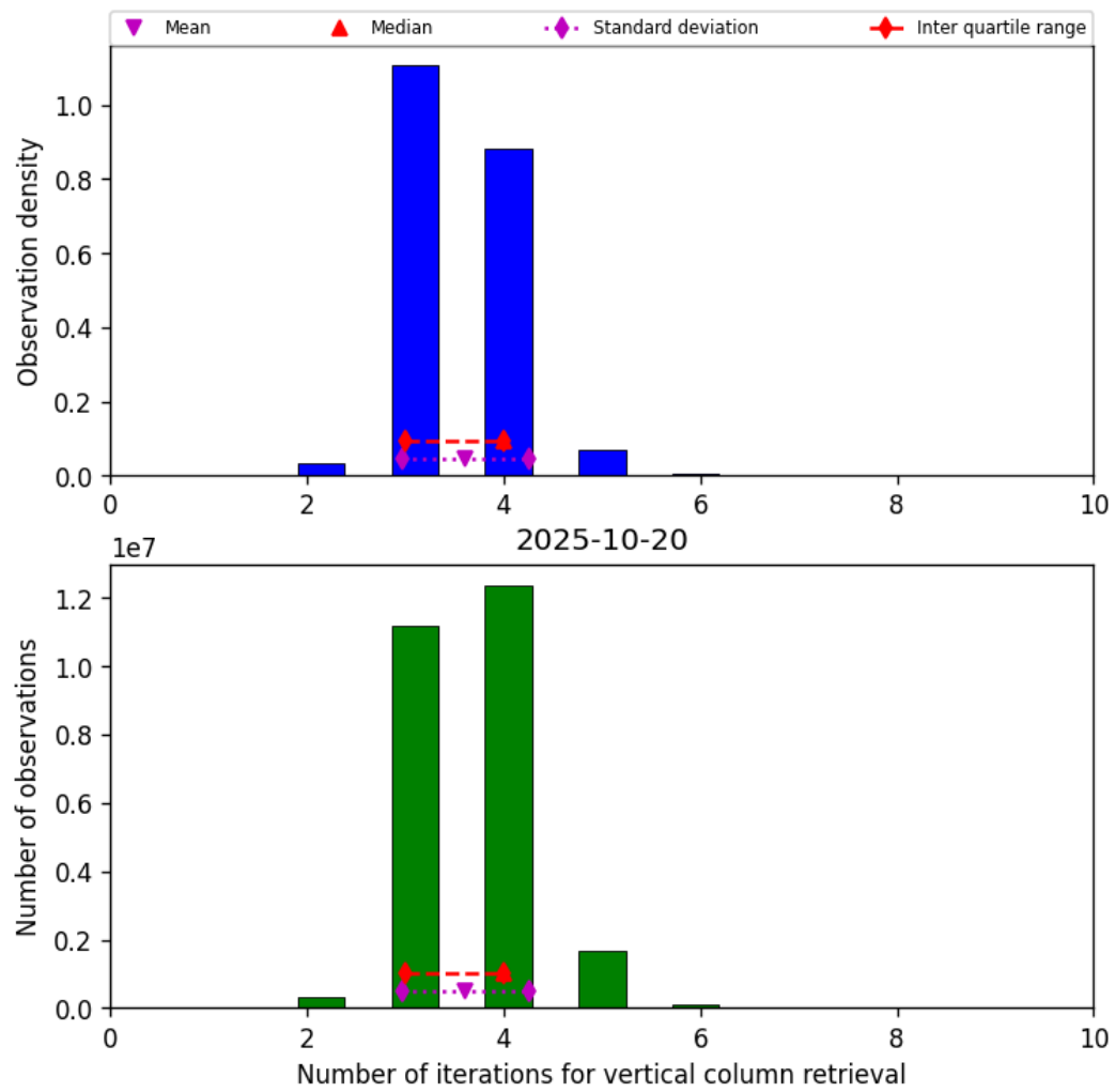
Figure 26: Histogram of “Number of iterations for vertical column retrieval” for 2025-10-19 to 2025-10-21
