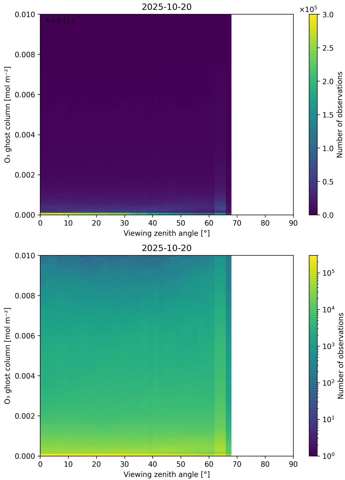
Figure 51: Scatter density plot of “Viewing zenith angle” against “O 3 ghost column” for 2025-10-19 to 2025-10-21.
