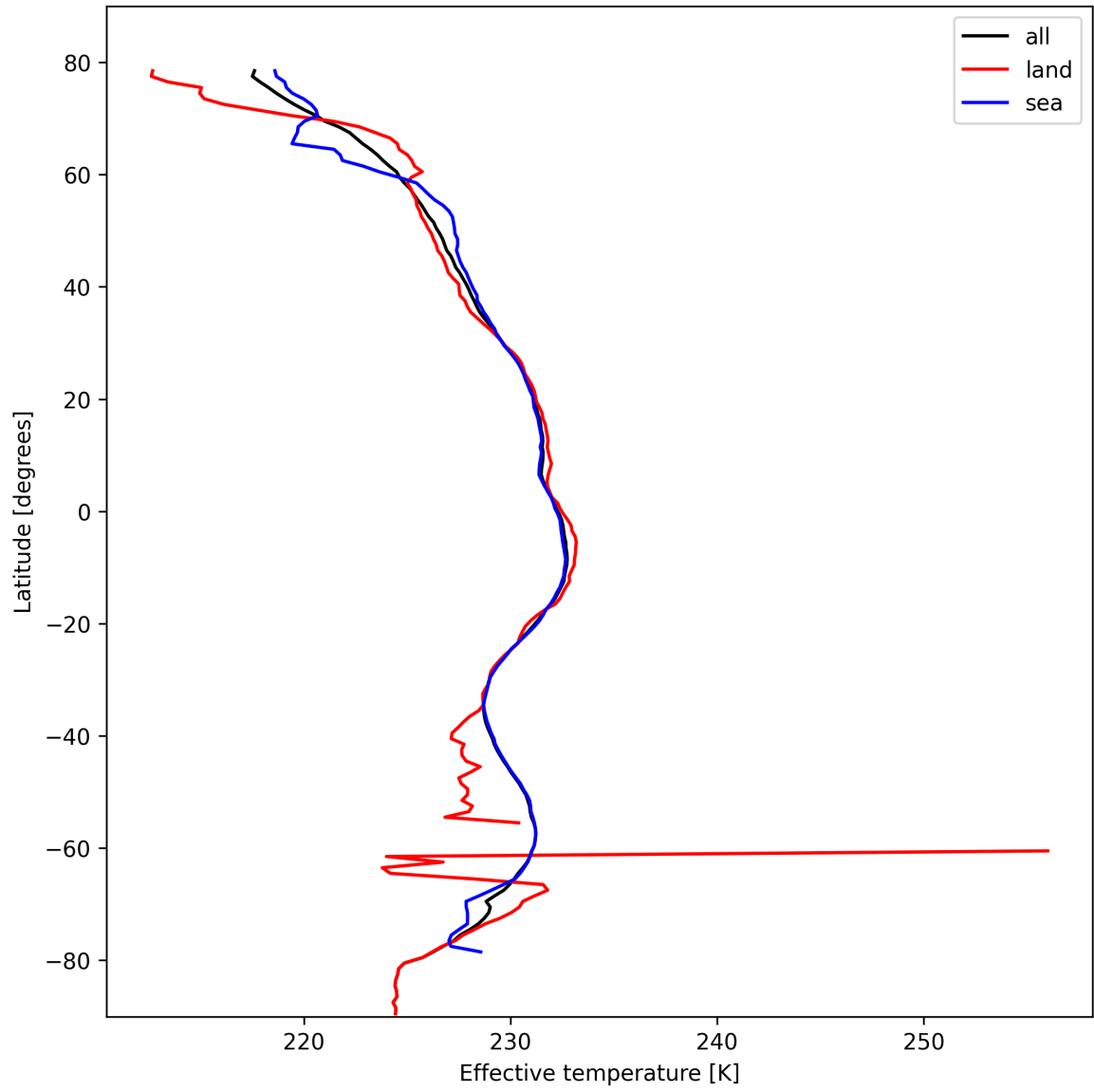
Figure 17: Zonal average of “Effective temperature” for 2025-10-19 to 2025-10-21.
