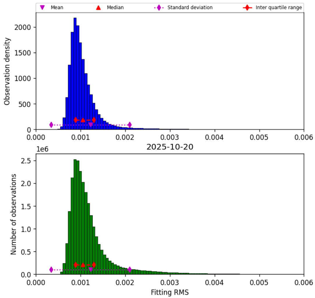
Figure 23: Histogram of “Fitting RMS” for 2025-10-19 to 2025-10-21
