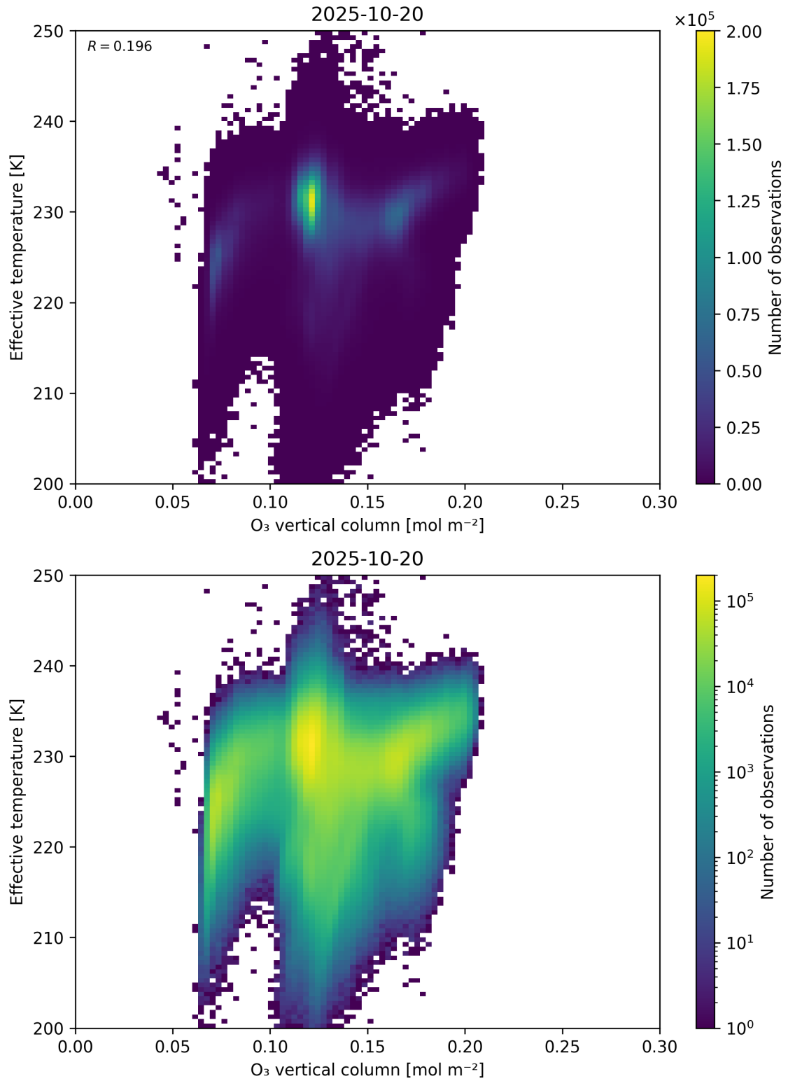
Figure 39: Scatter density plot of “O 3 vertical column” against “Effective temperature” for 2025-10-19 to 2025-10-21.
