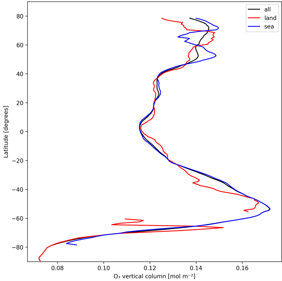
Figure 14: Zonal average of “O 3 vertical column” for 2025-10-19 to 2025-10-21.
