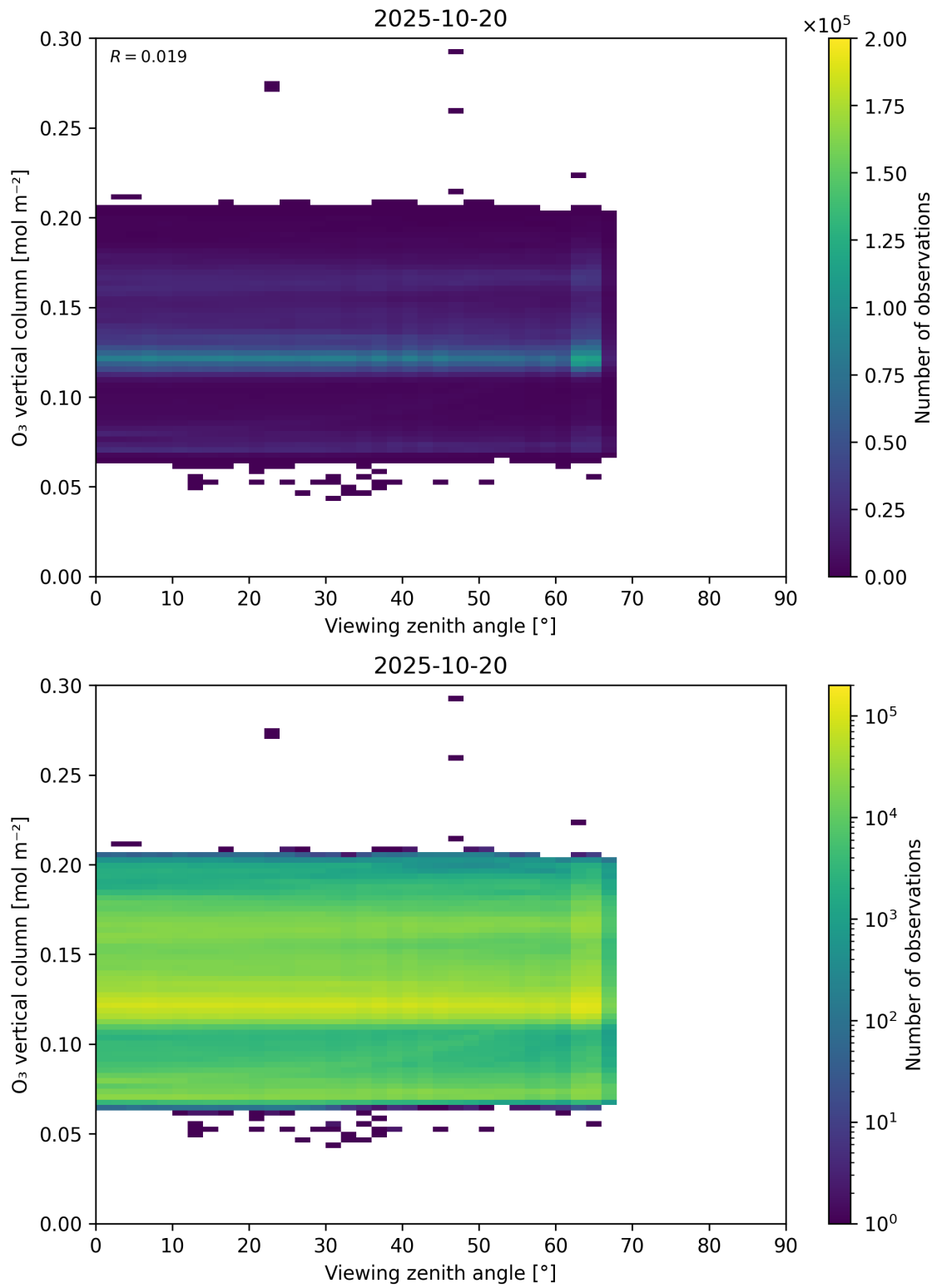
Figure 52: Scatter density plot of “Viewing zenith angle” against “O 3 vertical column” for 2025-10-19 to 2025-10-21.
