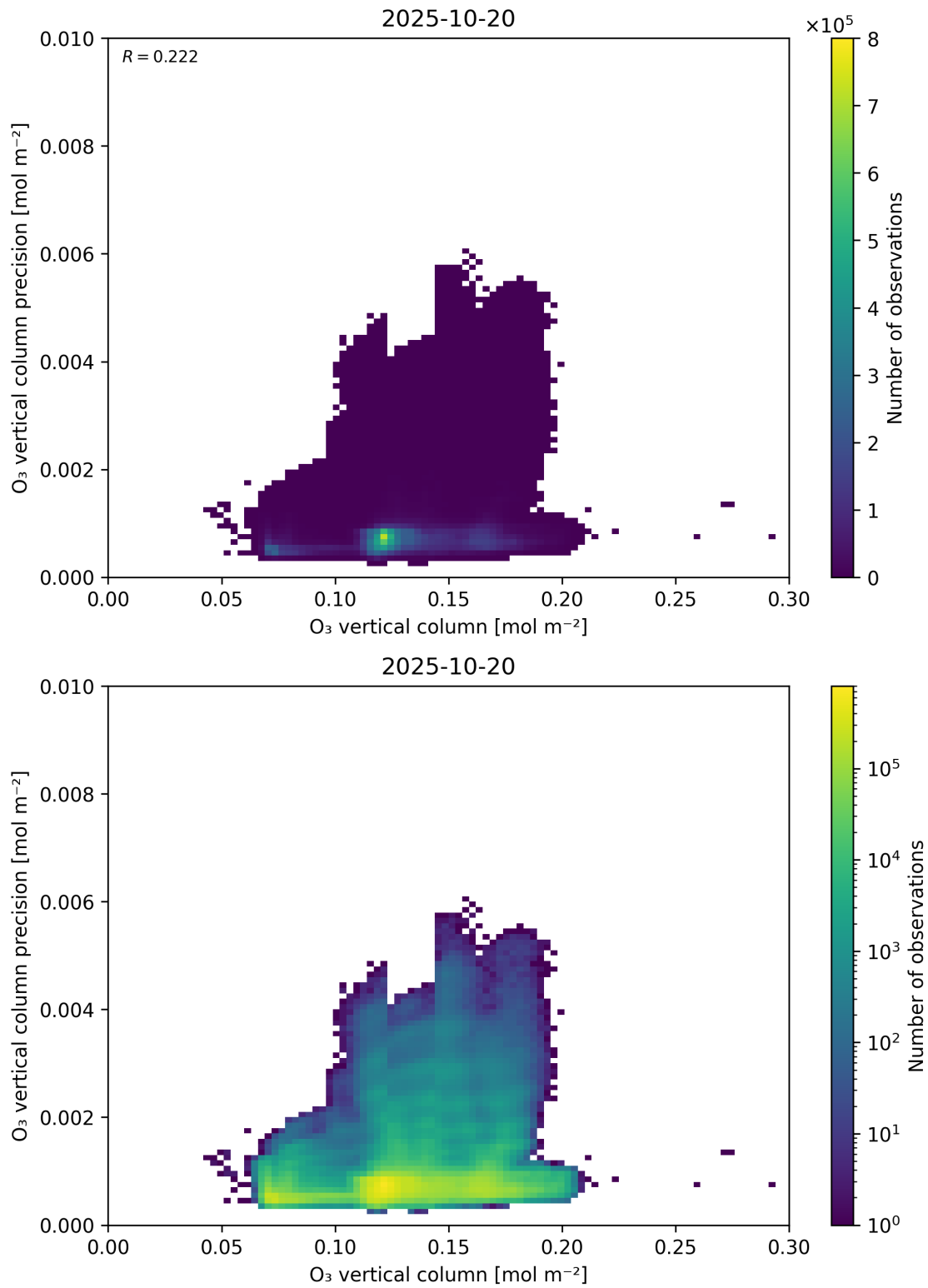
Figure 41: Scatter density plot of “O 3 vertical column” against “O 3 vertical column precision” for 2025-10-19 to 2025-10-21.
