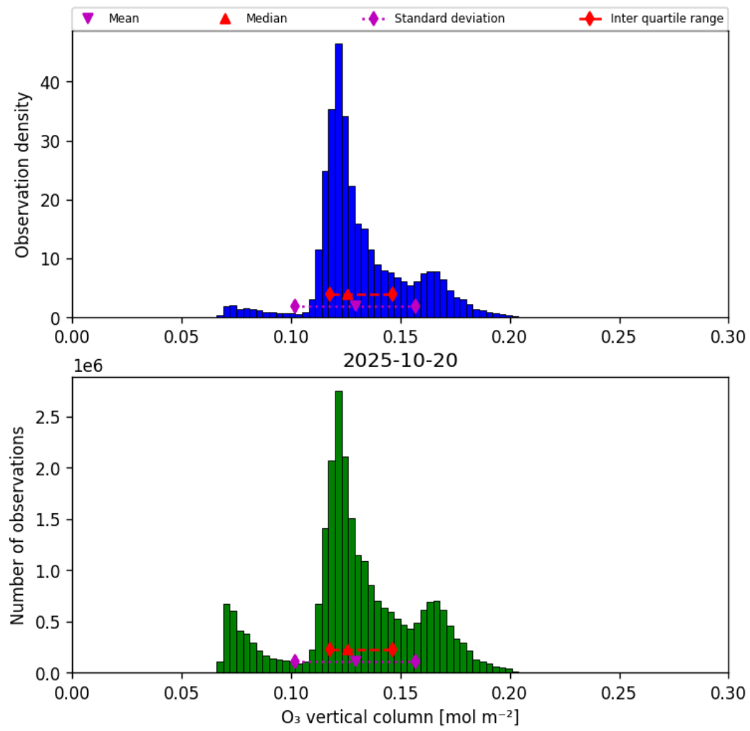
Figure 21: Histogram of “O 3 vertical column” for 2025-10-19 to 2025-10-21
