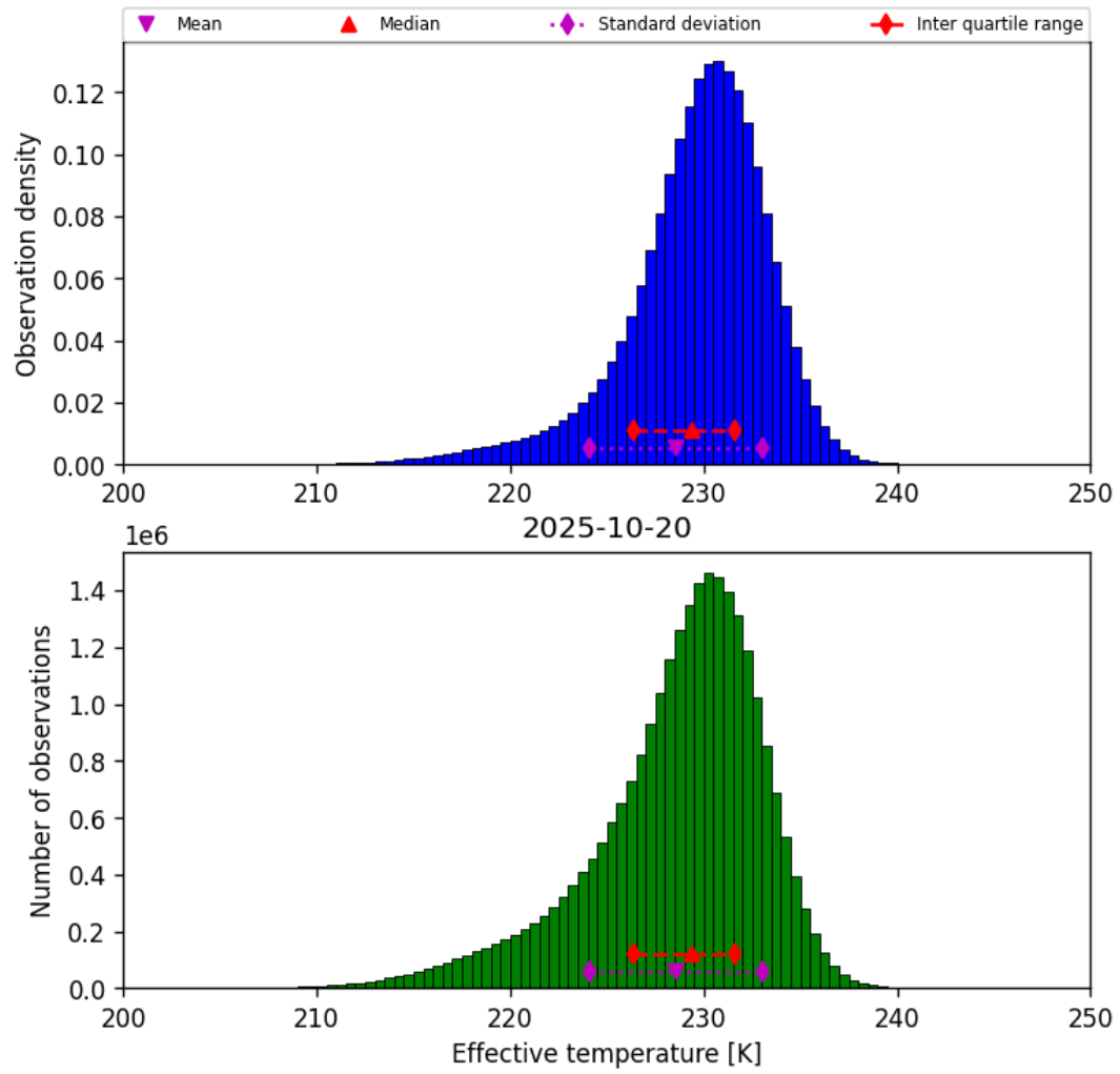
Figure 24: Histogram of “Effective temperature” for 2025-10-19 to 2025-10-21
