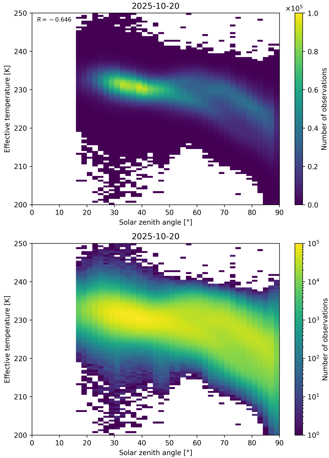
Figure 45: Scatter density plot of “Solar zenith angle” against “Effective temperature” for 2025-10-19 to 2025-10-21.
