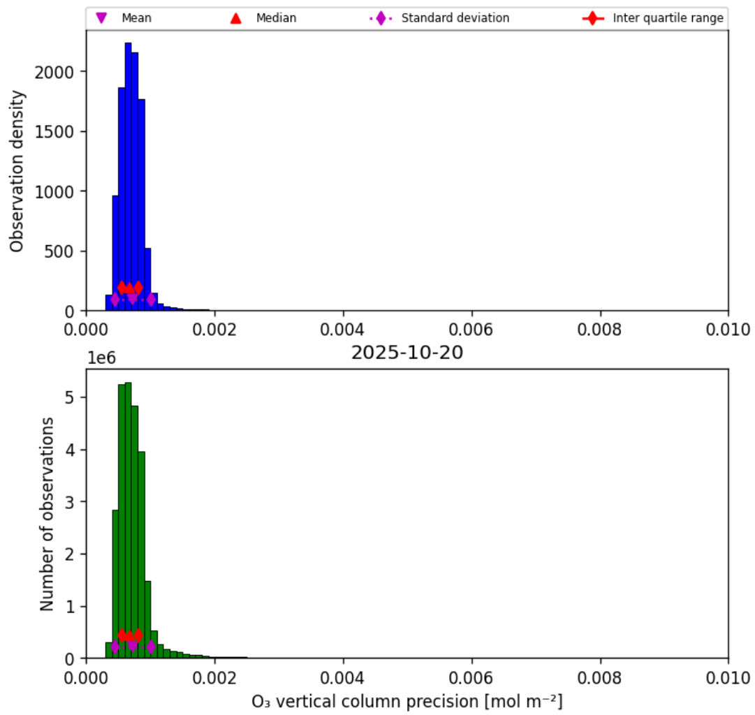
Figure 22: Histogram of “O 3 vertical column precision” for 2025-10-19 to 2025-10-21
