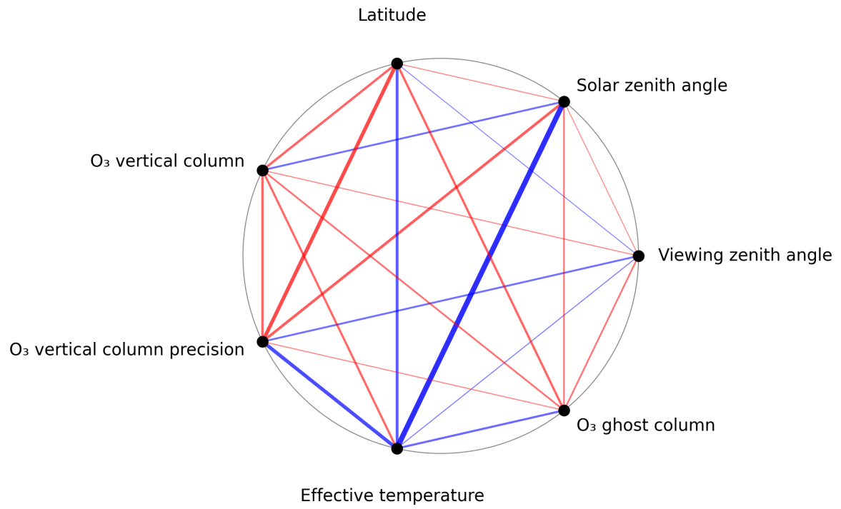
Figure 1: Map of correlation graph for 2025-10-19 to 2025-10-21.
