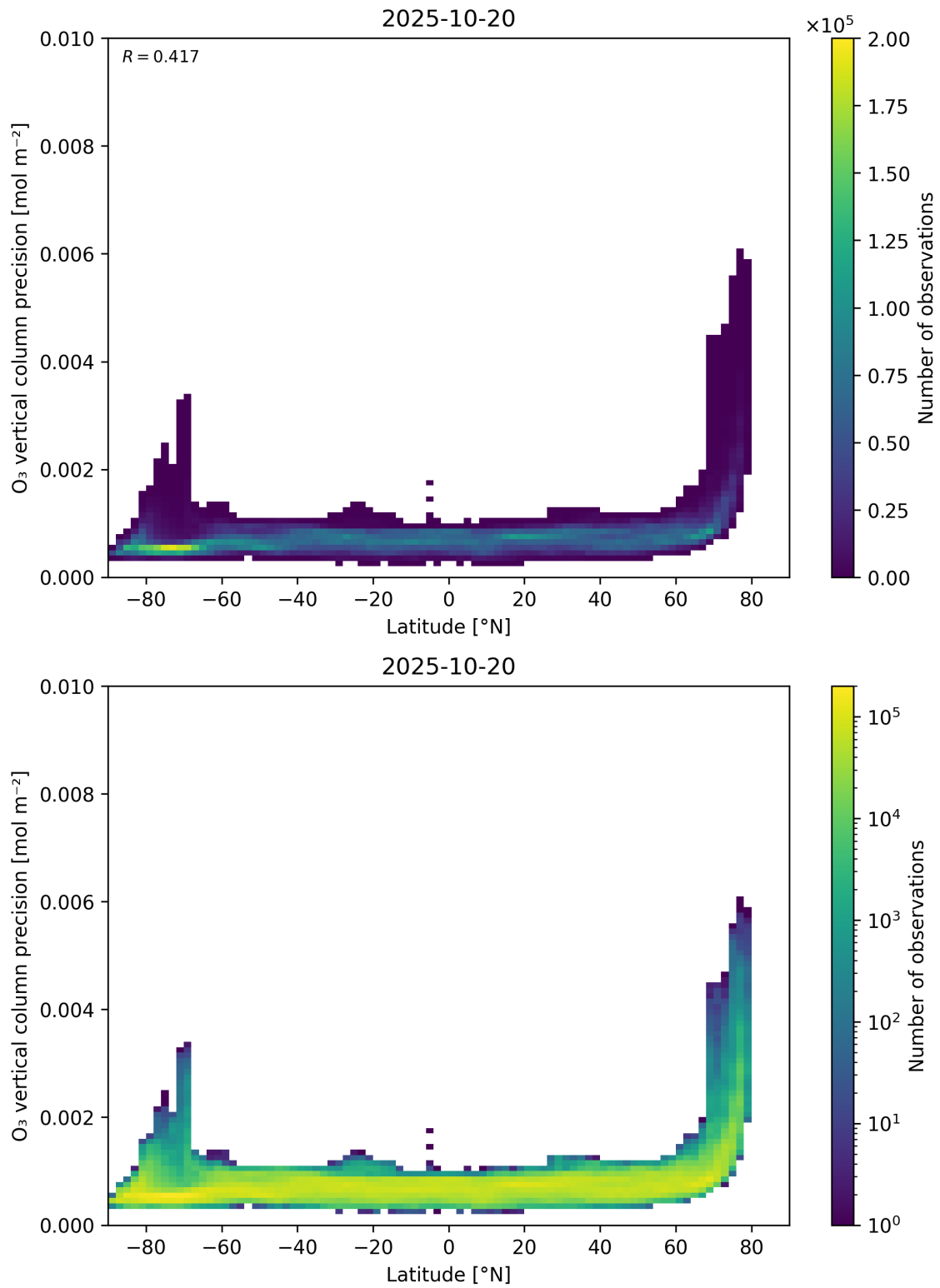
Figure 37: Scatter density plot of “Latitude” against “O 3 vertical column precision” for 2025-10-19 to 2025-10-21.
