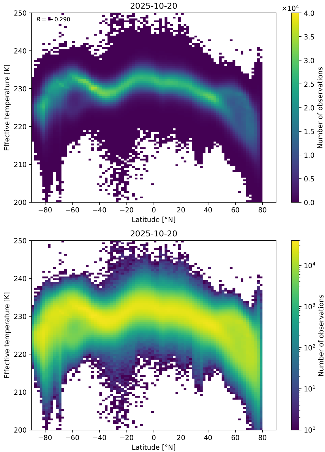
Figure 34: Scatter density plot of “Latitude” against “Effective temperature” for 2025-10-19 to 2025-10-21.
