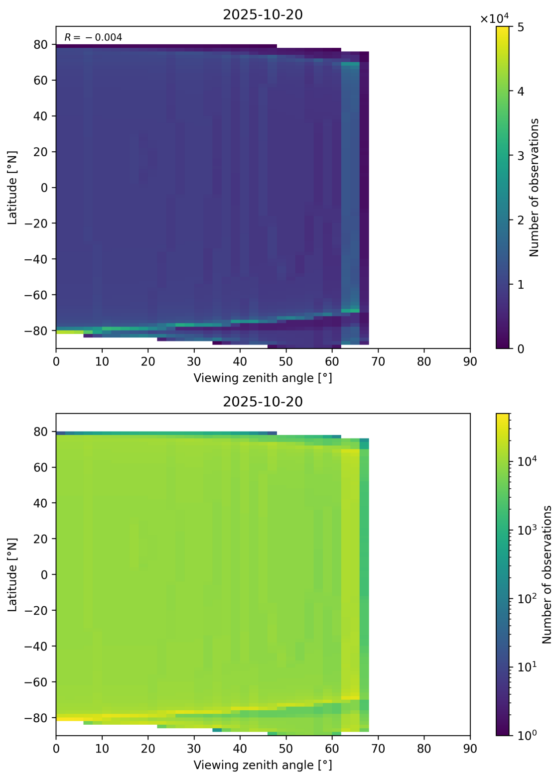
Figure 49: Scatter density plot of “Viewing zenith angle” against “Latitude” for 2025-10-19 to 2025-10-21.
