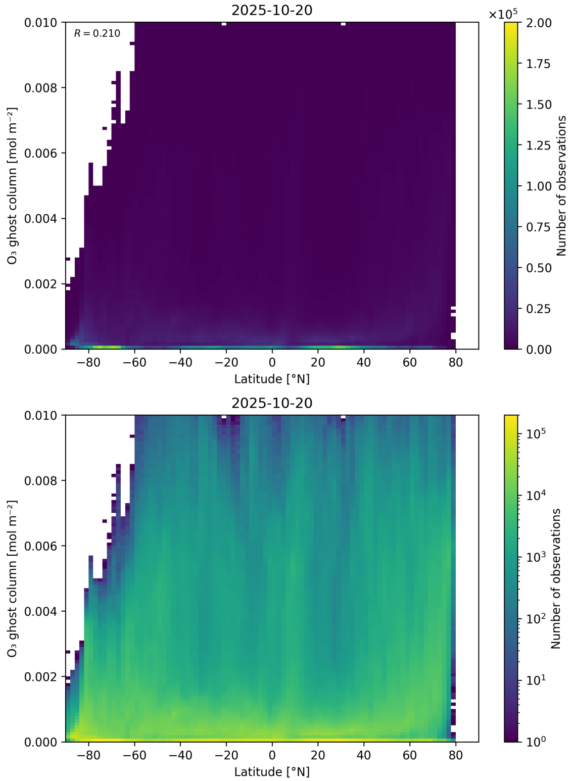
Figure 35: Scatter density plot of “Latitude” against “O 3 ghost column” for 2025-10-19 to 2025-10-21.
