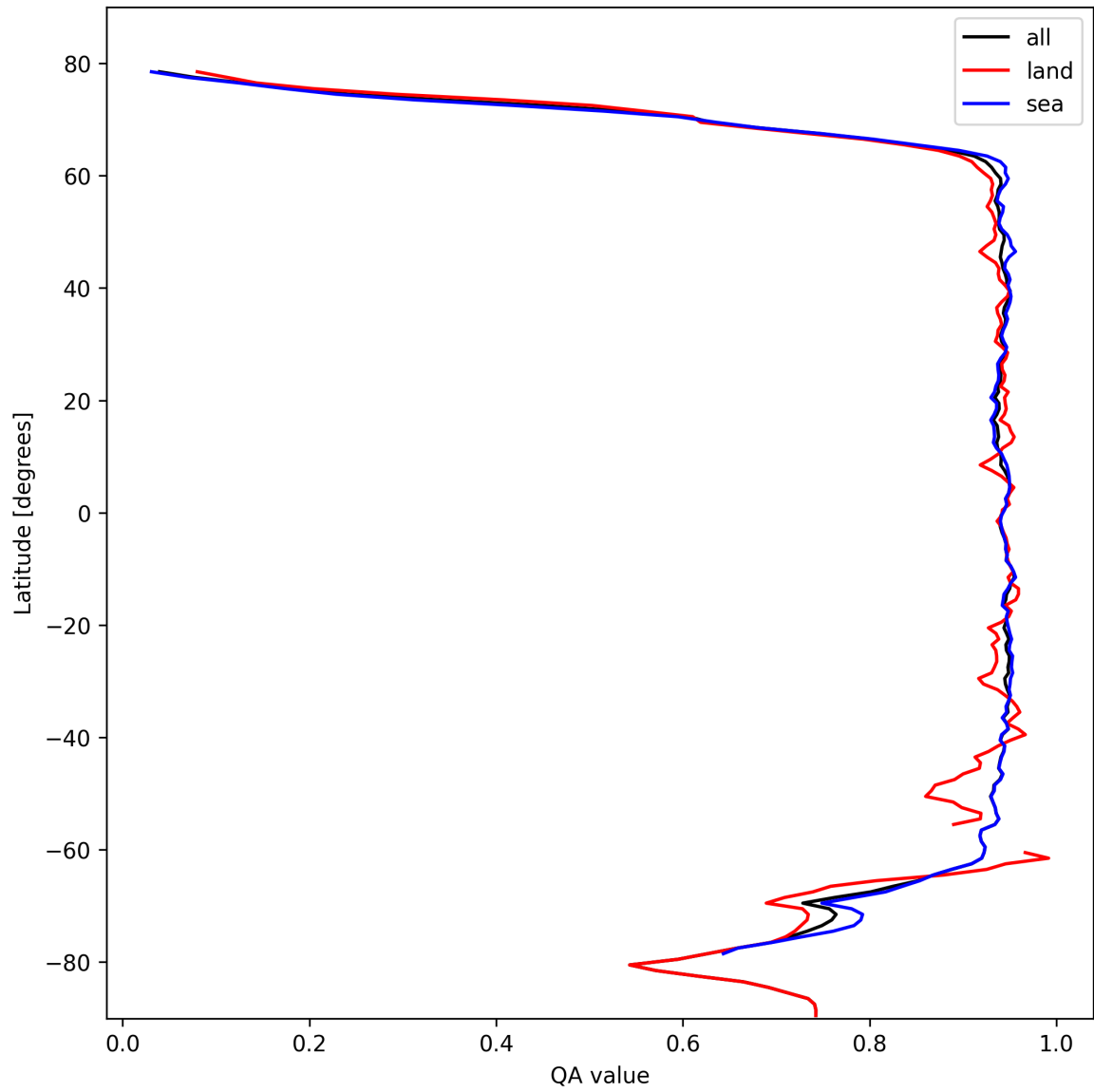
Figure 13: Zonal average of “QA value” for 2025-10-19 to 2025-10-21.
