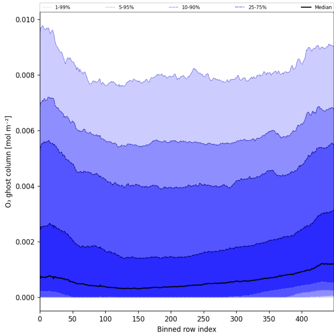
Figure 32: Along track statistics of “O 3 ghost column” for 2025-10-19 to 2025-10-21
