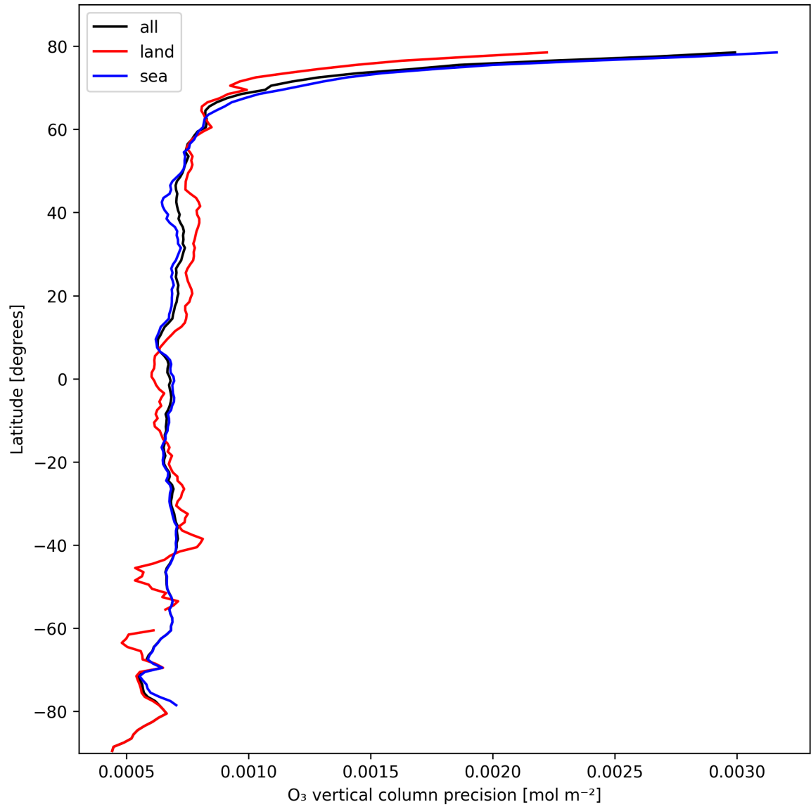
Figure 15: Zonal average of “O 3 vertical column precision” for 2025-10-19 to 2025-10-21.
