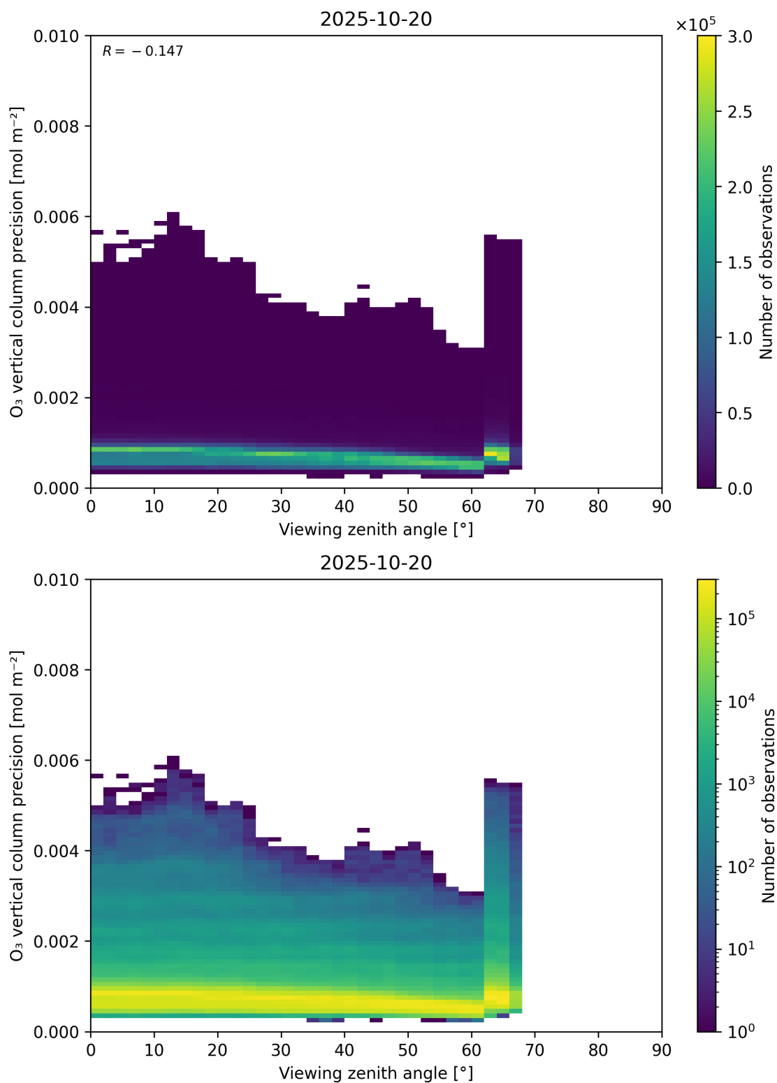
Figure 53: Scatter density plot of “Viewing zenith angle” against “O 3 vertical column precision” for 2025-10-19 to 2025-10-21.
