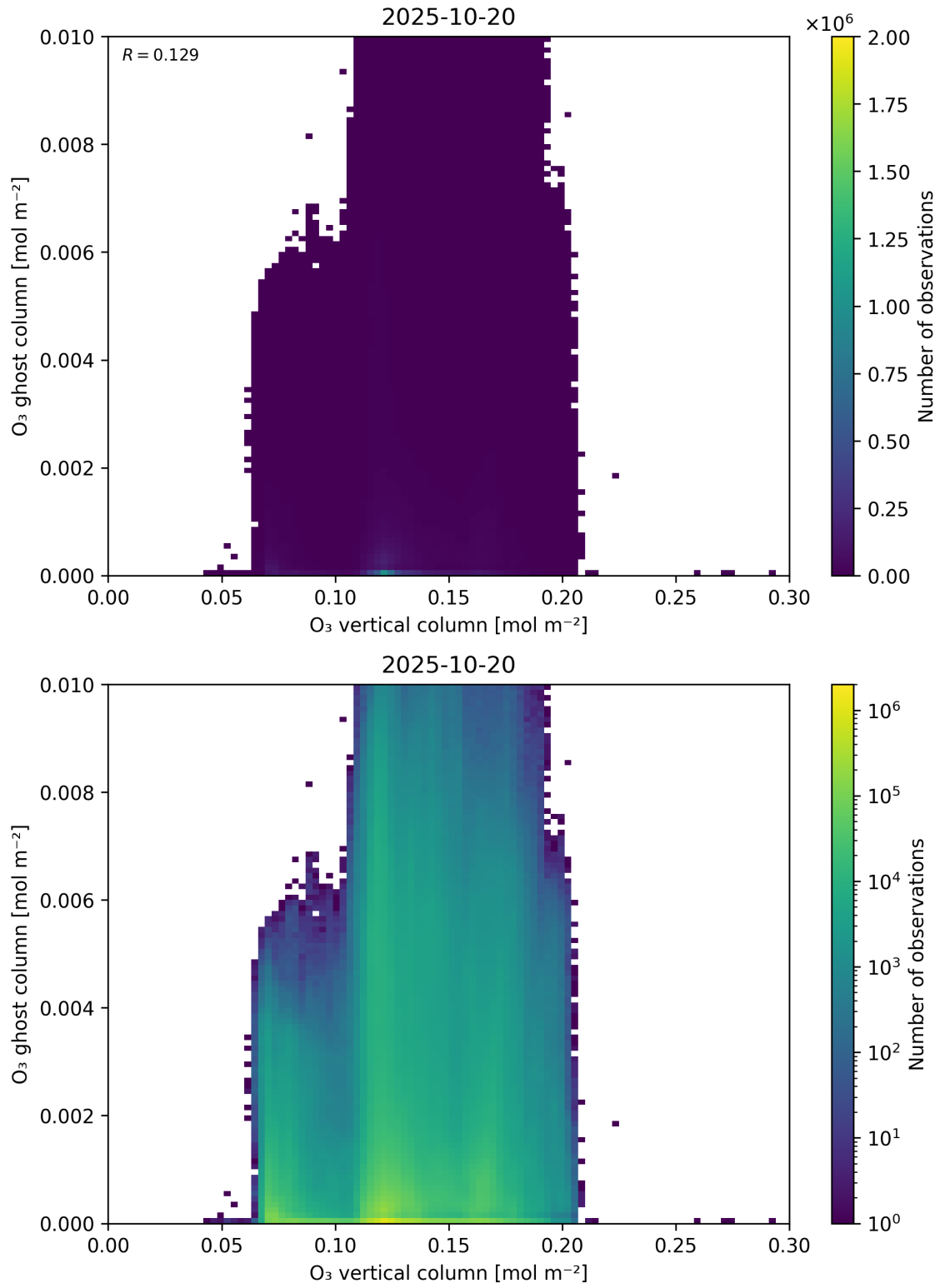
Figure 40: Scatter density plot of “O 3 vertical column” against “O 3 ghost column” for 2025-10-19 to 2025-10-21.
