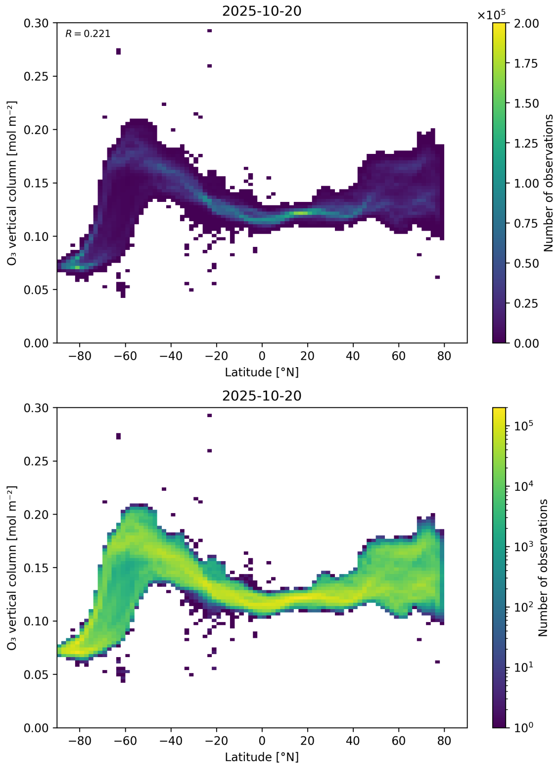
Figure 36: Scatter density plot of “Latitude” against “O 3 vertical column” for 2025-10-19 to 2025-10-21.
