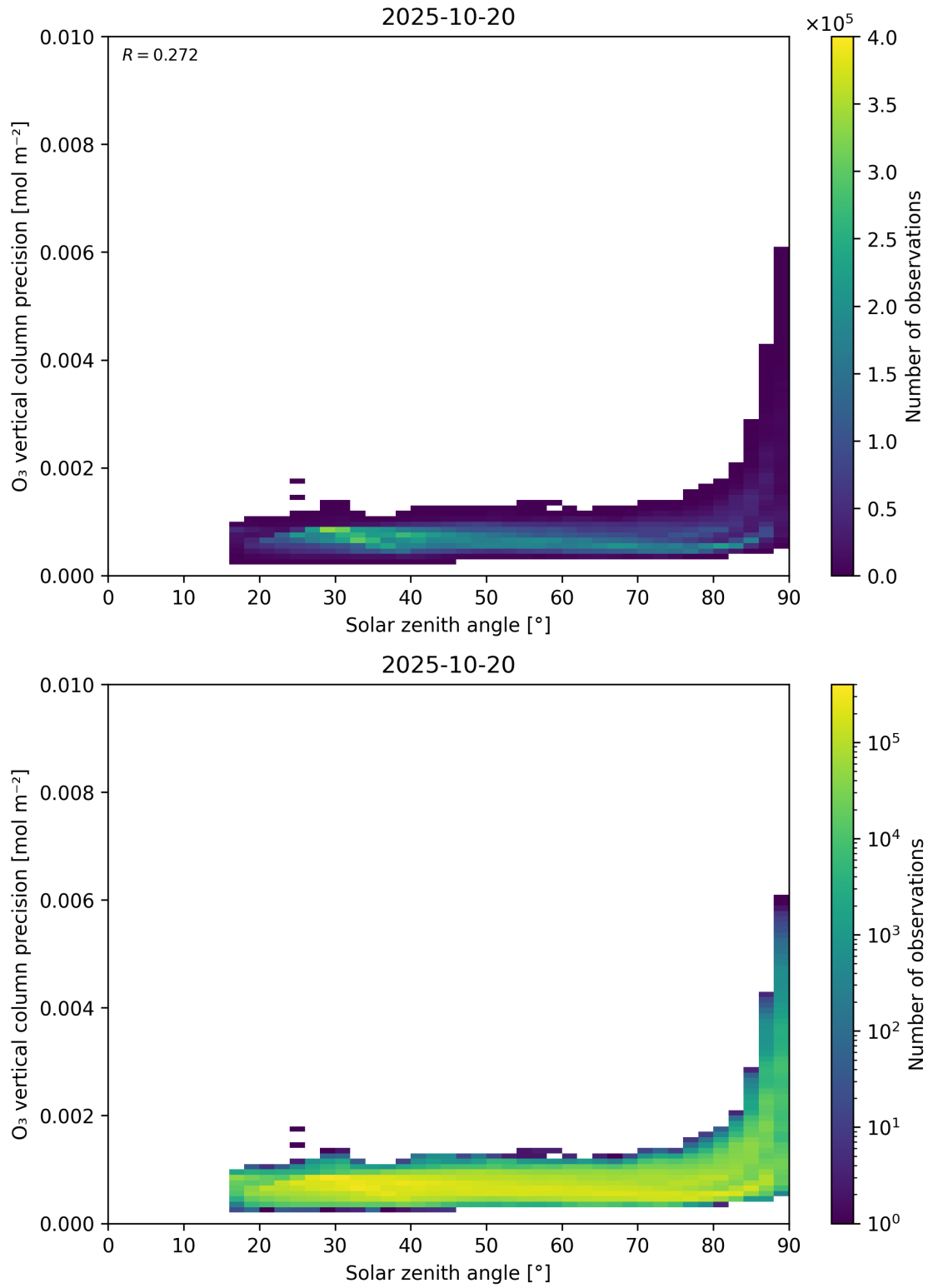
Figure 48: Scatter density plot of “Solar zenith angle” against “O 3 vertical column precision” for 2025-10-19 to 2025-10-21.
