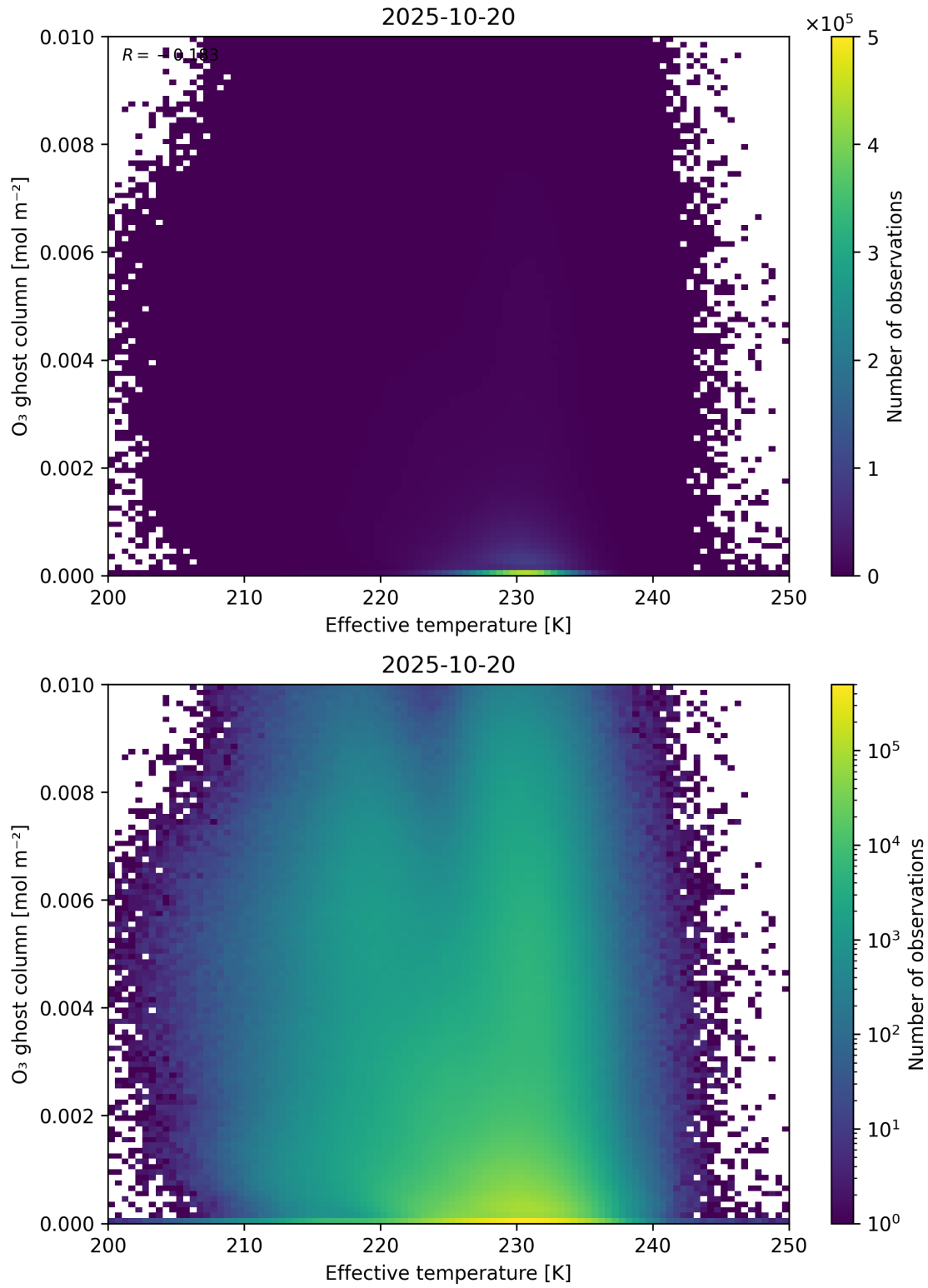
Figure 38: Scatter density plot of “Effective temperature” against “O 3 ghost column” for 2025-10-19 to 2025-10-21.
