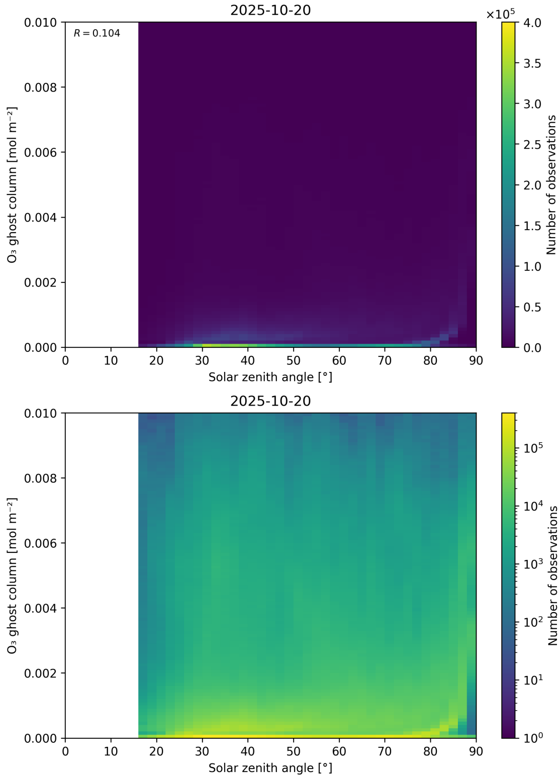
Figure 46: Scatter density plot of “Solar zenith angle” against “O 3 ghost column” for 2025-10-19 to 2025-10-21.
