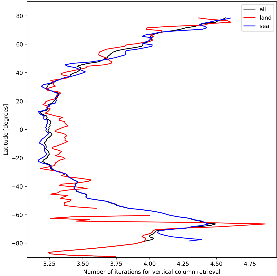
Figure 19: Zonal average of “Number of iterations for vertical column retrieval” for 2025-10-19 to 2025-10-21.
