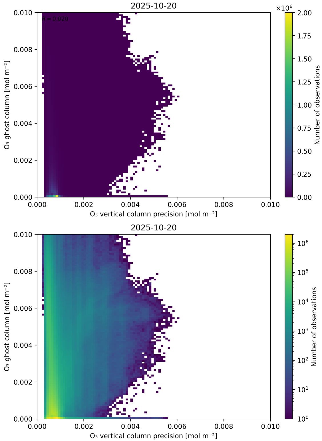
Figure 43: Scatter density plot of “O 3 vertical column precision” against “O 3 ghost column” for 2025-10-19 to 2025-10-21.
