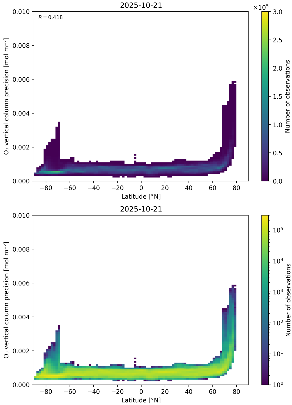
Figure 37: Scatter density plot of “Latitude” against “O 3 vertical column precision” for 2025-10-20 to 2025-10-22.
