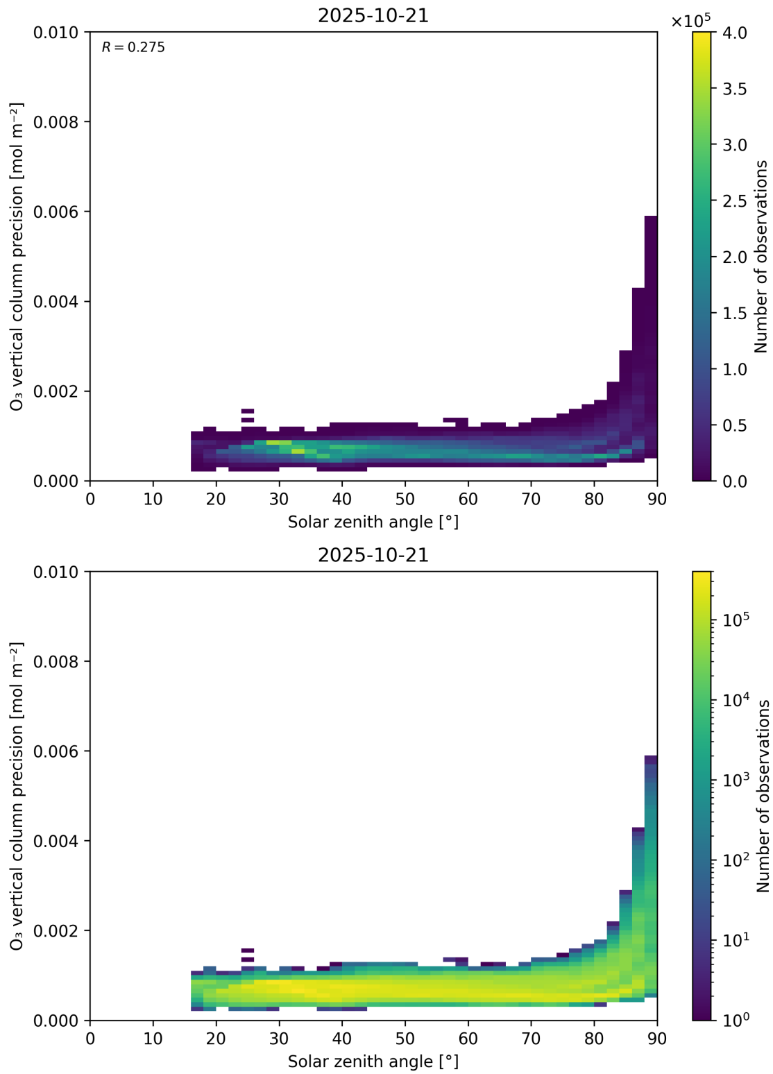
Figure 48: Scatter density plot of “Solar zenith angle” against “O 3 vertical column precision” for 2025-10-20 to 2025-10-22.
