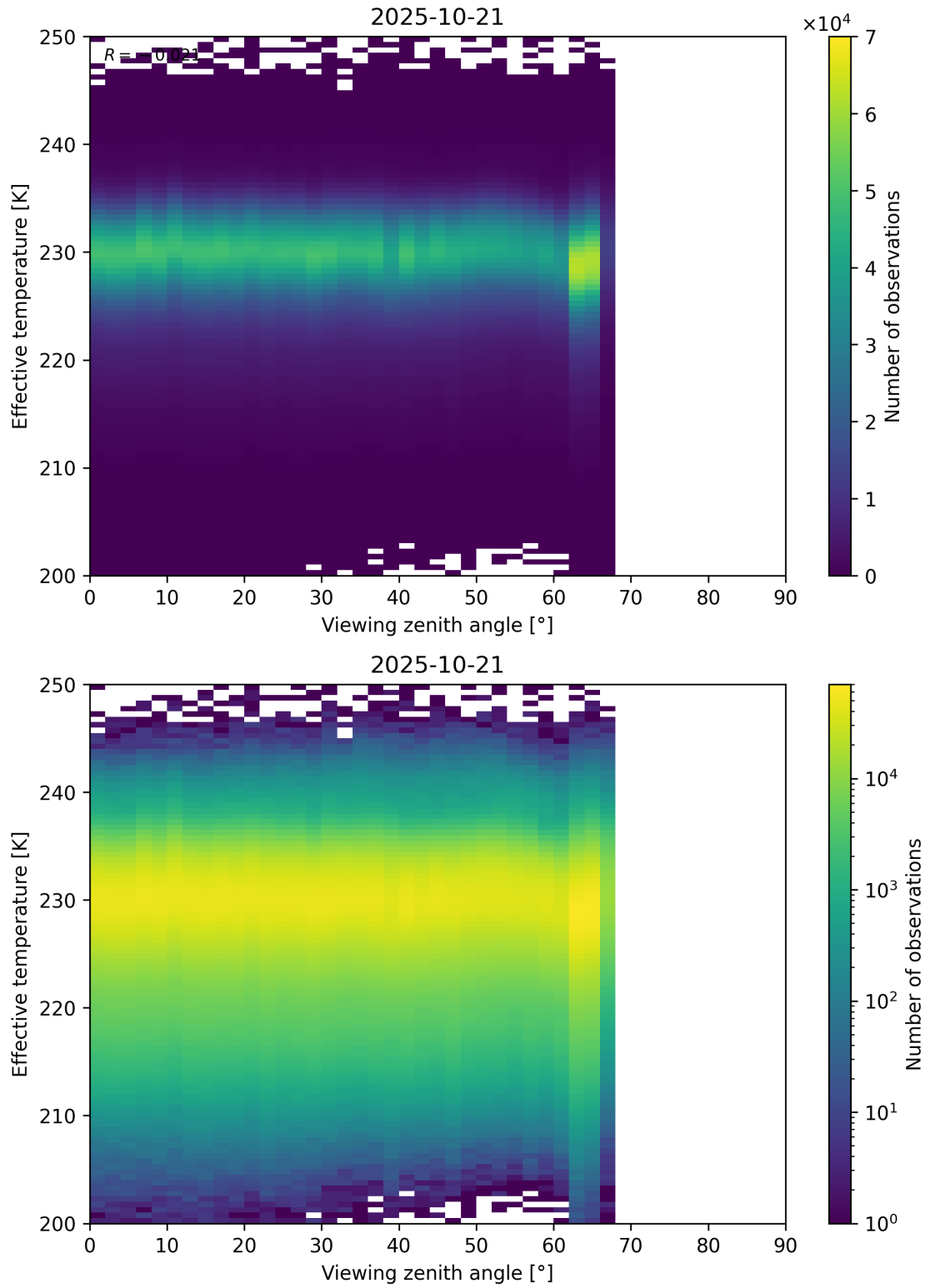
Figure 50: Scatter density plot of “Viewing zenith angle” against “Effective temperature” for 2025-10-20 to 2025-10-22.
