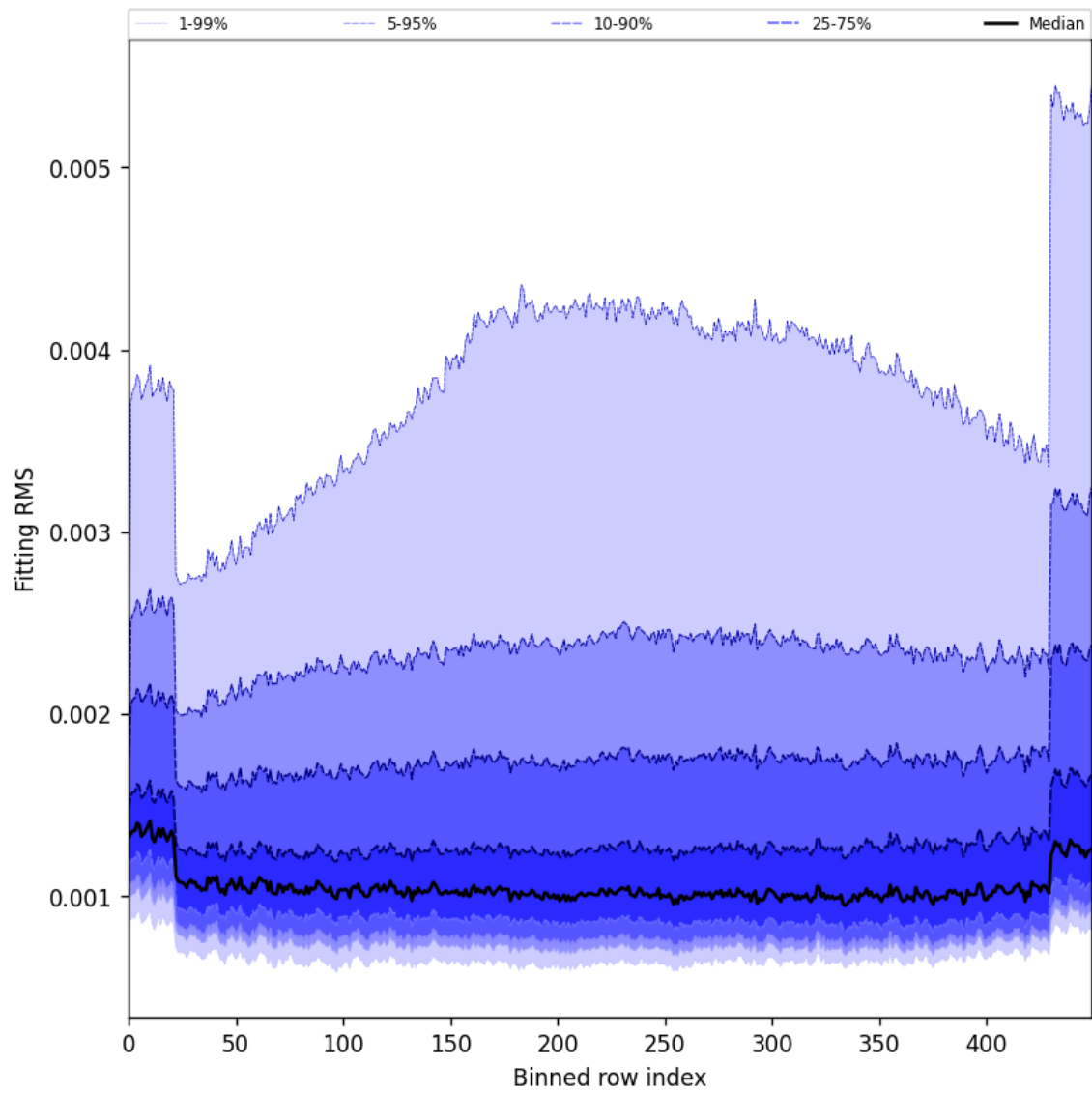
Figure 30: Along track statistics of “Fitting RMS” for 2025-10-20 to 2025-10-22
