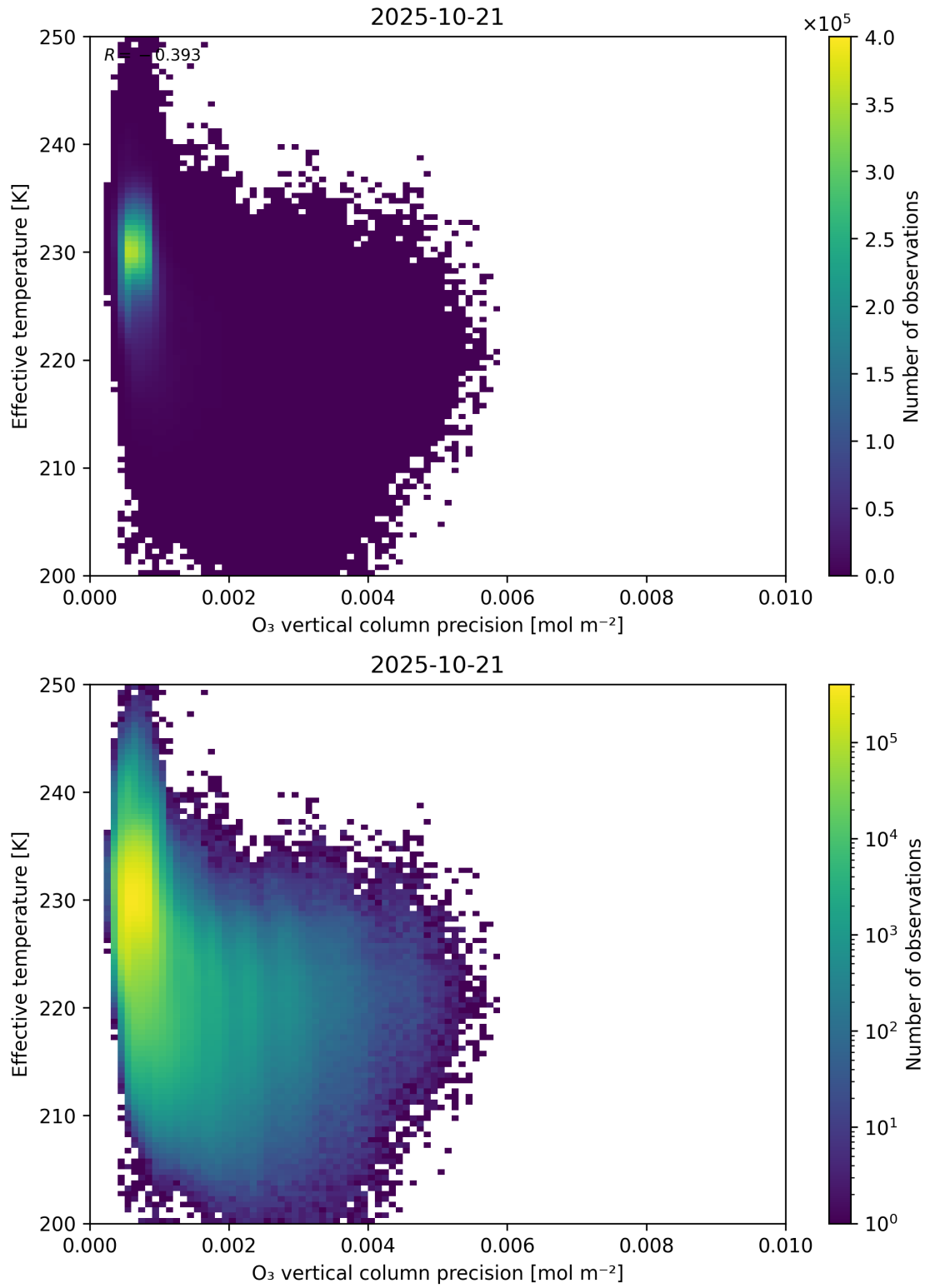
Figure 42: Scatter density plot of “O 3 vertical column precision” against “Effective temperature” for 2025-10-20 to 2025-10-22.
