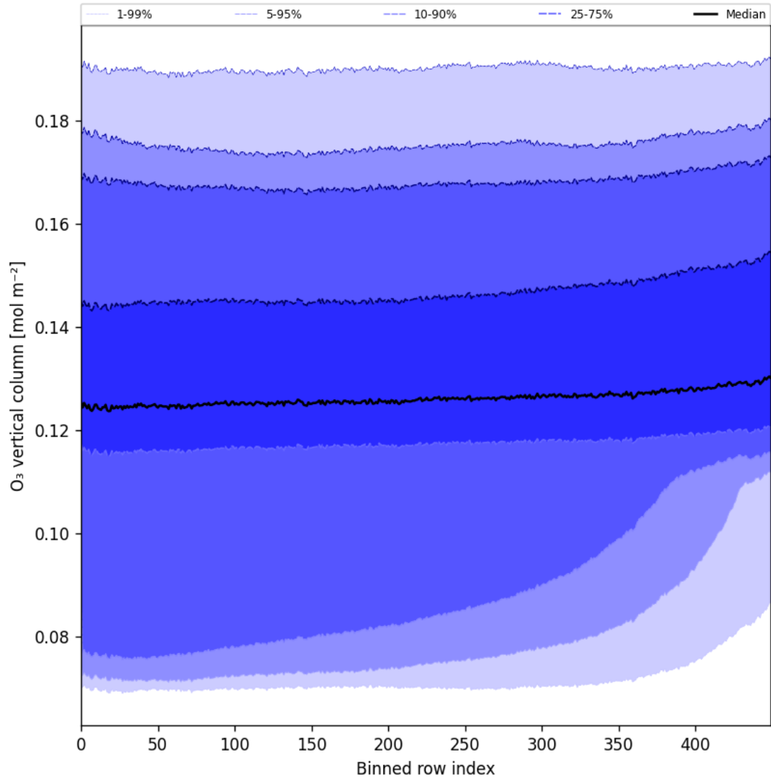
Figure 28: Along track statistics of "O 3 vertical column" for 2025-10-20 to 2025-10-22
