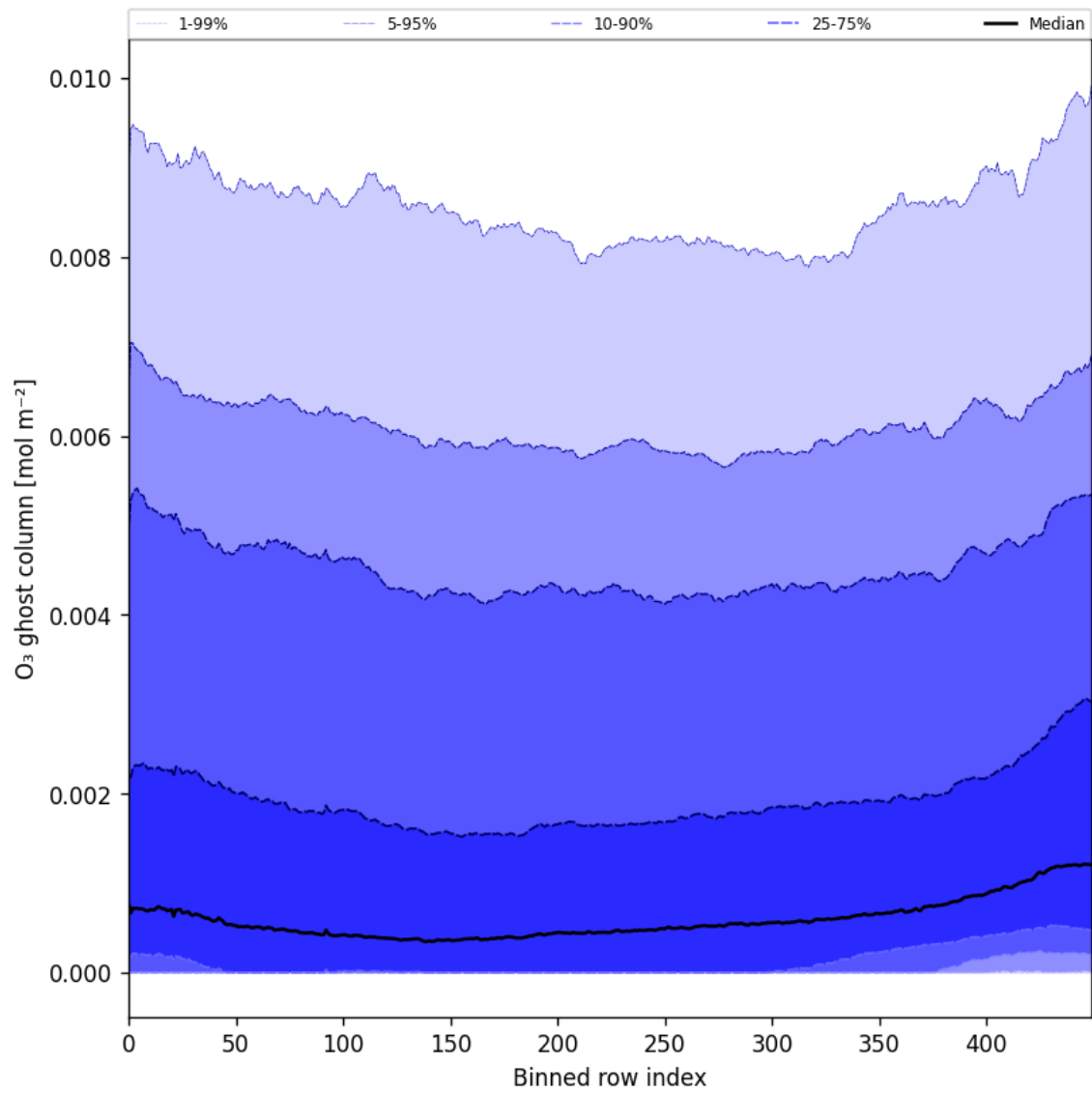
Figure 32: Along track statistics of “O 3 ghost column” for 2025-10-20 to 2025-10-22
