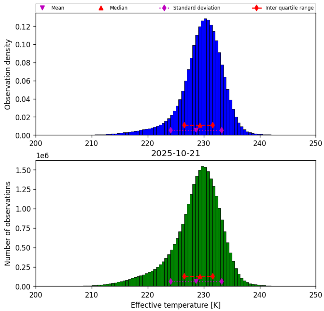
Figure 24: Histogram of “Effective temperature” for 2025-10-20 to 2025-10-22
