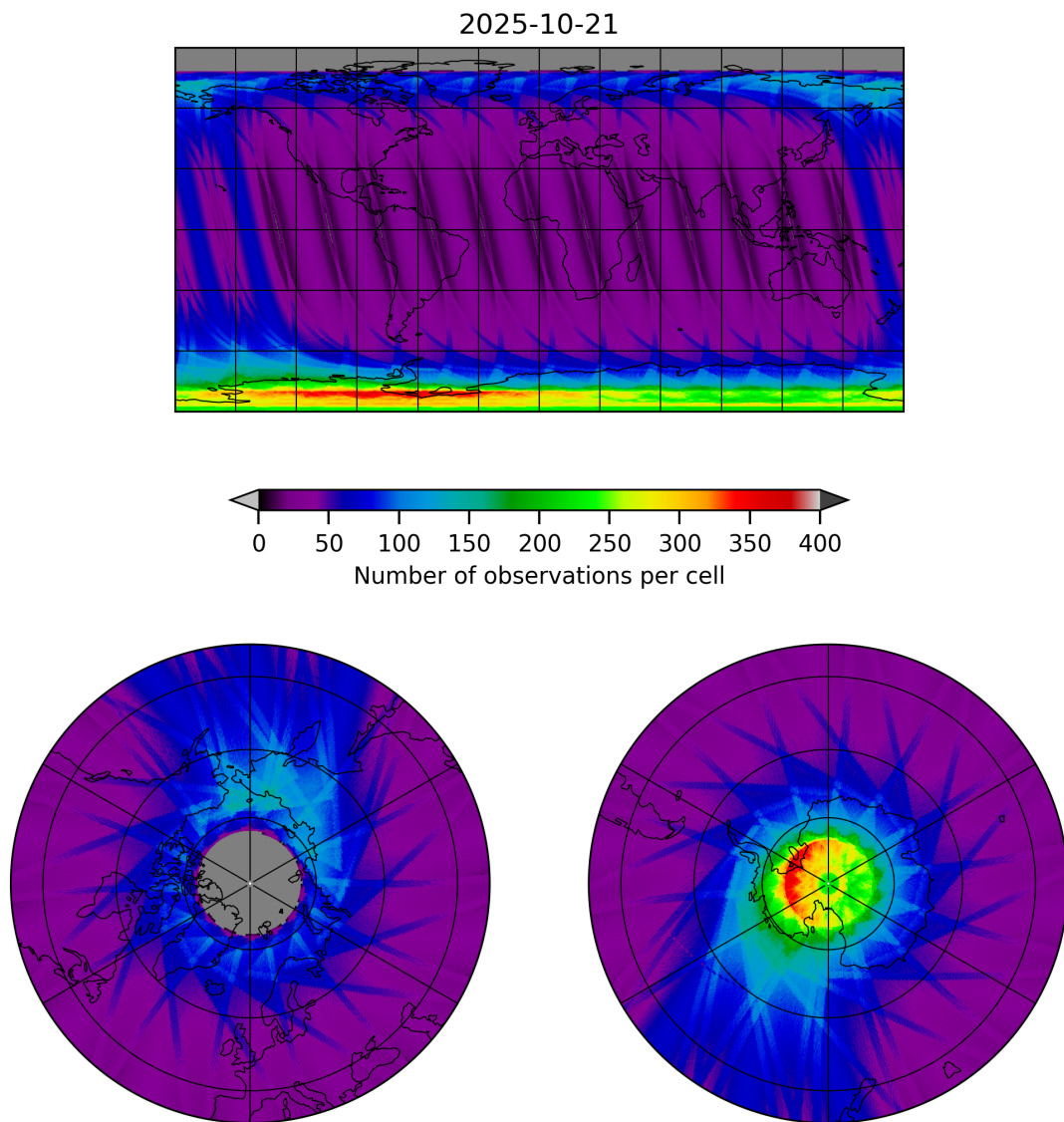
Figure 12: Map of the number of observations for 2025-10-20 to 2025-10-22
