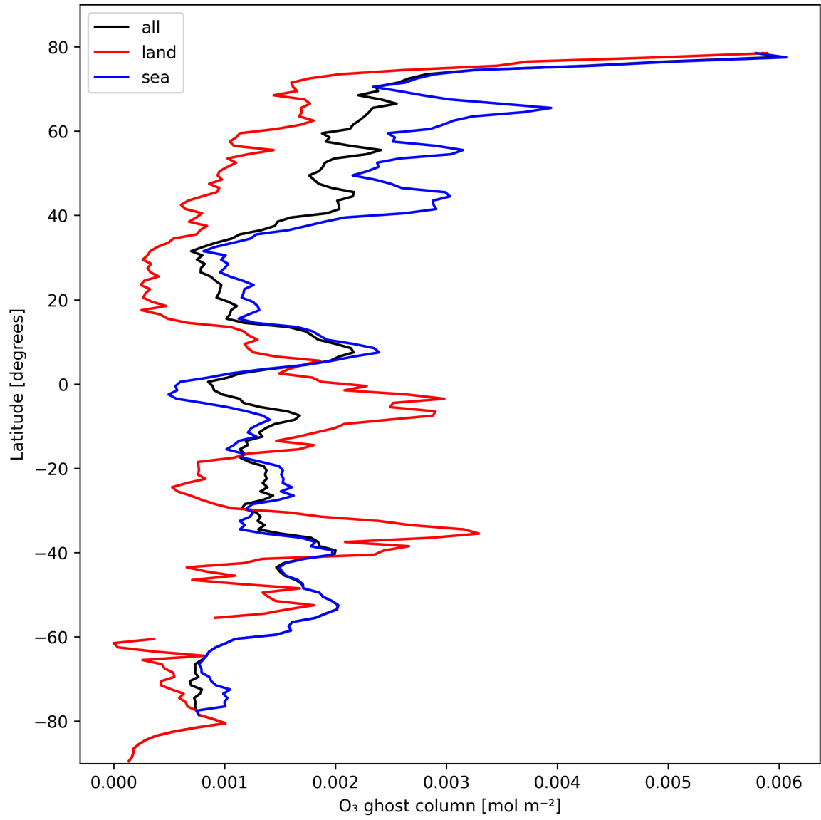
Figure 18: Zonal average of "O 3 ghost column" for 2025-10-20 to 2025-10-22.
