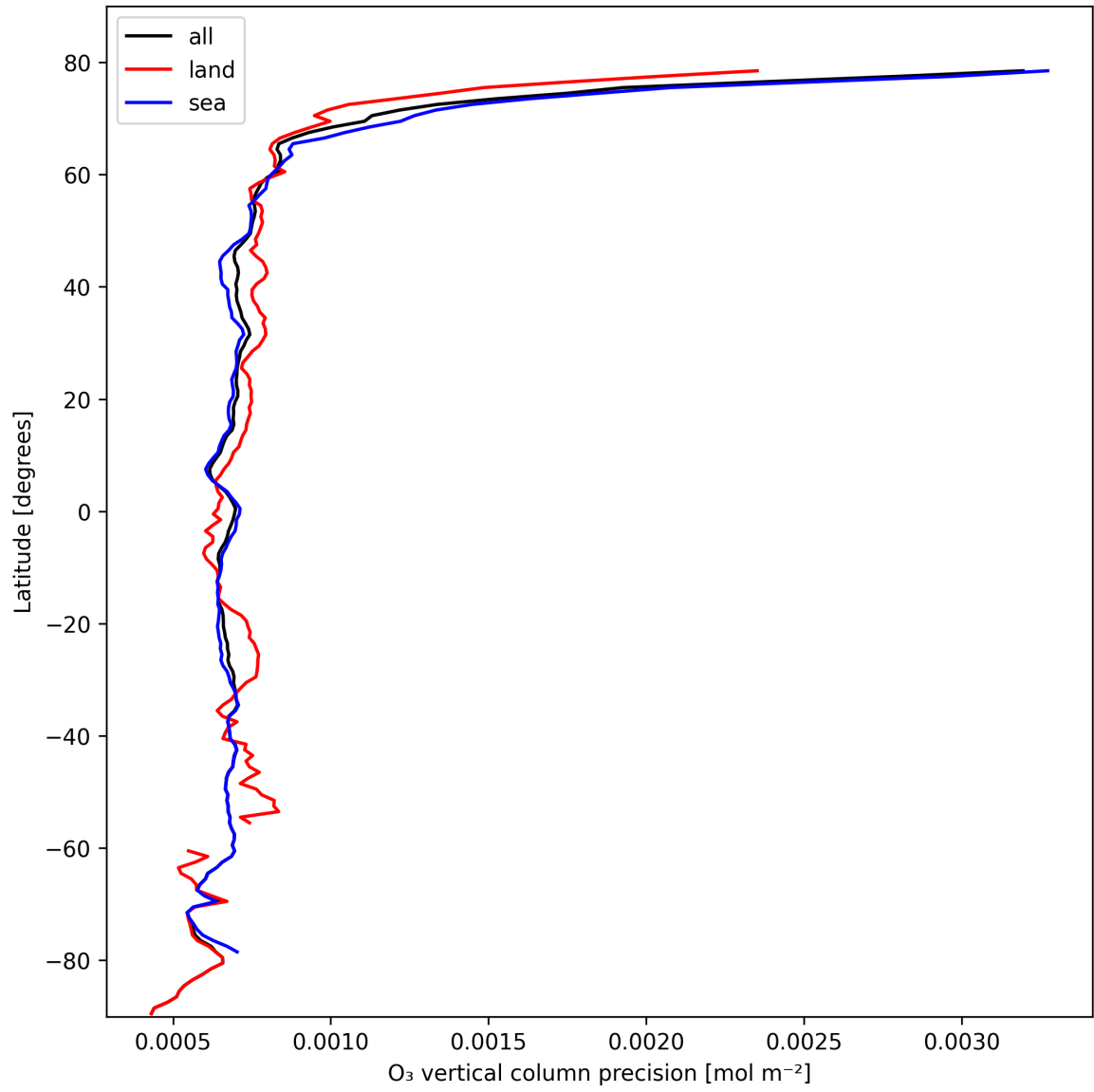
Figure 15: Zonal average of “O 3 vertical column precision” for 2025-10-20 to 2025-10-22.
