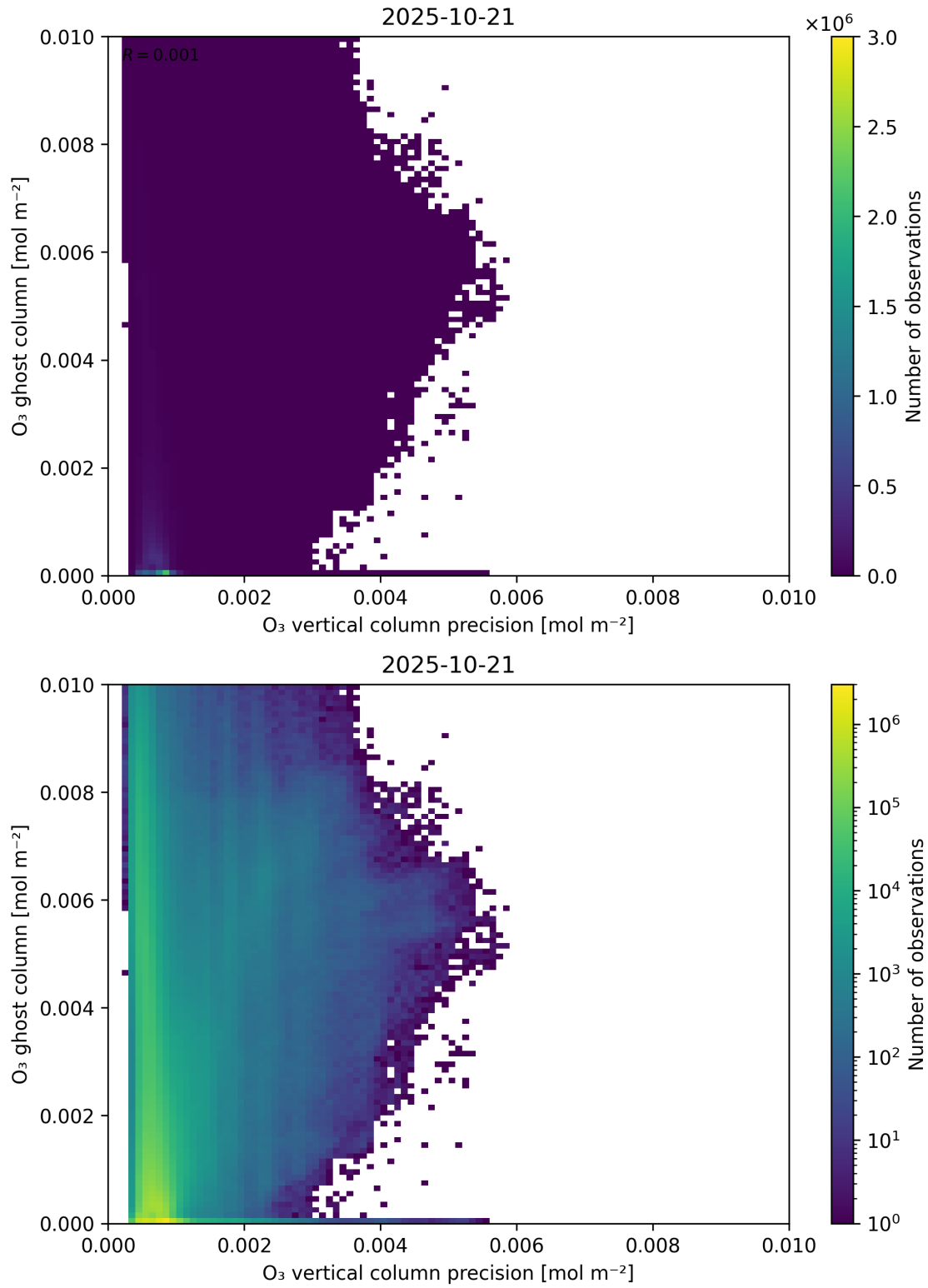
Figure 43: Scatter density plot of “O 3 vertical column precision” against “O 3 ghost column” for 2025-10-20 to 2025-10-22.
