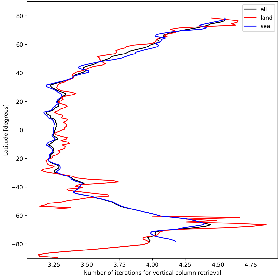
Figure 19: Zonal average of “Number of iterations for vertical column retrieval” for 2025-10-20 to 2025-10-22.
