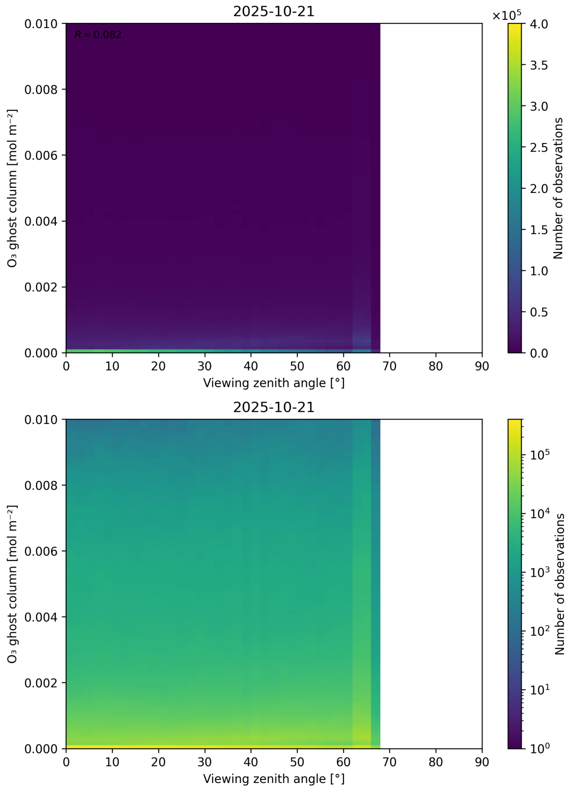
Figure 51: Scatter density plot of “Viewing zenith angle” against “O 3 ghost column” for 2025-10-20 to 2025-10-22.
