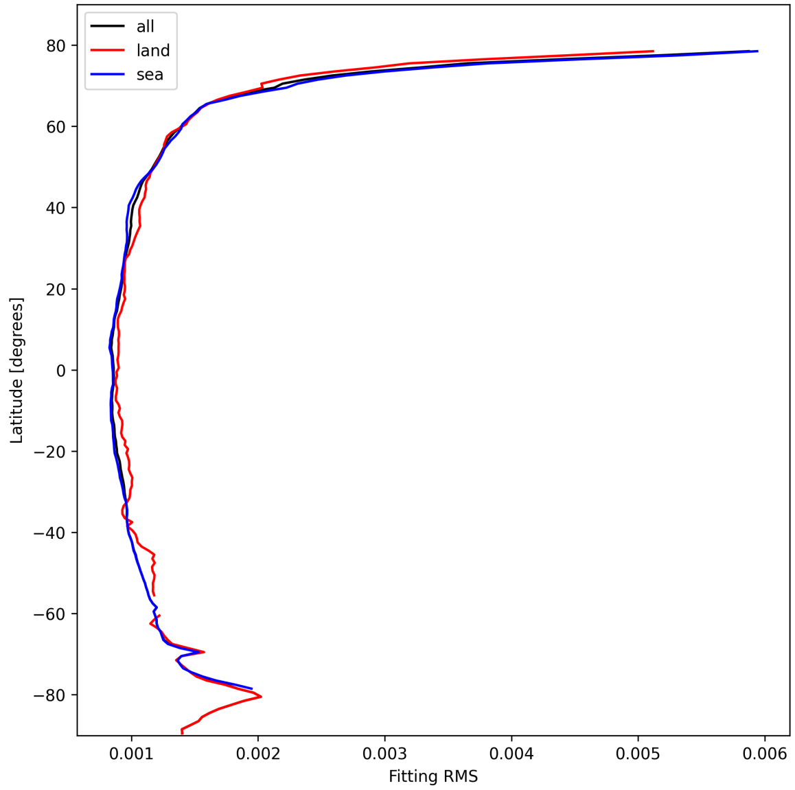
Figure 16: Zonal average of “Fitting RMS” for 2025-10-20 to 2025-10-22.
