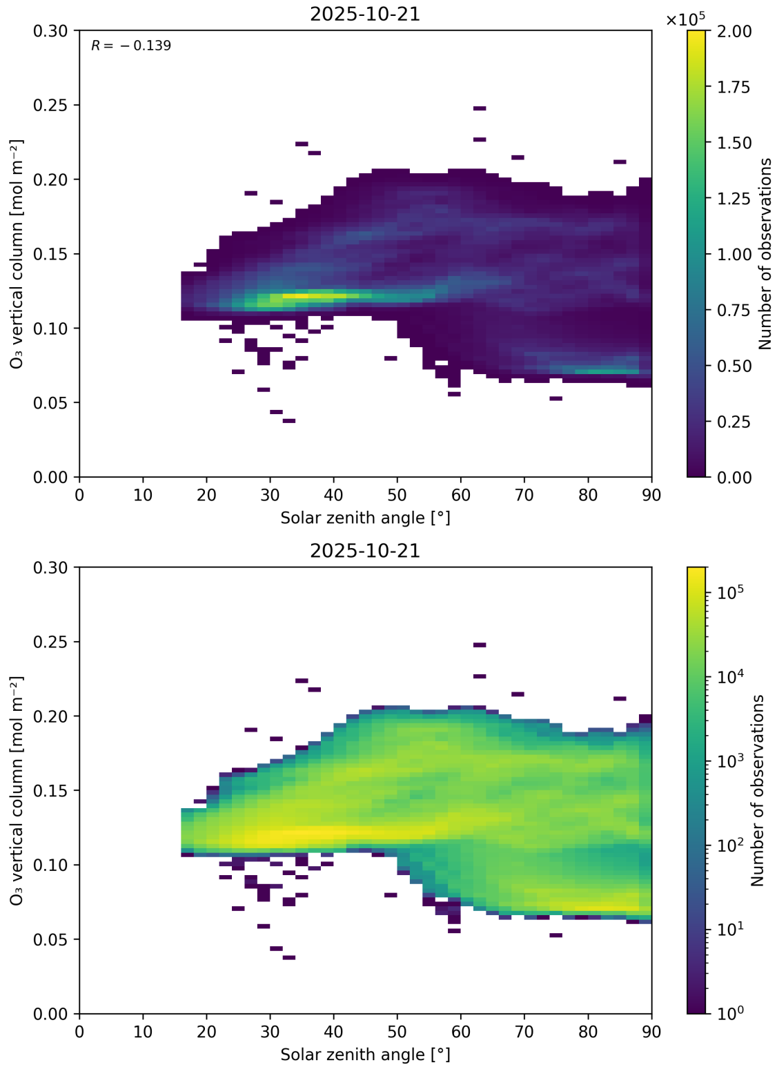
Figure 47: Scatter density plot of “Solar zenith angle” against “O 3 vertical column” for 2025-10-20 to 2025-10-22.
