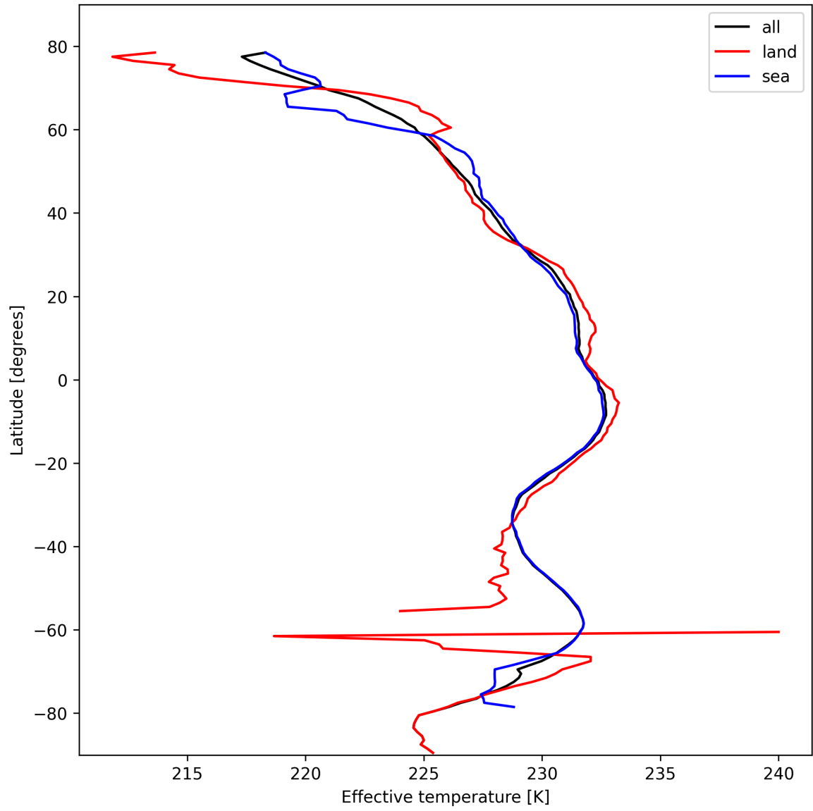
Figure 17: Zonal average of “Effective temperature” for 2025-10-20 to 2025-10-22.
