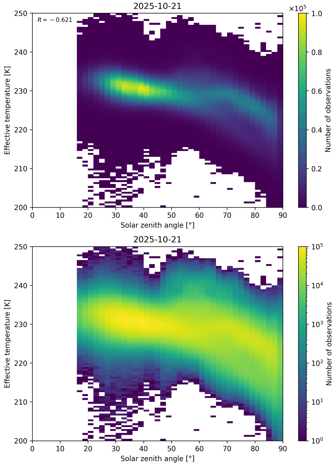
Figure 45: Scatter density plot of “Solar zenith angle” against “Effective temperature” for 2025-10-20 to 2025-10-22.
