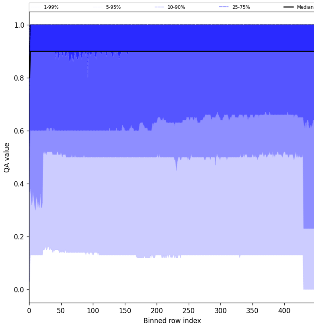
Figure 27: Along track statistics of “QA value” for 2025-10-20 to 2025-10-22
