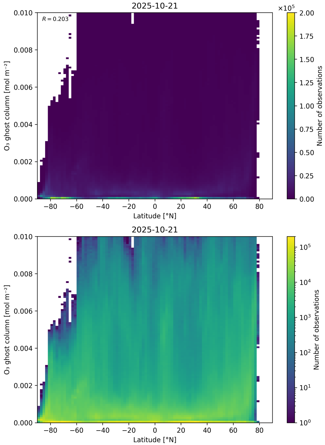
Figure 35: Scatter density plot of “Latitude” against “O 3 ghost column” for 2025-10-20 to 2025-10-22.
