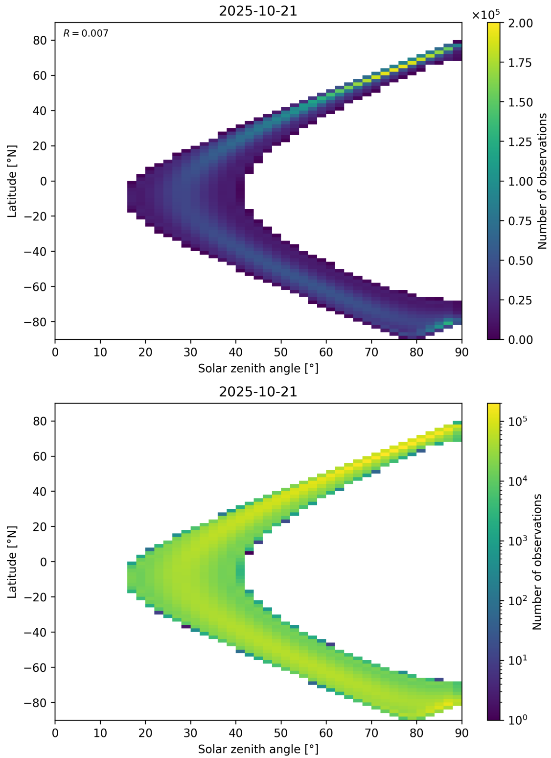
Figure 44: Scatter density plot of “Solar zenith angle” against “Latitude” for 2025-10-20 to 2025-10-22.
