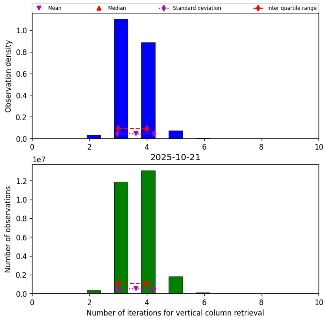
Figure 26: Histogram of “Number of iterations for vertical column retrieval” for 2025-10-20 to 2025-10-22
