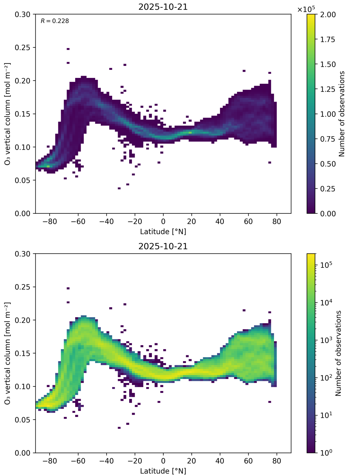
Figure 36: Scatter density plot of “Latitude” against “O 3 vertical column” for 2025-10-20 to 2025-10-22.
