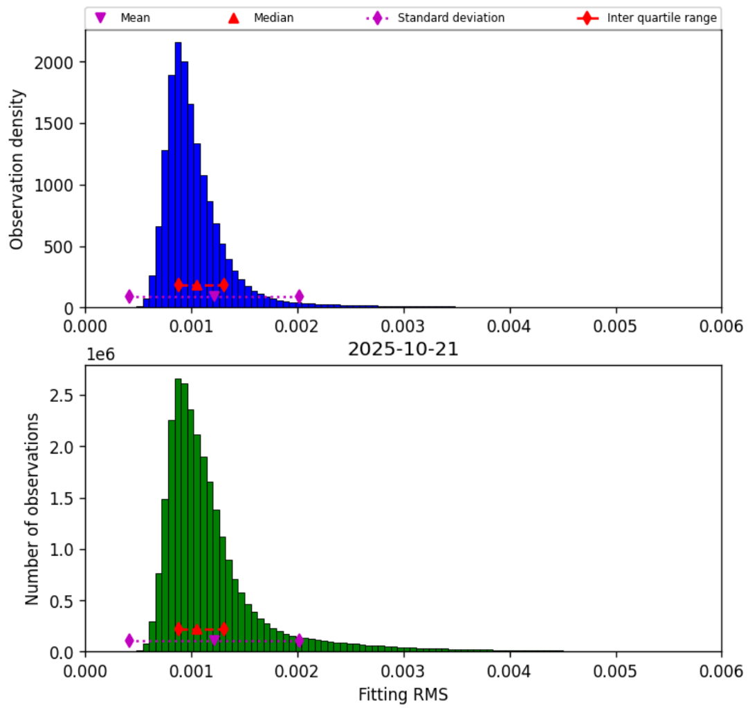
Figure 23: Histogram of “Fitting RMS” for 2025-10-20 to 2025-10-22
