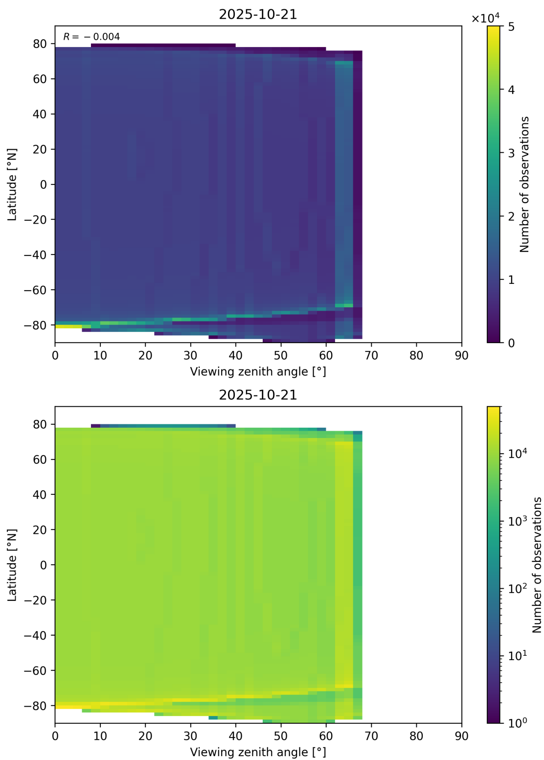
Figure 49: Scatter density plot of “Viewing zenith angle” against “Latitude” for 2025-10-20 to 2025-10-22.
