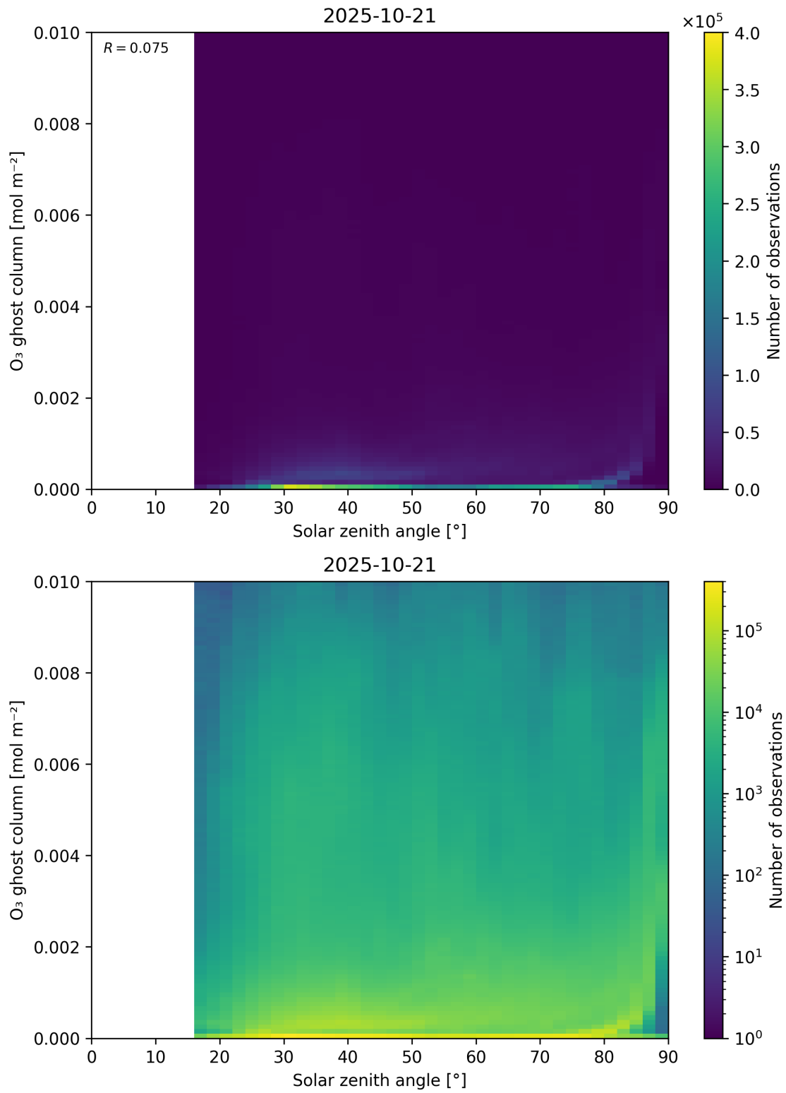
Figure 46: Scatter density plot of “Solar zenith angle” against “O 3 ghost column” for 2025-10-20 to 2025-10-22.
