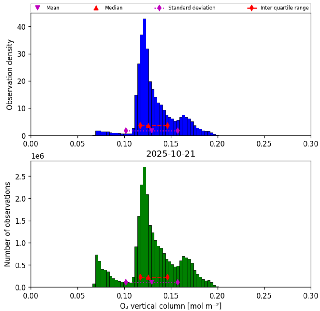
Figure 21: Histogram of “O 3 vertical column” for 2025-10-20 to 2025-10-22
