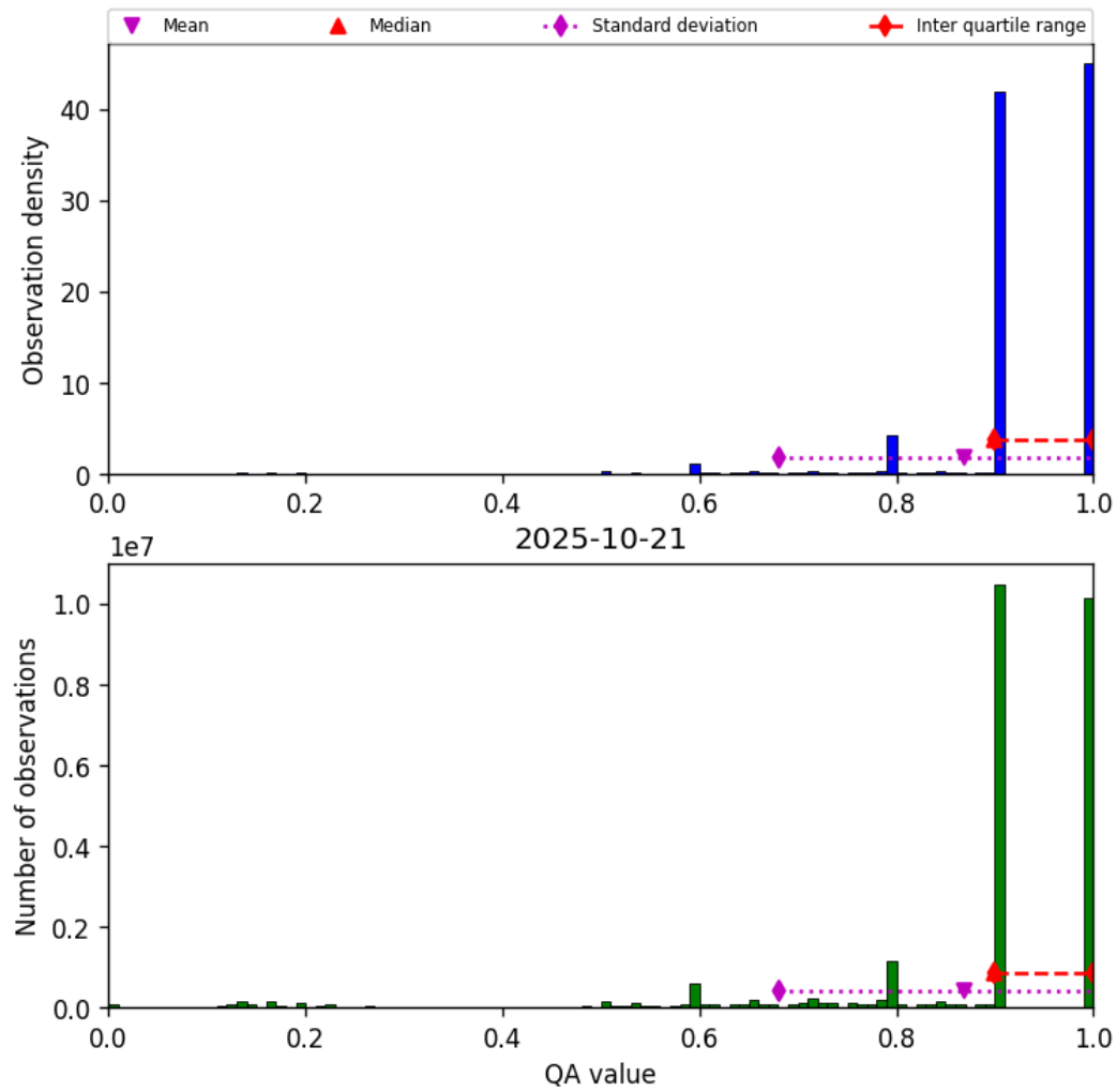
Figure 20: Histogram of “QA value” for 2025-10-20 to 2025-10-22
