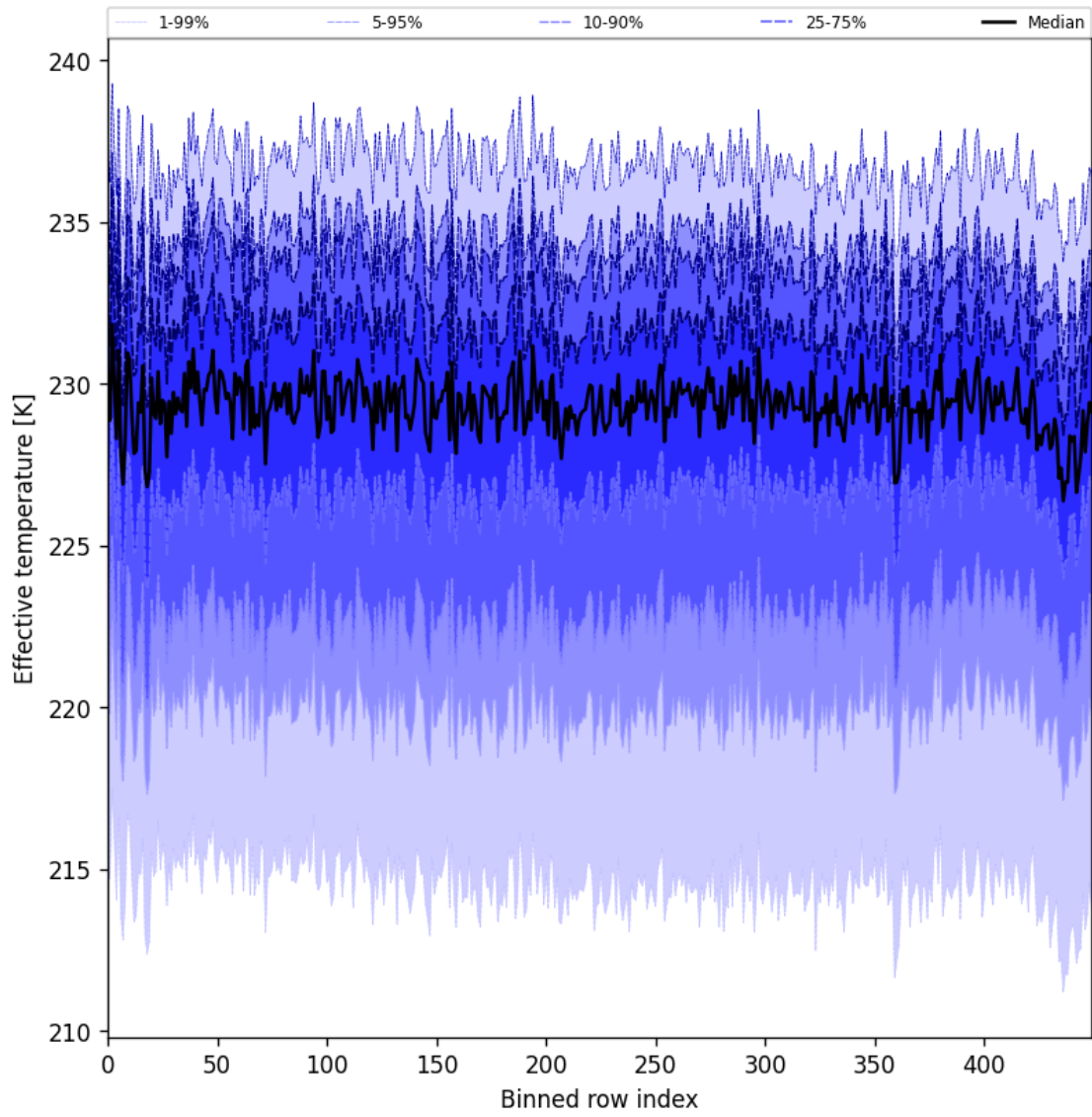
Figure 31: Along track statistics of “Effective temperature” for 2025-10-20 to 2025-10-22
