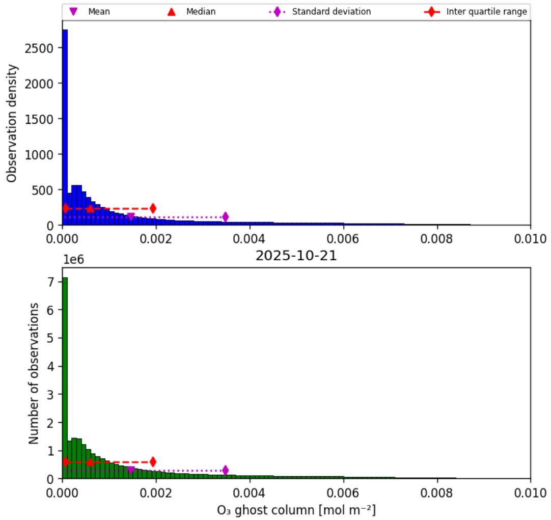
Figure 25: Histogram of “O 3 ghost column” for 2025-10-20 to 2025-10-22
