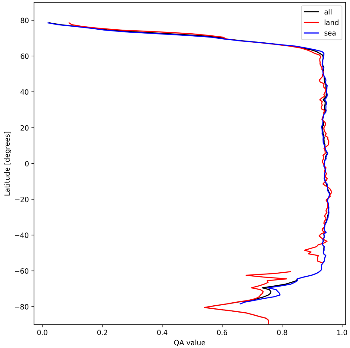
Figure 13: Zonal average of “QA value” for 2025-10-20 to 2025-10-22.
