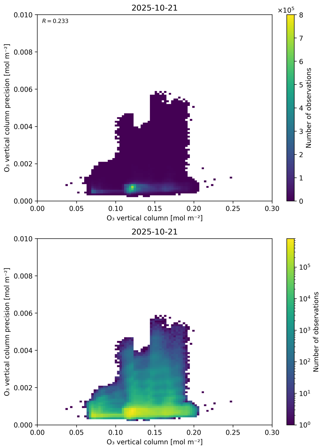
Figure 41: Scatter density plot of “O 3 vertical column” against “O 3 vertical column precision” for 2025-10-20 to 2025-10-22.
