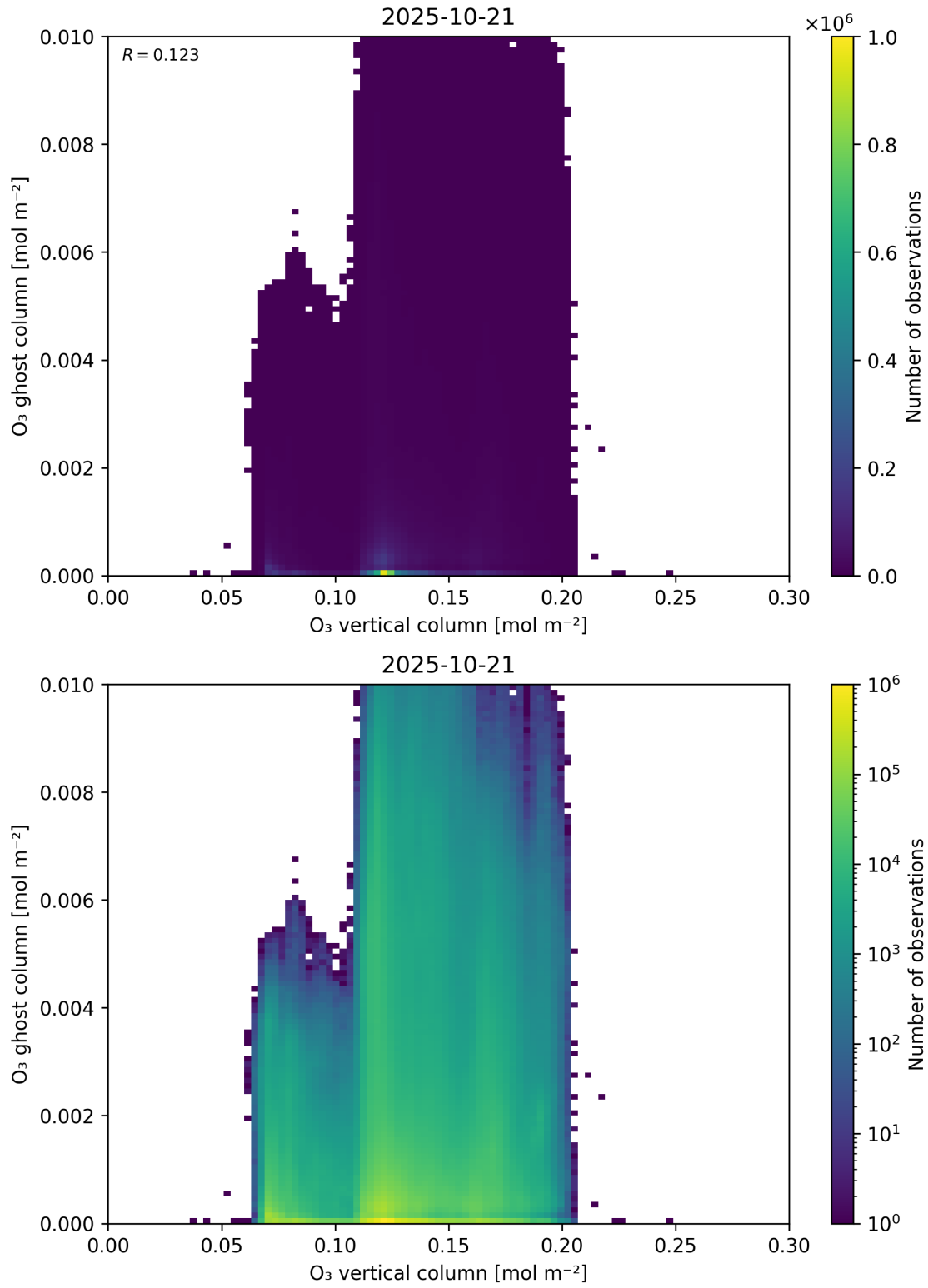
Figure 40: Scatter density plot of “O 3 vertical column” against “O 3 ghost column” for 2025-10-20 to 2025-10-22.
