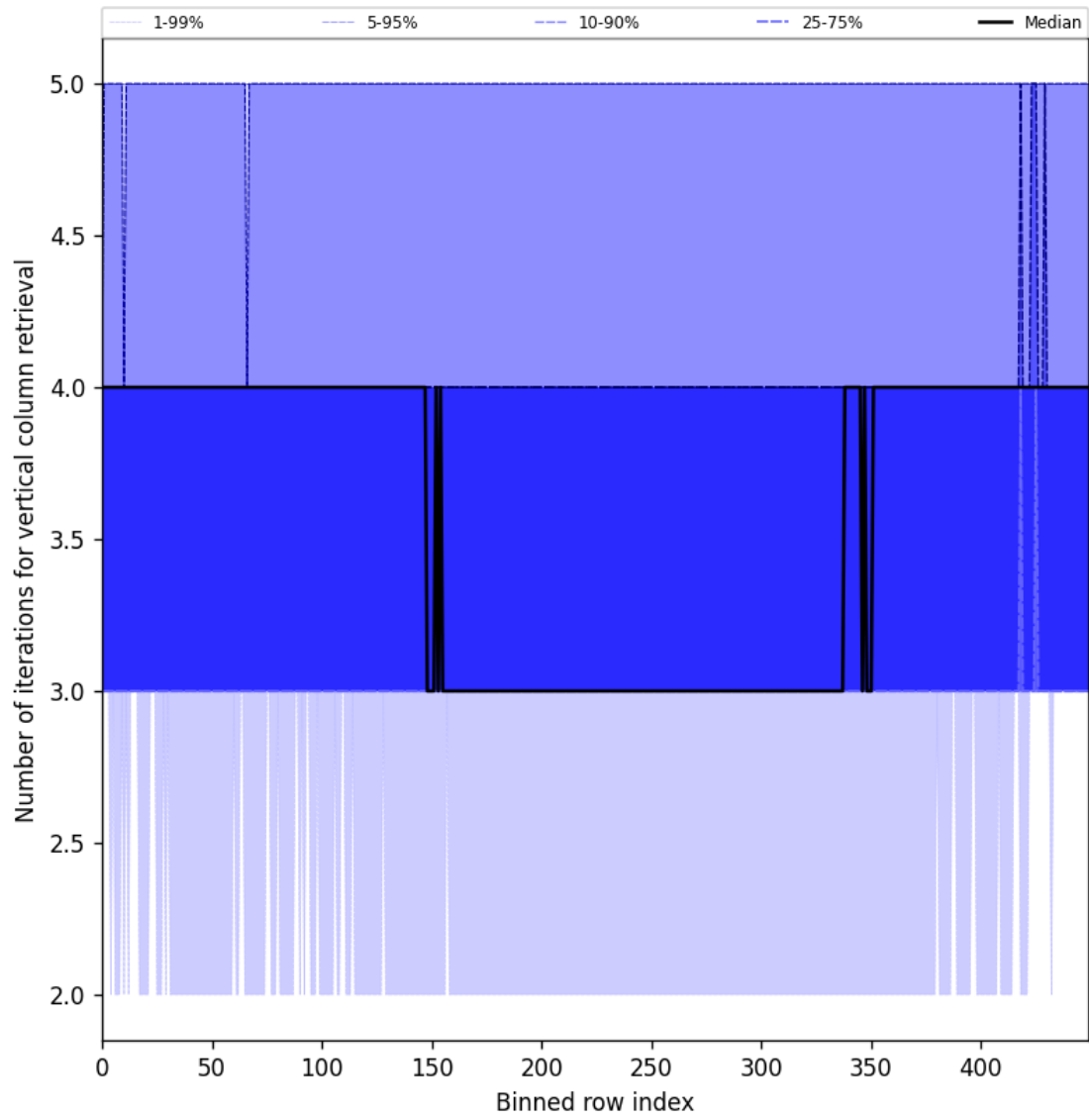
Figure 33: Along track statistics of “Number of iterations for vertical column retrieval” for 2025-10-20 to 2025-10-22
