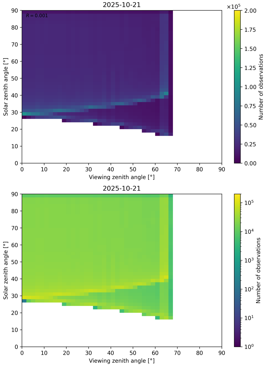
Figure 54: Scatter density plot of “Viewing zenith angle” against “Solar zenith angle” for 2025-10-20 to 2025-10-22.
