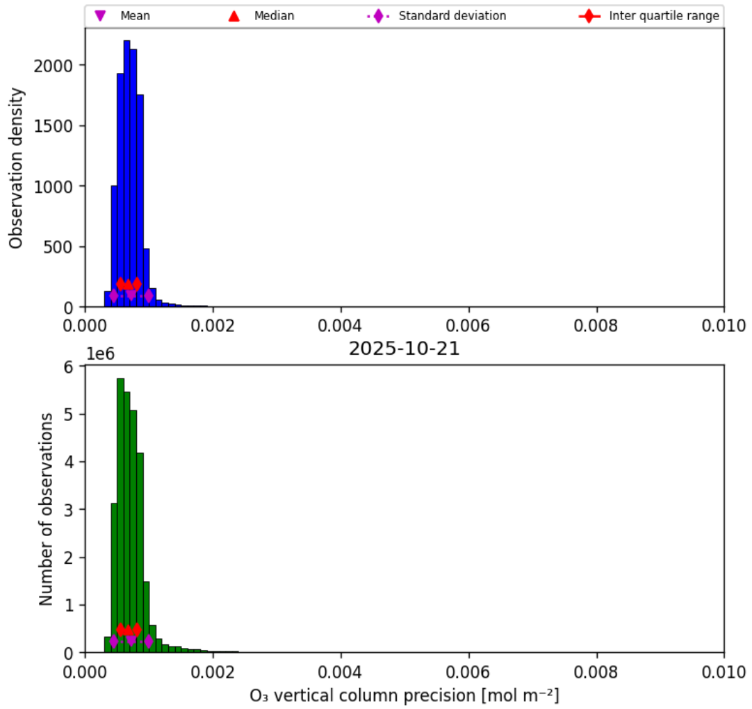
Figure 22: Histogram of “O 3 vertical column precision” for 2025-10-20 to 2025-10-22
