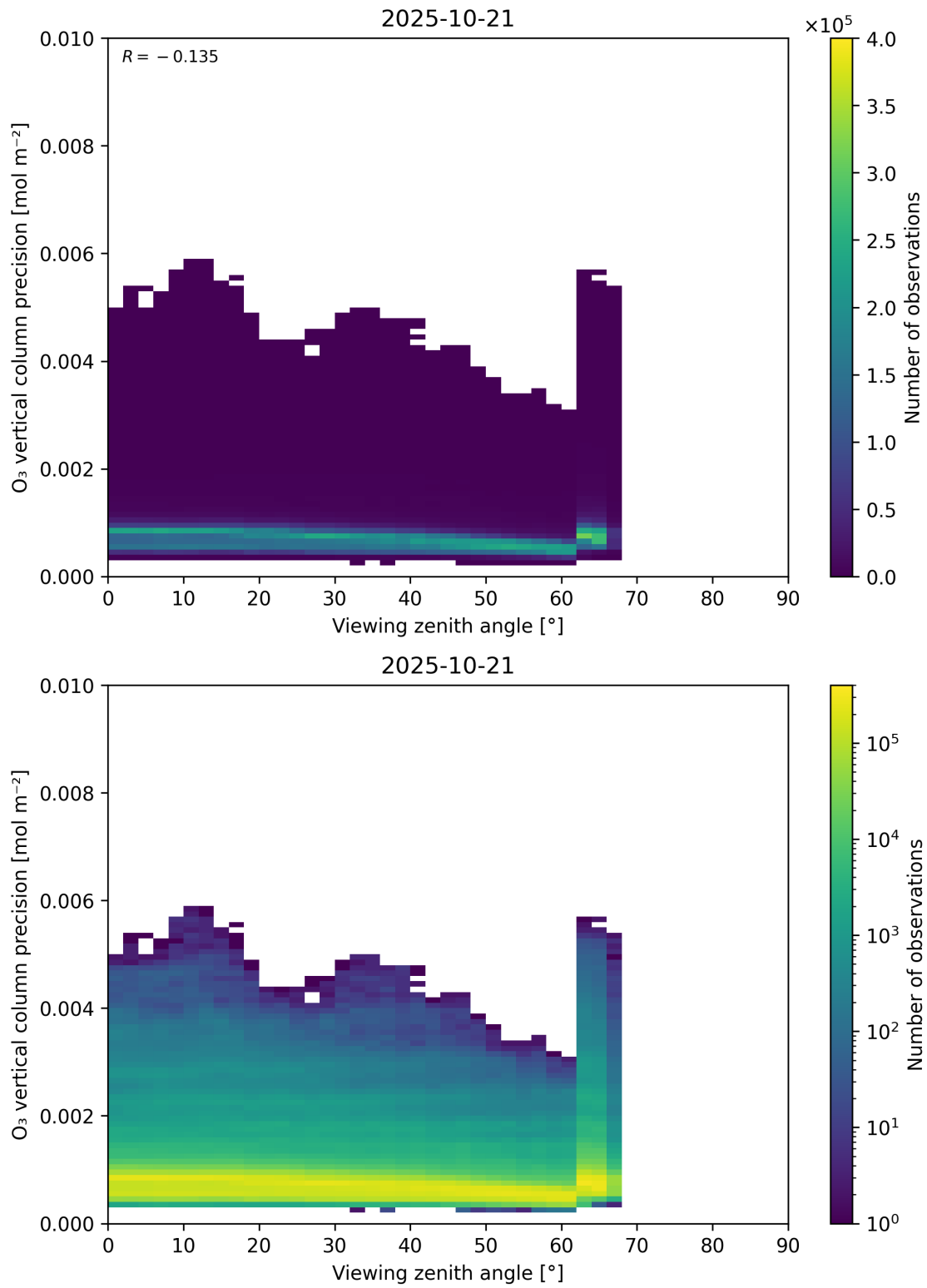
Figure 53: Scatter density plot of “Viewing zenith angle” against “O 3 vertical column precision” for 2025-10-20 to 2025-10-22.
