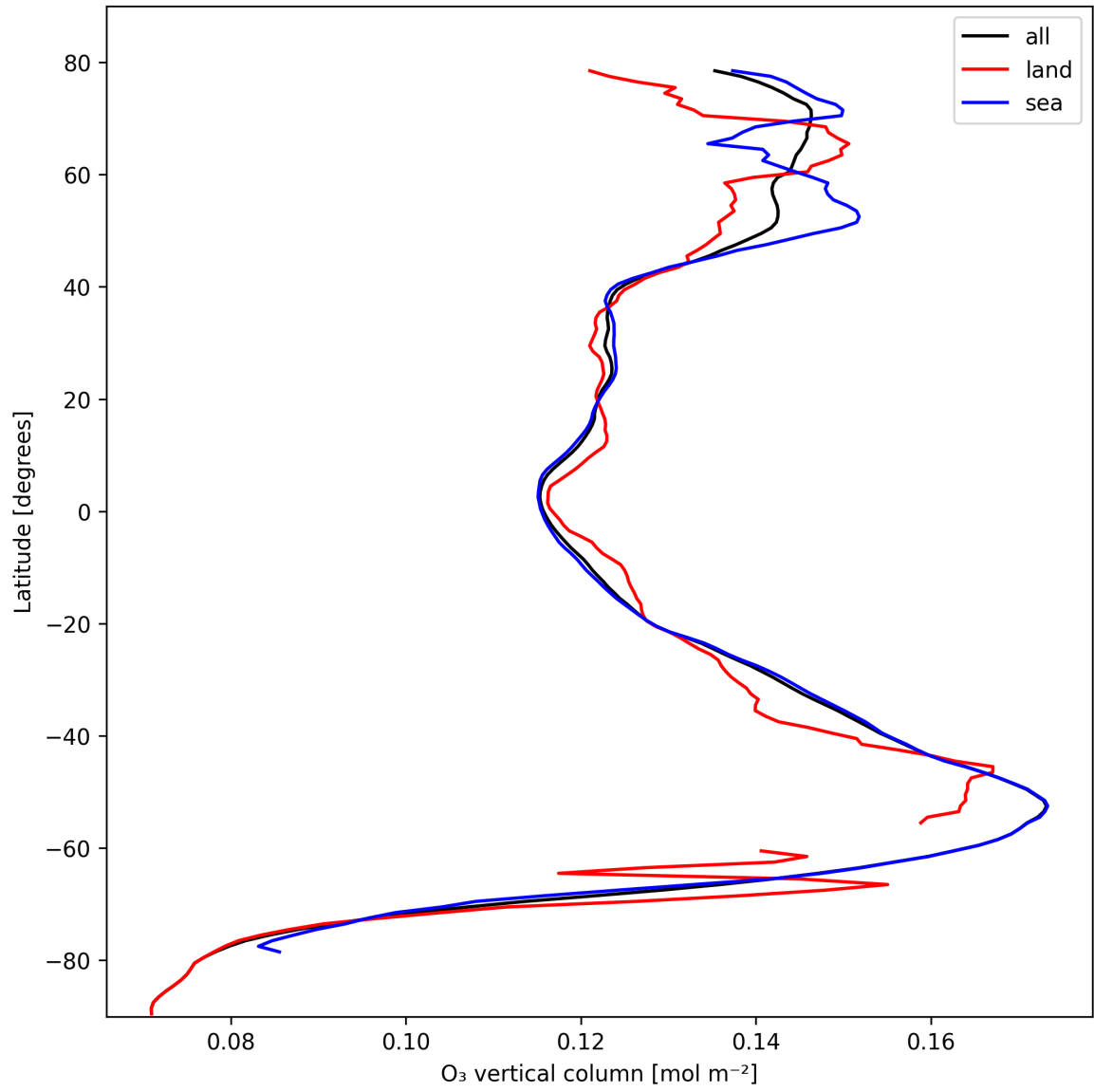
Figure 14: Zonal average of “O 3 vertical column” for 2025-10-20 to 2025-10-22.
