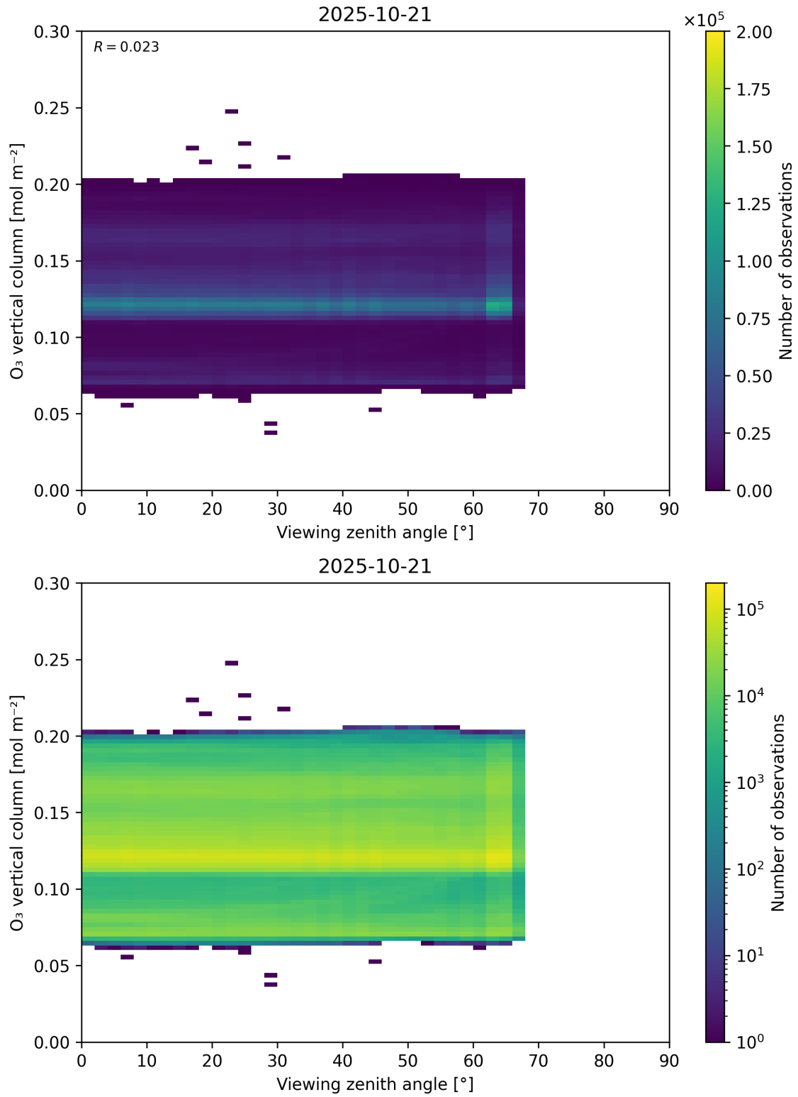
Figure 52: Scatter density plot of “Viewing zenith angle” against “O 3 vertical column” for 2025-10-20 to 2025-10-22.
