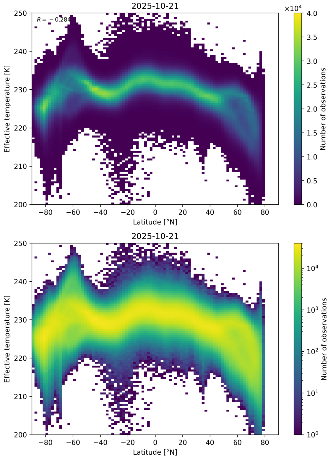
Figure 34: Scatter density plot of “Latitude” against “Effective temperature” for 2025-10-20 to 2025-10-22.
