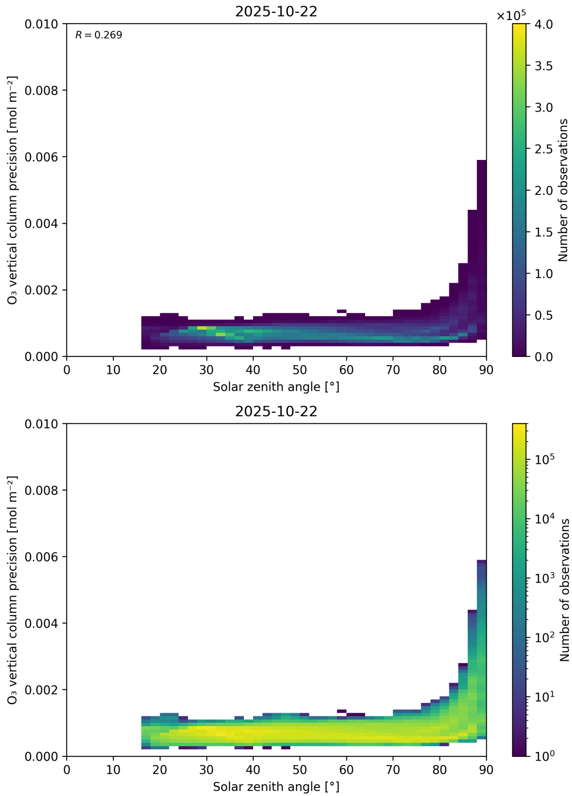
Figure 48: Scatter density plot of “Solar zenith angle” against “O 3 vertical column precision” for 2025-10-22 to 2025-10-23.
