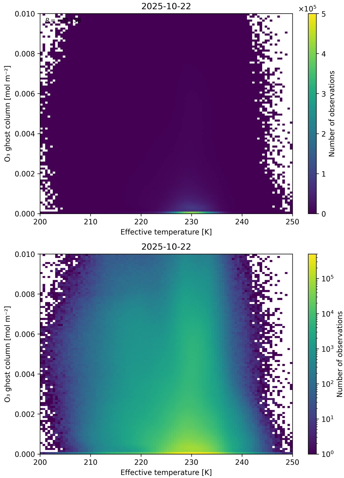
Figure 38: Scatter density plot of “Effective temperature” against “O 3 ghost column” for 2025-10-22 to 2025-10-23.
