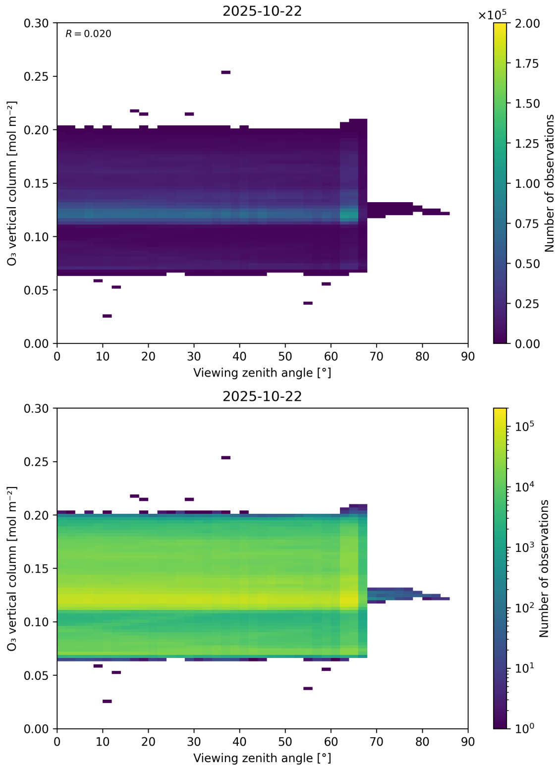
Figure 52: Scatter density plot of “Viewing zenith angle” against “O 3 vertical column” for 2025-10-22 to 2025-10-23.
