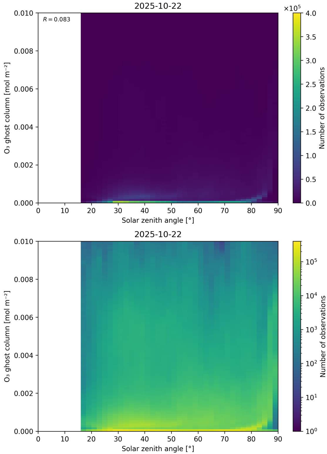
Figure 46: Scatter density plot of “Solar zenith angle” against “O 3 ghost column” for 2025-10-22 to 2025-10-23.
