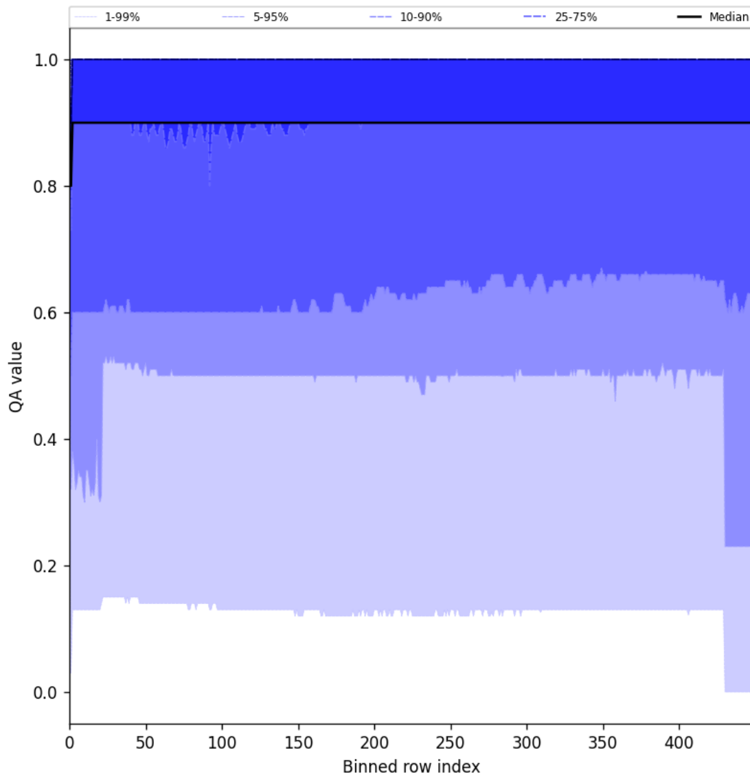
Figure 27: Along track statistics of “QA value” for 2025-10-22 to 2025-10-23
