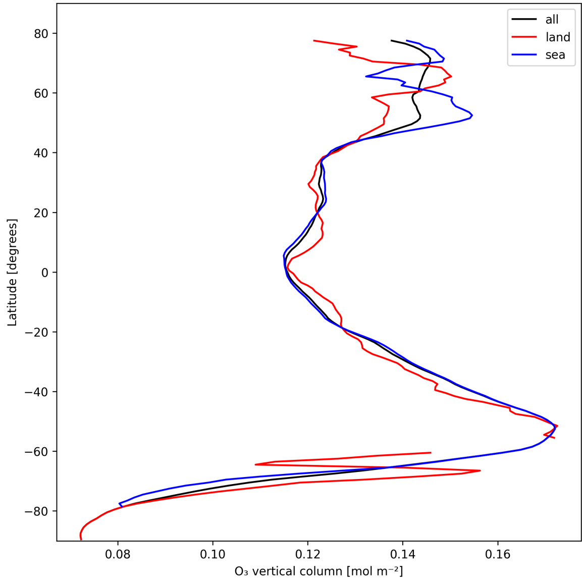
Figure 14: Zonal average of “O 3 vertical column” for 2025-10-22 to 2025-10-23.
