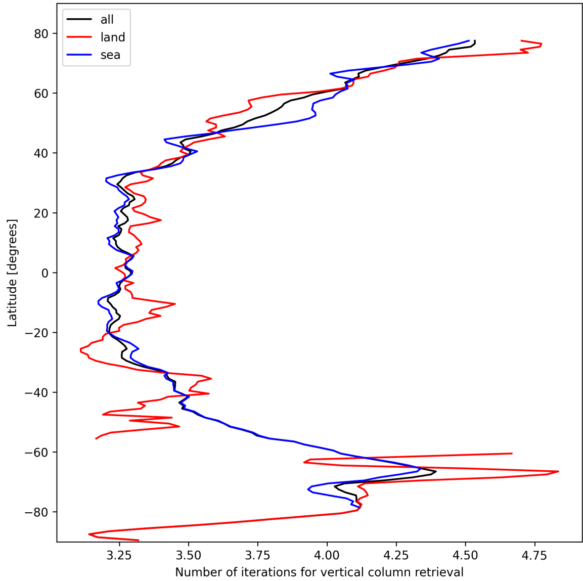
Figure 19: Zonal average of “Number of iterations for vertical column retrieval” for 2025-10-22 to 2025-10-23.
