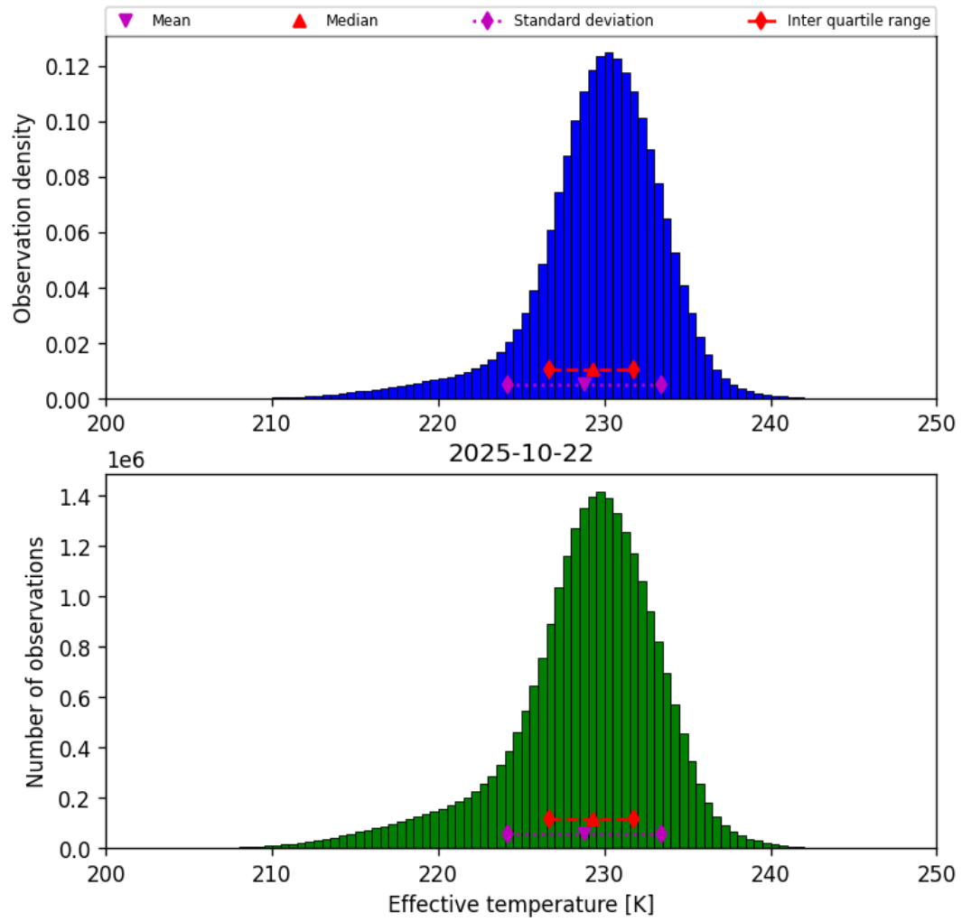
Figure 24: Histogram of “Effective temperature” for 2025-10-22 to 2025-10-23
