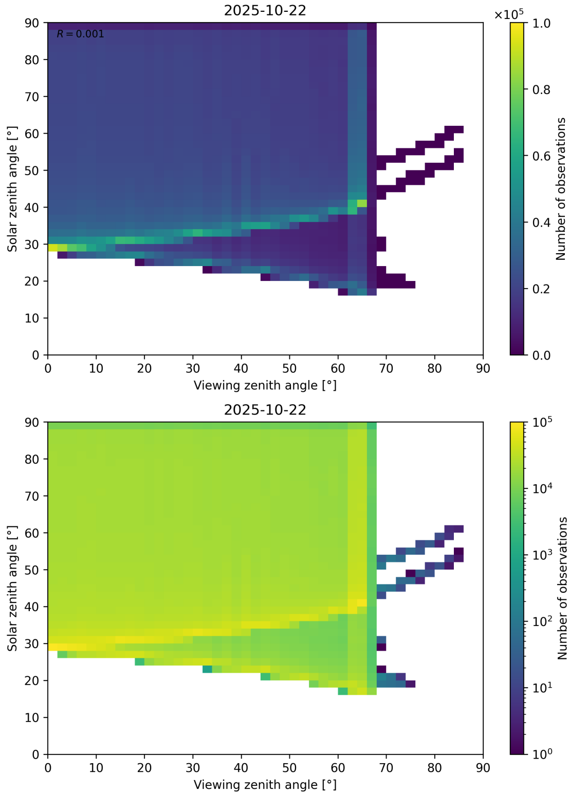
Figure 54: Scatter density plot of “Viewing zenith angle” against “Solar zenith angle” for 2025-10-22 to 2025-10-23.
