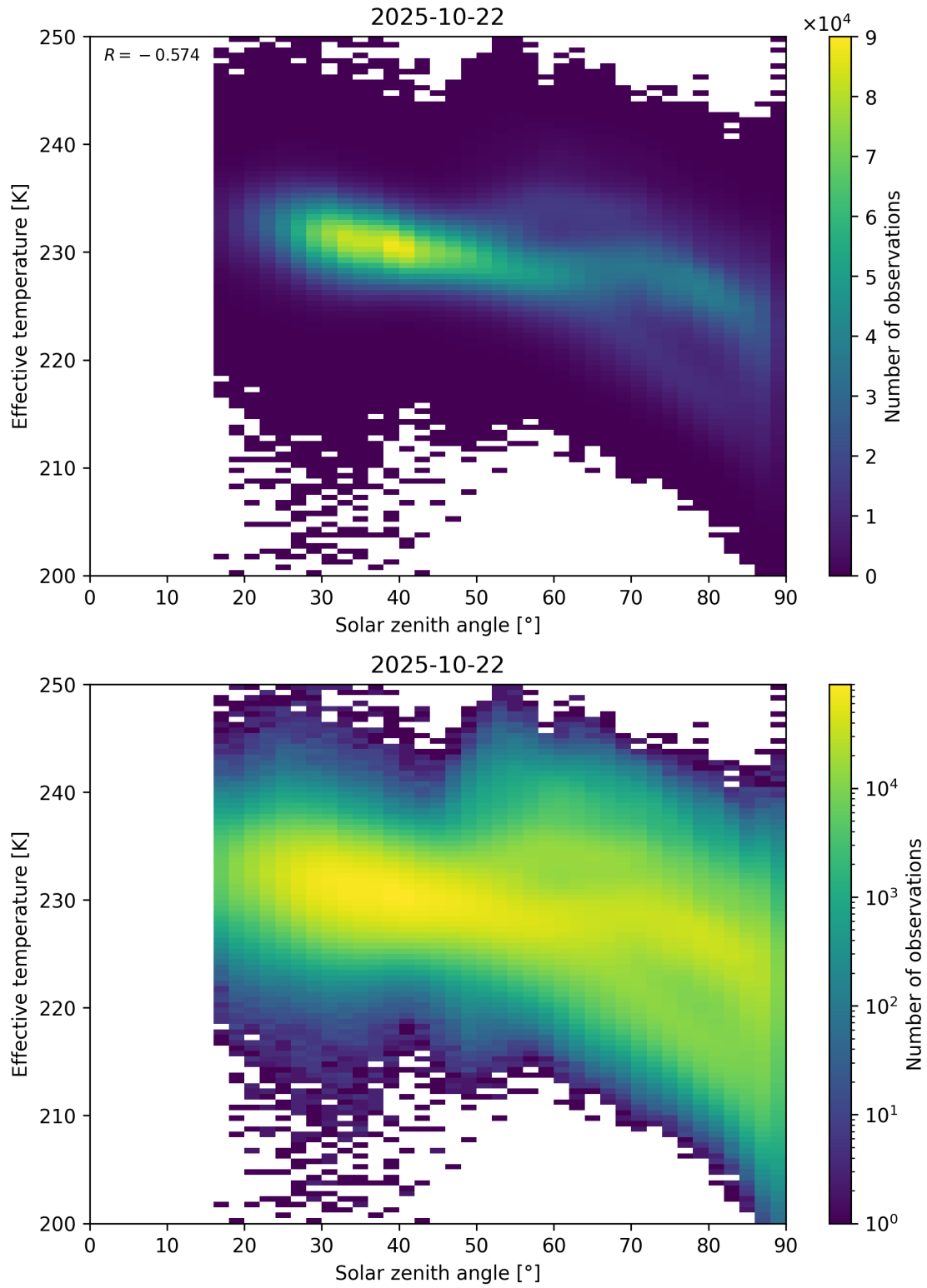
Figure 45: Scatter density plot of “Solar zenith angle” against “Effective temperature” for 2025-10-22 to 2025-10-23.
