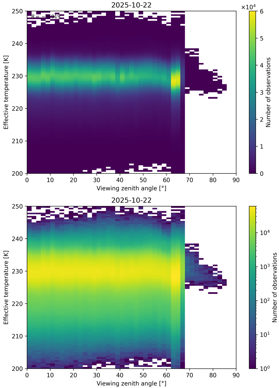
Figure 50: Scatter density plot of “Viewing zenith angle” against “Effective temperature” for 2025-10-22 to 2025-10-23.
