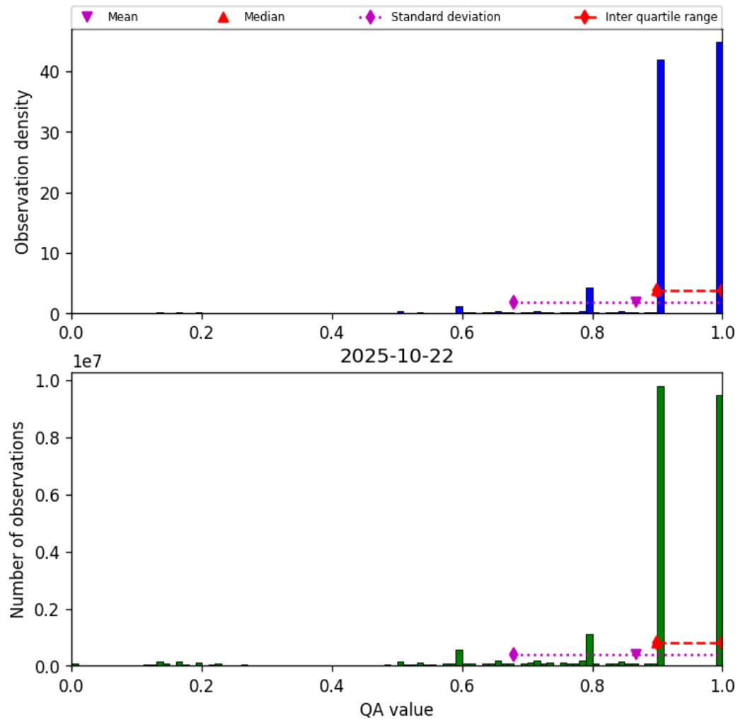
Figure 20: Histogram of “QA value” for 2025-10-22 to 2025-10-23
