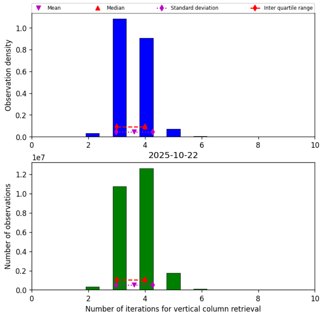
Figure 26: Histogram of “Number of iterations for vertical column retrieval” for 2025-10-22 to 2025-10-23
