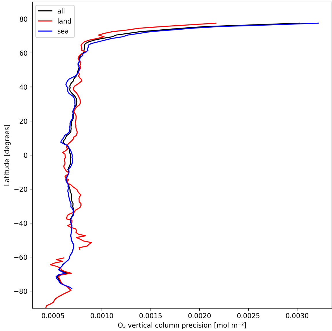
Figure 15: Zonal average of “O 3 vertical column precision” for 2025-10-22 to 2025-10-23.
