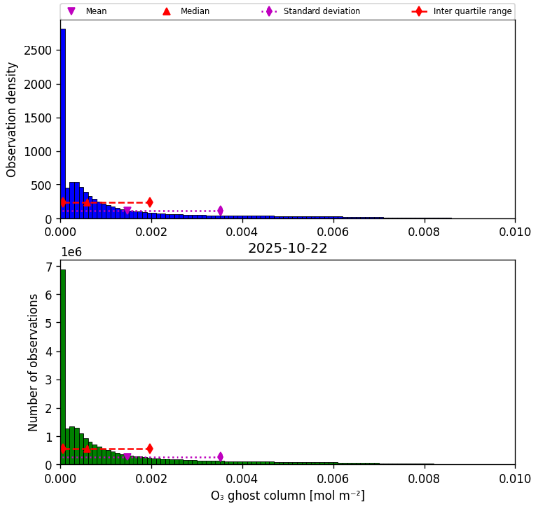
Figure 25: Histogram of “O 3 ghost column” for 2025-10-22 to 2025-10-23
