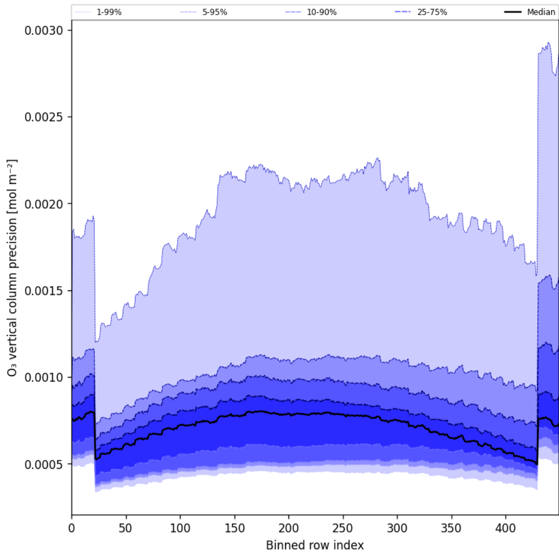
Figure 29: Along track statistics of “O 3 vertical column precision” for 2025-10-22 to 2025-10-23
