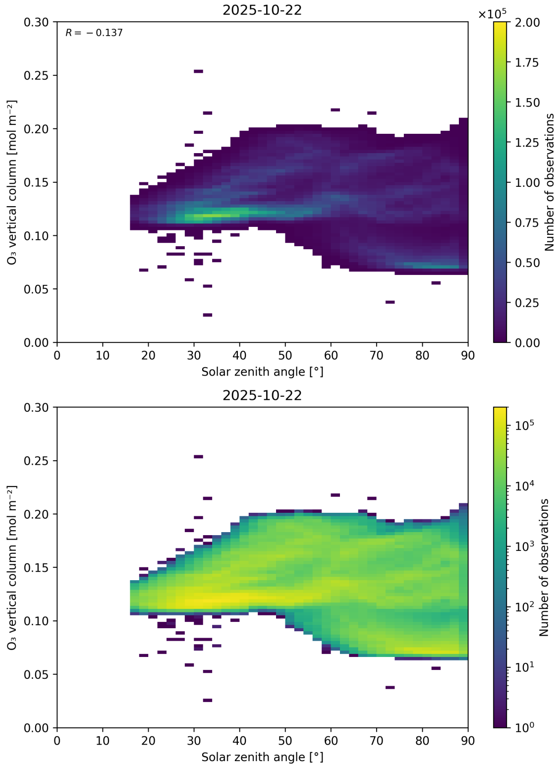
Figure 47: Scatter density plot of “Solar zenith angle” against “O 3 vertical column” for 2025-10-22 to 2025-10-23.
