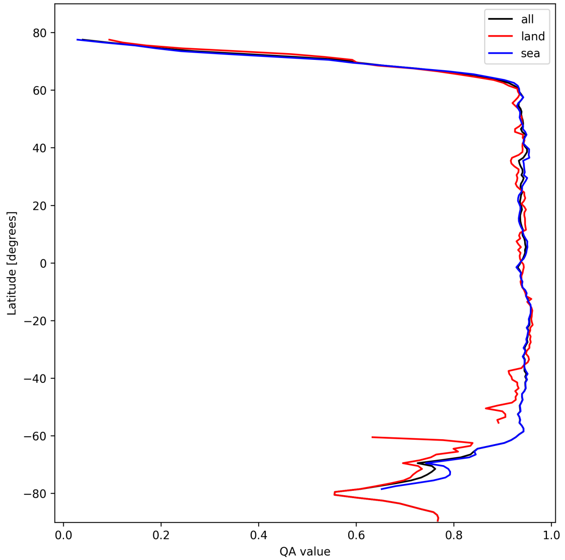
Figure 13: Zonal average of “QA value” for 2025-10-22 to 2025-10-23.
