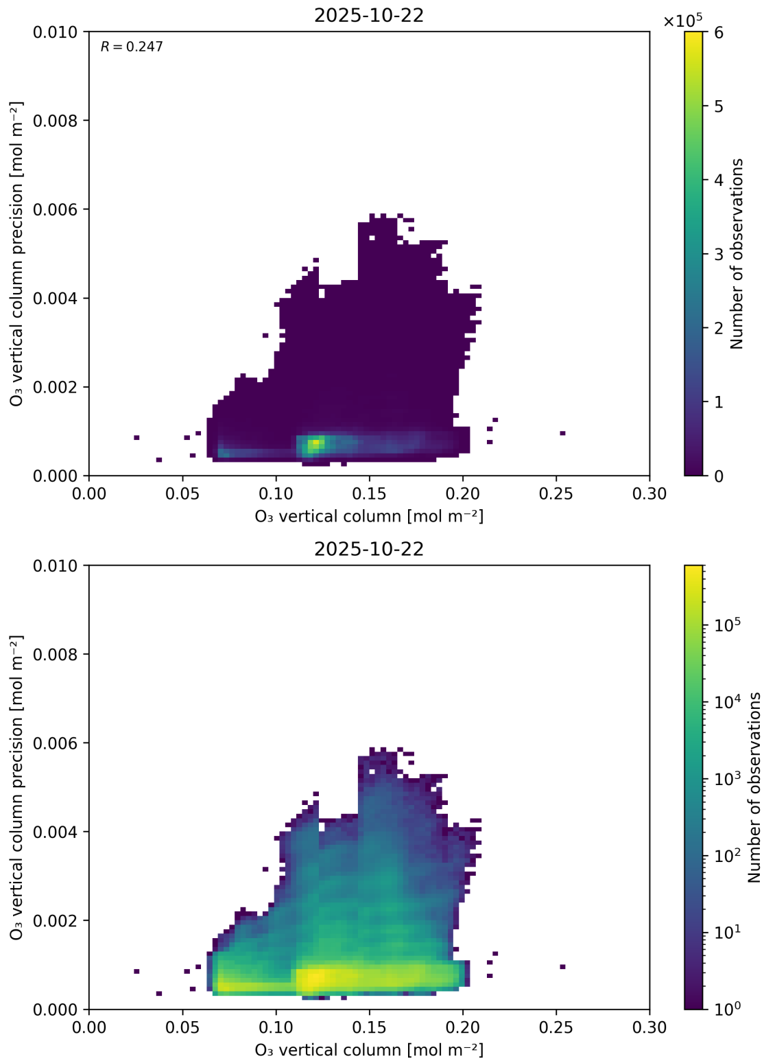
Figure 41: Scatter density plot of “O 3 vertical column” against “O 3 vertical column precision” for 2025-10-22 to 2025-10-23.
