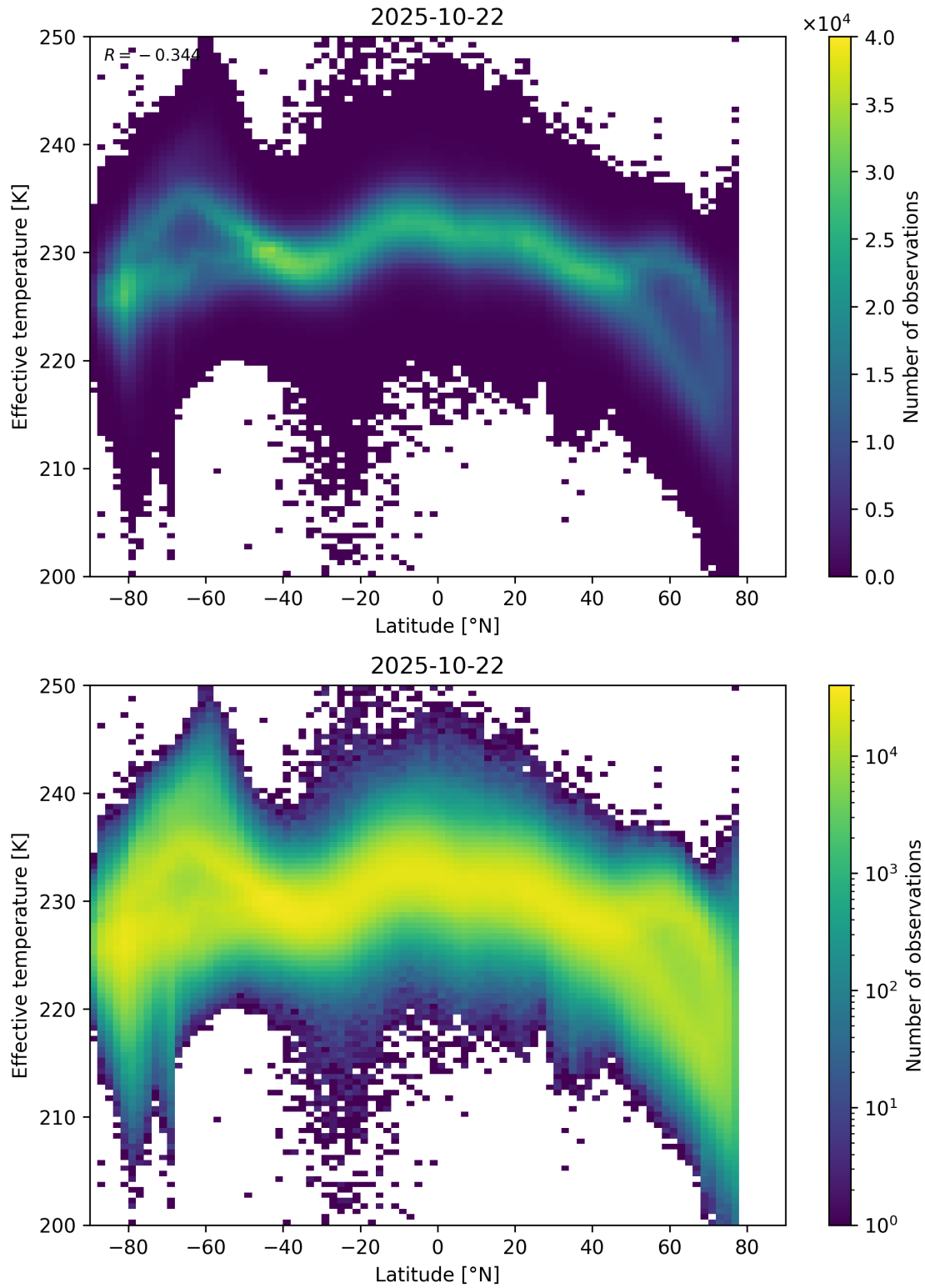
Figure 34: Scatter density plot of “Latitude” against “Effective temperature” for 2025-10-22 to 2025-10-23.
