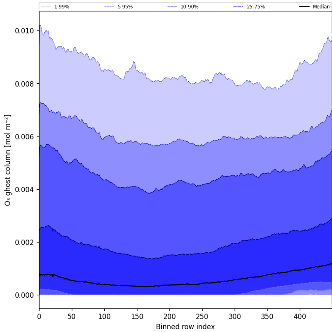
Figure 32: Along track statistics of “O 3 ghost column” for 2025-10-22 to 2025-10-23
