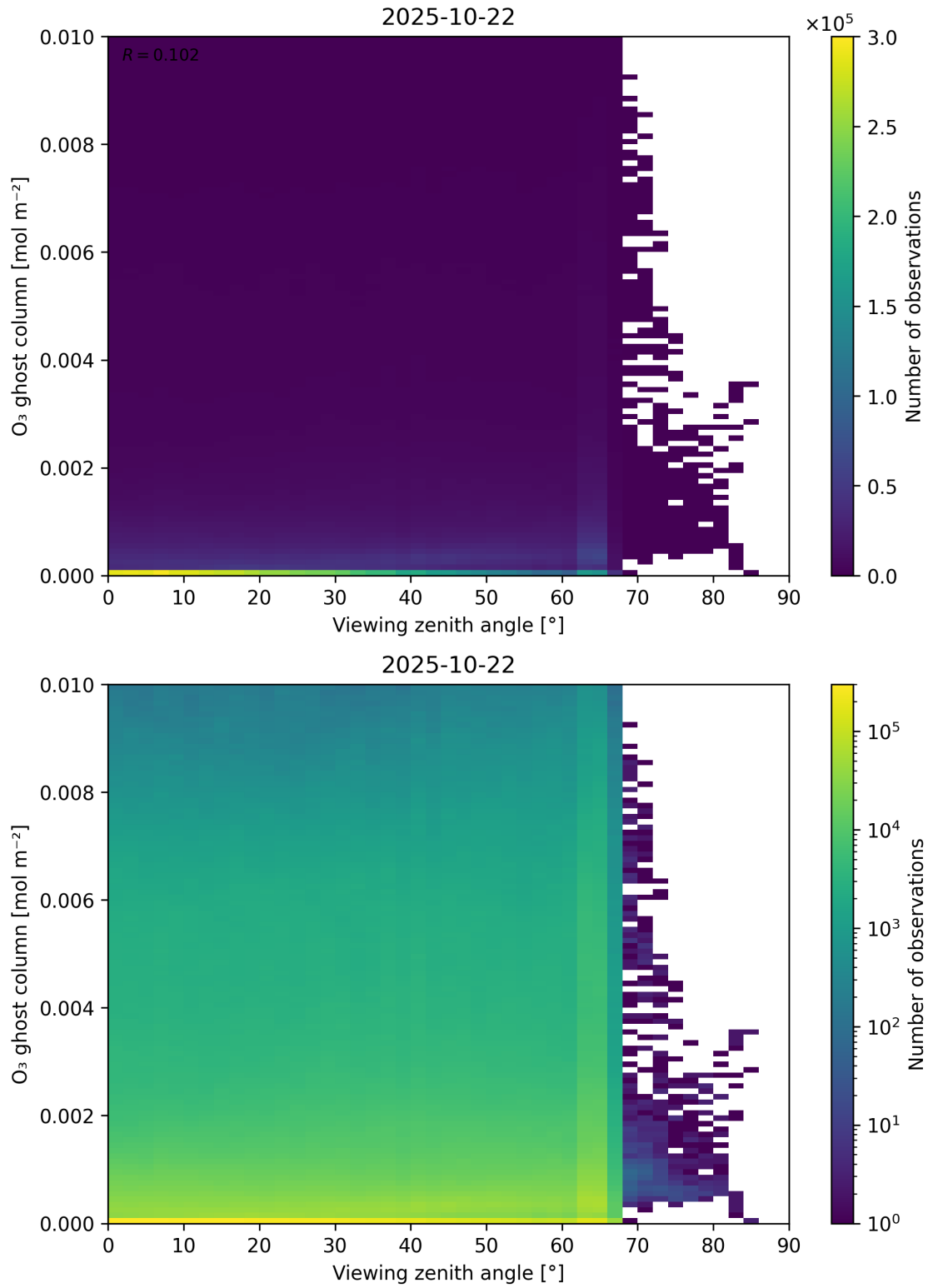
Figure 51: Scatter density plot of “Viewing zenith angle” against “O 3 ghost column” for 2025-10-22 to 2025-10-23.
