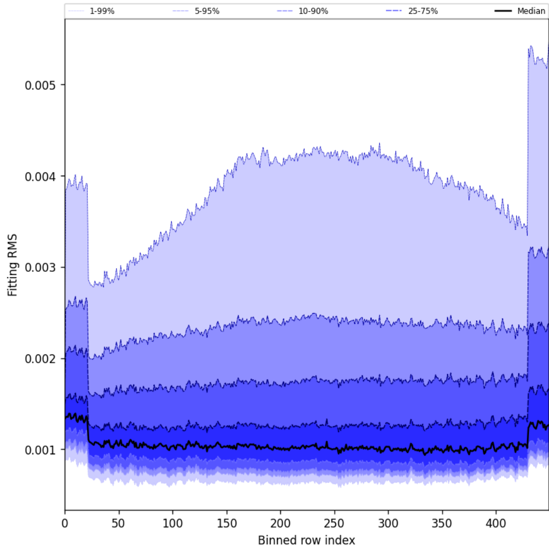
Figure 30: Along track statistics of “Fitting RMS” for 2025-10-22 to 2025-10-23
