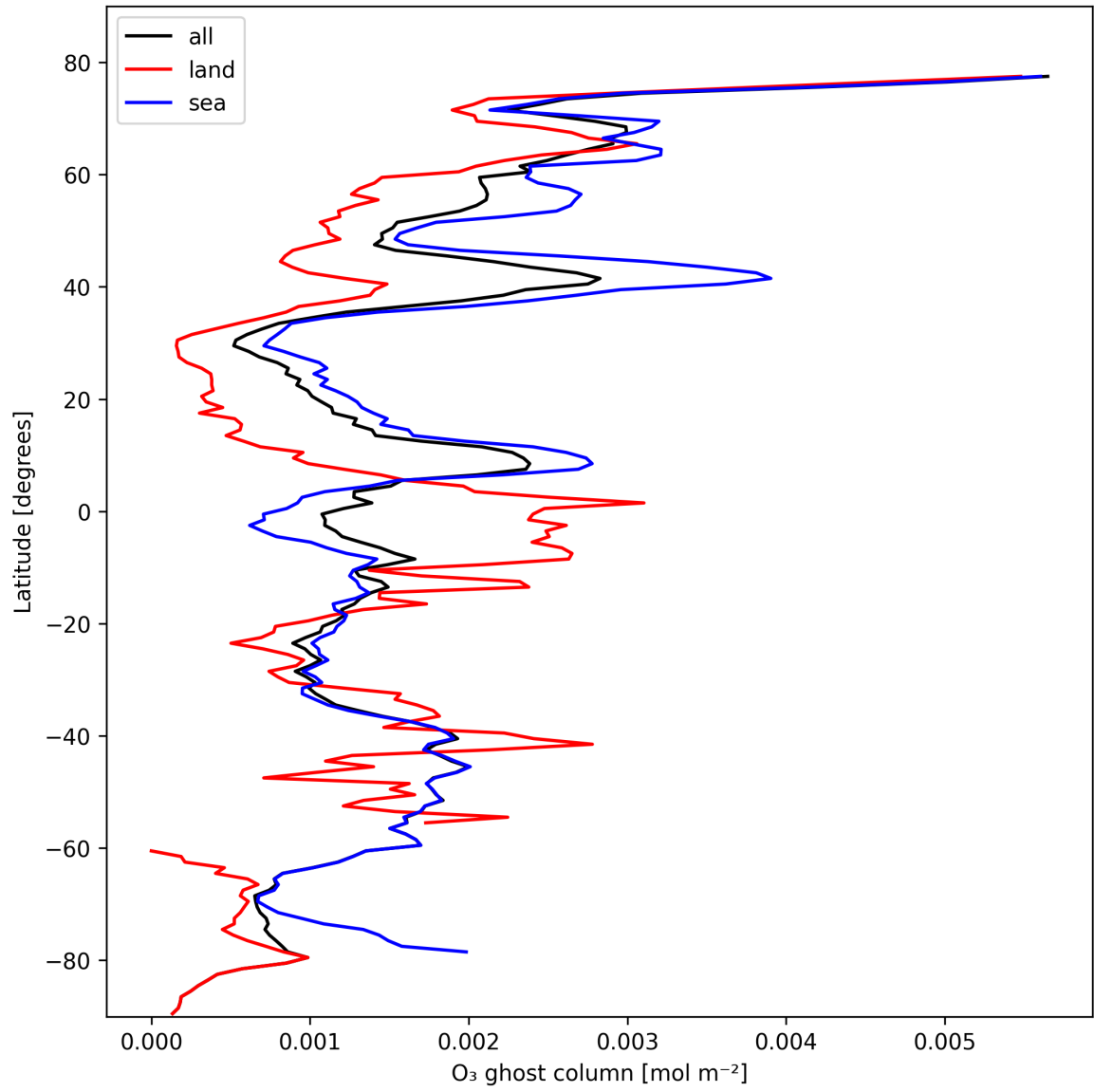
Figure 18: Zonal average of “O 3 ghost column” for 2025-10-22 to 2025-10-23.
