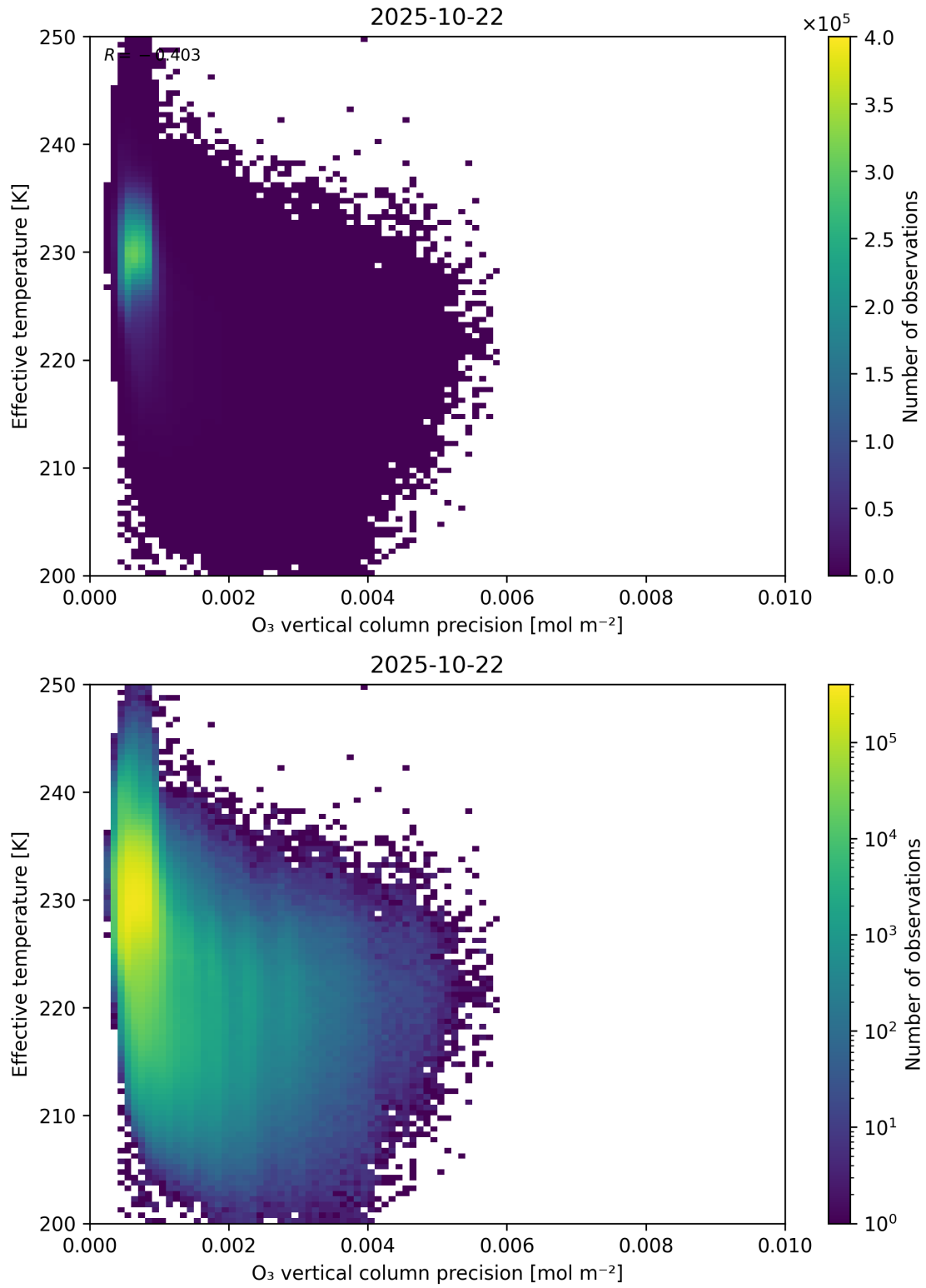
Figure 42: Scatter density plot of “O 3 vertical column precision” against “Effective temperature” for 2025-10-22 to 2025-10-23.
