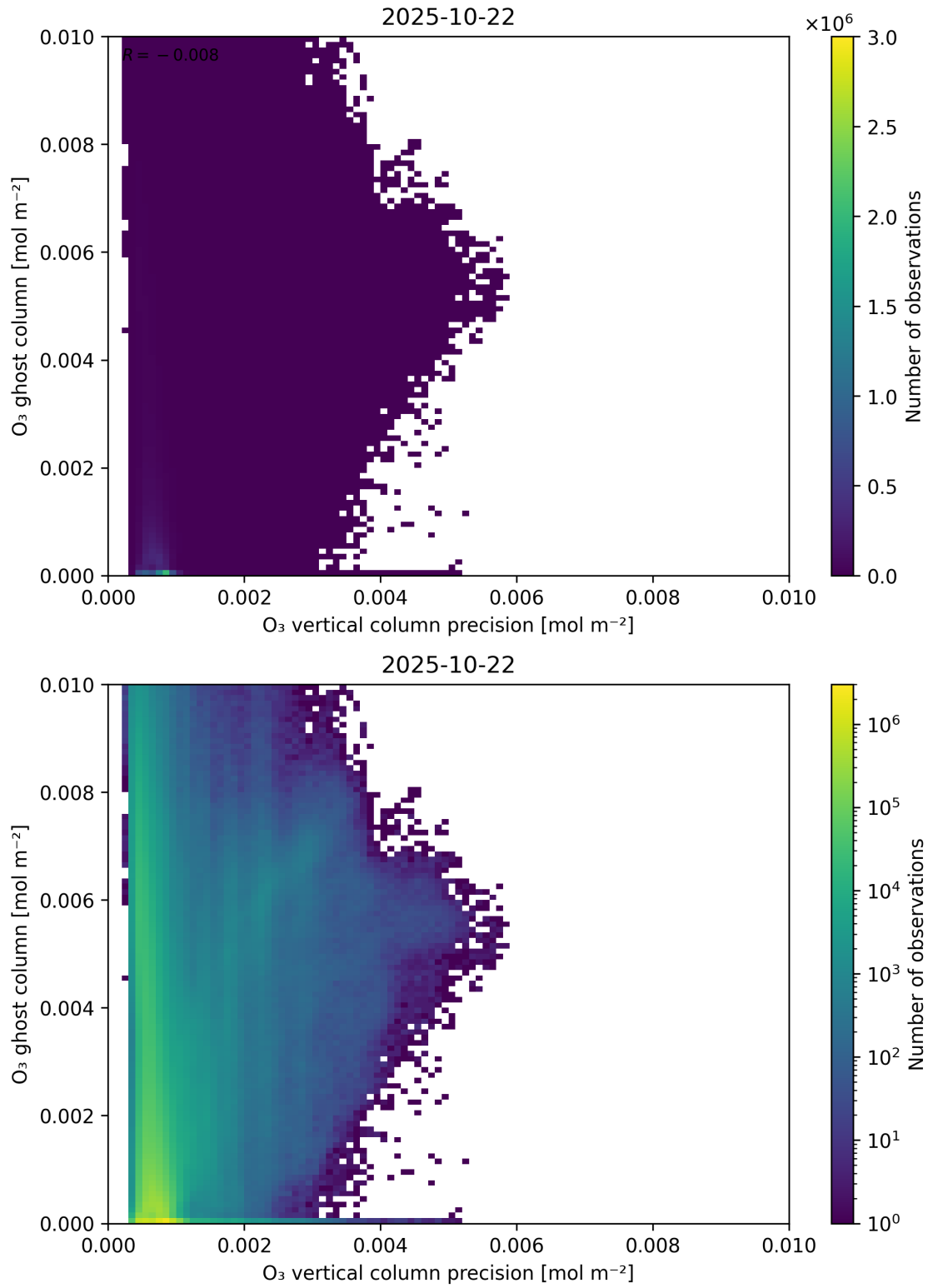
Figure 43: Scatter density plot of “ O_3 vertical column precision” against “ O_3 ghost column” for 2025-10-22 to 2025-10-23.
