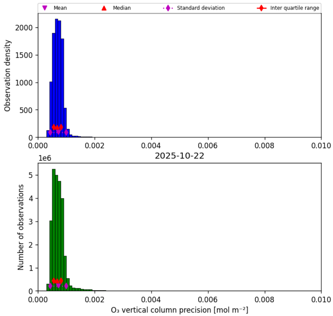
Figure 22: Histogram of “O 3 vertical column precision” for 2025-10-22 to 2025-10-23
