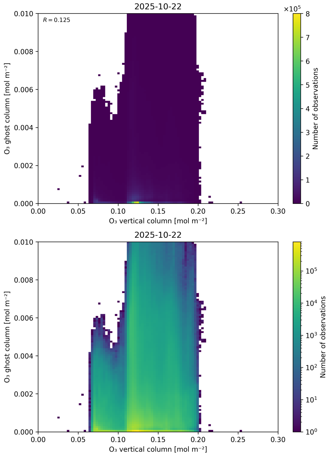
Figure 40: Scatter density plot of “O 3 vertical column” against “O 3 ghost column” for 2025-10-22 to 2025-10-23.
