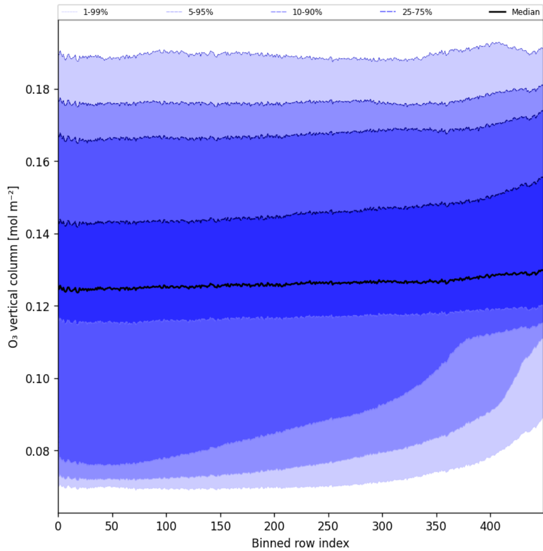
Figure 28: Along track statistics of “O 3 vertical column” for 2025-10-22 to 2025-10-23
