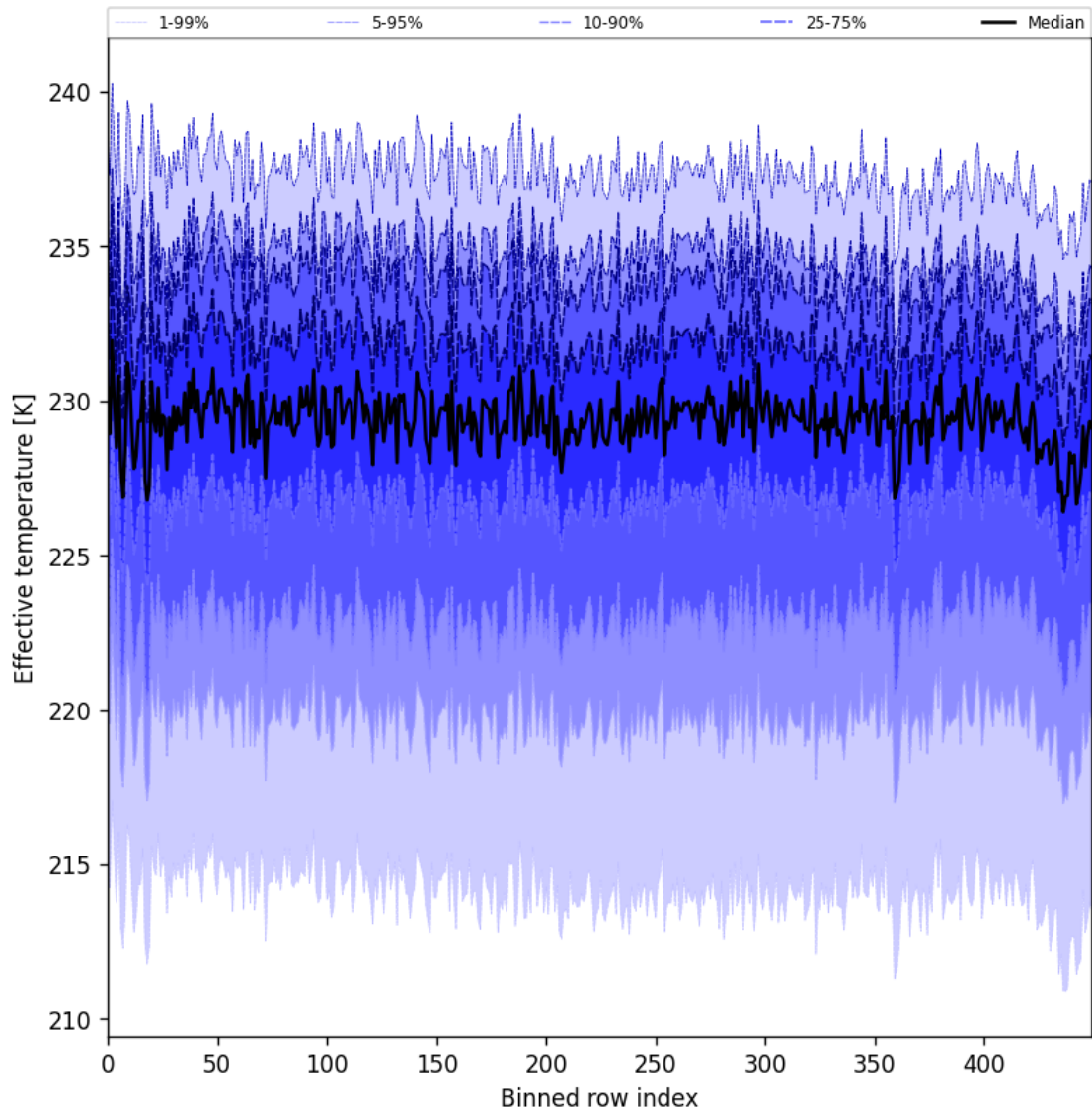
Figure 31: Along track statistics of “Effective temperature” for 2025-10-22 to 2025-10-23
