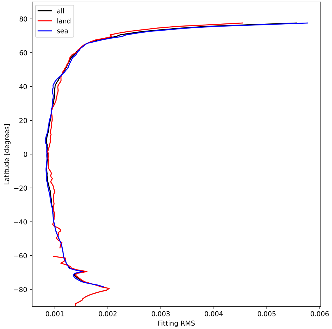
Figure 16: Zonal average of “Fitting RMS” for 2025-10-22 to 2025-10-23.
