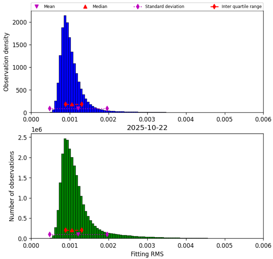
Figure 23: Histogram of “Fitting RMS” for 2025-10-22 to 2025-10-23
