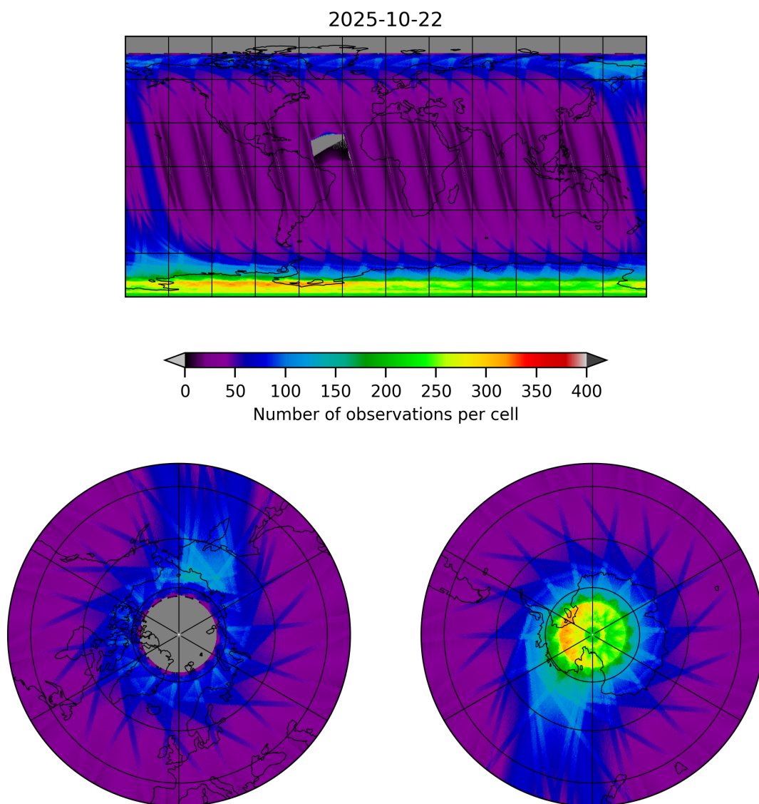
Figure 12: Map of the number of observations for 2025-10-22 to 2025-10-23
