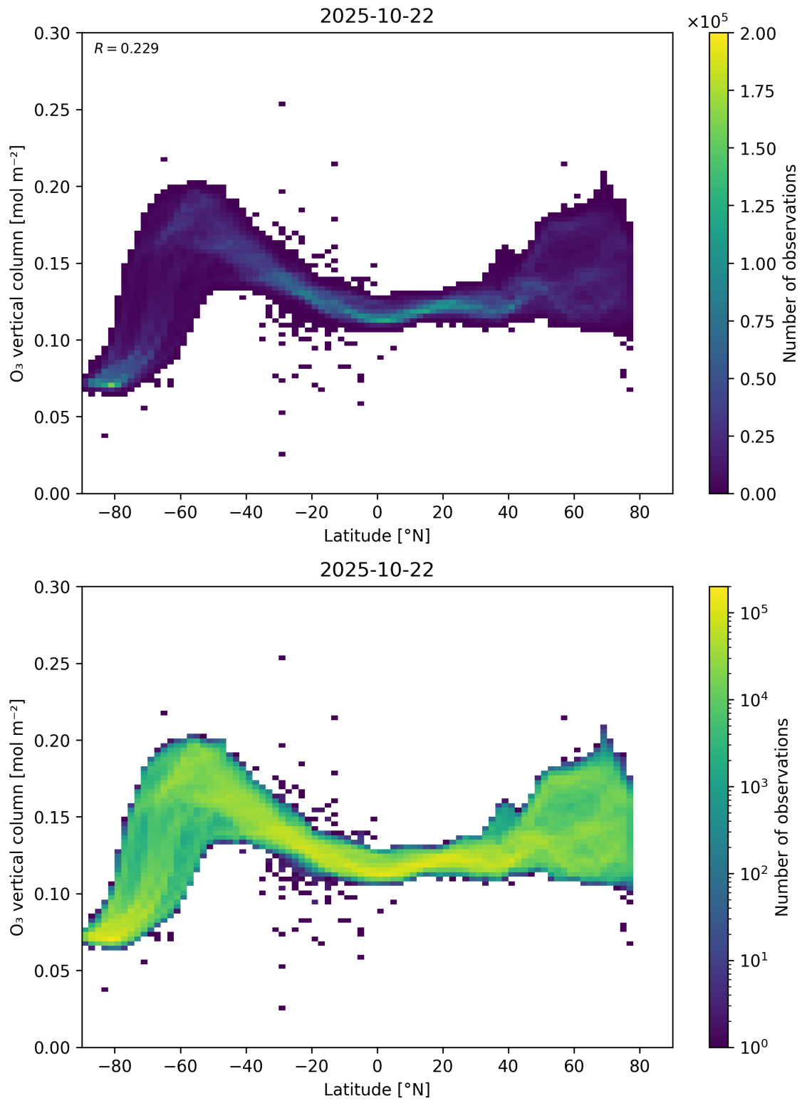
Figure 36: Scatter density plot of “Latitude” against “O 3 vertical column” for 2025-10-22 to 2025-10-23.
