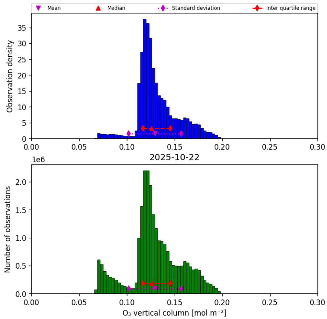
Figure 21: Histogram of “O 3 vertical column” for 2025-10-22 to 2025-10-23
