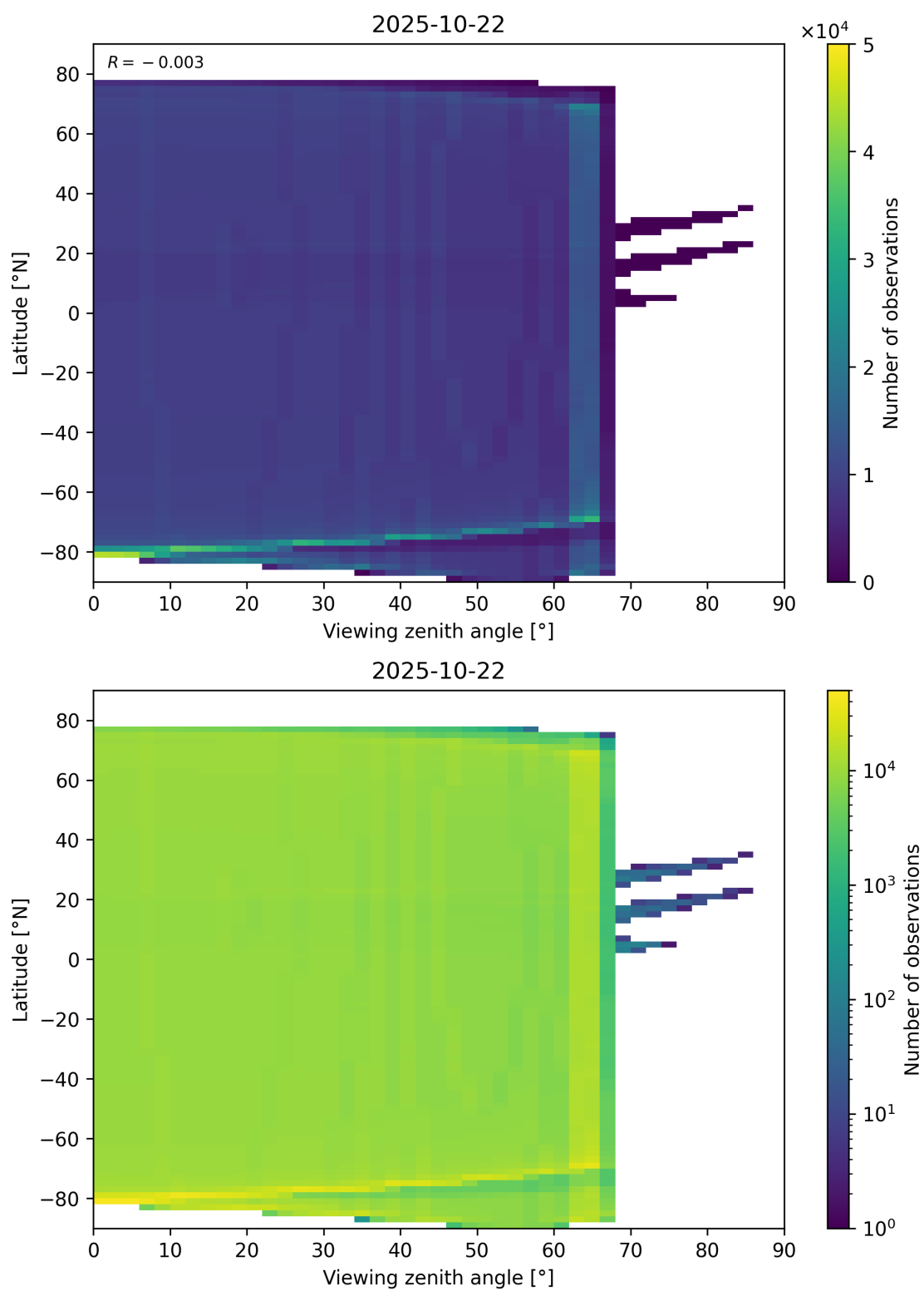
Figure 49: Scatter density plot of “Viewing zenith angle” against “Latitude” for 2025-10-22 to 2025-10-23.
