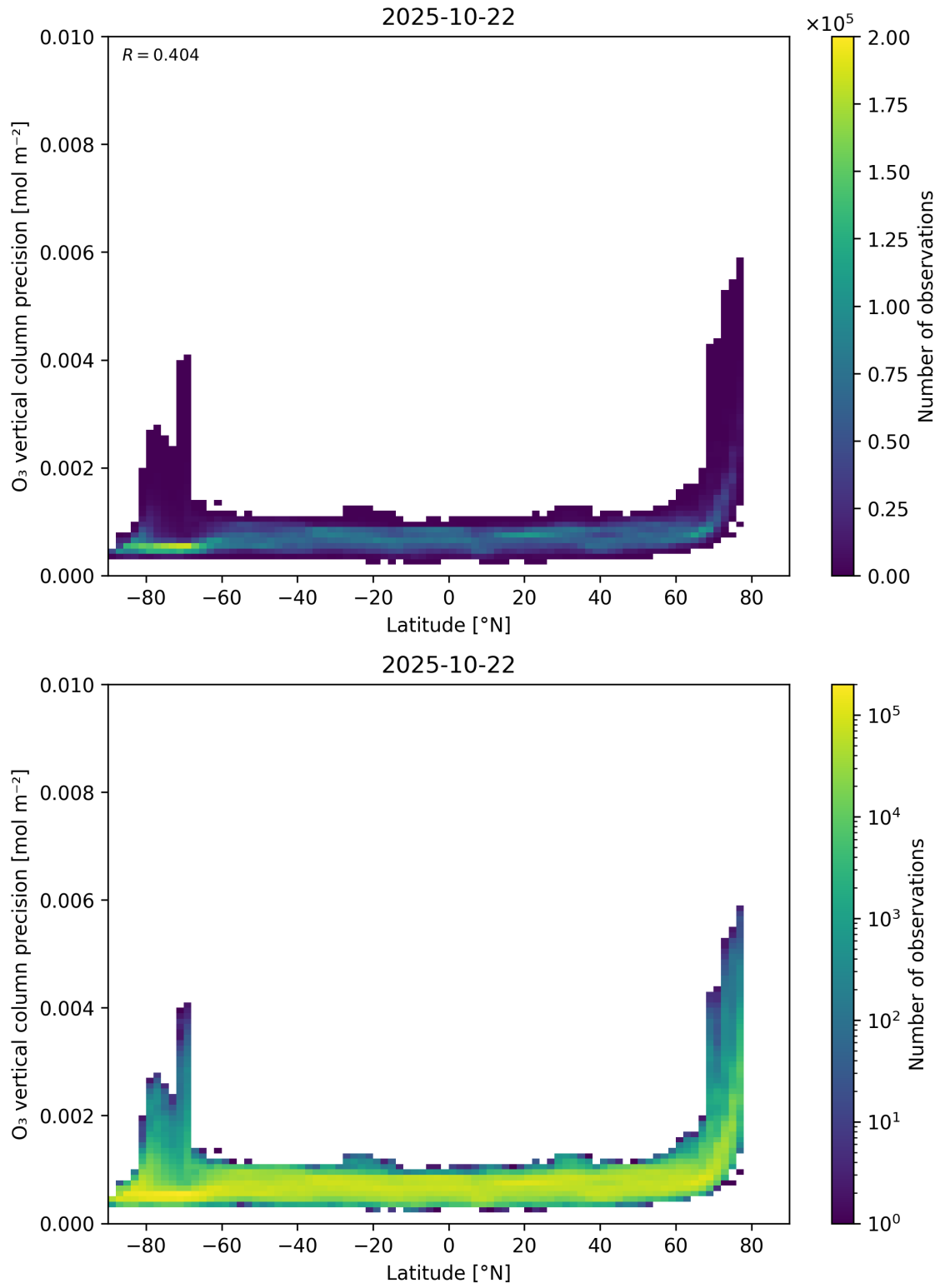
Figure 37: Scatter density plot of “Latitude” against “O 3 vertical column precision” for 2025-10-22 to 2025-10-23.
