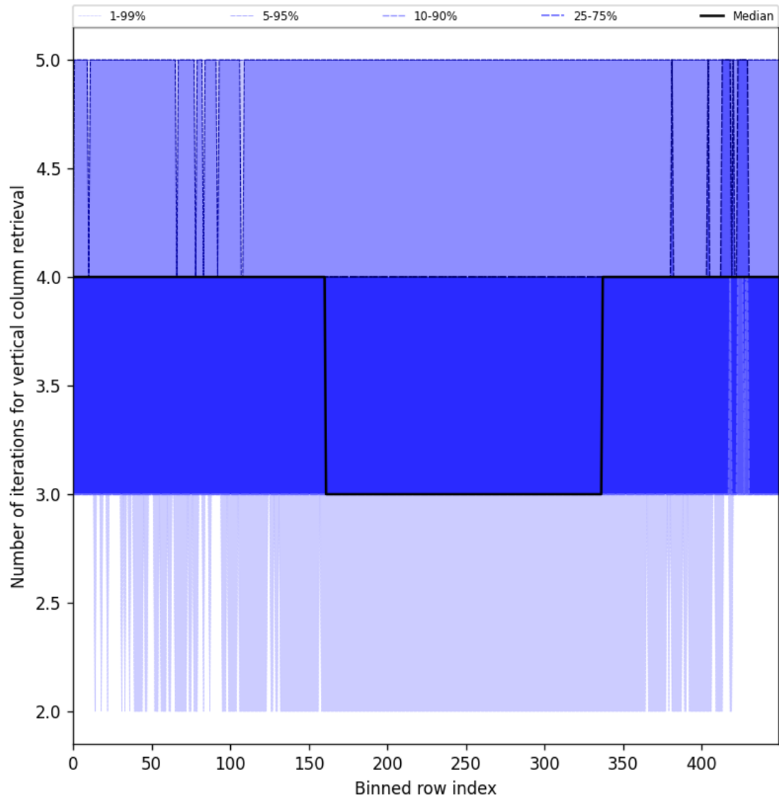
Figure 33: Along track statistics of “Number of iterations for vertical column retrieval” for 2025-10-22 to 2025-10-23
