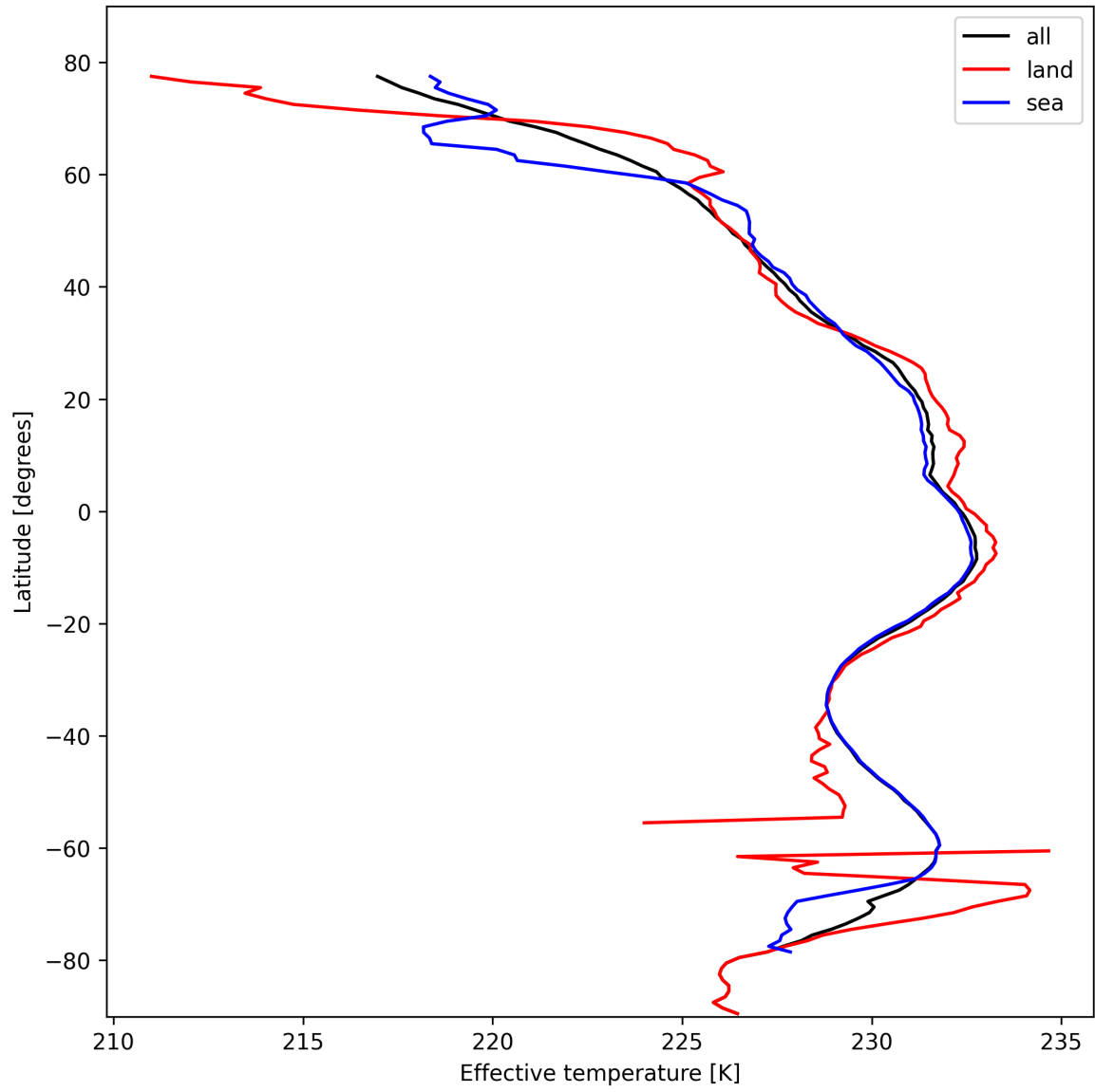
Figure 17: Zonal average of "Effective temperature" for 2025-10-22 to 2025-10-23.
