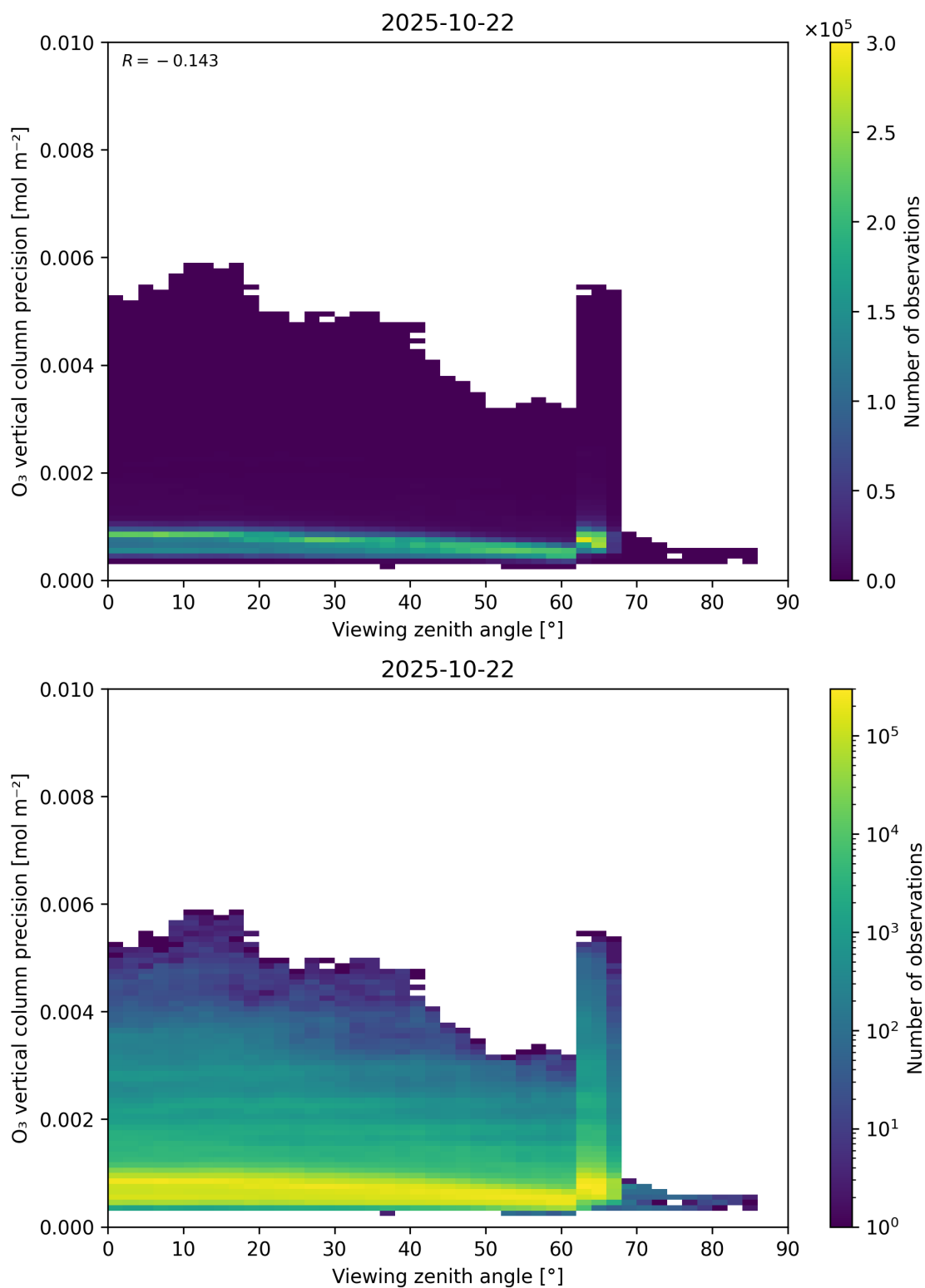
Figure 53: Scatter density plot of “Viewing zenith angle” against “O 3 vertical column precision” for 2025-10-22 to 2025-10-23.
