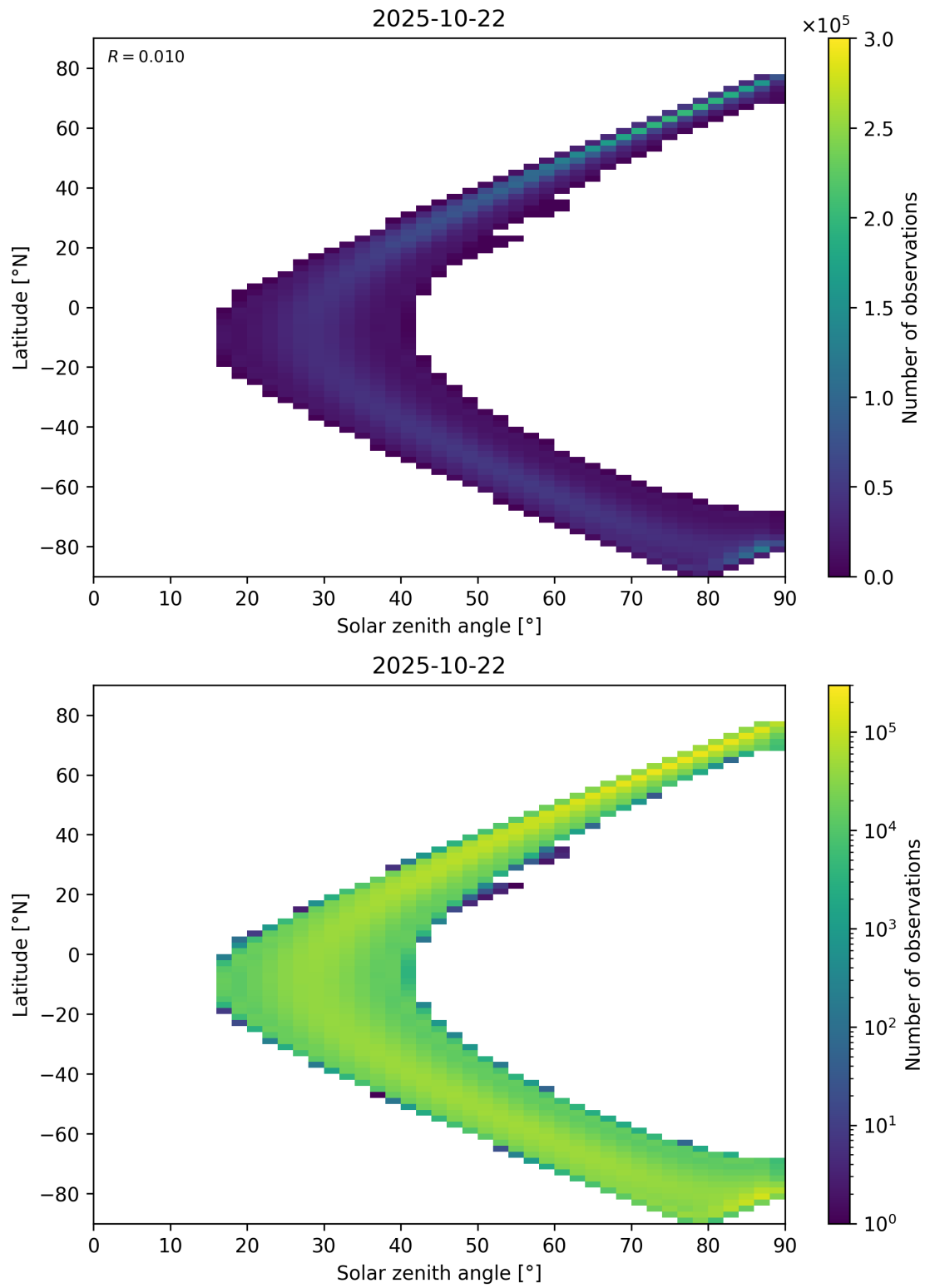
Figure 44: Scatter density plot of “Solar zenith angle” against “Latitude” for 2025-10-22 to 2025-10-23.
