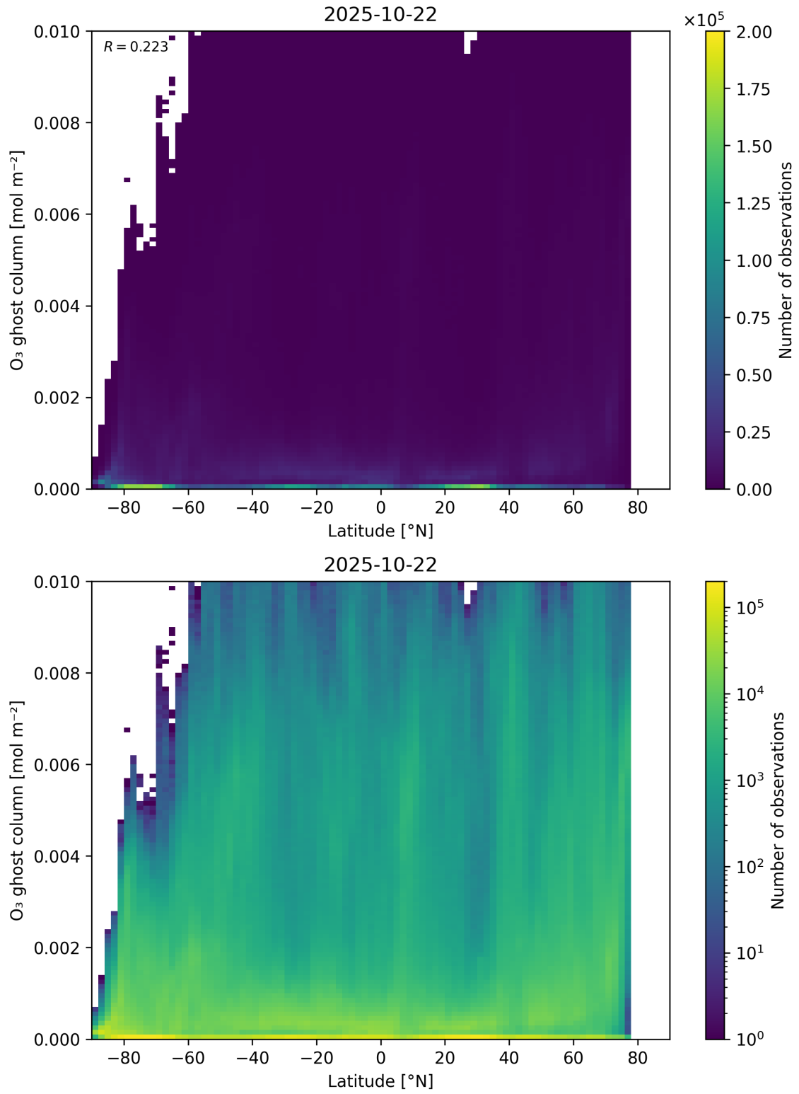
Figure 35: Scatter density plot of “Latitude” against “O 3 ghost column” for 2025-10-22 to 2025-10-23.
