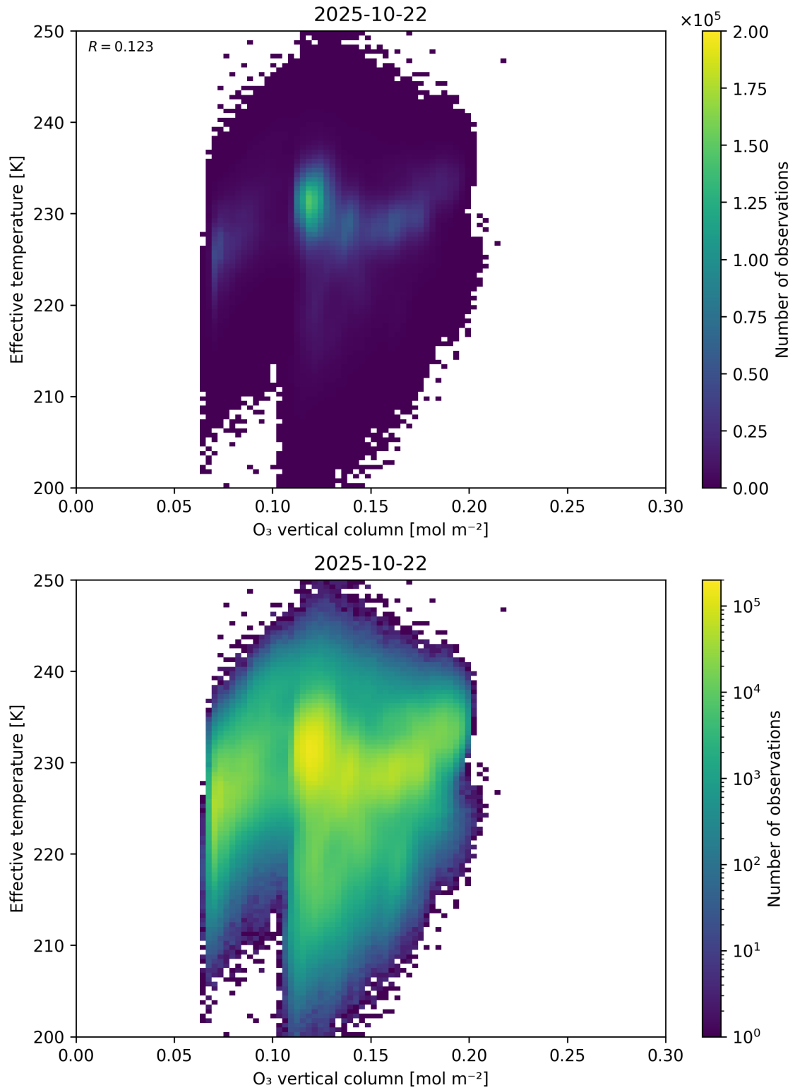
Figure 39: Scatter density plot of “O 3 vertical column” against “Effective temperature” for 2025-10-22 to 2025-10-23.
