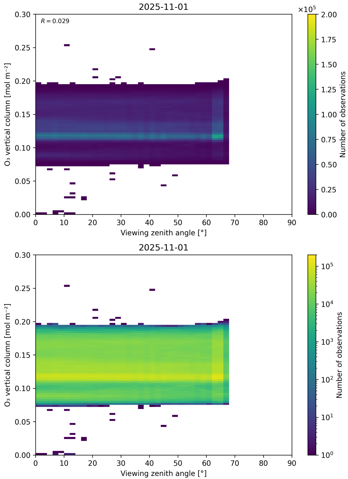
Figure 52: Scatter density plot of “Viewing zenith angle” against “O 3 vertical column” for 2025-10-31 to 2025-11-02.
