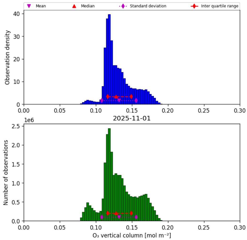
Figure 21: Histogram of “O 3 vertical column” for 2025-10-31 to 2025-11-02
