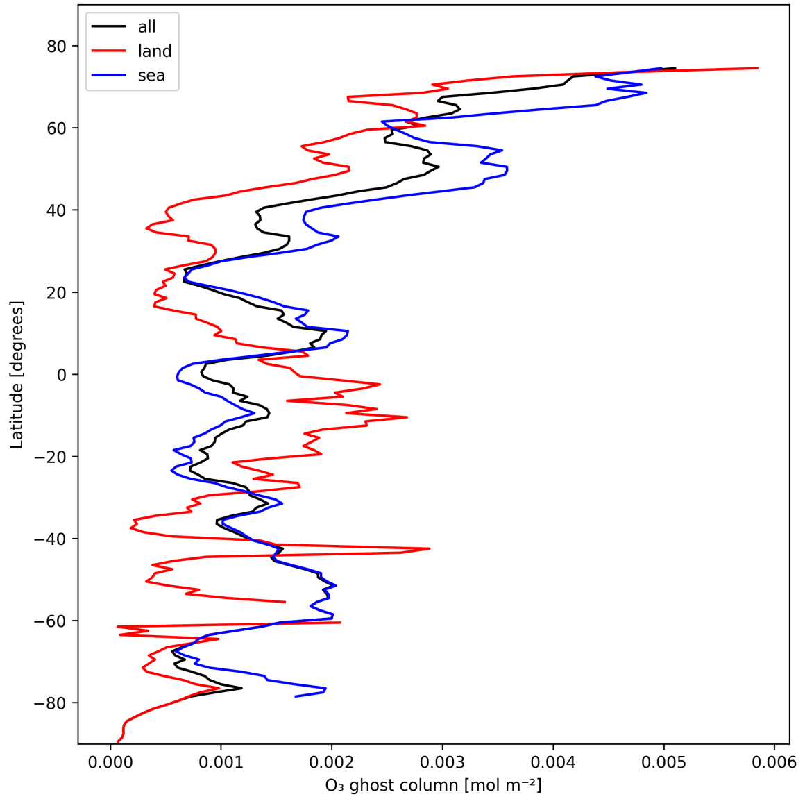
Figure 18: Zonal average of “O 3 ghost column” for 2025-10-31 to 2025-11-02.
