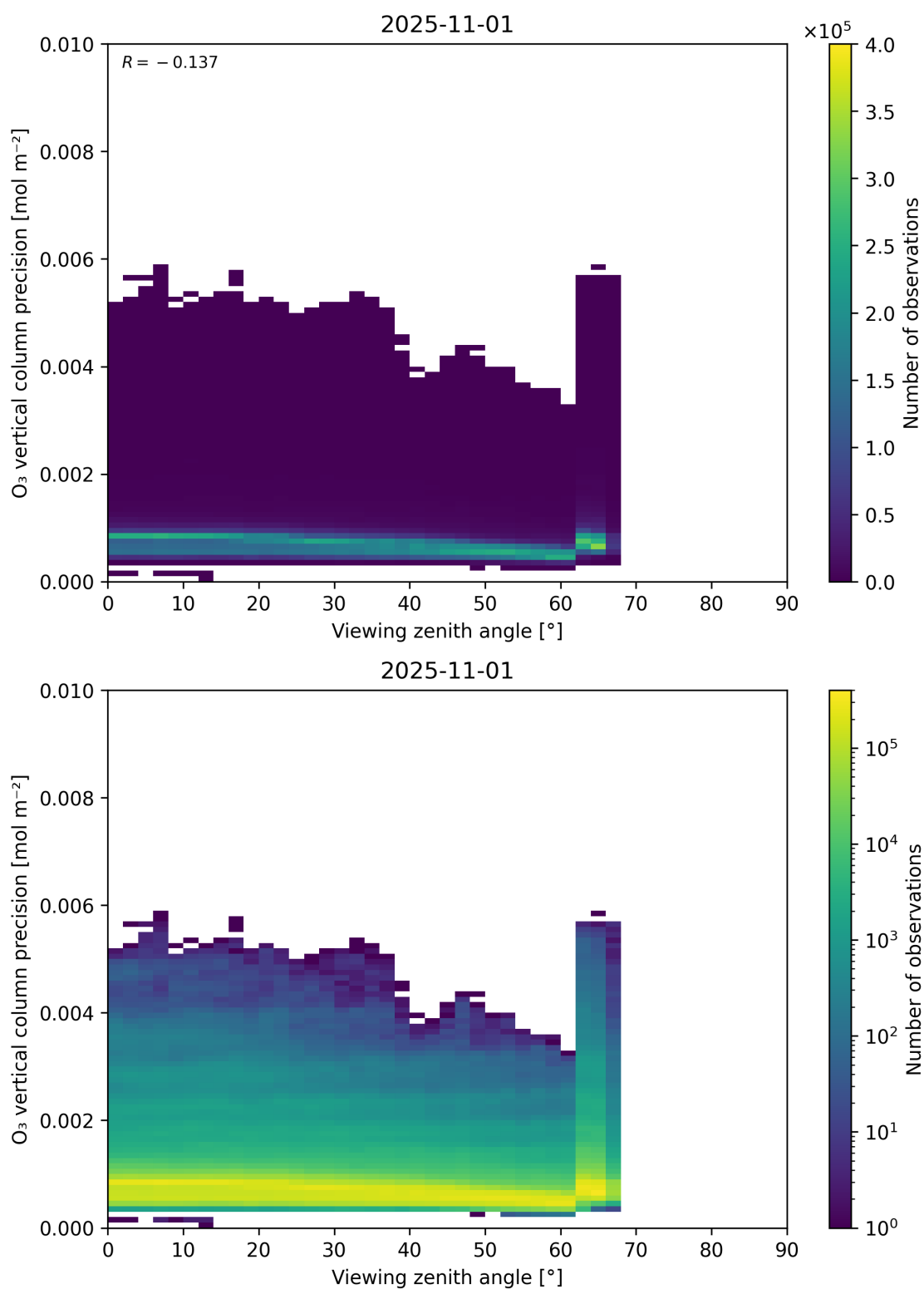
Figure 53: Scatter density plot of “Viewing zenith angle” against “O 3 vertical column precision” for 2025-10-31 to 2025-11-02.
