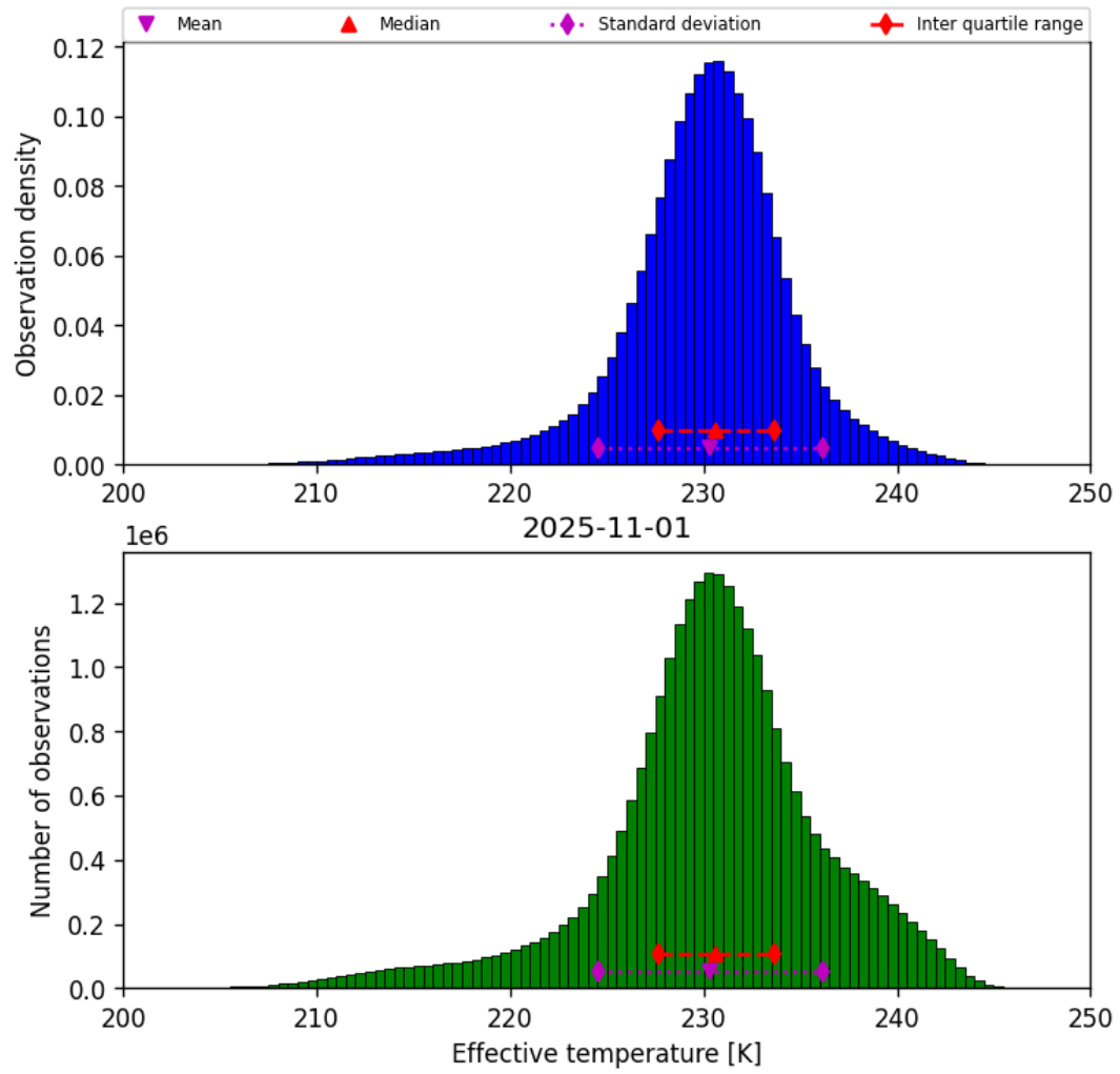
Figure 24: Histogram of “Effective temperature” for 2025-10-31 to 2025-11-02
