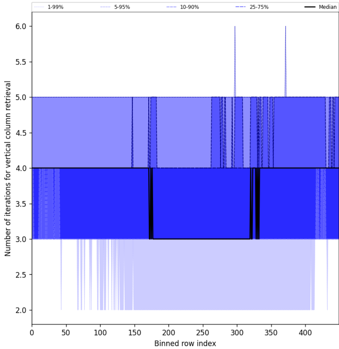
Figure 33: Along track statistics of “Number of iterations for vertical column retrieval” for 2025-10-31 to 2025-11-02
