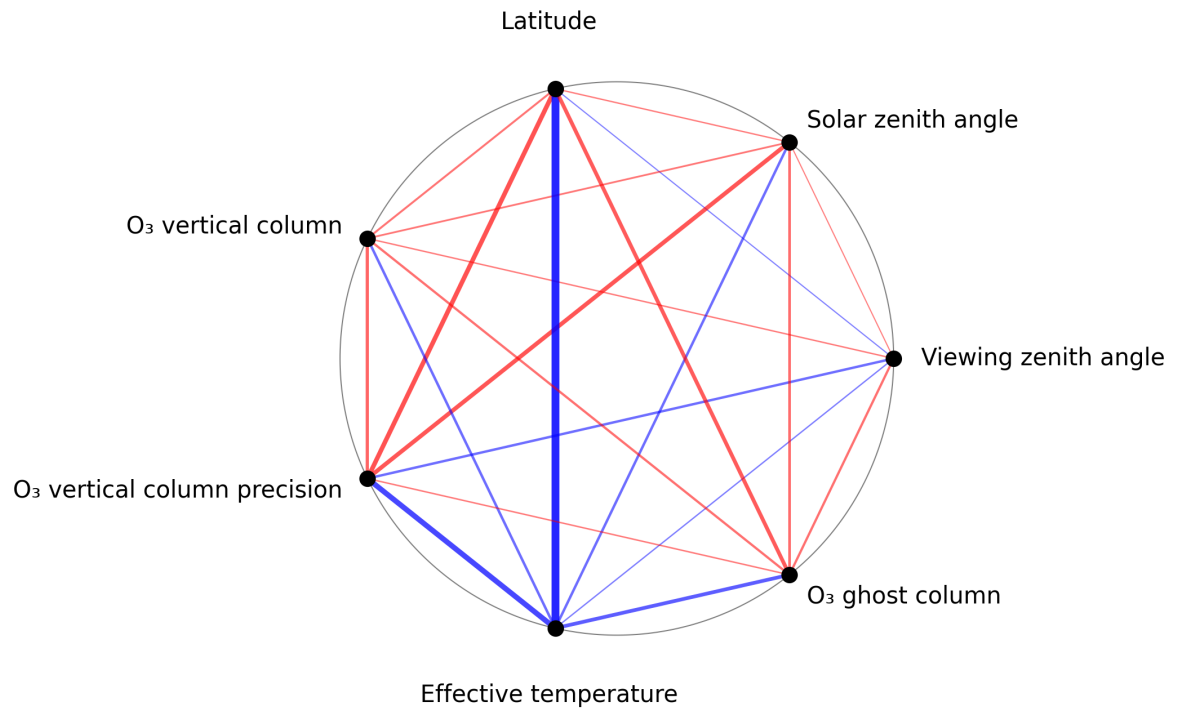
Figure 1: Map of correlation graph for 2025-10-31 to 2025-11-02.
