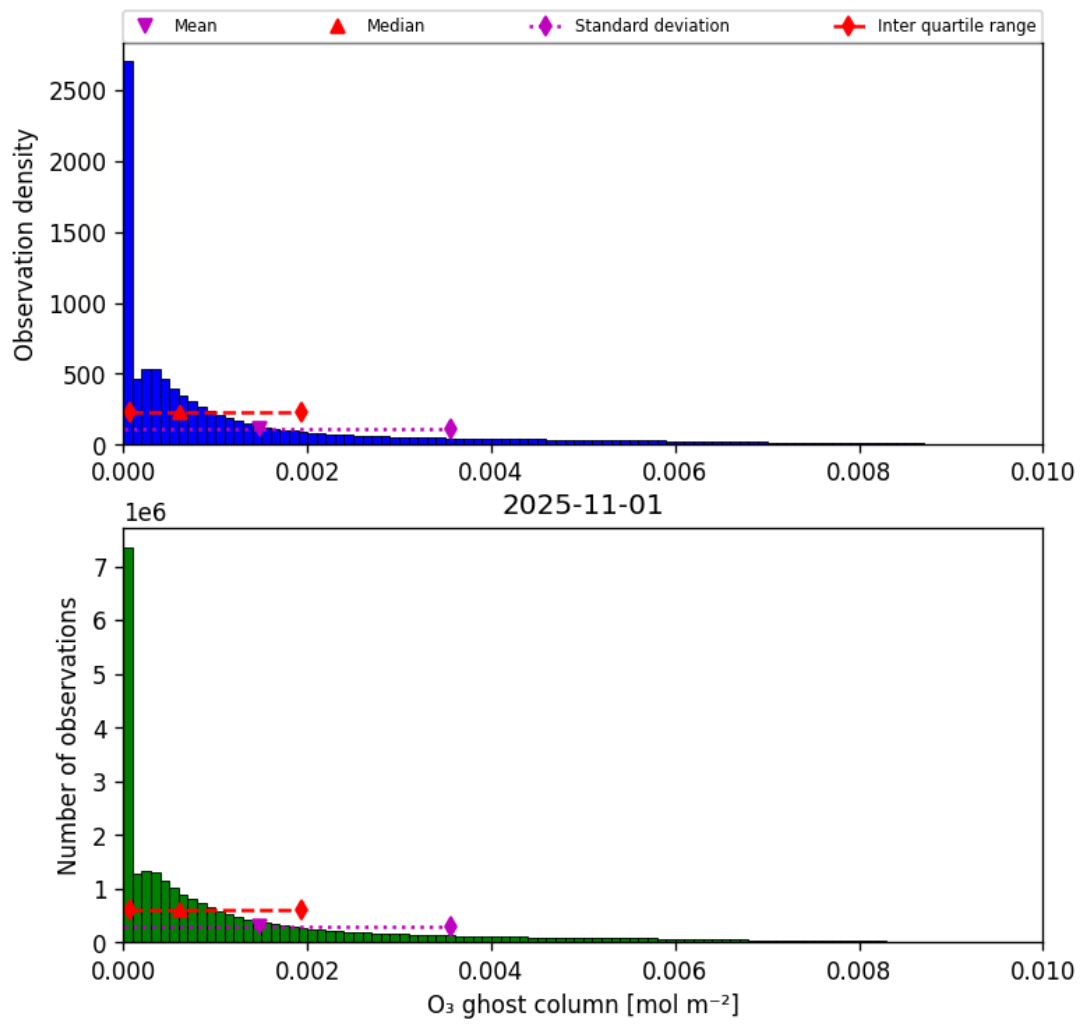
Figure 25: Histogram of “O 3 ghost column” for 2025-10-31 to 2025-11-02
