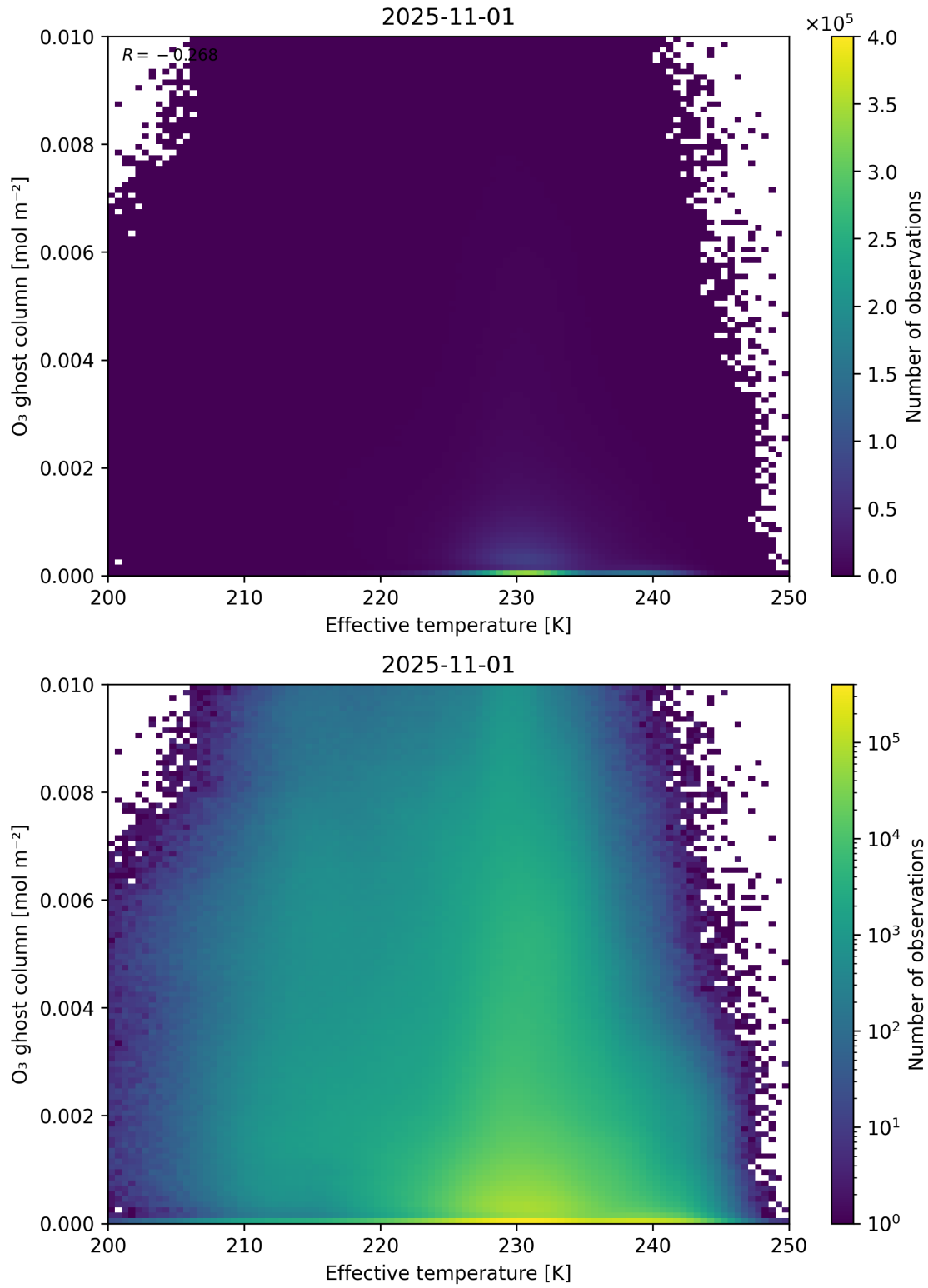
Figure 38: Scatter density plot of “Effective temperature” against “O 3 ghost column” for 2025-10-31 to 2025-11-02.
