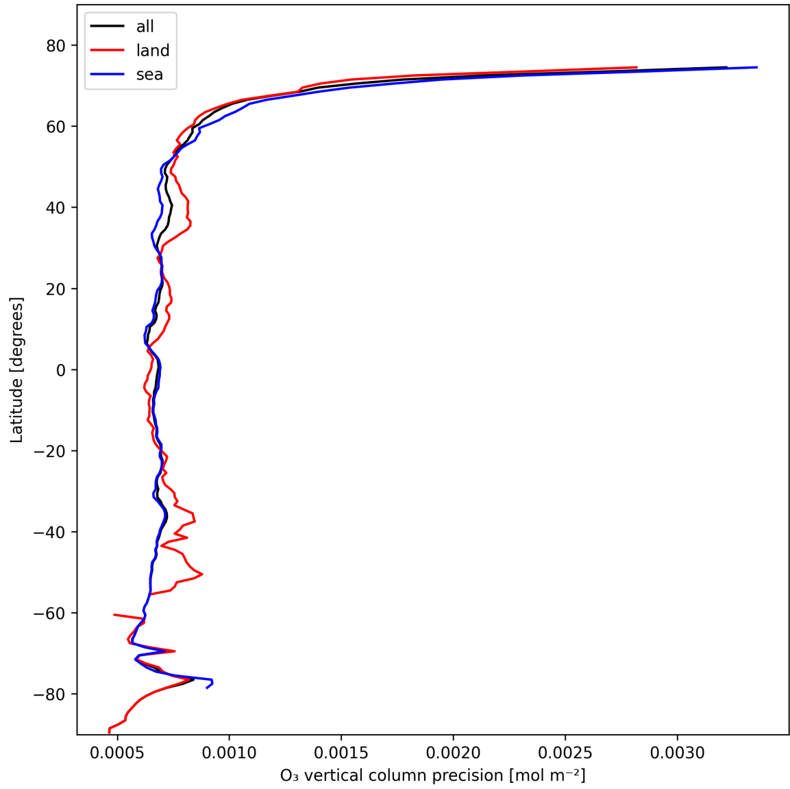
Figure 15: Zonal average of “O 3 vertical column precision” for 2025-10-31 to 2025-11-02.
