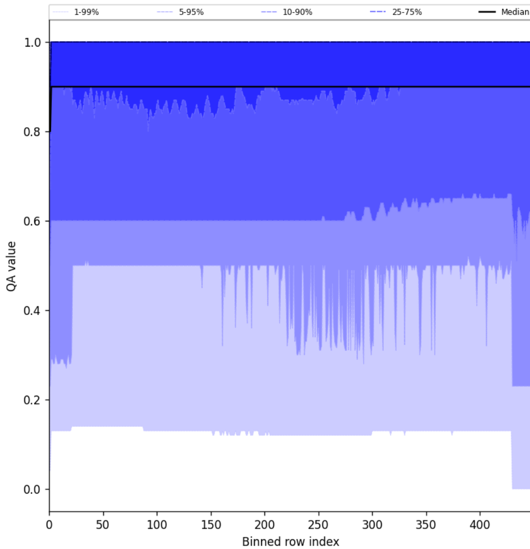
Figure 27: Along track statistics of “QA value” for 2025-10-31 to 2025-11-02
