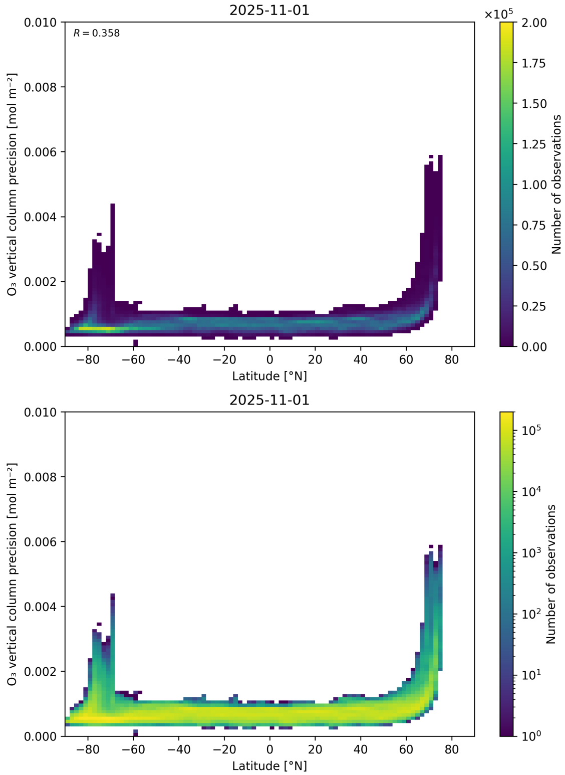
Figure 37: Scatter density plot of “Latitude” against “O 3 vertical column precision” for 2025-10-31 to 2025-11-02.
