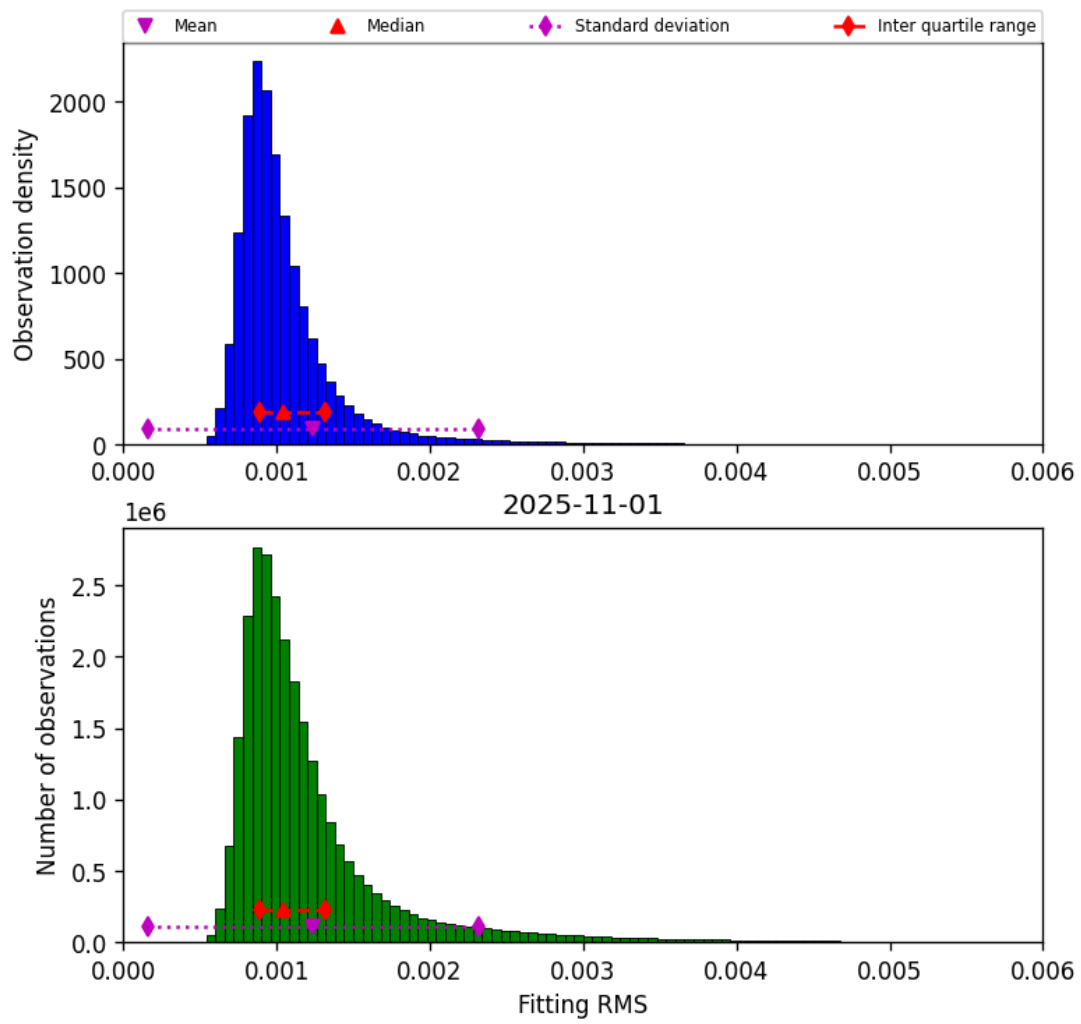
Figure 23: Histogram of “Fitting RMS” for 2025-10-31 to 2025-11-02
