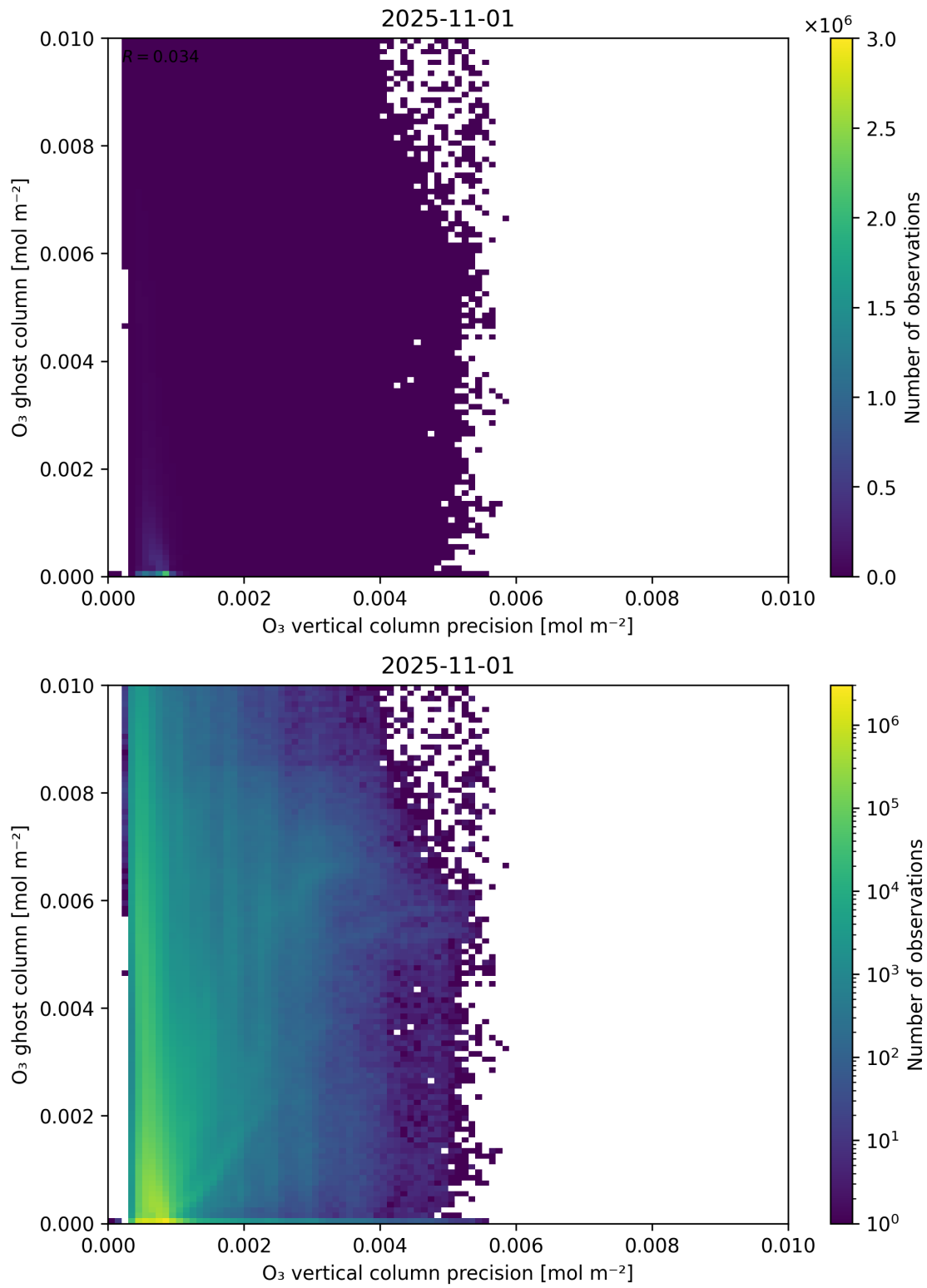
Figure 43: Scatter density plot of “O 3 vertical column precision” against “O 3 ghost column” for 2025-10-31 to 2025-11-02.
