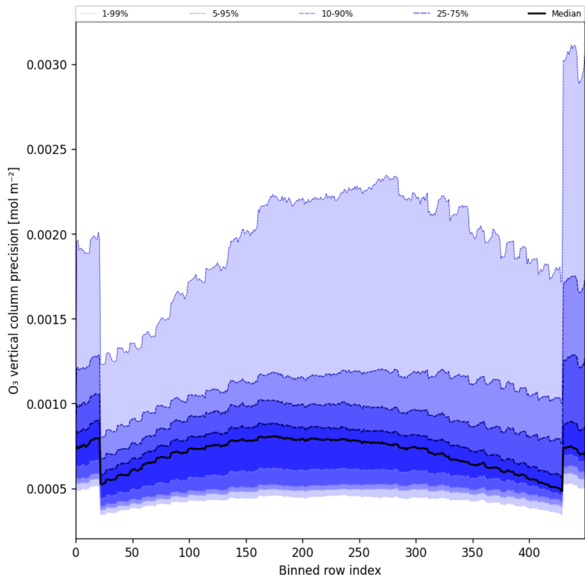
Figure 29: Along track statistics of “O 3 vertical column precision” for 2025-10-31 to 2025-11-02
