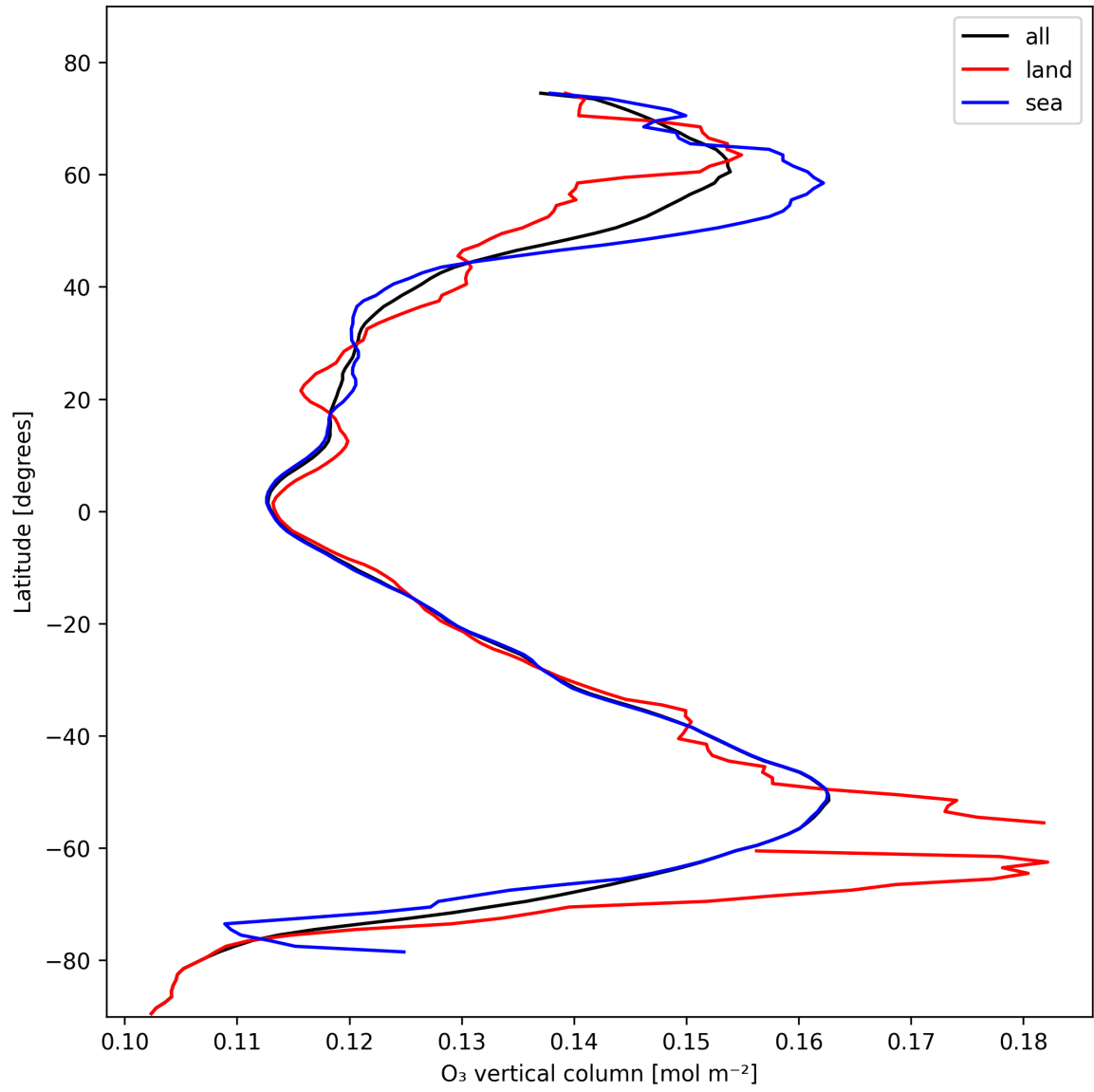
Figure 14: Zonal average of “O 3 vertical column” for 2025-10-31 to 2025-11-02.
