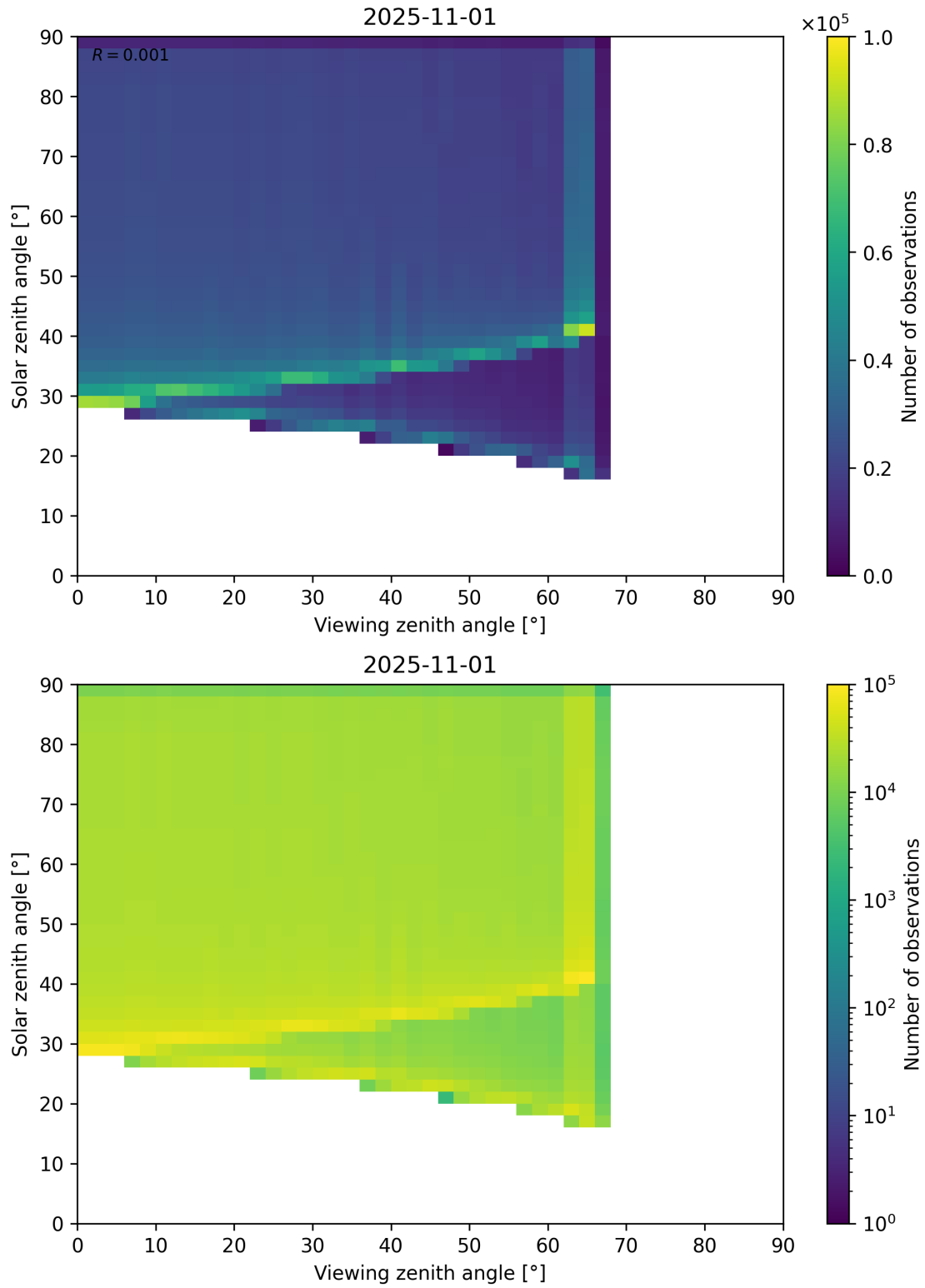
Figure 54: Scatter density plot of “Viewing zenith angle” against “Solar zenith angle” for 2025-10-31 to 2025-11-02.
