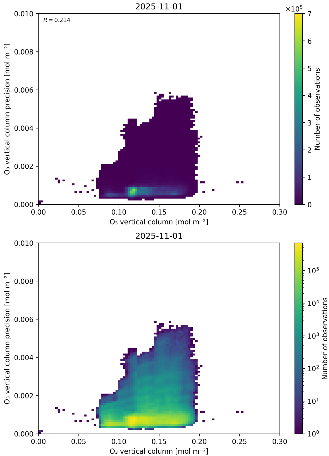
Figure 41: Scatter density plot of “O 3 vertical column” against “O 3 vertical column precision” for 2025-10-31 to 2025-11-02.
