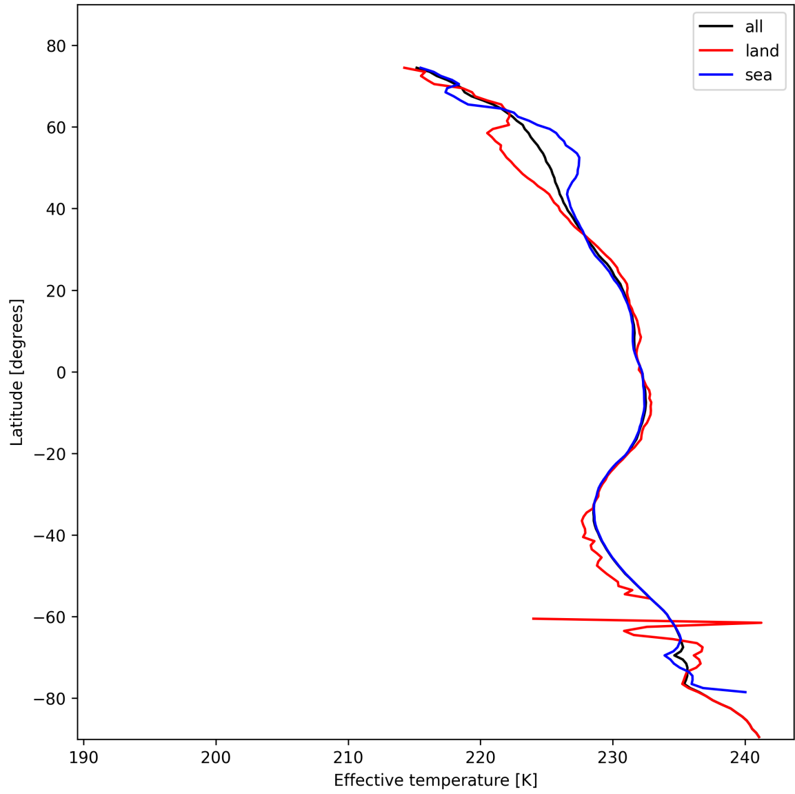
Figure 17: Zonal average of "Effective temperature" for 2025-10-31 to 2025-11-02.
