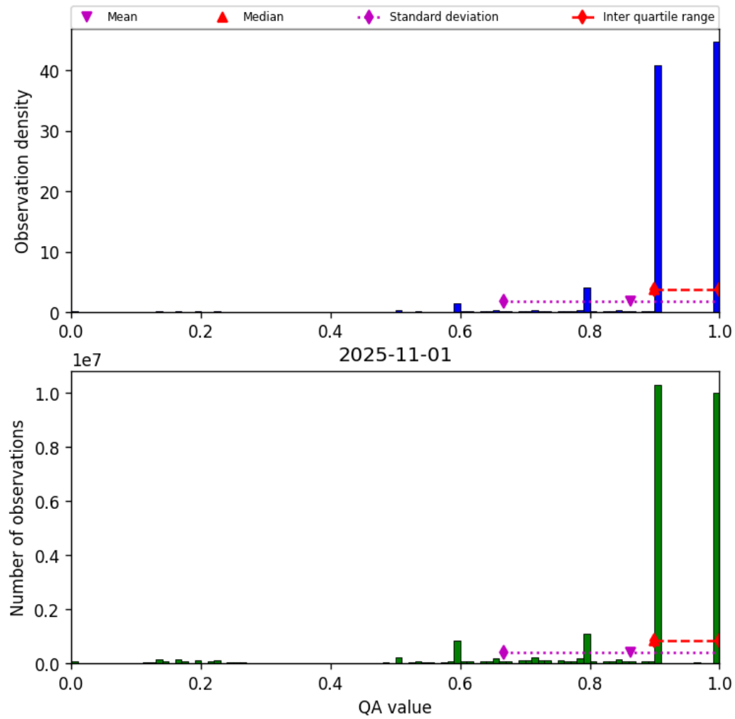
Figure 20: Histogram of “QA value” for 2025-10-31 to 2025-11-02
