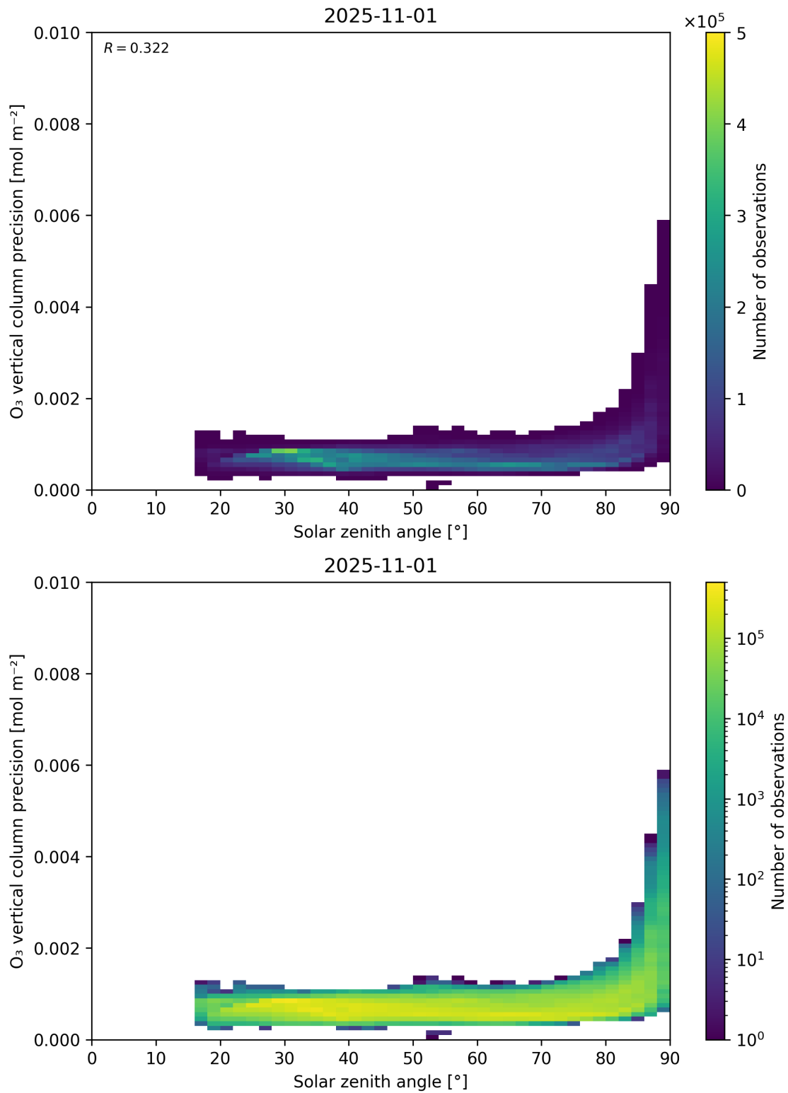
Figure 48: Scatter density plot of “Solar zenith angle” against “O 3 vertical column precision” for 2025-10-31 to 2025-11-02.
