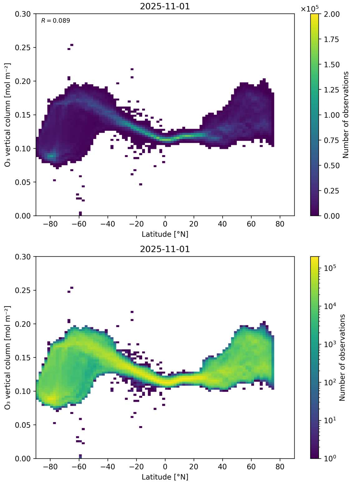
Figure 36: Scatter density plot of “Latitude” against “O 3 vertical column” for 2025-10-31 to 2025-11-02.
