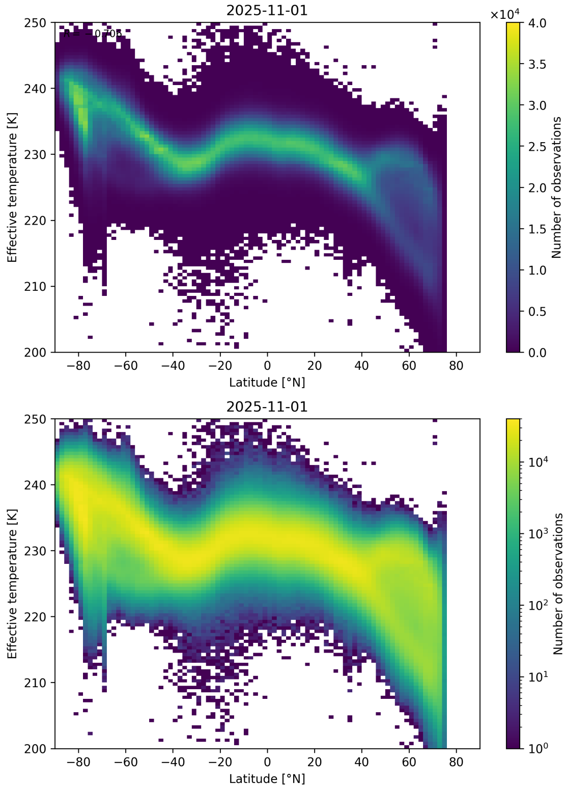
Figure 34: Scatter density plot of “Latitude” against “Effective temperature” for 2025-10-31 to 2025-11-02.
