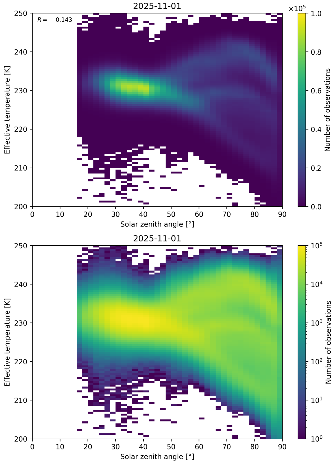
Figure 45: Scatter density plot of “Solar zenith angle” against “Effective temperature” for 2025-10-31 to 2025-11-02.
