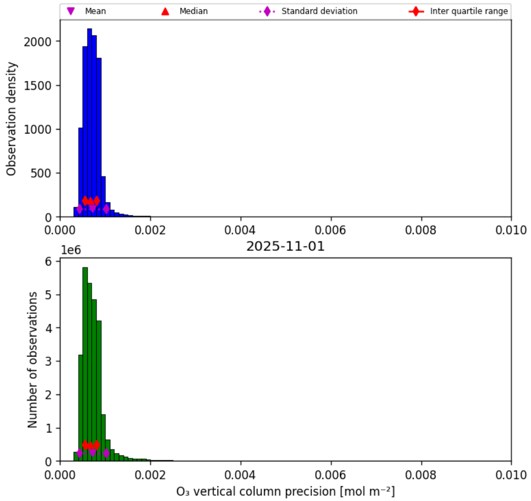
Figure 22: Histogram of “O 3 vertical column precision” for 2025-10-31 to 2025-11-02
