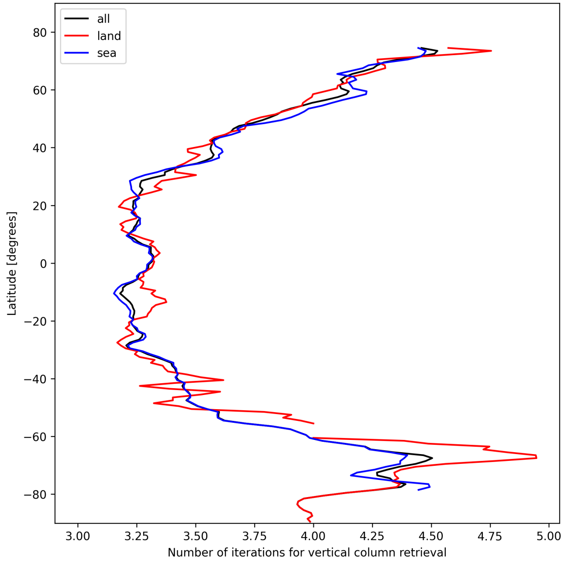
Figure 19: Zonal average of “Number of iterations for vertical column retrieval” for 2025-10-31 to 2025-11-02.
