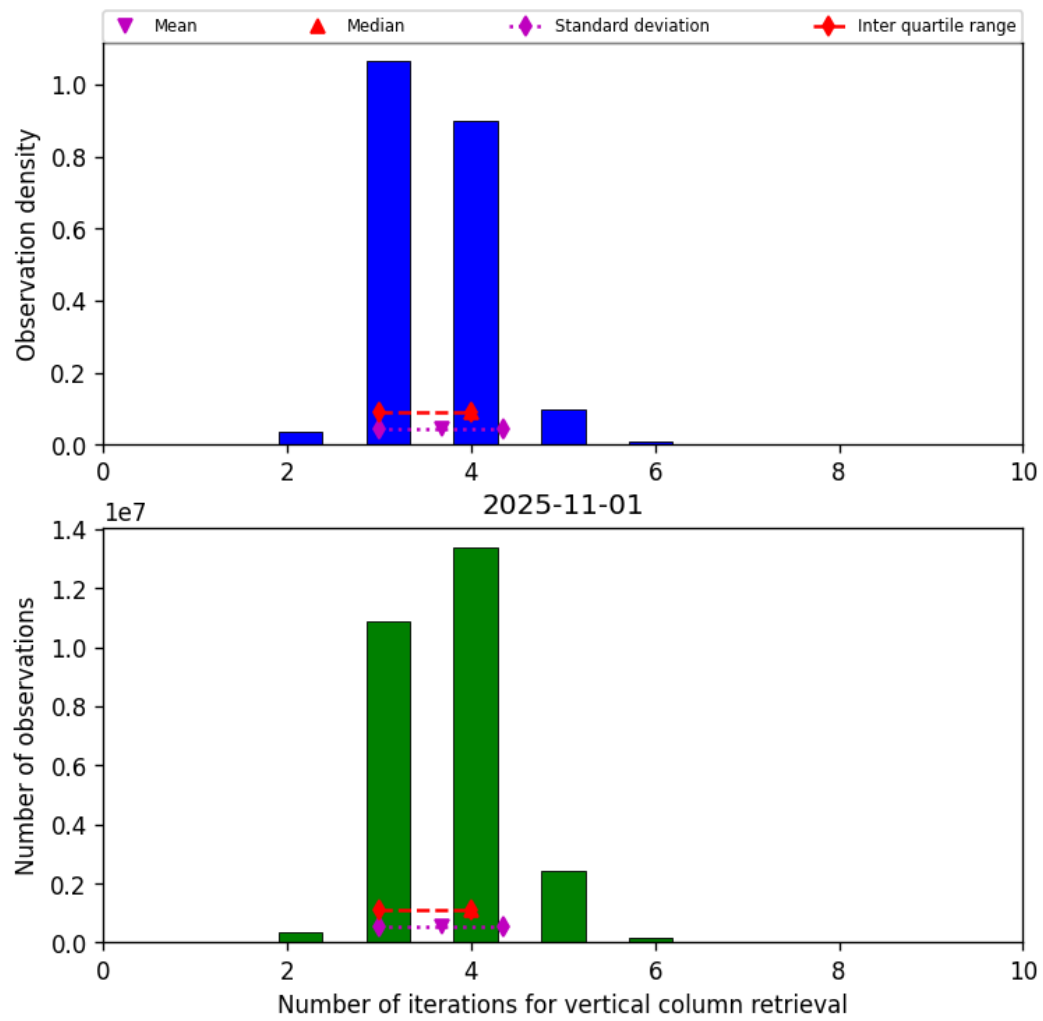
Figure 26: Histogram of “Number of iterations for vertical column retrieval” for 2025-10-31 to 2025-11-02
