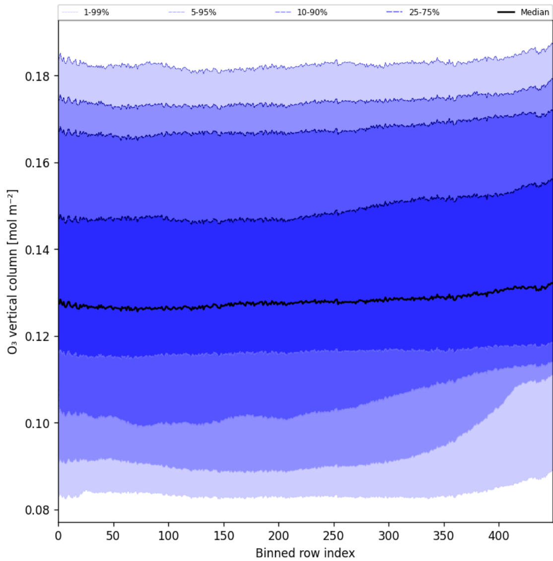
Figure 28: Along track statistics of “O 3 vertical column” for 2025-10-31 to 2025-11-02
