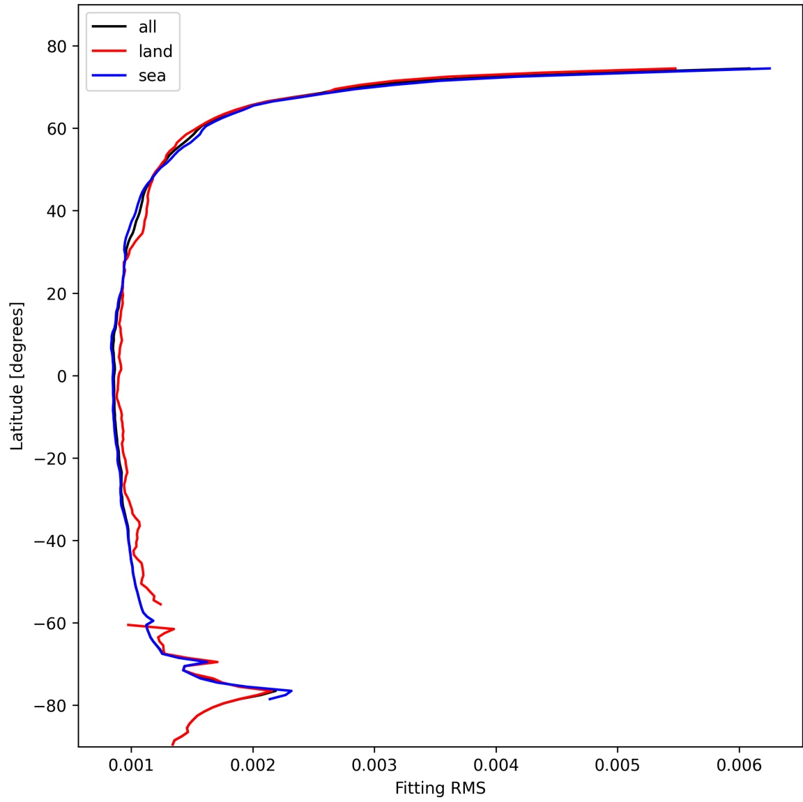
Figure 16: Zonal average of “Fitting RMS” for 2025-10-31 to 2025-11-02.
