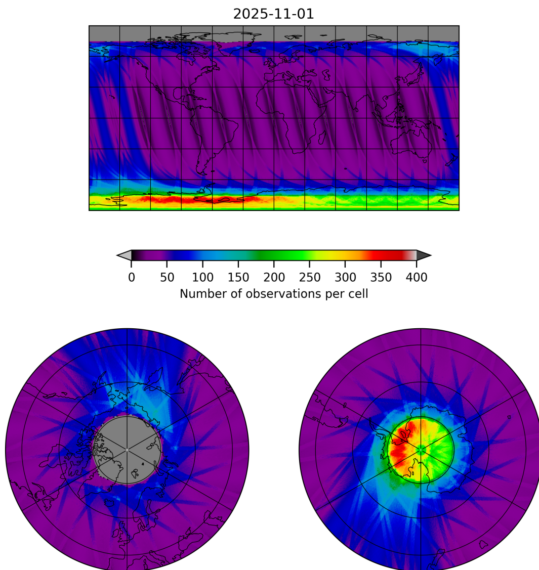
Figure 12: Map of the number of observations for 2025-10-31 to 2025-11-02
