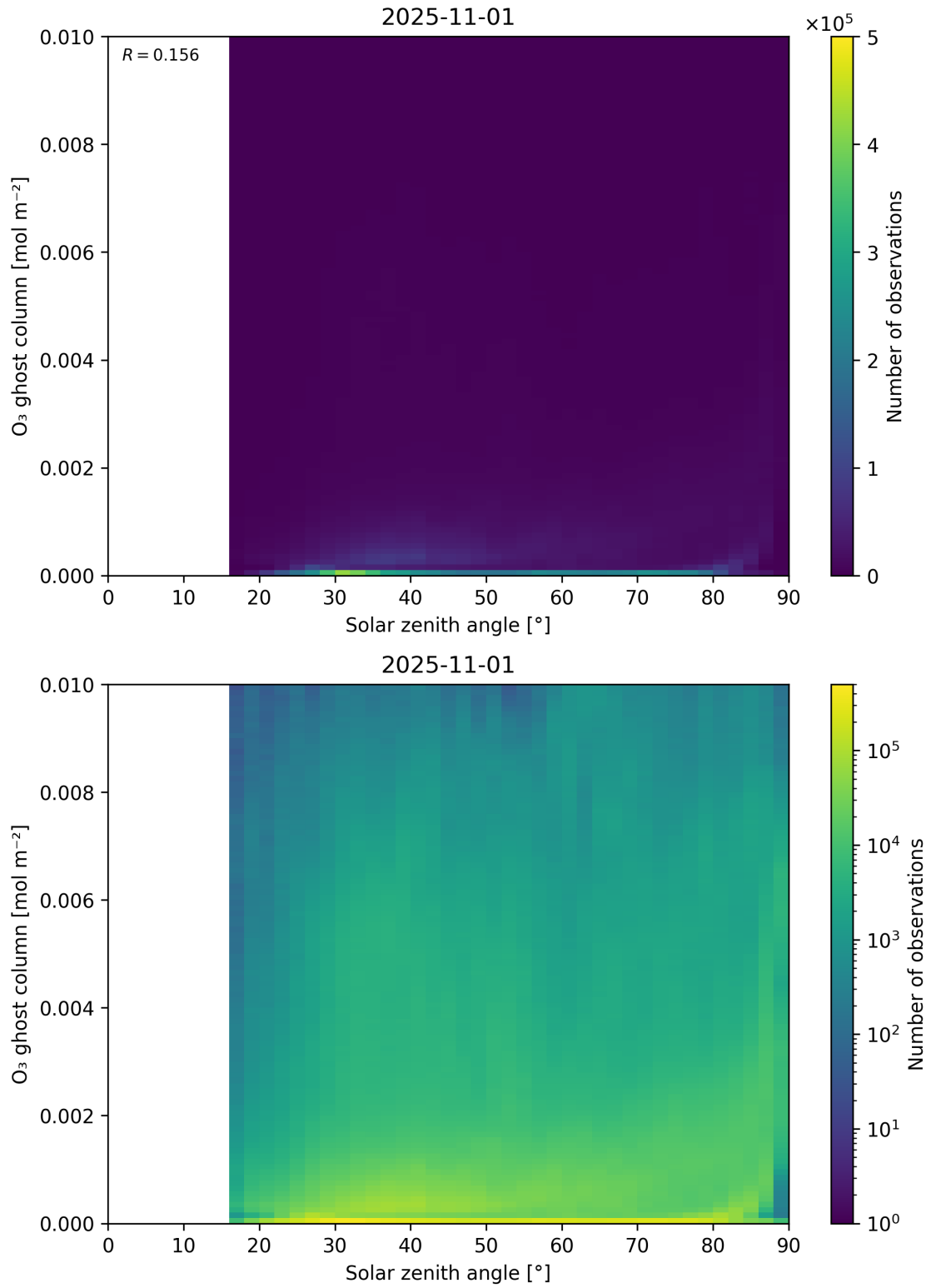
Figure 46: Scatter density plot of “Solar zenith angle” against “O 3 ghost column” for 2025-10-31 to 2025-11-02.
