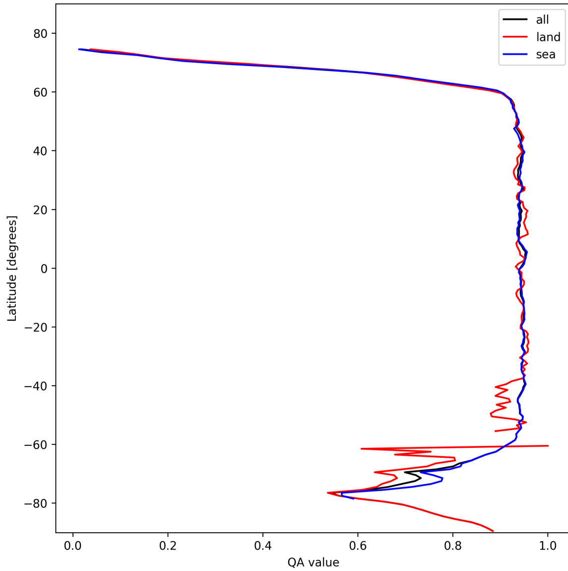
Figure 13: Zonal average of “QA value” for 2025-10-31 to 2025-11-02.
