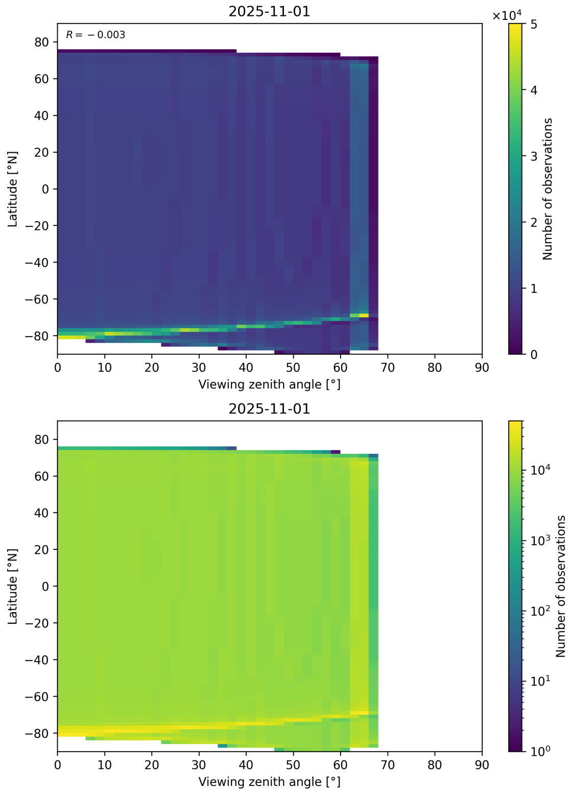
Figure 49: Scatter density plot of “Viewing zenith angle” against “Latitude” for 2025-10-31 to 2025-11-02.
