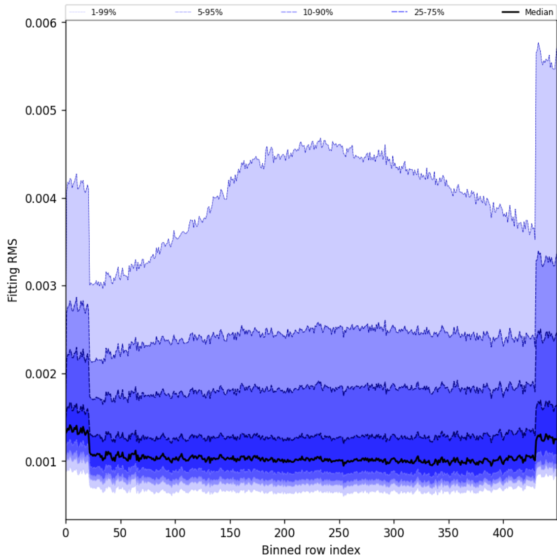
Figure 30: Along track statistics of “Fitting RMS” for 2025-10-31 to 2025-11-02
