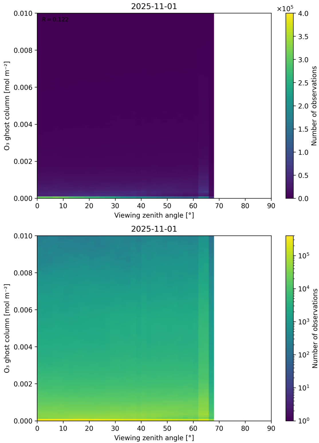
Figure 51: Scatter density plot of “Viewing zenith angle” against “O 3 ghost column” for 2025-10-31 to 2025-11-02.
