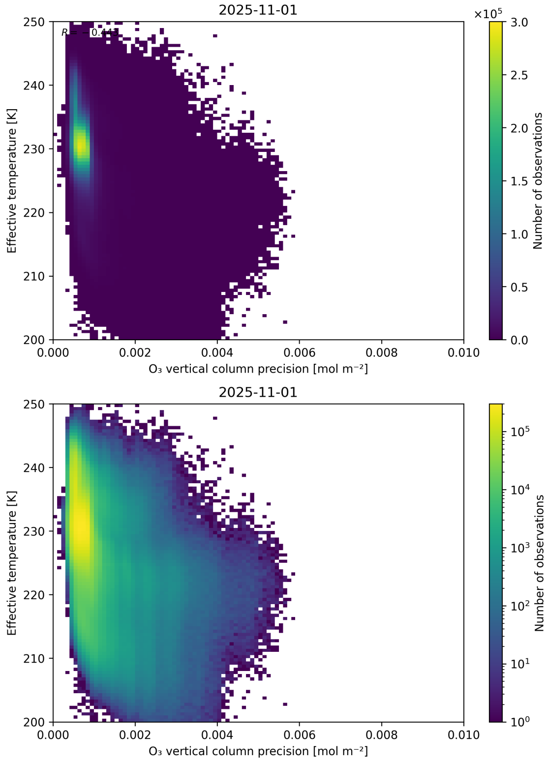
Figure 42: Scatter density plot of “O 3 vertical column precision” against “Effective temperature” for 2025-10-31 to 2025-11-02.
