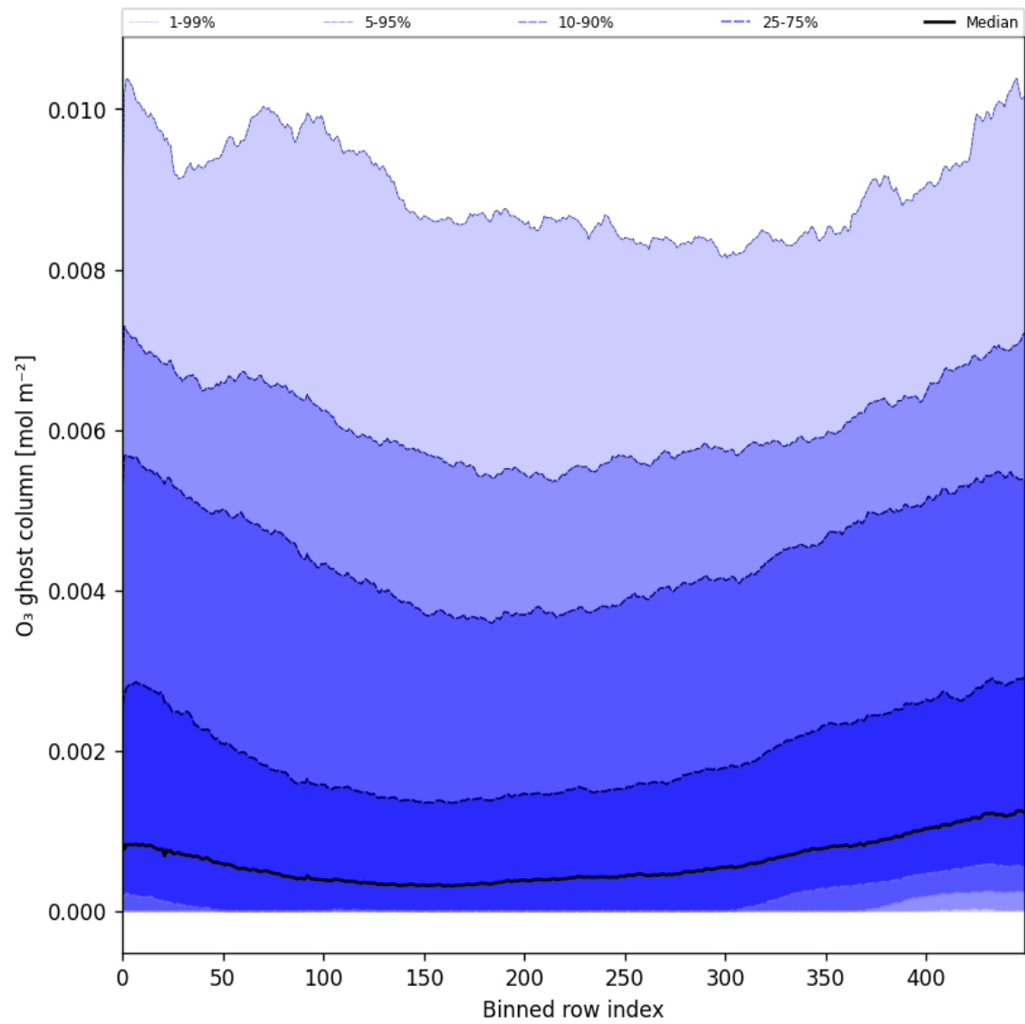
Figure 32: Along track statistics of “O 3 ghost column” for 2025-10-31 to 2025-11-02
