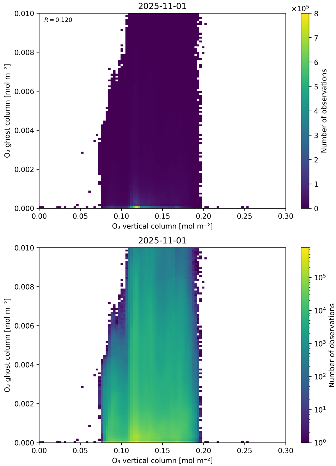
Figure 40: Scatter density plot of “O 3 vertical column” against “O 3 ghost column” for 2025-10-31 to 2025-11-02.
