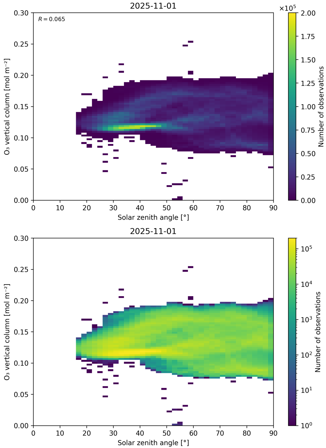
Figure 47: Scatter density plot of “Solar zenith angle” against “O 3 vertical column” for 2025-10-31 to 2025-11-02.
