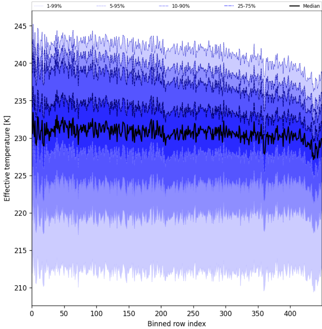
Figure 31: Along track statistics of “Effective temperature” for 2025-10-31 to 2025-11-02
