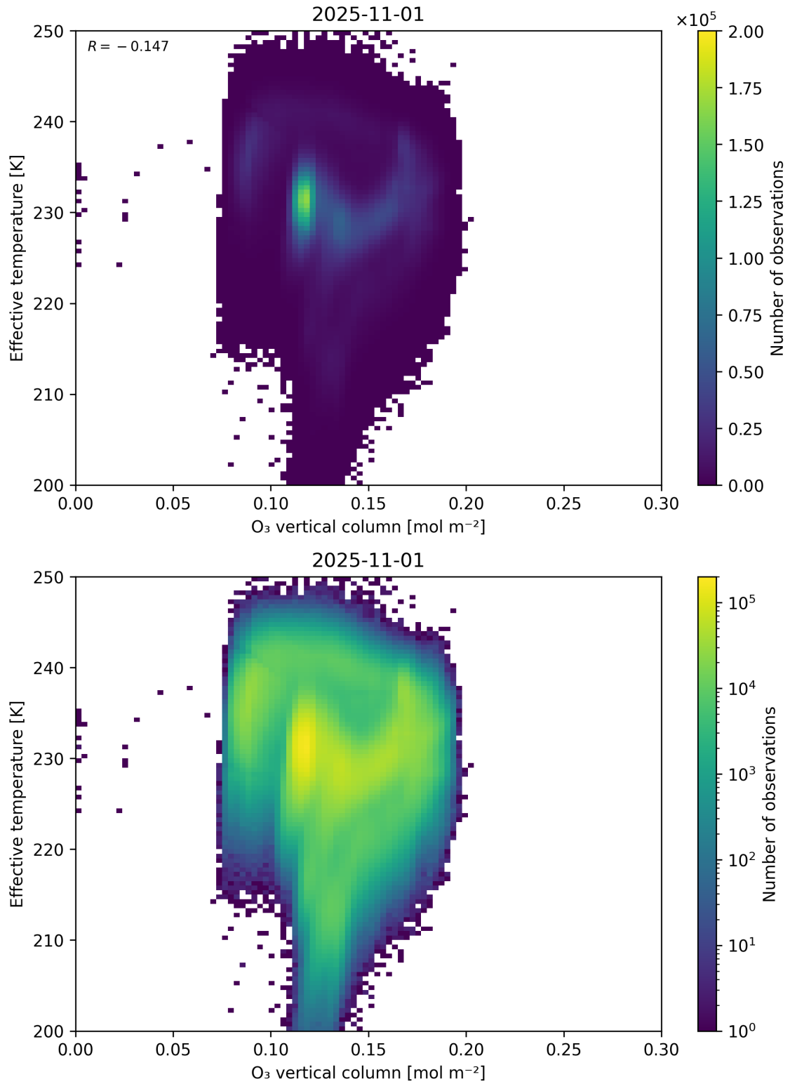
Figure 39: Scatter density plot of “O 3 vertical column” against “Effective temperature” for 2025-10-31 to 2025-11-02.
