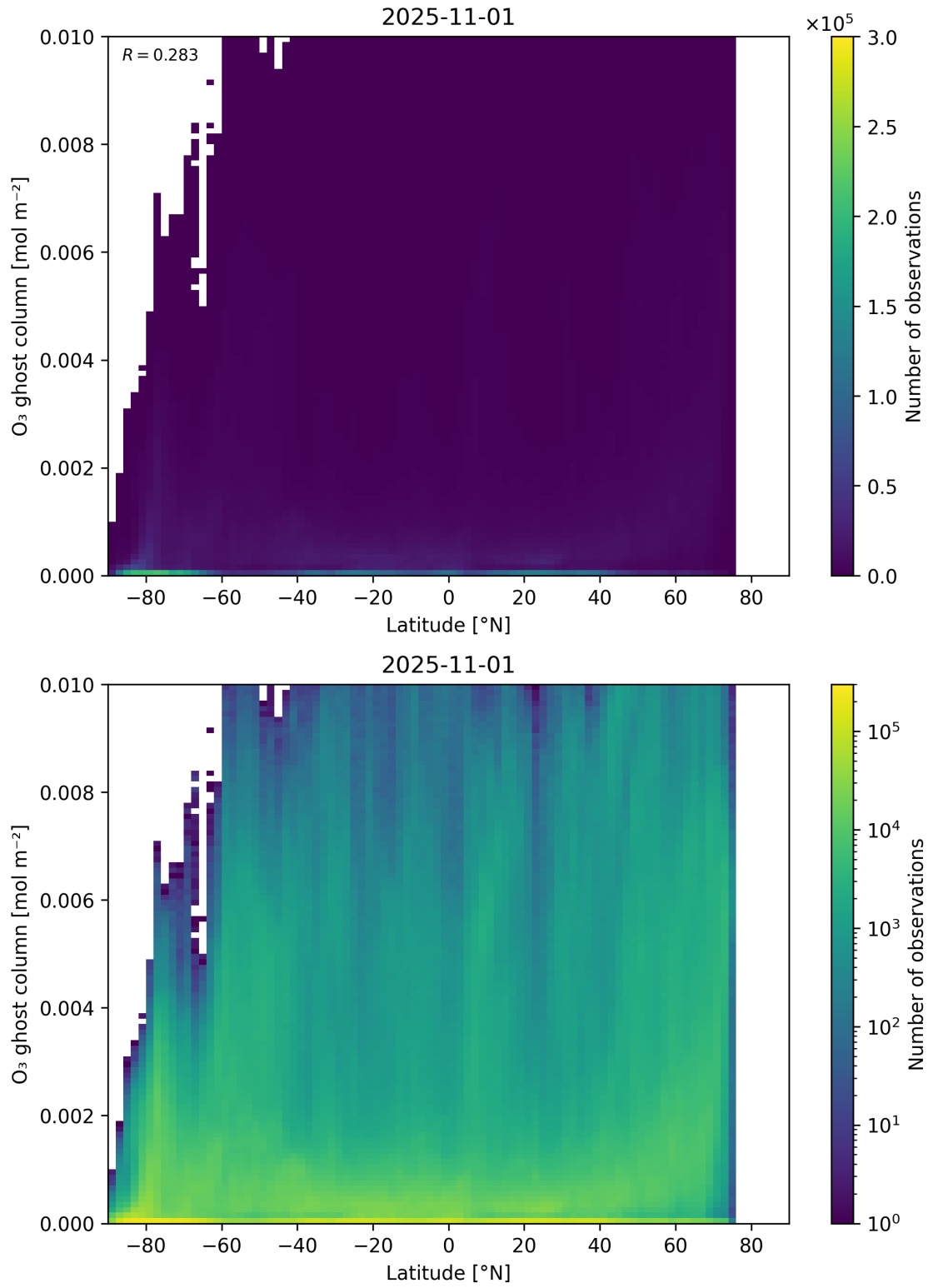
Figure 35: Scatter density plot of “Latitude” against “O 3 ghost column” for 2025-10-31 to 2025-11-02.
