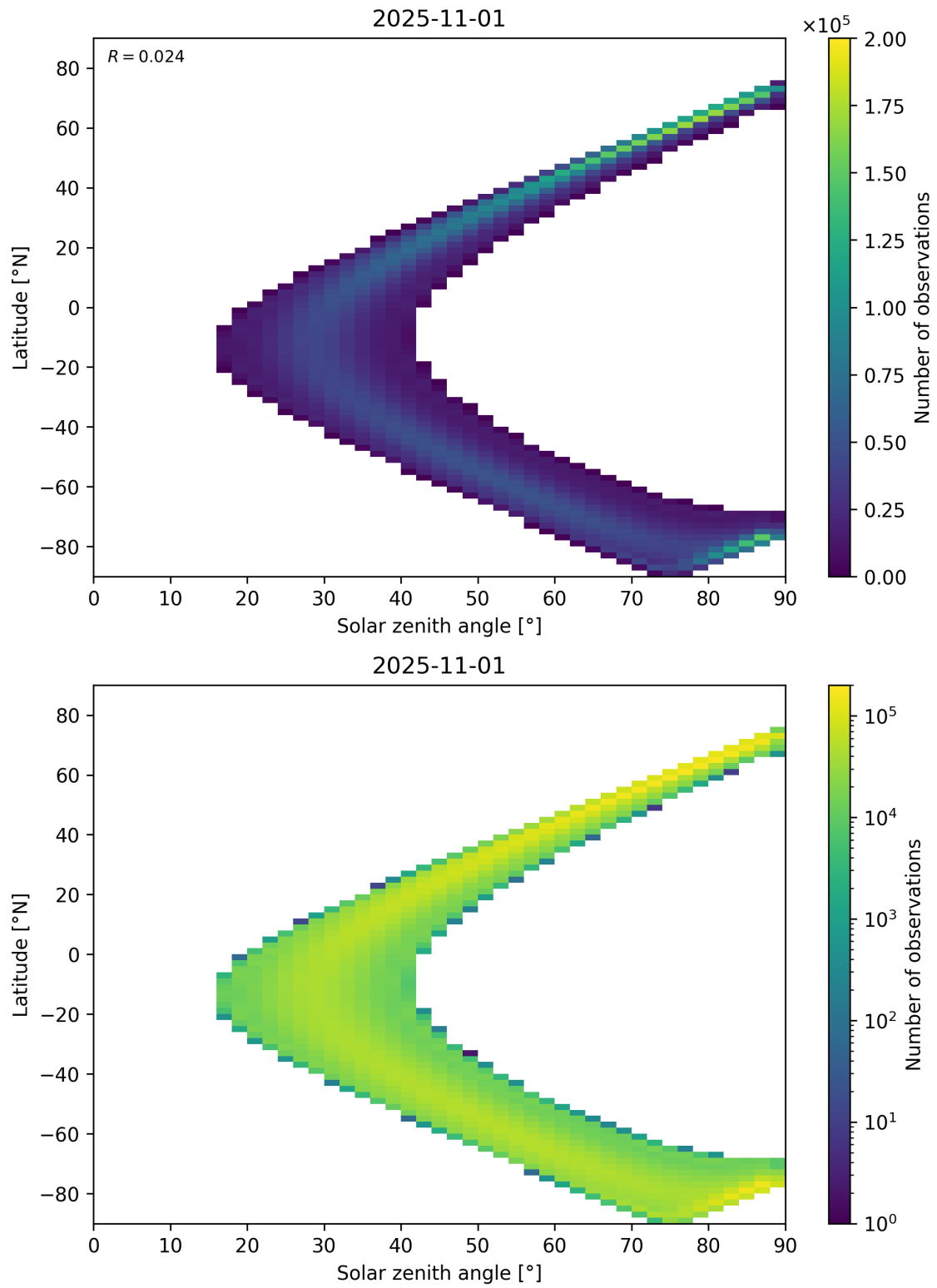
Figure 44: Scatter density plot of “Solar zenith angle” against “Latitude” for 2025-10-31 to 2025-11-02.
