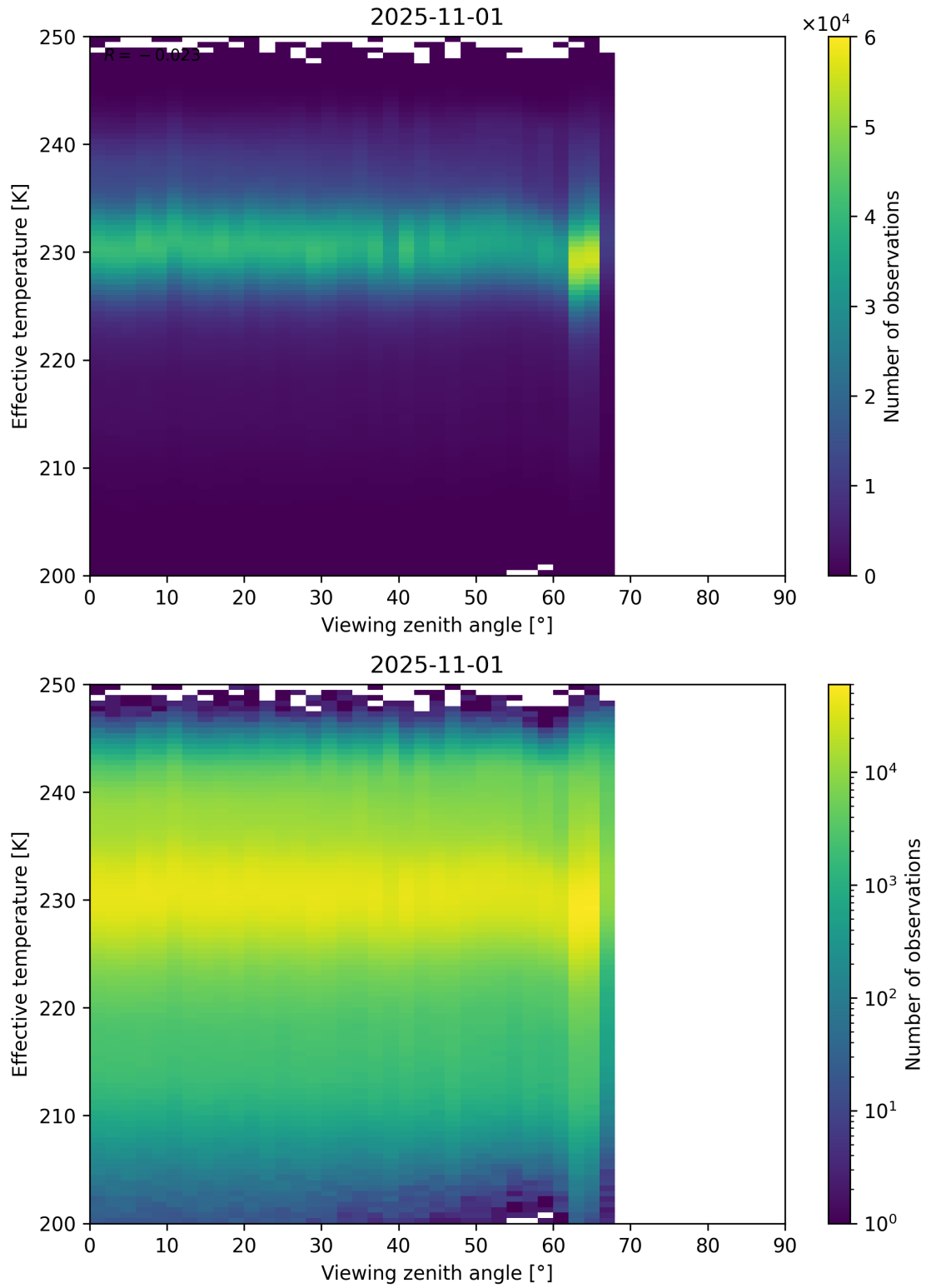
Figure 50: Scatter density plot of “Viewing zenith angle” against “Effective temperature” for 2025-10-31 to 2025-11-02.
