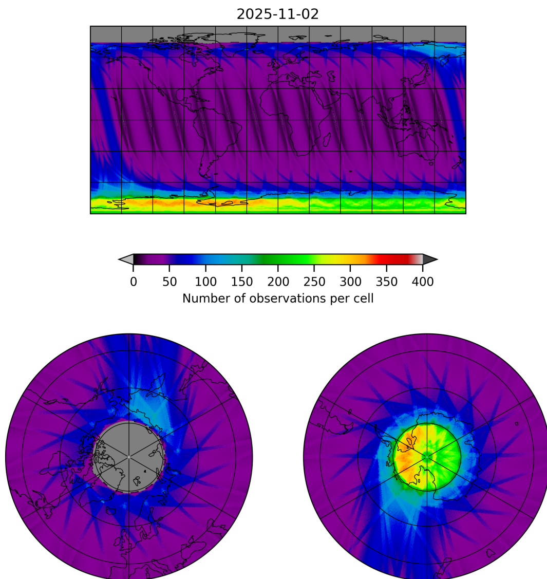
Figure 12: Map of the number of observations for 2025-11-02 to 2025-11-03
