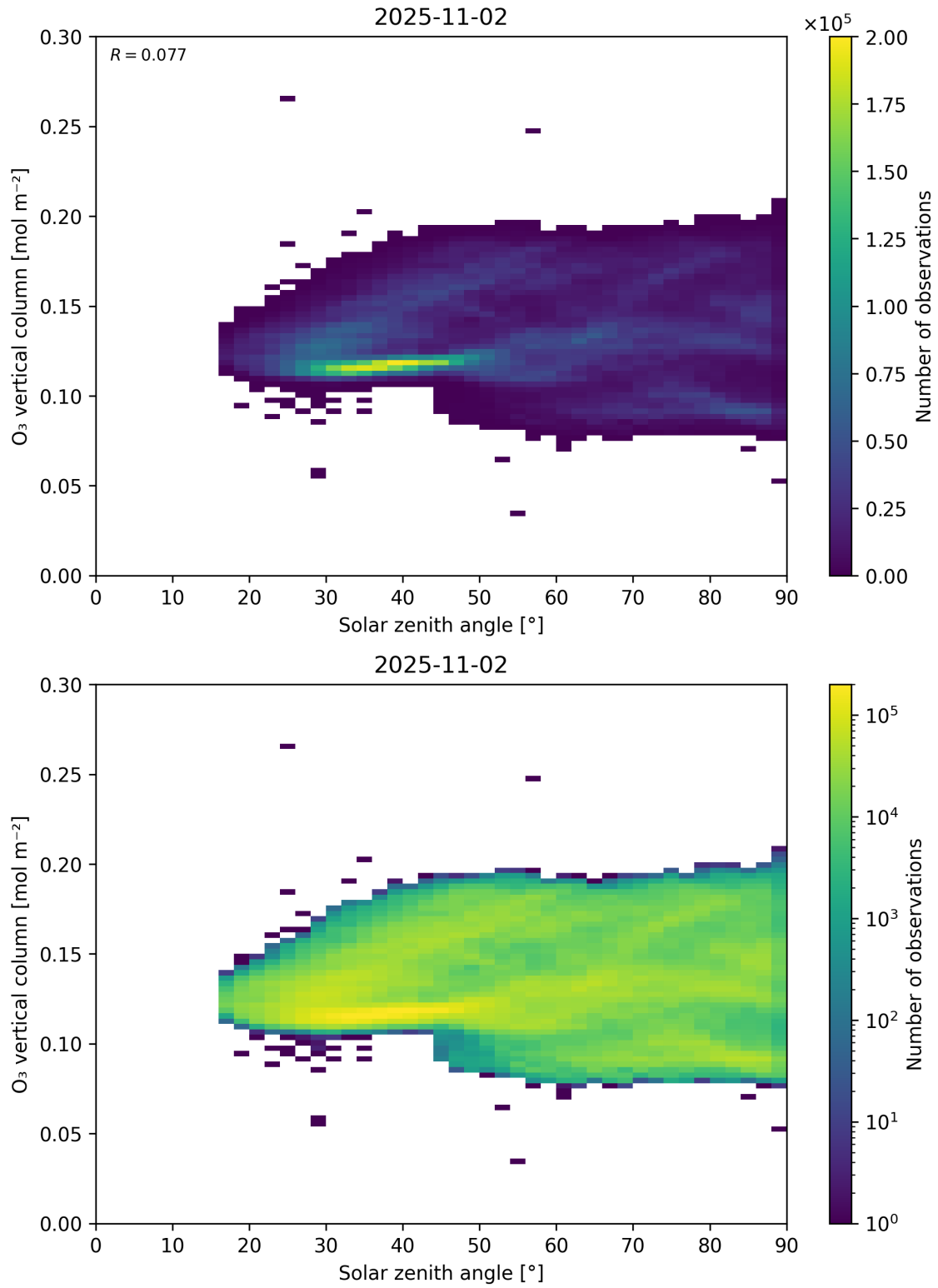
Figure 47: Scatter density plot of “Solar zenith angle” against “O 3 vertical column” for 2025-11-02 to 2025-11-03.
