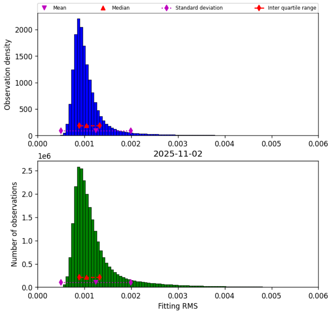
Figure 23: Histogram of “Fitting RMS” for 2025-11-02 to 2025-11-03
