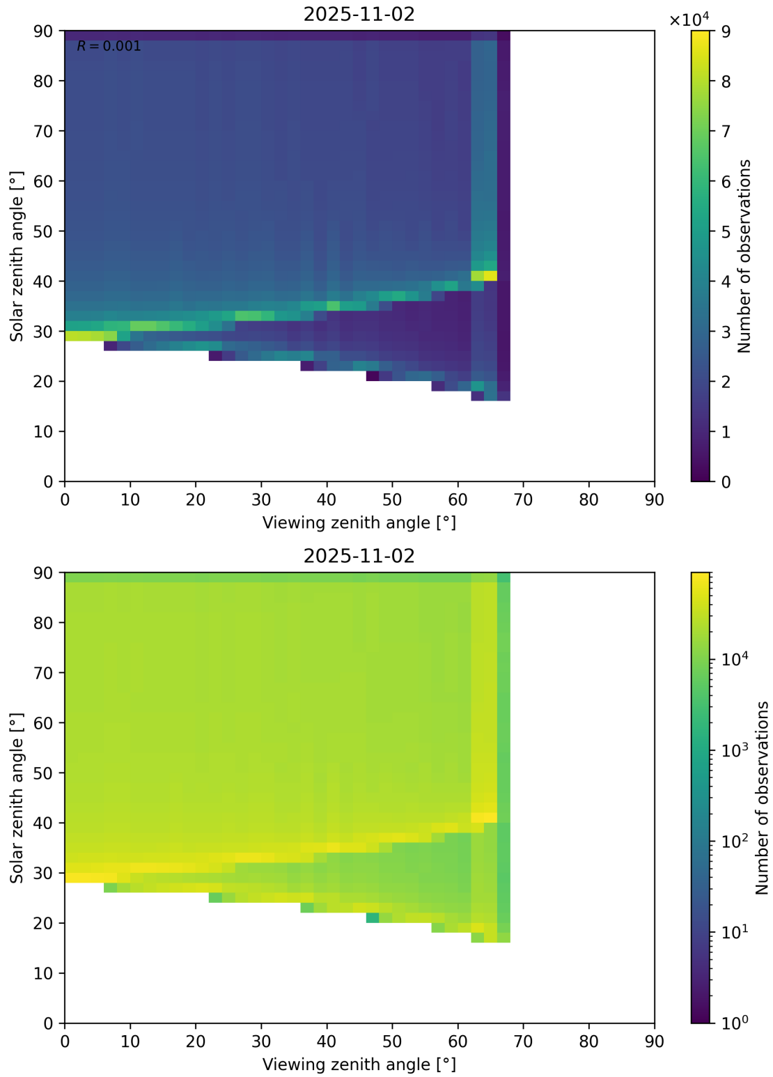
Figure 54: Scatter density plot of “Viewing zenith angle” against “Solar zenith angle” for 2025-11-02 to 2025-11-03.
