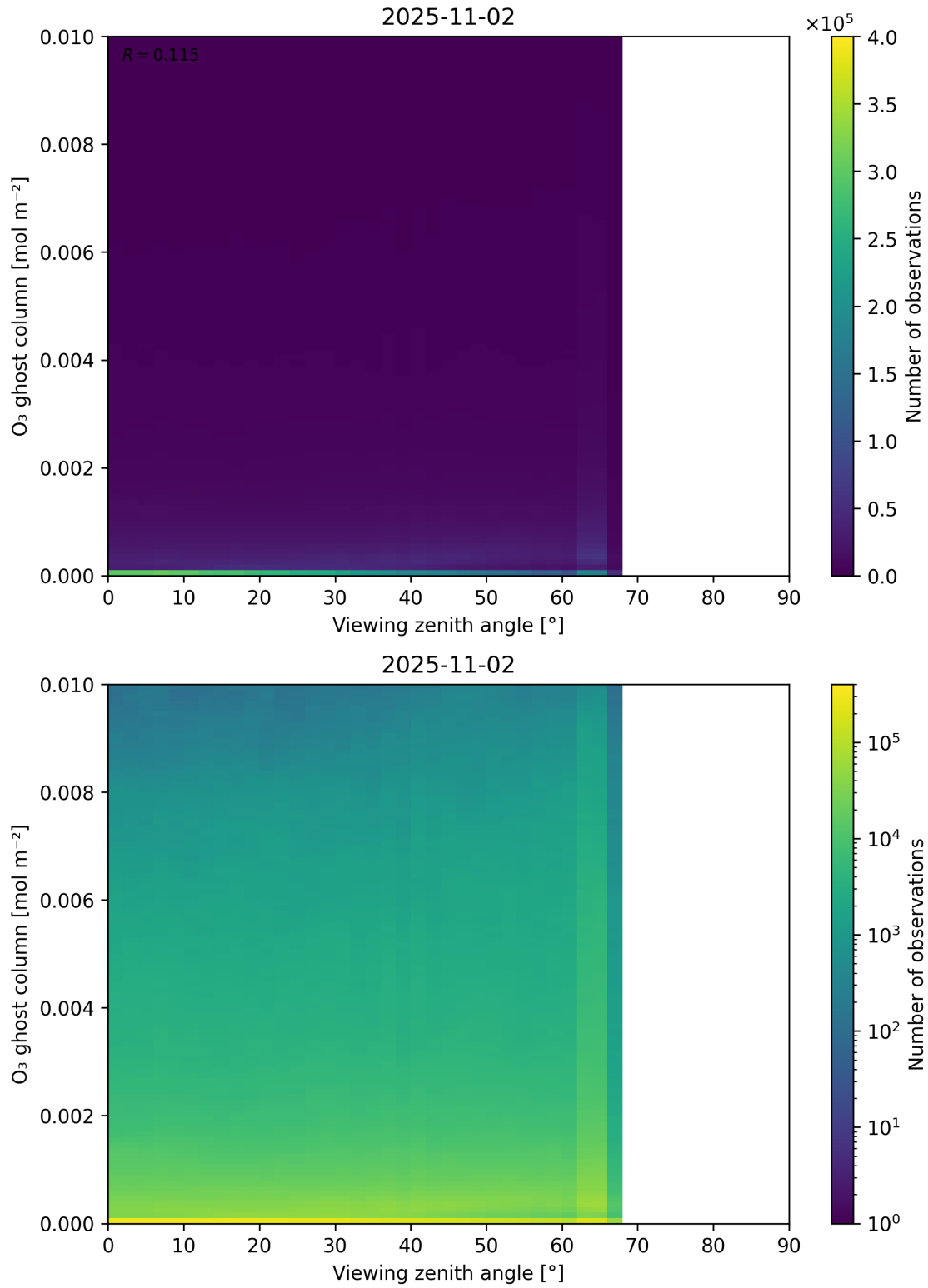
Figure 51: Scatter density plot of “Viewing zenith angle” against “O 3 ghost column” for 2025-11-02 to 2025-11-03.
