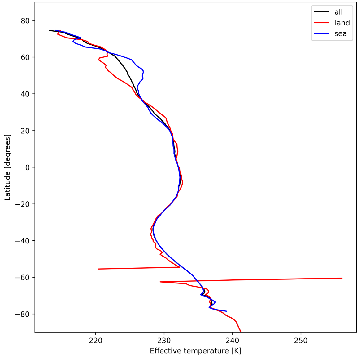
Figure 17: Zonal average of “Effective temperature” for 2025-11-02 to 2025-11-03.
