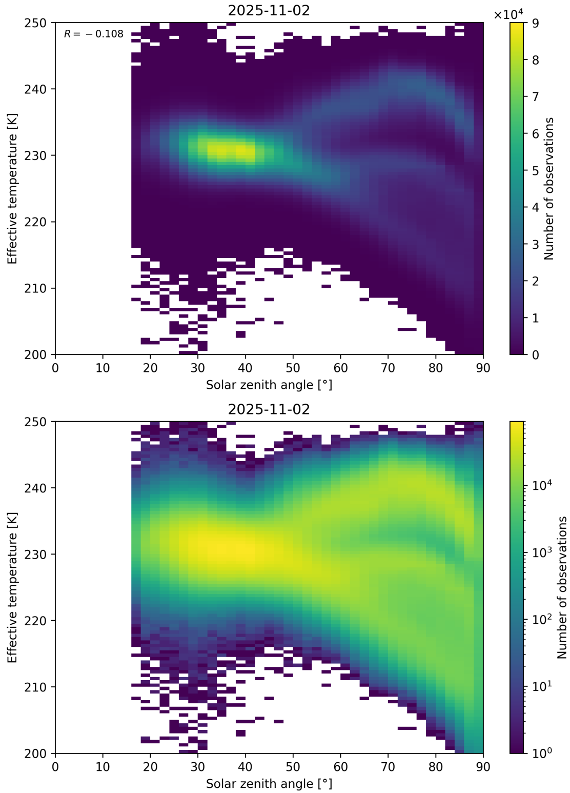
Figure 45: Scatter density plot of “Solar zenith angle” against “Effective temperature” for 2025-11-02 to 2025-11-03.
