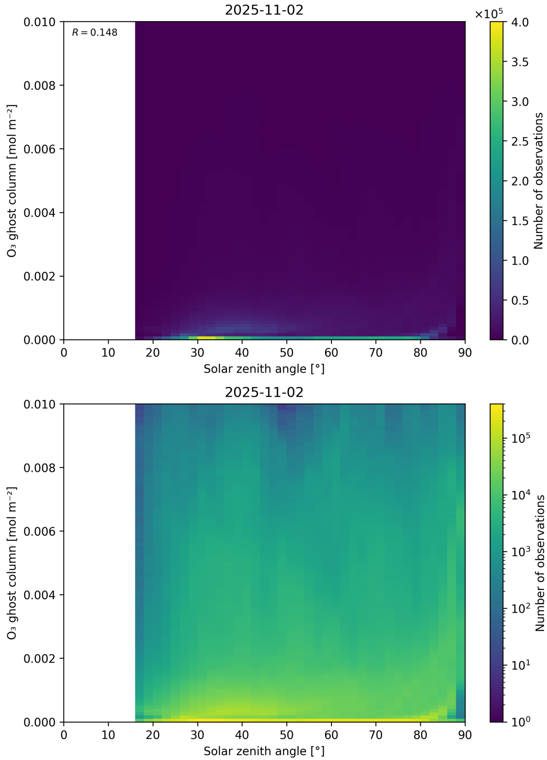
Figure 46: Scatter density plot of “Solar zenith angle” against “O 3 ghost column” for 2025-11-02 to 2025-11-03.
