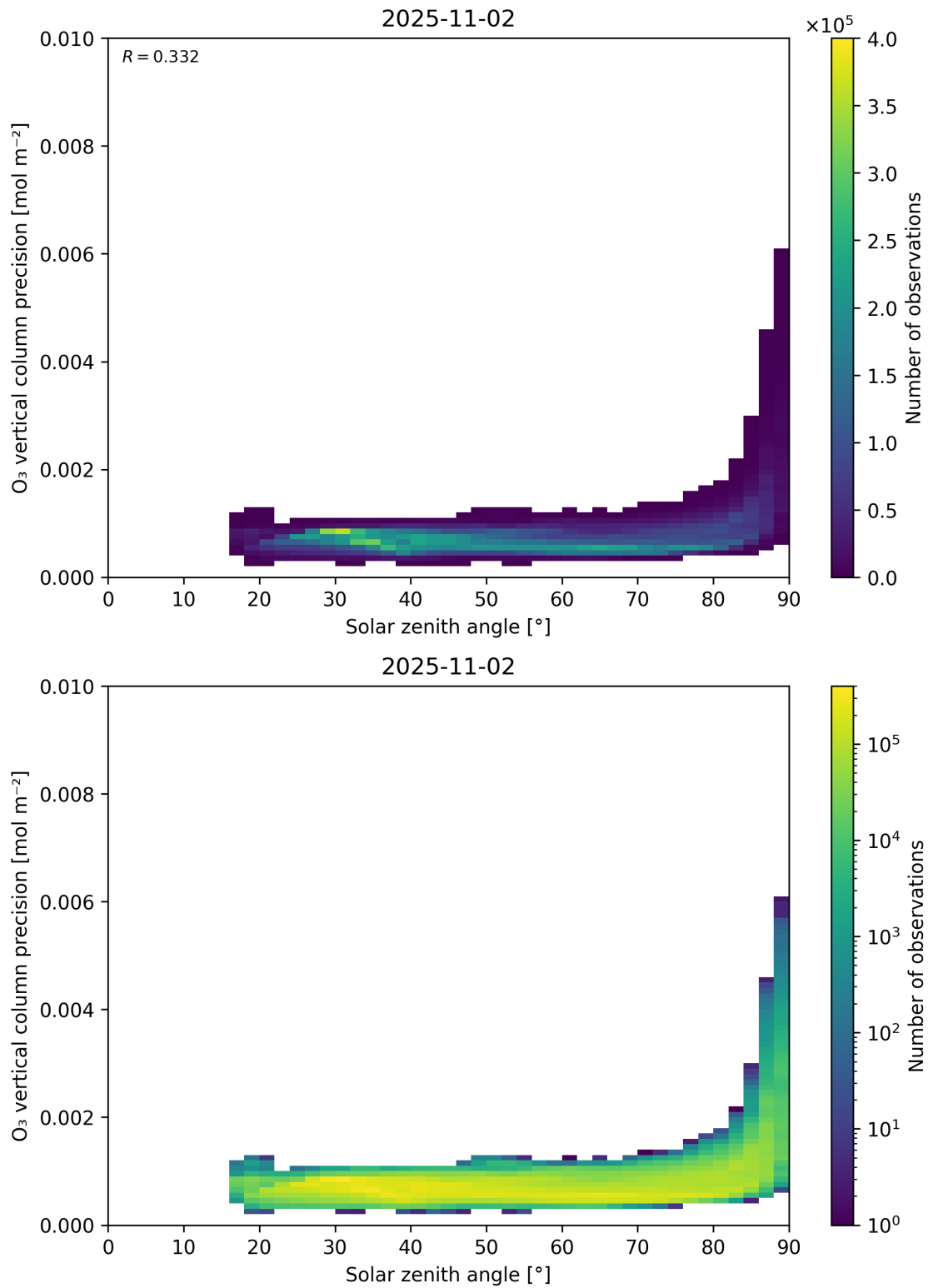
Figure 48: Scatter density plot of “Solar zenith angle” against “O 3 vertical column precision” for 2025-11-02 to 2025-11-03.
