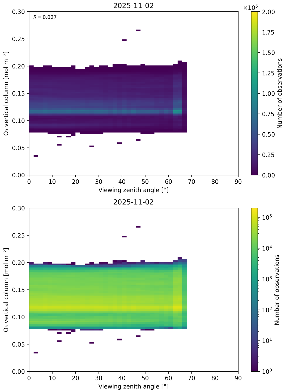
Figure 52: Scatter density plot of “Viewing zenith angle” against “O 3 vertical column” for 2025-11-02 to 2025-11-03.
