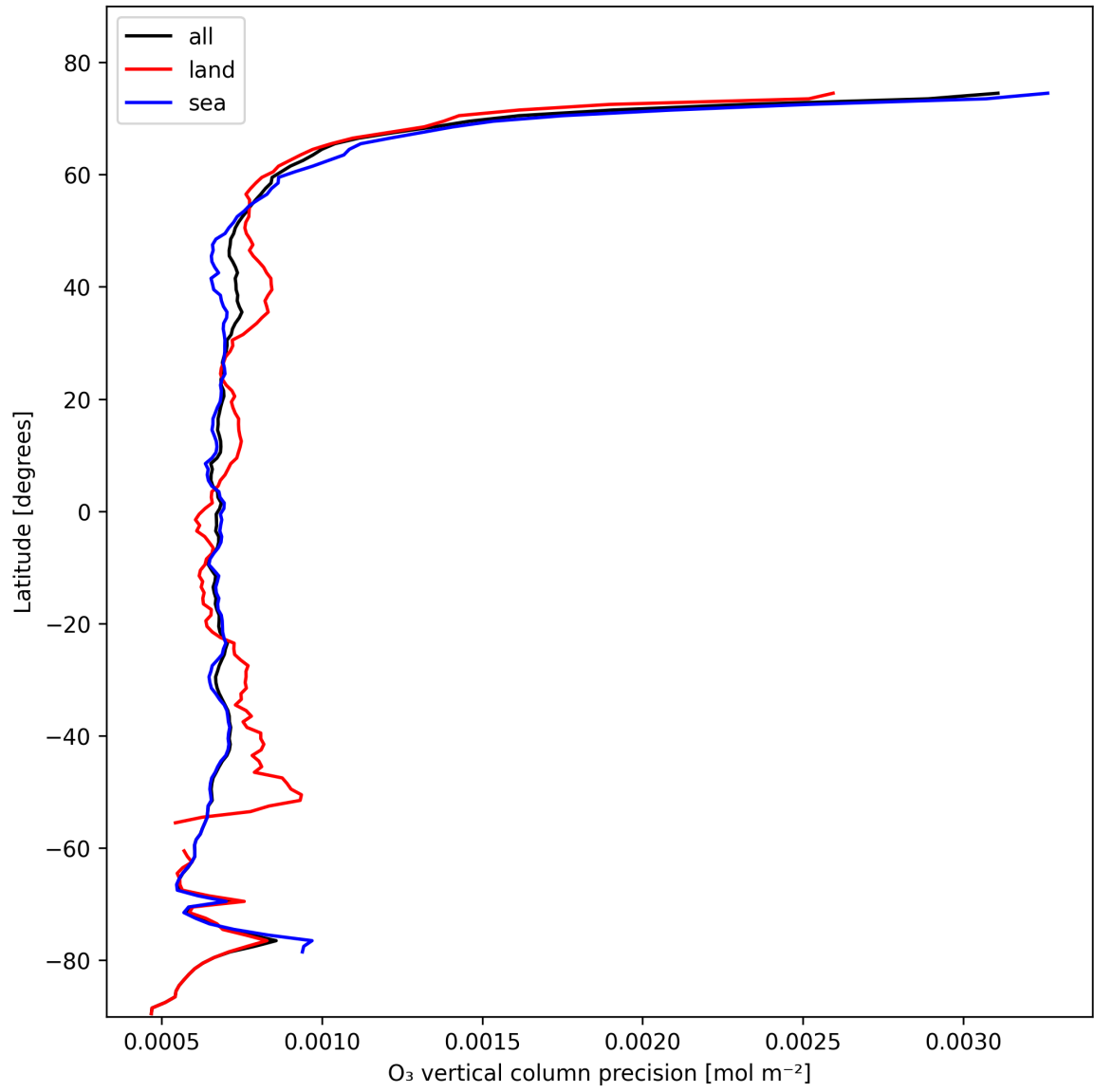
Figure 15: Zonal average of “O 3 vertical column precision” for 2025-11-02 to 2025-11-03.
