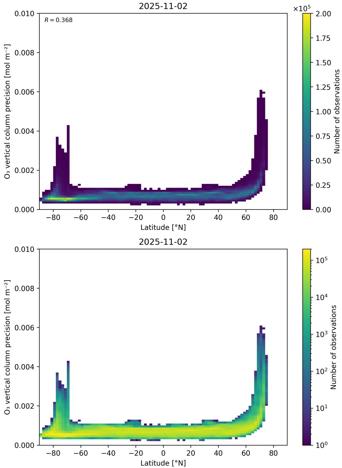
Figure 37: Scatter density plot of “Latitude” against “O 3 vertical column precision” for 2025-11-02 to 2025-11-03.
