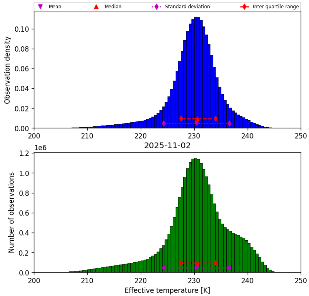
Figure 24: Histogram of “Effective temperature” for 2025-11-02 to 2025-11-03
