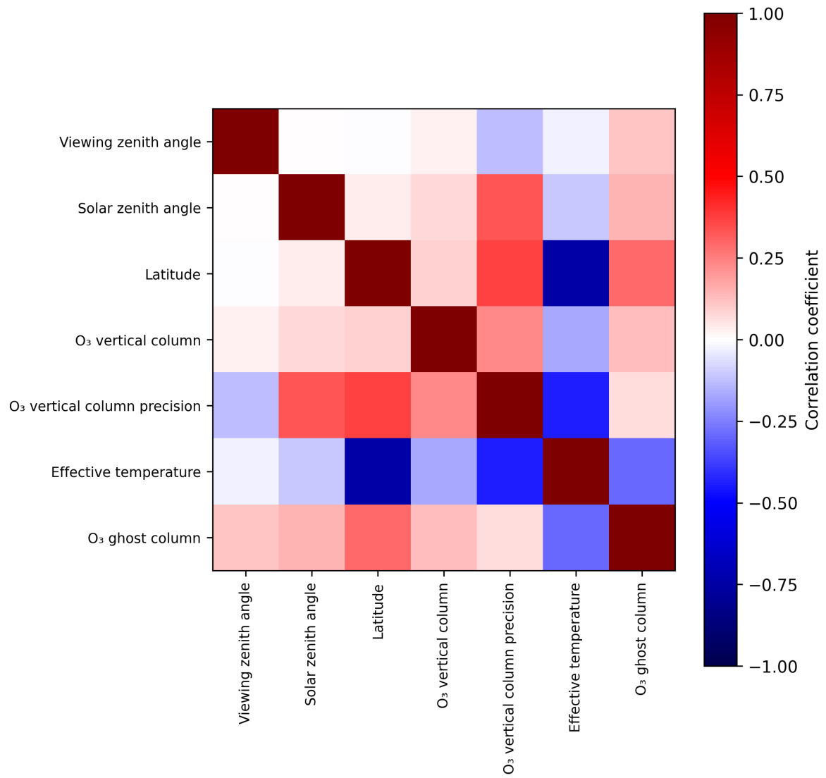
Figure 2: Map of correlation matrix for 2025-11-02 to 2025-11-03.
