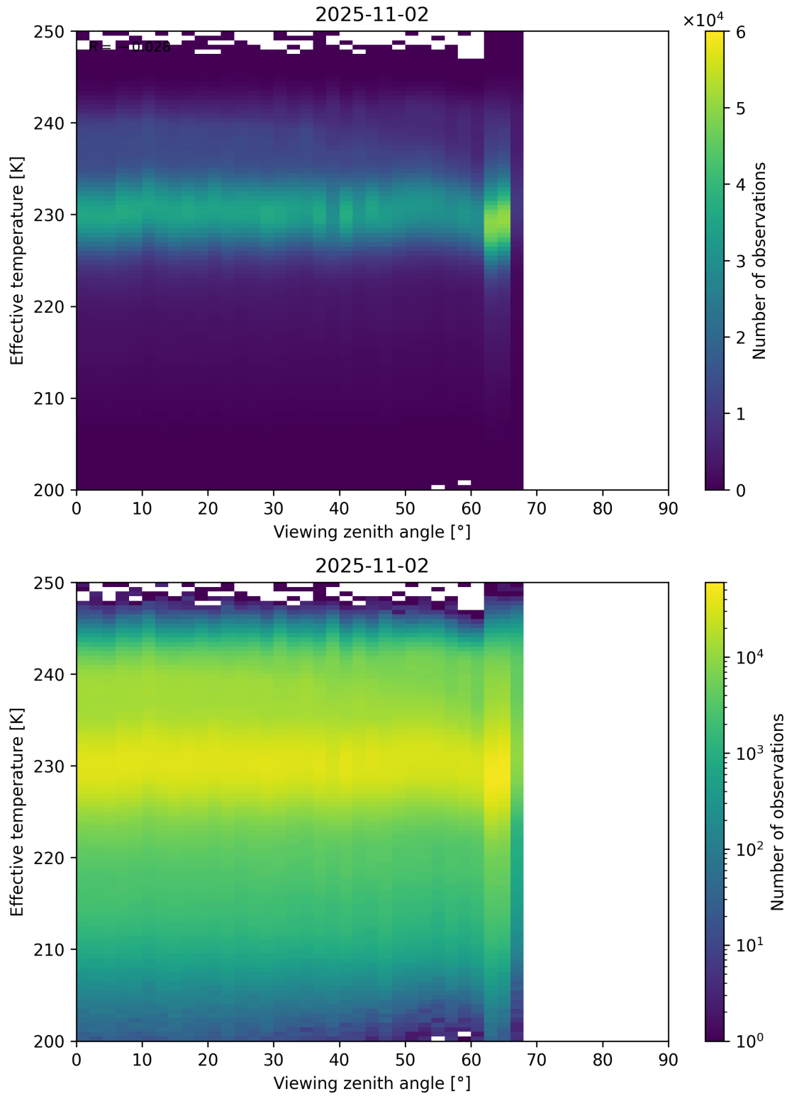
Figure 50: Scatter density plot of “Viewing zenith angle” against “Effective temperature” for 2025-11-02 to 2025-11-03.
