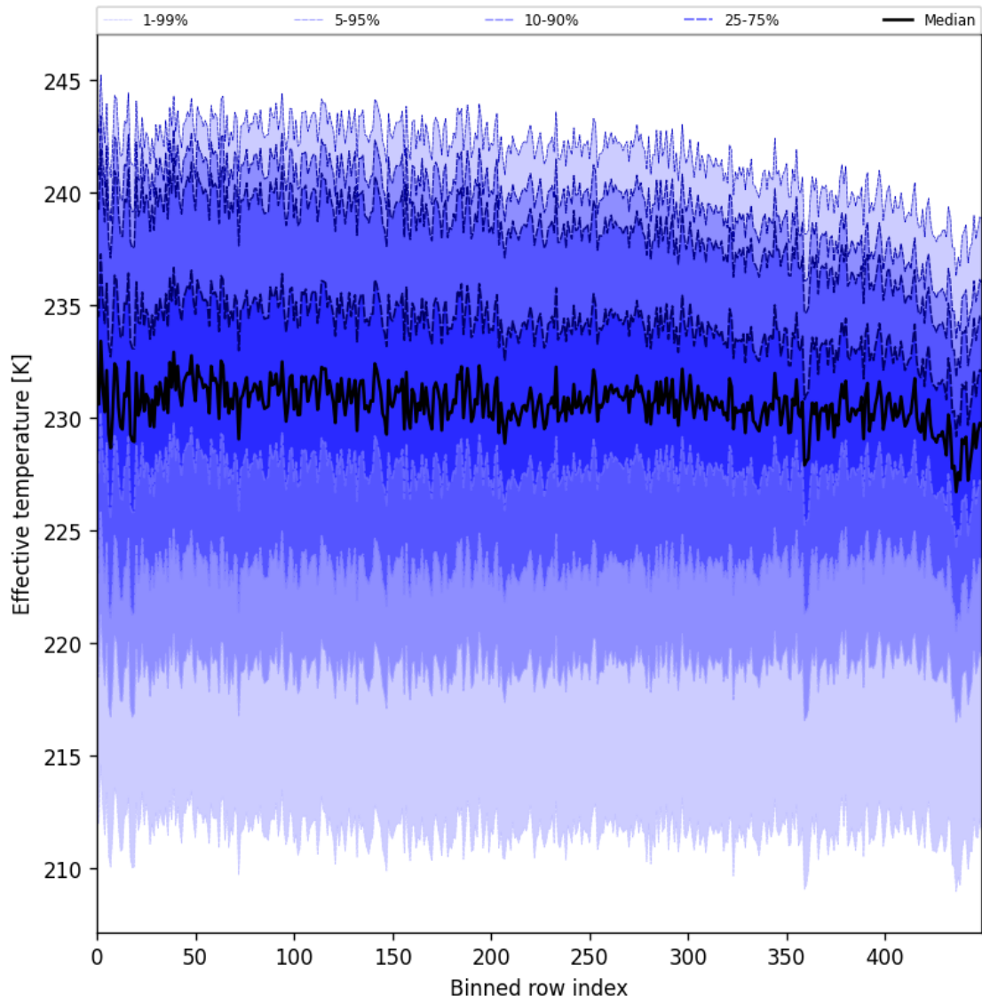
Figure 31: Along track statistics of “Effective temperature” for 2025-11-02 to 2025-11-03
