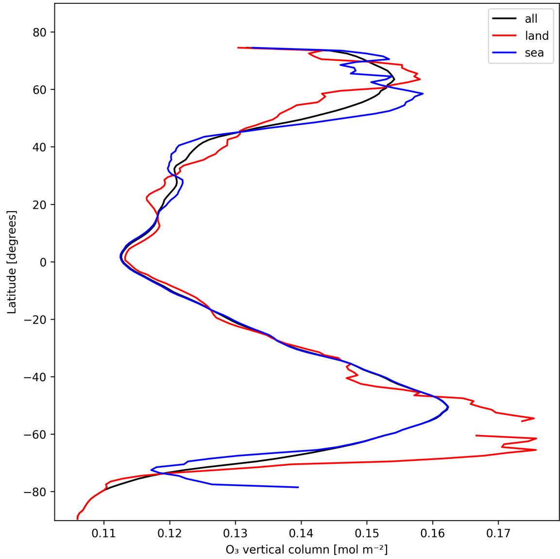
Figure 14: Zonal average of “O 3 vertical column” for 2025-11-02 to 2025-11-03.
