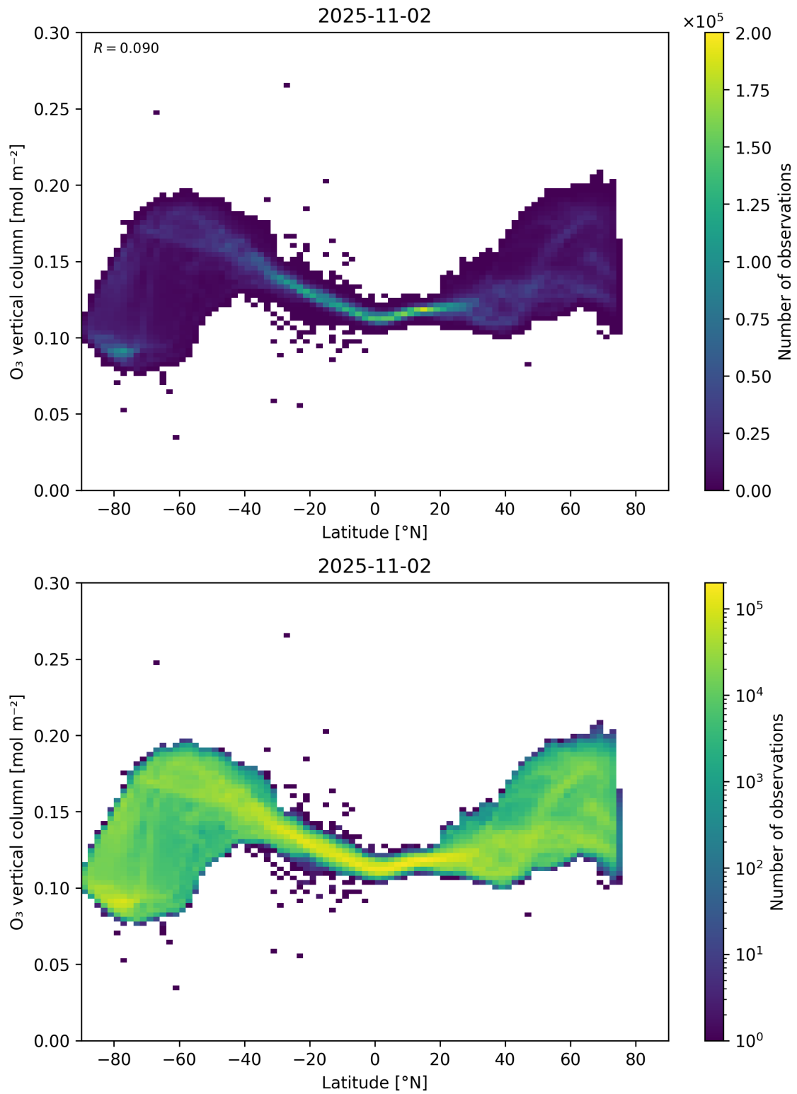
Figure 36: Scatter density plot of “Latitude” against “O 3 vertical column” for 2025-11-02 to 2025-11-03.
