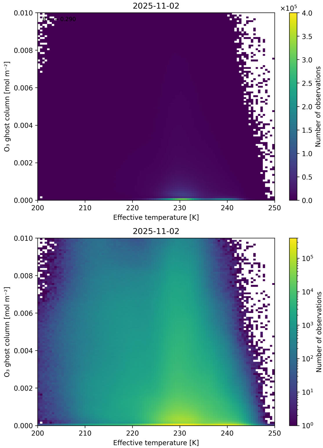
Figure 38: Scatter density plot of “Effective temperature” against “O 3 ghost column” for 2025-11-02 to 2025-11-03.
