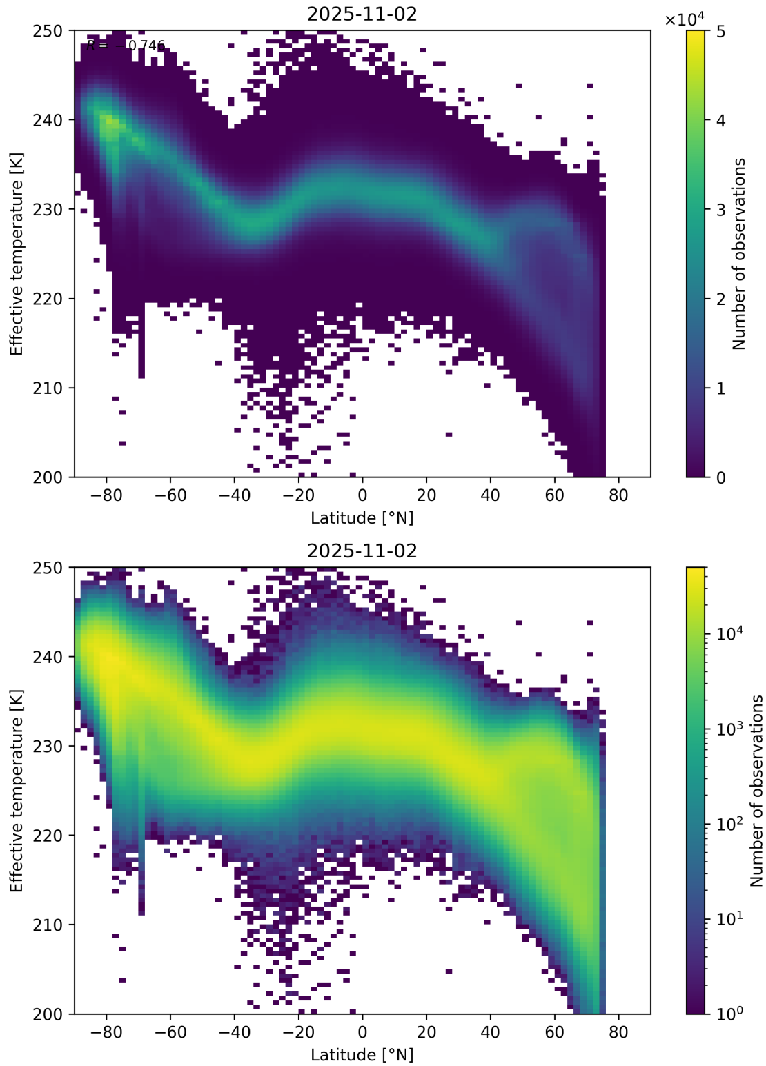
Figure 34: Scatter density plot of “Latitude” against “Effective temperature” for 2025-11-02 to 2025-11-03.
