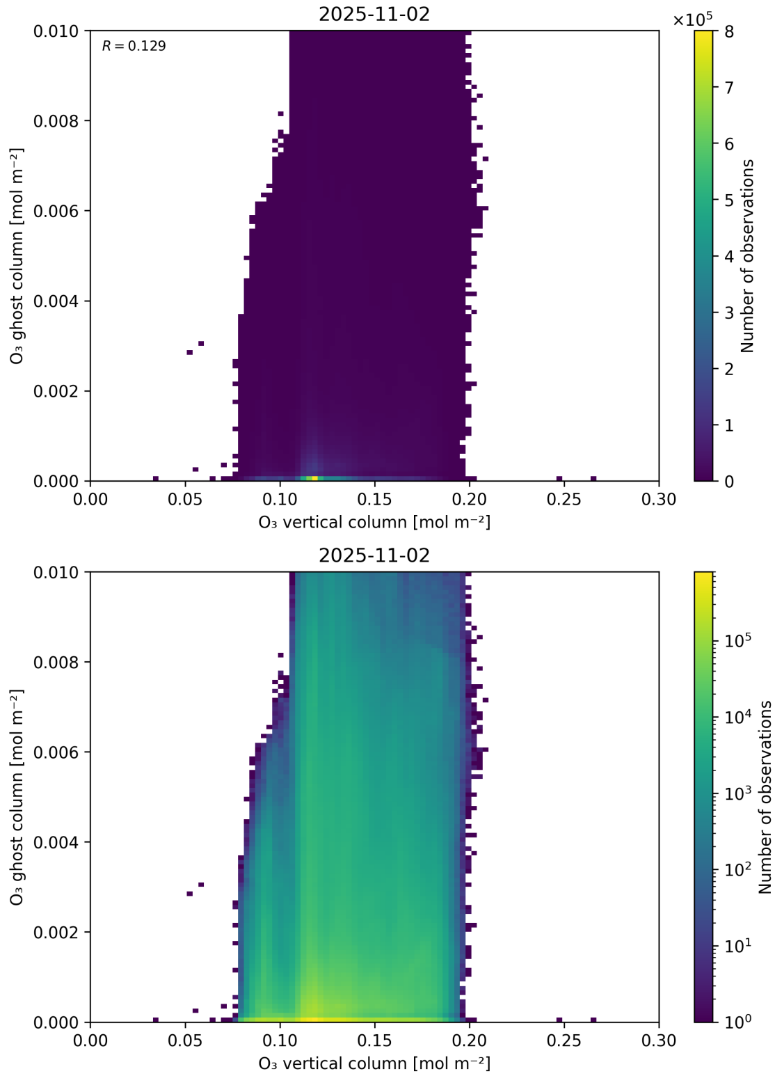
Figure 40: Scatter density plot of “O 3 vertical column” against “O 3 ghost column” for 2025-11-02 to 2025-11-03.
