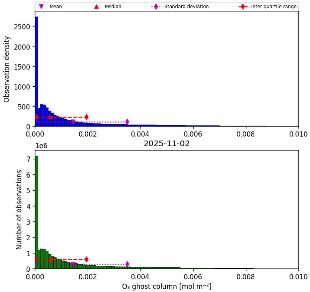
Figure 25: Histogram of “O 3 ghost column” for 2025-11-02 to 2025-11-03
