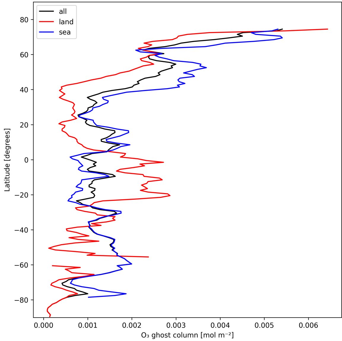
Figure 18: Zonal average of "O 3 ghost column" for 2025-11-02 to 2025-11-03.
