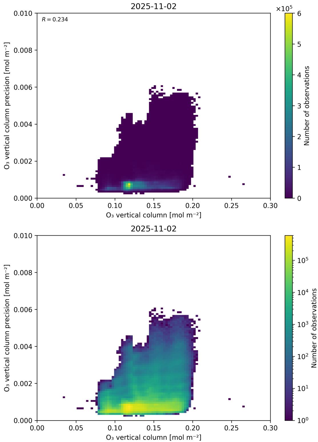
Figure 41: Scatter density plot of “O 3 vertical column” against “O 3 vertical column precision” for 2025-11-02 to 2025-11-03.
