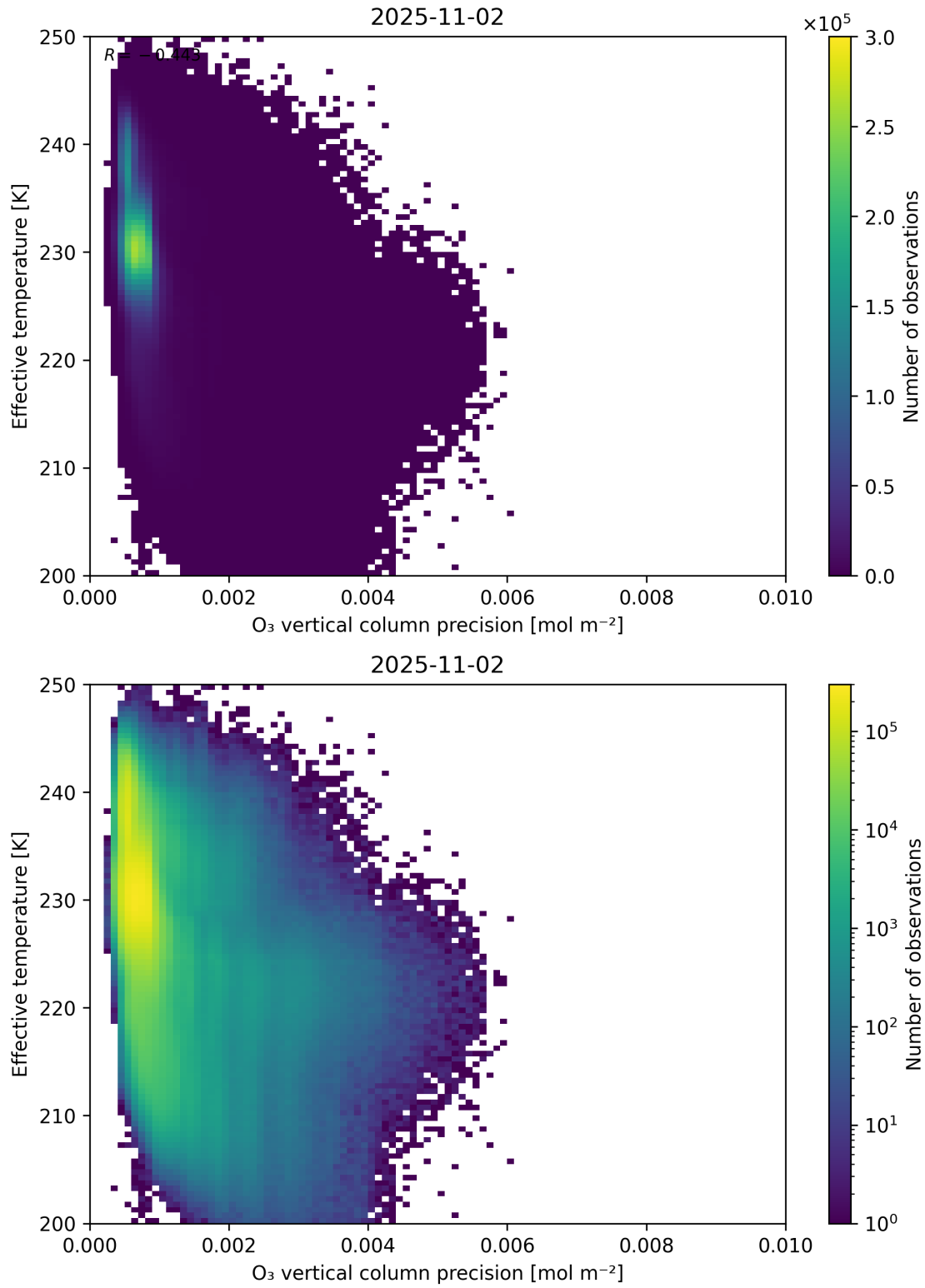
Figure 42: Scatter density plot of “ O_3 vertical column precision” against “Effective temperature” for 2025-11-02 to 2025-11-03.
