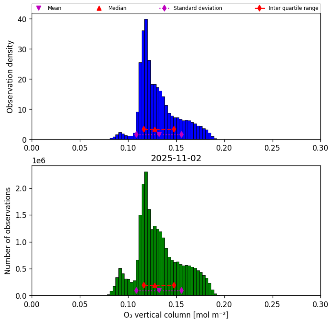
Figure 21: Histogram of “O 3 vertical column” for 2025-11-02 to 2025-11-03
