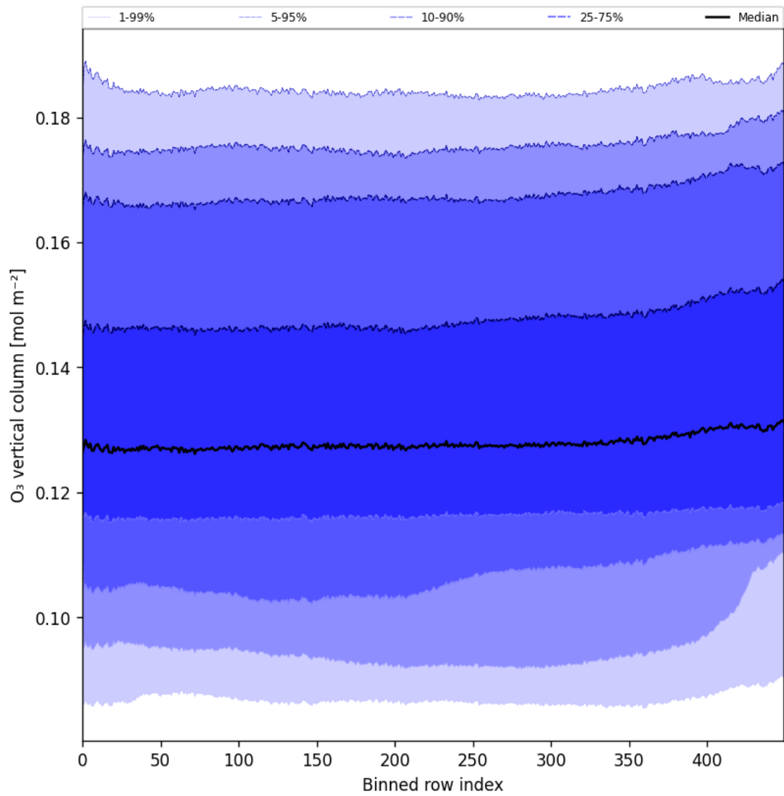
Figure 28: Along track statistics of “O 3 vertical column” for 2025-11-02 to 2025-11-03
