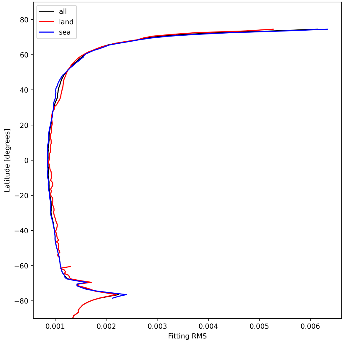
Figure 16: Zonal average of “Fitting RMS” for 2025-11-02 to 2025-11-03.
