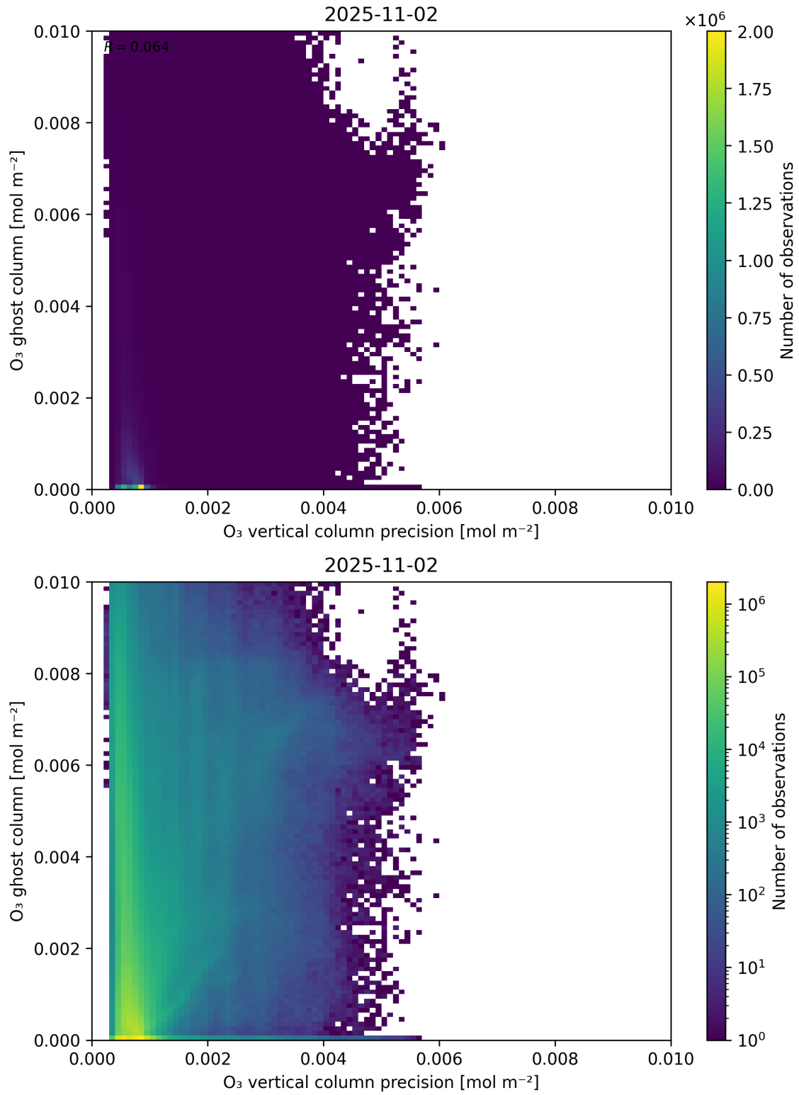
Figure 43: Scatter density plot of “O 3 vertical column precision” against “O 3 ghost column” for 2025-11-02 to 2025-11-03.
