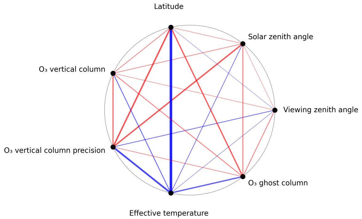
Figure 1: Map of correlation graph for 2025-11-02 to 2025-11-03.
