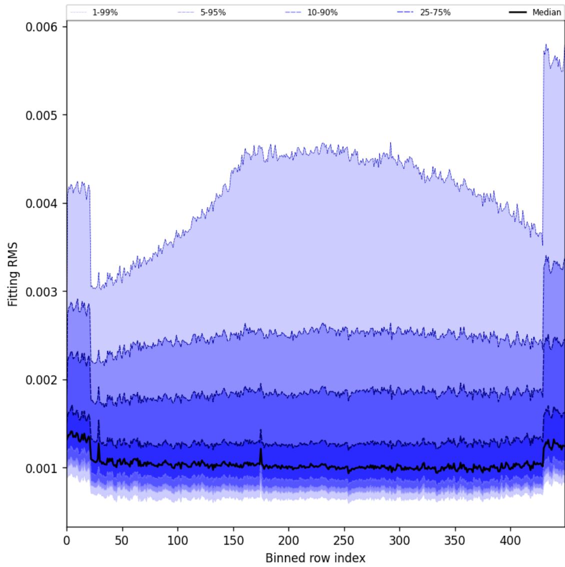
Figure 30: Along track statistics of “Fitting RMS” for 2025-11-02 to 2025-11-03
