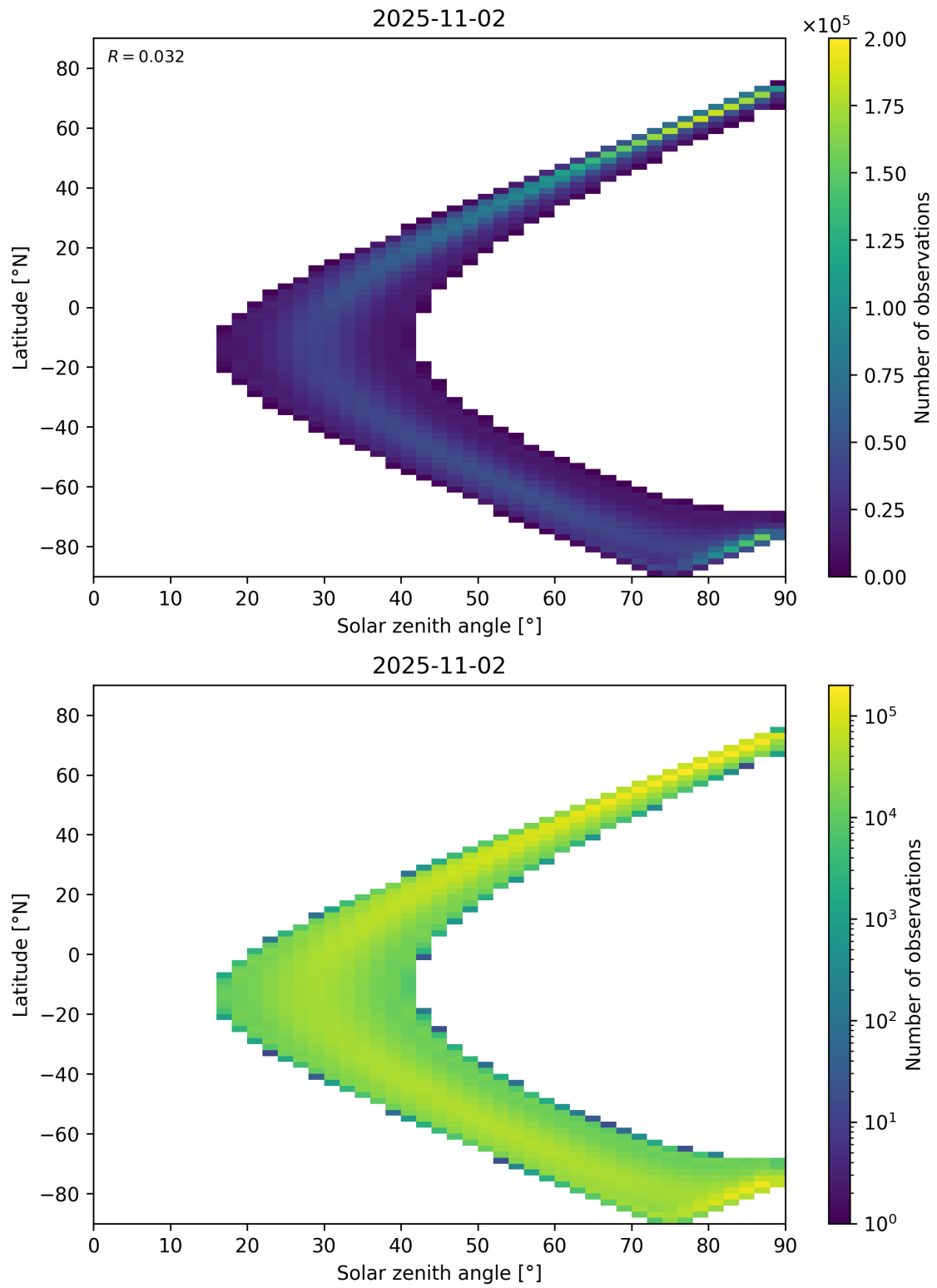
Figure 44: Scatter density plot of “Solar zenith angle” against “Latitude” for 2025-11-02 to 2025-11-03.
