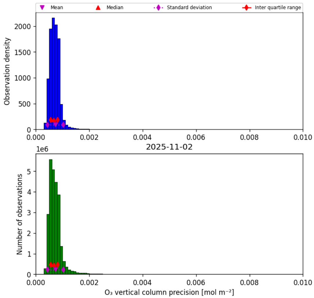
Figure 22: Histogram of “O 3 vertical column precision” for 2025-11-02 to 2025-11-03
