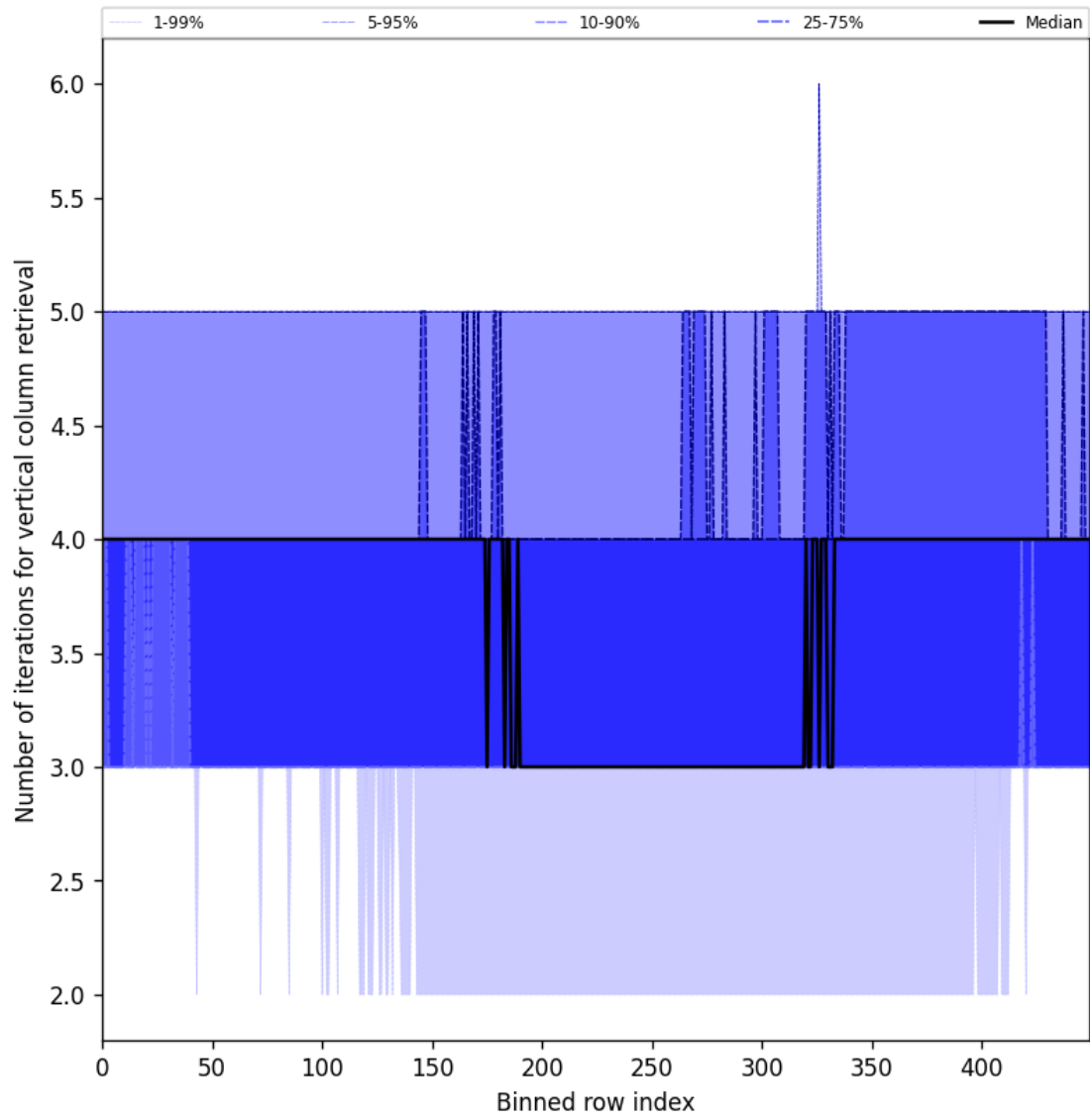
Figure 33: Along track statistics of “Number of iterations for vertical column retrieval” for 2025-11-02 to 2025-11-03
