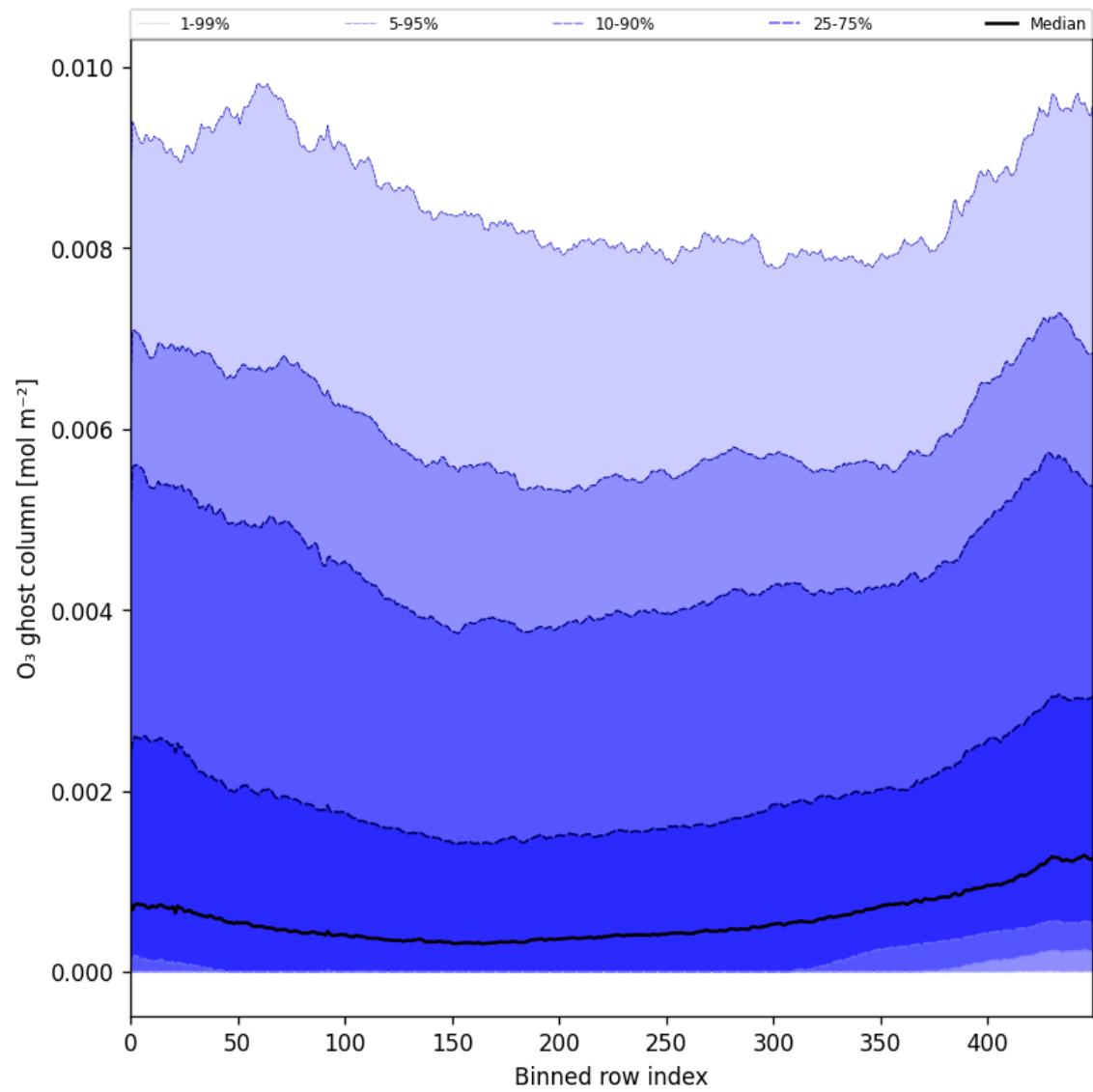
Figure 32: Along track statistics of "O 3 ghost column" for 2025-11-02 to 2025-11-03
