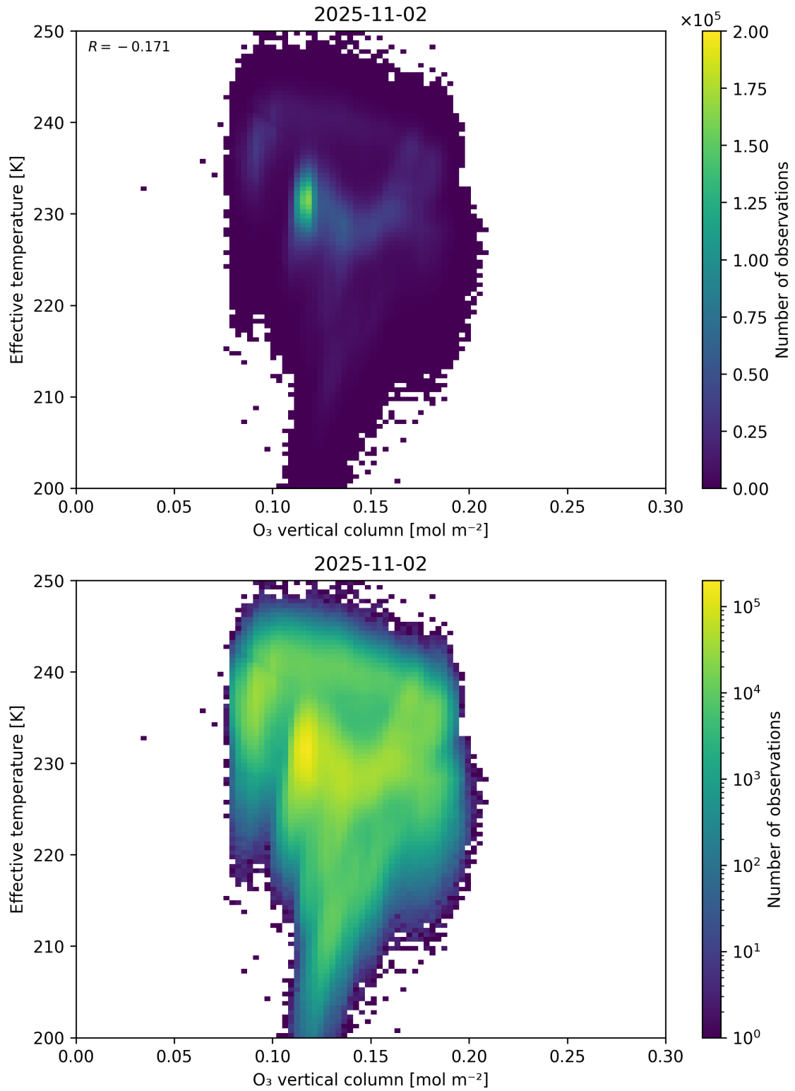
Figure 39: Scatter density plot of “O 3 vertical column” against “Effective temperature” for 2025-11-02 to 2025-11-03.
