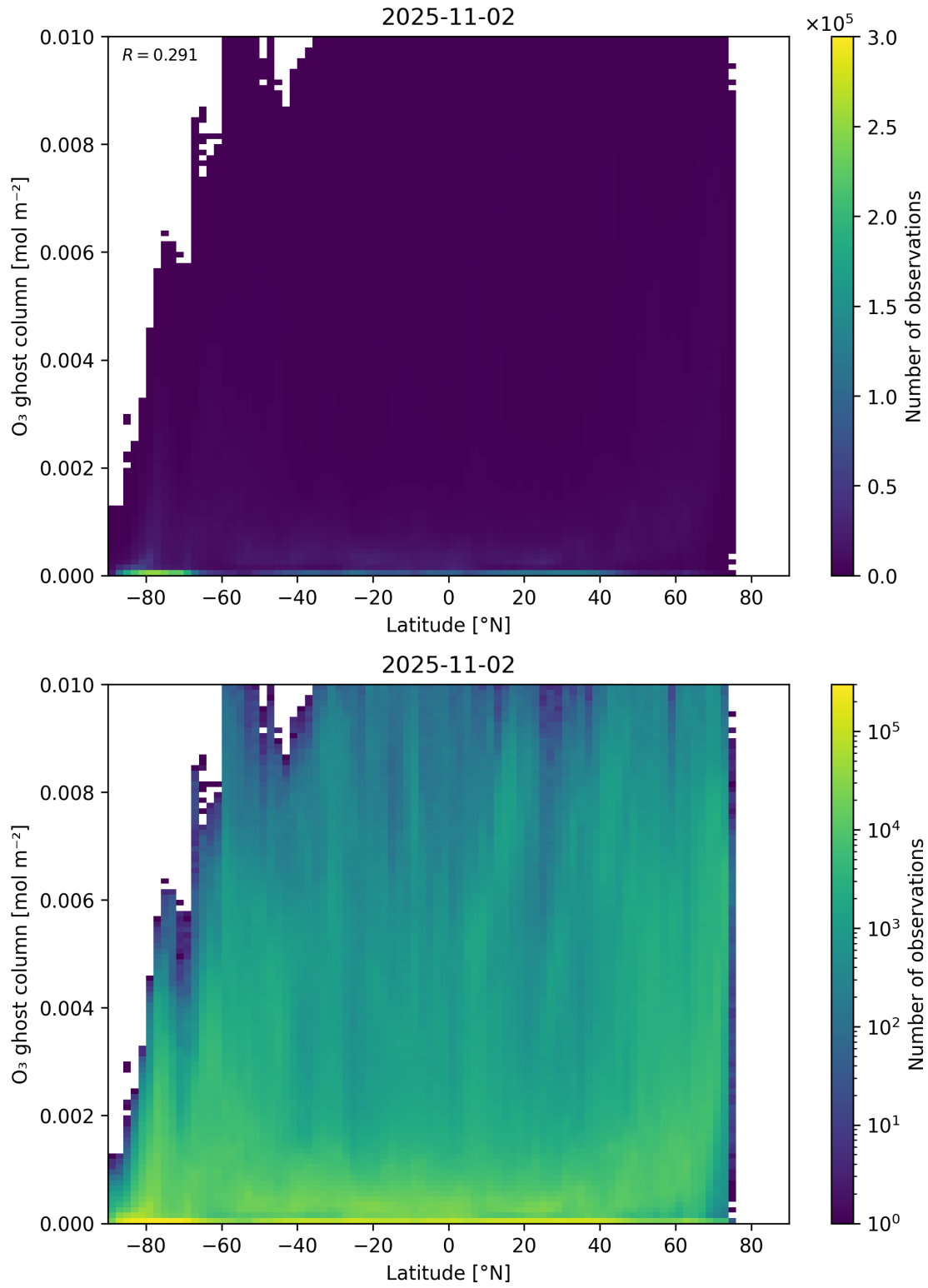
Figure 35: Scatter density plot of “Latitude” against “O 3 ghost column” for 2025-11-02 to 2025-11-03.
