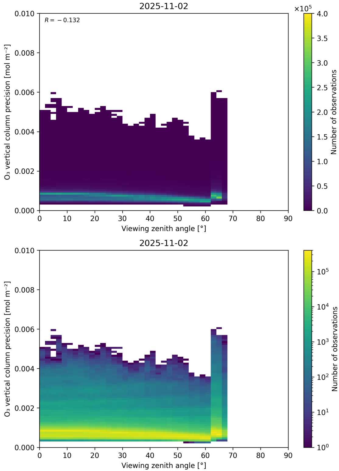
Figure 53: Scatter density plot of “Viewing zenith angle” against “O 3 vertical column precision” for 2025-11-02 to 2025-11-03.
