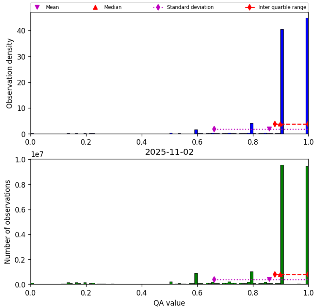
Figure 20: Histogram of “QA value” for 2025-11-02 to 2025-11-03
