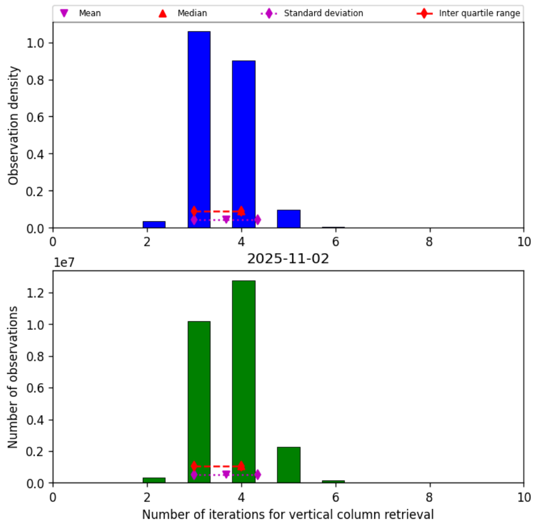
Figure 26: Histogram of “Number of iterations for vertical column retrieval” for 2025-11-02 to 2025-11-03
