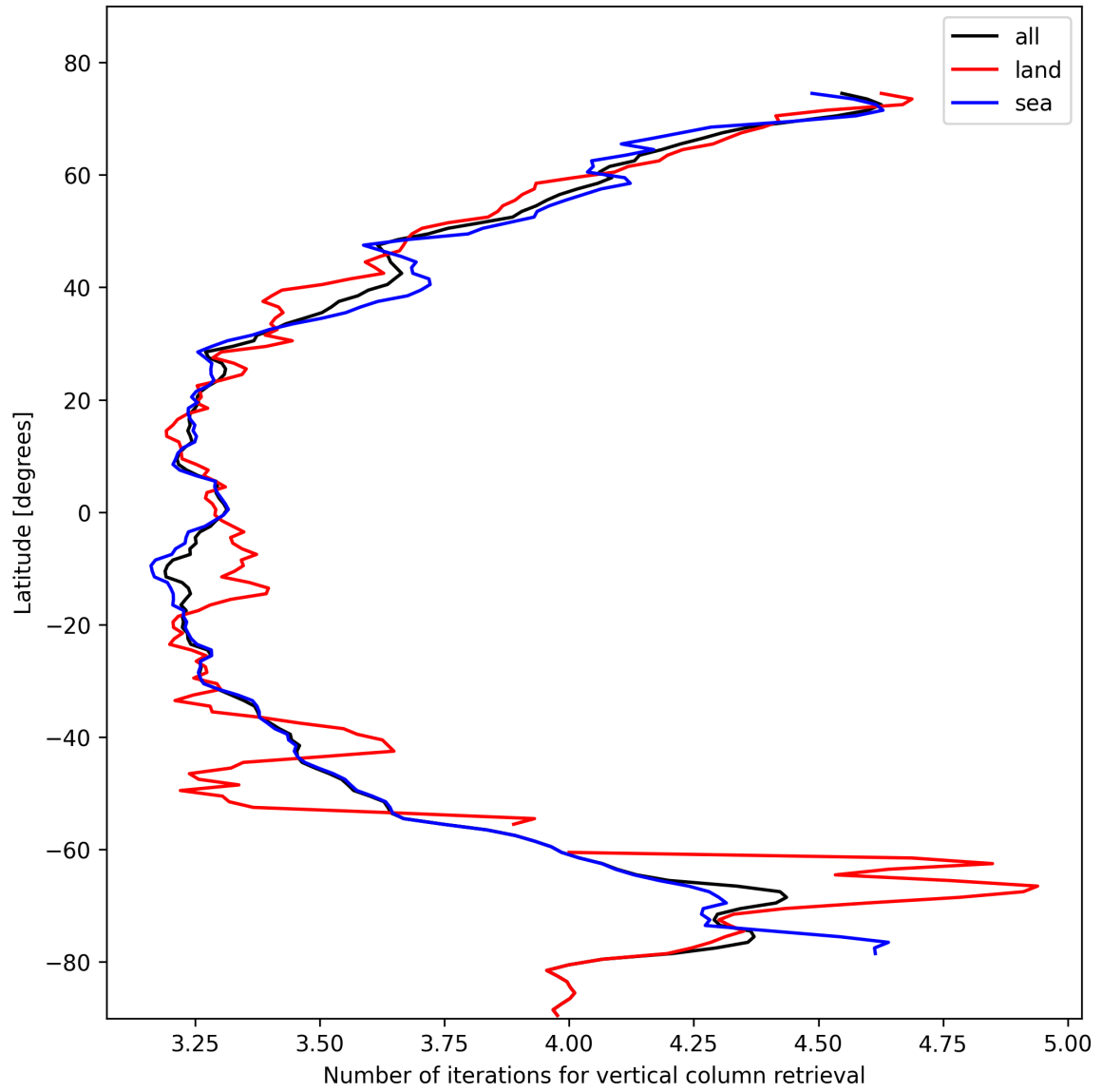
Figure 19: Zonal average of “Number of iterations for vertical column retrieval” for 2025-11-02 to 2025-11-03.
