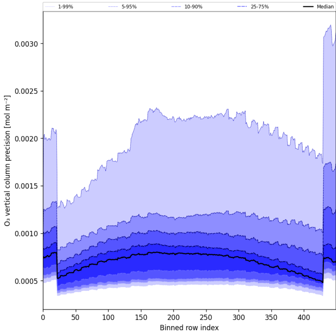
Figure 29: Along track statistics of “O 3 vertical column precision” for 2025-11-02 to 2025-11-03
