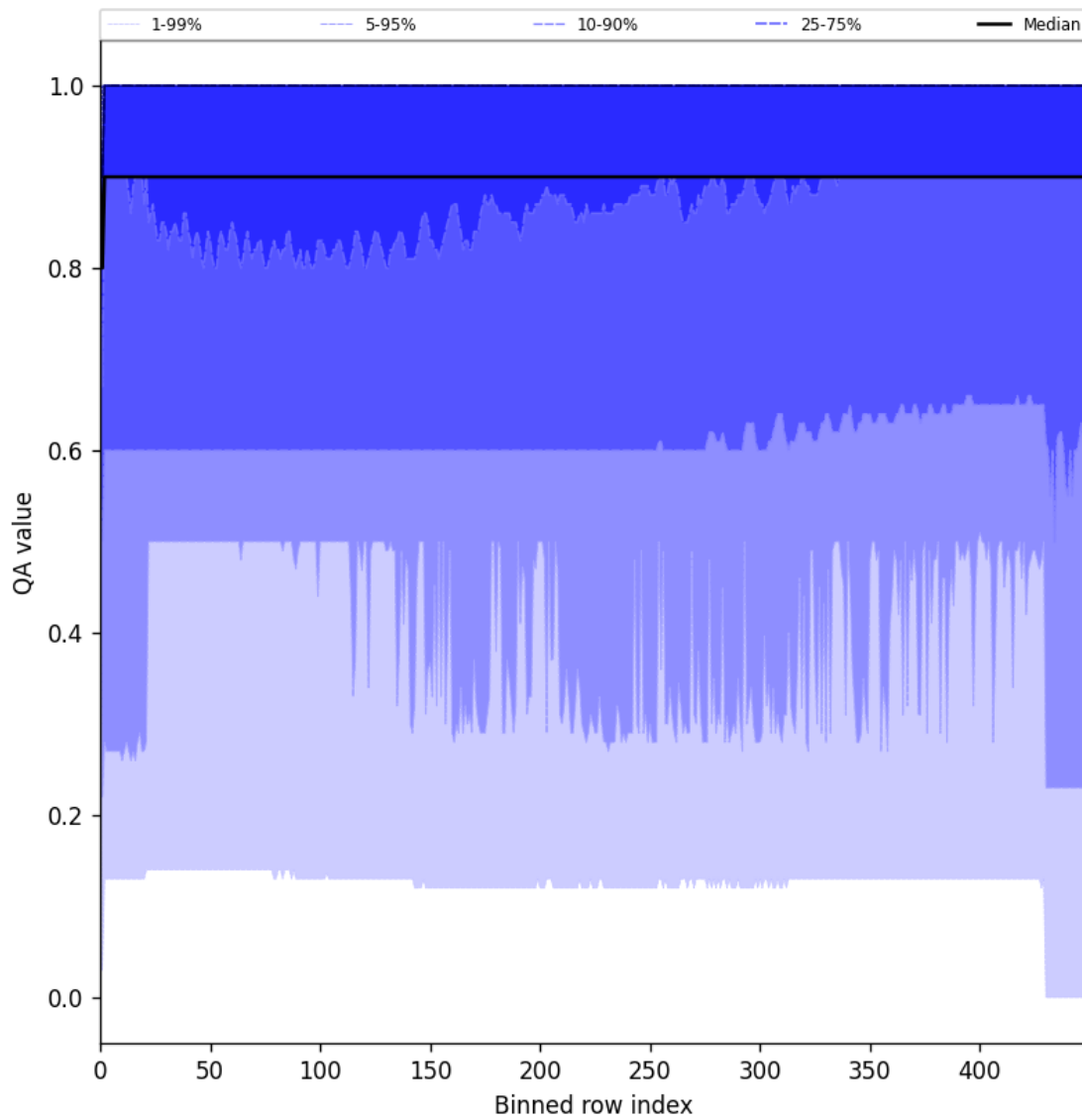
Figure 27: Along track statistics of “QA value” for 2025-11-02 to 2025-11-03
