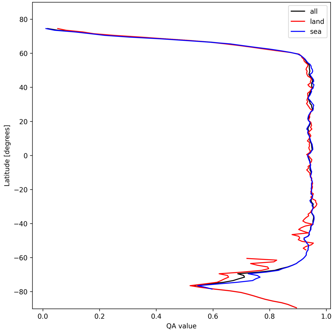
Figure 13: Zonal average of “QA value” for 2025-11-02 to 2025-11-03.
