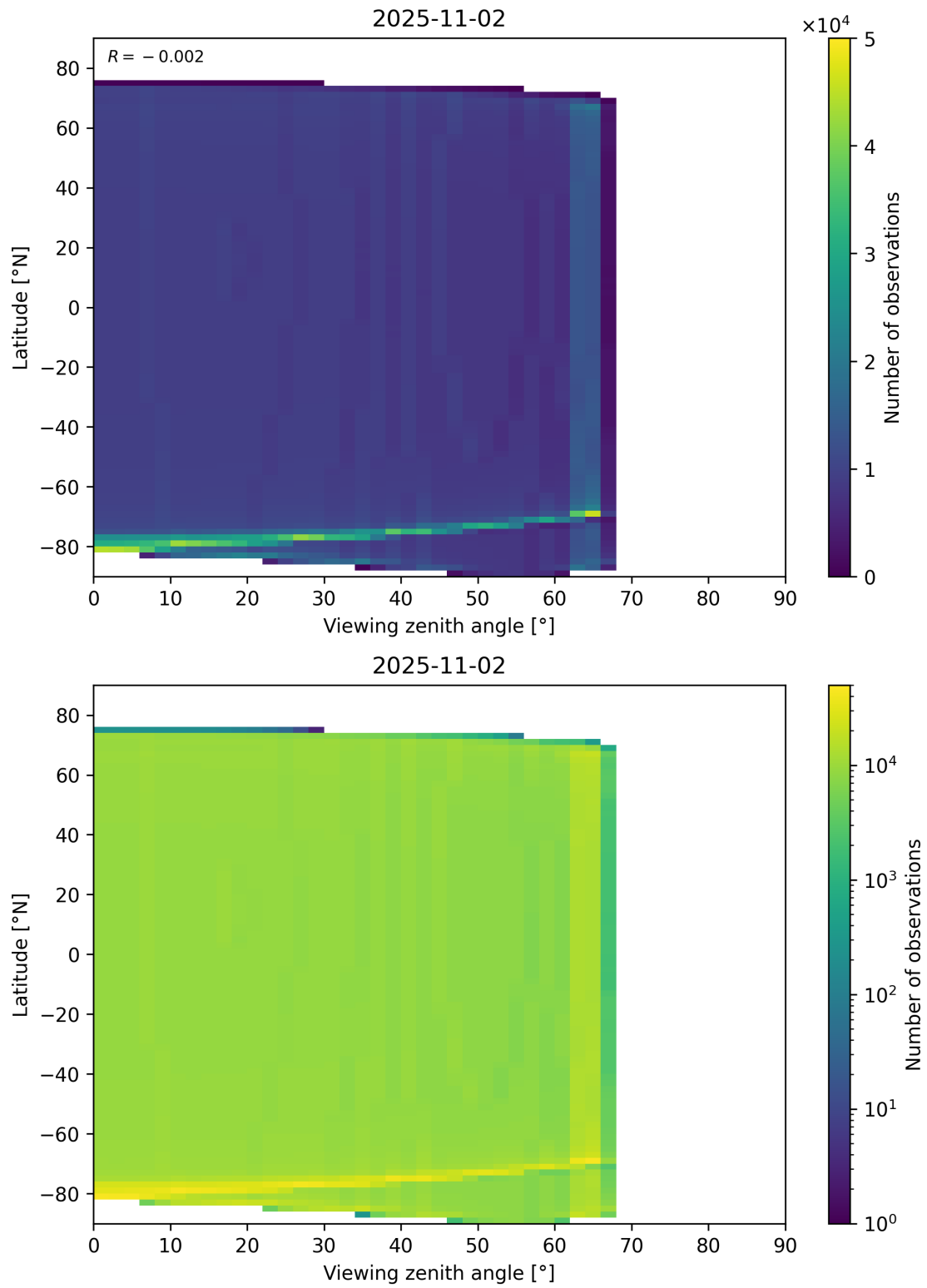
Figure 49: Scatter density plot of “Viewing zenith angle” against “Latitude” for 2025-11-02 to 2025-11-03.
