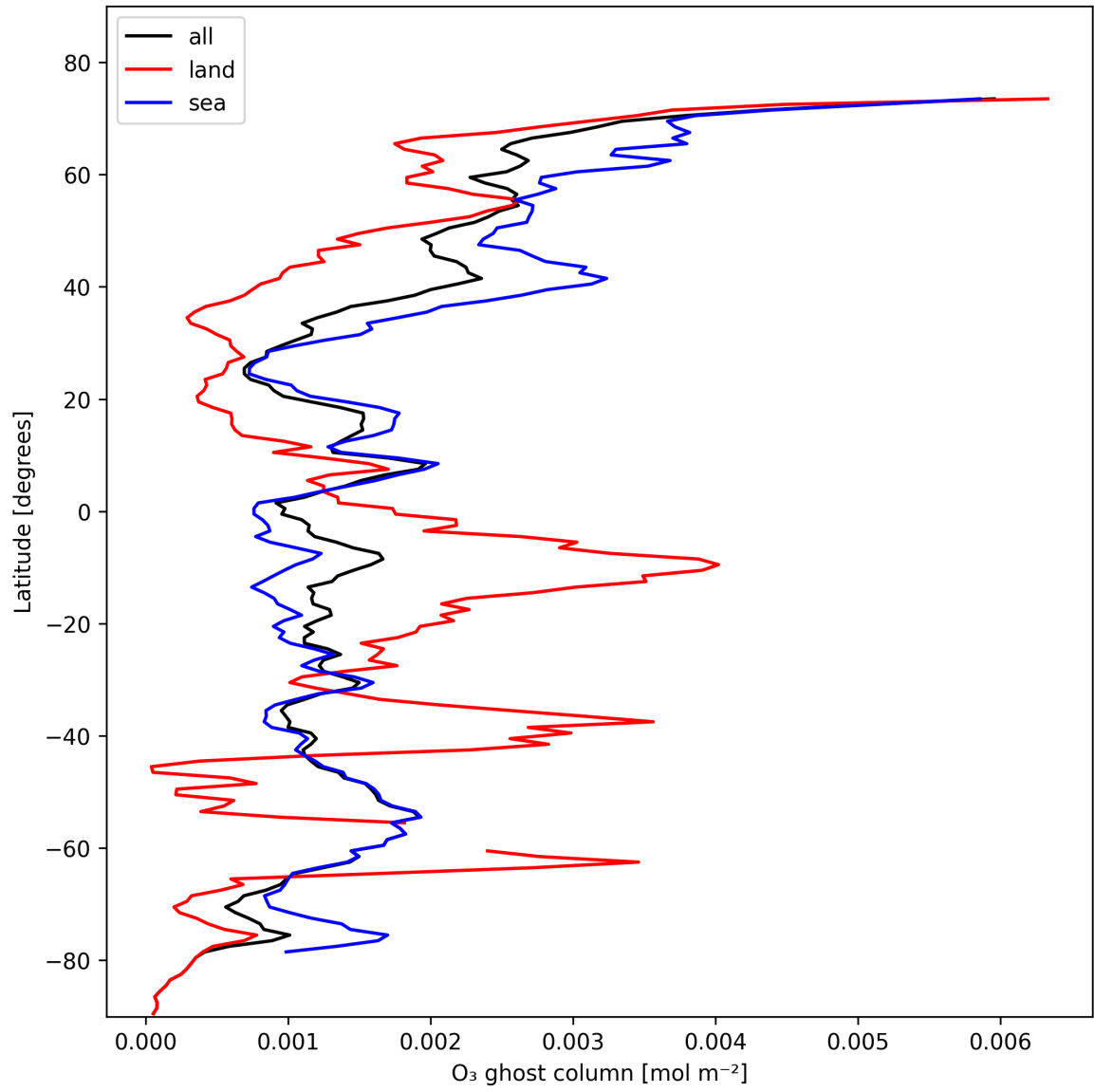
Figure 18: Zonal average of "O 3 ghost column" for 2025-11-02 to 2025-11-04.
