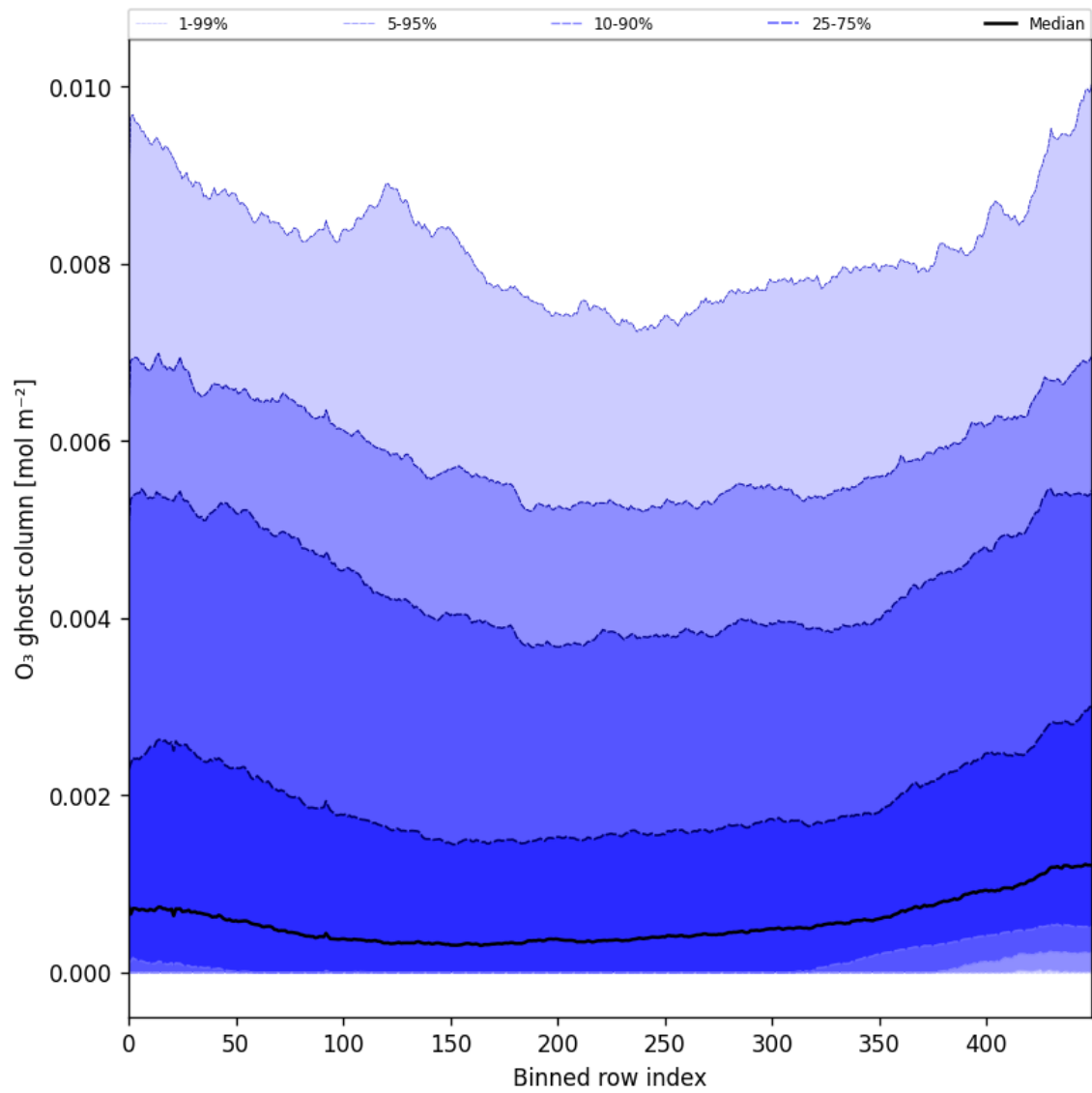
Figure 32: Along track statistics of “O 3 ghost column” for 2025-11-02 to 2025-11-04
