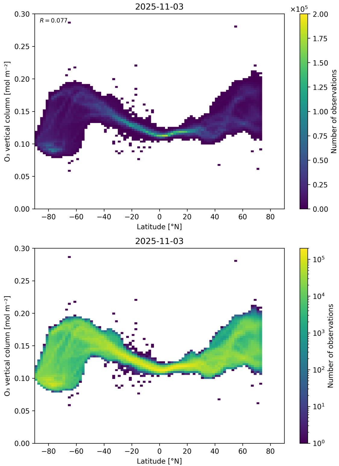
Figure 36: Scatter density plot of “Latitude” against “O 3 vertical column” for 2025-11-02 to 2025-11-04.
