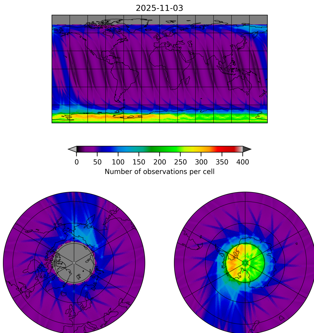
Figure 12: Map of the number of observations for 2025-11-02 to 2025-11-04
