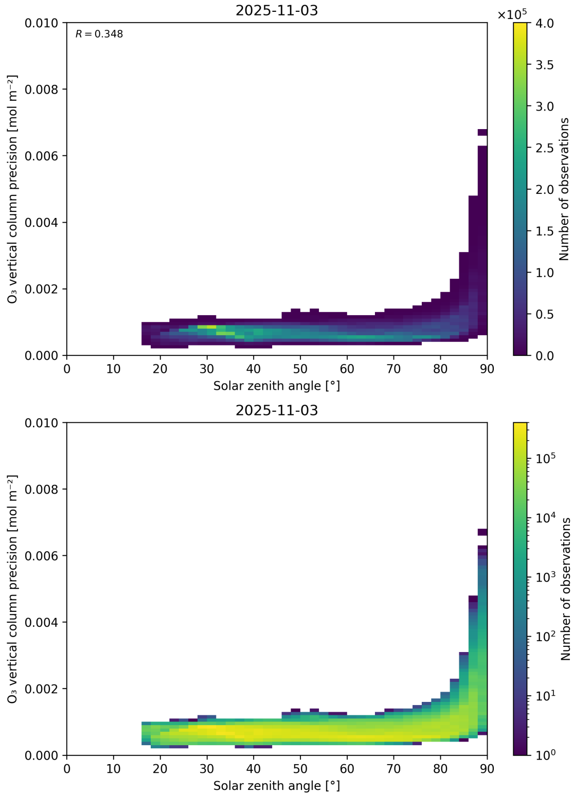
Figure 48: Scatter density plot of “Solar zenith angle” against “O 3 vertical column precision” for 2025-11-02 to 2025-11-04.
