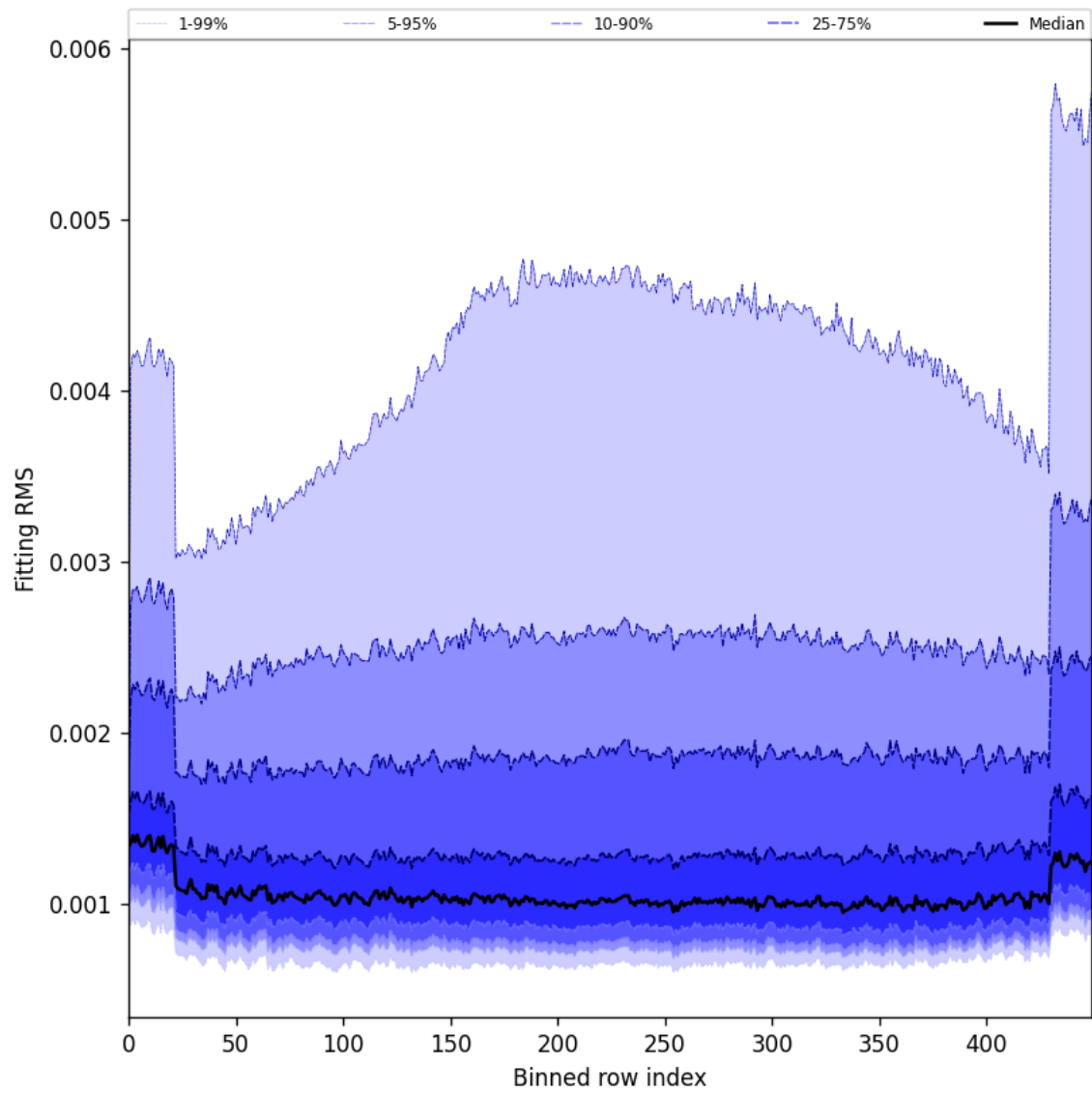
Figure 30: Along track statistics of “Fitting RMS” for 2025-11-02 to 2025-11-04
