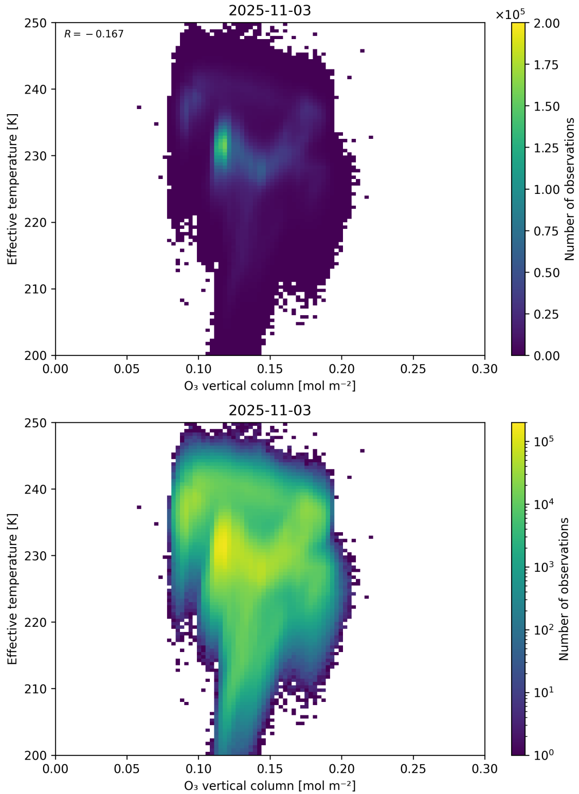
Figure 39: Scatter density plot of “O 3 vertical column” against “Effective temperature” for 2025-11-02 to 2025-11-04.
