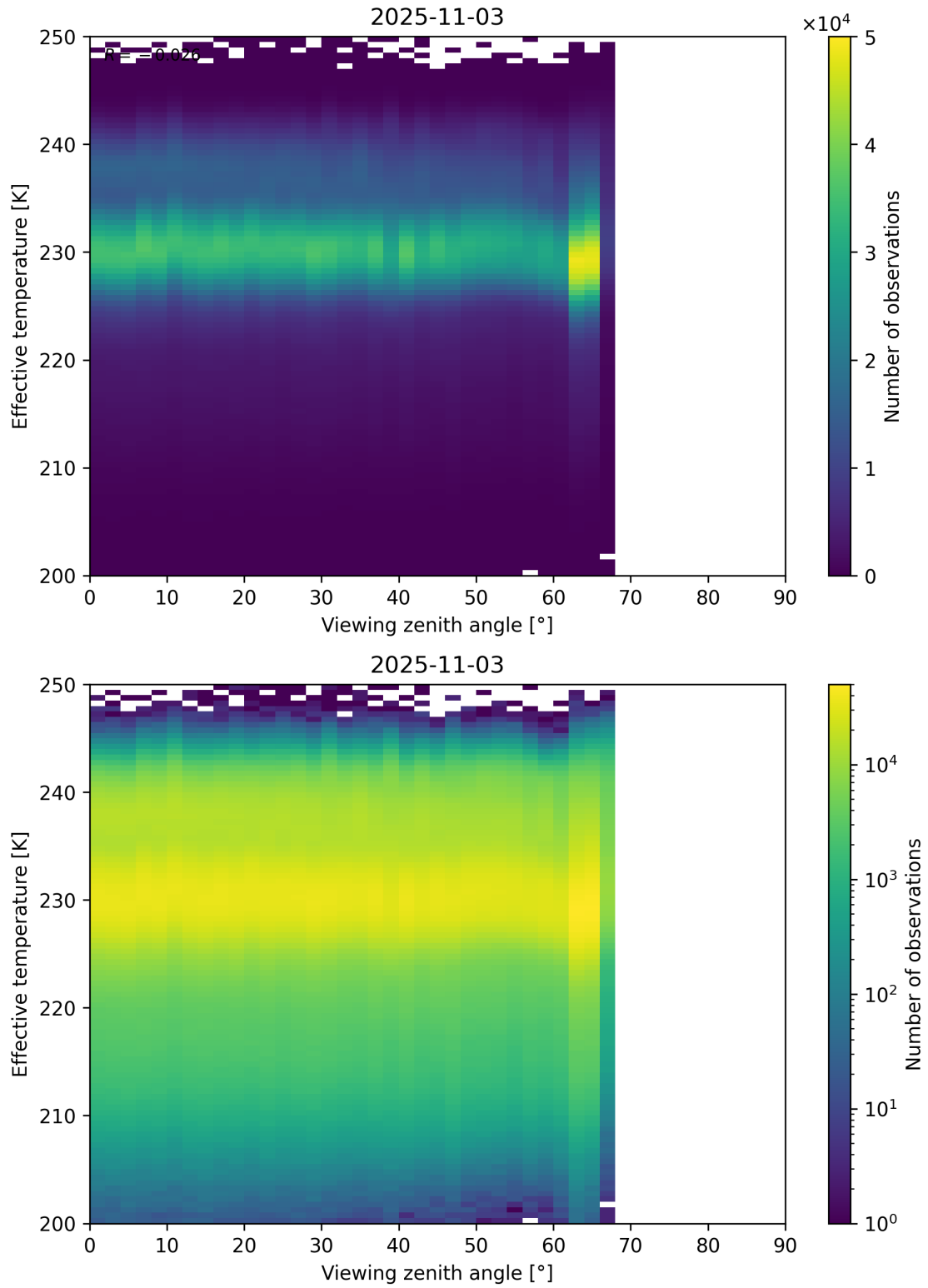
Figure 50: Scatter density plot of “Viewing zenith angle” against “Effective temperature” for 2025-11-02 to 2025-11-04.
