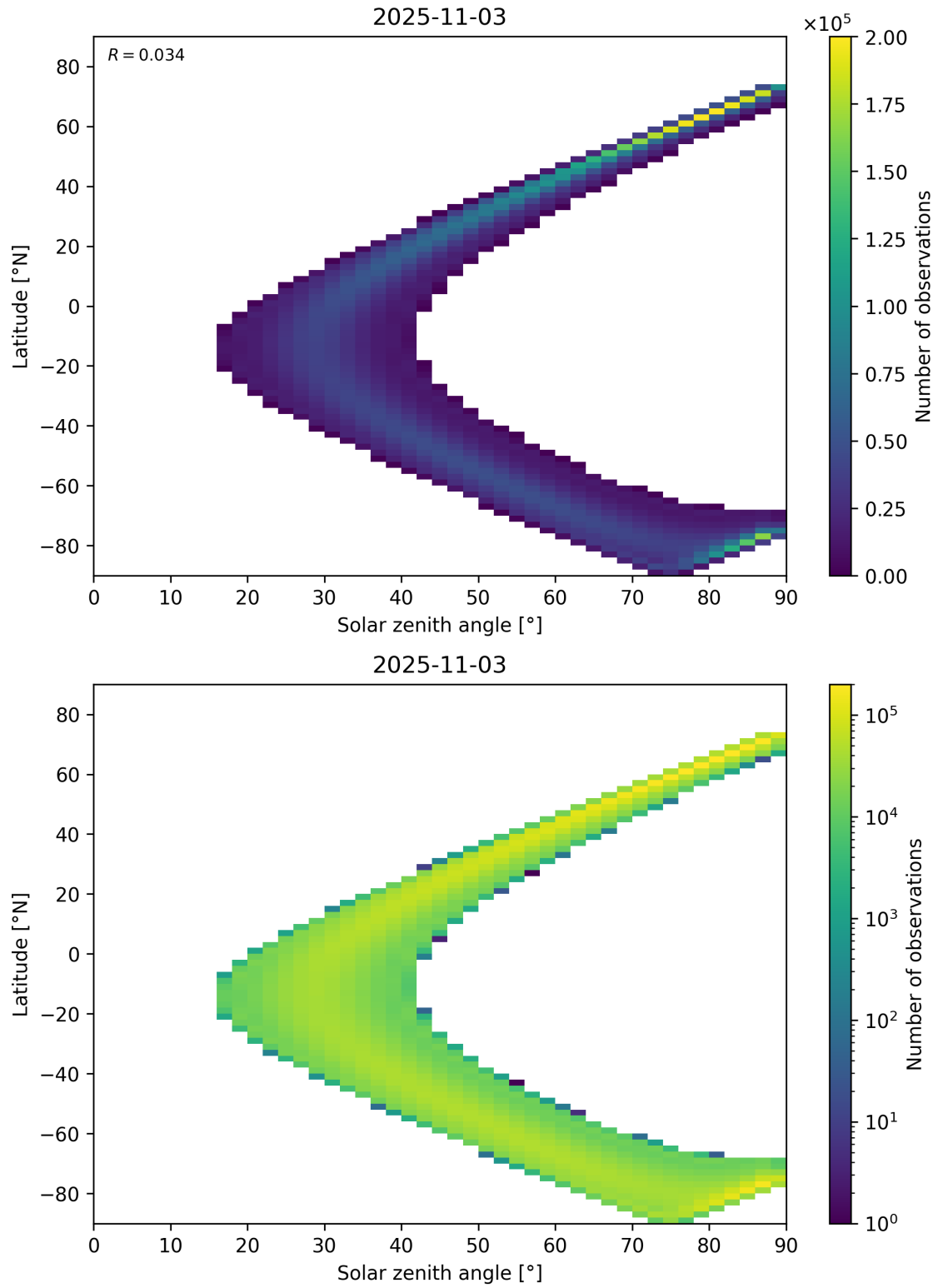
Figure 44: Scatter density plot of “Solar zenith angle” against “Latitude” for 2025-11-02 to 2025-11-04.
