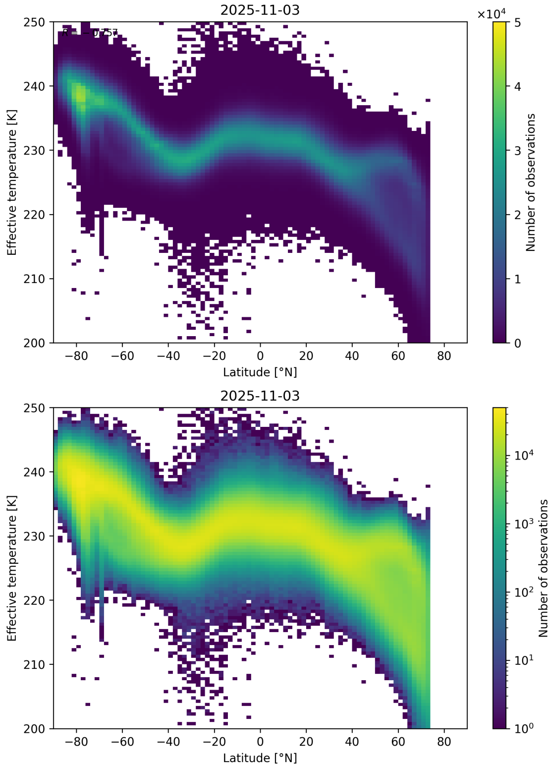
Figure 34: Scatter density plot of “Latitude” against “Effective temperature” for 2025-11-02 to 2025-11-04.
