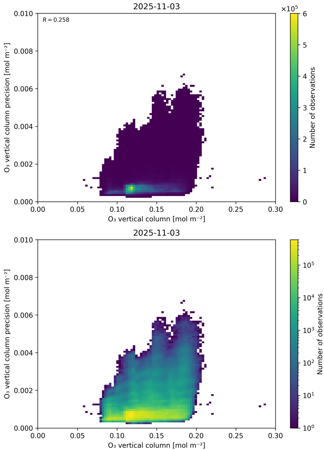
Figure 41: Scatter density plot of “O 3 vertical column” against “O 3 vertical column precision” for 2025-11-02 to 2025-11-04.
