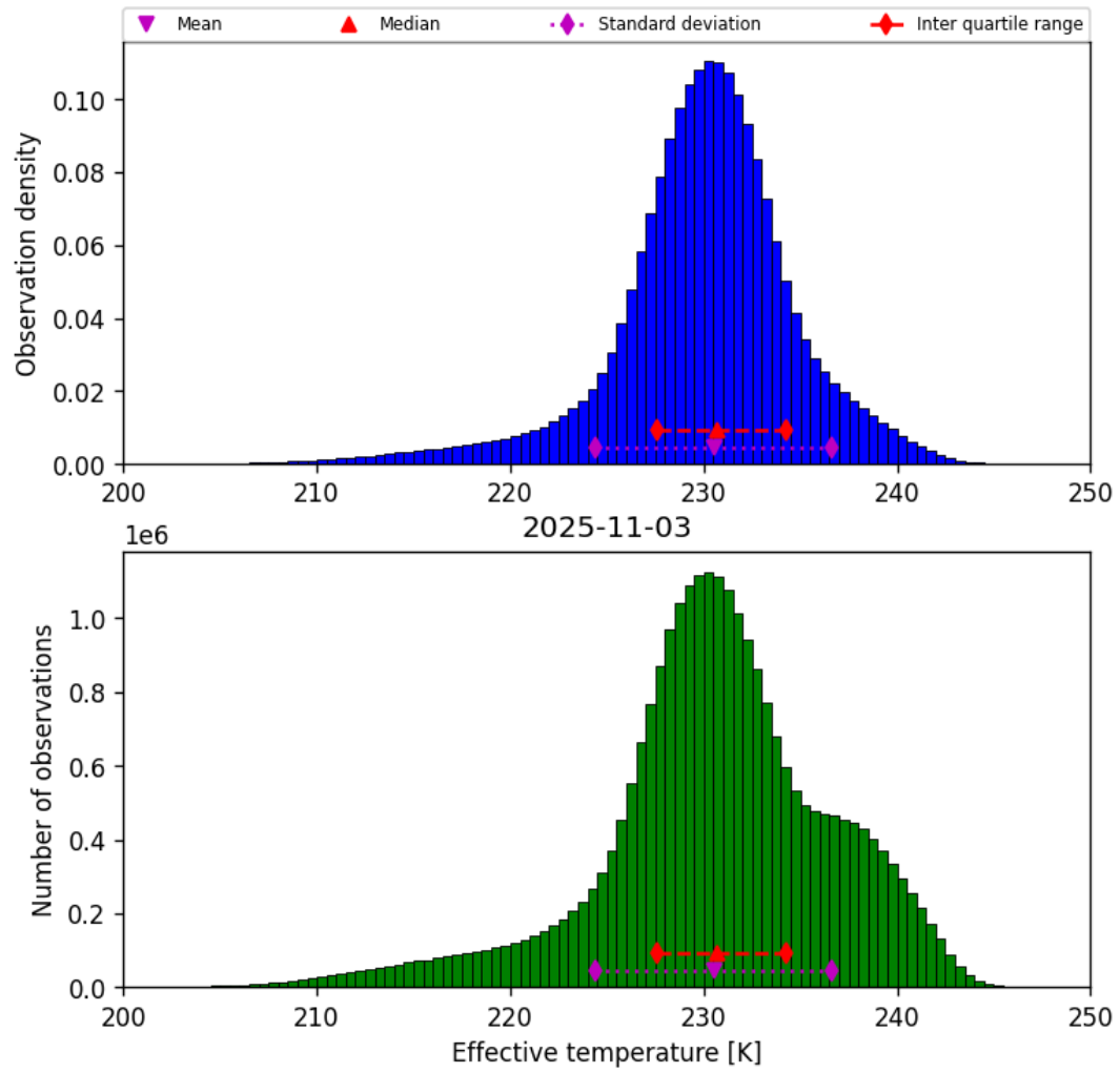
Figure 24: Histogram of “Effective temperature” for 2025-11-02 to 2025-11-04
