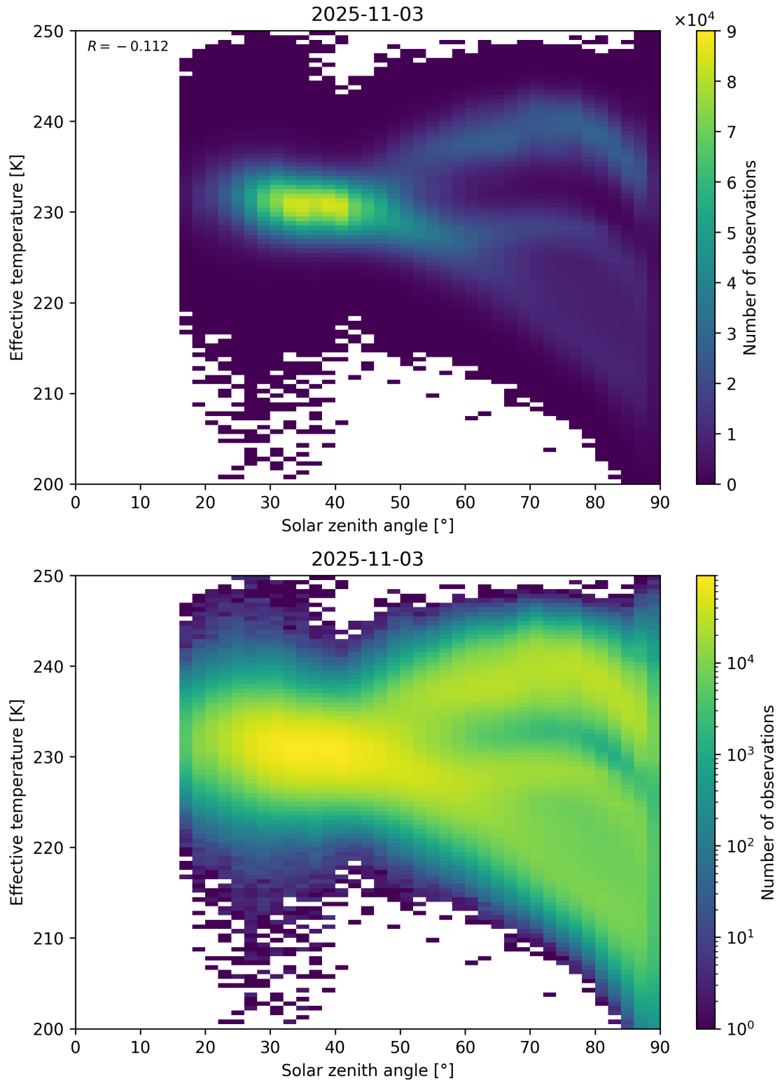
Figure 45: Scatter density plot of “Solar zenith angle” against “Effective temperature” for 2025-11-02 to 2025-11-04.
