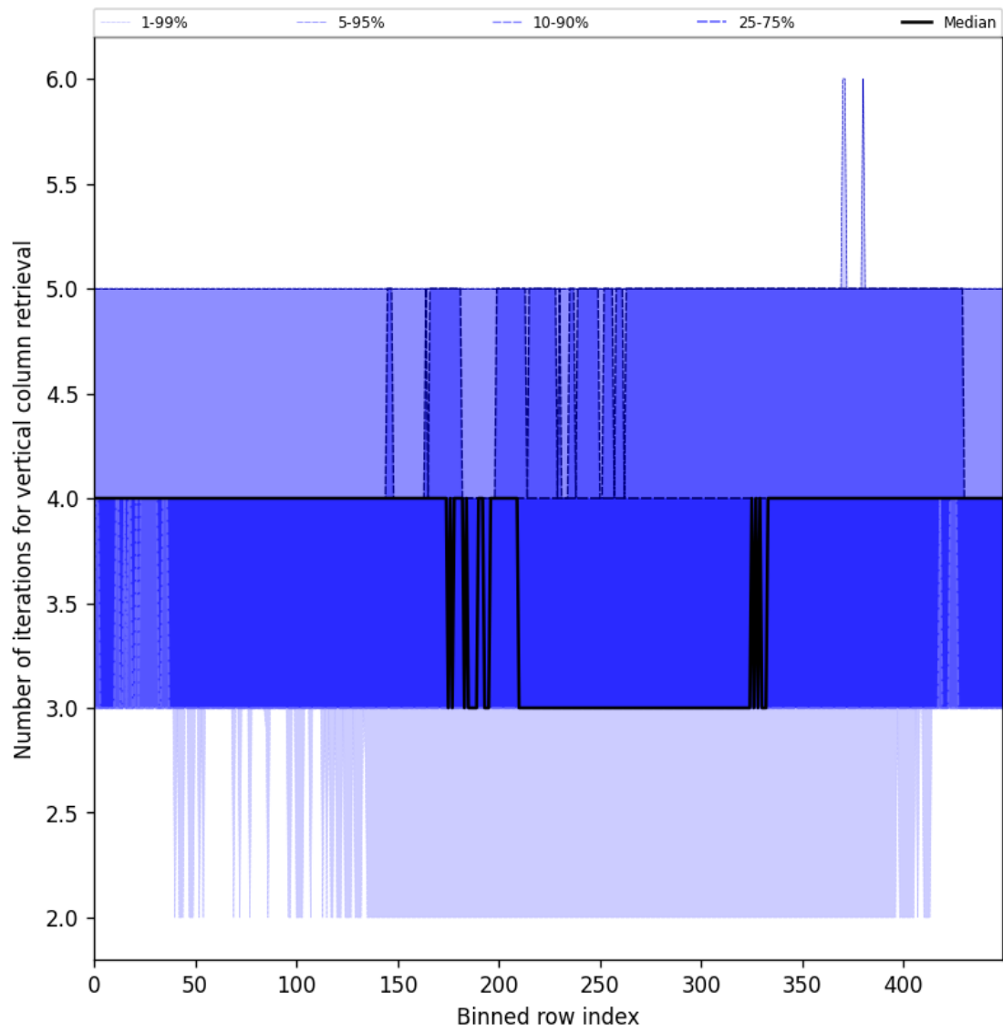
Figure 33: Along track statistics of “Number of iterations for vertical column retrieval” for 2025-11-02 to 2025-11-04
