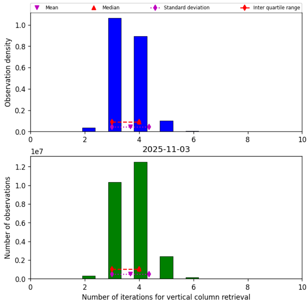
Figure 26: Histogram of “Number of iterations for vertical column retrieval” for 2025-11-02 to 2025-11-04
