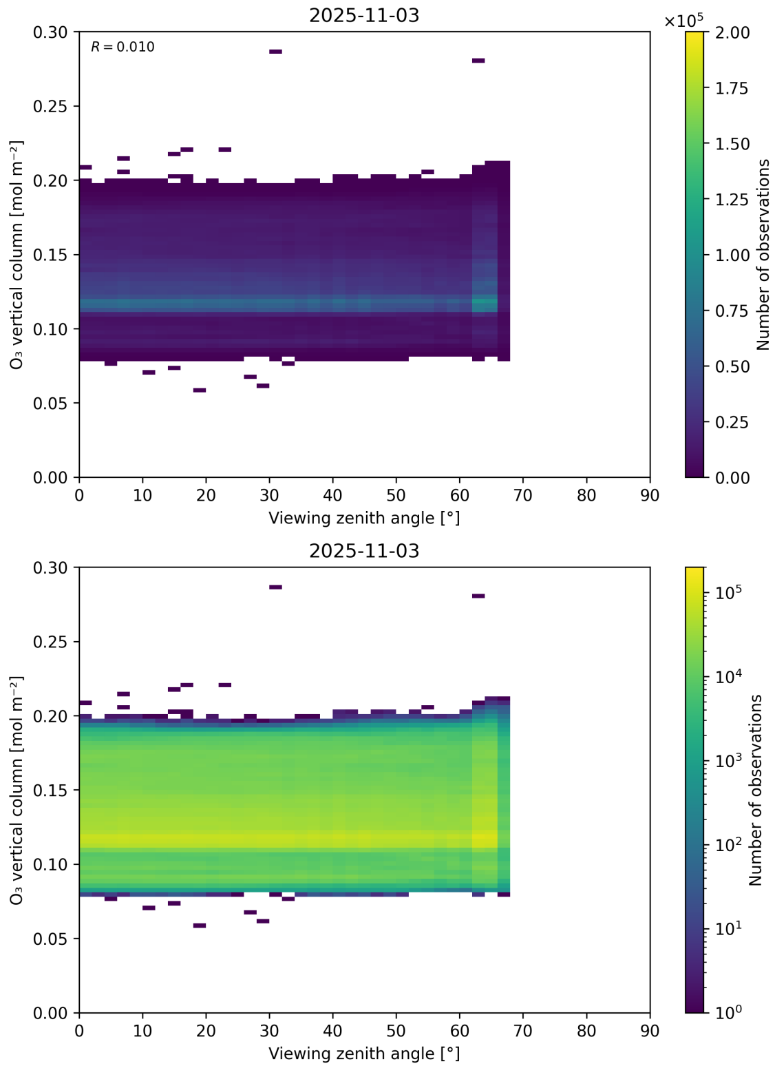
Figure 52: Scatter density plot of “Viewing zenith angle” against “O 3 vertical column” for 2025-11-02 to 2025-11-04.
