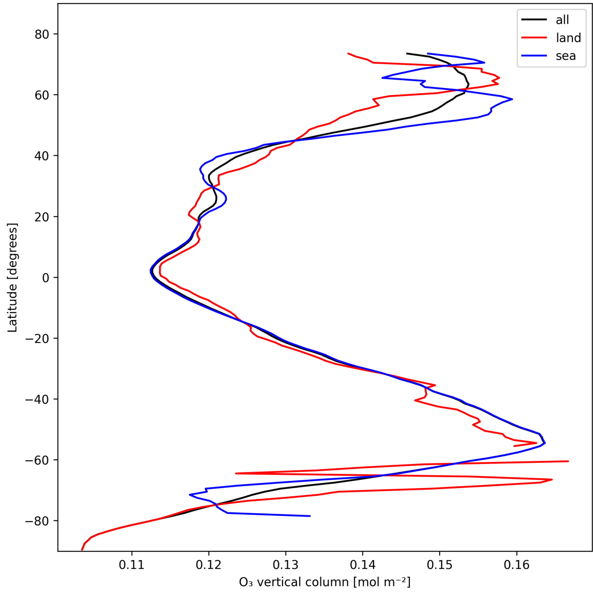
Figure 14: Zonal average of “O 3 vertical column” for 2025-11-02 to 2025-11-04.
