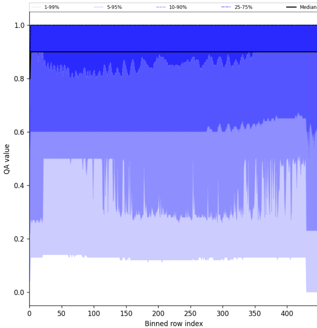
Figure 27: Along track statistics of “QA value” for 2025-11-02 to 2025-11-04
