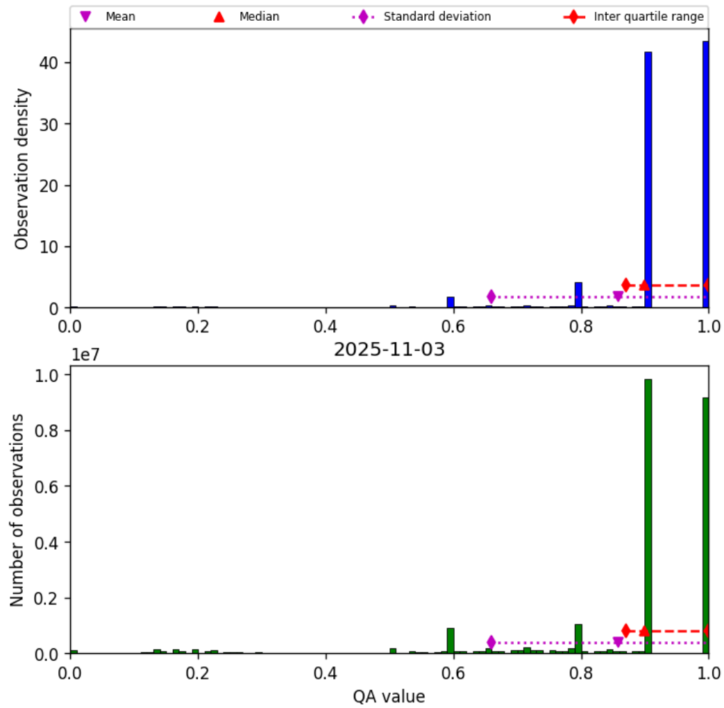
Figure 20: Histogram of “QA value” for 2025-11-02 to 2025-11-04
