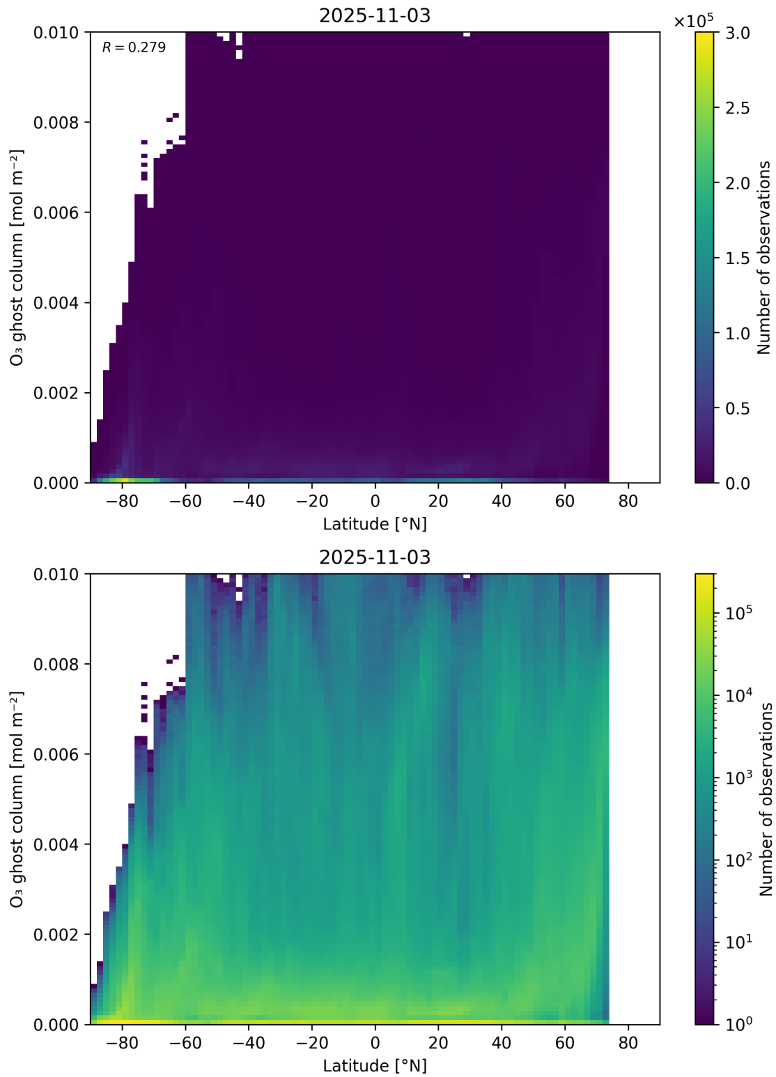
Figure 35: Scatter density plot of “Latitude” against “O 3 ghost column” for 2025-11-02 to 2025-11-04.
