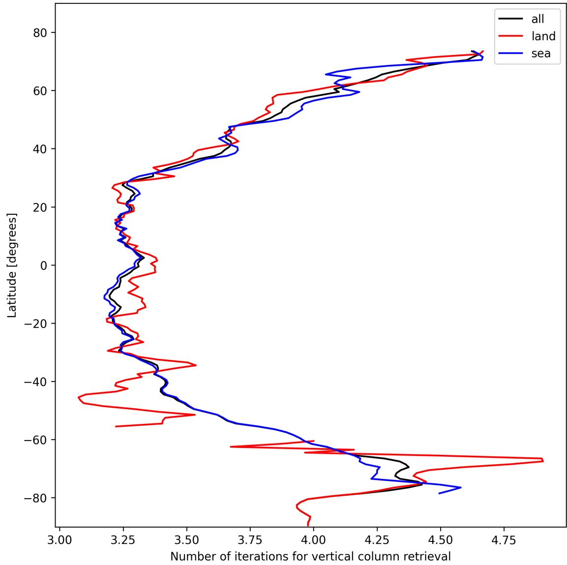
Figure 19: Zonal average of “Number of iterations for vertical column retrieval” for 2025-11-02 to 2025-11-04.
