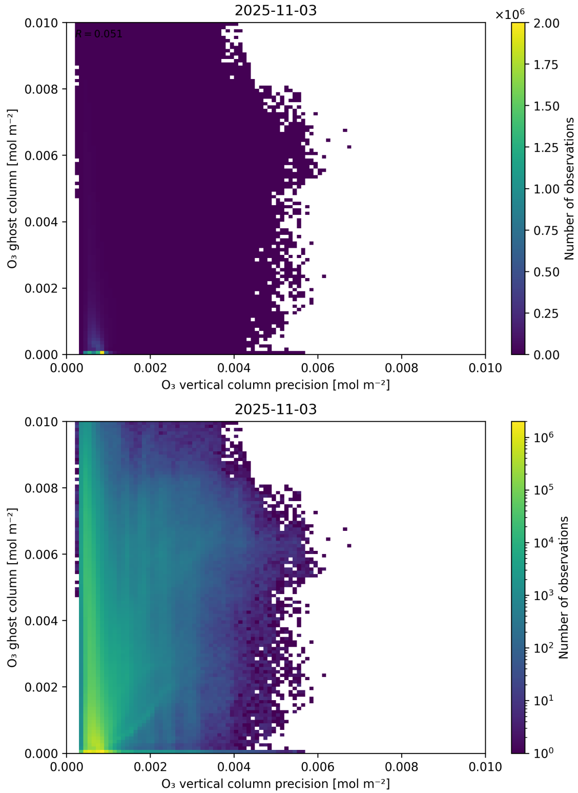
Figure 43: Scatter density plot of “O 3 vertical column precision” against “O 3 ghost column” for 2025-11-02 to 2025-11-04.
