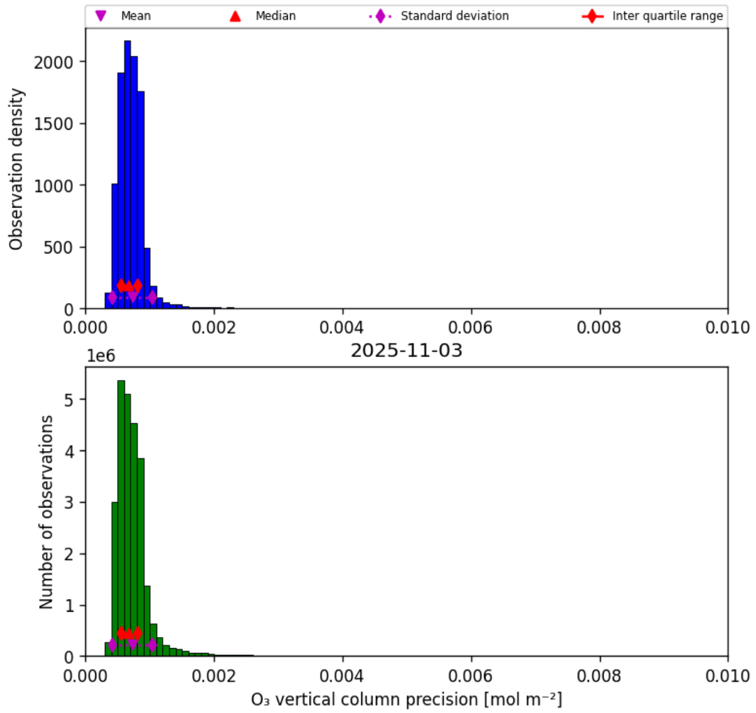
Figure 22: Histogram of “O 3 vertical column precision” for 2025-11-02 to 2025-11-04
