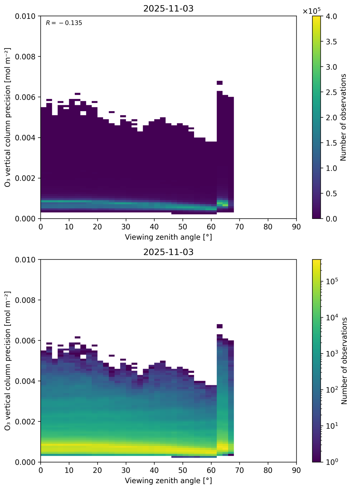
Figure 53: Scatter density plot of “Viewing zenith angle” against “O 3 vertical column precision” for 2025-11-02 to 2025-11-04.
