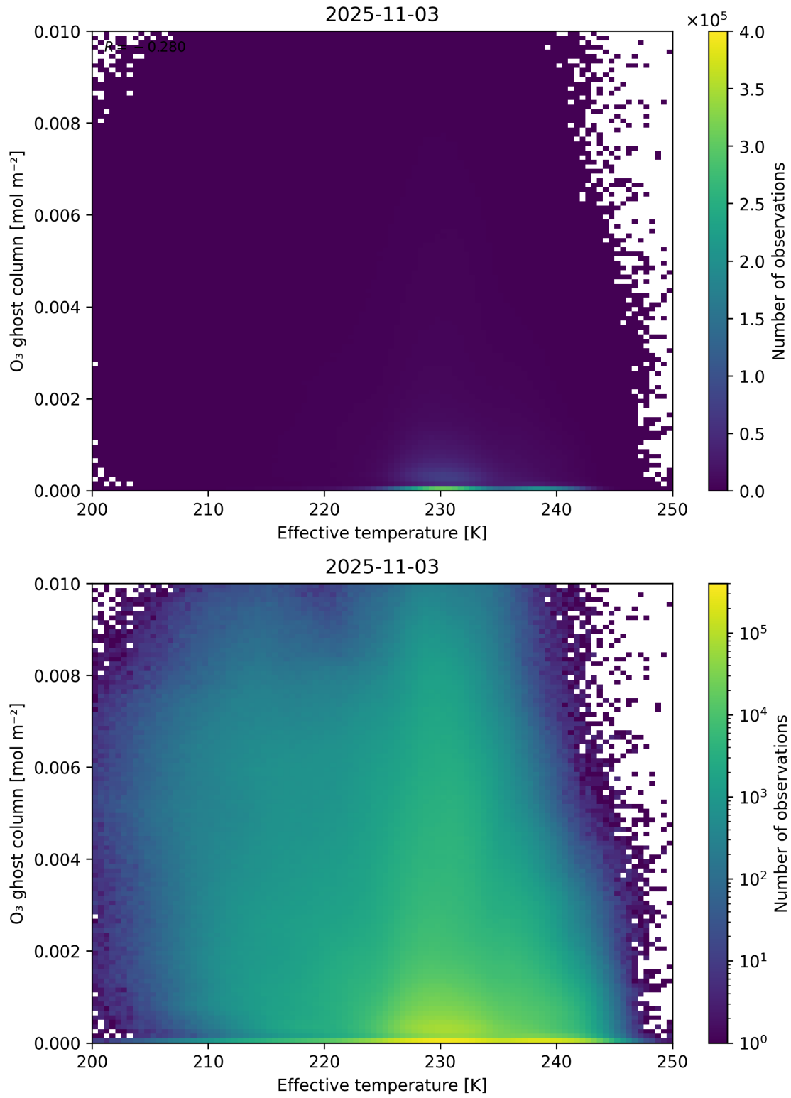
Figure 38: Scatter density plot of “Effective temperature” against “O 3 ghost column” for 2025-11-02 to 2025-11-04.
