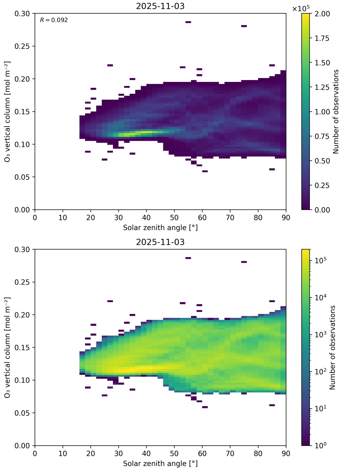
Figure 47: Scatter density plot of “Solar zenith angle” against “O 3 vertical column” for 2025-11-02 to 2025-11-04.
