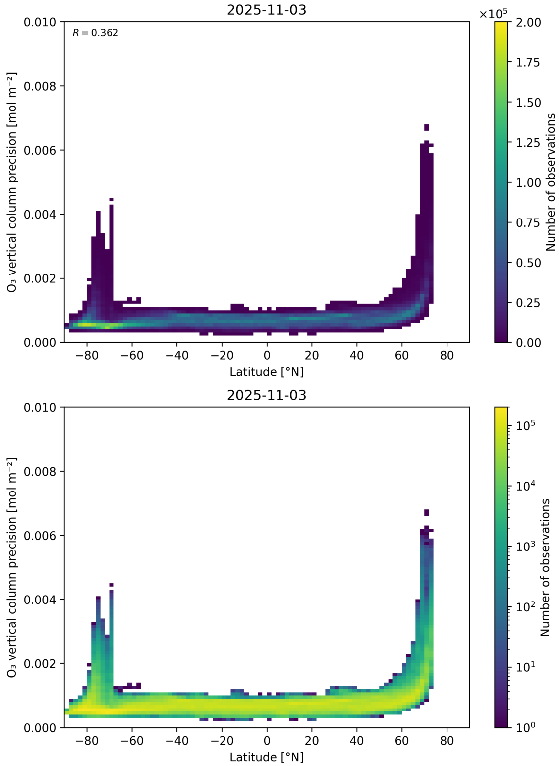
Figure 37: Scatter density plot of “Latitude” against “O 3 vertical column precision” for 2025-11-02 to 2025-11-04.
