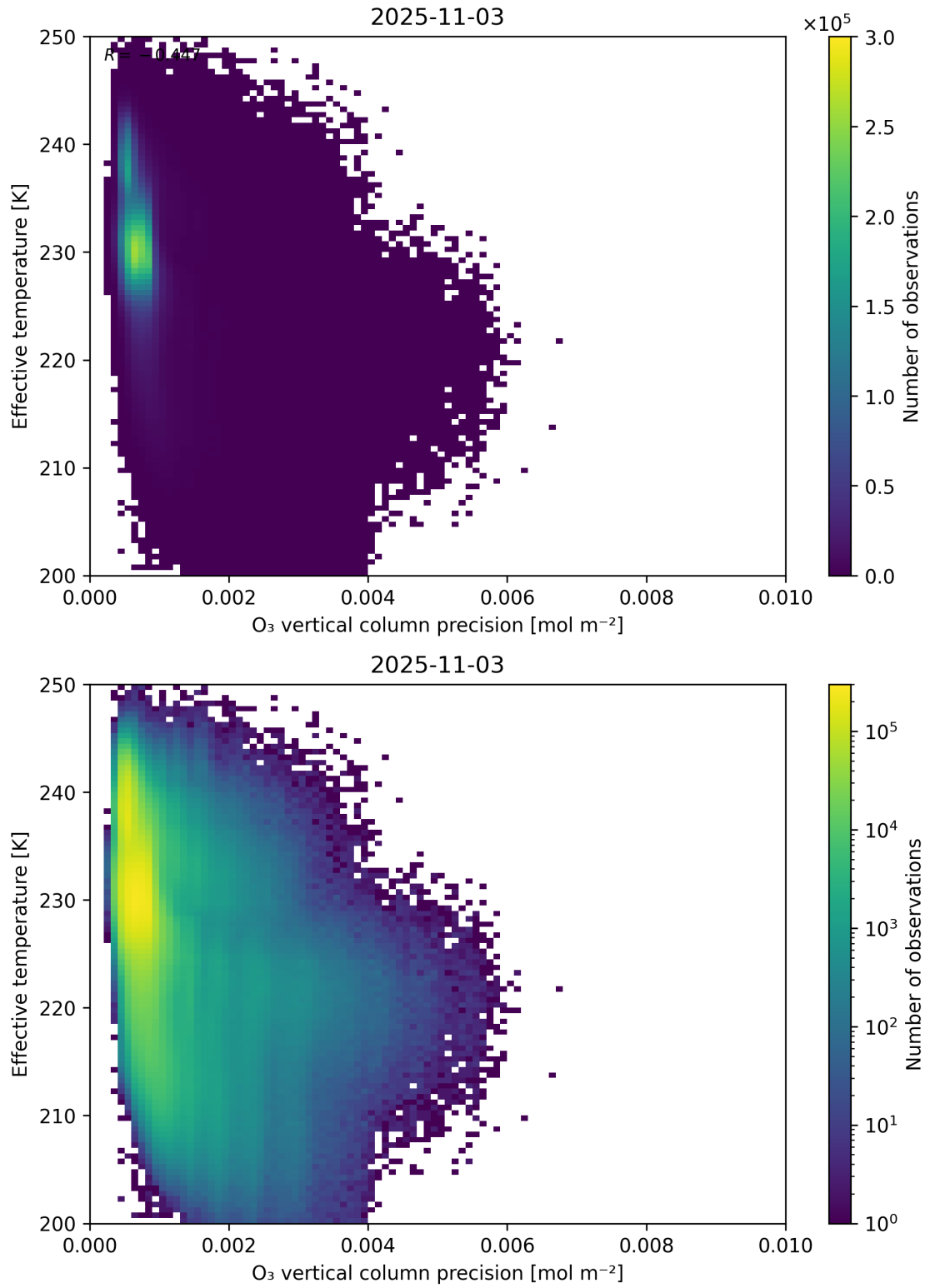
Figure 42: Scatter density plot of “O 3 vertical column precision” against “Effective temperature” for 2025-11-02 to 2025-11-04.
