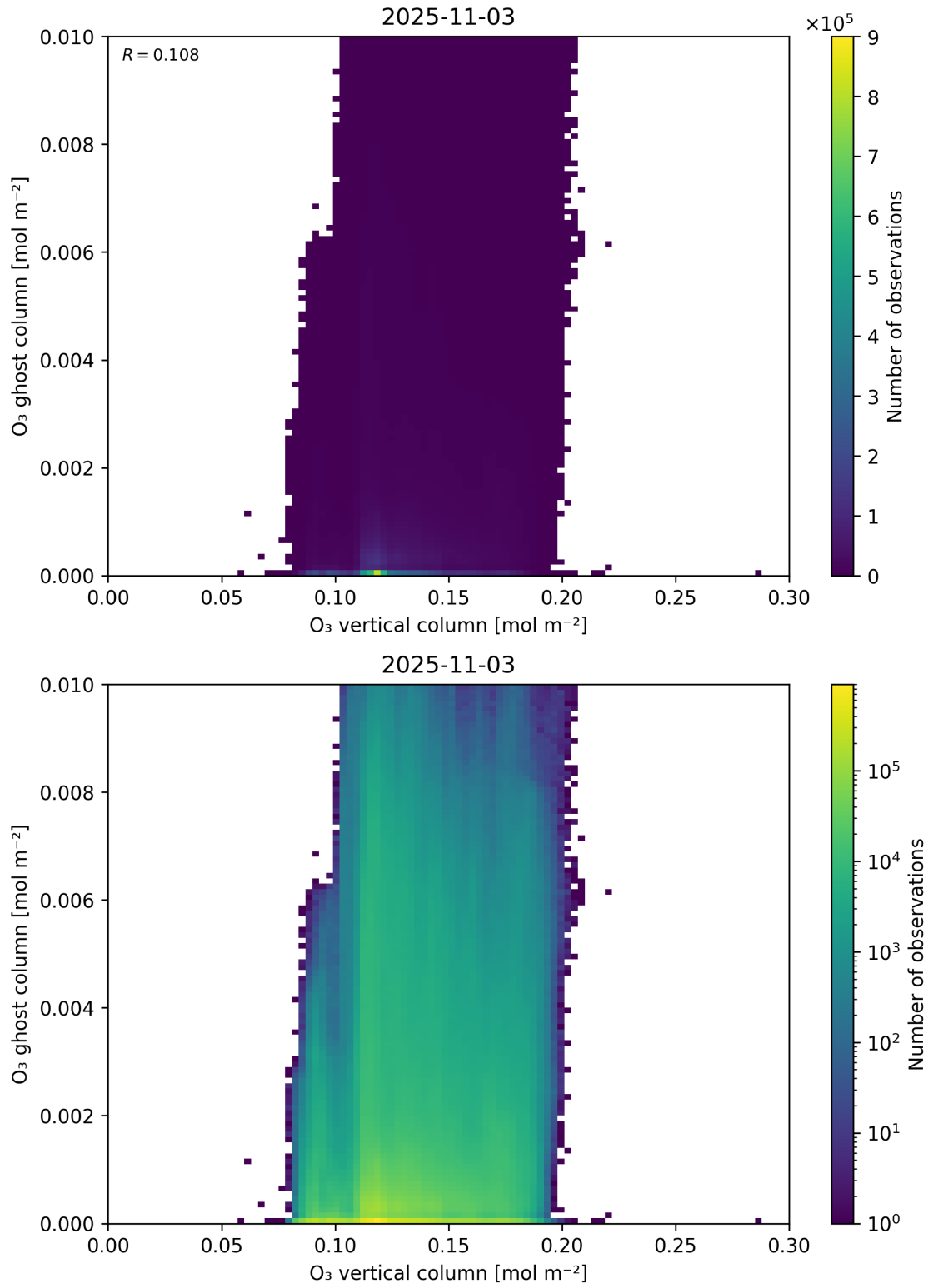
Figure 40: Scatter density plot of “O 3 vertical column” against “O 3 ghost column” for 2025-11-02 to 2025-11-04.
