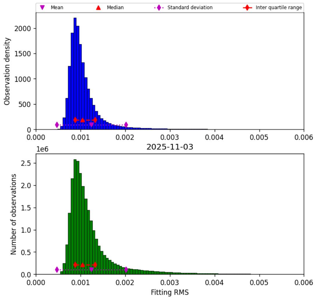
Figure 23: Histogram of “Fitting RMS” for 2025-11-02 to 2025-11-04
