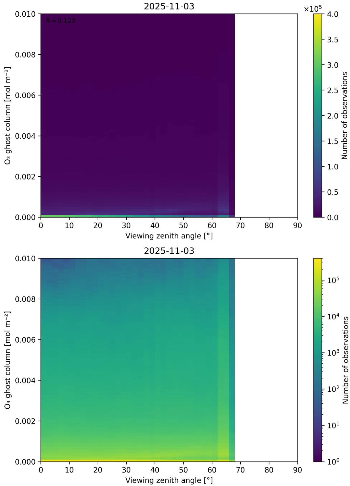
Figure 51: Scatter density plot of “Viewing zenith angle” against “O 3 ghost column” for 2025-11-02 to 2025-11-04.
