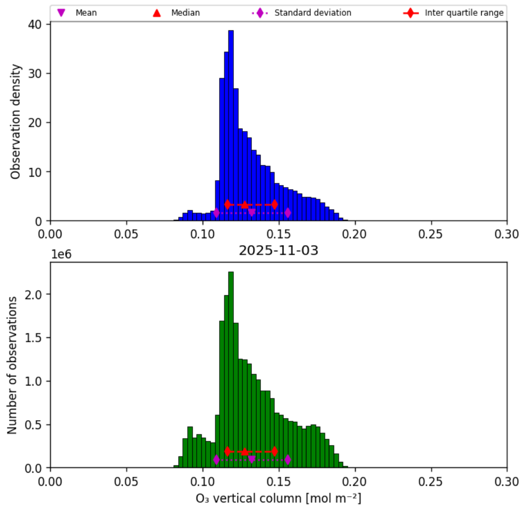
Figure 21: Histogram of “O 3 vertical column” for 2025-11-02 to 2025-11-04
