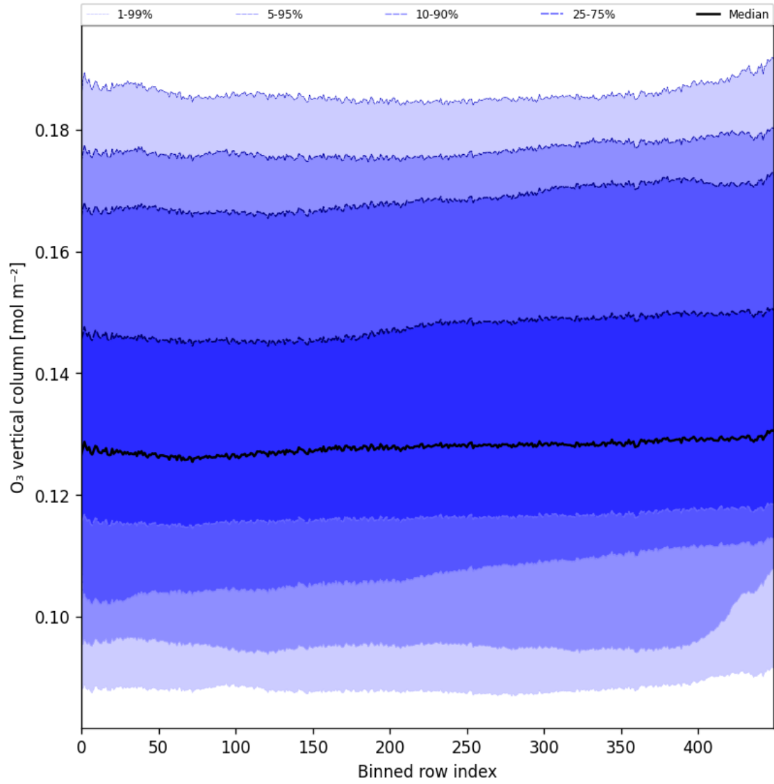
Figure 28: Along track statistics of “ O_3 vertical column” for 2025-11-02 to 2025-11-04
