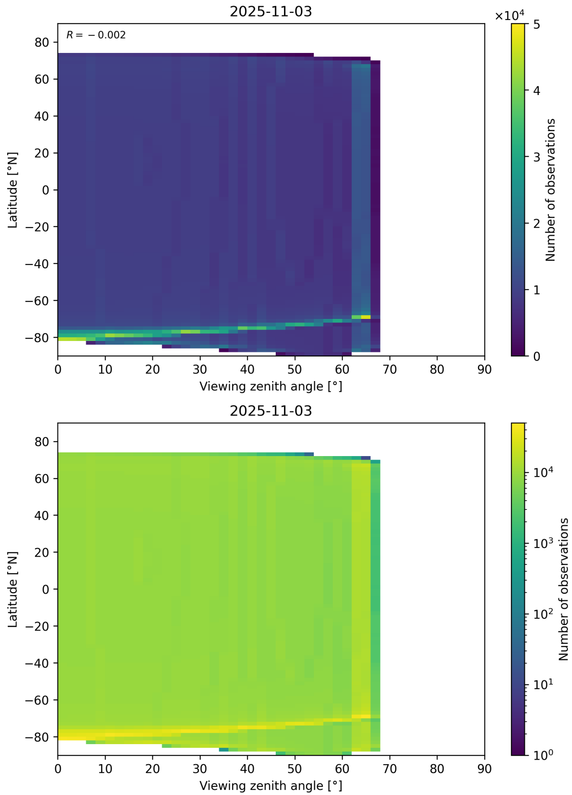
Figure 49: Scatter density plot of “Viewing zenith angle” against “Latitude” for 2025-11-02 to 2025-11-04.
