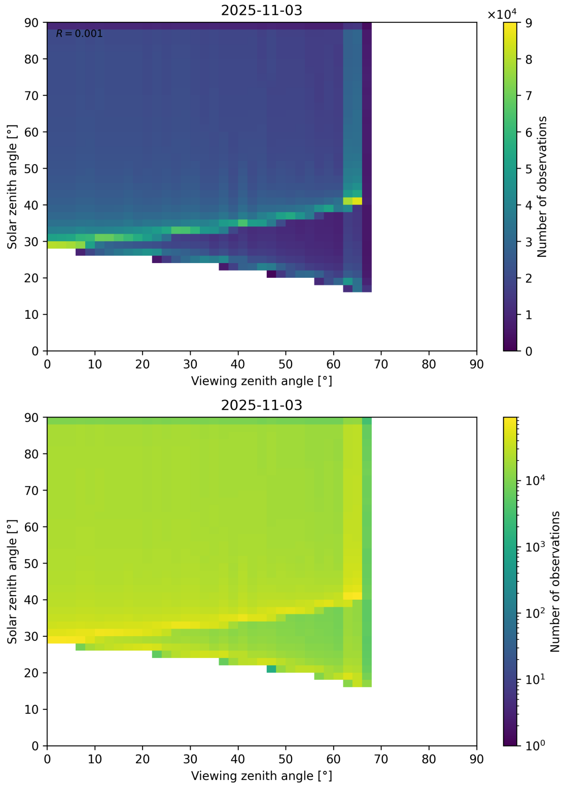
Figure 54: Scatter density plot of “Viewing zenith angle” against “Solar zenith angle” for 2025-11-02 to 2025-11-04.
