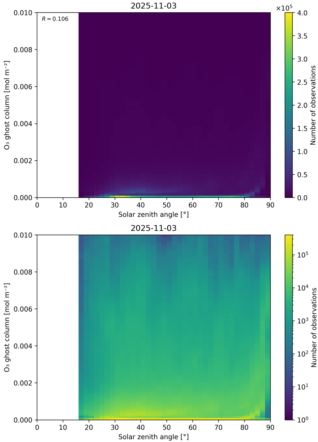
Figure 46: Scatter density plot of “Solar zenith angle” against “O 3 ghost column” for 2025-11-02 to 2025-11-04.
