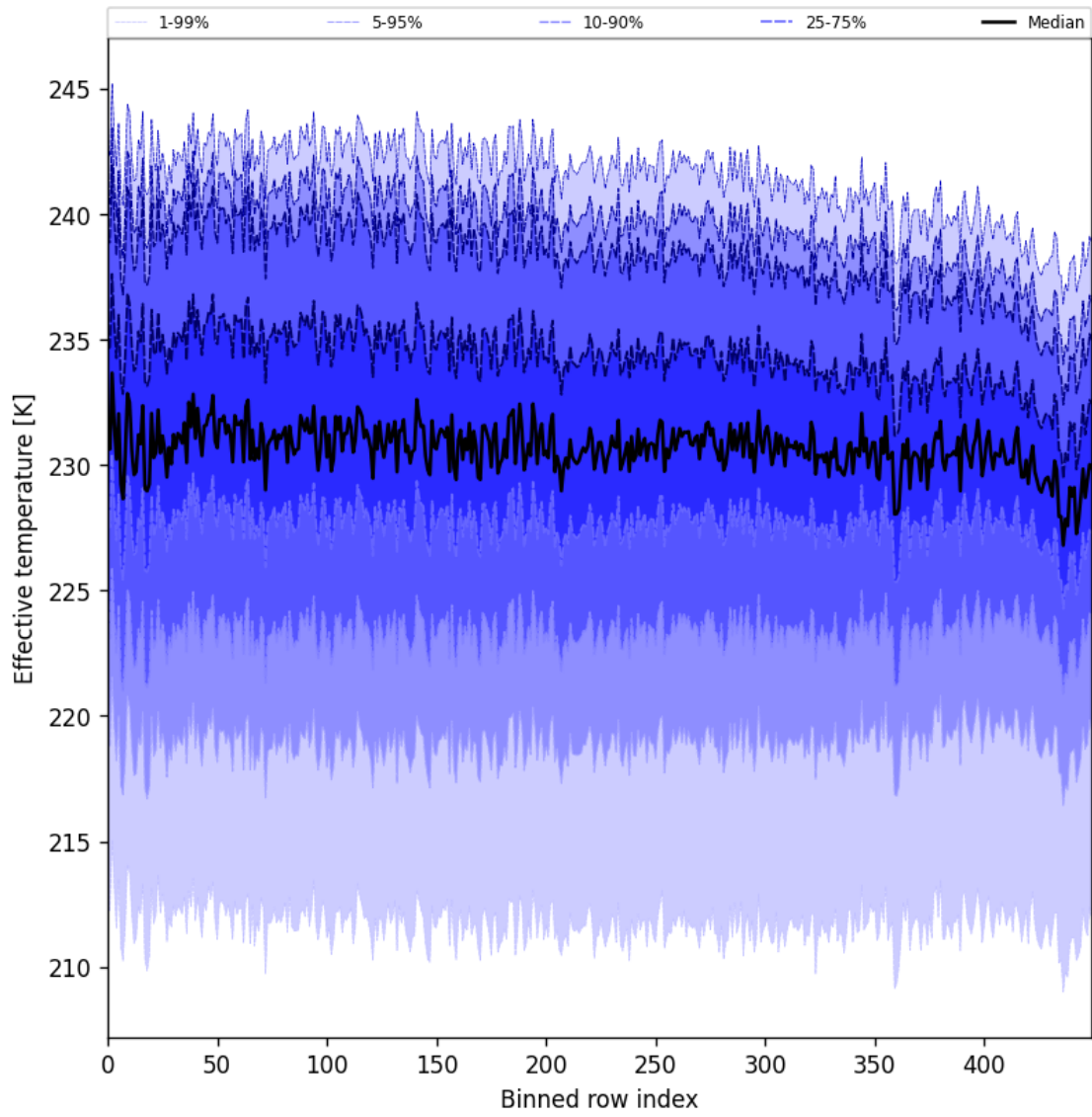
Figure 31: Along track statistics of “Effective temperature” for 2025-11-02 to 2025-11-04
