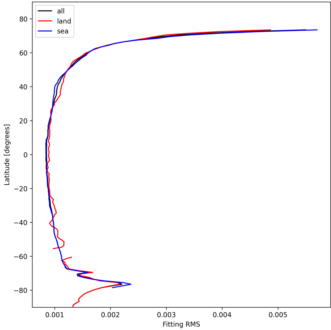
Figure 16: Zonal average of “Fitting RMS” for 2025-11-02 to 2025-11-04.
