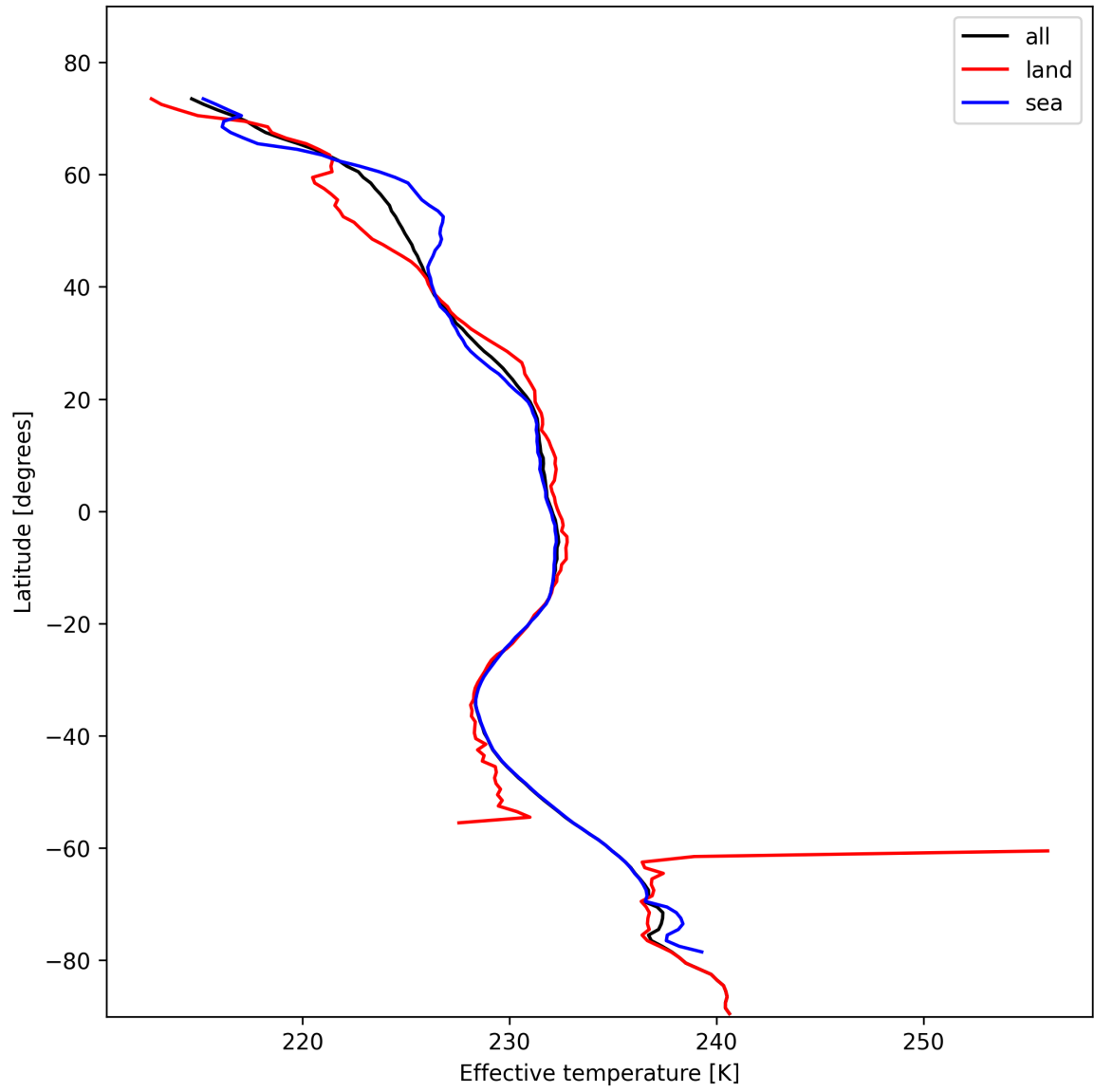
Figure 17: Zonal average of "Effective temperature" for 2025-11-02 to 2025-11-04.
