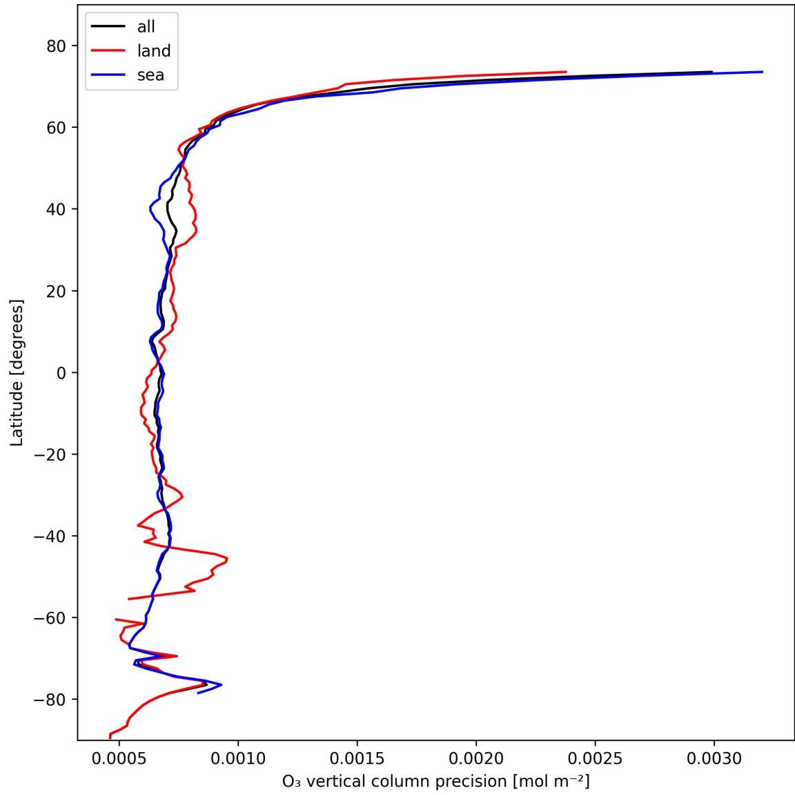
Figure 15: Zonal average of “O 3 vertical column precision” for 2025-11-02 to 2025-11-04.
