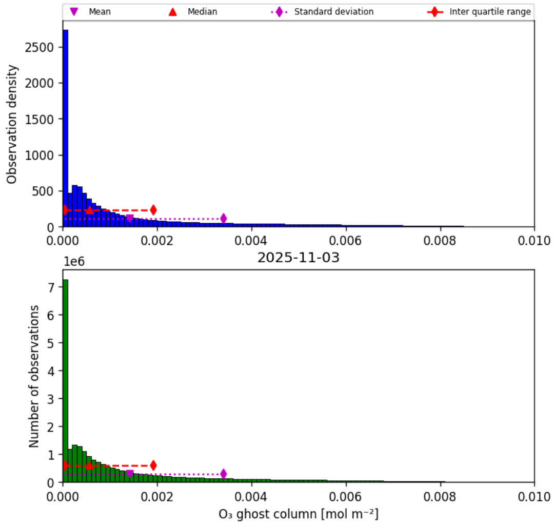
Figure 25: Histogram of “O 3 ghost column” for 2025-11-02 to 2025-11-04
