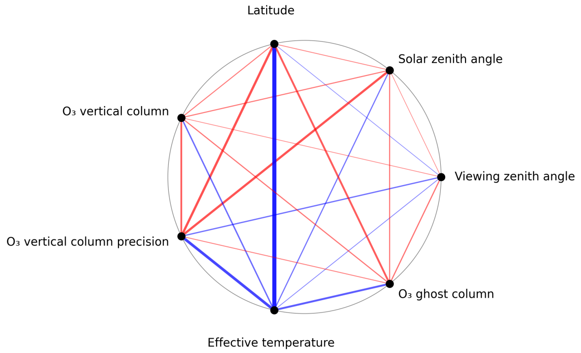
Figure 1: Map of correlation graph for 2025-11-02 to 2025-11-04.
