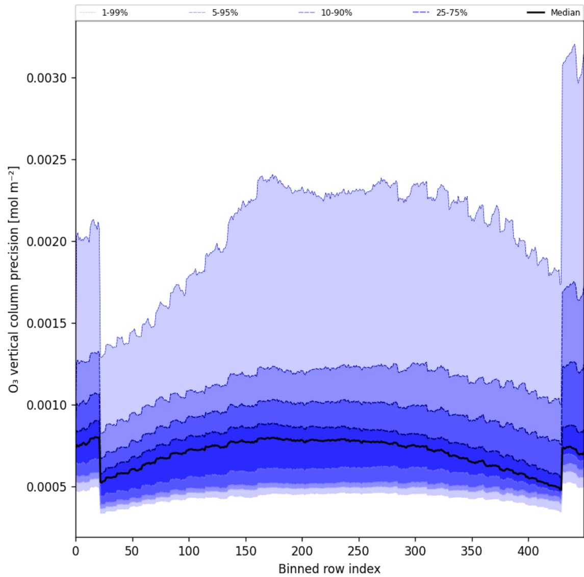
Figure 29: Along track statistics of “O 3 vertical column precision” for 2025-11-02 to 2025-11-04
