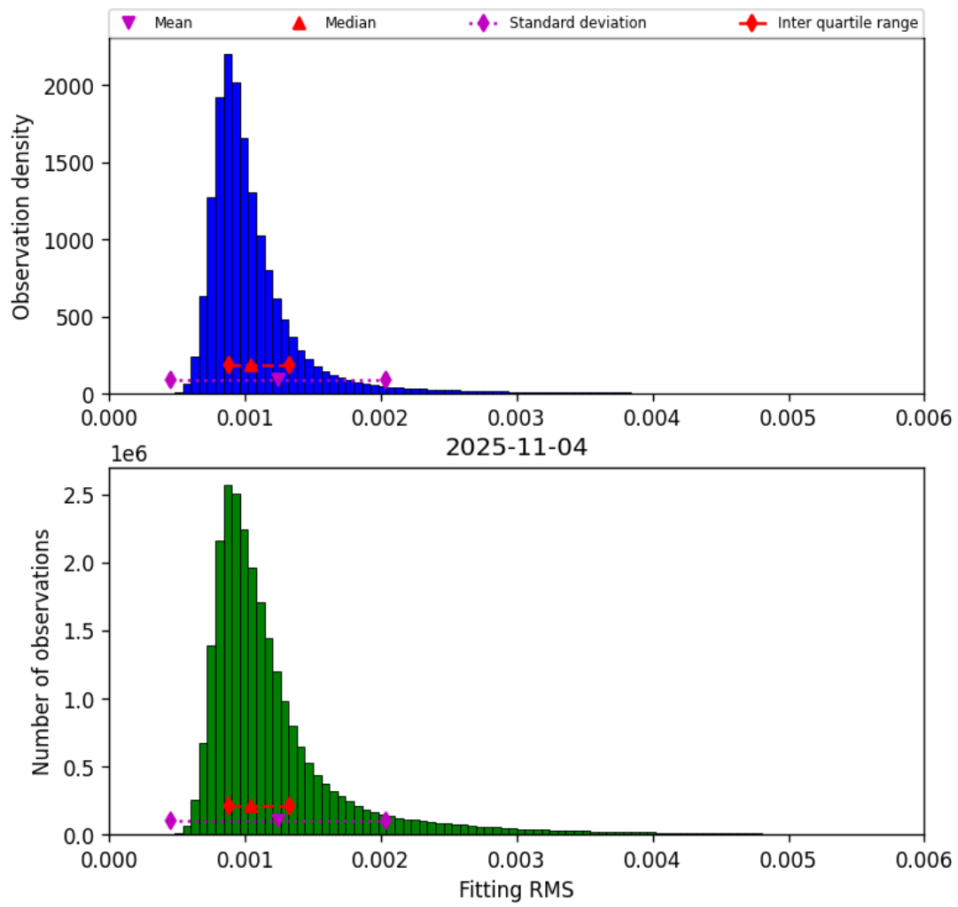
Figure 23: Histogram of “Fitting RMS” for 2025-11-03 to 2025-11-05
