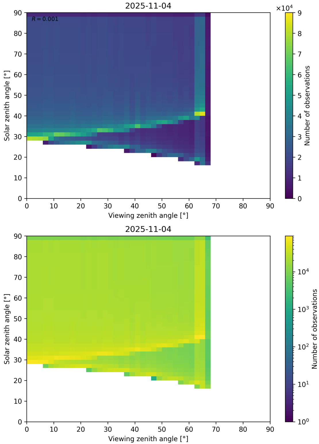
Figure 54: Scatter density plot of “Viewing zenith angle” against “Solar zenith angle” for 2025-11-03 to 2025-11-05.
