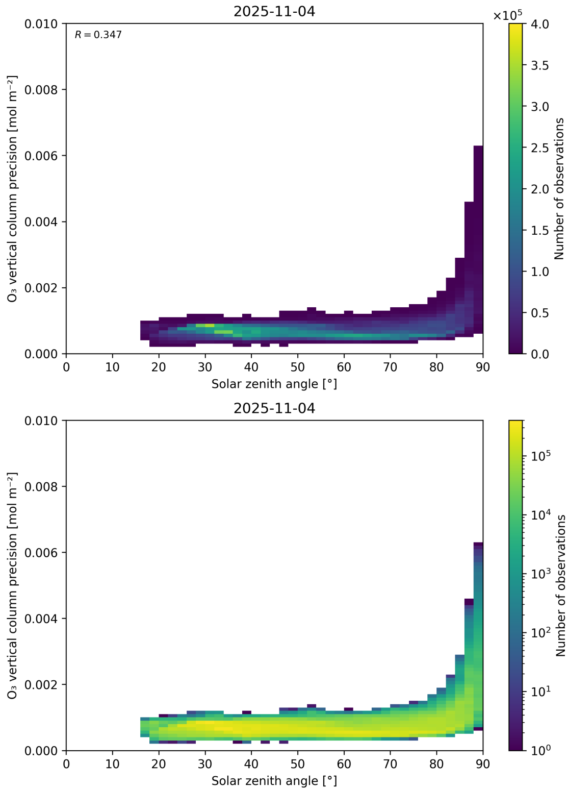
Figure 48: Scatter density plot of “Solar zenith angle” against “O 3 vertical column precision” for 2025-11-03 to 2025-11-05.
