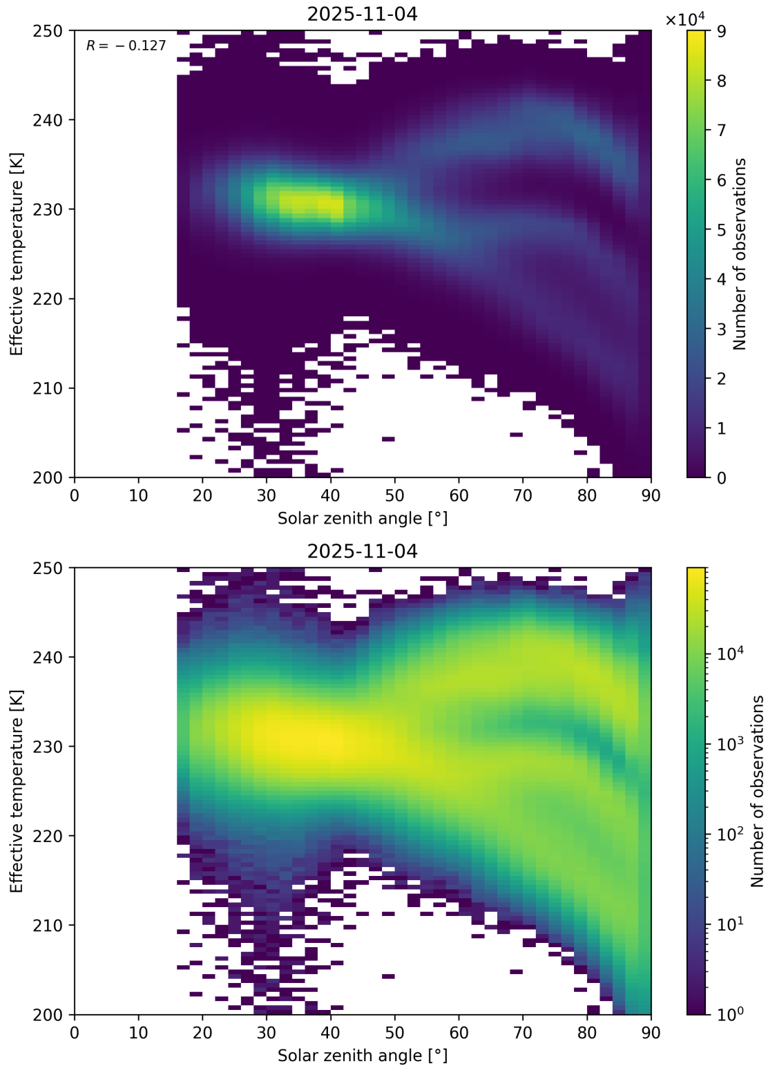
Figure 45: Scatter density plot of “Solar zenith angle” against “Effective temperature” for 2025-11-03 to 2025-11-05.
