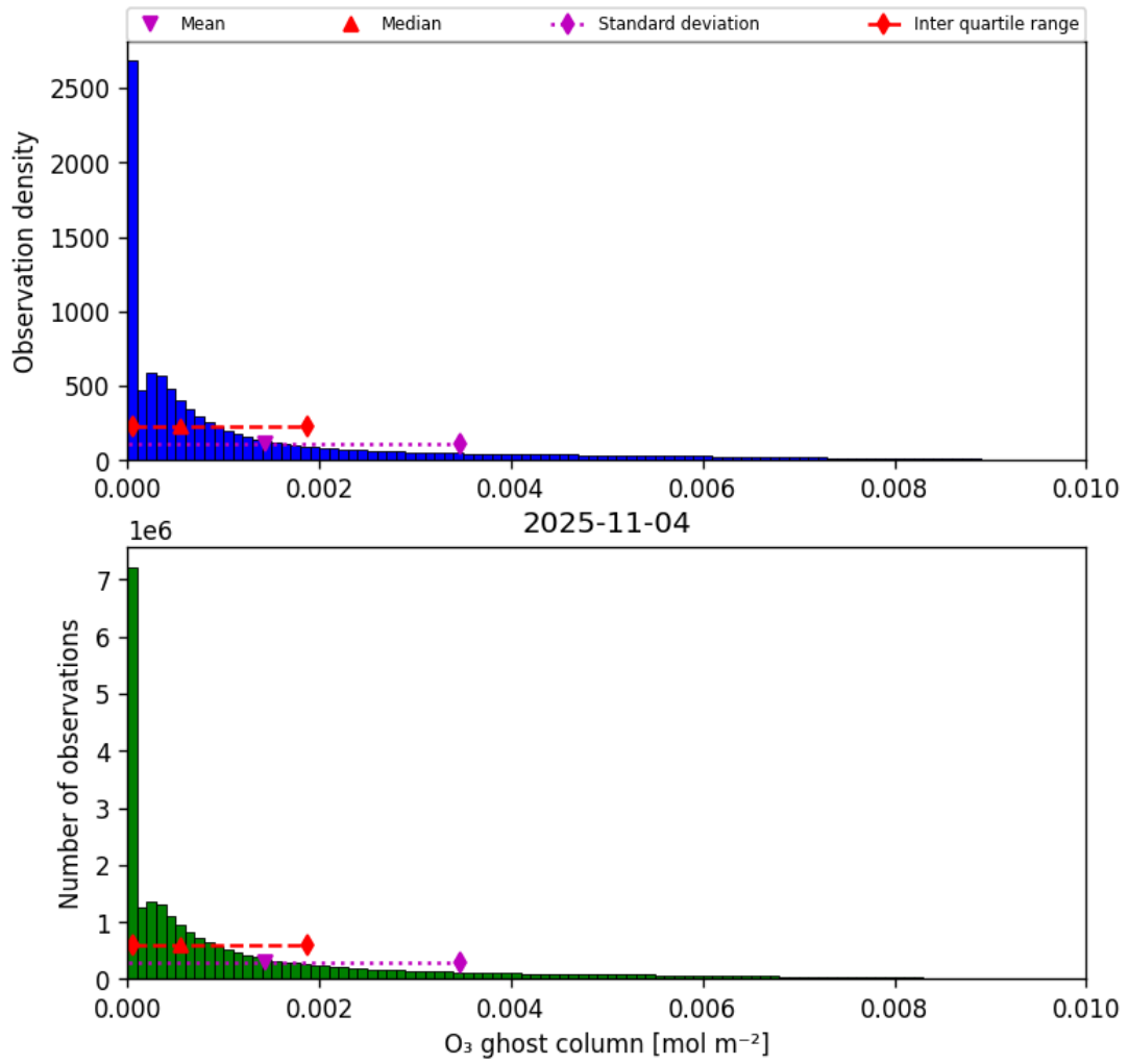
Figure 25: Histogram of “O 3 ghost column” for 2025-11-03 to 2025-11-05
