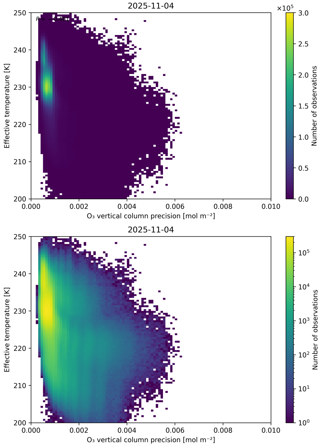
Figure 42: Scatter density plot of “O 3 vertical column precision” against “Effective temperature” for 2025-11-03 to 2025-11-05.
