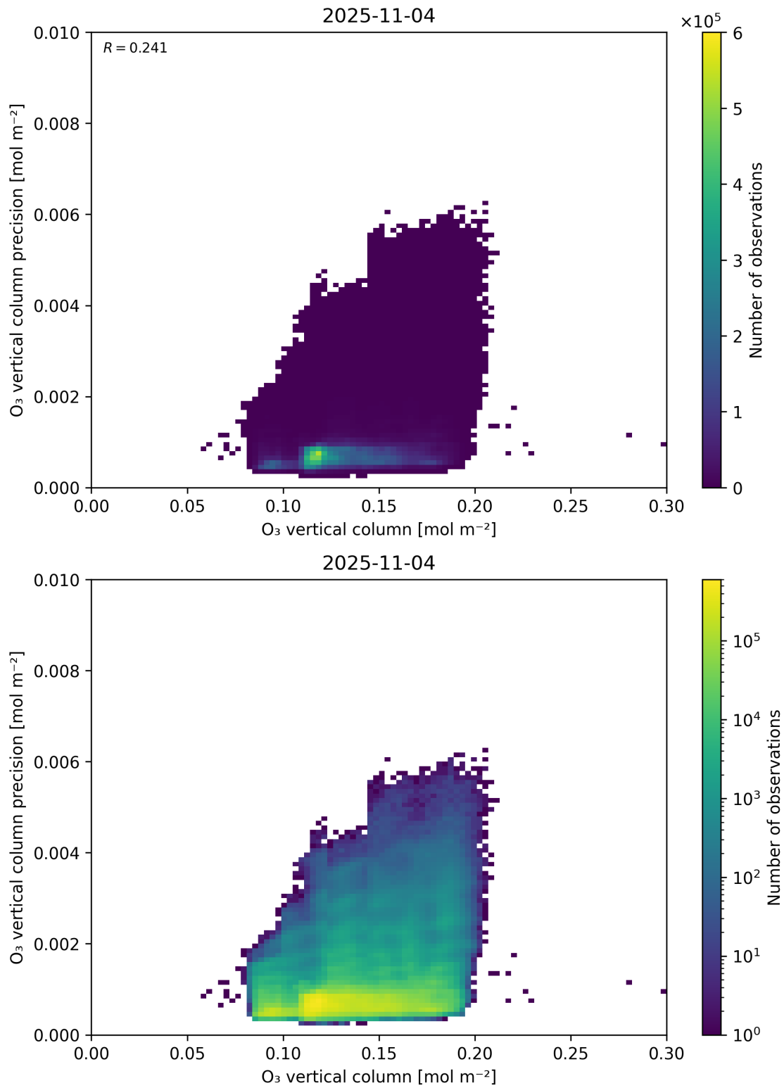
Figure 41: Scatter density plot of “O 3 vertical column” against “O 3 vertical column precision” for 2025-11-03 to 2025-11-05.
