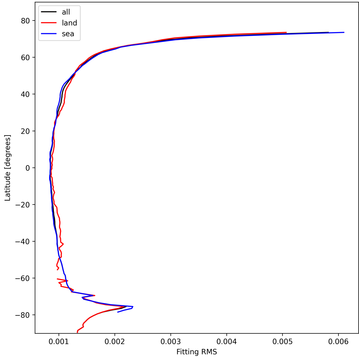
Figure 16: Zonal average of “Fitting RMS” for 2025-11-03 to 2025-11-05.
