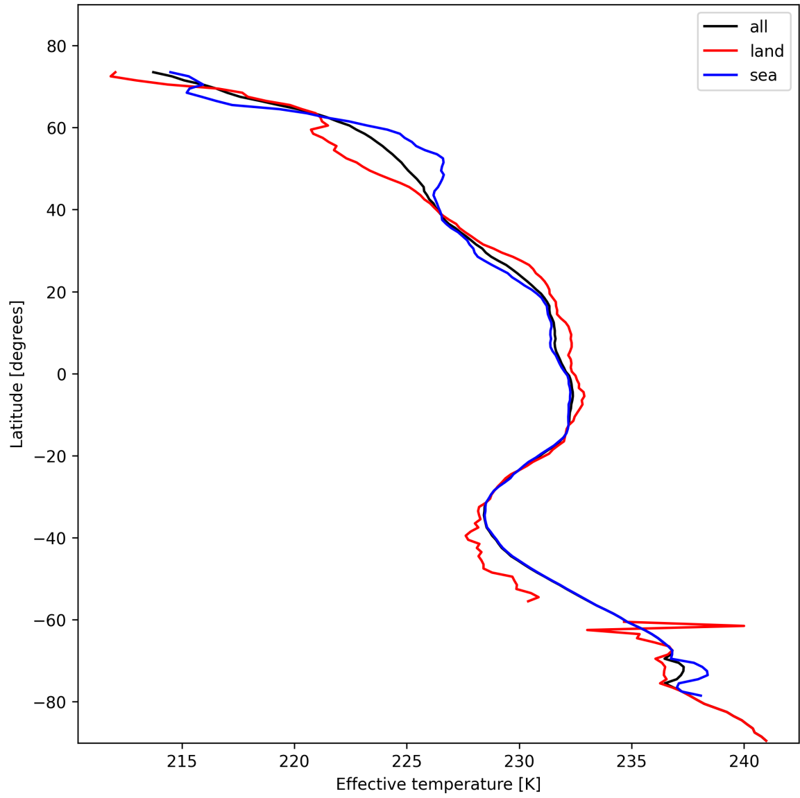
Figure 17: Zonal average of "Effective temperature" for 2025-11-03 to 2025-11-05.
