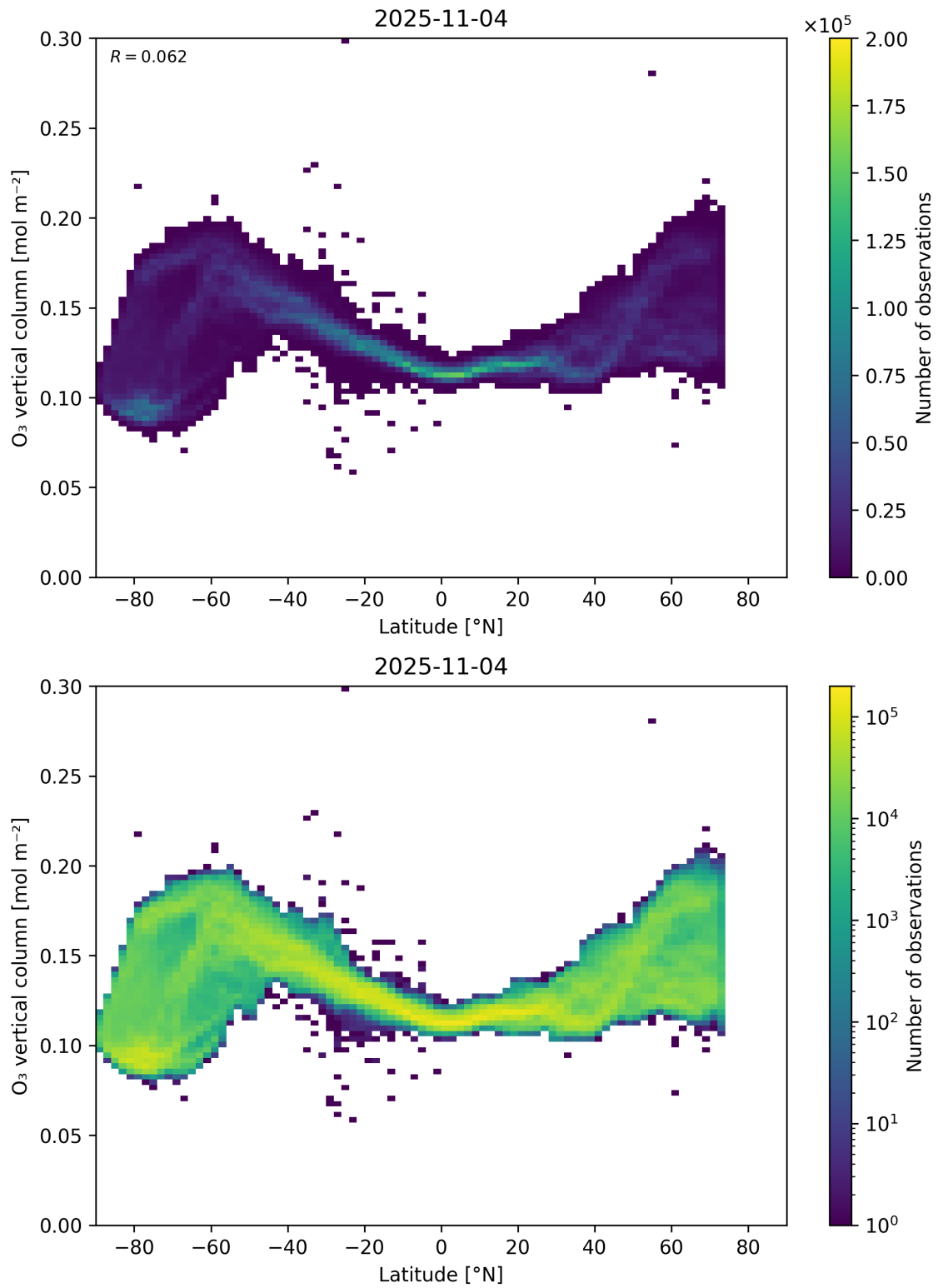
Figure 36: Scatter density plot of “Latitude” against “O 3 vertical column” for 2025-11-03 to 2025-11-05.
