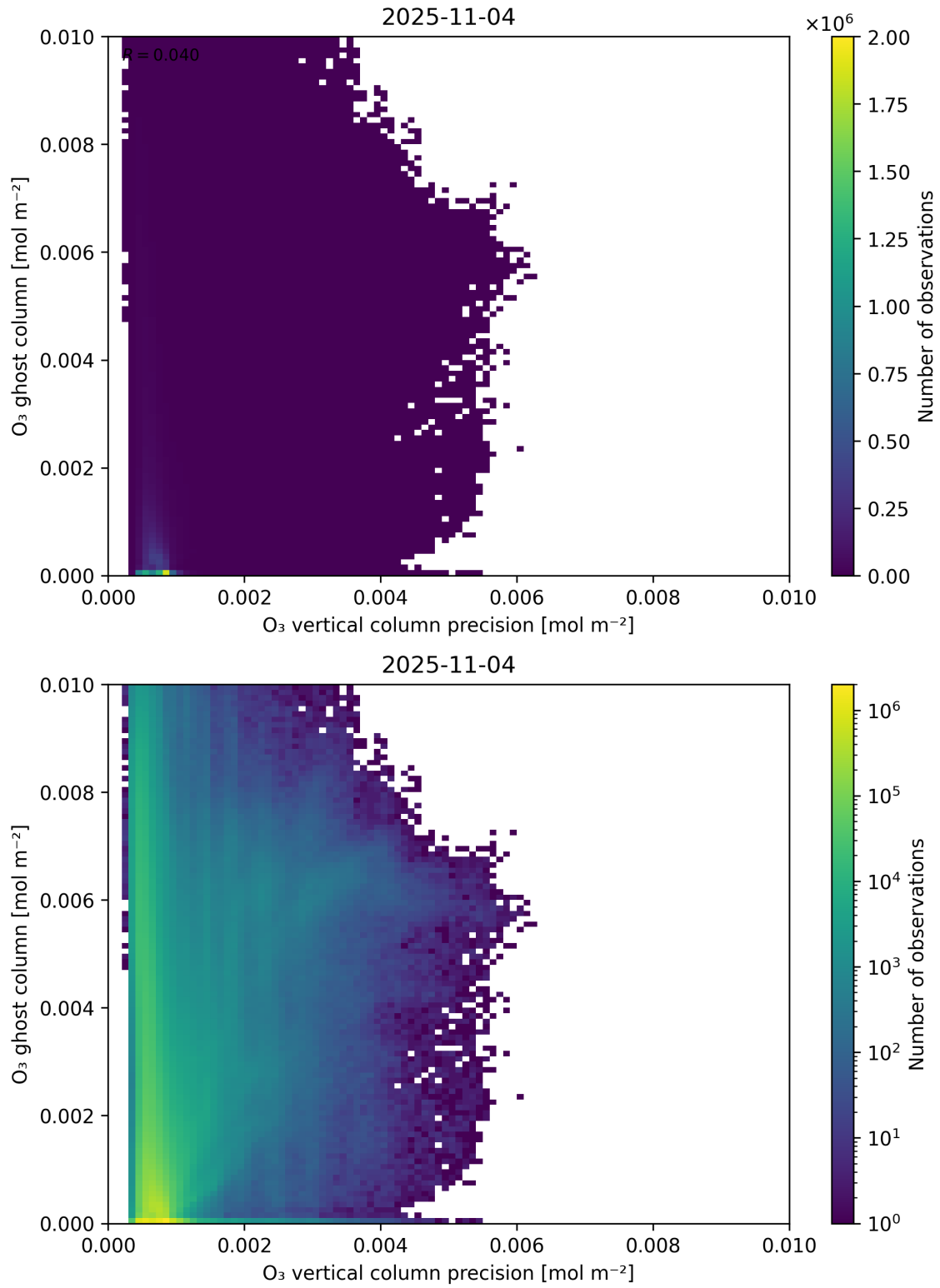
Figure 43: Scatter density plot of “ \text{O}_3 vertical column precision” against “ \text{O}_3 ghost column” for 2025-11-03 to 2025-11-05.
