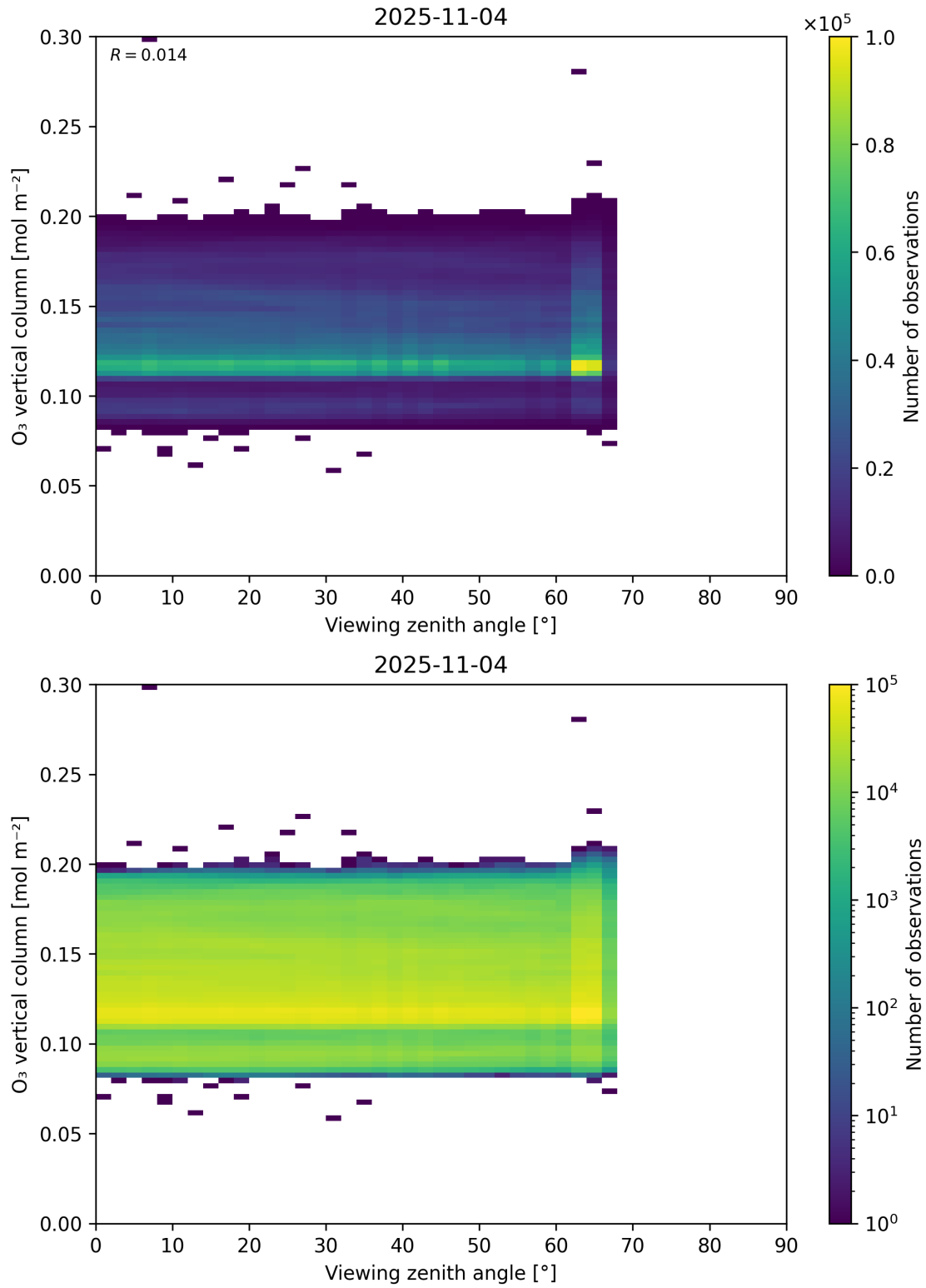
Figure 52: Scatter density plot of “Viewing zenith angle” against “O 3 vertical column” for 2025-11-03 to 2025-11-05.
