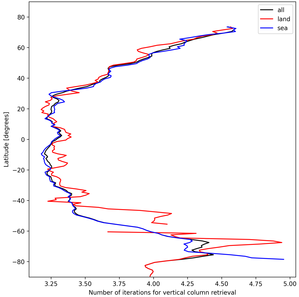
Figure 19: Zonal average of “Number of iterations for vertical column retrieval” for 2025-11-03 to 2025-11-05.
