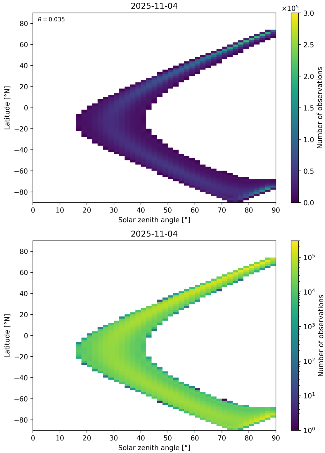
Figure 44: Scatter density plot of “Solar zenith angle” against “Latitude” for 2025-11-03 to 2025-11-05.
