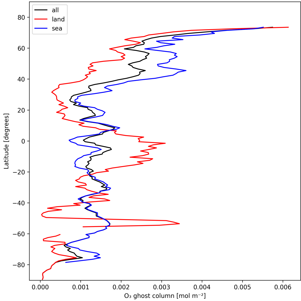
Figure 18: Zonal average of “O 3 ghost column” for 2025-11-03 to 2025-11-05.
