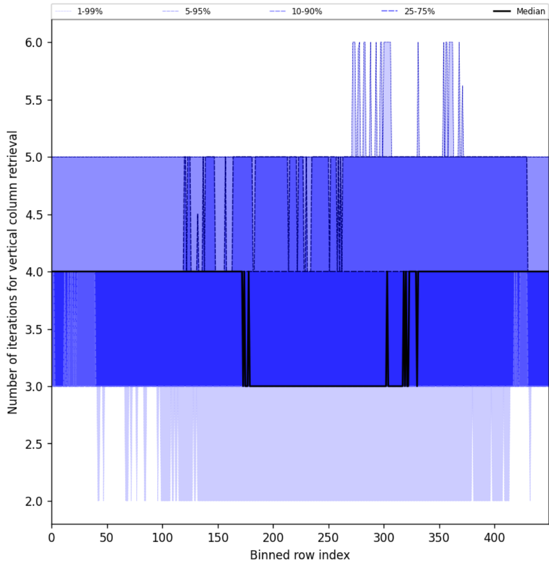
Figure 33: Along track statistics of “Number of iterations for vertical column retrieval” for 2025-11-03 to 2025-11-05
