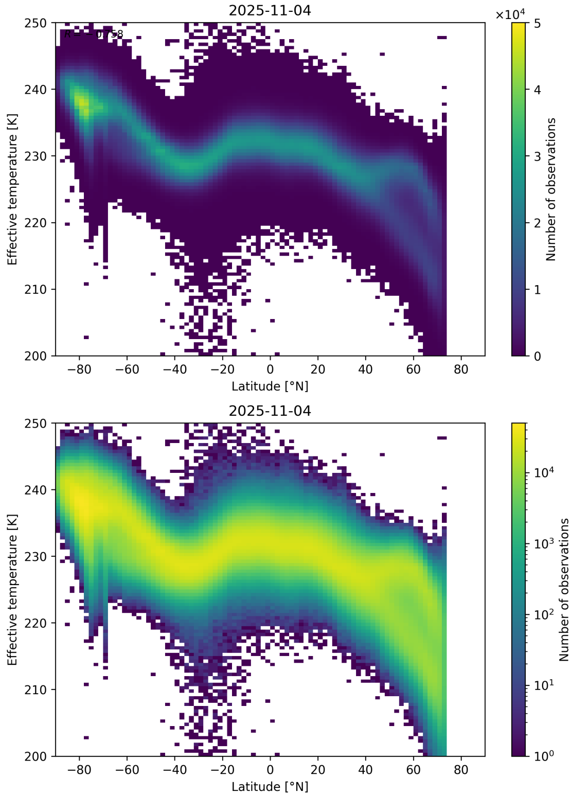
Figure 34: Scatter density plot of “Latitude” against “Effective temperature” for 2025-11-03 to 2025-11-05.
