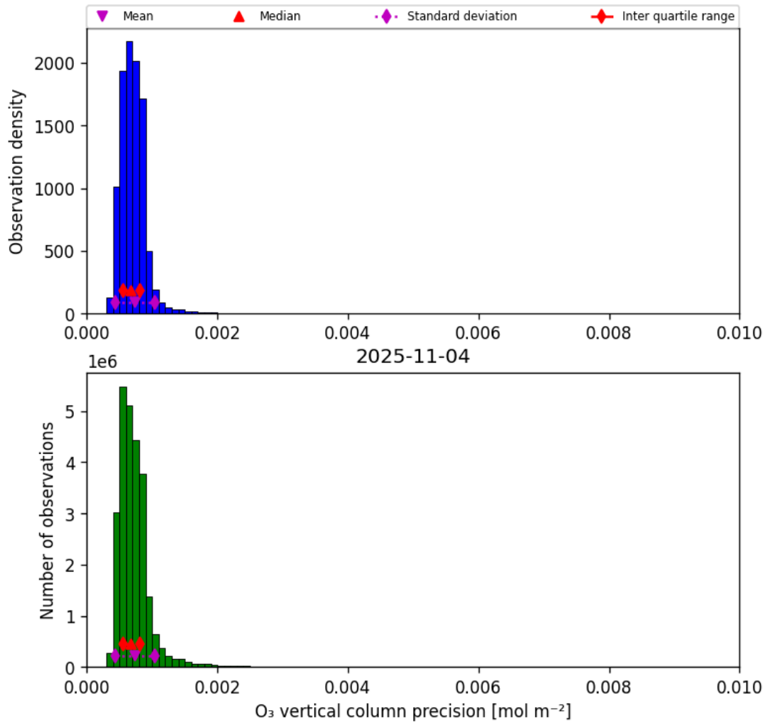
Figure 22: Histogram of “O 3 vertical column precision” for 2025-11-03 to 2025-11-05
