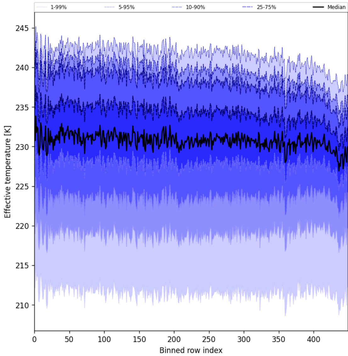
Figure 31: Along track statistics of “Effective temperature” for 2025-11-03 to 2025-11-05
