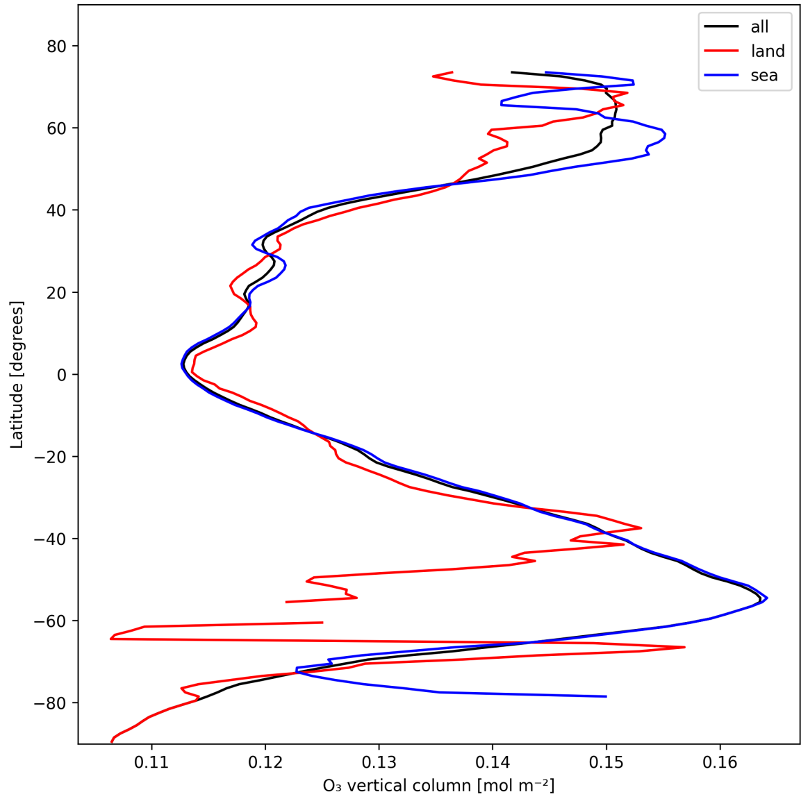
Figure 14: Zonal average of “O 3 vertical column” for 2025-11-03 to 2025-11-05.
