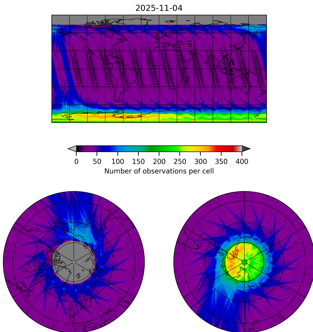
Figure 12: Map of the number of observations for 2025-11-03 to 2025-11-05
