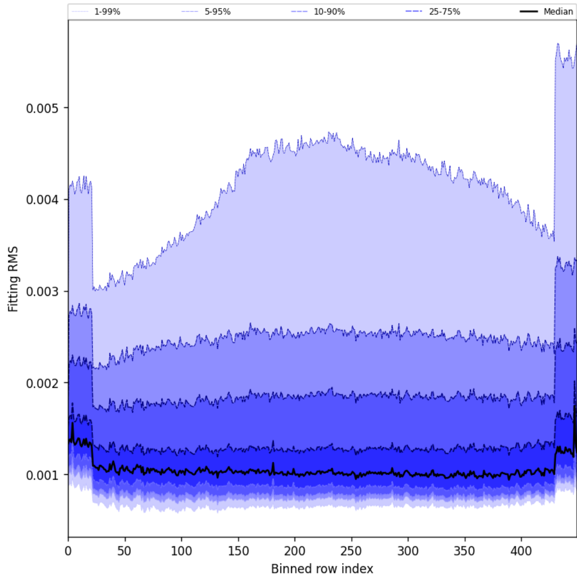
Figure 30: Along track statistics of “Fitting RMS” for 2025-11-03 to 2025-11-05
