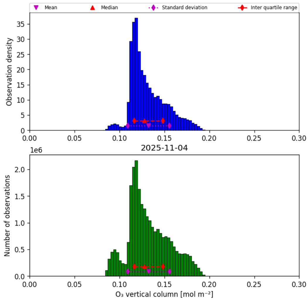
Figure 21: Histogram of “O 3 vertical column” for 2025-11-03 to 2025-11-05
