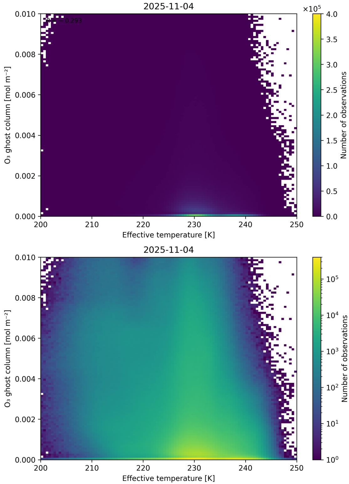
Figure 38: Scatter density plot of “Effective temperature” against “O 3 ghost column” for 2025-11-03 to 2025-11-05.
