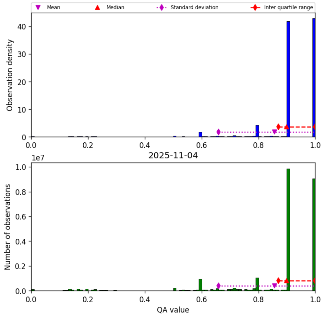
Figure 20: Histogram of “QA value” for 2025-11-03 to 2025-11-05
