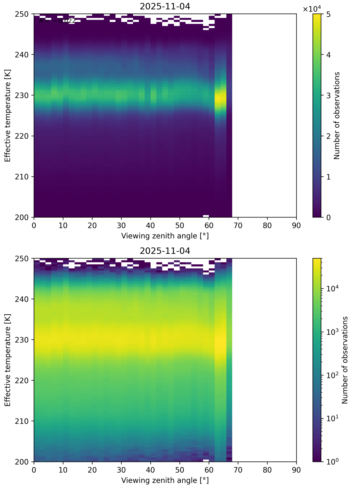
Figure 50: Scatter density plot of “Viewing zenith angle” against “Effective temperature” for 2025-11-03 to 2025-11-05.
