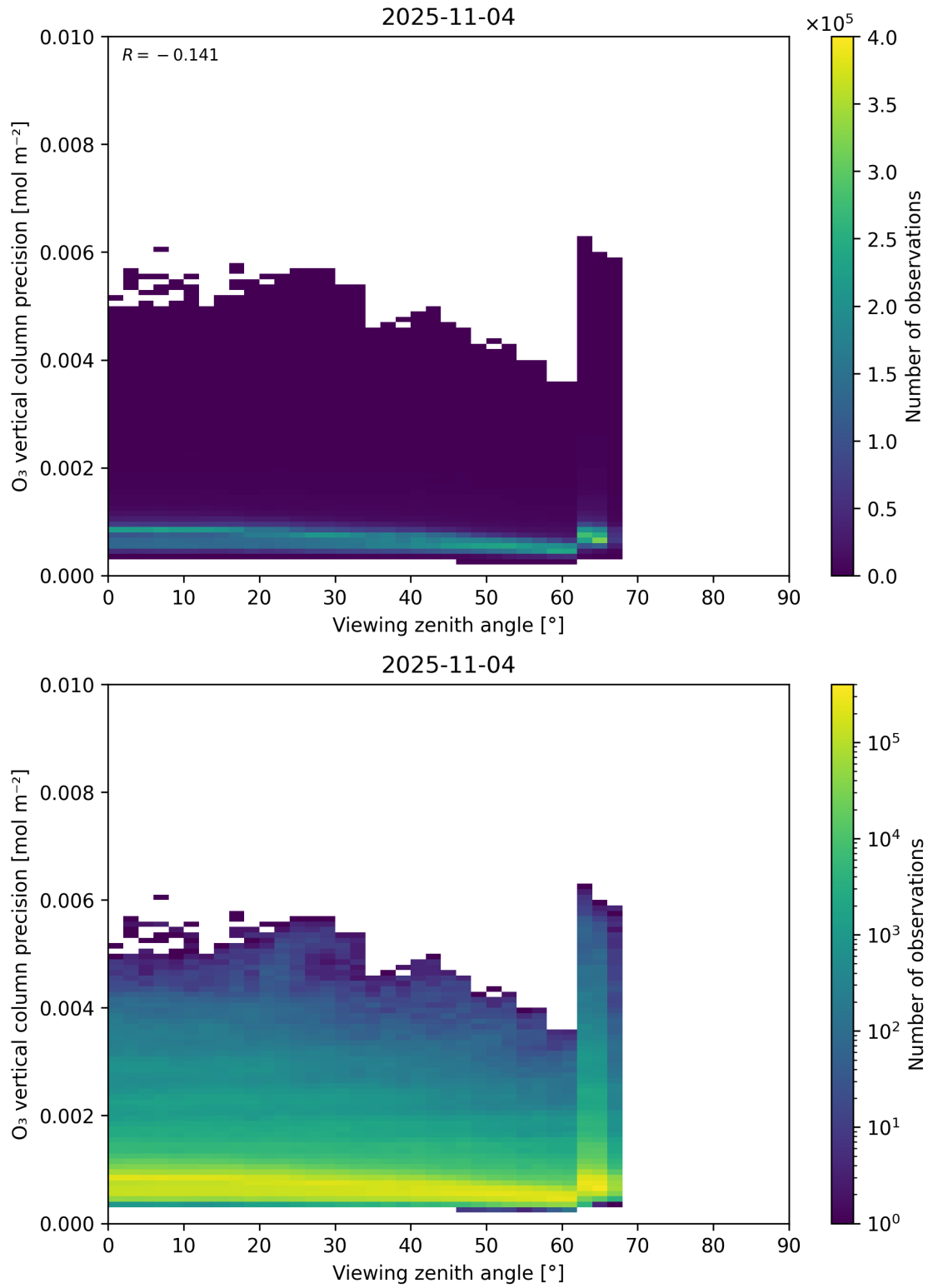
Figure 53: Scatter density plot of “Viewing zenith angle” against “O 3 vertical column precision” for 2025-11-03 to 2025-11-05.
