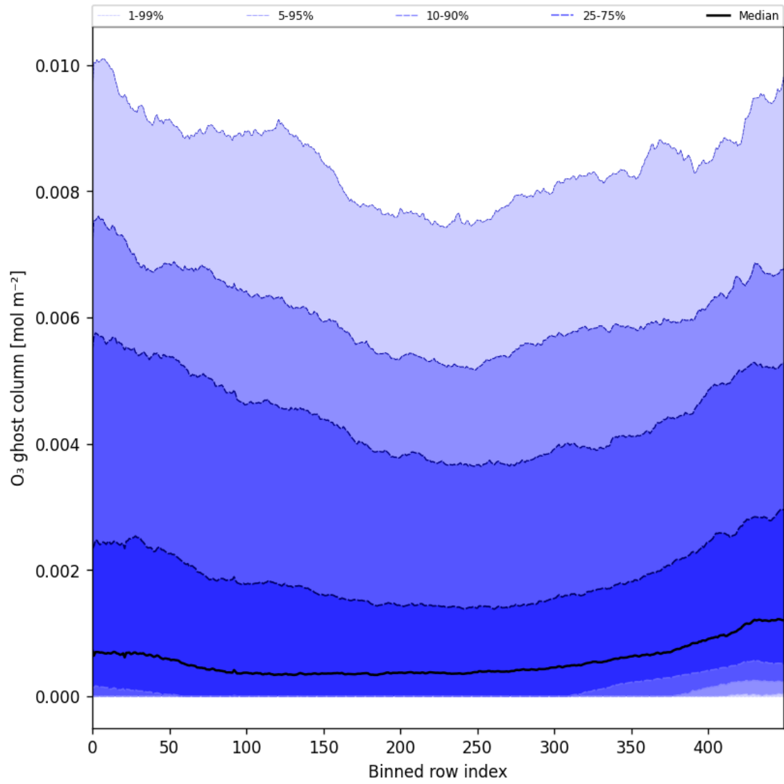
Figure 32: Along track statistics of “O 3 ghost column” for 2025-11-03 to 2025-11-05
