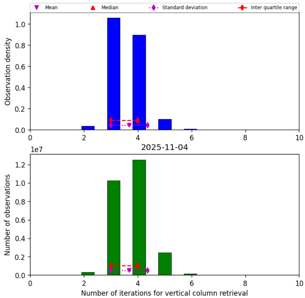
Figure 26: Histogram of “Number of iterations for vertical column retrieval” for 2025-11-03 to 2025-11-05
