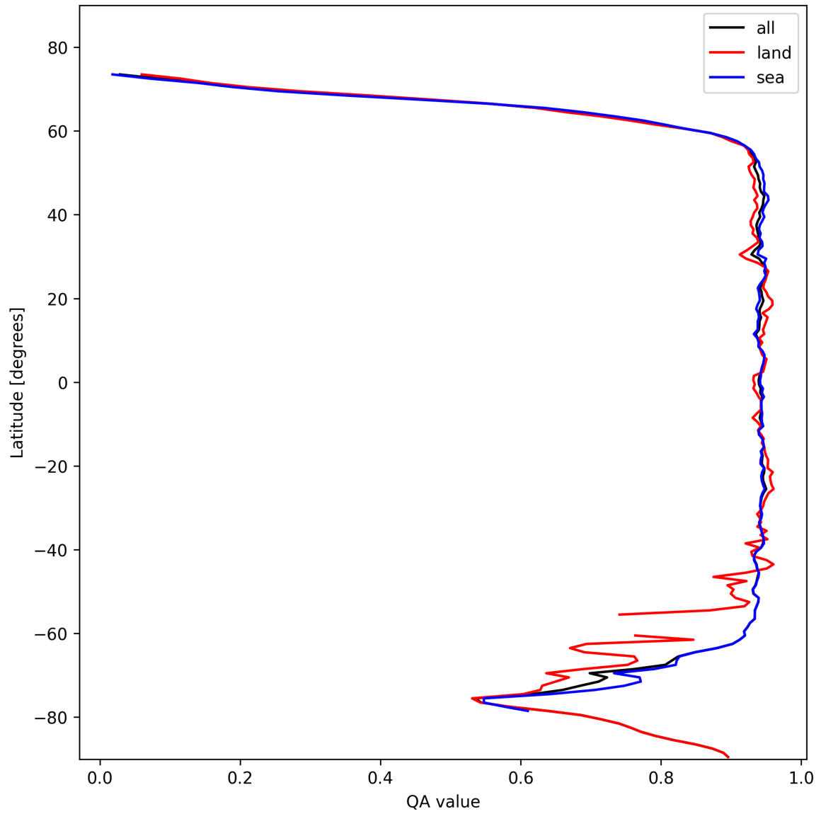
Figure 13: Zonal average of “QA value” for 2025-11-03 to 2025-11-05.
