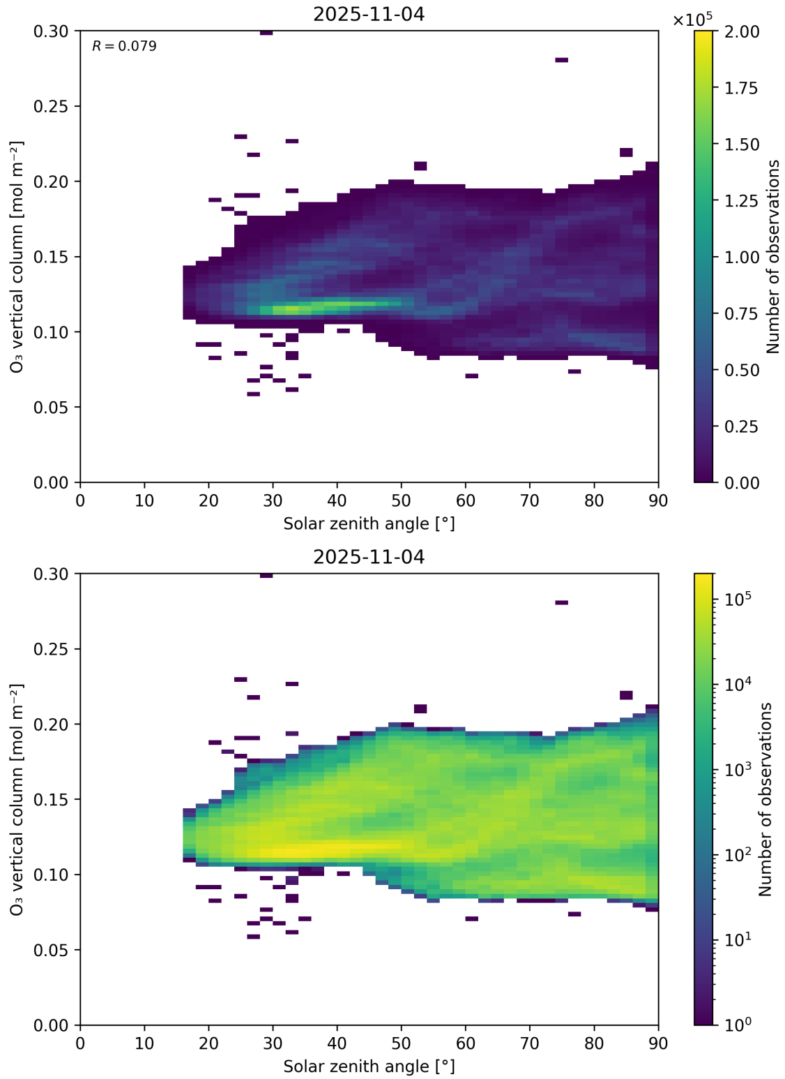
Figure 47: Scatter density plot of “Solar zenith angle” against “O 3 vertical column” for 2025-11-03 to 2025-11-05.
