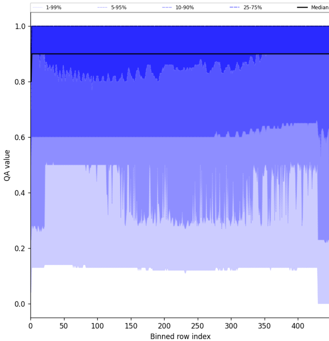
Figure 27: Along track statistics of “QA value” for 2025-11-03 to 2025-11-05
