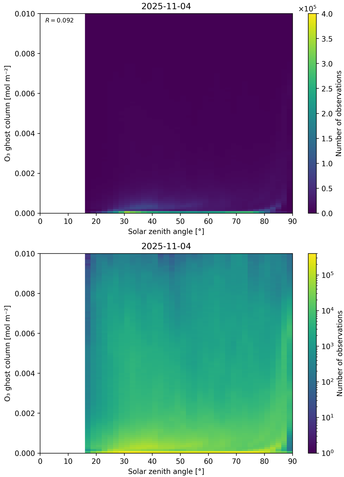
Figure 46: Scatter density plot of “Solar zenith angle” against “O 3 ghost column” for 2025-11-03 to 2025-11-05.
