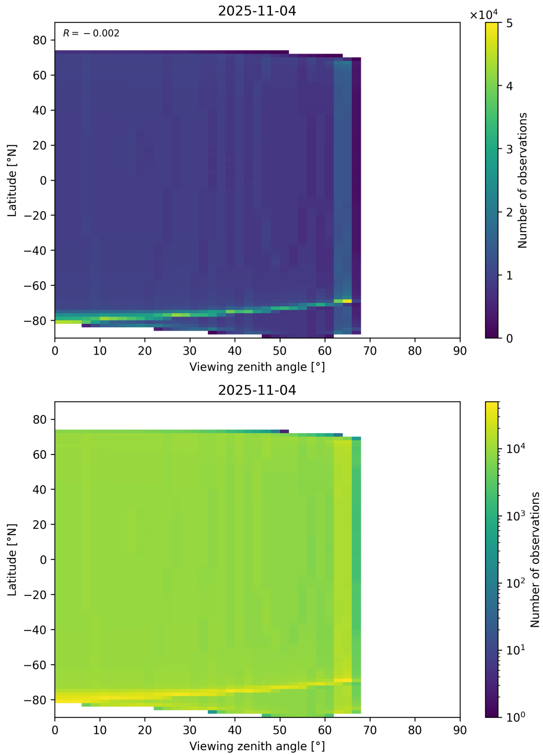
Figure 49: Scatter density plot of “Viewing zenith angle” against “Latitude” for 2025-11-03 to 2025-11-05.
