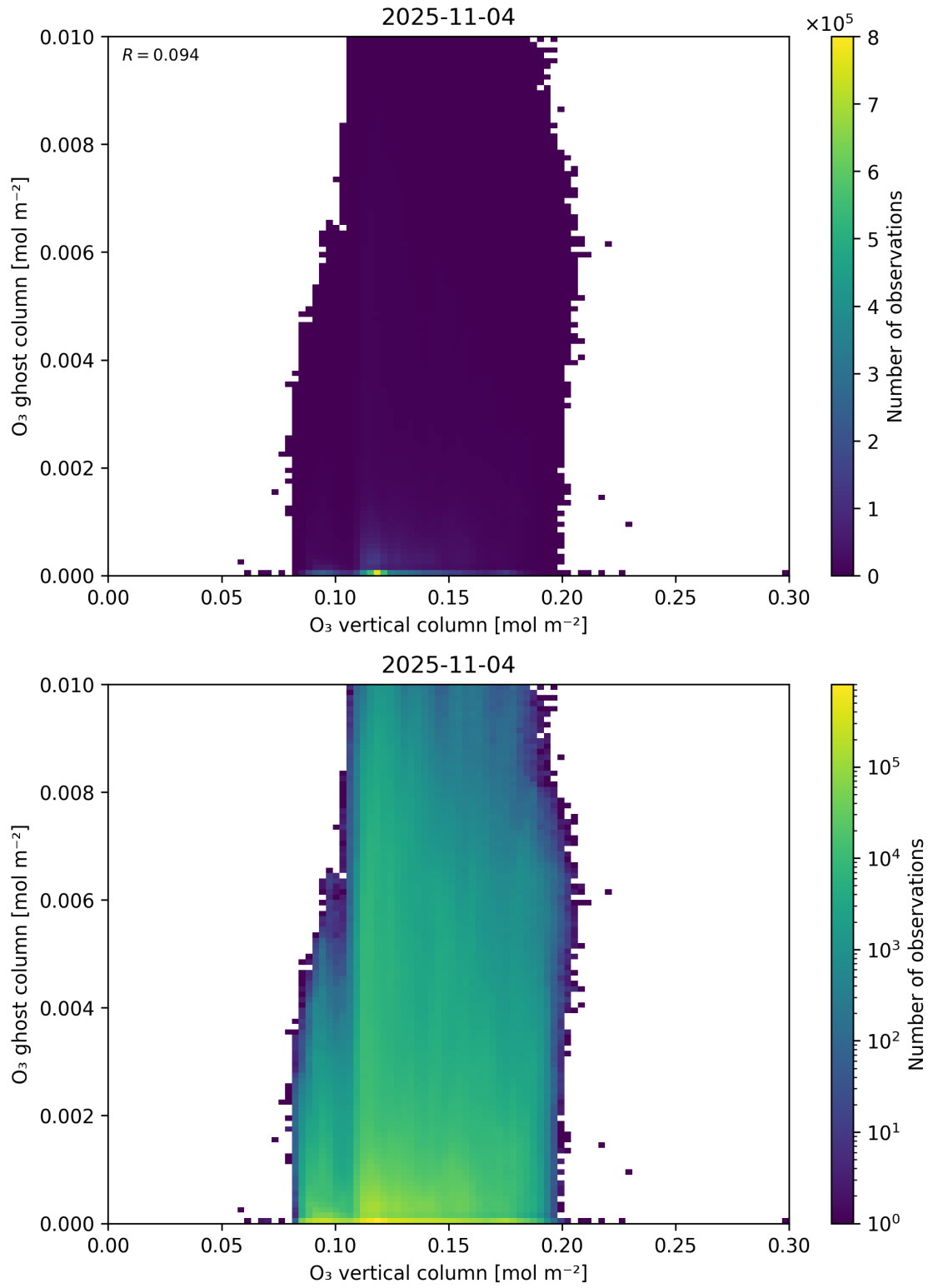
Figure 40: Scatter density plot of “O 3 vertical column” against “O 3 ghost column” for 2025-11-03 to 2025-11-05.
