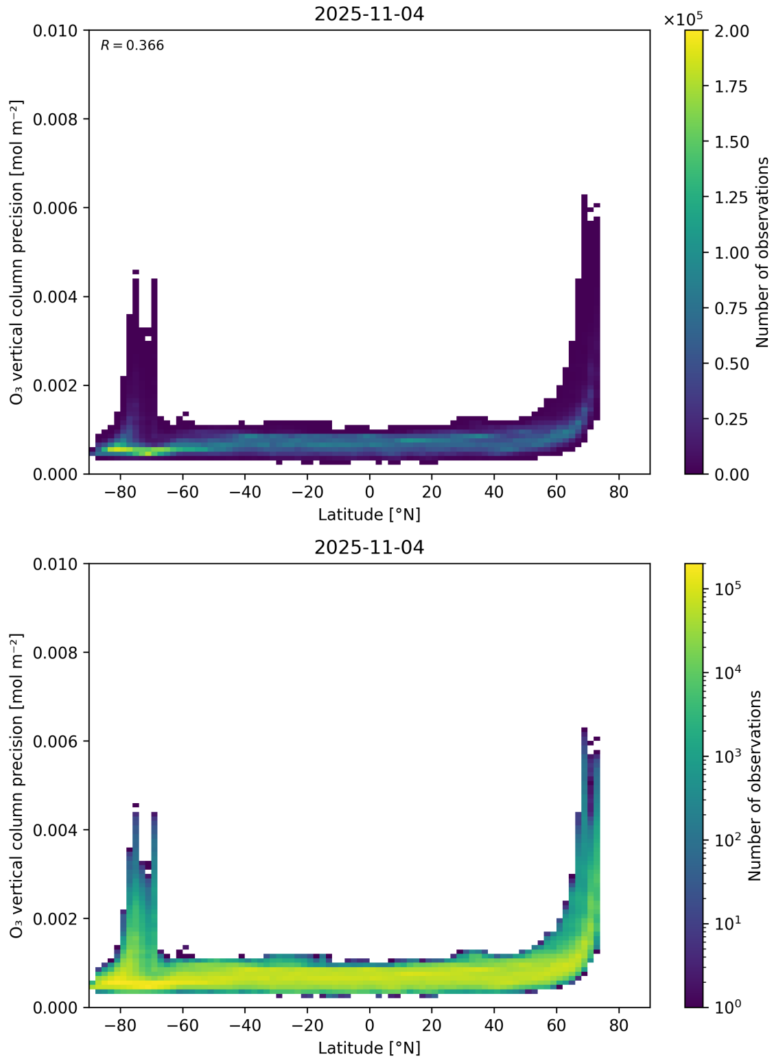
Figure 37: Scatter density plot of “Latitude” against “O 3 vertical column precision” for 2025-11-03 to 2025-11-05.
