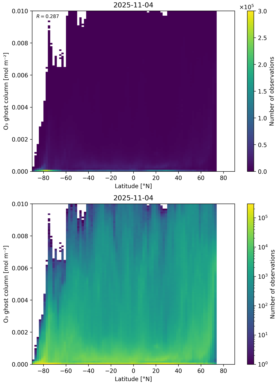
Figure 35: Scatter density plot of “Latitude” against “O 3 ghost column” for 2025-11-03 to 2025-11-05.
