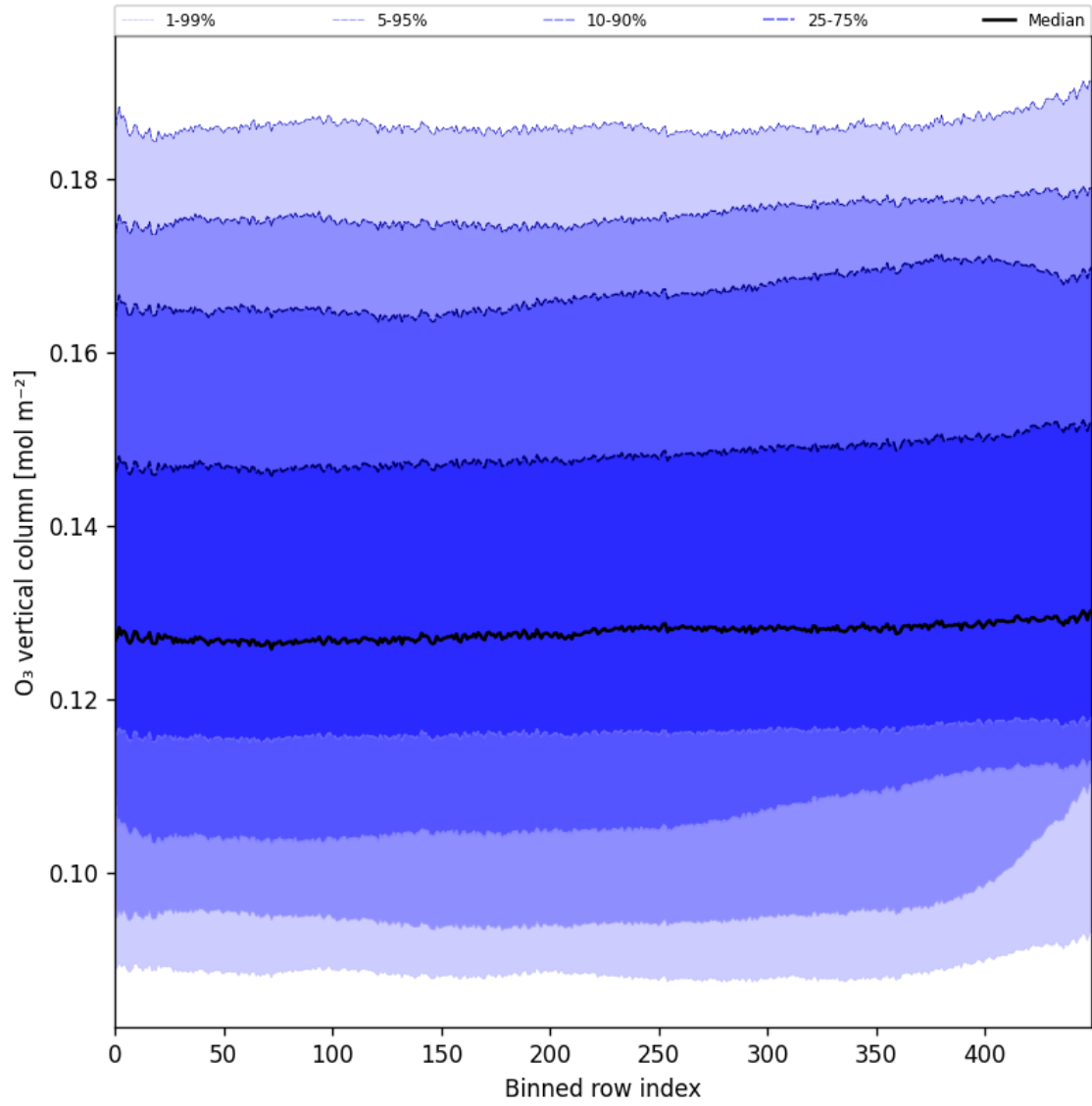
Figure 28: Along track statistics of “O 3 vertical column” for 2025-11-03 to 2025-11-05
