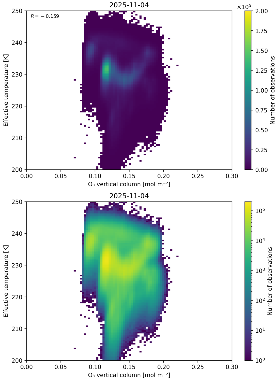
Figure 39: Scatter density plot of “O 3 vertical column” against “Effective temperature” for 2025-11-03 to 2025-11-05.
