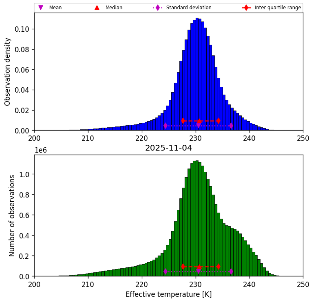
Figure 24: Histogram of “Effective temperature” for 2025-11-03 to 2025-11-05
