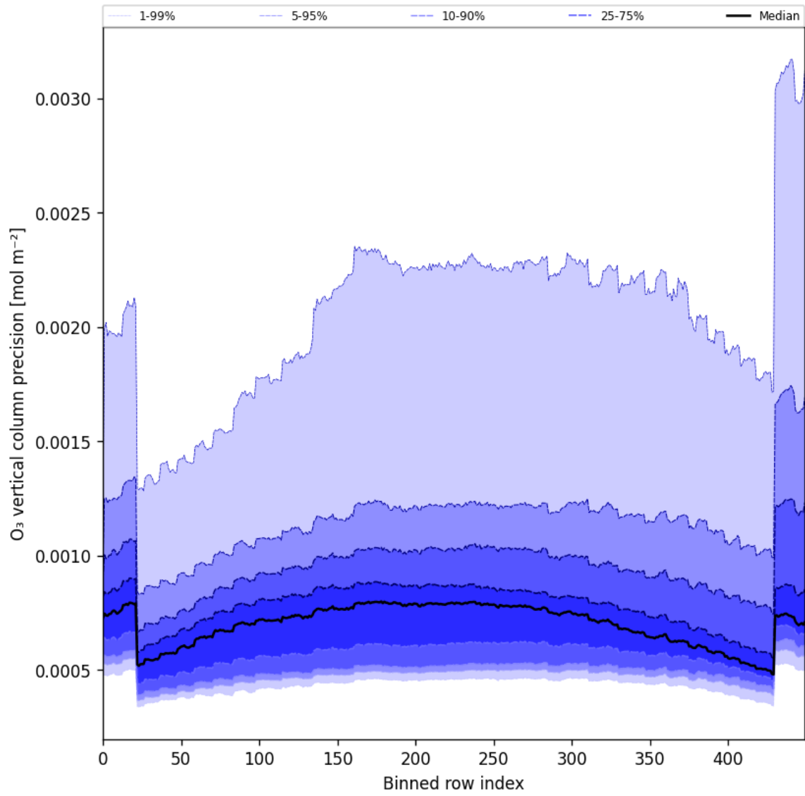
Figure 29: Along track statistics of “O 3 vertical column precision” for 2025-11-03 to 2025-11-05
