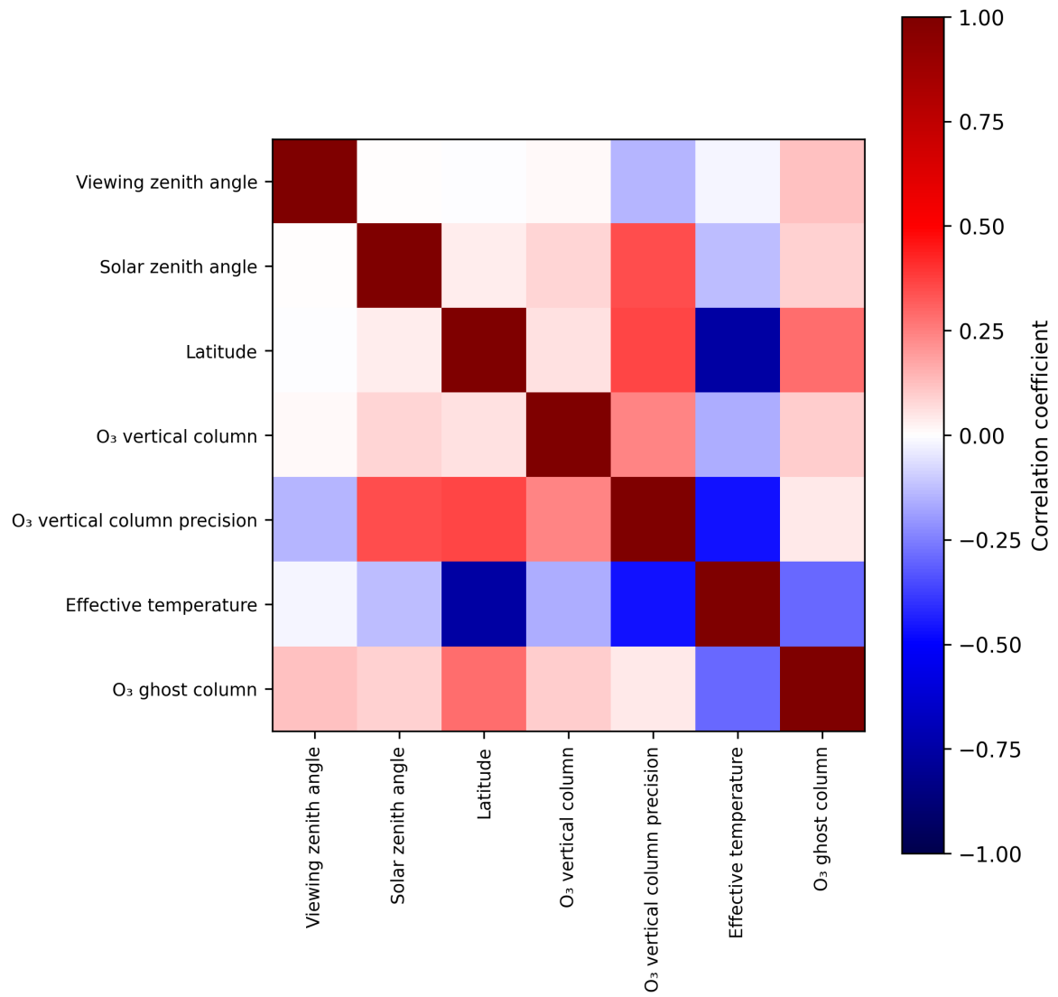
Figure 2: Map of correlation matrix for 2025-11-03 to 2025-11-05.
