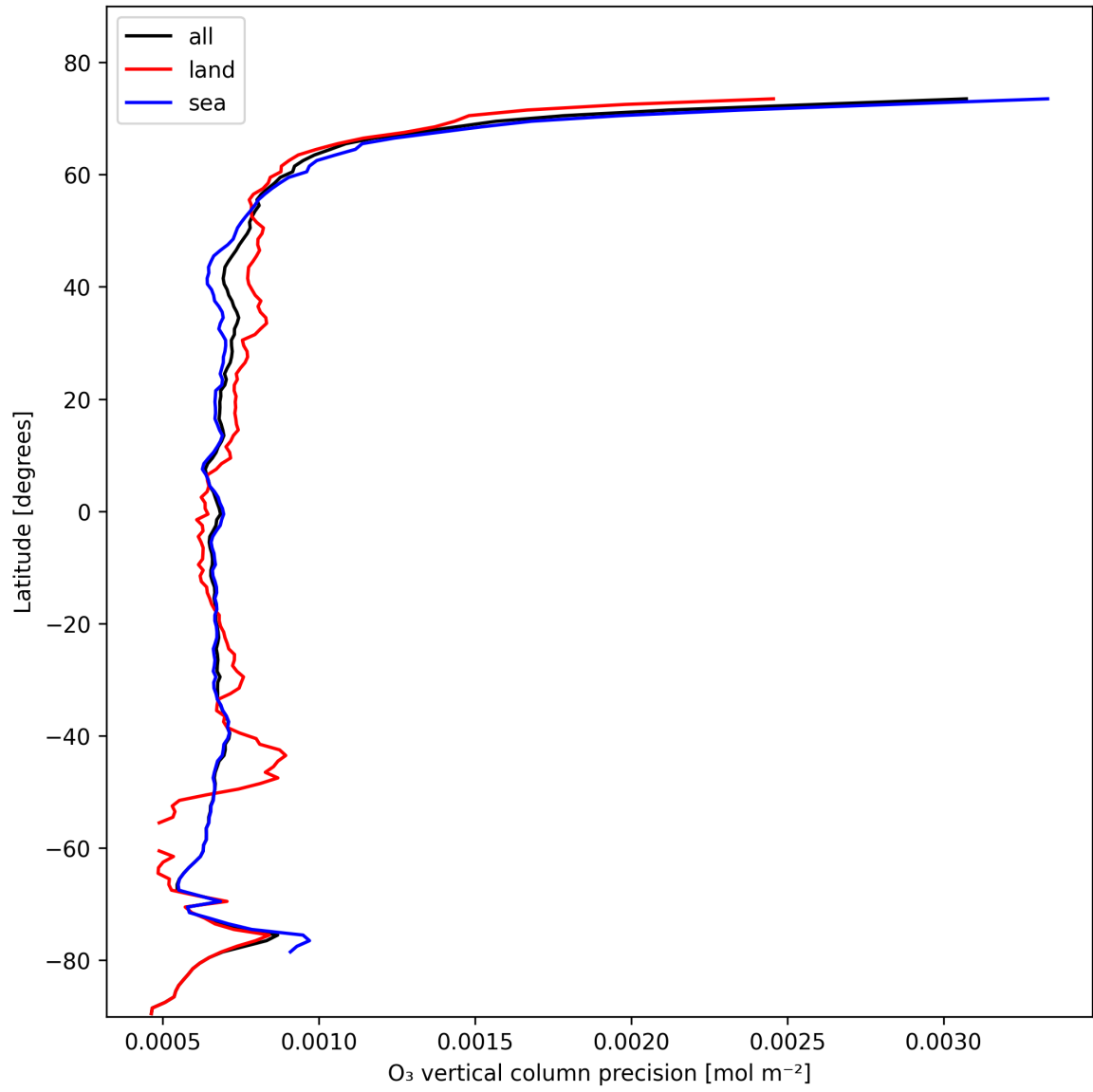
Figure 15: Zonal average of “O 3 vertical column precision” for 2025-11-03 to 2025-11-05.
