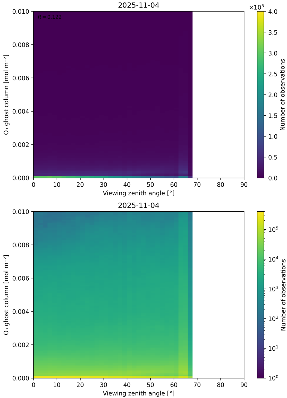
Figure 51: Scatter density plot of “Viewing zenith angle” against “O 3 ghost column” for 2025-11-03 to 2025-11-05.
