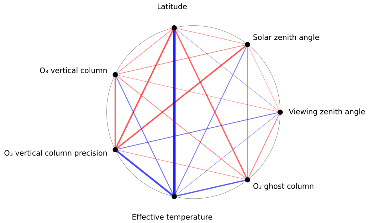
Figure 1: Map of correlation graph for 2025-11-03 to 2025-11-05.
