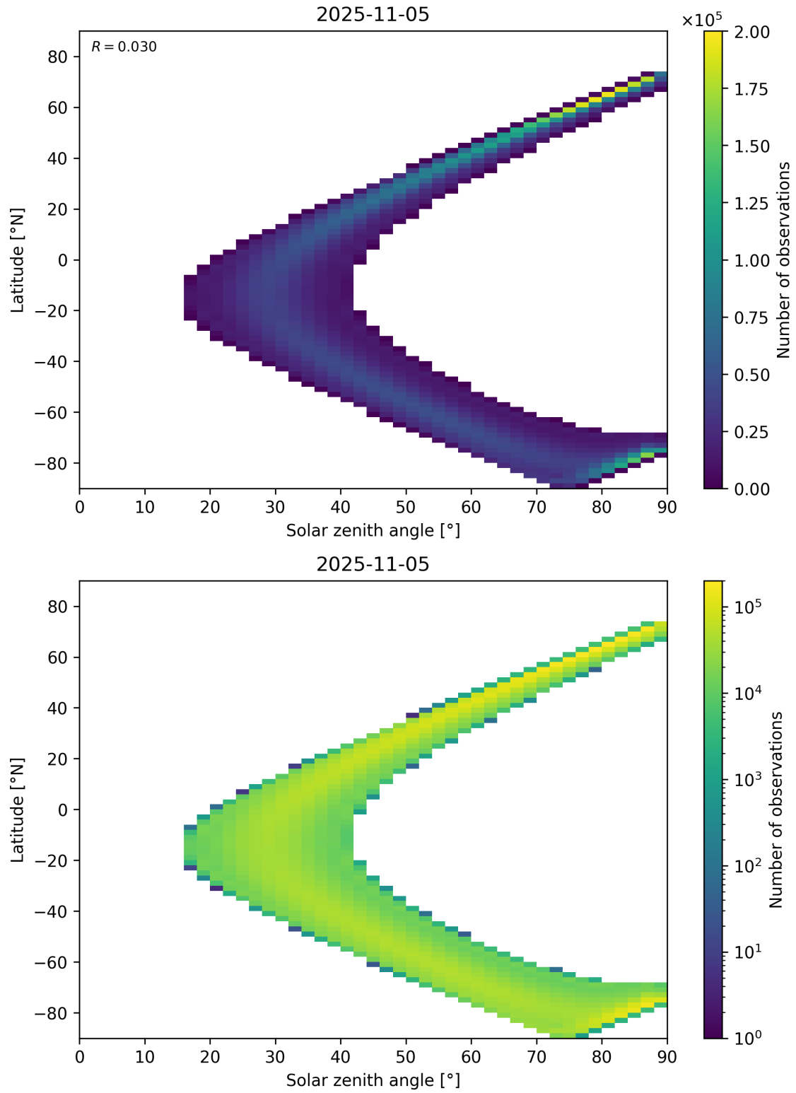
Figure 44: Scatter density plot of “Solar zenith angle” against “Latitude” for 2025-11-04 to 2025-11-06.
