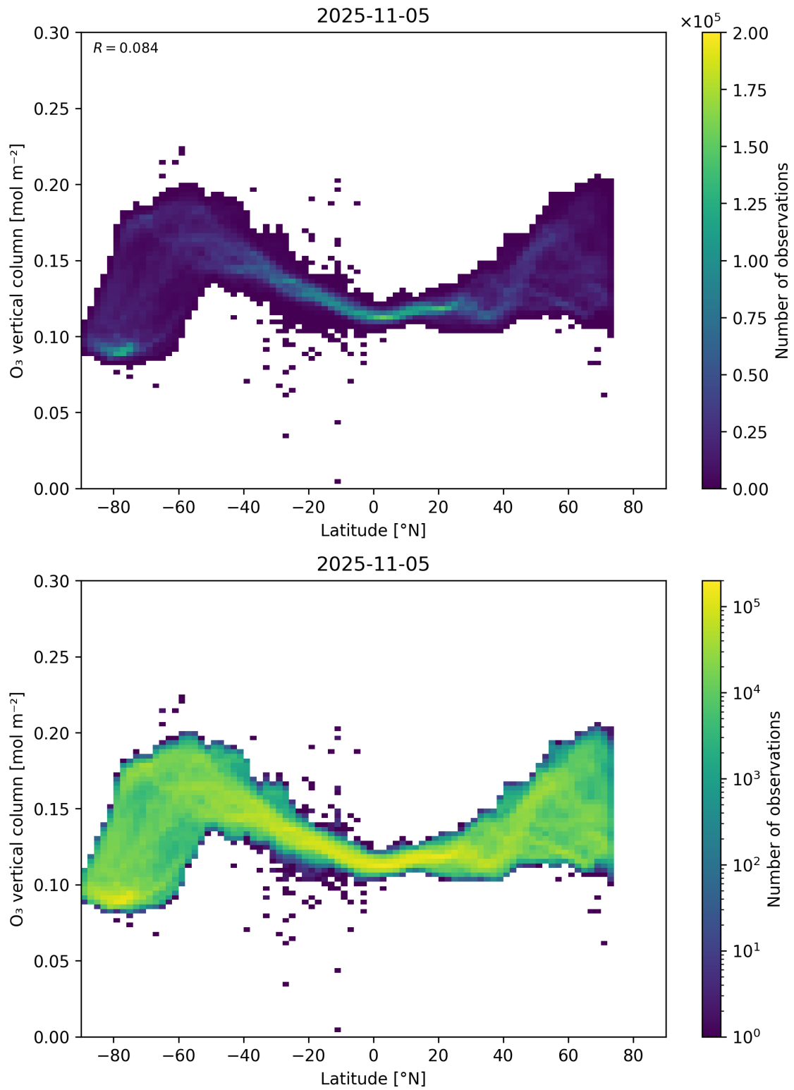
Figure 36: Scatter density plot of “Latitude” against “O 3 vertical column” for 2025-11-04 to 2025-11-06.
