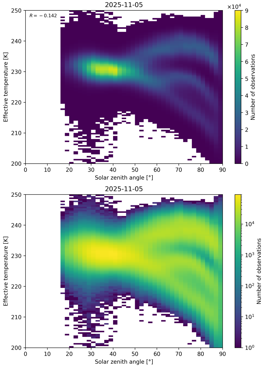
Figure 45: Scatter density plot of “Solar zenith angle” against “Effective temperature” for 2025-11-04 to 2025-11-06.
