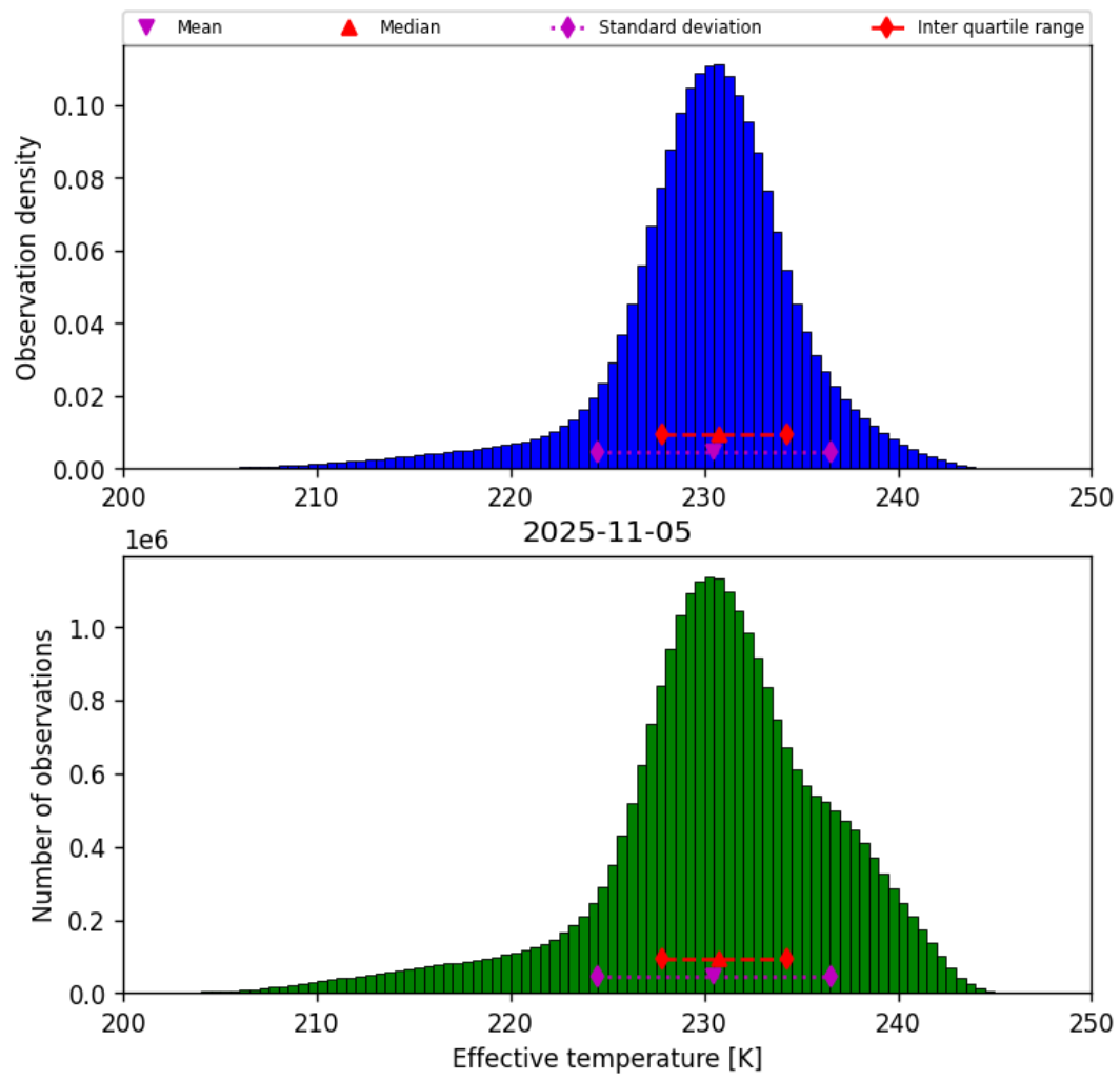
Figure 24: Histogram of “Effective temperature” for 2025-11-04 to 2025-11-06
