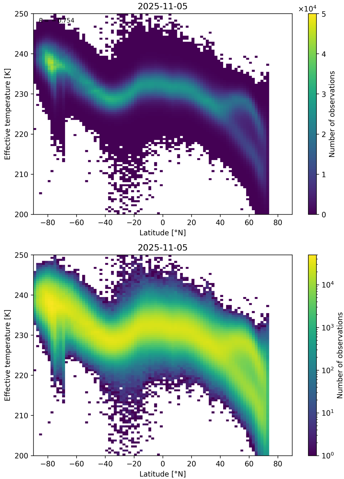
Figure 34: Scatter density plot of “Latitude” against “Effective temperature” for 2025-11-04 to 2025-11-06.
