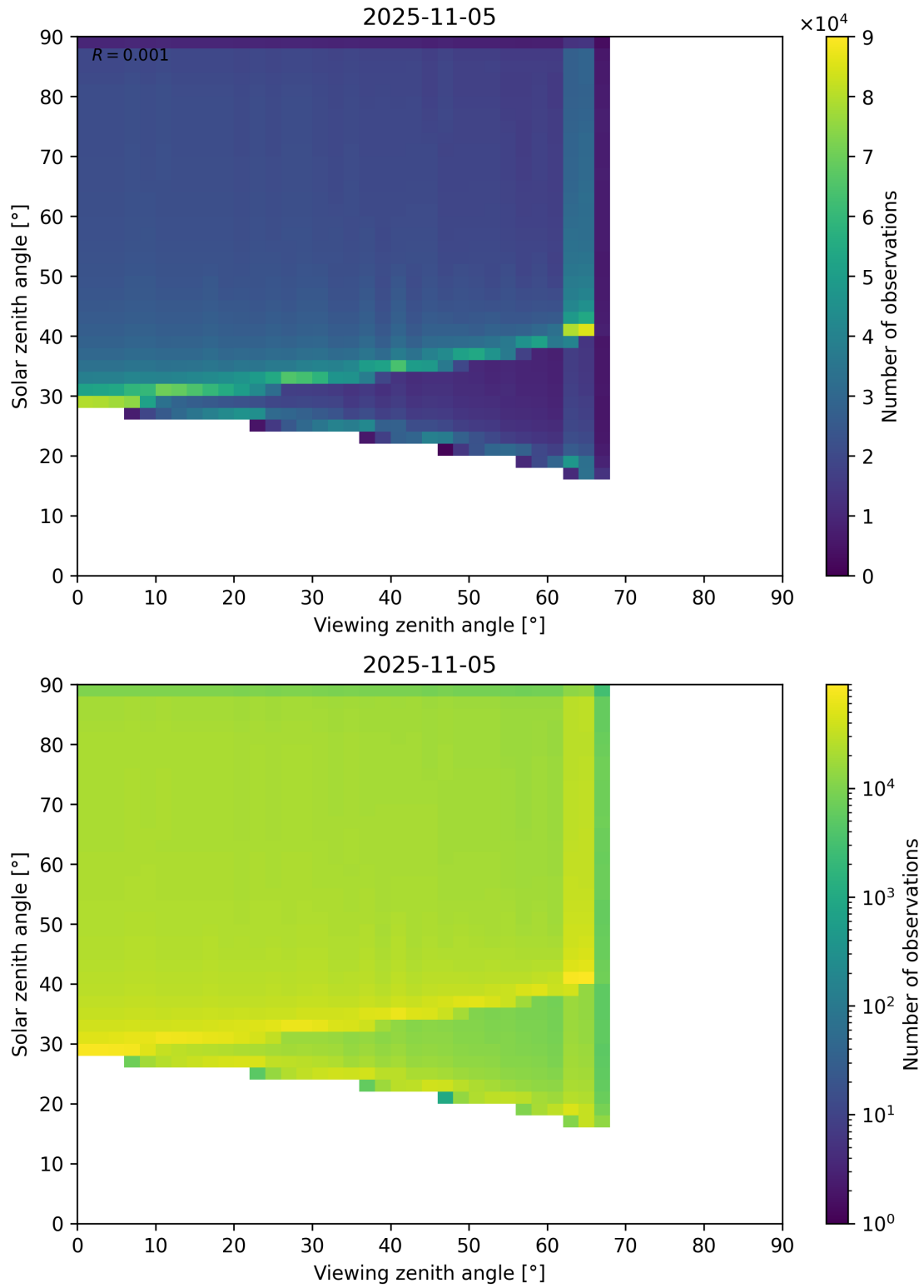
Figure 54: Scatter density plot of “Viewing zenith angle” against “Solar zenith angle” for 2025-11-04 to 2025-11-06.
