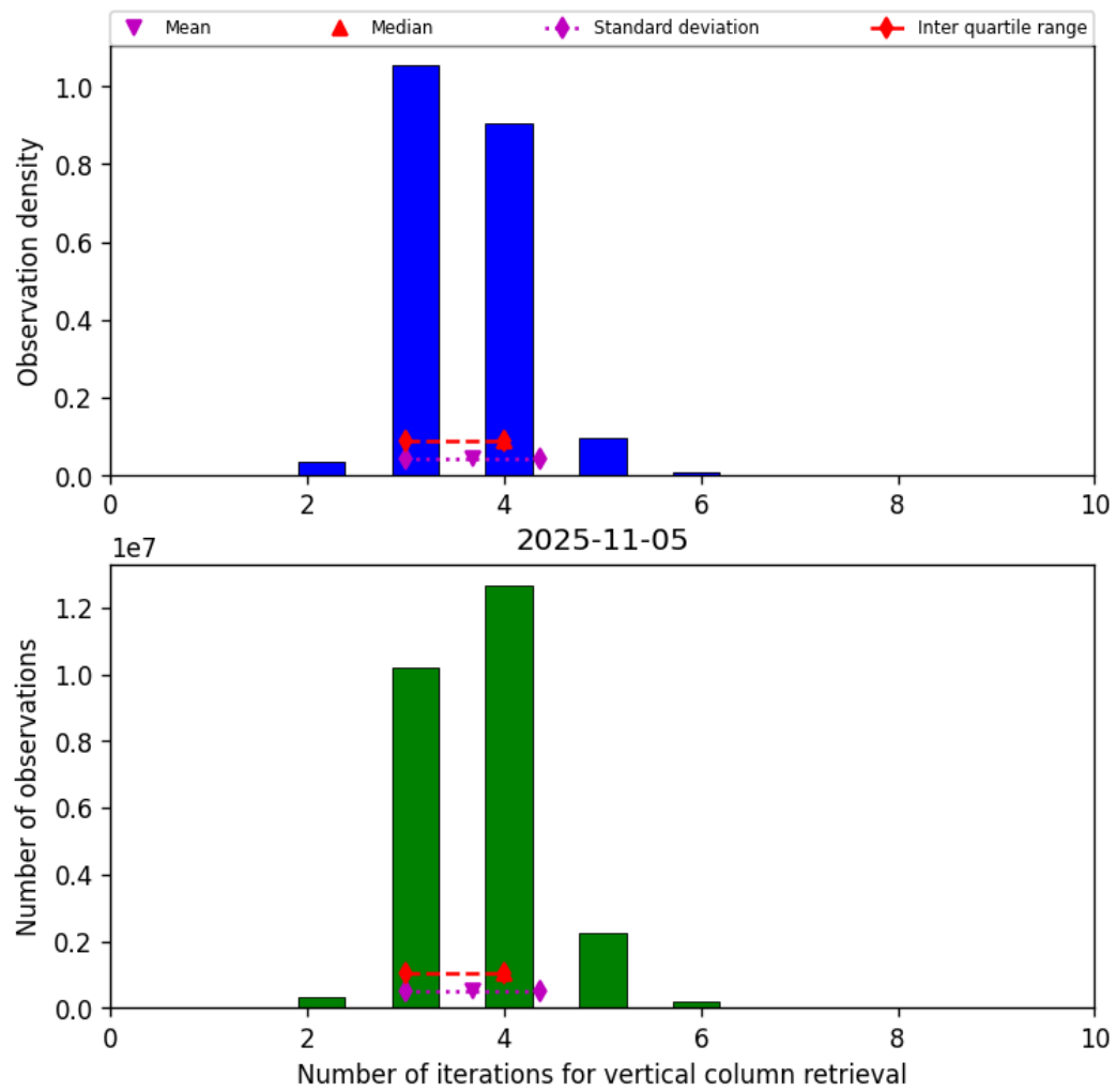
Figure 26: Histogram of “Number of iterations for vertical column retrieval” for 2025-11-04 to 2025-11-06
