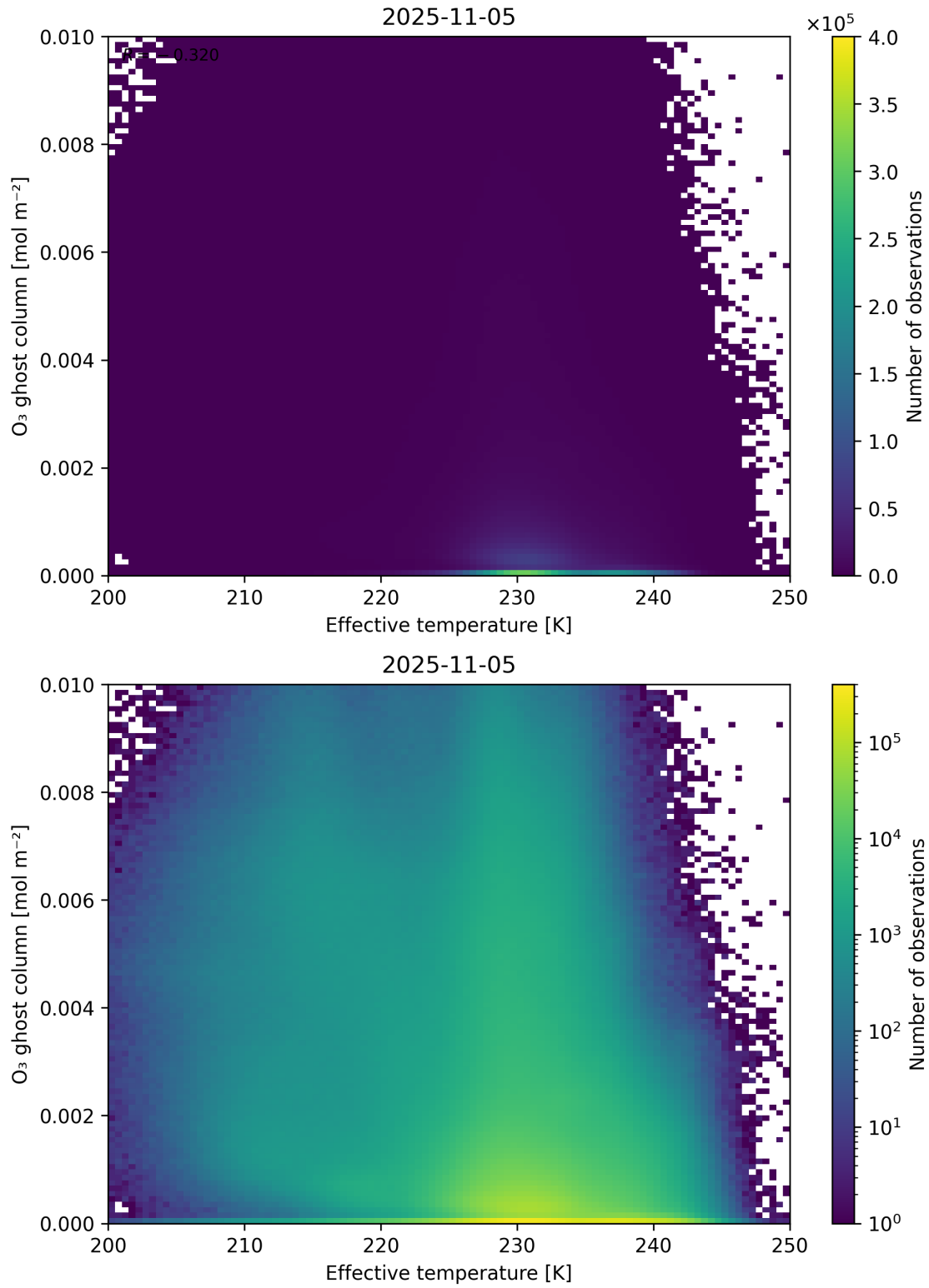
Figure 38: Scatter density plot of “Effective temperature” against “O 3 ghost column” for 2025-11-04 to 2025-11-06.
