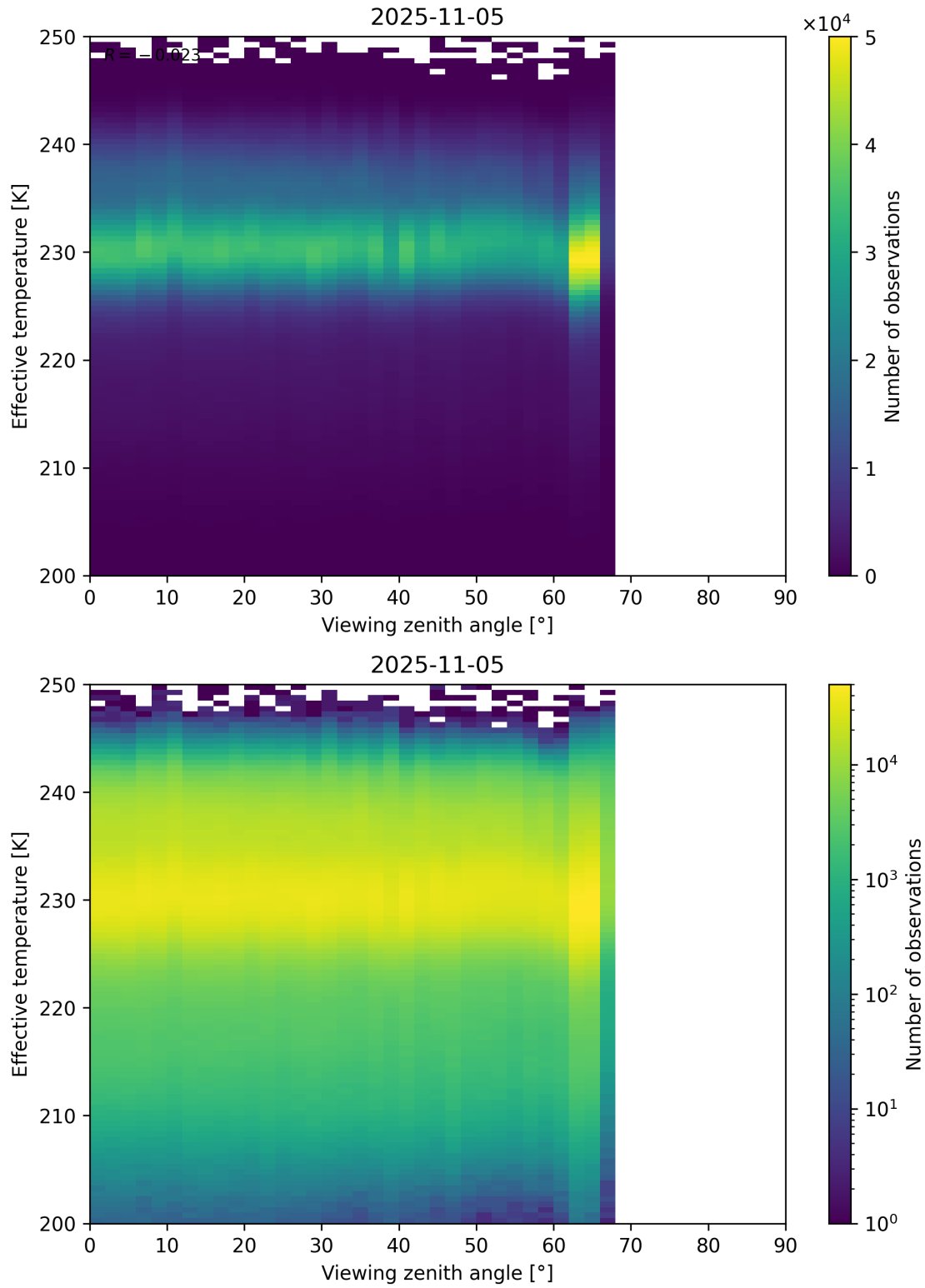
Figure 50: Scatter density plot of “Viewing zenith angle” against “Effective temperature” for 2025-11-04 to 2025-11-06.
