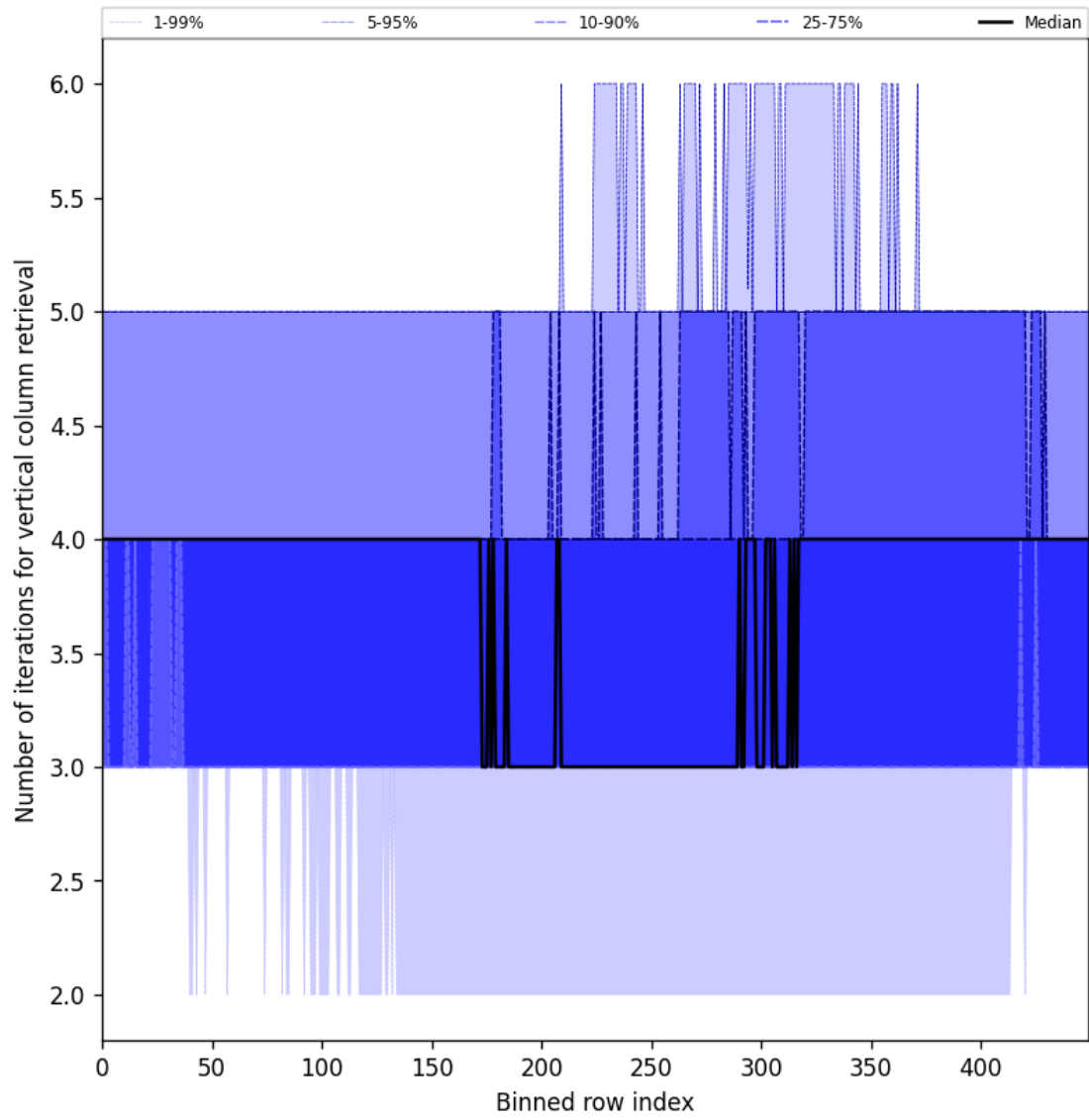
Figure 33: Along track statistics of “Number of iterations for vertical column retrieval” for 2025-11-04 to 2025-11-06
