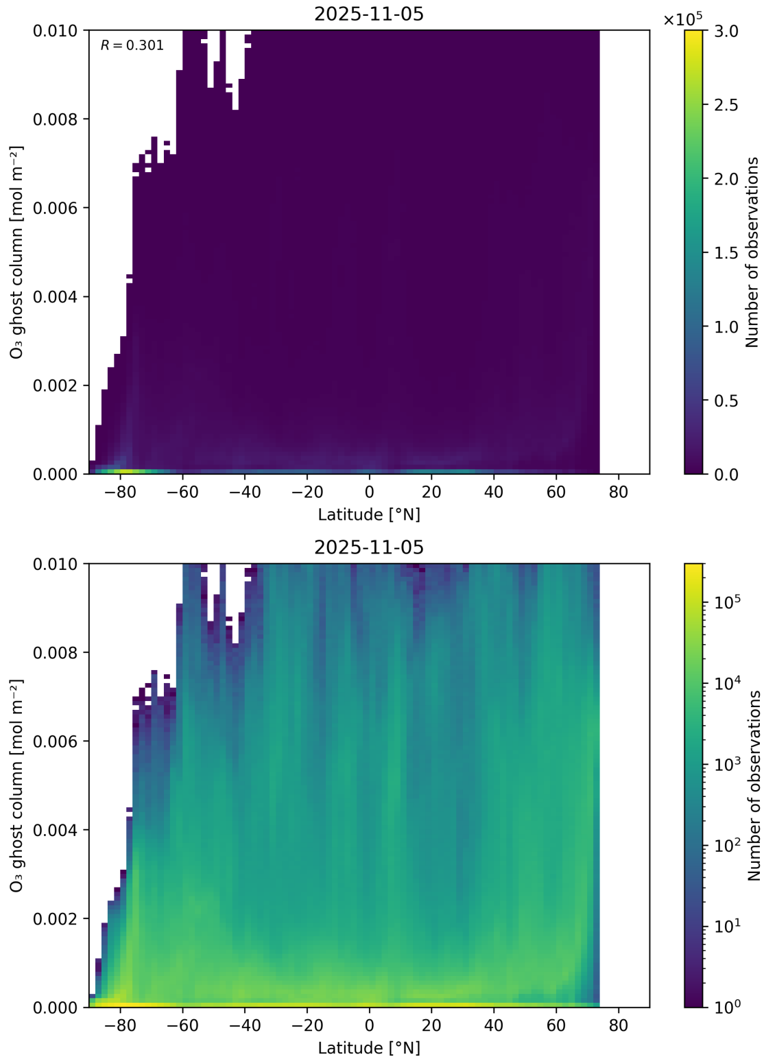
Figure 35: Scatter density plot of “Latitude” against “O 3 ghost column” for 2025-11-04 to 2025-11-06.
