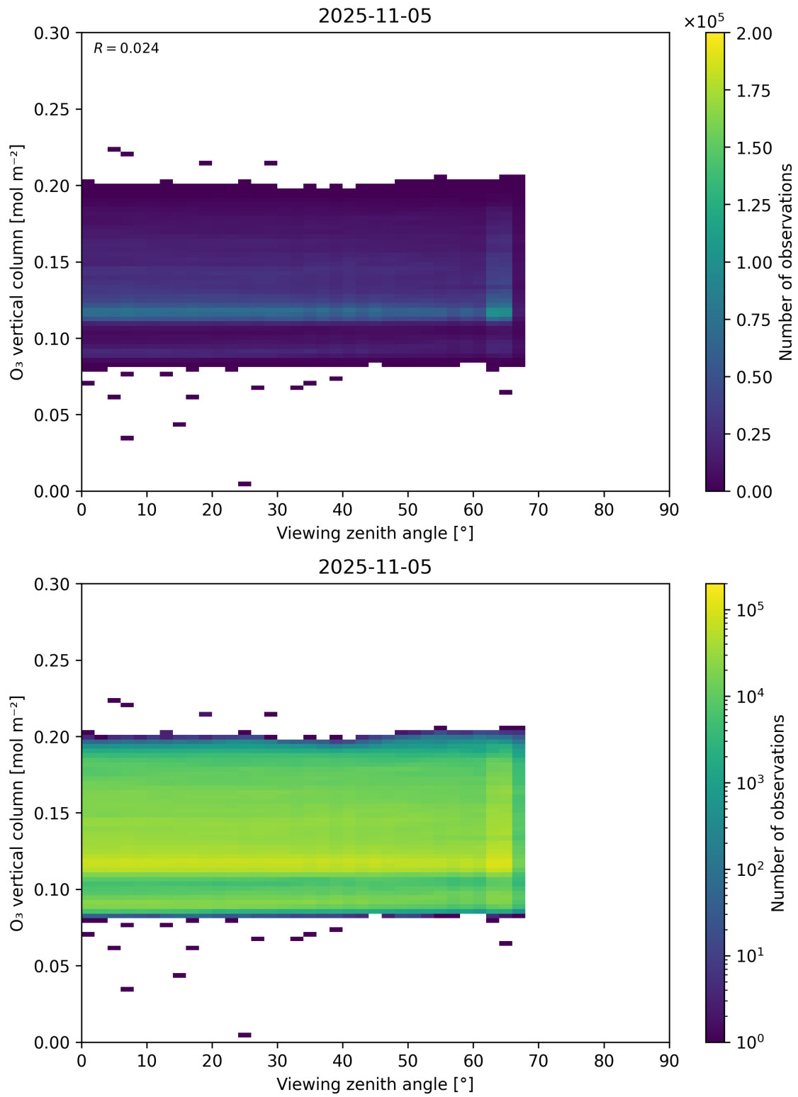
Figure 52: Scatter density plot of “Viewing zenith angle” against “O 3 vertical column” for 2025-11-04 to 2025-11-06.
