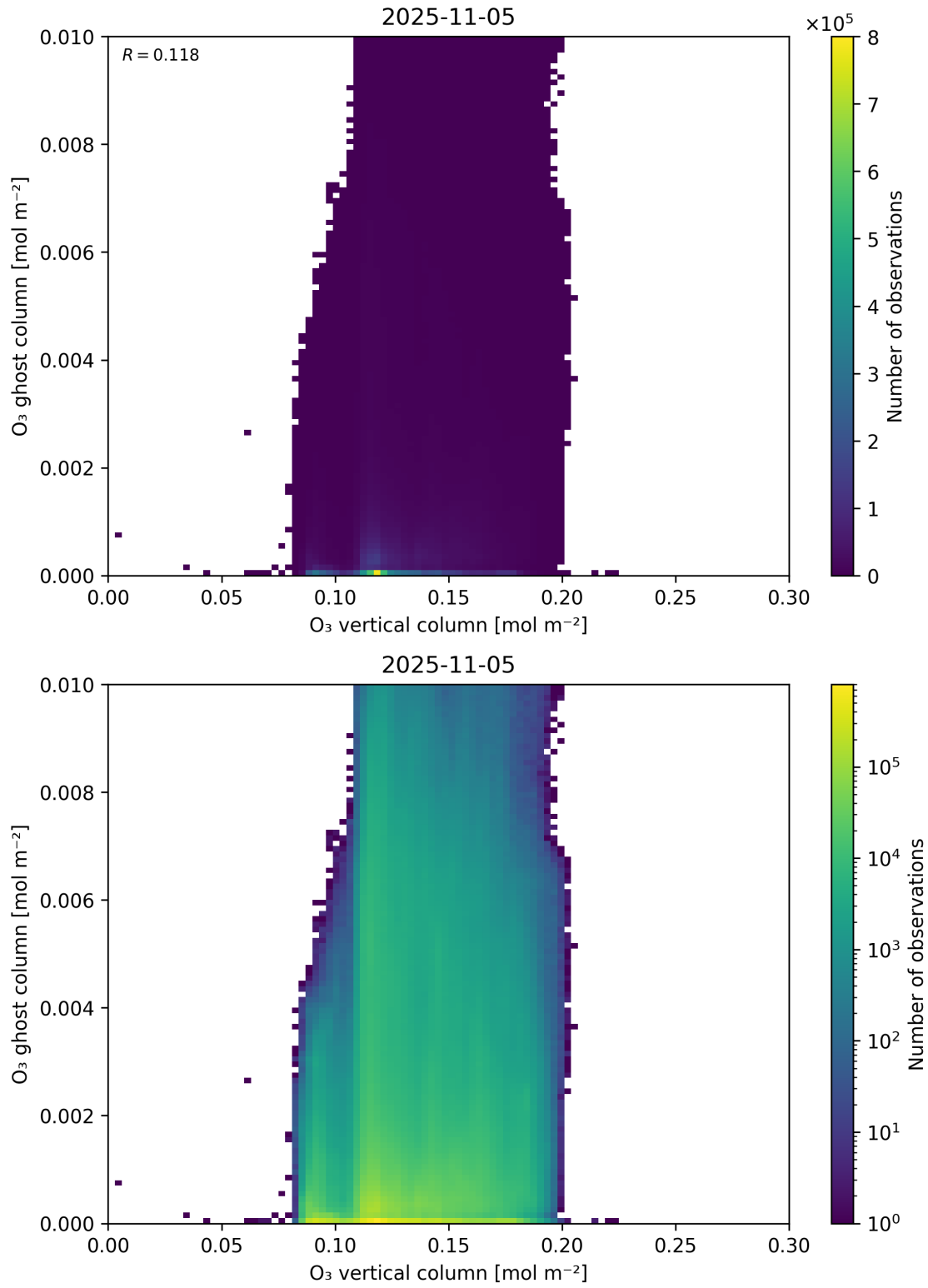
Figure 40: Scatter density plot of “O 3 vertical column” against “O 3 ghost column” for 2025-11-04 to 2025-11-06.
