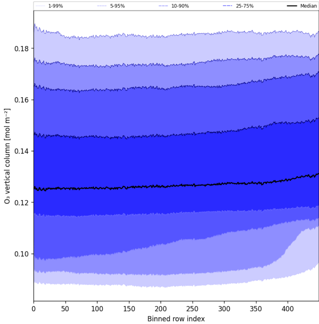
Figure 28: Along track statistics of “O 3 vertical column” for 2025-11-04 to 2025-11-06
