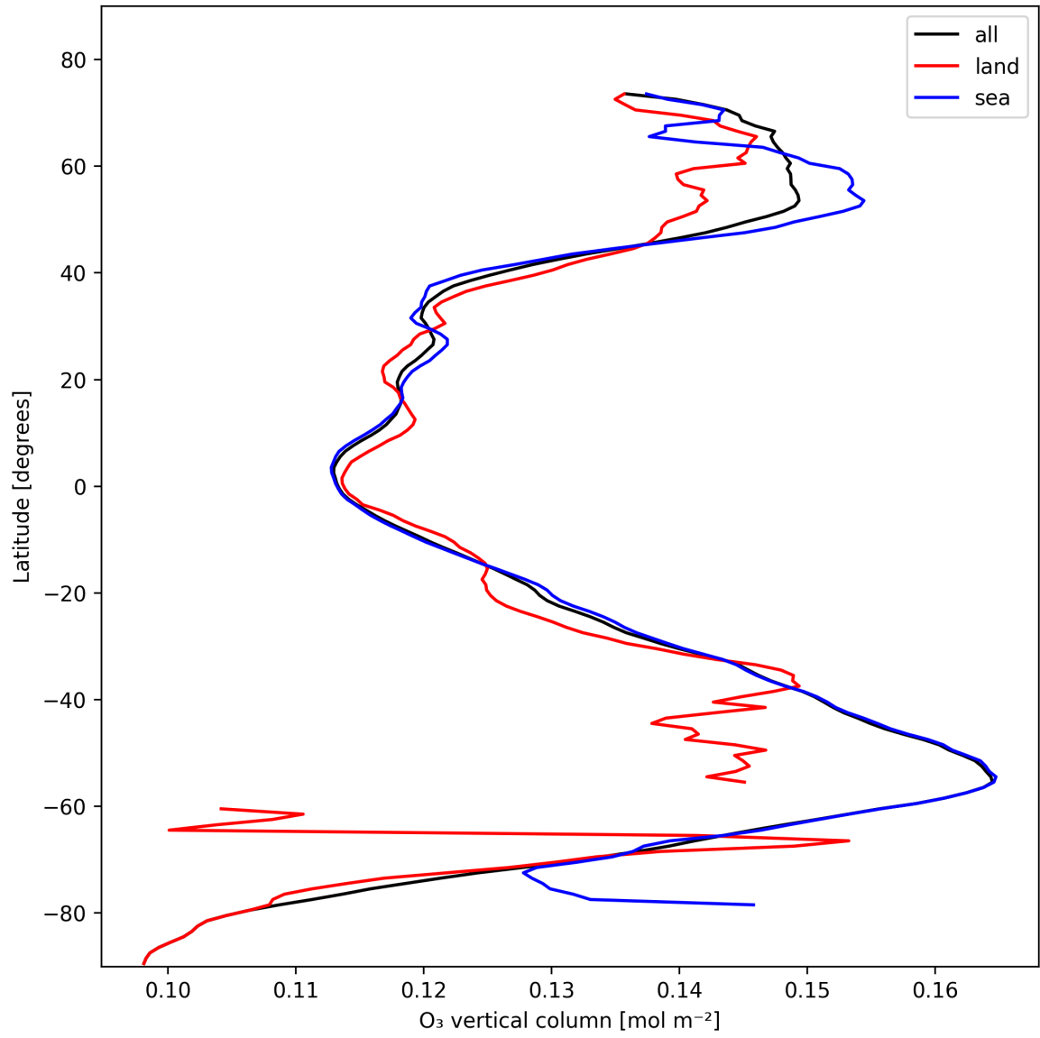
Figure 14: Zonal average of “O 3 vertical column” for 2025-11-04 to 2025-11-06.
