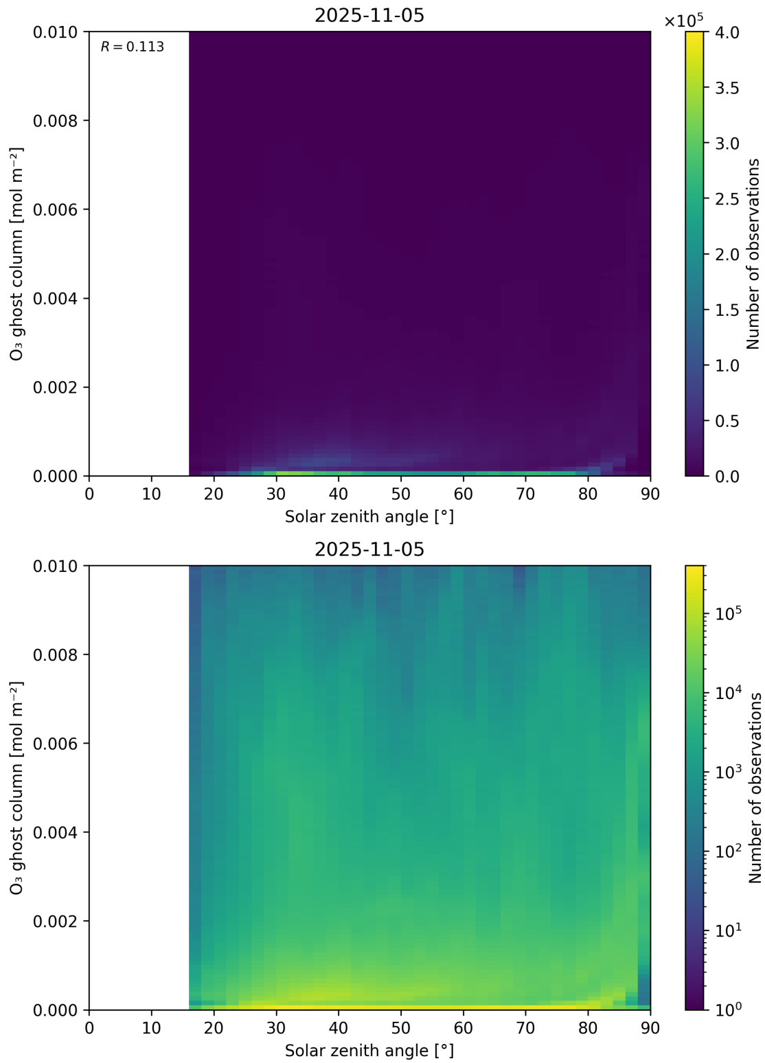
Figure 46: Scatter density plot of “Solar zenith angle” against “O 3 ghost column” for 2025-11-04 to 2025-11-06.
