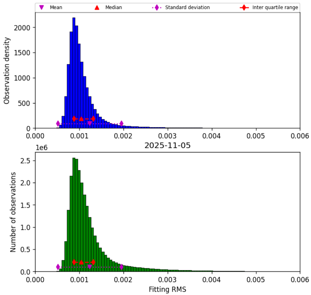
Figure 23: Histogram of “Fitting RMS” for 2025-11-04 to 2025-11-06
