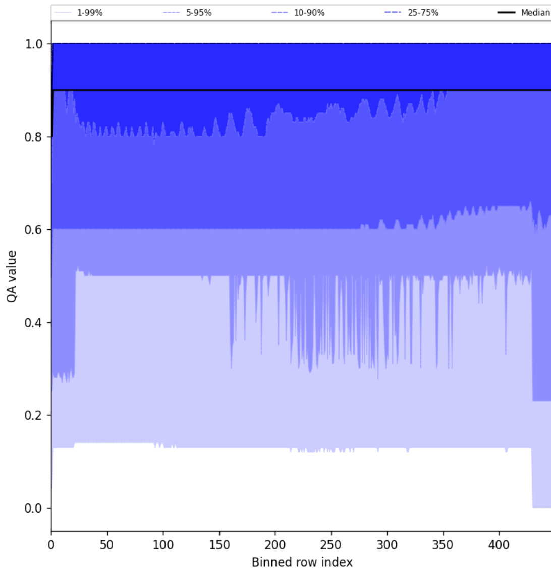
Figure 27: Along track statistics of “QA value” for 2025-11-04 to 2025-11-06
