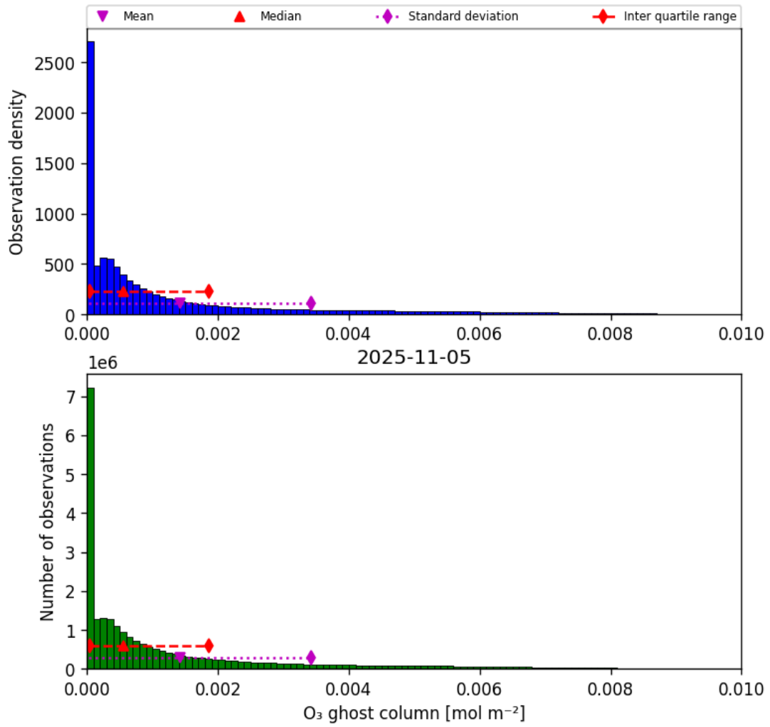
Figure 25: Histogram of “O 3 ghost column” for 2025-11-04 to 2025-11-06
