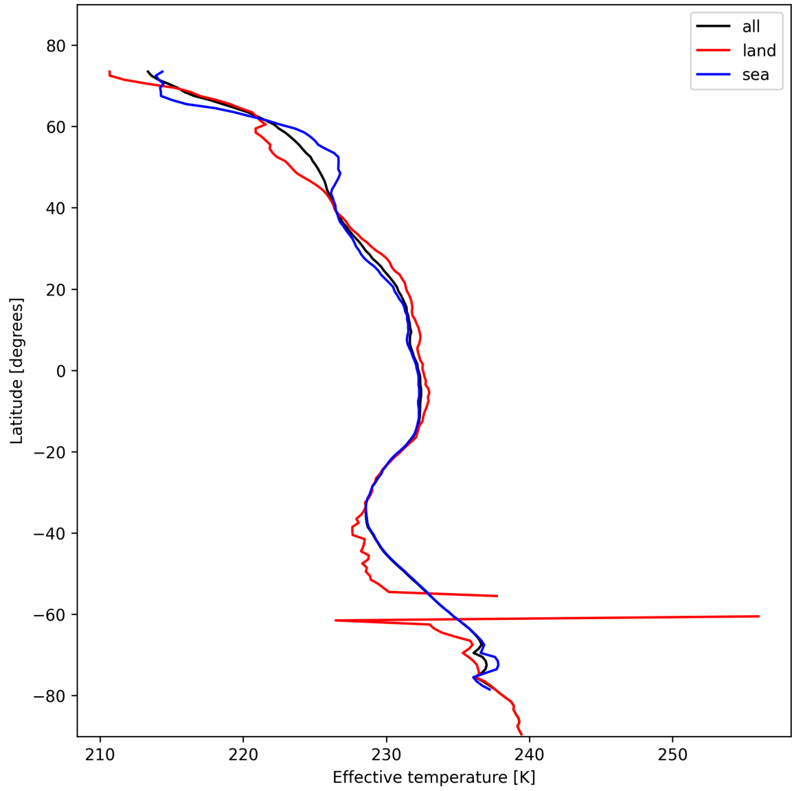
Figure 17: Zonal average of "Effective temperature" for 2025-11-04 to 2025-11-06.
