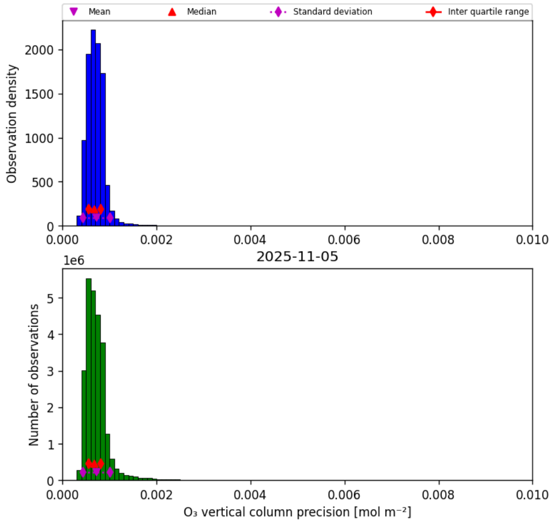
Figure 22: Histogram of "O 3 vertical column precision" for 2025-11-04 to 2025-11-06
