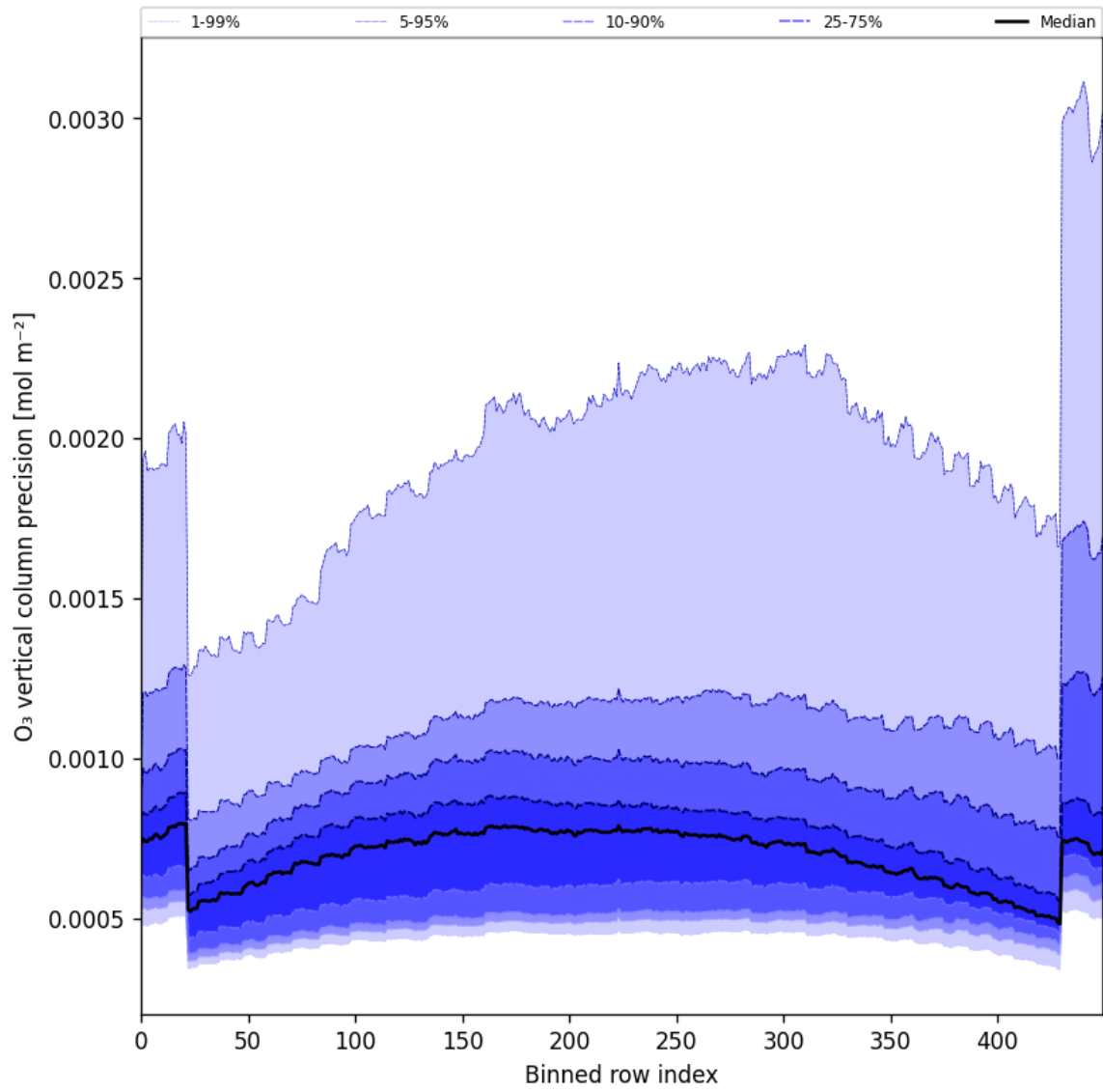
Figure 29: Along track statistics of “O 3 vertical column precision” for 2025-11-04 to 2025-11-06
