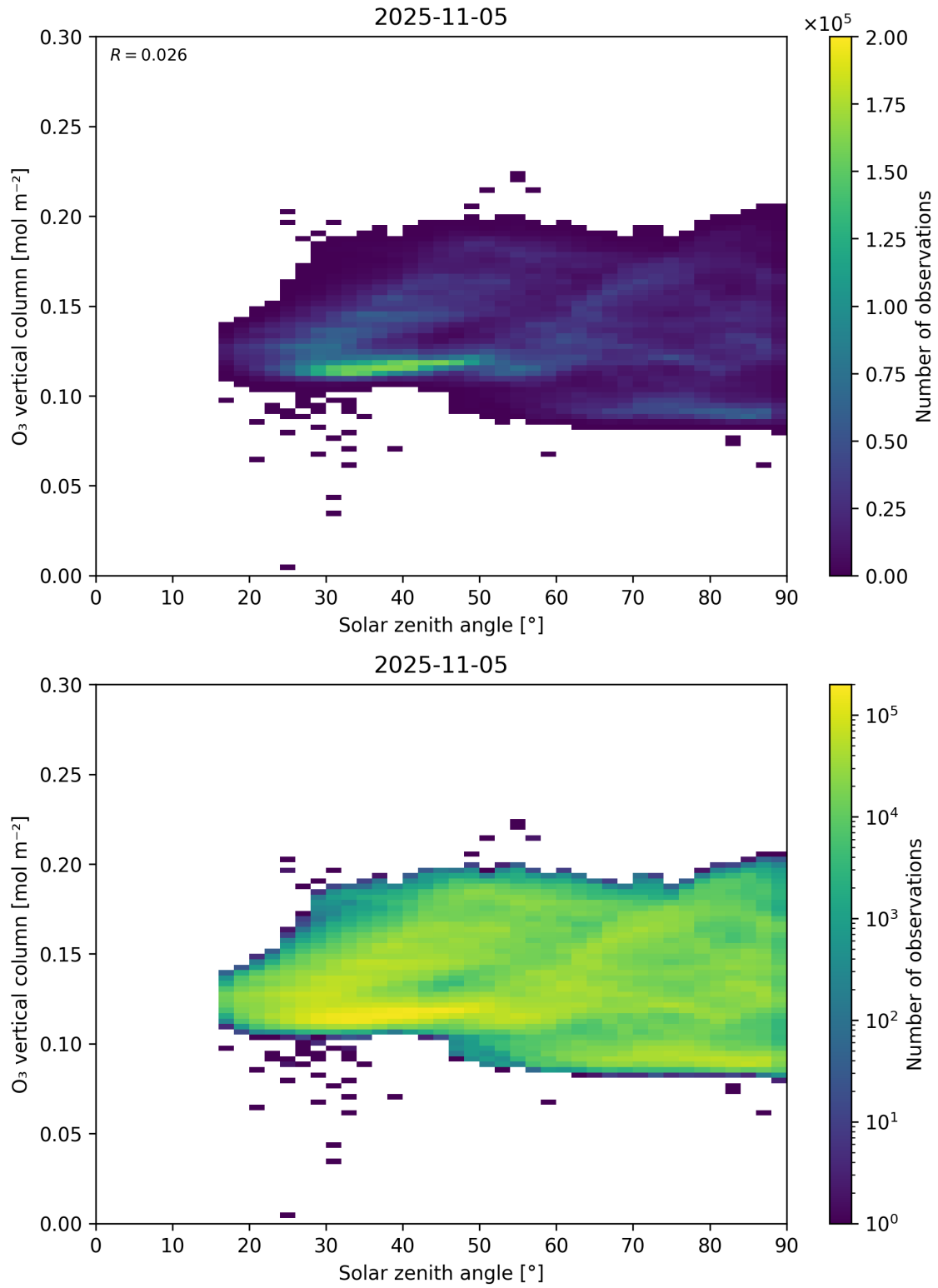
Figure 47: Scatter density plot of “Solar zenith angle” against “O 3 vertical column” for 2025-11-04 to 2025-11-06.
