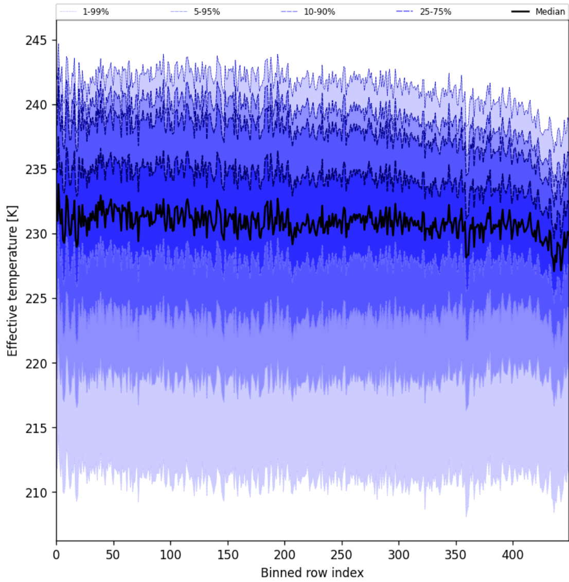
Figure 31: Along track statistics of “Effective temperature” for 2025-11-04 to 2025-11-06
