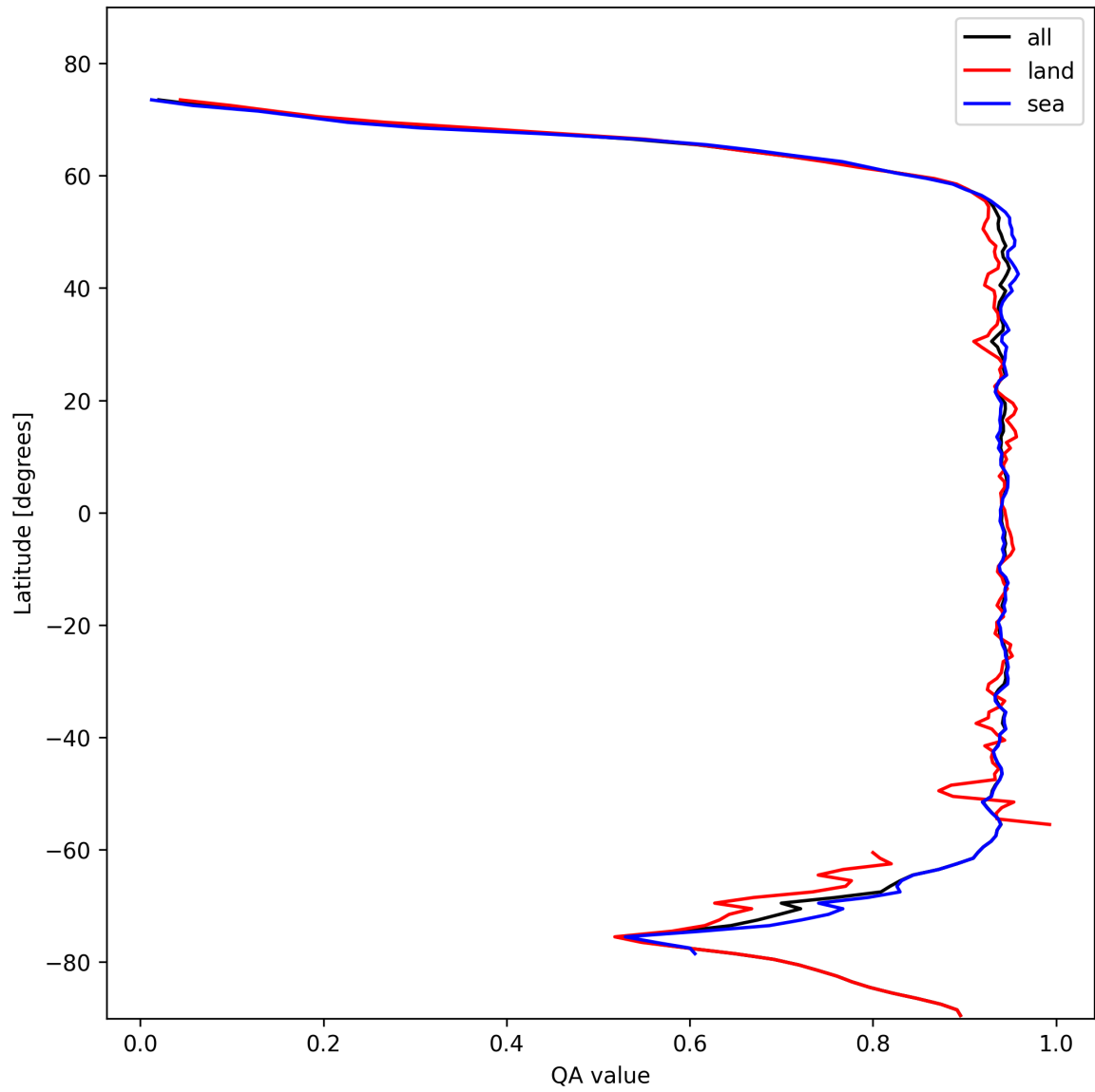
Figure 13: Zonal average of “QA value” for 2025-11-04 to 2025-11-06.
