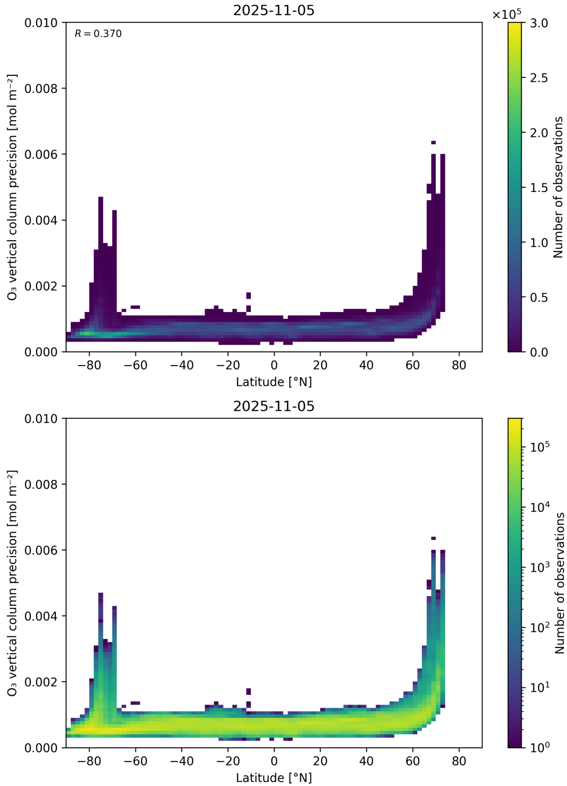
Figure 37: Scatter density plot of “Latitude” against “O 3 vertical column precision” for 2025-11-04 to 2025-11-06.
