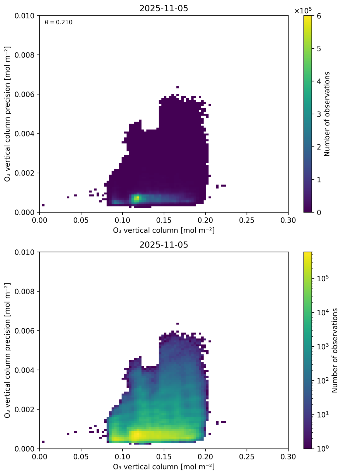
Figure 41: Scatter density plot of “O 3 vertical column” against “O 3 vertical column precision” for 2025-11-04 to 2025-11-06.
