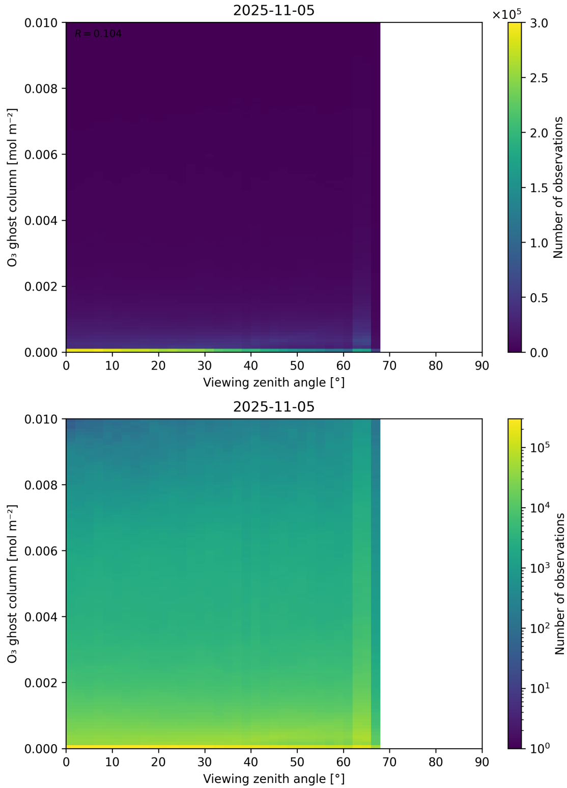
Figure 51: Scatter density plot of “Viewing zenith angle” against “O 3 ghost column” for 2025-11-04 to 2025-11-06.
