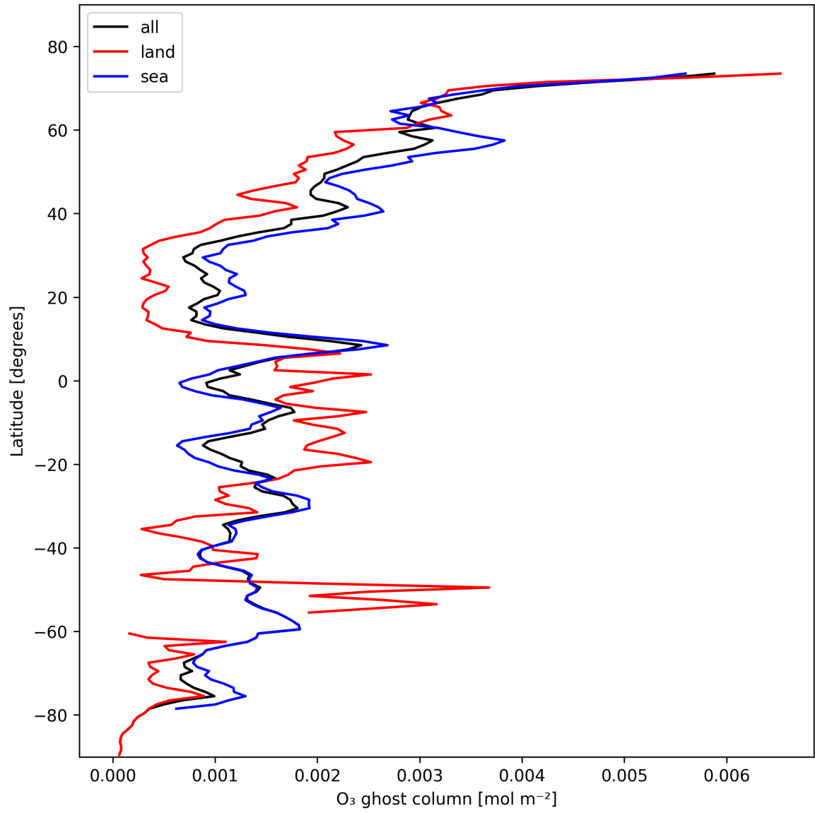
Figure 18: Zonal average of “O 3 ghost column” for 2025-11-04 to 2025-11-06.
