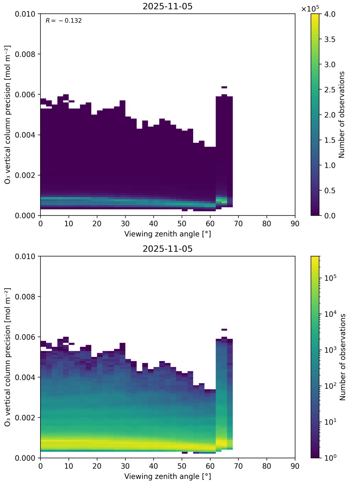
Figure 53: Scatter density plot of “Viewing zenith angle” against “O 3 vertical column precision” for 2025-11-04 to 2025-11-06.
