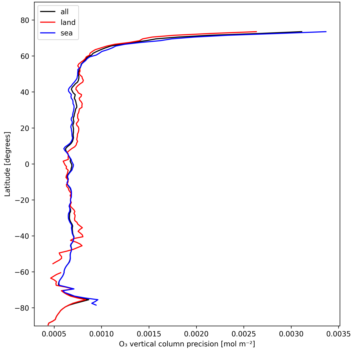
Figure 15: Zonal average of “O 3 vertical column precision” for 2025-11-04 to 2025-11-06.
