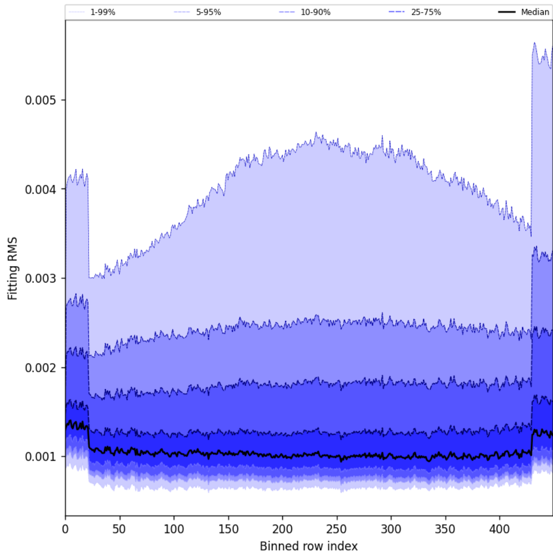
Figure 30: Along track statistics of “Fitting RMS” for 2025-11-04 to 2025-11-06
