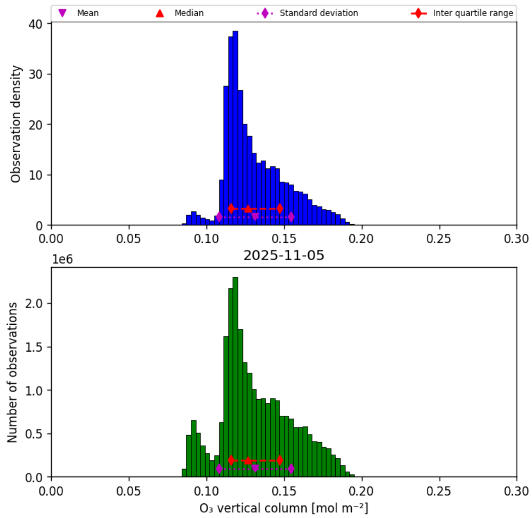
Figure 21: Histogram of “O 3 vertical column” for 2025-11-04 to 2025-11-06
