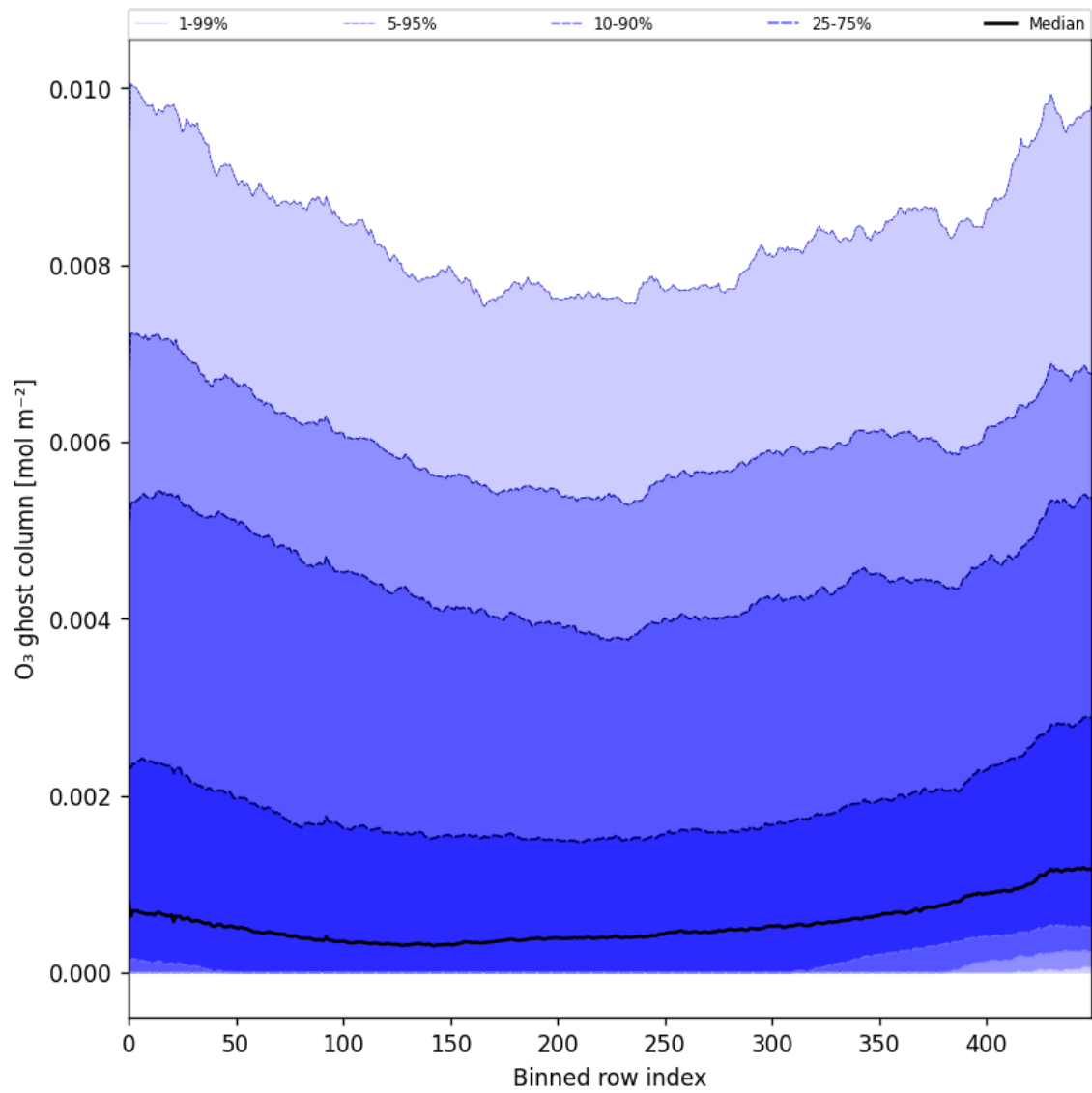
Figure 32: Along track statistics of “O 3 ghost column” for 2025-11-04 to 2025-11-06
