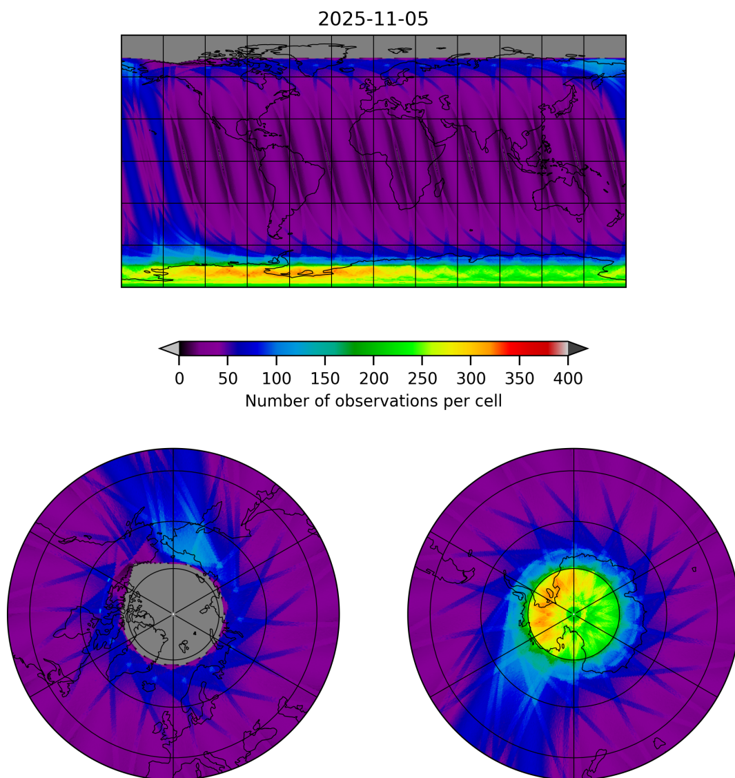
Figure 12: Map of the number of observations for 2025-11-04 to 2025-11-06
