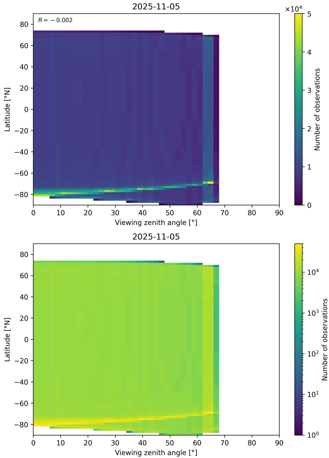
Figure 49: Scatter density plot of “Viewing zenith angle” against “Latitude” for 2025-11-04 to 2025-11-06.
