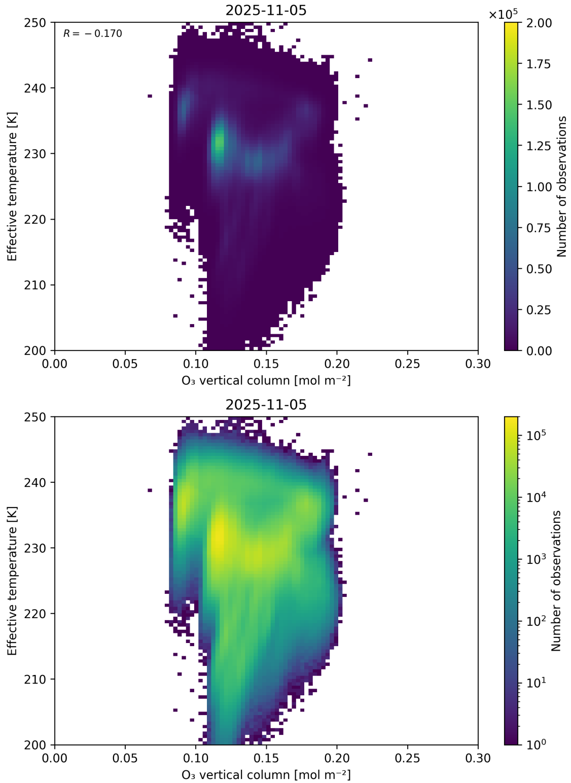
Figure 39: Scatter density plot of “O 3 vertical column” against “Effective temperature” for 2025-11-04 to 2025-11-06.
