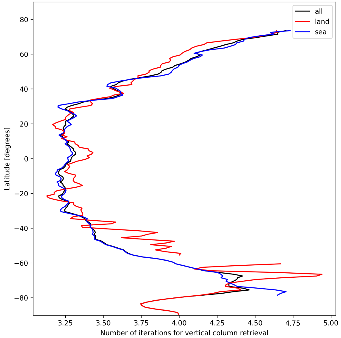
Figure 19: Zonal average of “Number of iterations for vertical column retrieval” for 2025-11-04 to 2025-11-06.
