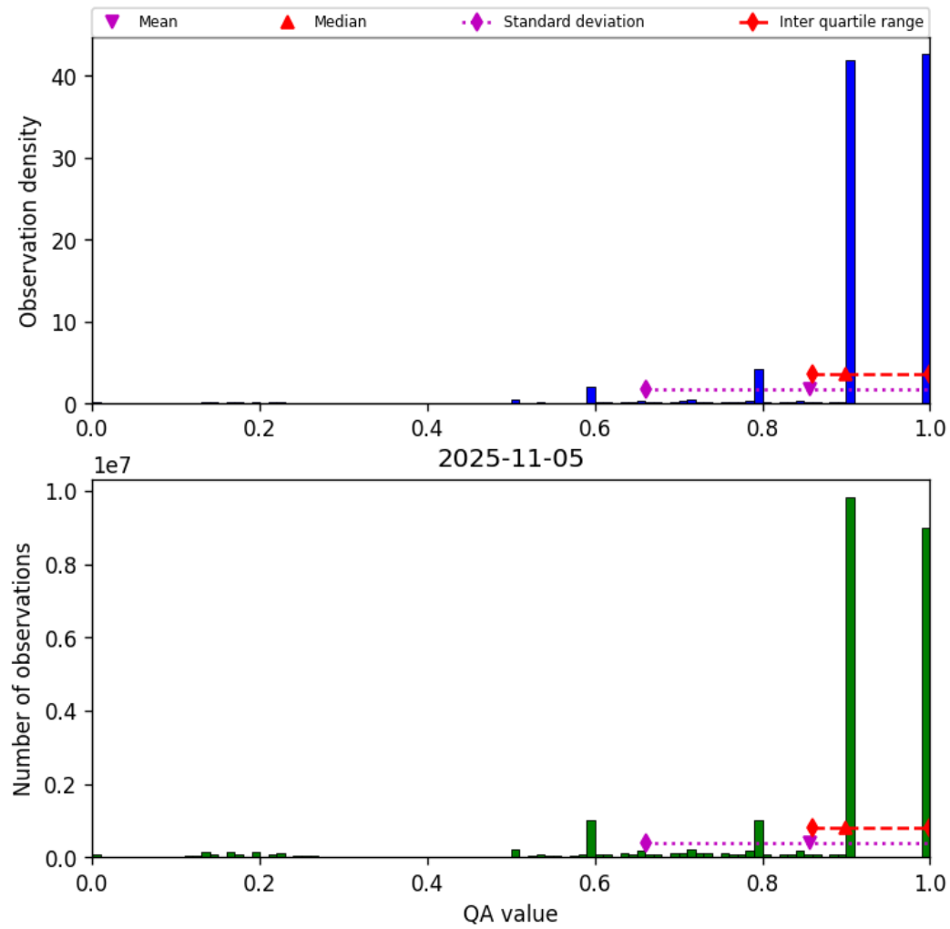
Figure 20: Histogram of “QA value” for 2025-11-04 to 2025-11-06
