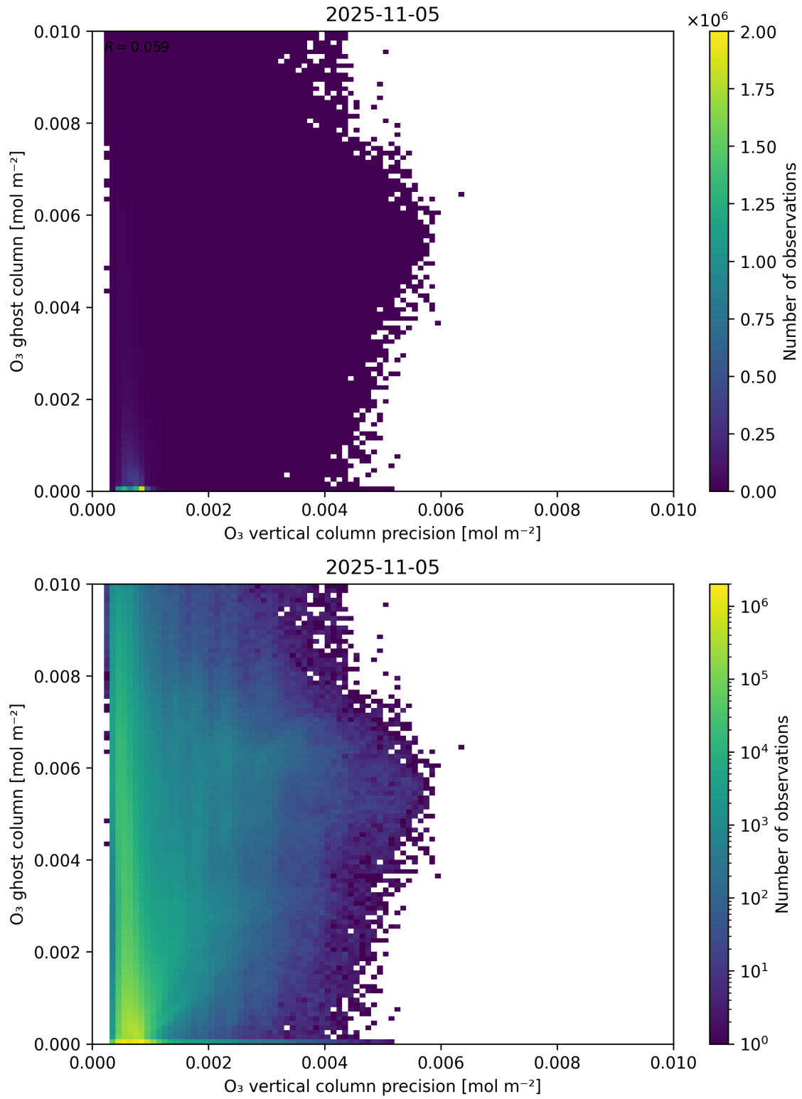
Figure 43: Scatter density plot of “O 3 vertical column precision” against “O 3 ghost column” for 2025-11-04 to 2025-11-06.
