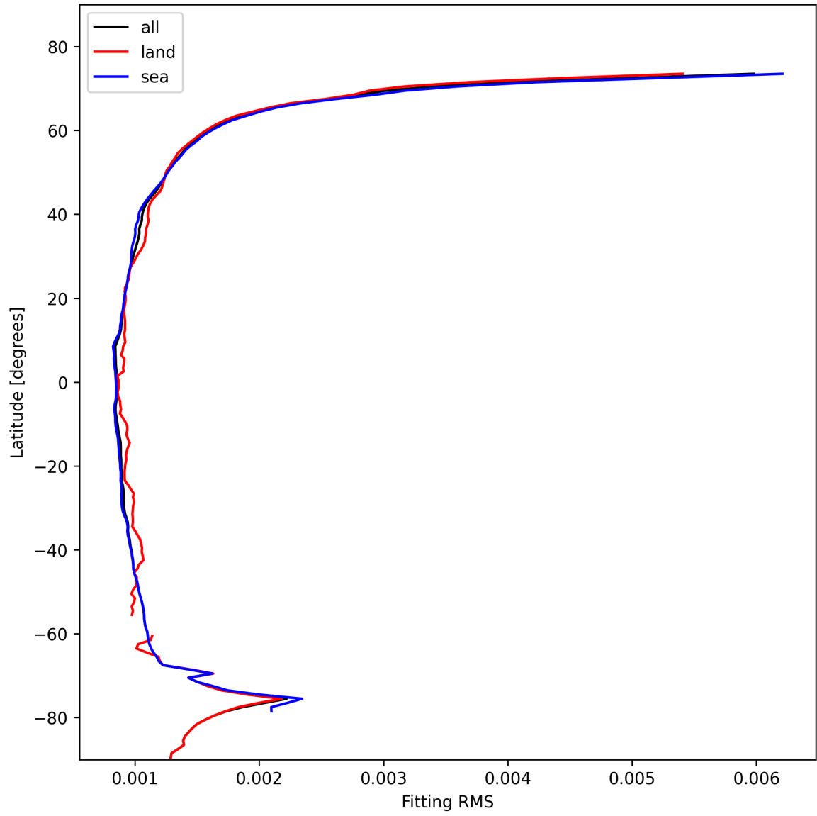
Figure 16: Zonal average of “Fitting RMS” for 2025-11-04 to 2025-11-06.
