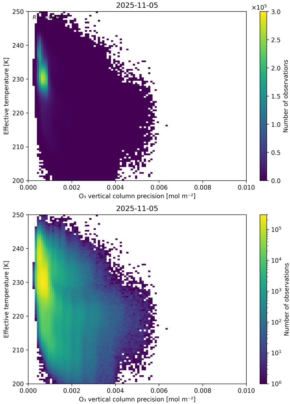
Figure 42: Scatter density plot of “O 3 vertical column precision” against “Effective temperature” for 2025-11-04 to 2025-11-06.
