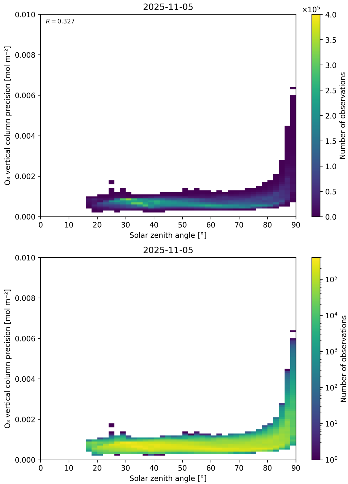
Figure 48: Scatter density plot of “Solar zenith angle” against “O 3 vertical column precision” for 2025-11-04 to 2025-11-06.
