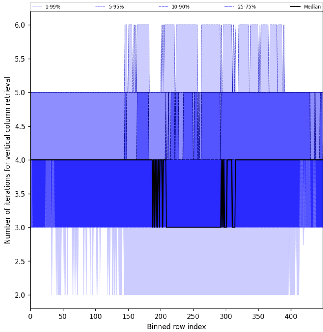
Figure 33: Along track statistics of “Number of iterations for vertical column retrieval” for 2025-11-07 to 2025-11-08
