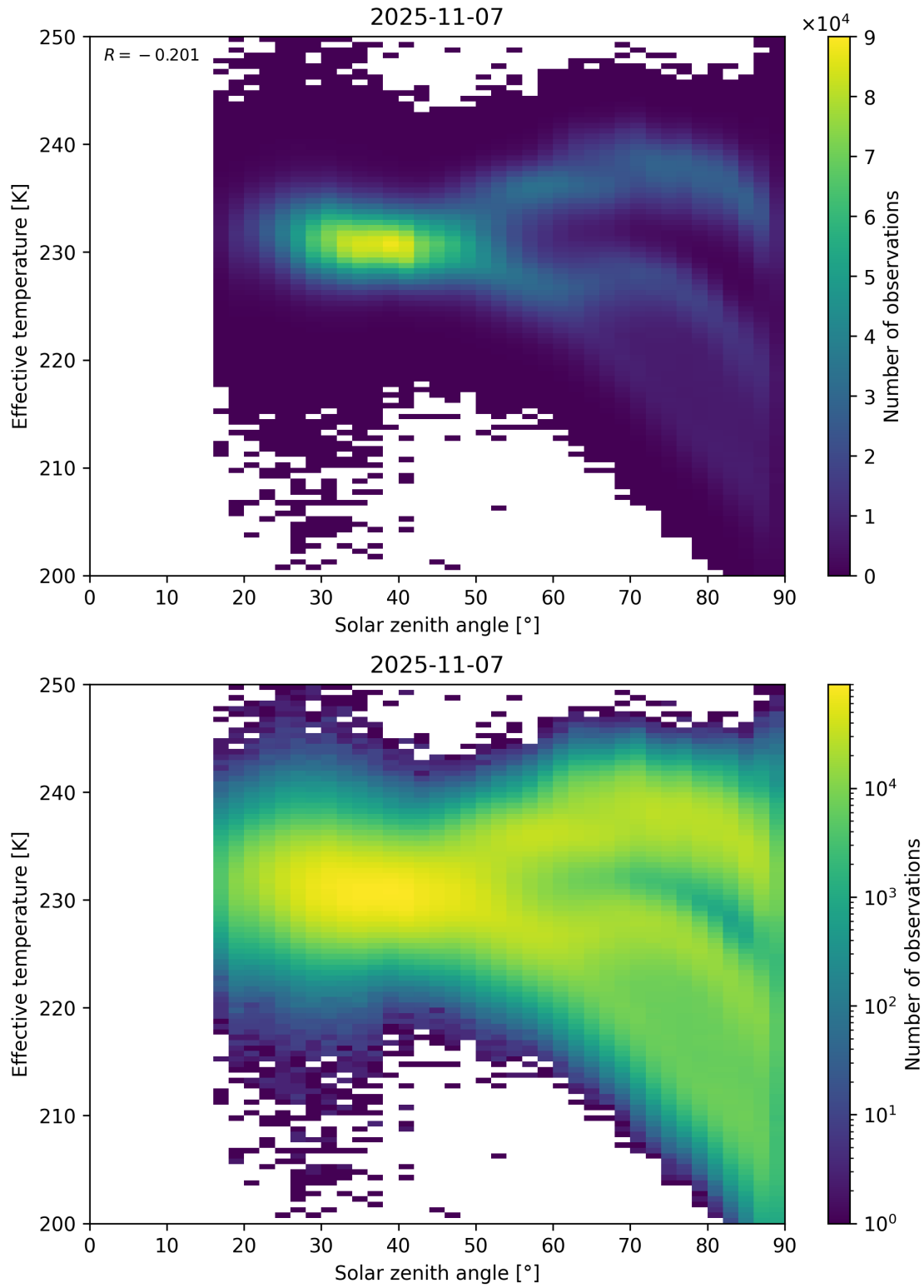
Figure 45: Scatter density plot of “Solar zenith angle” against “Effective temperature” for 2025-11-07 to 2025-11-08.
