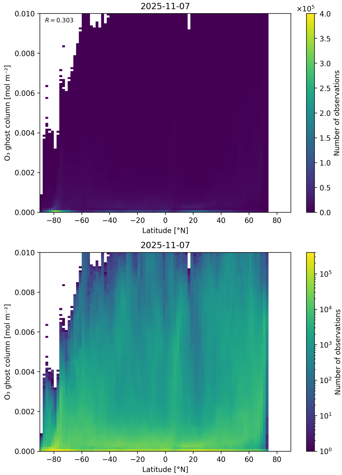
Figure 35: Scatter density plot of “Latitude” against “O 3 ghost column” for 2025-11-07 to 2025-11-08.
