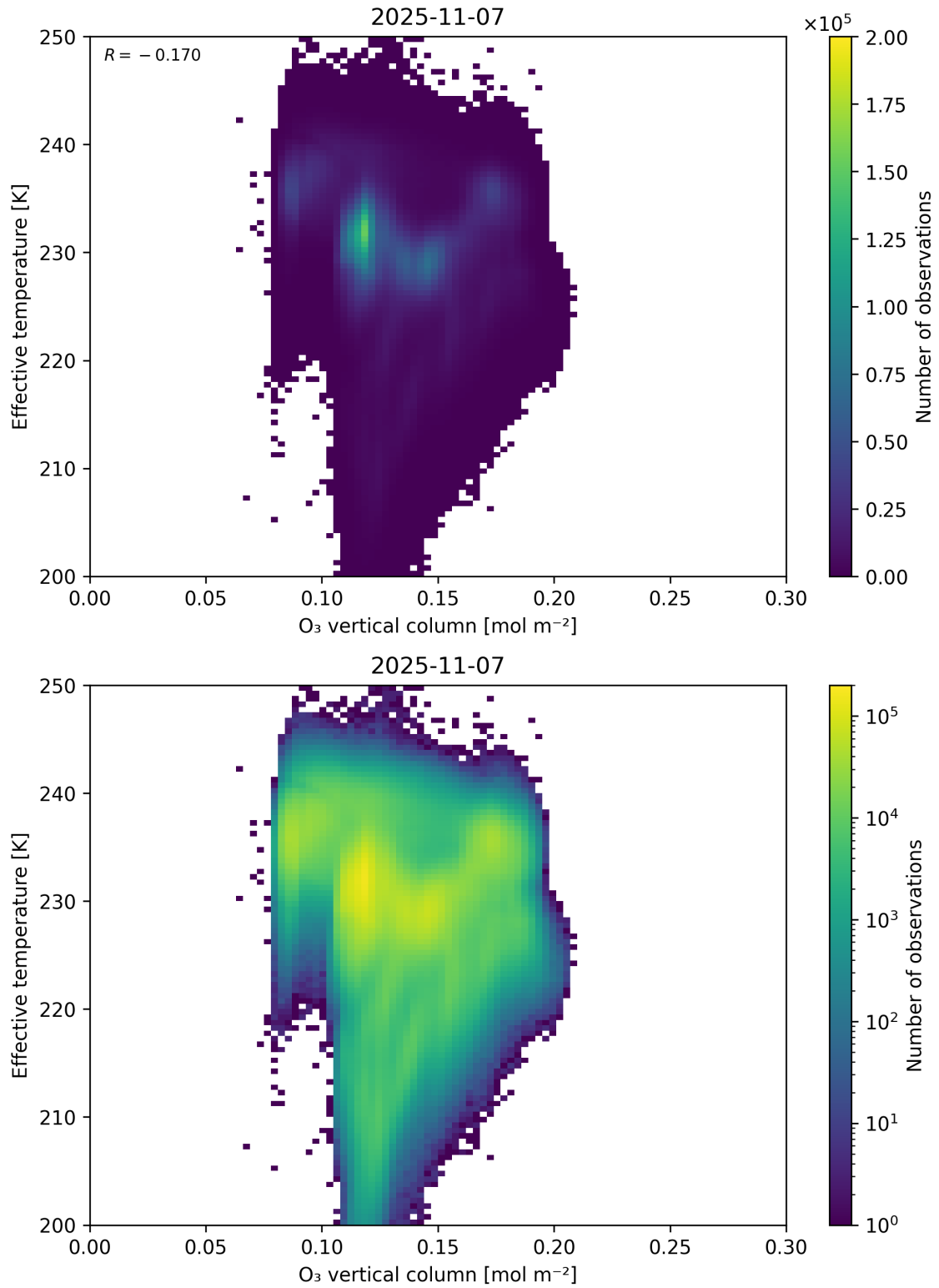
Figure 39: Scatter density plot of “O 3 vertical column” against “Effective temperature” for 2025-11-07 to 2025-11-08.
