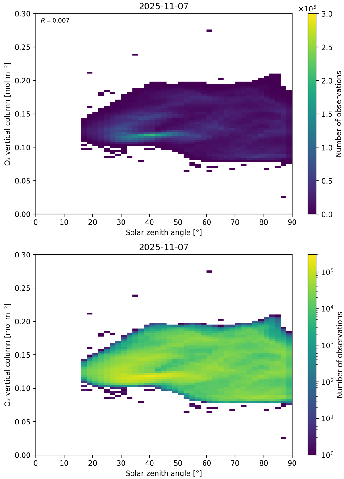
Figure 47: Scatter density plot of “Solar zenith angle” against “O 3 vertical column” for 2025-11-07 to 2025-11-08.
