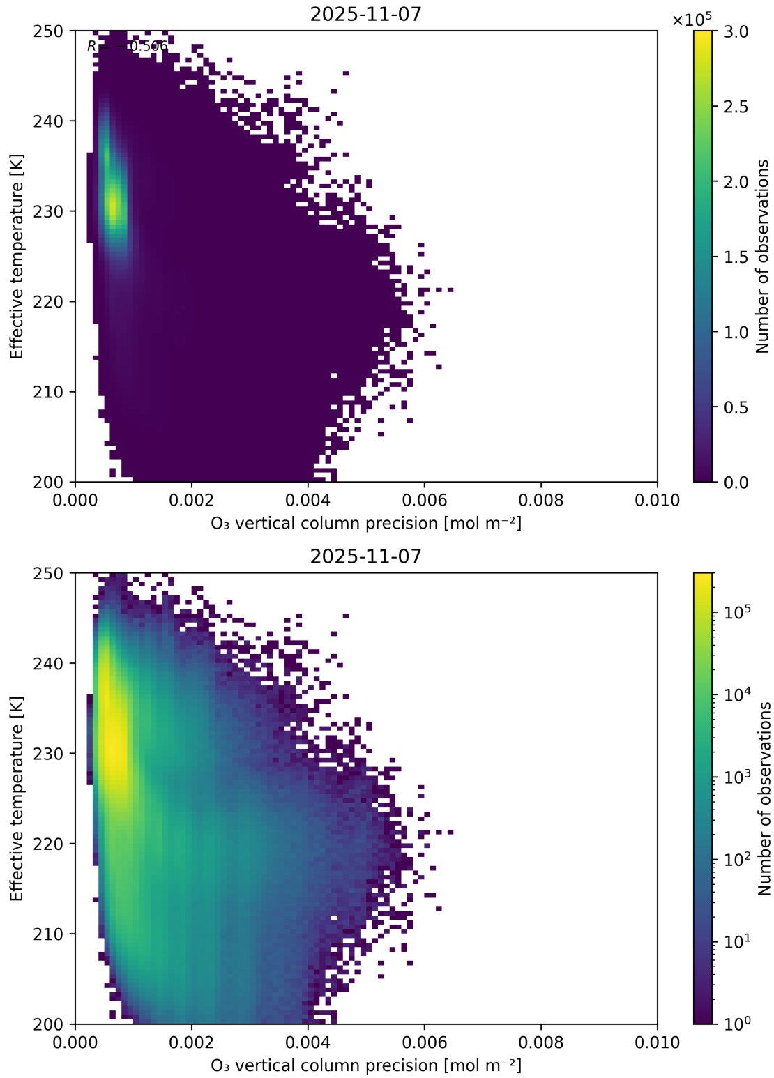
Figure 42: Scatter density plot of “O 3 vertical column precision” against “Effective temperature” for 2025-11-07 to 2025-11-08.
