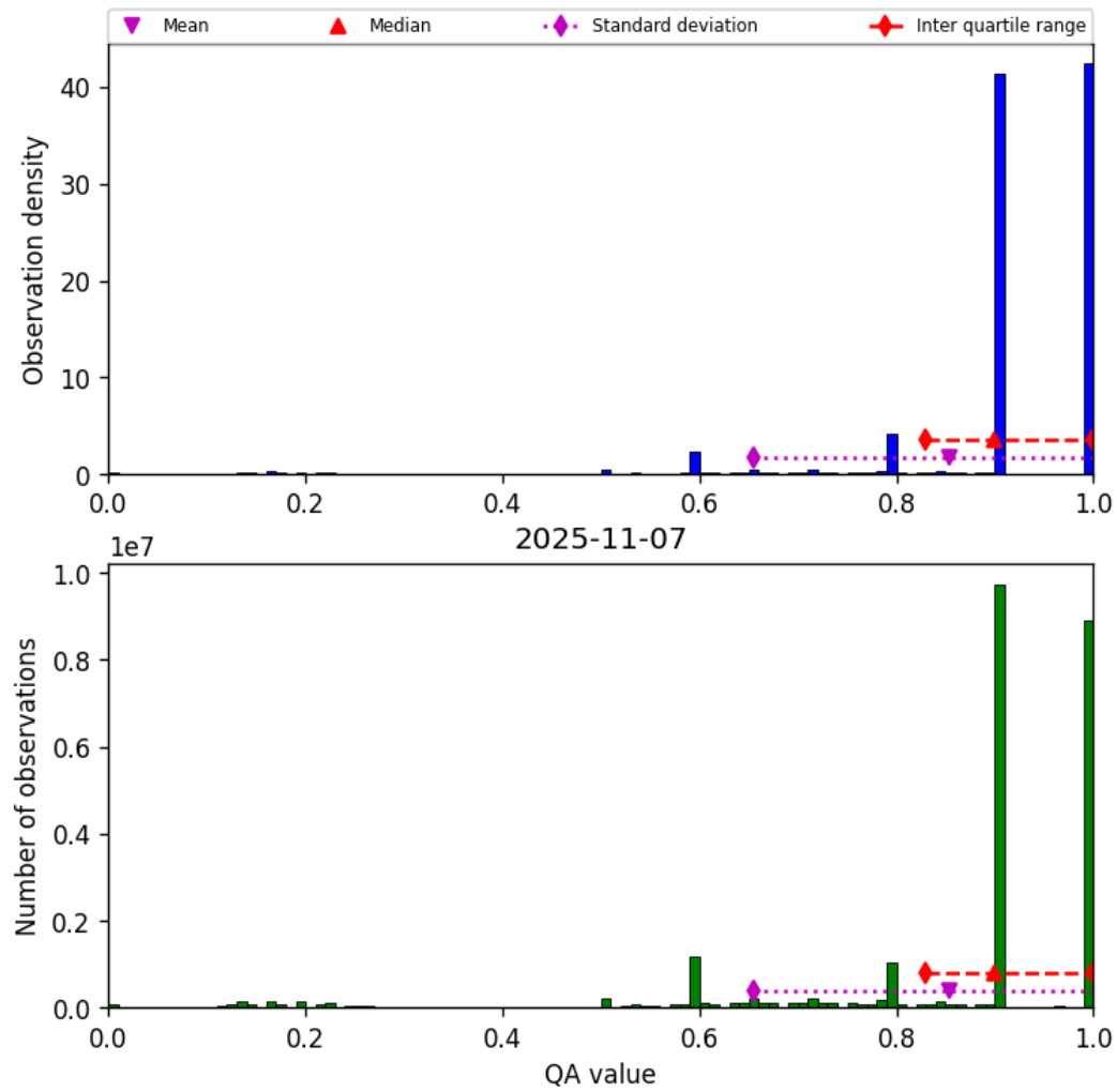
Figure 20: Histogram of “QA value” for 2025-11-07 to 2025-11-08
