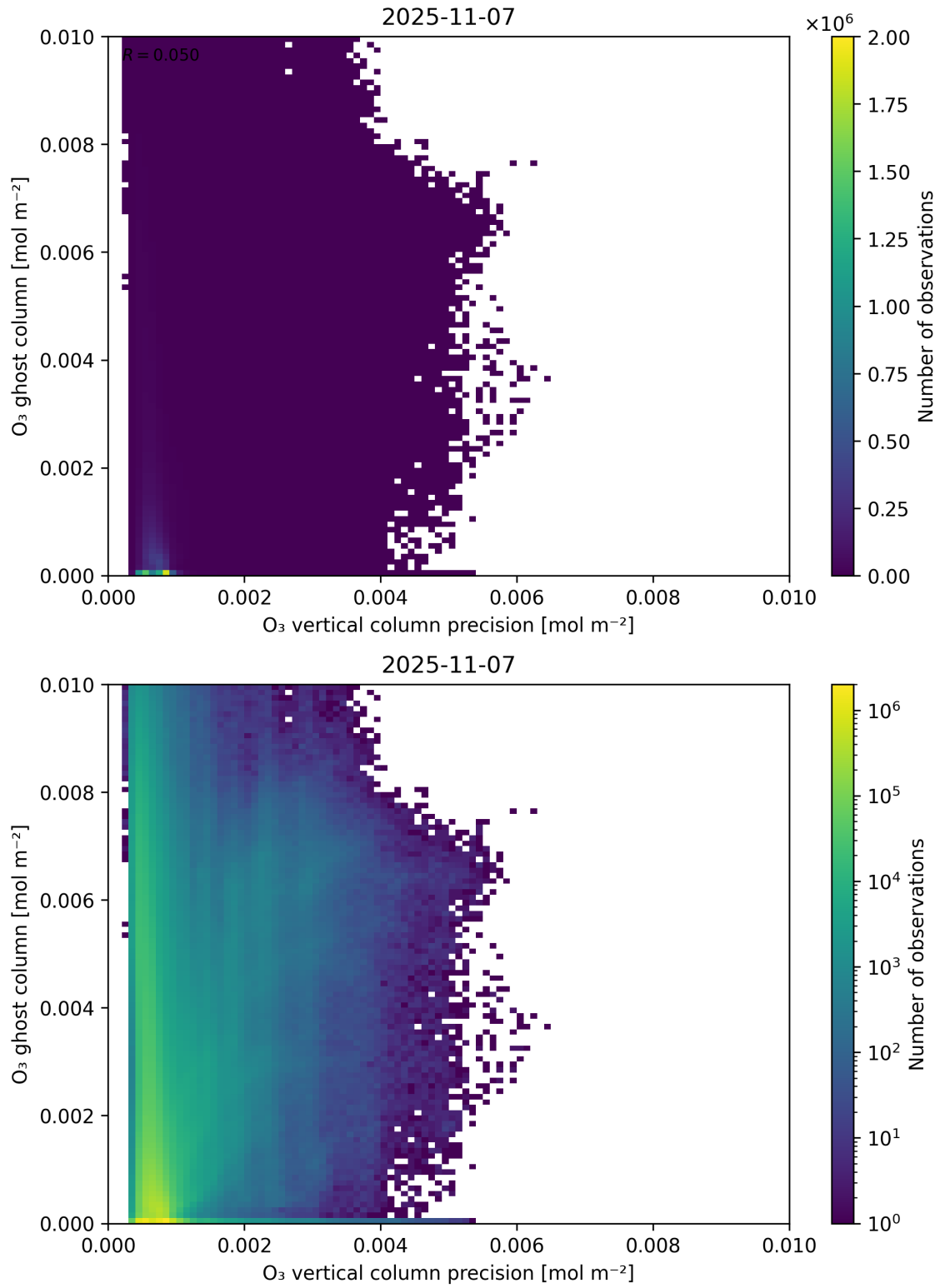
Figure 43: Scatter density plot of “ \text{O}_3 vertical column precision” against “ \text{O}_3 ghost column” for 2025-11-07 to 2025-11-08.
