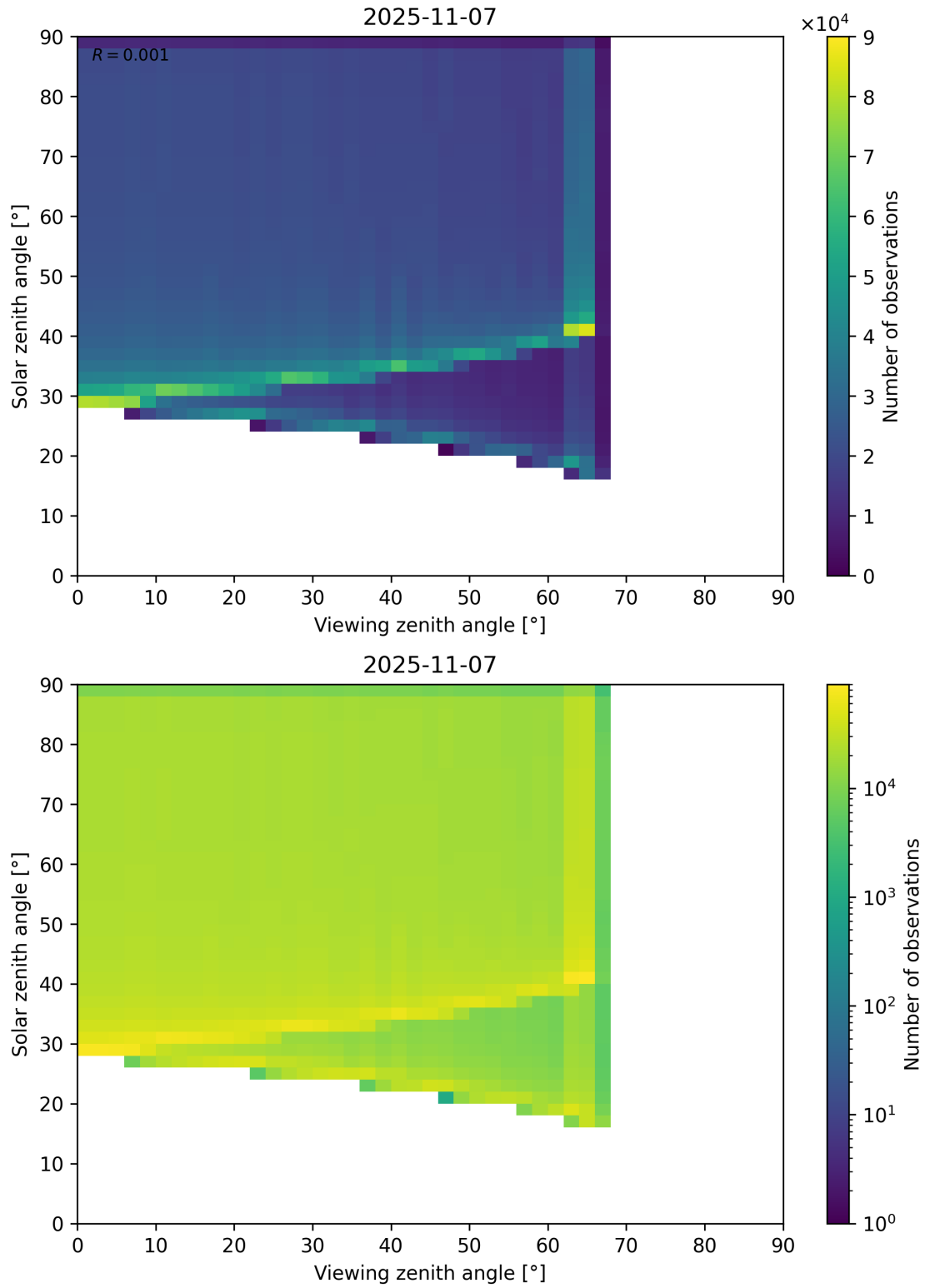
Figure 54: Scatter density plot of “Viewing zenith angle” against “Solar zenith angle” for 2025-11-07 to 2025-11-08.
