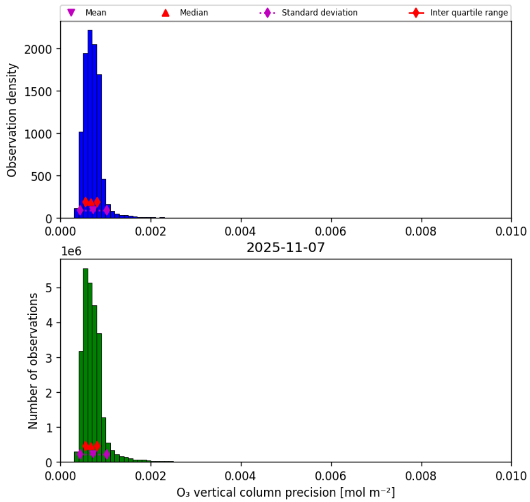
Figure 22: Histogram of “O 3 vertical column precision” for 2025-11-07 to 2025-11-08
