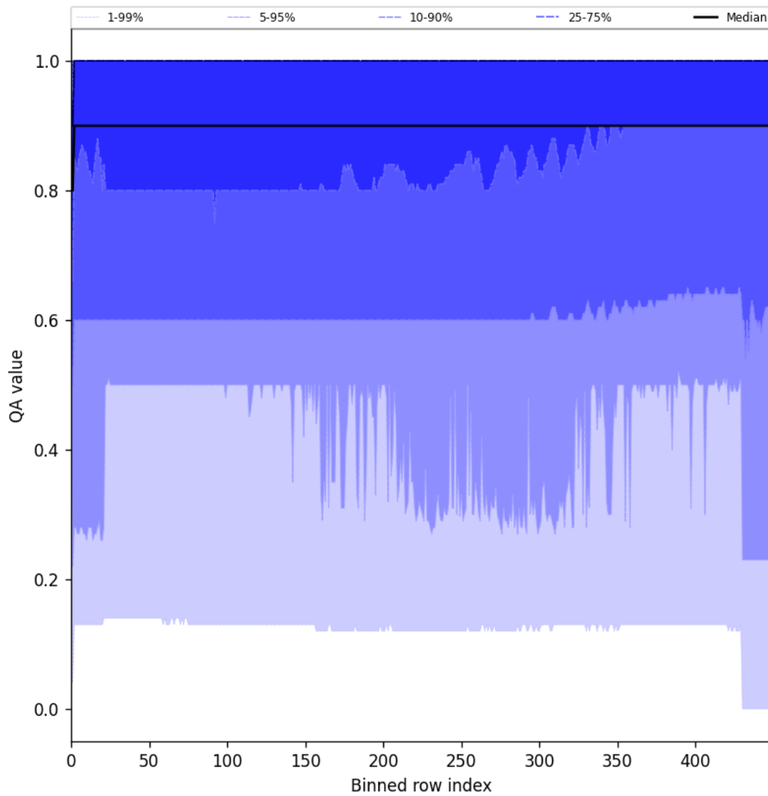
Figure 27: Along track statistics of “QA value” for 2025-11-07 to 2025-11-08
