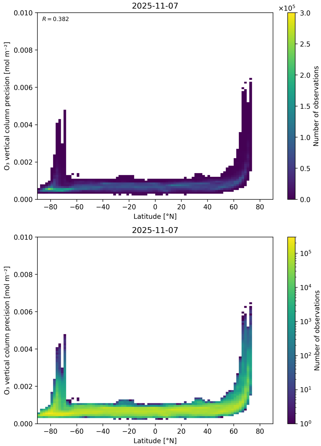
Figure 37: Scatter density plot of “Latitude” against “O 3 vertical column precision” for 2025-11-07 to 2025-11-08.
