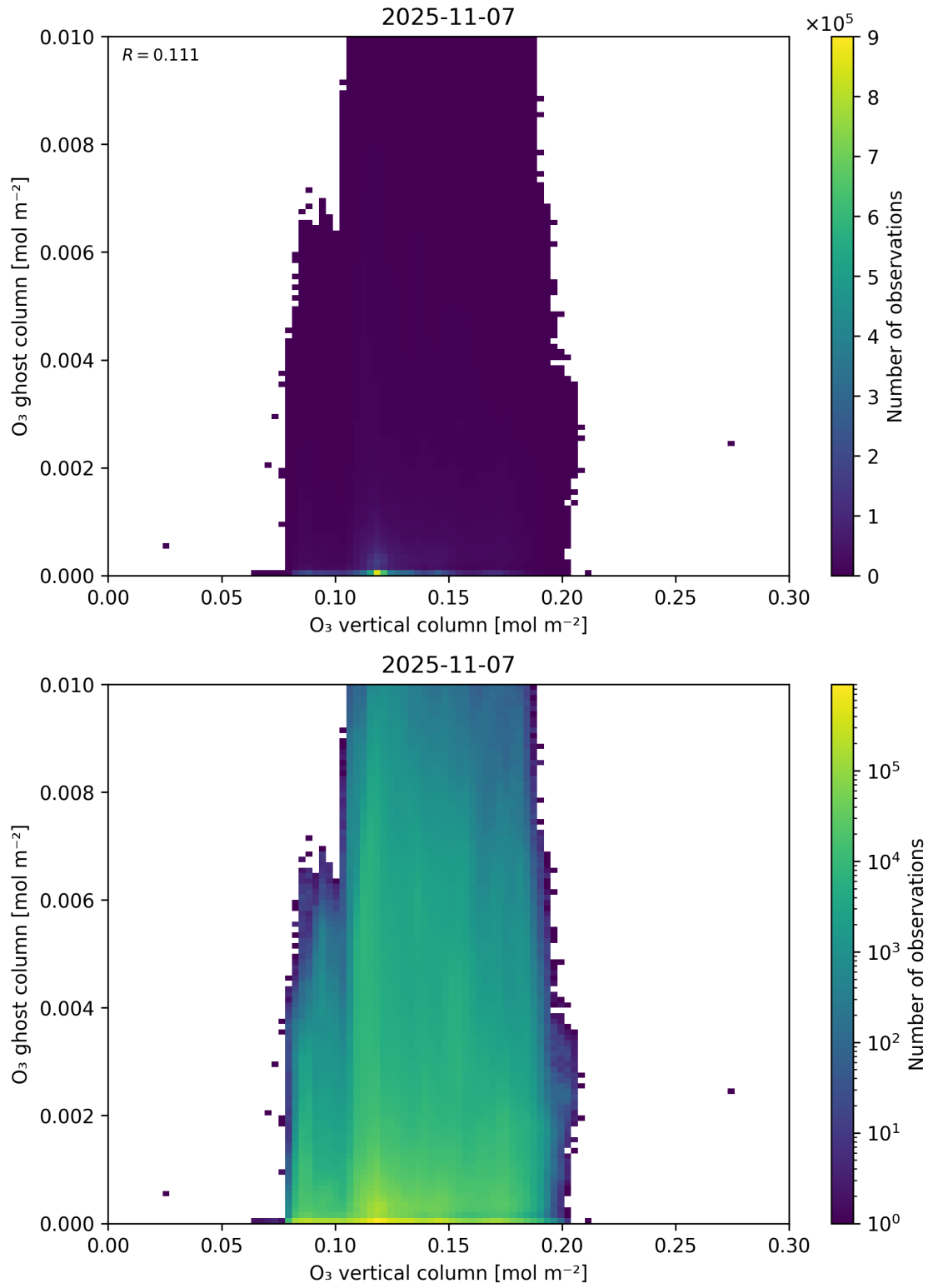
Figure 40: Scatter density plot of “O 3 vertical column” against “O 3 ghost column” for 2025-11-07 to 2025-11-08.
