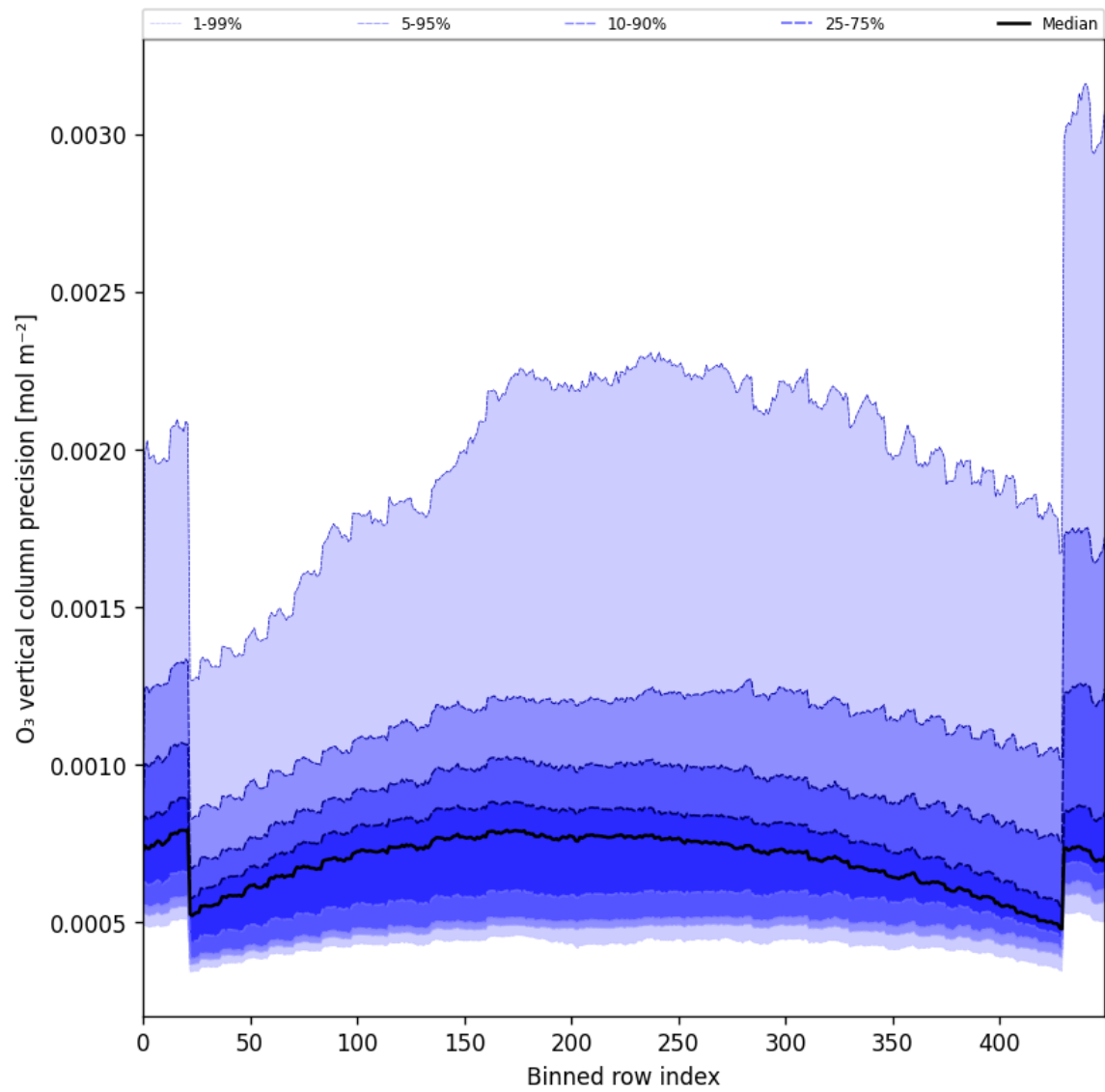
Figure 29: Along track statistics of “O 3 vertical column precision” for 2025-11-07 to 2025-11-08
