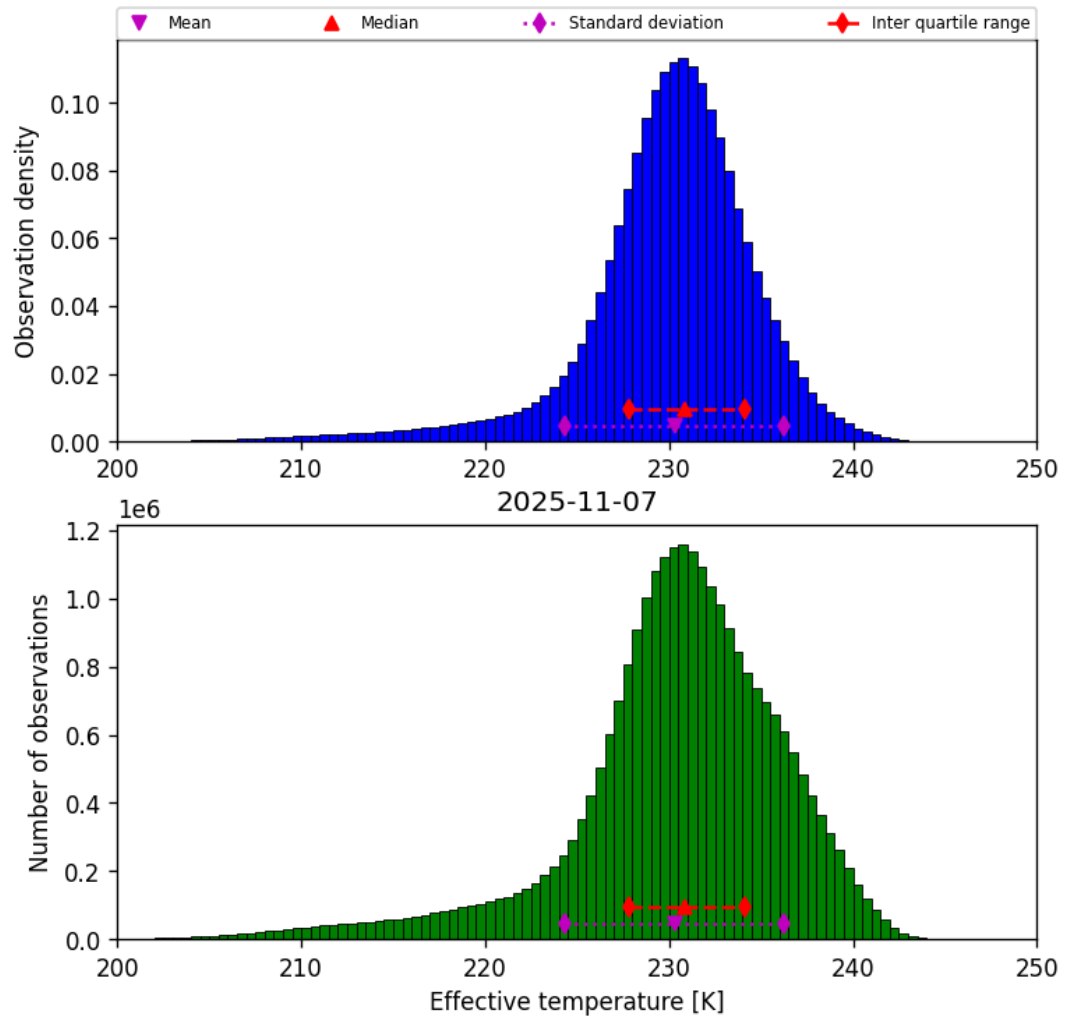
Figure 24: Histogram of “Effective temperature” for 2025-11-07 to 2025-11-08
