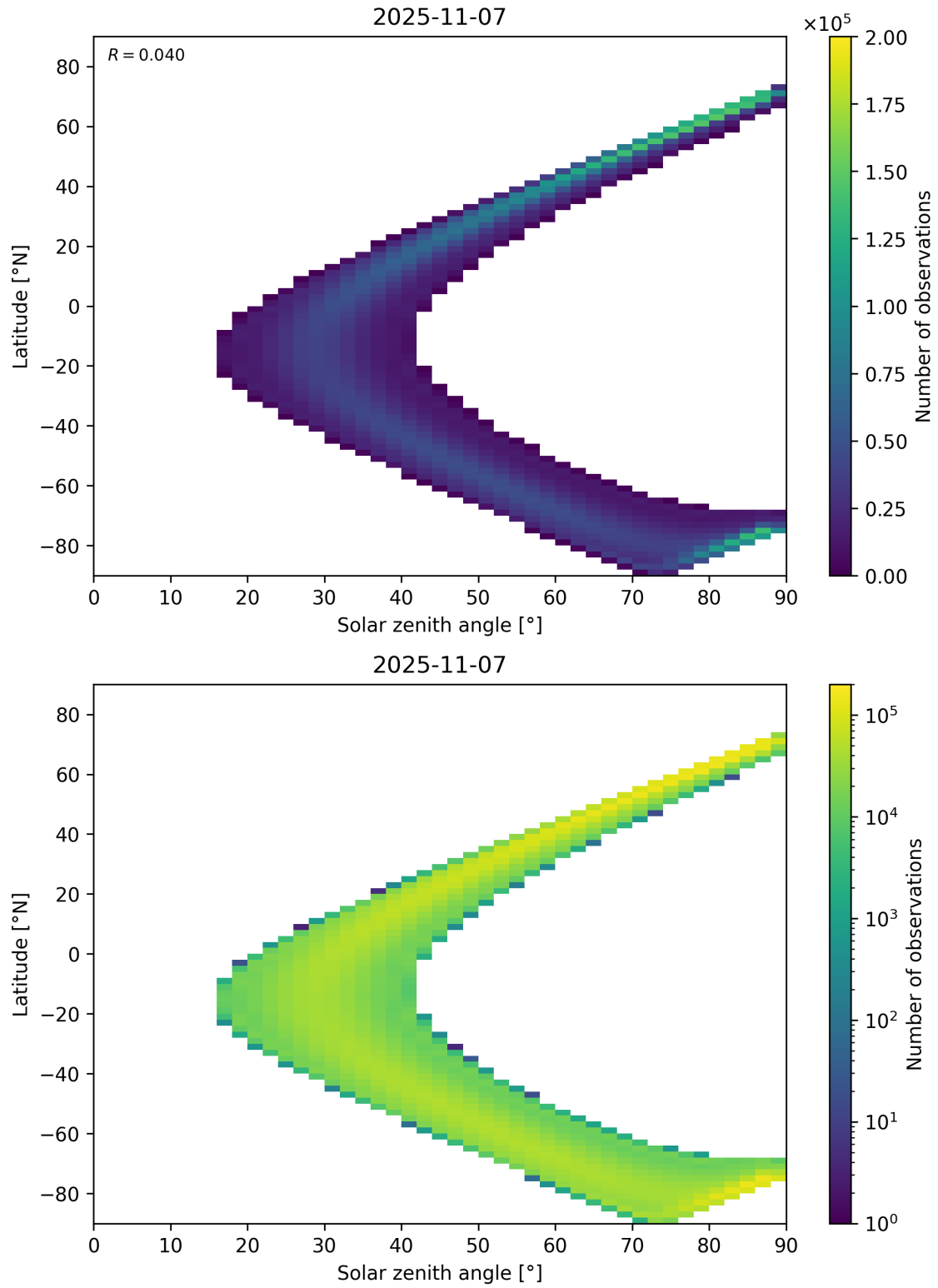
Figure 44: Scatter density plot of “Solar zenith angle” against “Latitude” for 2025-11-07 to 2025-11-08.
