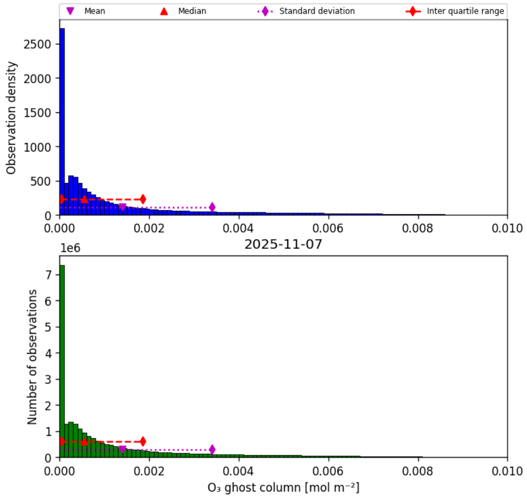
Figure 25: Histogram of “O 3 ghost column” for 2025-11-07 to 2025-11-08
