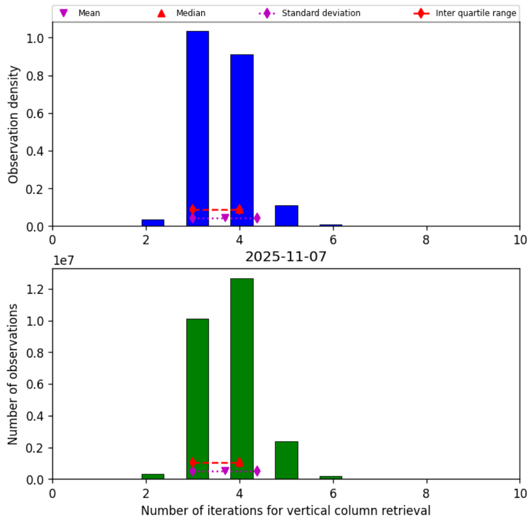
Figure 26: Histogram of “Number of iterations for vertical column retrieval” for 2025-11-07 to 2025-11-08
