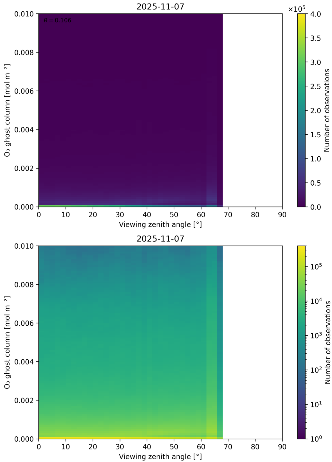
Figure 51: Scatter density plot of “Viewing zenith angle” against “O 3 ghost column” for 2025-11-07 to 2025-11-08.
