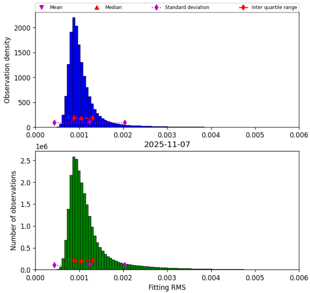
Figure 23: Histogram of “Fitting RMS” for 2025-11-07 to 2025-11-08
