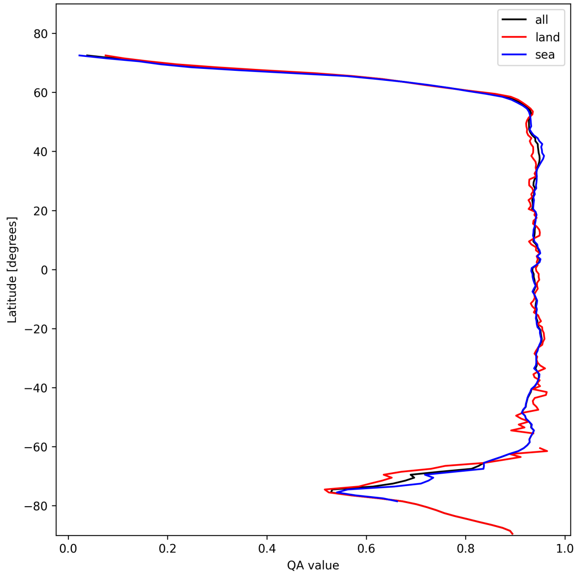
Figure 13: Zonal average of “QA value” for 2025-11-07 to 2025-11-08.
