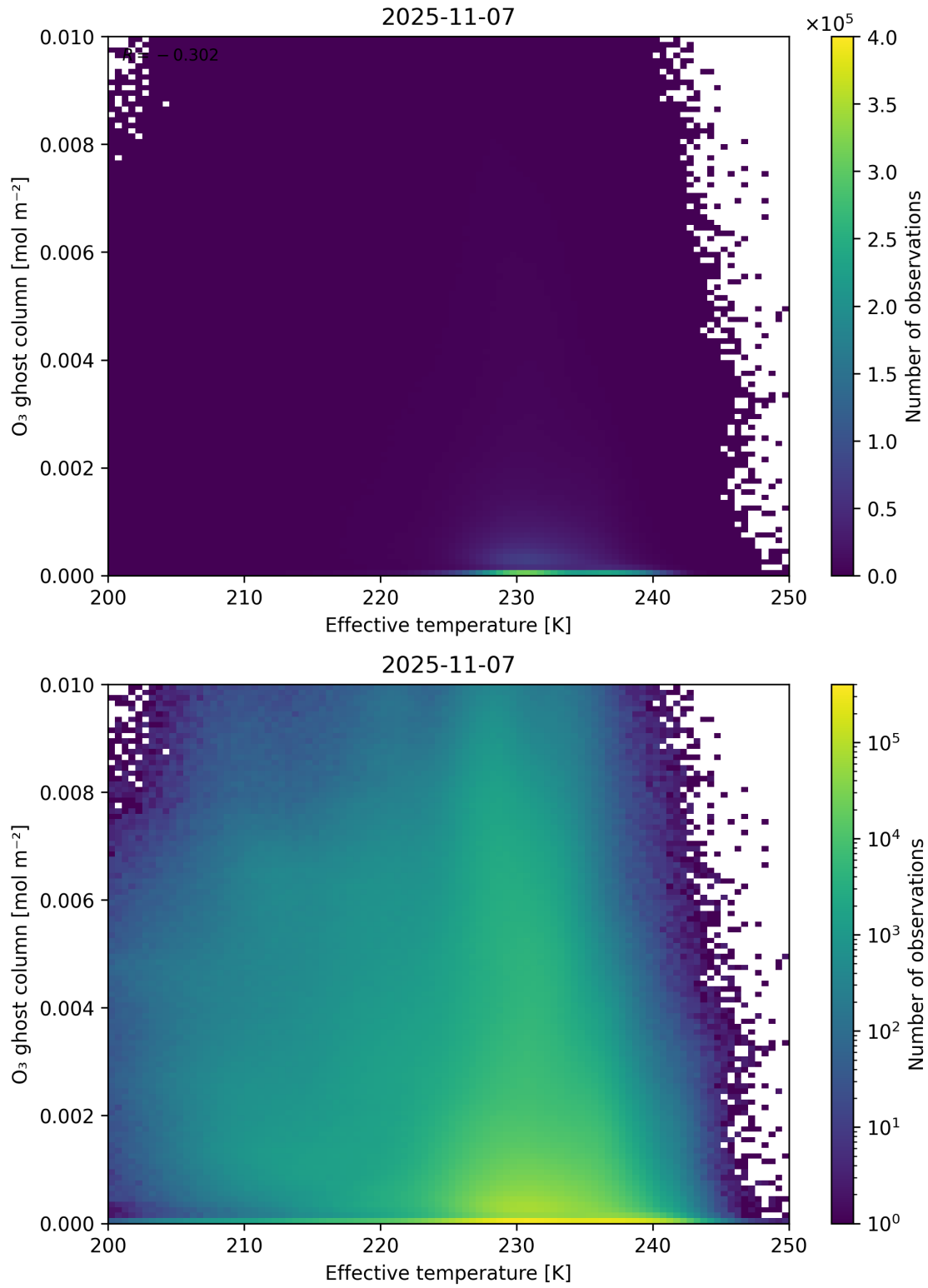
Figure 38: Scatter density plot of “Effective temperature” against “O 3 ghost column” for 2025-11-07 to 2025-11-08.
