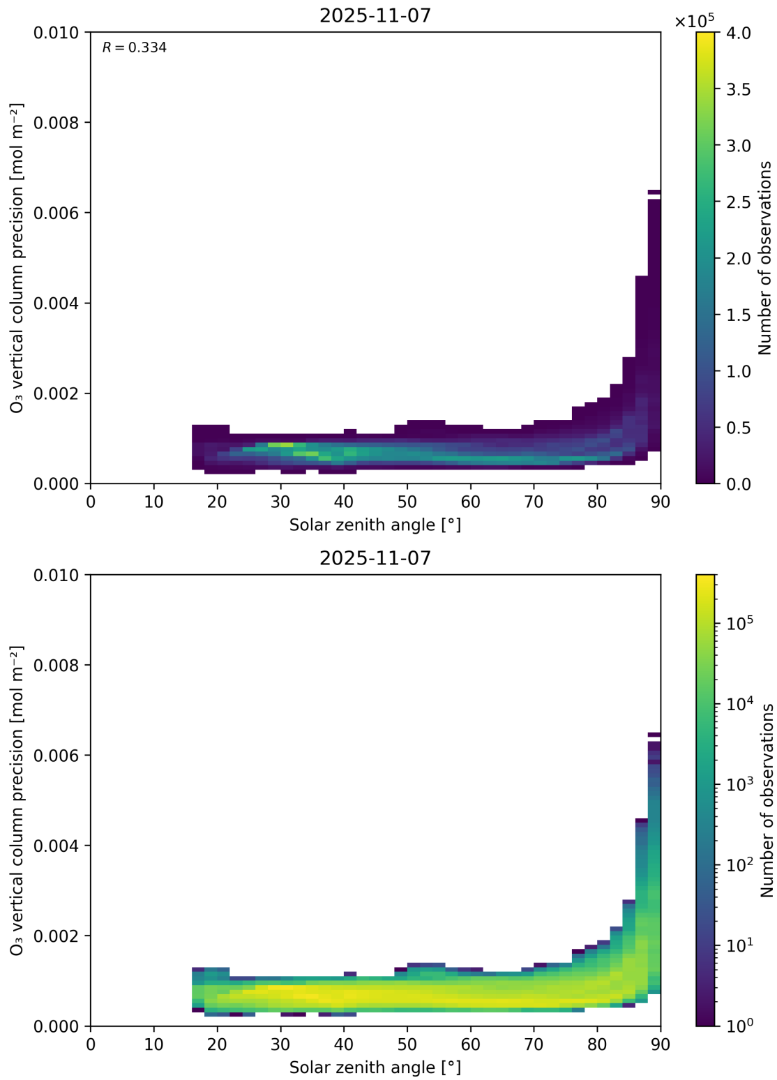
Figure 48: Scatter density plot of “Solar zenith angle” against “O 3 vertical column precision” for 2025-11-07 to 2025-11-08.
