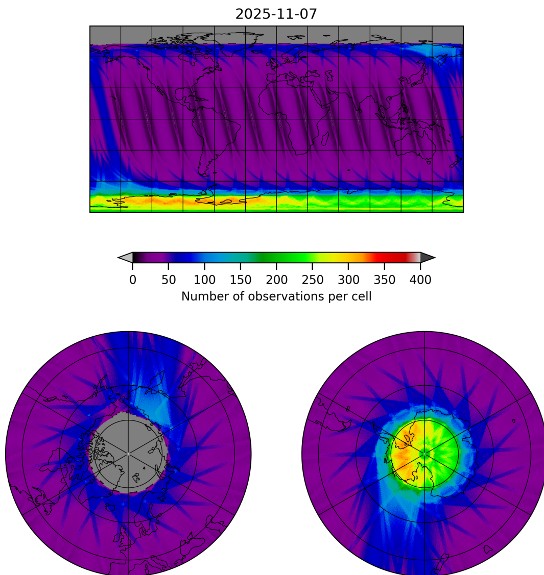
Figure 12: Map of the number of observations for 2025-11-07 to 2025-11-08
