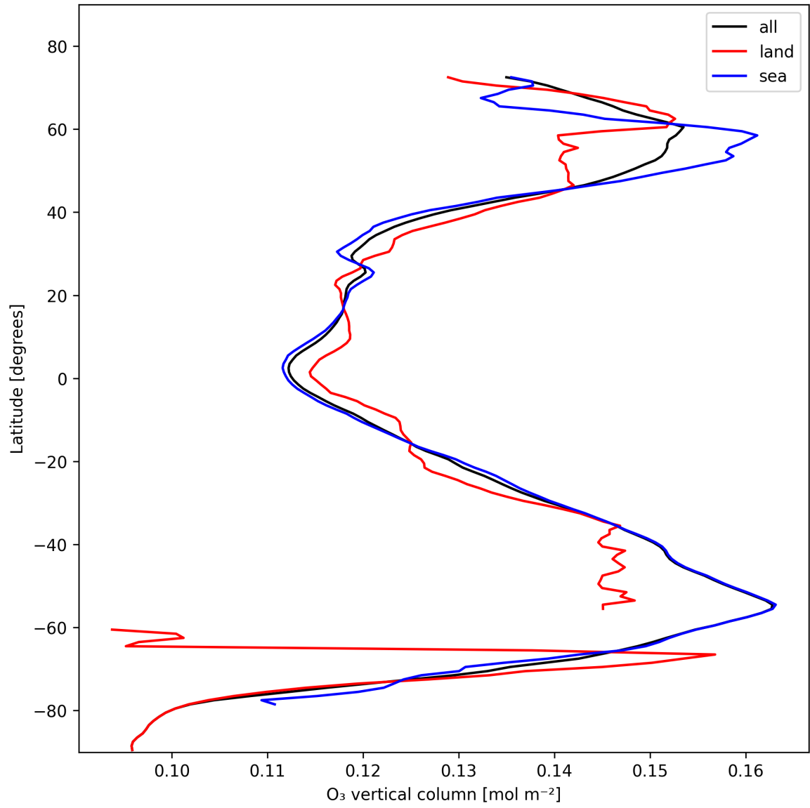
Figure 14: Zonal average of “O 3 vertical column” for 2025-11-07 to 2025-11-08.
