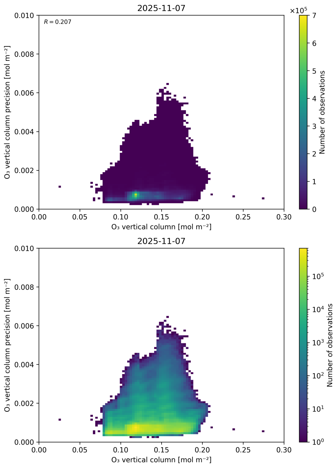
Figure 41: Scatter density plot of “O 3 vertical column” against “O 3 vertical column precision” for 2025-11-07 to 2025-11-08.
