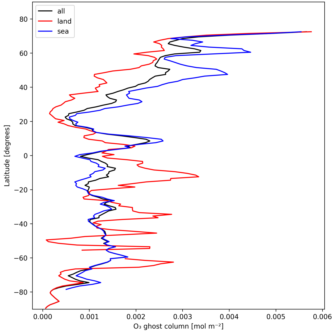
Figure 18: Zonal average of “O 3 ghost column” for 2025-11-07 to 2025-11-08.
