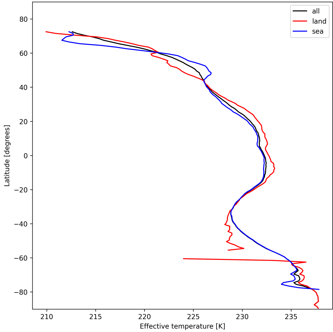
Figure 17: Zonal average of “Effective temperature” for 2025-11-07 to 2025-11-08.
