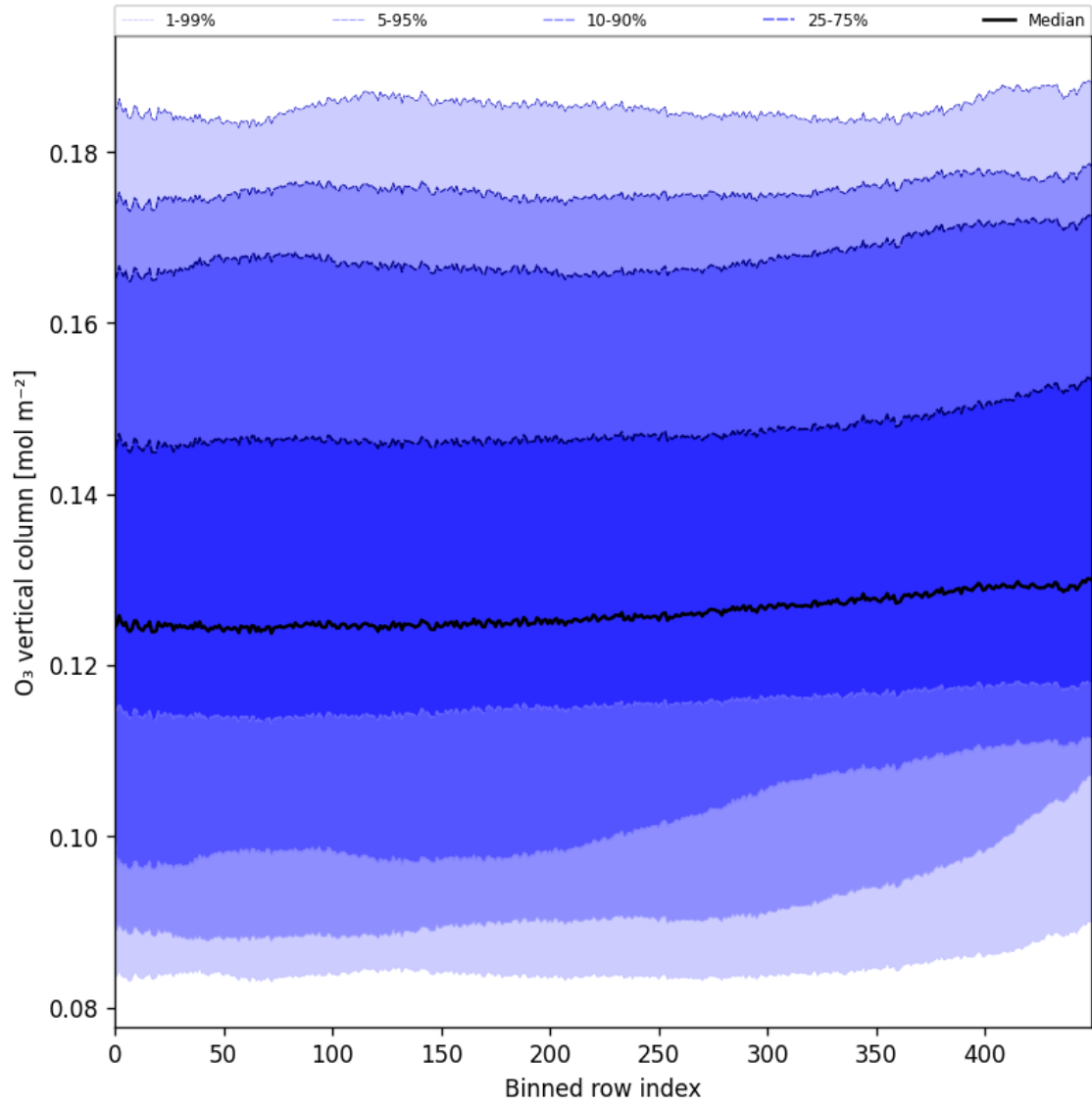
Figure 28: Along track statistics of “O 3 vertical column” for 2025-11-07 to 2025-11-08
