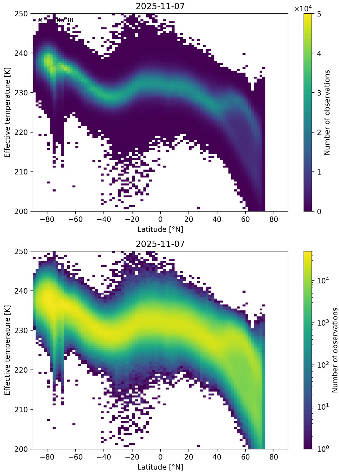
Figure 34: Scatter density plot of “Latitude” against “Effective temperature” for 2025-11-07 to 2025-11-08.
