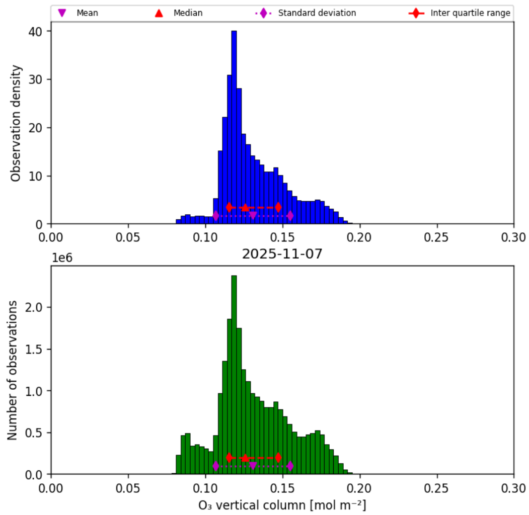
Figure 21: Histogram of “O 3 vertical column” for 2025-11-07 to 2025-11-08
