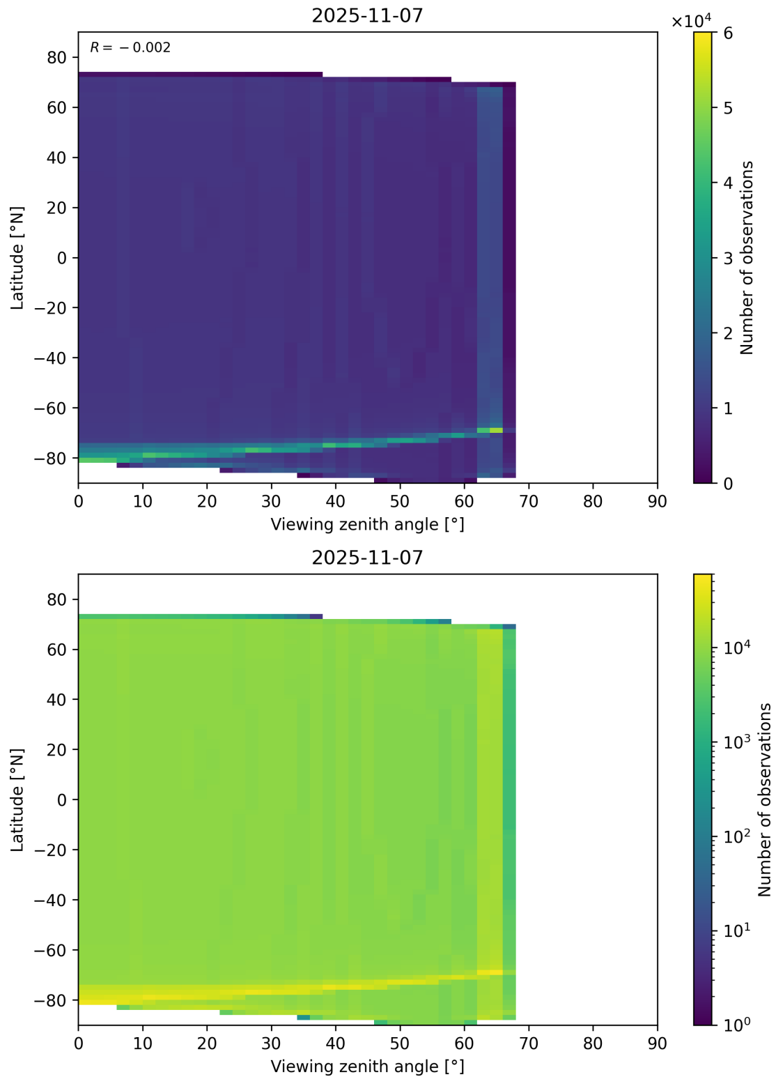
Figure 49: Scatter density plot of “Viewing zenith angle” against “Latitude” for 2025-11-07 to 2025-11-08.
