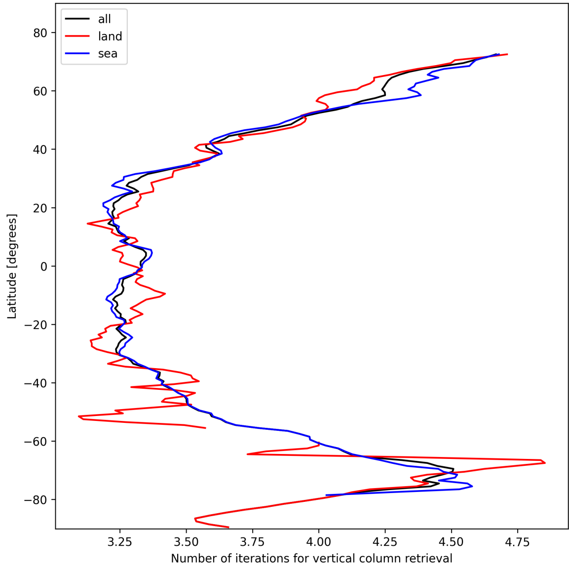
Figure 19: Zonal average of “Number of iterations for vertical column retrieval” for 2025-11-07 to 2025-11-08.
