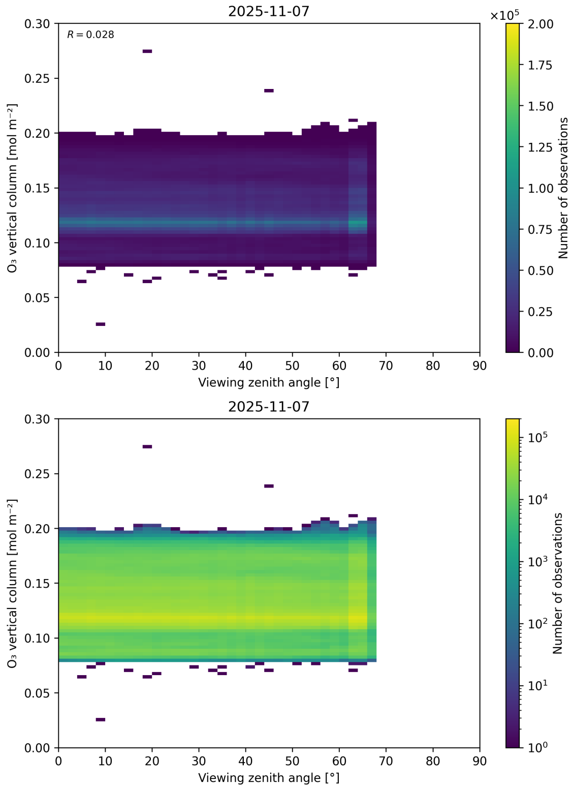
Figure 52: Scatter density plot of “Viewing zenith angle” against “O 3 vertical column” for 2025-11-07 to 2025-11-08.
