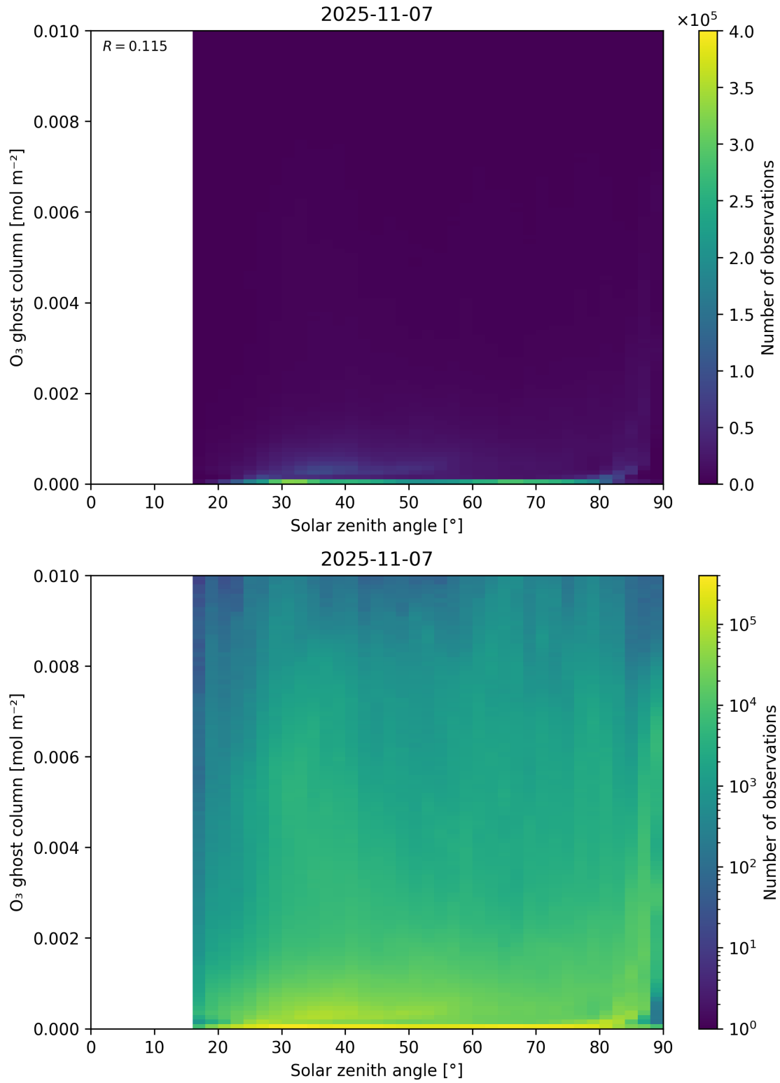
Figure 46: Scatter density plot of “Solar zenith angle” against “O 3 ghost column” for 2025-11-07 to 2025-11-08.
