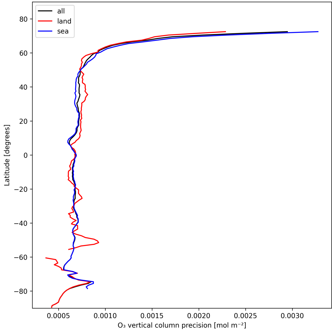
Figure 15: Zonal average of “O 3 vertical column precision” for 2025-11-07 to 2025-11-08.
