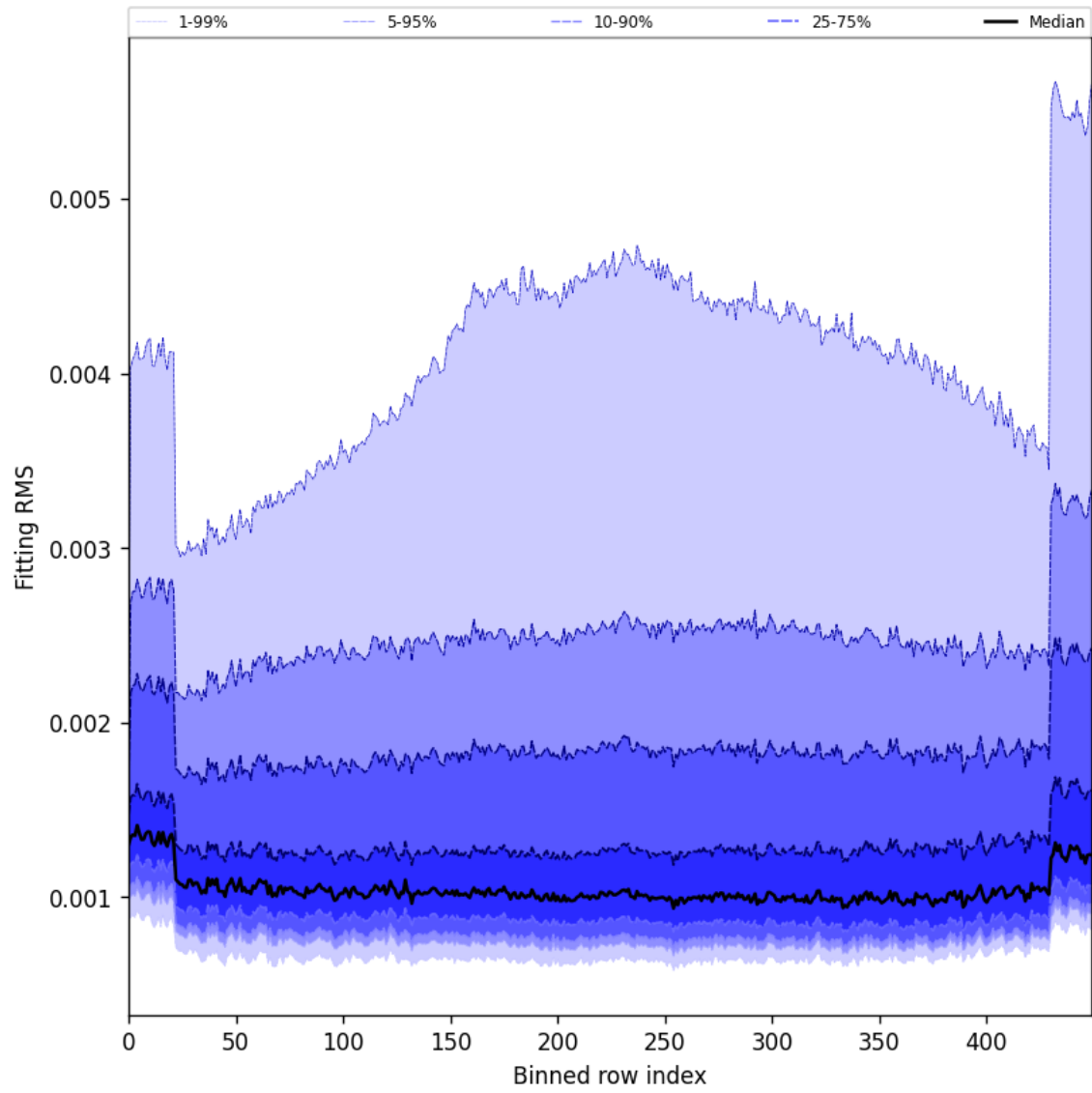
Figure 30: Along track statistics of “Fitting RMS” for 2025-11-07 to 2025-11-08
