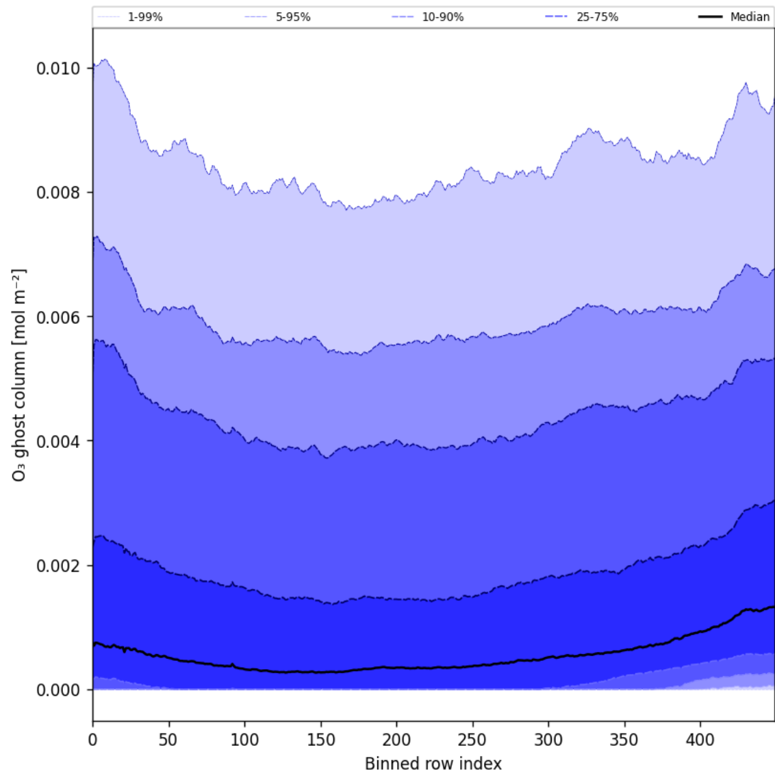
Figure 32: Along track statistics of “O 3 ghost column” for 2025-11-07 to 2025-11-08
