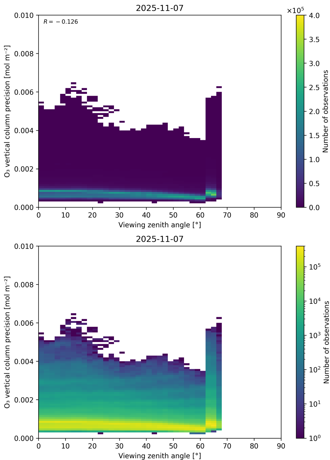
Figure 53: Scatter density plot of “Viewing zenith angle” against “O 3 vertical column precision” for 2025-11-07 to 2025-11-08.
