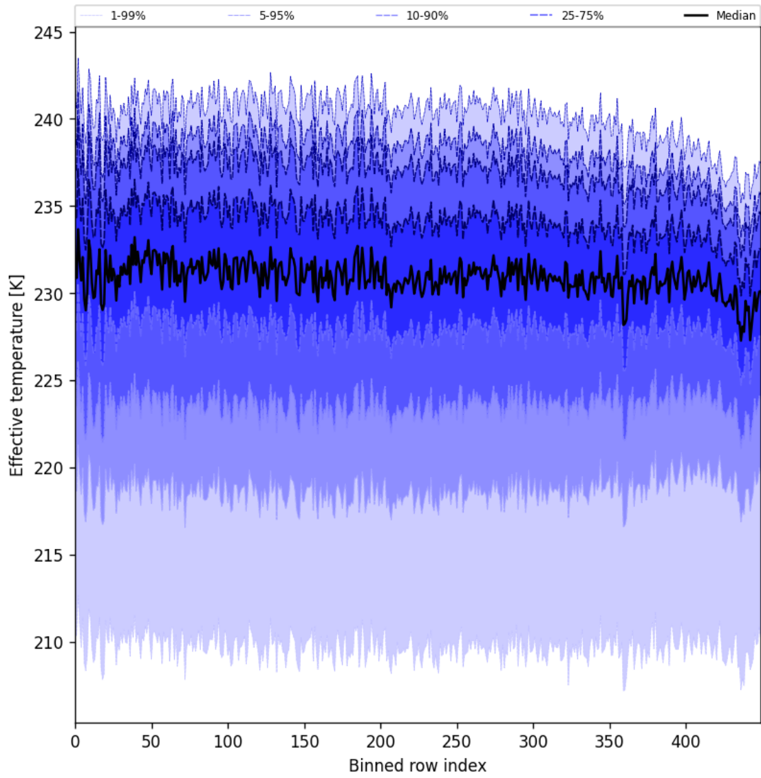
Figure 31: Along track statistics of “Effective temperature” for 2025-11-07 to 2025-11-08
