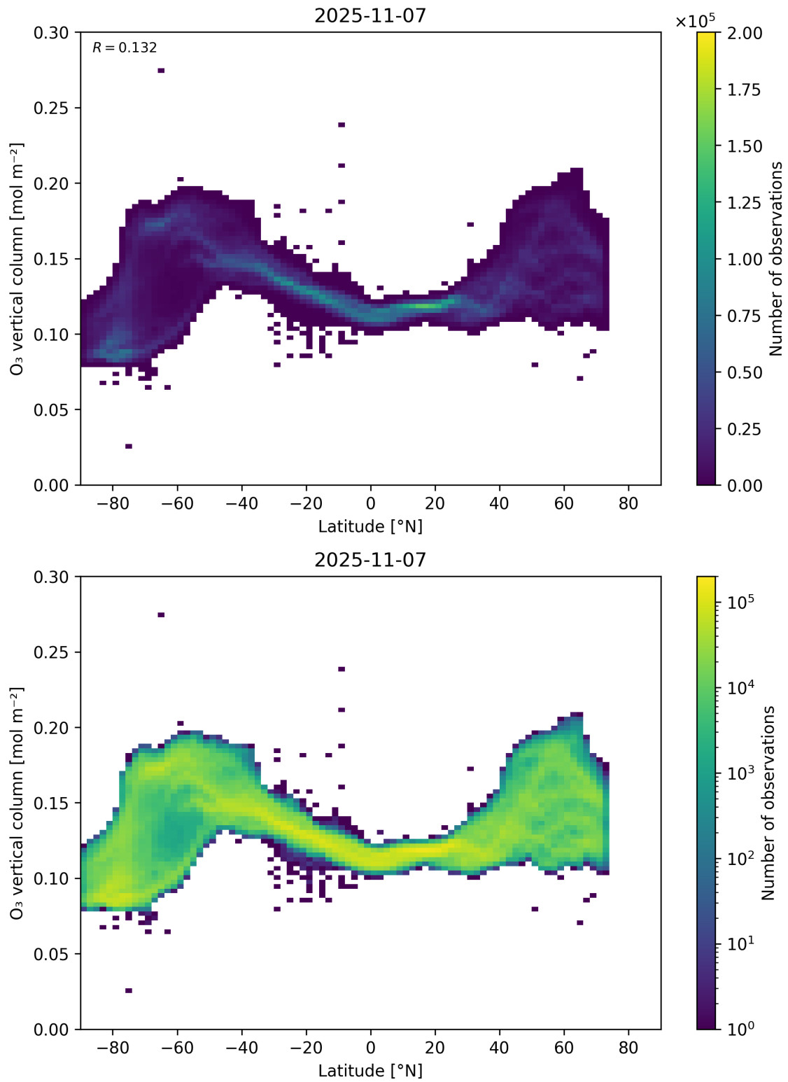
Figure 36: Scatter density plot of “Latitude” against “O 3 vertical column” for 2025-11-07 to 2025-11-08.
