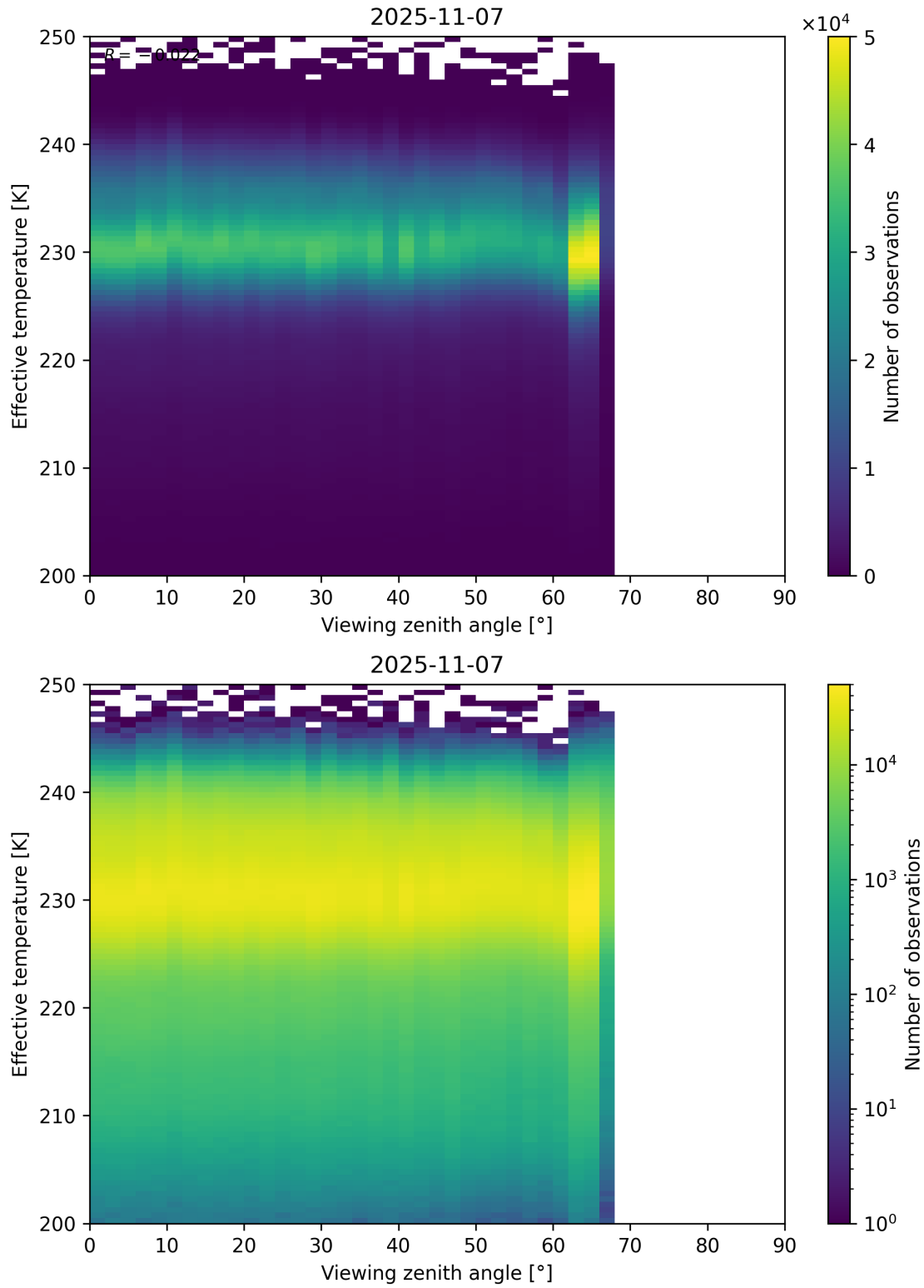
Figure 50: Scatter density plot of “Viewing zenith angle” against “Effective temperature” for 2025-11-07 to 2025-11-08.
