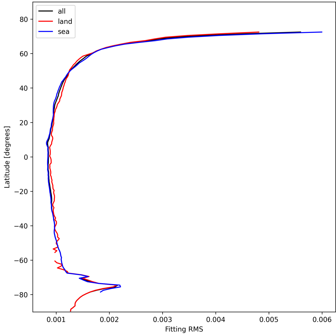
Figure 16: Zonal average of “Fitting RMS” for 2025-11-07 to 2025-11-08.
