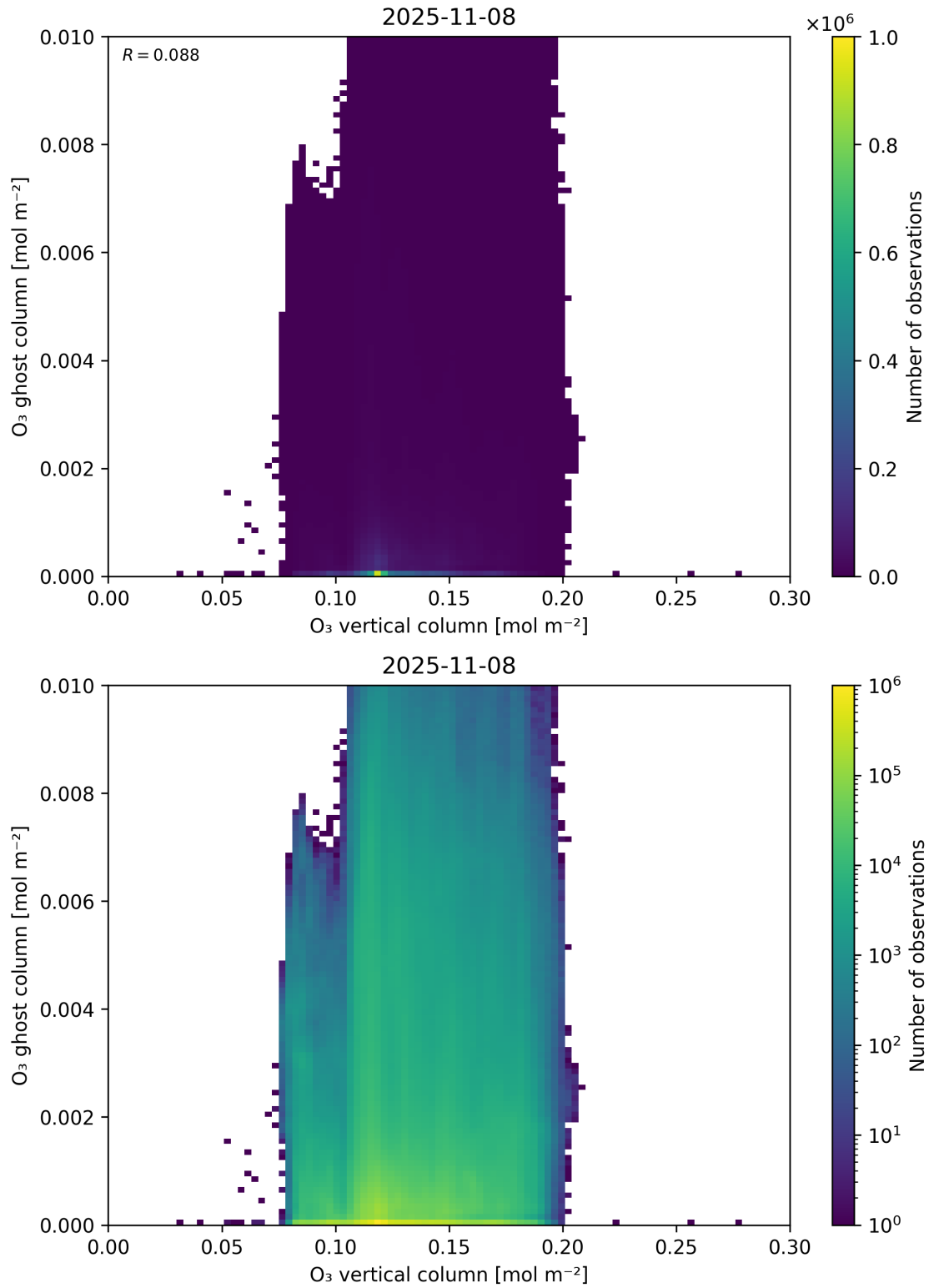
Figure 40: Scatter density plot of “O 3 vertical column” against “O 3 ghost column” for 2025-11-07 to 2025-11-09.
