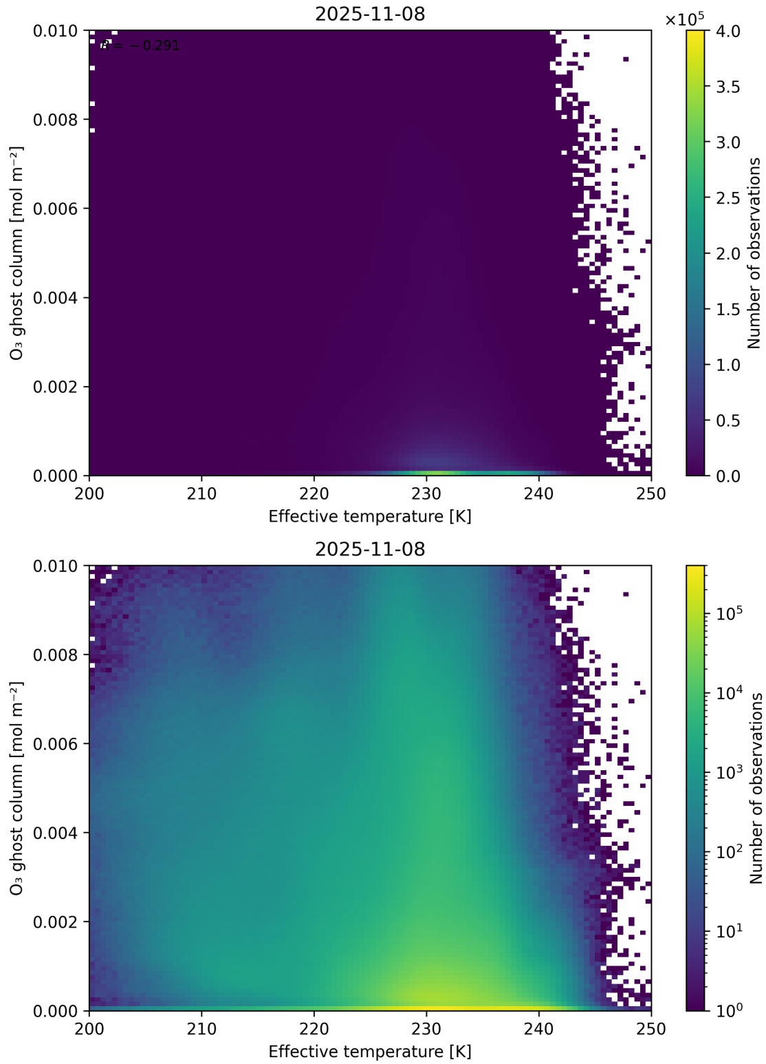
Figure 38: Scatter density plot of “Effective temperature” against “O 3 ghost column” for 2025-11-07 to 2025-11-09.
