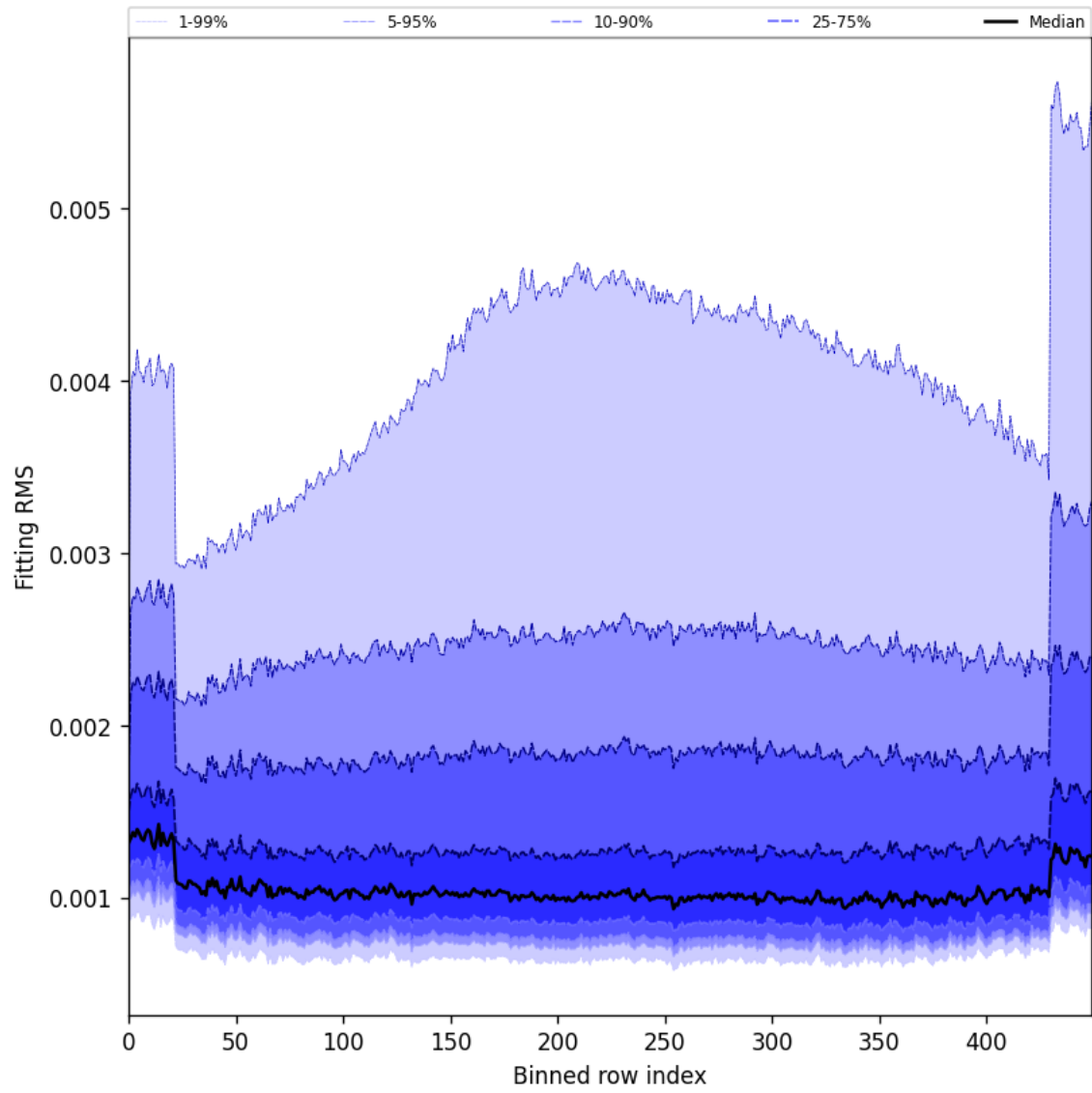
Figure 30: Along track statistics of “Fitting RMS” for 2025-11-07 to 2025-11-09
