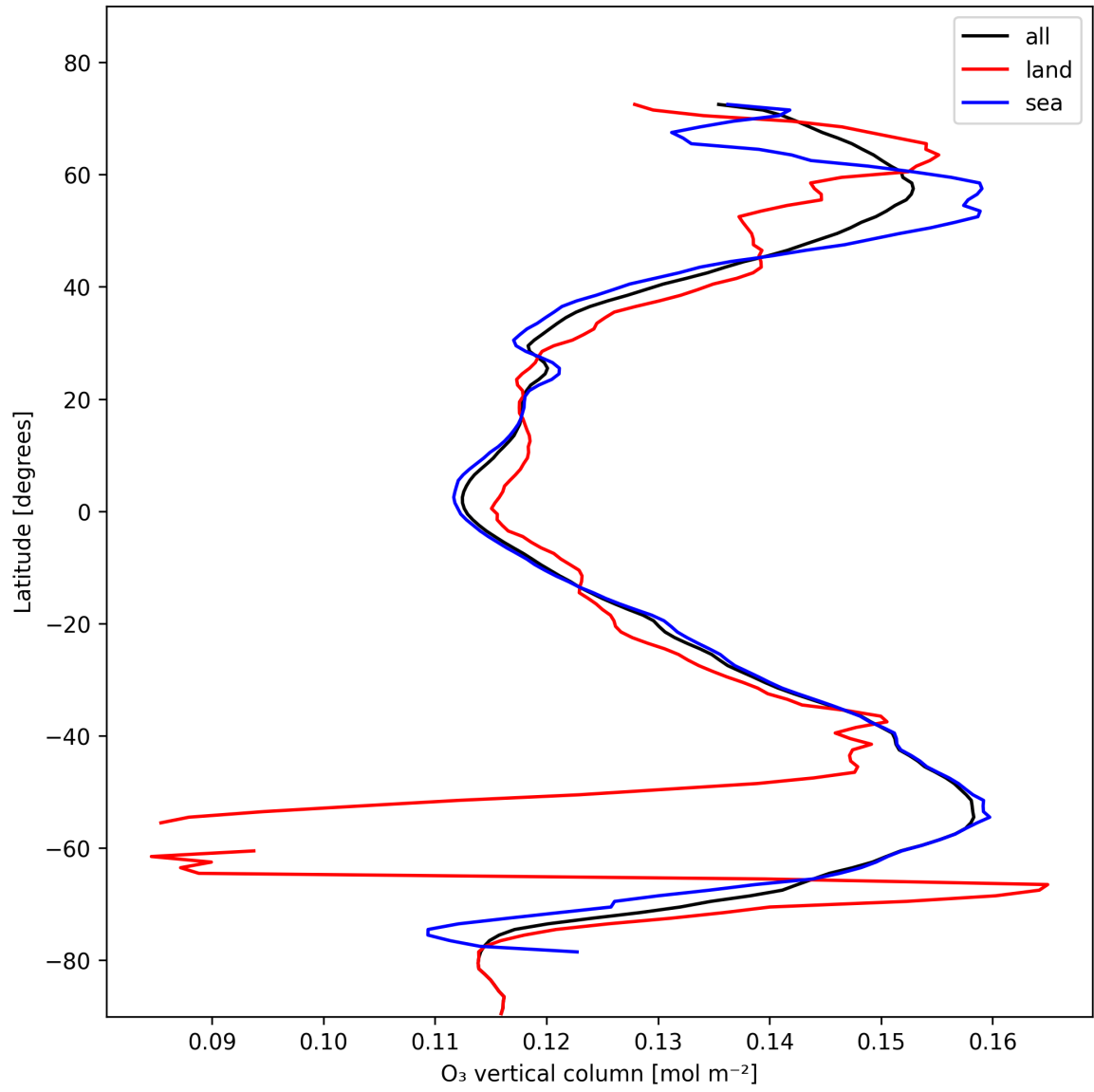
Figure 14: Zonal average of “O 3 vertical column” for 2025-11-07 to 2025-11-09.
