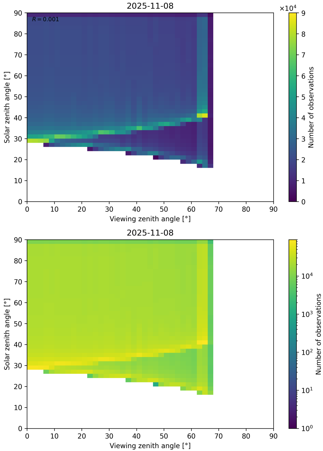
Figure 54: Scatter density plot of “Viewing zenith angle” against “Solar zenith angle” for 2025-11-07 to 2025-11-09.
