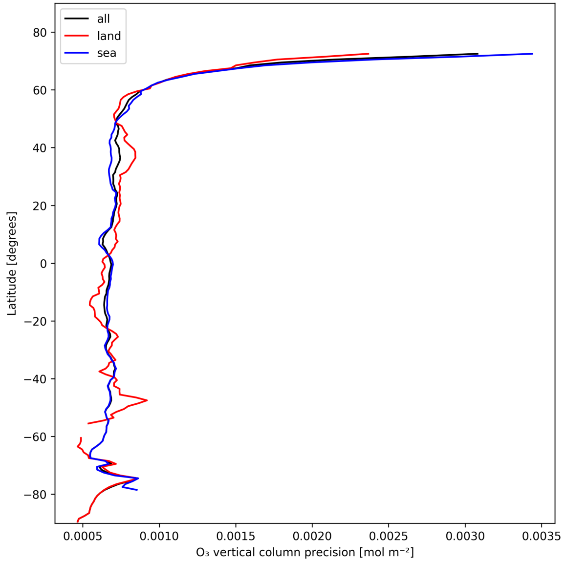
Figure 15: Zonal average of “O 3 vertical column precision” for 2025-11-07 to 2025-11-09.
