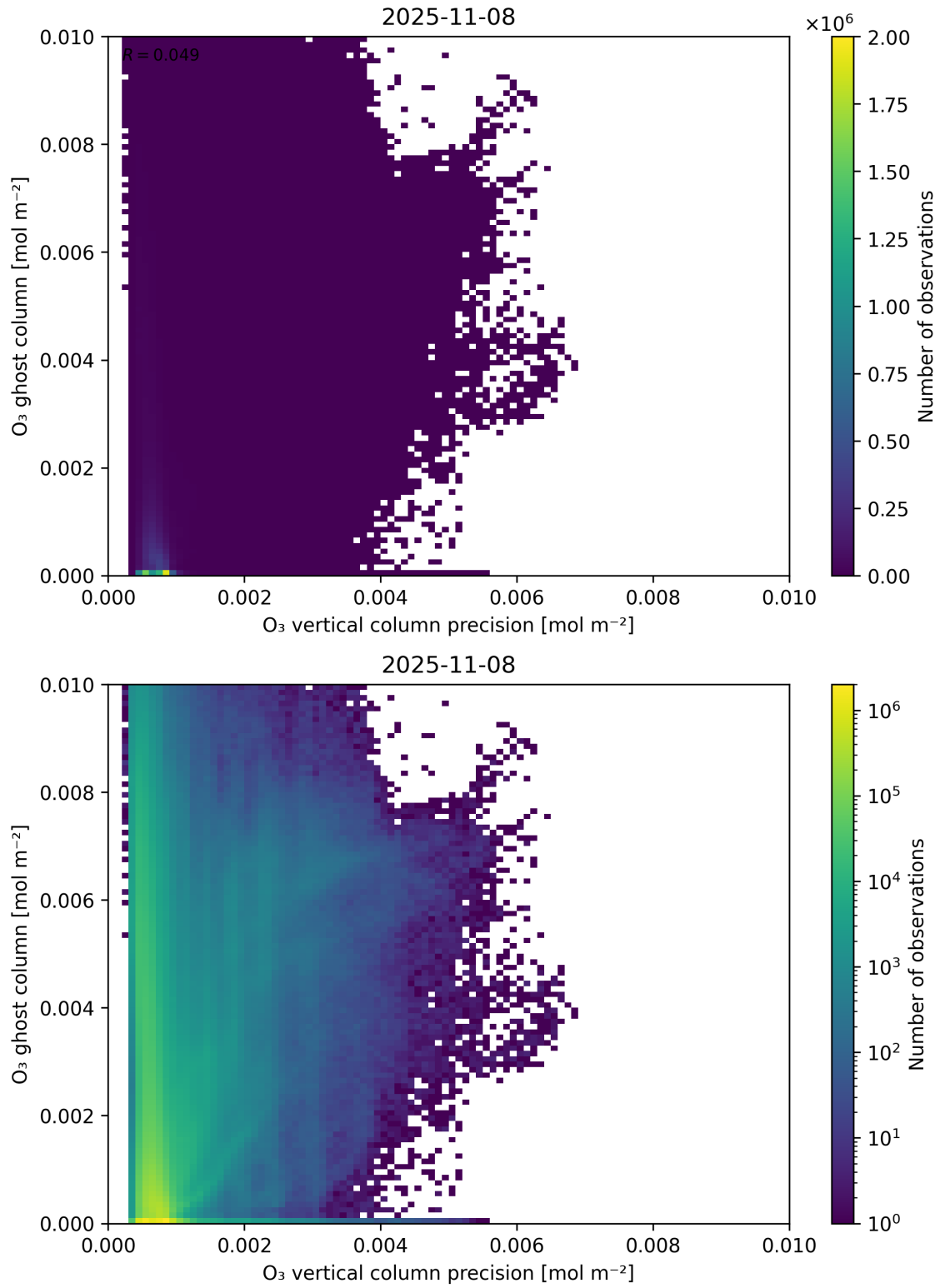
Figure 43: Scatter density plot of “O 3 vertical column precision” against “O 3 ghost column” for 2025-11-07 to 2025-11-09.
