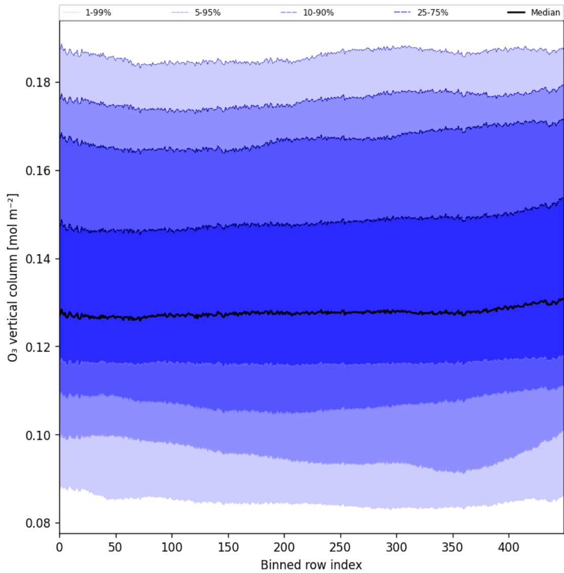
Figure 28: Along track statistics of “O 3 vertical column” for 2025-11-07 to 2025-11-09
