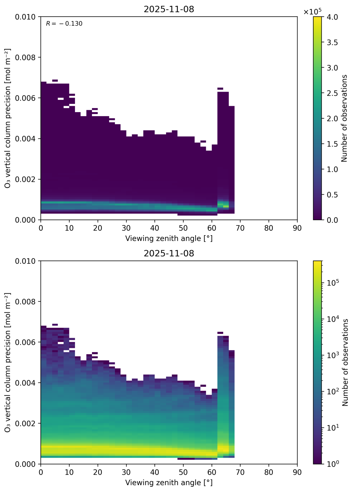
Figure 53: Scatter density plot of “Viewing zenith angle” against “O 3 vertical column precision” for 2025-11-07 to 2025-11-09.
