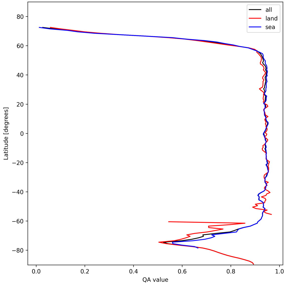
Figure 13: Zonal average of “QA value” for 2025-11-07 to 2025-11-09.
