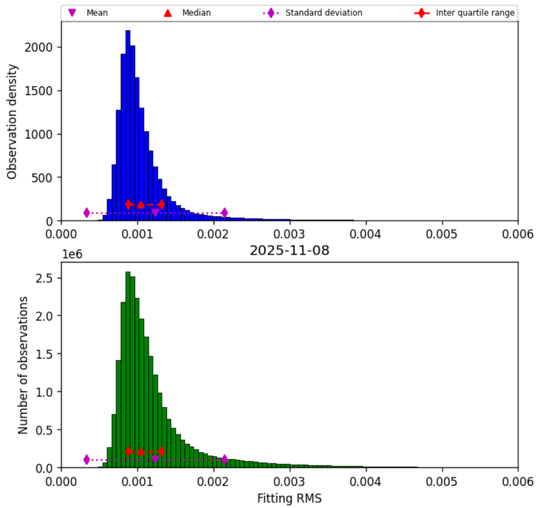
Figure 23: Histogram of “Fitting RMS” for 2025-11-07 to 2025-11-09
