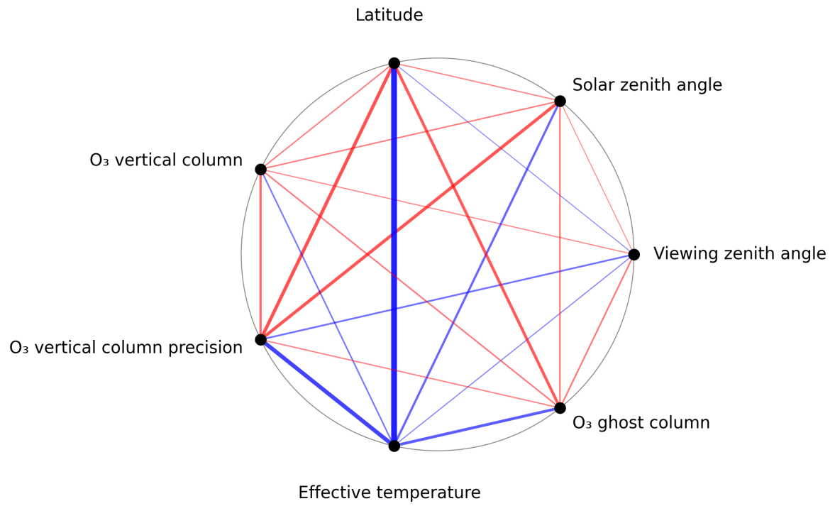
Figure 1: Map of correlation graph for 2025-11-07 to 2025-11-09.
