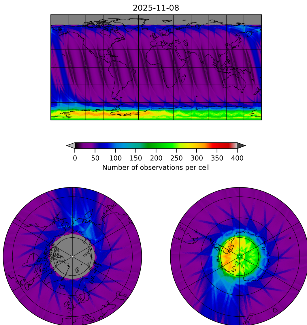
Figure 12: Map of the number of observations for 2025-11-07 to 2025-11-09
