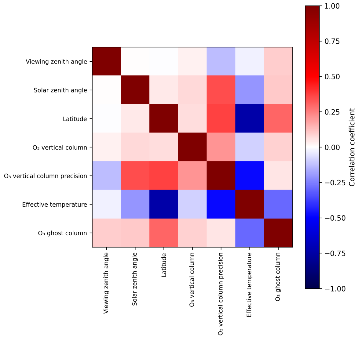
Figure 2: Map of correlation matrix for 2025-11-07 to 2025-11-09.
