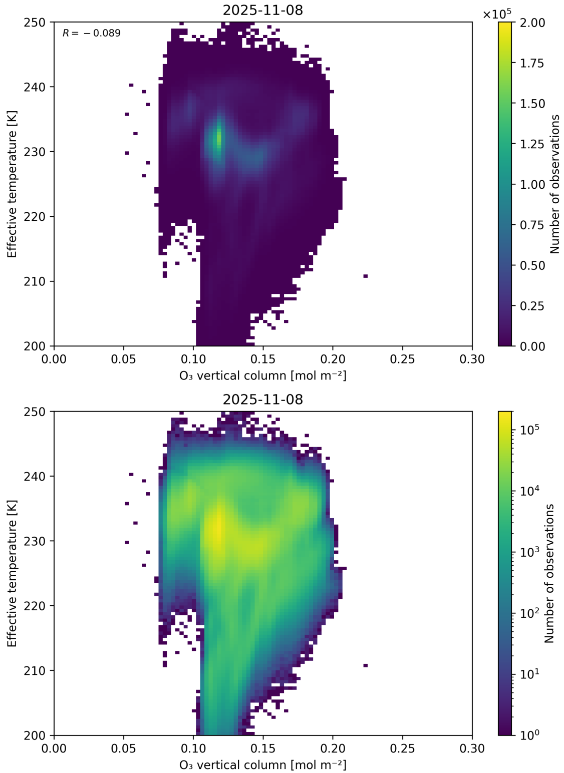
Figure 39: Scatter density plot of “O 3 vertical column” against “Effective temperature” for 2025-11-07 to 2025-11-09.
