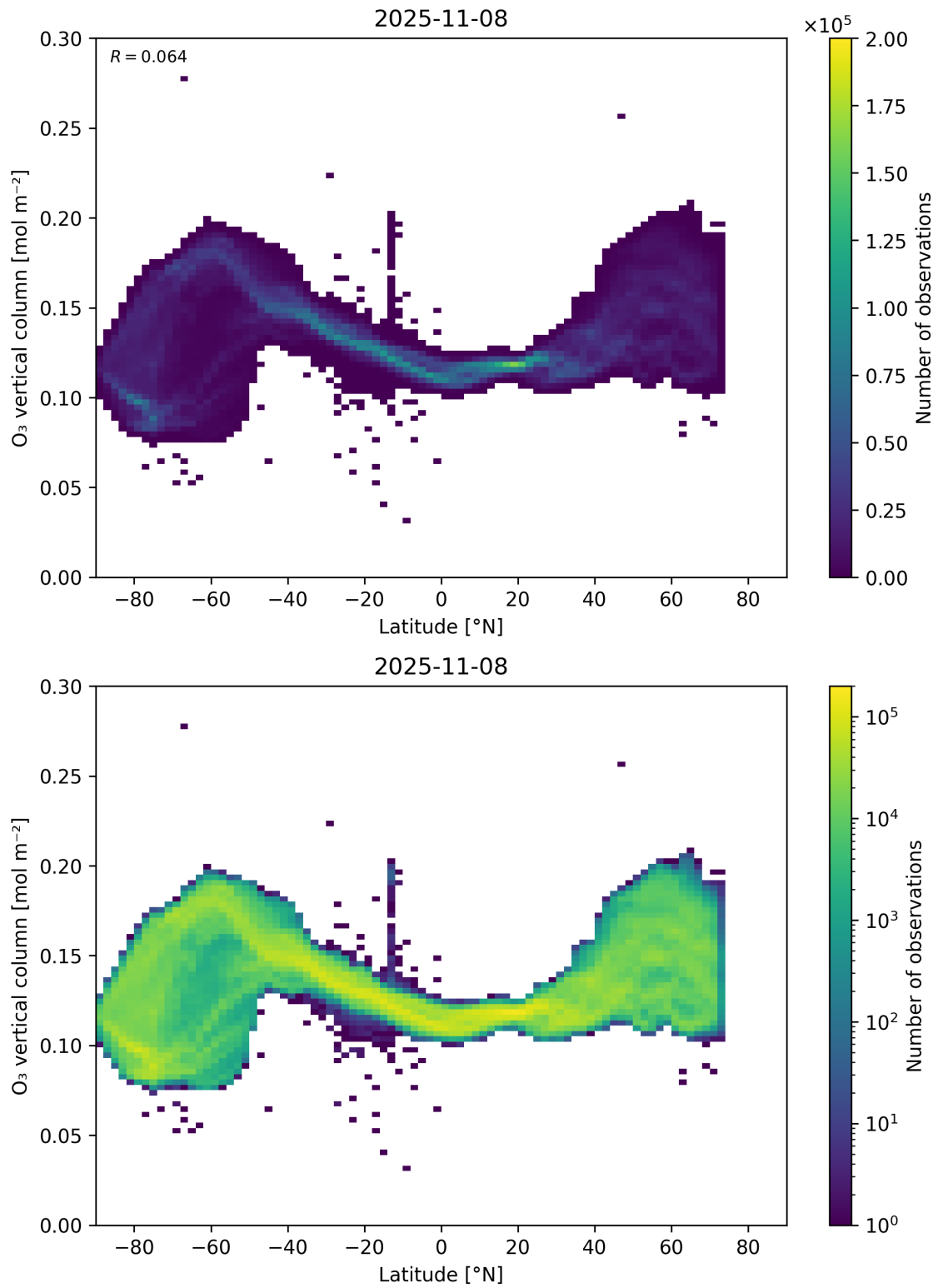
Figure 36: Scatter density plot of “Latitude” against “O 3 vertical column” for 2025-11-07 to 2025-11-09.
