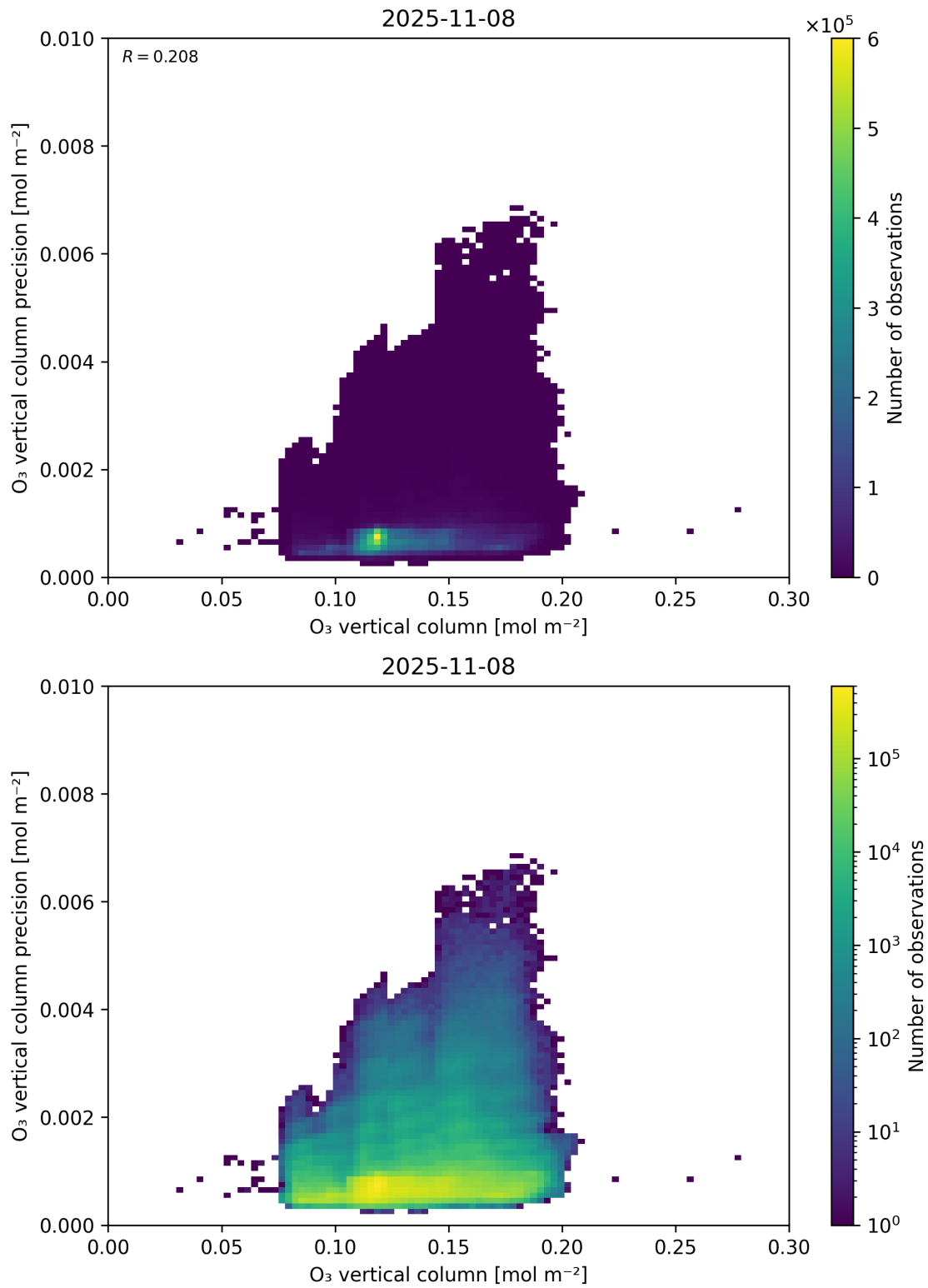
Figure 41: Scatter density plot of “O 3 vertical column” against “O 3 vertical column precision” for 2025-11-07 to 2025-11-09.
