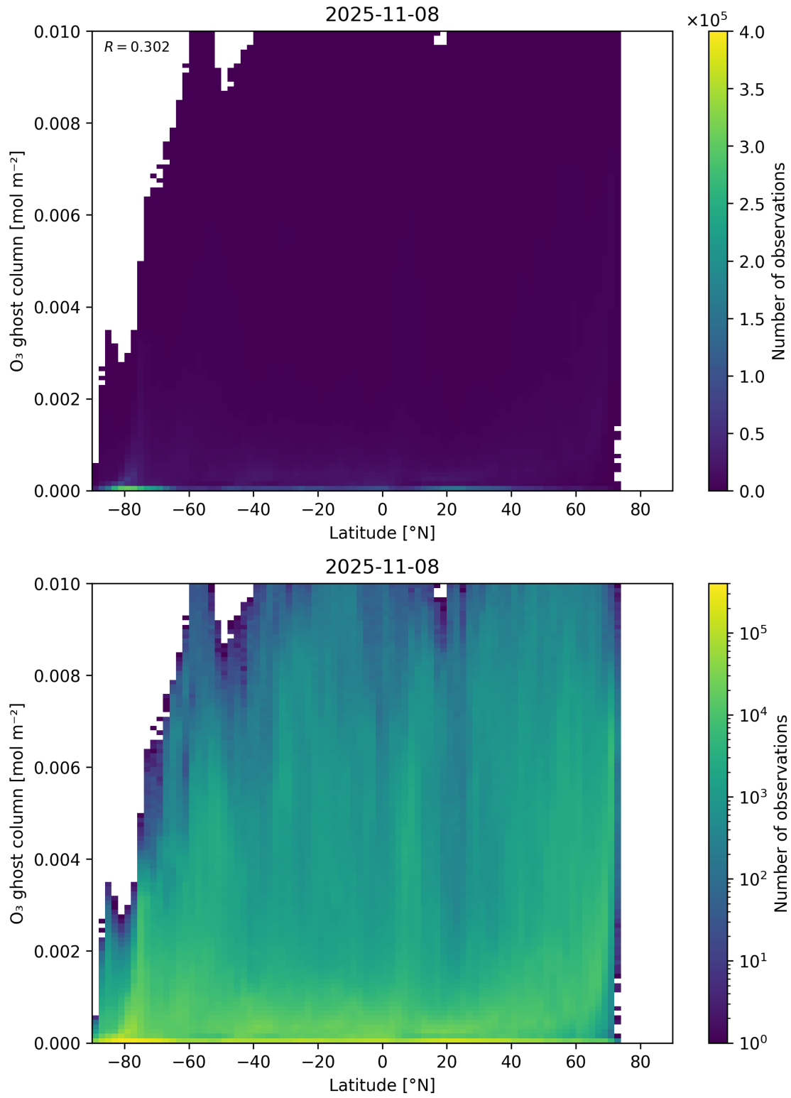
Figure 35: Scatter density plot of “Latitude” against “O 3 ghost column” for 2025-11-07 to 2025-11-09.
