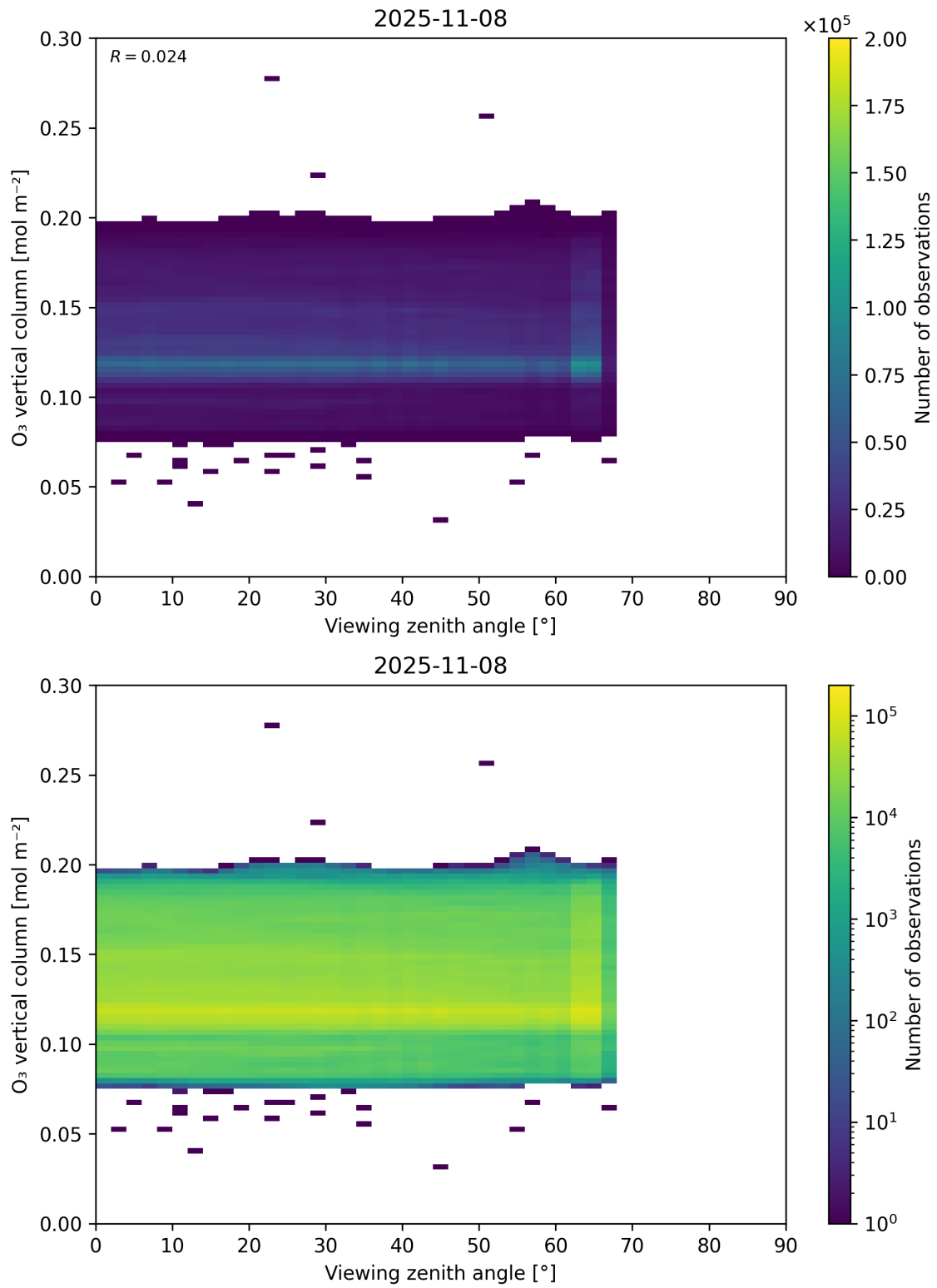
Figure 52: Scatter density plot of “Viewing zenith angle” against “O 3 vertical column” for 2025-11-07 to 2025-11-09.
