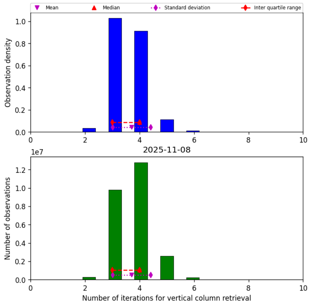
Figure 26: Histogram of “Number of iterations for vertical column retrieval” for 2025-11-07 to 2025-11-09
