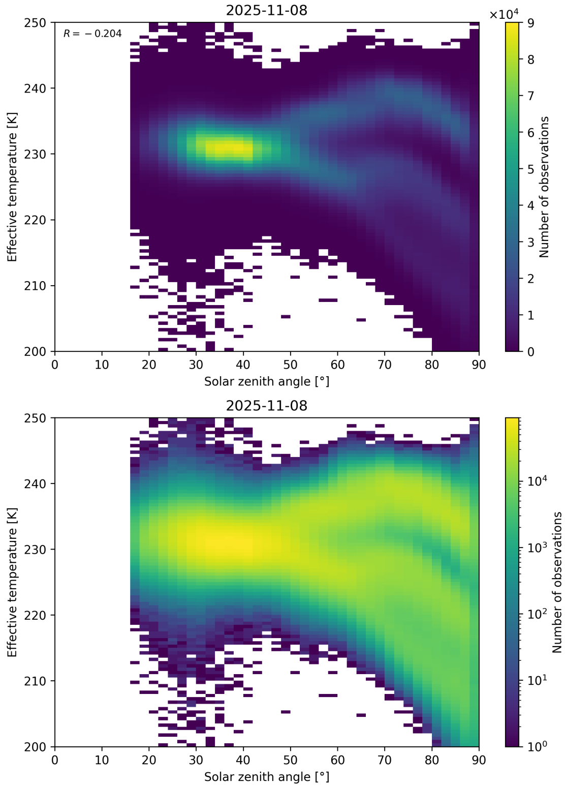
Figure 45: Scatter density plot of “Solar zenith angle” against “Effective temperature” for 2025-11-07 to 2025-11-09.
