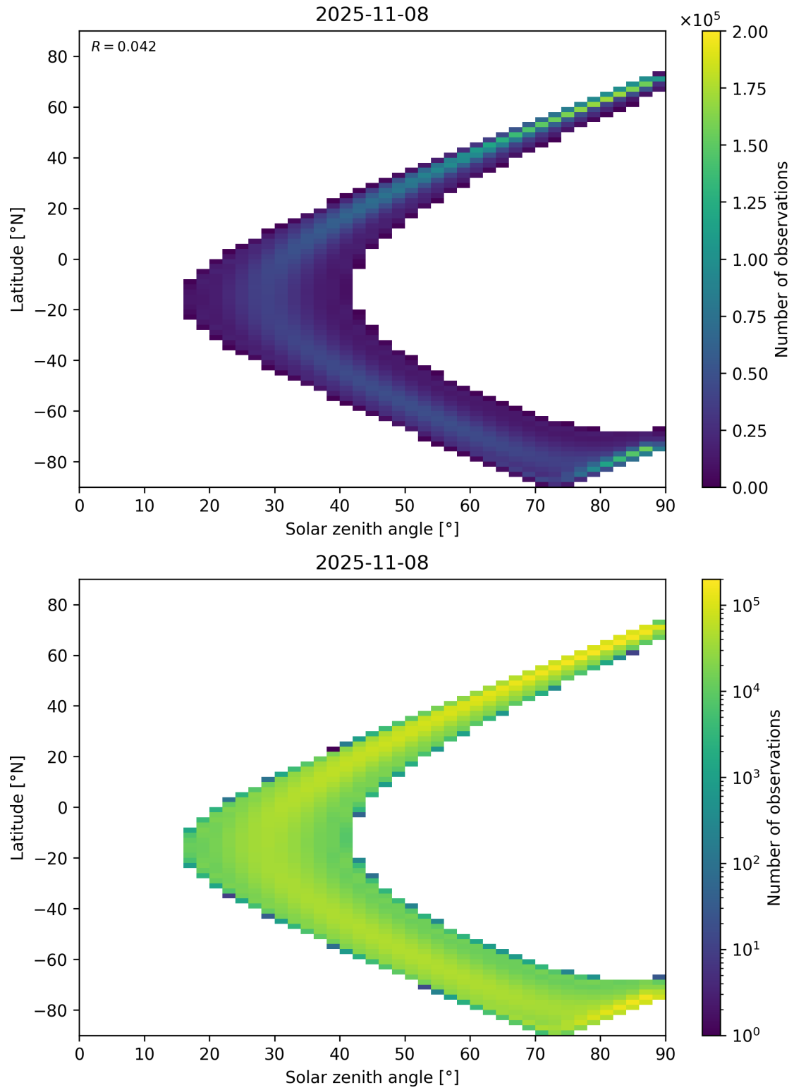
Figure 44: Scatter density plot of “Solar zenith angle” against “Latitude” for 2025-11-07 to 2025-11-09.
