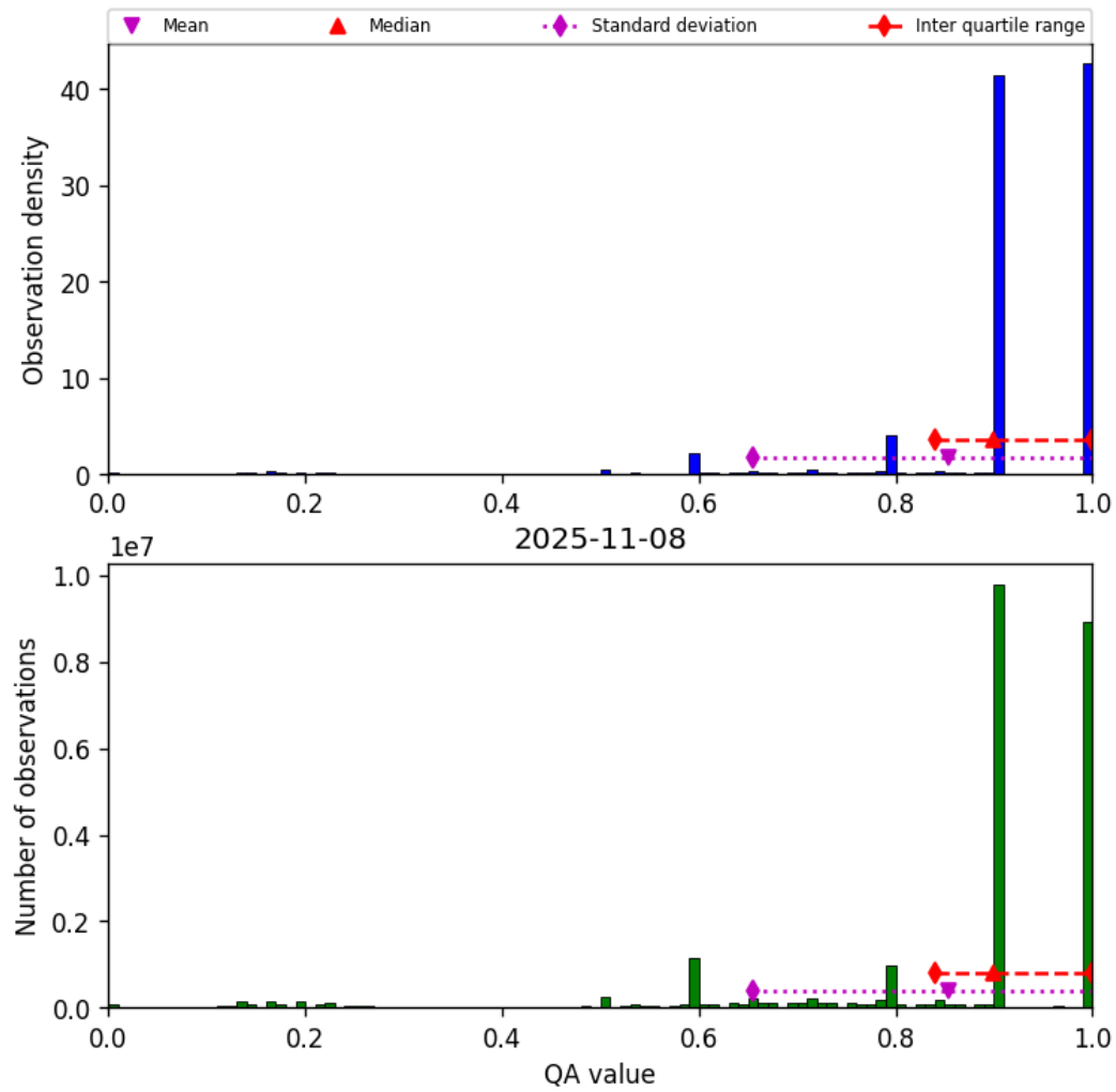
Figure 20: Histogram of “QA value” for 2025-11-07 to 2025-11-09
