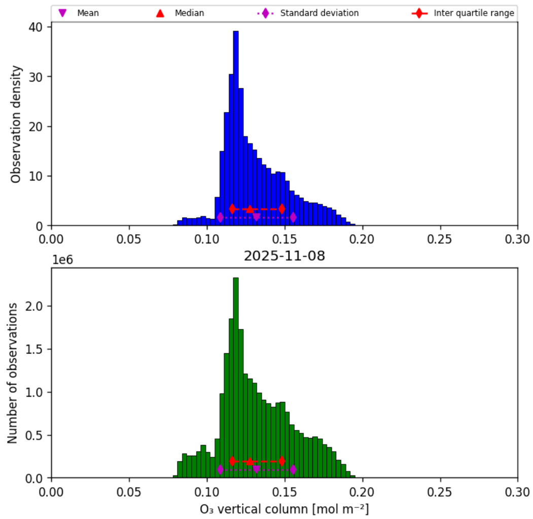
Figure 21: Histogram of “O 3 vertical column” for 2025-11-07 to 2025-11-09
