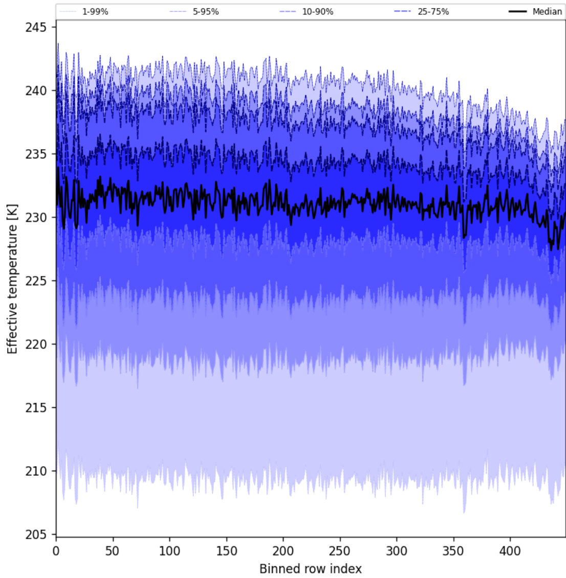
Figure 31: Along track statistics of “Effective temperature” for 2025-11-07 to 2025-11-09
