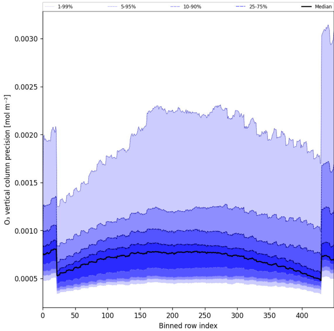
Figure 29: Along track statistics of “O 3 vertical column precision” for 2025-11-07 to 2025-11-09
