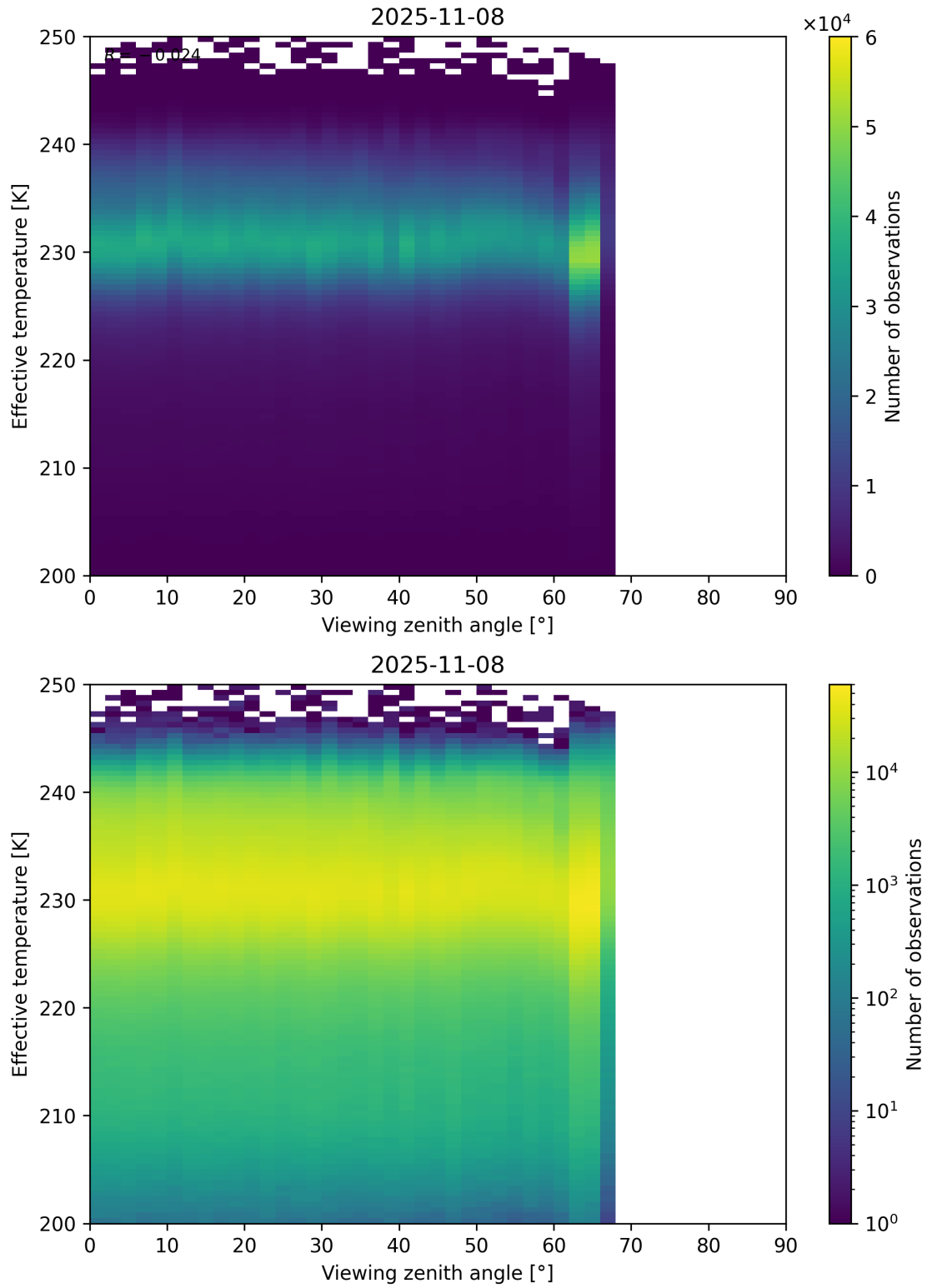
Figure 50: Scatter density plot of “Viewing zenith angle” against “Effective temperature” for 2025-11-07 to 2025-11-09.
