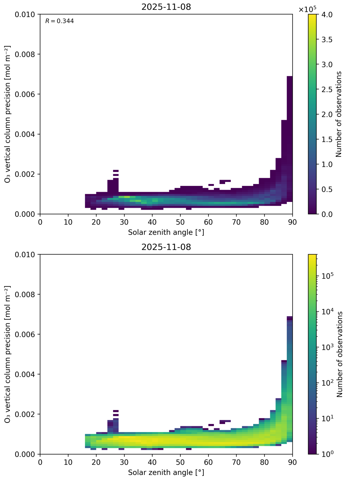
Figure 48: Scatter density plot of “Solar zenith angle” against “O 3 vertical column precision” for 2025-11-07 to 2025-11-09.
