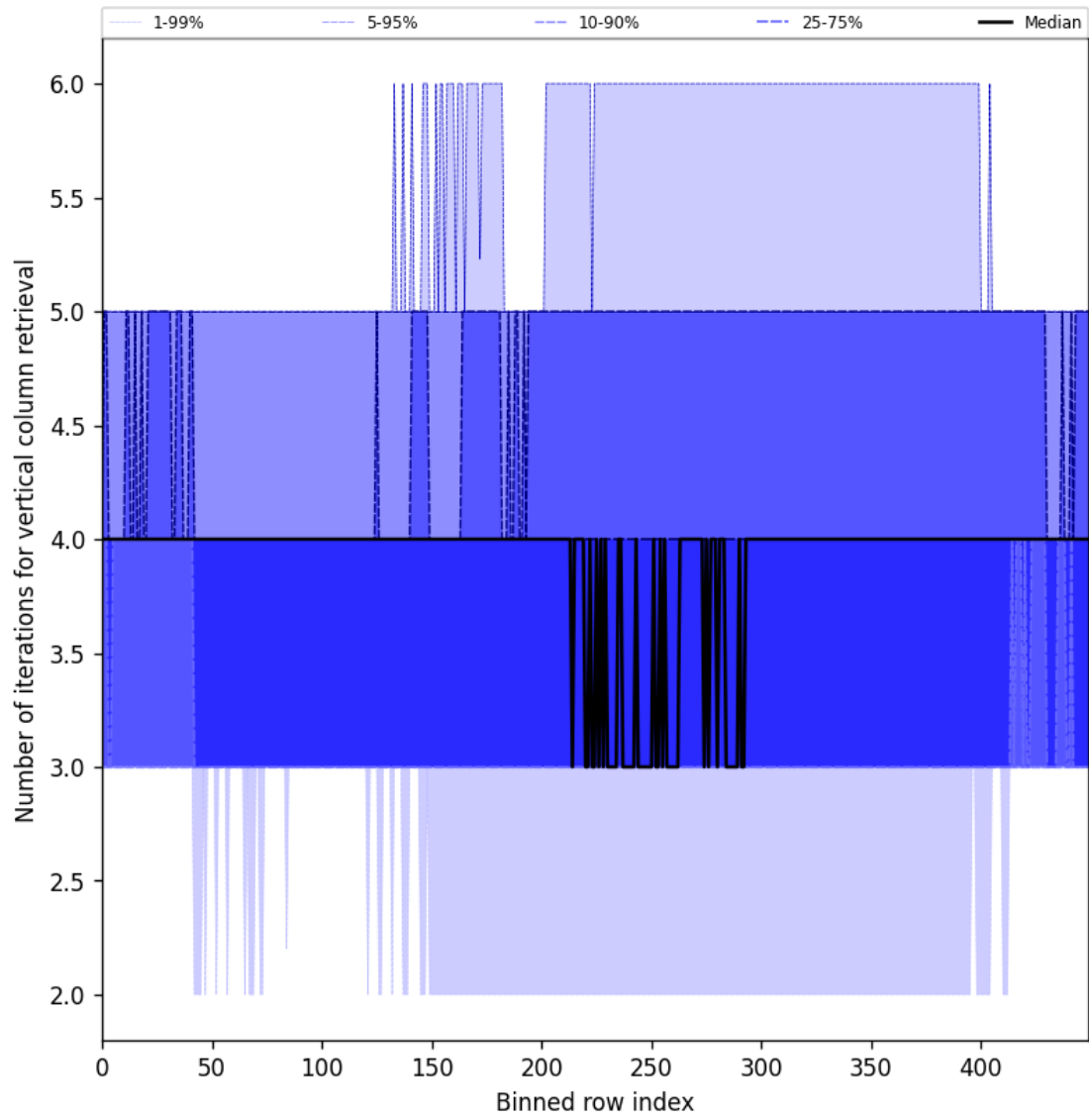
Figure 33: Along track statistics of “Number of iterations for vertical column retrieval” for 2025-11-07 to 2025-11-09
