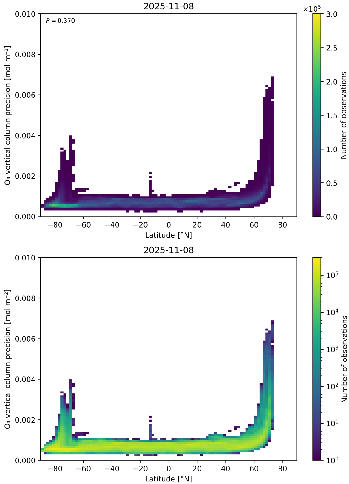
Figure 37: Scatter density plot of “Latitude” against “O 3 vertical column precision” for 2025-11-07 to 2025-11-09.
