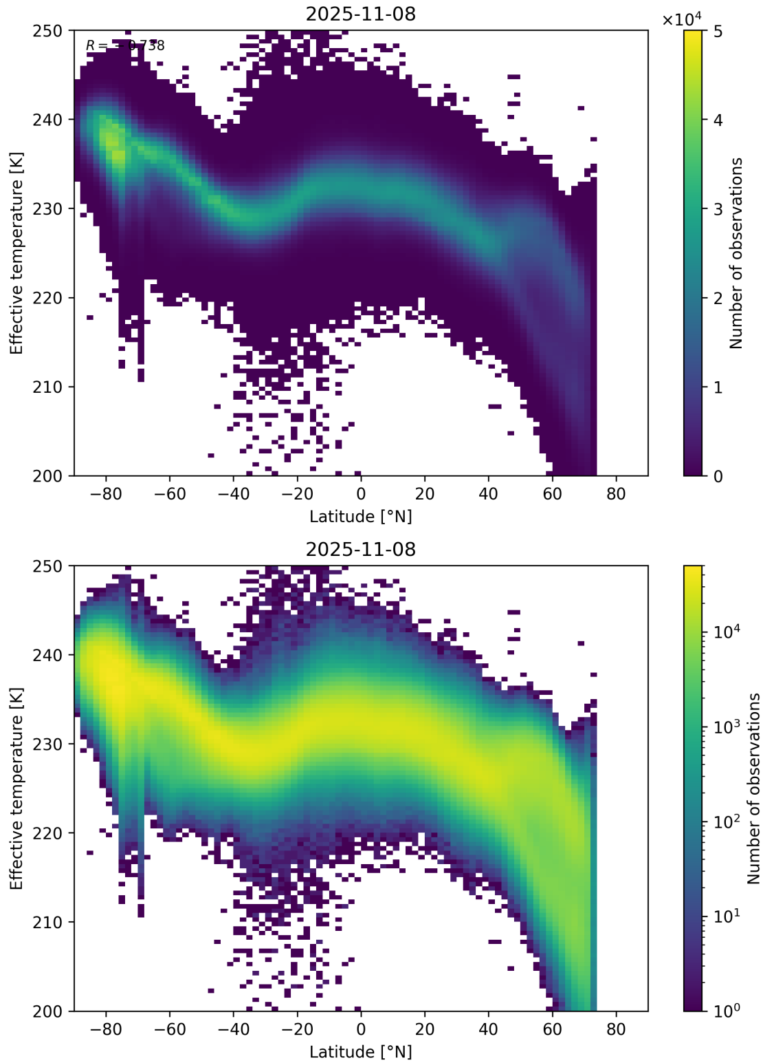
Figure 34: Scatter density plot of “Latitude” against “Effective temperature” for 2025-11-07 to 2025-11-09.
