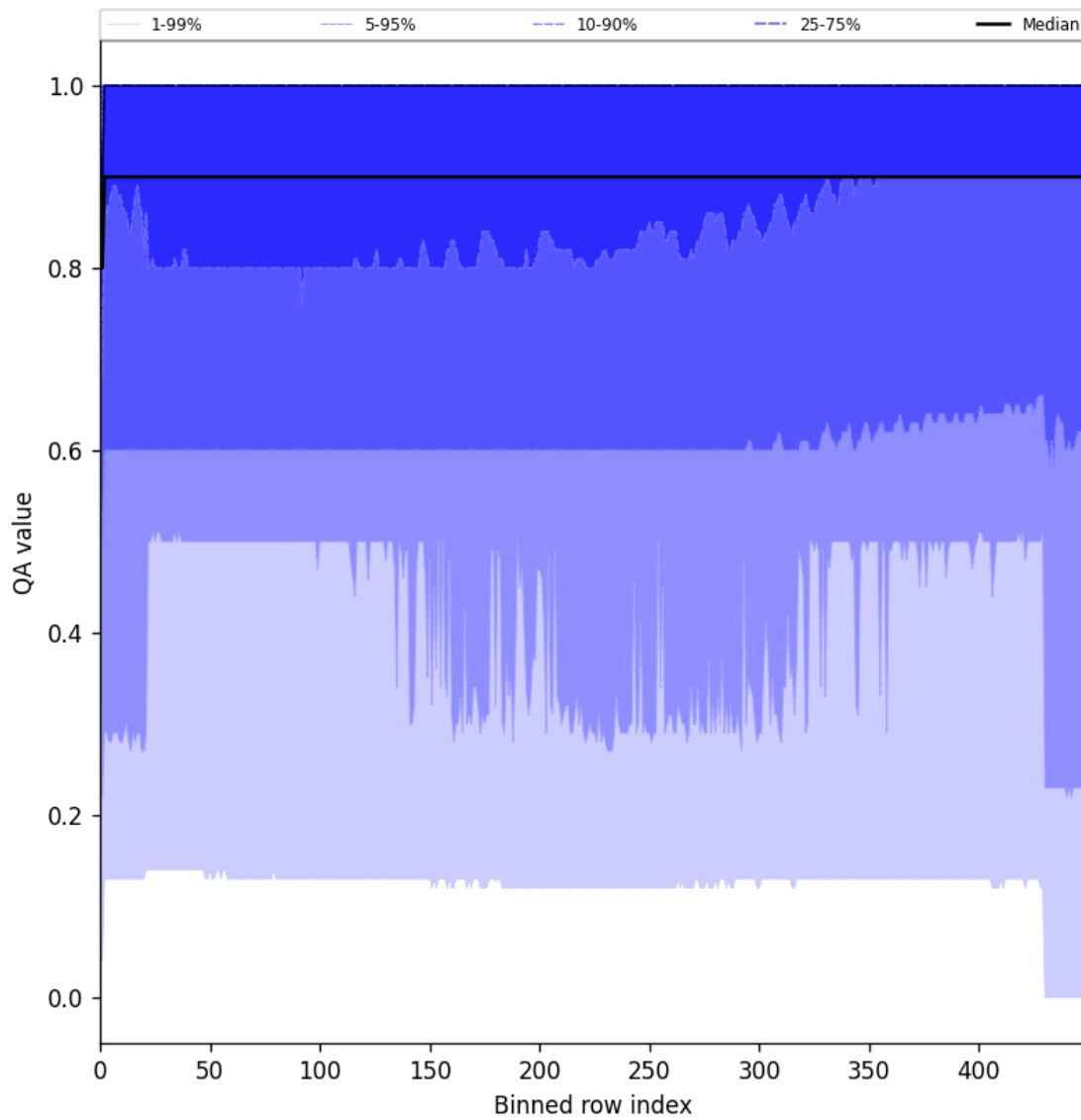
Figure 27: Along track statistics of “QA value” for 2025-11-07 to 2025-11-09
