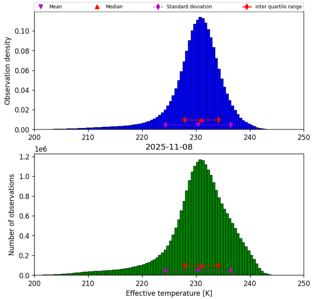
Figure 24: Histogram of “Effective temperature” for 2025-11-07 to 2025-11-09
