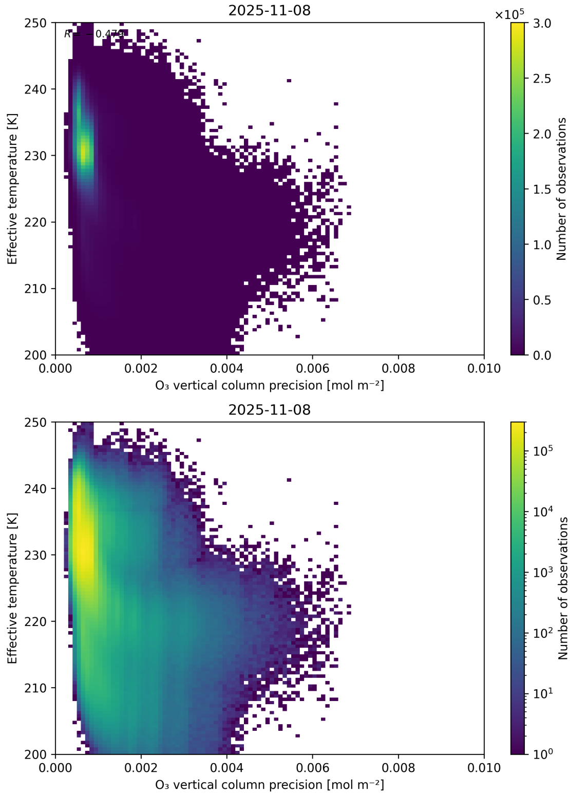
Figure 42: Scatter density plot of “O 3 vertical column precision” against “Effective temperature” for 2025-11-07 to 2025-11-09.
