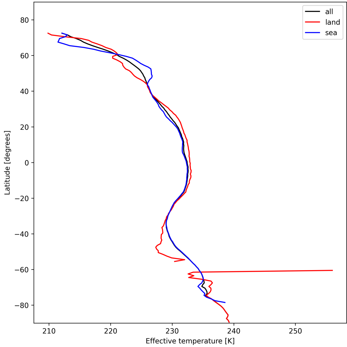
Figure 17: Zonal average of “Effective temperature” for 2025-11-07 to 2025-11-09.
