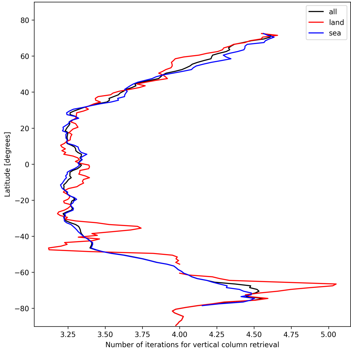
Figure 19: Zonal average of “Number of iterations for vertical column retrieval” for 2025-11-07 to 2025-11-09.
