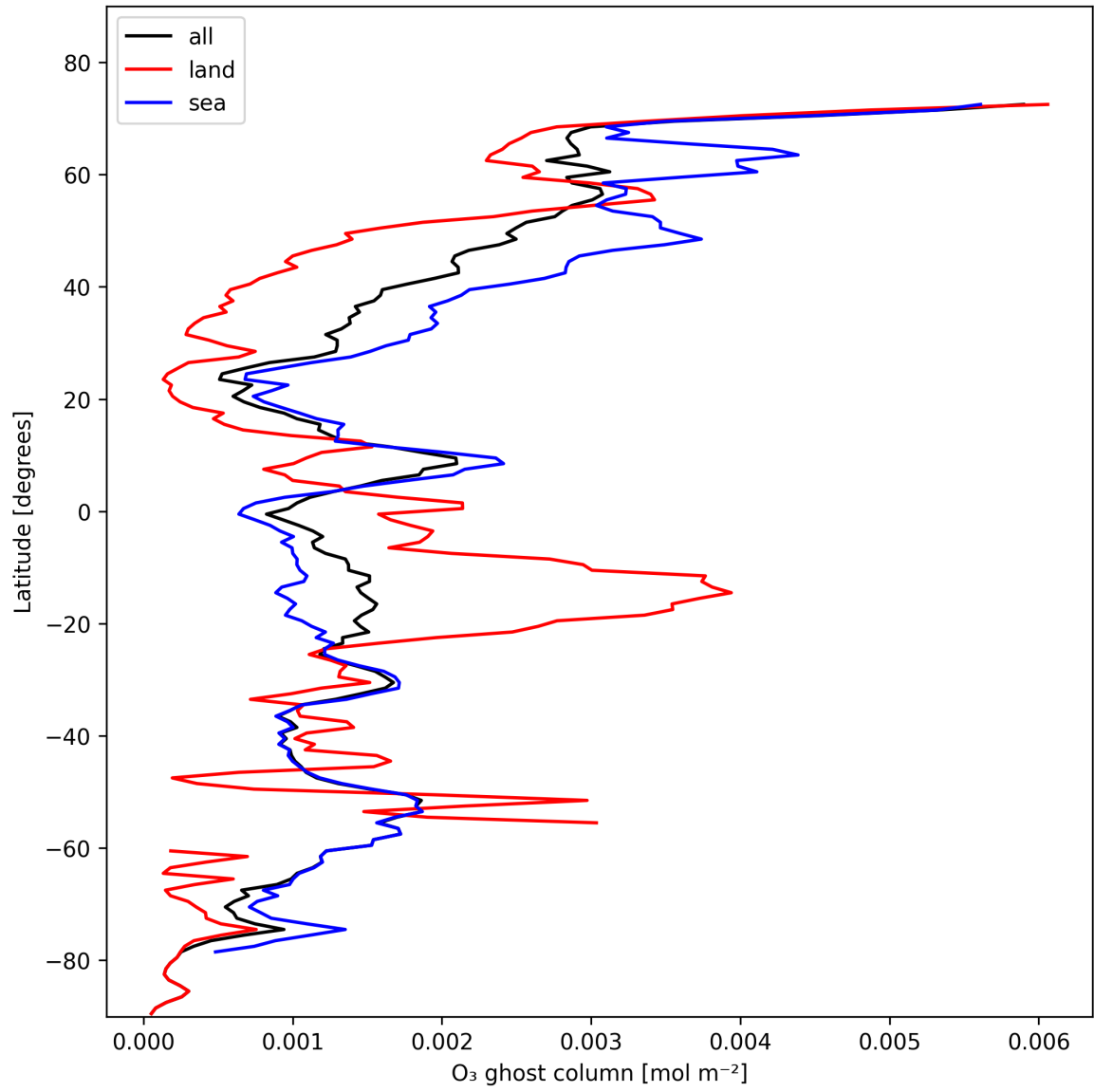
Figure 18: Zonal average of “O 3 ghost column” for 2025-11-07 to 2025-11-09.
