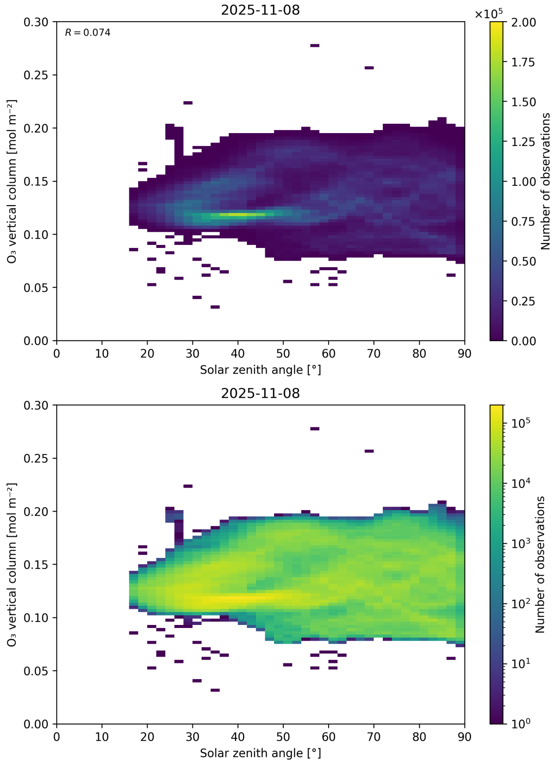
Figure 47: Scatter density plot of “Solar zenith angle” against “O 3 vertical column” for 2025-11-07 to 2025-11-09.
