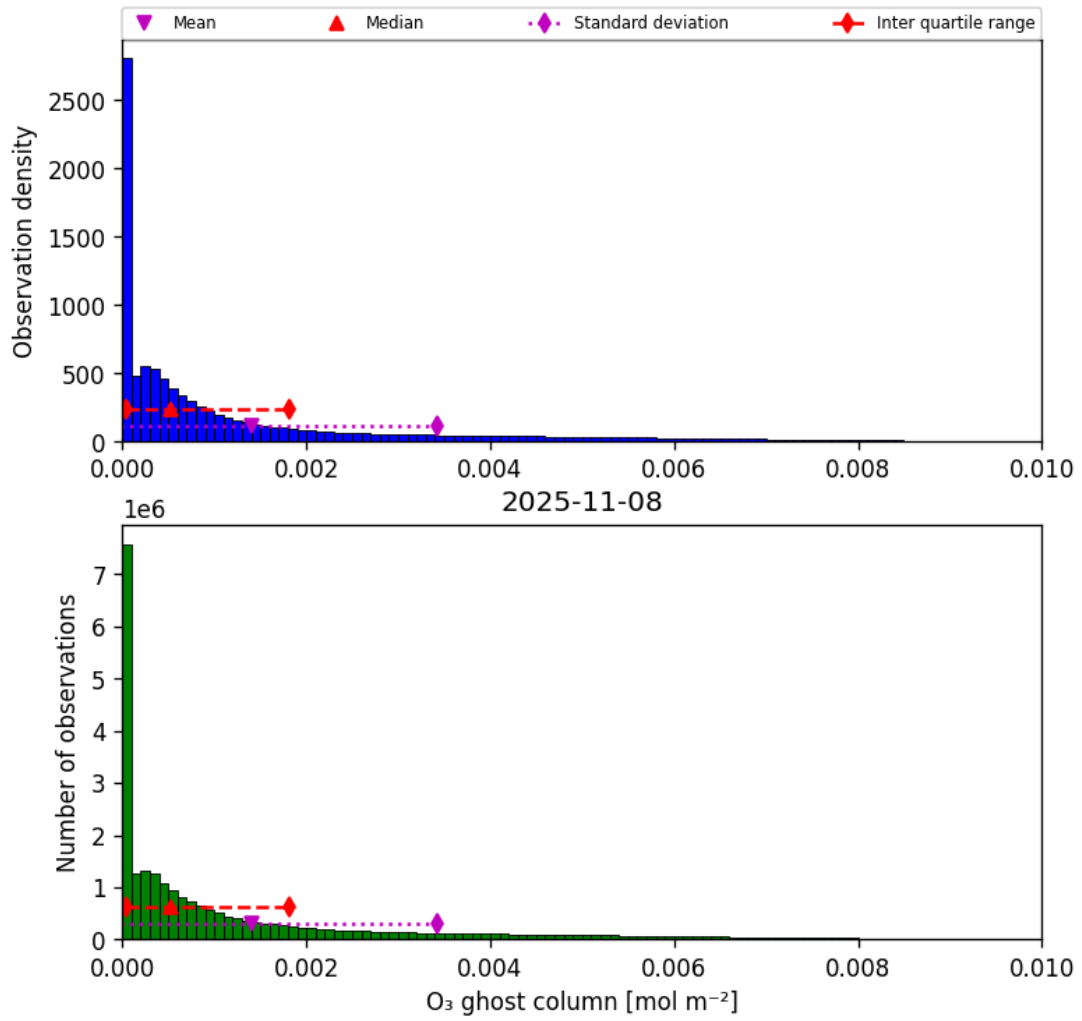
Figure 25: Histogram of “O 3 ghost column” for 2025-11-07 to 2025-11-09
