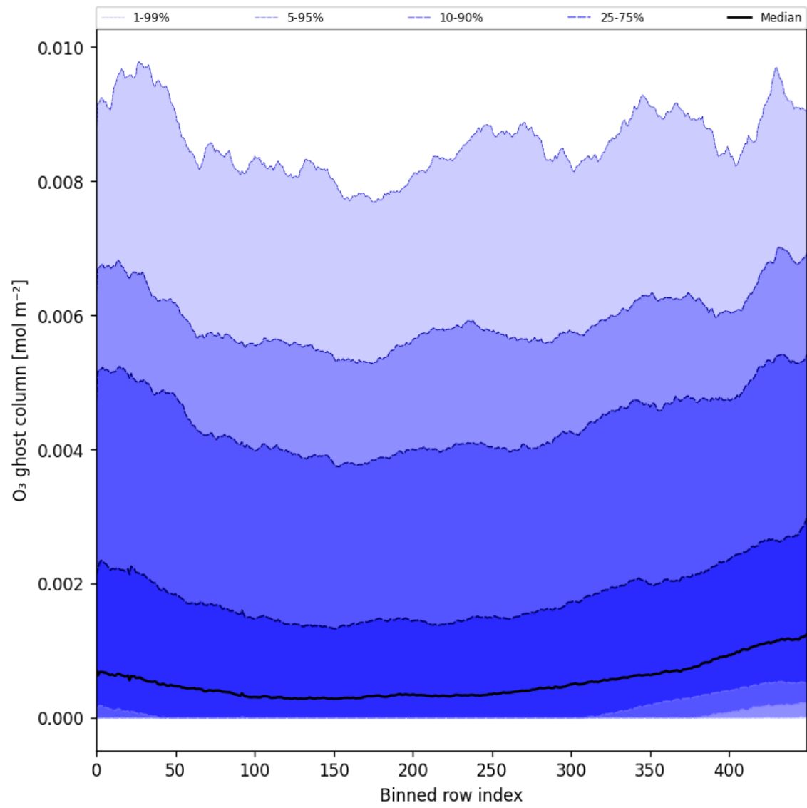
Figure 32: Along track statistics of “O 3 ghost column” for 2025-11-07 to 2025-11-09
