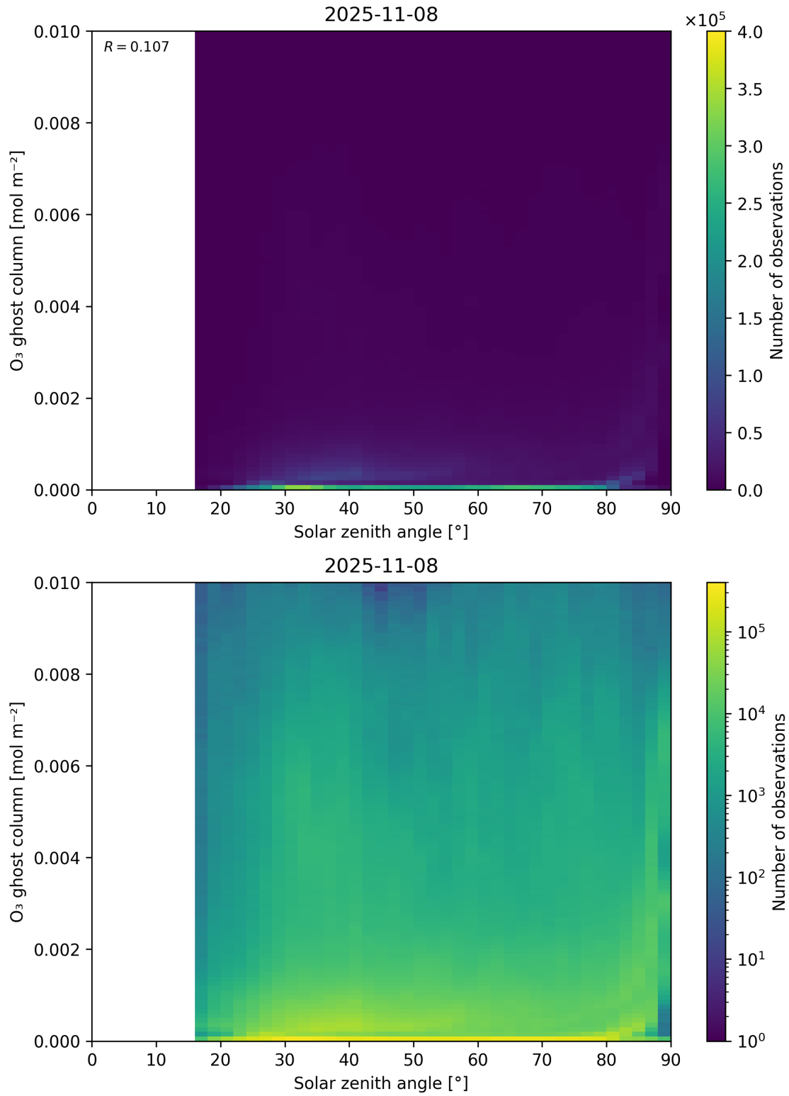
Figure 46: Scatter density plot of “Solar zenith angle” against “O 3 ghost column” for 2025-11-07 to 2025-11-09.
