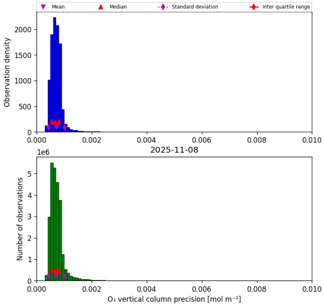
Figure 22: Histogram of “O 3 vertical column precision” for 2025-11-07 to 2025-11-09
