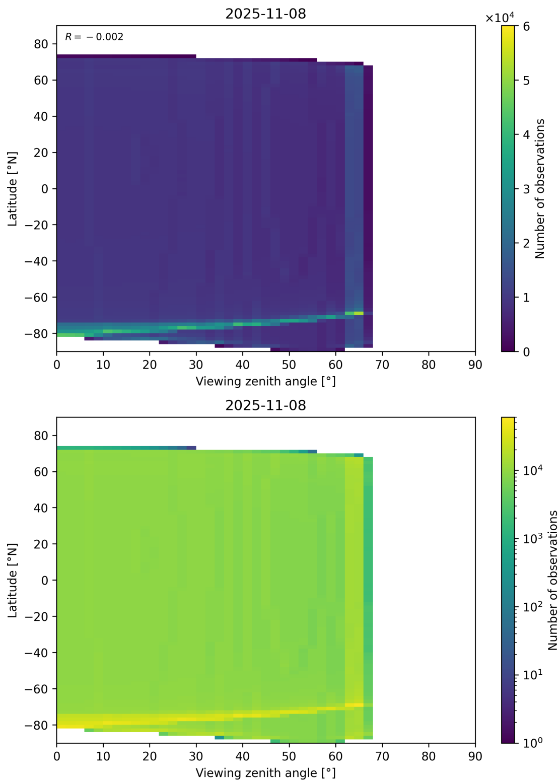
Figure 49: Scatter density plot of “Viewing zenith angle” against “Latitude” for 2025-11-07 to 2025-11-09.
