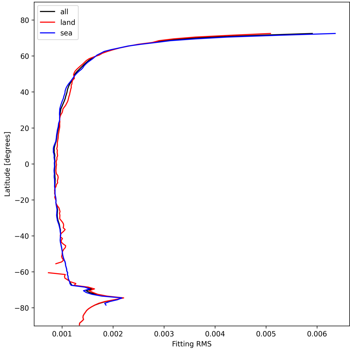
Figure 16: Zonal average of “Fitting RMS” for 2025-11-07 to 2025-11-09.
