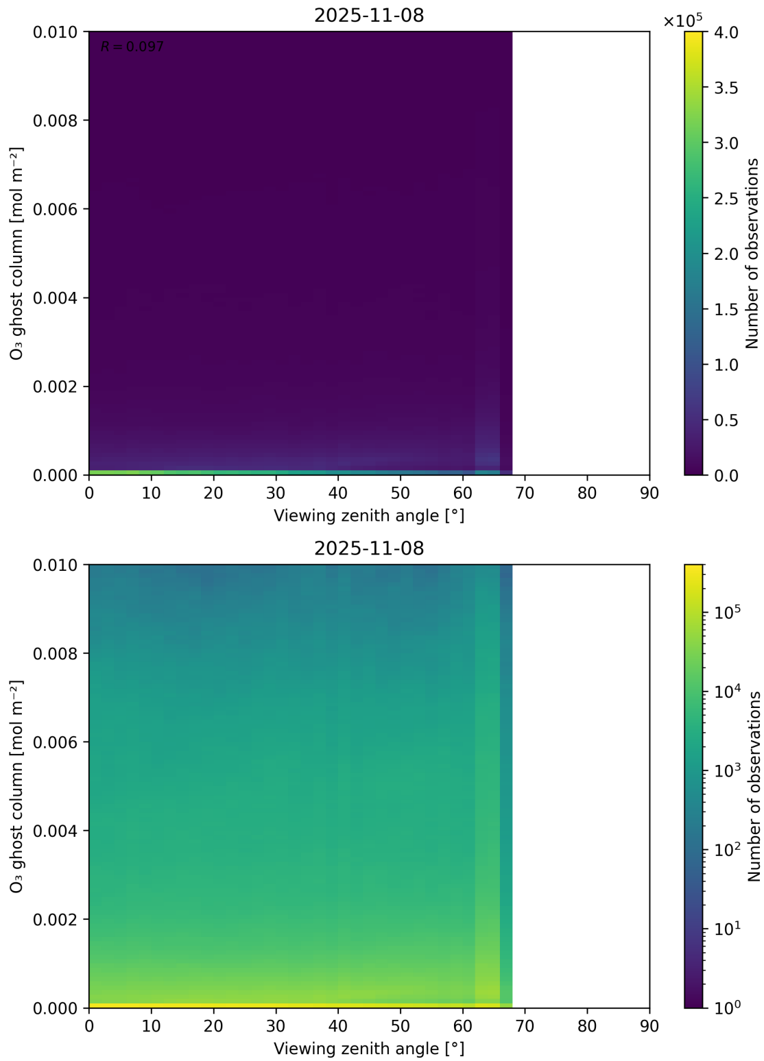
Figure 51: Scatter density plot of “Viewing zenith angle” against “O 3 ghost column” for 2025-11-07 to 2025-11-09.
