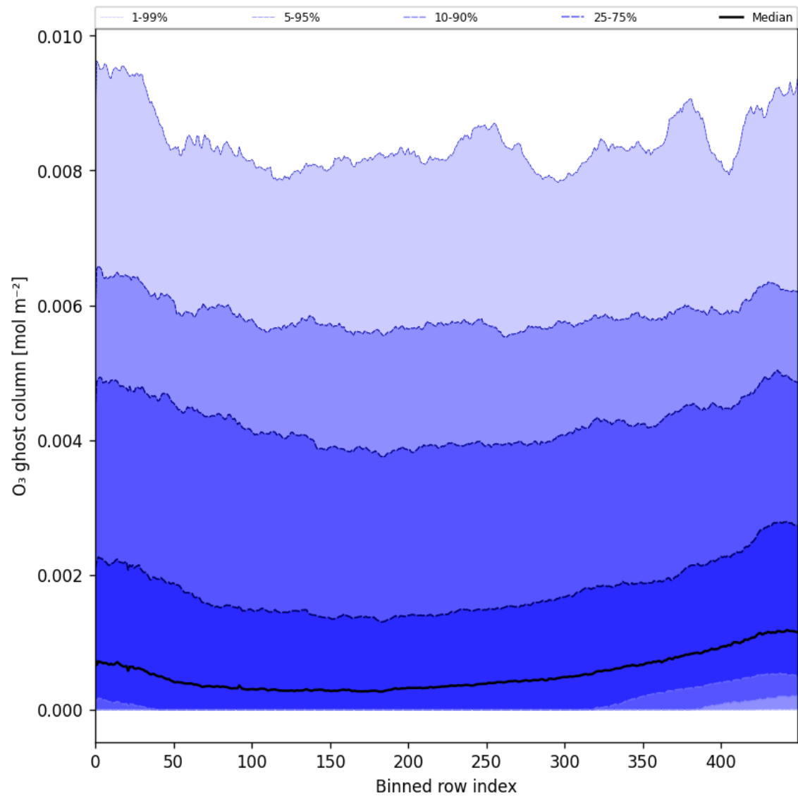
Figure 32: Along track statistics of “O 3 ghost column” for 2025-11-08 to 2025-11-10
