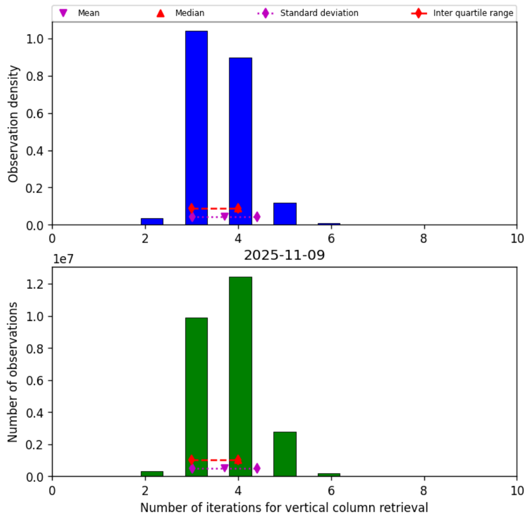
Figure 26: Histogram of “Number of iterations for vertical column retrieval” for 2025-11-08 to 2025-11-10
