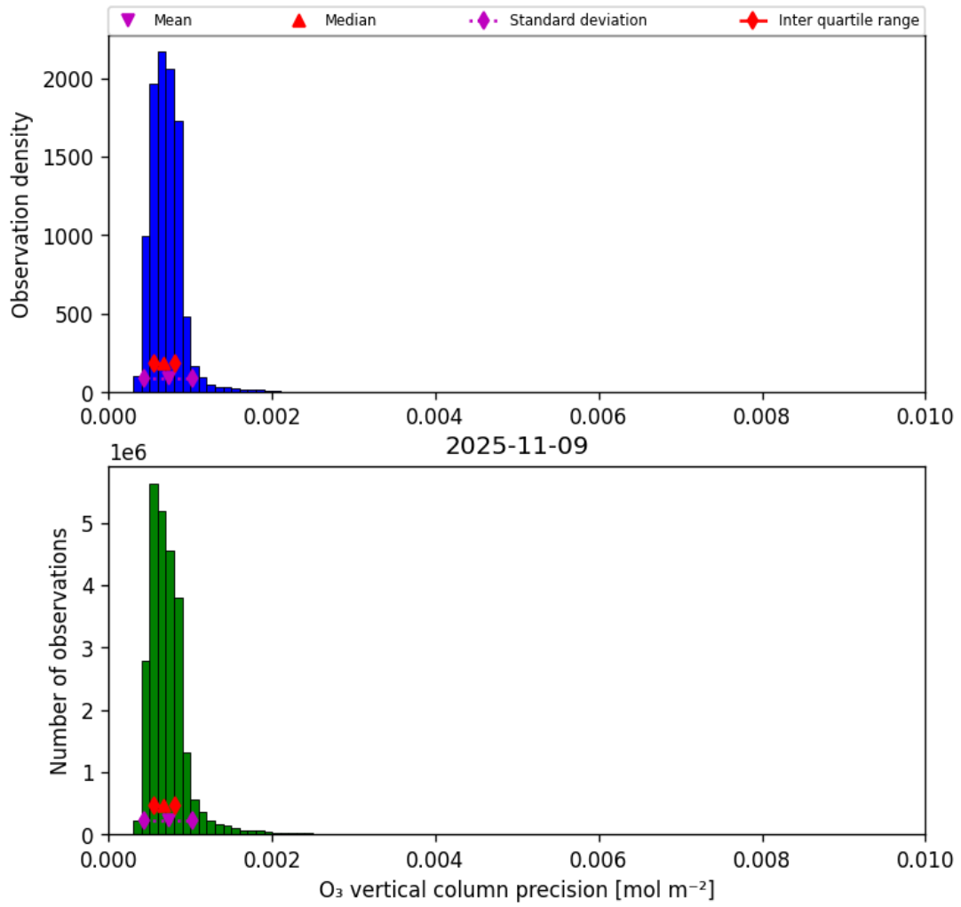
Figure 22: Histogram of “O 3 vertical column precision” for 2025-11-08 to 2025-11-10
