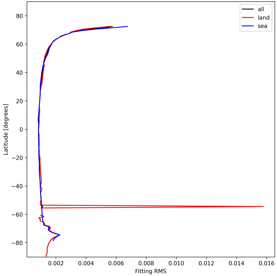
Figure 16: Zonal average of “Fitting RMS” for 2025-11-08 to 2025-11-10.
