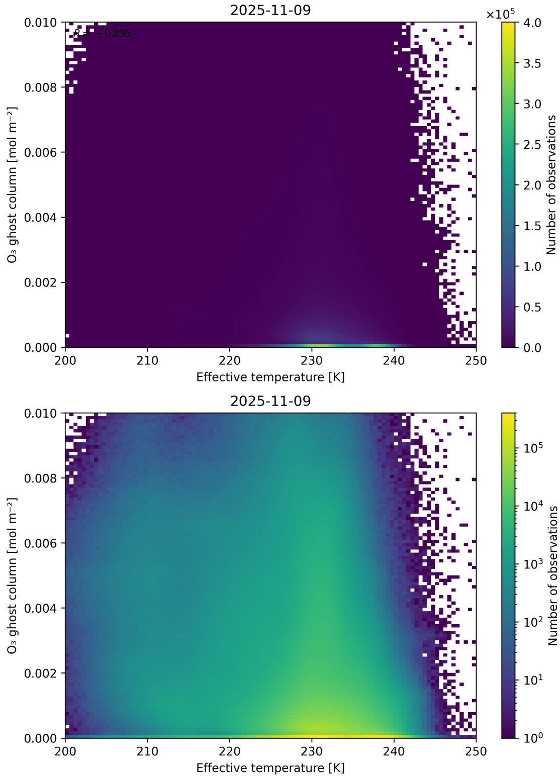
Figure 38: Scatter density plot of “Effective temperature” against “O 3 ghost column” for 2025-11-08 to 2025-11-10.
