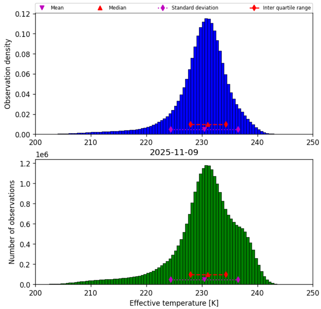
Figure 24: Histogram of “Effective temperature” for 2025-11-08 to 2025-11-10
