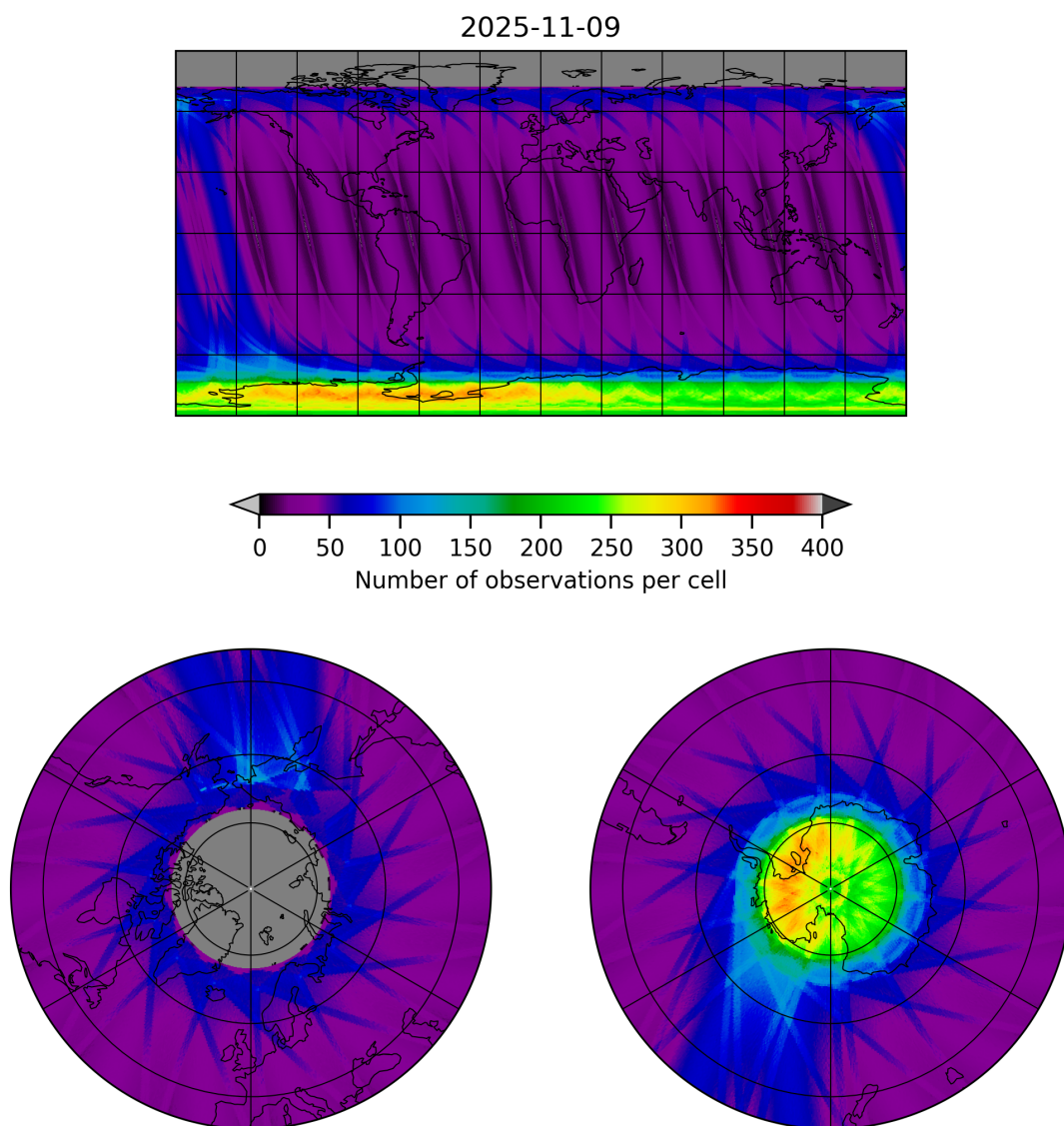
Figure 12: Map of the number of observations for 2025-11-08 to 2025-11-10
