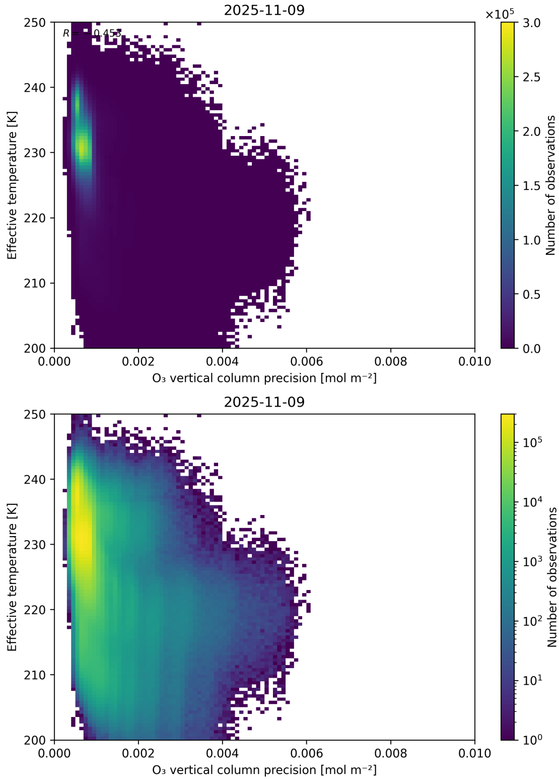
Figure 42: Scatter density plot of “ O_3 vertical column precision” against “Effective temperature” for 2025-11-08 to 2025-11-10.
