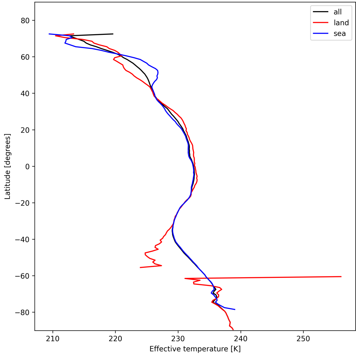
Figure 17: Zonal average of “Effective temperature” for 2025-11-08 to 2025-11-10.
