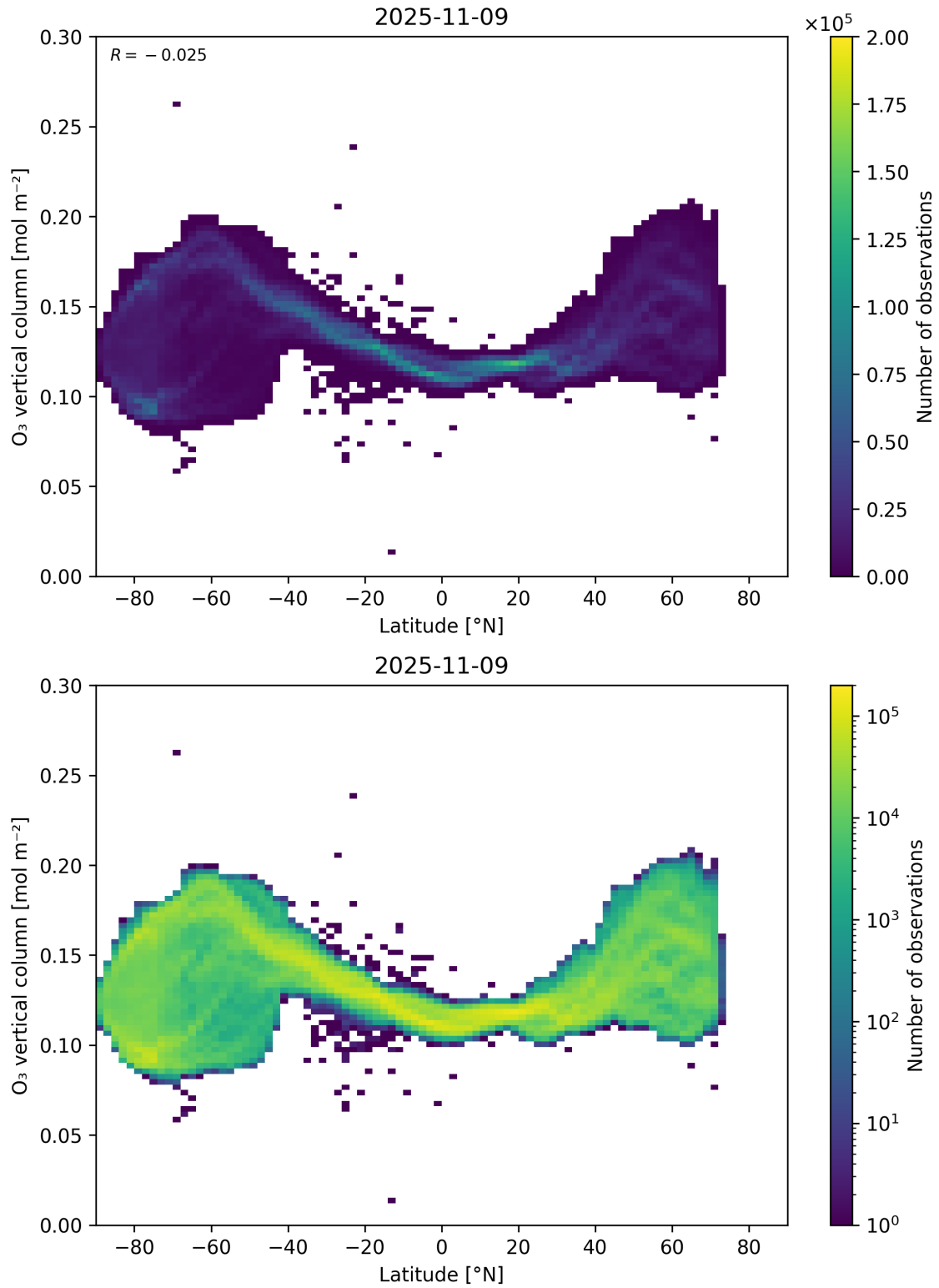
Figure 36: Scatter density plot of “Latitude” against “O 3 vertical column” for 2025-11-08 to 2025-11-10.
