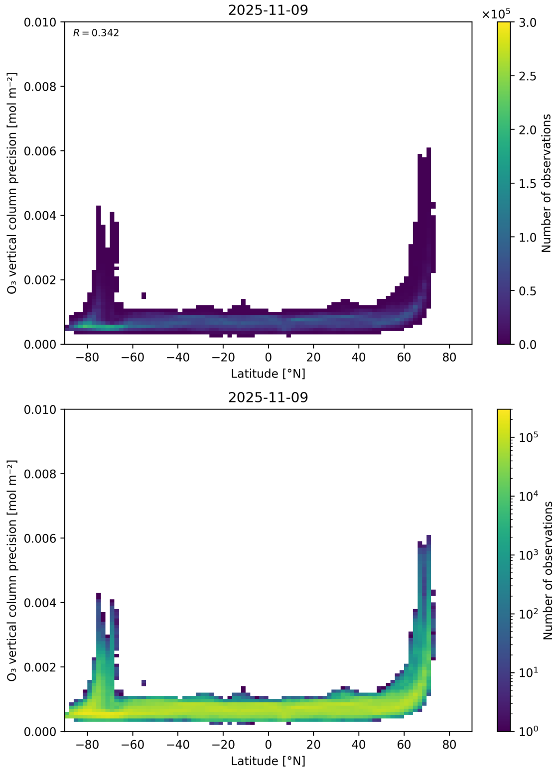
Figure 37: Scatter density plot of “Latitude” against “O 3 vertical column precision” for 2025-11-08 to 2025-11-10.
