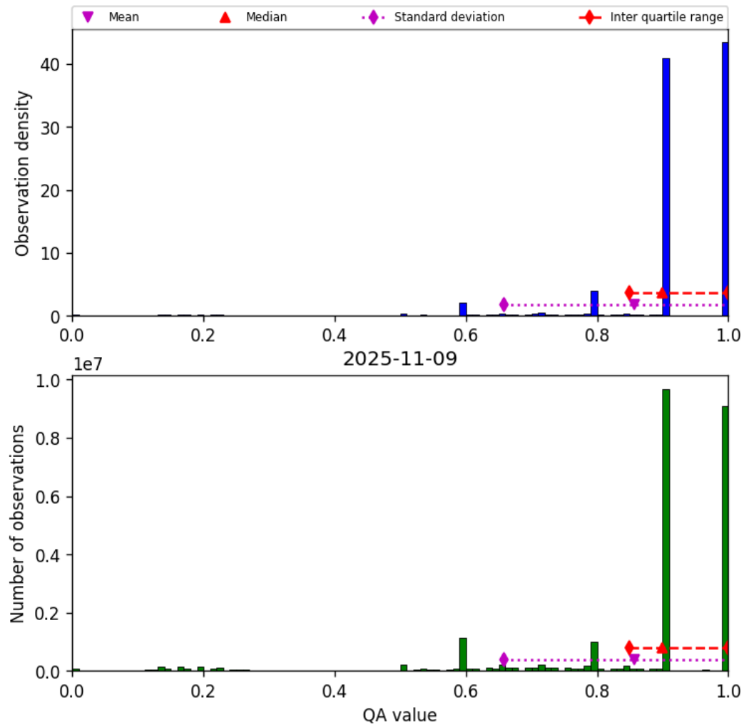
Figure 20: Histogram of “QA value” for 2025-11-08 to 2025-11-10
