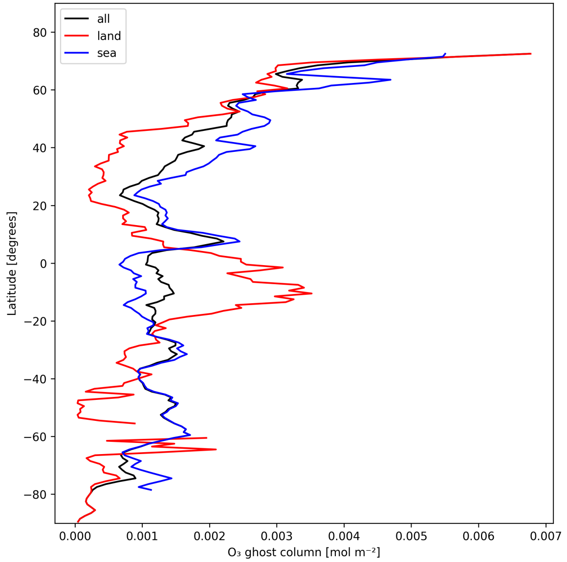
Figure 18: Zonal average of “O 3 ghost column” for 2025-11-08 to 2025-11-10.
