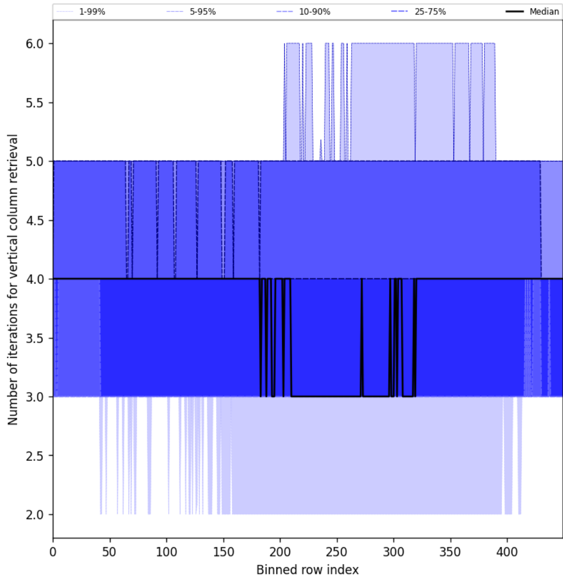
Figure 33: Along track statistics of “Number of iterations for vertical column retrieval” for 2025-11-08 to 2025-11-10
