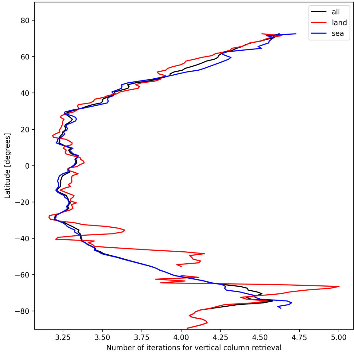
Figure 19: Zonal average of “Number of iterations for vertical column retrieval” for 2025-11-08 to 2025-11-10.
