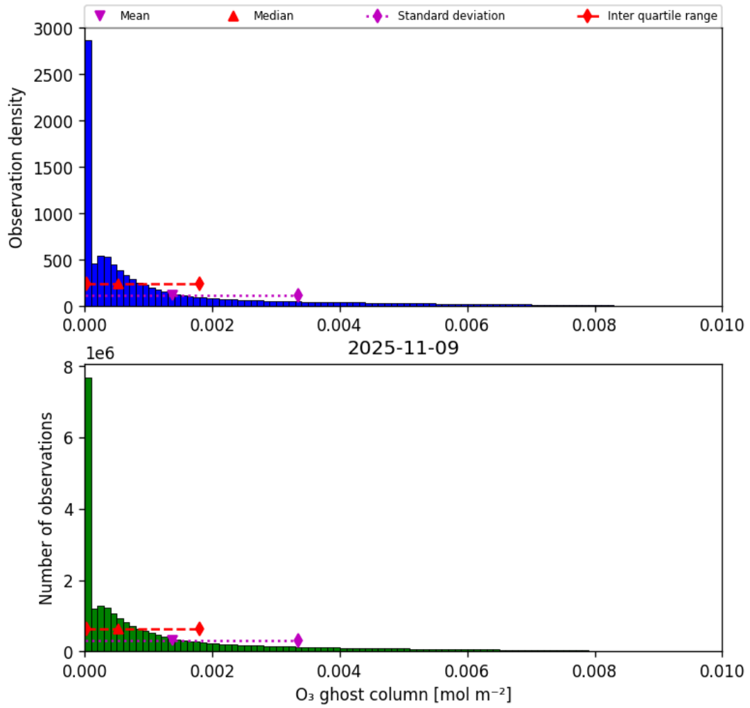
Figure 25: Histogram of “O 3 ghost column” for 2025-11-08 to 2025-11-10
