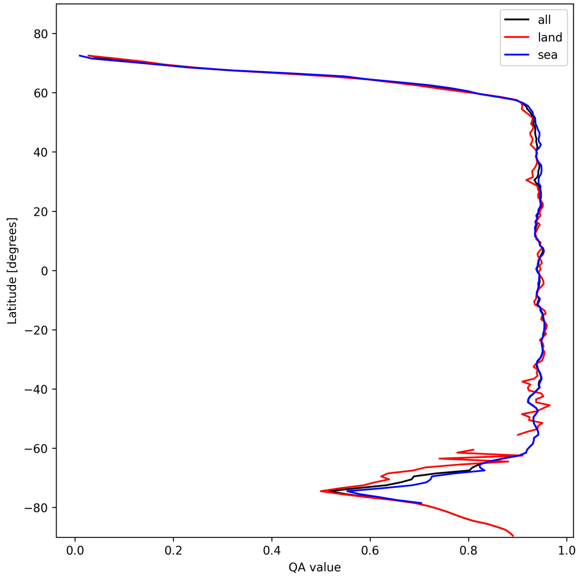
Figure 13: Zonal average of “QA value” for 2025-11-08 to 2025-11-10.
