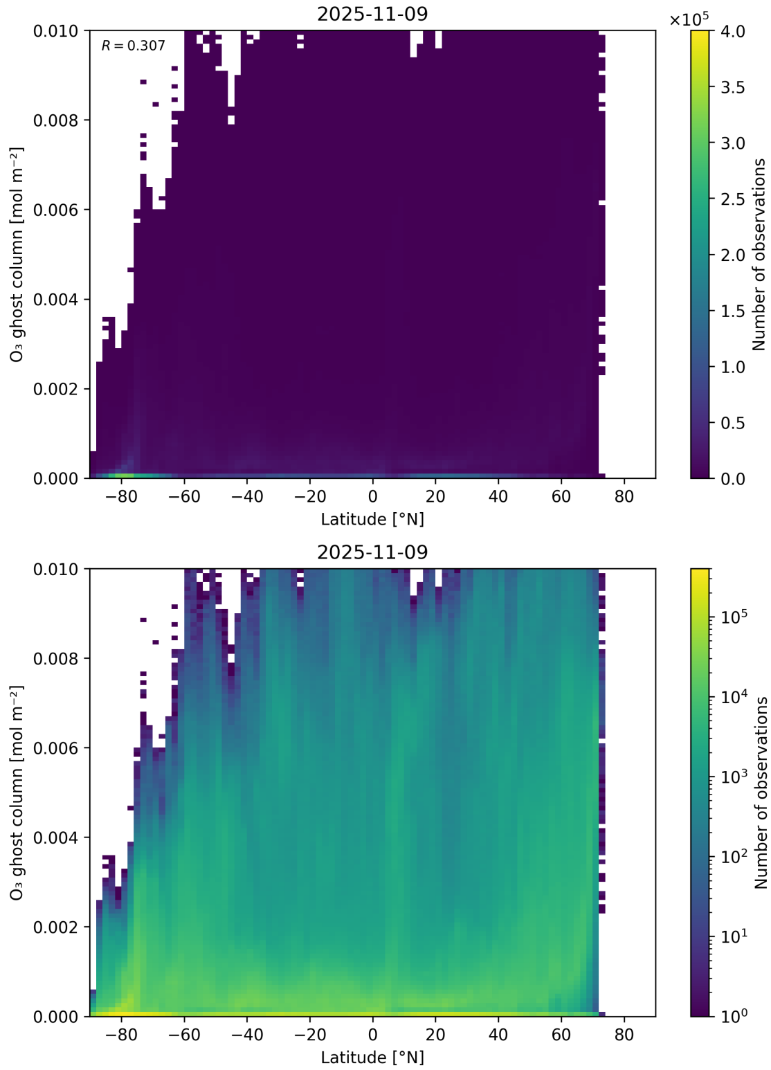
Figure 35: Scatter density plot of “Latitude” against “O 3 ghost column” for 2025-11-08 to 2025-11-10.
