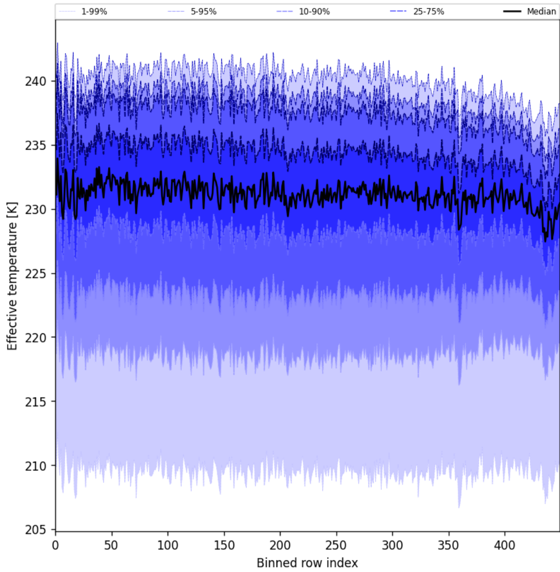
Figure 31: Along track statistics of “Effective temperature” for 2025-11-08 to 2025-11-10
