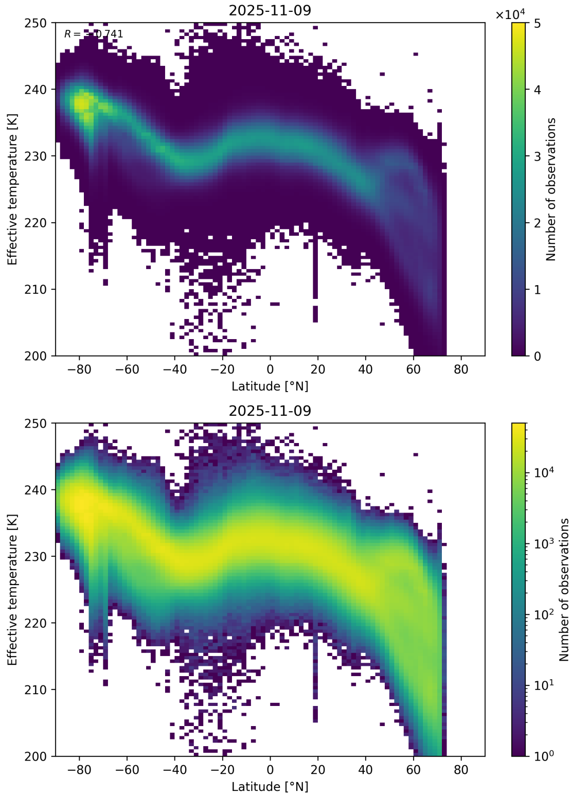
Figure 34: Scatter density plot of “Latitude” against “Effective temperature” for 2025-11-08 to 2025-11-10.
