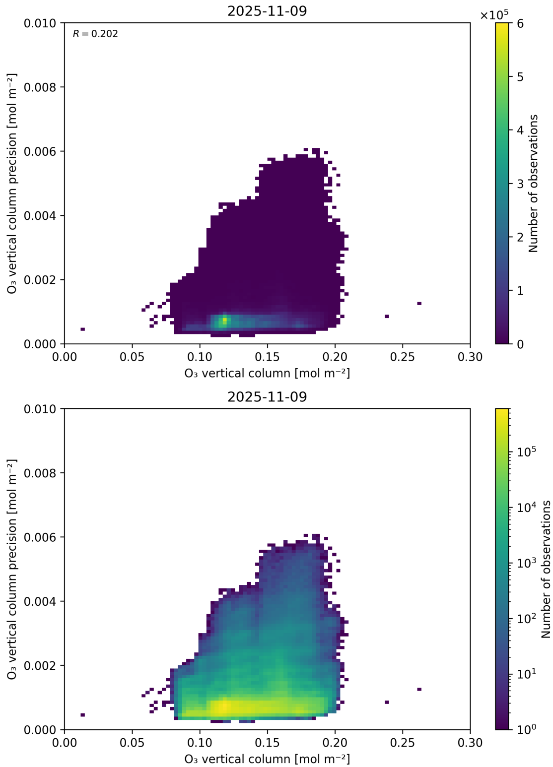
Figure 41: Scatter density plot of “O 3 vertical column” against “O 3 vertical column precision” for 2025-11-08 to 2025-11-10.
