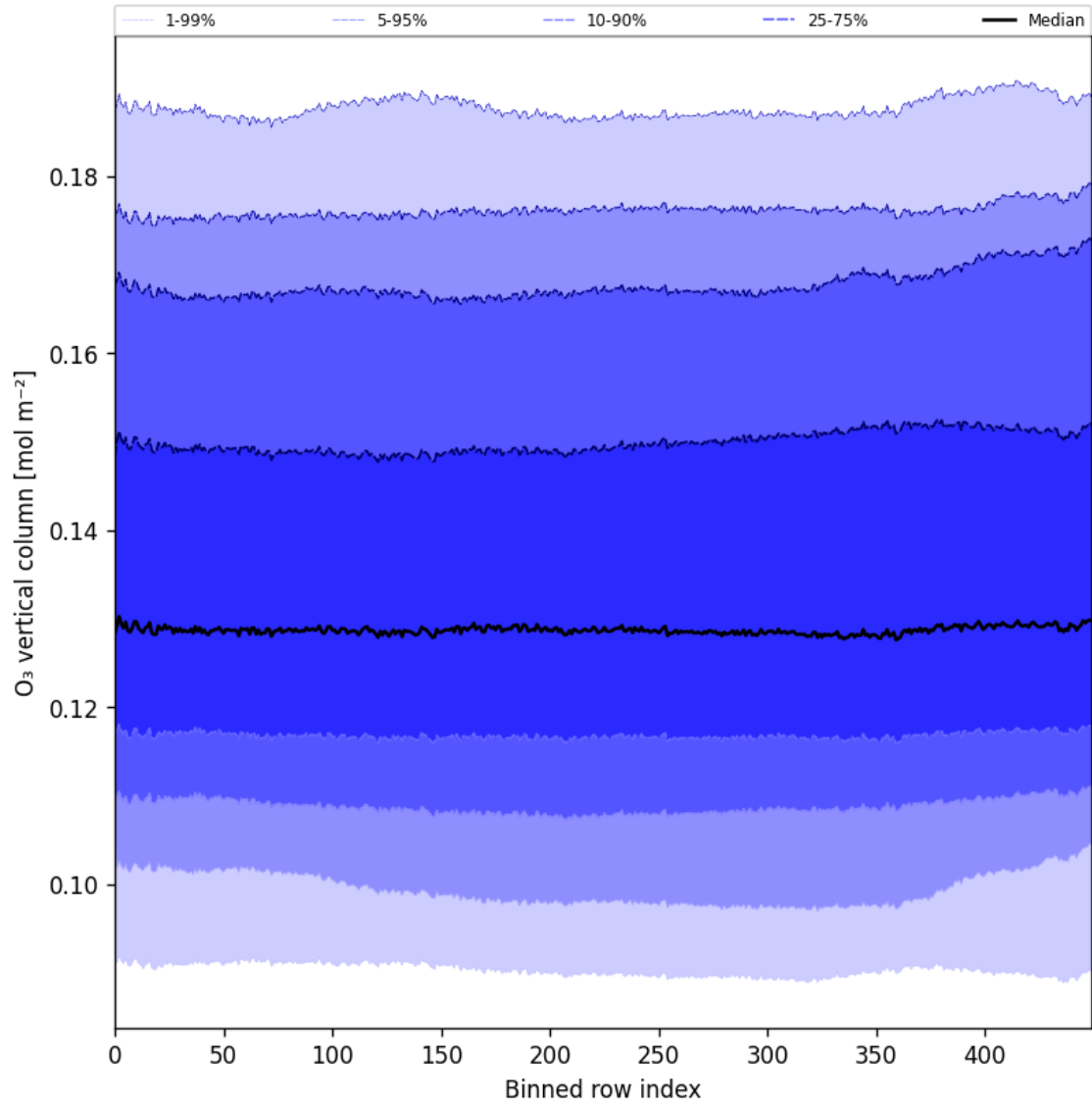
Figure 28: Along track statistics of “O 3 vertical column” for 2025-11-08 to 2025-11-10
