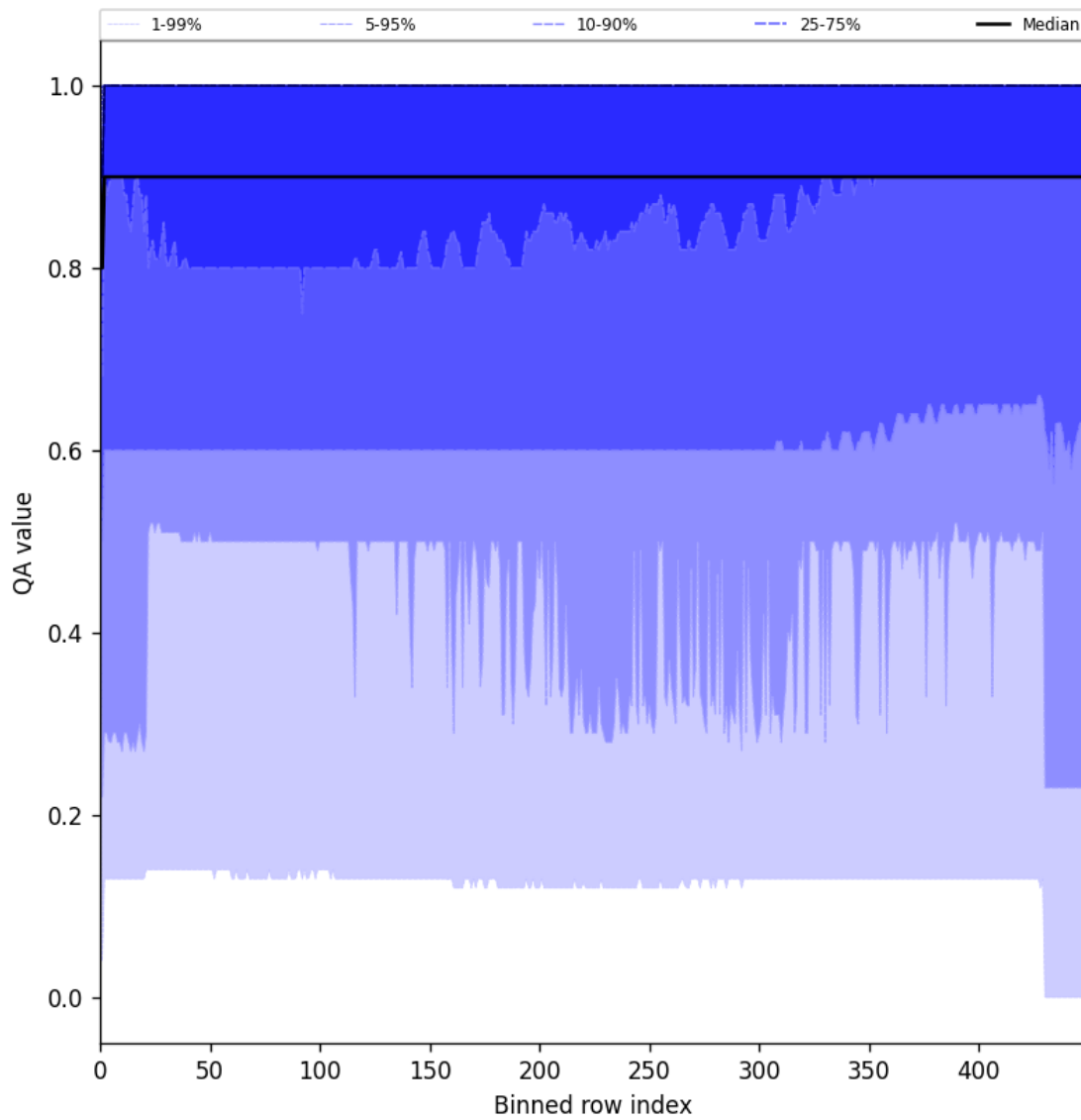
Figure 27: Along track statistics of “QA value” for 2025-11-08 to 2025-11-10
