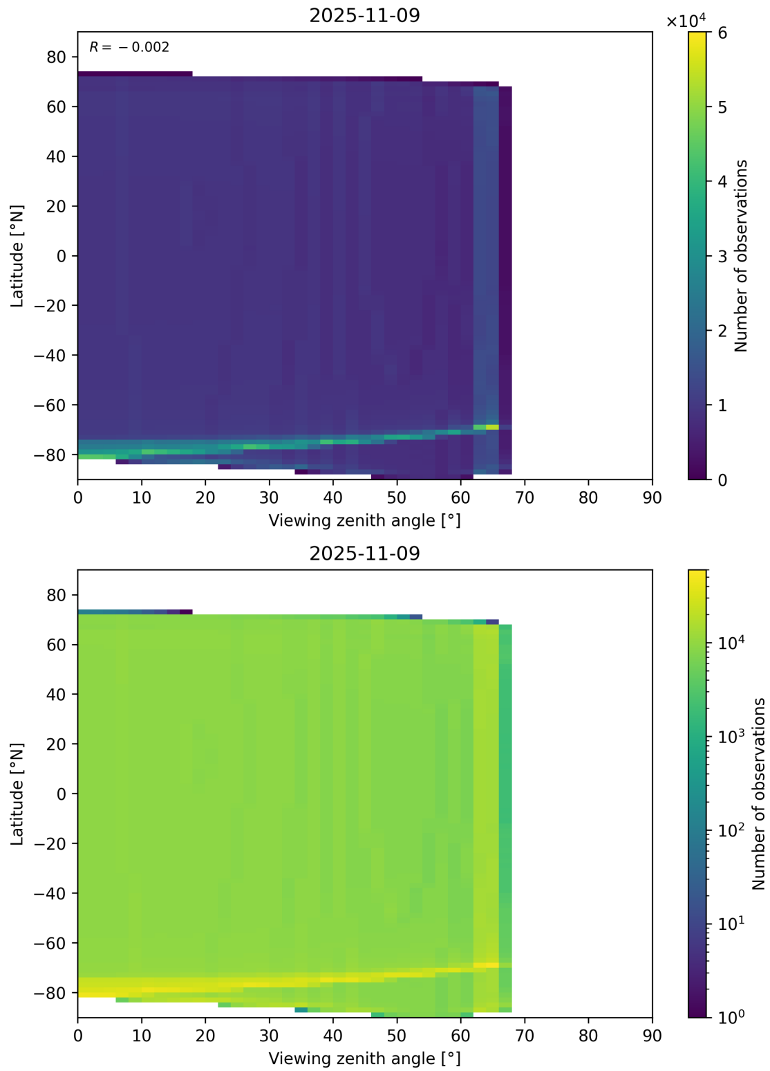
Figure 49: Scatter density plot of “Viewing zenith angle” against “Latitude” for 2025-11-08 to 2025-11-10.
