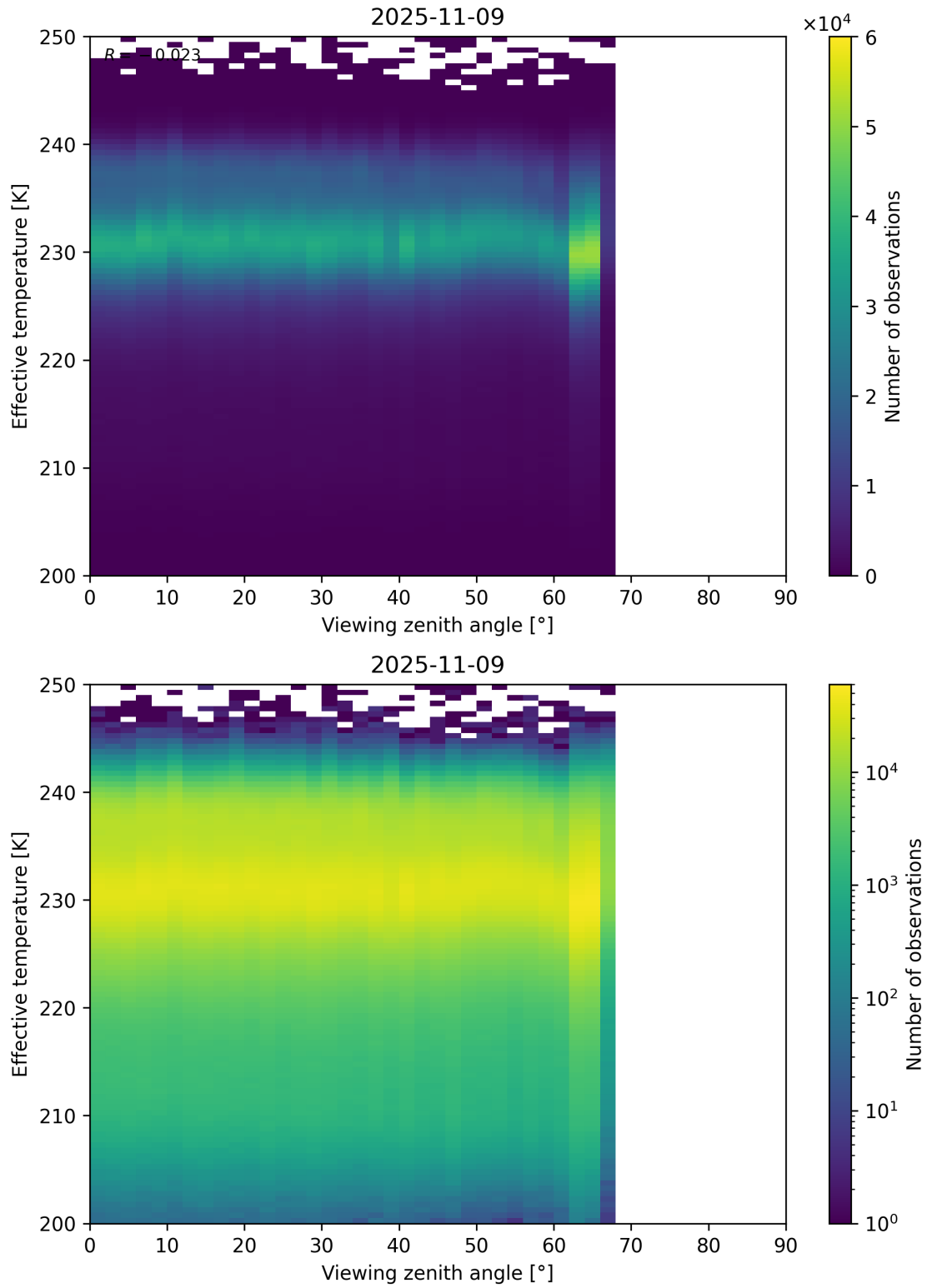
Figure 50: Scatter density plot of “Viewing zenith angle” against “Effective temperature” for 2025-11-08 to 2025-11-10.
