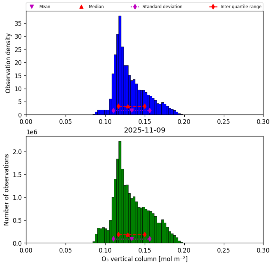
Figure 21: Histogram of “O 3 vertical column” for 2025-11-08 to 2025-11-10
