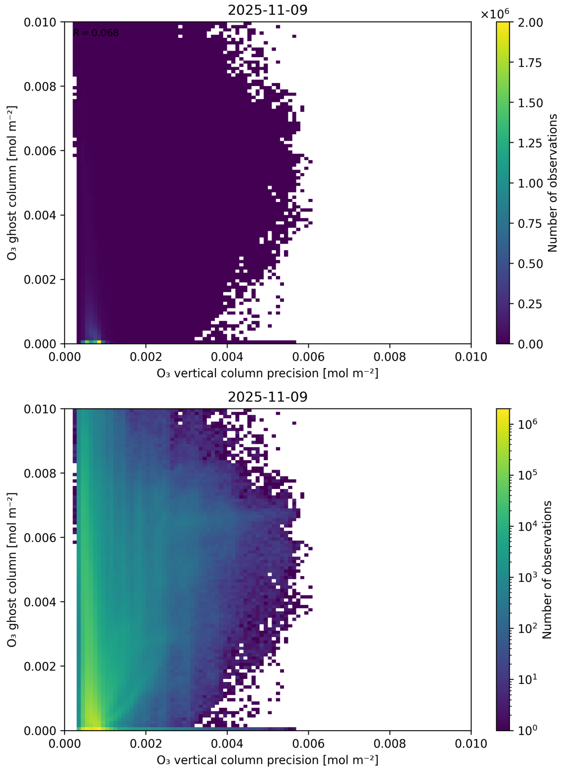
Figure 43: Scatter density plot of “O 3 vertical column precision” against “O 3 ghost column” for 2025-11-08 to 2025-11-10.
