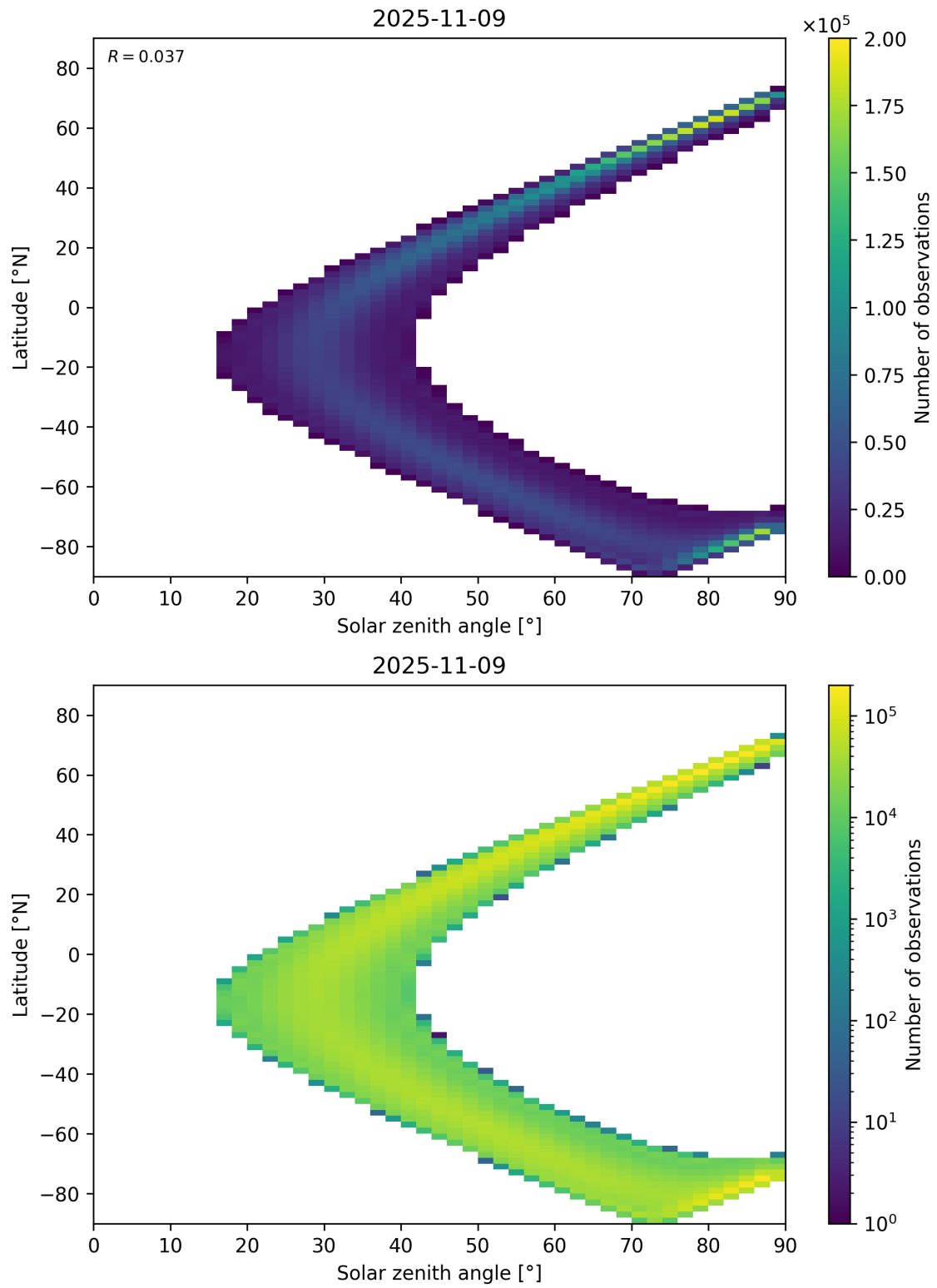
Figure 44: Scatter density plot of “Solar zenith angle” against “Latitude” for 2025-11-08 to 2025-11-10.
