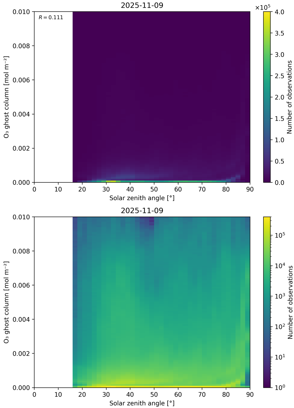
Figure 46: Scatter density plot of “Solar zenith angle” against “O 3 ghost column” for 2025-11-08 to 2025-11-10.
