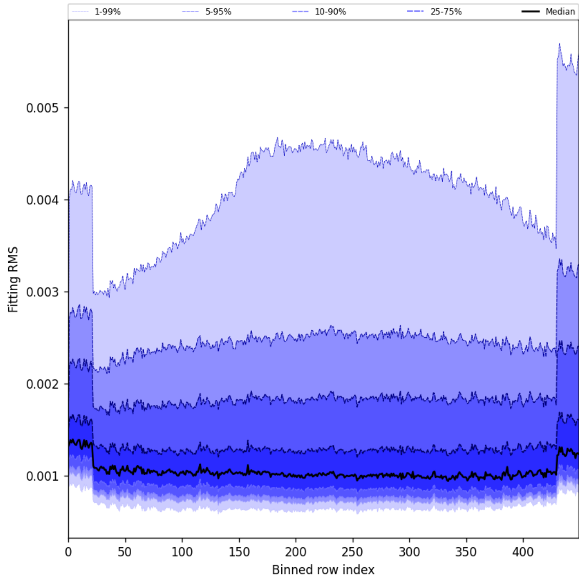
Figure 30: Along track statistics of “Fitting RMS” for 2025-11-08 to 2025-11-10
