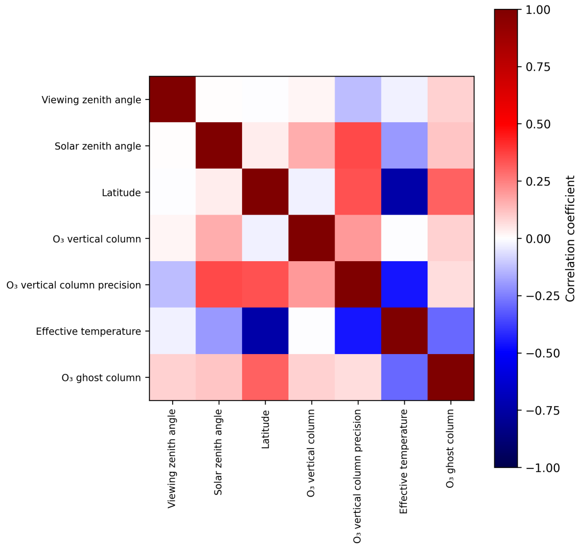
Figure 2: Map of correlation matrix for 2025-11-08 to 2025-11-10.
