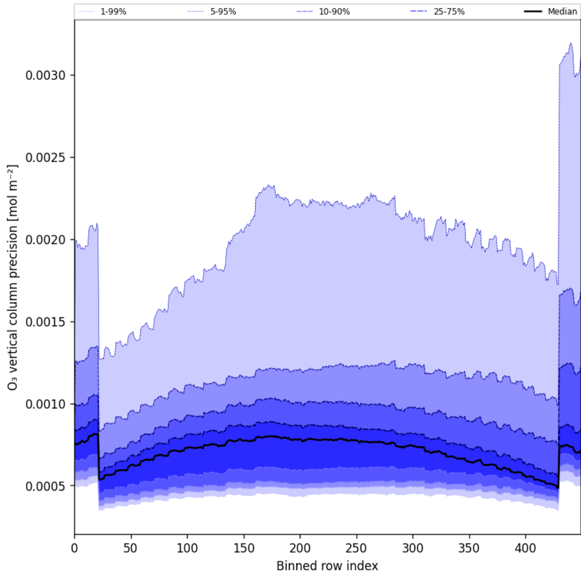
Figure 29: Along track statistics of “O 3 vertical column precision” for 2025-11-08 to 2025-11-10
