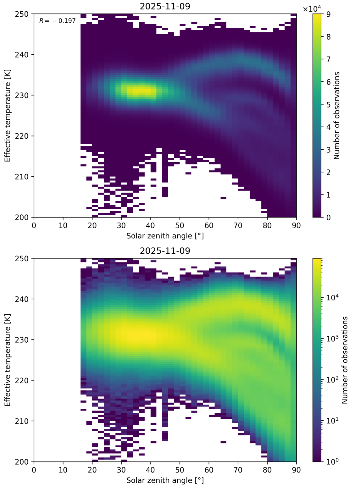
Figure 45: Scatter density plot of “Solar zenith angle” against “Effective temperature” for 2025-11-08 to 2025-11-10.
