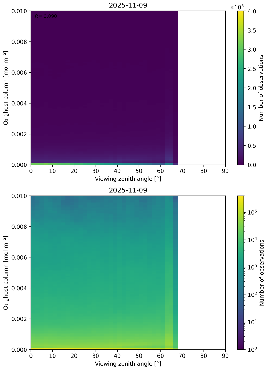
Figure 51: Scatter density plot of “Viewing zenith angle” against “O 3 ghost column” for 2025-11-08 to 2025-11-10.
