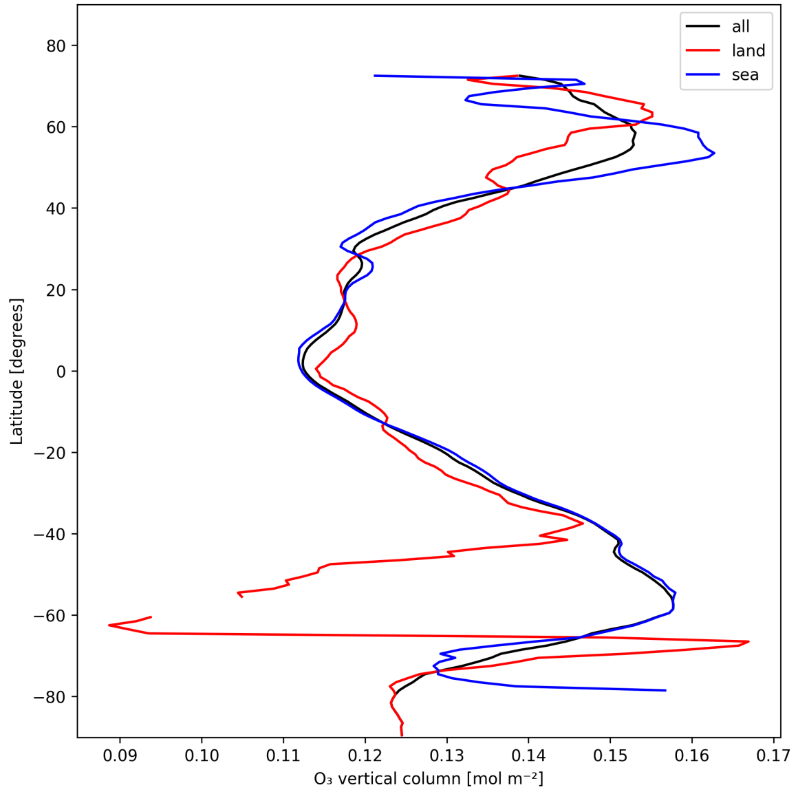
Figure 14: Zonal average of “O 3 vertical column” for 2025-11-08 to 2025-11-10.
