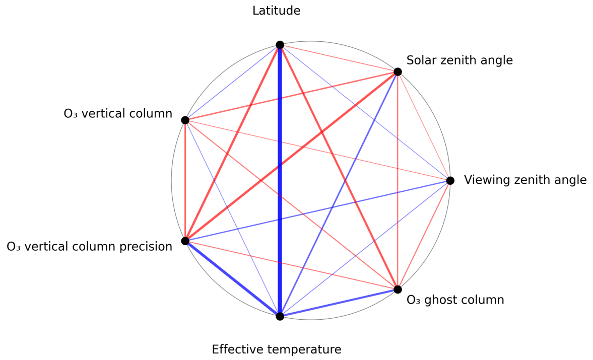
Figure 1: Map of correlation graph for 2025-11-08 to 2025-11-10.
