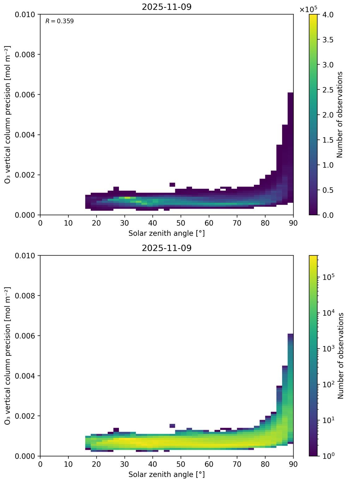
Figure 48: Scatter density plot of “Solar zenith angle” against “O 3 vertical column precision” for 2025-11-08 to 2025-11-10.
