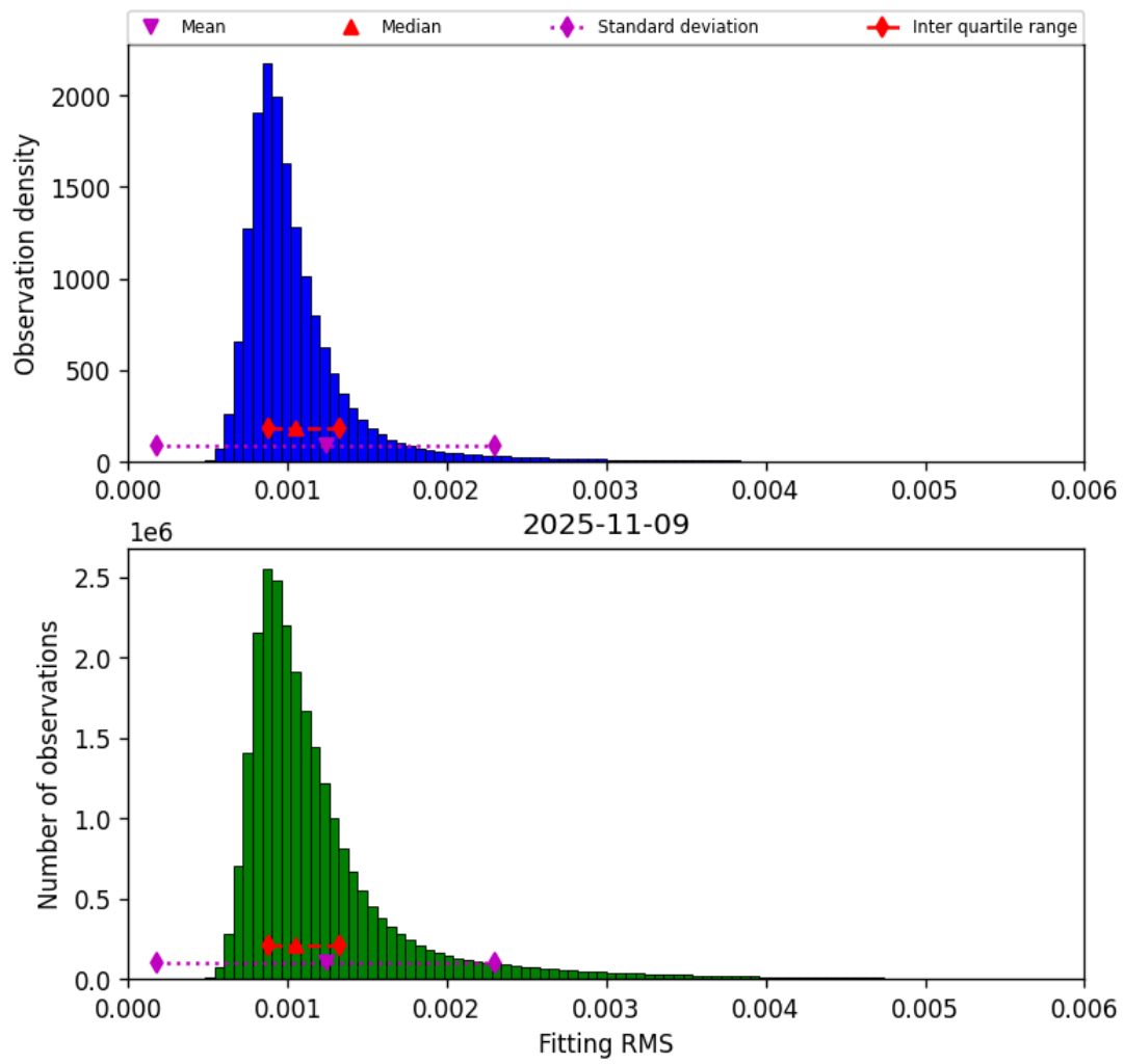
Figure 23: Histogram of “Fitting RMS” for 2025-11-08 to 2025-11-10
