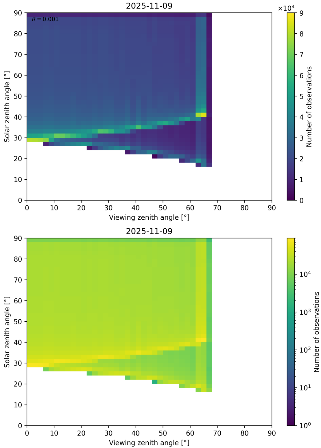
Figure 54: Scatter density plot of “Viewing zenith angle” against “Solar zenith angle” for 2025-11-08 to 2025-11-10.
