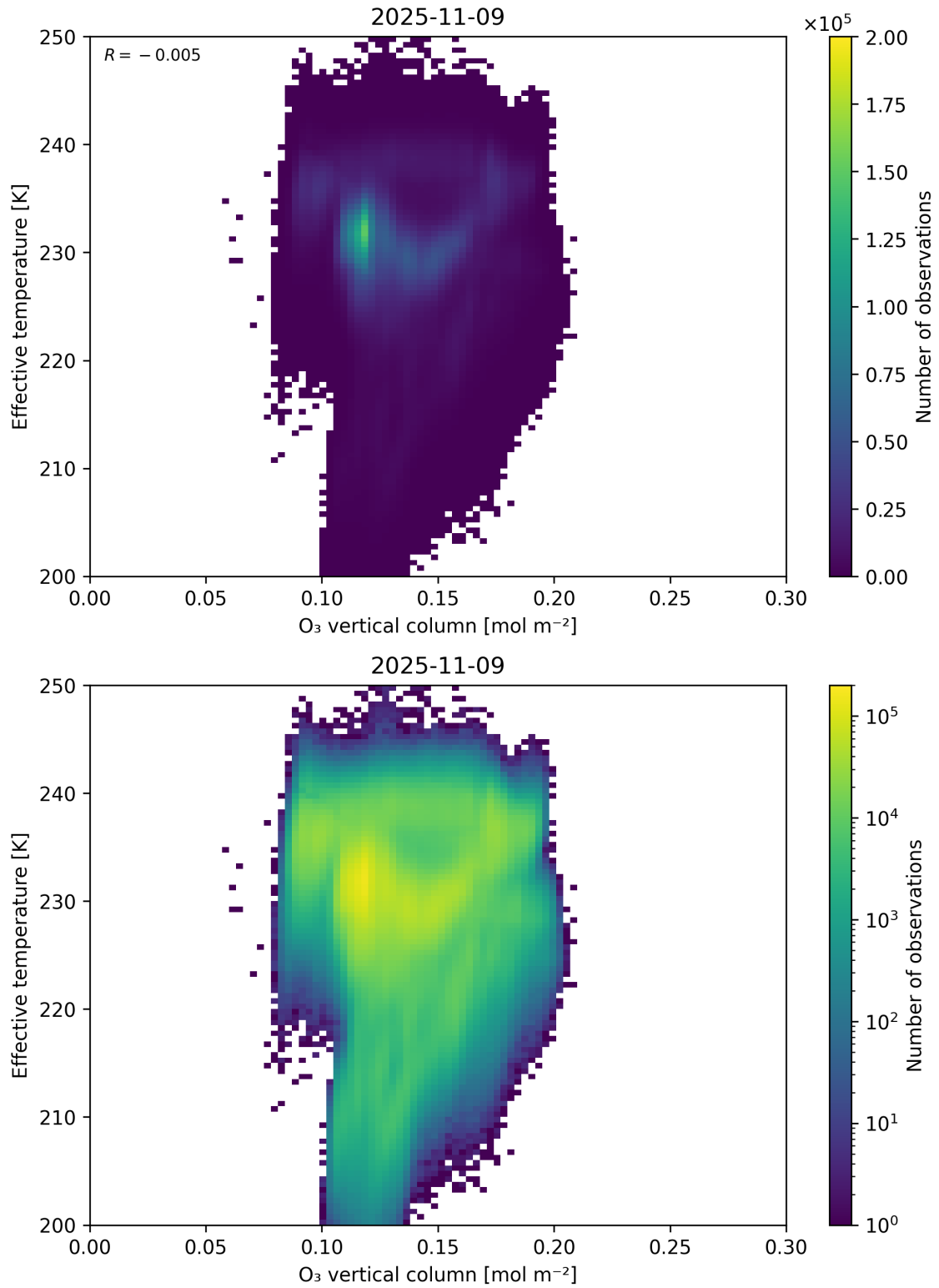
Figure 39: Scatter density plot of “O 3 vertical column” against “Effective temperature” for 2025-11-08 to 2025-11-10.
