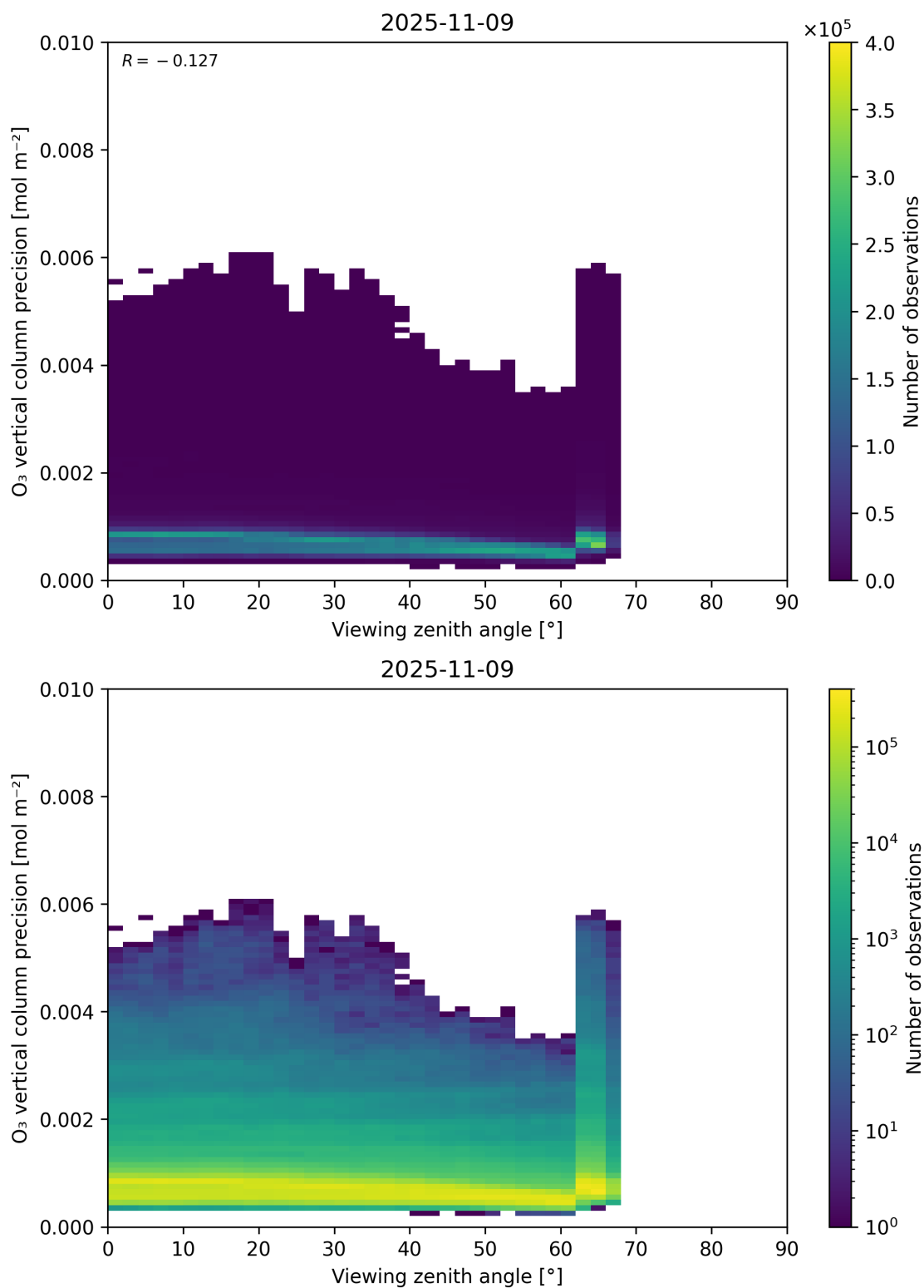
Figure 53: Scatter density plot of “Viewing zenith angle” against “O 3 vertical column precision” for 2025-11-08 to 2025-11-10.
