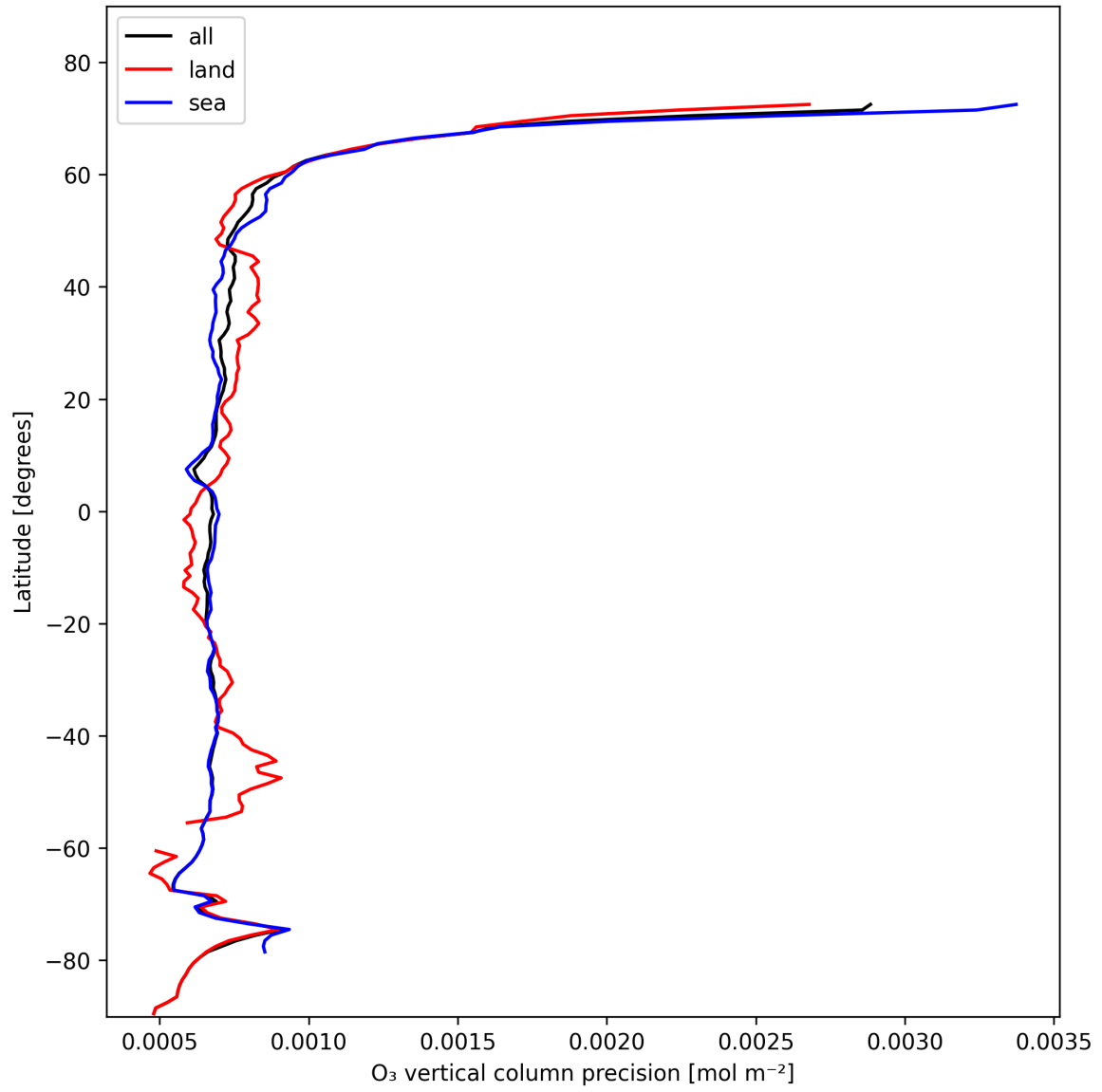
Figure 15: Zonal average of “O 3 vertical column precision” for 2025-11-08 to 2025-11-10.
