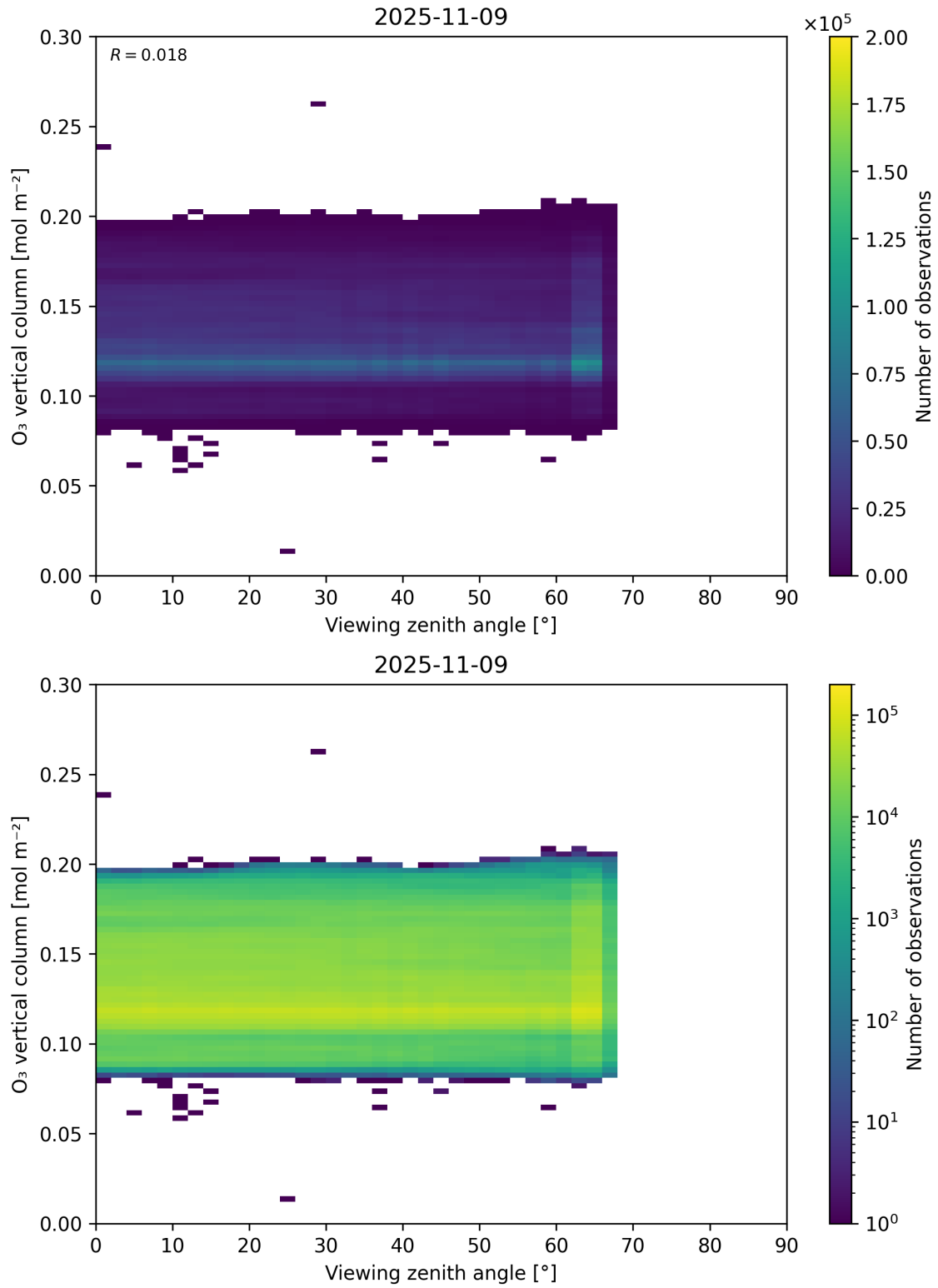
Figure 52: Scatter density plot of “Viewing zenith angle” against “O 3 vertical column” for 2025-11-08 to 2025-11-10.
