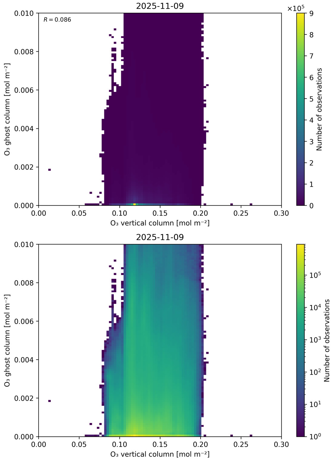
Figure 40: Scatter density plot of “O 3 vertical column” against “O 3 ghost column” for 2025-11-08 to 2025-11-10.
