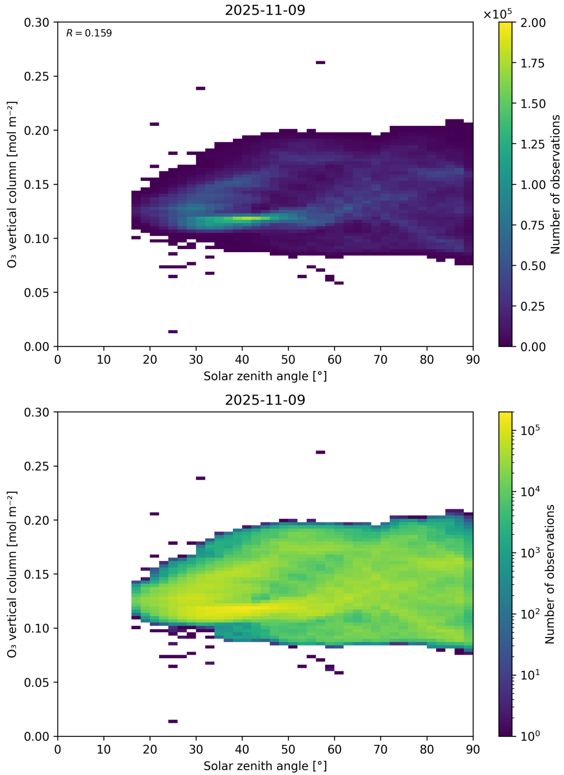
Figure 47: Scatter density plot of “Solar zenith angle” against “O 3 vertical column” for 2025-11-08 to 2025-11-10.
