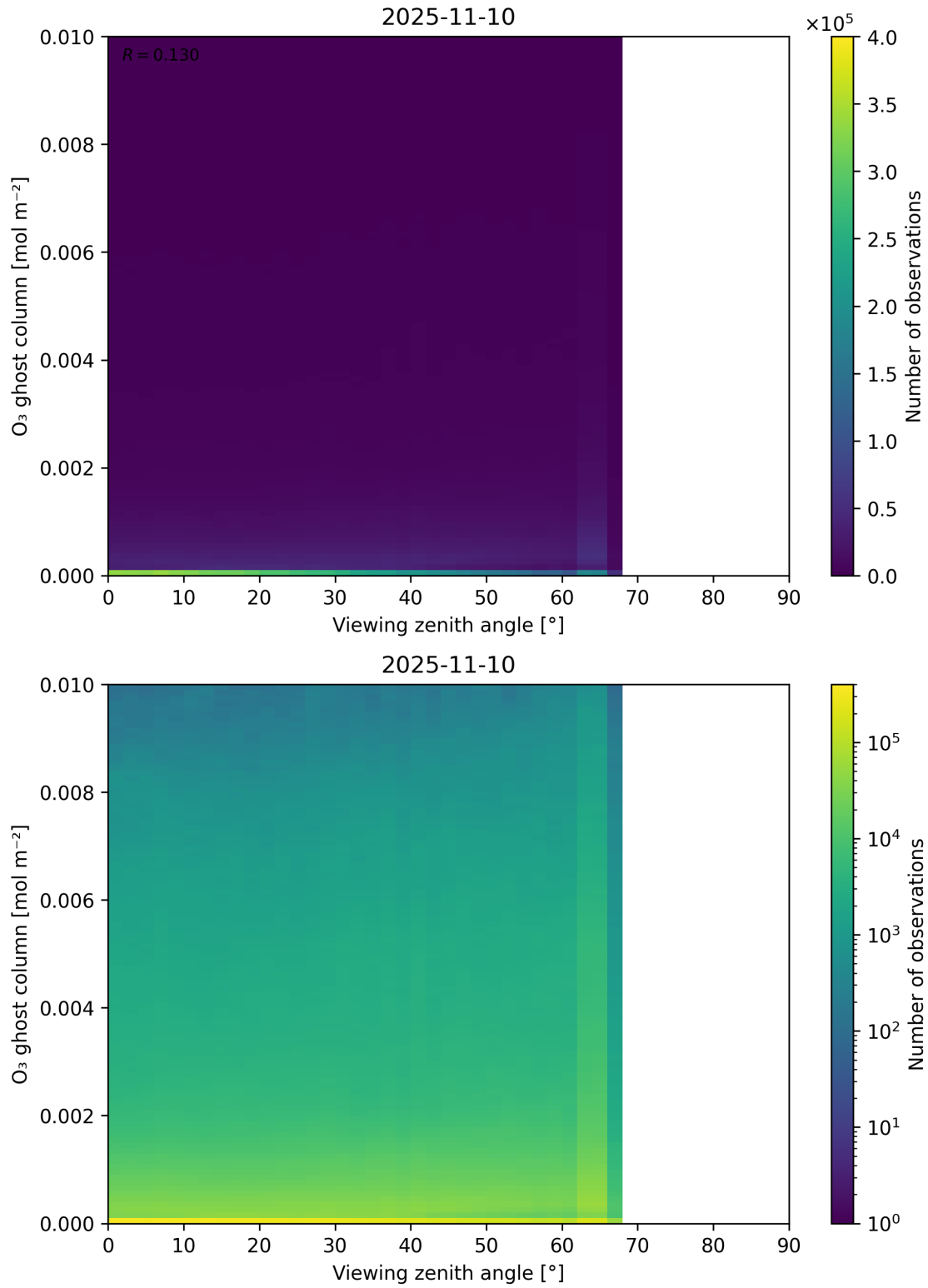
Figure 51: Scatter density plot of “Viewing zenith angle” against “O 3 ghost column” for 2025-11-09 to 2025-11-11.
