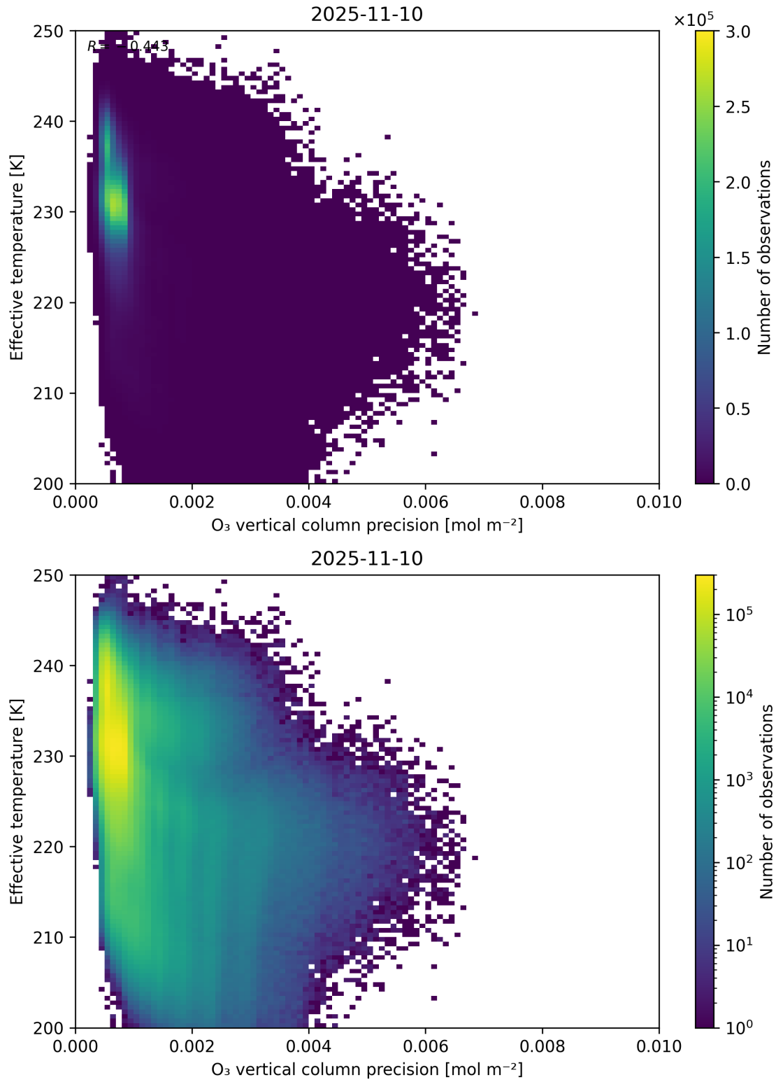
Figure 42: Scatter density plot of “O 3 vertical column precision” against “Effective temperature” for 2025-11-09 to 2025-11-11.
