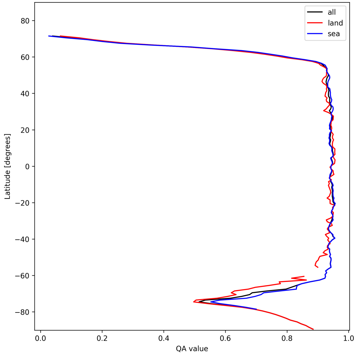
Figure 13: Zonal average of “QA value” for 2025-11-09 to 2025-11-11.
