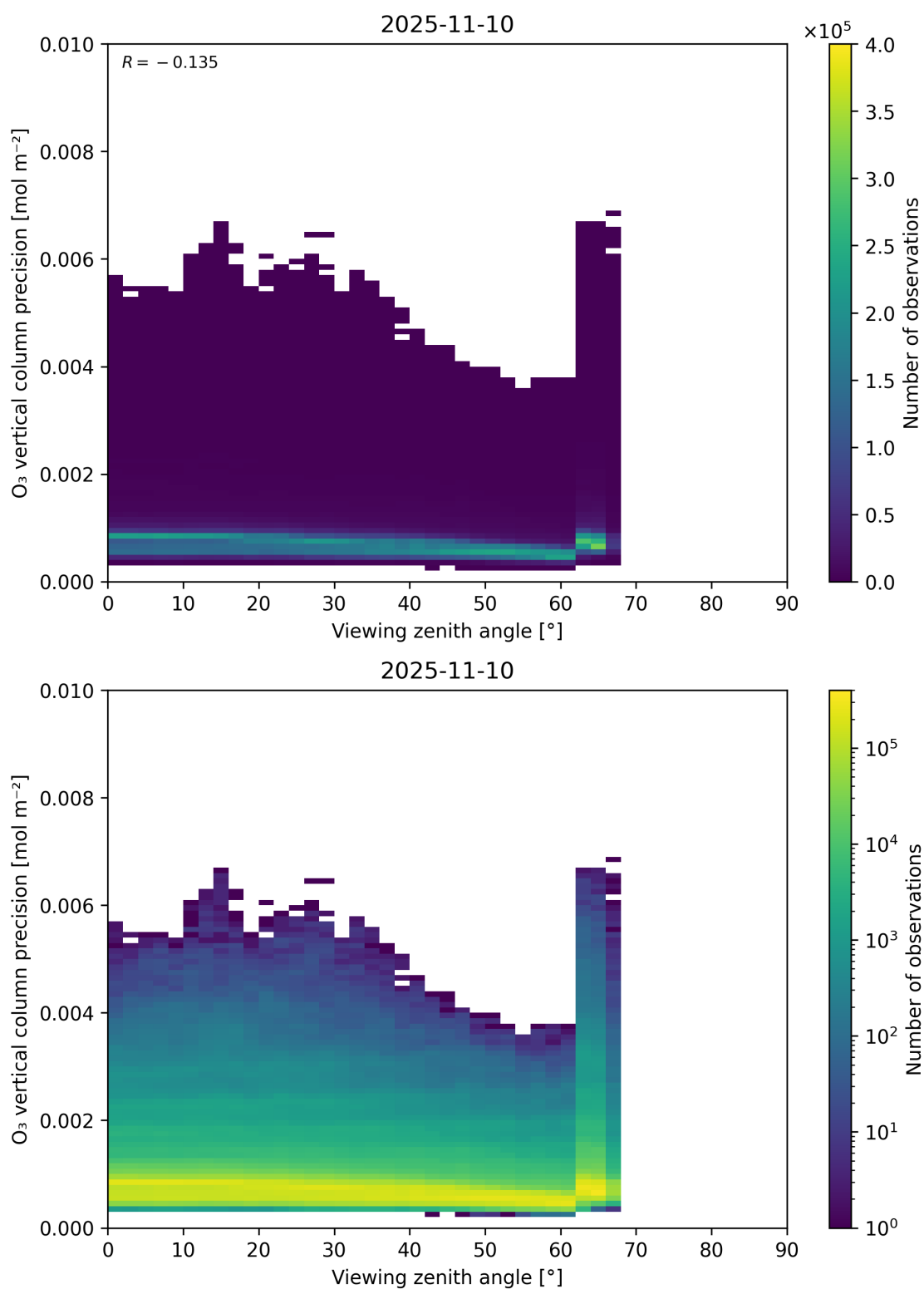
Figure 53: Scatter density plot of “Viewing zenith angle” against “O 3 vertical column precision” for 2025-11-09 to 2025-11-11.
