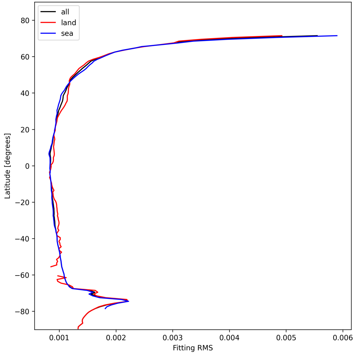
Figure 16: Zonal average of “Fitting RMS” for 2025-11-09 to 2025-11-11.
