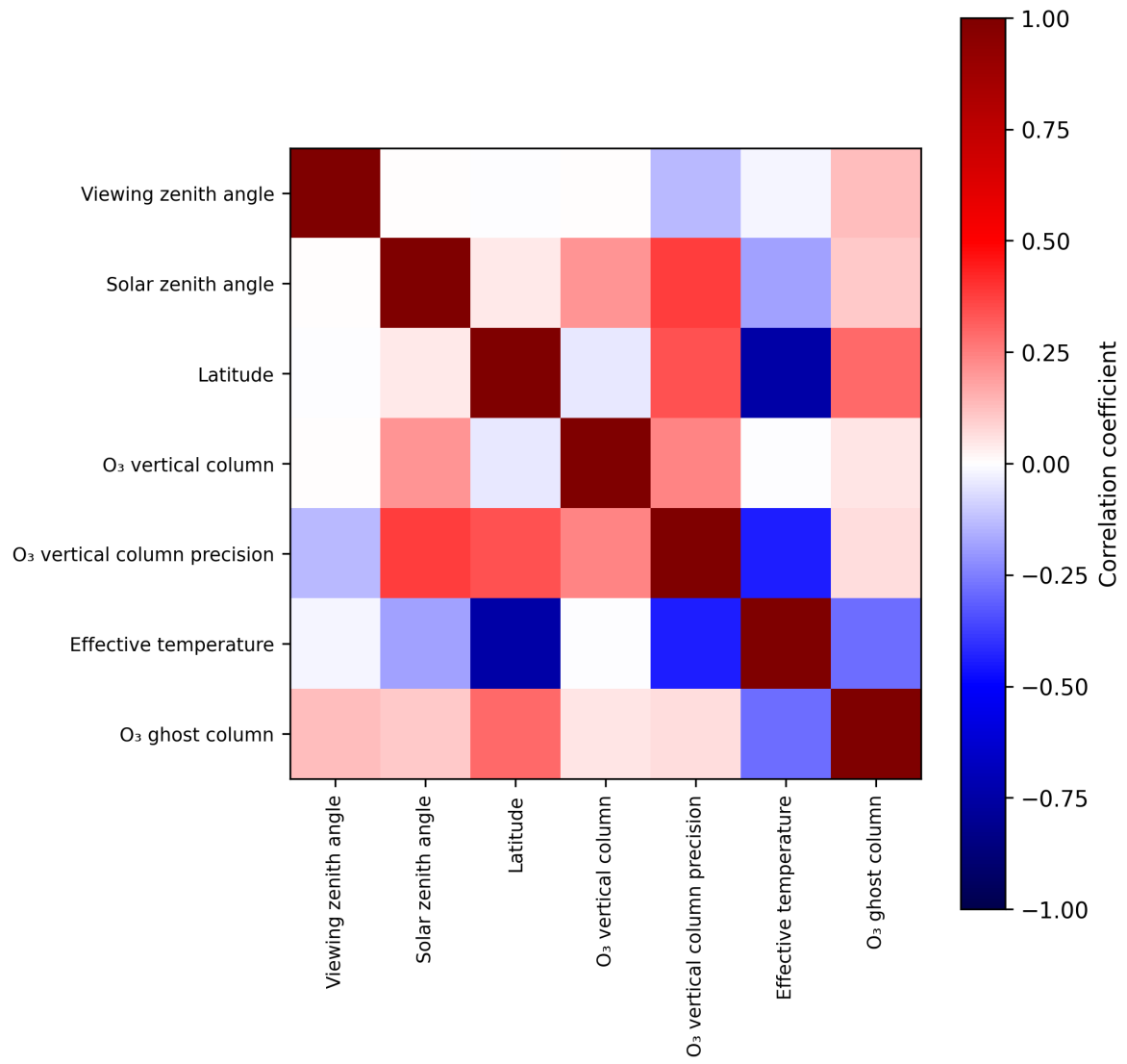
Figure 2: Map of correlation matrix for 2025-11-09 to 2025-11-11.
