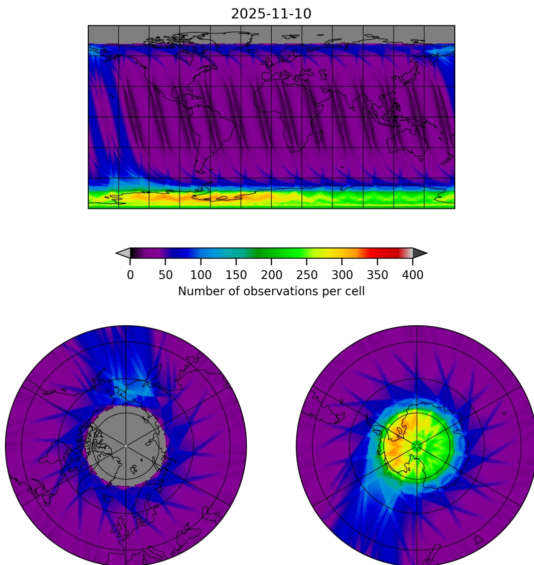
Figure 12: Map of the number of observations for 2025-11-09 to 2025-11-11
