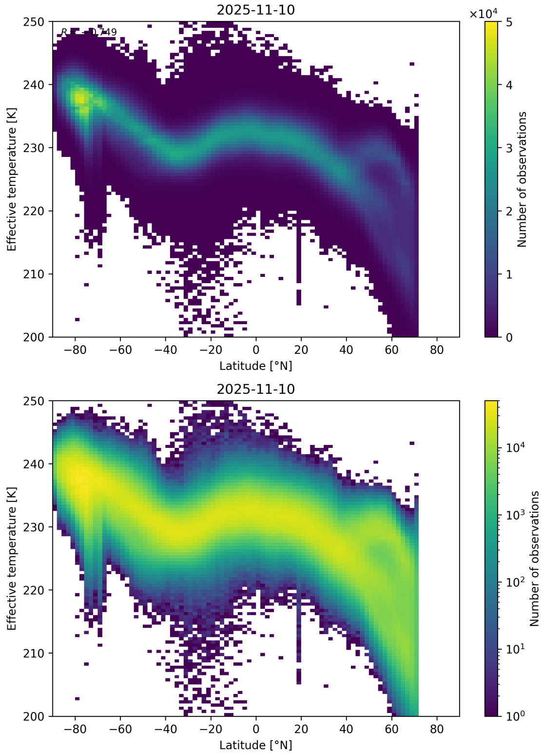
Figure 34: Scatter density plot of “Latitude” against “Effective temperature” for 2025-11-09 to 2025-11-11.
