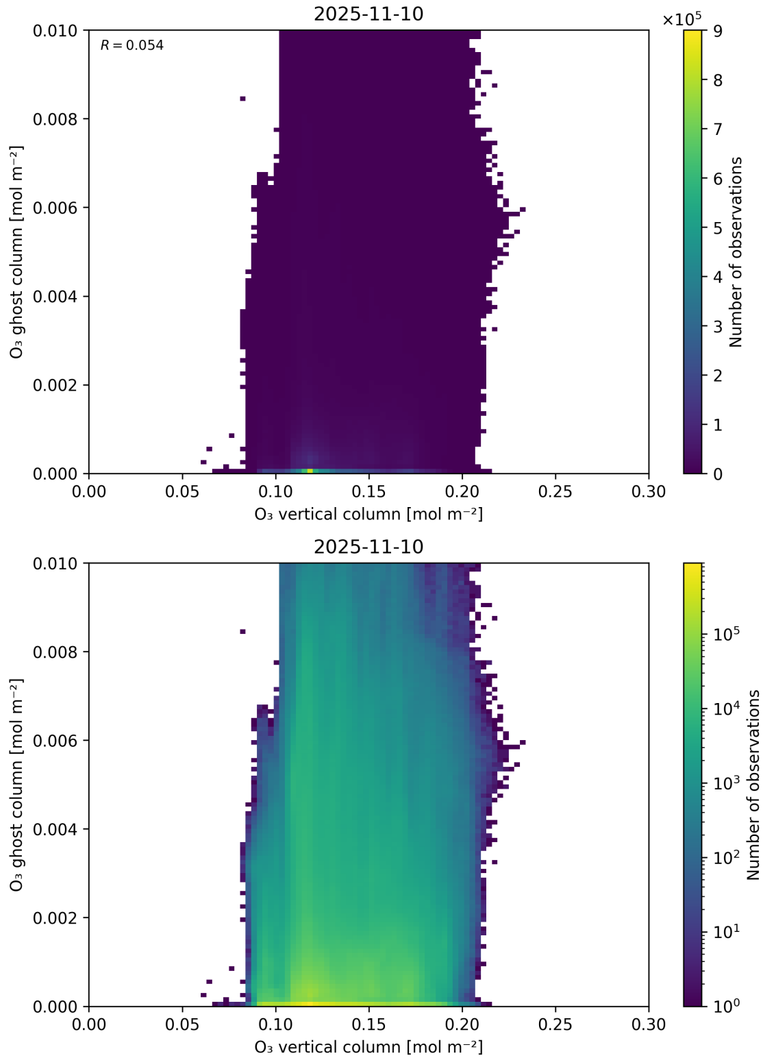
Figure 40: Scatter density plot of “O 3 vertical column” against “O 3 ghost column” for 2025-11-09 to 2025-11-11.
