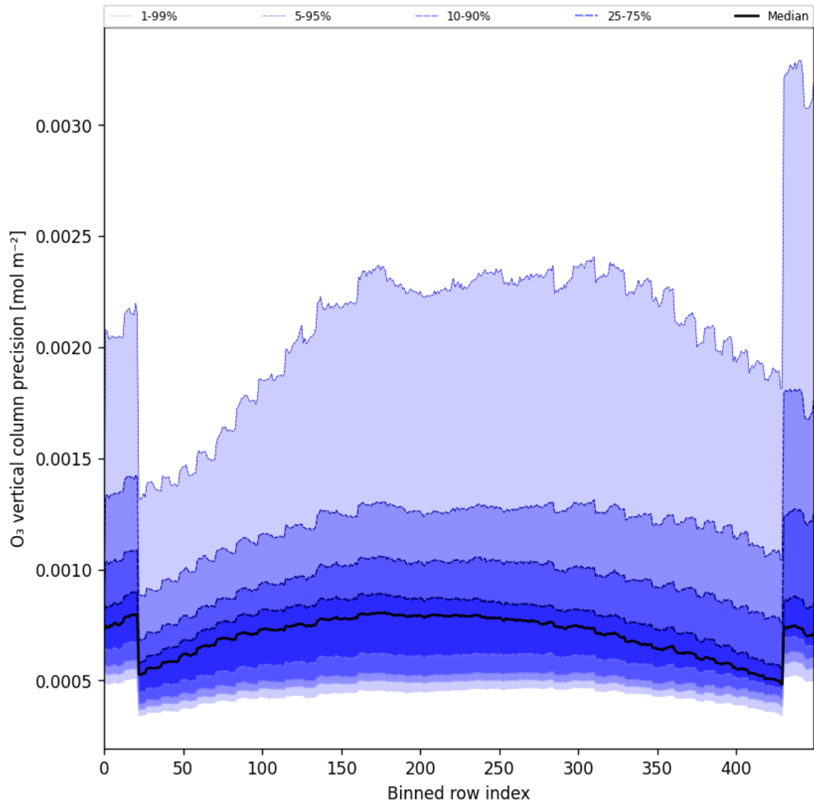
Figure 29: Along track statistics of “O 3 vertical column precision” for 2025-11-09 to 2025-11-11
