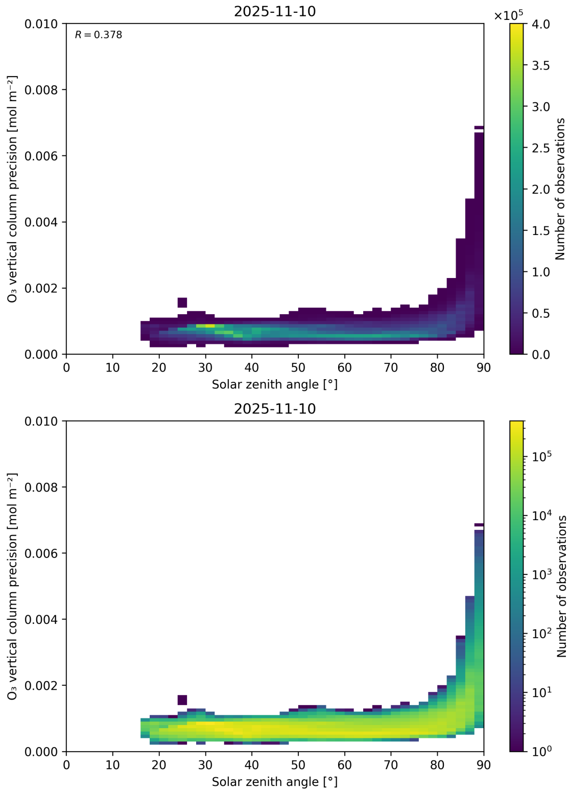
Figure 48: Scatter density plot of “Solar zenith angle” against “O 3 vertical column precision” for 2025-11-09 to 2025-11-11.
