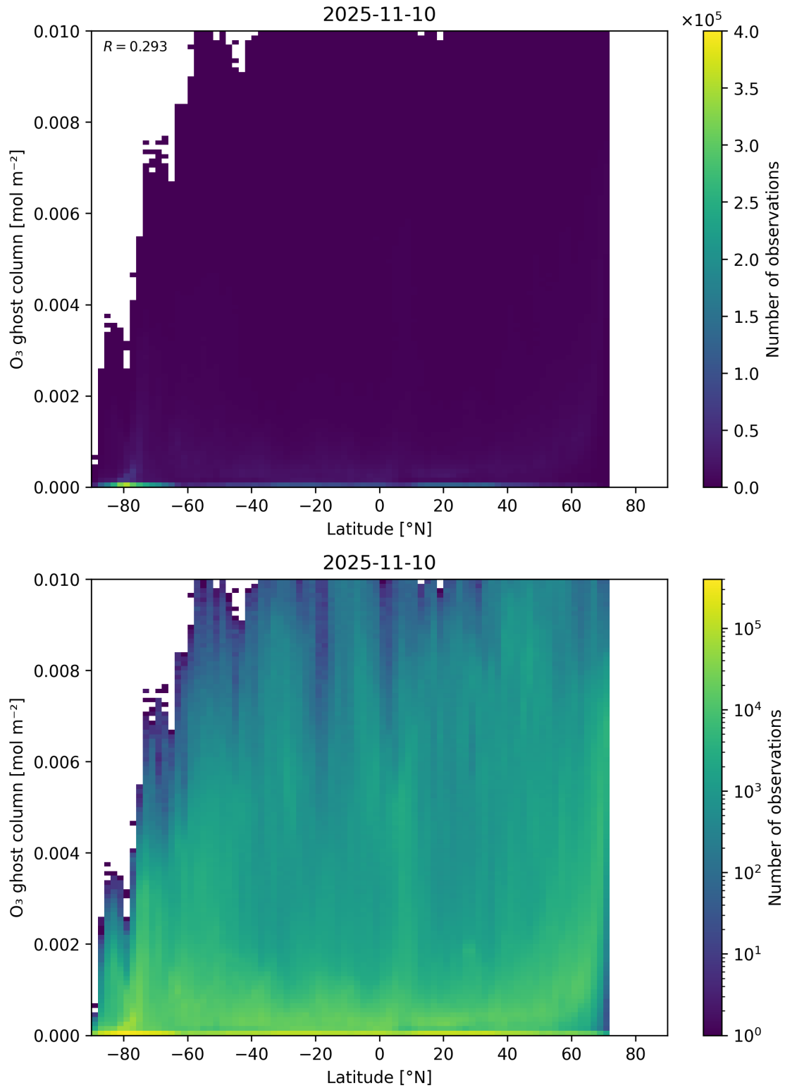
Figure 35: Scatter density plot of “Latitude” against “O 3 ghost column” for 2025-11-09 to 2025-11-11.
