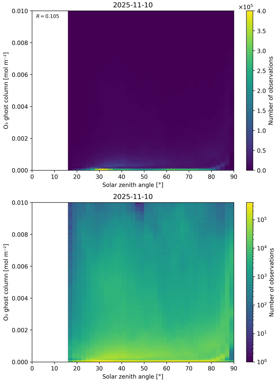
Figure 46: Scatter density plot of “Solar zenith angle” against “O 3 ghost column” for 2025-11-09 to 2025-11-11.
