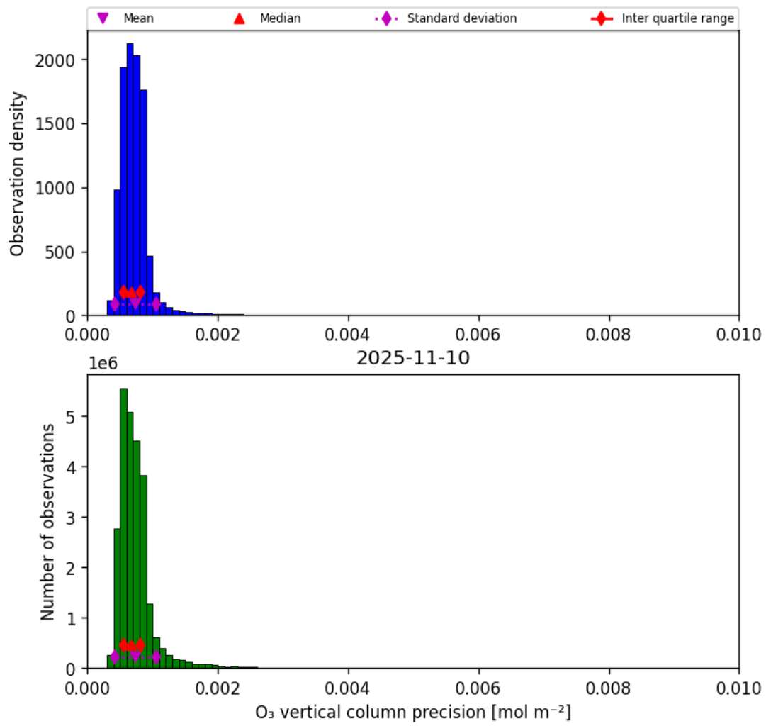
Figure 22: Histogram of “O 3 vertical column precision” for 2025-11-09 to 2025-11-11
