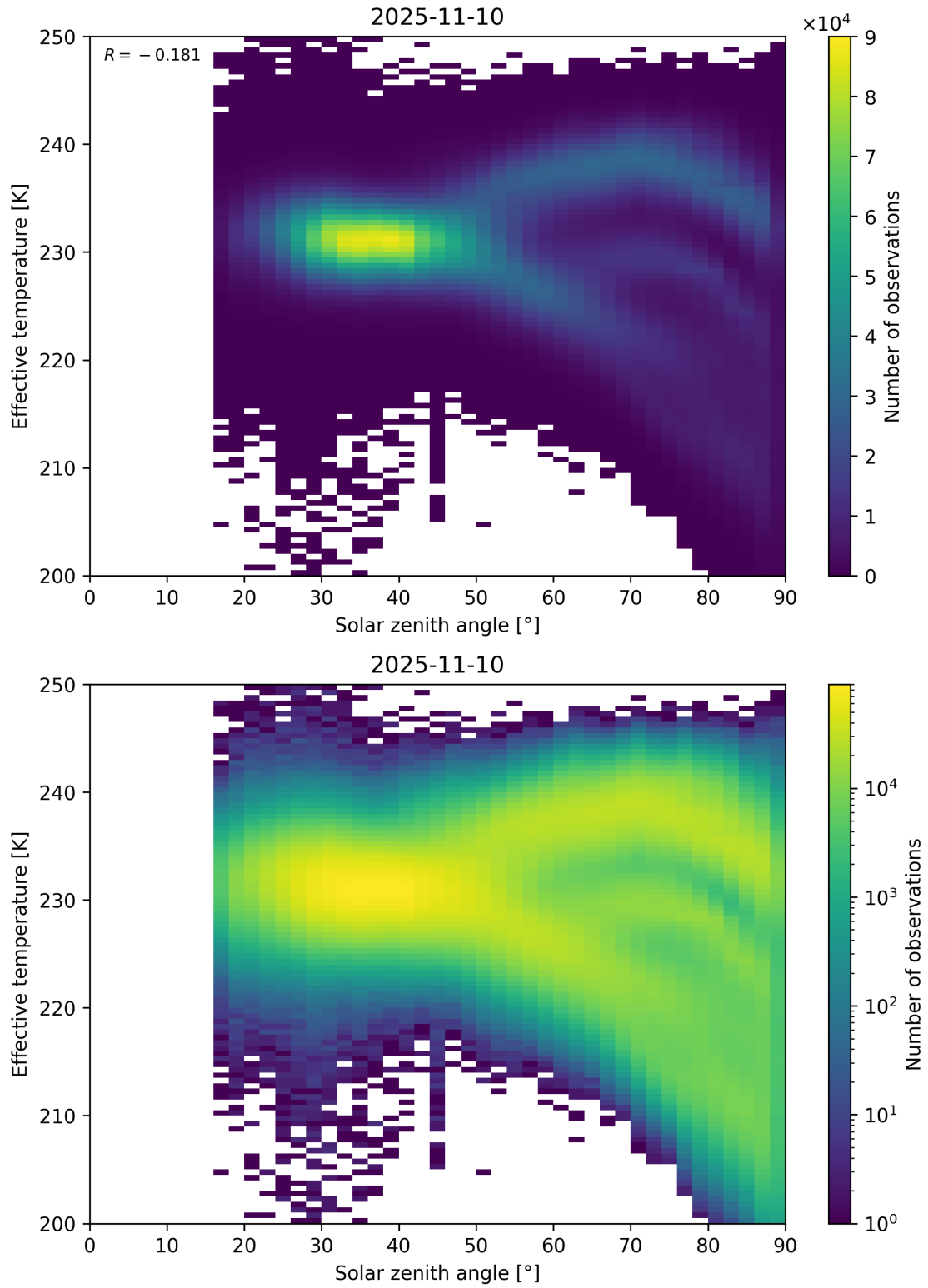
Figure 45: Scatter density plot of “Solar zenith angle” against “Effective temperature” for 2025-11-09 to 2025-11-11.
