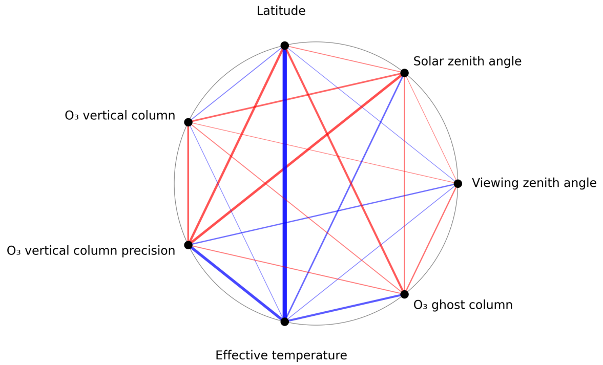
Figure 1: Map of correlation graph for 2025-11-09 to 2025-11-11.
