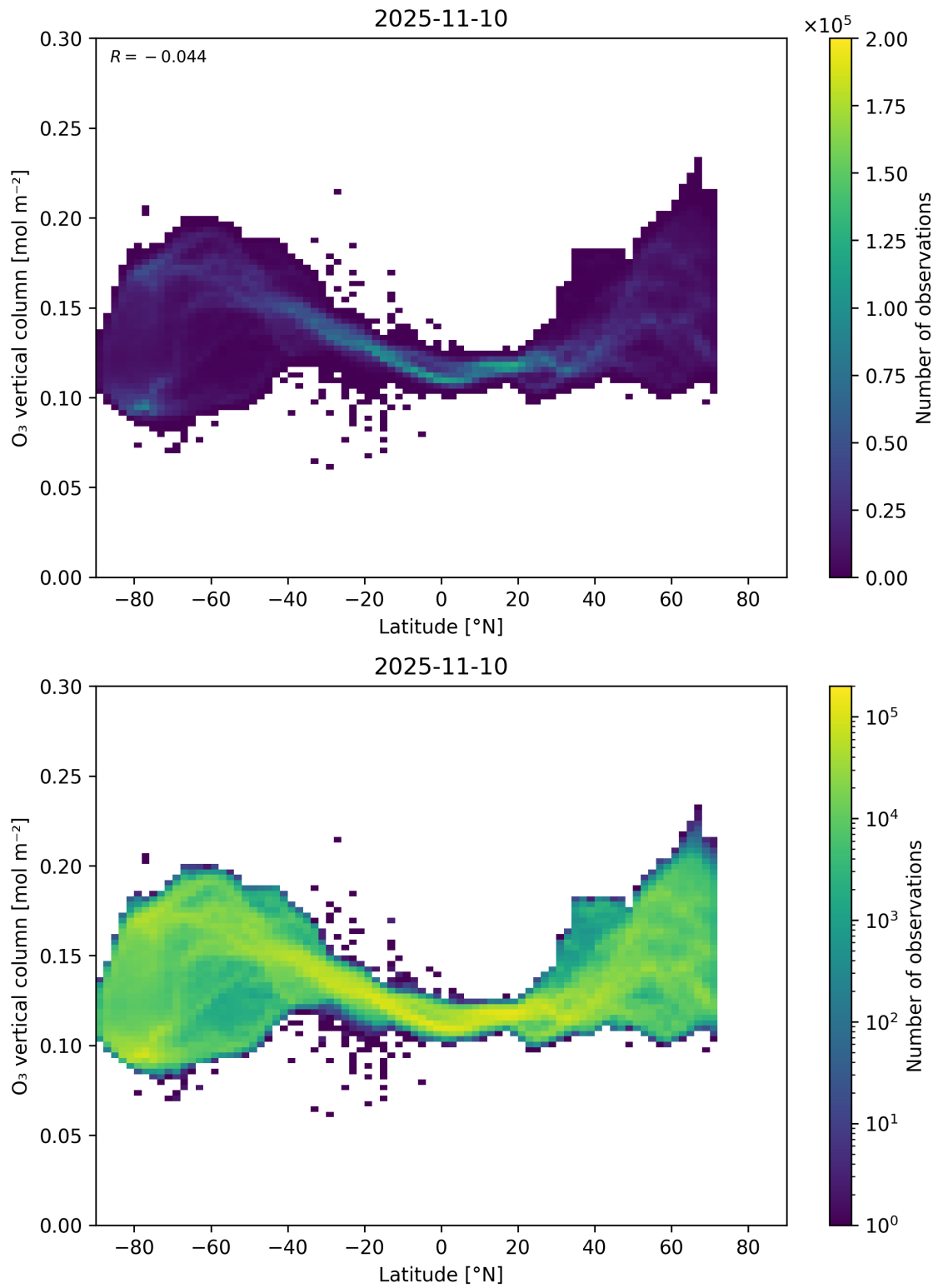
Figure 36: Scatter density plot of “Latitude” against “O 3 vertical column” for 2025-11-09 to 2025-11-11.
