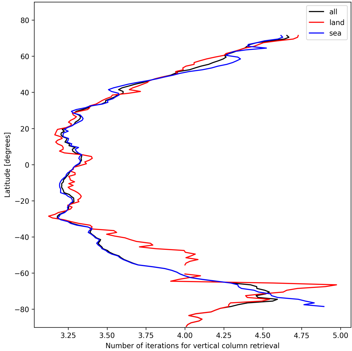
Figure 19: Zonal average of “Number of iterations for vertical column retrieval” for 2025-11-09 to 2025-11-11.
