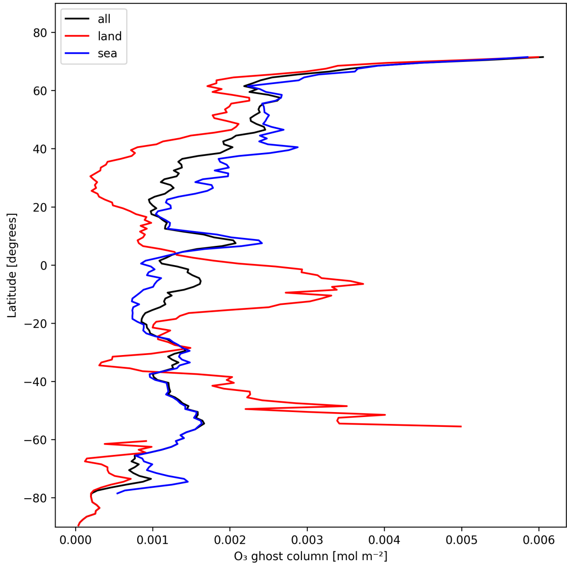
Figure 18: Zonal average of “O 3 ghost column” for 2025-11-09 to 2025-11-11.
