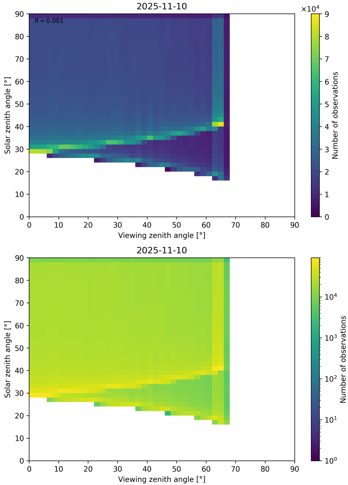
Figure 54: Scatter density plot of “Viewing zenith angle” against “Solar zenith angle” for 2025-11-09 to 2025-11-11.
