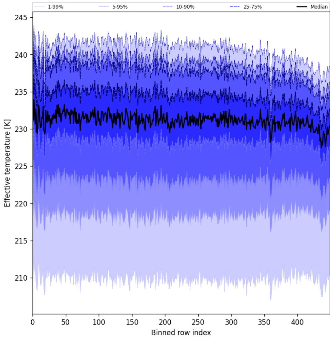
Figure 31: Along track statistics of “Effective temperature” for 2025-11-09 to 2025-11-11
