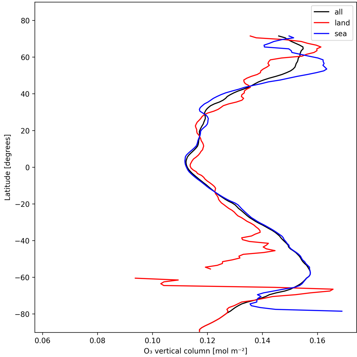
Figure 14: Zonal average of “O 3 vertical column” for 2025-11-09 to 2025-11-11.
