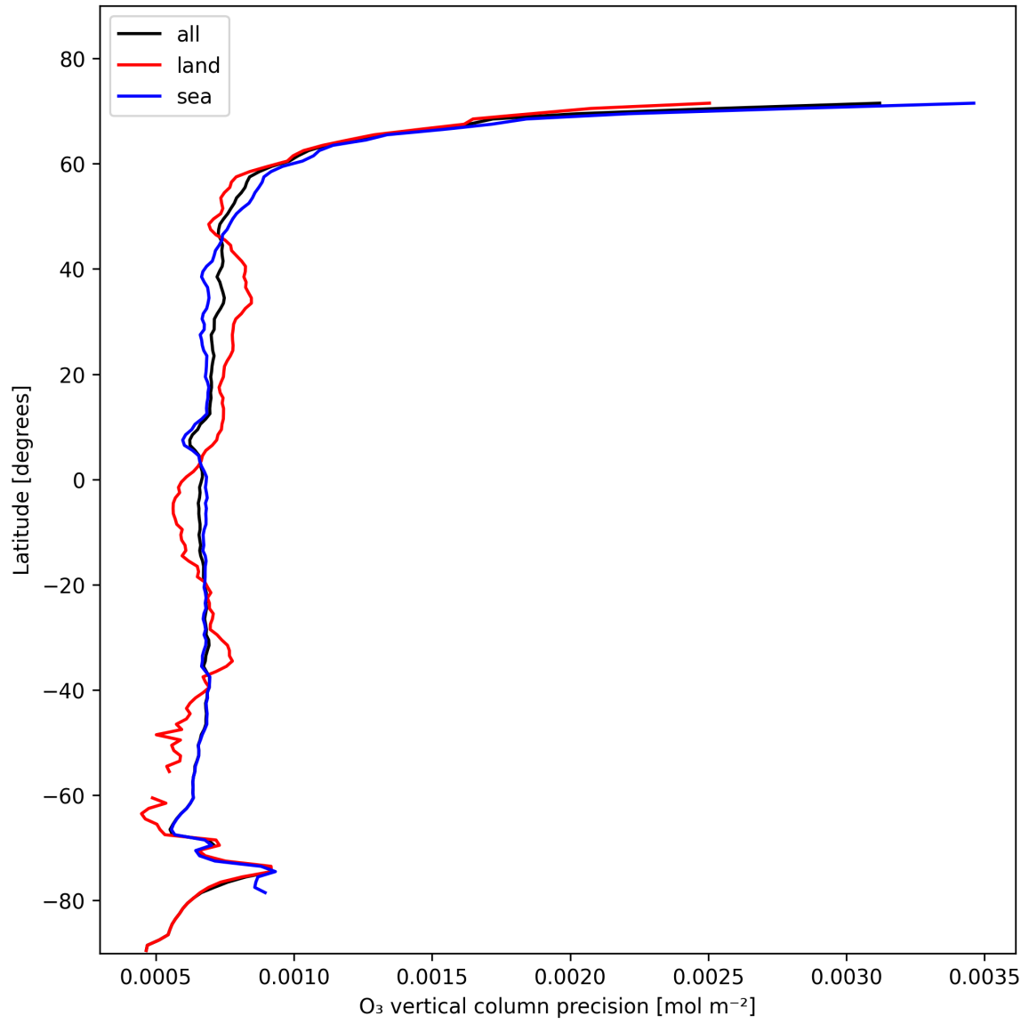
Figure 15: Zonal average of “O 3 vertical column precision” for 2025-11-09 to 2025-11-11.
