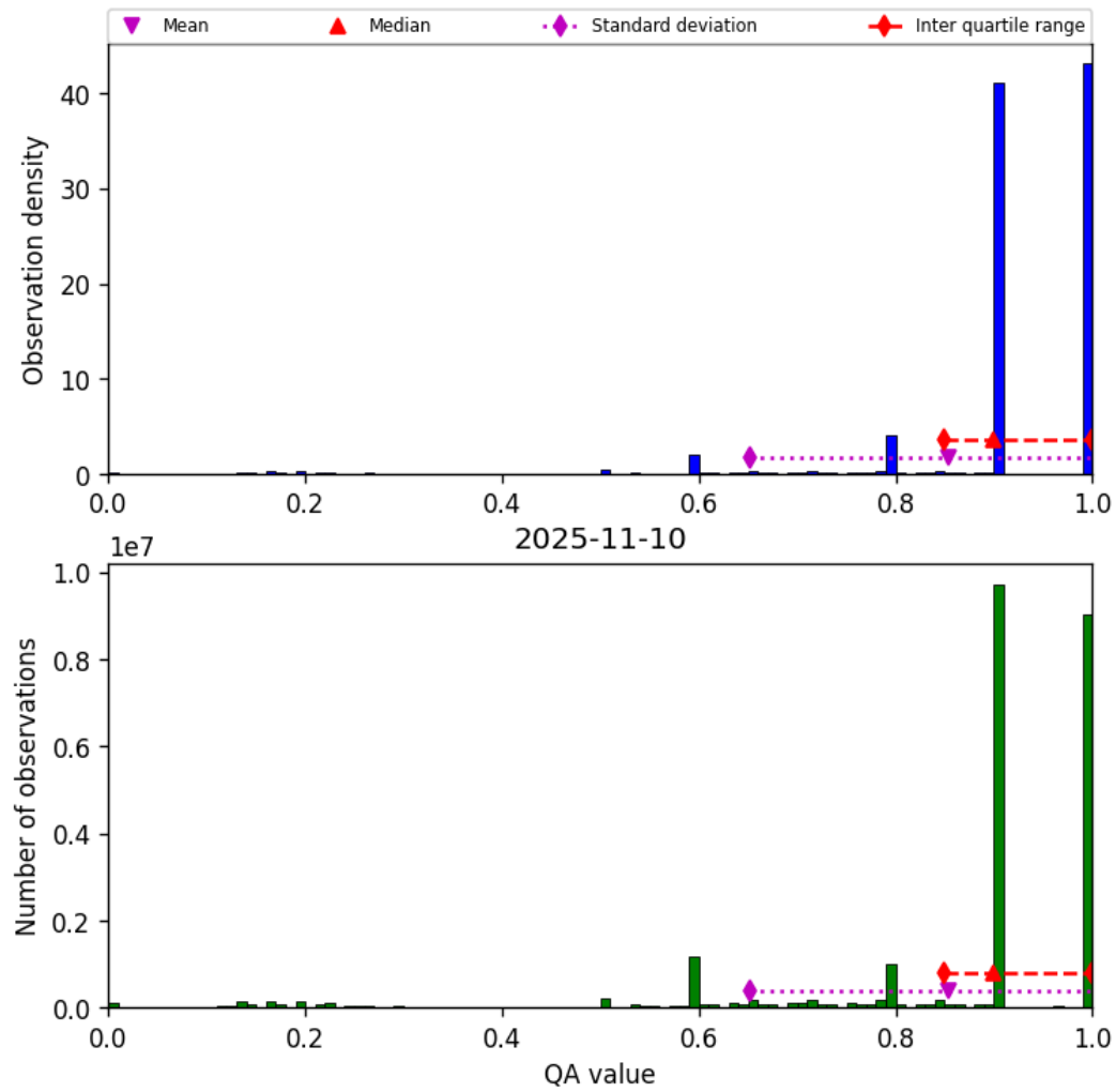
Figure 20: Histogram of “QA value” for 2025-11-09 to 2025-11-11
