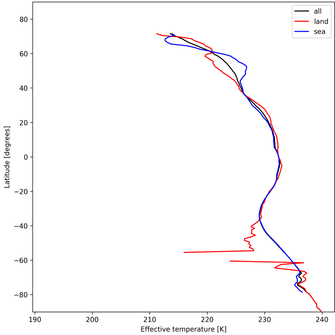
Figure 17: Zonal average of "Effective temperature" for 2025-11-09 to 2025-11-11.
