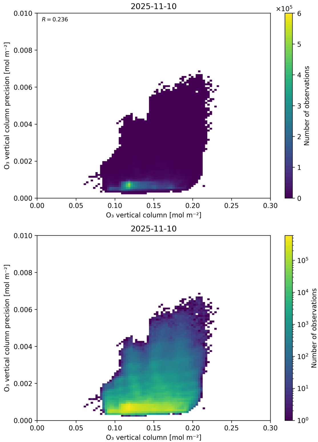
Figure 41: Scatter density plot of “O 3 vertical column” against “O 3 vertical column precision” for 2025-11-09 to 2025-11-11.
