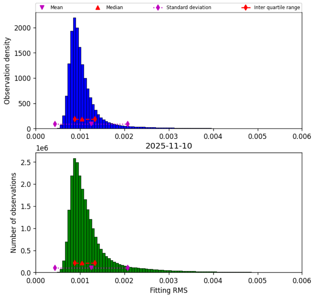
Figure 23: Histogram of “Fitting RMS” for 2025-11-09 to 2025-11-11
