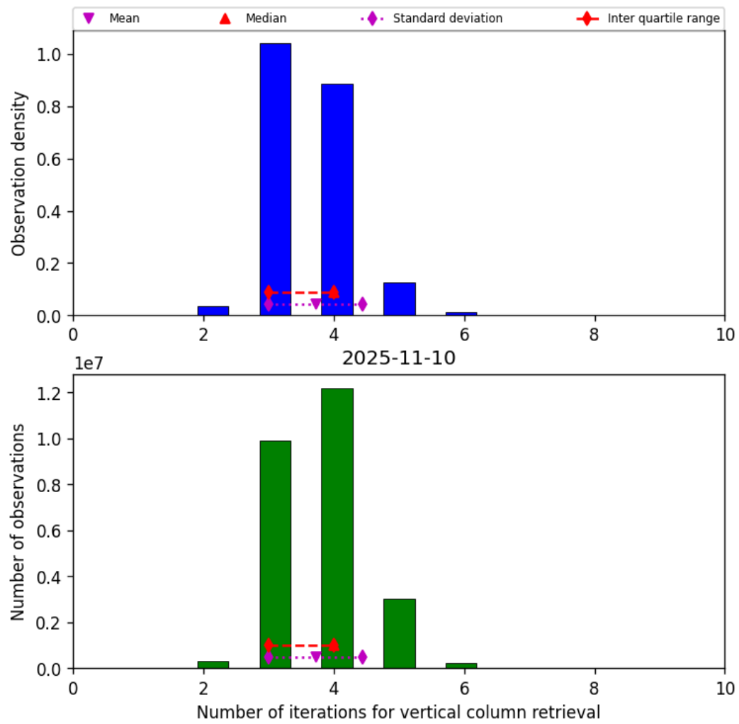
Figure 26: Histogram of “Number of iterations for vertical column retrieval” for 2025-11-09 to 2025-11-11
