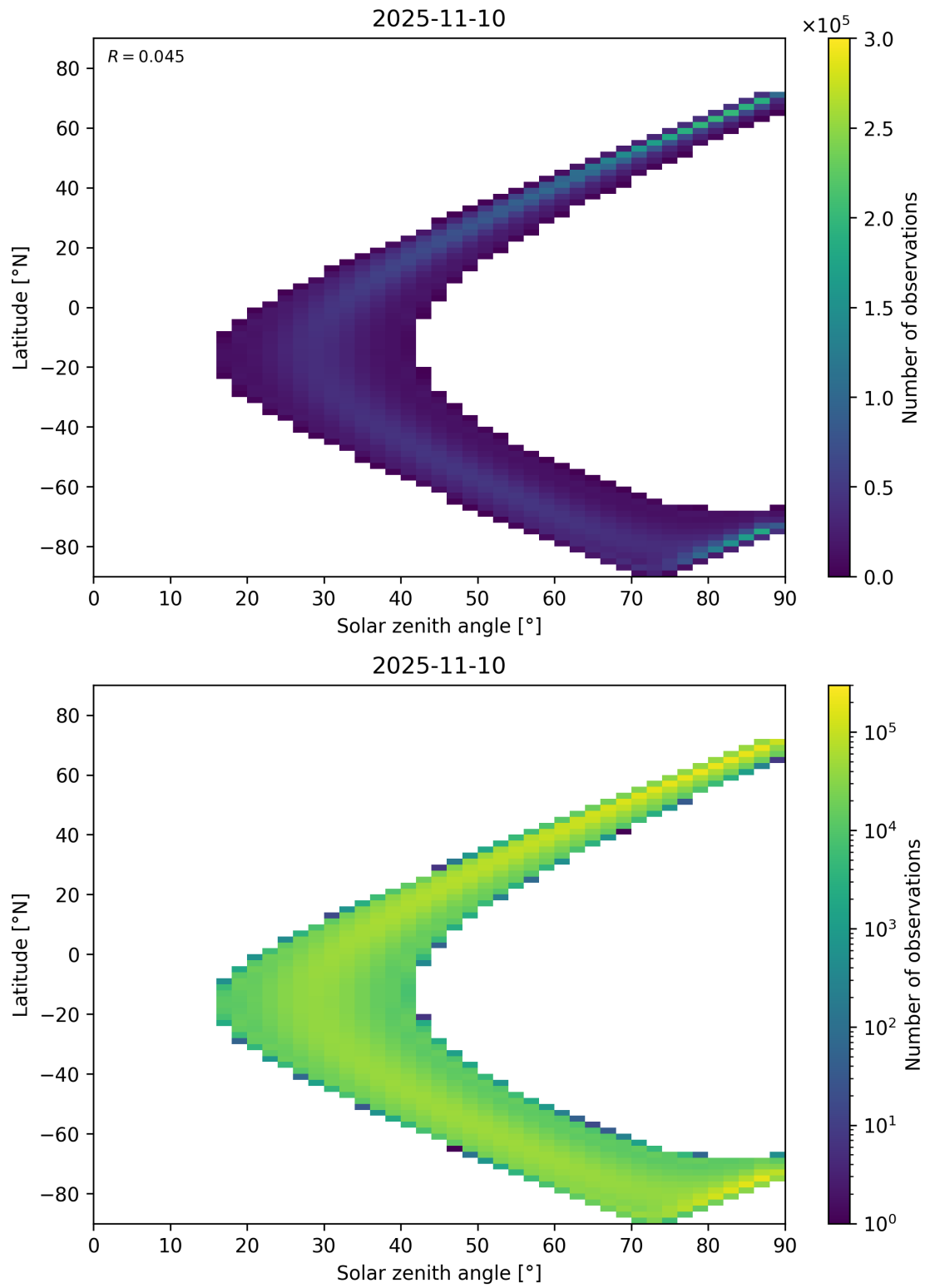
Figure 44: Scatter density plot of “Solar zenith angle” against “Latitude” for 2025-11-09 to 2025-11-11.
