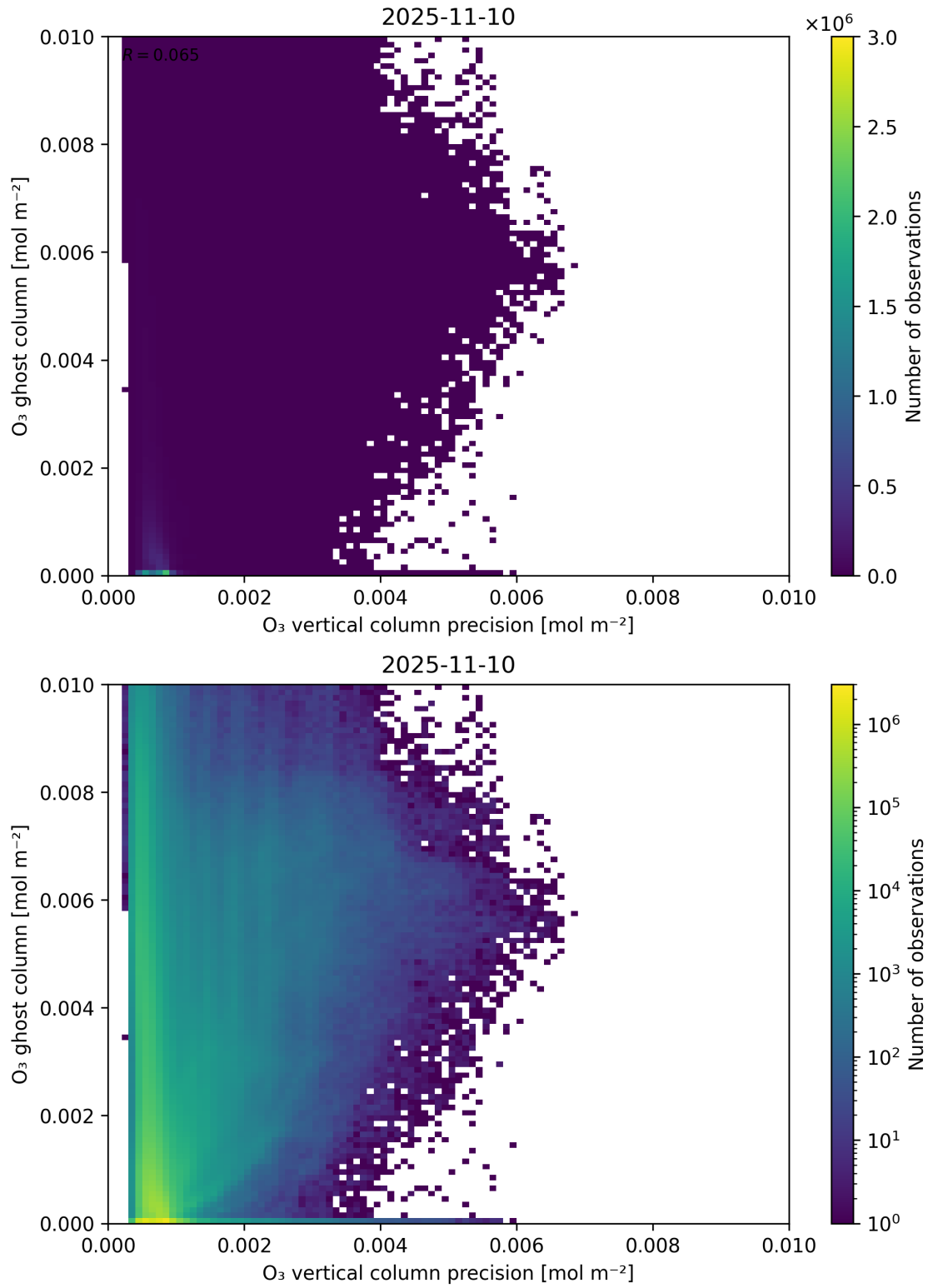
Figure 43: Scatter density plot of “O 3 vertical column precision” against “O 3 ghost column” for 2025-11-09 to 2025-11-11.
