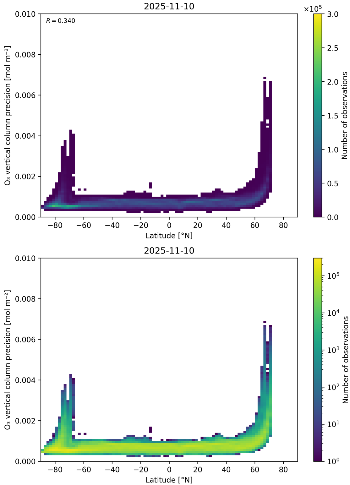
Figure 37: Scatter density plot of “Latitude” against “O 3 vertical column precision” for 2025-11-09 to 2025-11-11.
