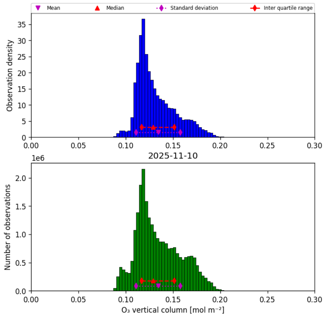
Figure 21: Histogram of “O 3 vertical column” for 2025-11-09 to 2025-11-11
