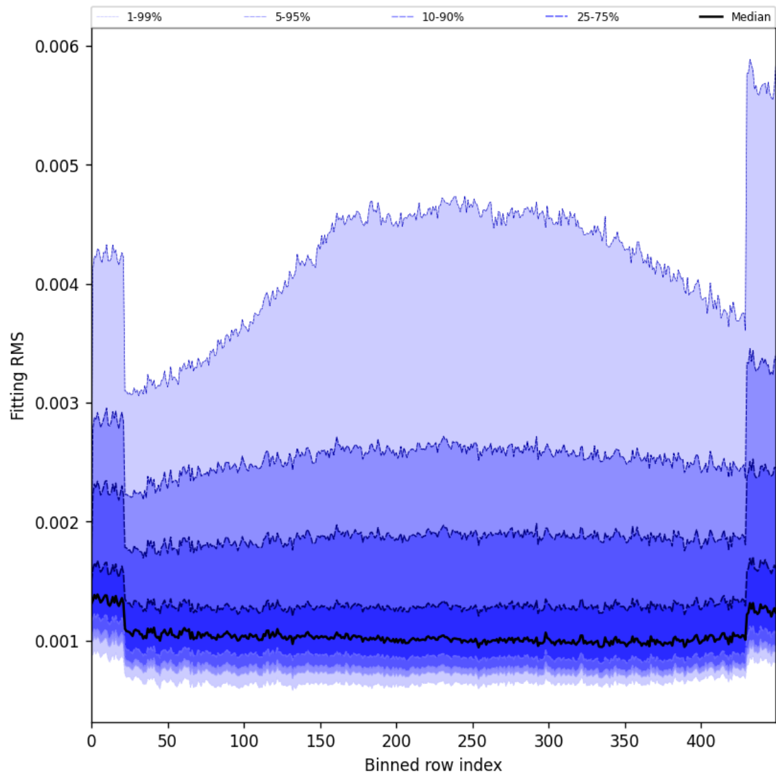
Figure 30: Along track statistics of “Fitting RMS” for 2025-11-09 to 2025-11-11
