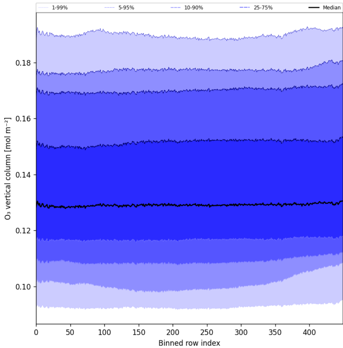
Figure 28: Along track statistics of “O 3 vertical column” for 2025-11-09 to 2025-11-11
