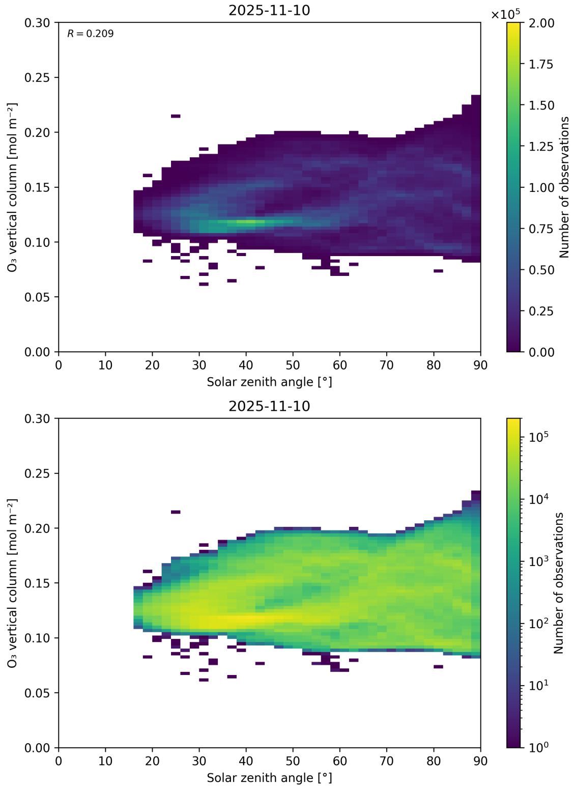
Figure 47: Scatter density plot of “Solar zenith angle” against “O 3 vertical column” for 2025-11-09 to 2025-11-11.
