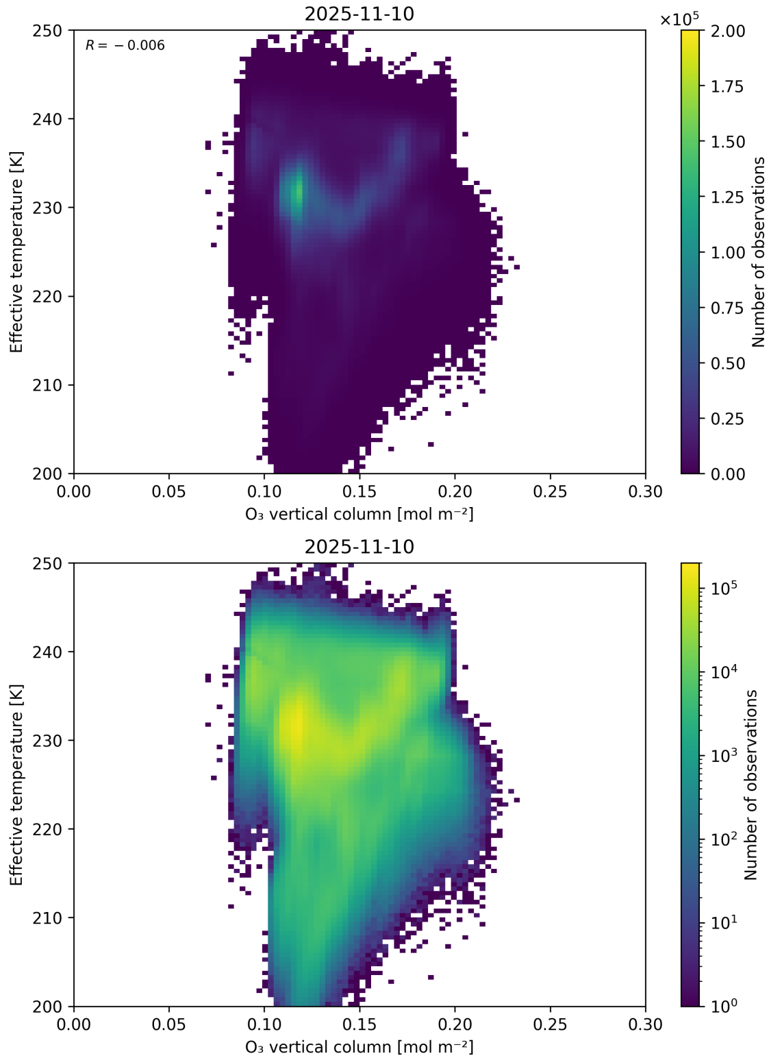
Figure 39: Scatter density plot of “O 3 vertical column” against “Effective temperature” for 2025-11-09 to 2025-11-11.
