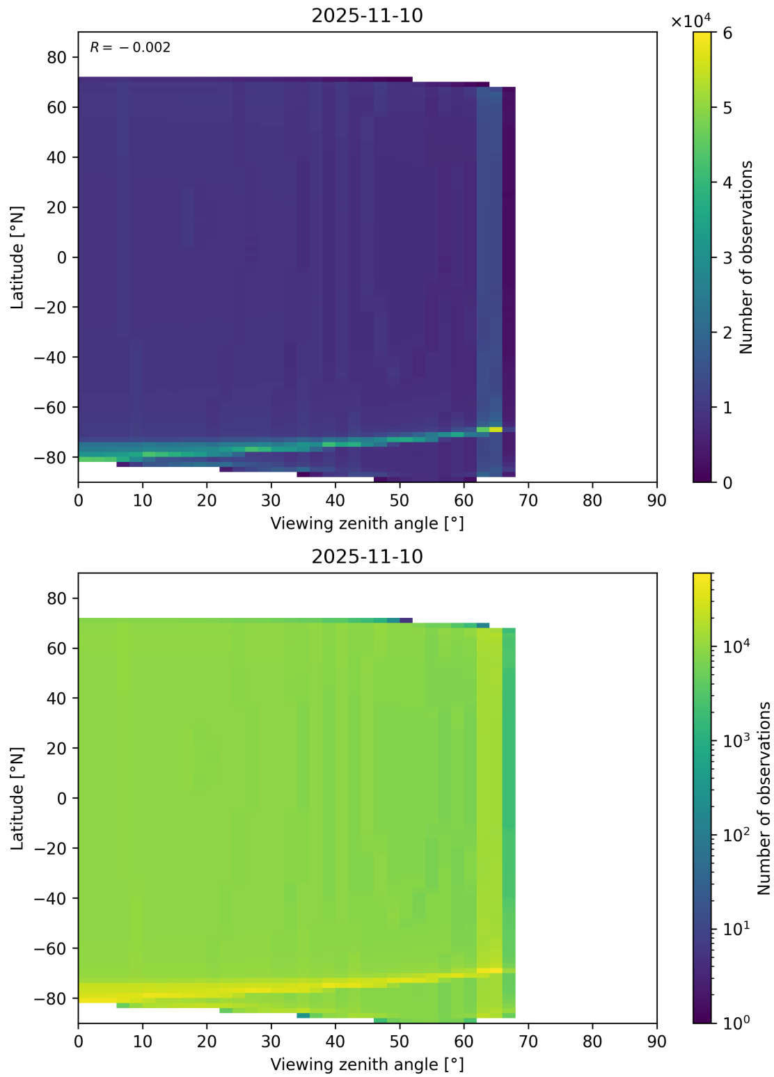
Figure 49: Scatter density plot of “Viewing zenith angle” against “Latitude” for 2025-11-09 to 2025-11-11.
