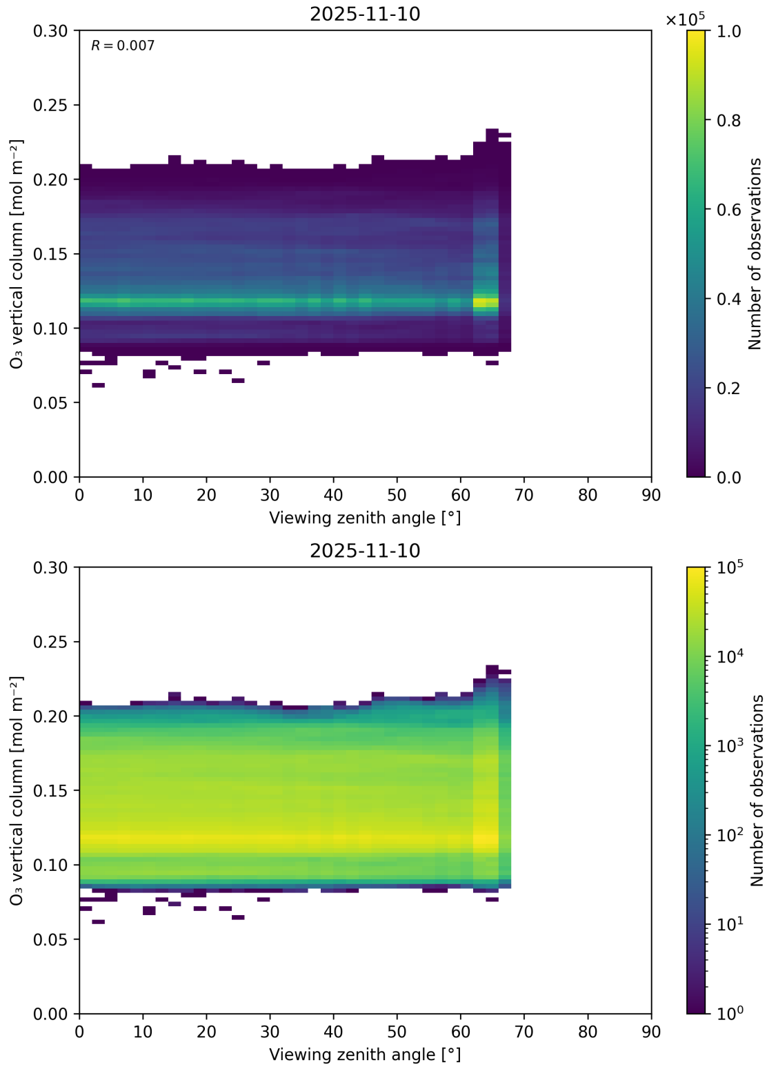
Figure 52: Scatter density plot of “Viewing zenith angle” against “O 3 vertical column” for 2025-11-09 to 2025-11-11.
