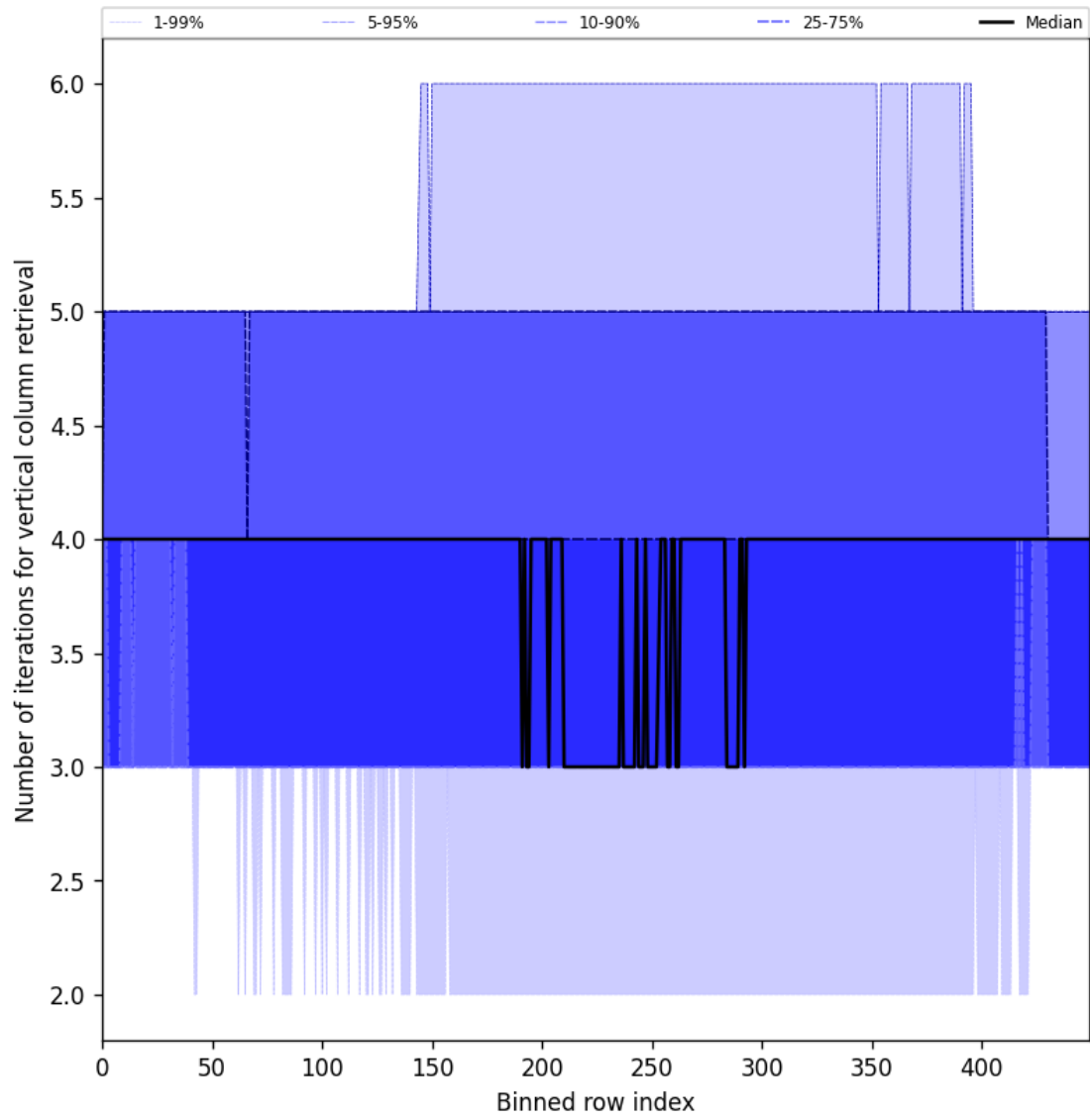
Figure 33: Along track statistics of “Number of iterations for vertical column retrieval” for 2025-11-09 to 2025-11-11
