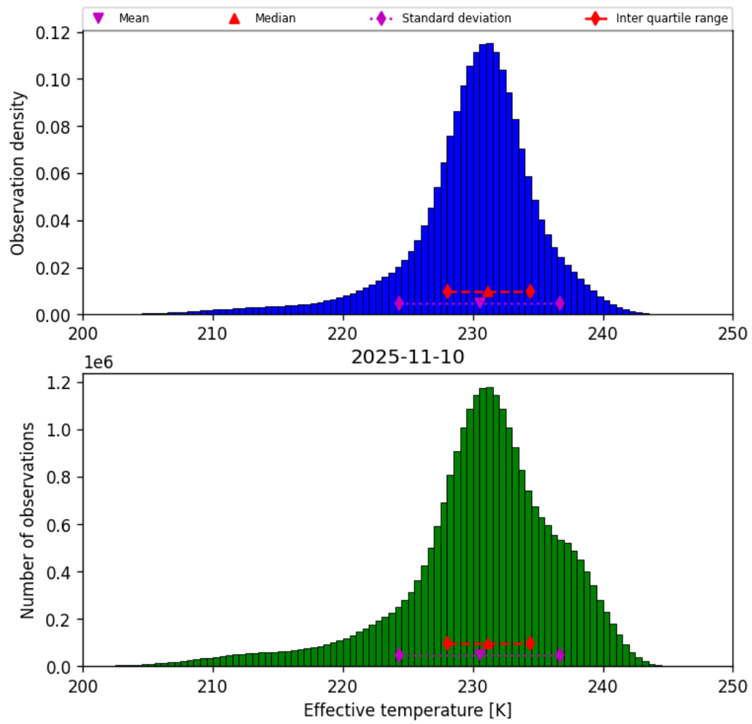
Figure 24: Histogram of “Effective temperature” for 2025-11-09 to 2025-11-11
