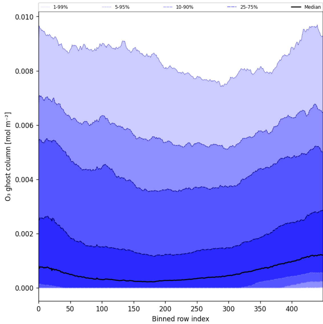
Figure 32: Along track statistics of "O 3 ghost column" for 2025-11-09 to 2025-11-11
