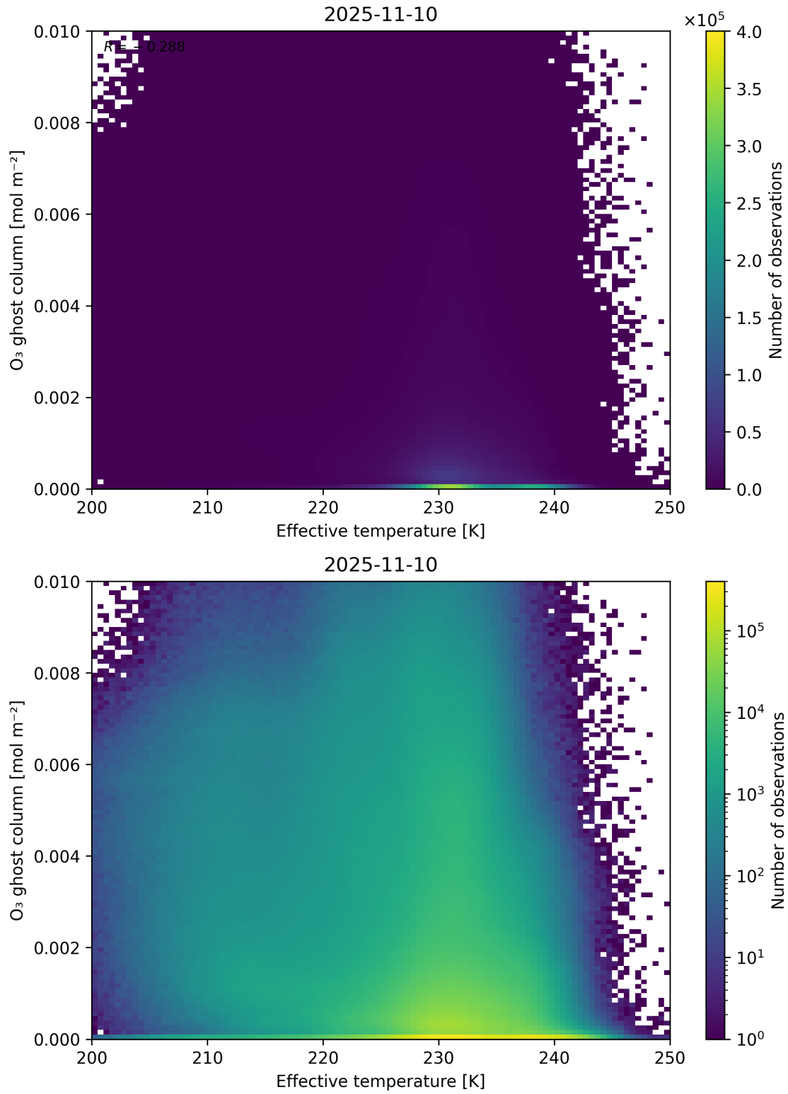
Figure 38: Scatter density plot of “Effective temperature” against “O 3 ghost column” for 2025-11-09 to 2025-11-11.
