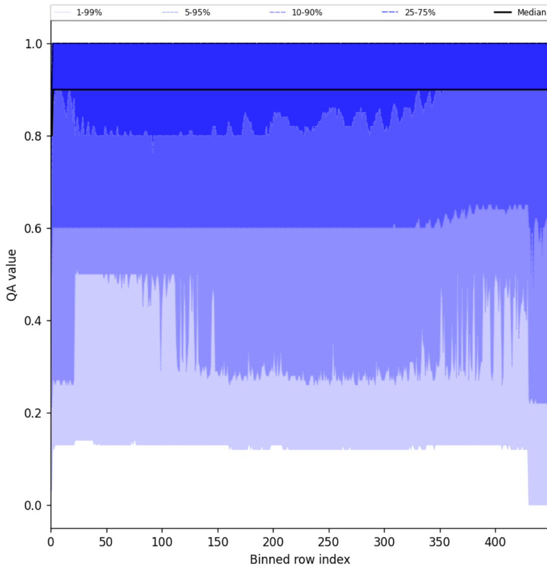
Figure 27: Along track statistics of “QA value” for 2025-11-09 to 2025-11-11
