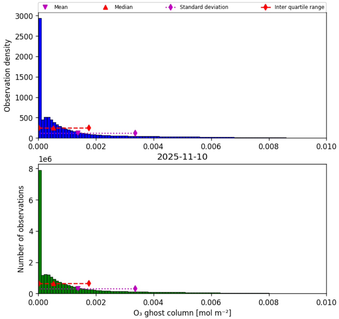
Figure 25: Histogram of “O 3 ghost column” for 2025-11-09 to 2025-11-11
