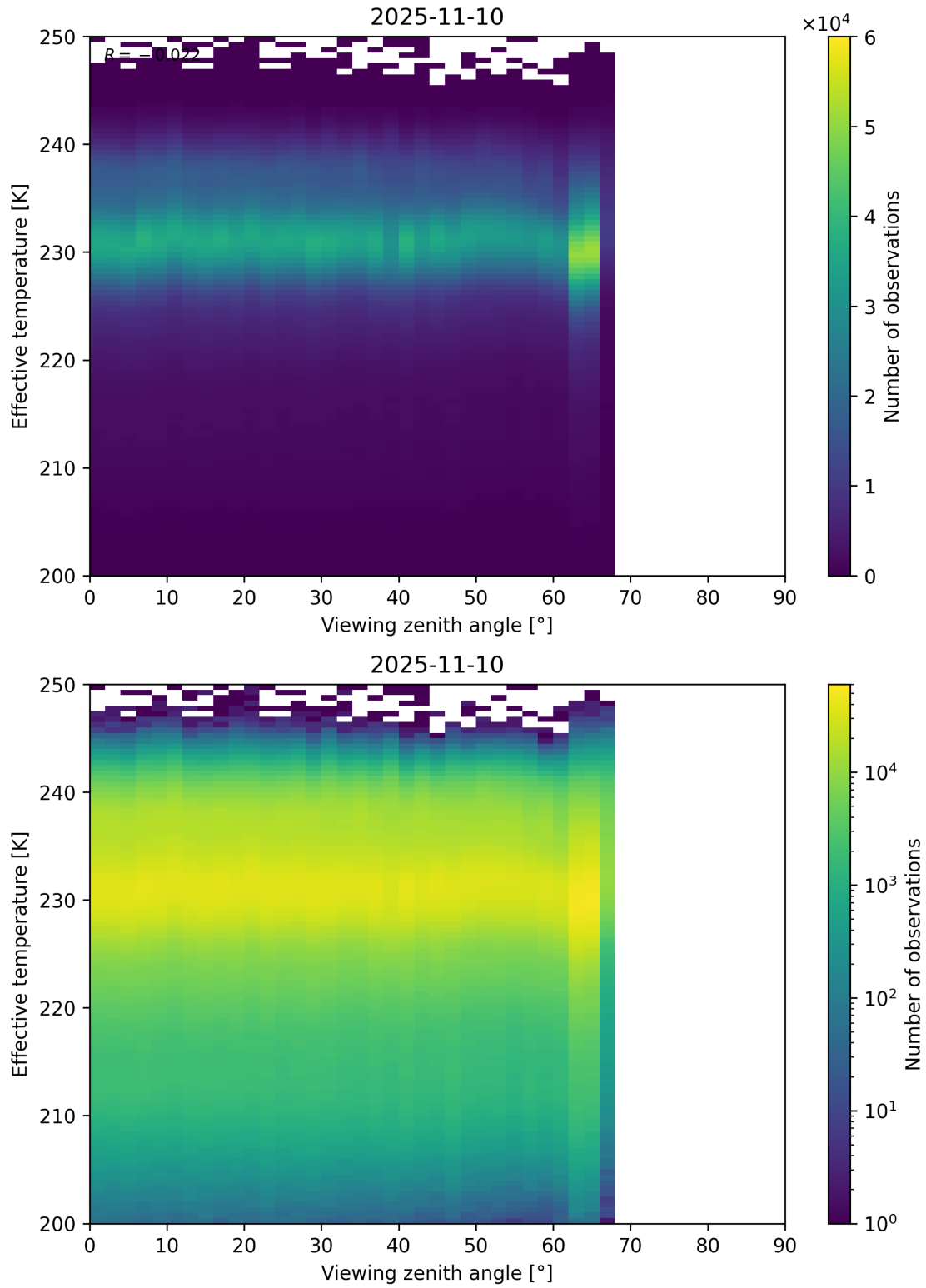
Figure 50: Scatter density plot of “Viewing zenith angle” against “Effective temperature” for 2025-11-09 to 2025-11-11.
