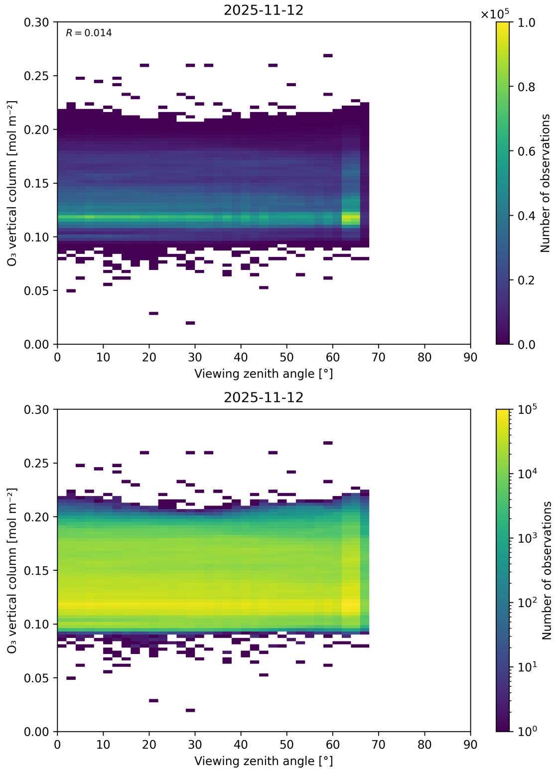
Figure 52: Scatter density plot of “Viewing zenith angle” against “O 3 vertical column” for 2025-11-12 to 2025-11-13.
