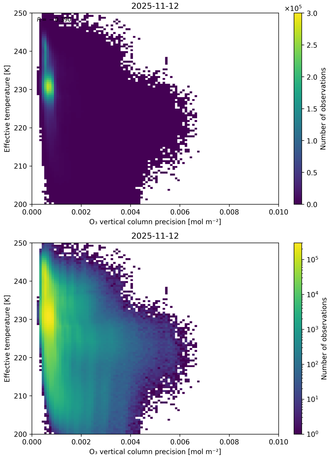
Figure 42: Scatter density plot of “O 3 vertical column precision” against “Effective temperature” for 2025-11-12 to 2025-11-13.
