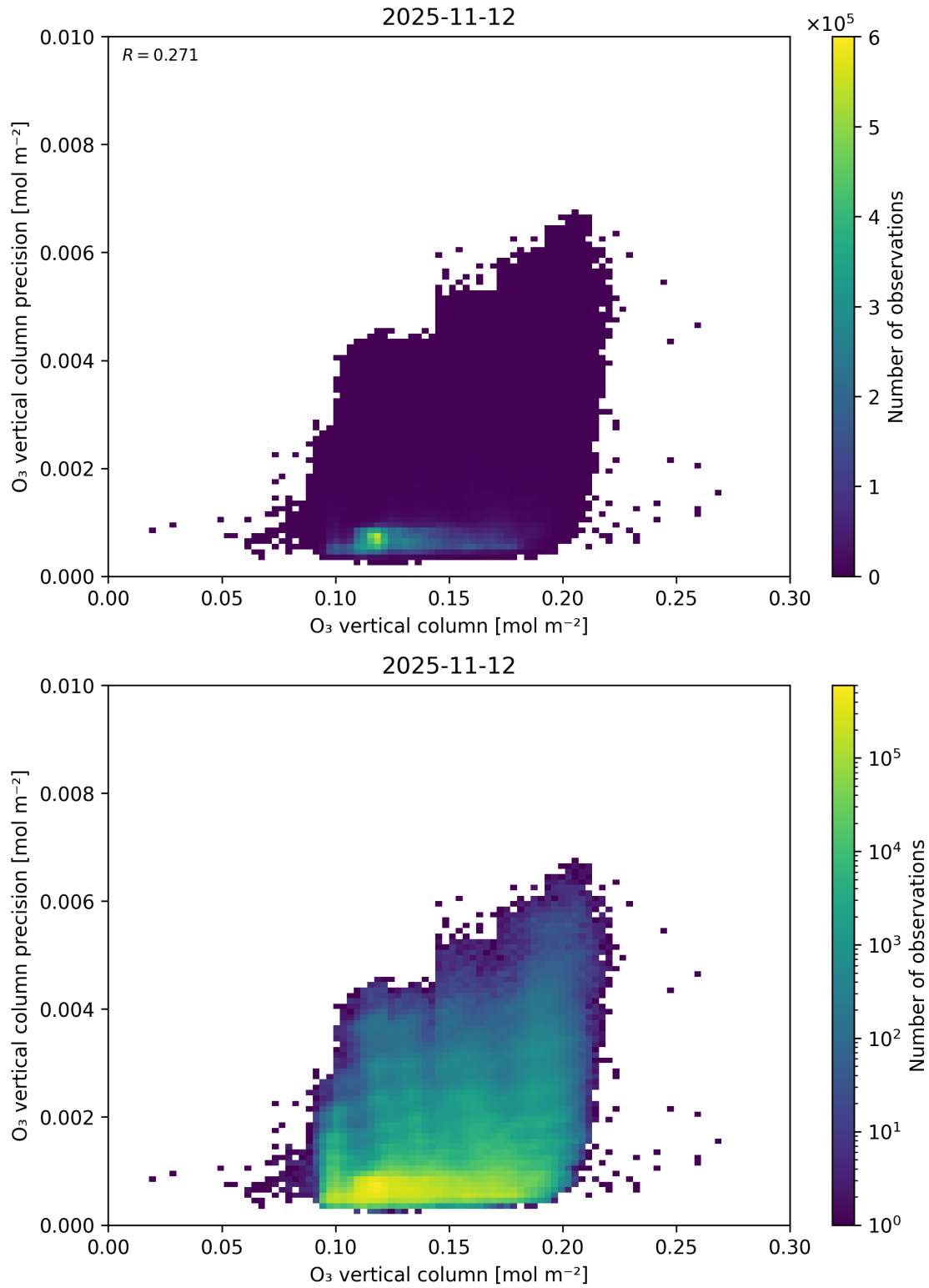
Figure 41: Scatter density plot of “O 3 vertical column” against “O 3 vertical column precision” for 2025-11-12 to 2025-11-13.
