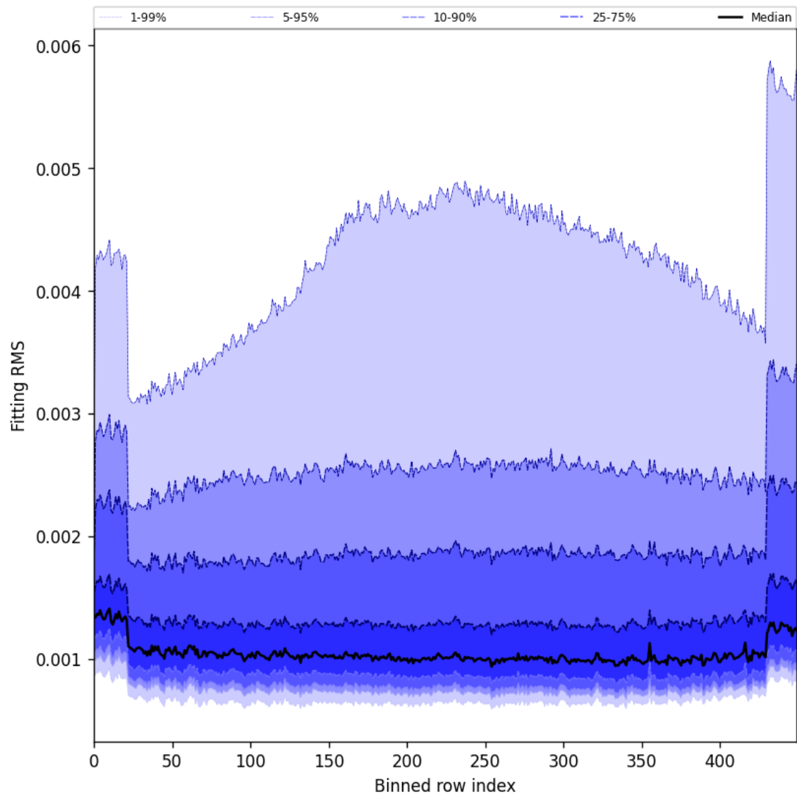
Figure 30: Along track statistics of “Fitting RMS” for 2025-11-12 to 2025-11-13
