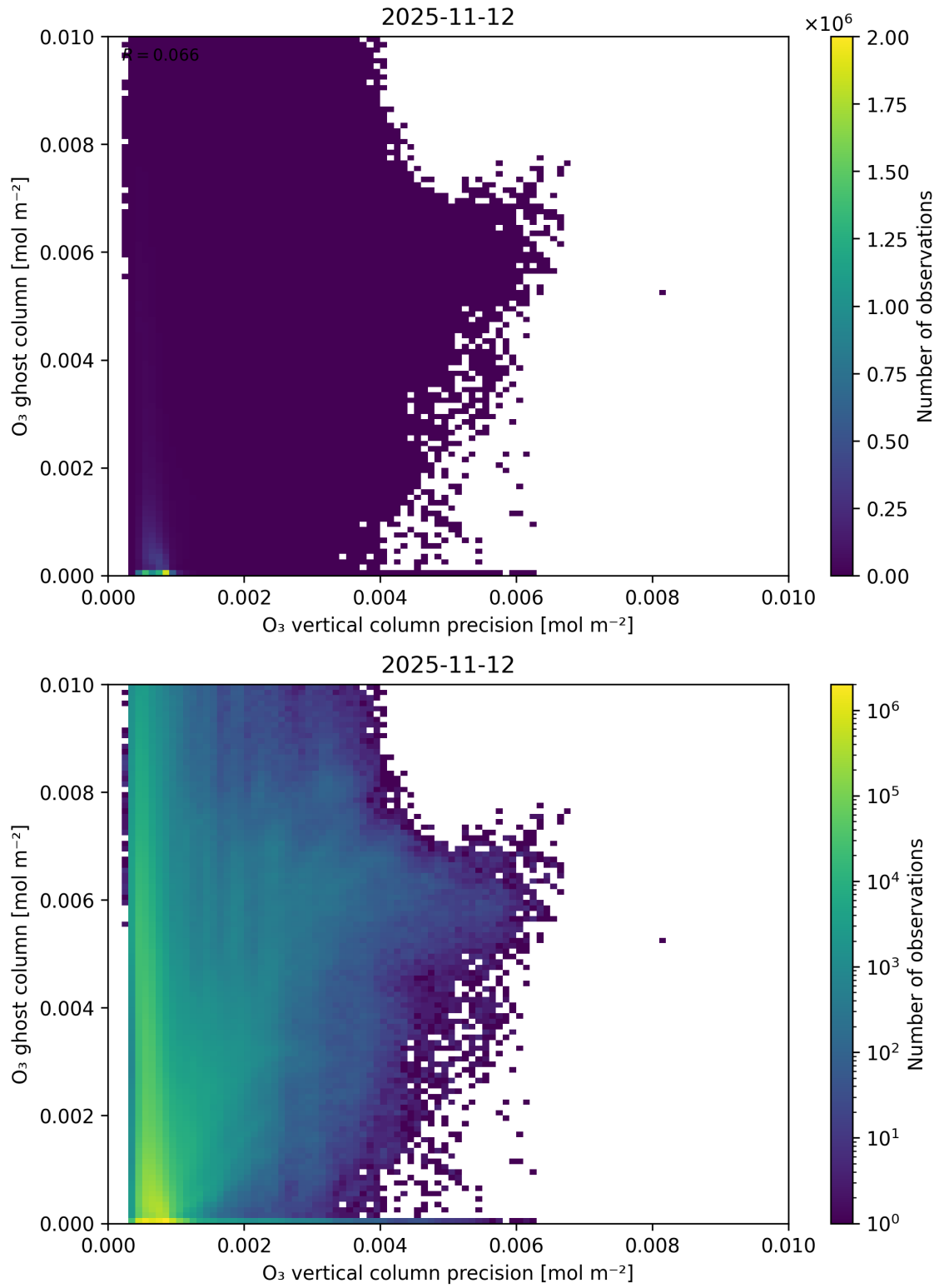
Figure 43: Scatter density plot of “ \text{O}_3 vertical column precision” against “ \text{O}_3 ghost column” for 2025-11-12 to 2025-11-13.
