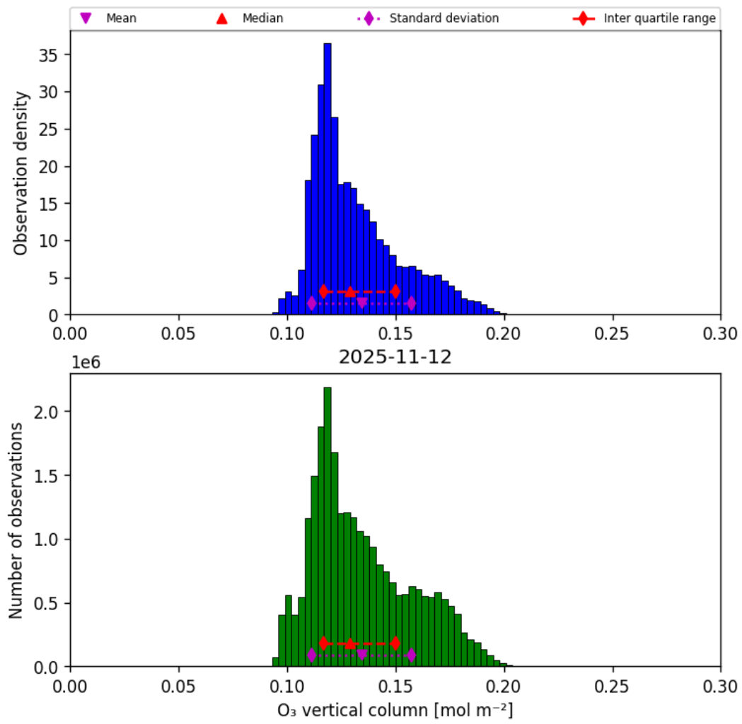
Figure 21: Histogram of “O 3 vertical column” for 2025-11-12 to 2025-11-13
