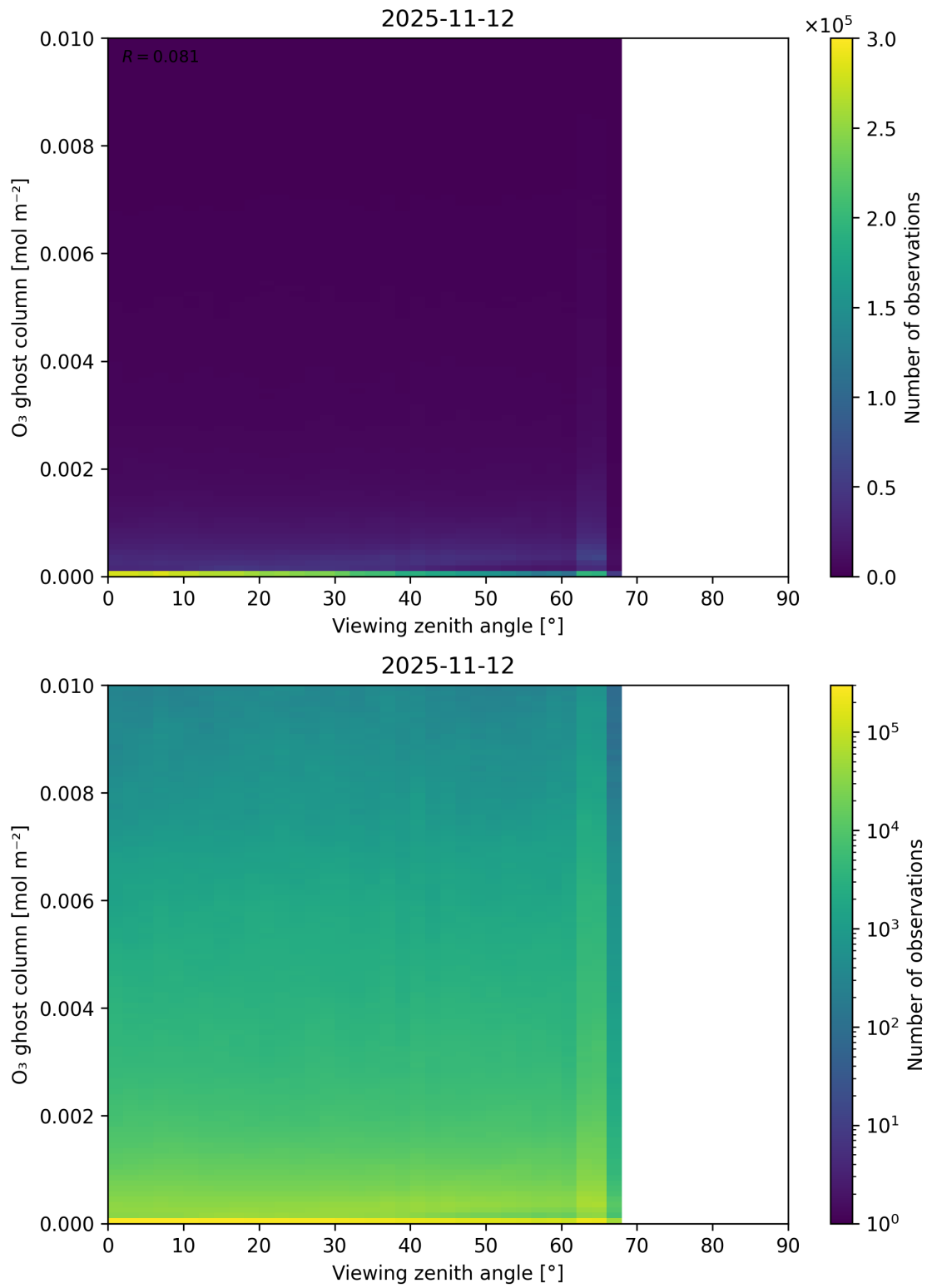
Figure 51: Scatter density plot of “Viewing zenith angle” against “O 3 ghost column” for 2025-11-12 to 2025-11-13.
