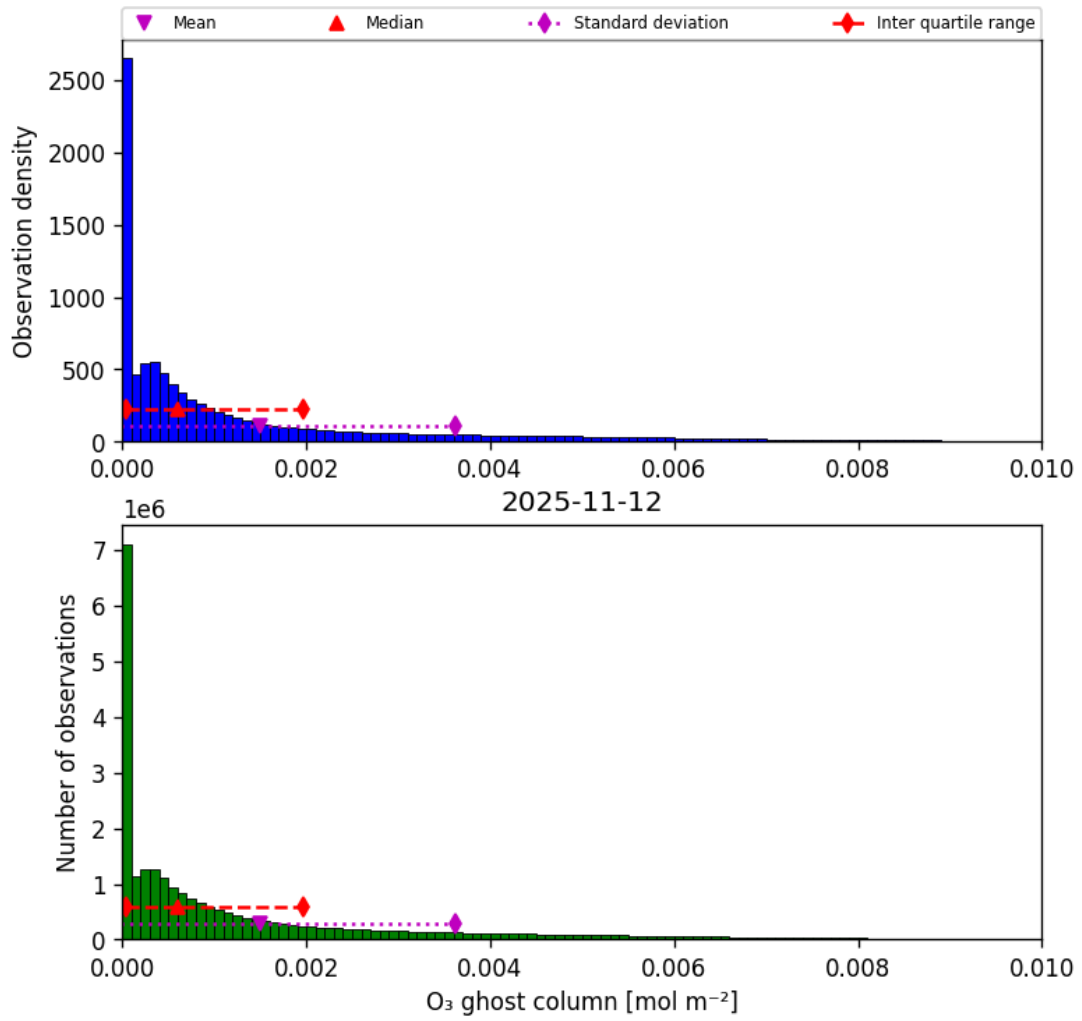
Figure 25: Histogram of “O 3 ghost column” for 2025-11-12 to 2025-11-13
