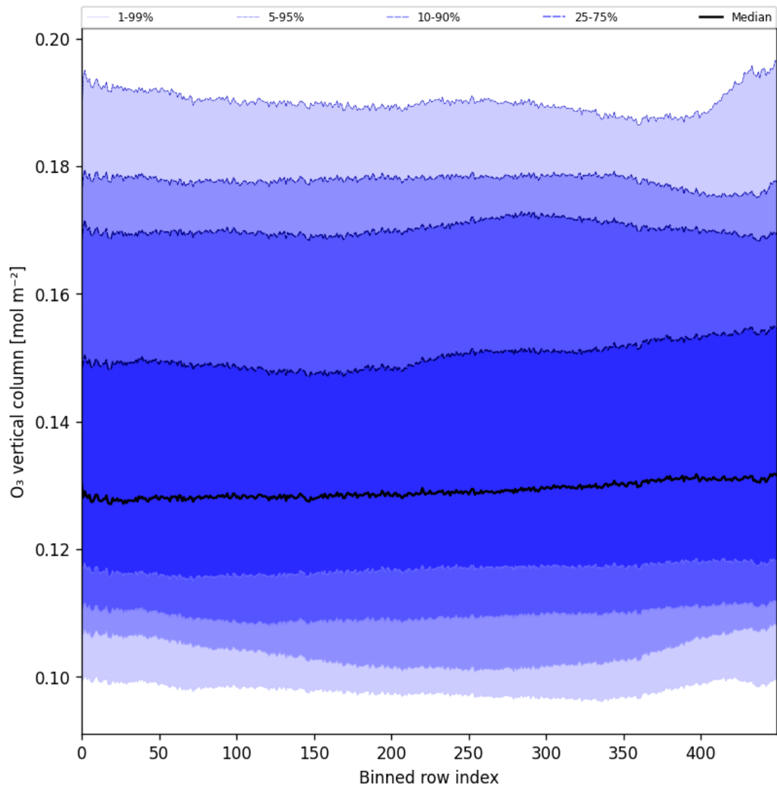
Figure 28: Along track statistics of “O 3 vertical column” for 2025-11-12 to 2025-11-13
