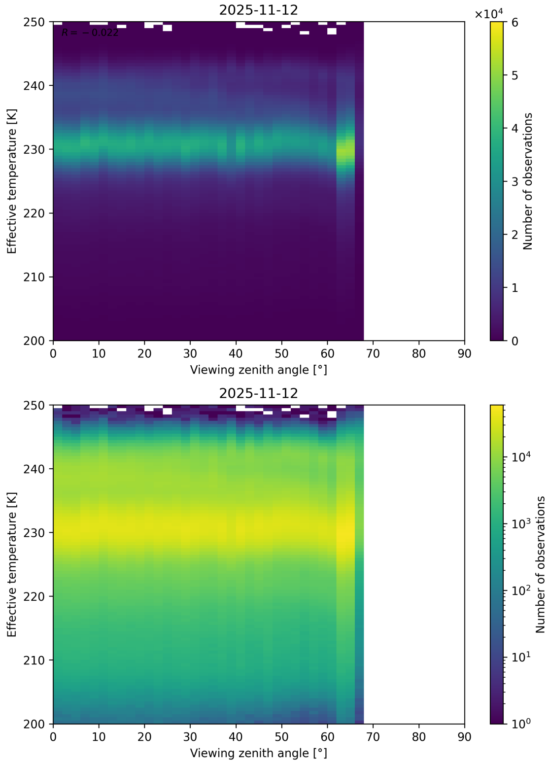
Figure 50: Scatter density plot of “Viewing zenith angle” against “Effective temperature” for 2025-11-12 to 2025-11-13.
