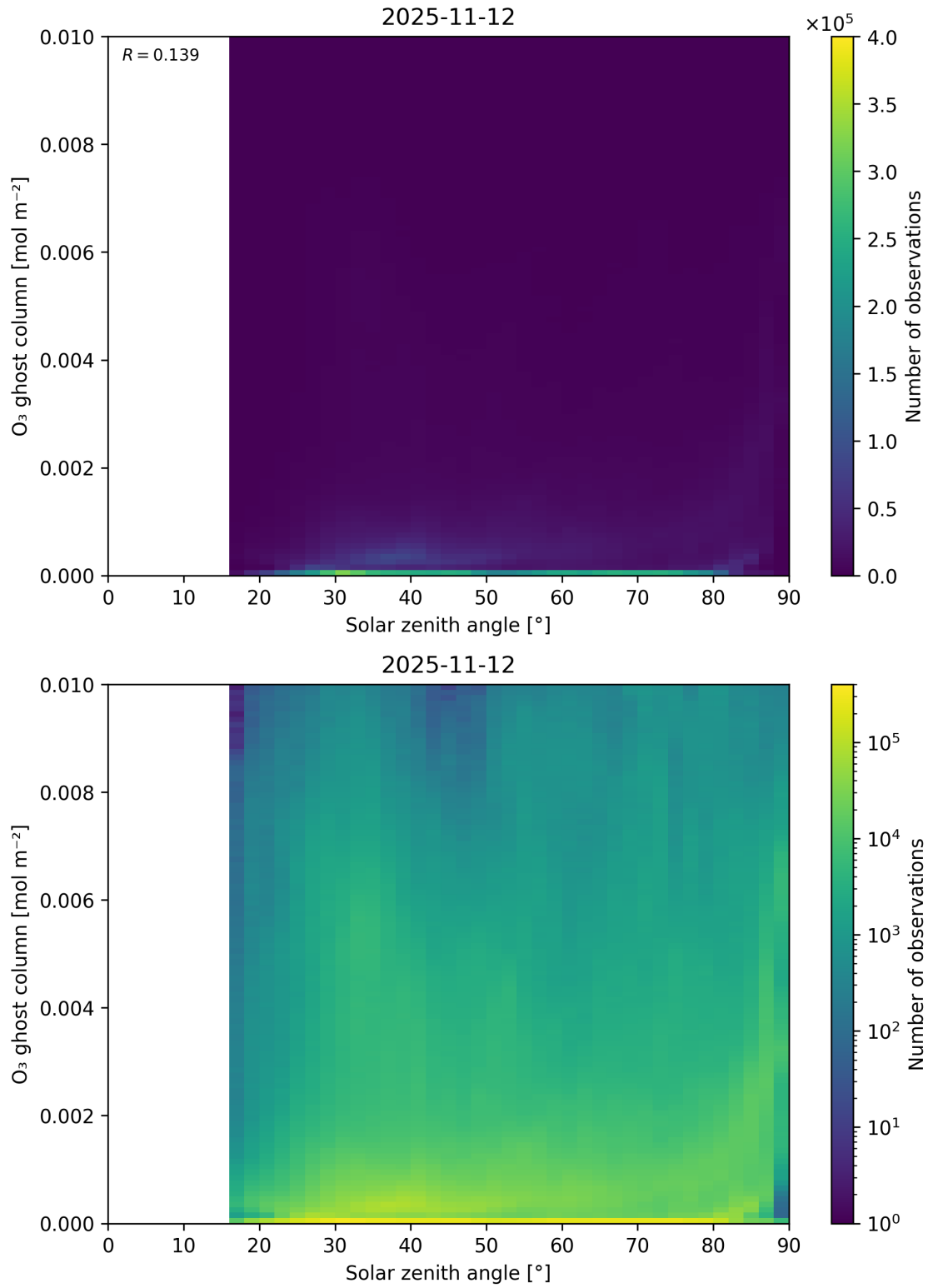
Figure 46: Scatter density plot of “Solar zenith angle” against “O 3 ghost column” for 2025-11-12 to 2025-11-13.
