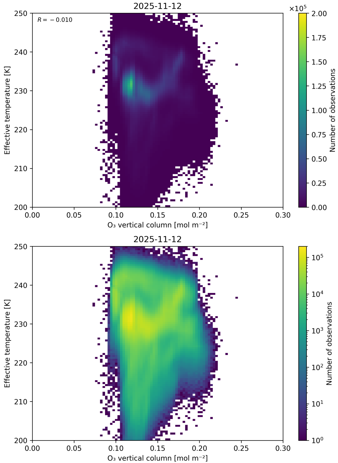
Figure 39: Scatter density plot of “O 3 vertical column” against “Effective temperature” for 2025-11-12 to 2025-11-13.
