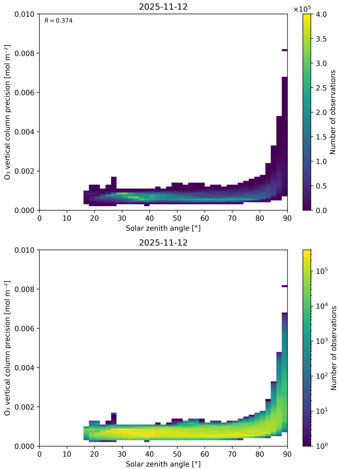
Figure 48: Scatter density plot of “Solar zenith angle” against “O 3 vertical column precision” for 2025-11-12 to 2025-11-13.
