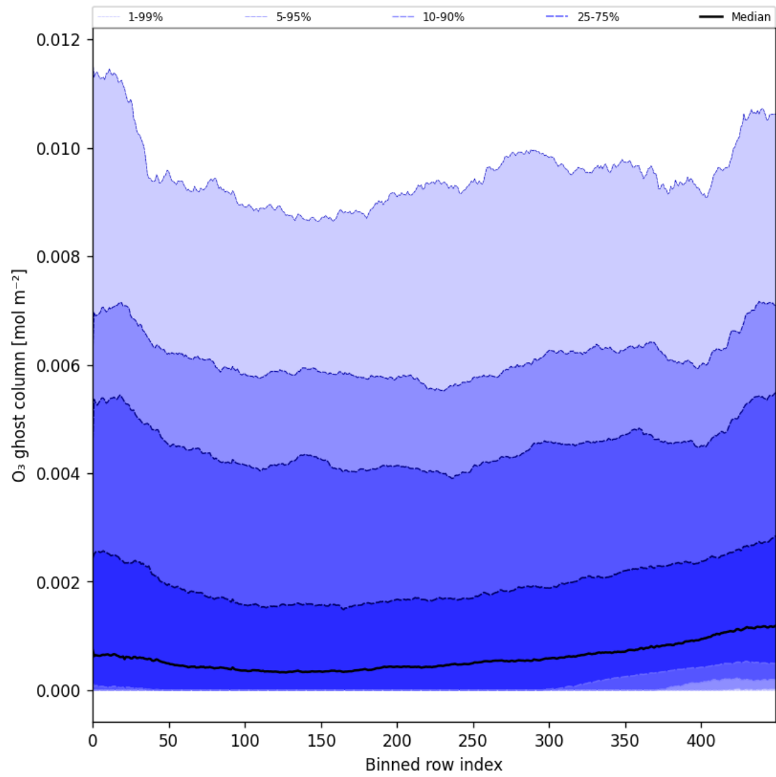
Figure 32: Along track statistics of “O 3 ghost column” for 2025-11-12 to 2025-11-13
