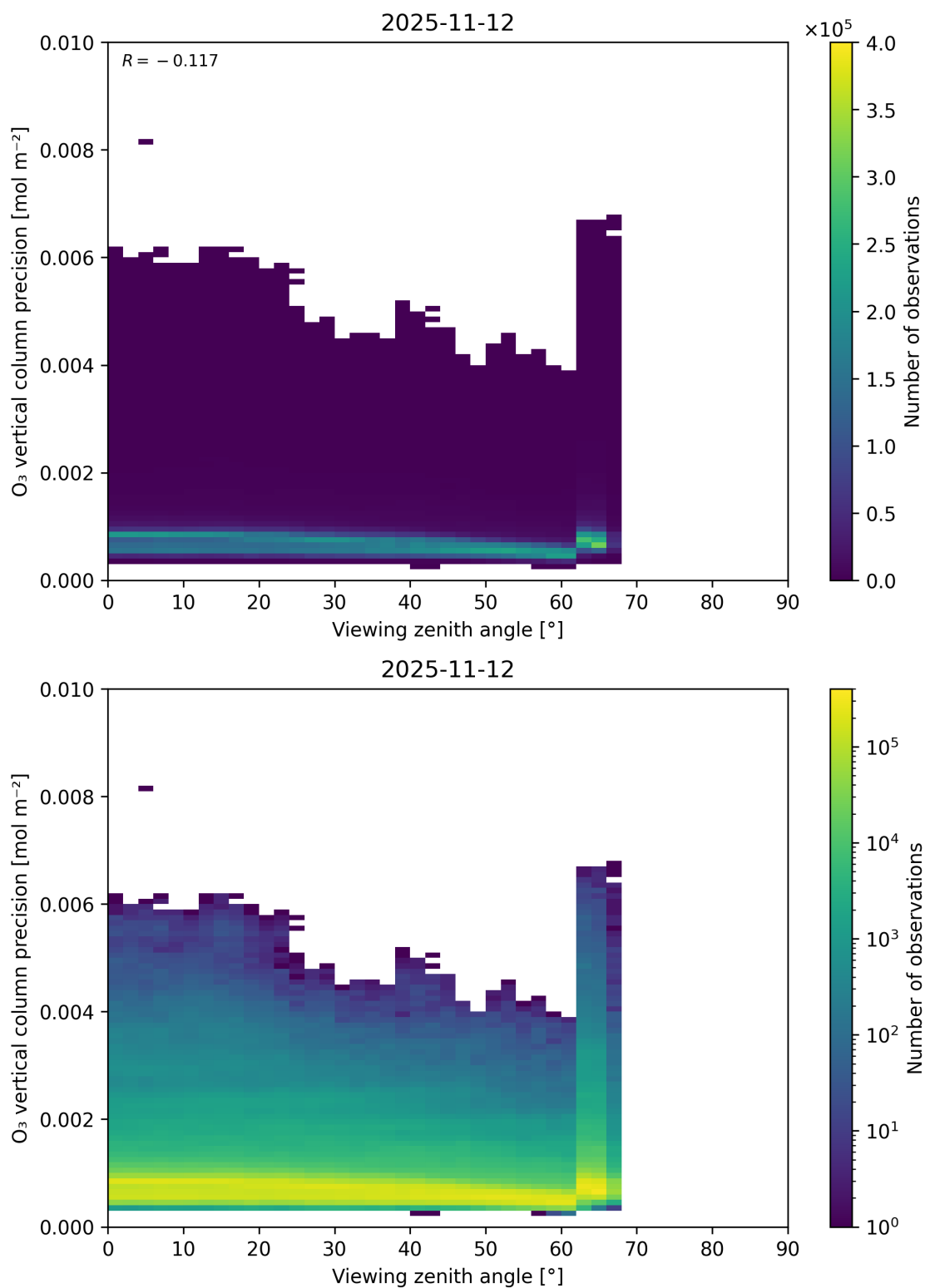
Figure 53: Scatter density plot of “Viewing zenith angle” against “O 3 vertical column precision” for 2025-11-12 to 2025-11-13.
