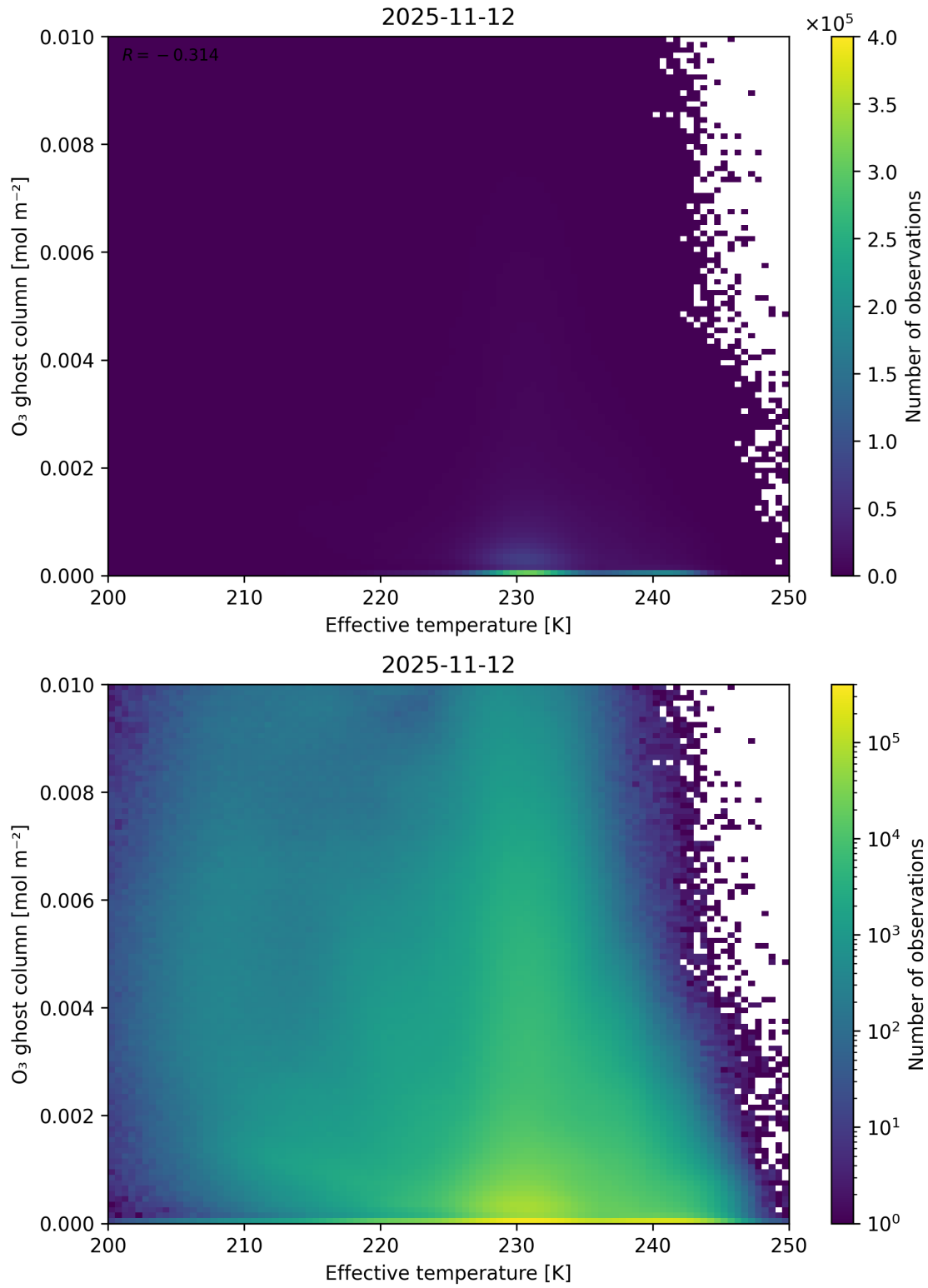
Figure 38: Scatter density plot of “Effective temperature” against “O 3 ghost column” for 2025-11-12 to 2025-11-13.
