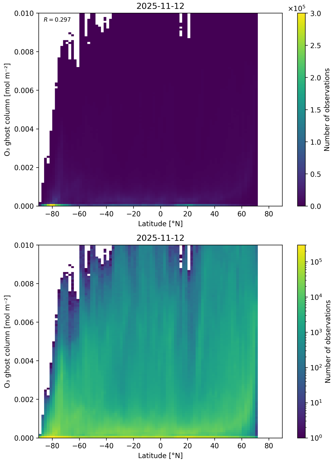
Figure 35: Scatter density plot of “Latitude” against “O 3 ghost column” for 2025-11-12 to 2025-11-13.
