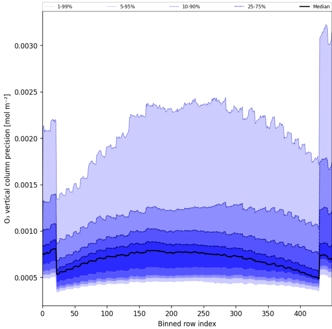
Figure 29: Along track statistics of “O 3 vertical column precision” for 2025-11-12 to 2025-11-13
