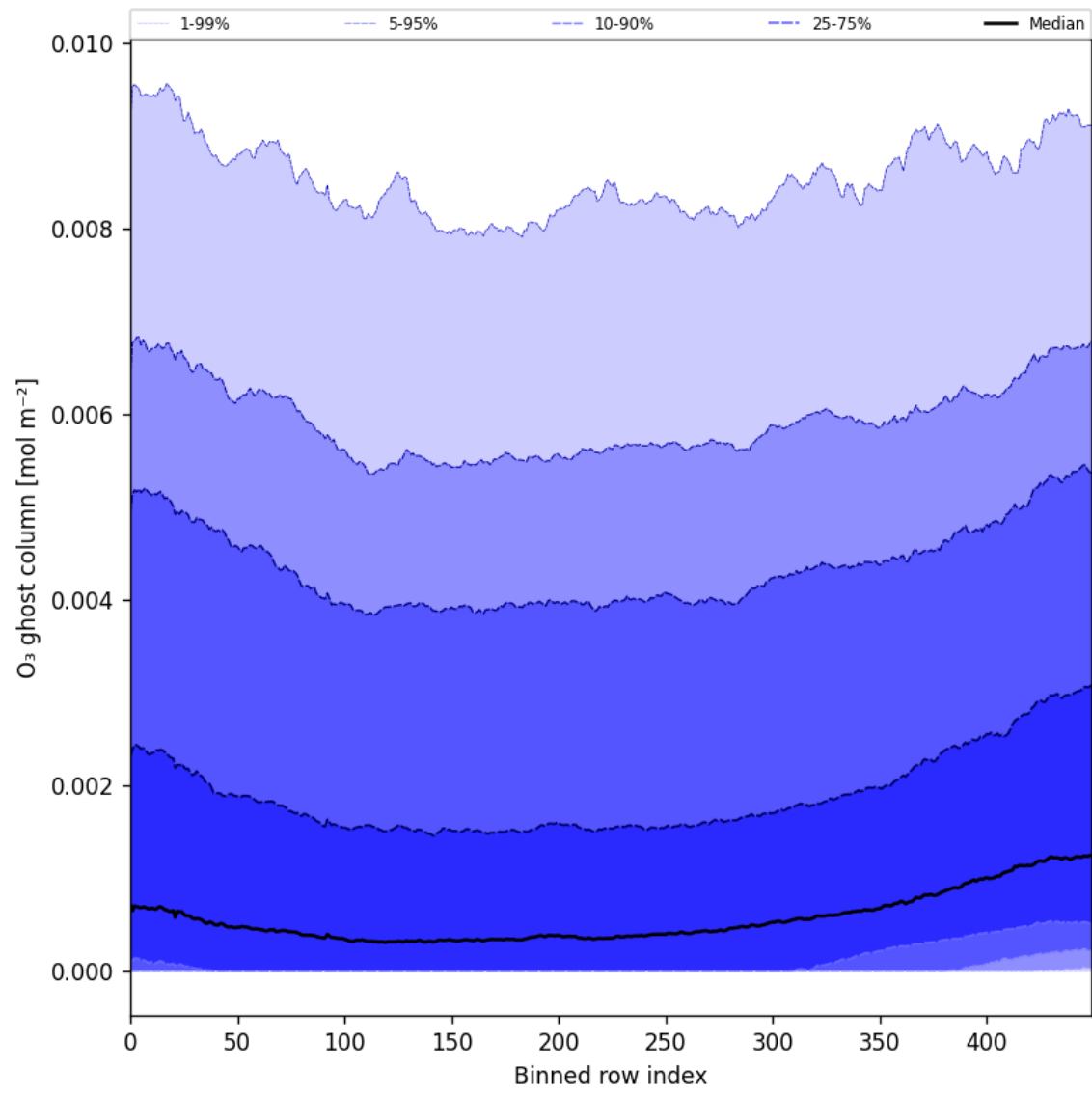
Figure 32: Along track statistics of “O 3 ghost column” for 2025-11-12 to 2025-11-14
