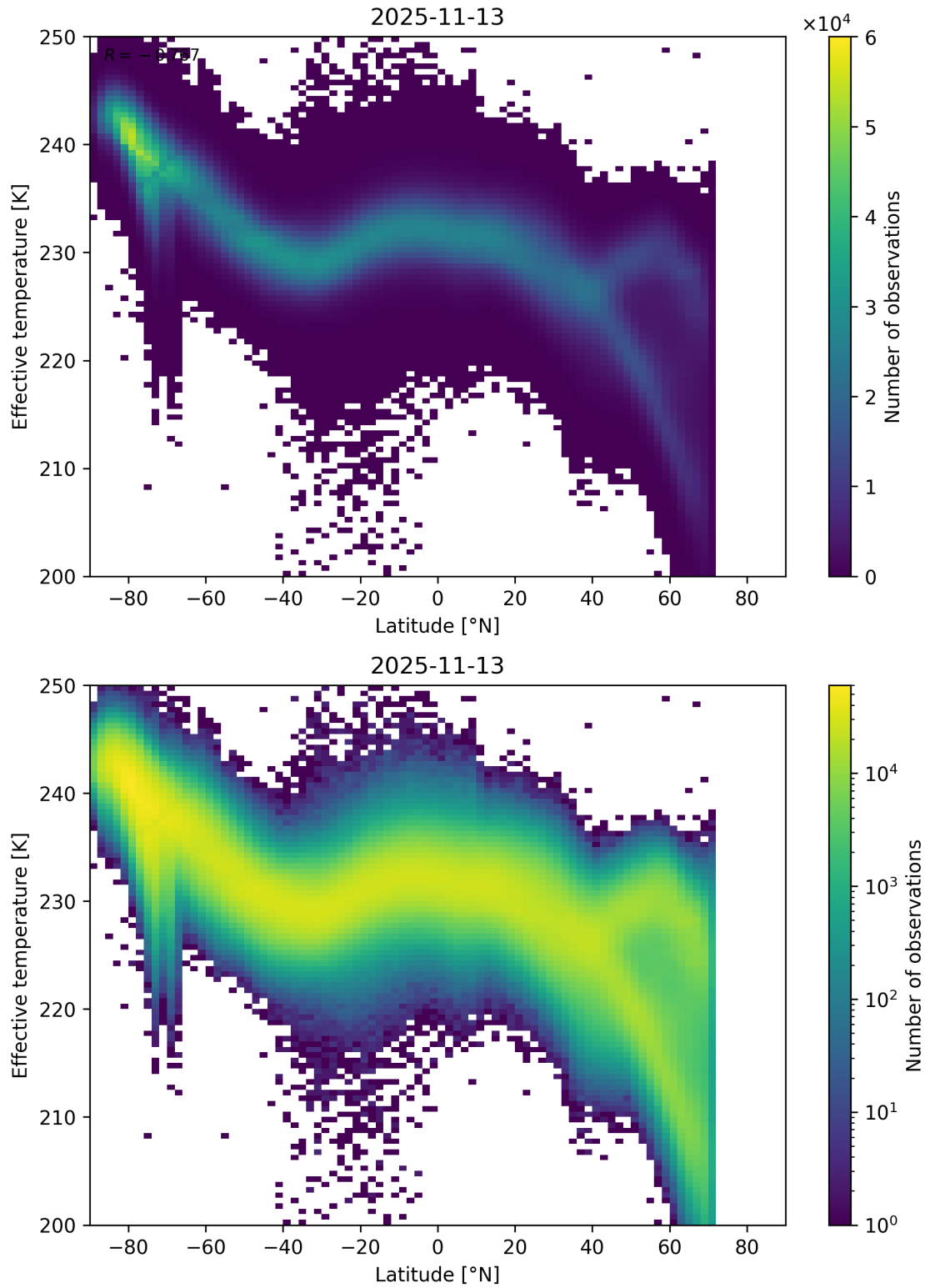
Figure 34: Scatter density plot of “Latitude” against “Effective temperature” for 2025-11-12 to 2025-11-14.
