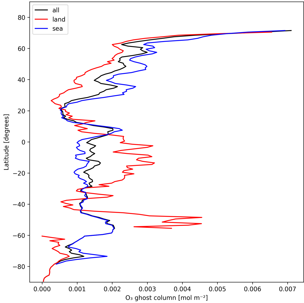
Figure 18: Zonal average of "O 3 ghost column" for 2025-11-12 to 2025-11-14.
