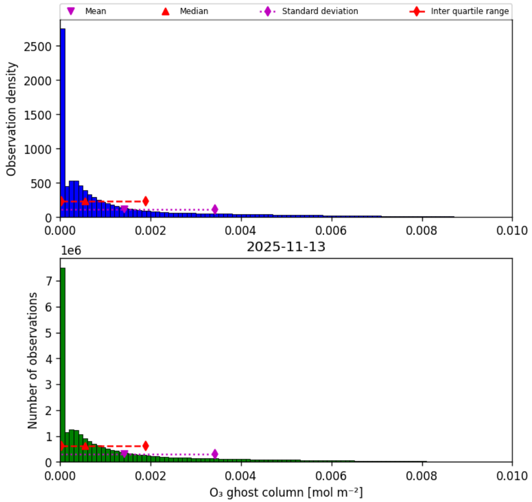
Figure 25: Histogram of "O 3 ghost column" for 2025-11-12 to 2025-11-14
