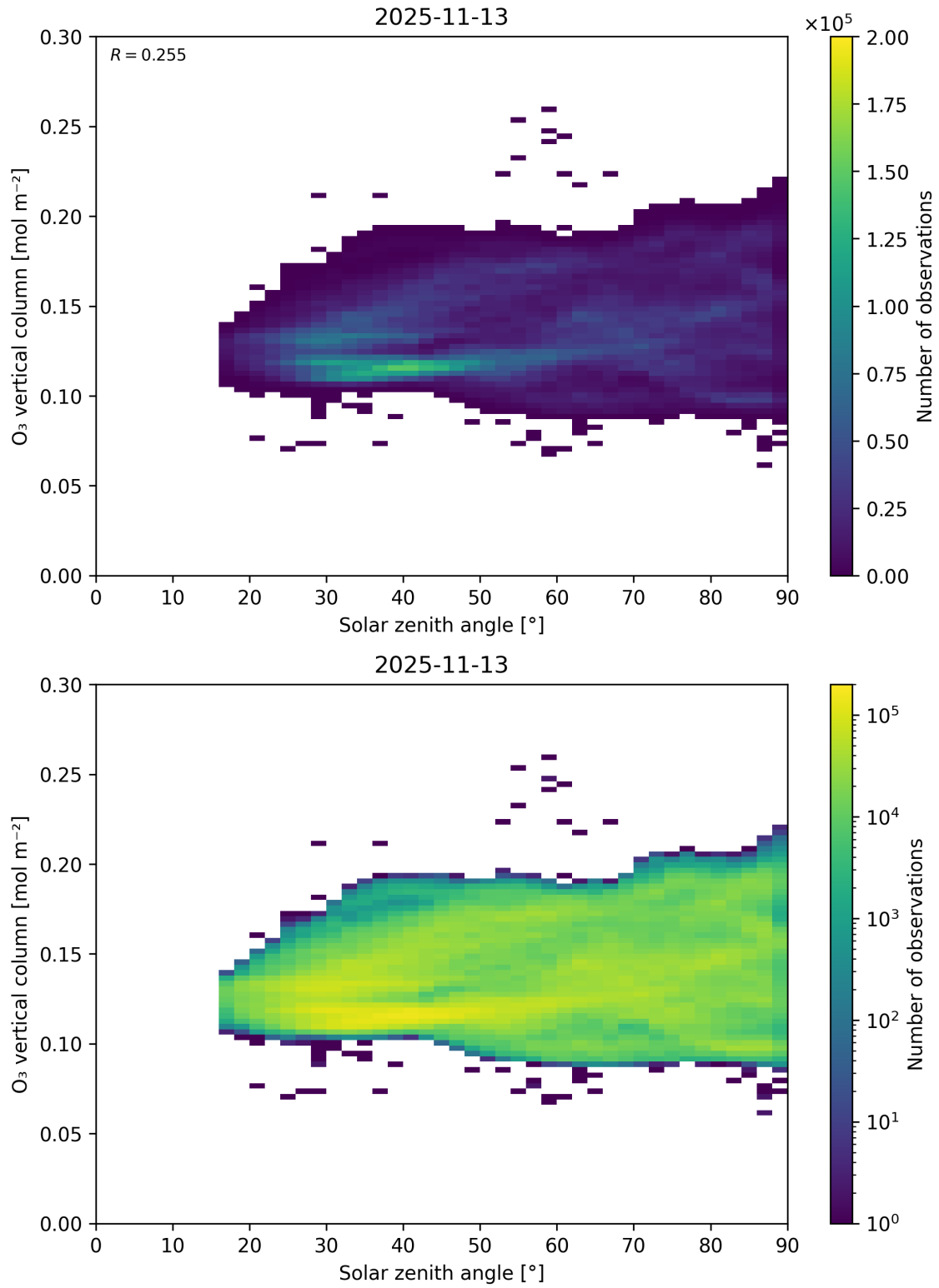
Figure 47: Scatter density plot of “Solar zenith angle” against “O 3 vertical column” for 2025-11-12 to 2025-11-14.
