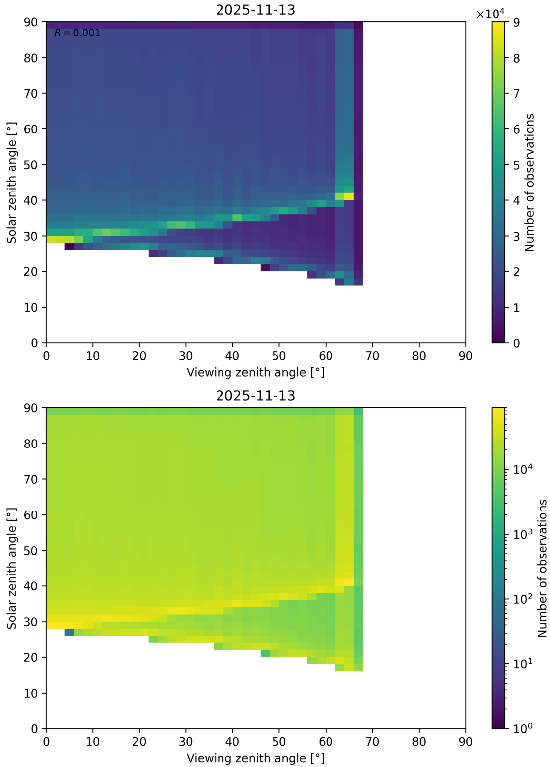
Figure 54: Scatter density plot of “Viewing zenith angle” against “Solar zenith angle” for 2025-11-12 to 2025-11-14.
