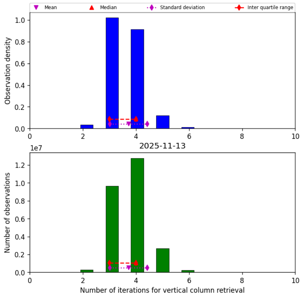
Figure 26: Histogram of “Number of iterations for vertical column retrieval” for 2025-11-12 to 2025-11-14
