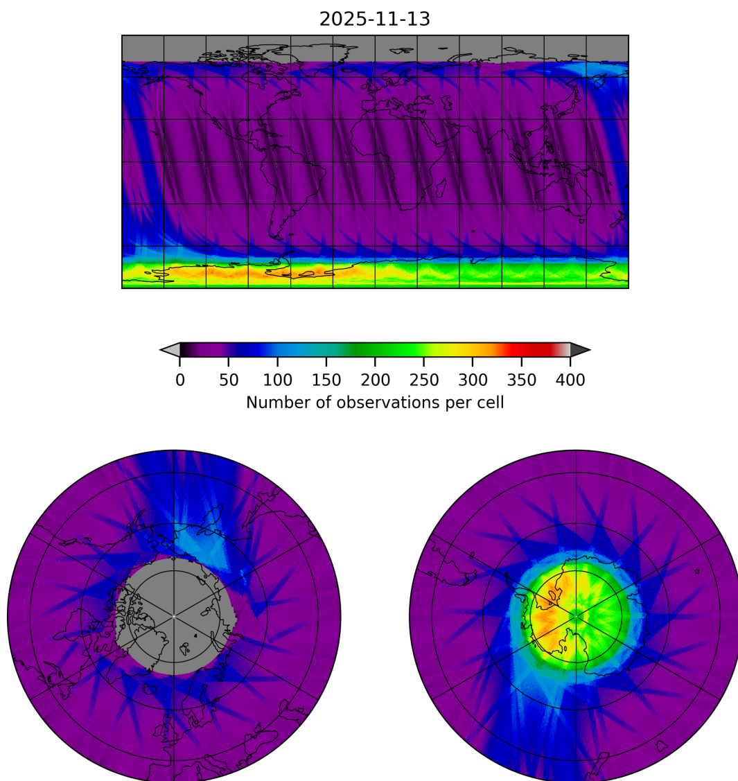
Figure 12: Map of the number of observations for 2025-11-12 to 2025-11-14
