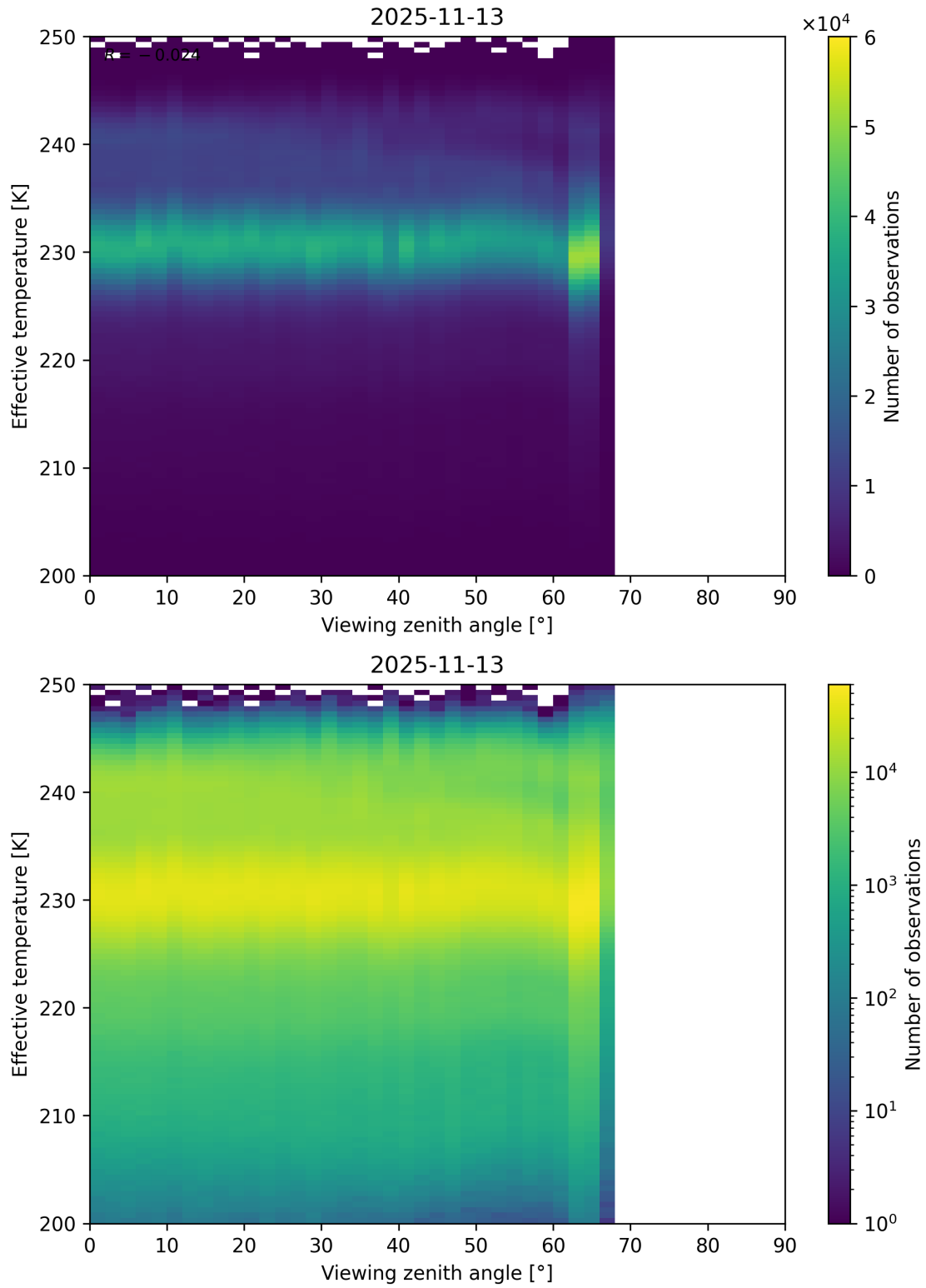
Figure 50: Scatter density plot of “Viewing zenith angle” against “Effective temperature” for 2025-11-12 to 2025-11-14.
