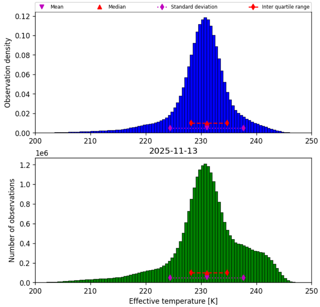
Figure 24: Histogram of “Effective temperature” for 2025-11-12 to 2025-11-14
