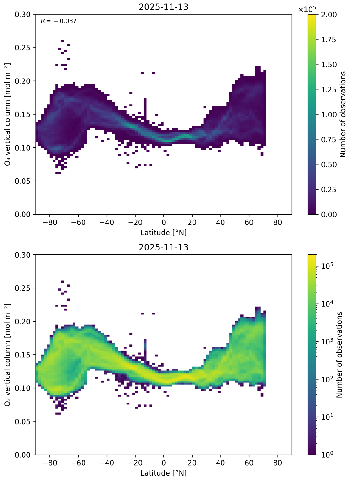
Figure 36: Scatter density plot of “Latitude” against “O 3 vertical column” for 2025-11-12 to 2025-11-14.
