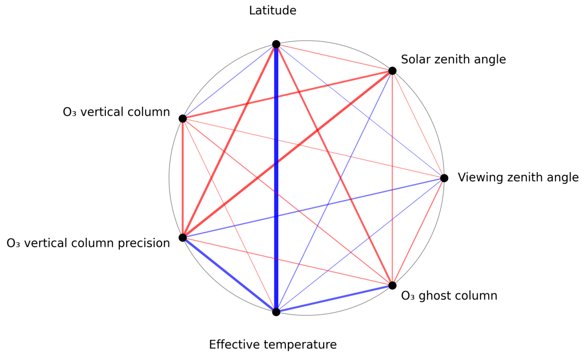
Figure 1: Map of correlation graph for 2025-11-12 to 2025-11-14.
