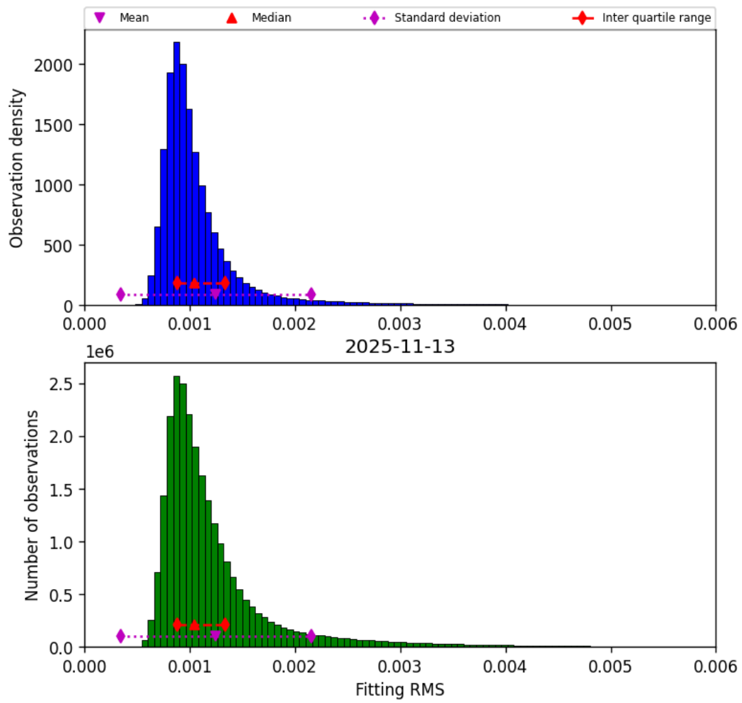
Figure 23: Histogram of “Fitting RMS” for 2025-11-12 to 2025-11-14
