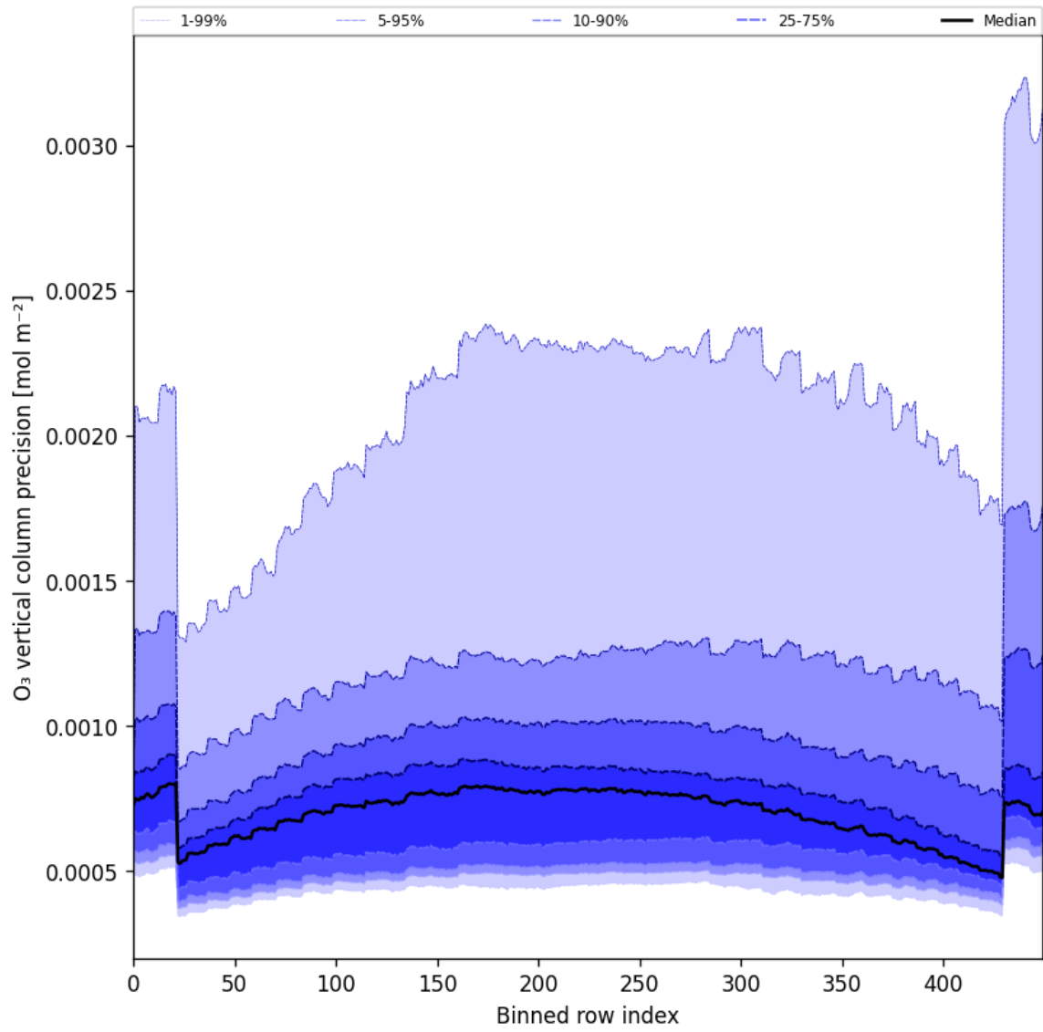
Figure 29: Along track statistics of “O 3 vertical column precision” for 2025-11-12 to 2025-11-14
