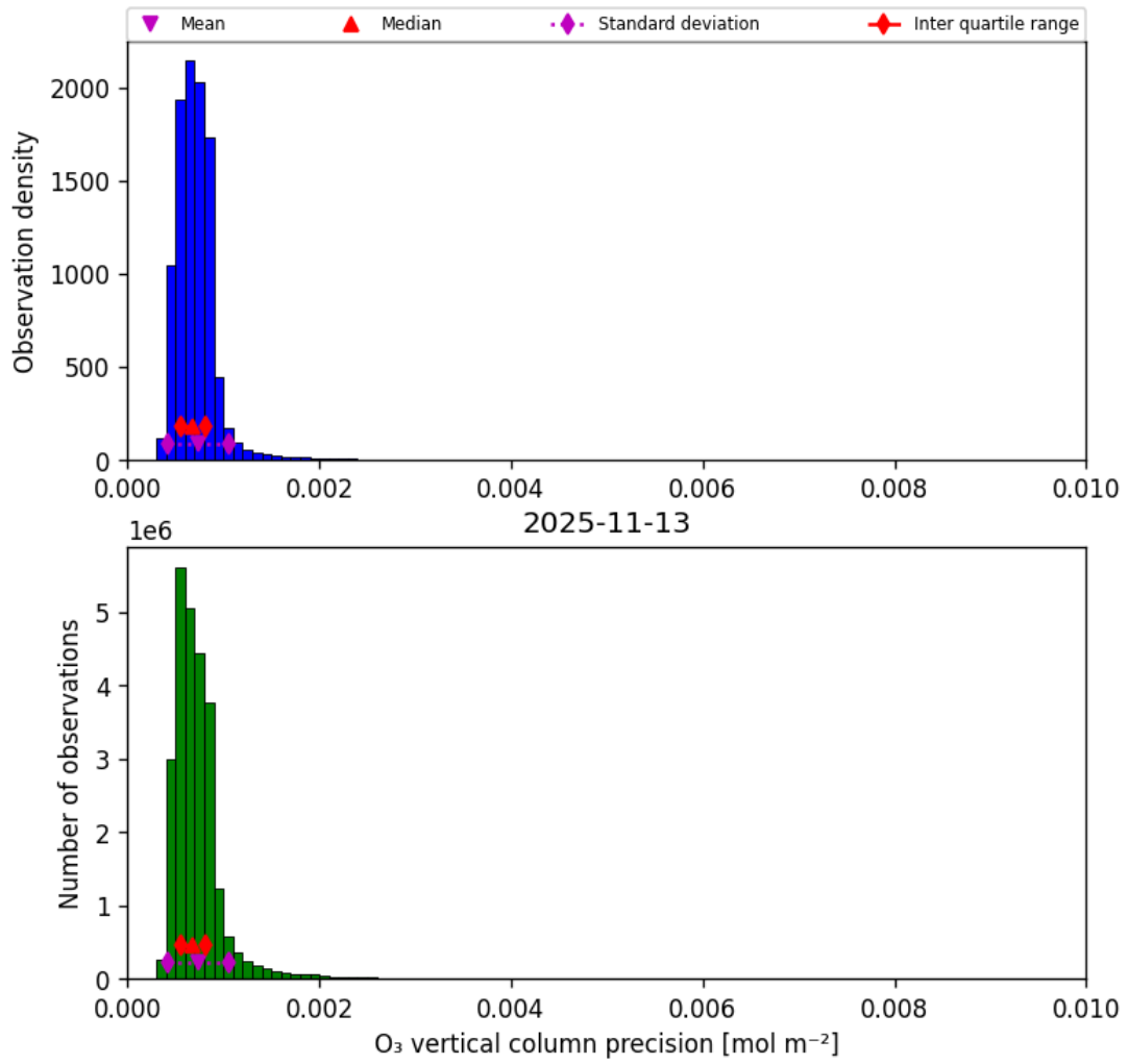
Figure 22: Histogram of “O 3 vertical column precision” for 2025-11-12 to 2025-11-14
