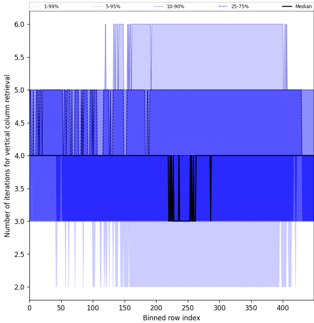
Figure 33: Along track statistics of “Number of iterations for vertical column retrieval” for 2025-11-12 to 2025-11-14
