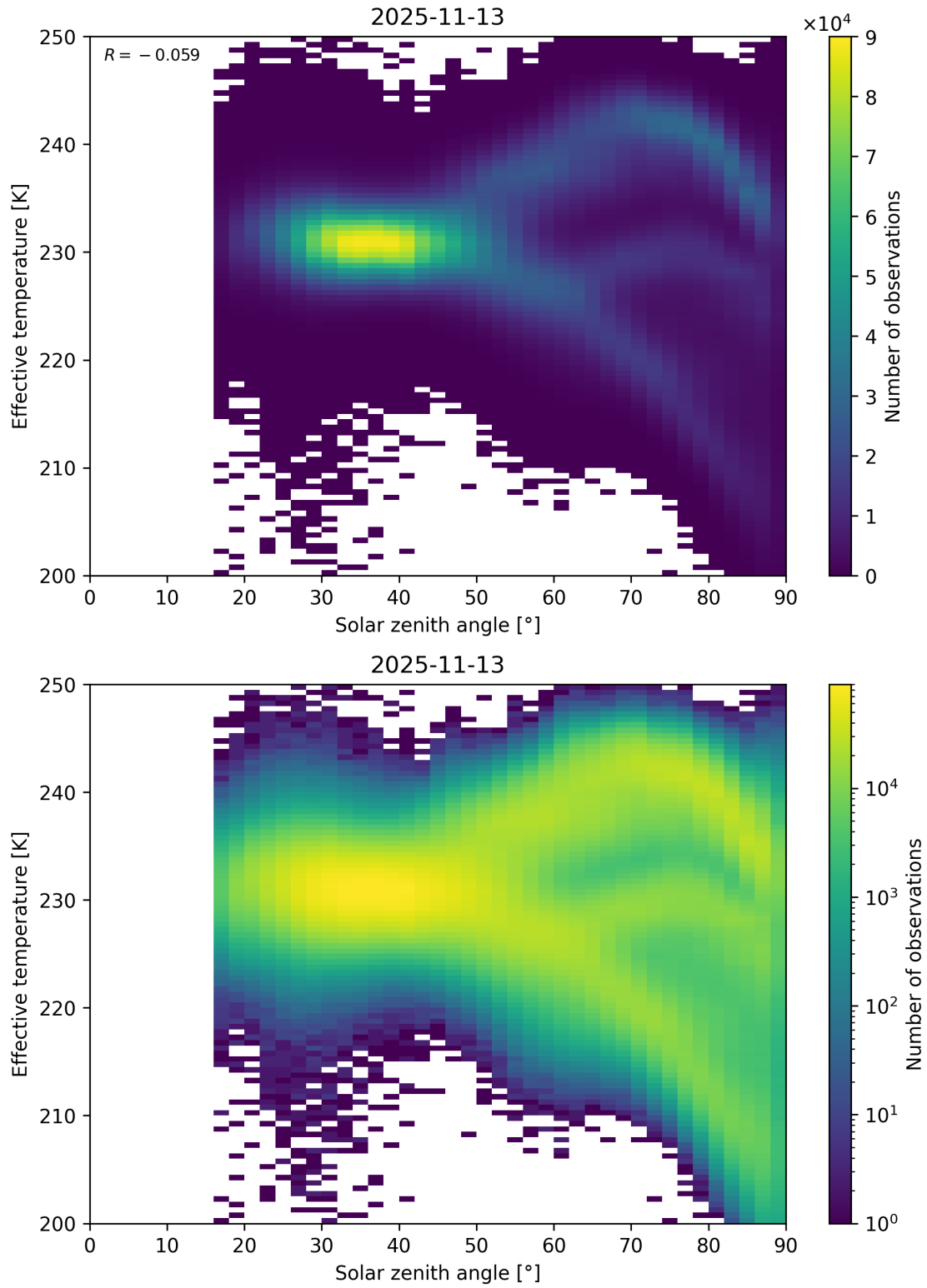
Figure 45: Scatter density plot of “Solar zenith angle” against “Effective temperature” for 2025-11-12 to 2025-11-14.
