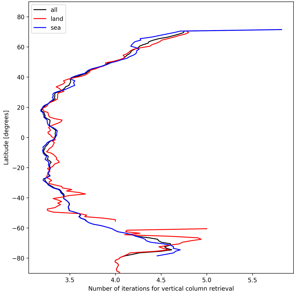
Figure 19: Zonal average of “Number of iterations for vertical column retrieval” for 2025-11-12 to 2025-11-14.
