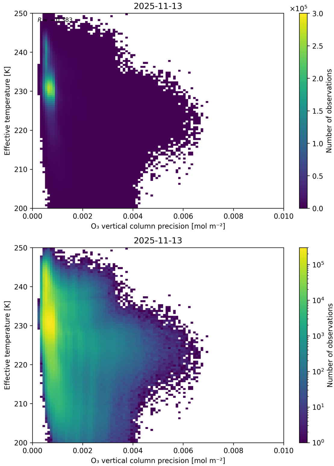
Figure 42: Scatter density plot of “O 3 vertical column precision” against “Effective temperature” for 2025-11-12 to 2025-11-14.
