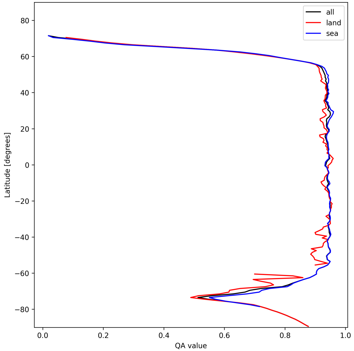
Figure 13: Zonal average of “QA value” for 2025-11-12 to 2025-11-14.
