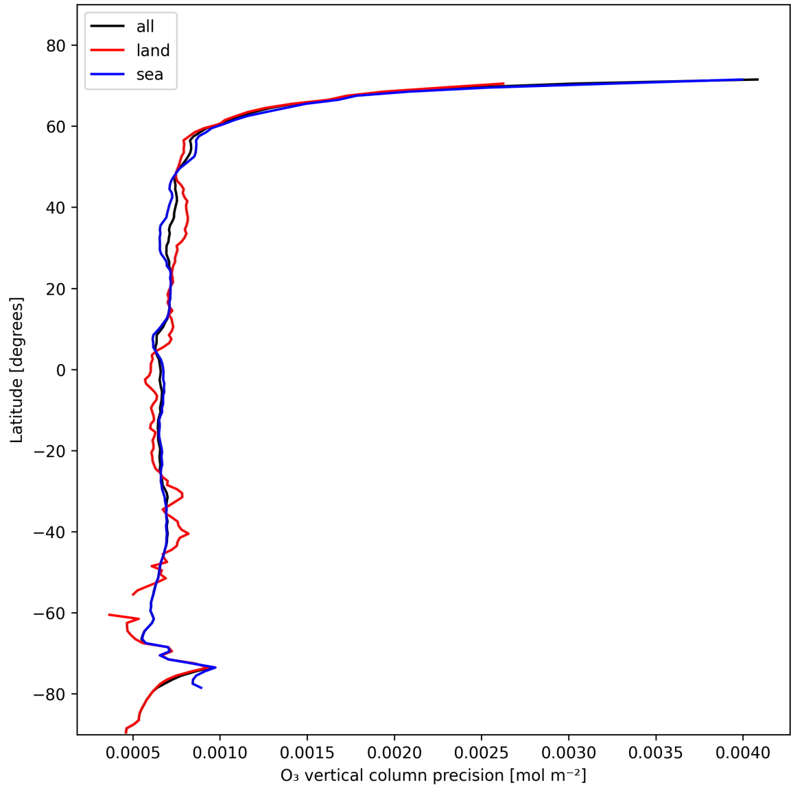
Figure 15: Zonal average of “O 3 vertical column precision” for 2025-11-12 to 2025-11-14.
