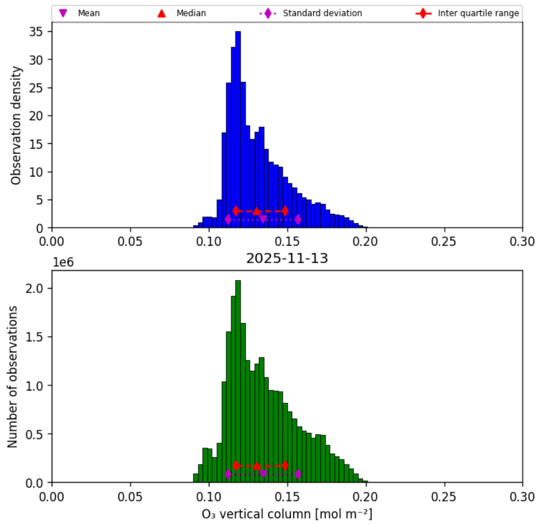
Figure 21: Histogram of “O 3 vertical column” for 2025-11-12 to 2025-11-14
