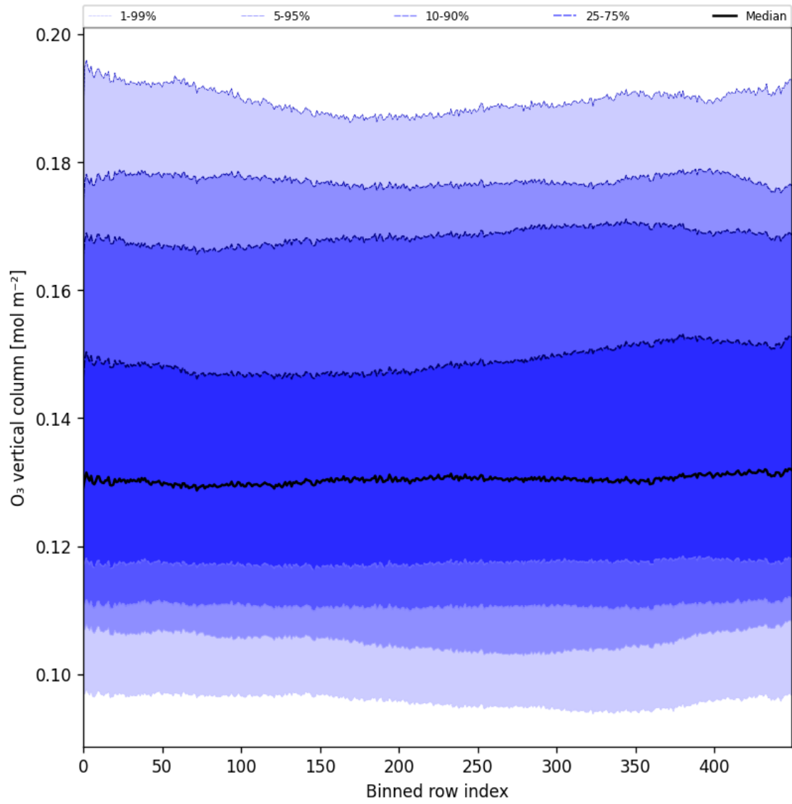
Figure 28: Along track statistics of “O 3 vertical column” for 2025-11-12 to 2025-11-14
