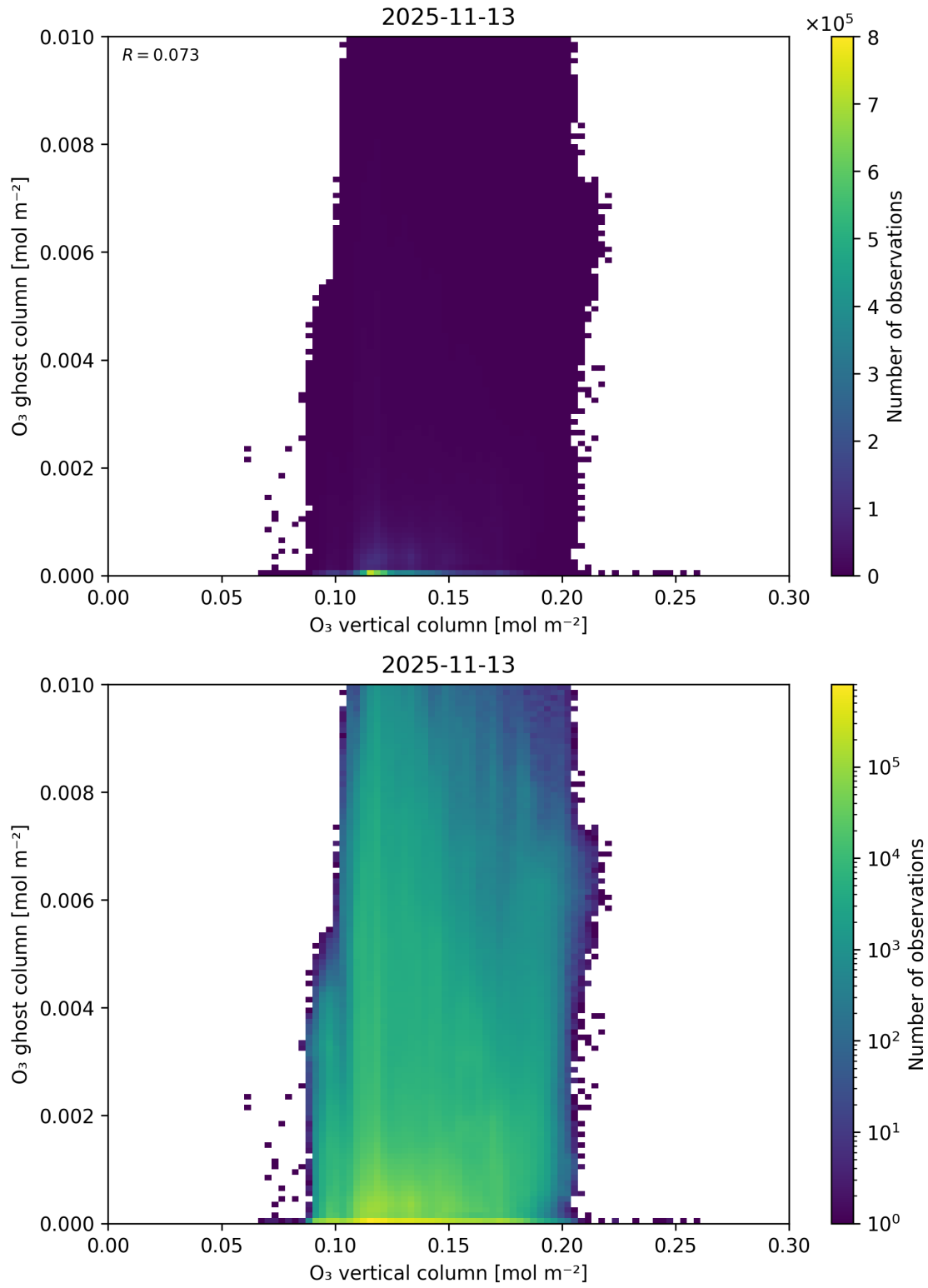
Figure 40: Scatter density plot of “O 3 vertical column” against “O 3 ghost column” for 2025-11-12 to 2025-11-14.
