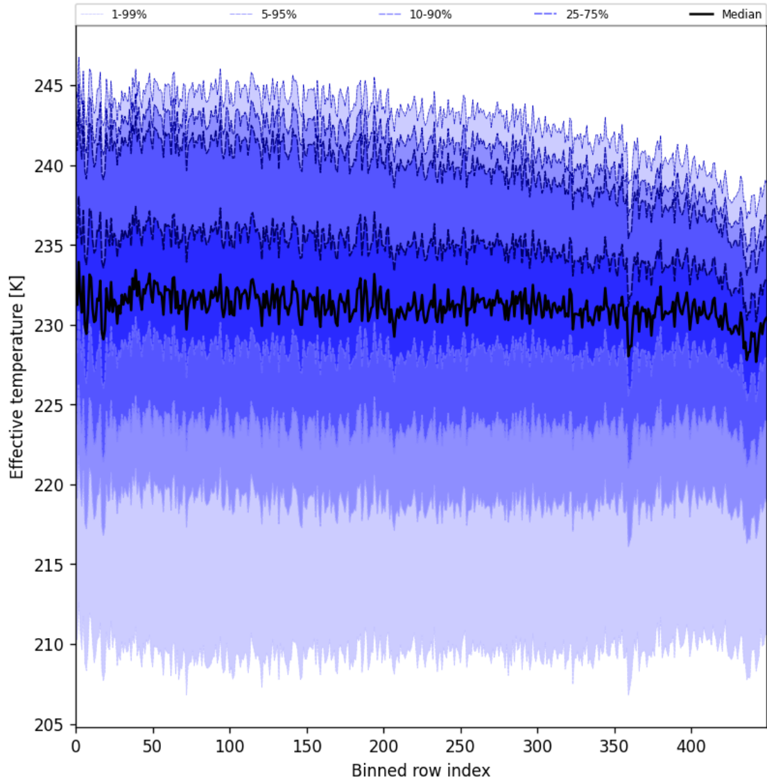
Figure 31: Along track statistics of “Effective temperature” for 2025-11-12 to 2025-11-14
