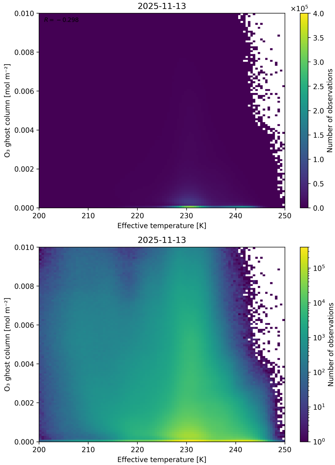
Figure 38: Scatter density plot of “Effective temperature” against “O 3 ghost column” for 2025-11-12 to 2025-11-14.
