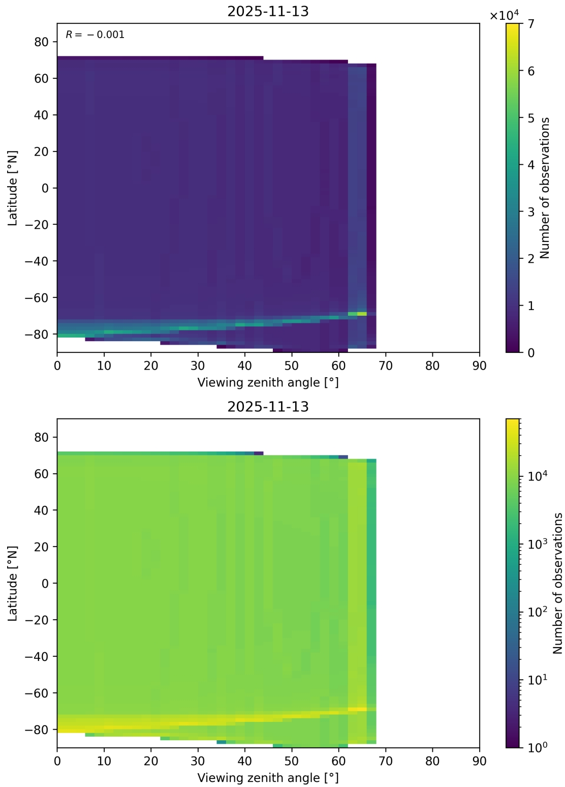
Figure 49: Scatter density plot of “Viewing zenith angle” against “Latitude” for 2025-11-12 to 2025-11-14.
