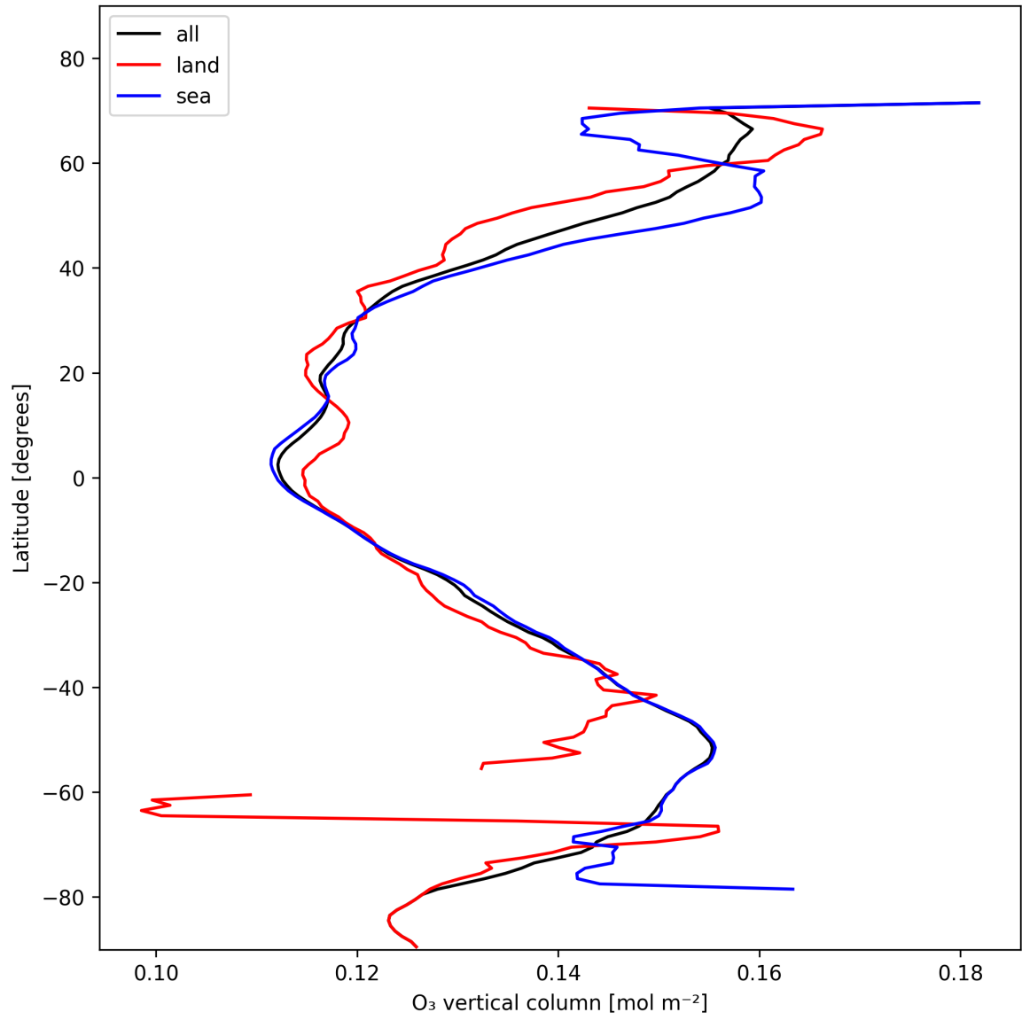
Figure 14: Zonal average of “O 3 vertical column” for 2025-11-12 to 2025-11-14.
