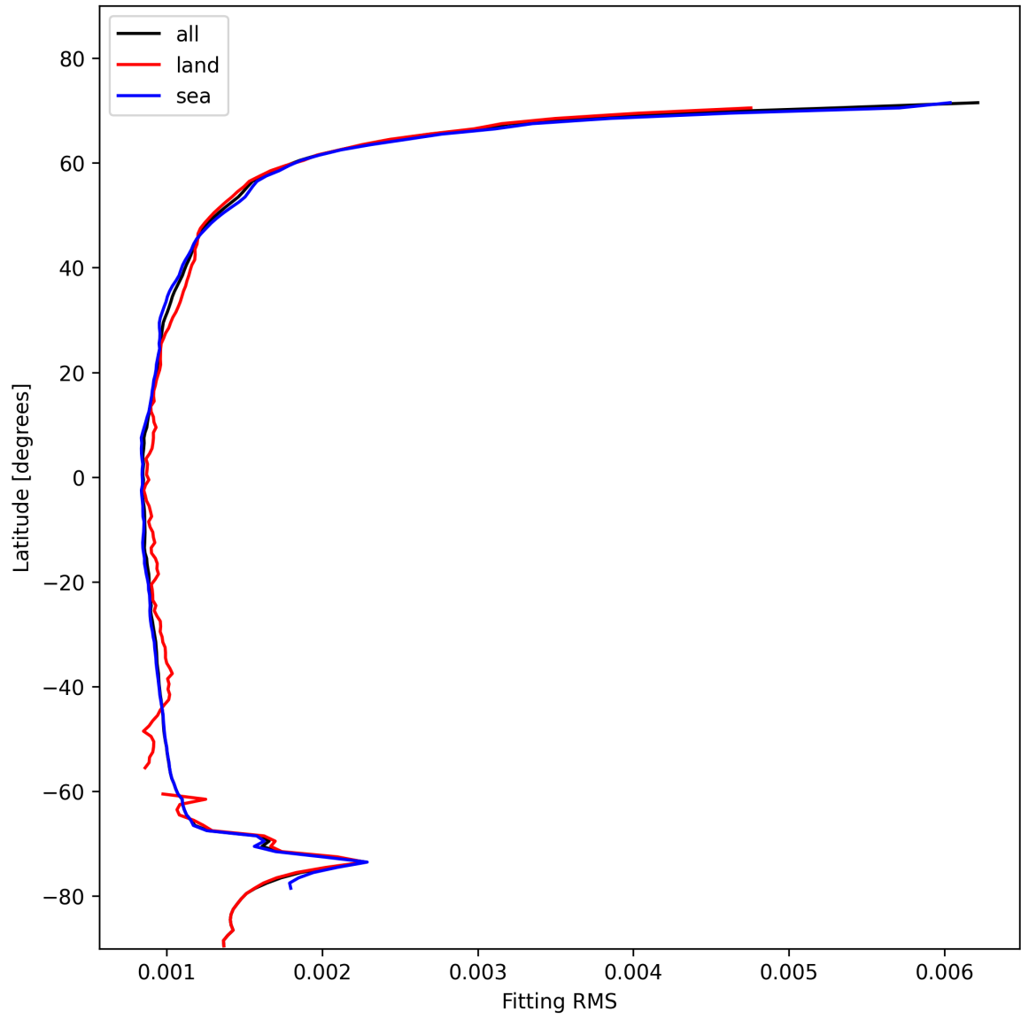
Figure 16: Zonal average of “Fitting RMS” for 2025-11-12 to 2025-11-14.
