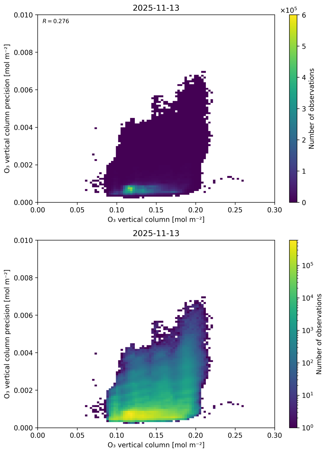
Figure 41: Scatter density plot of “O 3 vertical column” against “O 3 vertical column precision” for 2025-11-12 to 2025-11-14.
