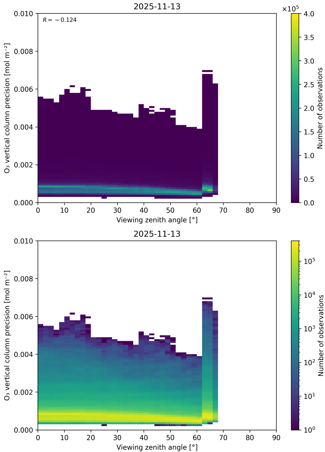
Figure 53: Scatter density plot of “Viewing zenith angle” against “O 3 vertical column precision” for 2025-11-12 to 2025-11-14.
