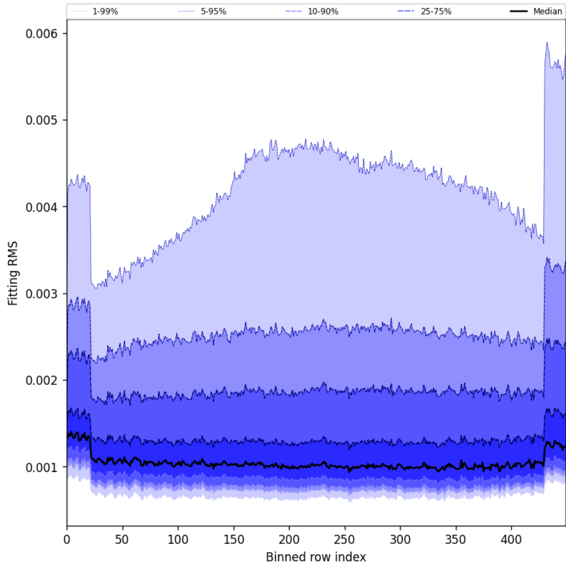
Figure 30: Along track statistics of “Fitting RMS” for 2025-11-12 to 2025-11-14
