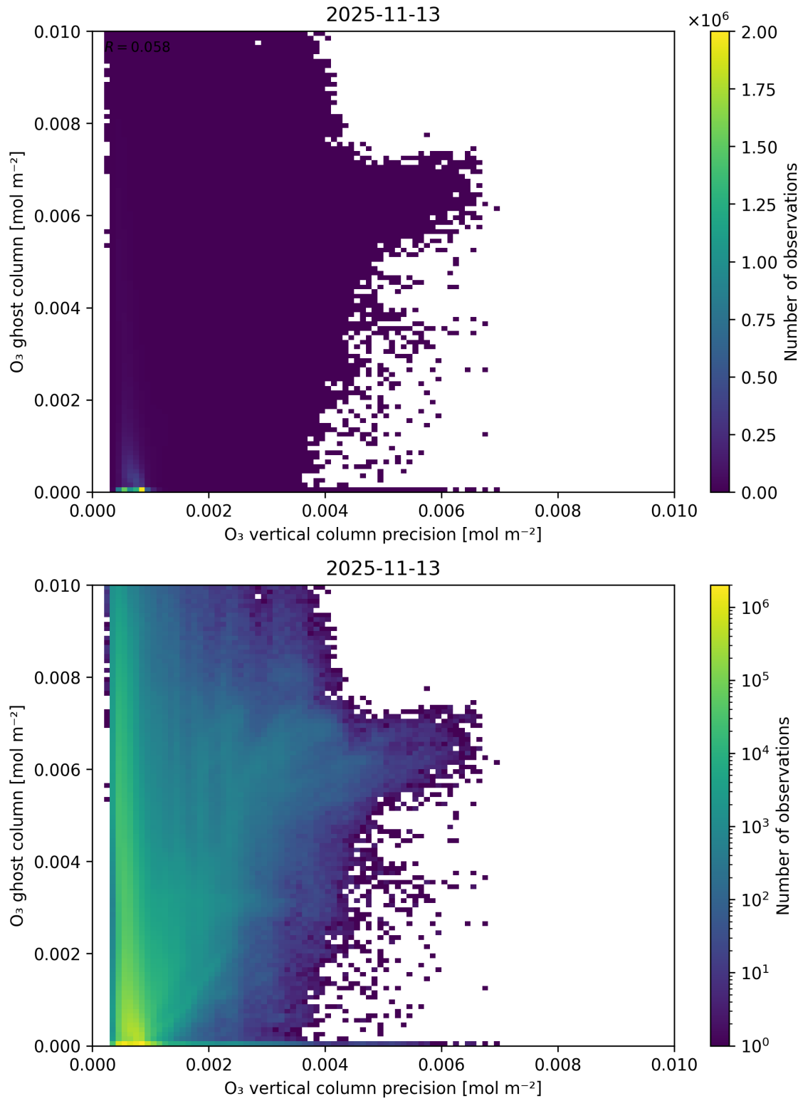
Figure 43: Scatter density plot of “ \text{O}_3 vertical column precision” against “ \text{O}_3 ghost column” for 2025-11-12 to 2025-11-14.
