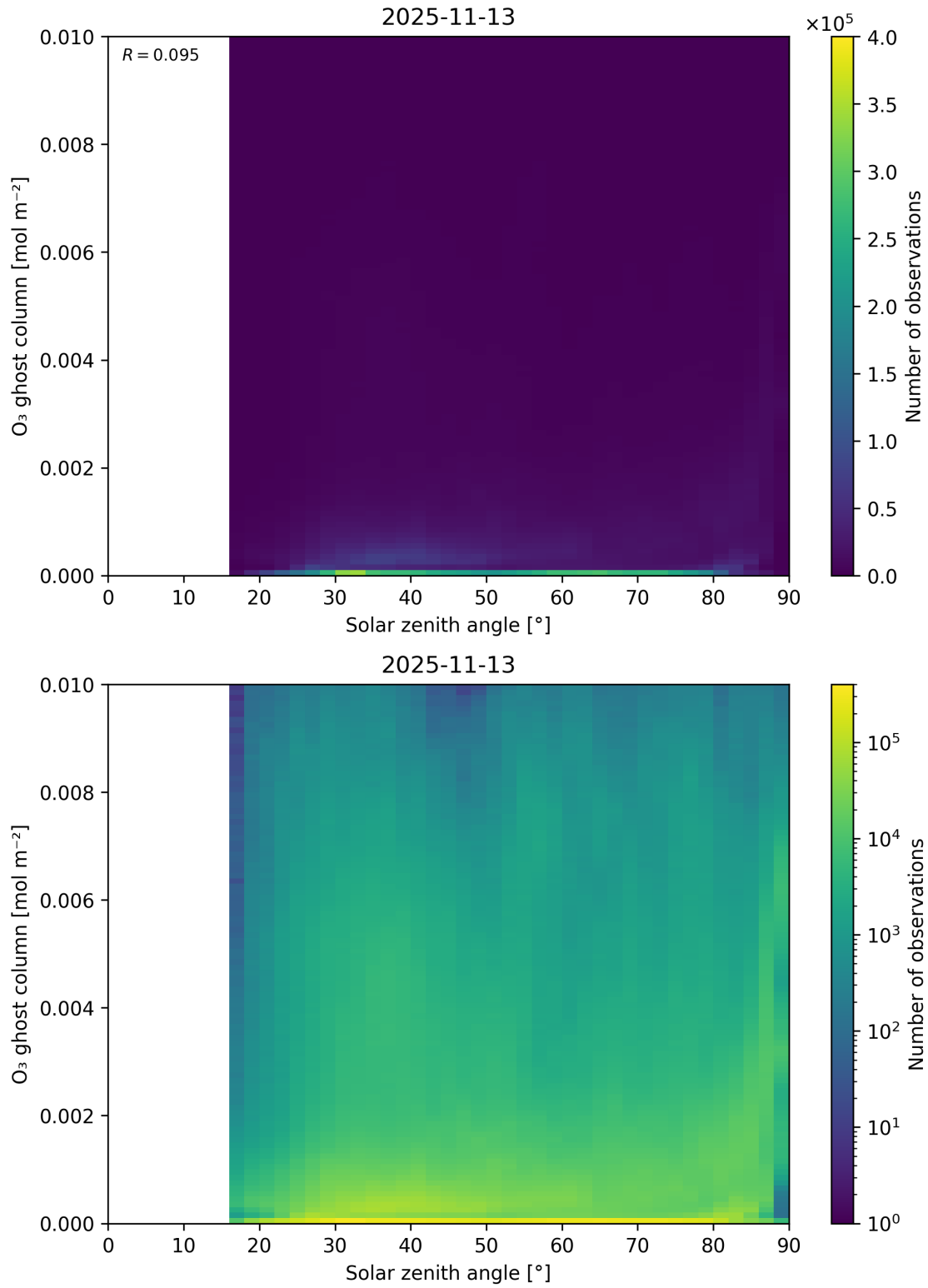
Figure 46: Scatter density plot of “Solar zenith angle” against “O 3 ghost column” for 2025-11-12 to 2025-11-14.
