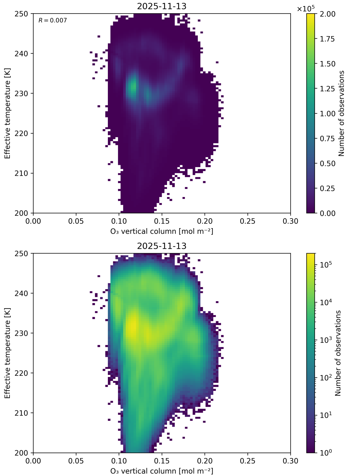
Figure 39: Scatter density plot of “O 3 vertical column” against “Effective temperature” for 2025-11-12 to 2025-11-14.
