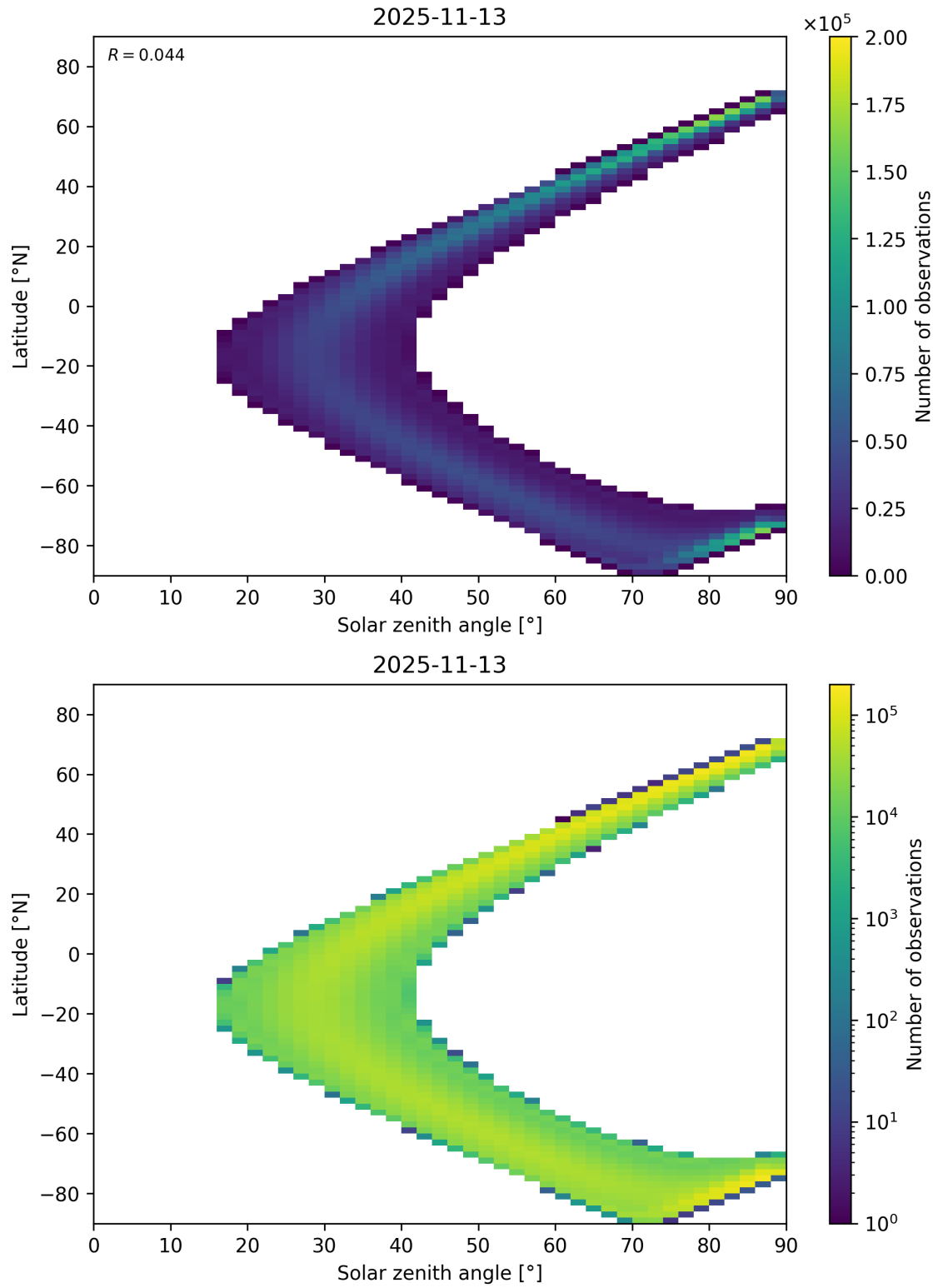
Figure 44: Scatter density plot of “Solar zenith angle” against “Latitude” for 2025-11-12 to 2025-11-14.
