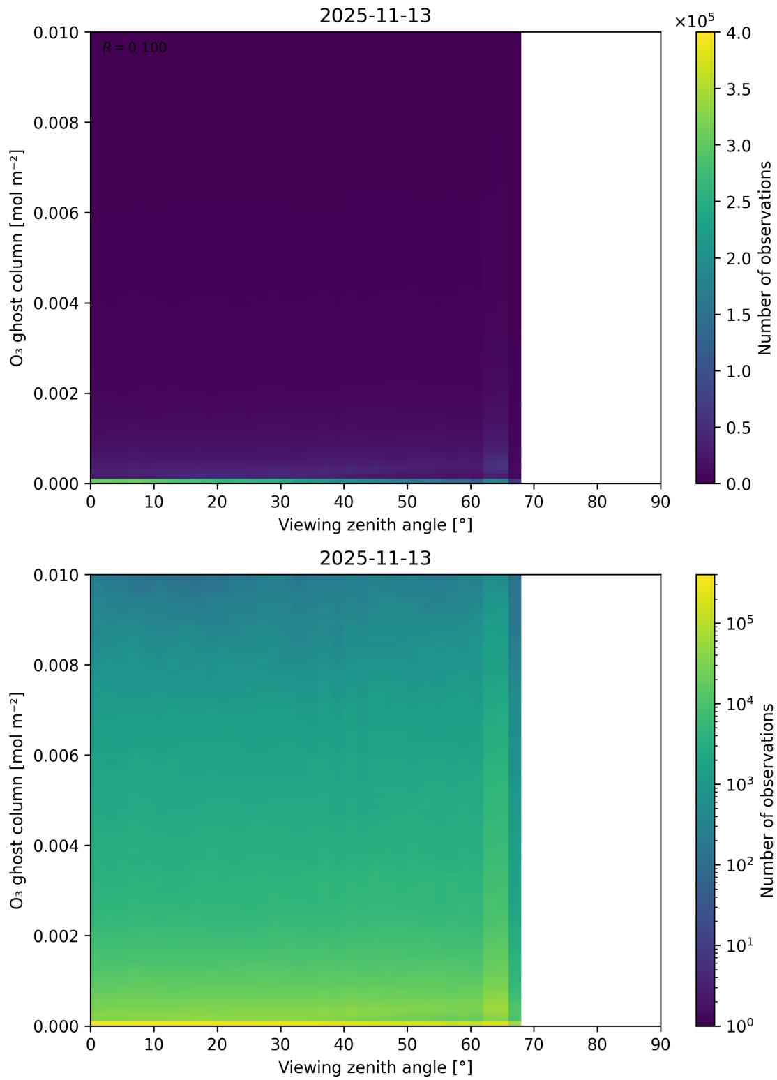
Figure 51: Scatter density plot of “Viewing zenith angle” against “O 3 ghost column” for 2025-11-12 to 2025-11-14.
