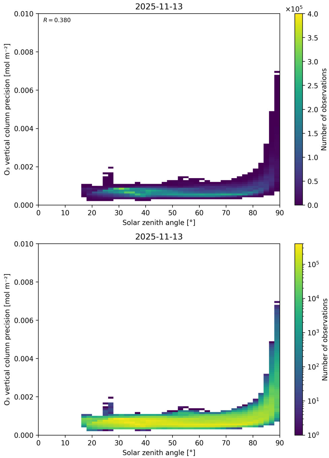
Figure 48: Scatter density plot of “Solar zenith angle” against “O 3 vertical column precision” for 2025-11-12 to 2025-11-14.
