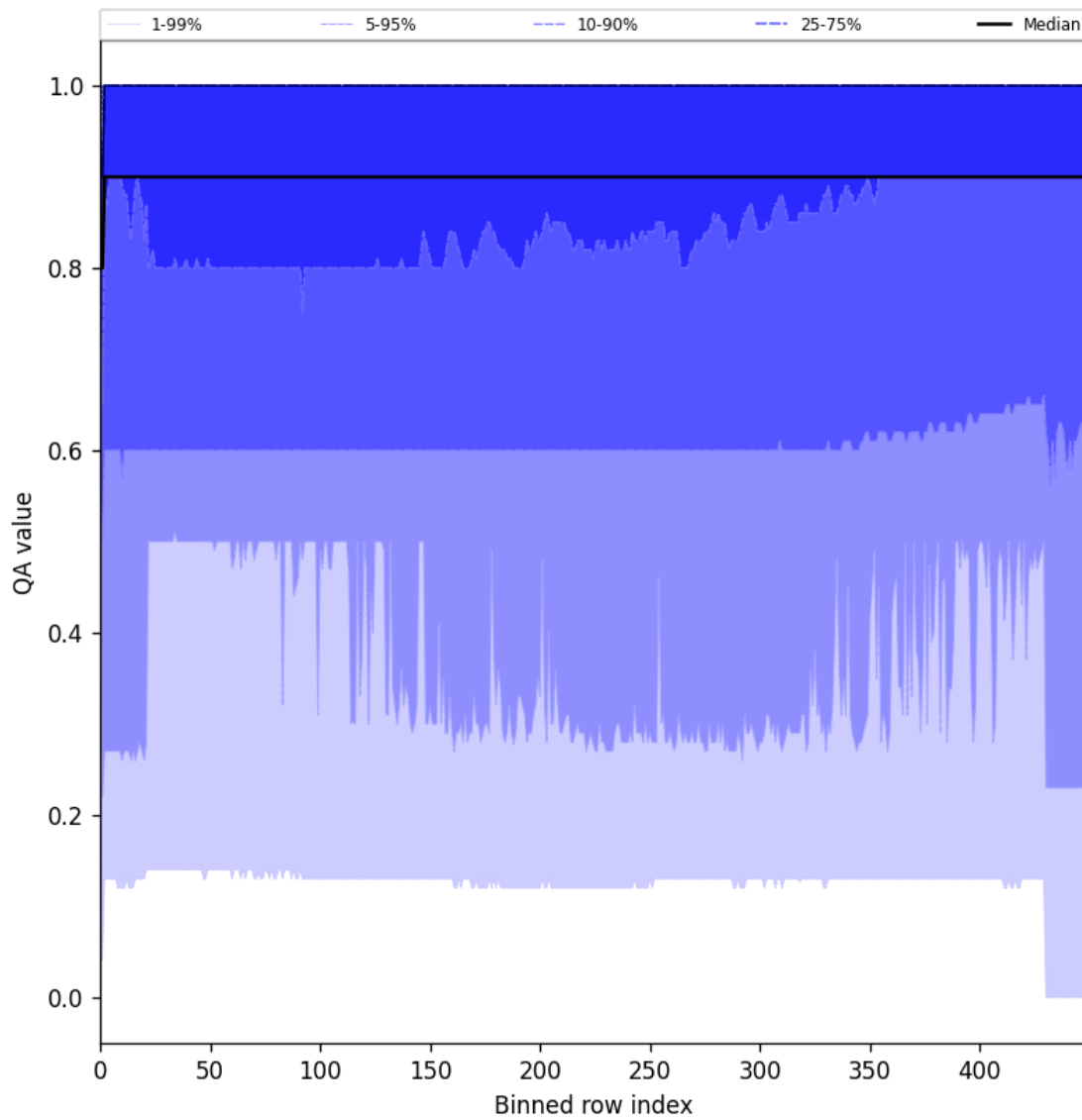
Figure 27: Along track statistics of “QA value” for 2025-11-12 to 2025-11-14
