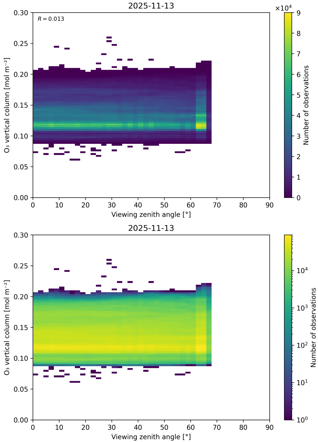
Figure 52: Scatter density plot of “Viewing zenith angle” against “O 3 vertical column” for 2025-11-12 to 2025-11-14.
