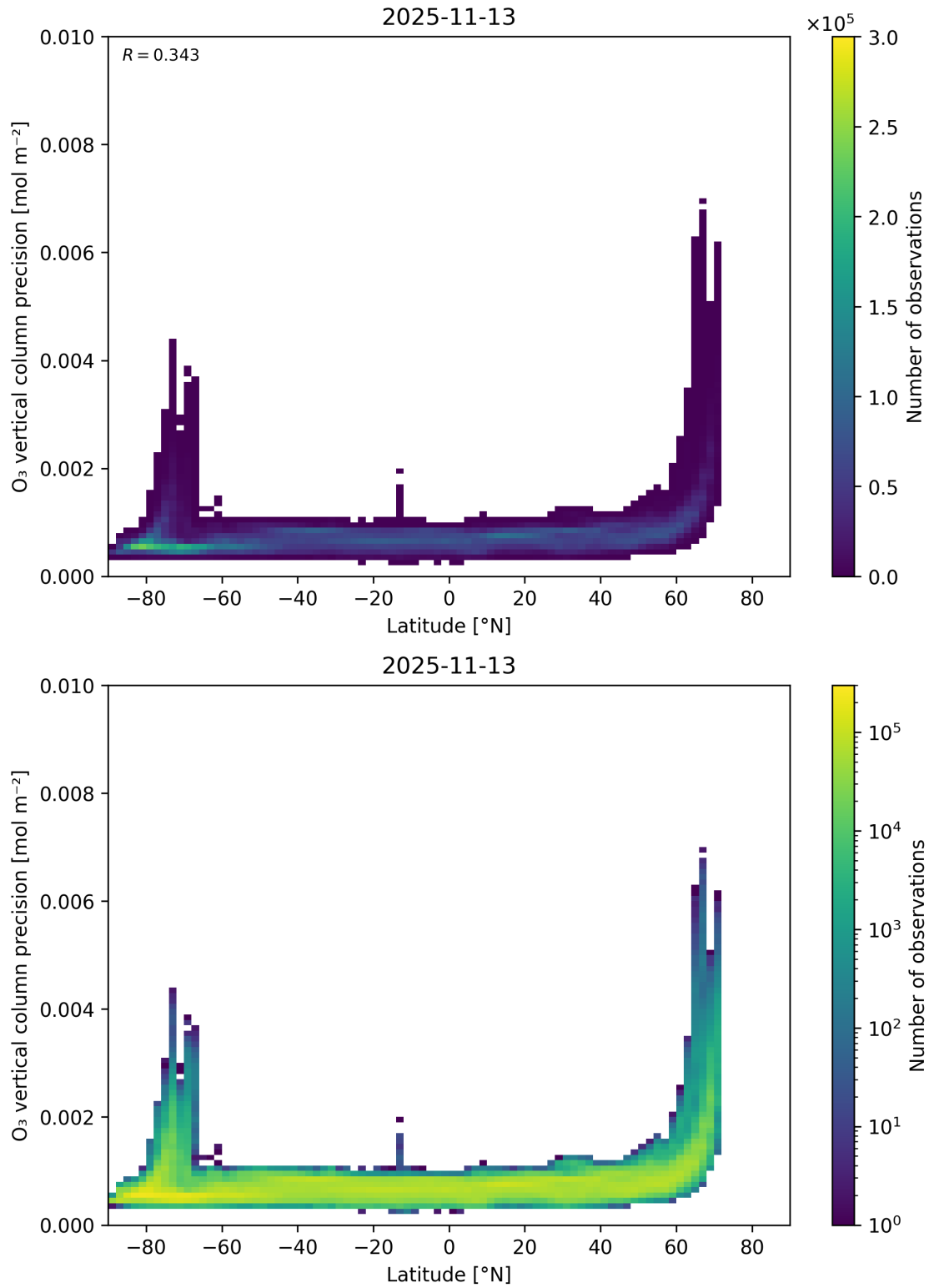
Figure 37: Scatter density plot of “Latitude” against “O 3 vertical column precision” for 2025-11-12 to 2025-11-14.
