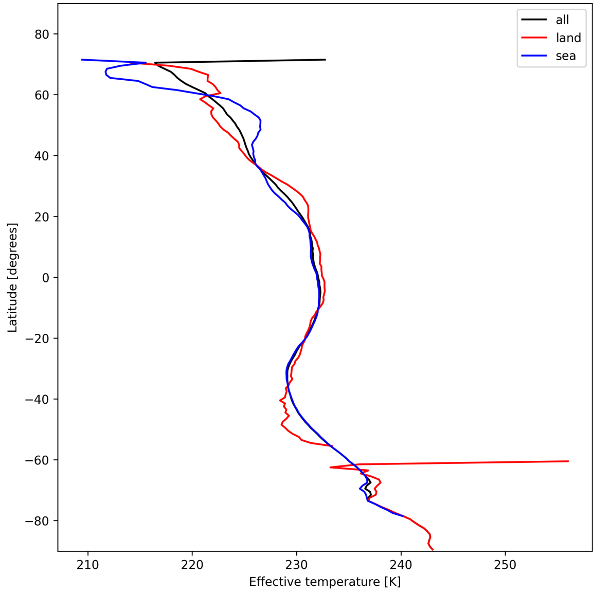
Figure 17: Zonal average of "Effective temperature" for 2025-11-12 to 2025-11-14.
