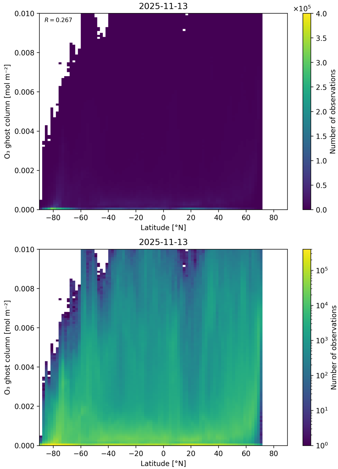
Figure 35: Scatter density plot of “Latitude” against “O 3 ghost column” for 2025-11-12 to 2025-11-14.
