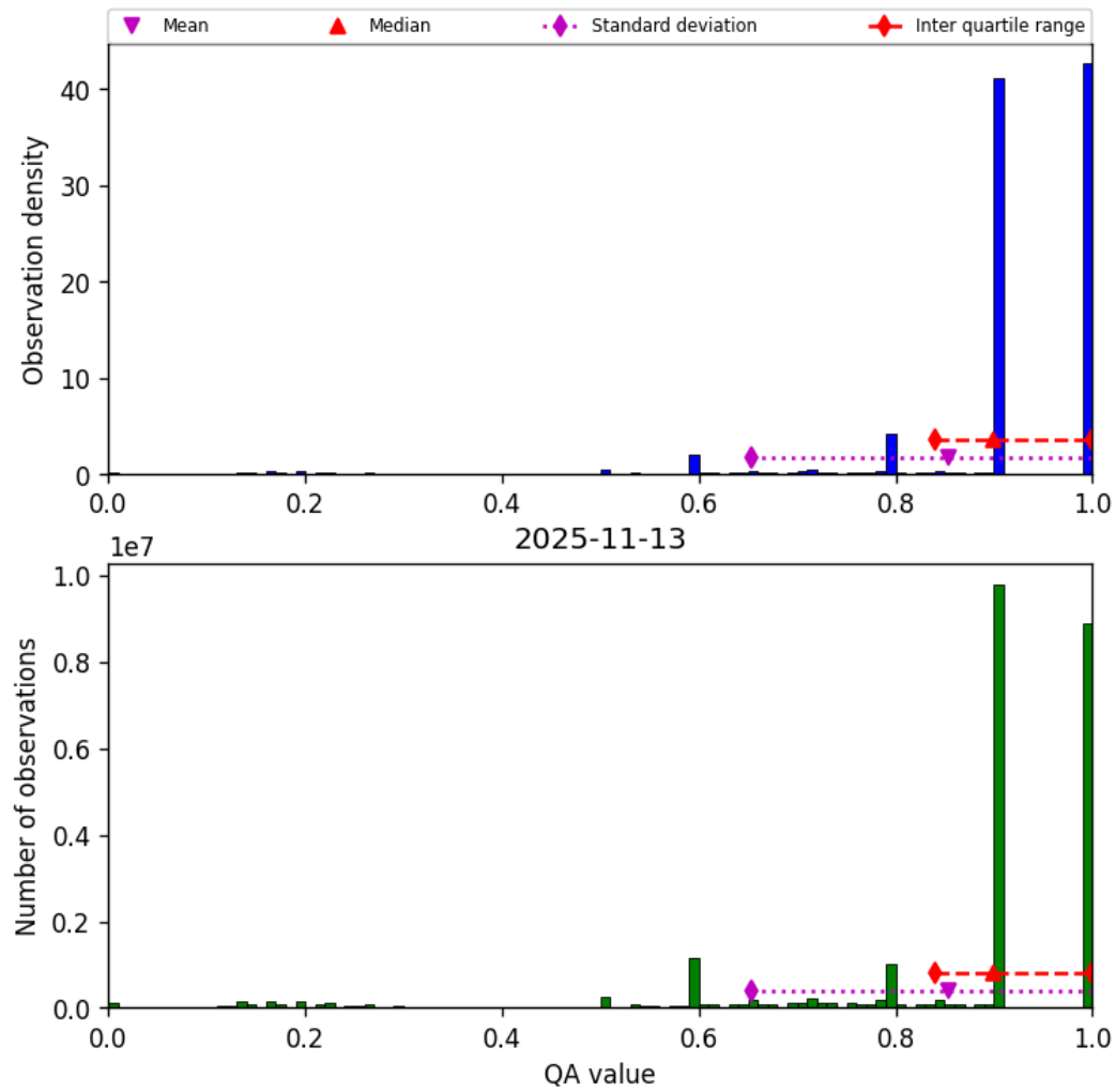
Figure 20: Histogram of “QA value” for 2025-11-12 to 2025-11-14
