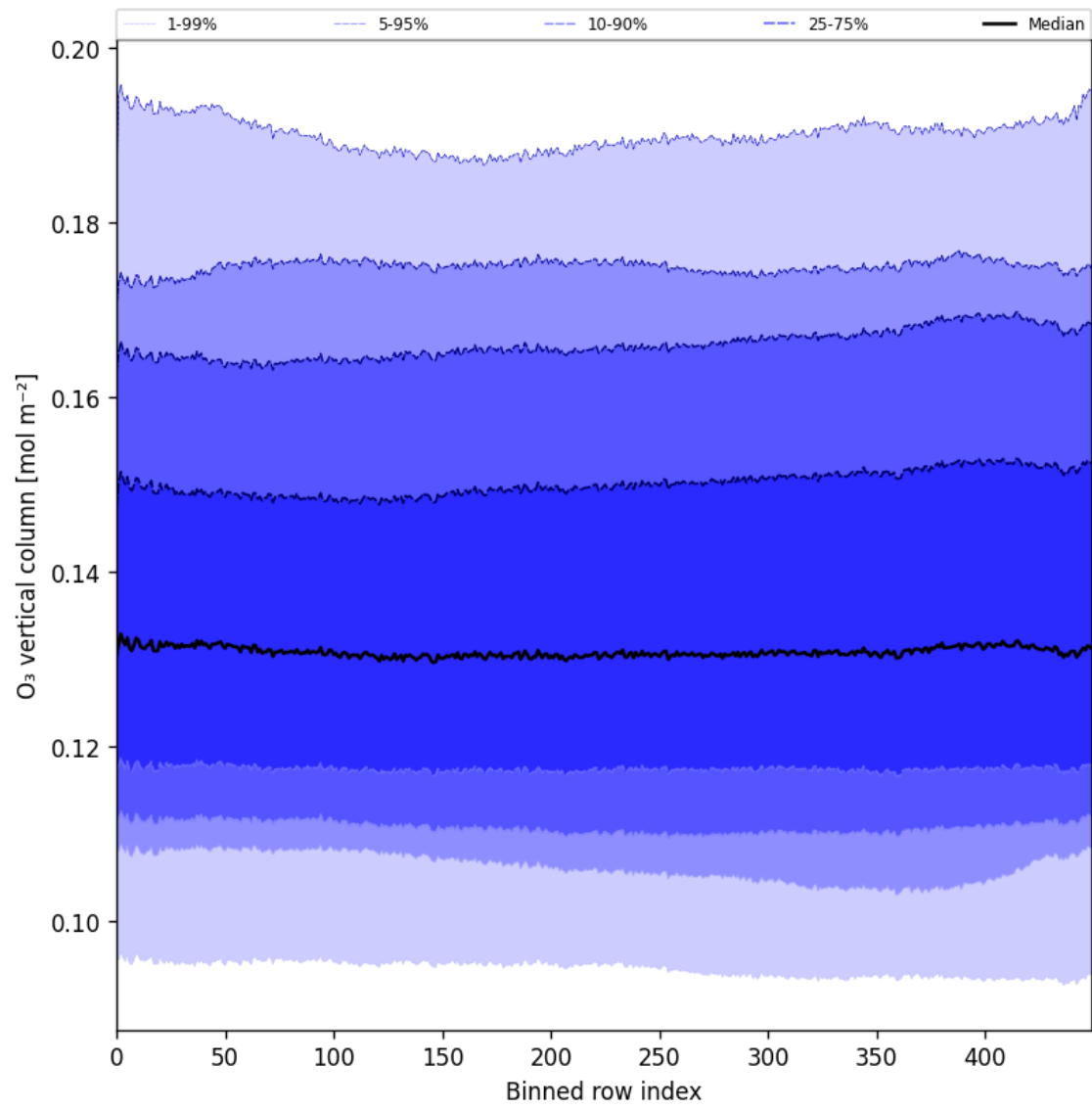
Figure 28: Along track statistics of “O 3 vertical column” for 2025-11-13 to 2025-11-15
