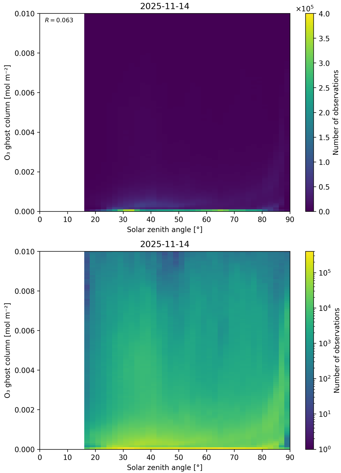
Figure 46: Scatter density plot of “Solar zenith angle” against “O 3 ghost column” for 2025-11-13 to 2025-11-15.
