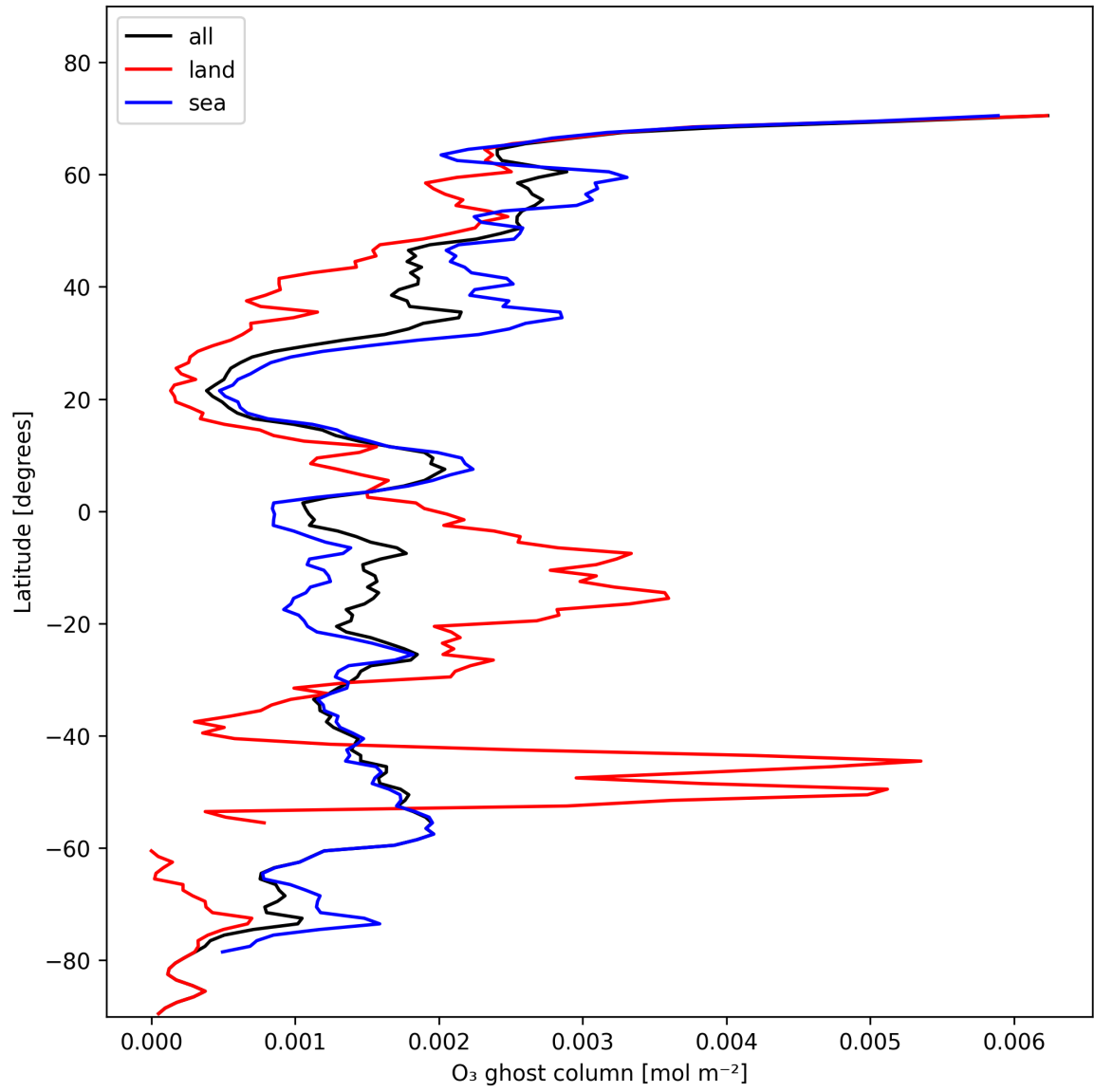
Figure 18: Zonal average of “O 3 ghost column” for 2025-11-13 to 2025-11-15.
