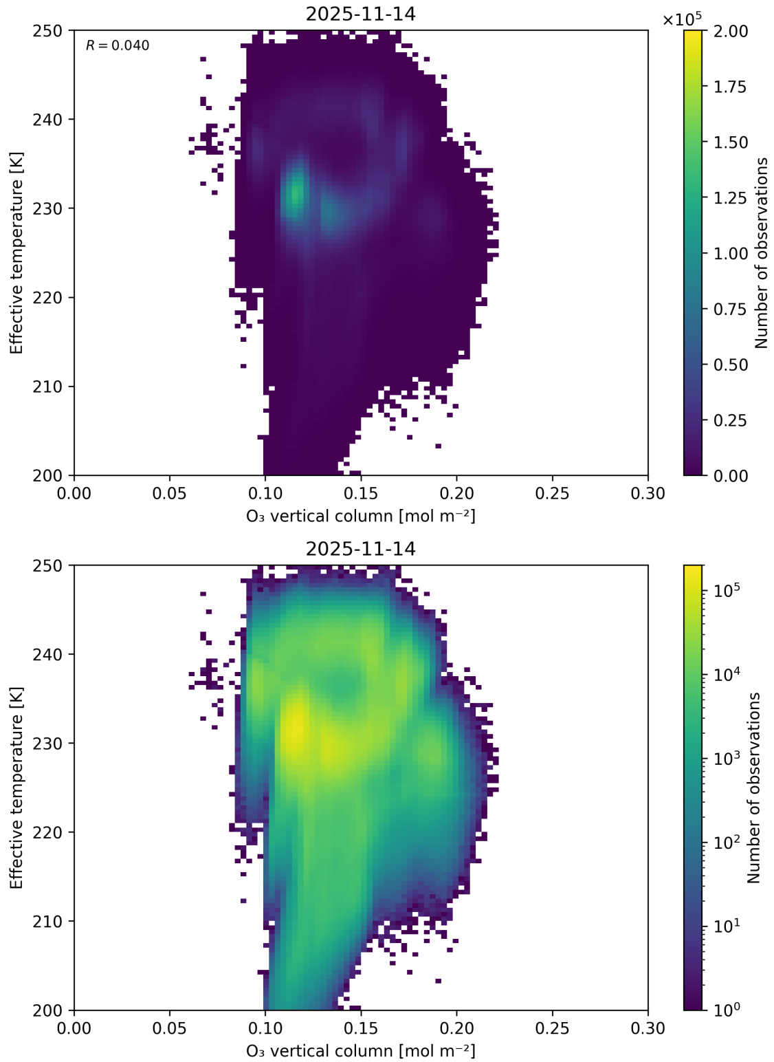
Figure 39: Scatter density plot of “O 3 vertical column” against “Effective temperature” for 2025-11-13 to 2025-11-15.
