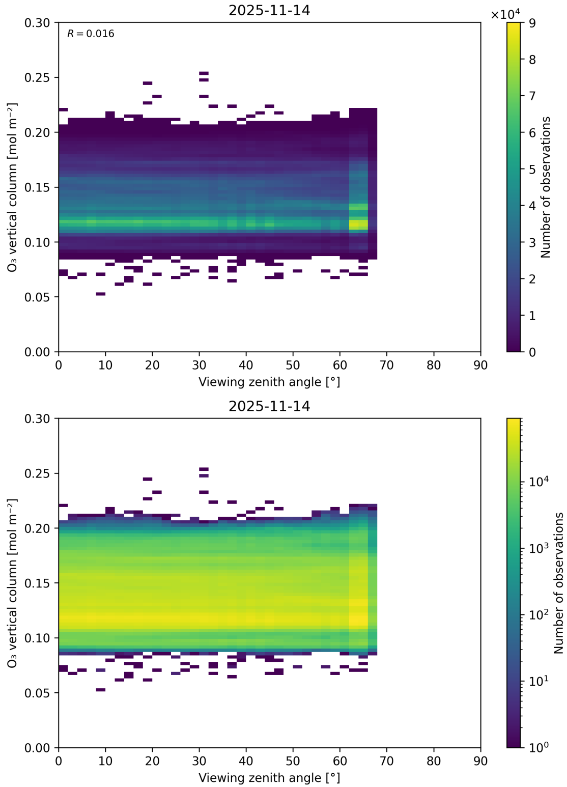
Figure 52: Scatter density plot of “Viewing zenith angle” against “O 3 vertical column” for 2025-11-13 to 2025-11-15.
