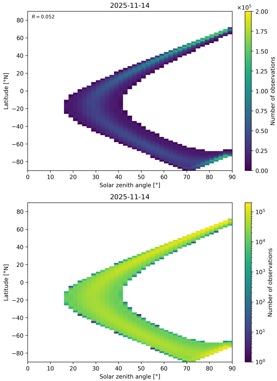
Figure 44: Scatter density plot of “Solar zenith angle” against “Latitude” for 2025-11-13 to 2025-11-15.
