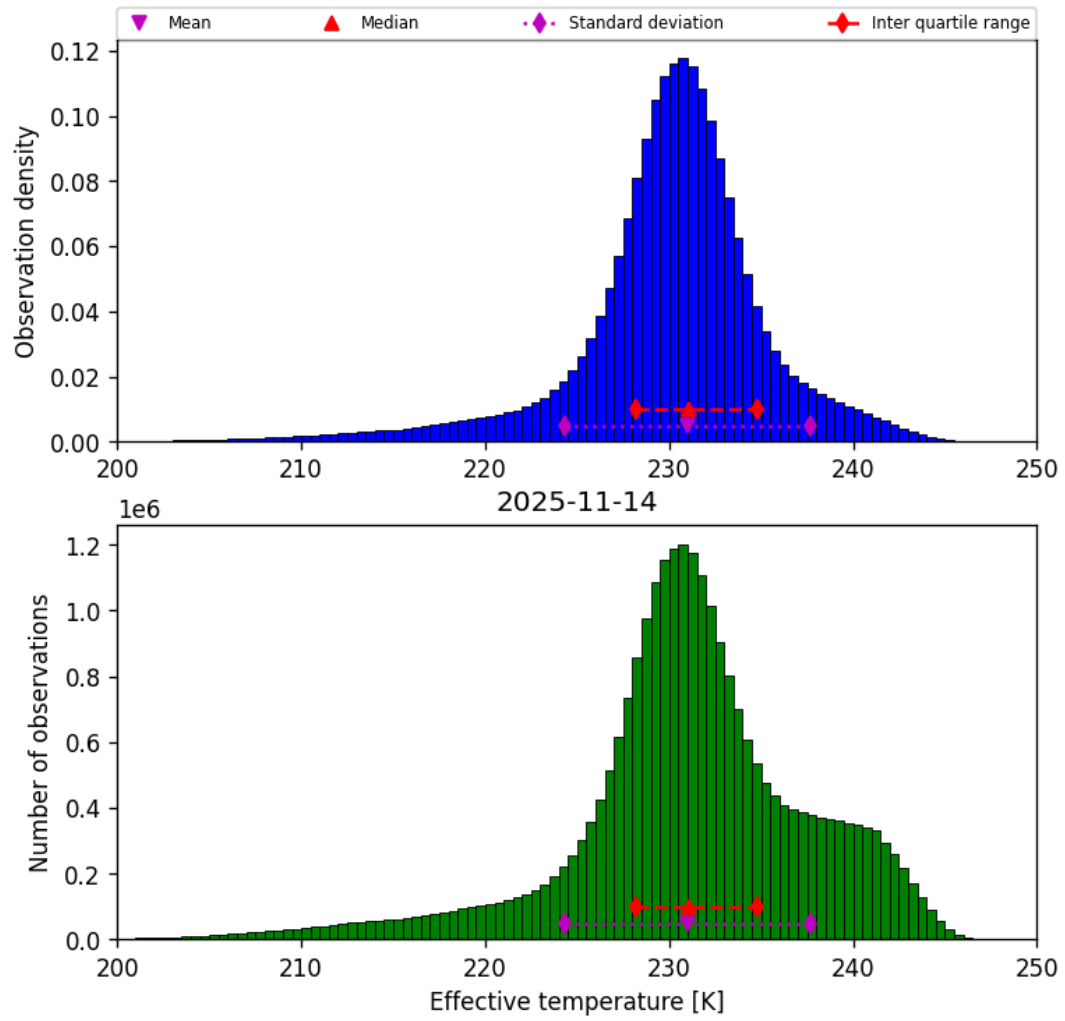
Figure 24: Histogram of “Effective temperature” for 2025-11-13 to 2025-11-15
