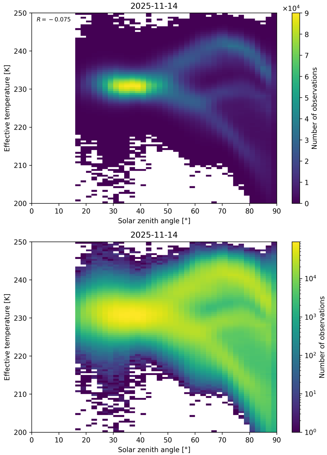
Figure 45: Scatter density plot of “Solar zenith angle” against “Effective temperature” for 2025-11-13 to 2025-11-15.
