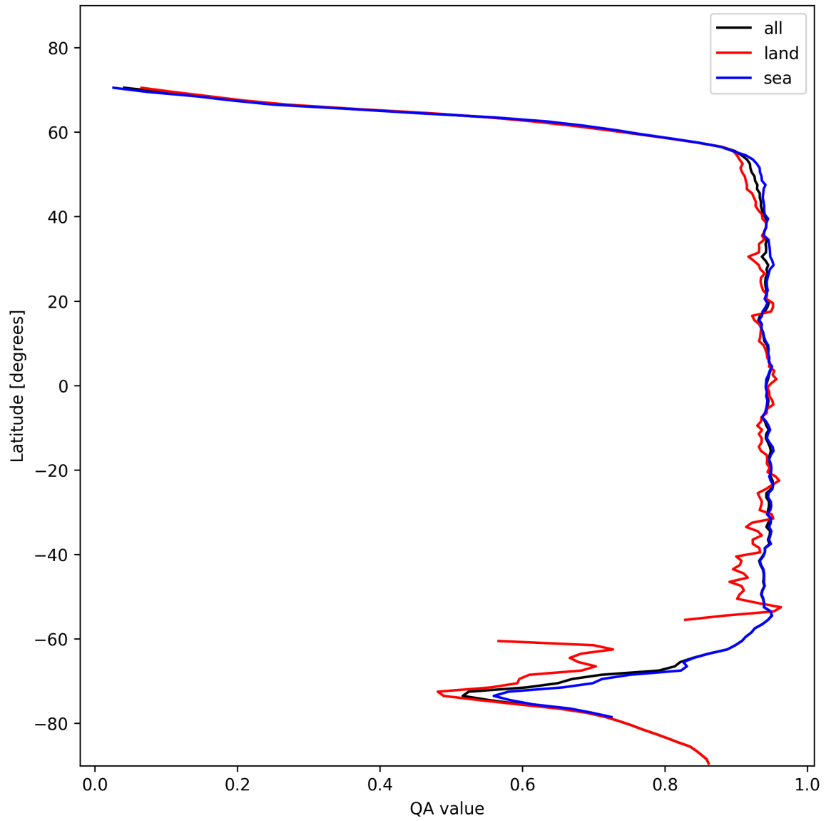
Figure 13: Zonal average of “QA value” for 2025-11-13 to 2025-11-15.
