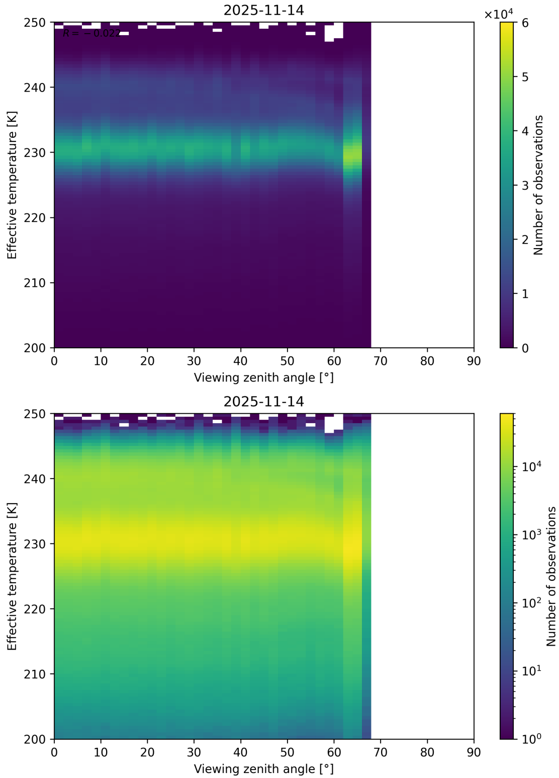
Figure 50: Scatter density plot of “Viewing zenith angle” against “Effective temperature” for 2025-11-13 to 2025-11-15.
