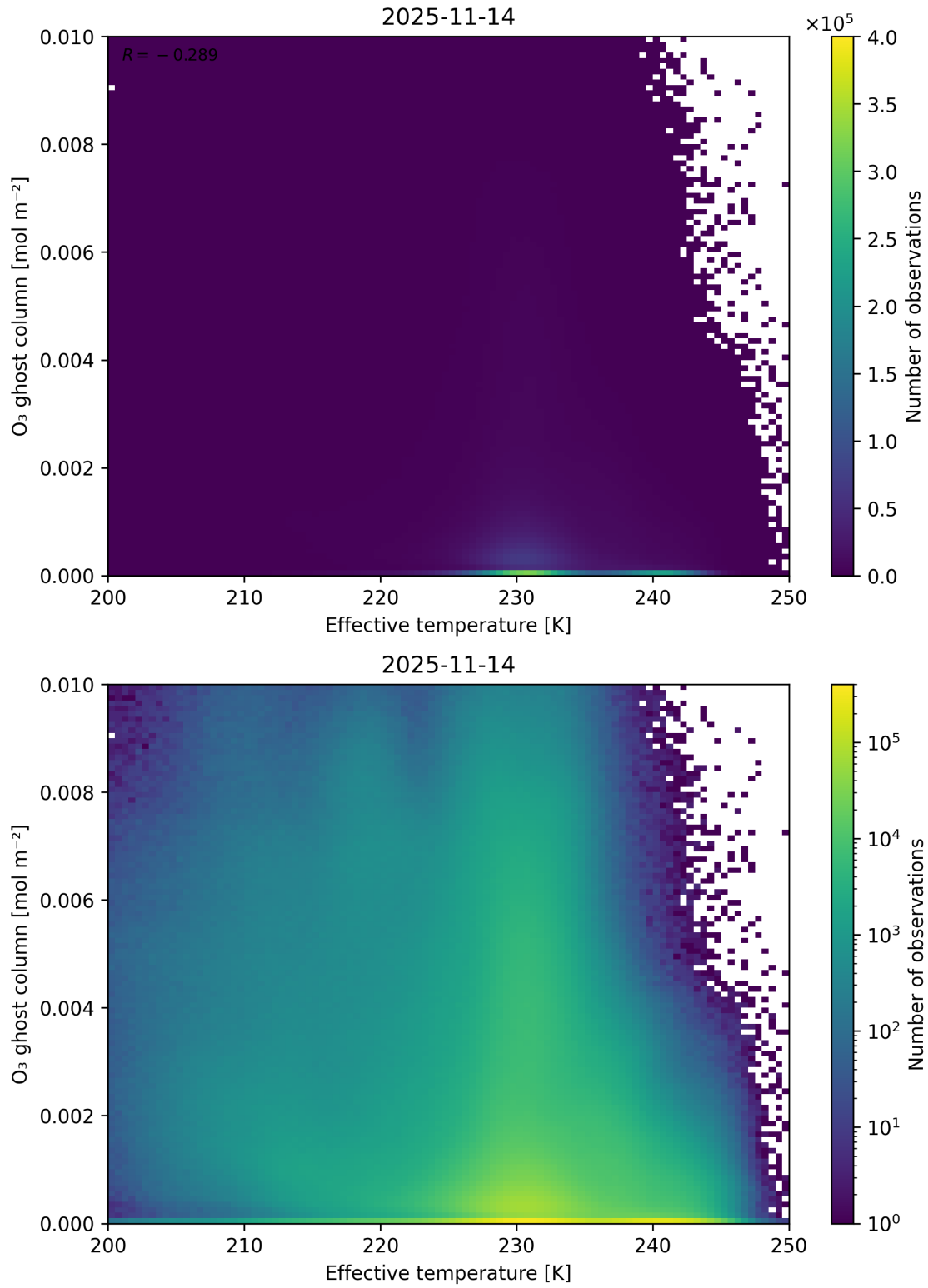
Figure 38: Scatter density plot of “Effective temperature” against “O 3 ghost column” for 2025-11-13 to 2025-11-15.
