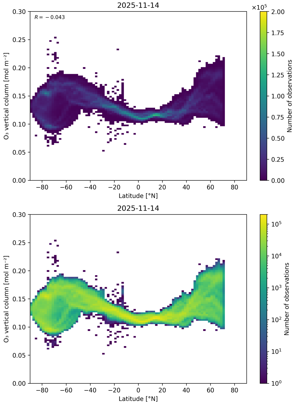
Figure 36: Scatter density plot of “Latitude” against “O 3 vertical column” for 2025-11-13 to 2025-11-15.
