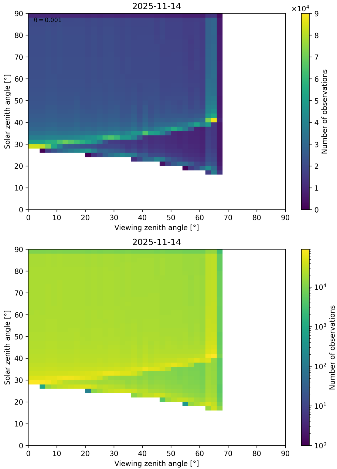
Figure 54: Scatter density plot of “Viewing zenith angle” against “Solar zenith angle” for 2025-11-13 to 2025-11-15.
