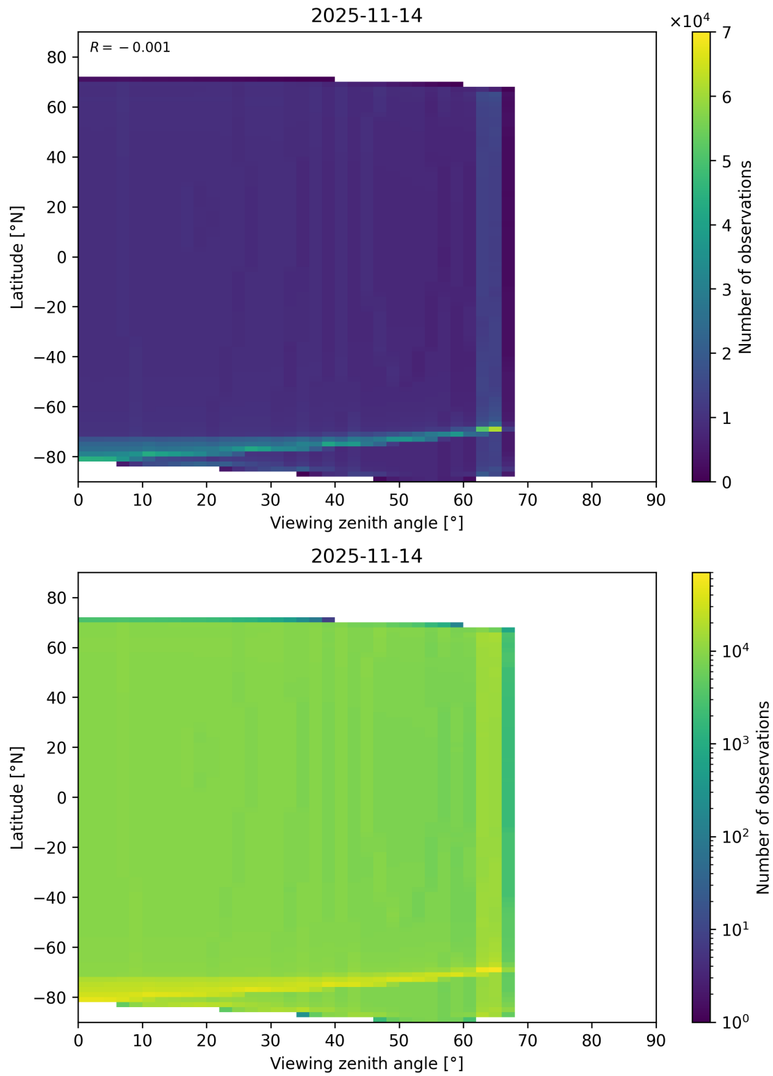
Figure 49: Scatter density plot of “Viewing zenith angle” against “Latitude” for 2025-11-13 to 2025-11-15.
