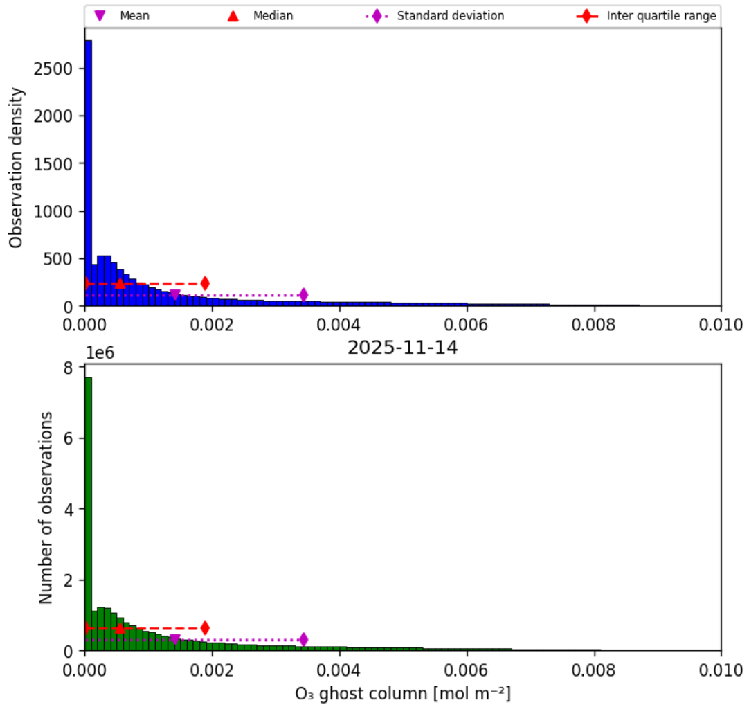
Figure 25: Histogram of “O 3 ghost column” for 2025-11-13 to 2025-11-15
