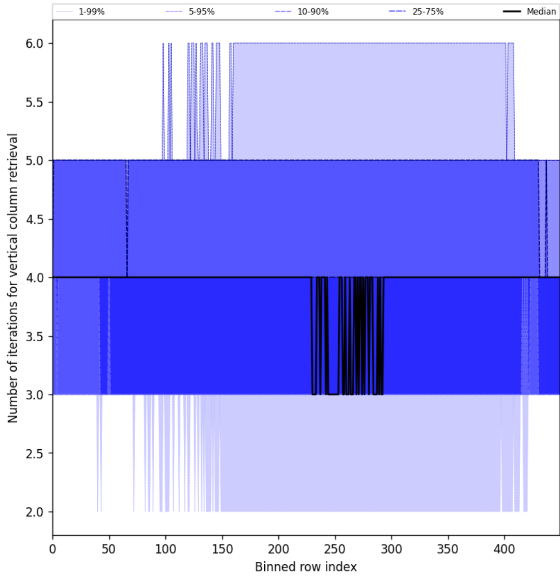
Figure 33: Along track statistics of “Number of iterations for vertical column retrieval” for 2025-11-13 to 2025-11-15
