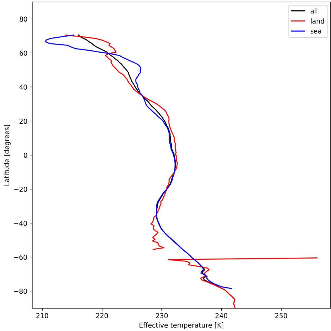
Figure 17: Zonal average of “Effective temperature” for 2025-11-13 to 2025-11-15.
