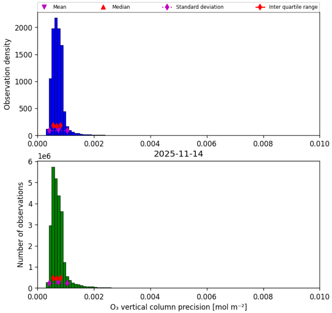
Figure 22: Histogram of “O 3 vertical column precision” for 2025-11-13 to 2025-11-15
