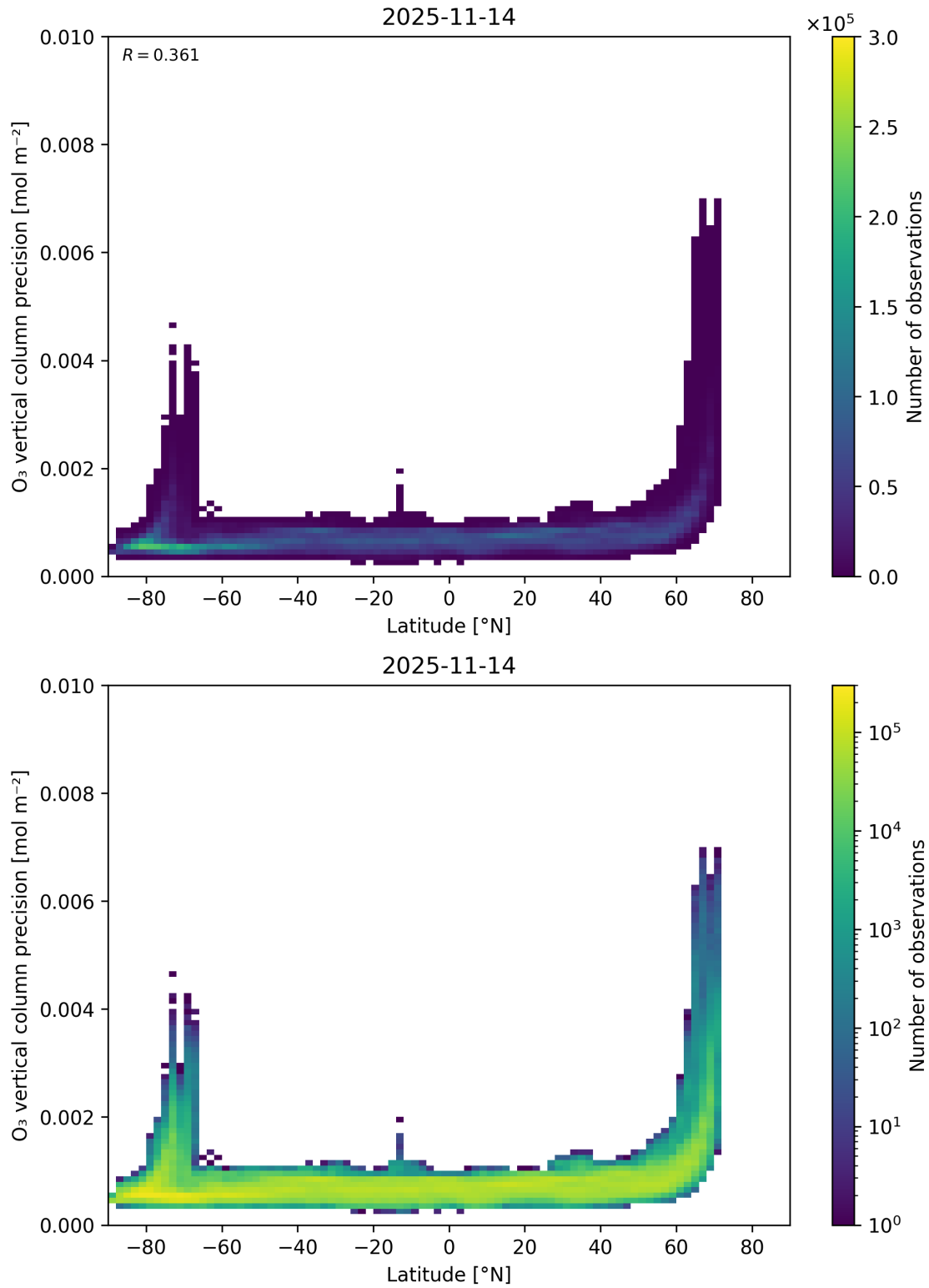
Figure 37: Scatter density plot of “Latitude” against “O 3 vertical column precision” for 2025-11-13 to 2025-11-15.
