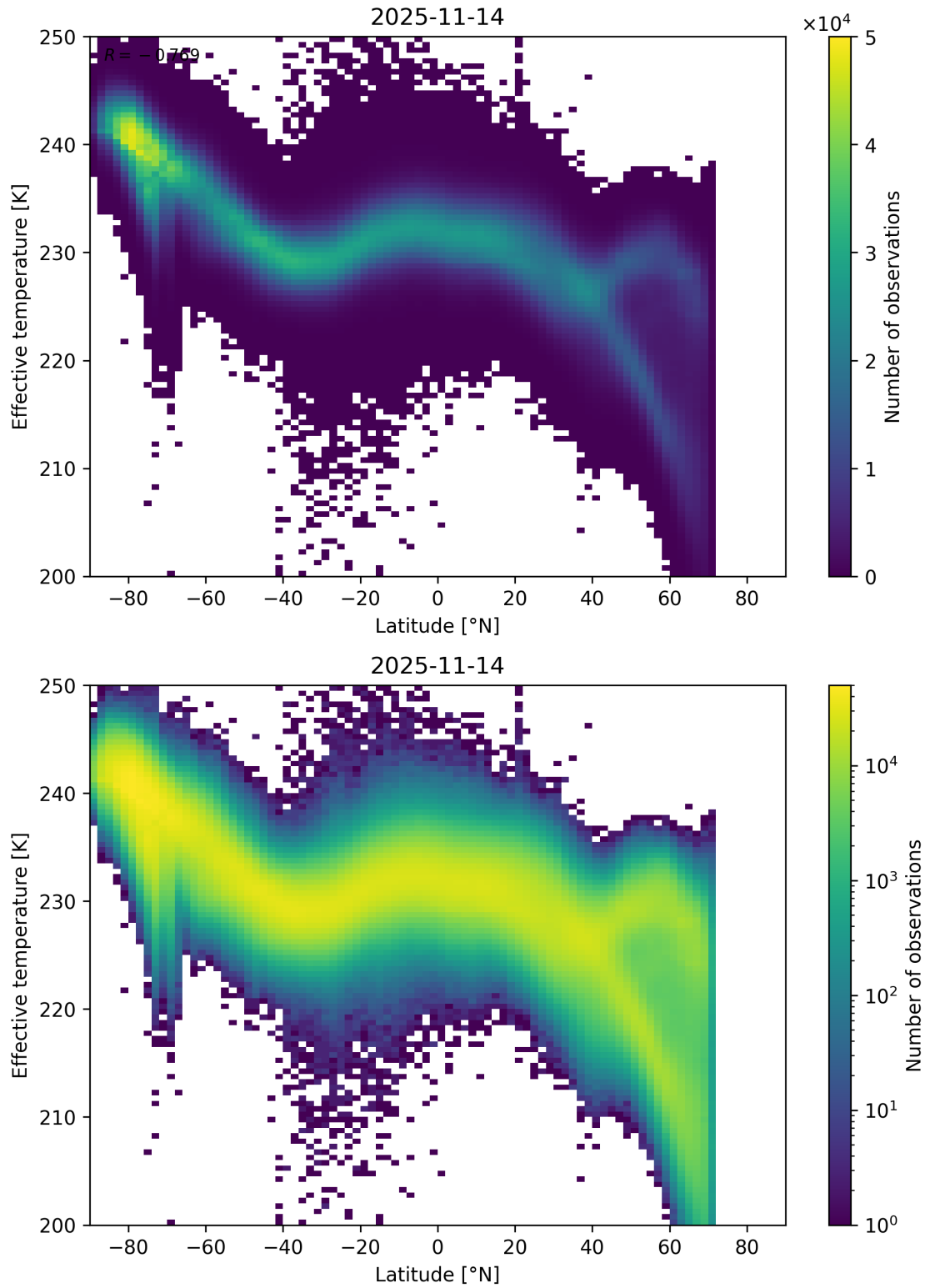
Figure 34: Scatter density plot of “Latitude” against “Effective temperature” for 2025-11-13 to 2025-11-15.
