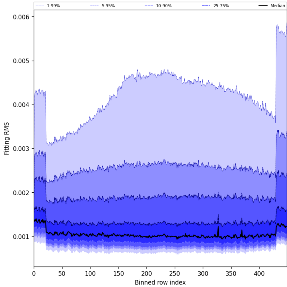
Figure 30: Along track statistics of “Fitting RMS” for 2025-11-13 to 2025-11-15
