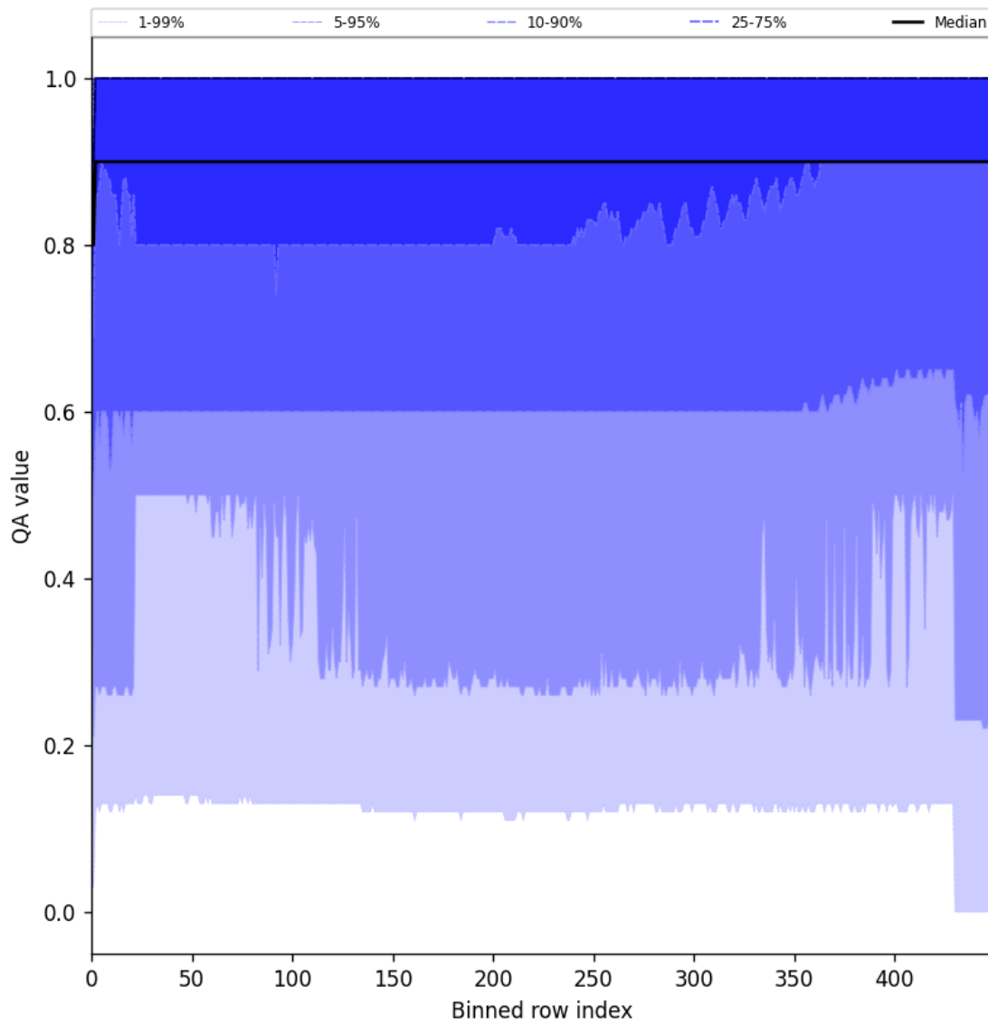
Figure 27: Along track statistics of “QA value” for 2025-11-13 to 2025-11-15
