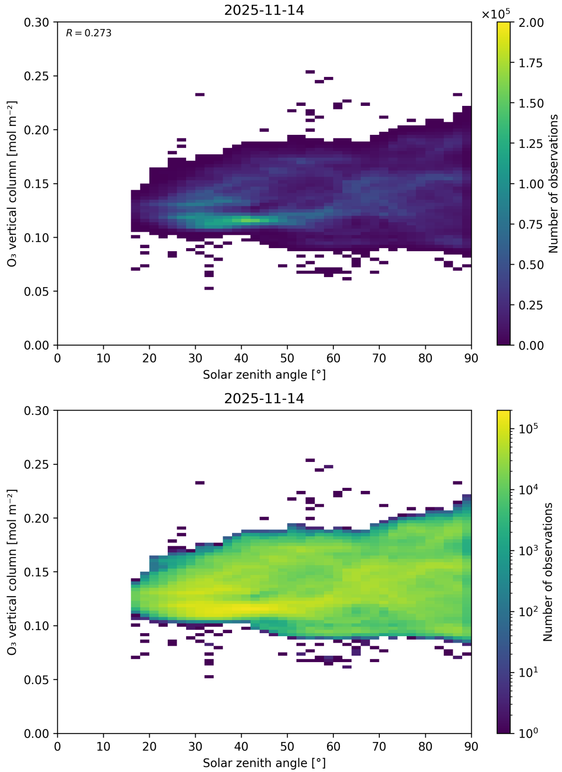
Figure 47: Scatter density plot of “Solar zenith angle” against “O 3 vertical column” for 2025-11-13 to 2025-11-15.
