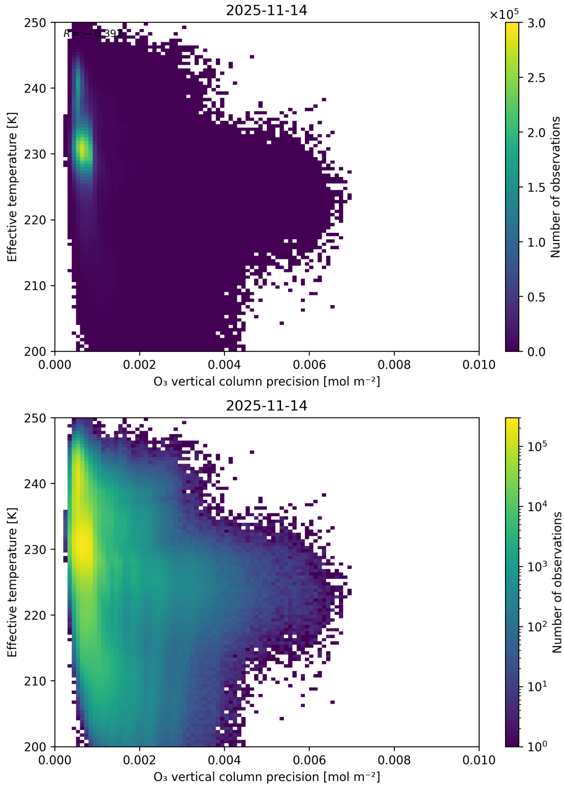
Figure 42: Scatter density plot of “O 3 vertical column precision” against “Effective temperature” for 2025-11-13 to 2025-11-15.
