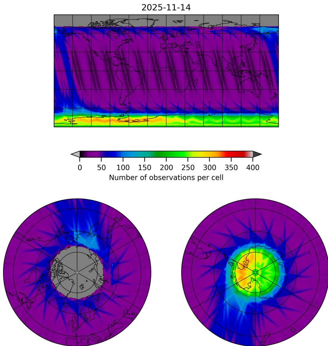
Figure 12: Map of the number of observations for 2025-11-13 to 2025-11-15
