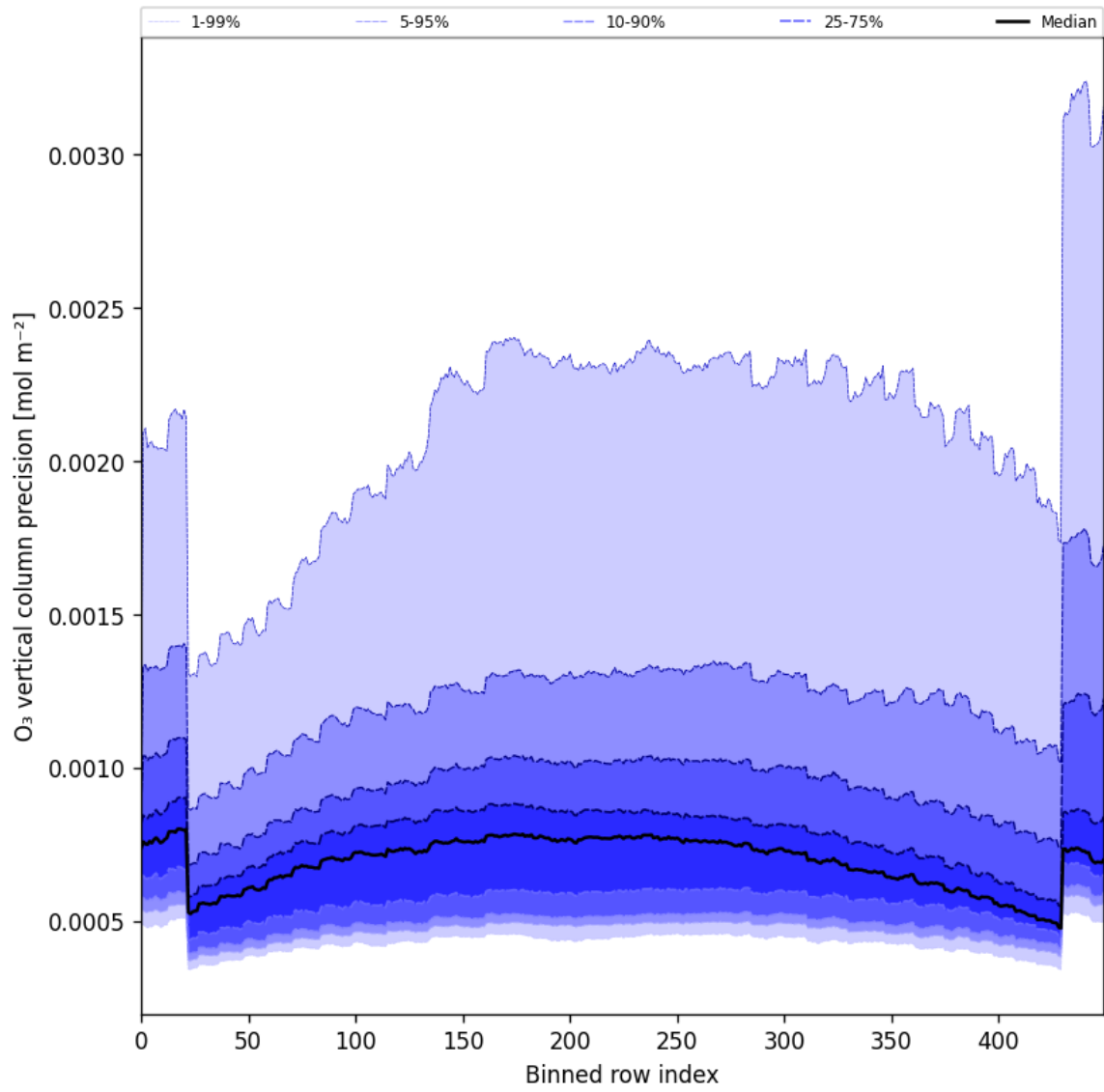
Figure 29: Along track statistics of “O 3 vertical column precision” for 2025-11-13 to 2025-11-15
