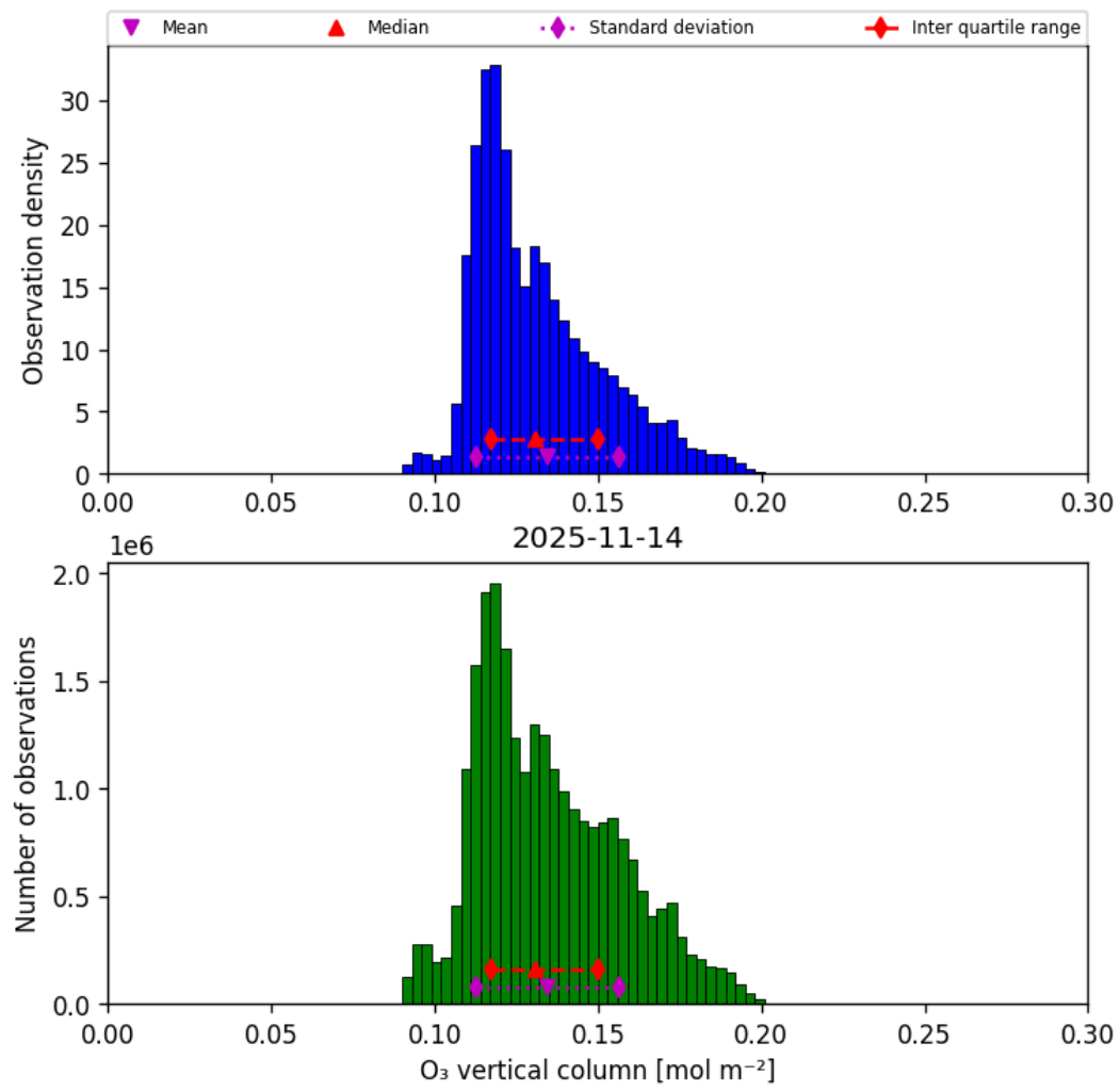
Figure 21: Histogram of “O 3 vertical column” for 2025-11-13 to 2025-11-15
