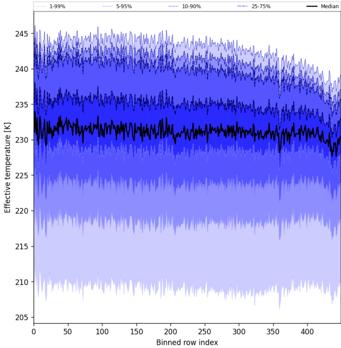
Figure 31: Along track statistics of “Effective temperature” for 2025-11-13 to 2025-11-15
