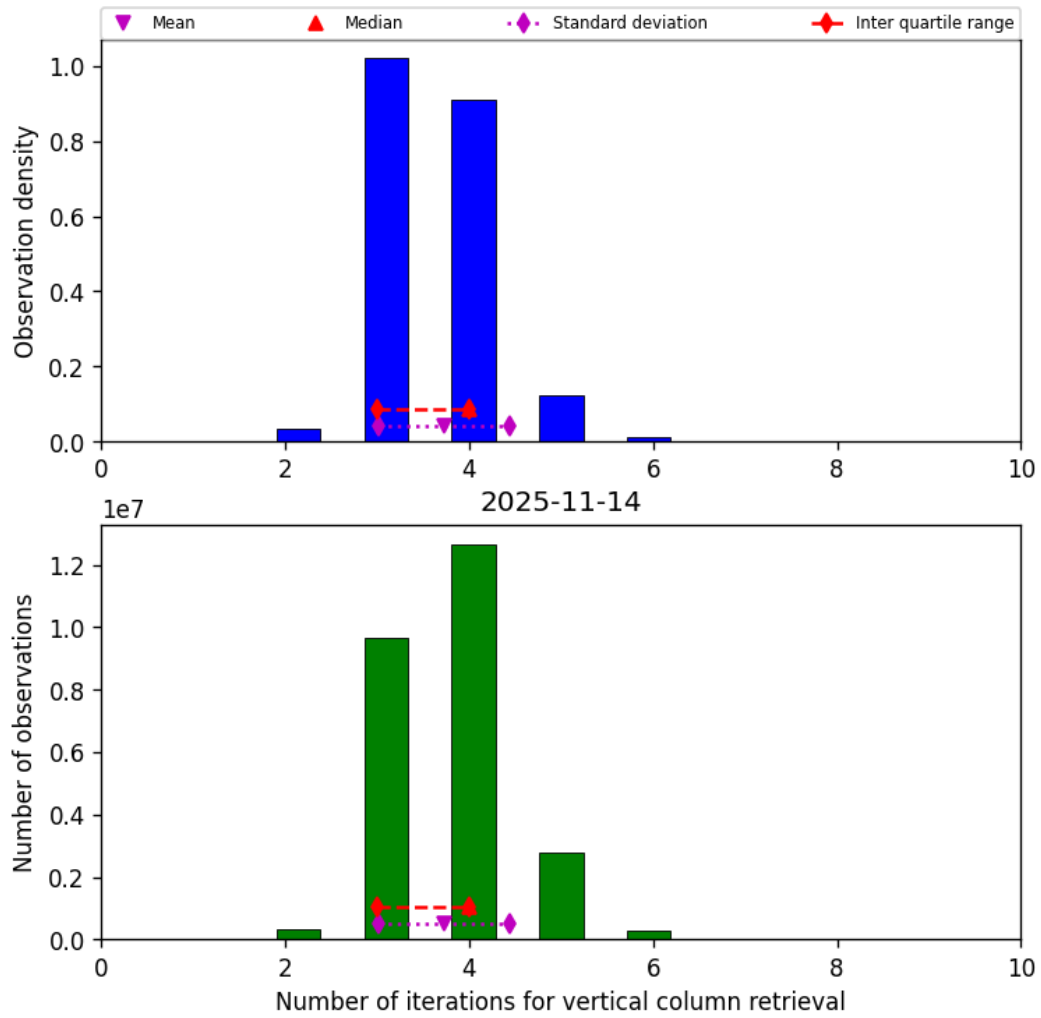
Figure 26: Histogram of “Number of iterations for vertical column retrieval” for 2025-11-13 to 2025-11-15
