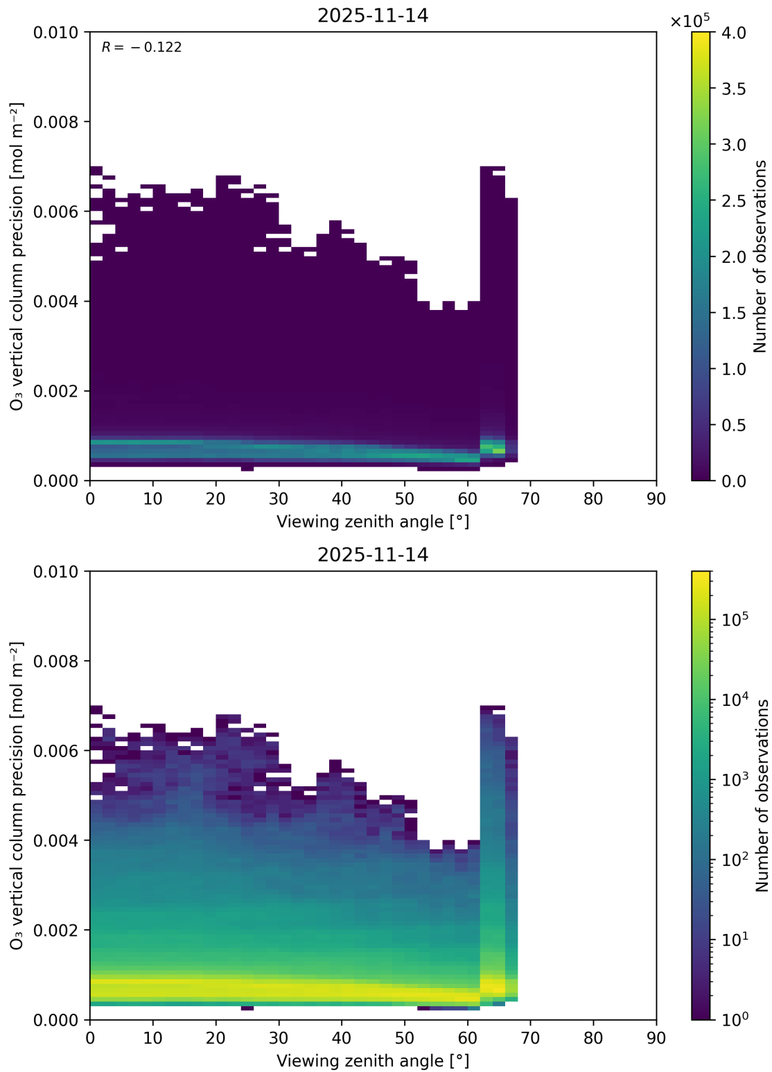
Figure 53: Scatter density plot of “Viewing zenith angle” against “O 3 vertical column precision” for 2025-11-13 to 2025-11-15.
