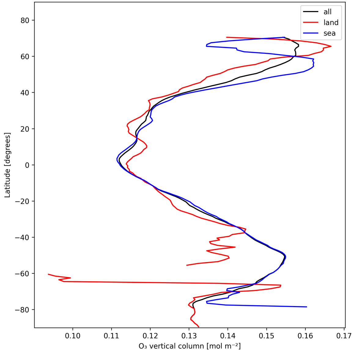
Figure 14: Zonal average of “O 3 vertical column” for 2025-11-13 to 2025-11-15.
