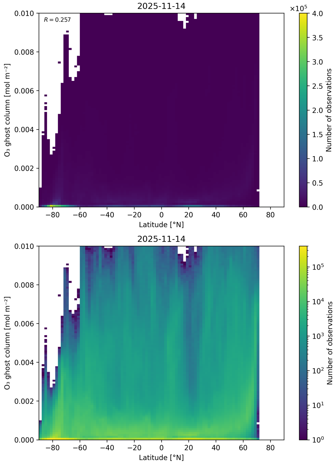
Figure 35: Scatter density plot of “Latitude” against “O 3 ghost column” for 2025-11-13 to 2025-11-15.
