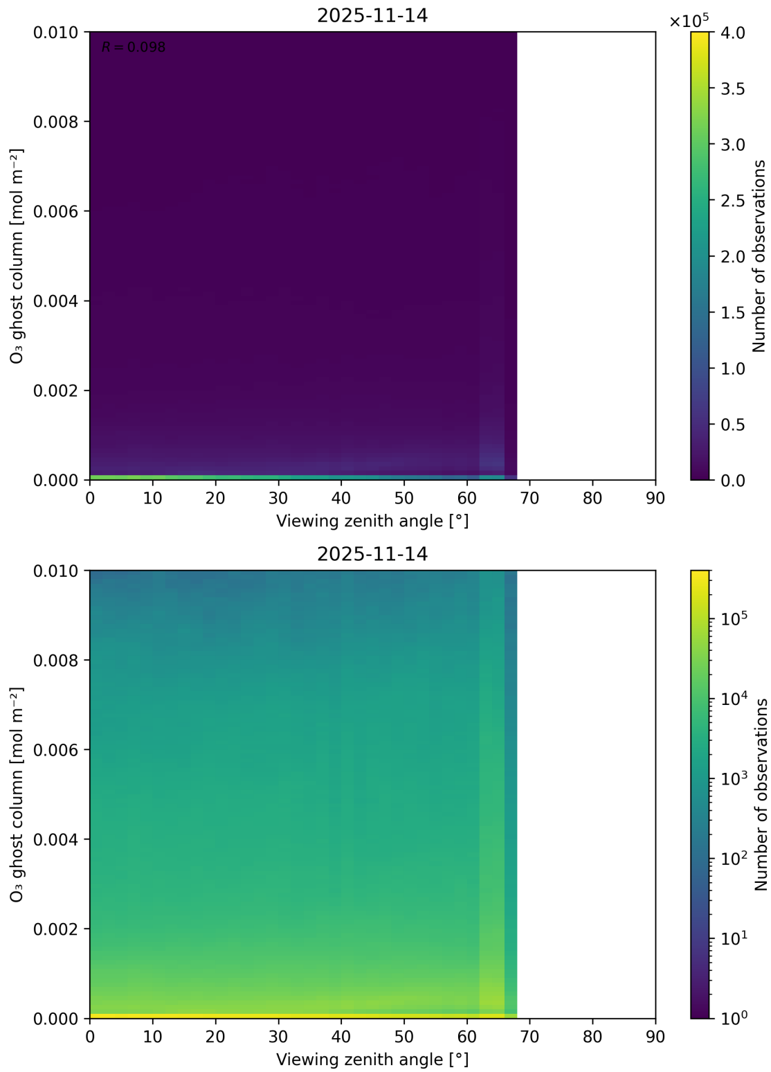
Figure 51: Scatter density plot of “Viewing zenith angle” against “O 3 ghost column” for 2025-11-13 to 2025-11-15.
