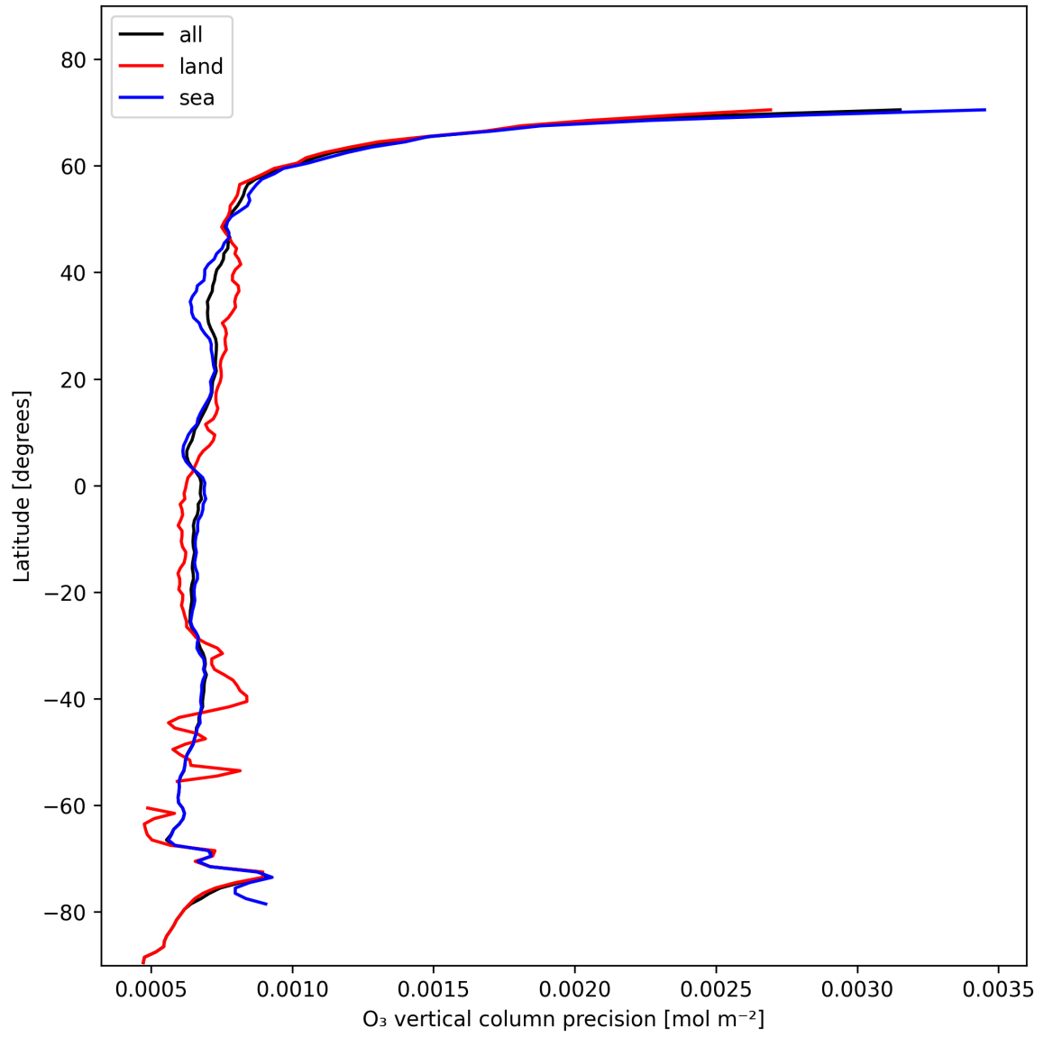
Figure 15: Zonal average of “O 3 vertical column precision” for 2025-11-13 to 2025-11-15.
