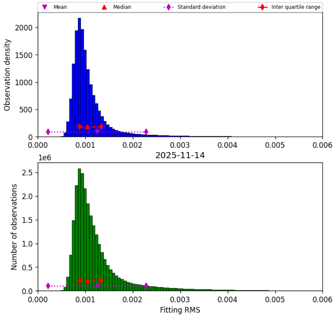
Figure 23: Histogram of “Fitting RMS” for 2025-11-13 to 2025-11-15
