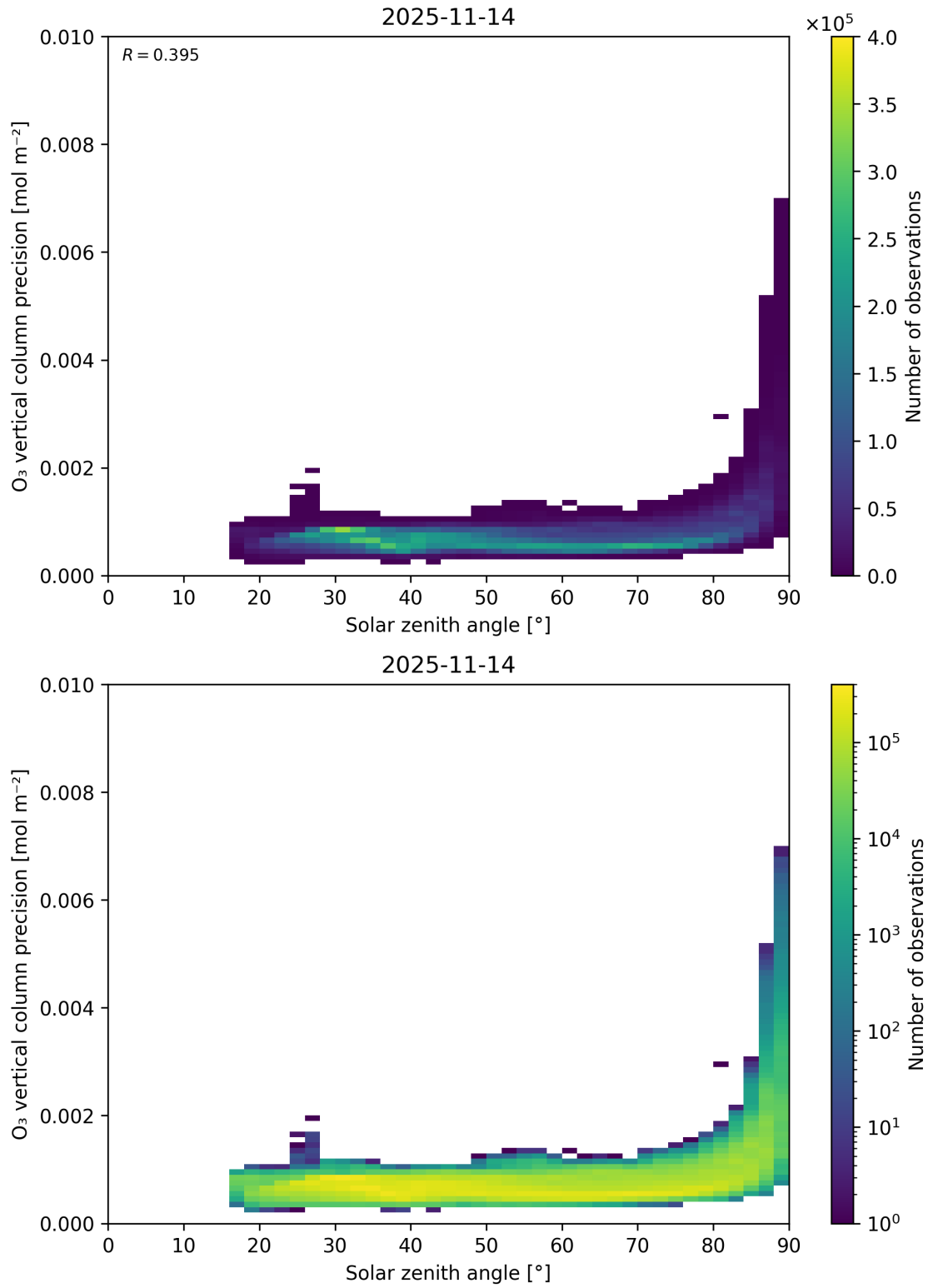
Figure 48: Scatter density plot of “Solar zenith angle” against “O 3 vertical column precision” for 2025-11-13 to 2025-11-15.
