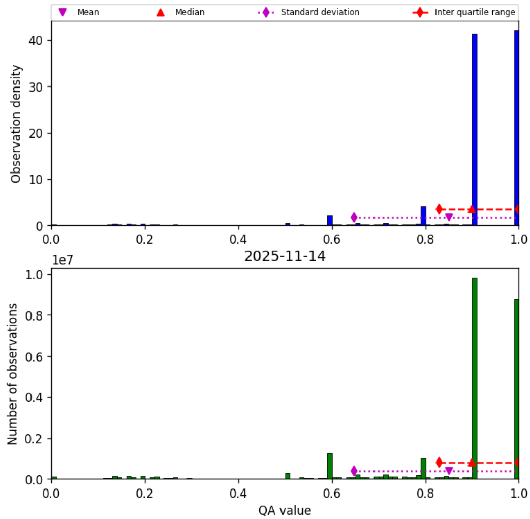
Figure 20: Histogram of “QA value” for 2025-11-13 to 2025-11-15
