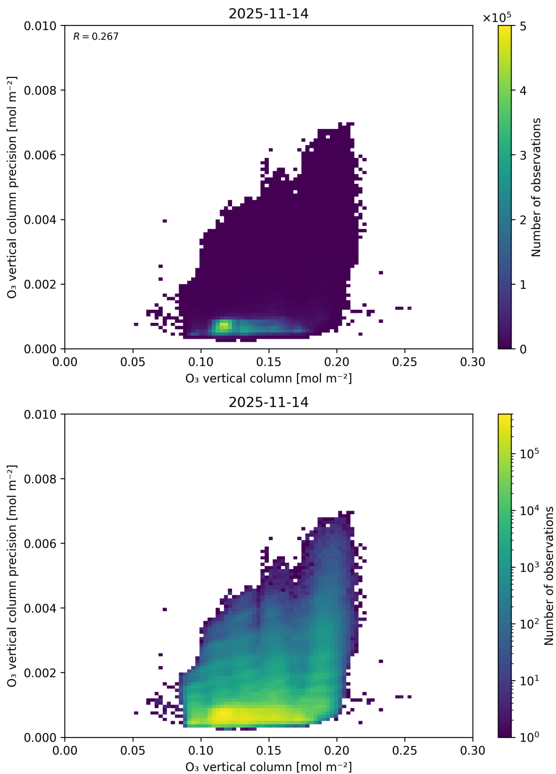
Figure 41: Scatter density plot of “O 3 vertical column” against “O 3 vertical column precision” for 2025-11-13 to 2025-11-15.
