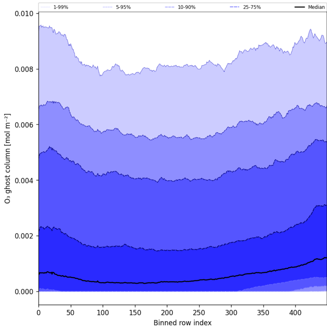
Figure 32: Along track statistics of “O 3 ghost column” for 2025-11-13 to 2025-11-15
