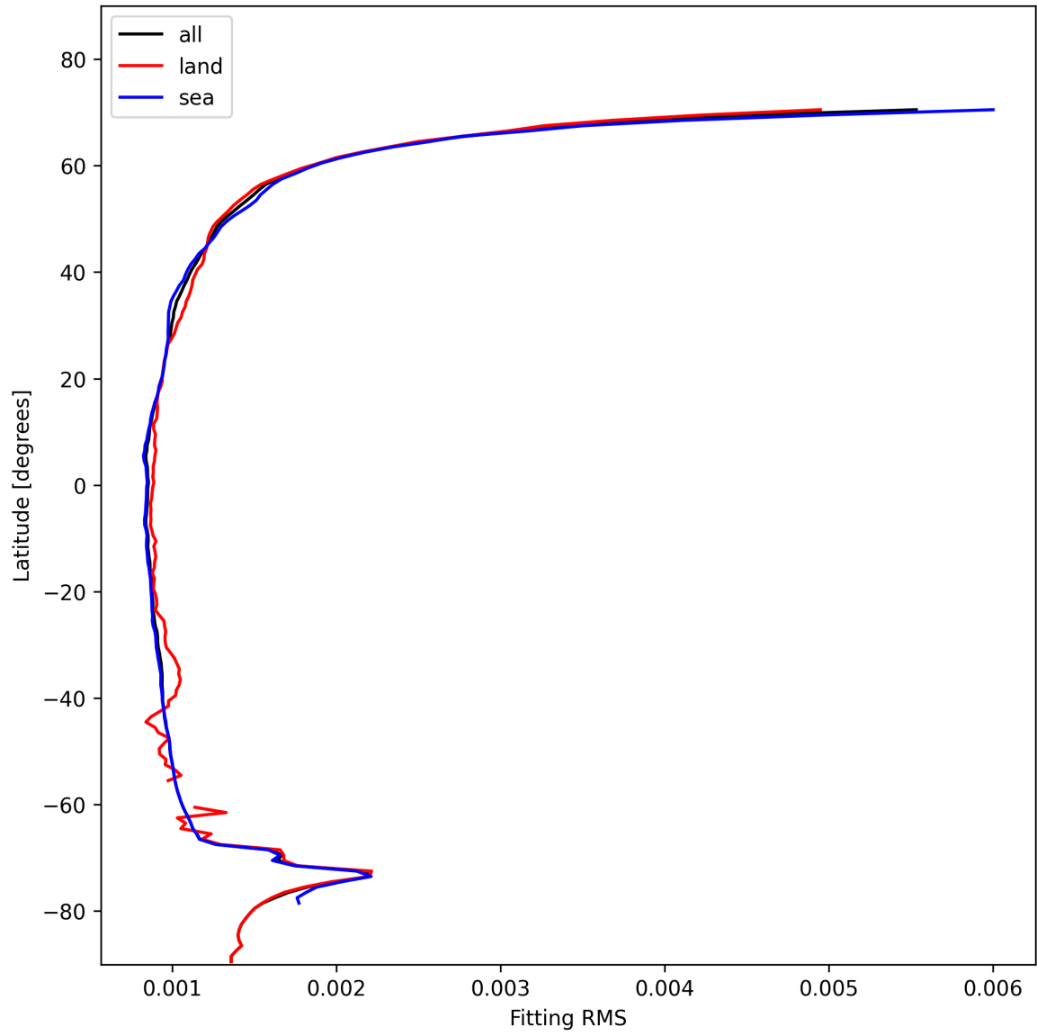
Figure 16: Zonal average of “Fitting RMS” for 2025-11-13 to 2025-11-15.
