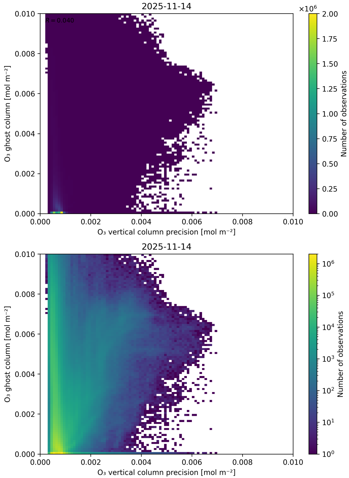
Figure 43: Scatter density plot of “O 3 vertical column precision” against “O 3 ghost column” for 2025-11-13 to 2025-11-15.
