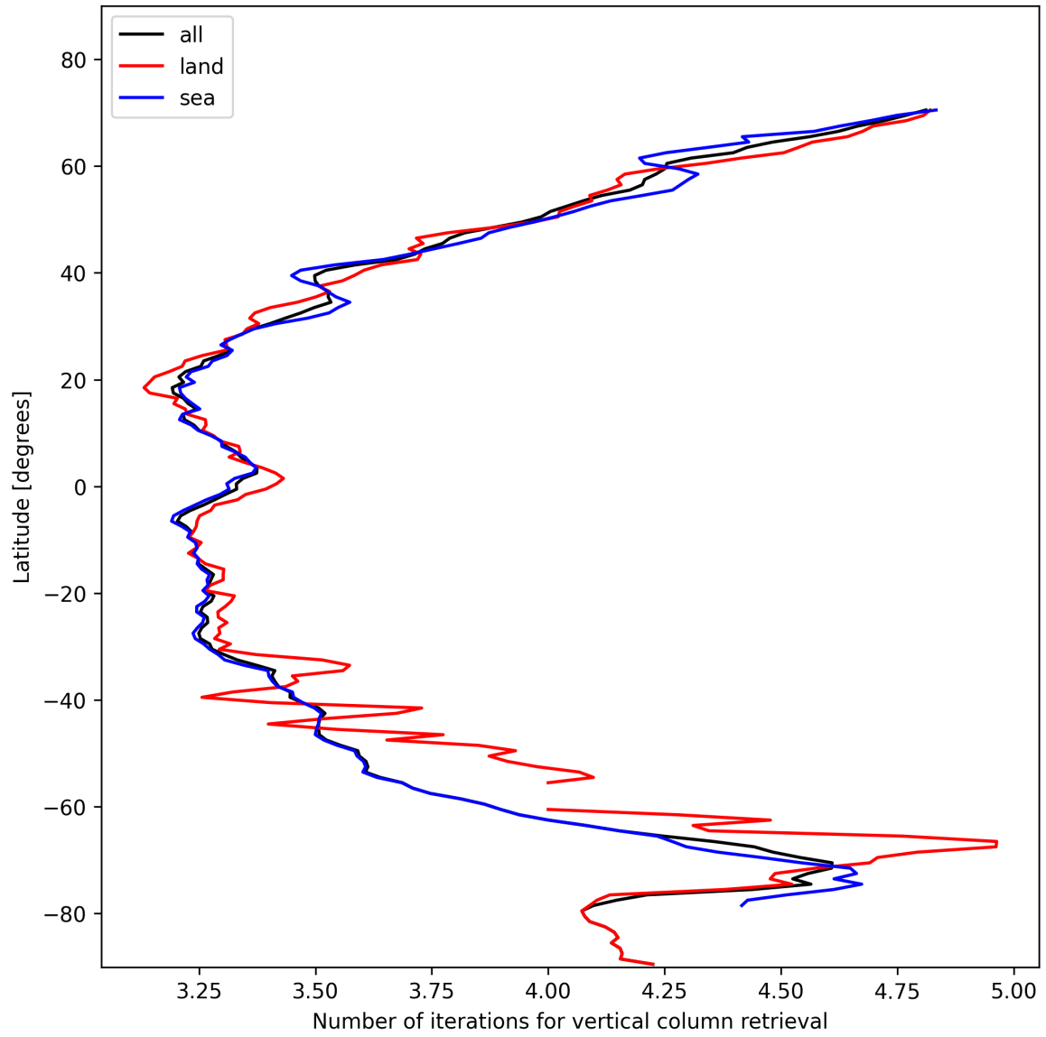
Figure 19: Zonal average of “Number of iterations for vertical column retrieval” for 2025-11-13 to 2025-11-15.
