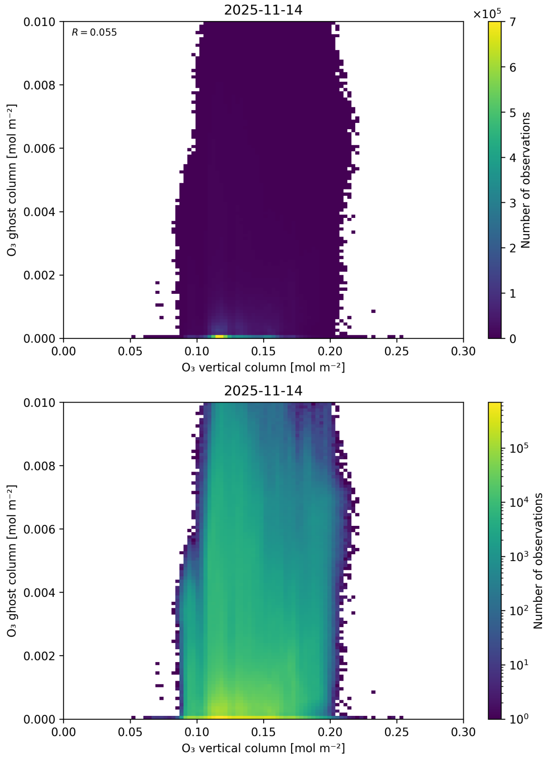
Figure 40: Scatter density plot of “O 3 vertical column” against “O 3 ghost column” for 2025-11-13 to 2025-11-15.
