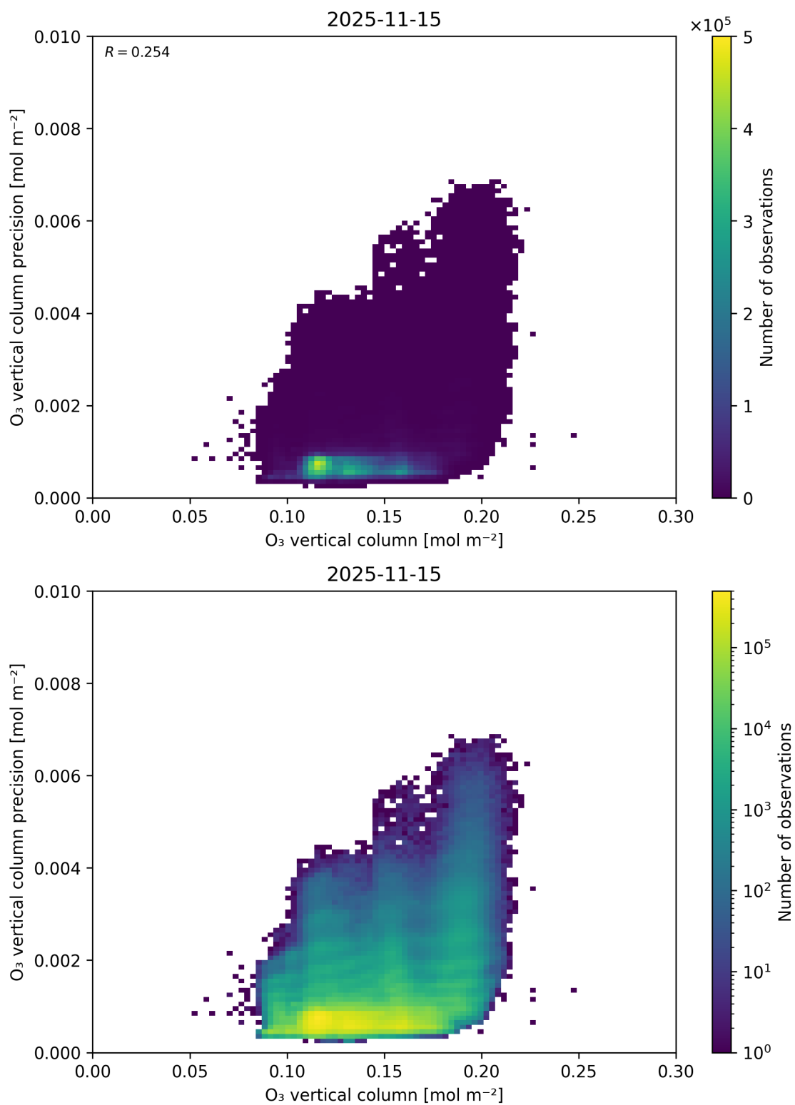
Figure 41: Scatter density plot of “O 3 vertical column” against “O 3 vertical column precision” for 2025-11-14 to 2025-11-16.
