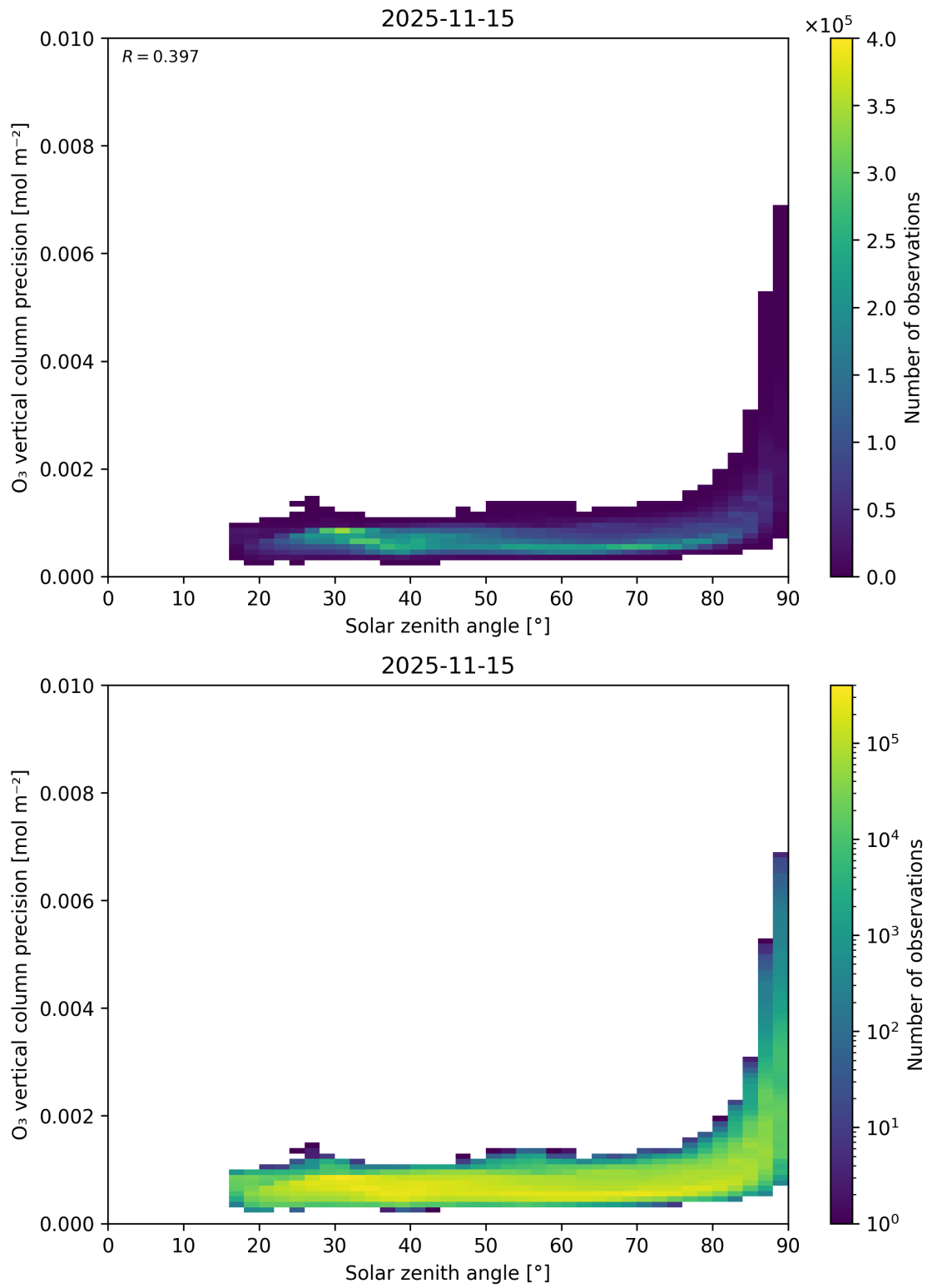
Figure 48: Scatter density plot of “Solar zenith angle” against “O 3 vertical column precision” for 2025-11-14 to 2025-11-16.
