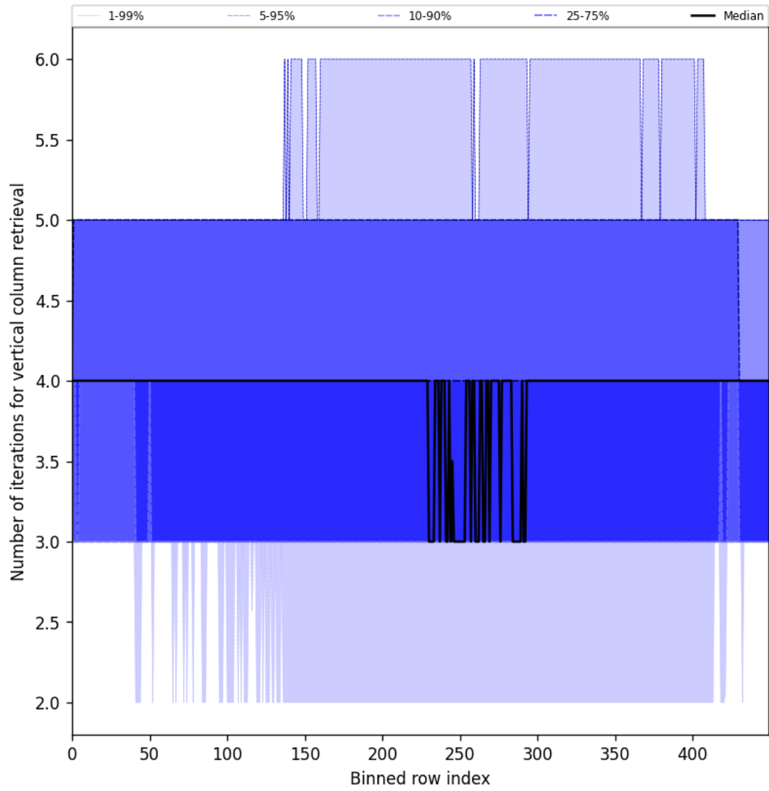
Figure 33: Along track statistics of “Number of iterations for vertical column retrieval” for 2025-11-14 to 2025-11-16
