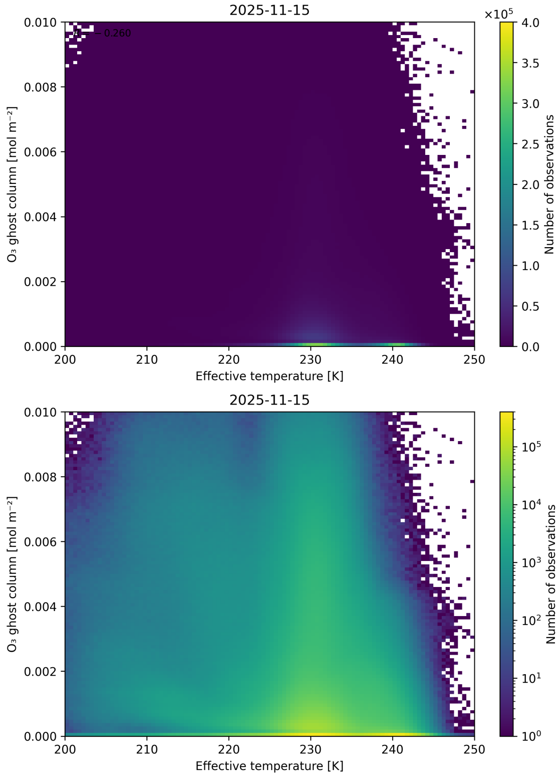
Figure 38: Scatter density plot of “Effective temperature” against “O 3 ghost column” for 2025-11-14 to 2025-11-16.
