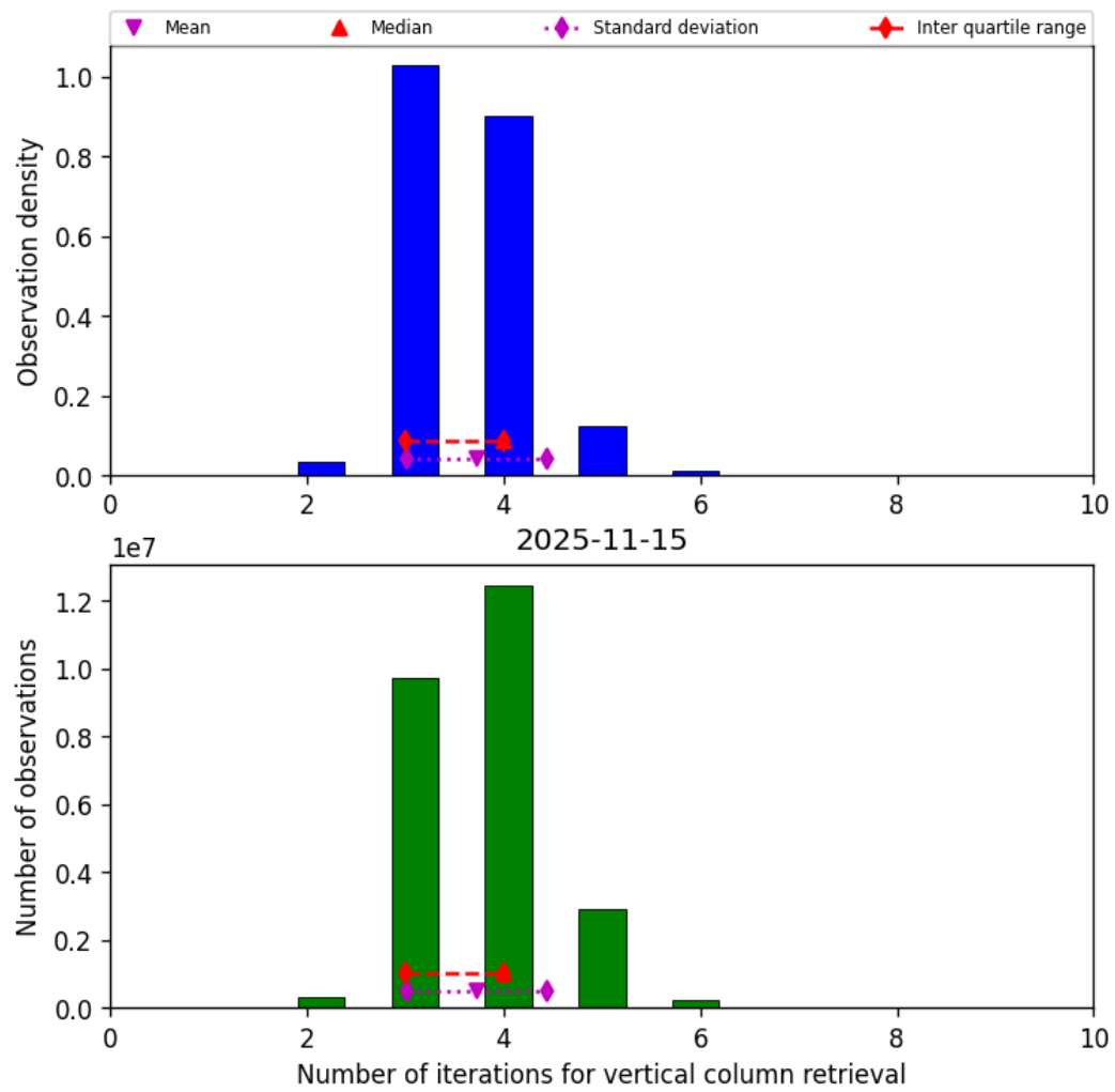
Figure 26: Histogram of “Number of iterations for vertical column retrieval” for 2025-11-14 to 2025-11-16
