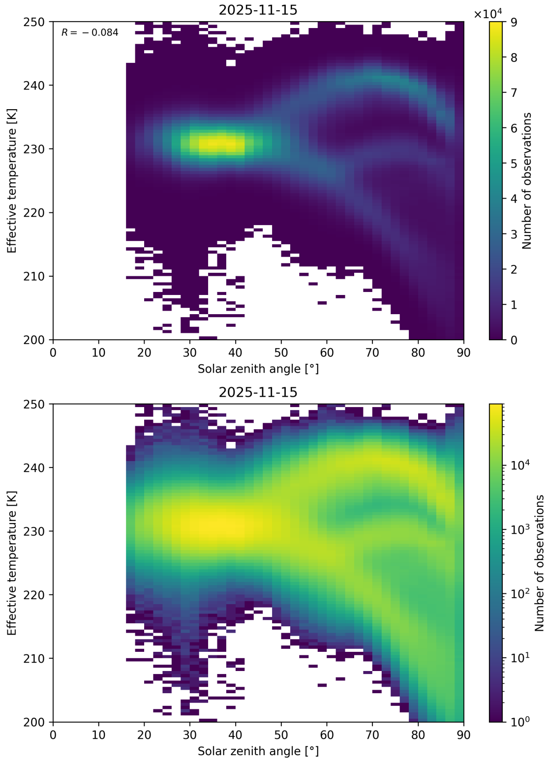
Figure 45: Scatter density plot of “Solar zenith angle” against “Effective temperature” for 2025-11-14 to 2025-11-16.
