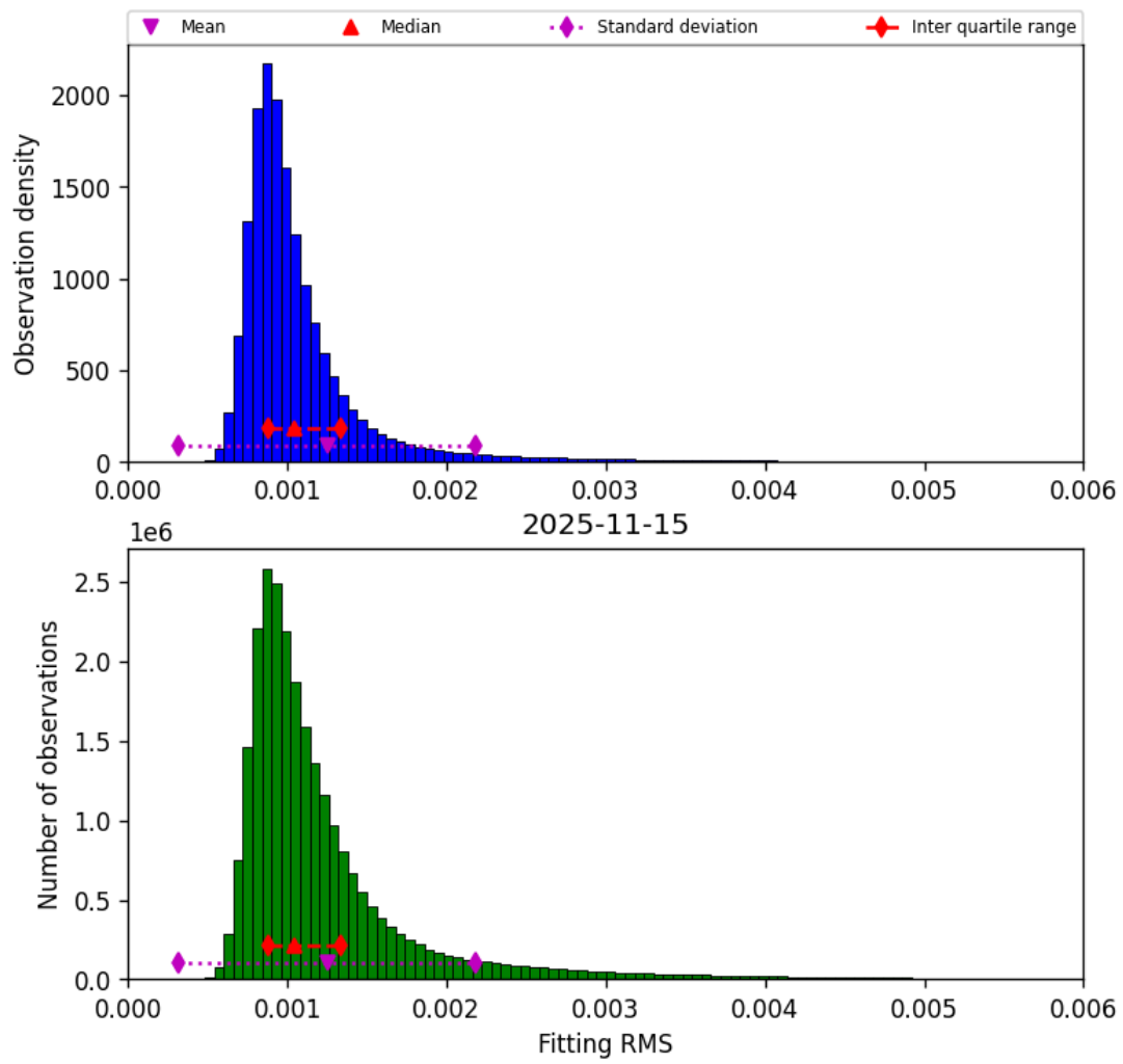
Figure 23: Histogram of “Fitting RMS” for 2025-11-14 to 2025-11-16
