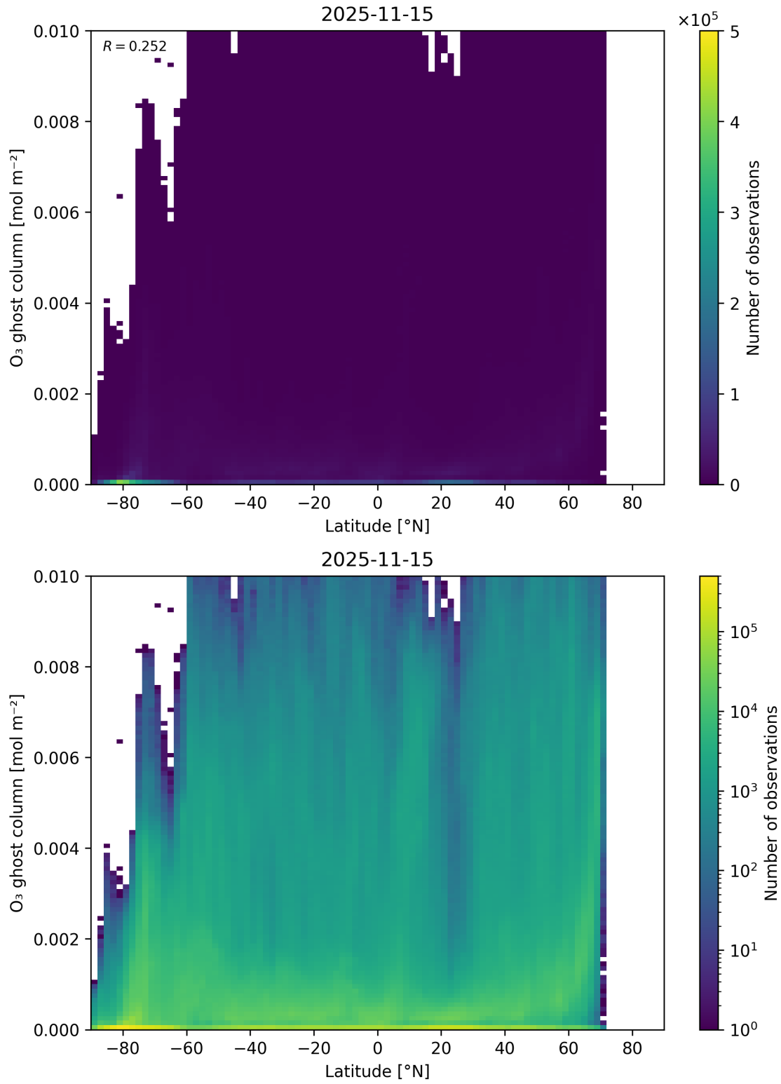
Figure 35: Scatter density plot of “Latitude” against “O 3 ghost column” for 2025-11-14 to 2025-11-16.
