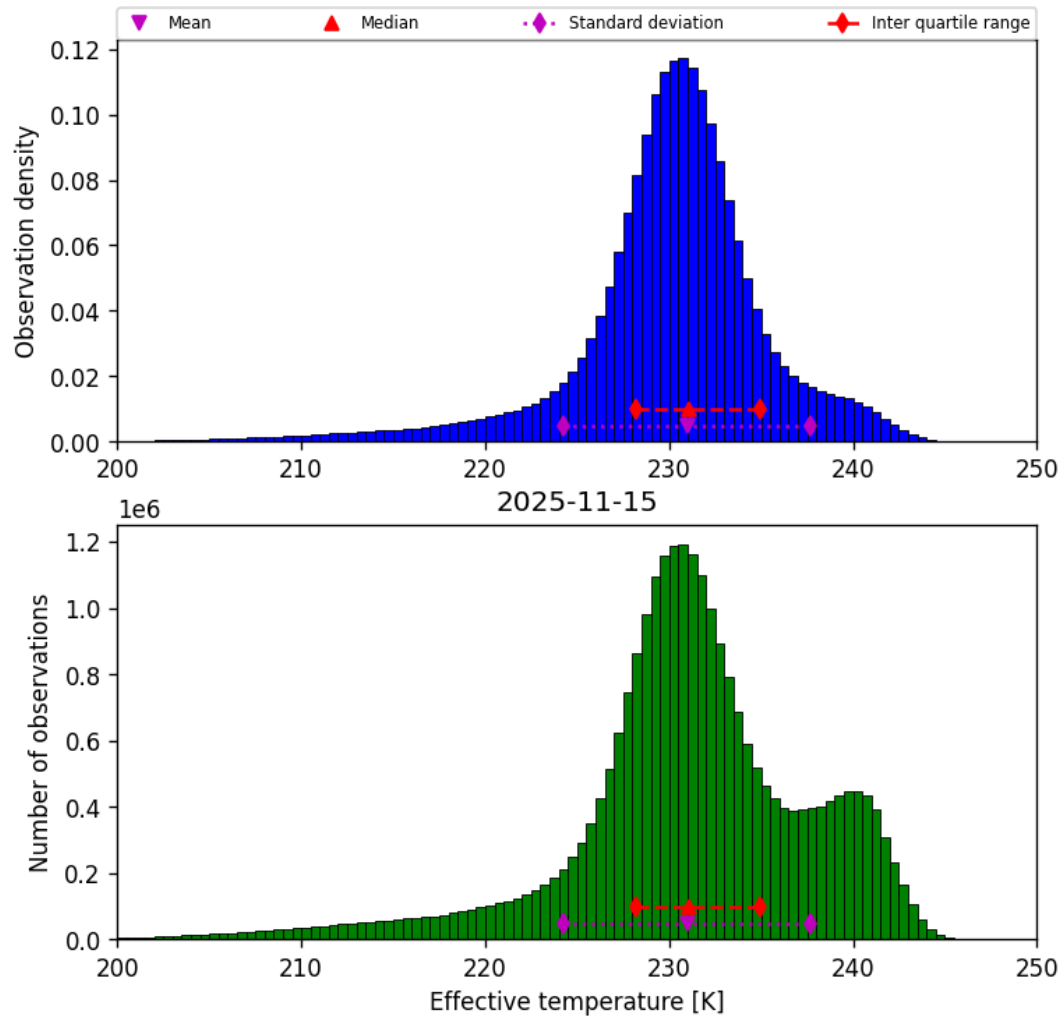
Figure 24: Histogram of “Effective temperature” for 2025-11-14 to 2025-11-16
