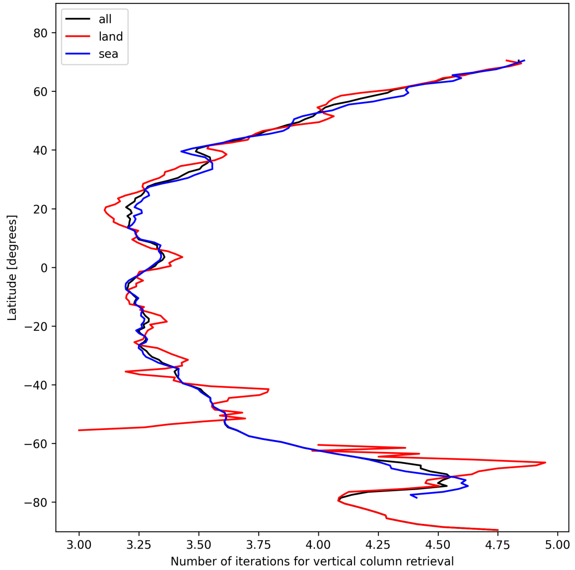
Figure 19: Zonal average of “Number of iterations for vertical column retrieval” for 2025-11-14 to 2025-11-16.
