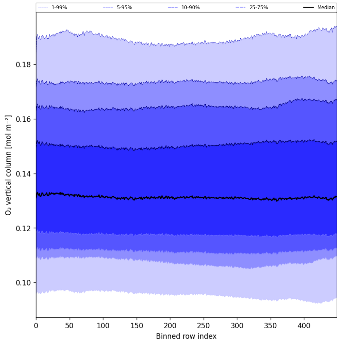
Figure 28: Along track statistics of “O 3 vertical column” for 2025-11-14 to 2025-11-16
