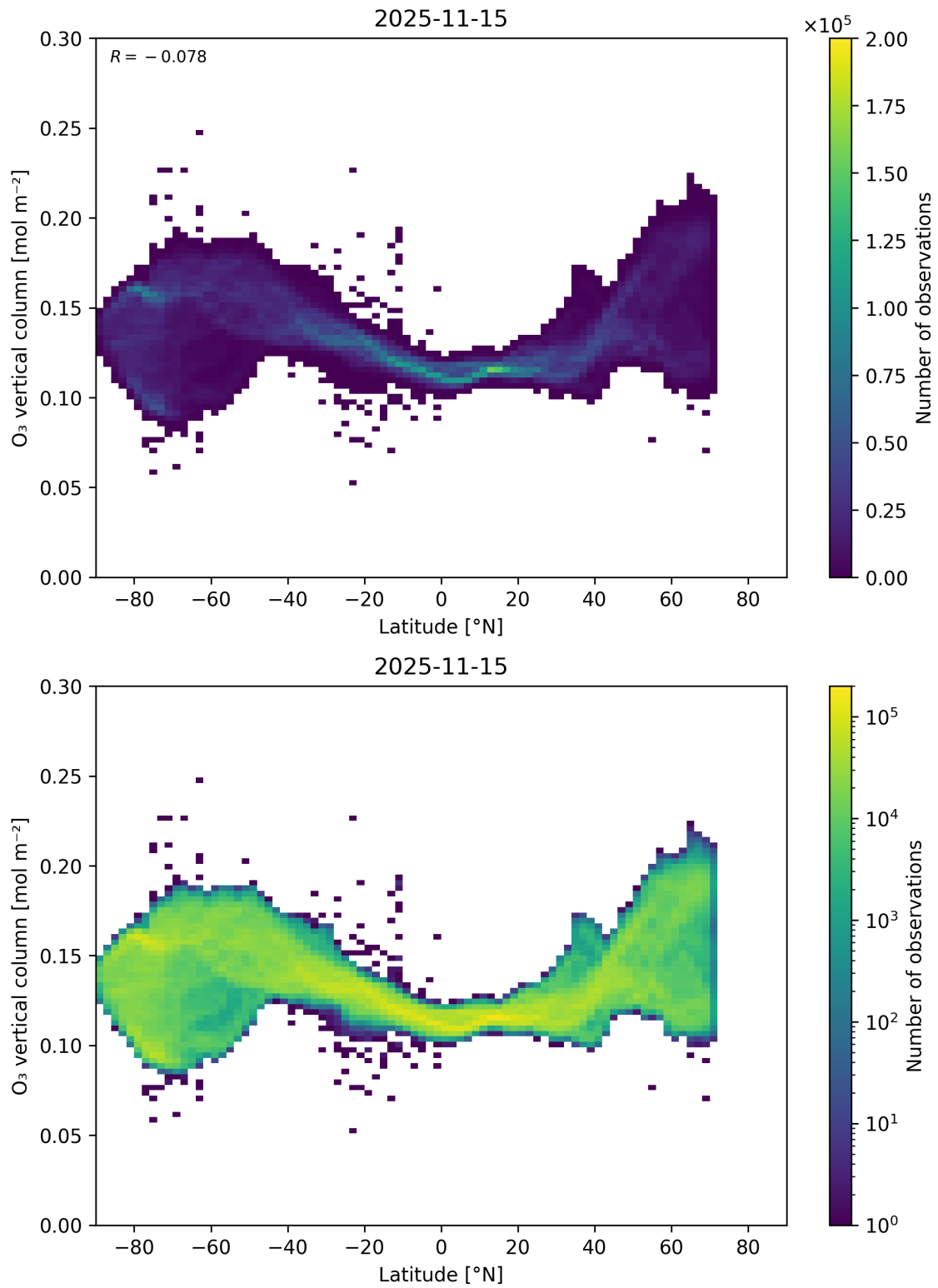
Figure 36: Scatter density plot of “Latitude” against “O 3 vertical column” for 2025-11-14 to 2025-11-16.
