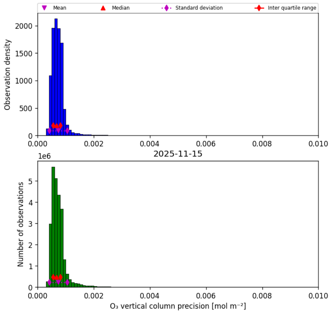
Figure 22: Histogram of “O 3 vertical column precision” for 2025-11-14 to 2025-11-16
