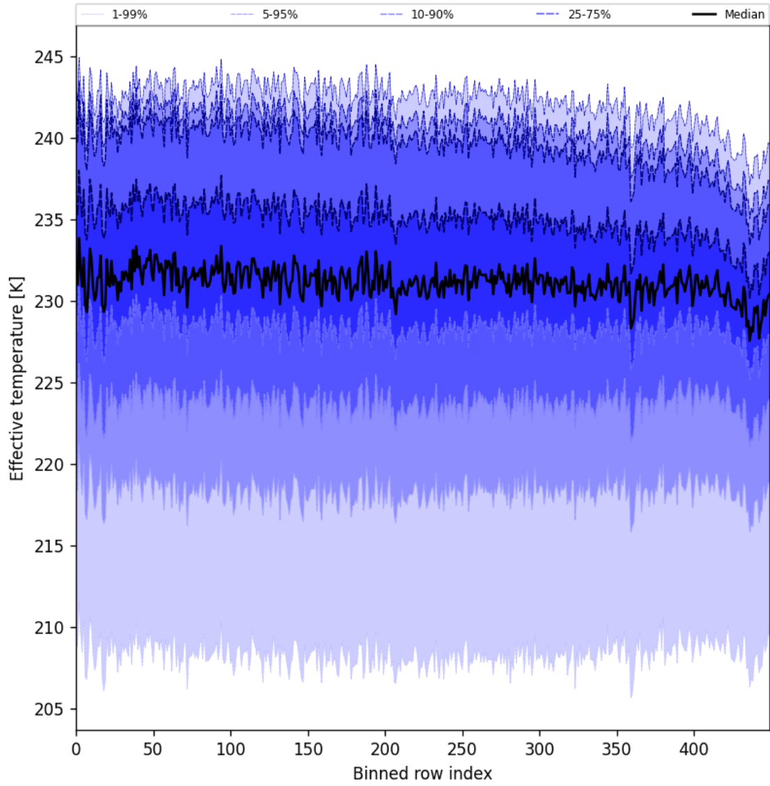
Figure 31: Along track statistics of “Effective temperature” for 2025-11-14 to 2025-11-16
