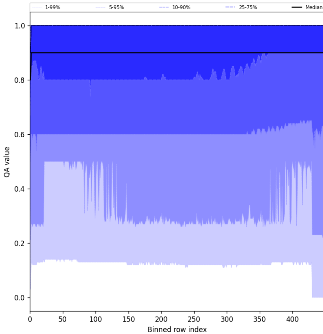
Figure 27: Along track statistics of “QA value” for 2025-11-14 to 2025-11-16
