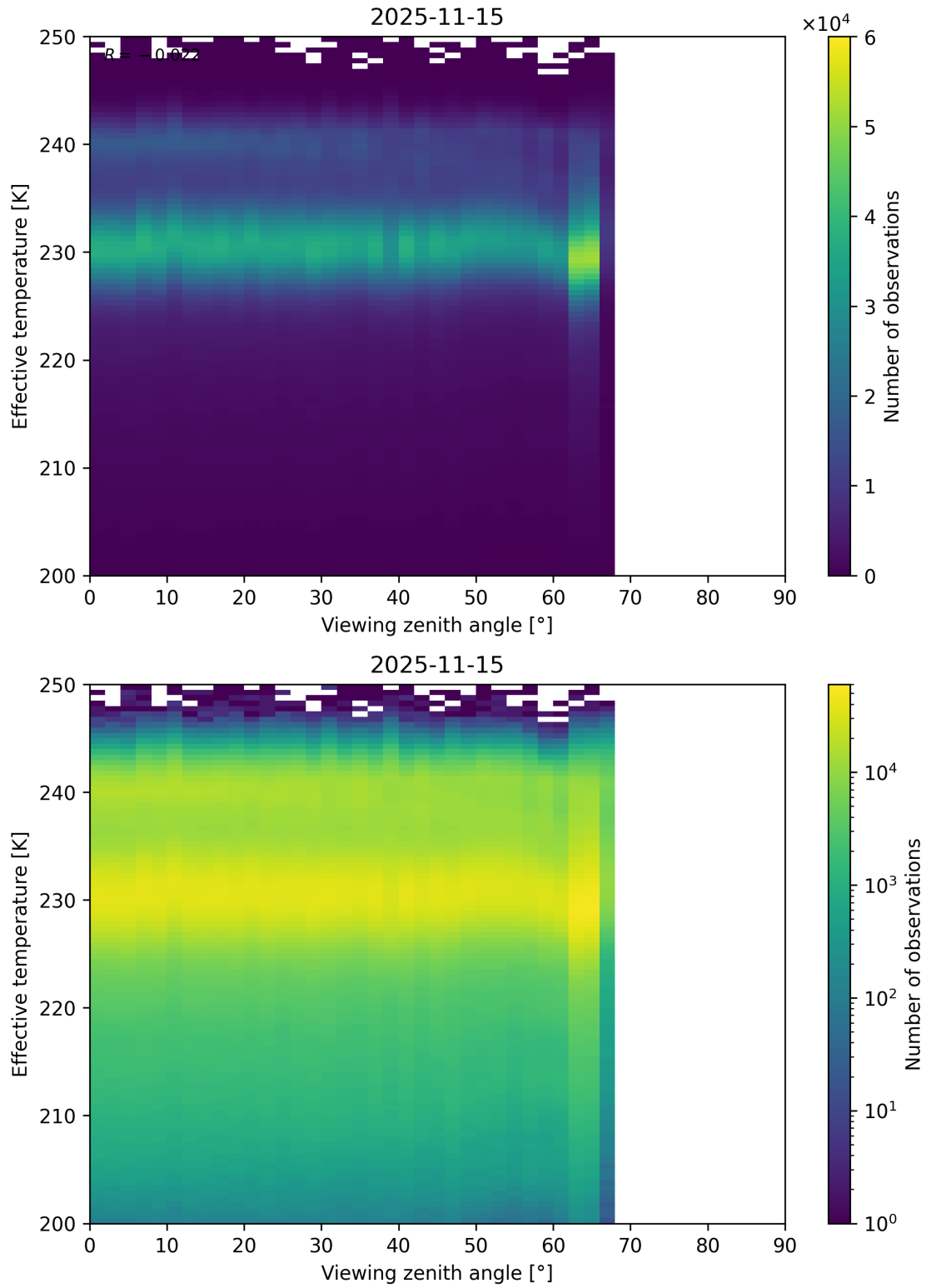
Figure 50: Scatter density plot of “Viewing zenith angle” against “Effective temperature” for 2025-11-14 to 2025-11-16.
