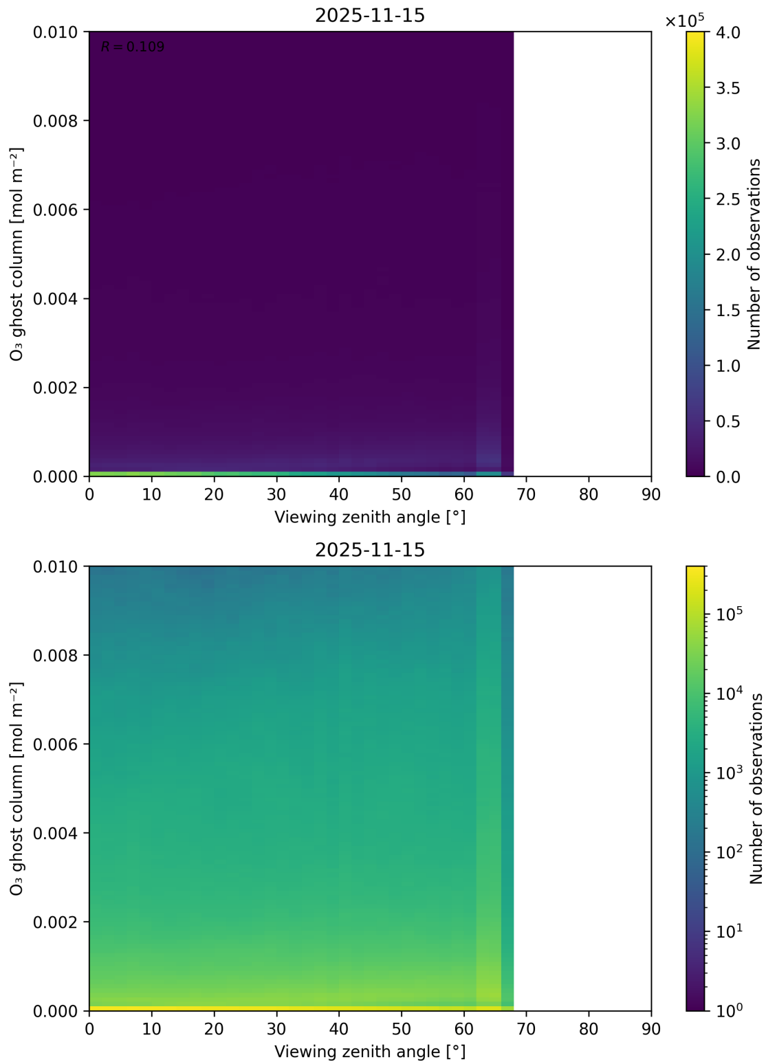
Figure 51: Scatter density plot of “Viewing zenith angle” against “O 3 ghost column” for 2025-11-14 to 2025-11-16.
