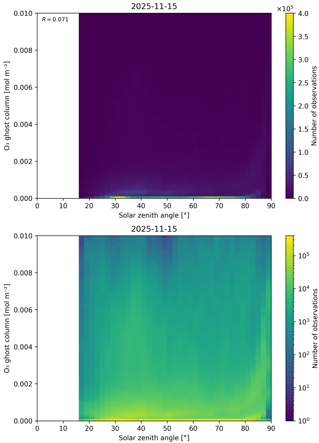
Figure 46: Scatter density plot of “Solar zenith angle” against “O 3 ghost column” for 2025-11-14 to 2025-11-16.
