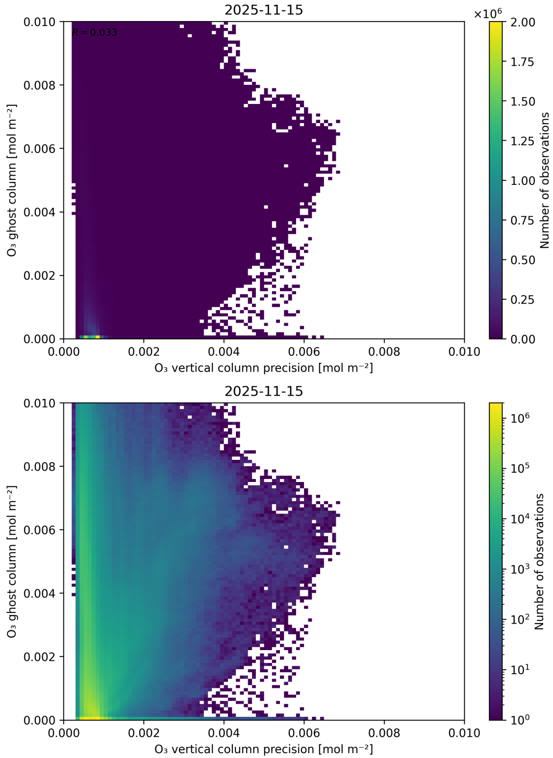
Figure 43: Scatter density plot of “O 3 vertical column precision” against “O 3 ghost column” for 2025-11-14 to 2025-11-16.
