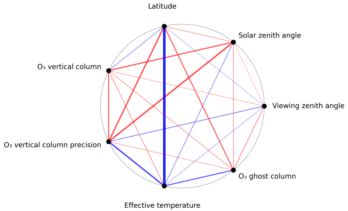
Figure 1: Map of correlation graph for 2025-11-14 to 2025-11-16.
