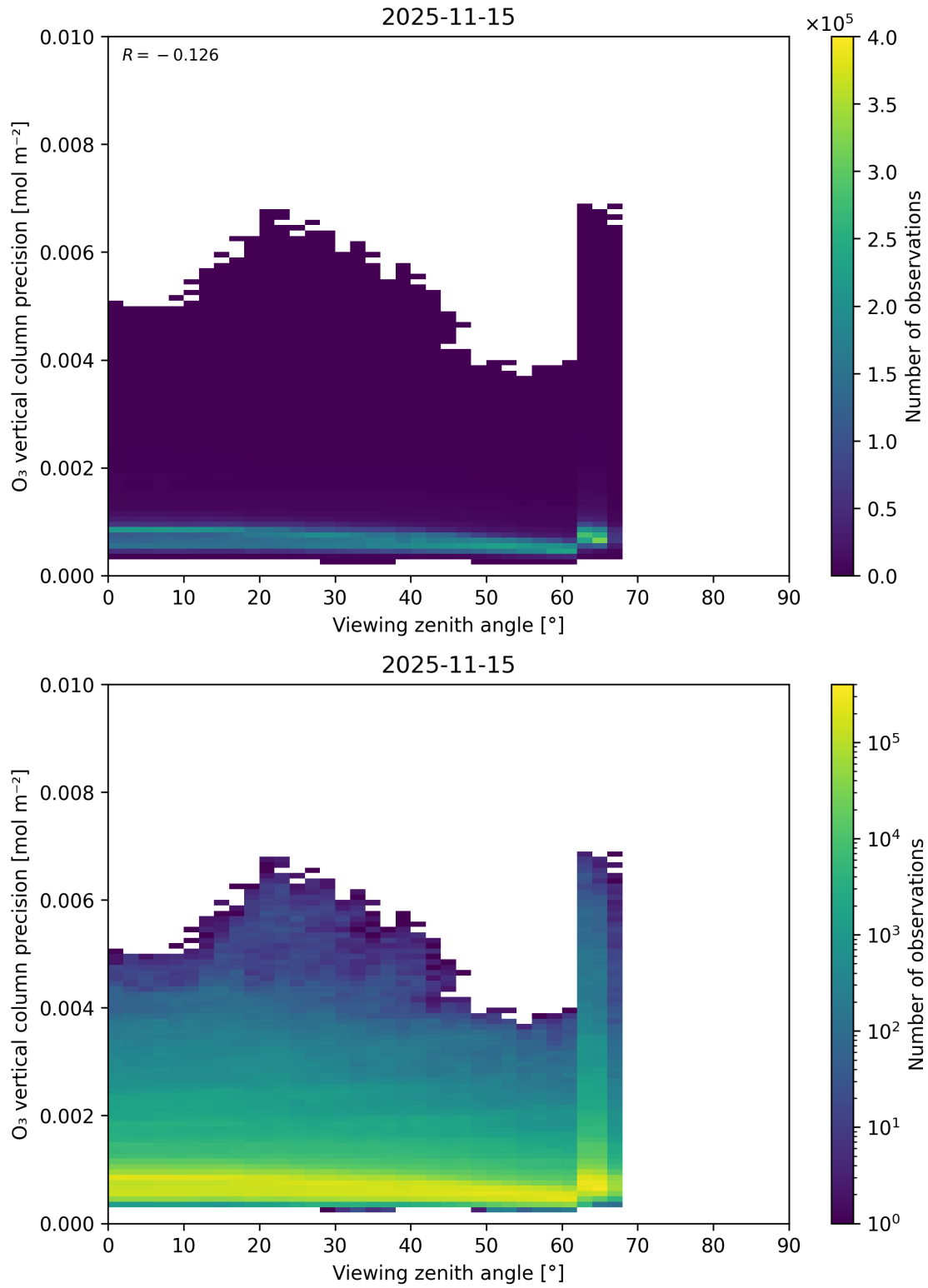
Figure 53: Scatter density plot of “Viewing zenith angle” against “O 3 vertical column precision” for 2025-11-14 to 2025-11-16.
