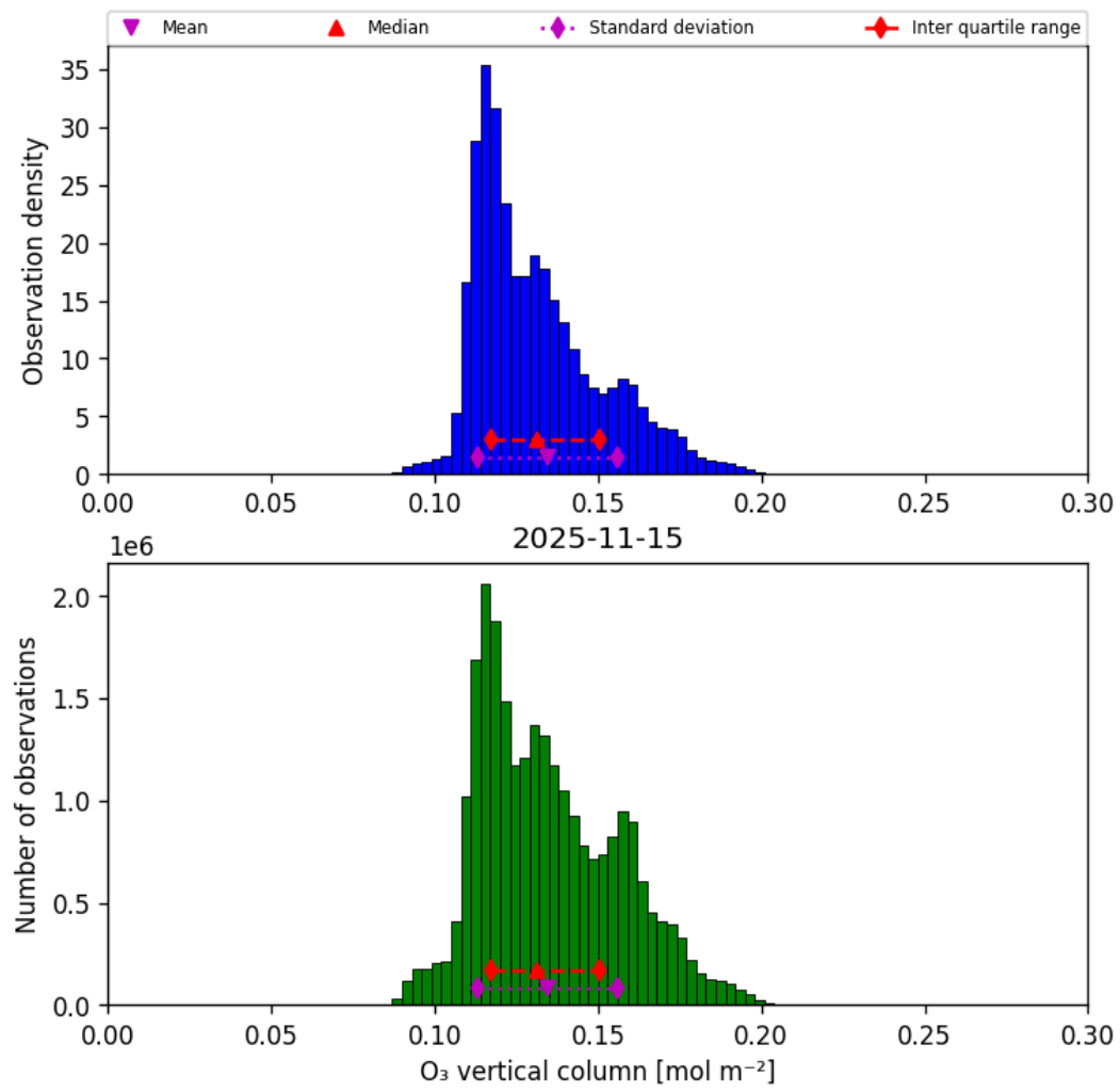
Figure 21: Histogram of “O 3 vertical column” for 2025-11-14 to 2025-11-16
