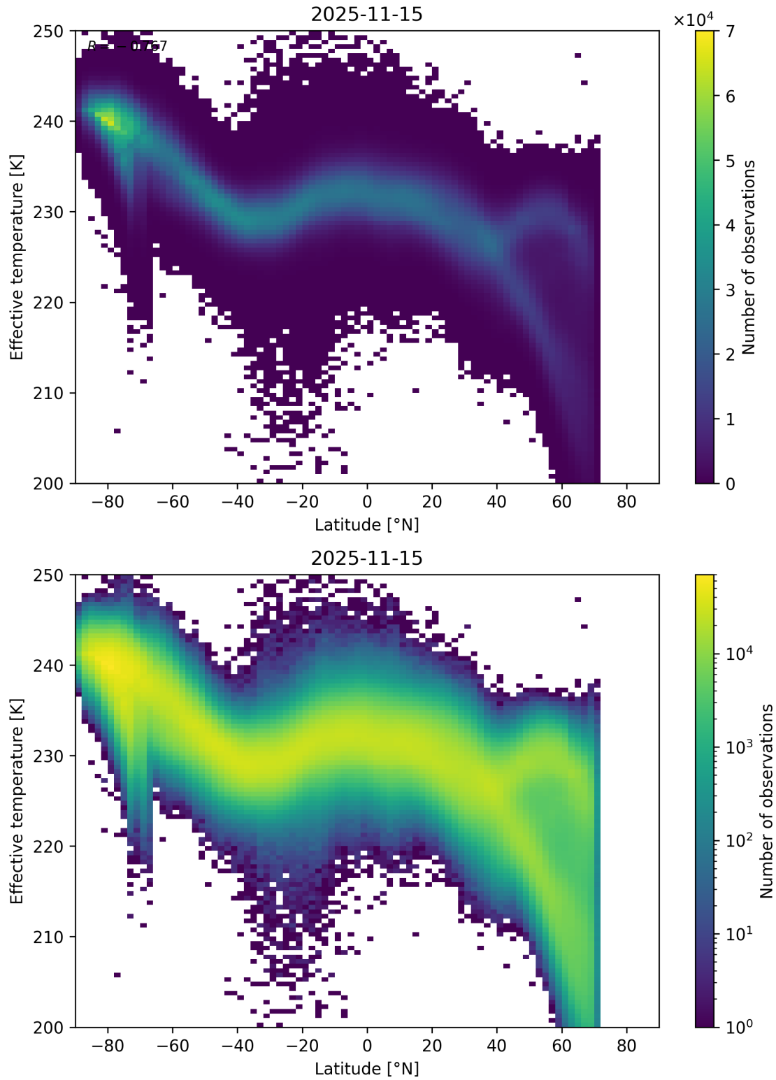
Figure 34: Scatter density plot of “Latitude” against “Effective temperature” for 2025-11-14 to 2025-11-16.
