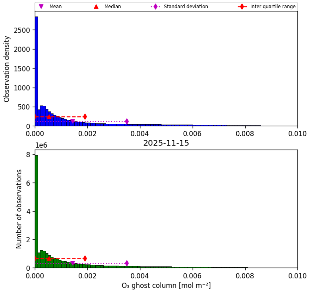
Figure 25: Histogram of “O 3 ghost column” for 2025-11-14 to 2025-11-16
