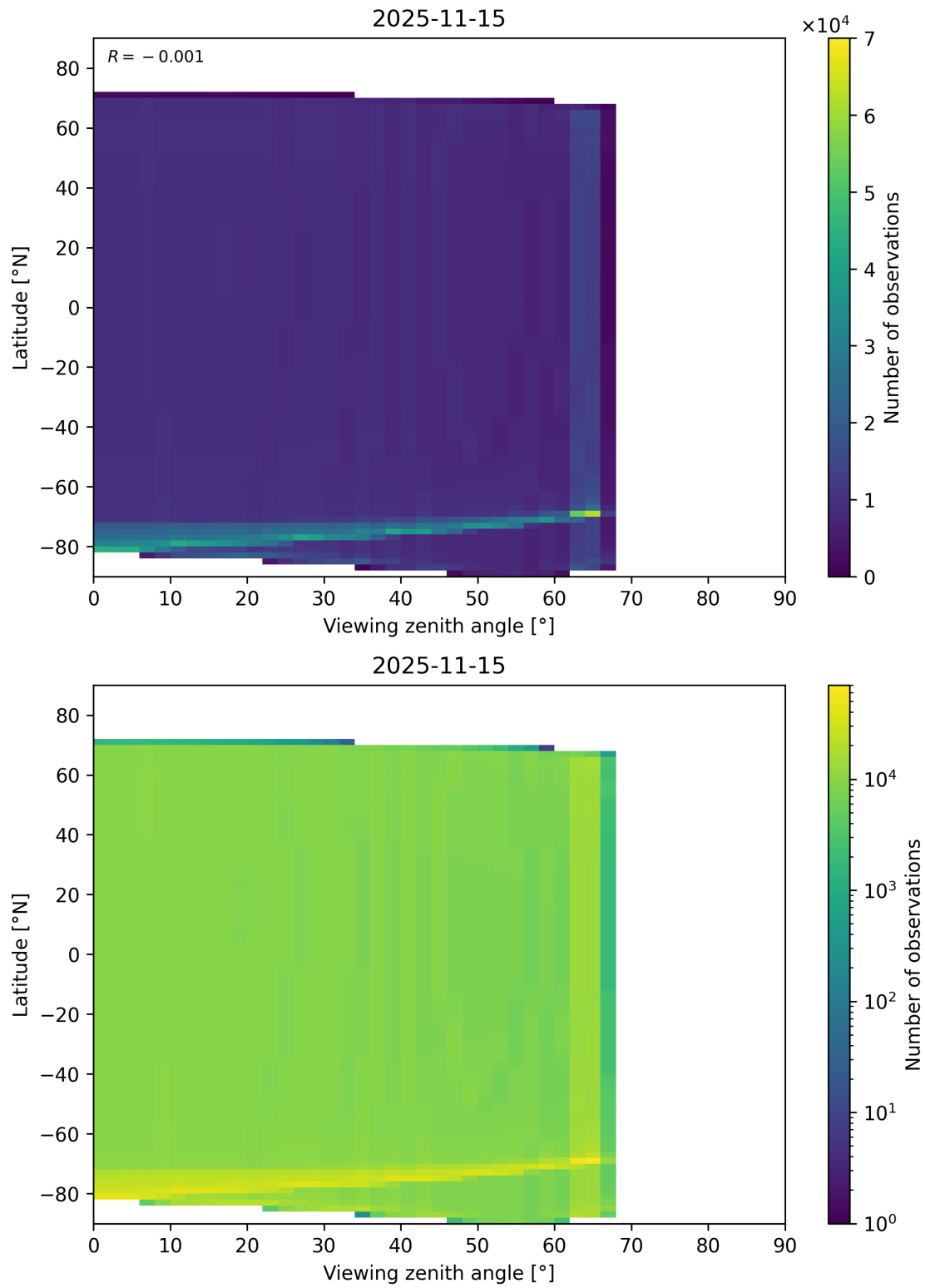
Figure 49: Scatter density plot of “Viewing zenith angle” against “Latitude” for 2025-11-14 to 2025-11-16.
