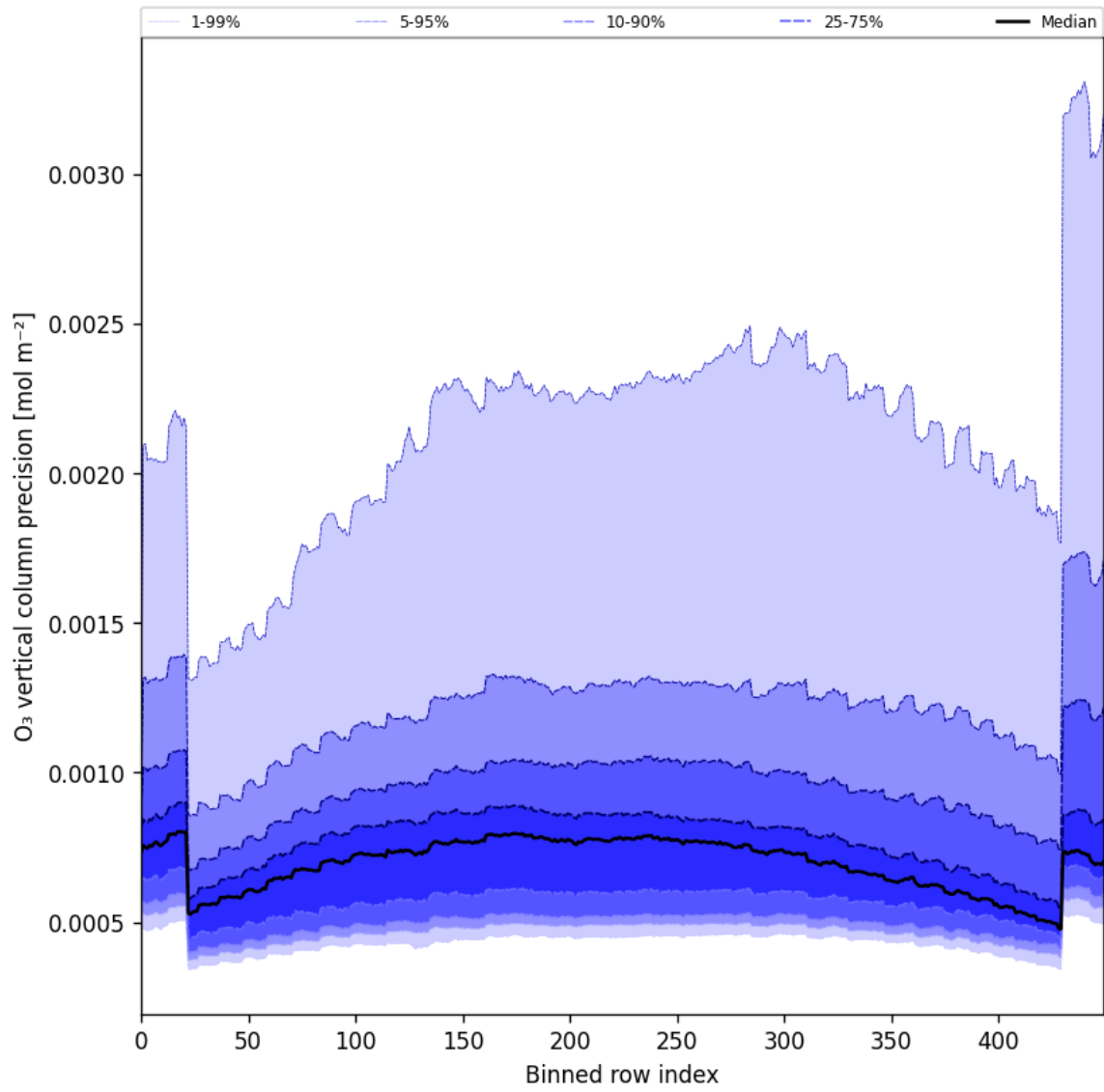
Figure 29: Along track statistics of “O 3 vertical column precision” for 2025-11-14 to 2025-11-16
