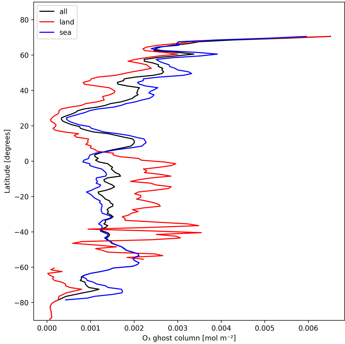
Figure 18: Zonal average of "O 3 ghost column" for 2025-11-14 to 2025-11-16.
