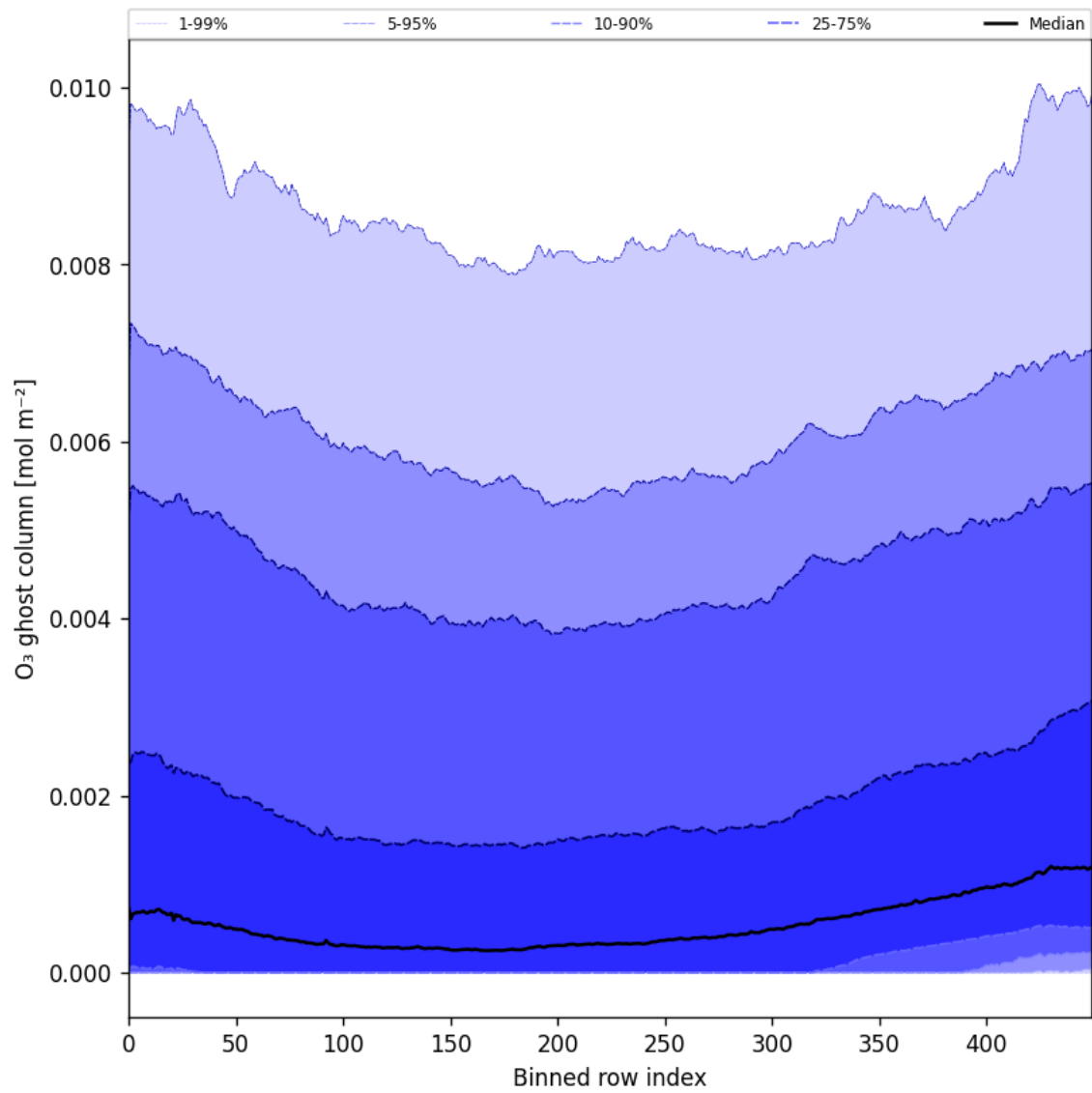
Figure 32: Along track statistics of “O 3 ghost column” for 2025-11-14 to 2025-11-16
