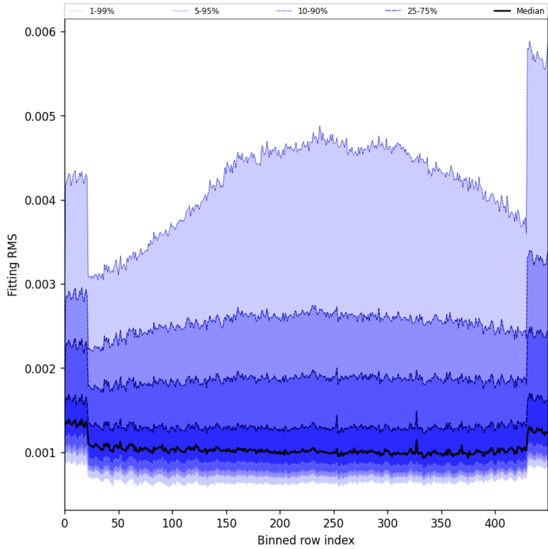
Figure 30: Along track statistics of “Fitting RMS” for 2025-11-14 to 2025-11-16
