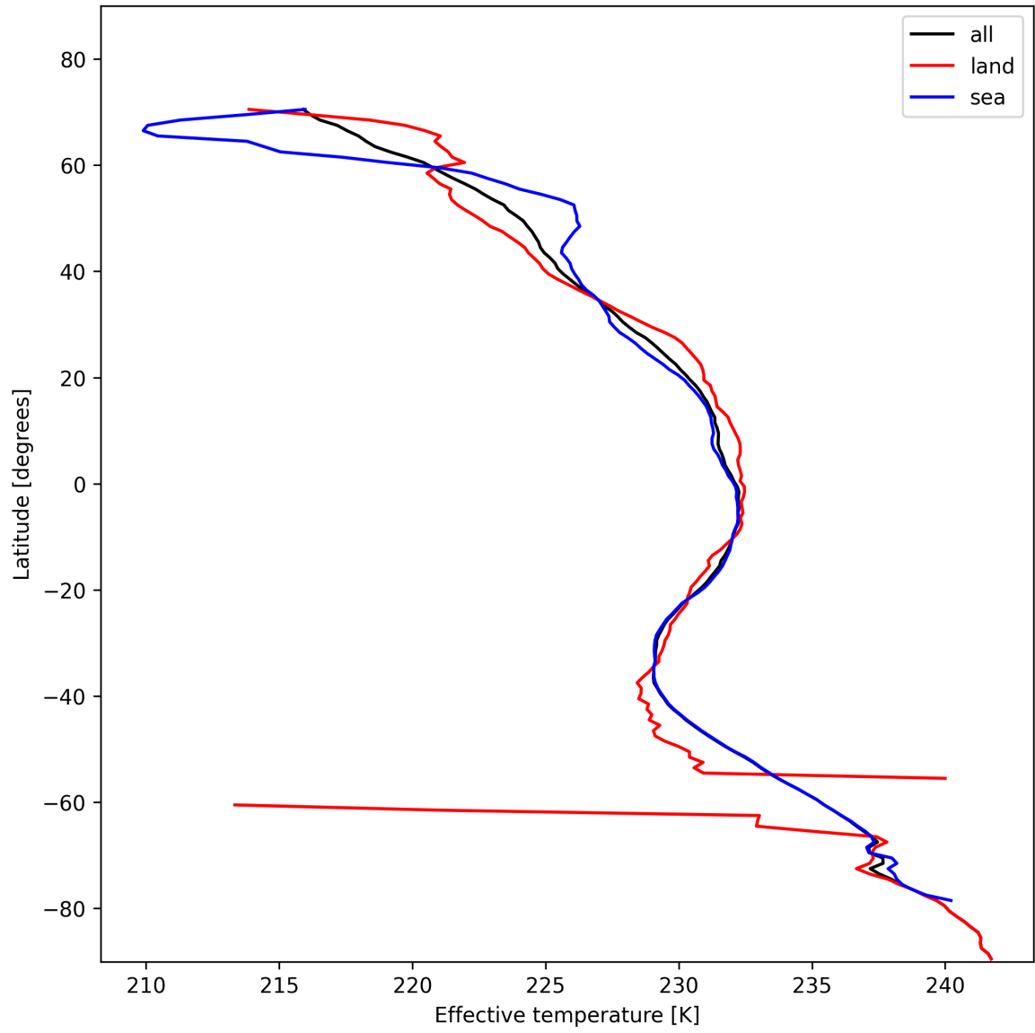
Figure 17: Zonal average of “Effective temperature” for 2025-11-14 to 2025-11-16.
