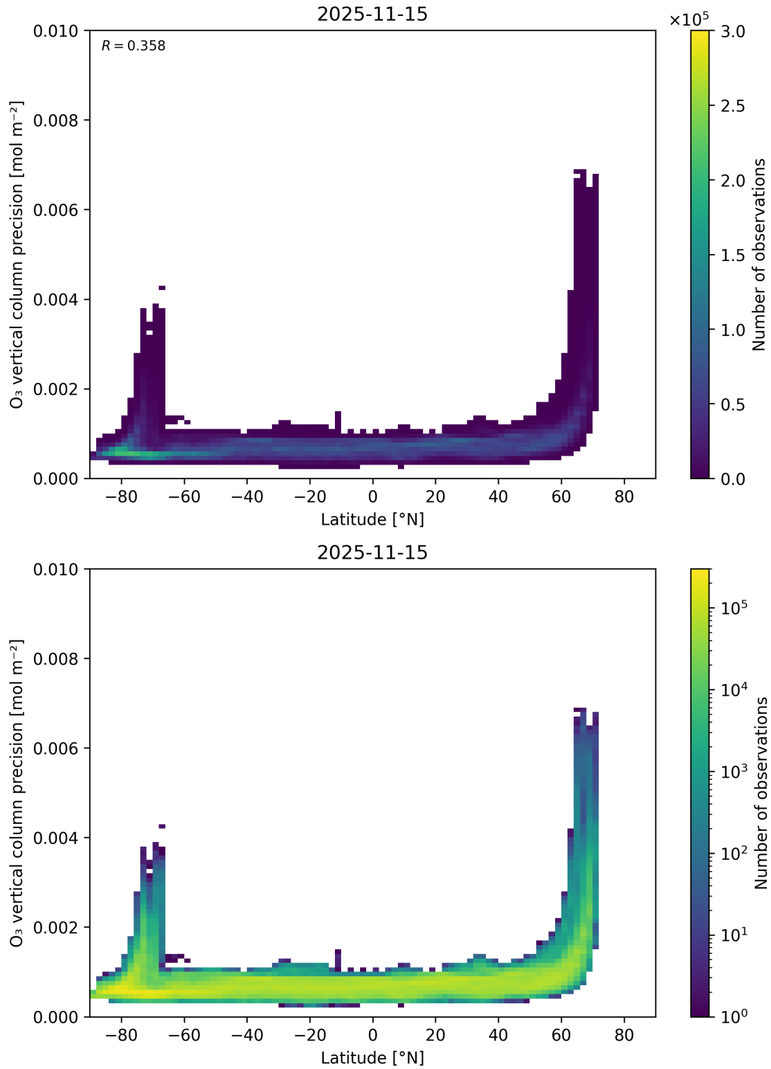
Figure 37: Scatter density plot of “Latitude” against “O 3 vertical column precision” for 2025-11-14 to 2025-11-16.
