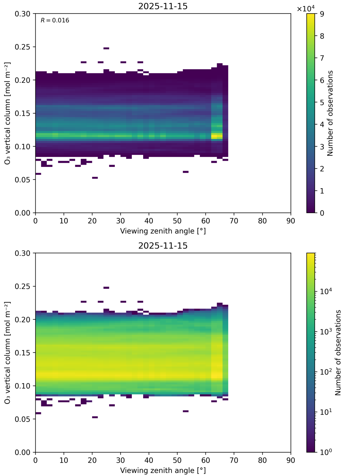
Figure 52: Scatter density plot of “Viewing zenith angle” against “O 3 vertical column” for 2025-11-14 to 2025-11-16.
