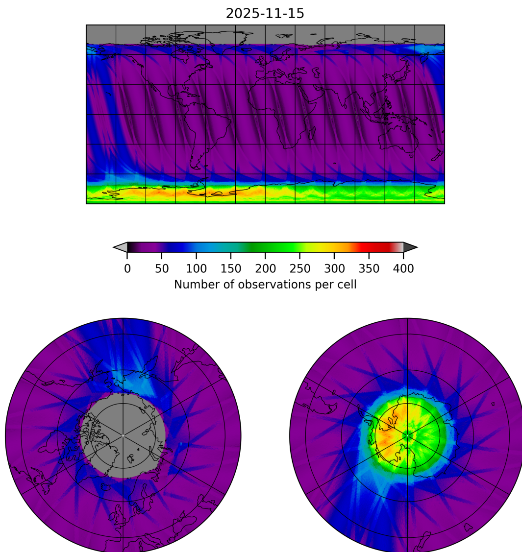
Figure 12: Map of the number of observations for 2025-11-14 to 2025-11-16
