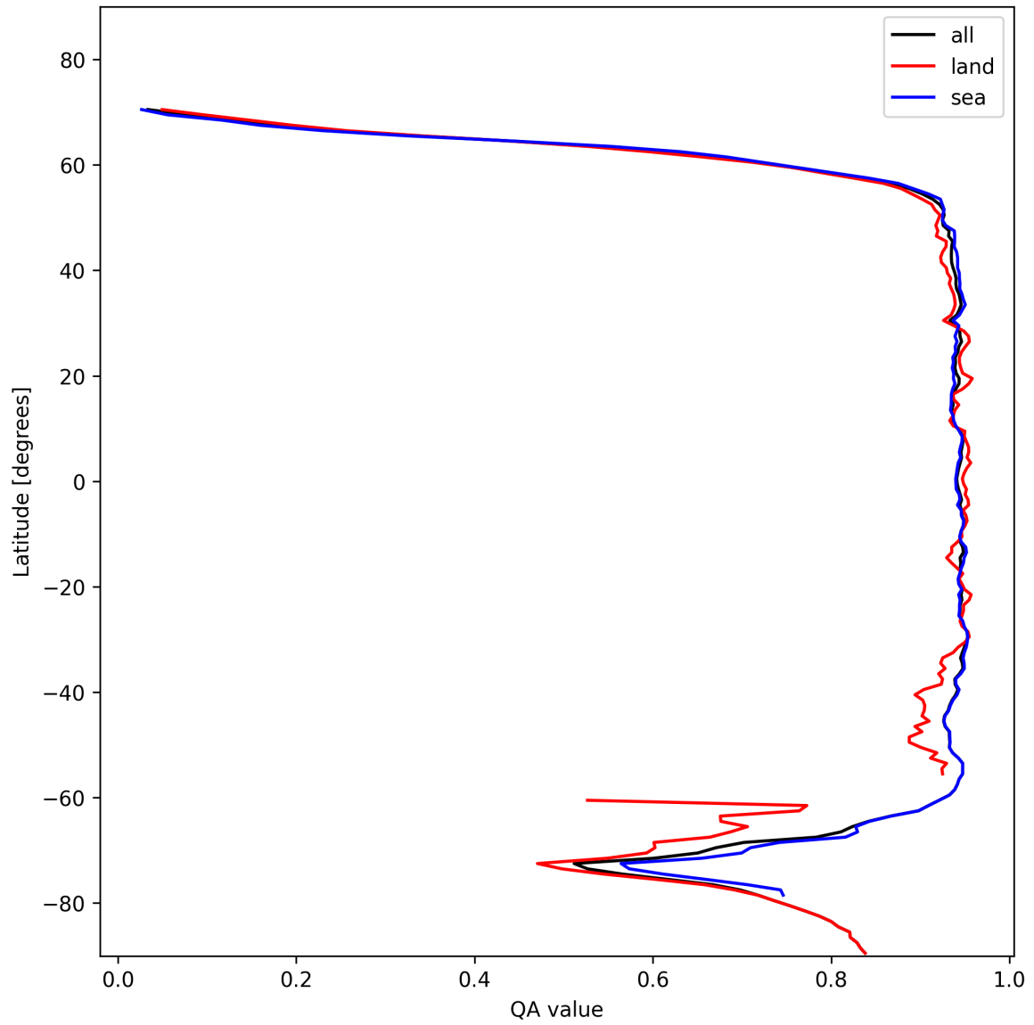
Figure 13: Zonal average of “QA value” for 2025-11-14 to 2025-11-16.
