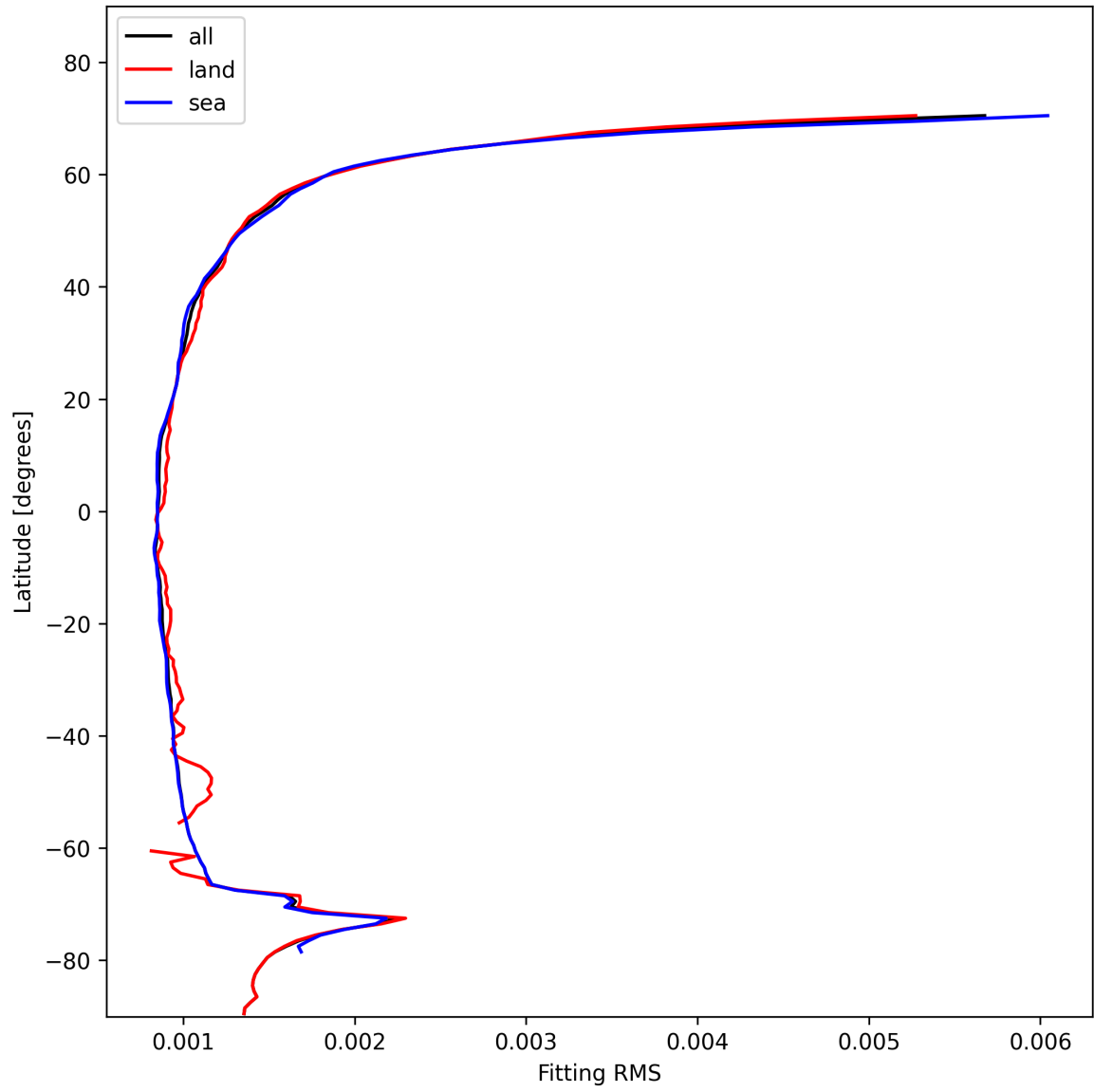
Figure 16: Zonal average of “Fitting RMS” for 2025-11-14 to 2025-11-16.
