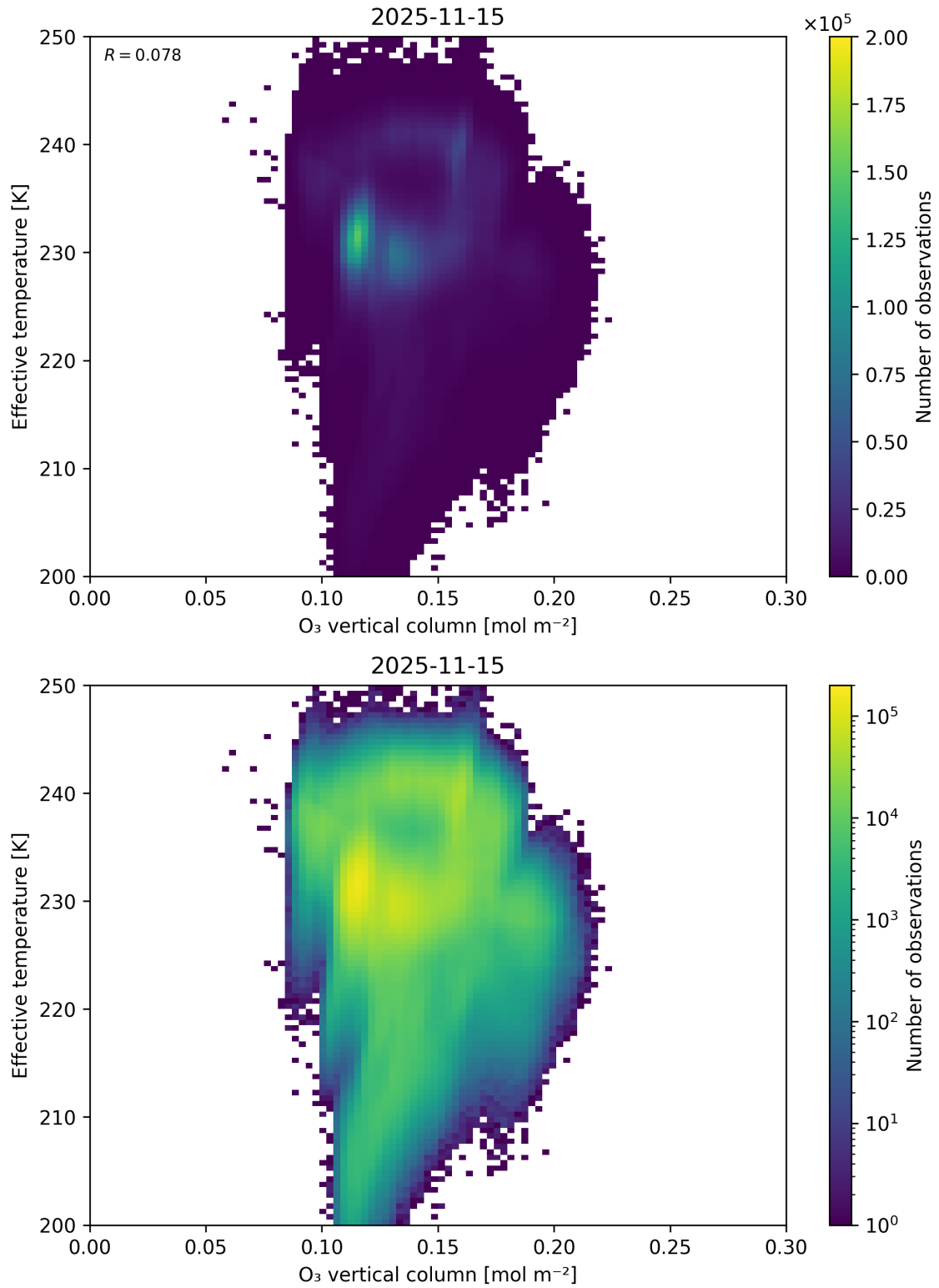
Figure 39: Scatter density plot of “O 3 vertical column” against “Effective temperature” for 2025-11-14 to 2025-11-16.
