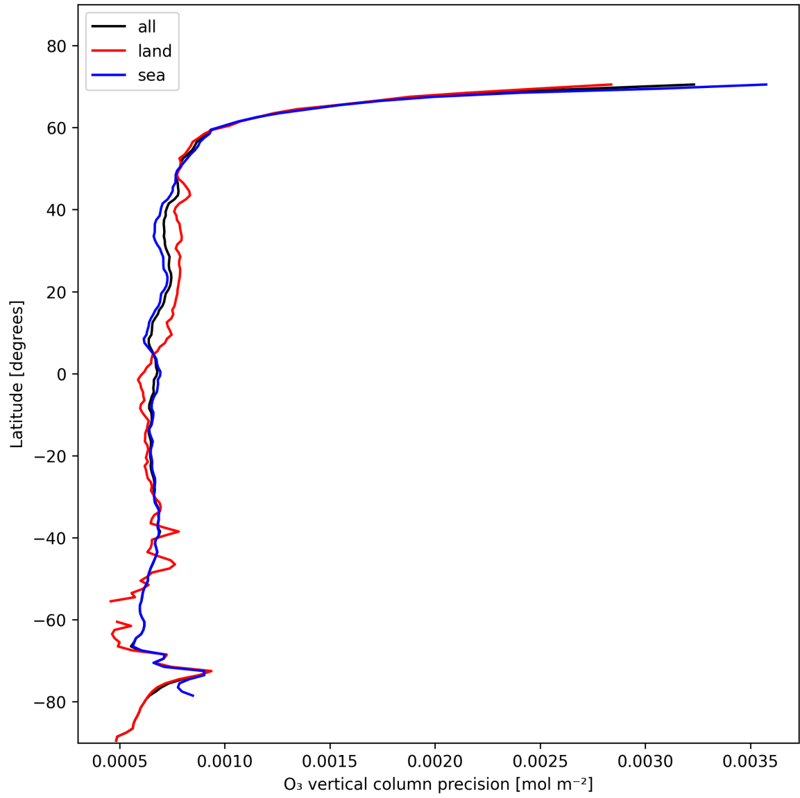
Figure 15: Zonal average of “O 3 vertical column precision” for 2025-11-14 to 2025-11-16.
