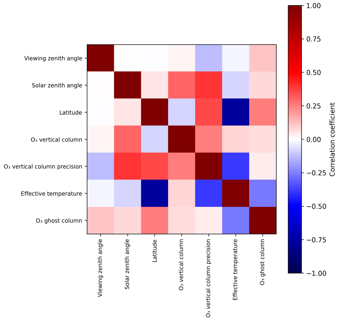
Figure 2: Map of correlation matrix for 2025-11-14 to 2025-11-16.
