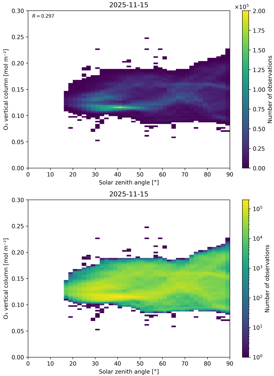
Figure 47: Scatter density plot of “Solar zenith angle” against “O 3 vertical column” for 2025-11-14 to 2025-11-16.
