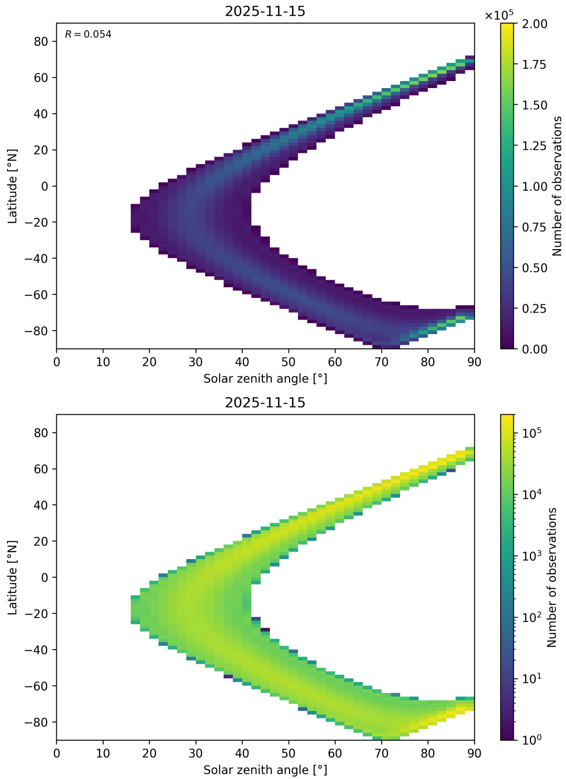
Figure 44: Scatter density plot of “Solar zenith angle” against “Latitude” for 2025-11-14 to 2025-11-16.
