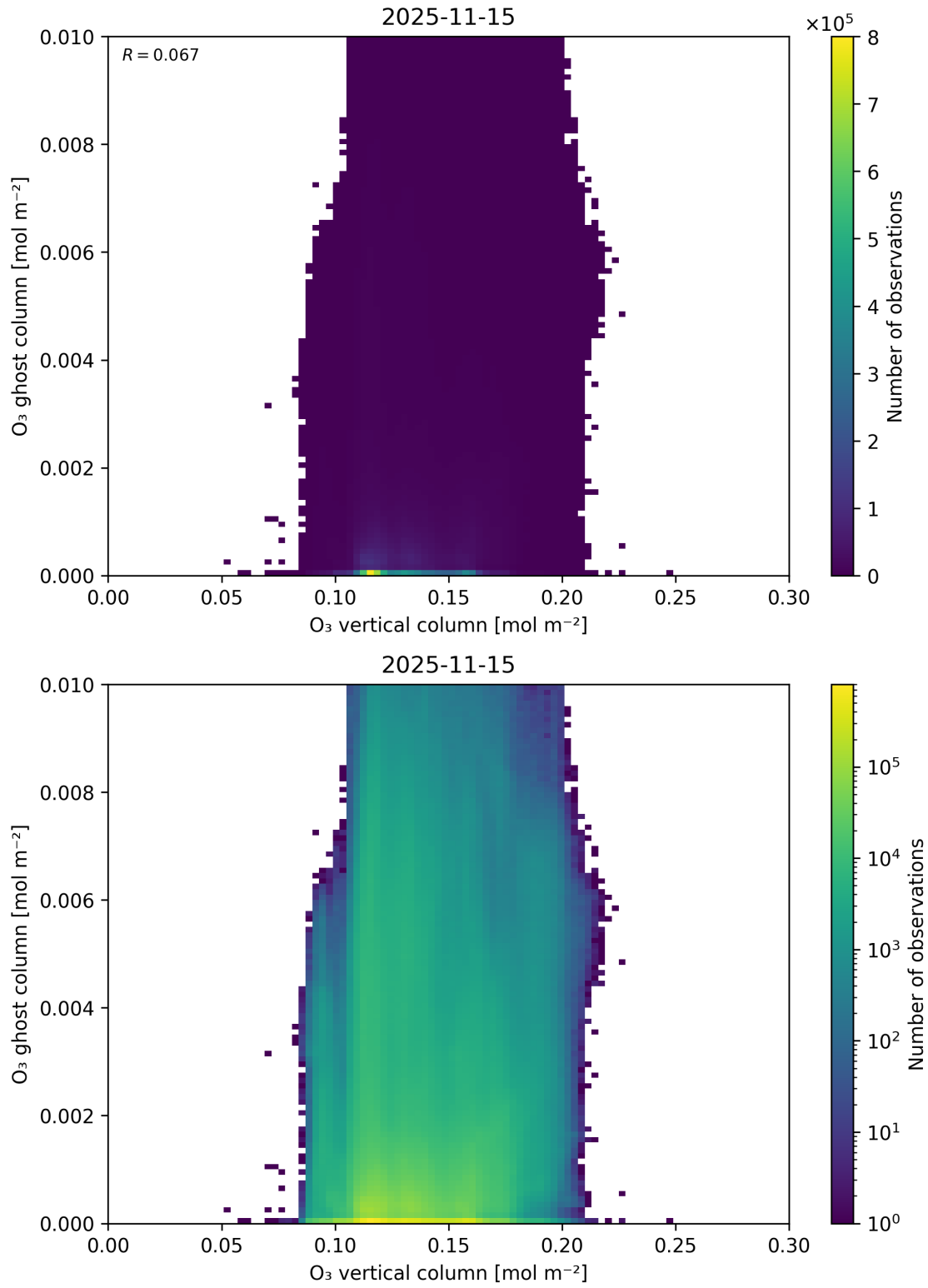
Figure 40: Scatter density plot of “O 3 vertical column” against “O 3 ghost column” for 2025-11-14 to 2025-11-16.
