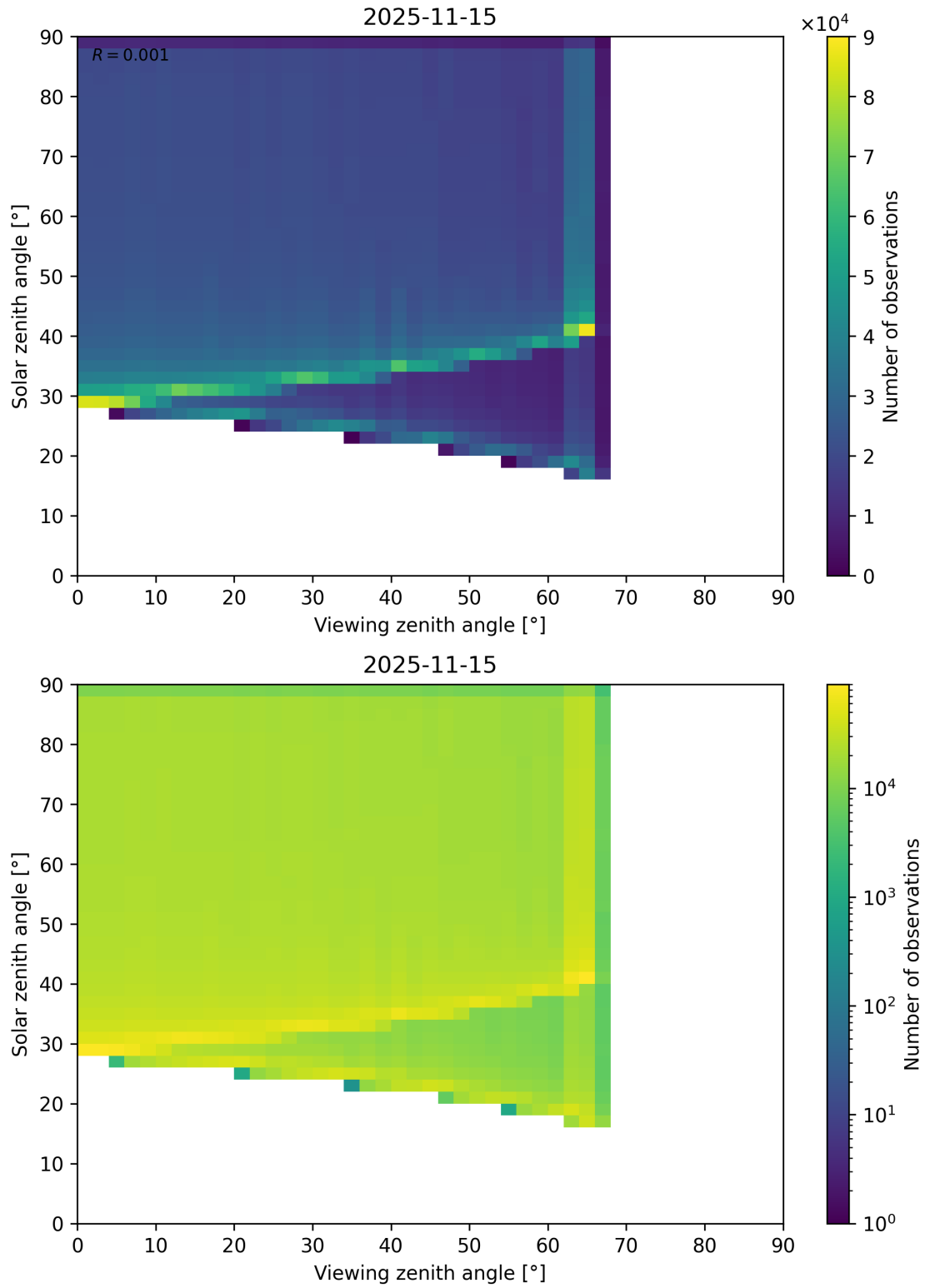
Figure 54: Scatter density plot of “Viewing zenith angle” against “Solar zenith angle” for 2025-11-14 to 2025-11-16.
