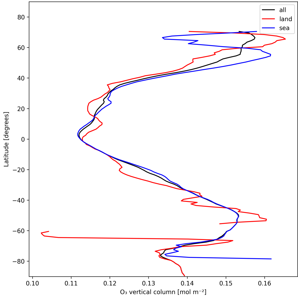
Figure 14: Zonal average of “O 3 vertical column” for 2025-11-14 to 2025-11-16.
