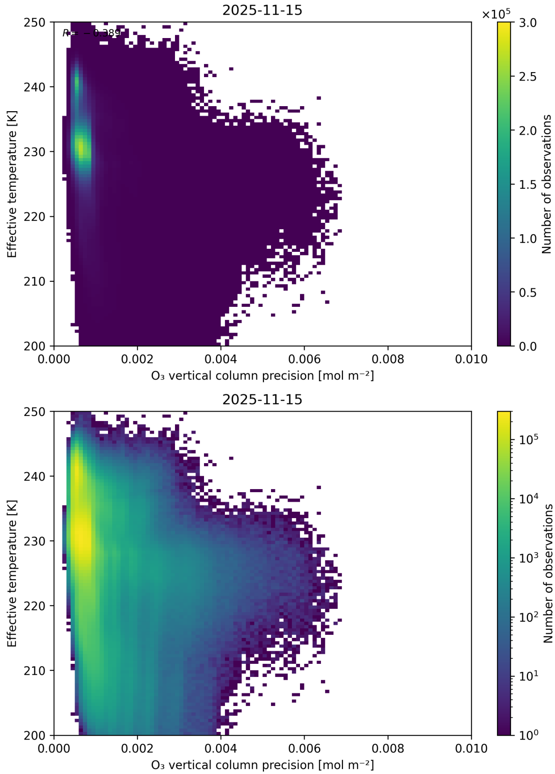
Figure 42: Scatter density plot of “O 3 vertical column precision” against “Effective temperature” for 2025-11-14 to 2025-11-16.
