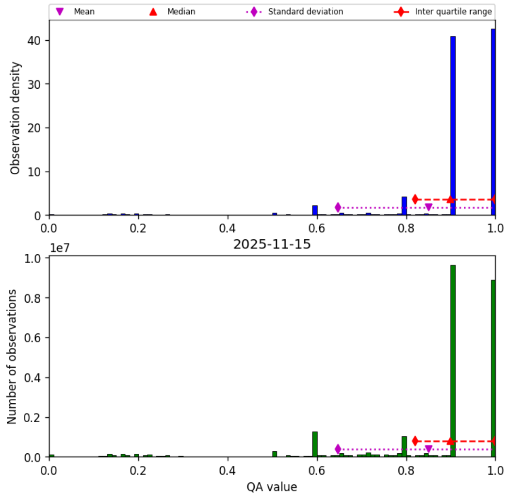
Figure 20: Histogram of “QA value” for 2025-11-14 to 2025-11-16
