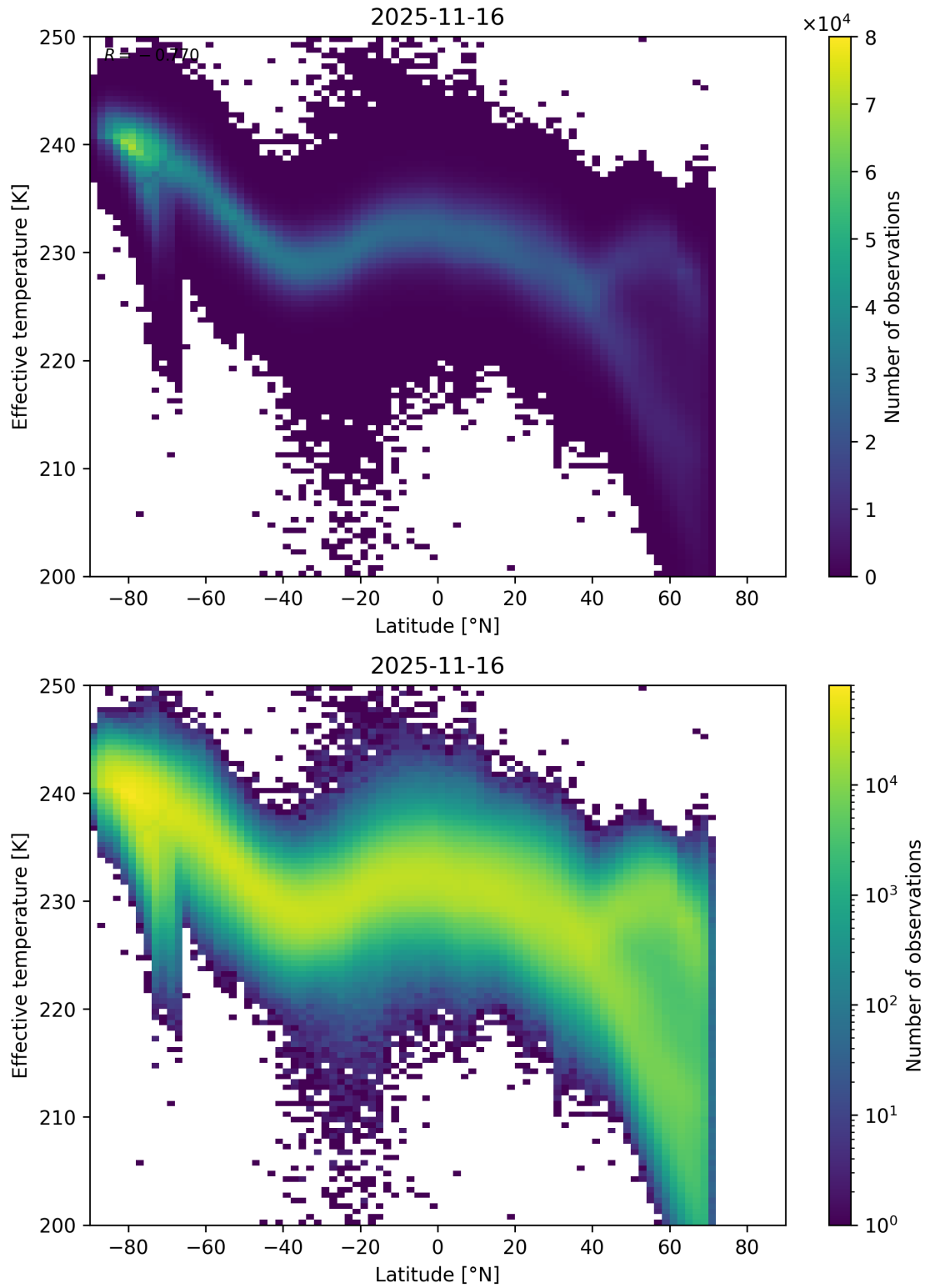
Figure 34: Scatter density plot of “Latitude” against “Effective temperature” for 2025-11-15 to 2025-11-17.
