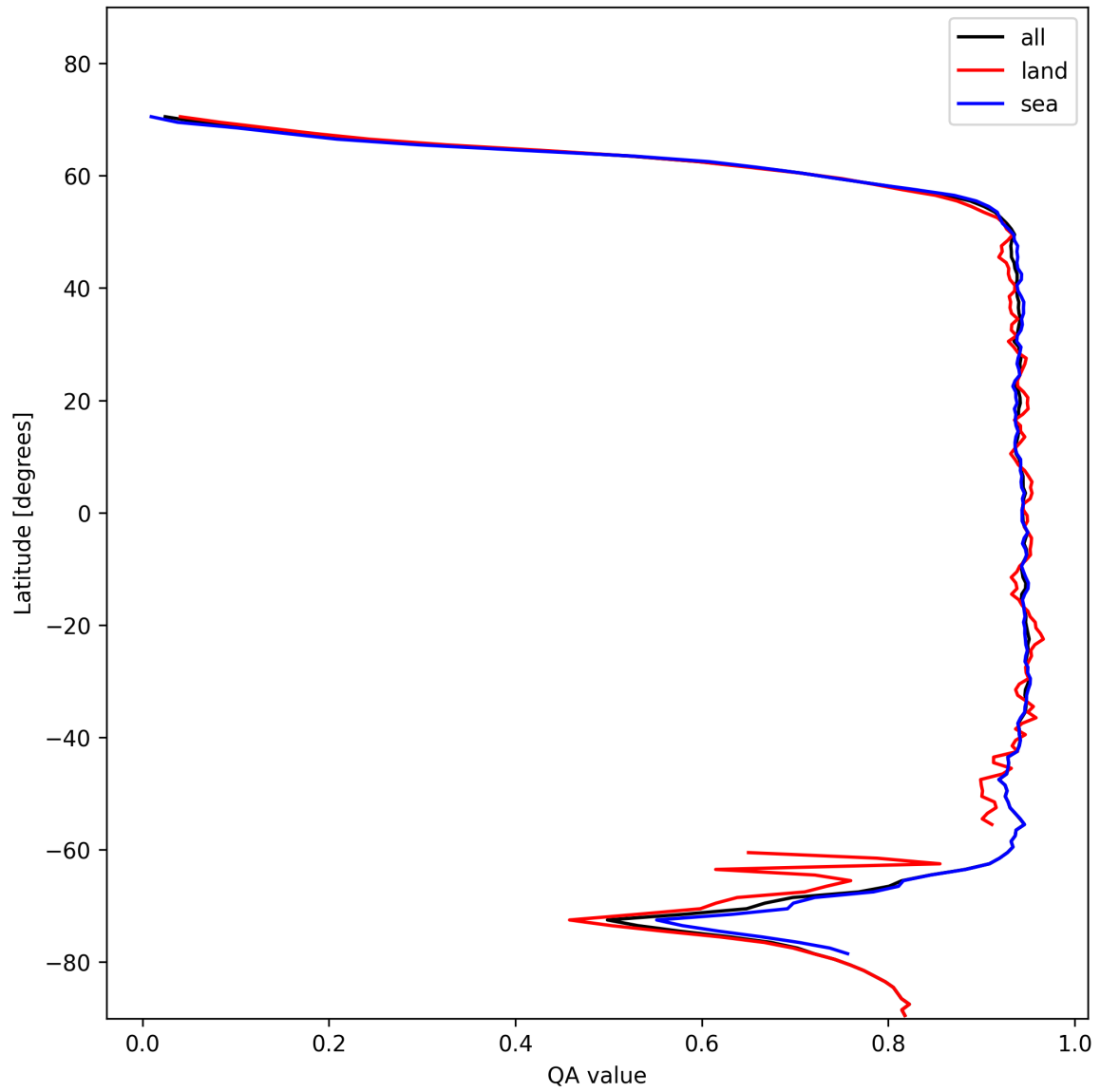
Figure 13: Zonal average of “QA value” for 2025-11-15 to 2025-11-17.
