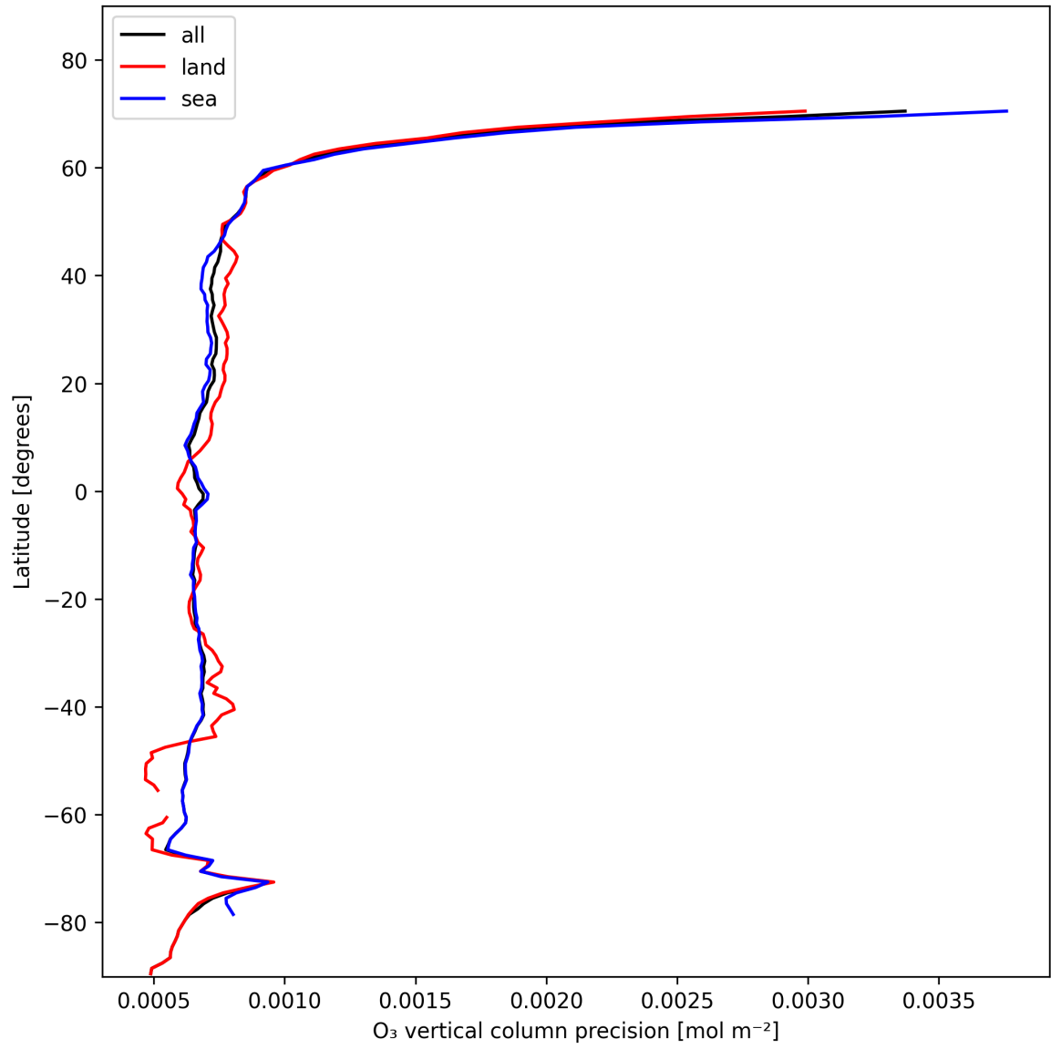
Figure 15: Zonal average of “O 3 vertical column precision” for 2025-11-15 to 2025-11-17.
