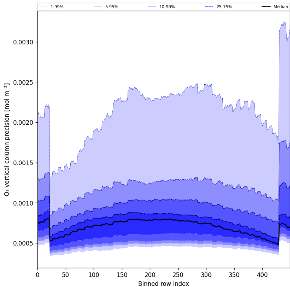
Figure 29: Along track statistics of “O 3 vertical column precision” for 2025-11-15 to 2025-11-17
