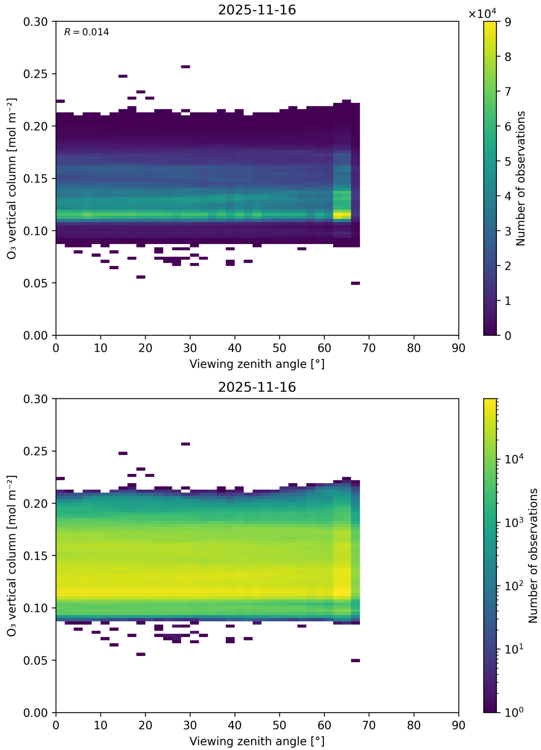
Figure 52: Scatter density plot of “Viewing zenith angle” against “O 3 vertical column” for 2025-11-15 to 2025-11-17.
