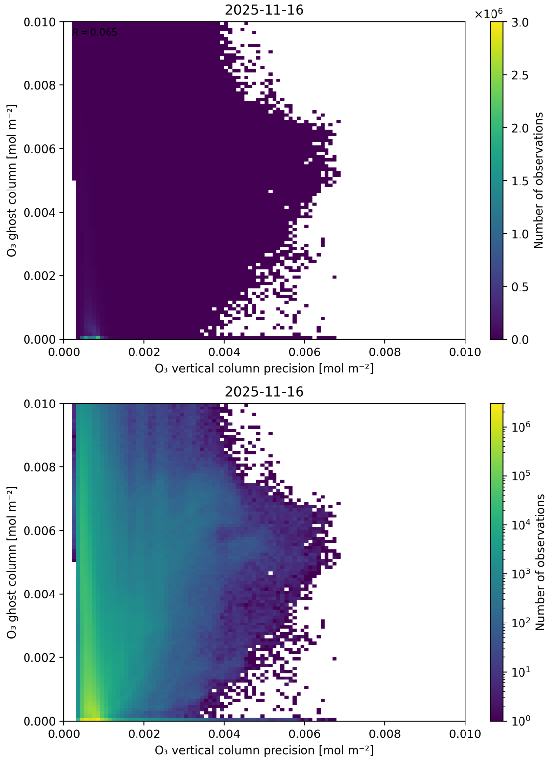
Figure 43: Scatter density plot of “ \text{O}_3 vertical column precision” against “ \text{O}_3 ghost column” for 2025-11-15 to 2025-11-17.
