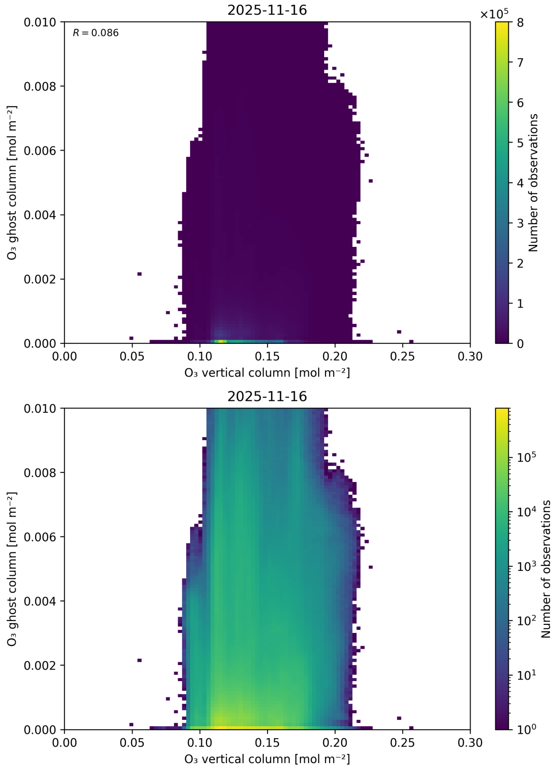
Figure 40: Scatter density plot of “O 3 vertical column” against “O 3 ghost column” for 2025-11-15 to 2025-11-17.
