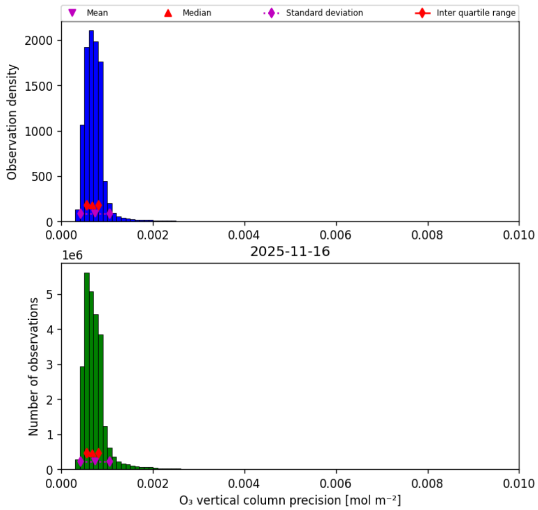
Figure 22: Histogram of “O 3 vertical column precision” for 2025-11-15 to 2025-11-17
