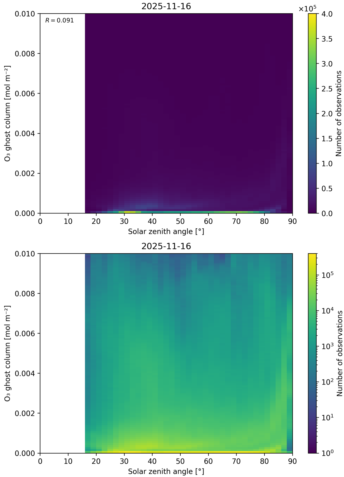
Figure 46: Scatter density plot of “Solar zenith angle” against “O 3 ghost column” for 2025-11-15 to 2025-11-17.
