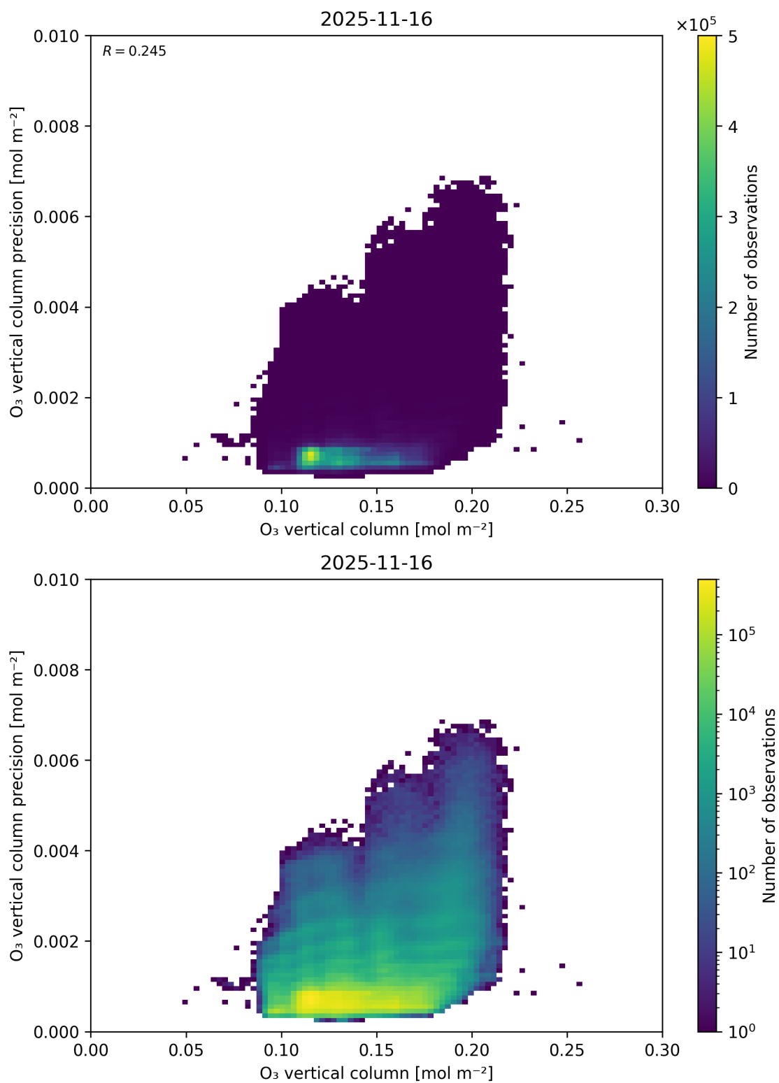
Figure 41: Scatter density plot of “O 3 vertical column” against “O 3 vertical column precision” for 2025-11-15 to 2025-11-17.
