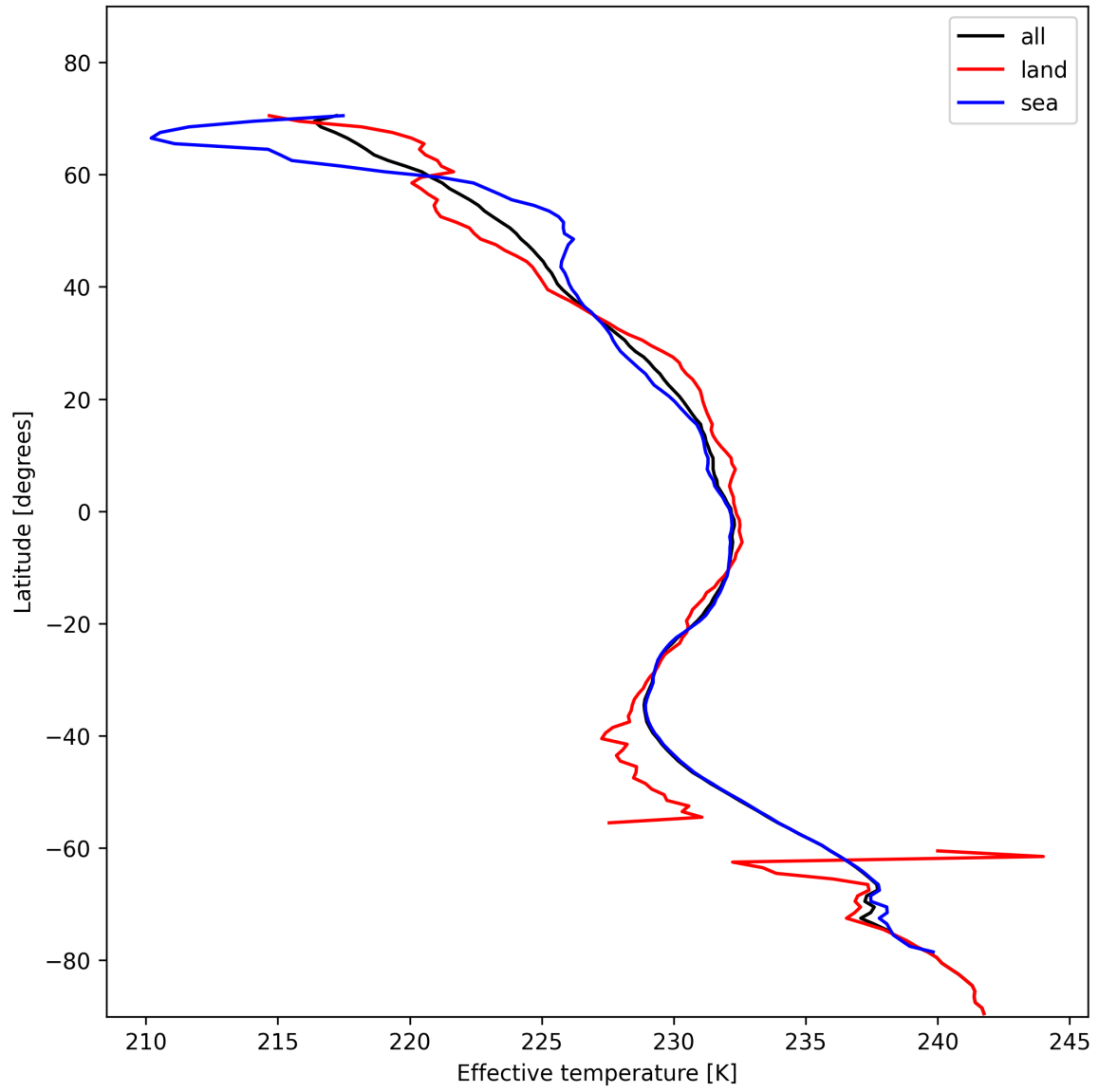
Figure 17: Zonal average of "Effective temperature" for 2025-11-15 to 2025-11-17.
