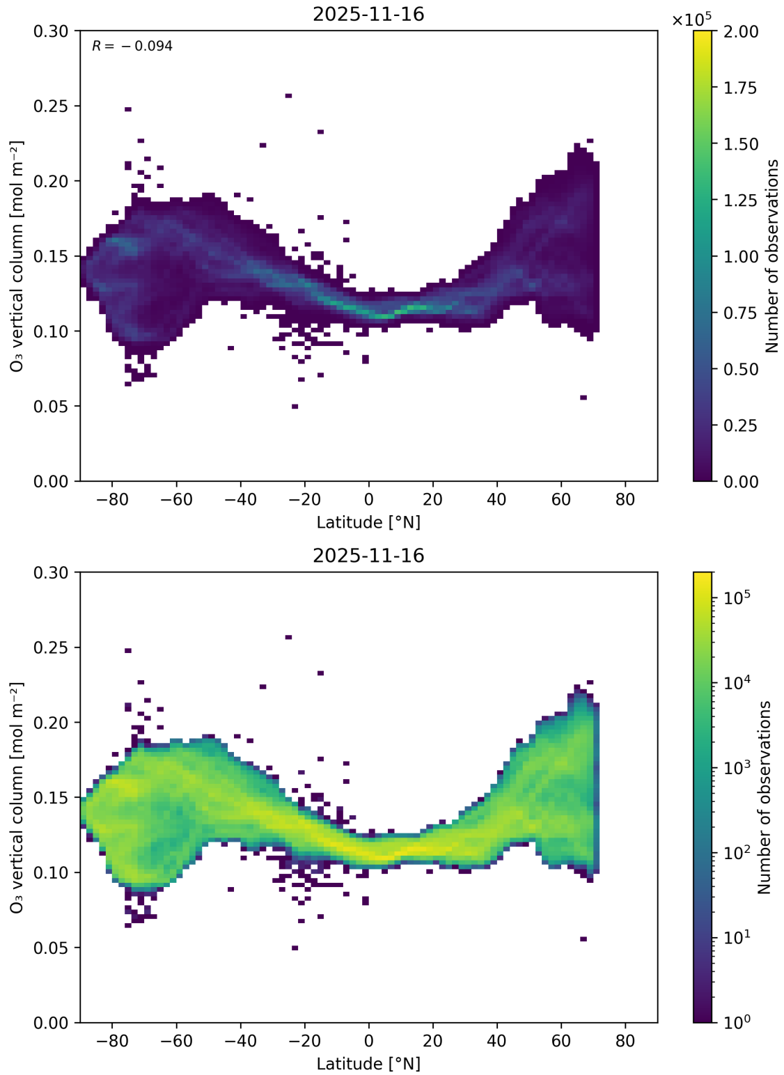
Figure 36: Scatter density plot of “Latitude” against “O 3 vertical column” for 2025-11-15 to 2025-11-17.
