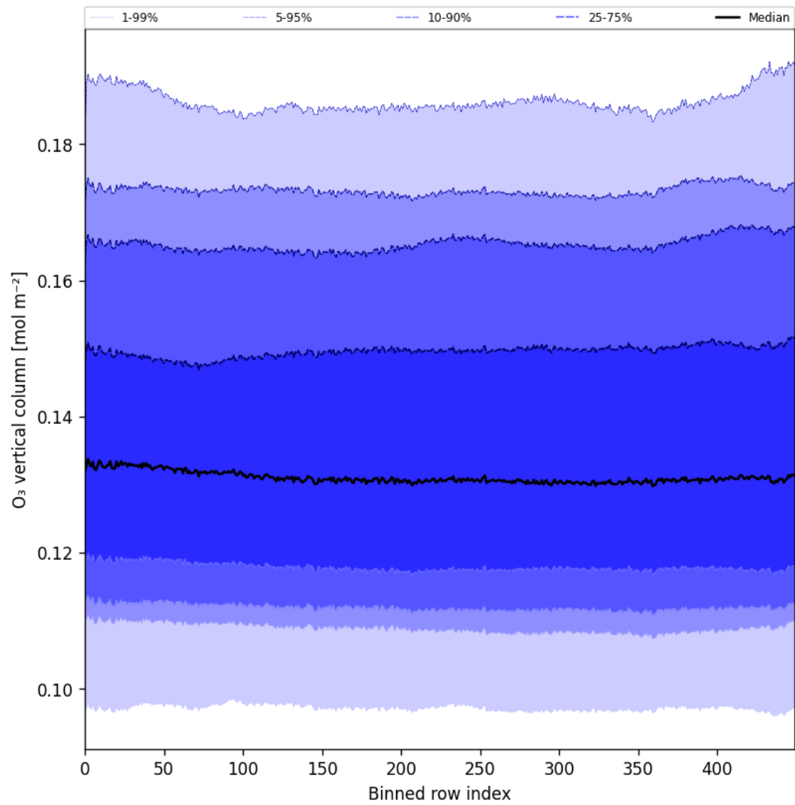
Figure 28: Along track statistics of “O 3 vertical column” for 2025-11-15 to 2025-11-17
