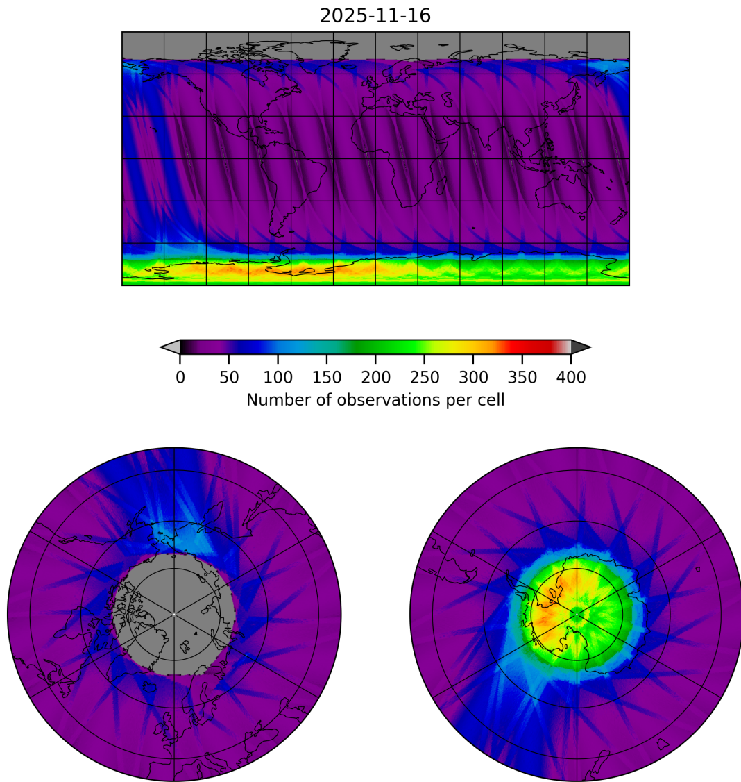
Figure 12: Map of the number of observations for 2025-11-15 to 2025-11-17
