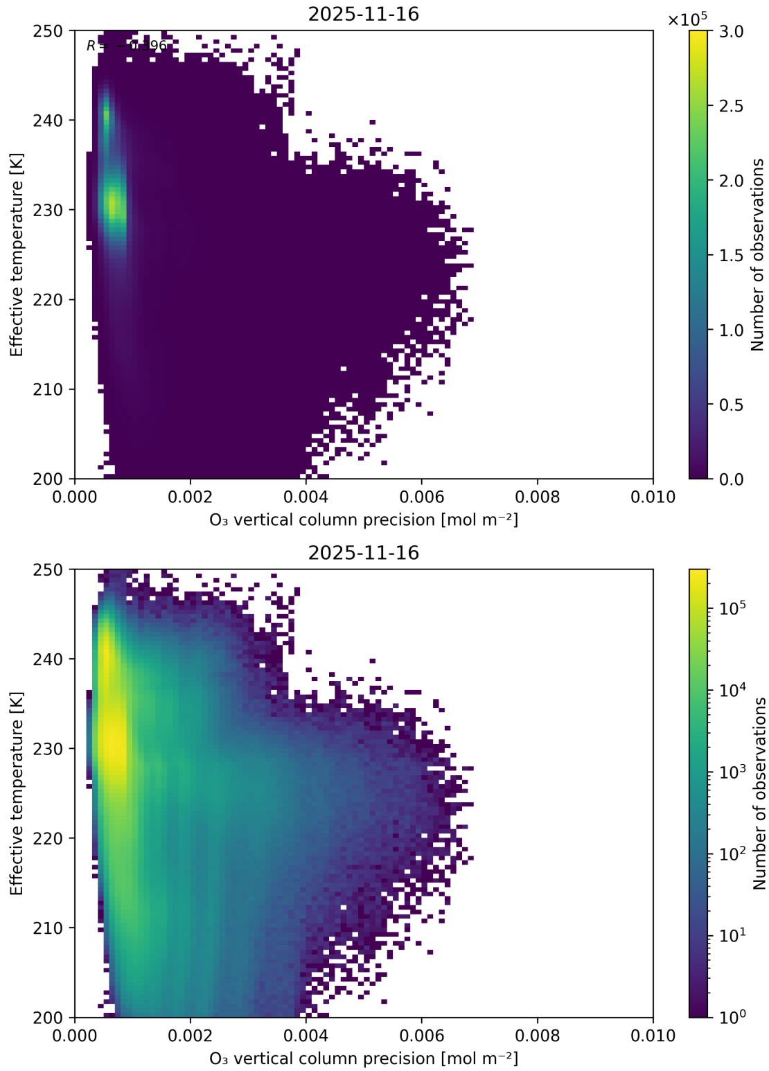
Figure 42: Scatter density plot of “O 3 vertical column precision” against “Effective temperature” for 2025-11-15 to 2025-11-17.
