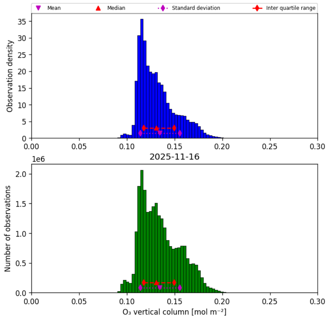
Figure 21: Histogram of “O 3 vertical column” for 2025-11-15 to 2025-11-17
