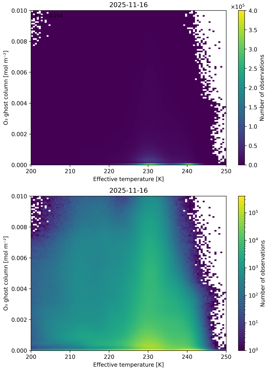
Figure 38: Scatter density plot of “Effective temperature” against “O 3 ghost column” for 2025-11-15 to 2025-11-17.
