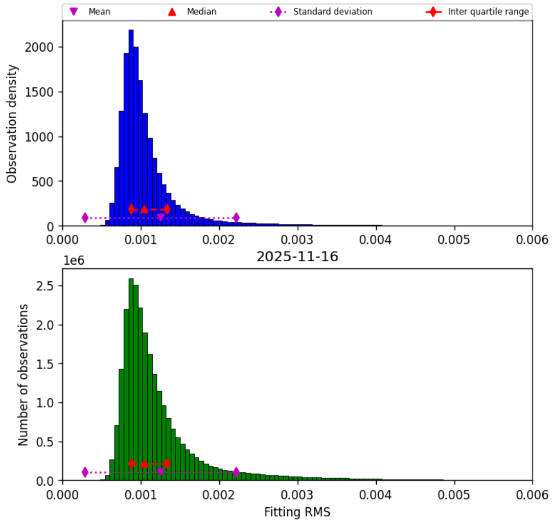
Figure 23: Histogram of “Fitting RMS” for 2025-11-15 to 2025-11-17
