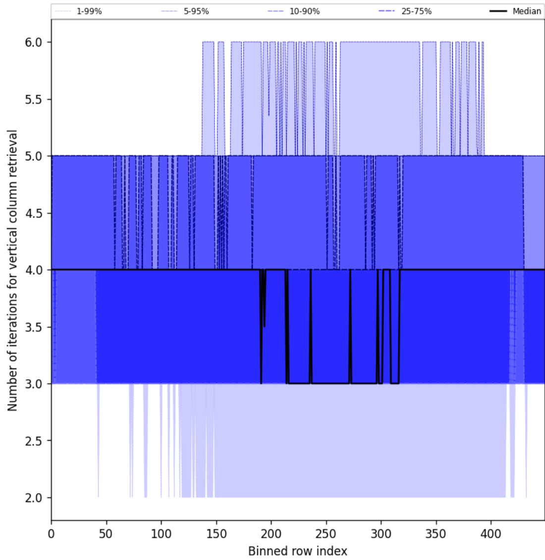
Figure 33: Along track statistics of “Number of iterations for vertical column retrieval” for 2025-11-15 to 2025-11-17
