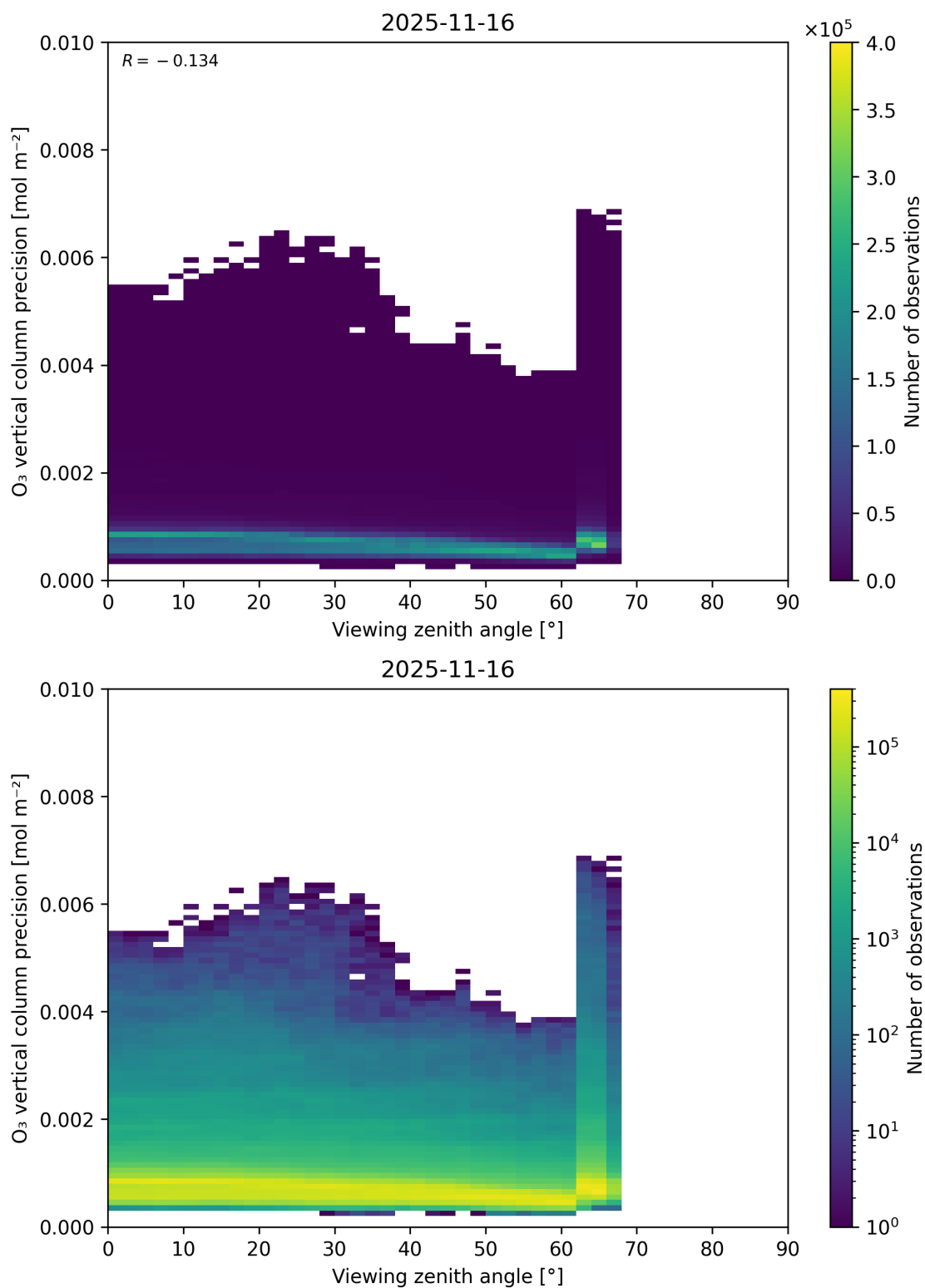
Figure 53: Scatter density plot of “Viewing zenith angle” against “O 3 vertical column precision” for 2025-11-15 to 2025-11-17.
