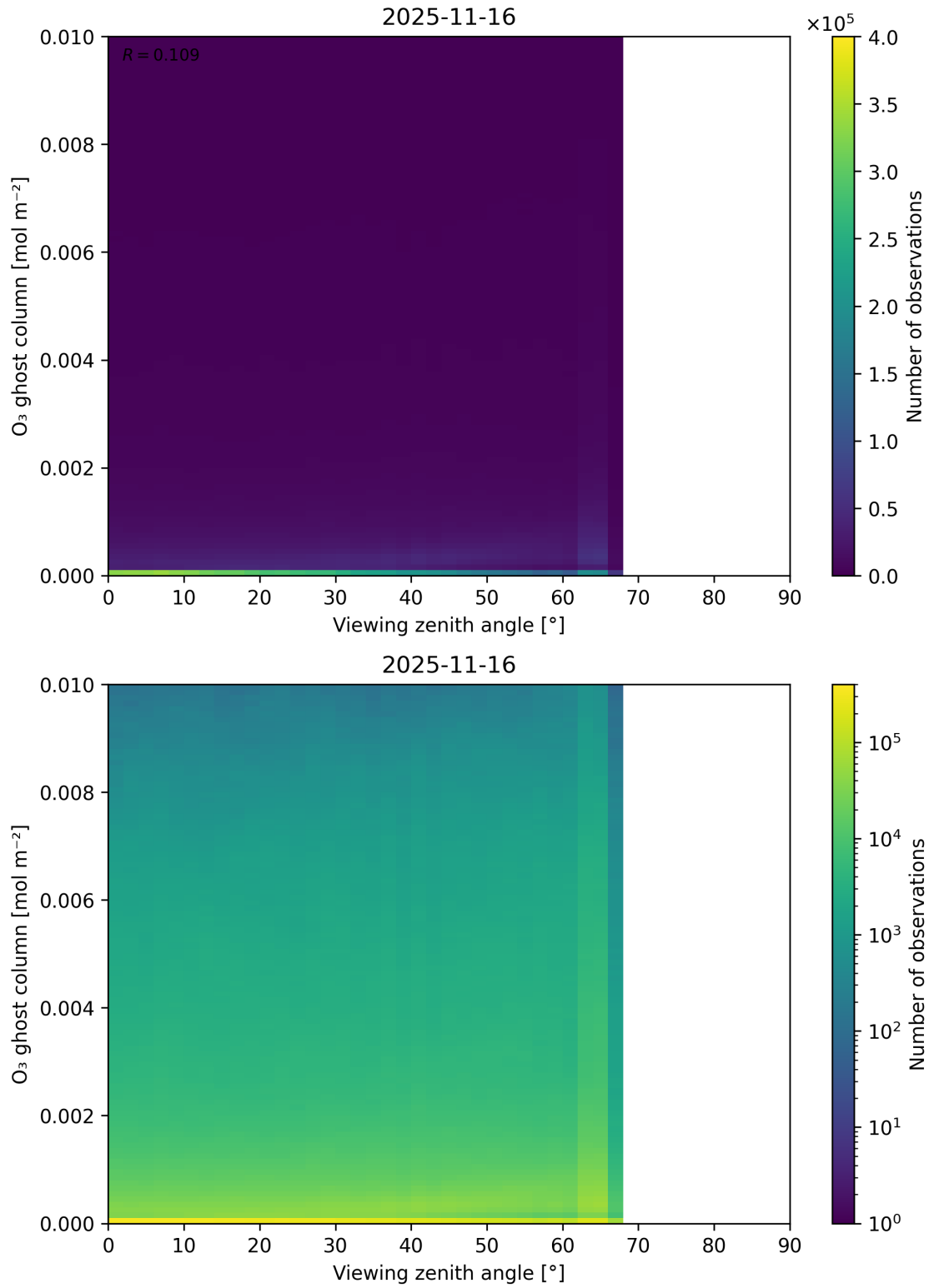
Figure 51: Scatter density plot of “Viewing zenith angle” against “O 3 ghost column” for 2025-11-15 to 2025-11-17.
