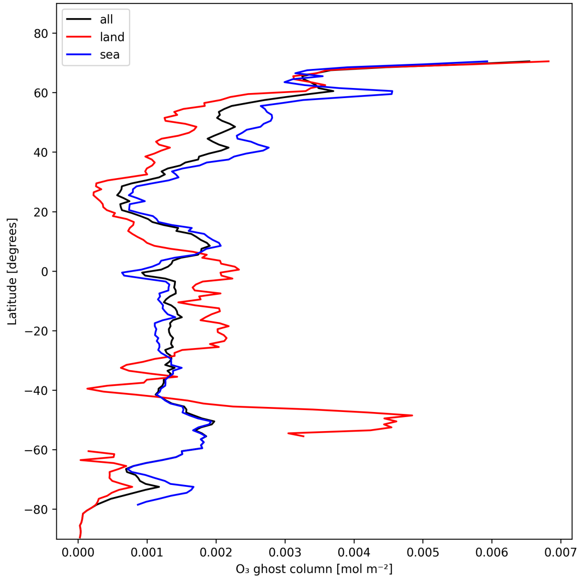
Figure 18: Zonal average of “O 3 ghost column” for 2025-11-15 to 2025-11-17.
