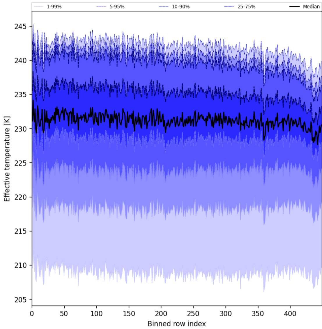
Figure 31: Along track statistics of "Effective temperature" for 2025-11-15 to 2025-11-17
