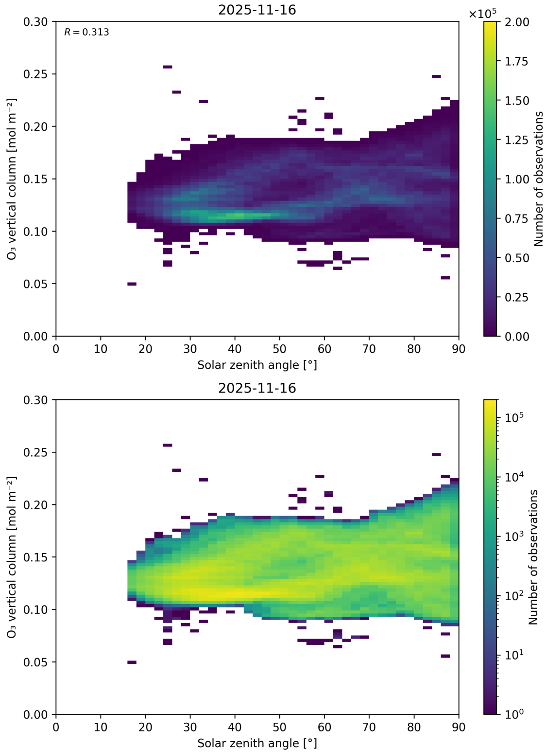
Figure 47: Scatter density plot of “Solar zenith angle” against “O 3 vertical column” for 2025-11-15 to 2025-11-17.
