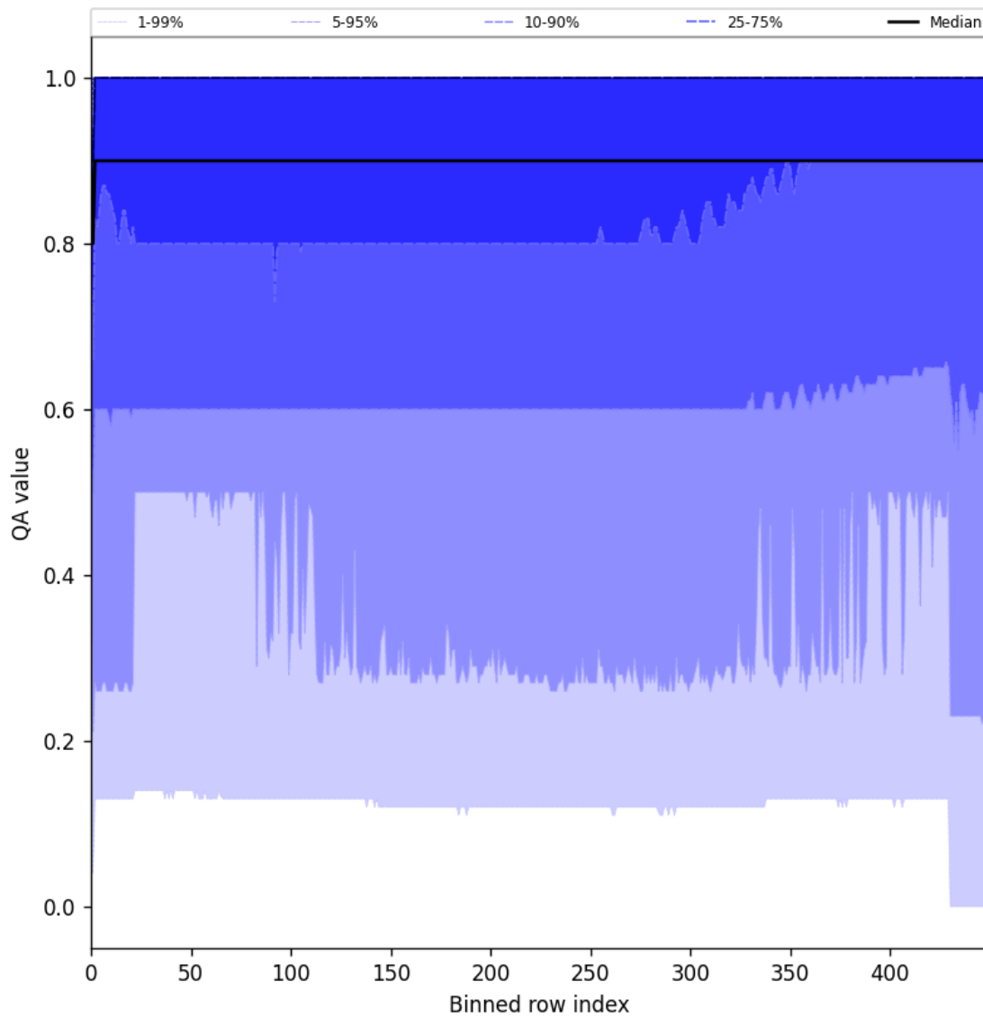
Figure 27: Along track statistics of “QA value” for 2025-11-15 to 2025-11-17
