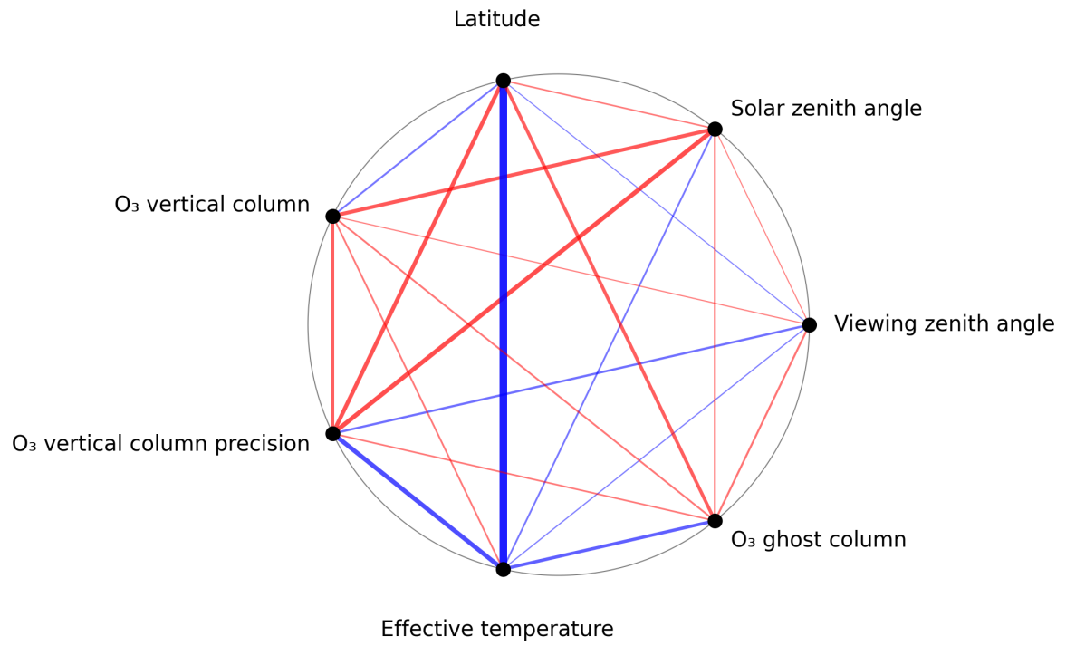
Figure 1: Map of correlation graph for 2025-11-15 to 2025-11-17.
