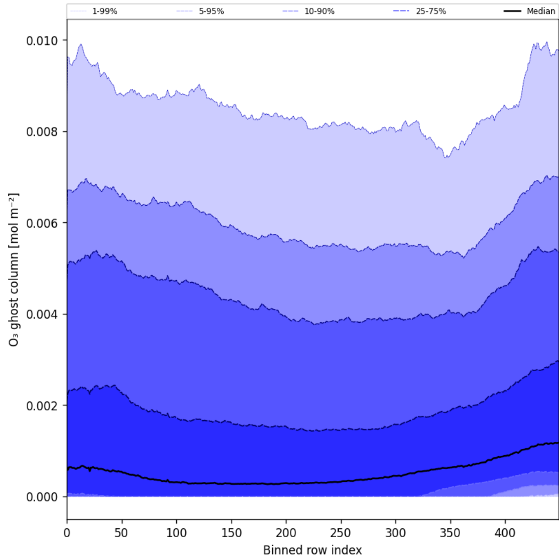
Figure 32: Along track statistics of “O 3 ghost column” for 2025-11-15 to 2025-11-17
