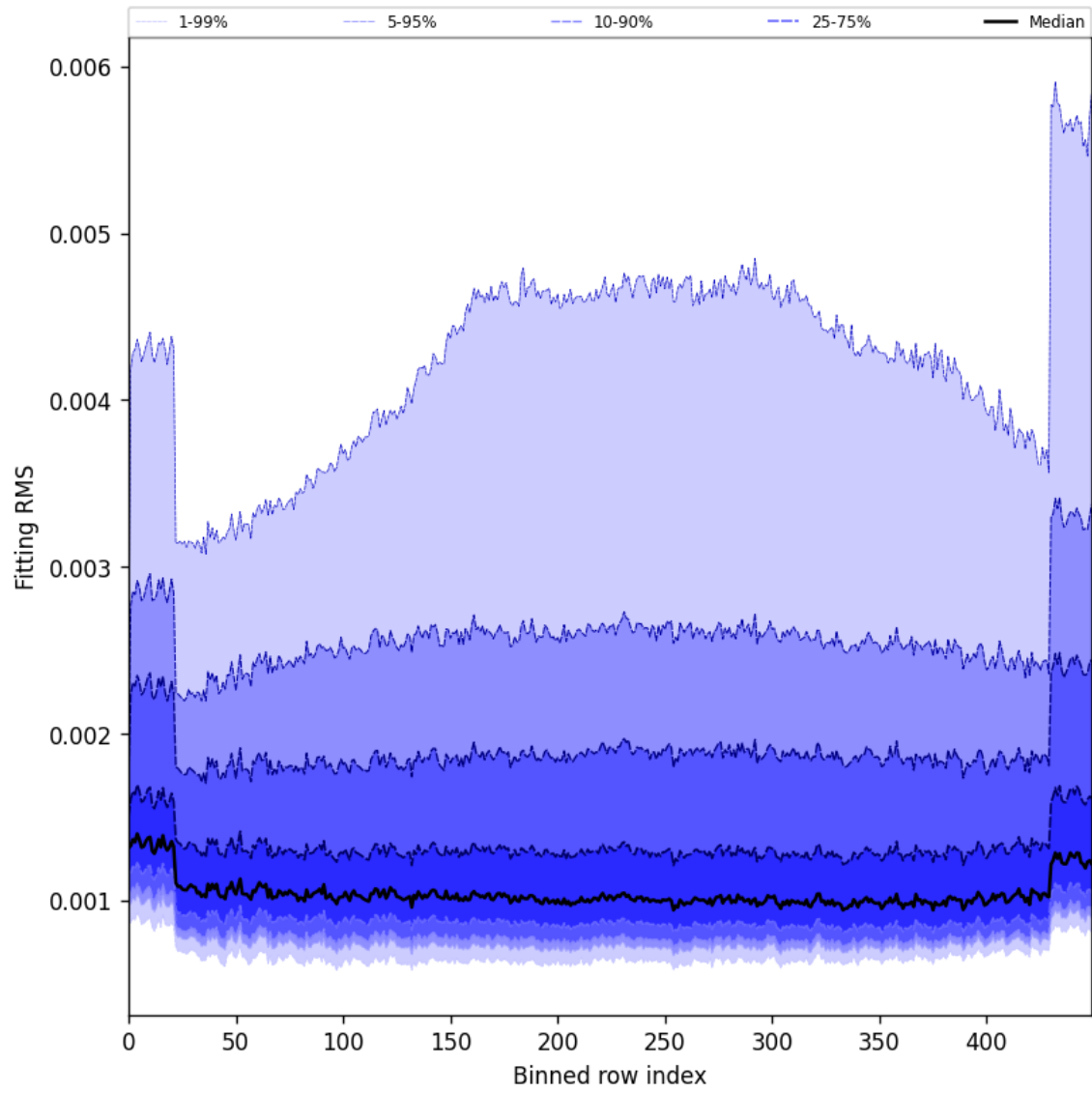
Figure 30: Along track statistics of “Fitting RMS” for 2025-11-15 to 2025-11-17
