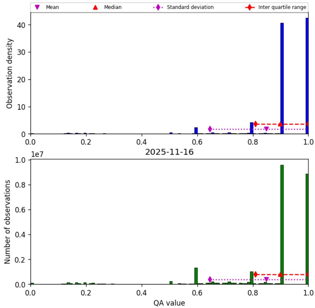
Figure 20: Histogram of “QA value” for 2025-11-15 to 2025-11-17
