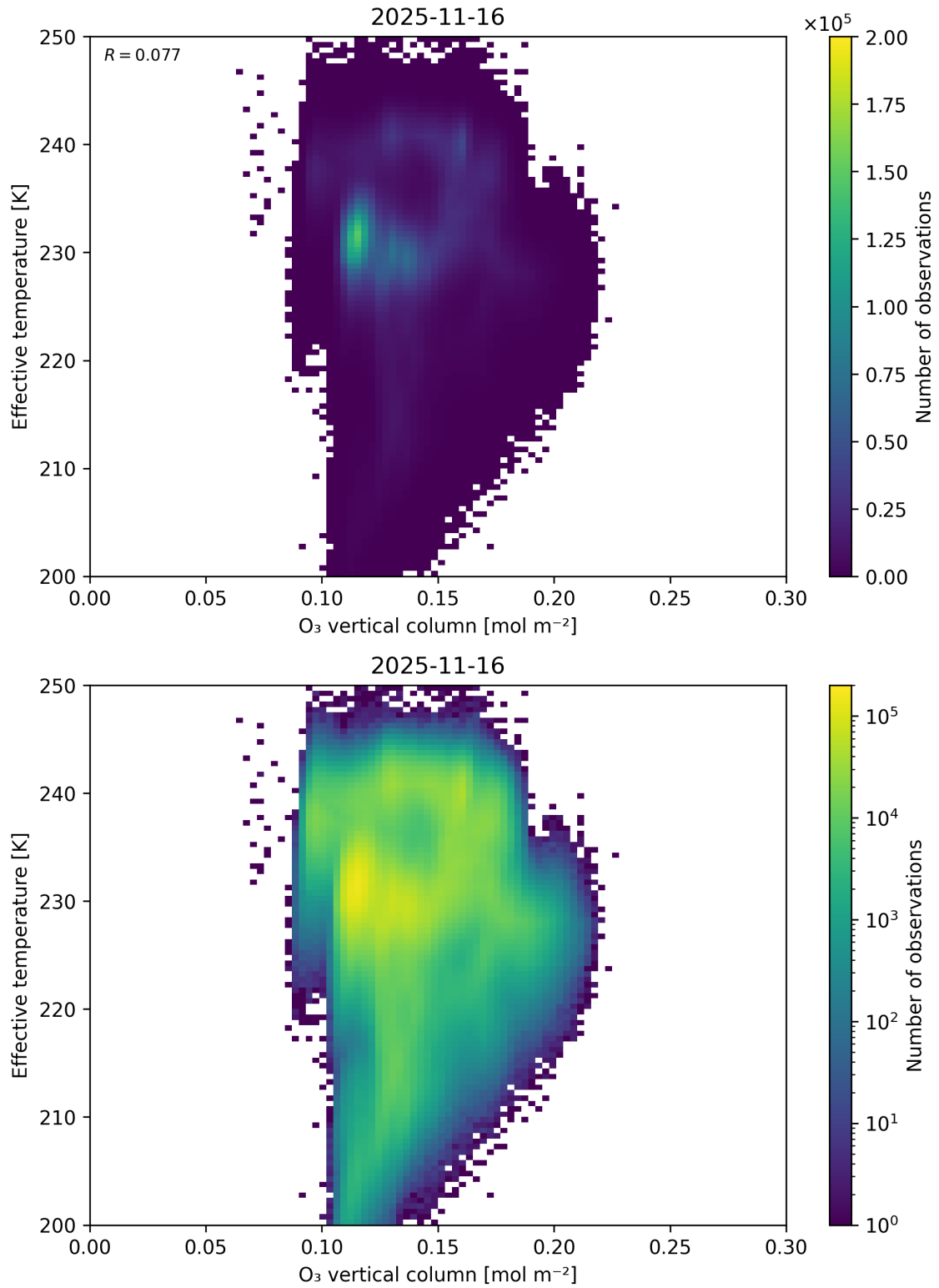
Figure 39: Scatter density plot of “O 3 vertical column” against “Effective temperature” for 2025-11-15 to 2025-11-17.
