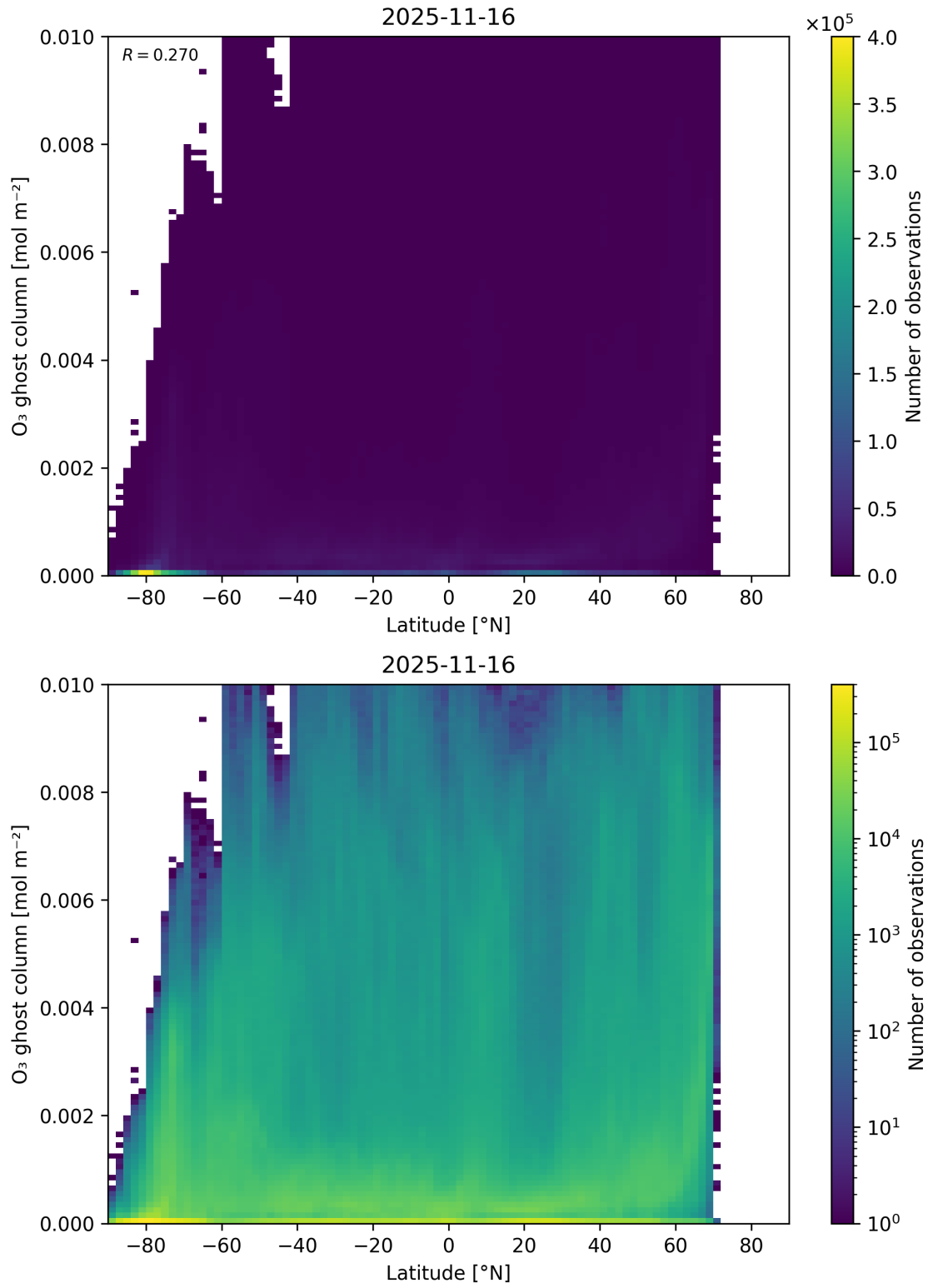
Figure 35: Scatter density plot of “Latitude” against “O 3 ghost column” for 2025-11-15 to 2025-11-17.
