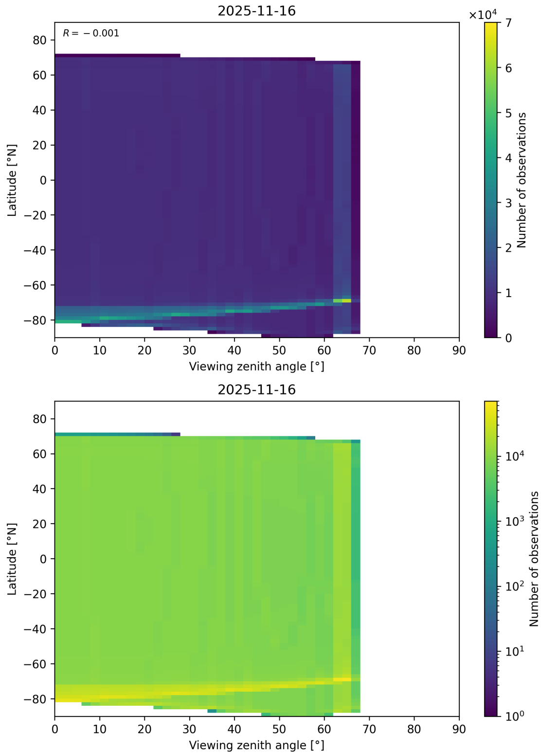
Figure 49: Scatter density plot of “Viewing zenith angle” against “Latitude” for 2025-11-15 to 2025-11-17.
