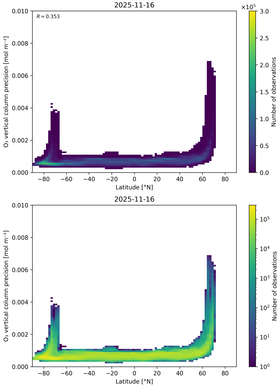
Figure 37: Scatter density plot of “Latitude” against “O 3 vertical column precision” for 2025-11-15 to 2025-11-17.
