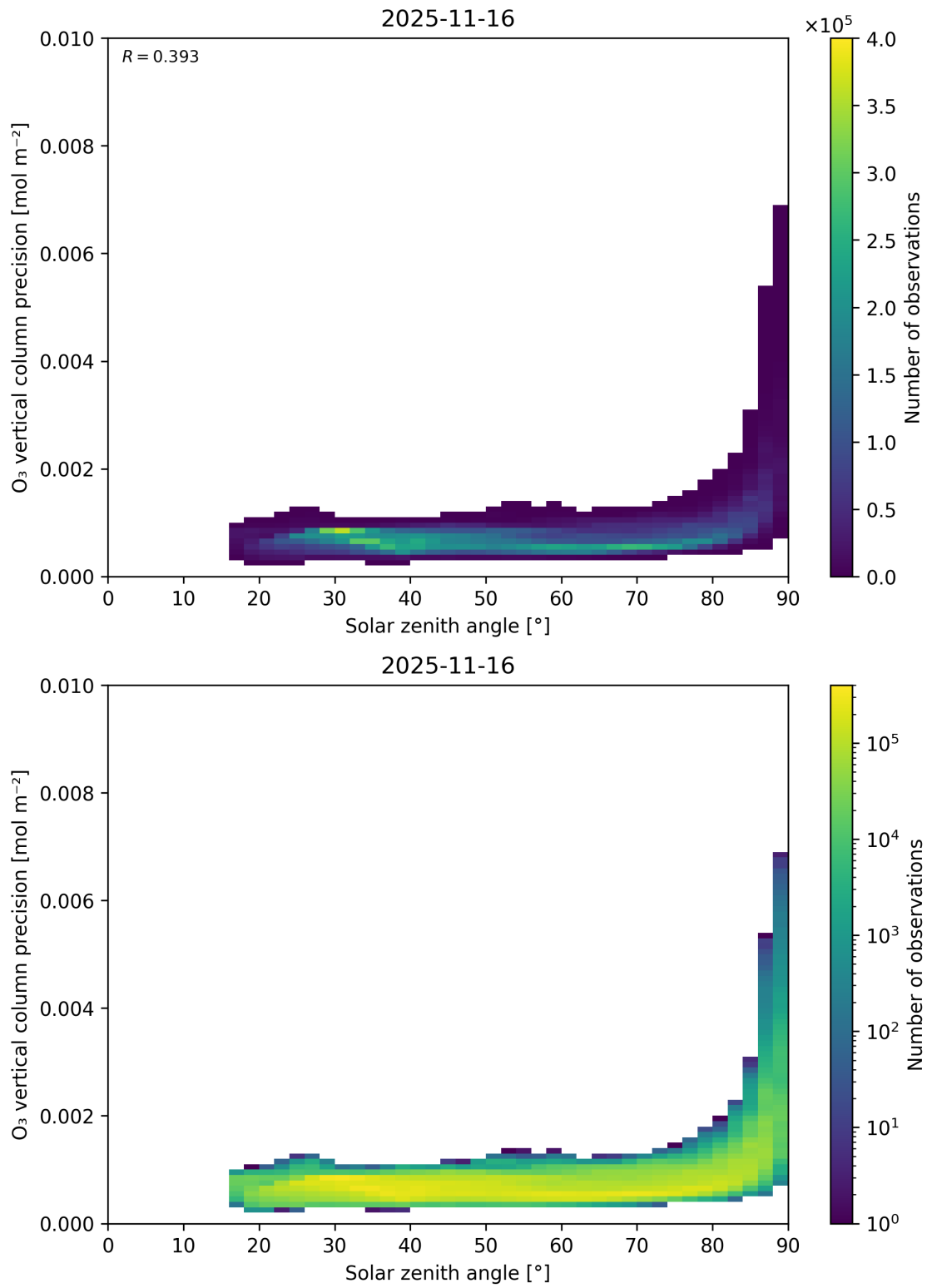
Figure 48: Scatter density plot of “Solar zenith angle” against “O 3 vertical column precision” for 2025-11-15 to 2025-11-17.
