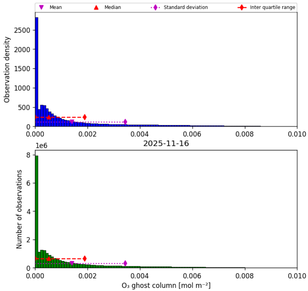
Figure 25: Histogram of “O 3 ghost column” for 2025-11-15 to 2025-11-17
