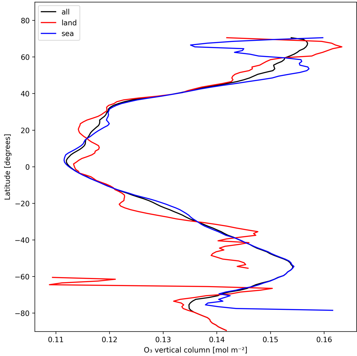
Figure 14: Zonal average of “O 3 vertical column” for 2025-11-15 to 2025-11-17.
