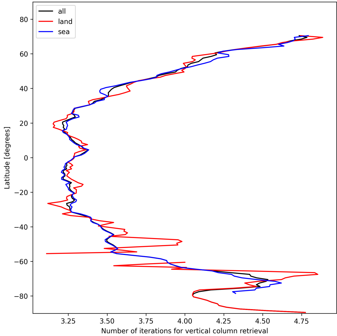
Figure 19: Zonal average of “Number of iterations for vertical column retrieval” for 2025-11-15 to 2025-11-17.
