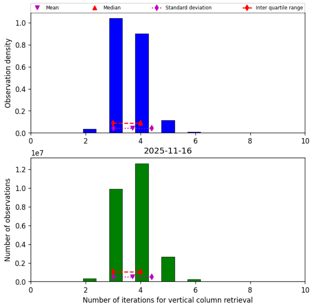
Figure 26: Histogram of “Number of iterations for vertical column retrieval” for 2025-11-15 to 2025-11-17
