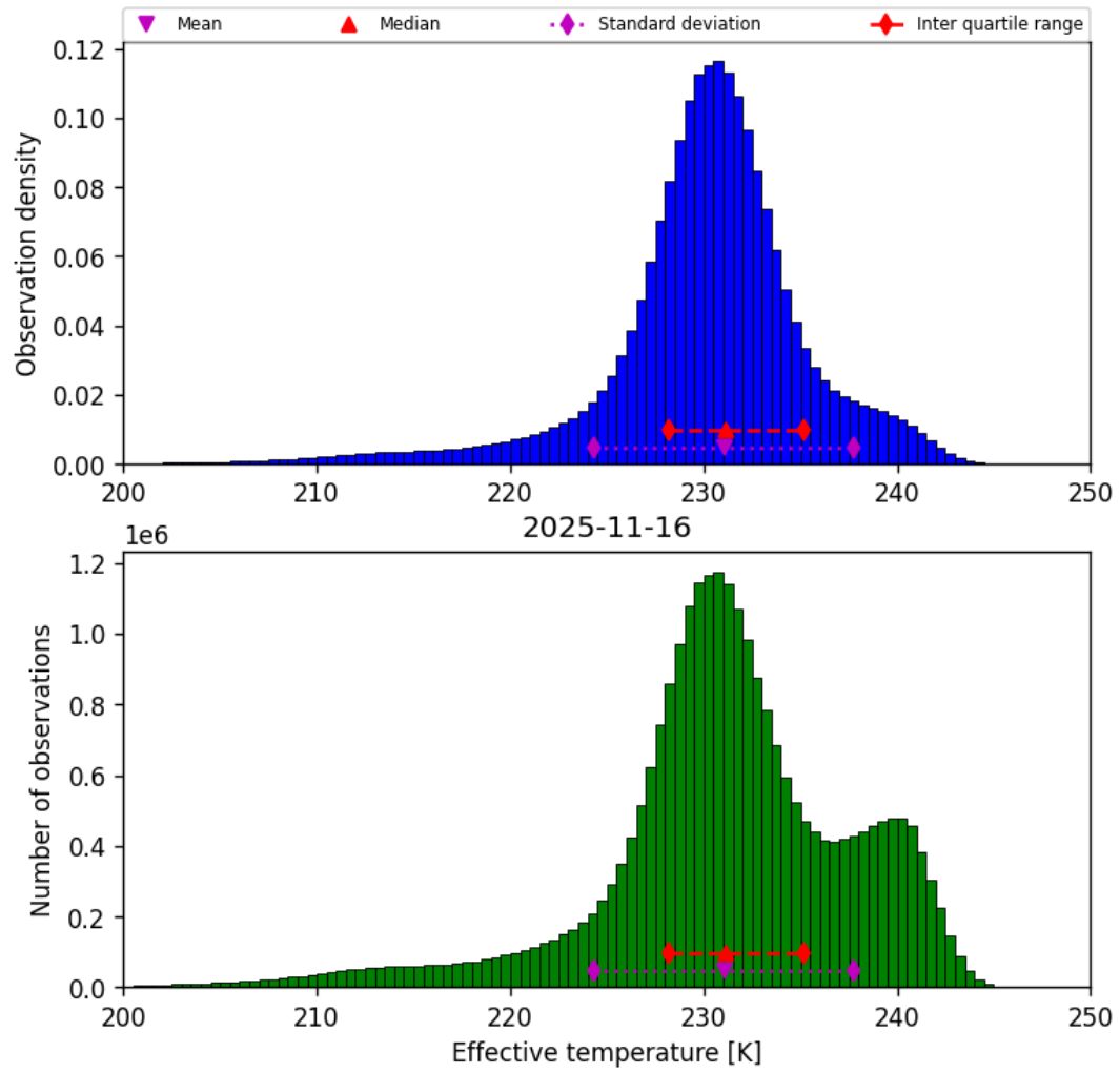
Figure 24: Histogram of “Effective temperature” for 2025-11-15 to 2025-11-17
