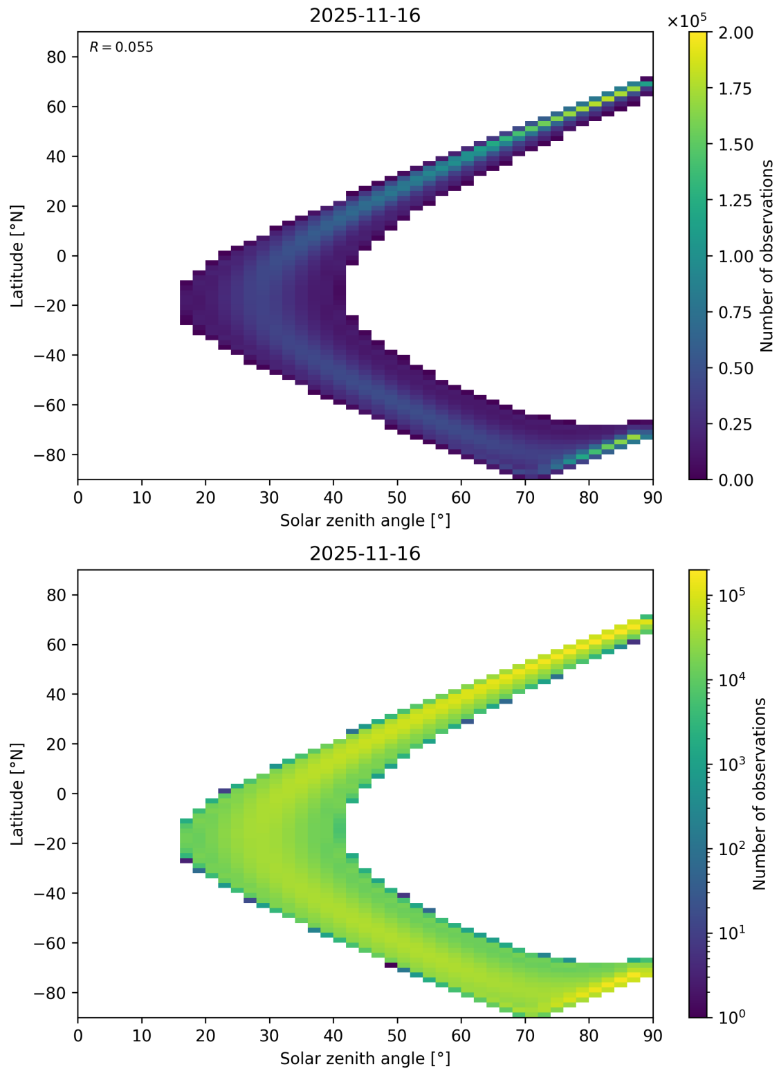
Figure 44: Scatter density plot of “Solar zenith angle” against “Latitude” for 2025-11-15 to 2025-11-17.
