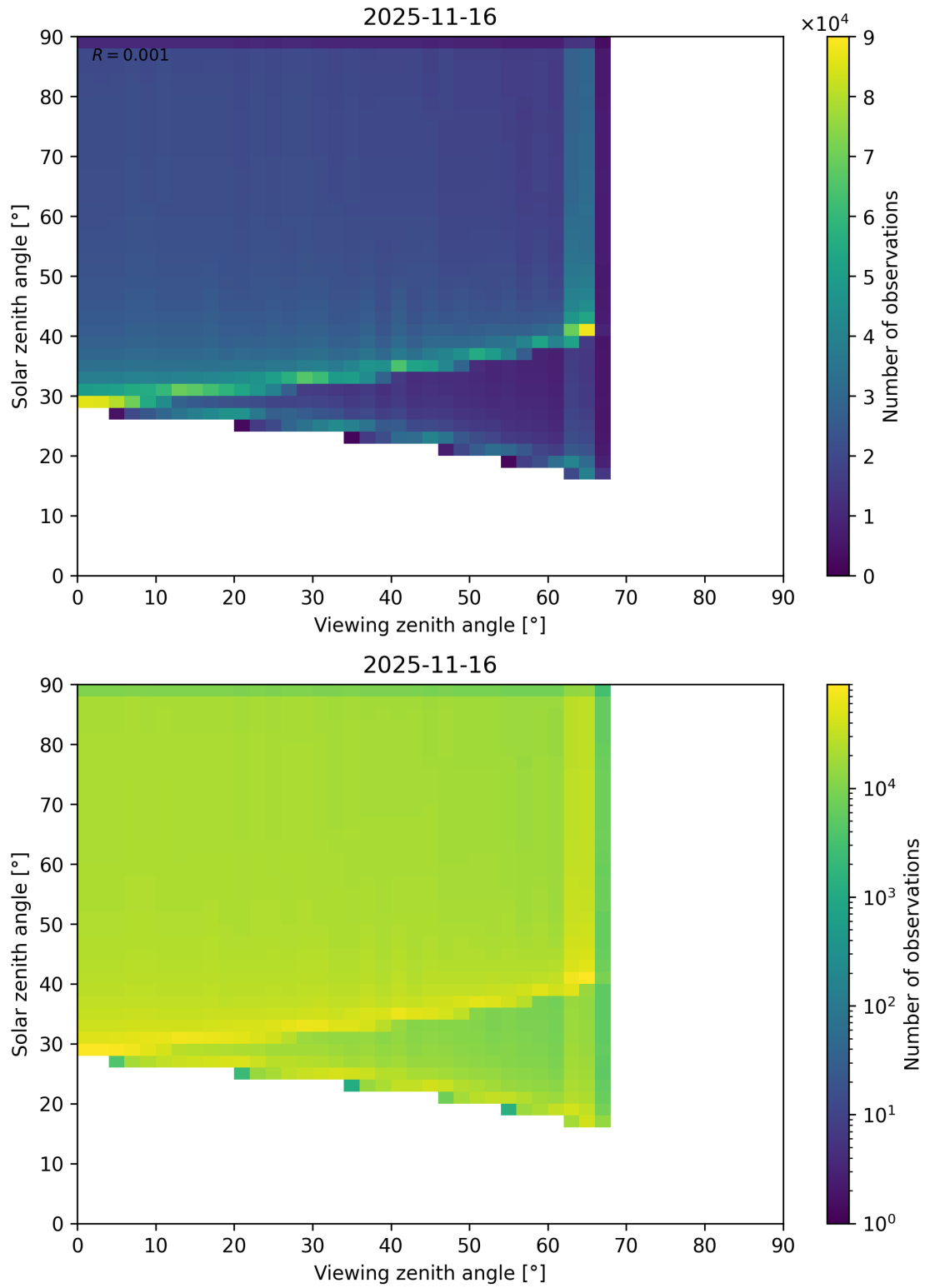
Figure 54: Scatter density plot of “Viewing zenith angle” against “Solar zenith angle” for 2025-11-15 to 2025-11-17.
