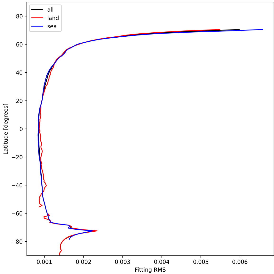
Figure 16: Zonal average of “Fitting RMS” for 2025-11-15 to 2025-11-17.
