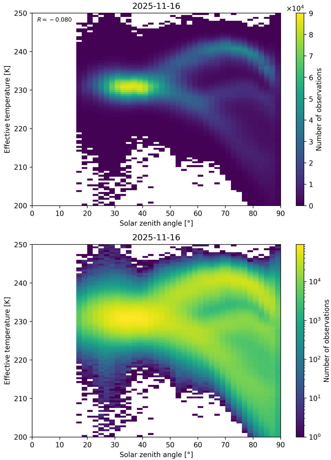
Figure 45: Scatter density plot of “Solar zenith angle” against “Effective temperature” for 2025-11-15 to 2025-11-17.
