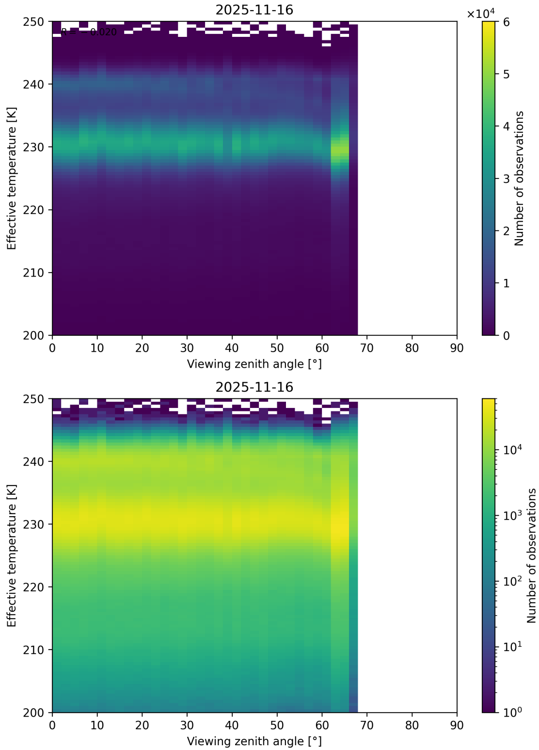
Figure 50: Scatter density plot of “Viewing zenith angle” against “Effective temperature” for 2025-11-15 to 2025-11-17.
