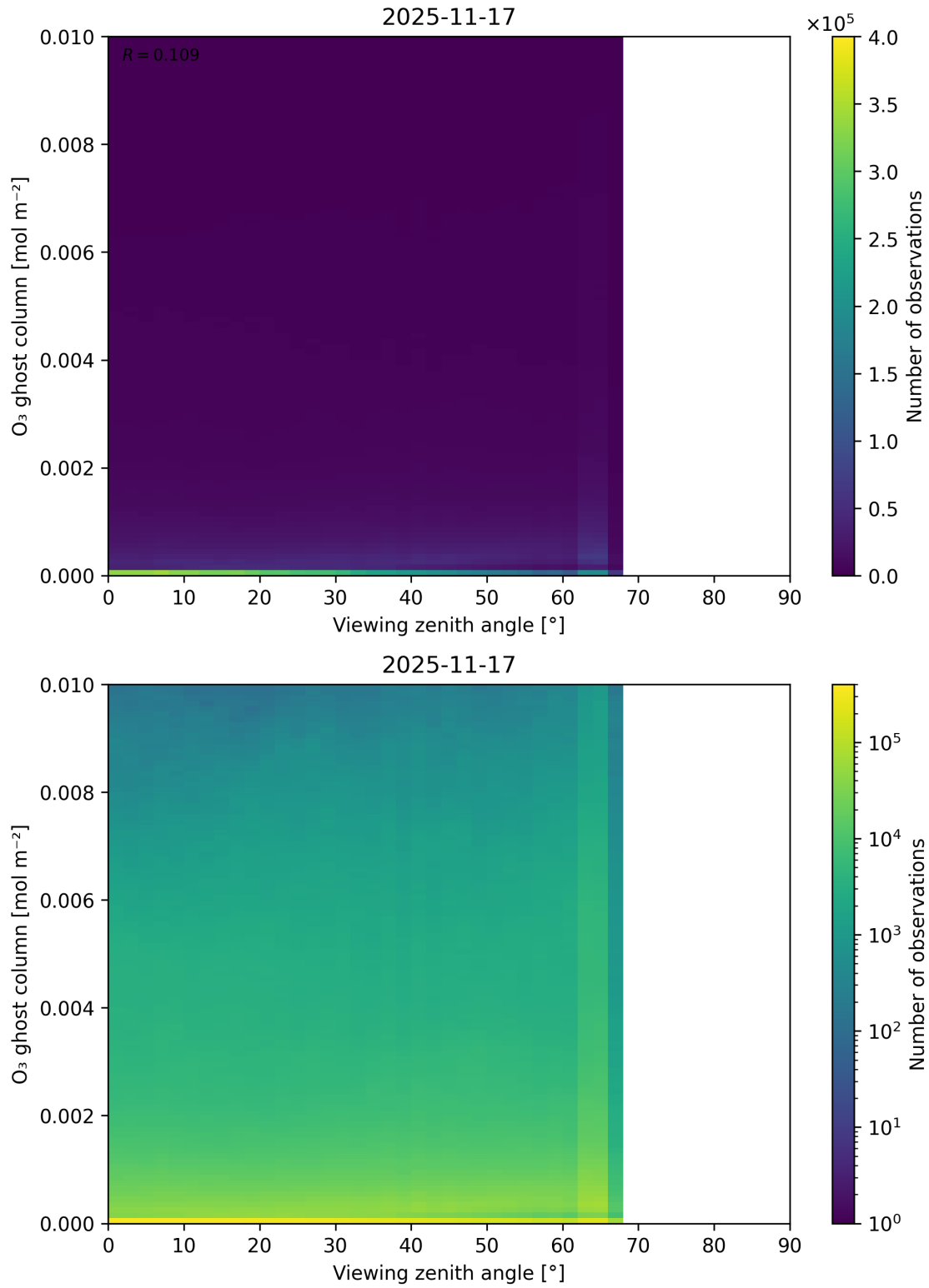
Figure 51: Scatter density plot of “Viewing zenith angle” against “O 3 ghost column” for 2025-11-16 to 2025-11-18.
