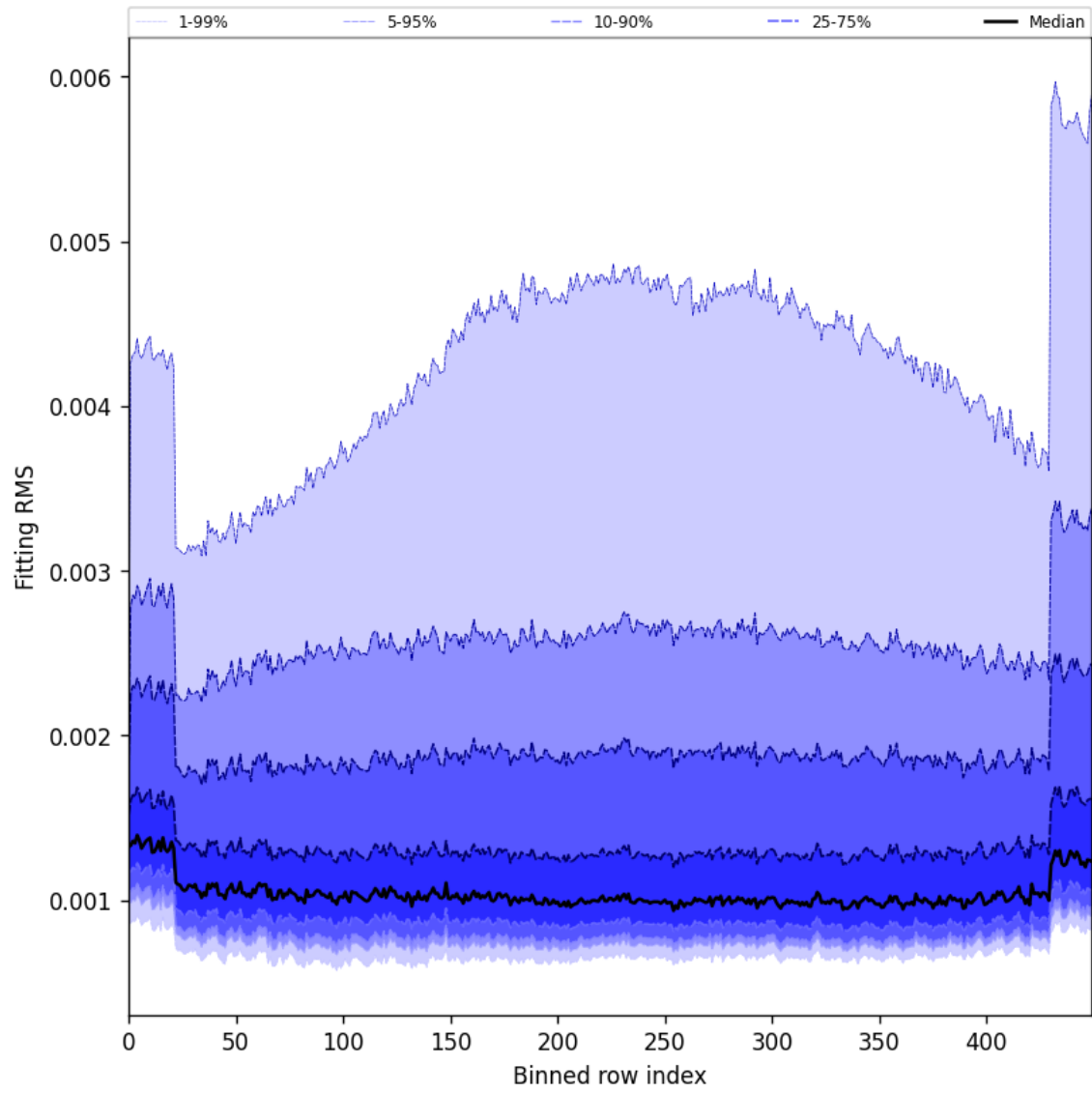
Figure 30: Along track statistics of “Fitting RMS” for 2025-11-16 to 2025-11-18
