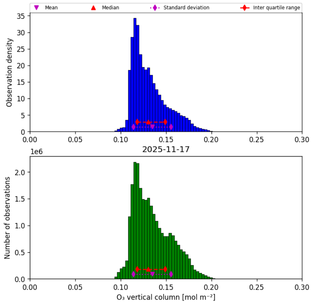
Figure 21: Histogram of “O 3 vertical column” for 2025-11-16 to 2025-11-18
