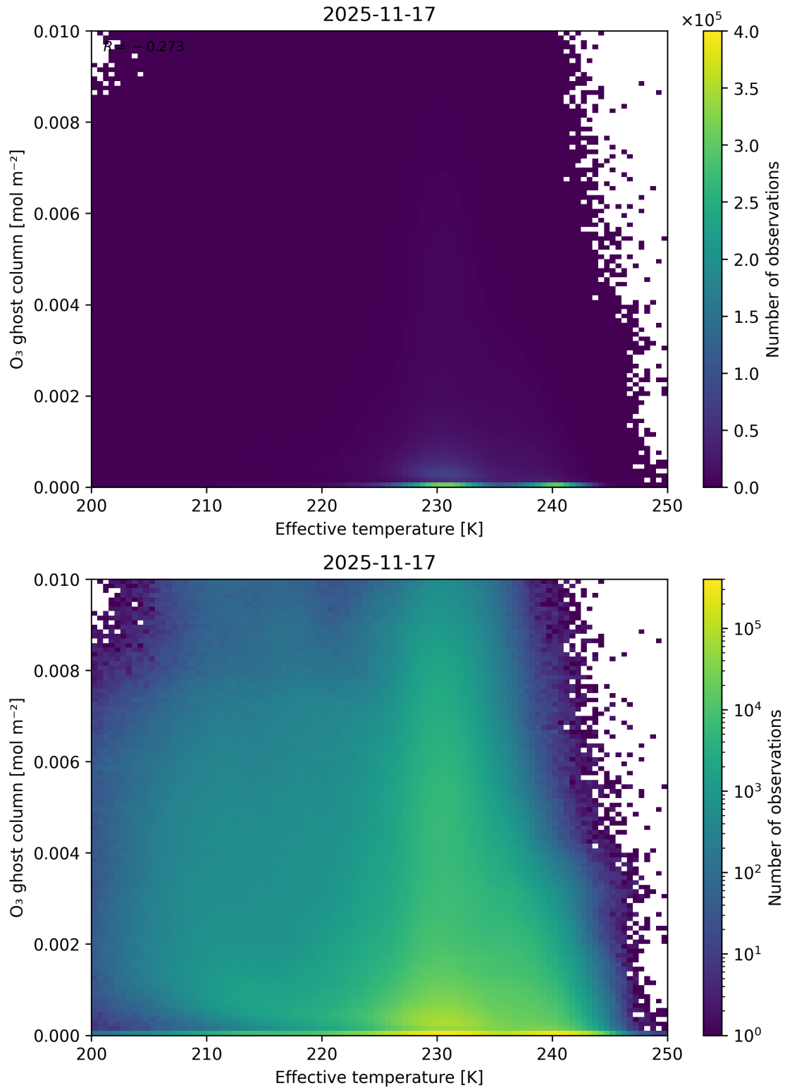
Figure 38: Scatter density plot of “Effective temperature” against “O 3 ghost column” for 2025-11-16 to 2025-11-18.
