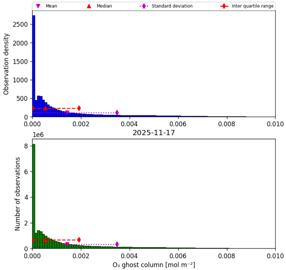
Figure 25: Histogram of “O 3 ghost column” for 2025-11-16 to 2025-11-18
