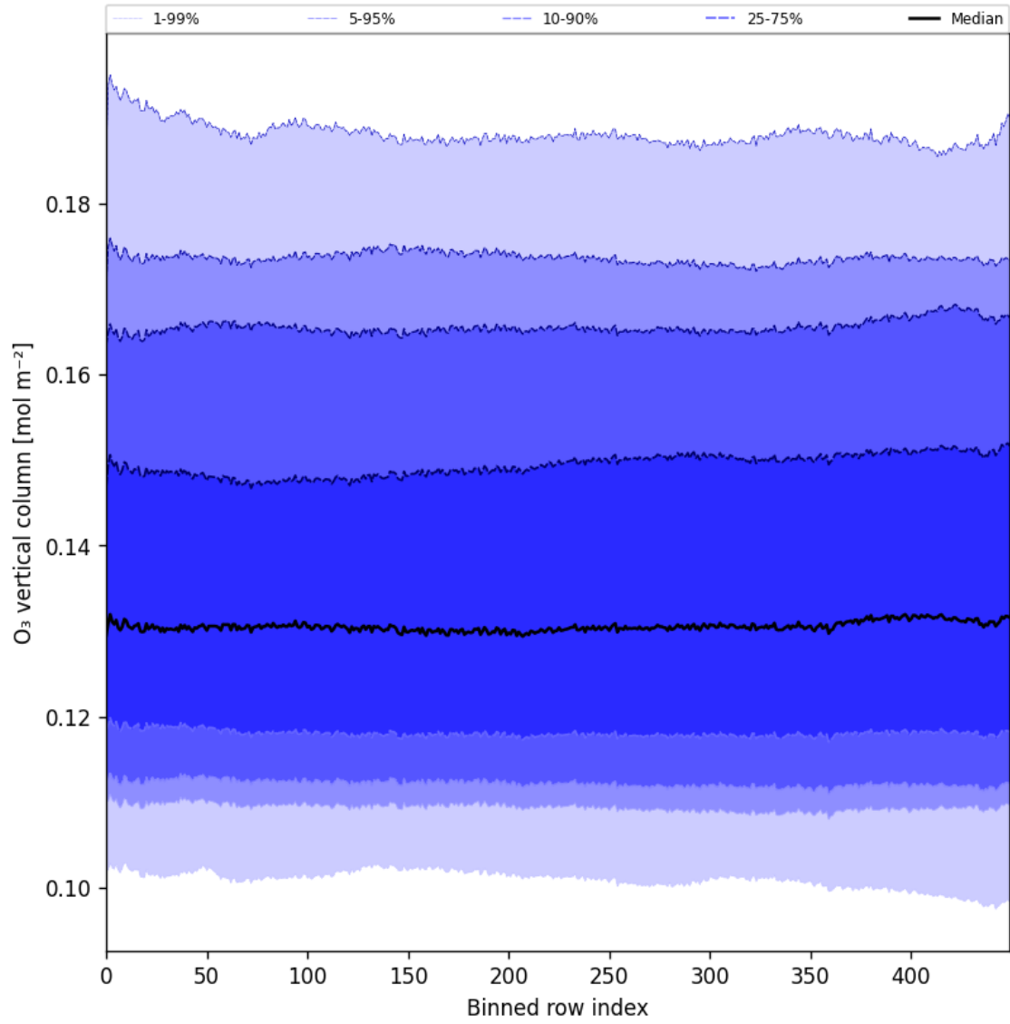
Figure 28: Along track statistics of “ \text{O}_3 vertical column” for 2025-11-16 to 2025-11-18
