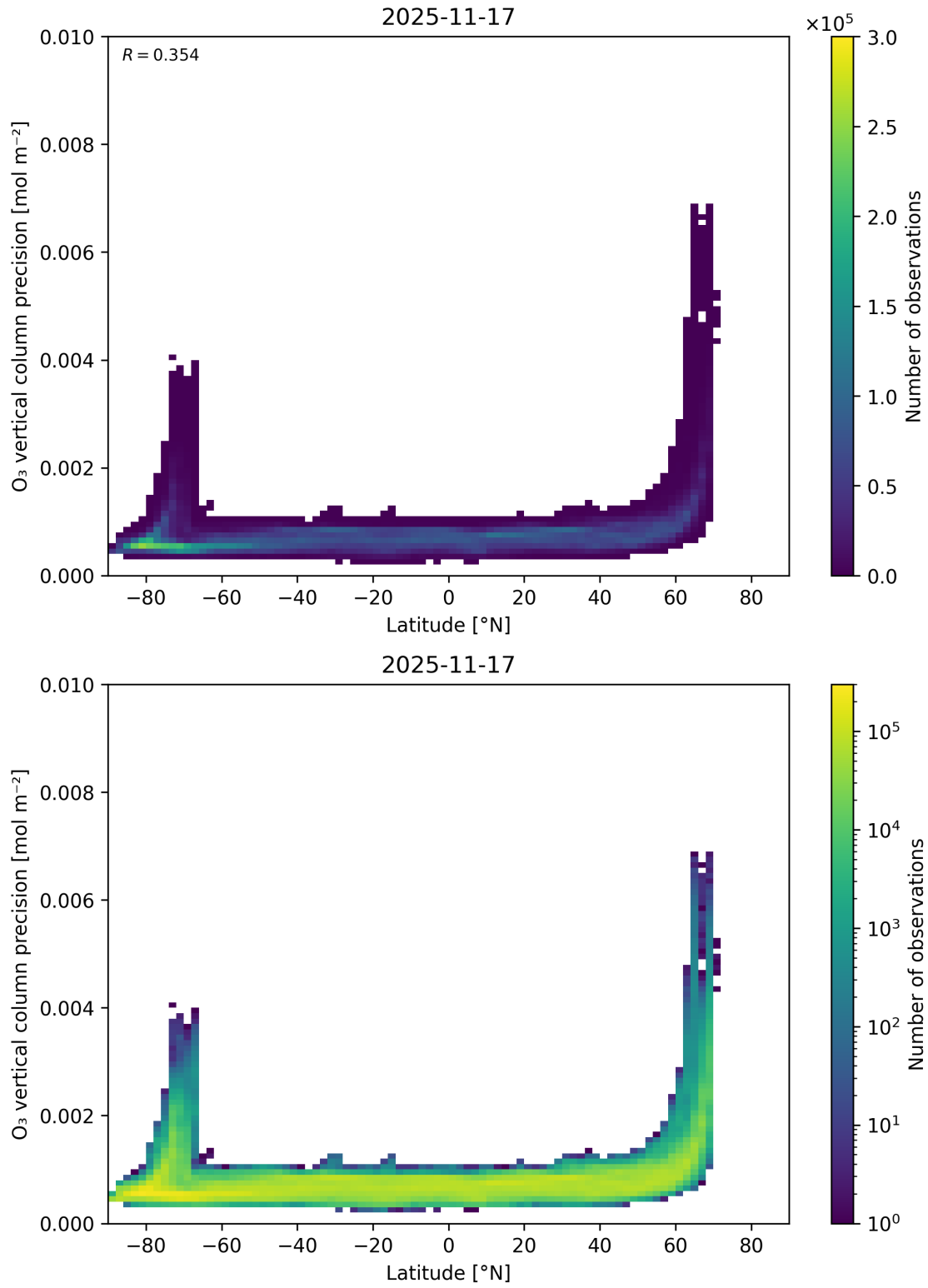
Figure 37: Scatter density plot of “Latitude” against “O 3 vertical column precision” for 2025-11-16 to 2025-11-18.
