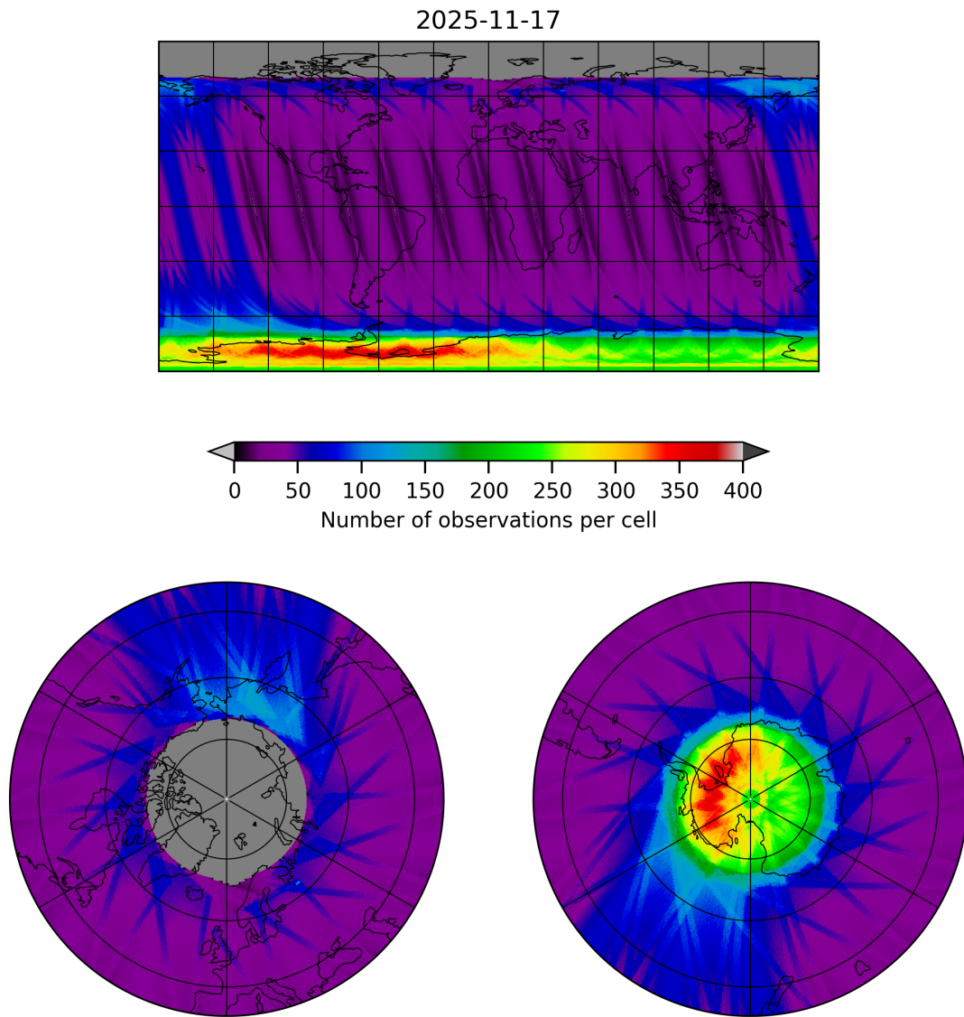
Figure 12: Map of the number of observations for 2025-11-16 to 2025-11-18
