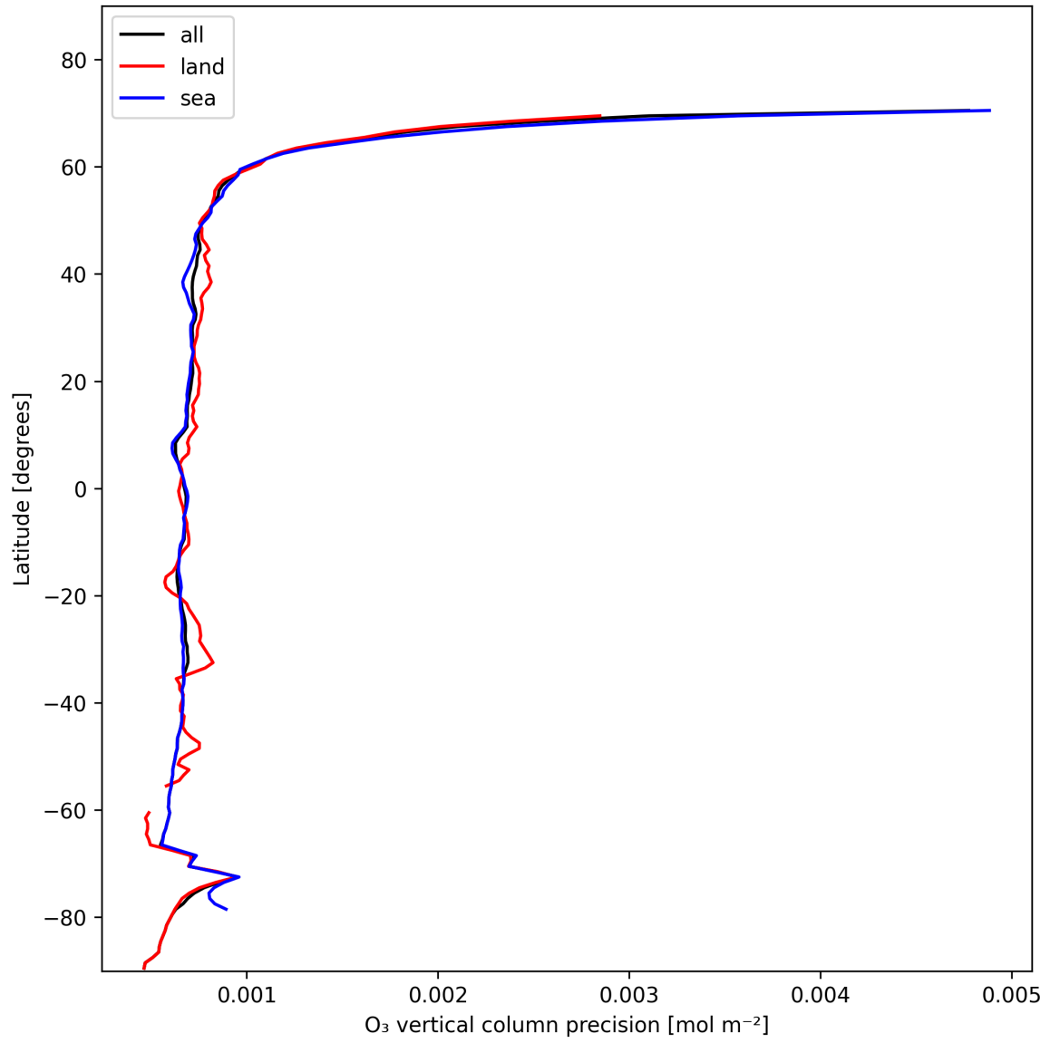
Figure 15: Zonal average of “O 3 vertical column precision” for 2025-11-16 to 2025-11-18.
