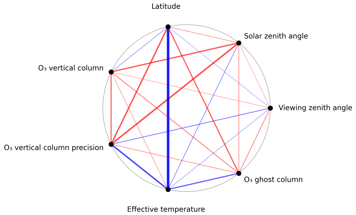
Figure 1: Map of correlation graph for 2025-11-16 to 2025-11-18.
