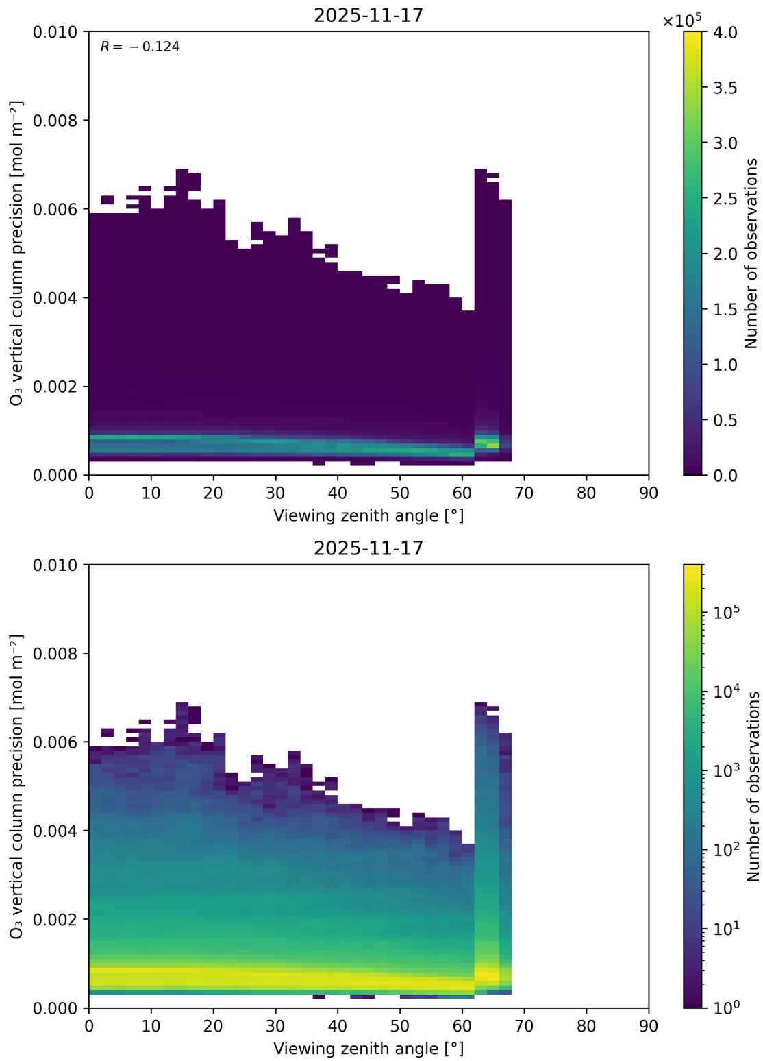
Figure 53: Scatter density plot of “Viewing zenith angle” against “O 3 vertical column precision” for 2025-11-16 to 2025-11-18.
