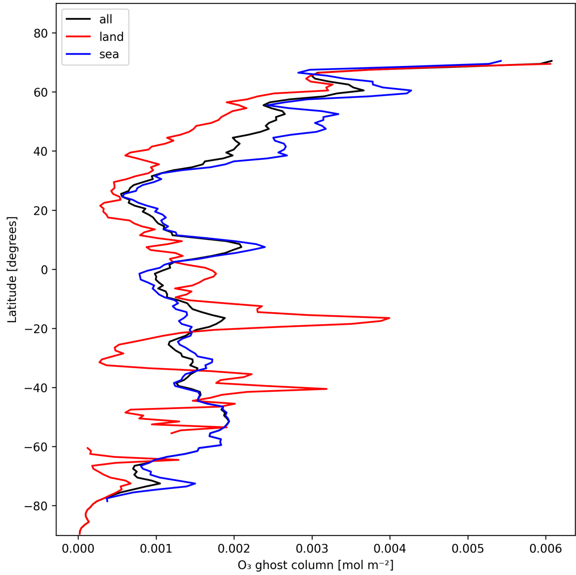
Figure 18: Zonal average of "O 3 ghost column" for 2025-11-16 to 2025-11-18.
