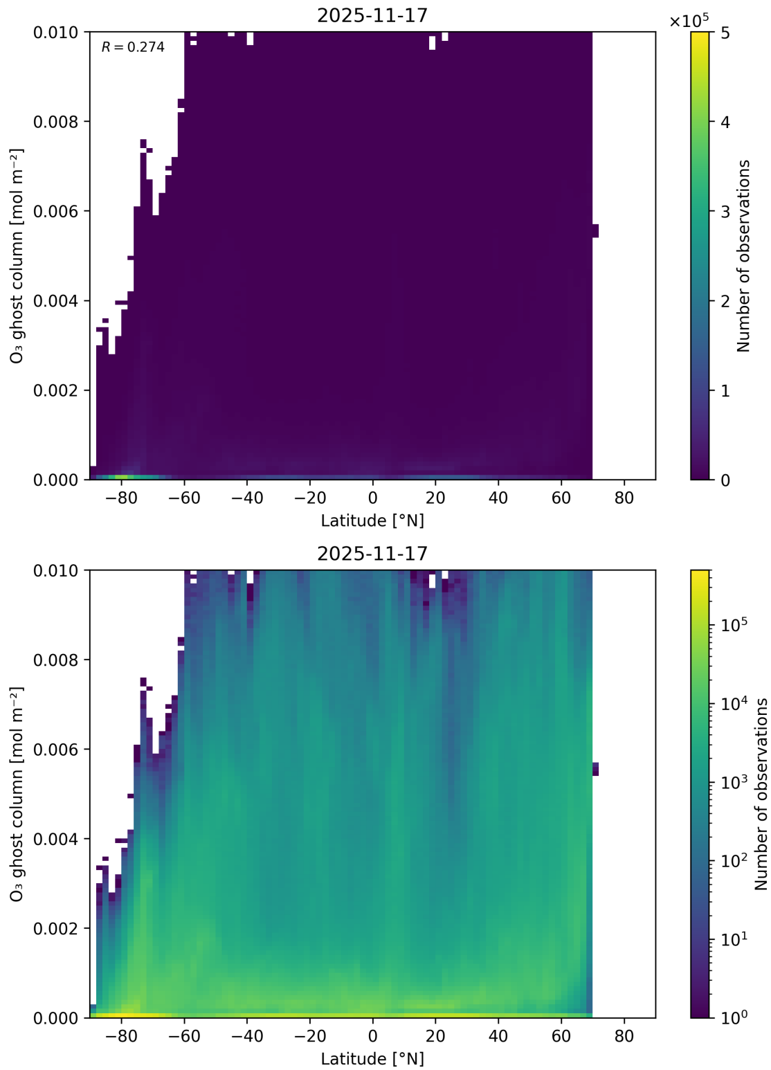
Figure 35: Scatter density plot of “Latitude” against “O 3 ghost column” for 2025-11-16 to 2025-11-18.
