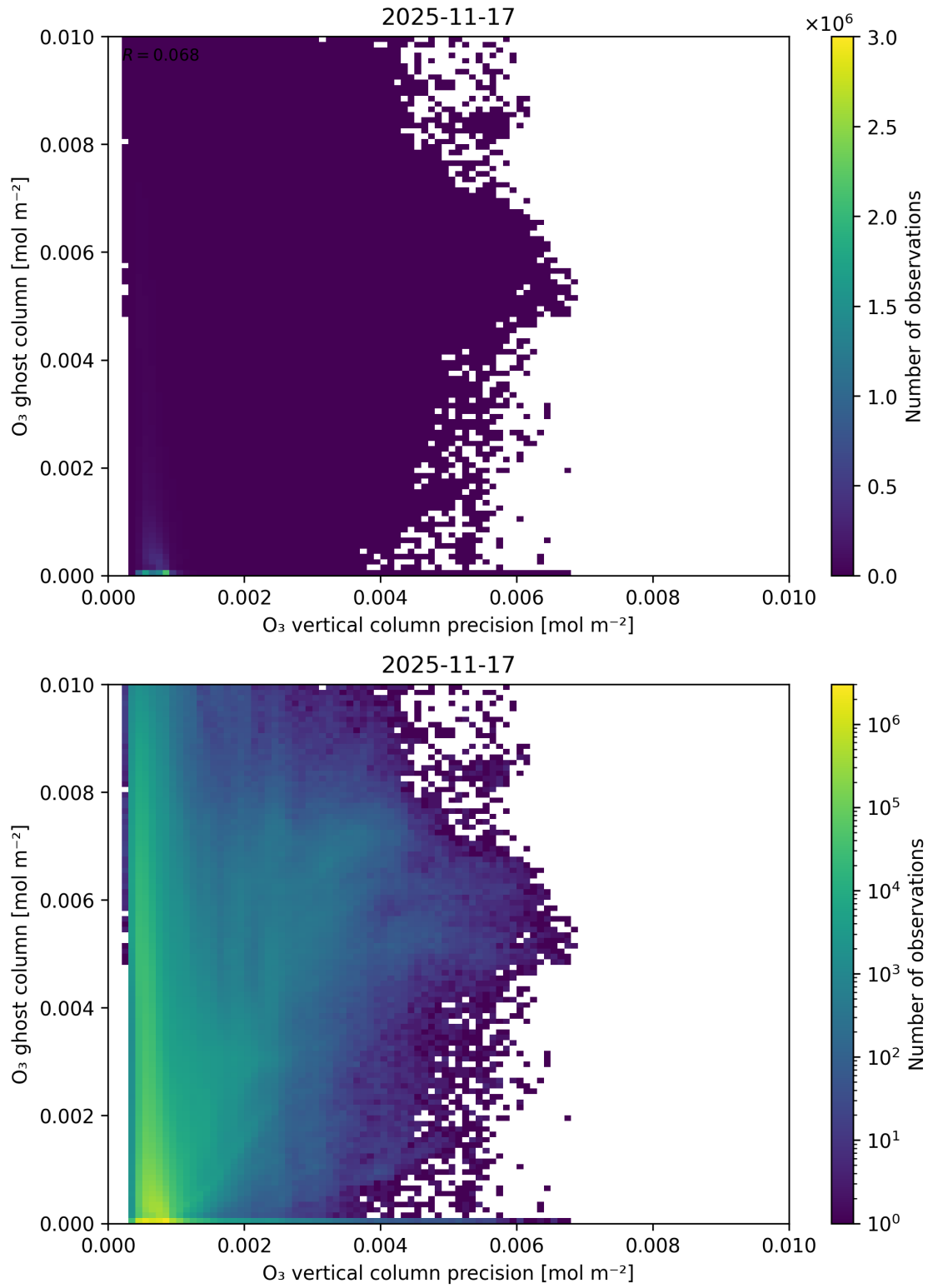
Figure 43: Scatter density plot of “ \text{O}_3 vertical column precision” against “ \text{O}_3 ghost column” for 2025-11-16 to 2025-11-18.
