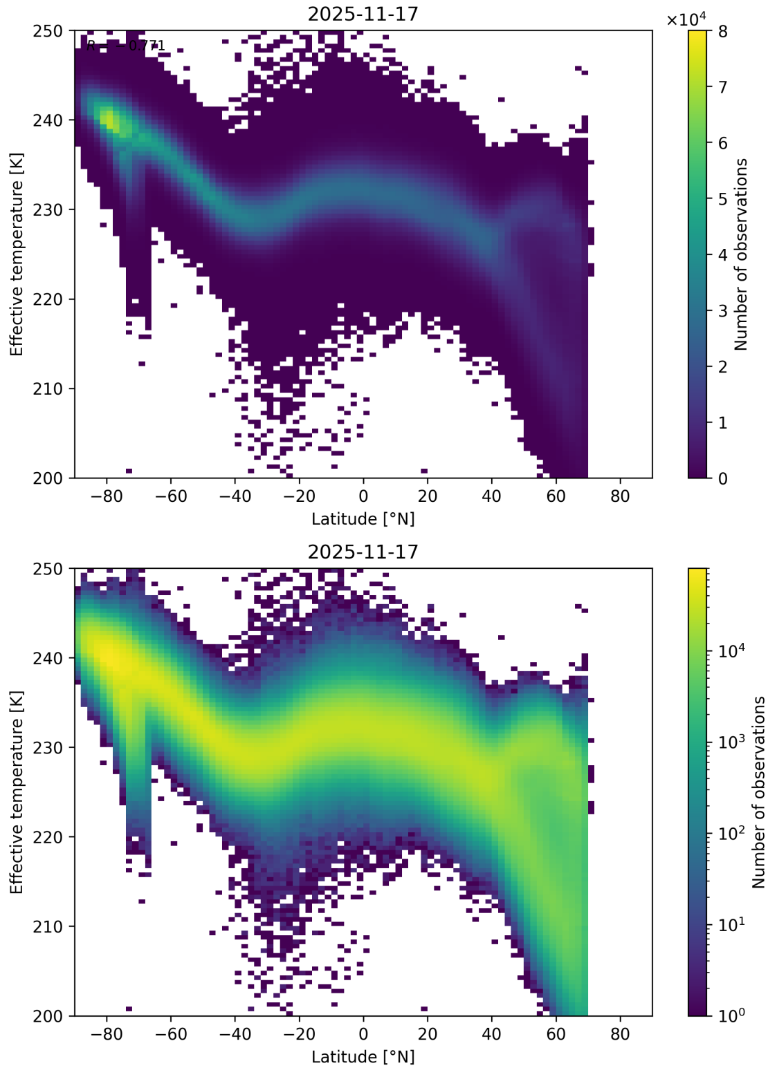
Figure 34: Scatter density plot of “Latitude” against “Effective temperature” for 2025-11-16 to 2025-11-18.
