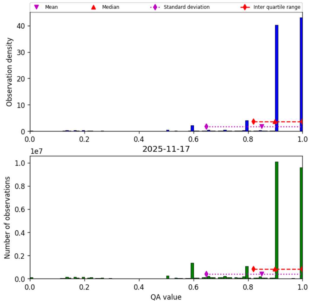
Figure 20: Histogram of “QA value” for 2025-11-16 to 2025-11-18
