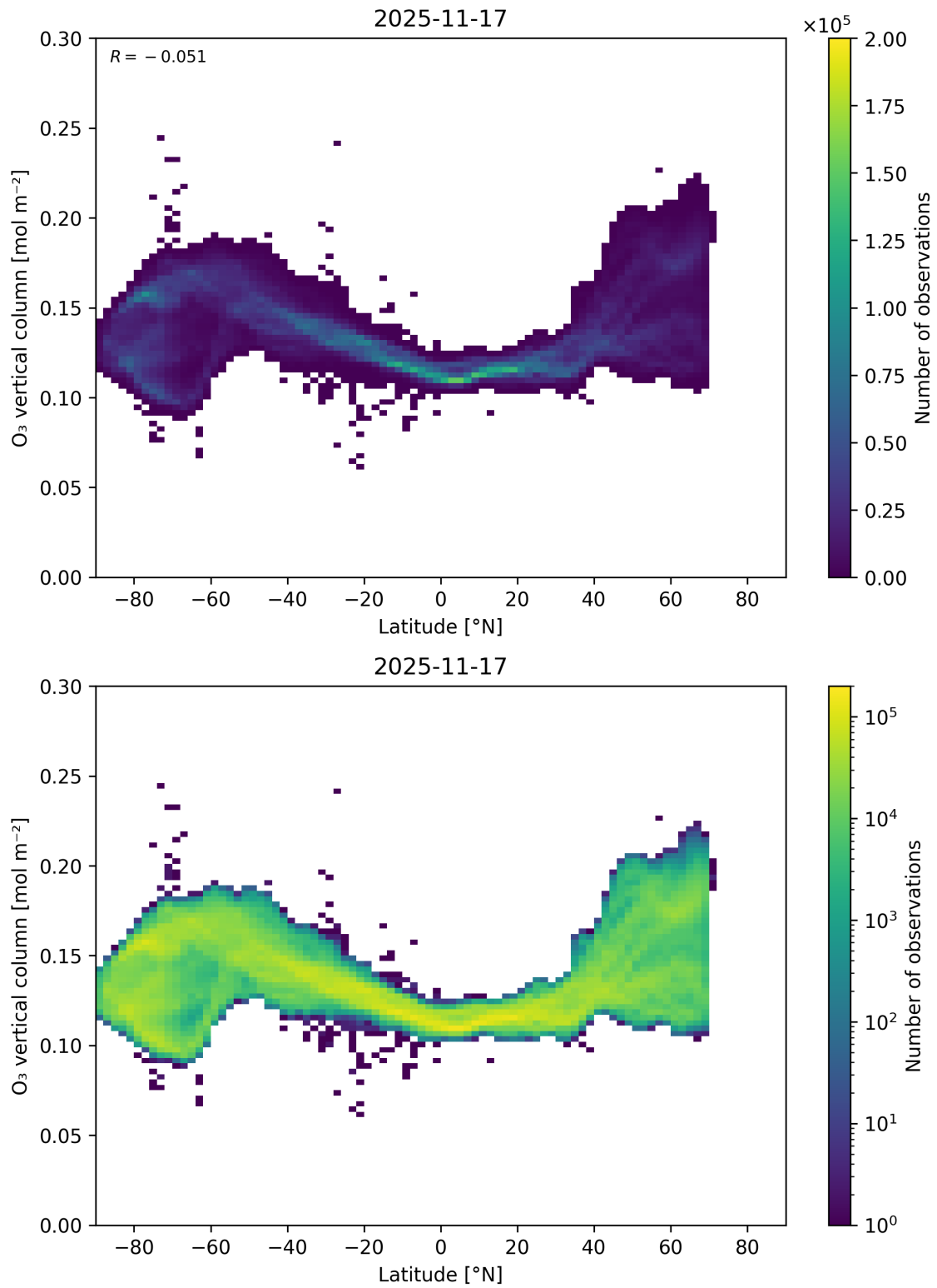
Figure 36: Scatter density plot of “Latitude” against “O 3 vertical column” for 2025-11-16 to 2025-11-18.
