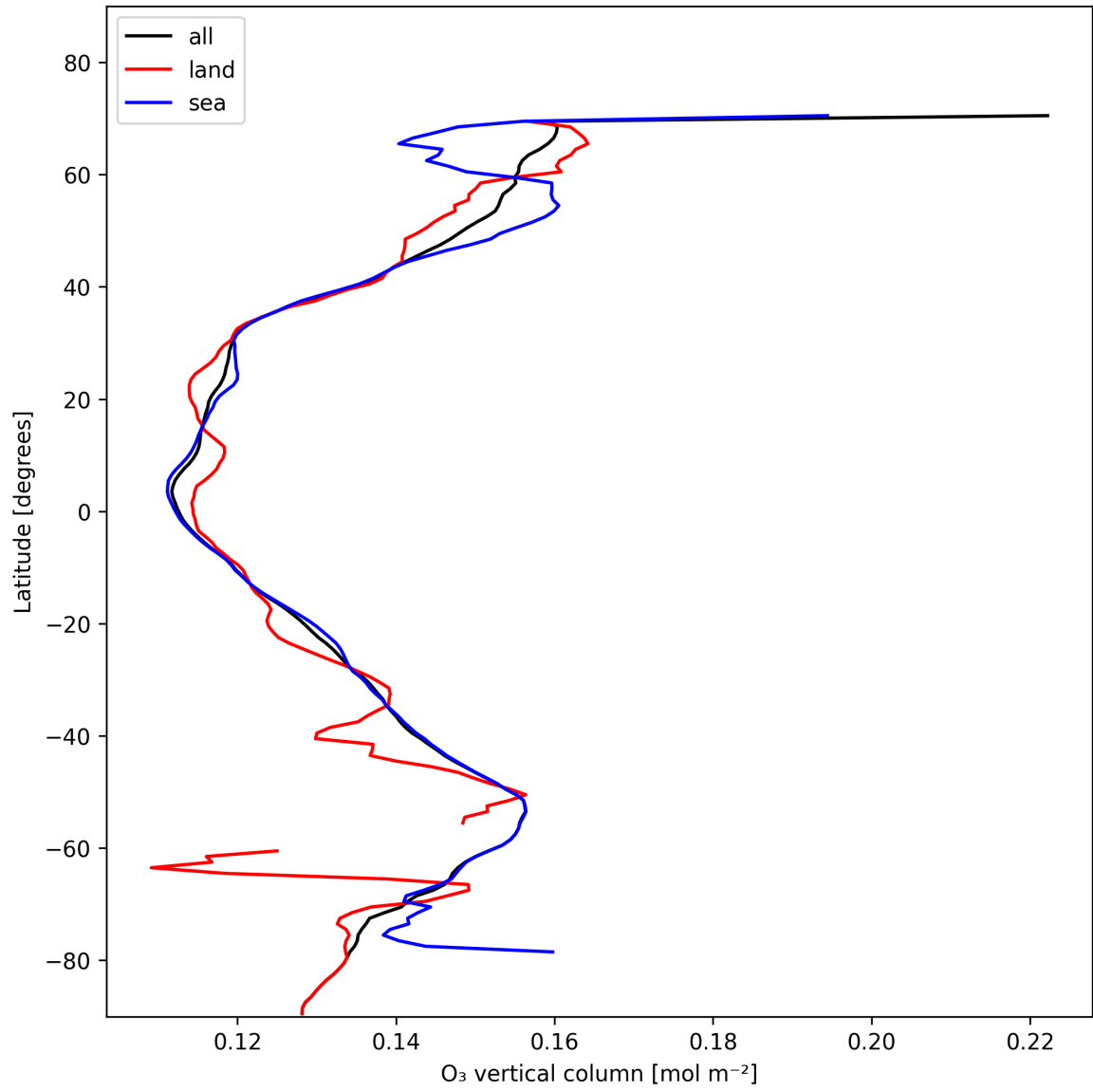
Figure 14: Zonal average of “O 3 vertical column” for 2025-11-16 to 2025-11-18.
