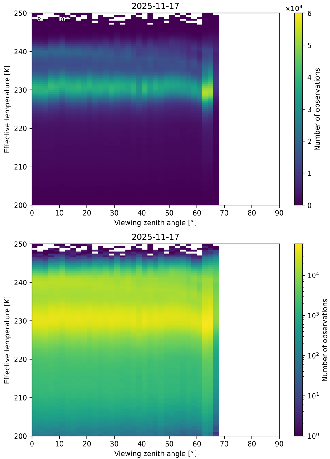
Figure 50: Scatter density plot of “Viewing zenith angle” against “Effective temperature” for 2025-11-16 to 2025-11-18.
