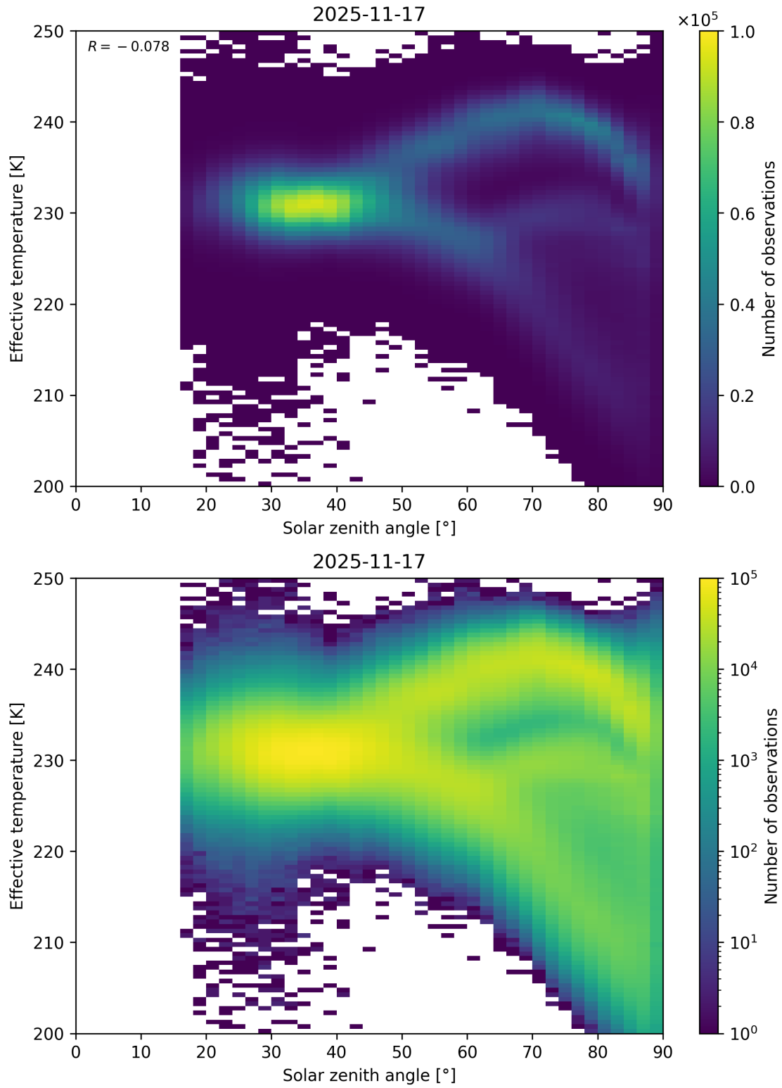
Figure 45: Scatter density plot of “Solar zenith angle” against “Effective temperature” for 2025-11-16 to 2025-11-18.
