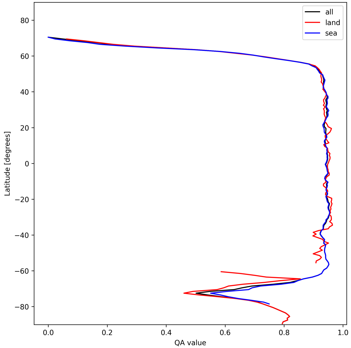
Figure 13: Zonal average of “QA value” for 2025-11-16 to 2025-11-18.
