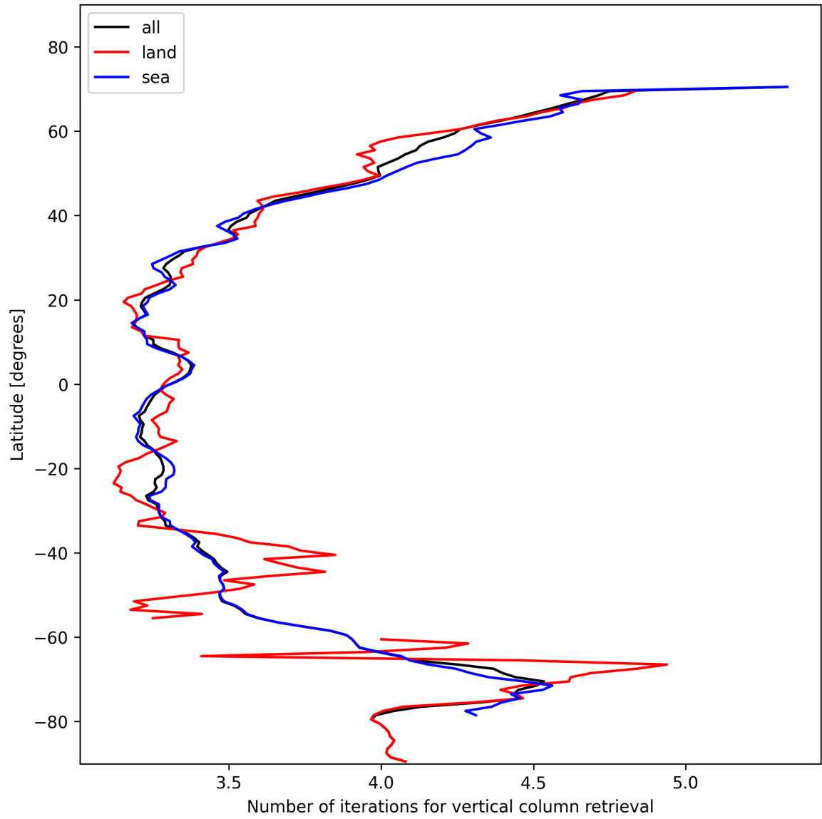
Figure 19: Zonal average of “Number of iterations for vertical column retrieval” for 2025-11-16 to 2025-11-18.
