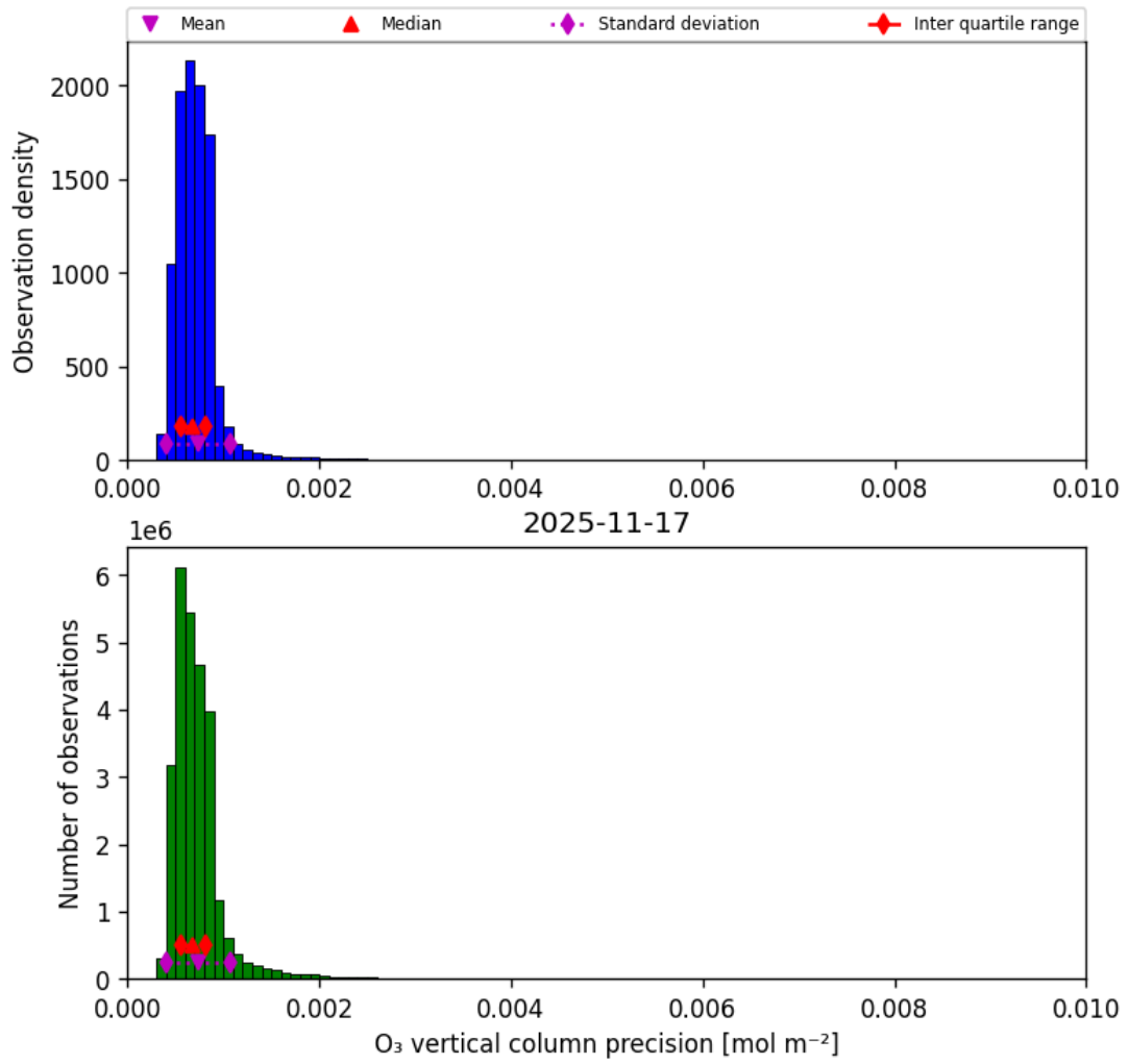
Figure 22: Histogram of “O 3 vertical column precision” for 2025-11-16 to 2025-11-18
