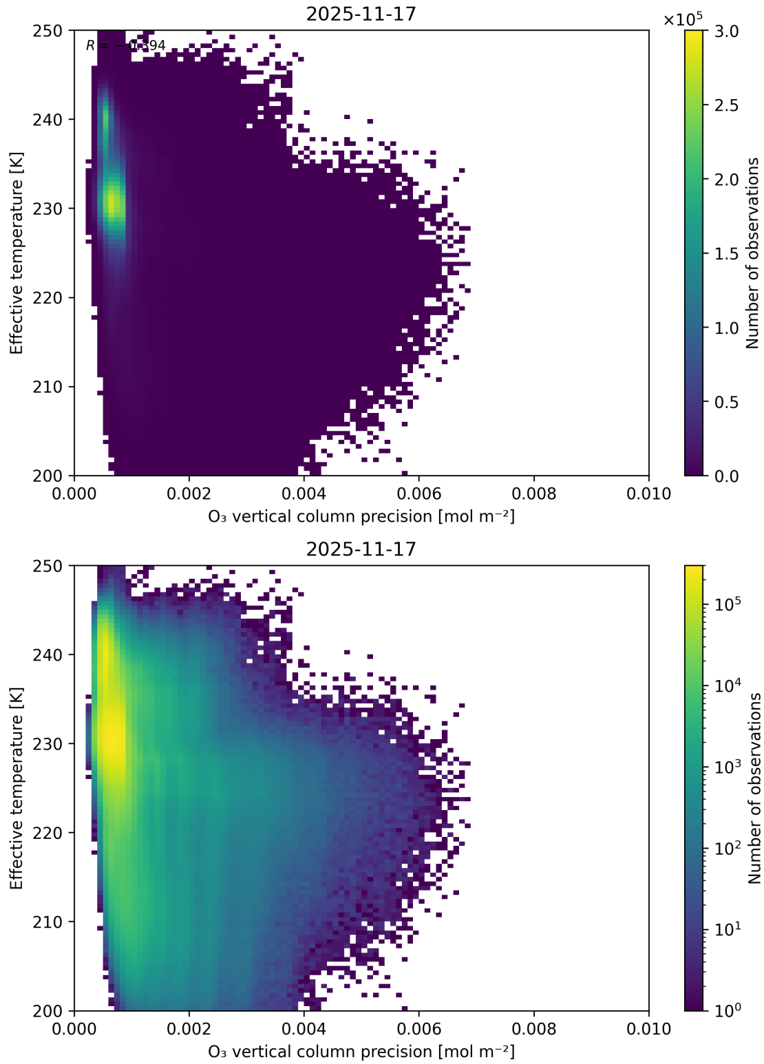
Figure 42: Scatter density plot of “O 3 vertical column precision” against “Effective temperature” for 2025-11-16 to 2025-11-18.
