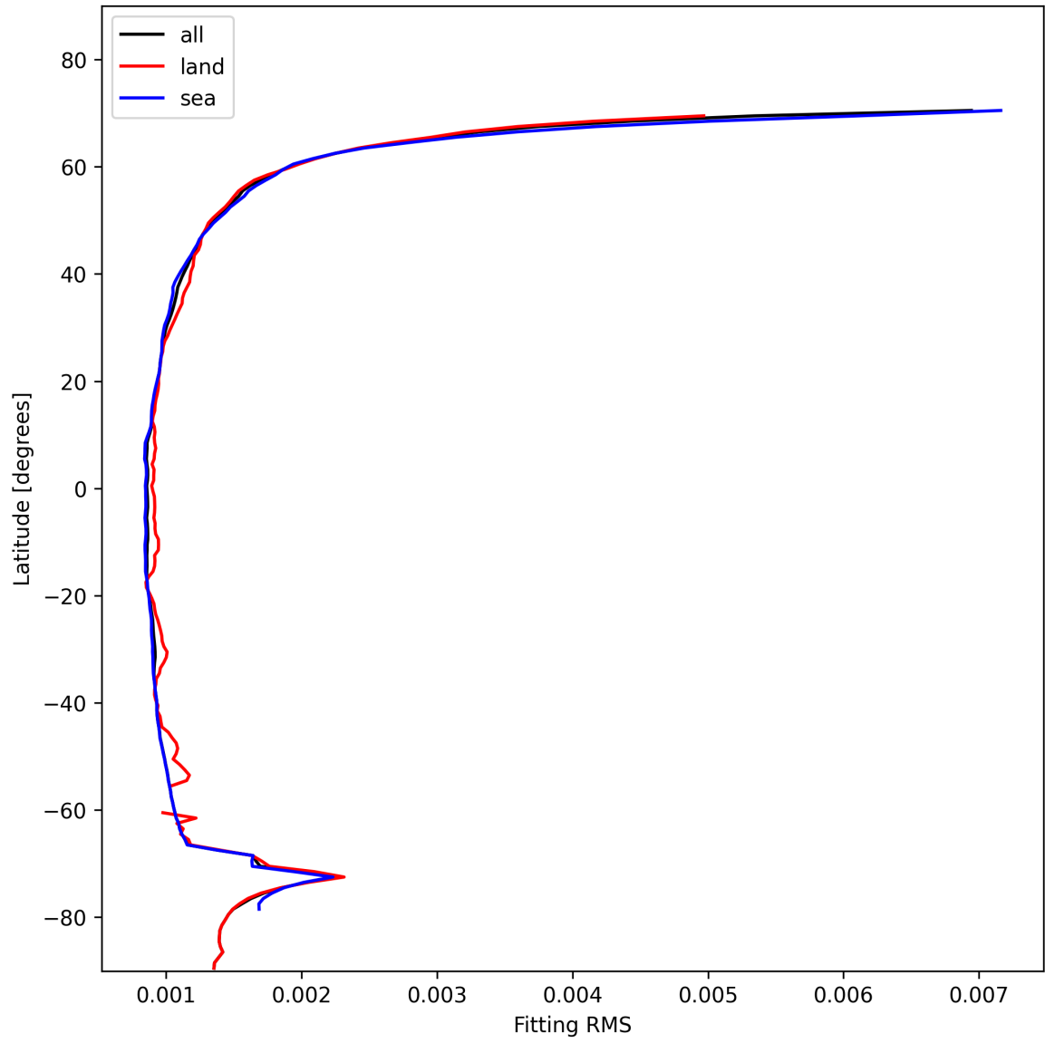
Figure 16: Zonal average of “Fitting RMS” for 2025-11-16 to 2025-11-18.
