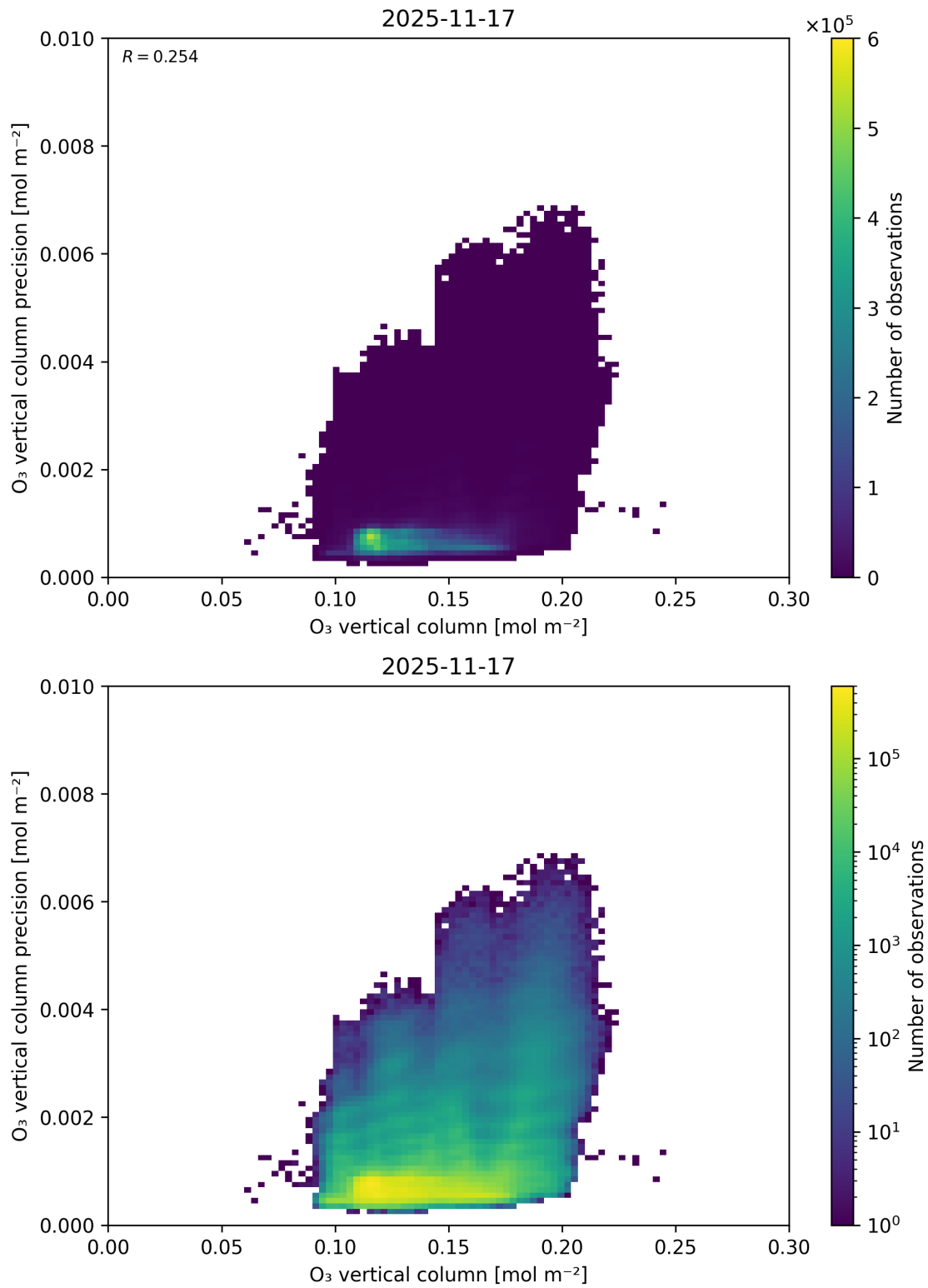
Figure 41: Scatter density plot of “O 3 vertical column” against “O 3 vertical column precision” for 2025-11-16 to 2025-11-18.
