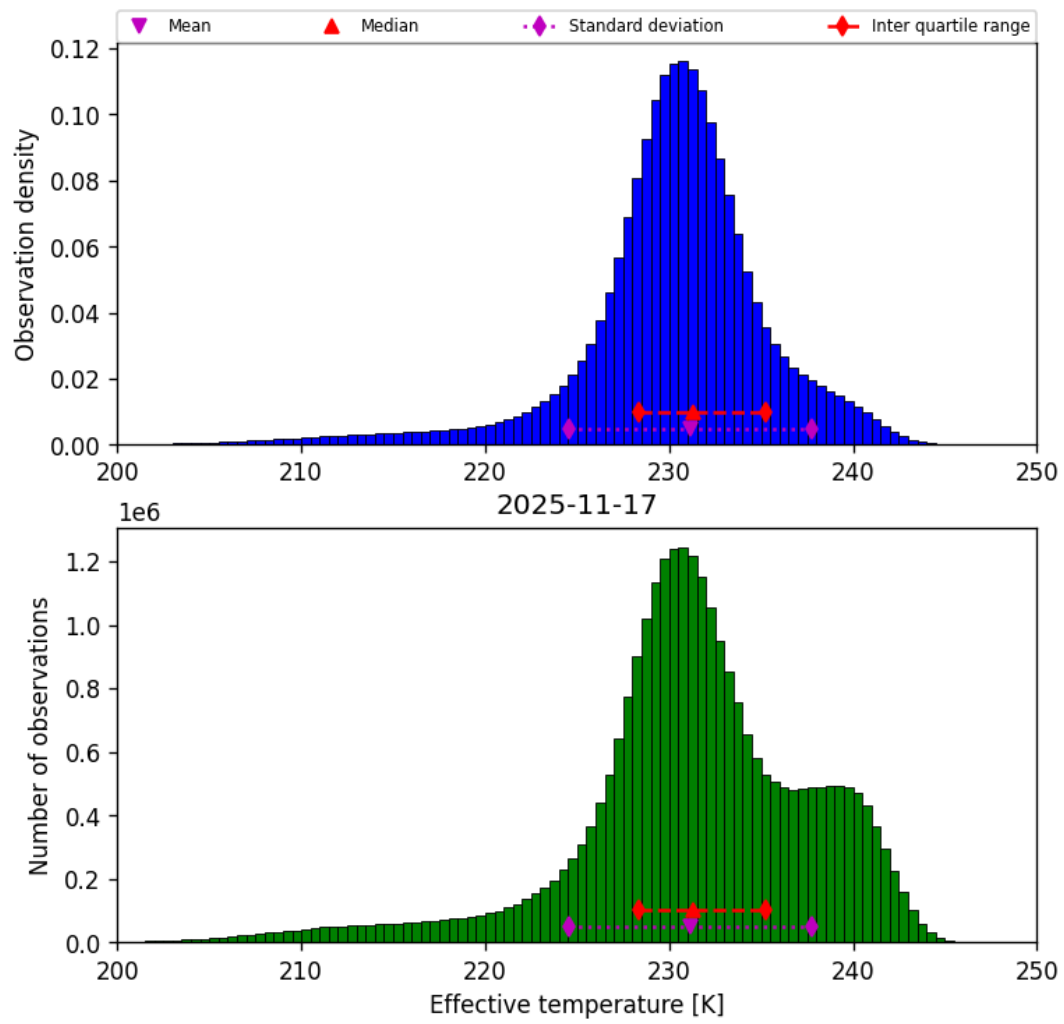
Figure 24: Histogram of “Effective temperature” for 2025-11-16 to 2025-11-18
