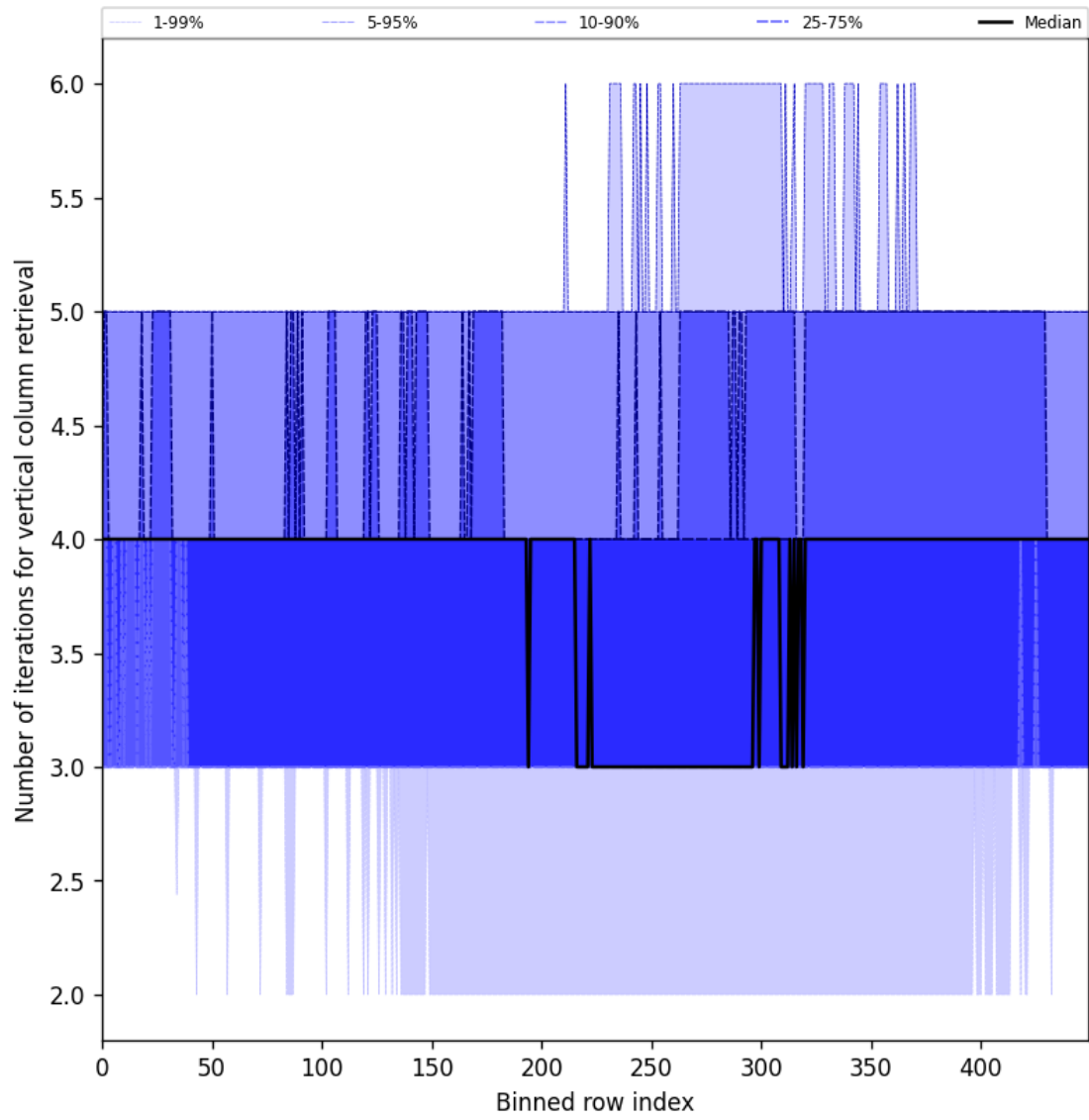
Figure 33: Along track statistics of “Number of iterations for vertical column retrieval” for 2025-11-16 to 2025-11-18
