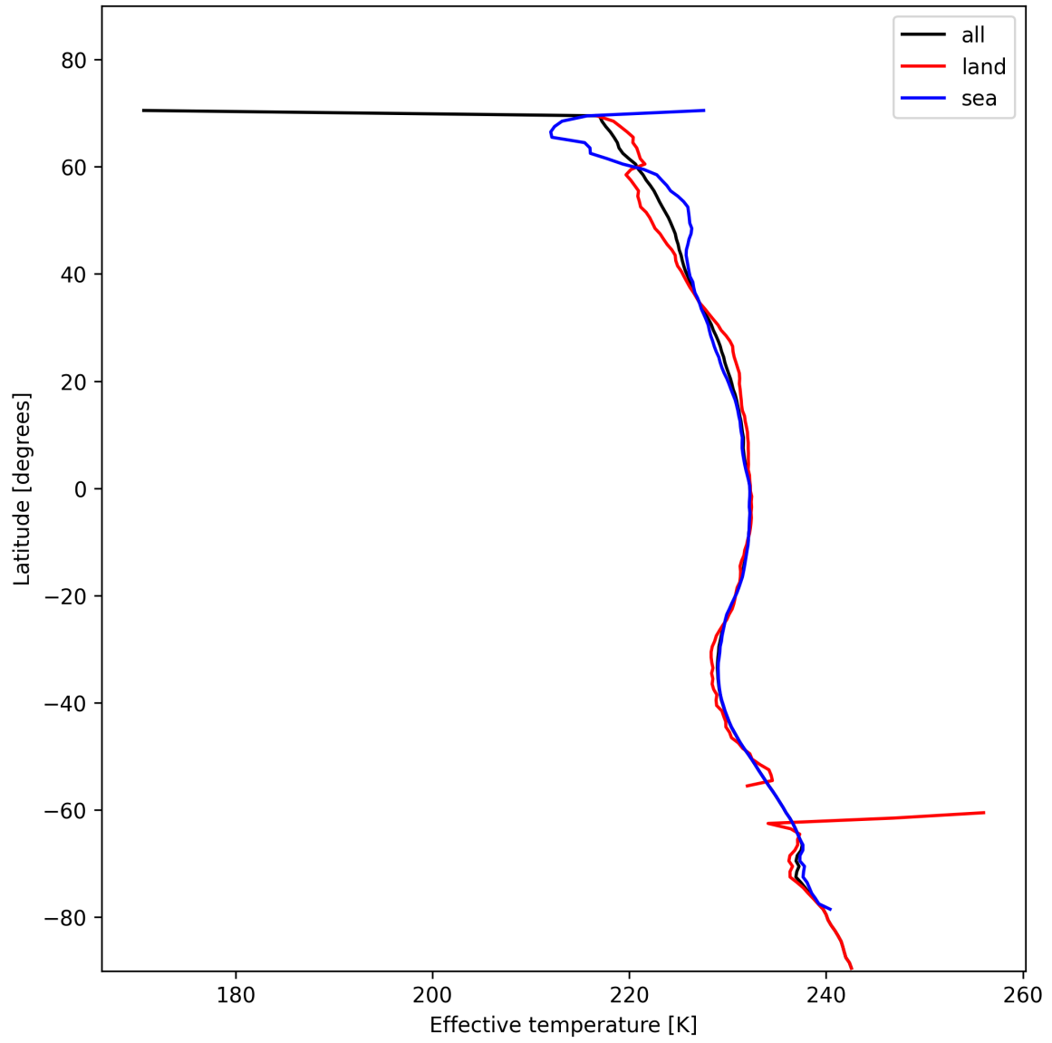
Figure 17: Zonal average of “Effective temperature” for 2025-11-16 to 2025-11-18.
