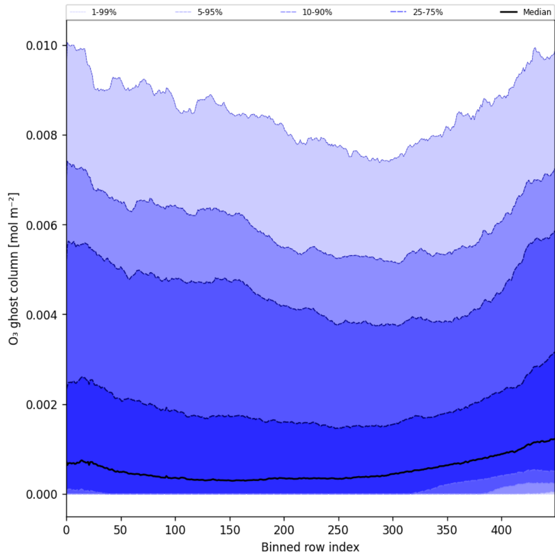
Figure 32: Along track statistics of “O 3 ghost column” for 2025-11-16 to 2025-11-18
