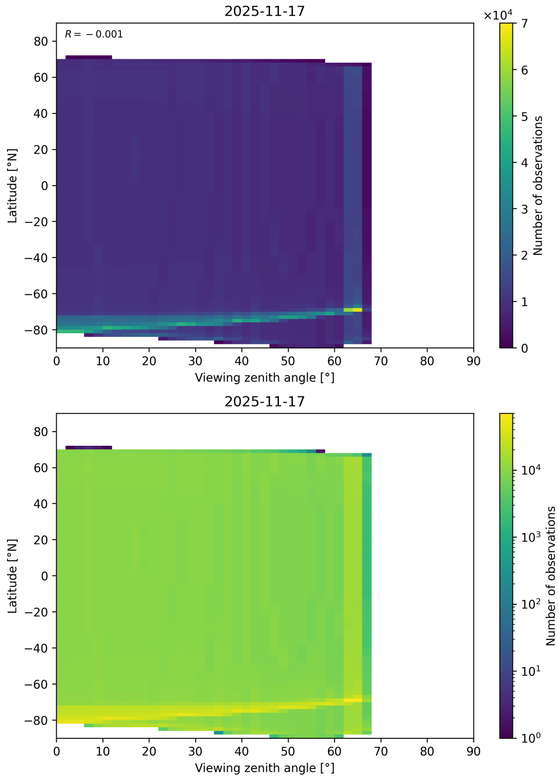
Figure 49: Scatter density plot of “Viewing zenith angle” against “Latitude” for 2025-11-16 to 2025-11-18.
