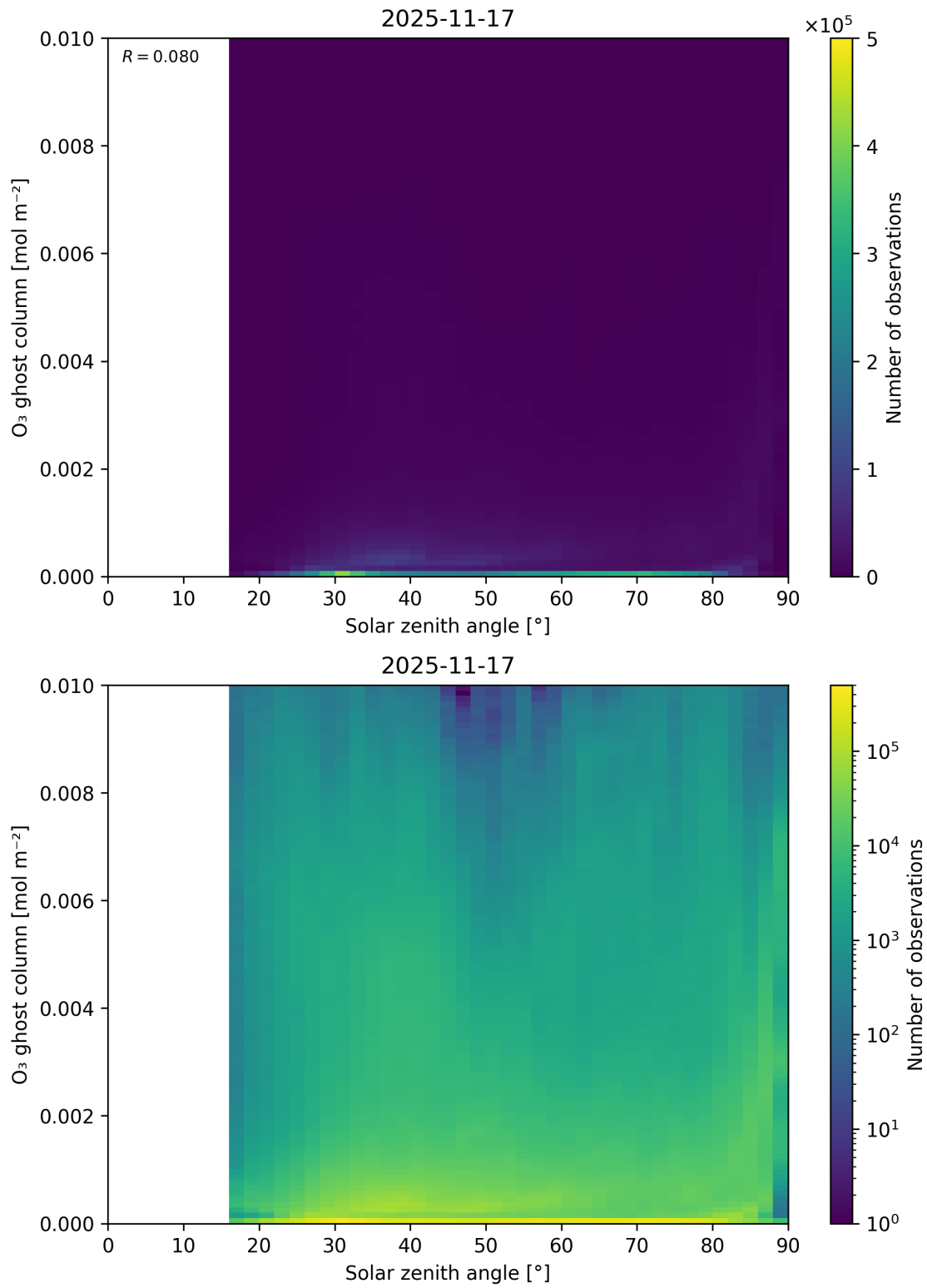
Figure 46: Scatter density plot of “Solar zenith angle” against “O 3 ghost column” for 2025-11-16 to 2025-11-18.
