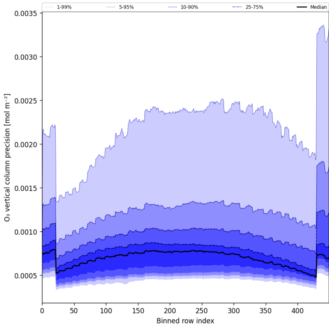
Figure 29: Along track statistics of “O 3 vertical column precision” for 2025-11-16 to 2025-11-18
