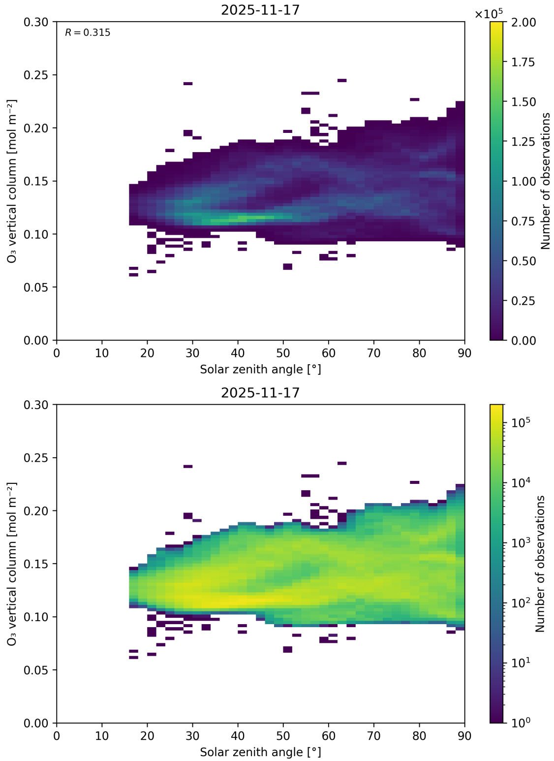
Figure 47: Scatter density plot of “Solar zenith angle” against “O 3 vertical column” for 2025-11-16 to 2025-11-18.
