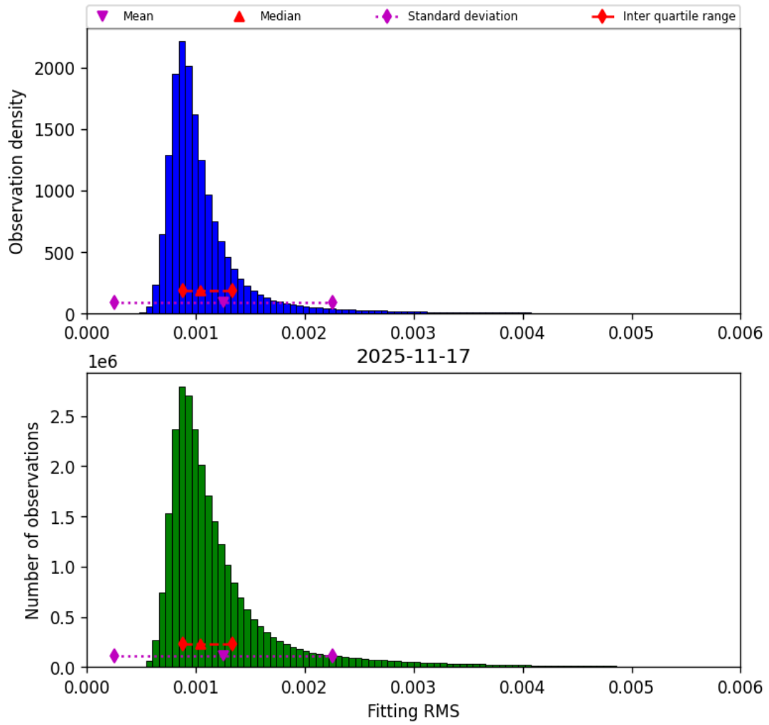
Figure 23: Histogram of “Fitting RMS” for 2025-11-16 to 2025-11-18
