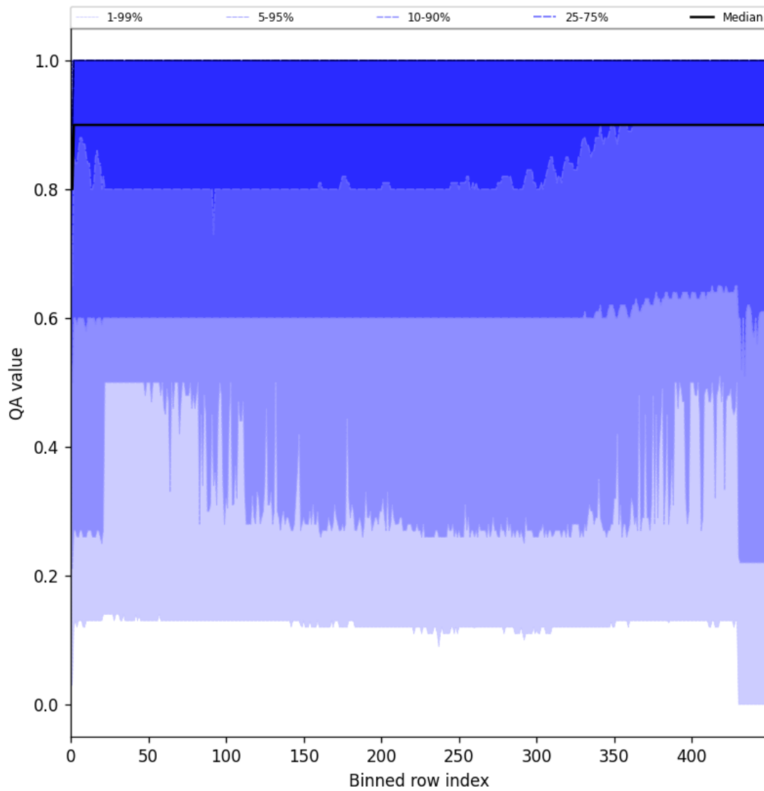
Figure 27: Along track statistics of “QA value” for 2025-11-16 to 2025-11-18
