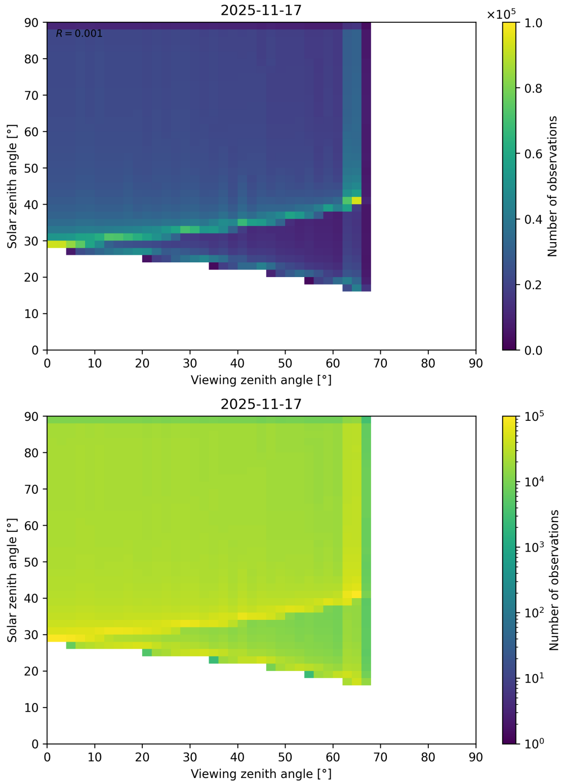
Figure 54: Scatter density plot of “Viewing zenith angle” against “Solar zenith angle” for 2025-11-16 to 2025-11-18.
