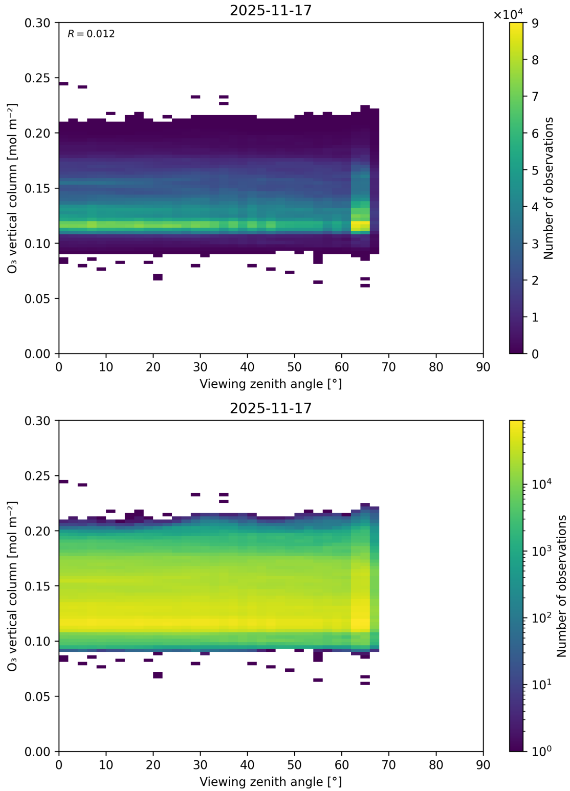
Figure 52: Scatter density plot of “Viewing zenith angle” against “O 3 vertical column” for 2025-11-16 to 2025-11-18.
