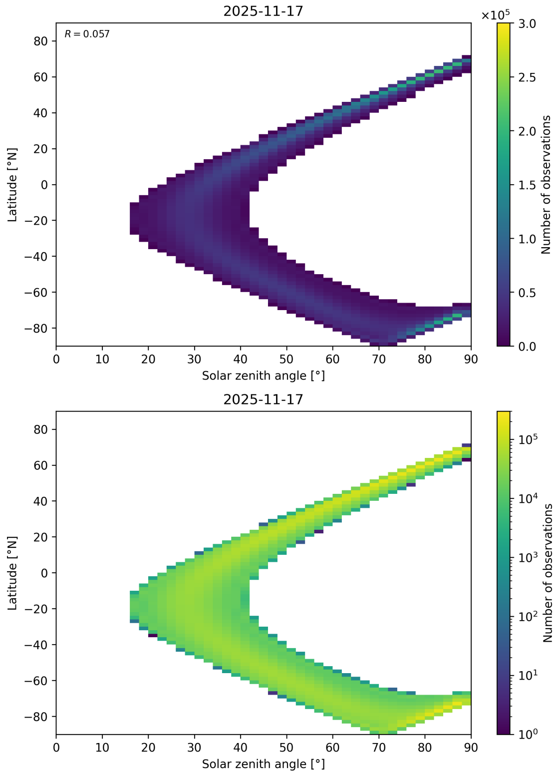
Figure 44: Scatter density plot of “Solar zenith angle” against “Latitude” for 2025-11-16 to 2025-11-18.
