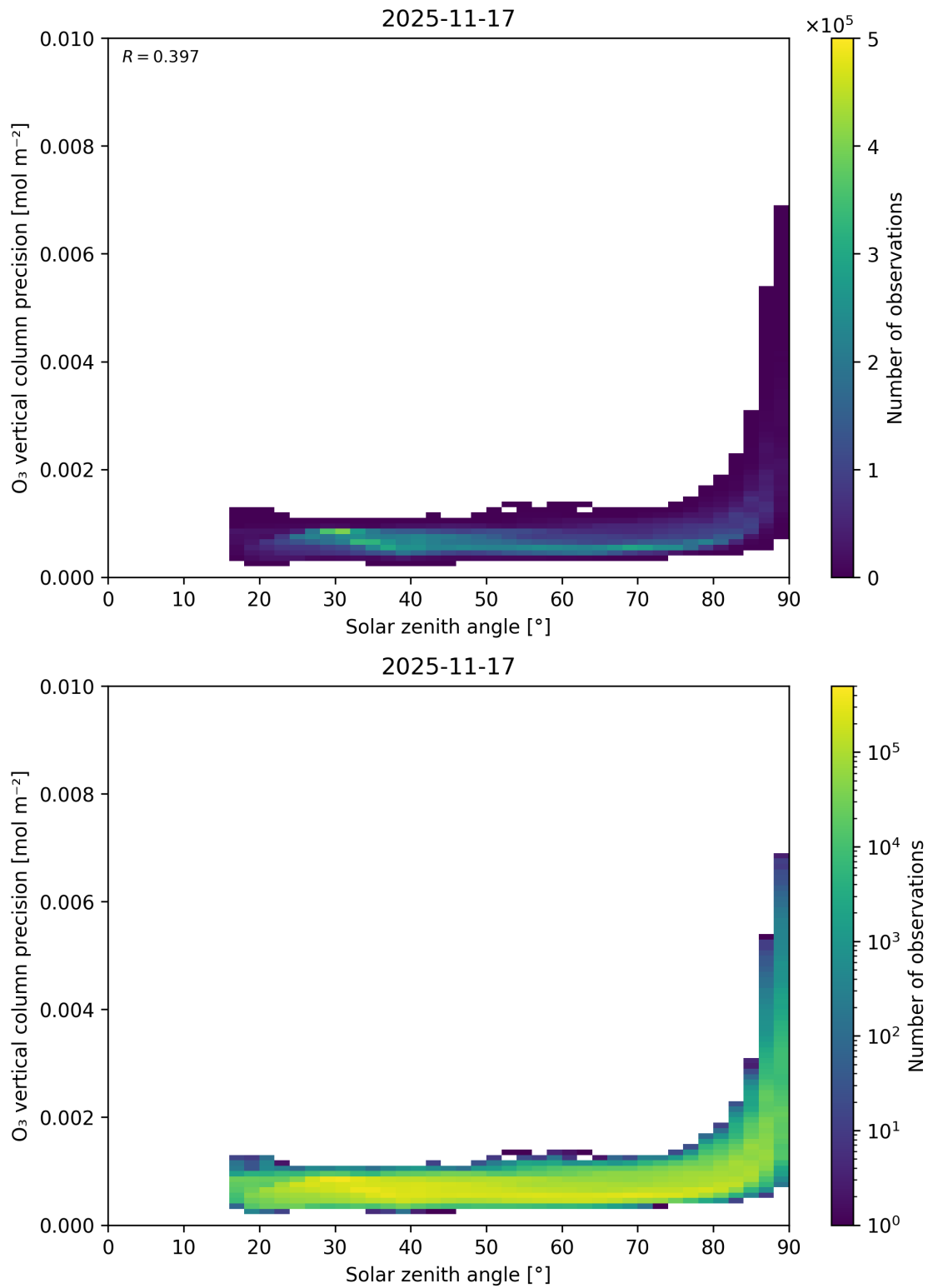
Figure 48: Scatter density plot of “Solar zenith angle” against “O 3 vertical column precision” for 2025-11-16 to 2025-11-18.
