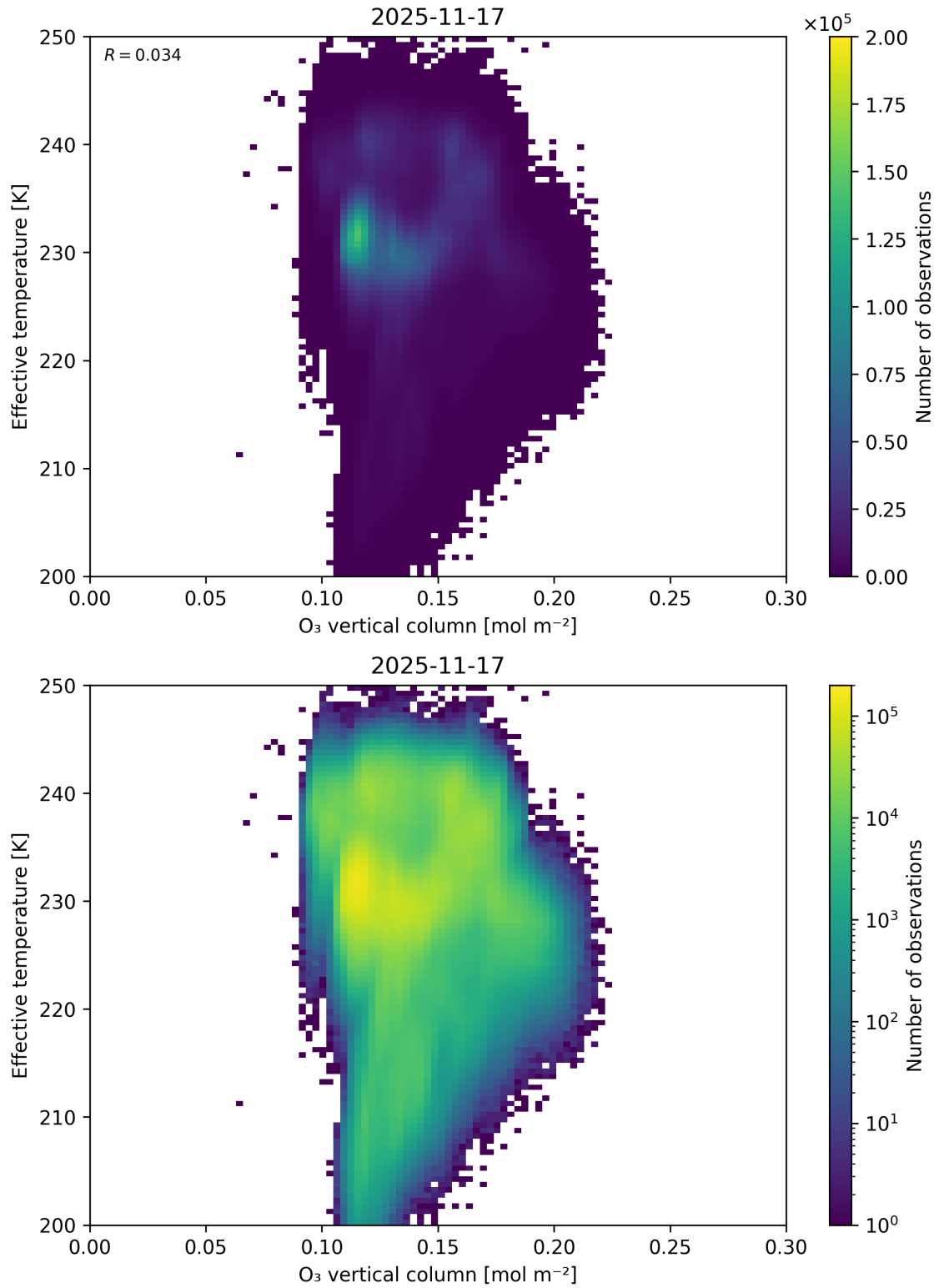
Figure 39: Scatter density plot of “O 3 vertical column” against “Effective temperature” for 2025-11-16 to 2025-11-18.
