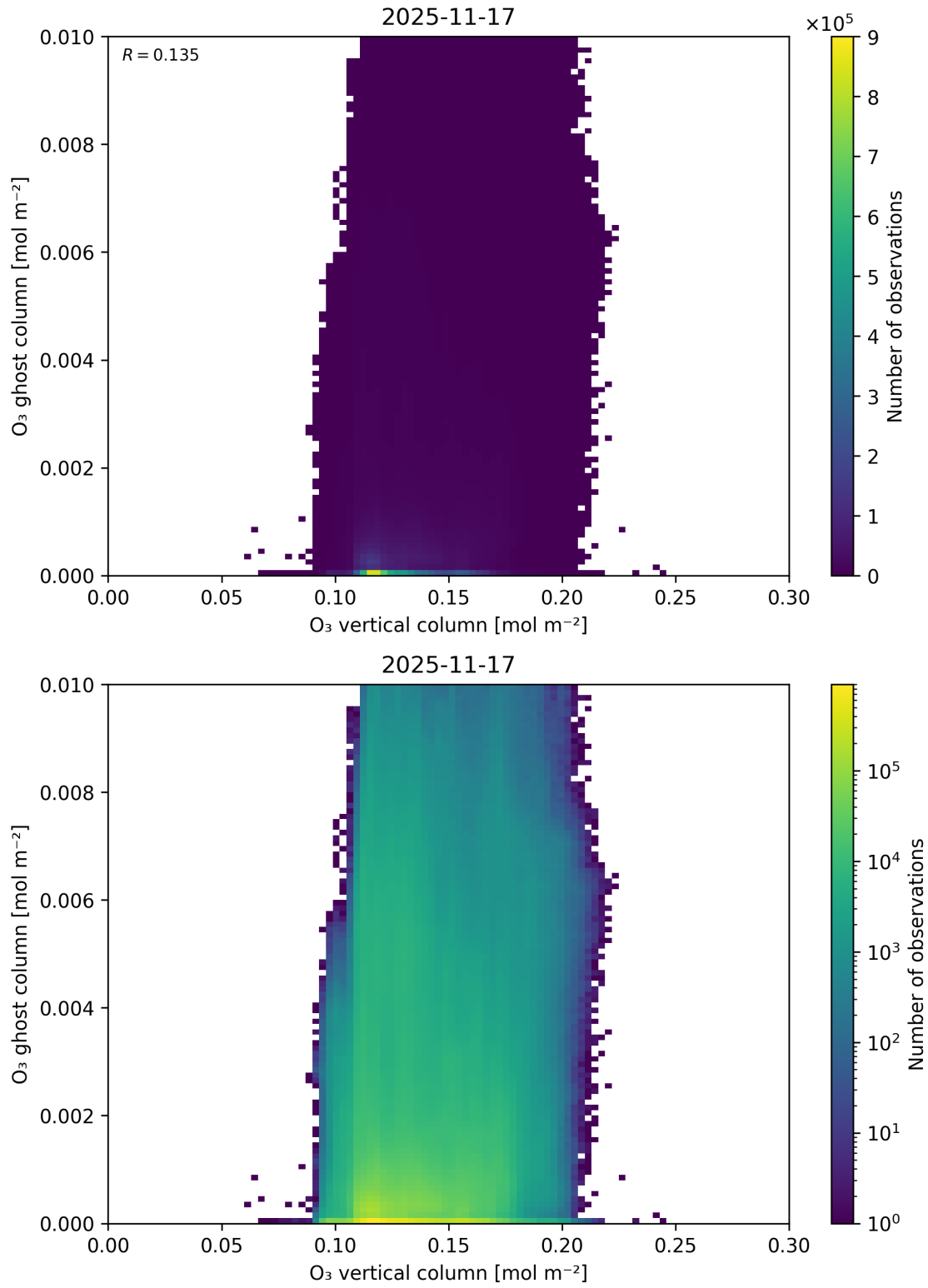
Figure 40: Scatter density plot of “O 3 vertical column” against “O 3 ghost column” for 2025-11-16 to 2025-11-18.
