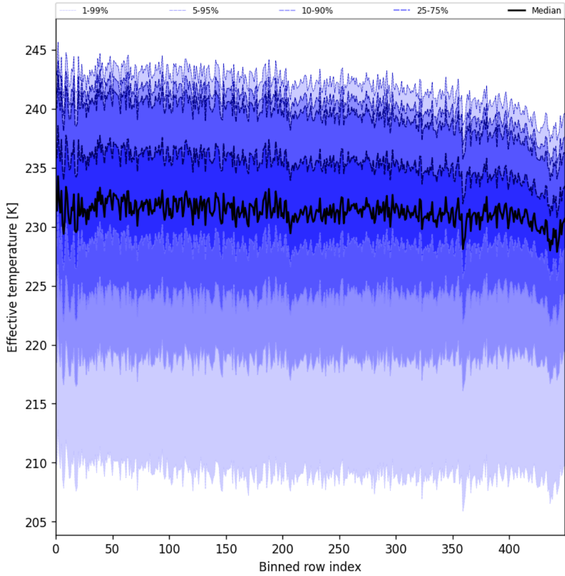
Figure 31: Along track statistics of “Effective temperature” for 2025-11-16 to 2025-11-18
