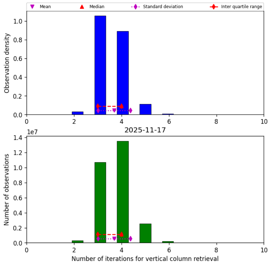
Figure 26: Histogram of “Number of iterations for vertical column retrieval” for 2025-11-16 to 2025-11-18
