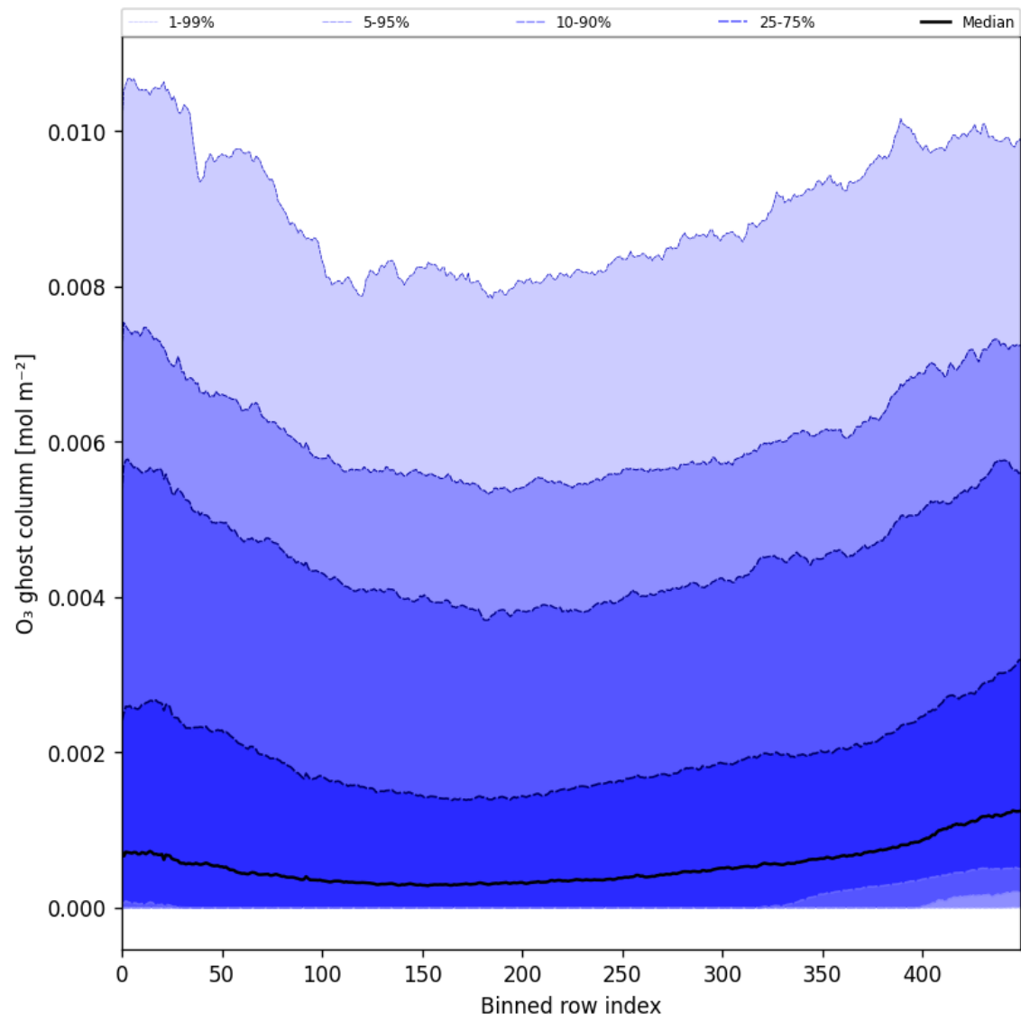
Figure 32: Along track statistics of “O 3 ghost column” for 2025-11-18 to 2025-11-19
