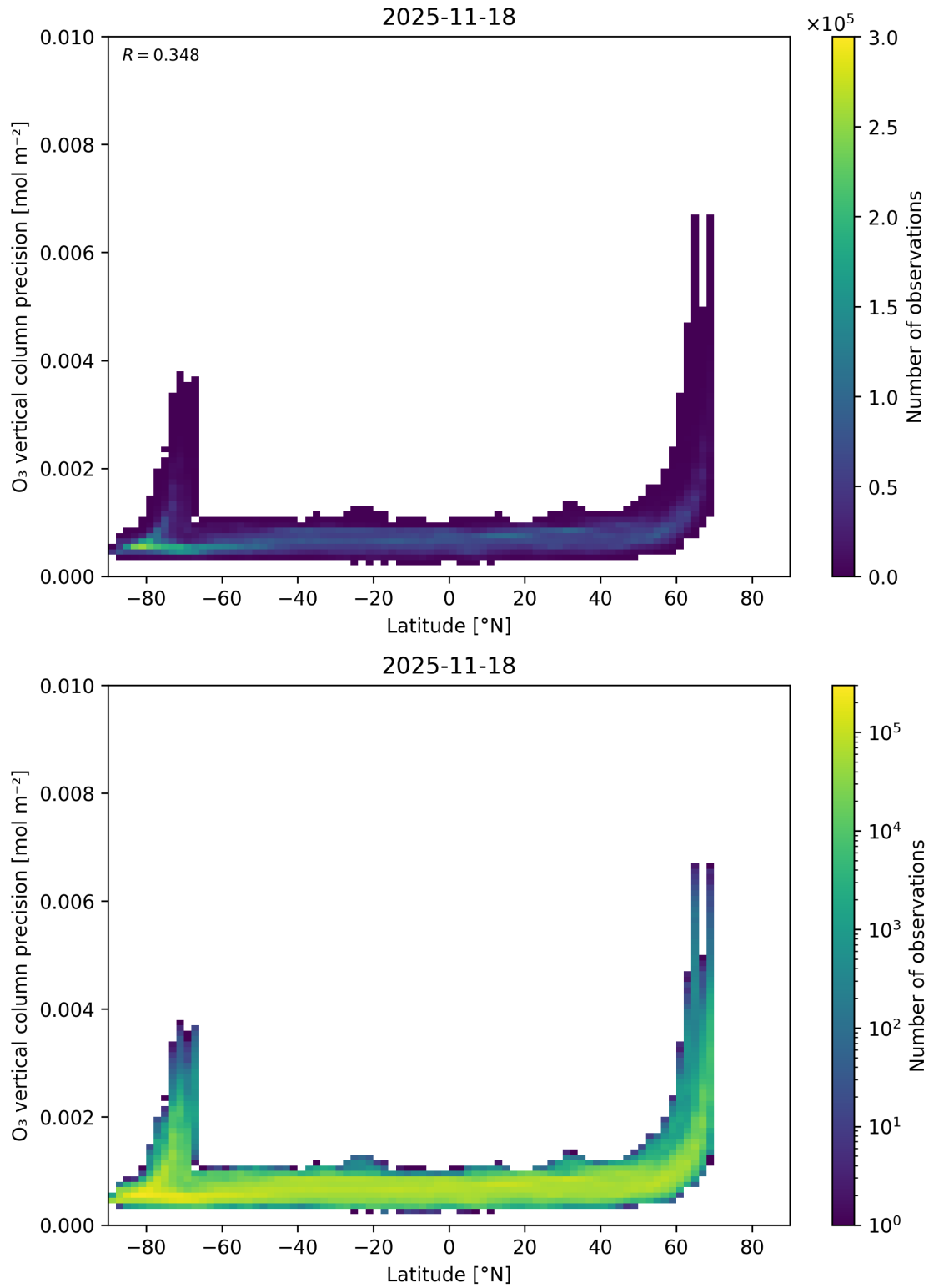
Figure 37: Scatter density plot of “Latitude” against “O 3 vertical column precision” for 2025-11-18 to 2025-11-19.
