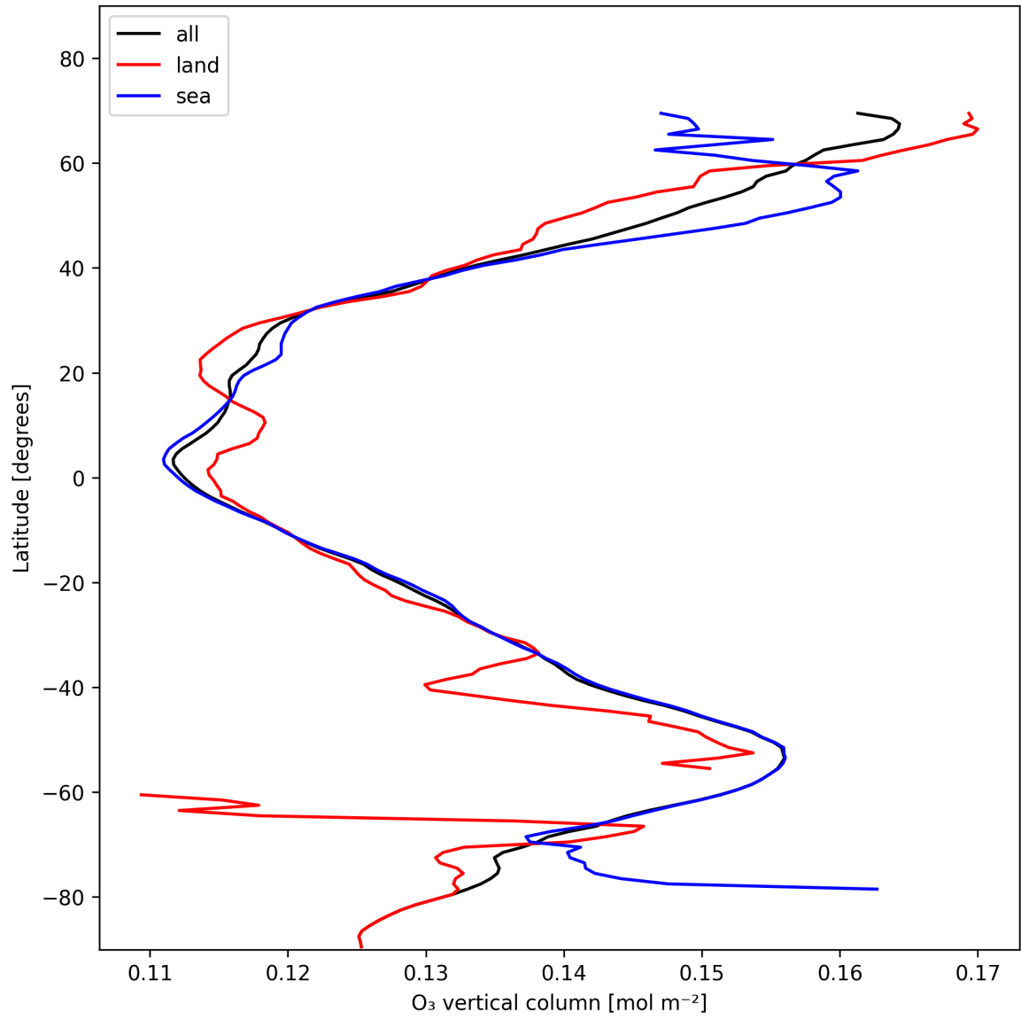
Figure 14: Zonal average of “O 3 vertical column” for 2025-11-18 to 2025-11-19.
