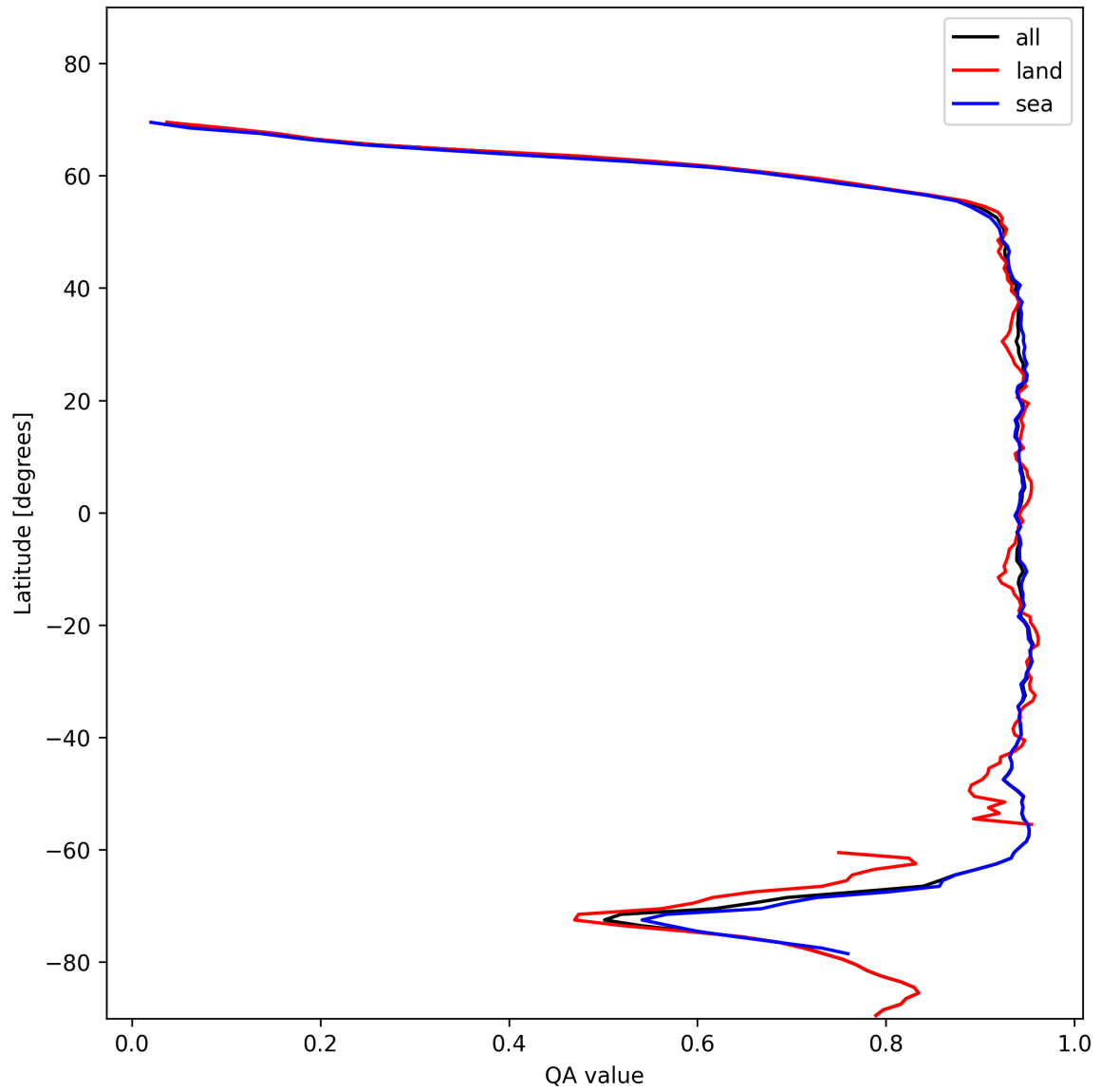
Figure 13: Zonal average of “QA value” for 2025-11-18 to 2025-11-19.
