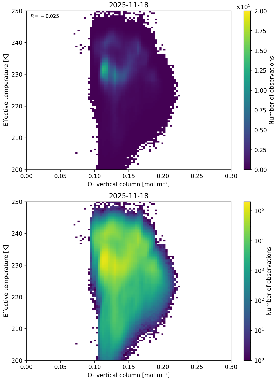
Figure 39: Scatter density plot of “O 3 vertical column” against “Effective temperature” for 2025-11-18 to 2025-11-19.
