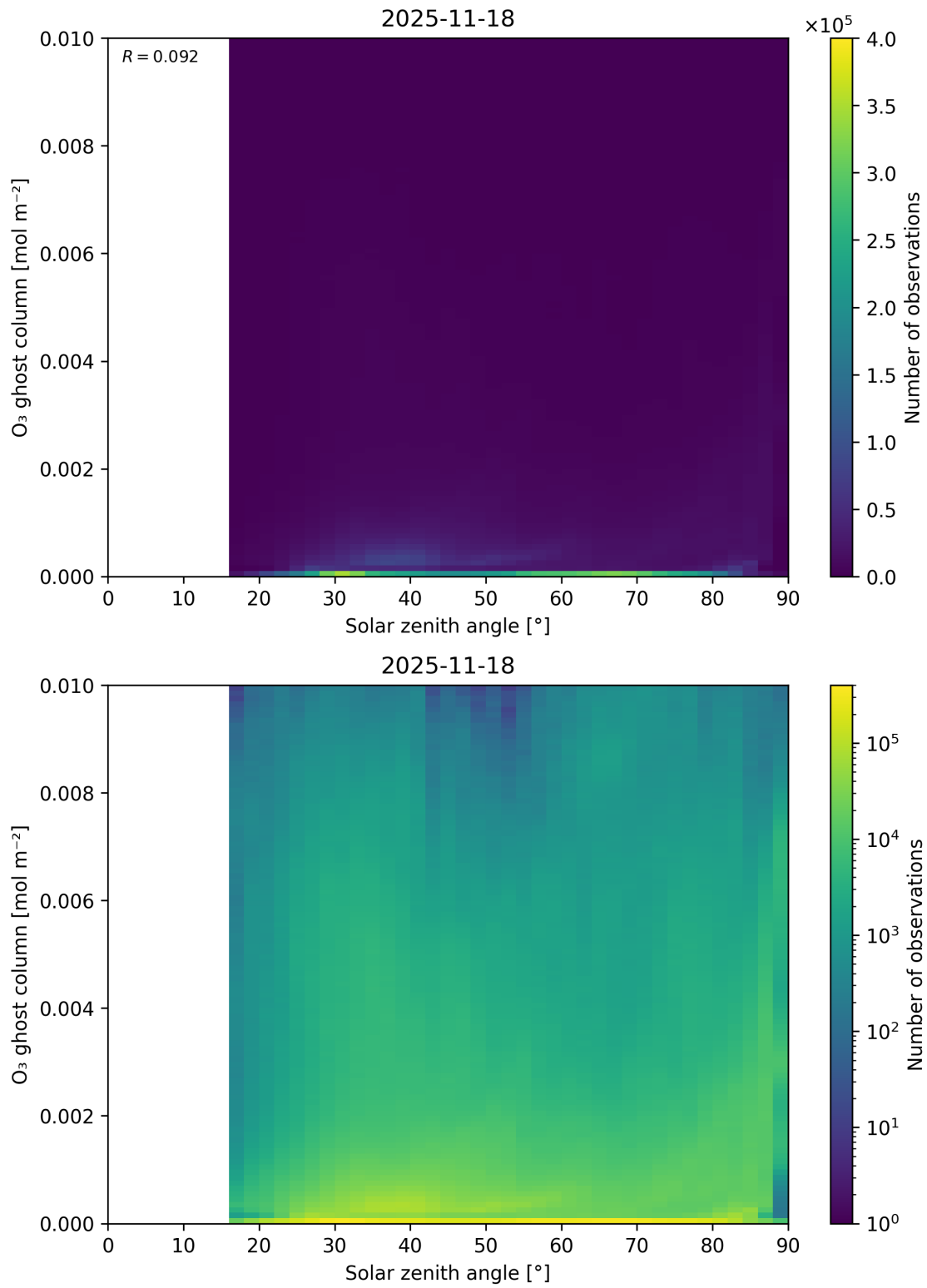
Figure 46: Scatter density plot of “Solar zenith angle” against “O 3 ghost column” for 2025-11-18 to 2025-11-19.
