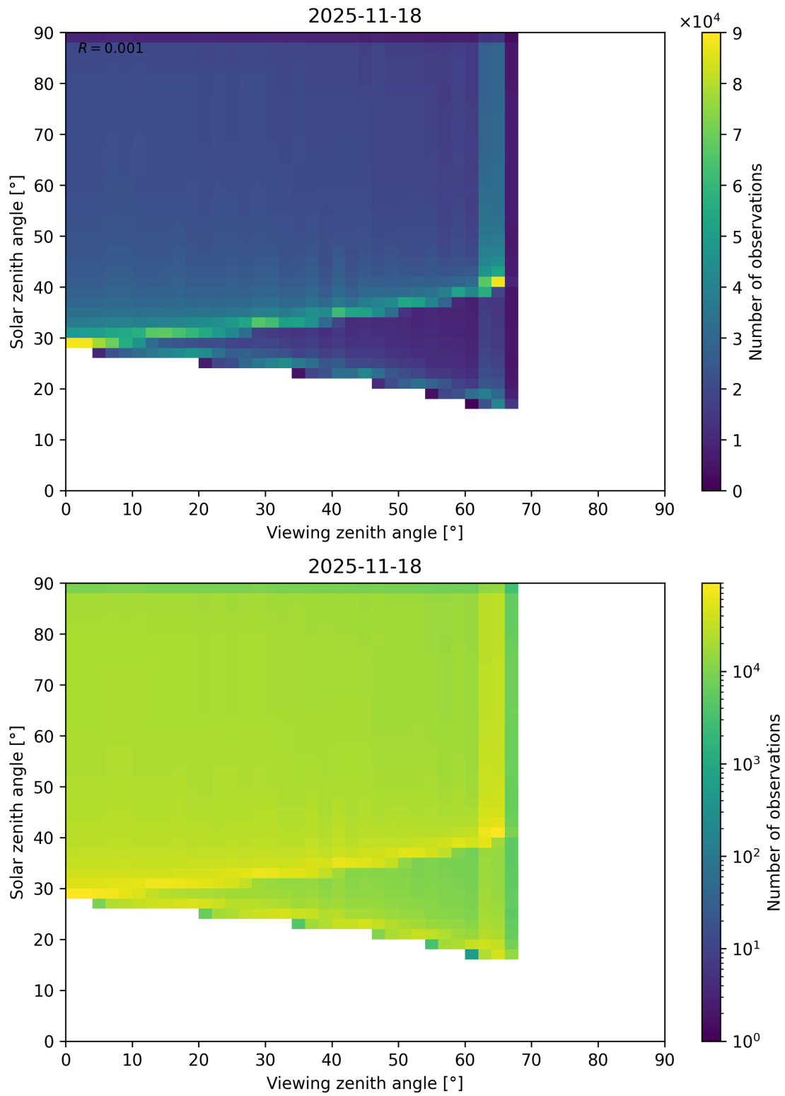
Figure 54: Scatter density plot of “Viewing zenith angle” against “Solar zenith angle” for 2025-11-18 to 2025-11-19.
