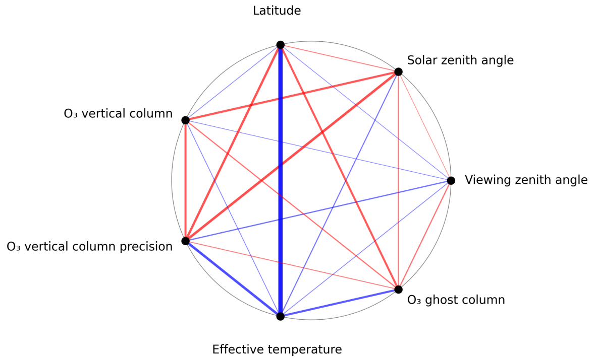
Figure 1: Map of correlation graph for 2025-11-18 to 2025-11-19.
