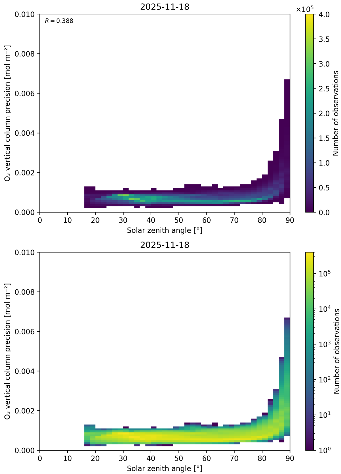
Figure 48: Scatter density plot of “Solar zenith angle” against “O 3 vertical column precision” for 2025-11-18 to 2025-11-19.
