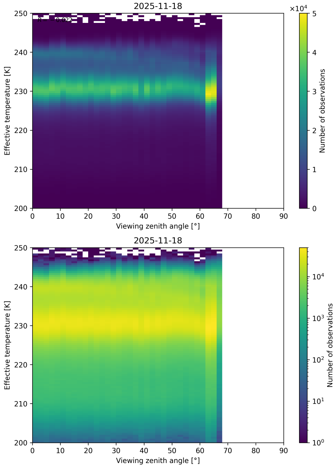
Figure 50: Scatter density plot of “Viewing zenith angle” against “Effective temperature” for 2025-11-18 to 2025-11-19.
