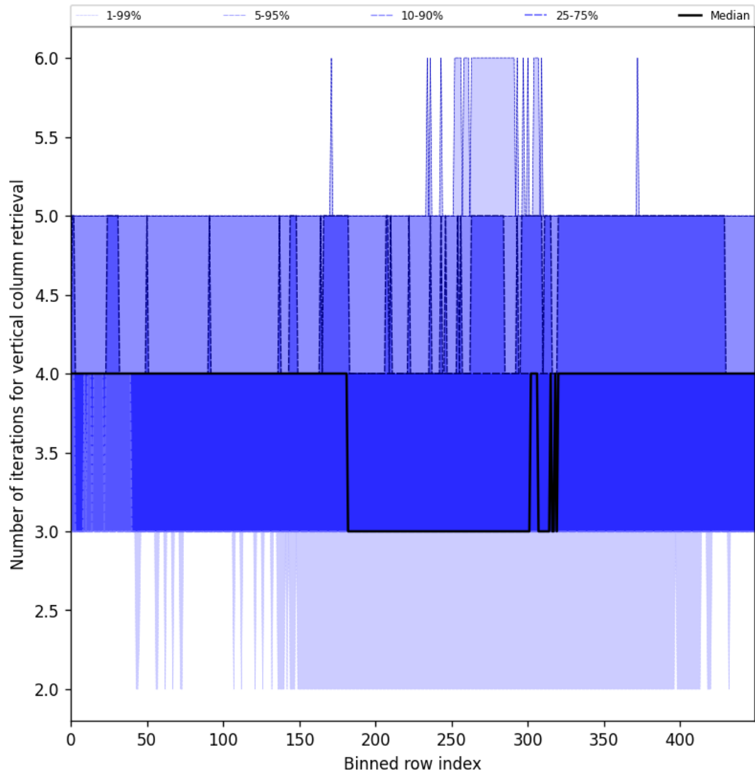
Figure 33: Along track statistics of “Number of iterations for vertical column retrieval” for 2025-11-18 to 2025-11-19
