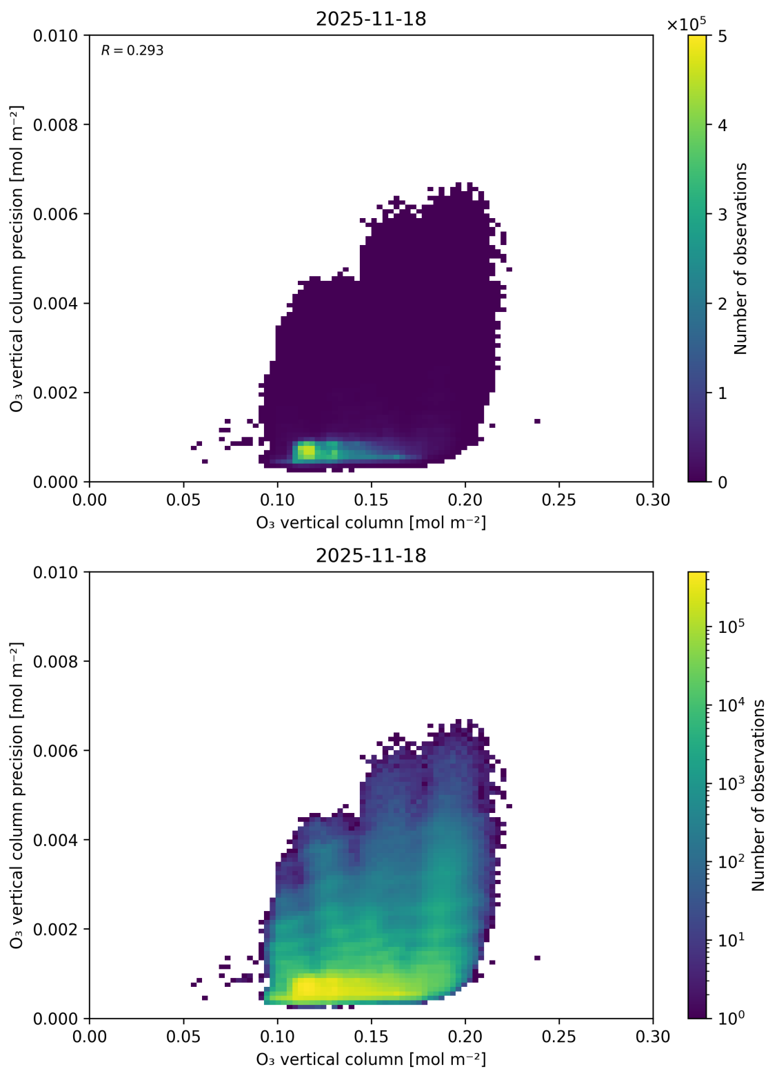
Figure 41: Scatter density plot of “O 3 vertical column” against “O 3 vertical column precision” for 2025-11-18 to 2025-11-19.
