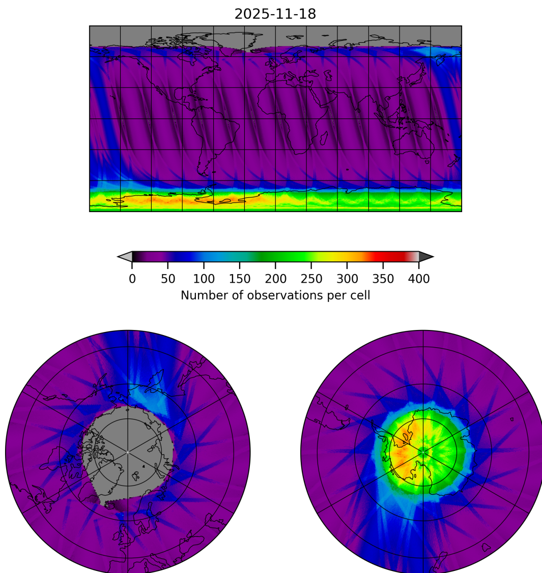
Figure 12: Map of the number of observations for 2025-11-18 to 2025-11-19
