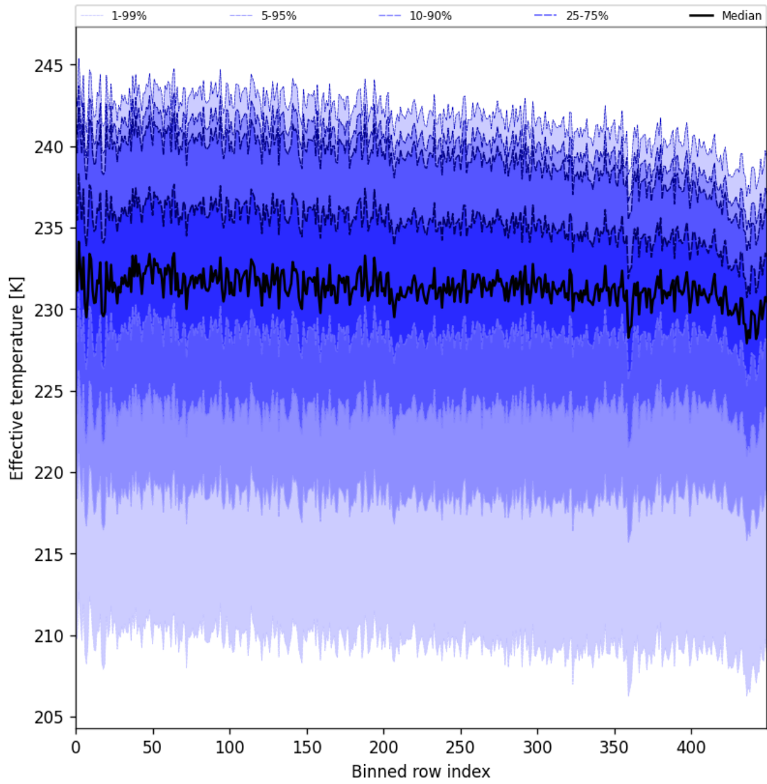
Figure 31: Along track statistics of “Effective temperature” for 2025-11-18 to 2025-11-19
