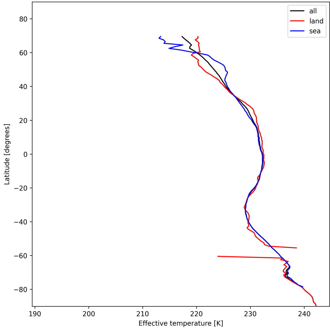
Figure 17: Zonal average of "Effective temperature" for 2025-11-18 to 2025-11-19.
