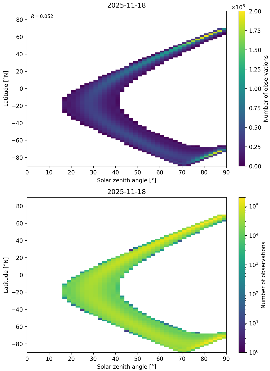
Figure 44: Scatter density plot of “Solar zenith angle” against “Latitude” for 2025-11-18 to 2025-11-19.
