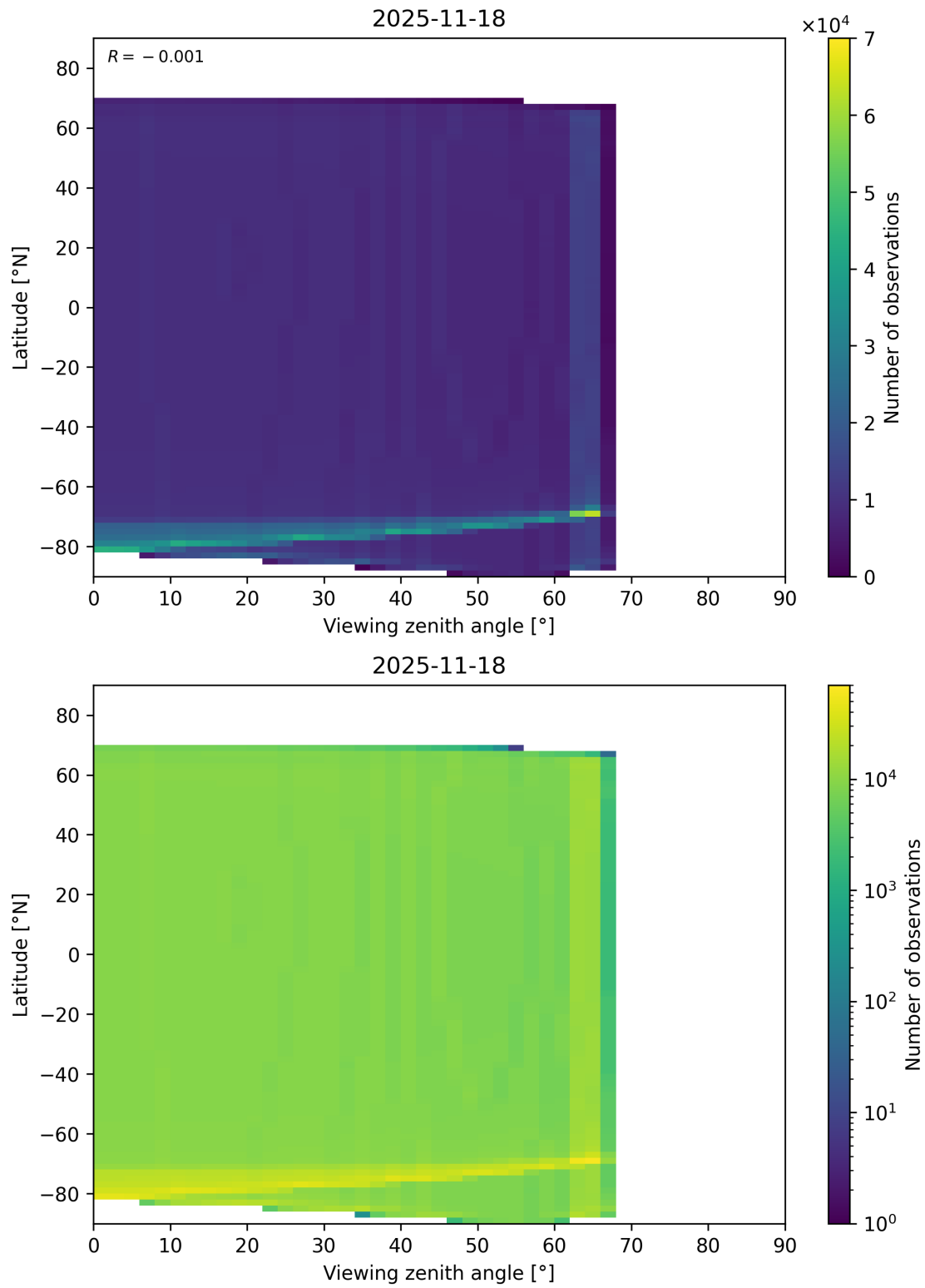
Figure 49: Scatter density plot of “Viewing zenith angle” against “Latitude” for 2025-11-18 to 2025-11-19.
