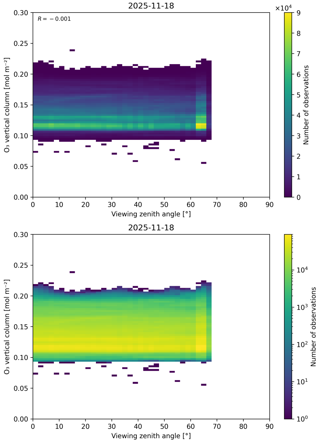
Figure 52: Scatter density plot of “Viewing zenith angle” against “O 3 vertical column” for 2025-11-18 to 2025-11-19.
