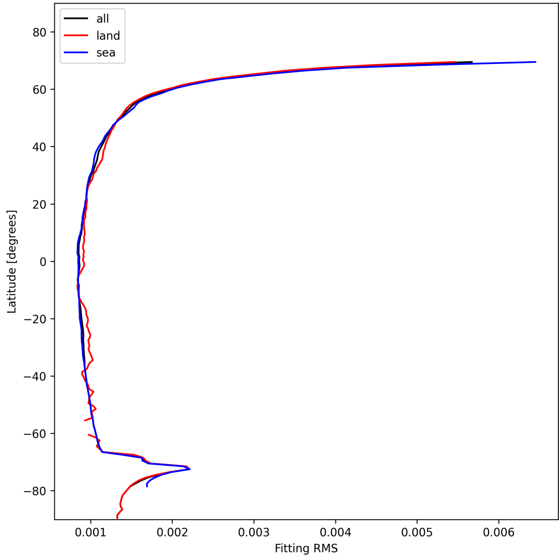
Figure 16: Zonal average of “Fitting RMS” for 2025-11-18 to 2025-11-19.
