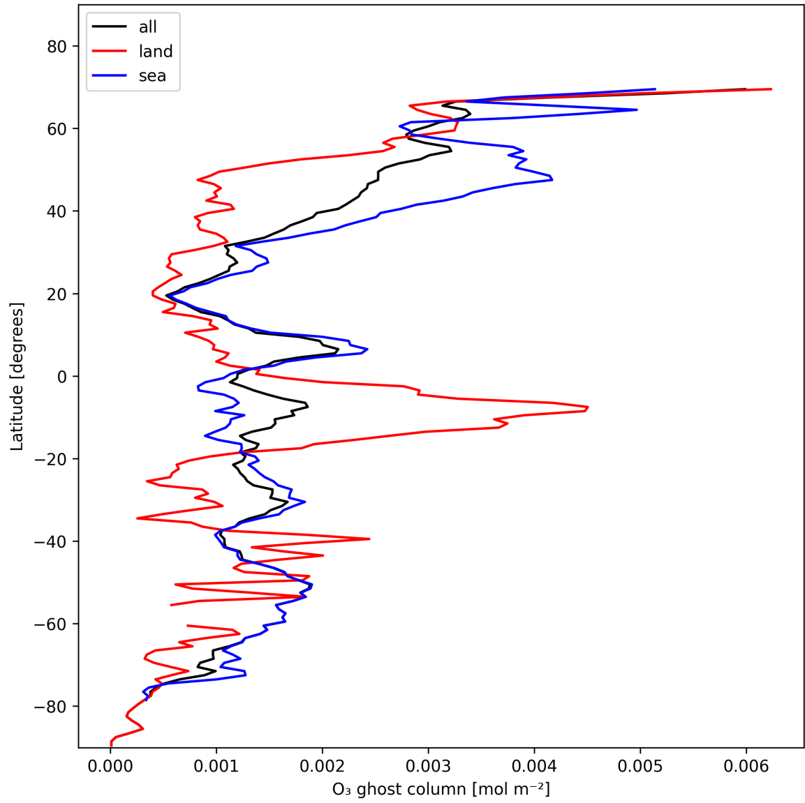
Figure 18: Zonal average of “O 3 ghost column” for 2025-11-18 to 2025-11-19.
