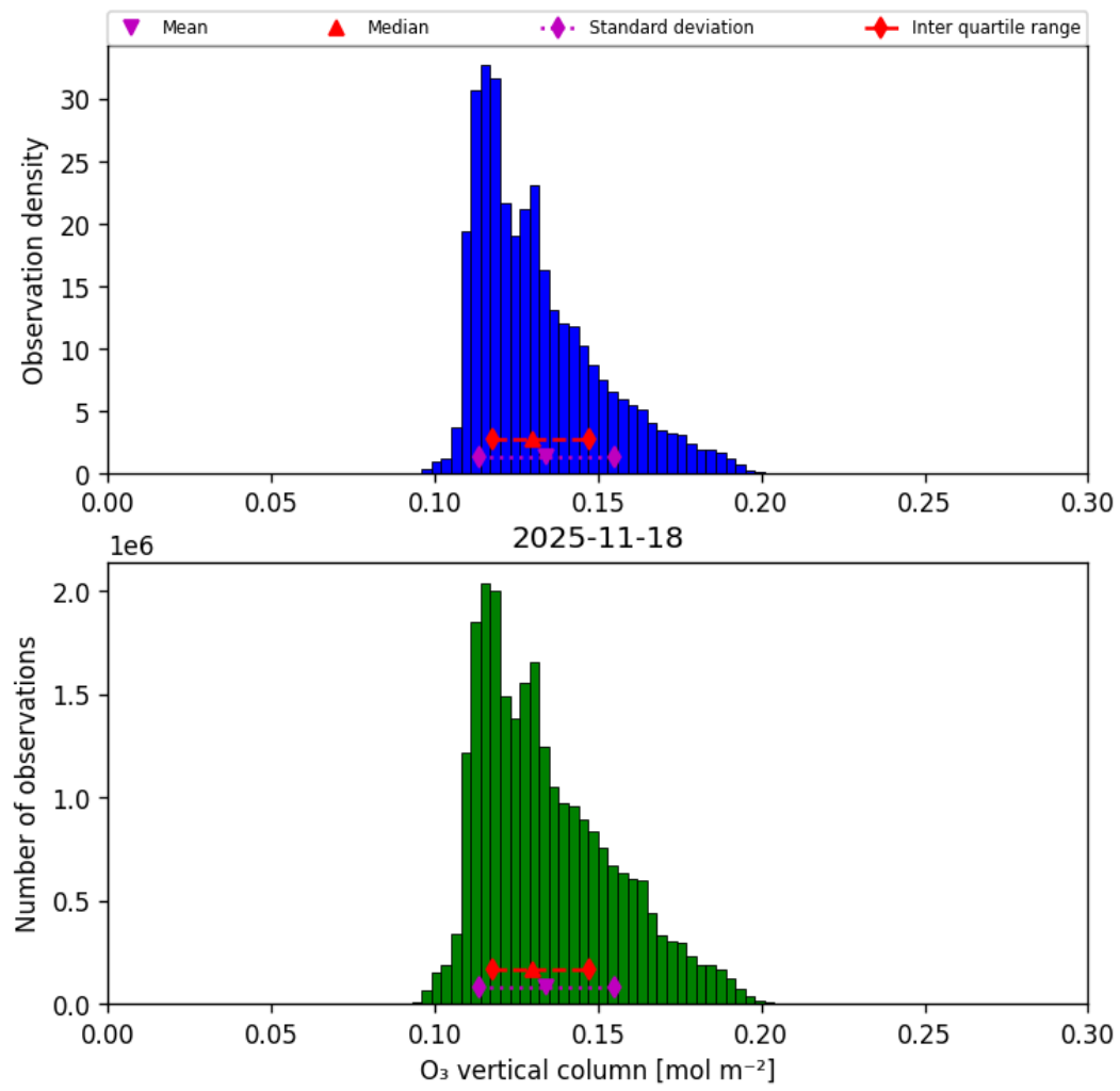
Figure 21: Histogram of “O 3 vertical column” for 2025-11-18 to 2025-11-19
