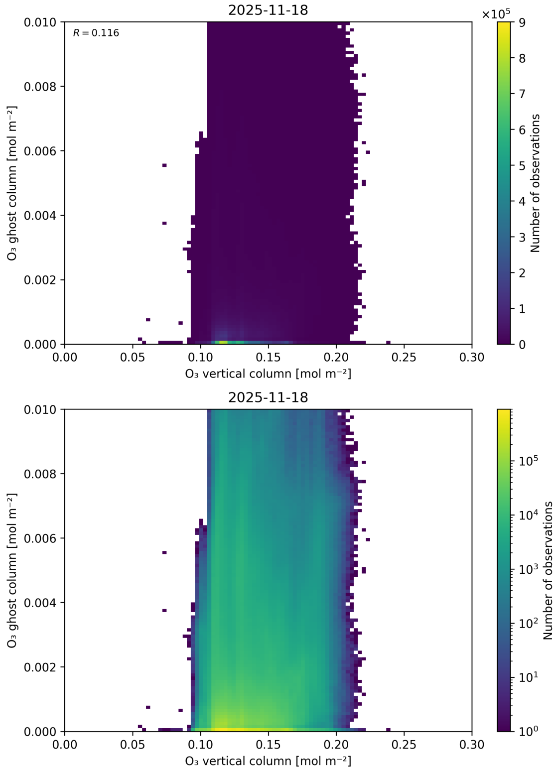
Figure 40: Scatter density plot of “O 3 vertical column” against “O 3 ghost column” for 2025-11-18 to 2025-11-19.
