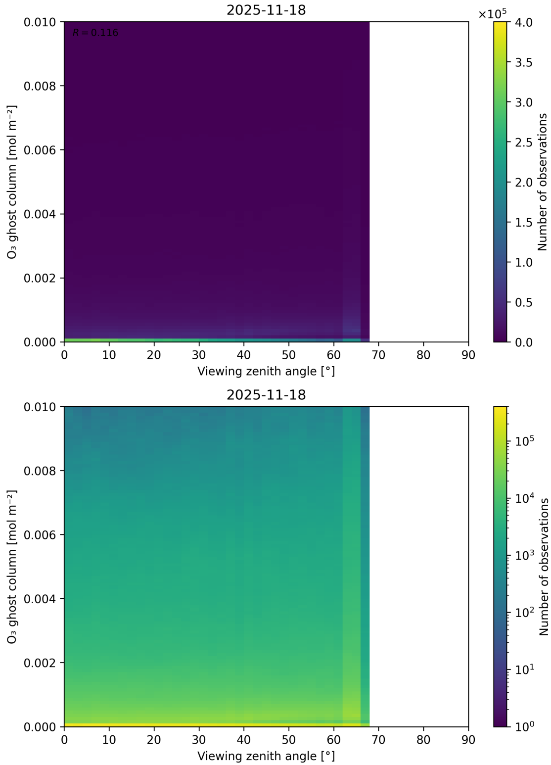
Figure 51: Scatter density plot of “Viewing zenith angle” against “O 3 ghost column” for 2025-11-18 to 2025-11-19.
