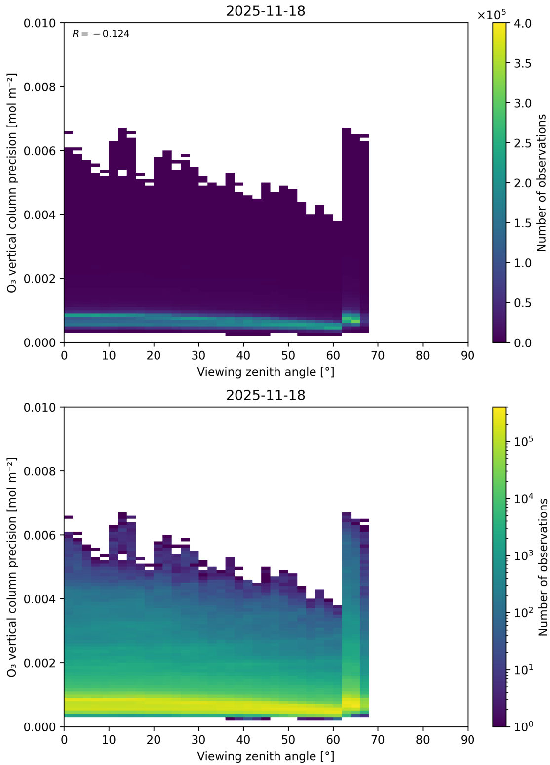
Figure 53: Scatter density plot of “Viewing zenith angle” against “O 3 vertical column precision” for 2025-11-18 to 2025-11-19.
