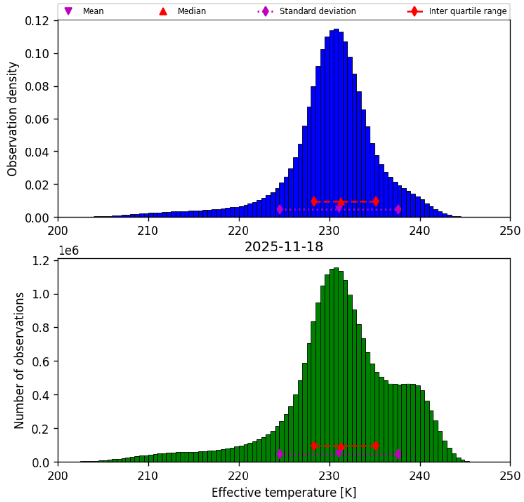
Figure 24: Histogram of “Effective temperature” for 2025-11-18 to 2025-11-19
