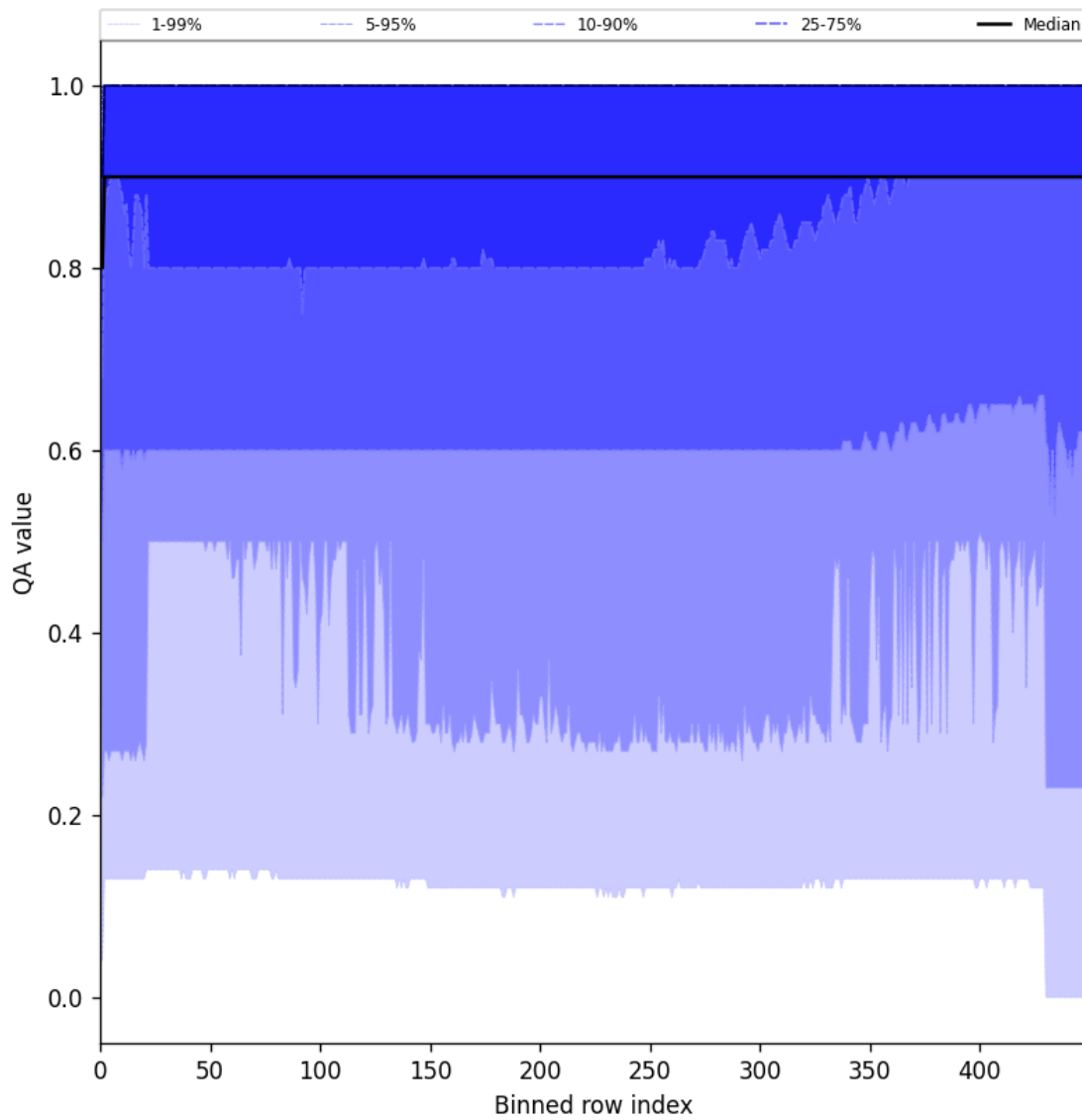
Figure 27: Along track statistics of “QA value” for 2025-11-18 to 2025-11-19
