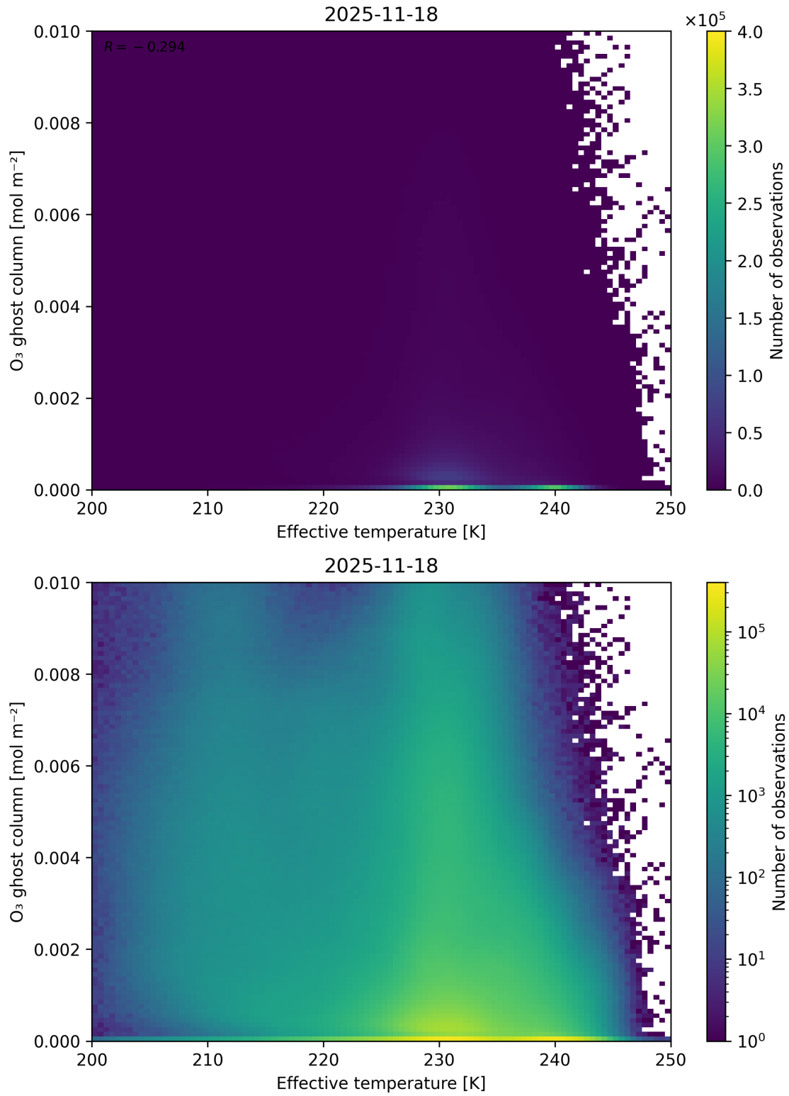
Figure 38: Scatter density plot of “Effective temperature” against “O 3 ghost column” for 2025-11-18 to 2025-11-19.
