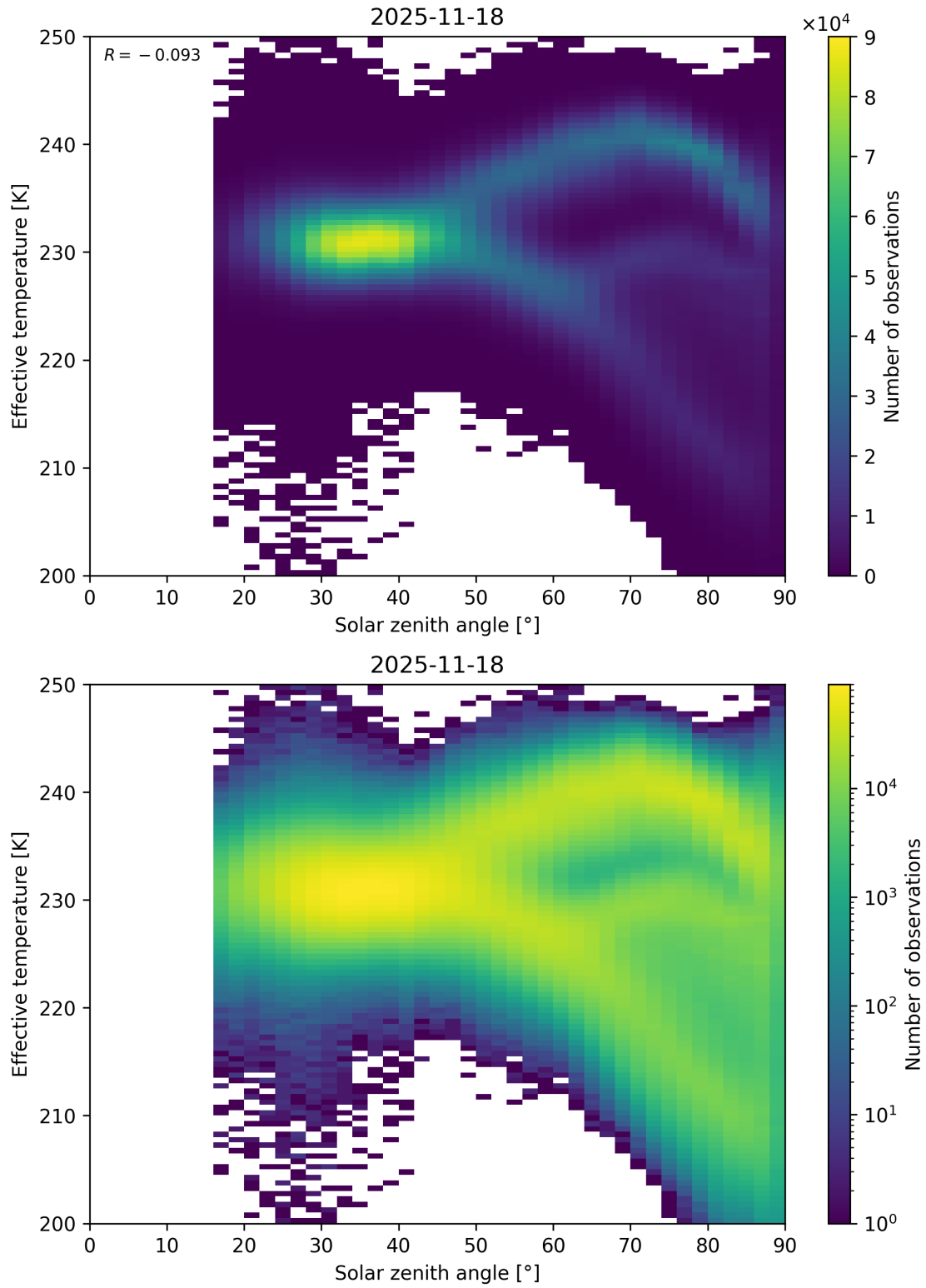
Figure 45: Scatter density plot of “Solar zenith angle” against “Effective temperature” for 2025-11-18 to 2025-11-19.
