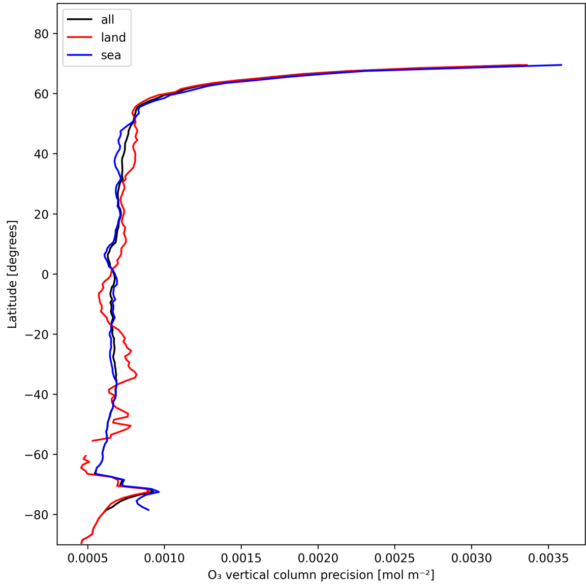
Figure 15: Zonal average of “O 3 vertical column precision” for 2025-11-18 to 2025-11-19.
