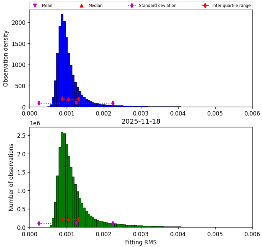
Figure 23: Histogram of “Fitting RMS” for 2025-11-18 to 2025-11-19
