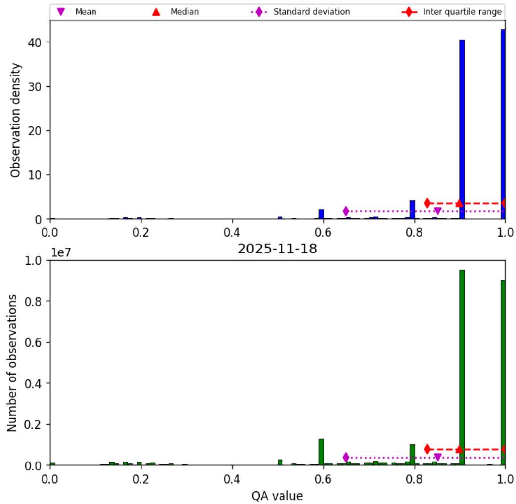
Figure 20: Histogram of “QA value” for 2025-11-18 to 2025-11-19
