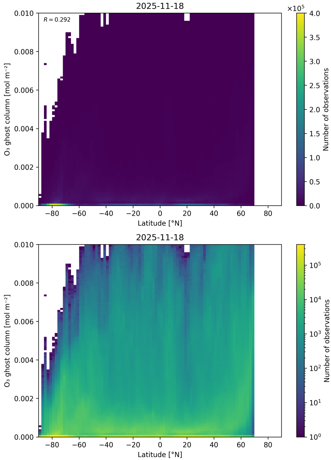
Figure 35: Scatter density plot of “Latitude” against “O 3 ghost column” for 2025-11-18 to 2025-11-19.
