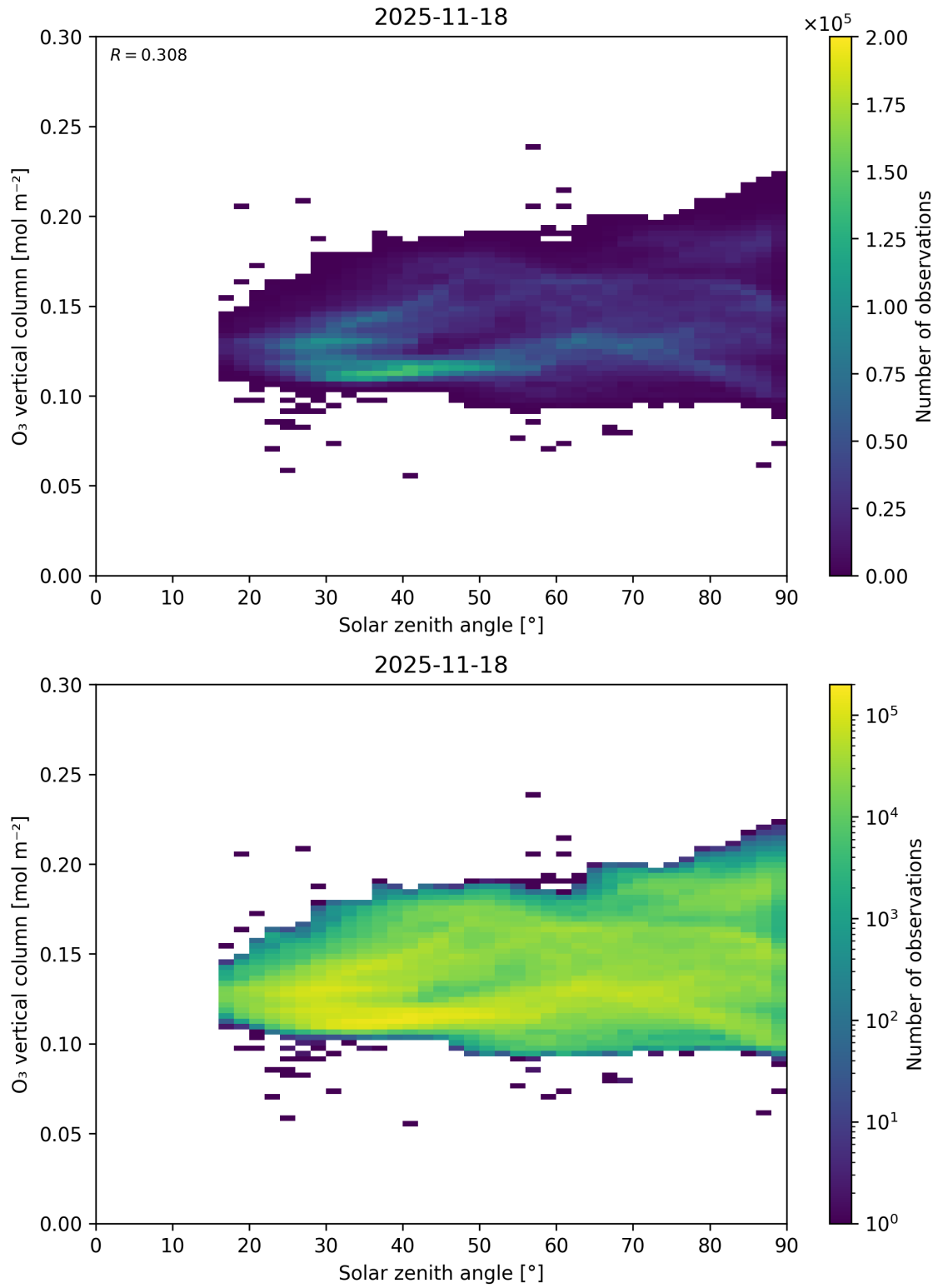
Figure 47: Scatter density plot of “Solar zenith angle” against “O 3 vertical column” for 2025-11-18 to 2025-11-19.
