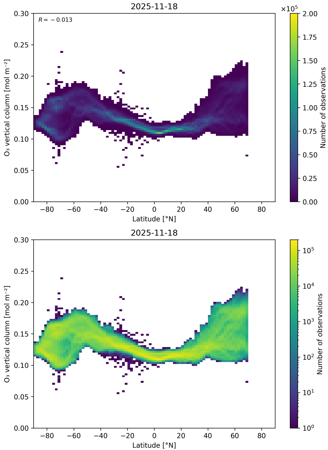
Figure 36: Scatter density plot of “Latitude” against “O 3 vertical column” for 2025-11-18 to 2025-11-19.
