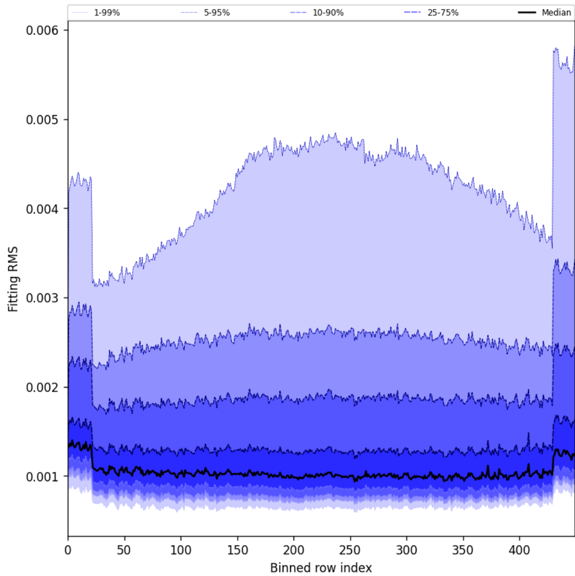
Figure 30: Along track statistics of “Fitting RMS” for 2025-11-18 to 2025-11-19
