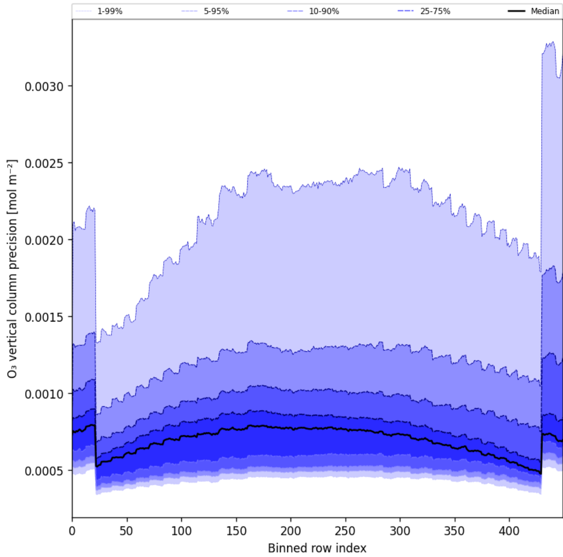
Figure 29: Along track statistics of “O 3 vertical column precision” for 2025-11-18 to 2025-11-19
