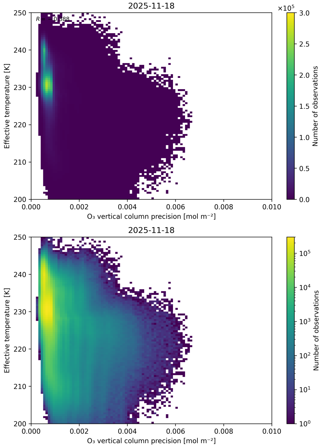
Figure 42: Scatter density plot of “O 3 vertical column precision” against “Effective temperature” for 2025-11-18 to 2025-11-19.
