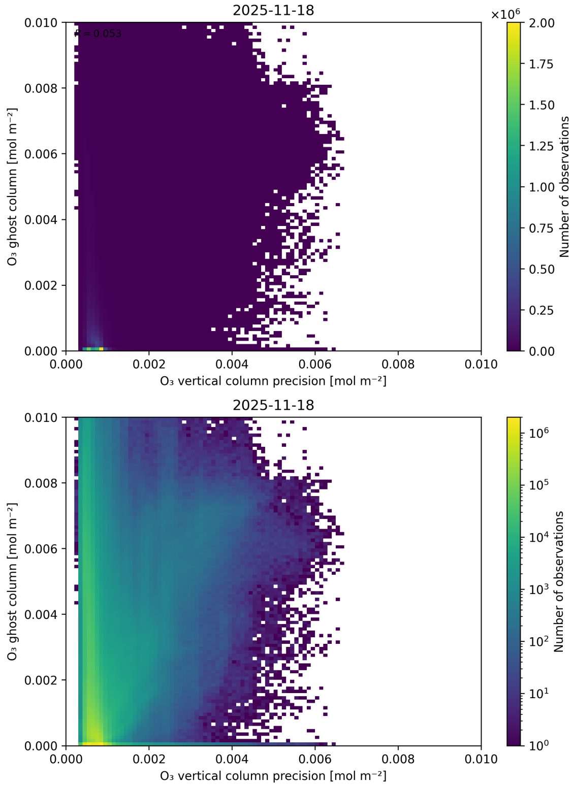
Figure 43: Scatter density plot of “O 3 vertical column precision” against “O 3 ghost column” for 2025-11-18 to 2025-11-19.
