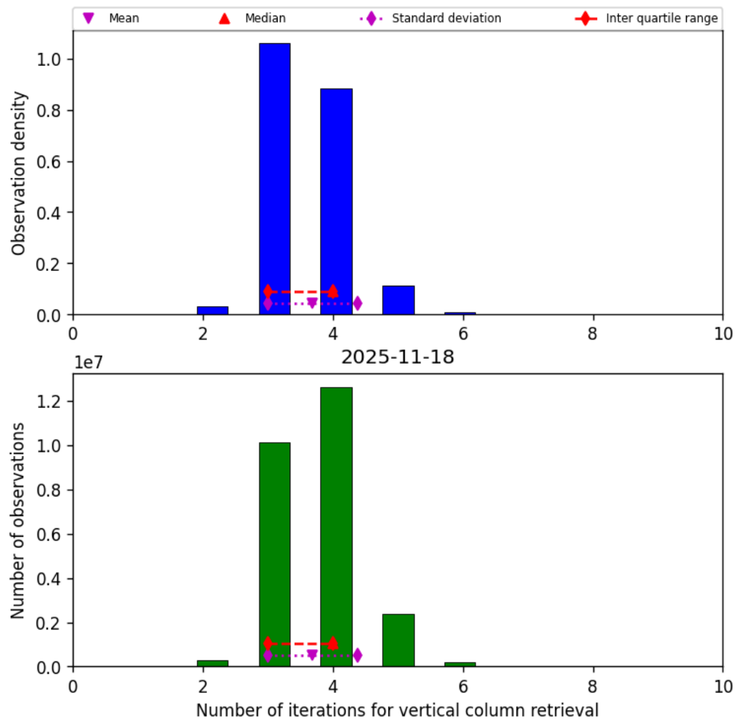
Figure 26: Histogram of “Number of iterations for vertical column retrieval” for 2025-11-18 to 2025-11-19
