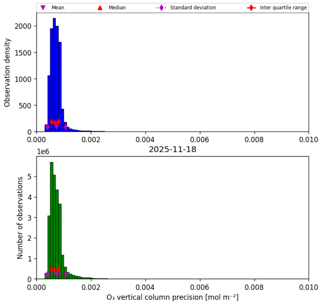
Figure 22: Histogram of “O 3 vertical column precision” for 2025-11-18 to 2025-11-19
