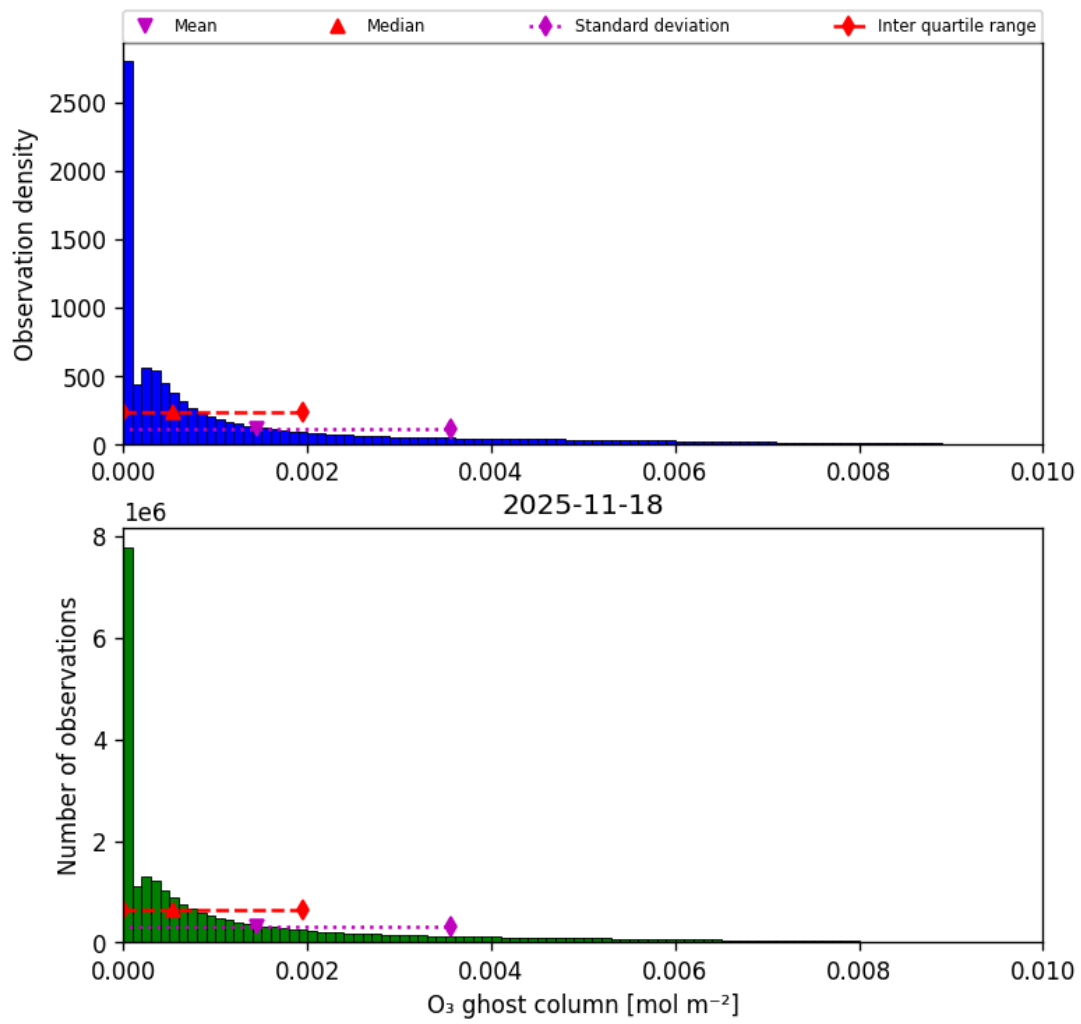
Figure 25: Histogram of “O 3 ghost column” for 2025-11-18 to 2025-11-19
