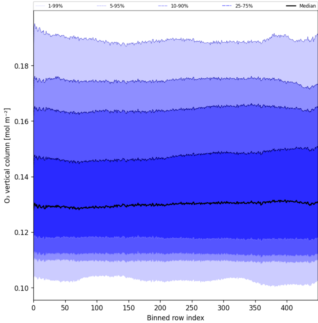
Figure 28: Along track statistics of “O 3 vertical column” for 2025-11-18 to 2025-11-19
