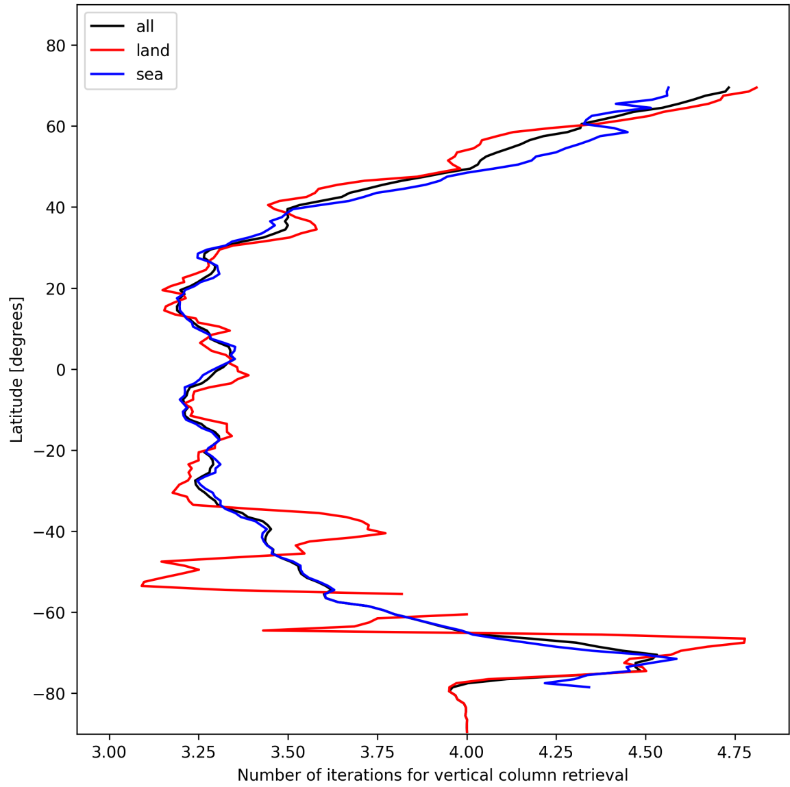
Figure 19: Zonal average of “Number of iterations for vertical column retrieval” for 2025-11-18 to 2025-11-19.
