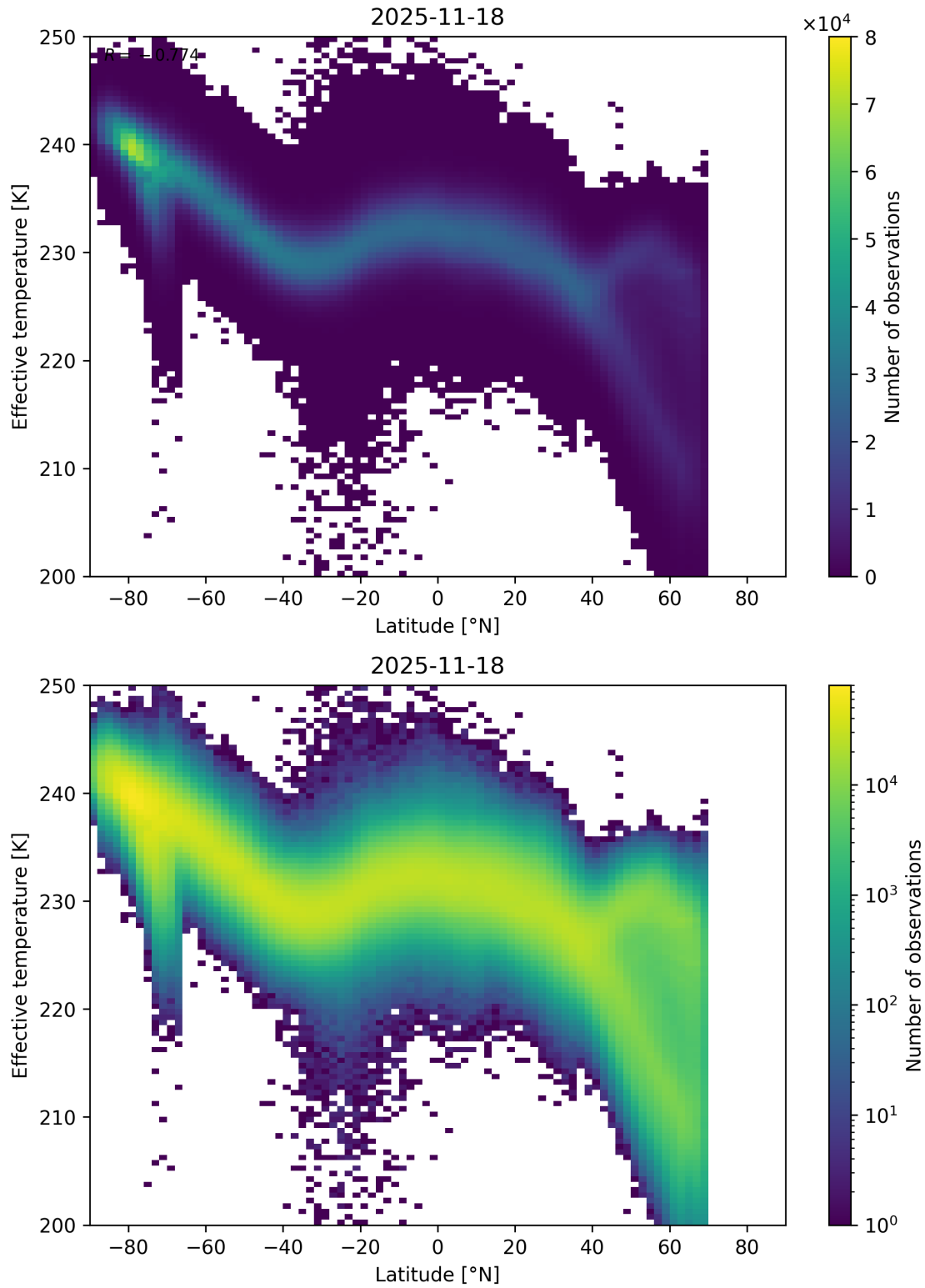
Figure 34: Scatter density plot of “Latitude” against “Effective temperature” for 2025-11-18 to 2025-11-19.
