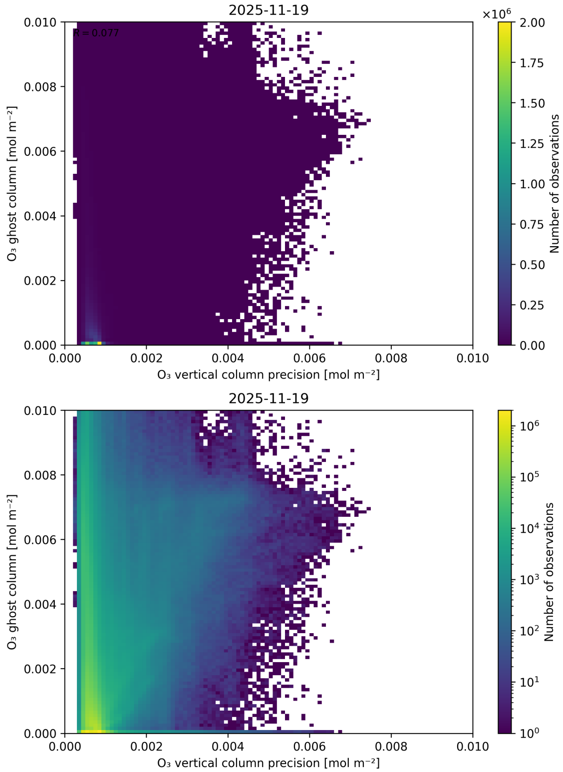
Figure 43: Scatter density plot of “ O_3 vertical column precision” against “ O_3 ghost column” for 2025-11-18 to 2025-11-20.
