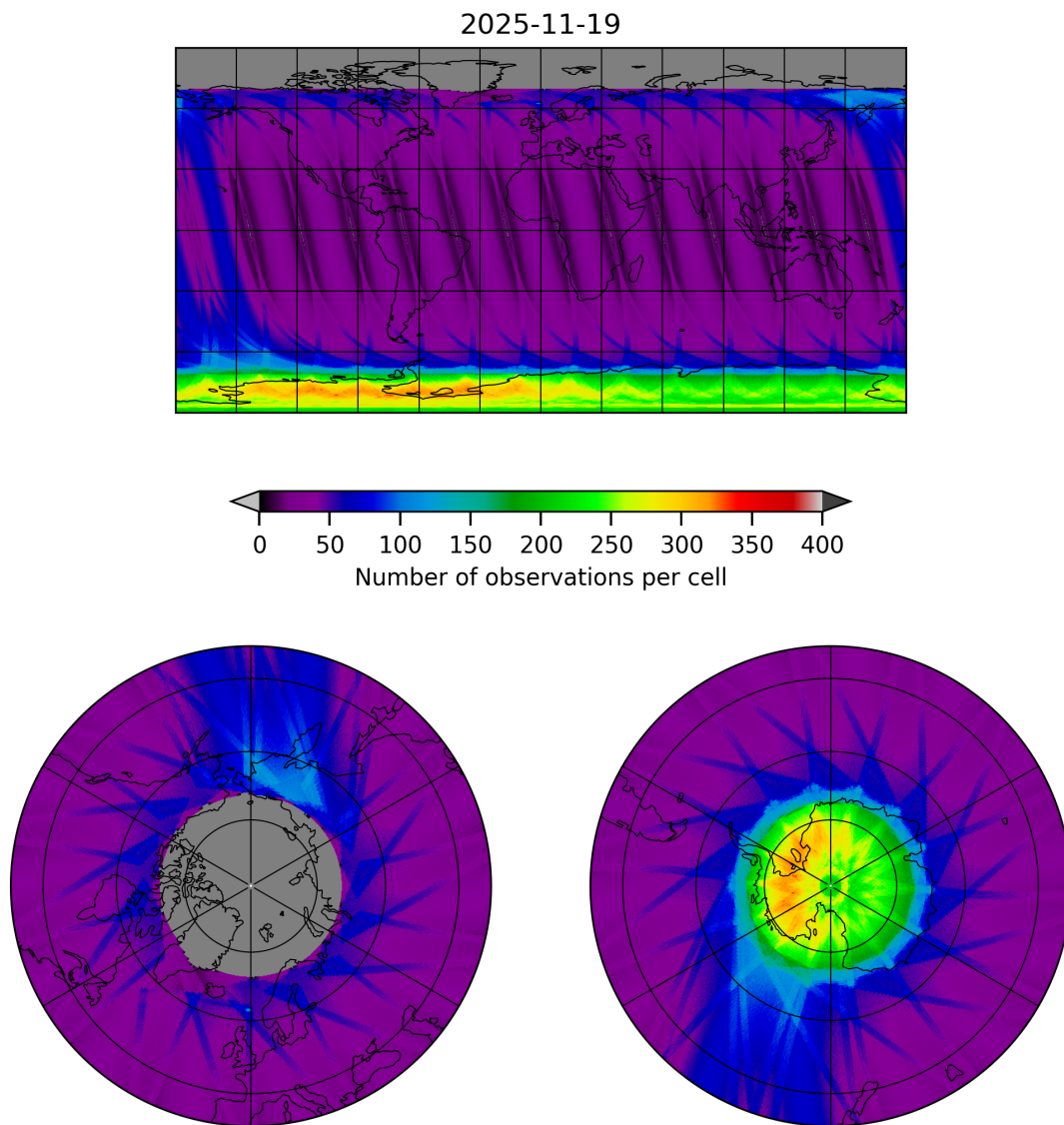
Figure 12: Map of the number of observations for 2025-11-18 to 2025-11-20
