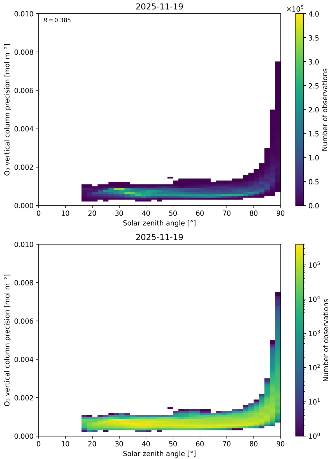
Figure 48: Scatter density plot of “Solar zenith angle” against “O 3 vertical column precision” for 2025-11-18 to 2025-11-20.
