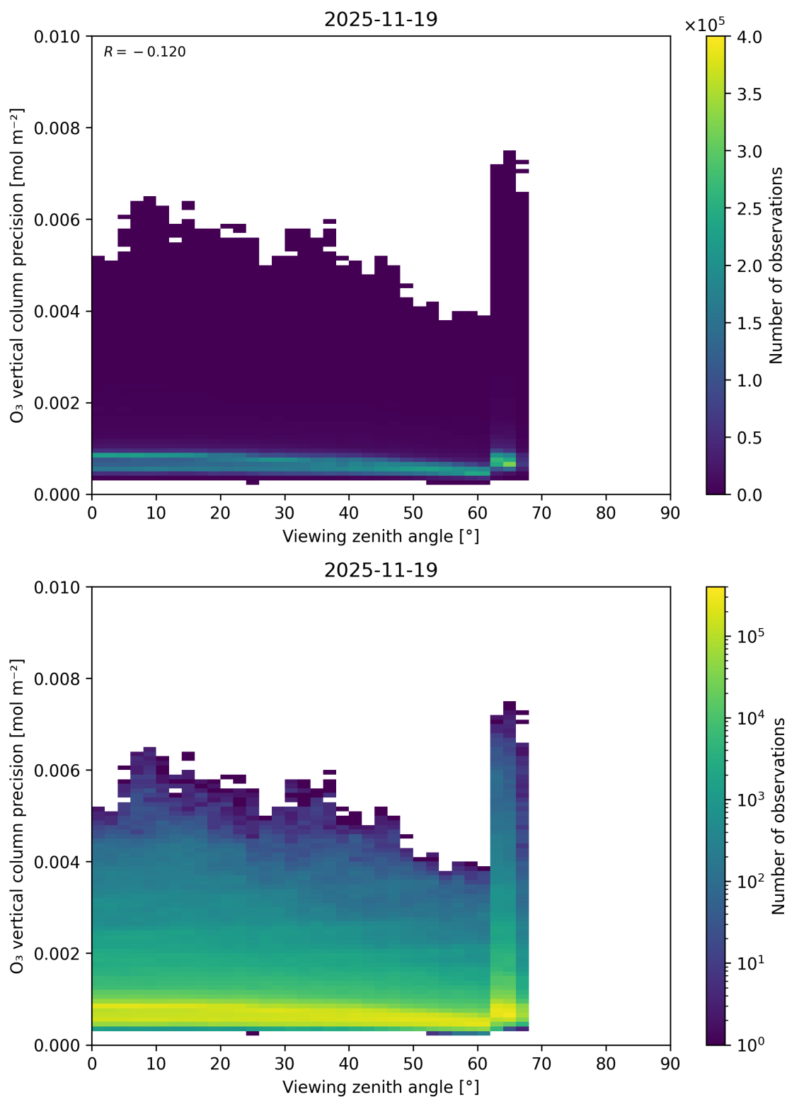
Figure 53: Scatter density plot of “Viewing zenith angle” against “O 3 vertical column precision” for 2025-11-18 to 2025-11-20.
