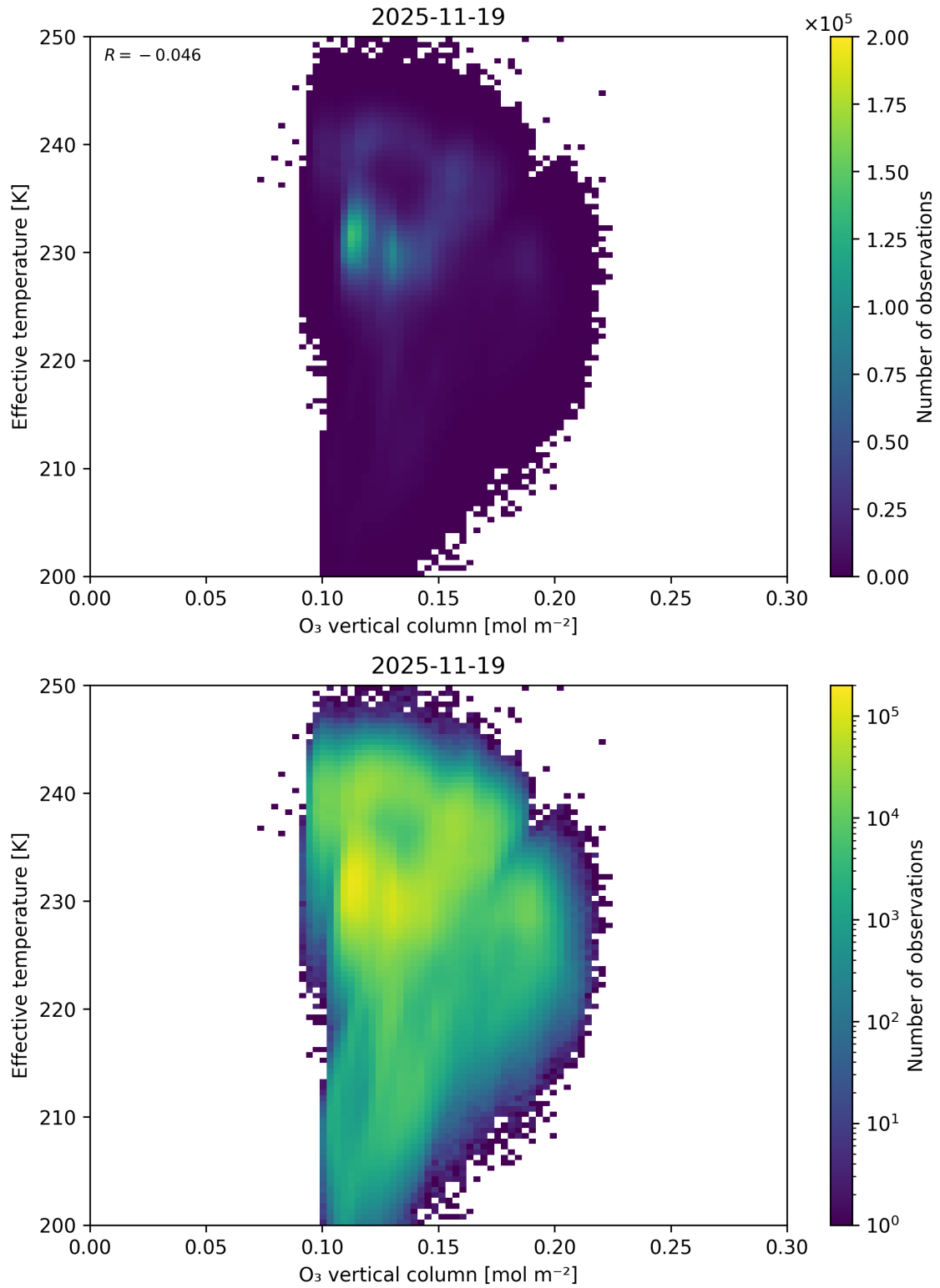
Figure 39: Scatter density plot of “O 3 vertical column” against “Effective temperature” for 2025-11-18 to 2025-11-20.
