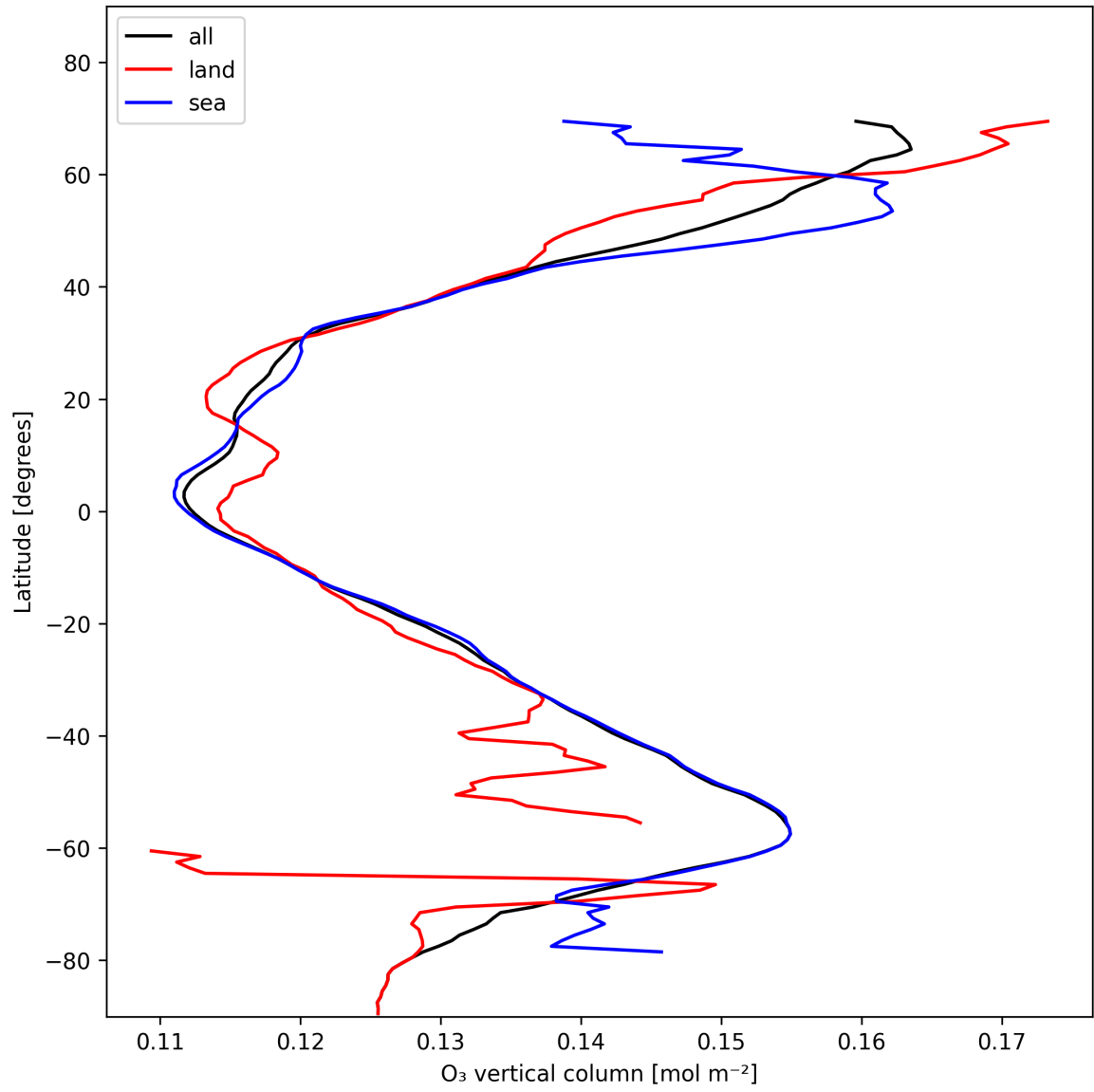
Figure 14: Zonal average of “O 3 vertical column” for 2025-11-18 to 2025-11-20.
