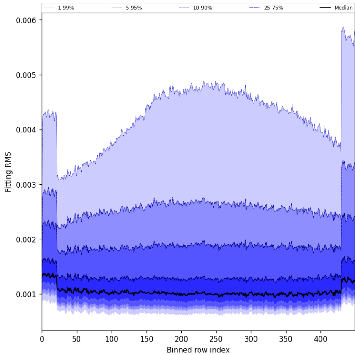
Figure 30: Along track statistics of “Fitting RMS” for 2025-11-18 to 2025-11-20
