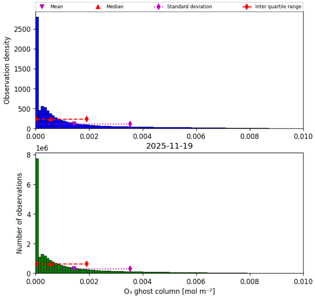
Figure 25: Histogram of “O 3 ghost column” for 2025-11-18 to 2025-11-20
