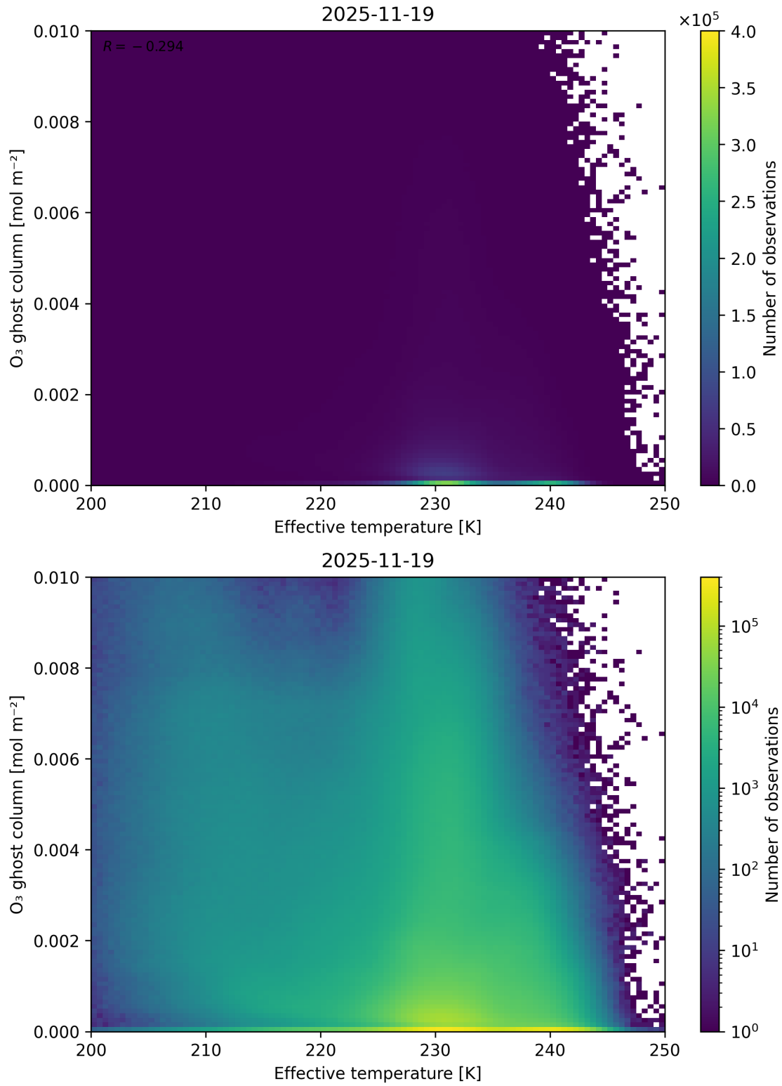
Figure 38: Scatter density plot of “Effective temperature” against “O 3 ghost column” for 2025-11-18 to 2025-11-20.
