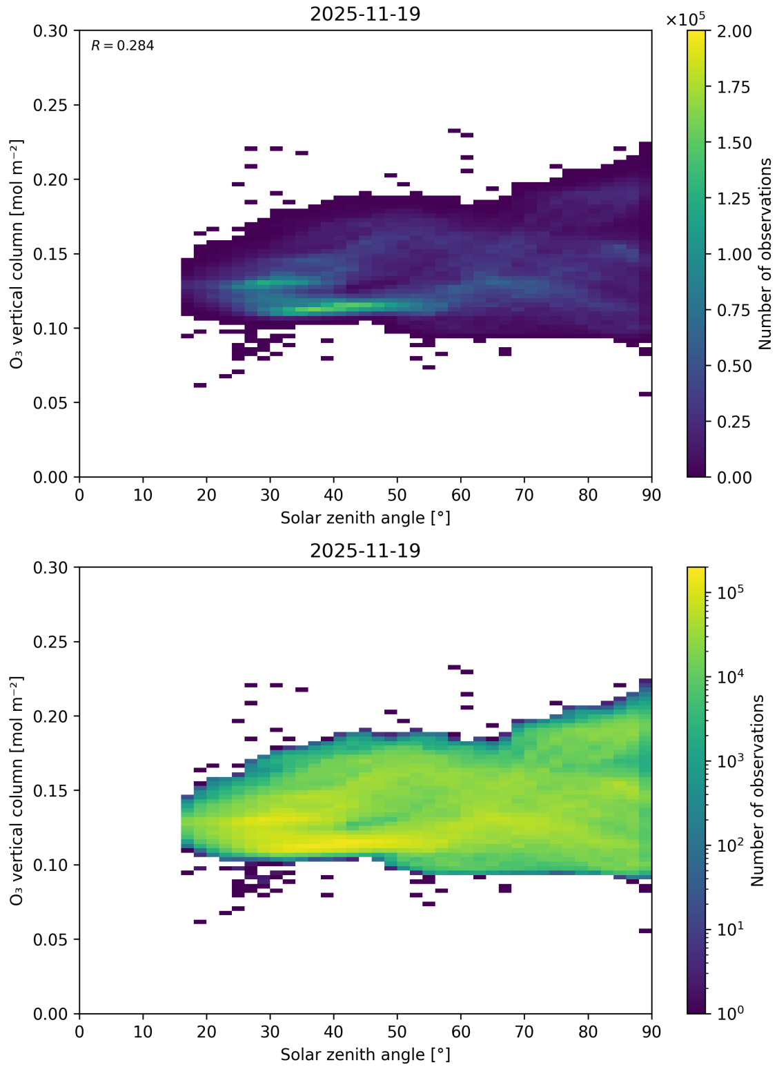
Figure 47: Scatter density plot of “Solar zenith angle” against “O 3 vertical column” for 2025-11-18 to 2025-11-20.
