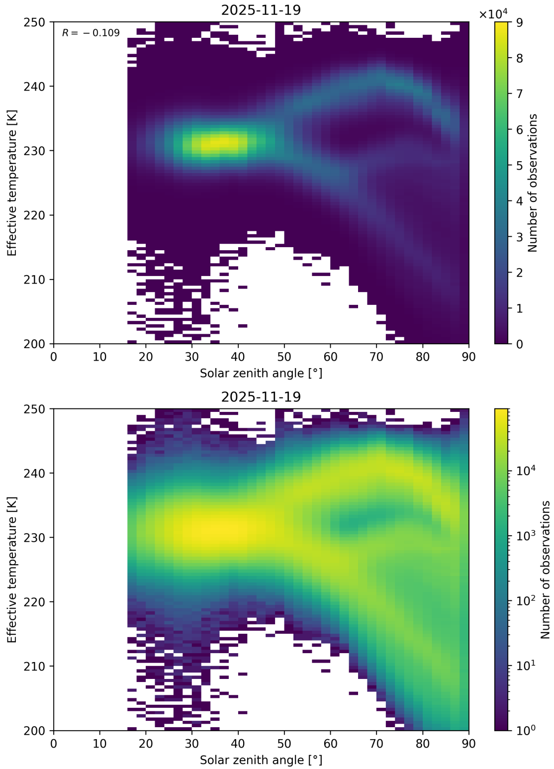
Figure 45: Scatter density plot of “Solar zenith angle” against “Effective temperature” for 2025-11-18 to 2025-11-20.
