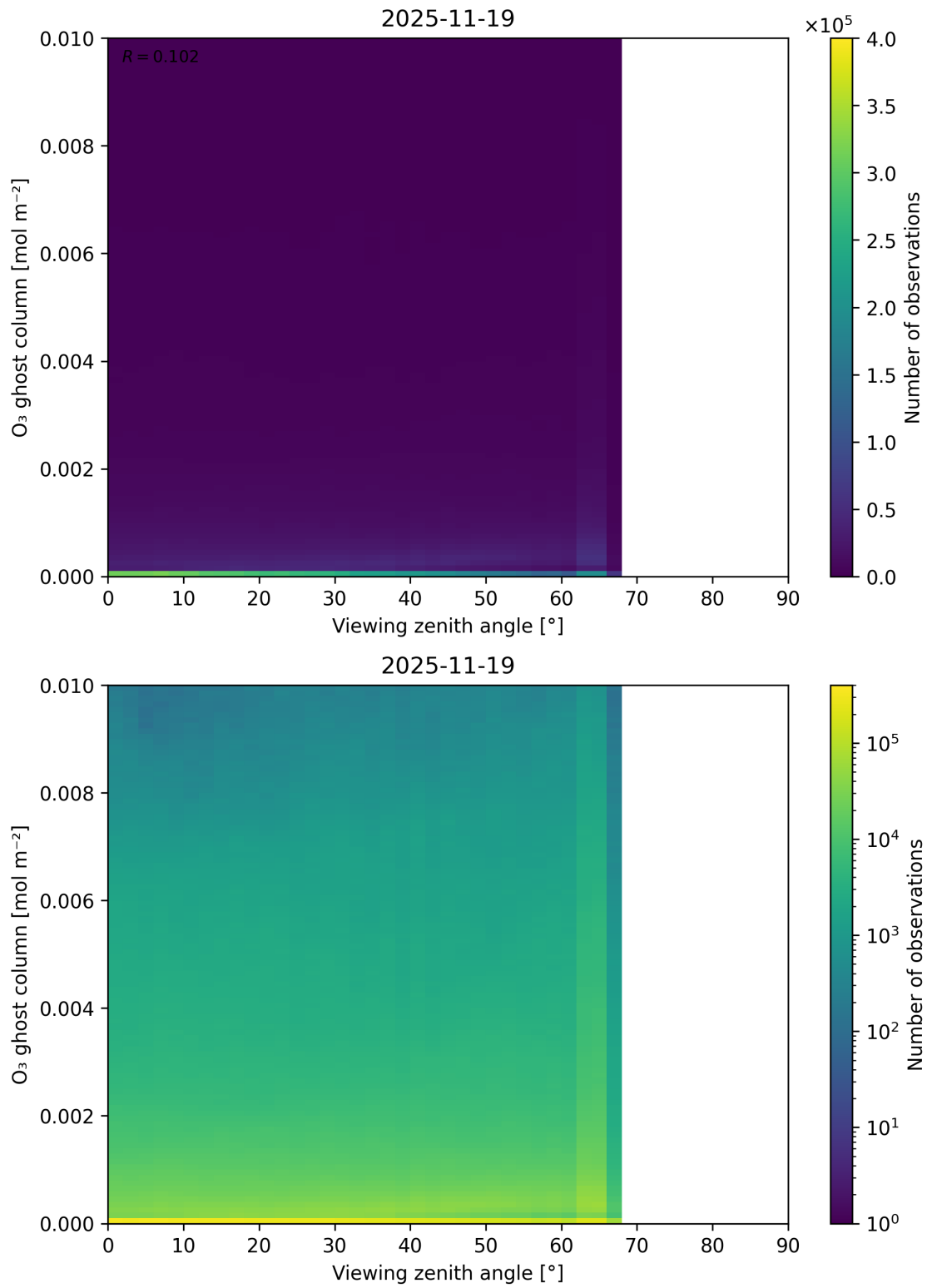
Figure 51: Scatter density plot of “Viewing zenith angle” against “O 3 ghost column” for 2025-11-18 to 2025-11-20.
