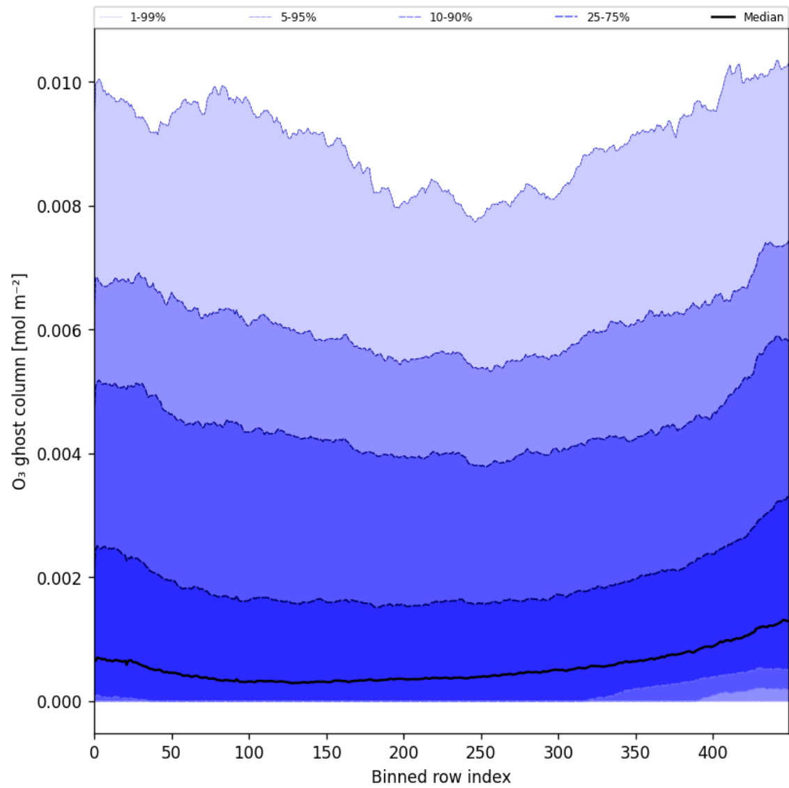
Figure 32: Along track statistics of “O 3 ghost column” for 2025-11-18 to 2025-11-20
