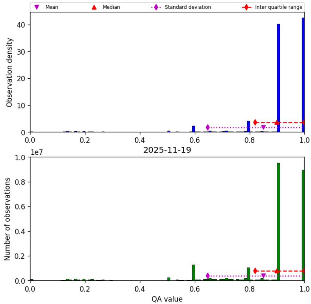
Figure 20: Histogram of “QA value” for 2025-11-18 to 2025-11-20
