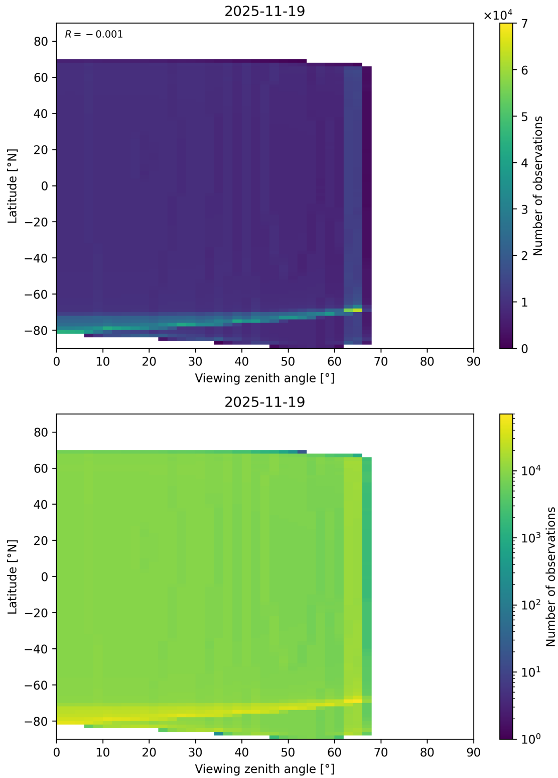
Figure 49: Scatter density plot of “Viewing zenith angle” against “Latitude” for 2025-11-18 to 2025-11-20.
