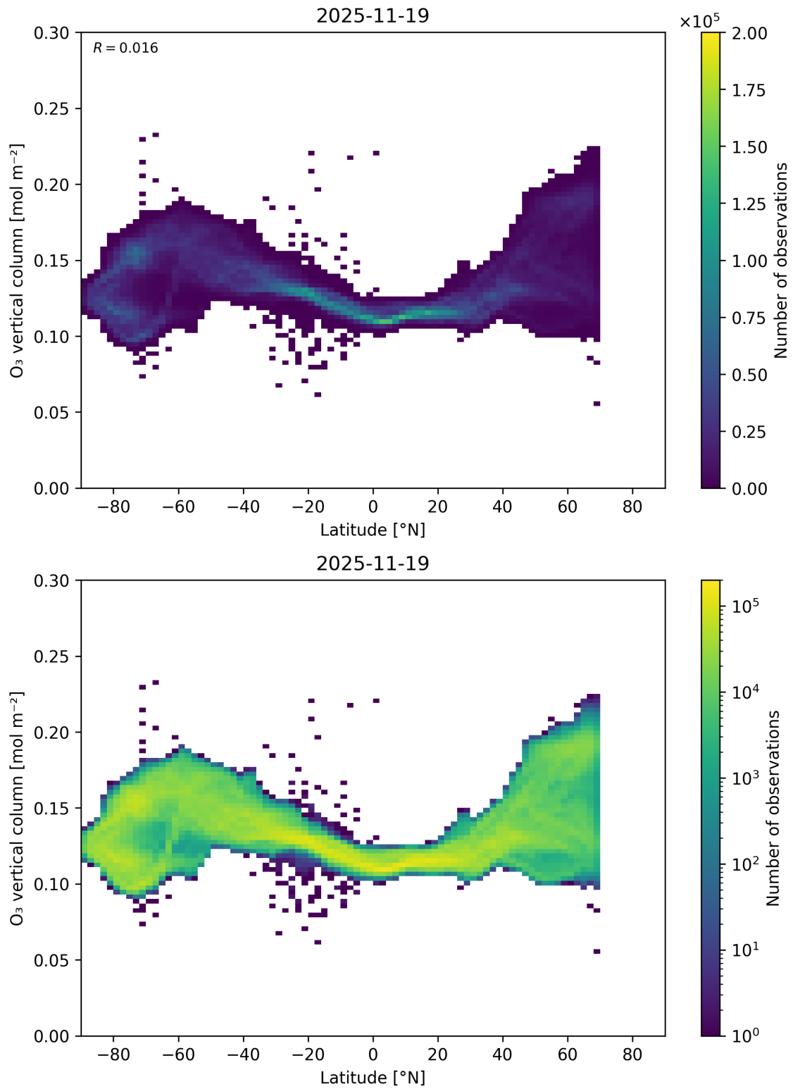
Figure 36: Scatter density plot of “Latitude” against “O 3 vertical column” for 2025-11-18 to 2025-11-20.
