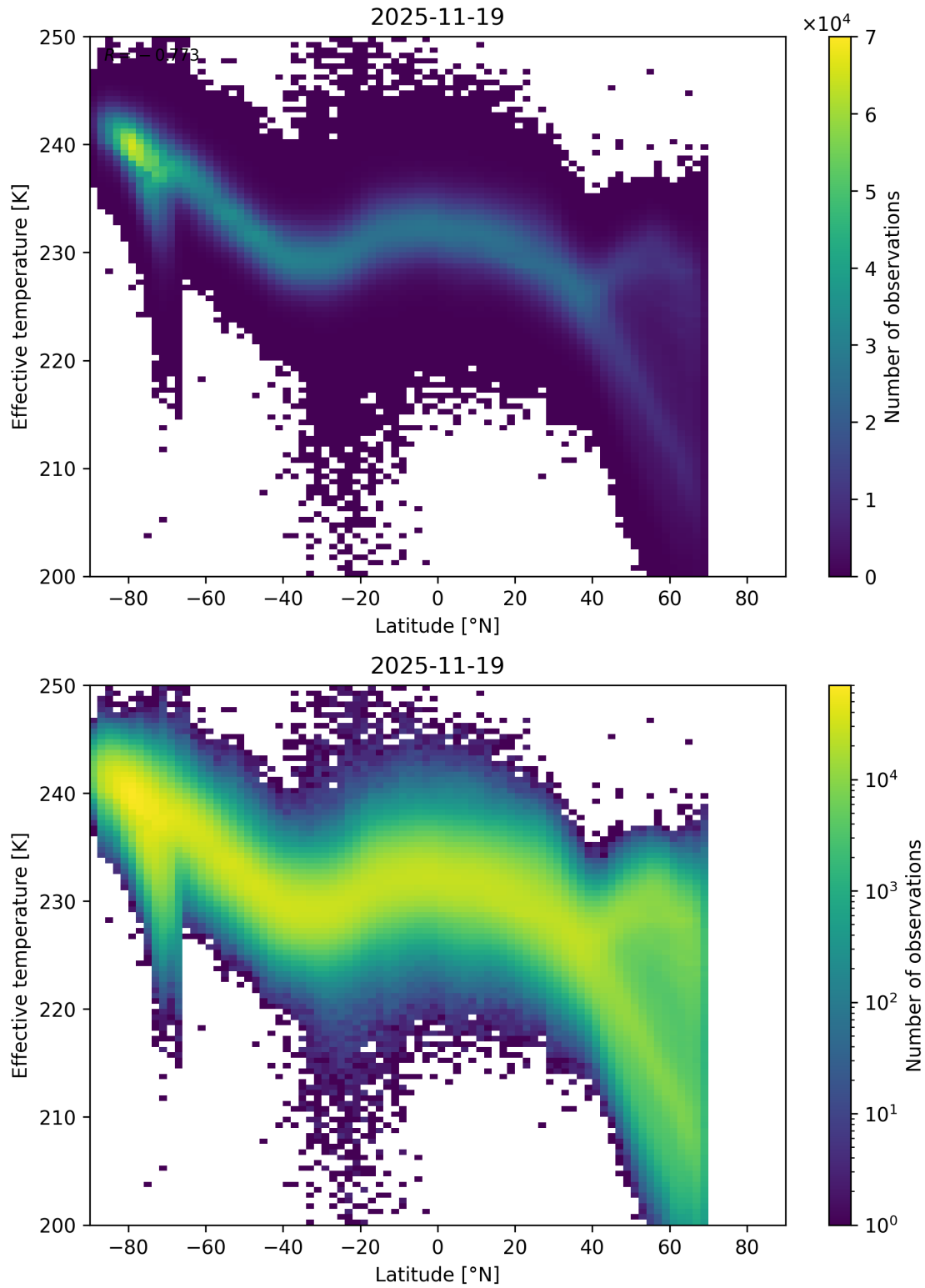
Figure 34: Scatter density plot of “Latitude” against “Effective temperature” for 2025-11-18 to 2025-11-20.
