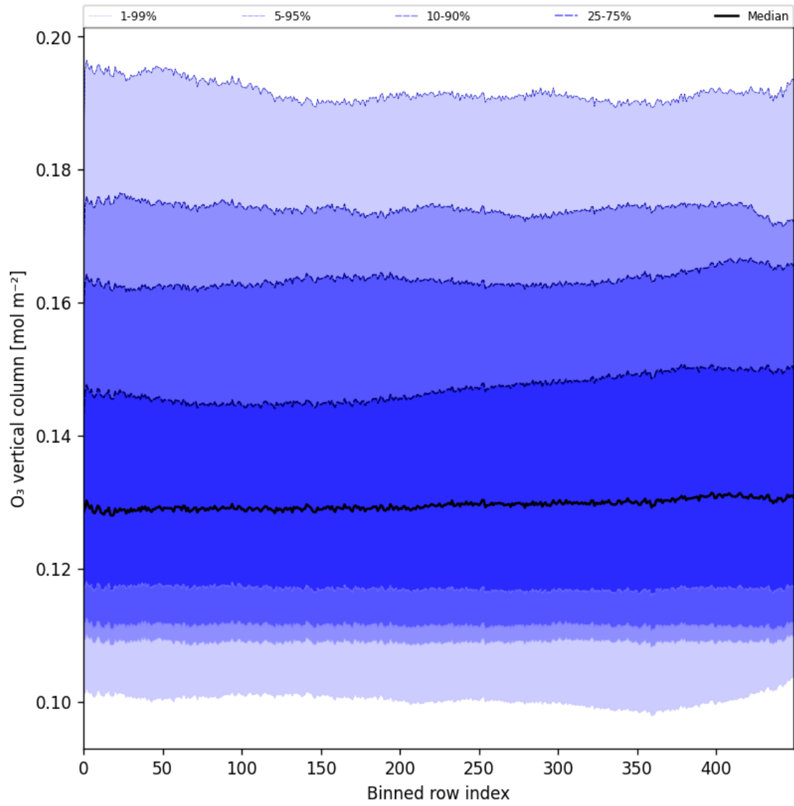
Figure 28: Along track statistics of “O 3 vertical column” for 2025-11-18 to 2025-11-20
