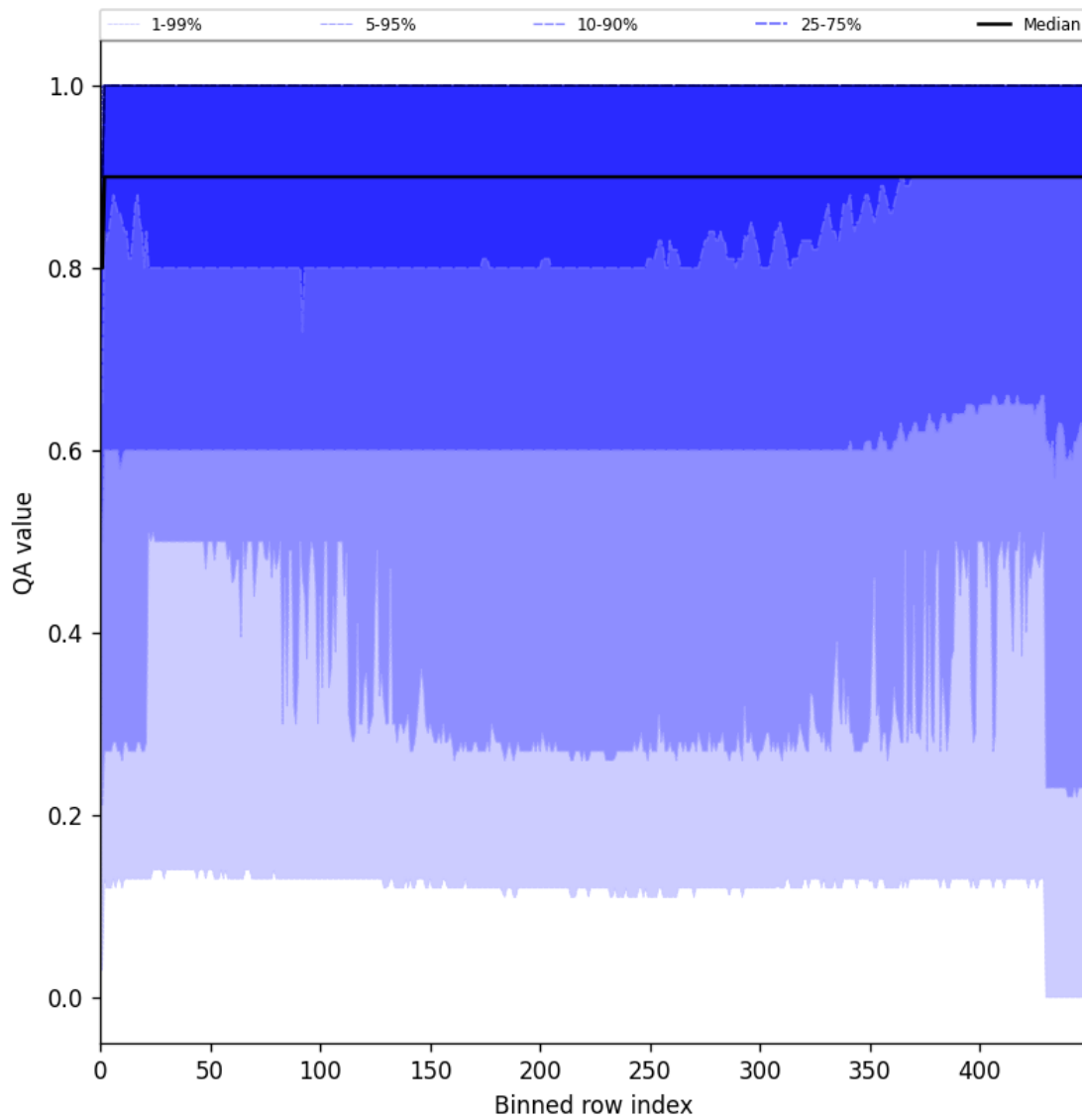
Figure 27: Along track statistics of “QA value” for 2025-11-18 to 2025-11-20
