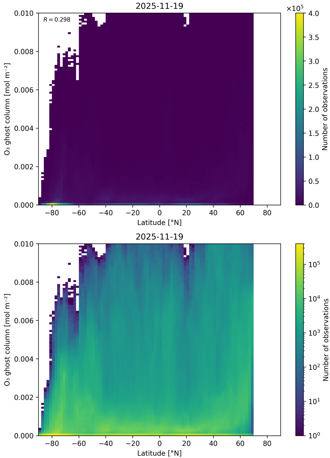
Figure 35: Scatter density plot of “Latitude” against “O 3 ghost column” for 2025-11-18 to 2025-11-20.
