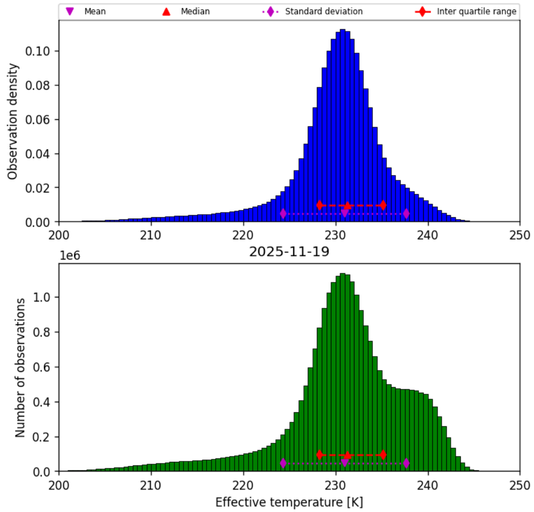
Figure 24: Histogram of “Effective temperature” for 2025-11-18 to 2025-11-20
