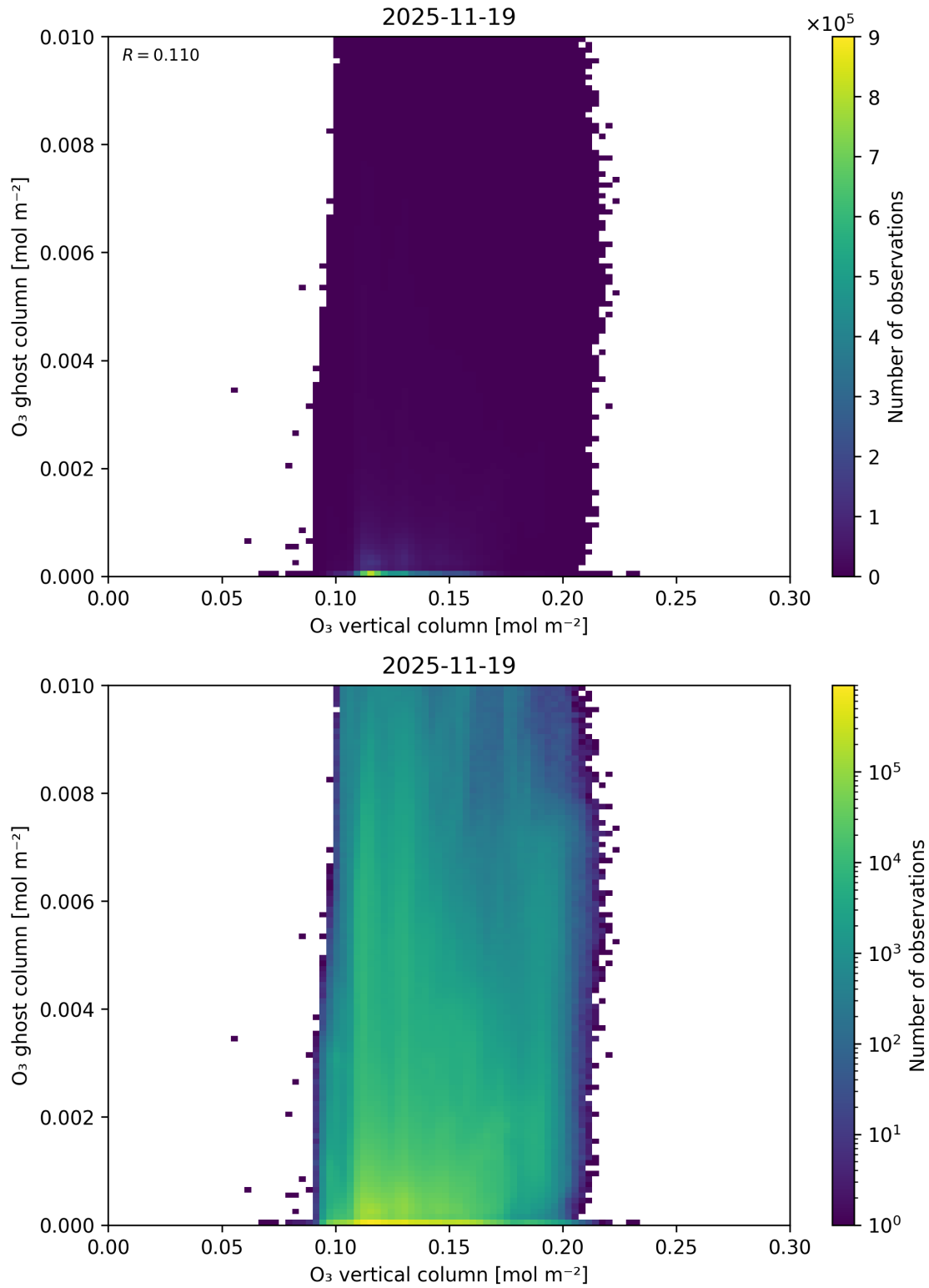
Figure 40: Scatter density plot of “O 3 vertical column” against “O 3 ghost column” for 2025-11-18 to 2025-11-20.
