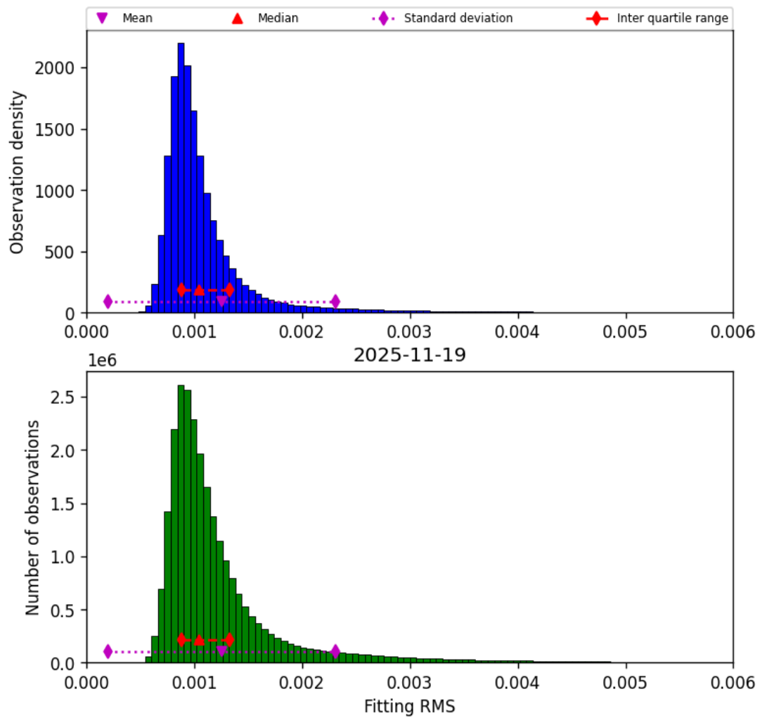
Figure 23: Histogram of “Fitting RMS” for 2025-11-18 to 2025-11-20
