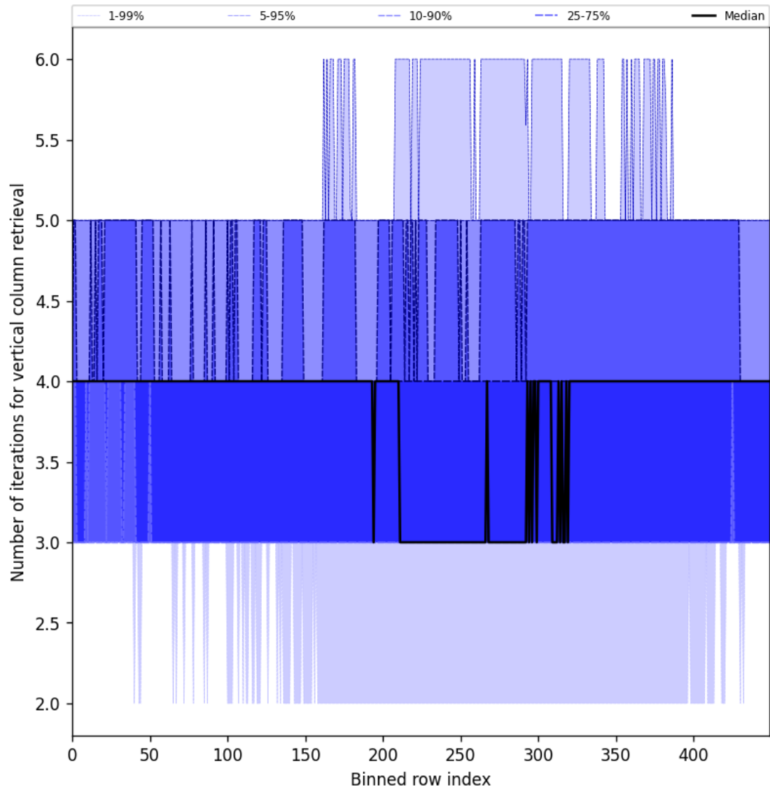
Figure 33: Along track statistics of “Number of iterations for vertical column retrieval” for 2025-11-18 to 2025-11-20
