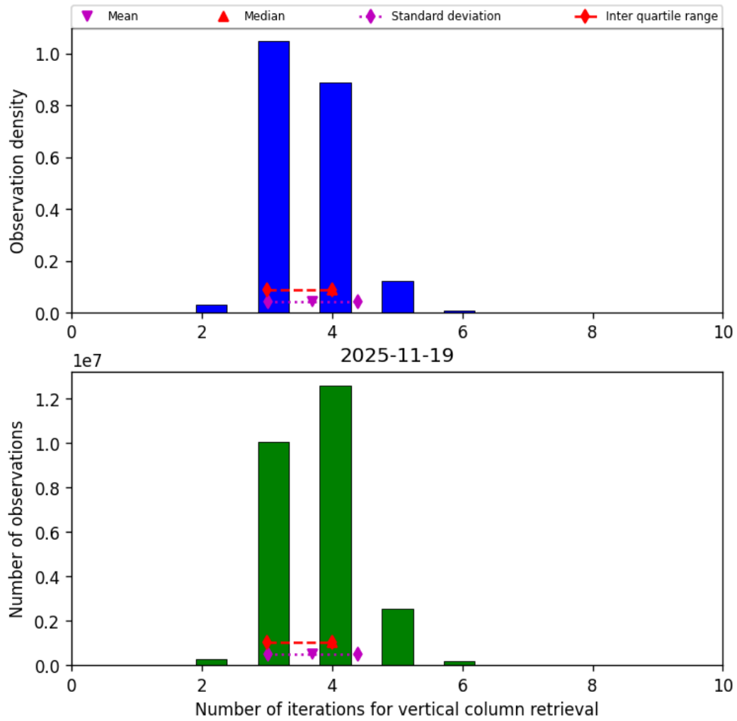
Figure 26: Histogram of “Number of iterations for vertical column retrieval” for 2025-11-18 to 2025-11-20
