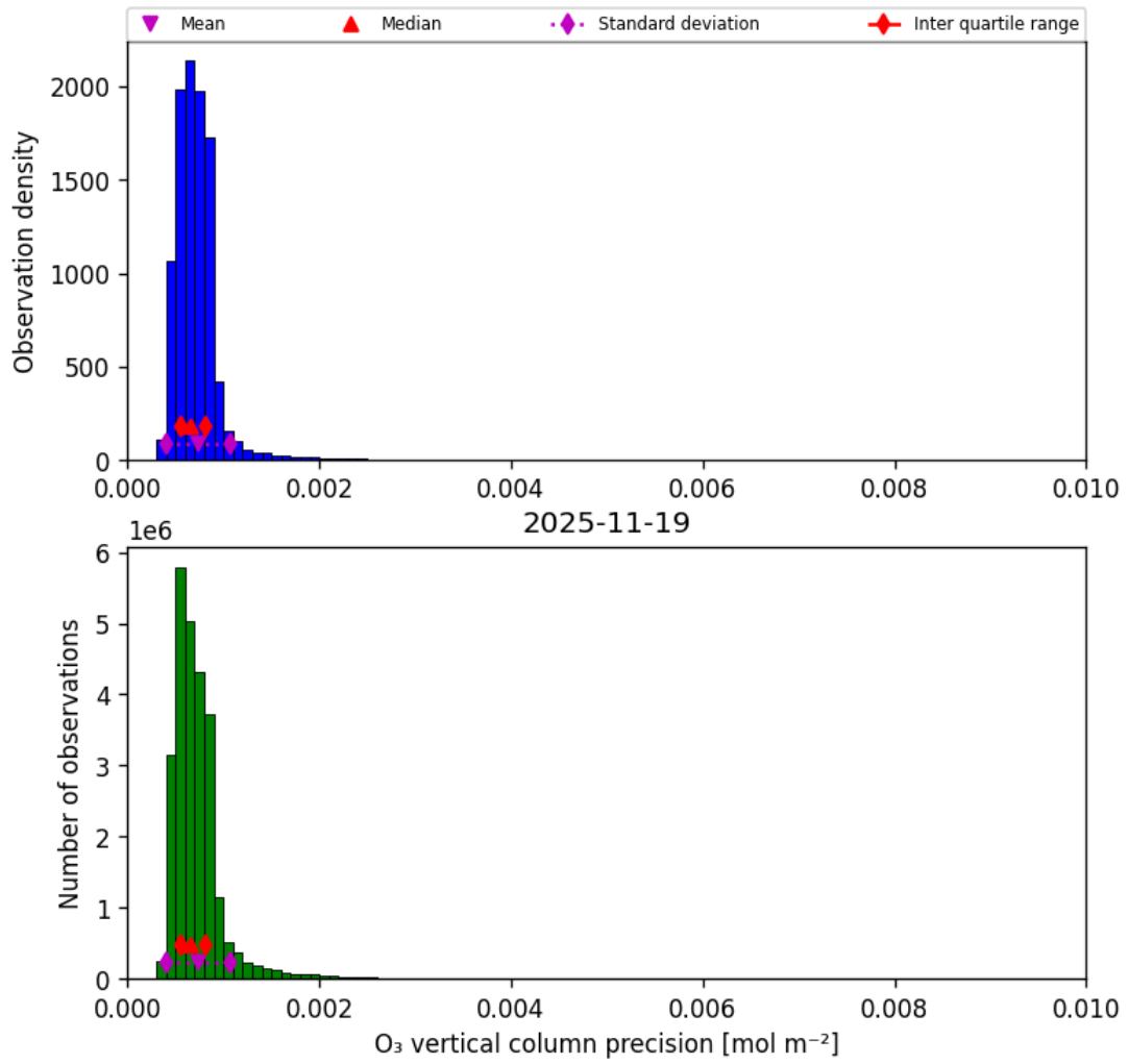
Figure 22: Histogram of "O 3 vertical column precision" for 2025-11-18 to 2025-11-20
