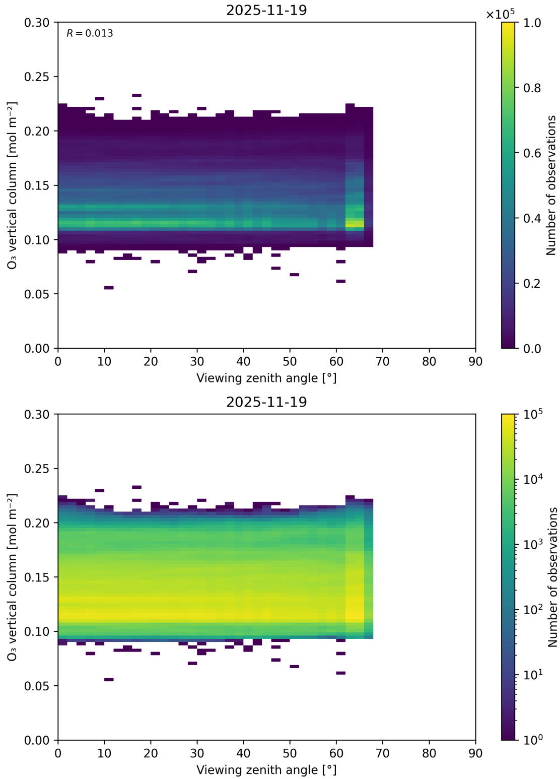
Figure 52: Scatter density plot of “Viewing zenith angle” against “O 3 vertical column” for 2025-11-18 to 2025-11-20.
