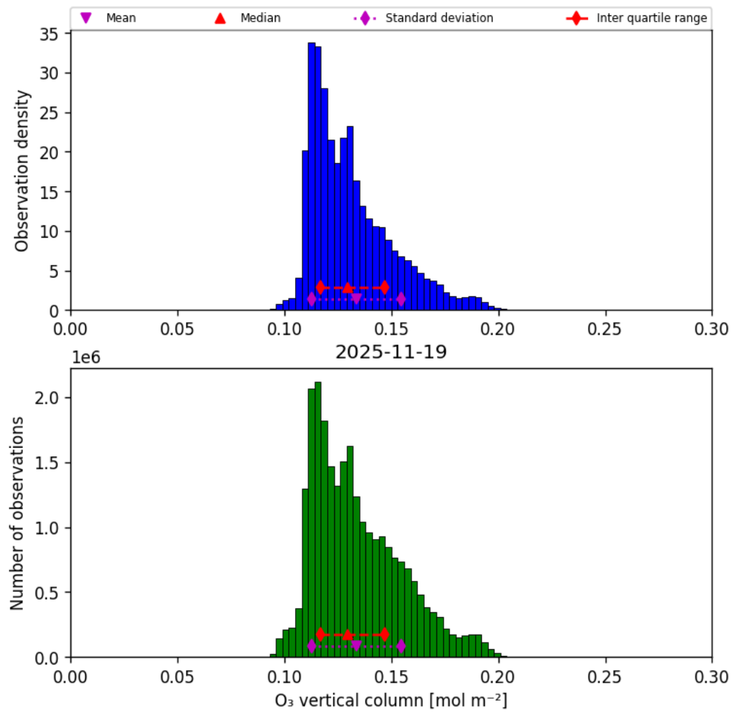
Figure 21: Histogram of “O 3 vertical column” for 2025-11-18 to 2025-11-20
