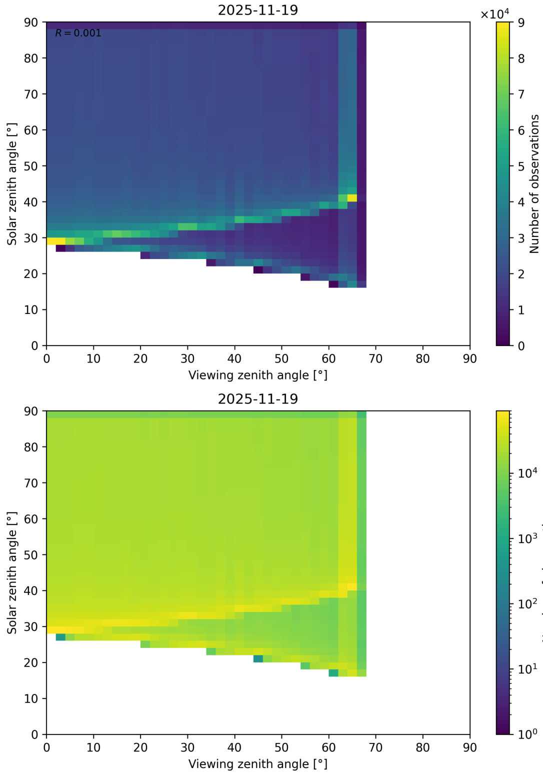
Figure 54: Scatter density plot of “Viewing zenith angle” against “Solar zenith angle” for 2025-11-18 to 2025-11-20.
