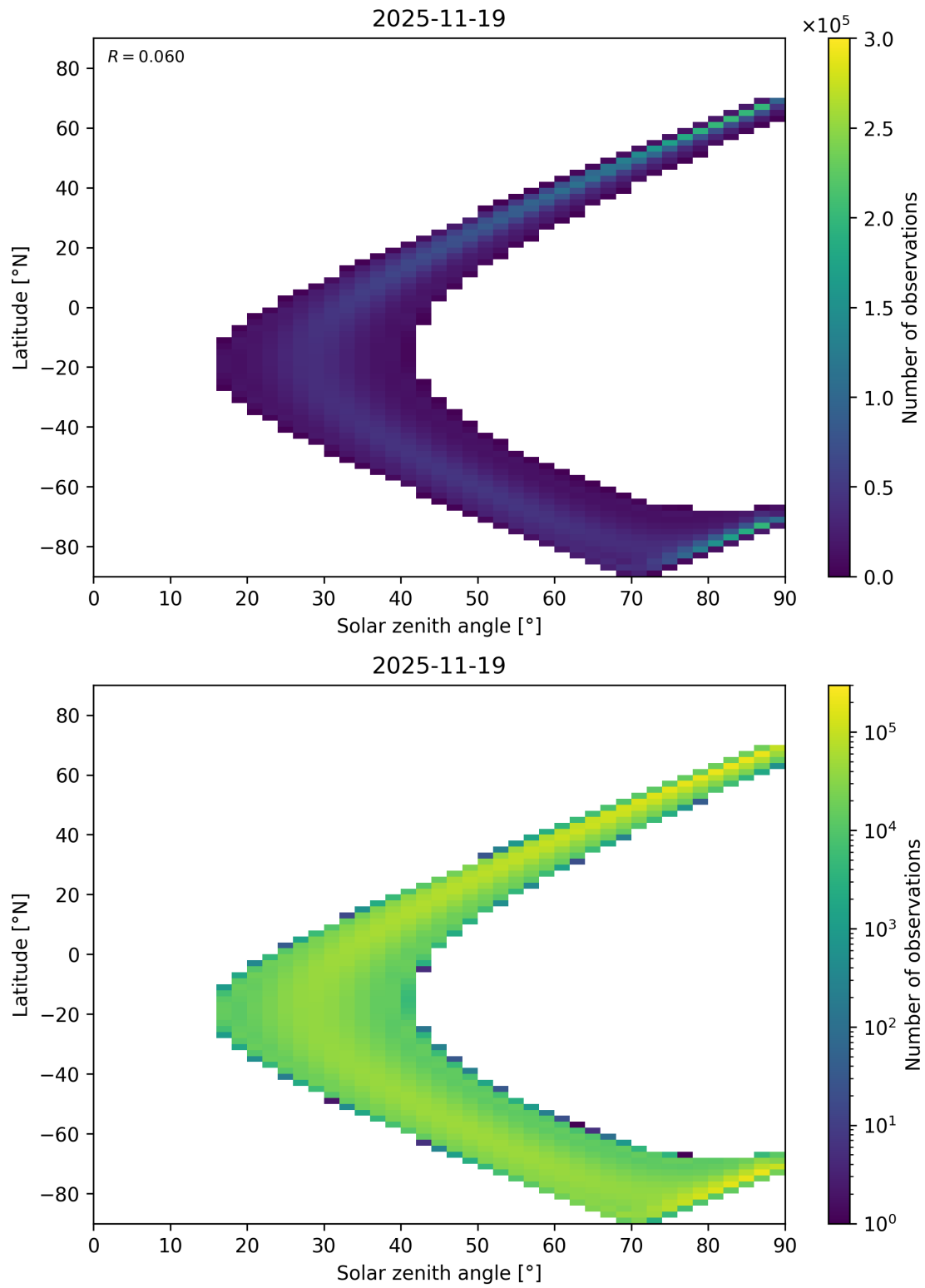
Figure 44: Scatter density plot of “Solar zenith angle” against “Latitude” for 2025-11-18 to 2025-11-20.
