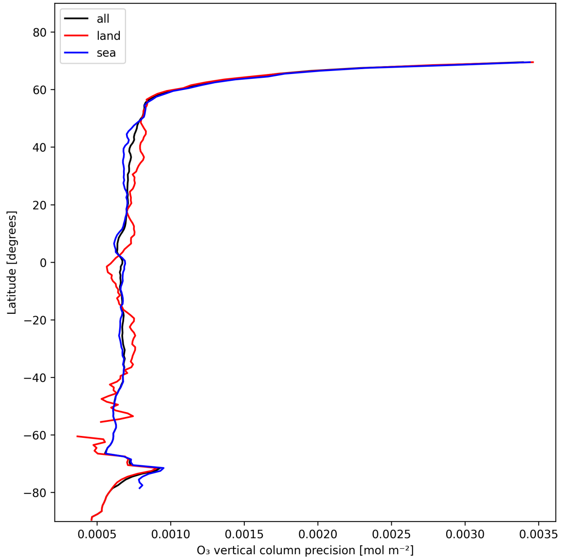
Figure 15: Zonal average of “O 3 vertical column precision” for 2025-11-18 to 2025-11-20.
