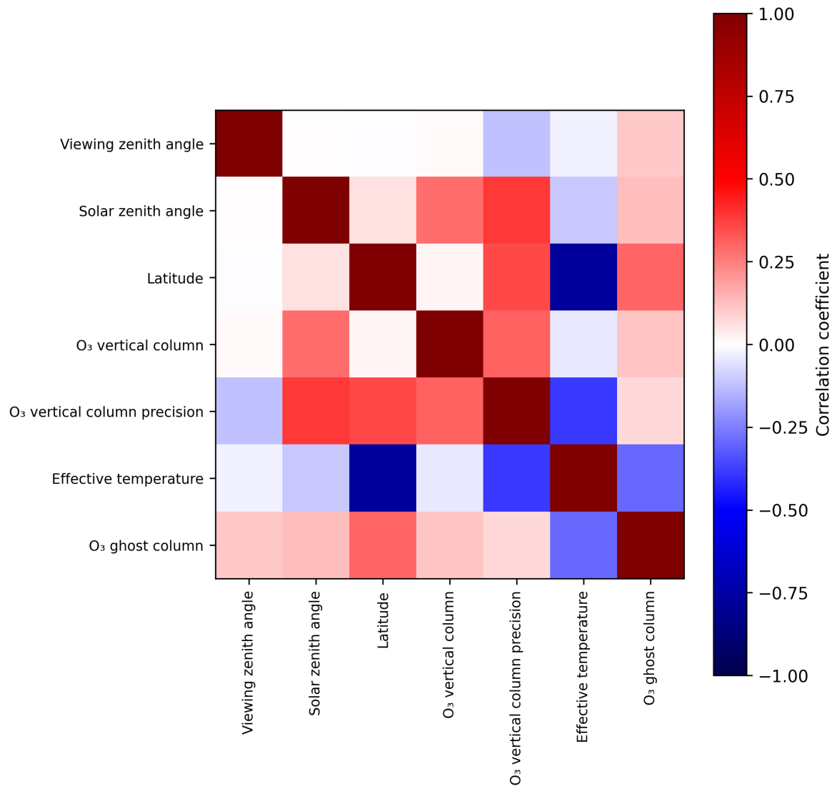
Figure 2: Map of correlation matrix for 2025-11-18 to 2025-11-20.
