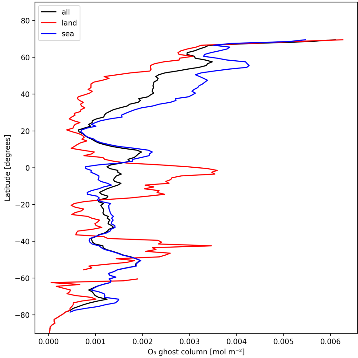
Figure 18: Zonal average of "O 3 ghost column" for 2025-11-18 to 2025-11-20.
