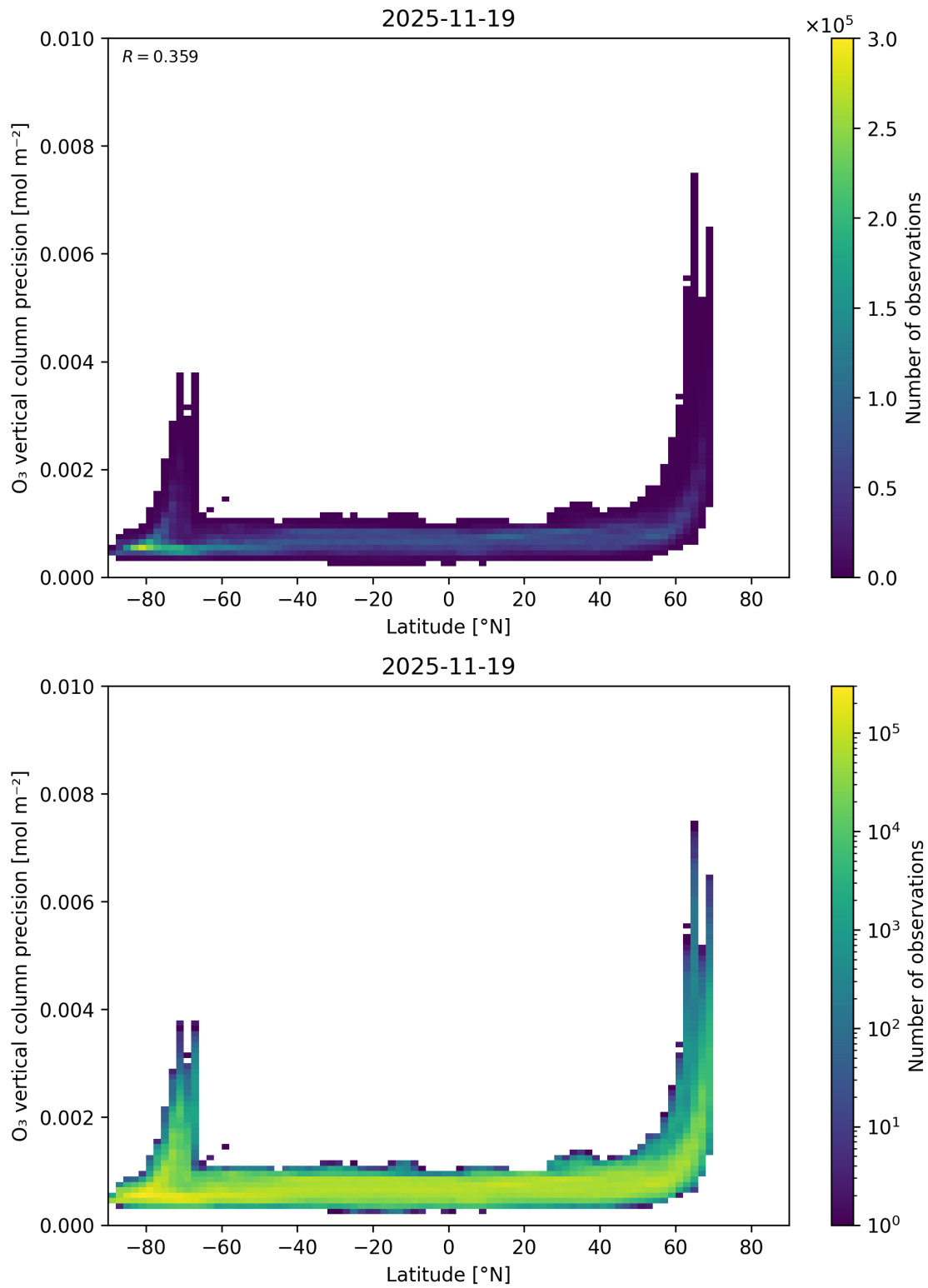
Figure 37: Scatter density plot of “Latitude” against “O 3 vertical column precision” for 2025-11-18 to 2025-11-20.
