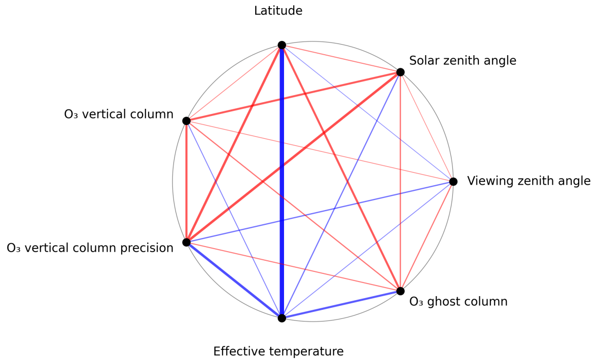
Figure 1: Map of correlation graph for 2025-11-18 to 2025-11-20.
