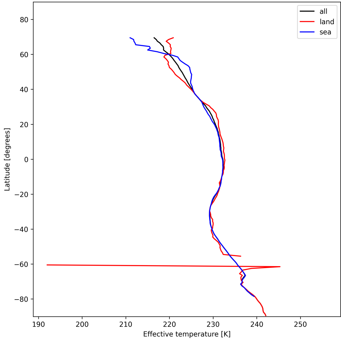
Figure 17: Zonal average of "Effective temperature" for 2025-11-18 to 2025-11-20.
