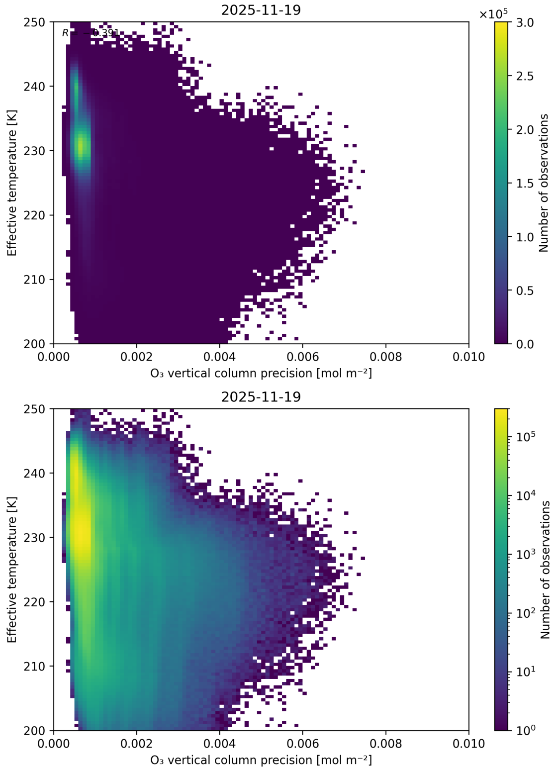
Figure 42: Scatter density plot of “O 3 vertical column precision” against “Effective temperature” for 2025-11-18 to 2025-11-20.
