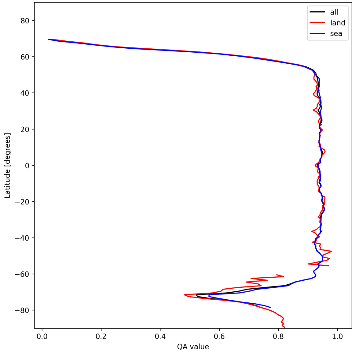
Figure 13: Zonal average of “QA value” for 2025-11-18 to 2025-11-20.
