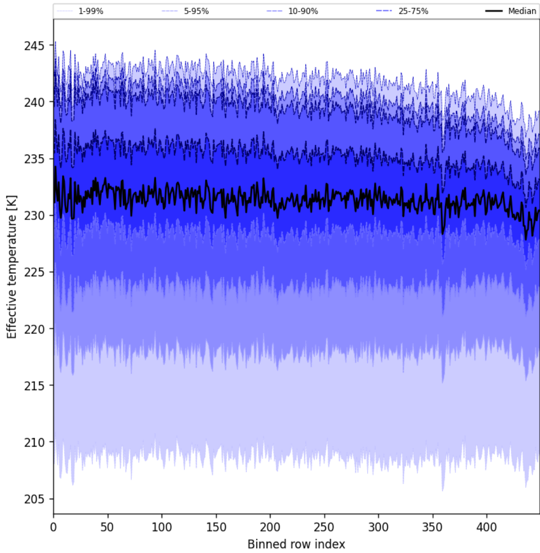
Figure 31: Along track statistics of “Effective temperature” for 2025-11-18 to 2025-11-20
