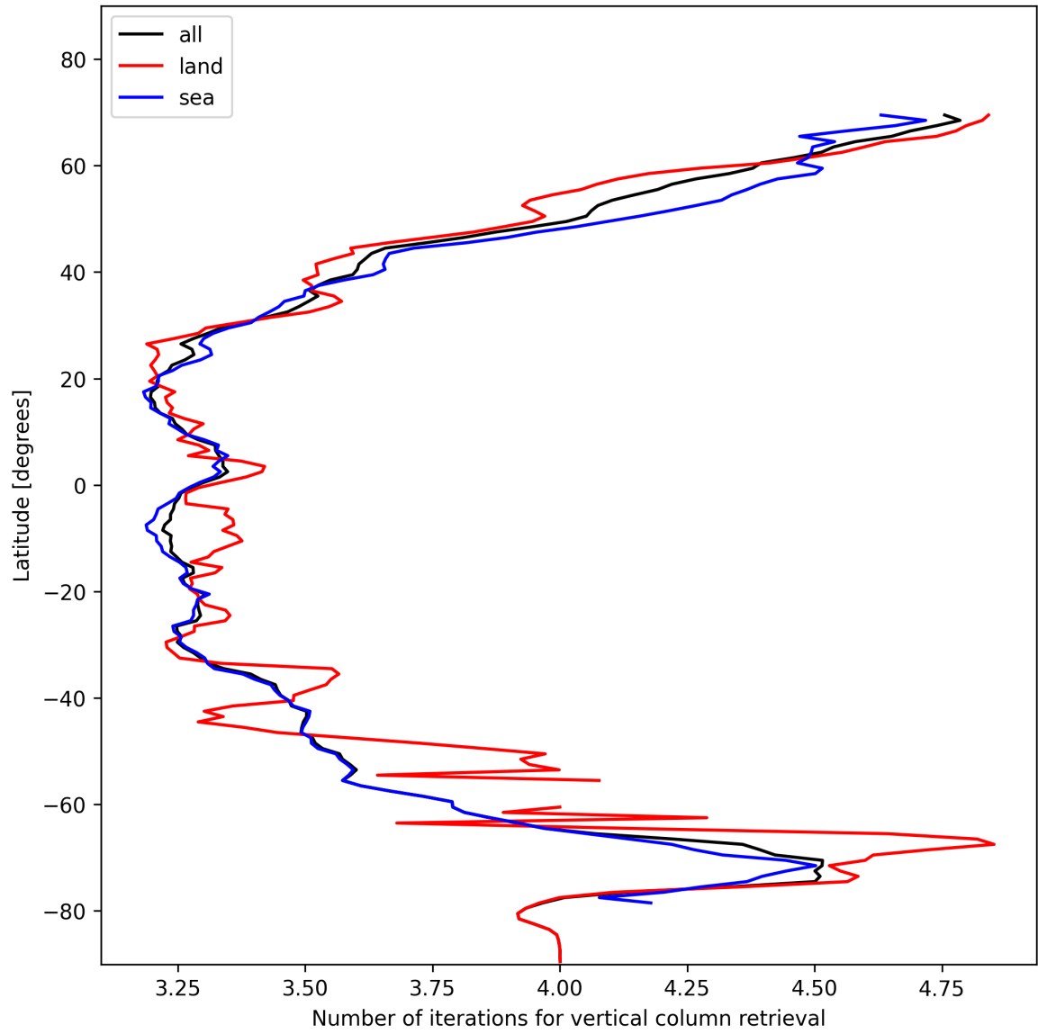
Figure 19: Zonal average of “Number of iterations for vertical column retrieval” for 2025-11-18 to 2025-11-20.
