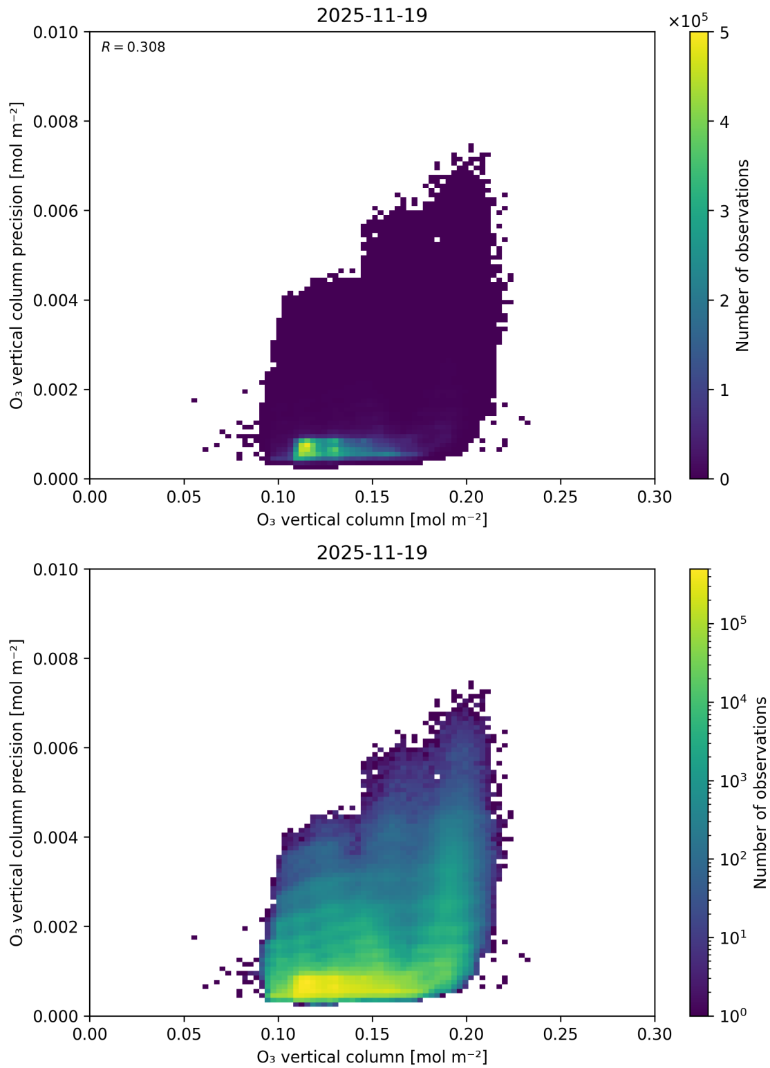
Figure 41: Scatter density plot of “O 3 vertical column” against “O 3 vertical column precision” for 2025-11-18 to 2025-11-20.
