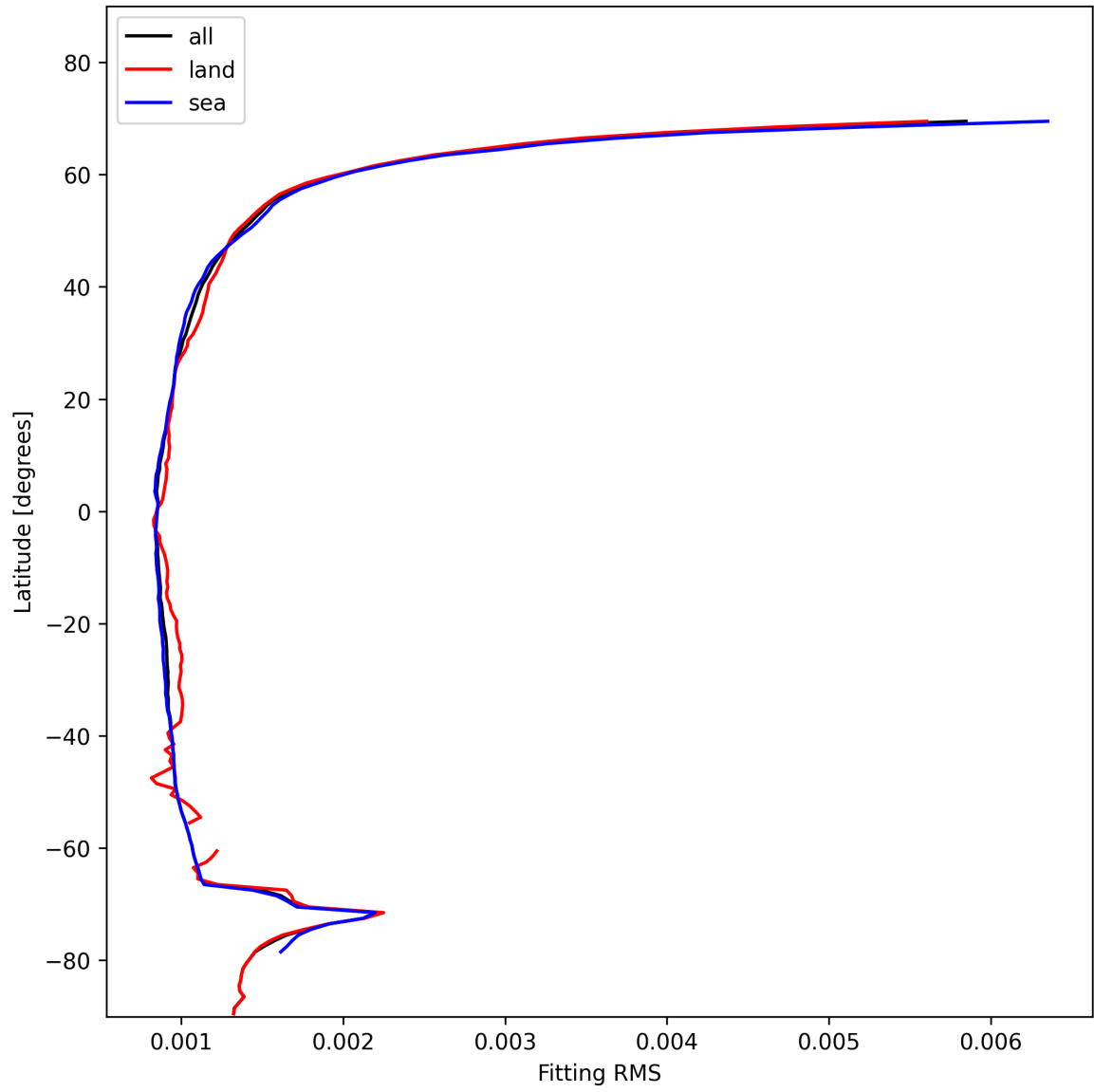
Figure 16: Zonal average of “Fitting RMS” for 2025-11-18 to 2025-11-20.
