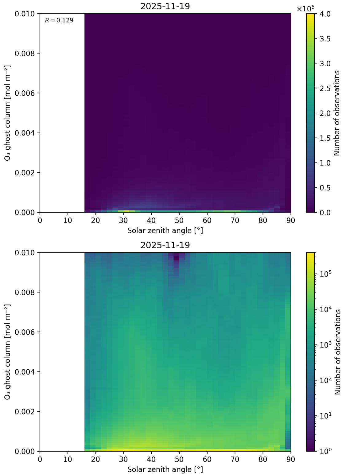
Figure 46: Scatter density plot of “Solar zenith angle” against “O 3 ghost column” for 2025-11-18 to 2025-11-20.
