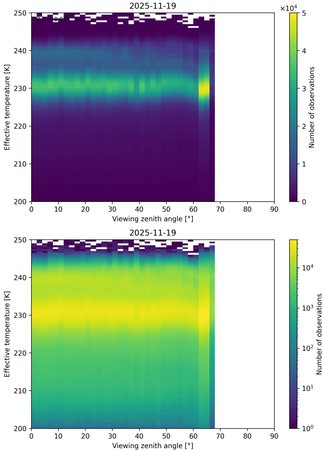
Figure 50: Scatter density plot of “Viewing zenith angle” against “Effective temperature” for 2025-11-18 to 2025-11-20.
