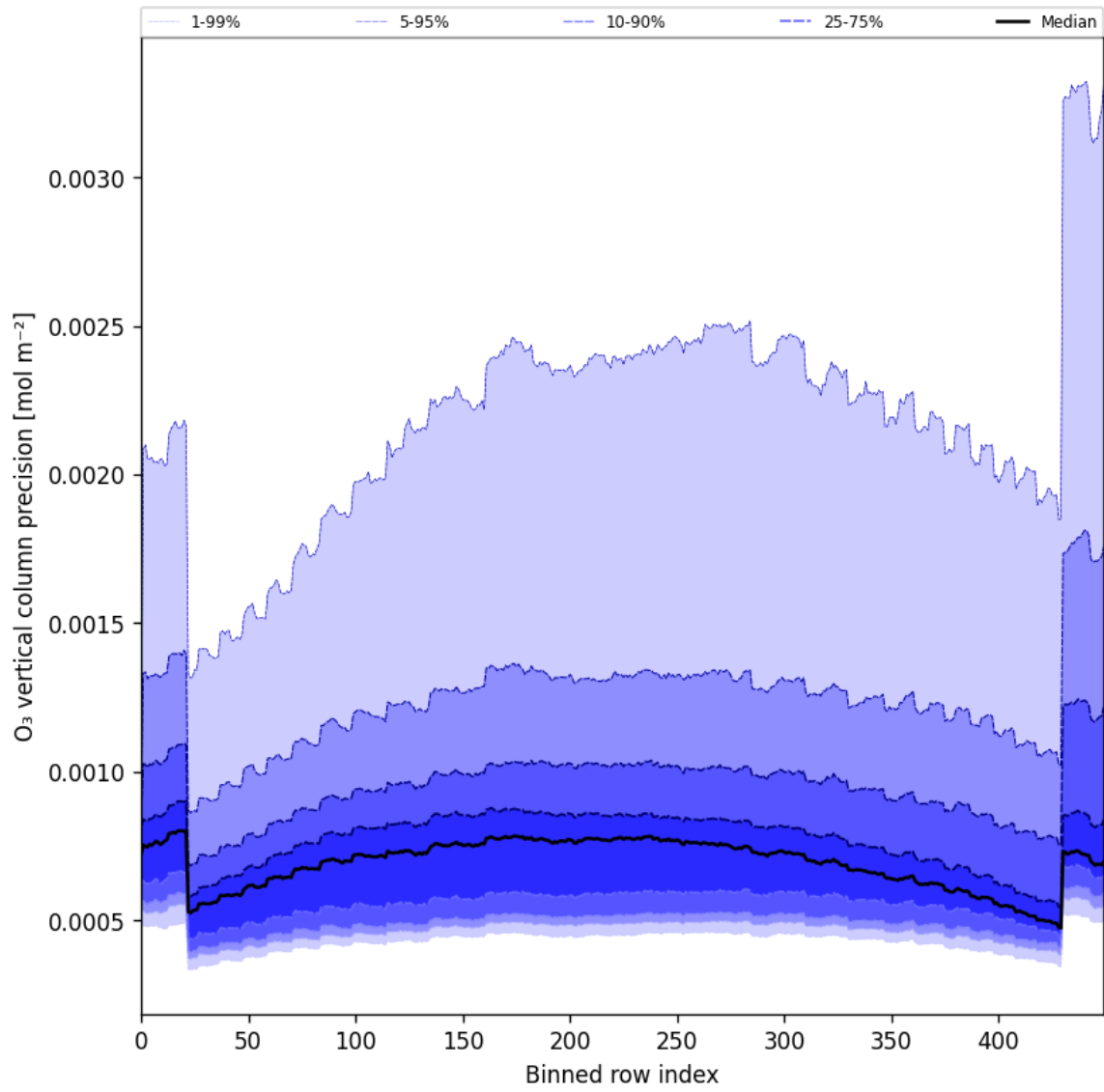
Figure 29: Along track statistics of “O 3 vertical column precision” for 2025-11-18 to 2025-11-20
