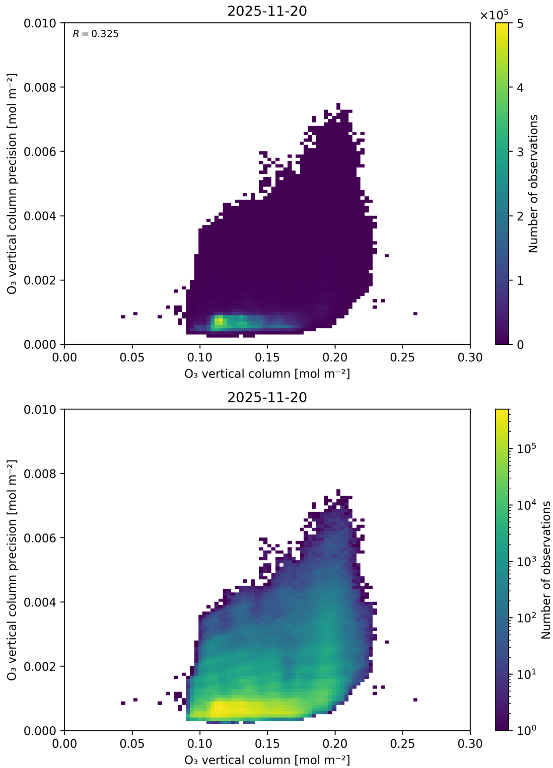
Figure 41: Scatter density plot of “O 3 vertical column” against “O 3 vertical column precision” for 2025-11-19 to 2025-11-21.
