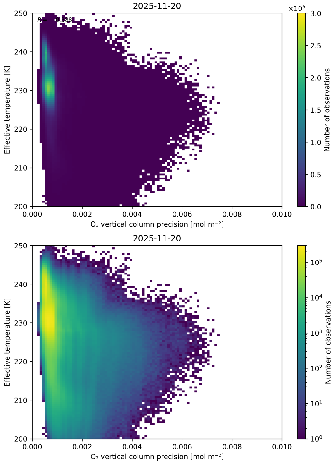
Figure 42: Scatter density plot of “ O_3 vertical column precision” against “Effective temperature” for 2025-11-19 to 2025-11-21.
