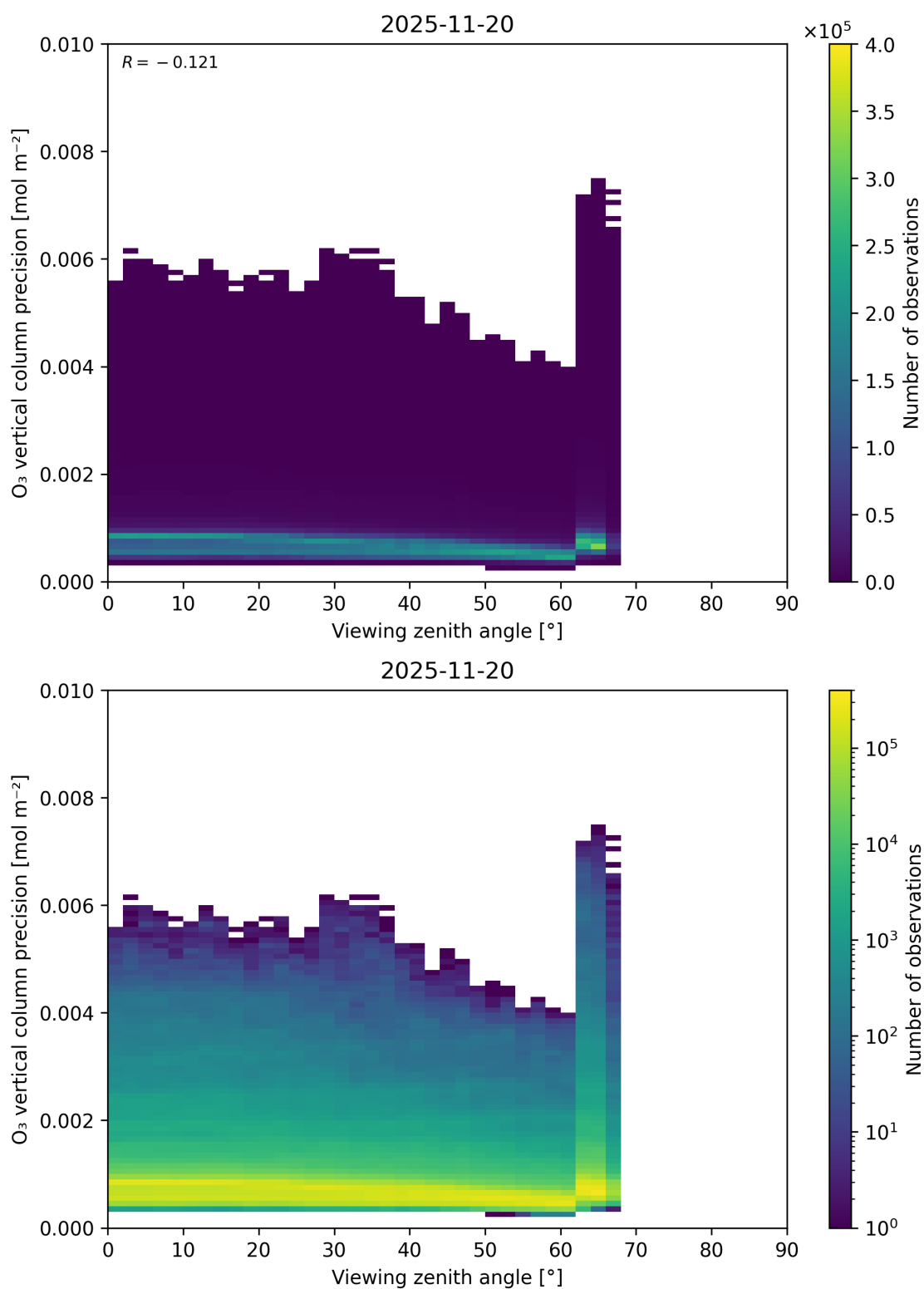
Figure 53: Scatter density plot of “Viewing zenith angle” against “O 3 vertical column precision” for 2025-11-19 to 2025-11-21.
