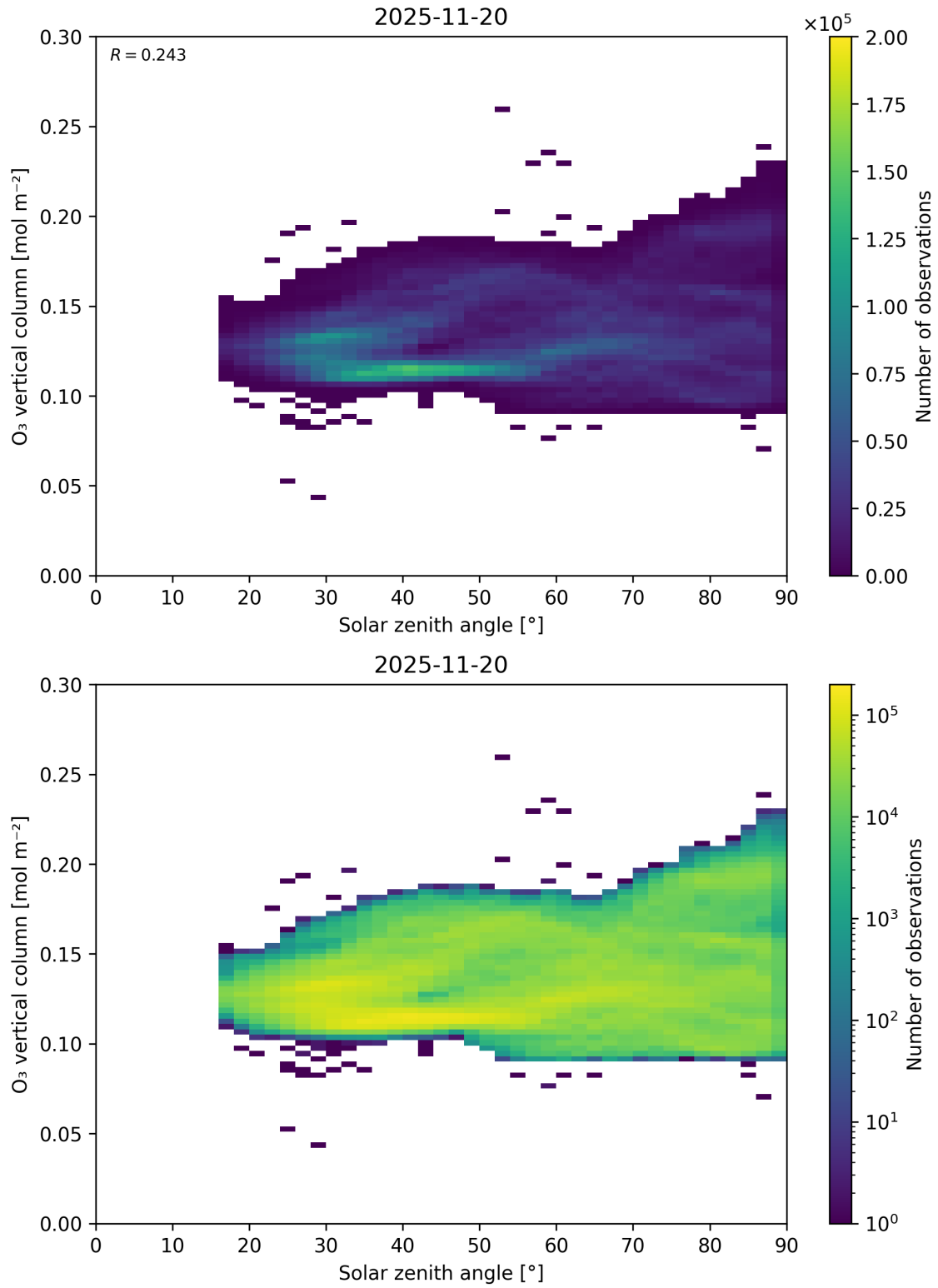
Figure 47: Scatter density plot of “Solar zenith angle” against “O 3 vertical column” for 2025-11-19 to 2025-11-21.
