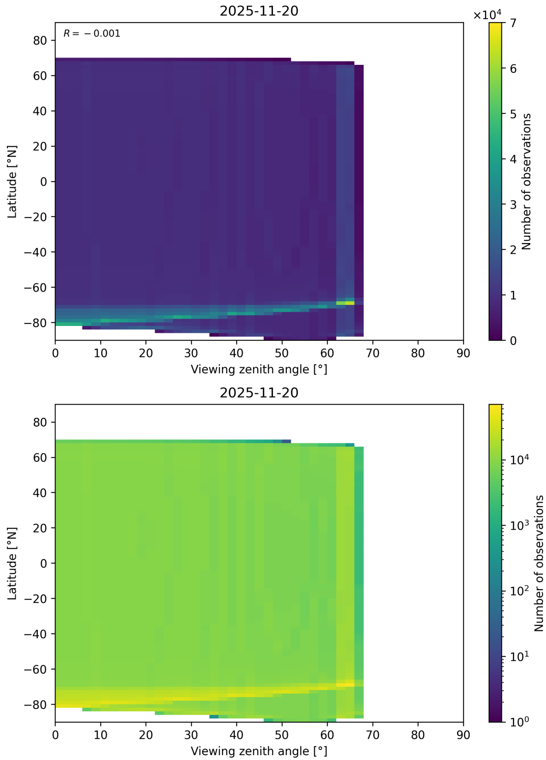
Figure 49: Scatter density plot of “Viewing zenith angle” against “Latitude” for 2025-11-19 to 2025-11-21.
