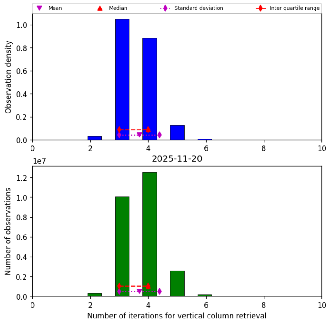
Figure 26: Histogram of “Number of iterations for vertical column retrieval” for 2025-11-19 to 2025-11-21
