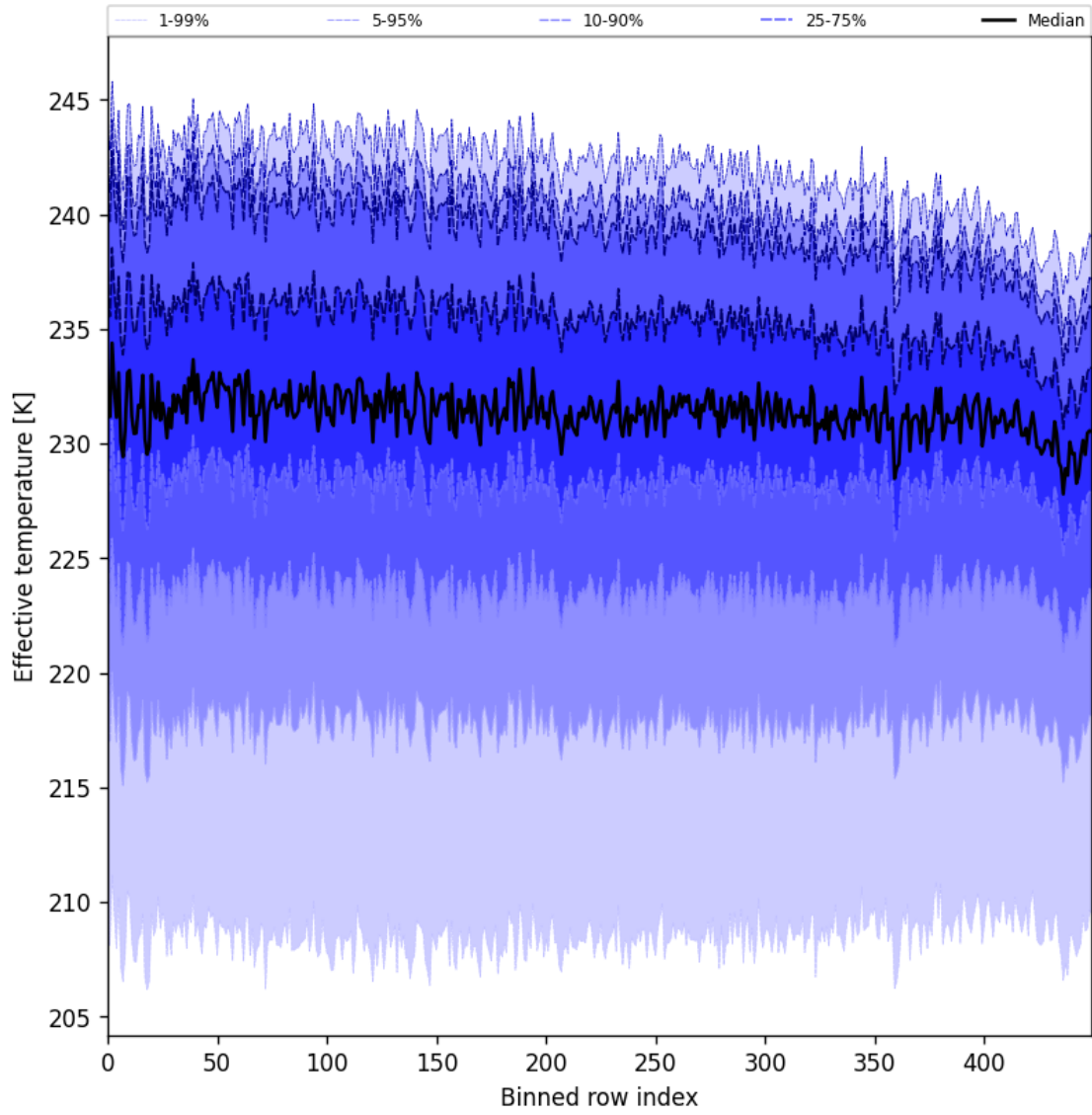
Figure 31: Along track statistics of “Effective temperature” for 2025-11-19 to 2025-11-21
