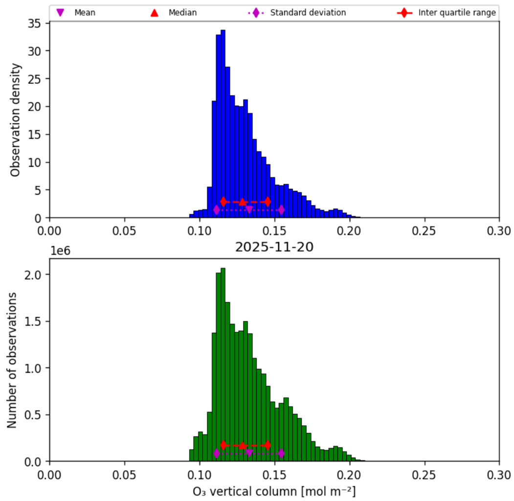
Figure 21: Histogram of “O 3 vertical column” for 2025-11-19 to 2025-11-21
