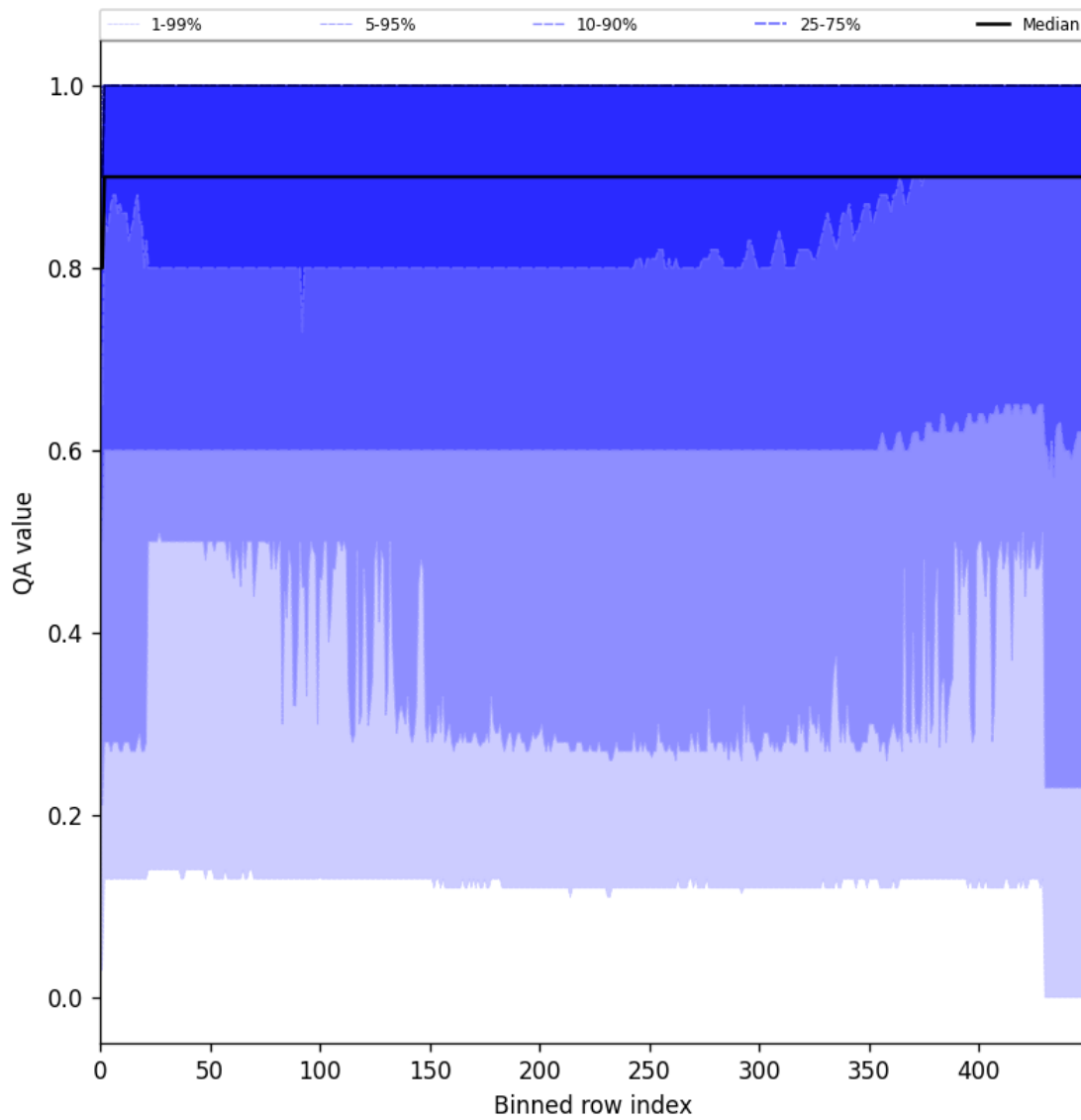
Figure 27: Along track statistics of “QA value” for 2025-11-19 to 2025-11-21
