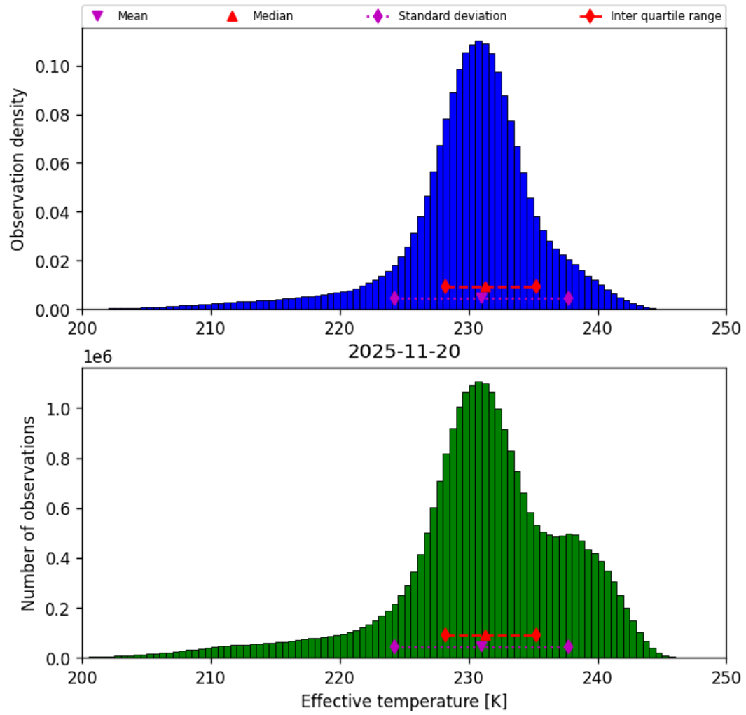
Figure 24: Histogram of “Effective temperature” for 2025-11-19 to 2025-11-21
