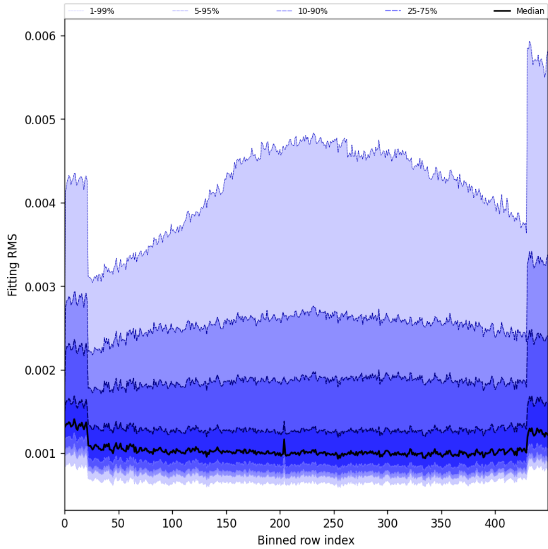
Figure 30: Along track statistics of “Fitting RMS” for 2025-11-19 to 2025-11-21
