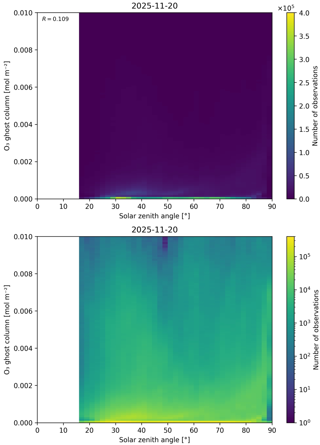
Figure 46: Scatter density plot of “Solar zenith angle” against “O 3 ghost column” for 2025-11-19 to 2025-11-21.
