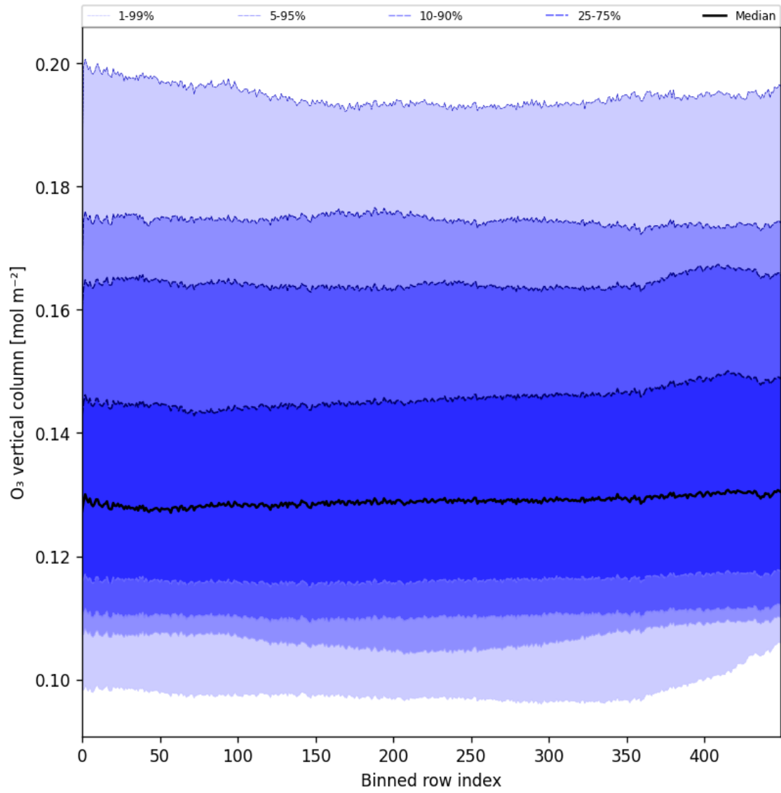
Figure 28: Along track statistics of “O 3 vertical column” for 2025-11-19 to 2025-11-21
