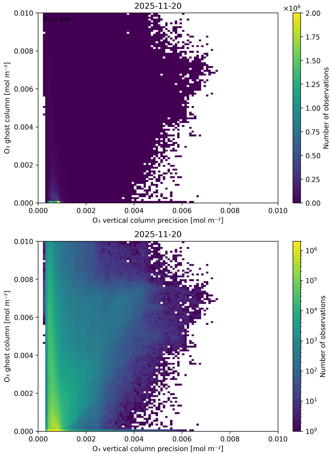
Figure 43: Scatter density plot of “ \text{O}_3 vertical column precision” against “ \text{O}_3 ghost column” for 2025-11-19 to 2025-11-21.
