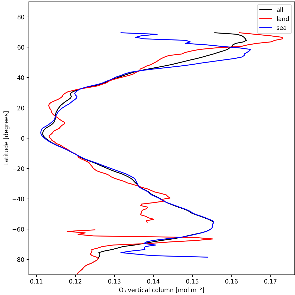
Figure 14: Zonal average of “O 3 vertical column” for 2025-11-19 to 2025-11-21.
