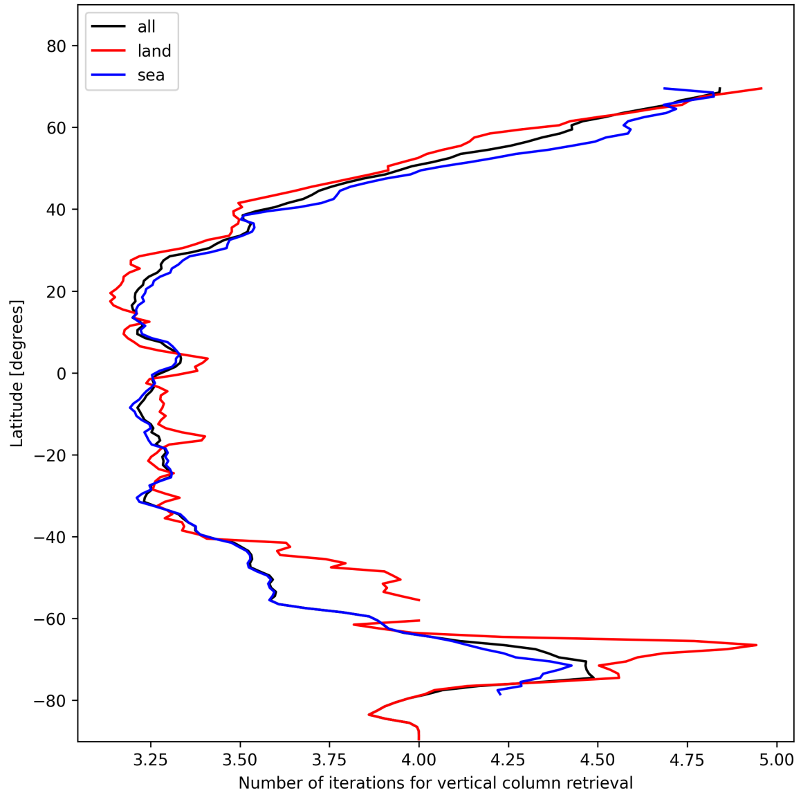
Figure 19: Zonal average of “Number of iterations for vertical column retrieval” for 2025-11-19 to 2025-11-21.
