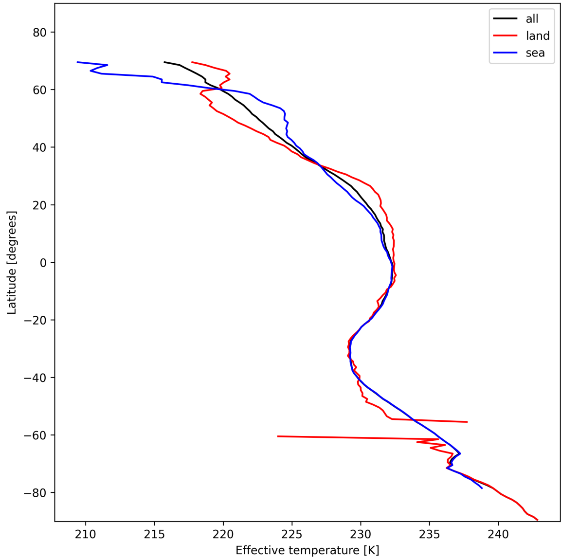
Figure 17: Zonal average of “Effective temperature” for 2025-11-19 to 2025-11-21.
