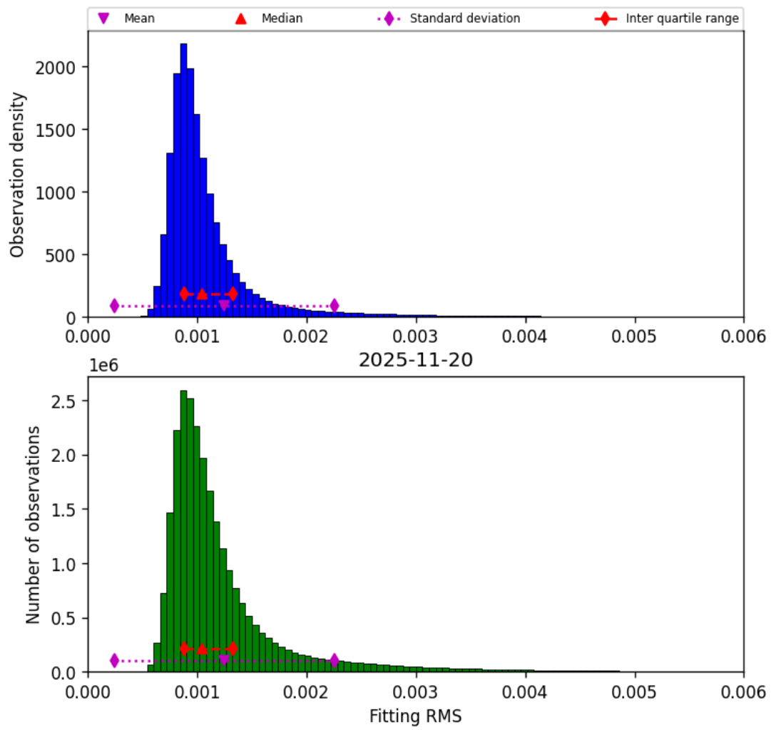
Figure 23: Histogram of “Fitting RMS” for 2025-11-19 to 2025-11-21
