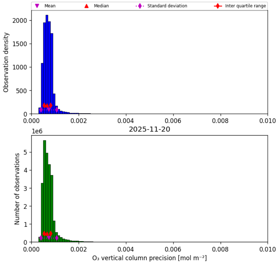
Figure 22: Histogram of “O 3 vertical column precision” for 2025-11-19 to 2025-11-21
