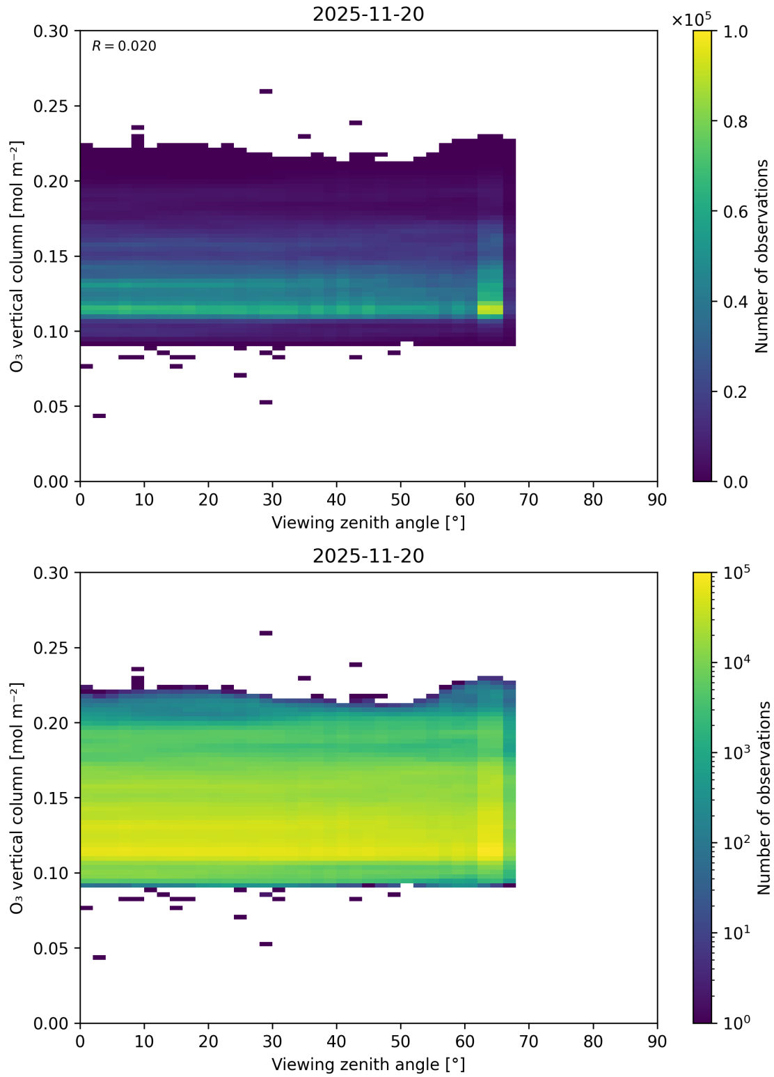
Figure 52: Scatter density plot of “Viewing zenith angle” against “O 3 vertical column” for 2025-11-19 to 2025-11-21.
