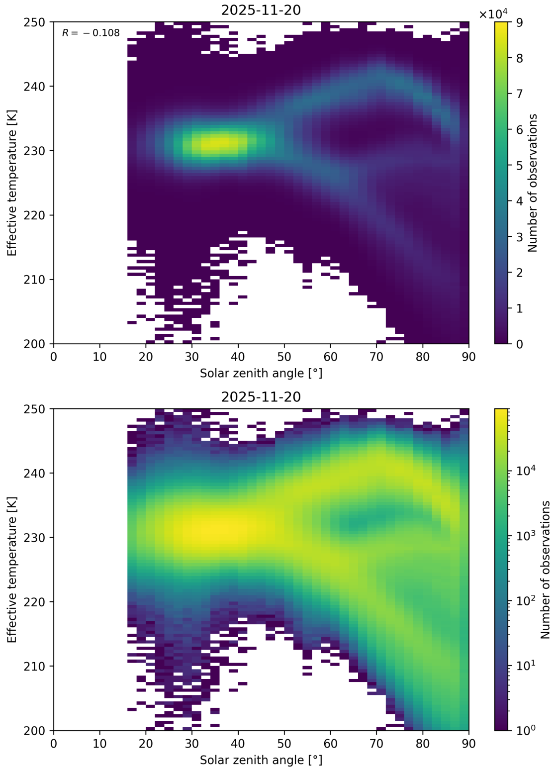
Figure 45: Scatter density plot of “Solar zenith angle” against “Effective temperature” for 2025-11-19 to 2025-11-21.
