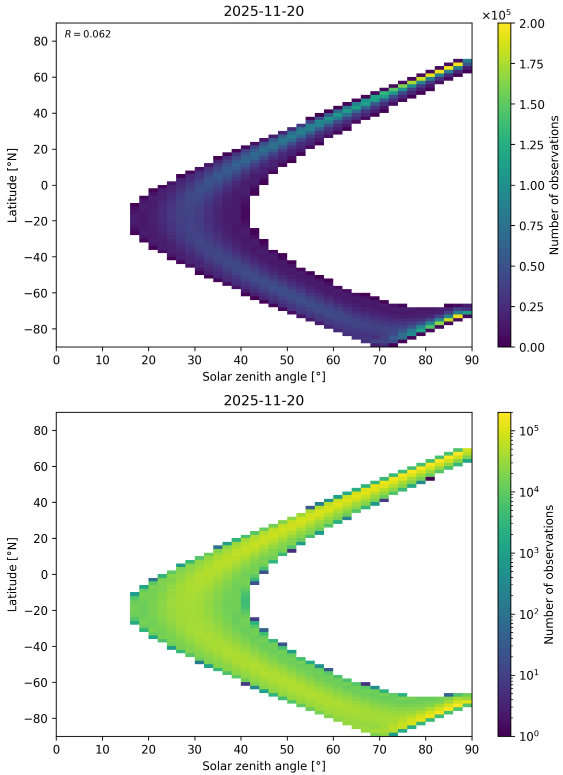
Figure 44: Scatter density plot of “Solar zenith angle” against “Latitude” for 2025-11-19 to 2025-11-21.
