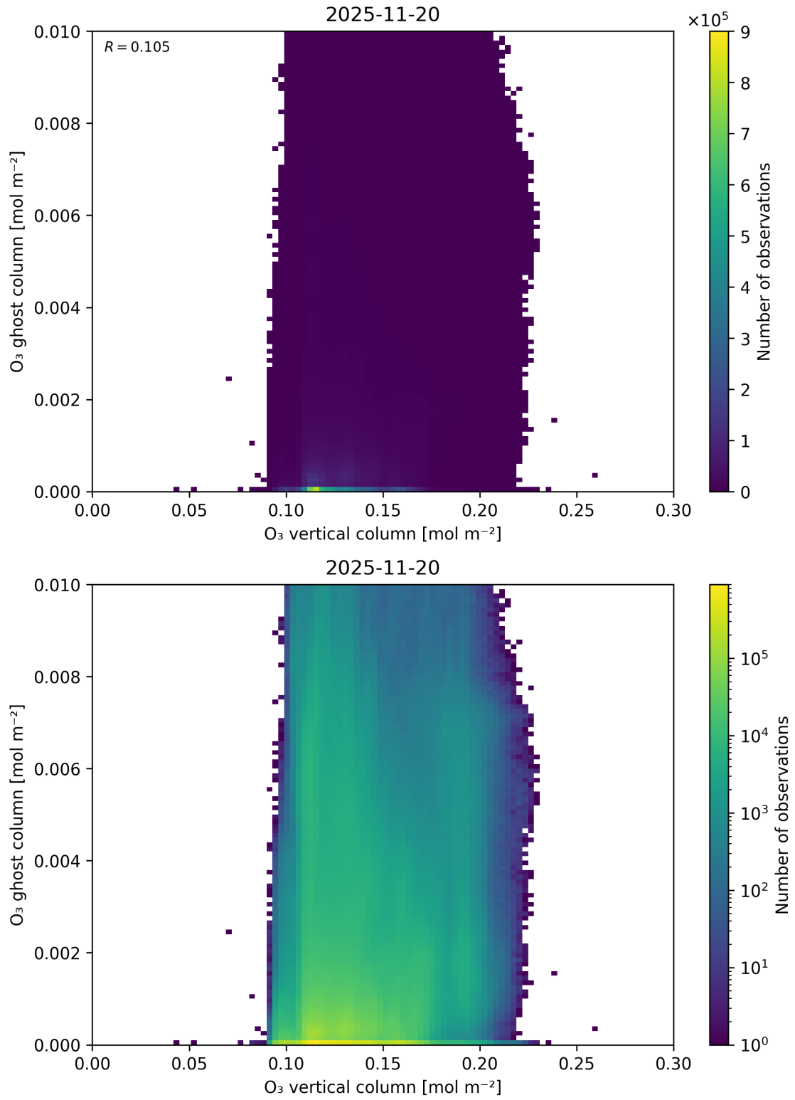
Figure 40: Scatter density plot of “O 3 vertical column” against “O 3 ghost column” for 2025-11-19 to 2025-11-21.
