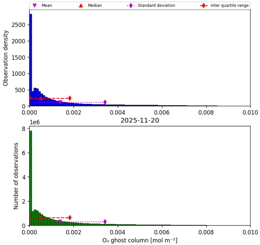
Figure 25: Histogram of “O 3 ghost column” for 2025-11-19 to 2025-11-21
