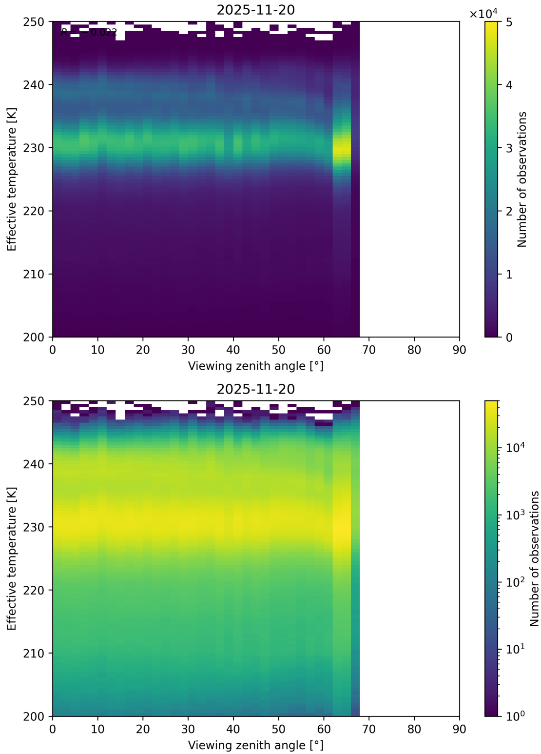
Figure 50: Scatter density plot of “Viewing zenith angle” against “Effective temperature” for 2025-11-19 to 2025-11-21.
