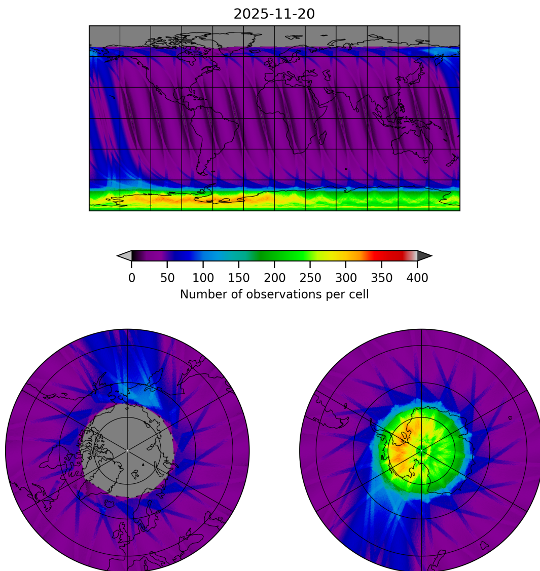
Figure 12: Map of the number of observations for 2025-11-19 to 2025-11-21
