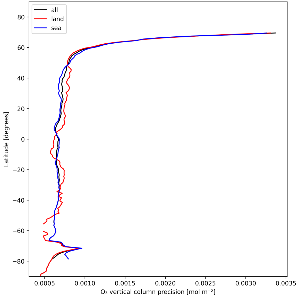
Figure 15: Zonal average of “O 3 vertical column precision” for 2025-11-19 to 2025-11-21.
