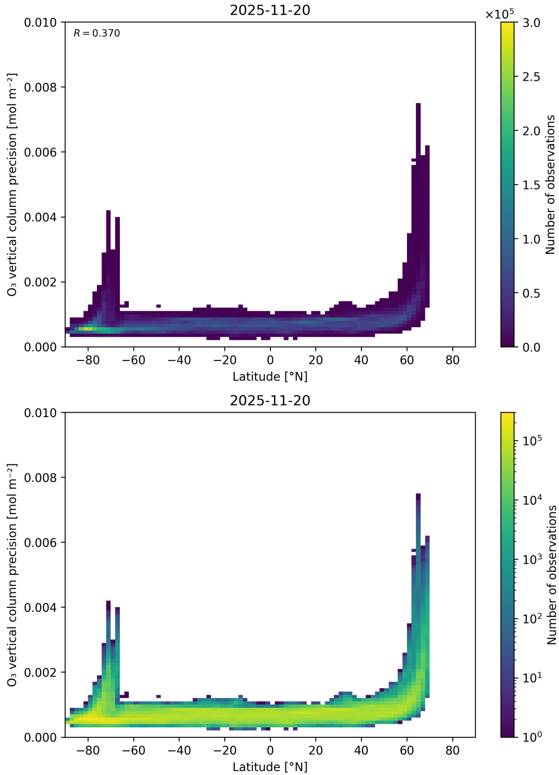
Figure 37: Scatter density plot of “Latitude” against “O 3 vertical column precision” for 2025-11-19 to 2025-11-21.
