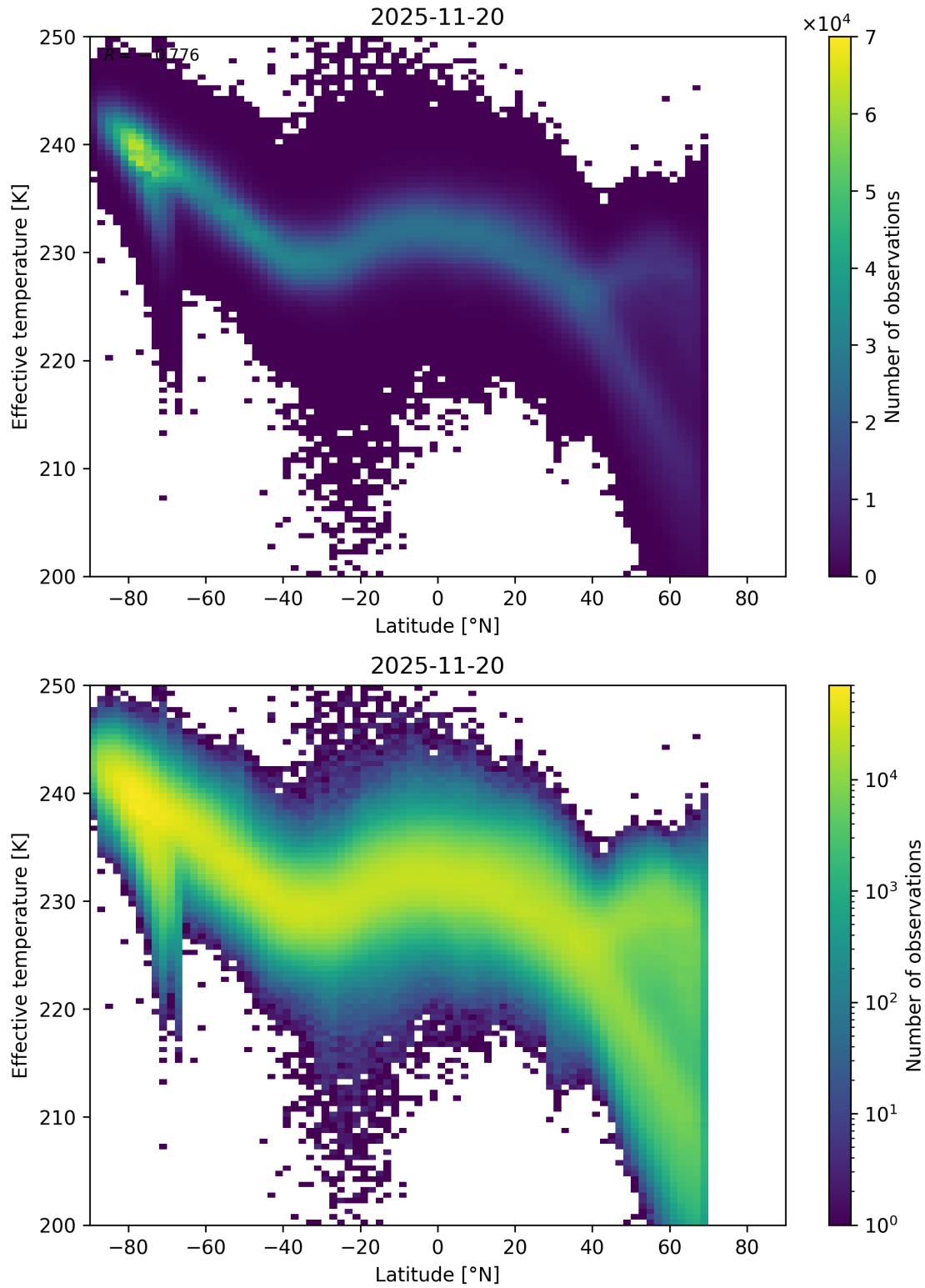
Figure 34: Scatter density plot of “Latitude” against “Effective temperature” for 2025-11-19 to 2025-11-21.
