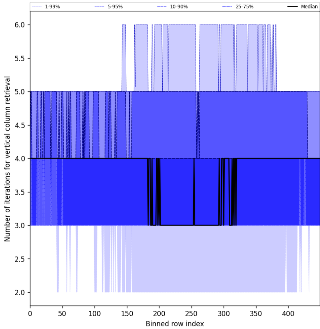
Figure 33: Along track statistics of “Number of iterations for vertical column retrieval” for 2025-11-19 to 2025-11-21
