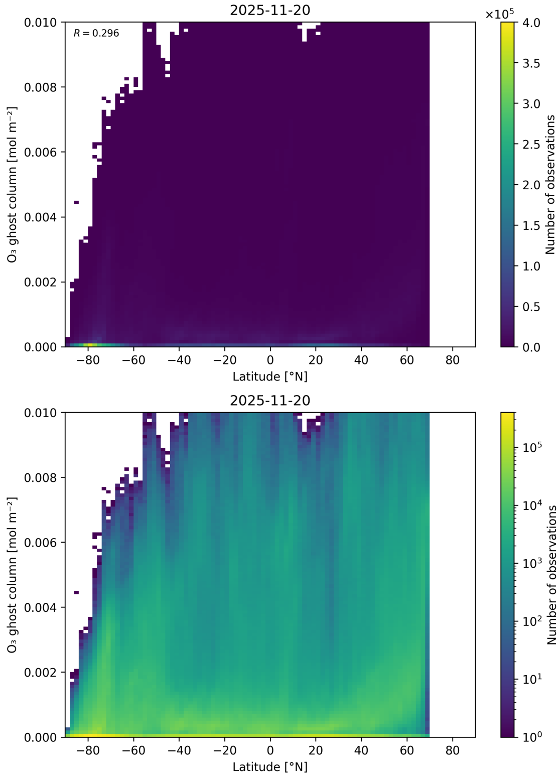
Figure 35: Scatter density plot of “Latitude” against “O 3 ghost column” for 2025-11-19 to 2025-11-21.
