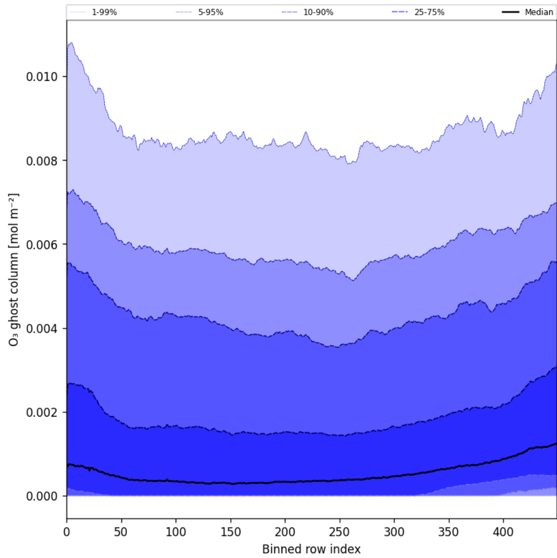
Figure 32: Along track statistics of “O 3 ghost column” for 2025-11-19 to 2025-11-21
