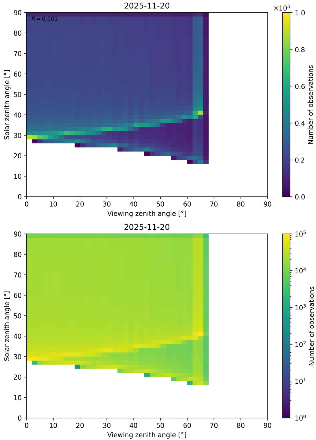
Figure 54: Scatter density plot of “Viewing zenith angle” against “Solar zenith angle” for 2025-11-19 to 2025-11-21.
