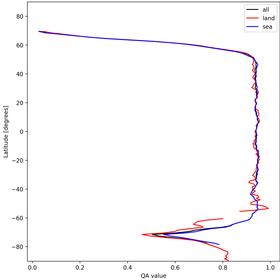
Figure 13: Zonal average of “QA value” for 2025-11-19 to 2025-11-21.
