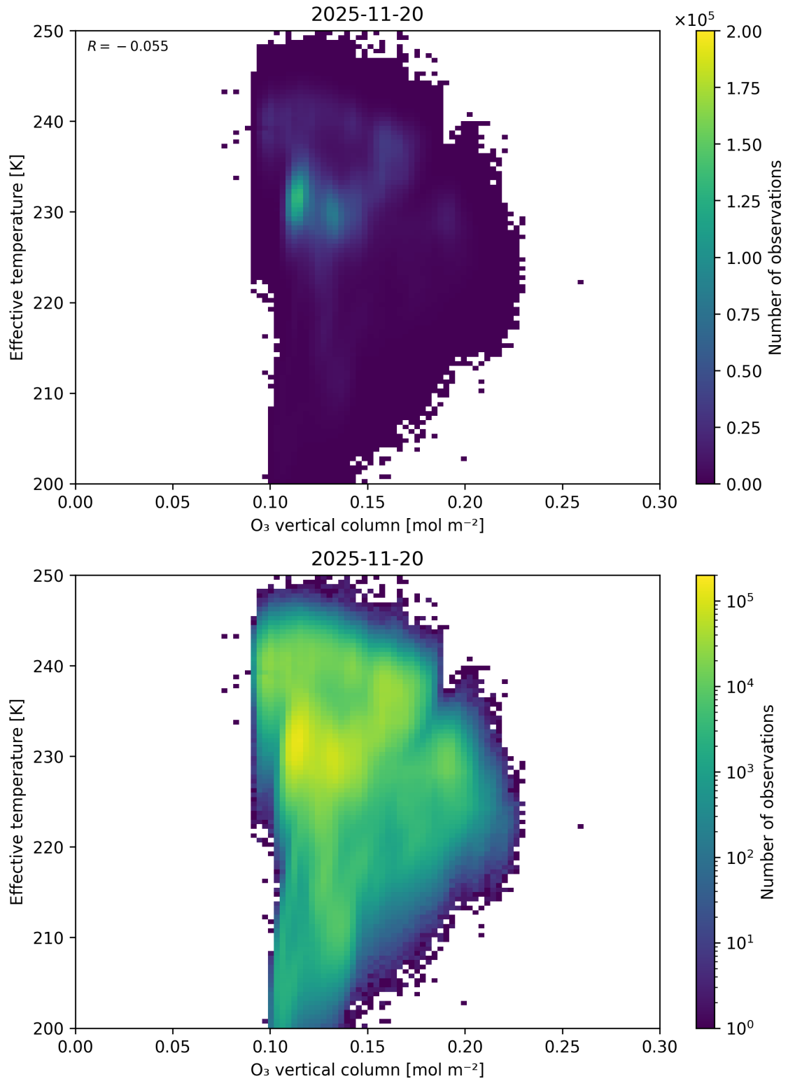
Figure 39: Scatter density plot of “O 3 vertical column” against “Effective temperature” for 2025-11-19 to 2025-11-21.
