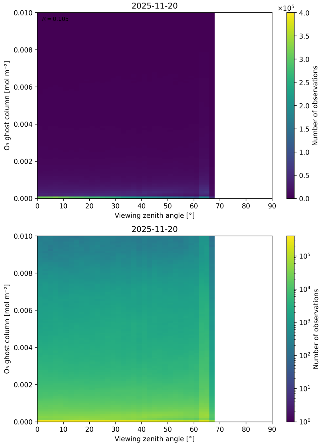
Figure 51: Scatter density plot of “Viewing zenith angle” against “O 3 ghost column” for 2025-11-19 to 2025-11-21.
