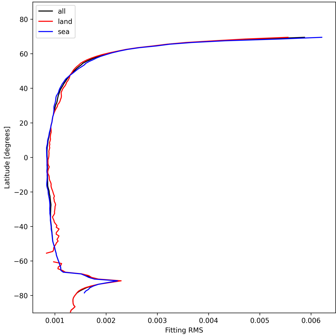
Figure 16: Zonal average of “Fitting RMS” for 2025-11-19 to 2025-11-21.
