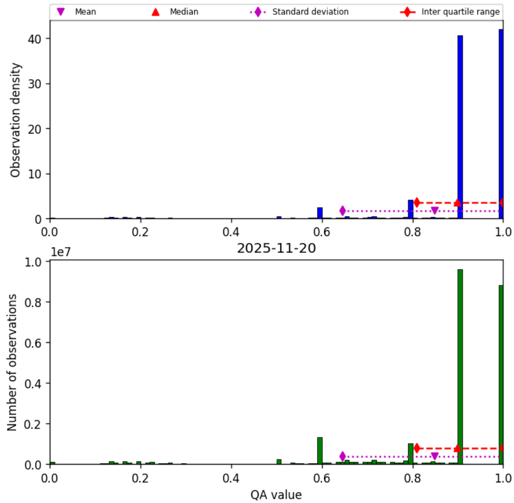
Figure 20: Histogram of “QA value” for 2025-11-19 to 2025-11-21
