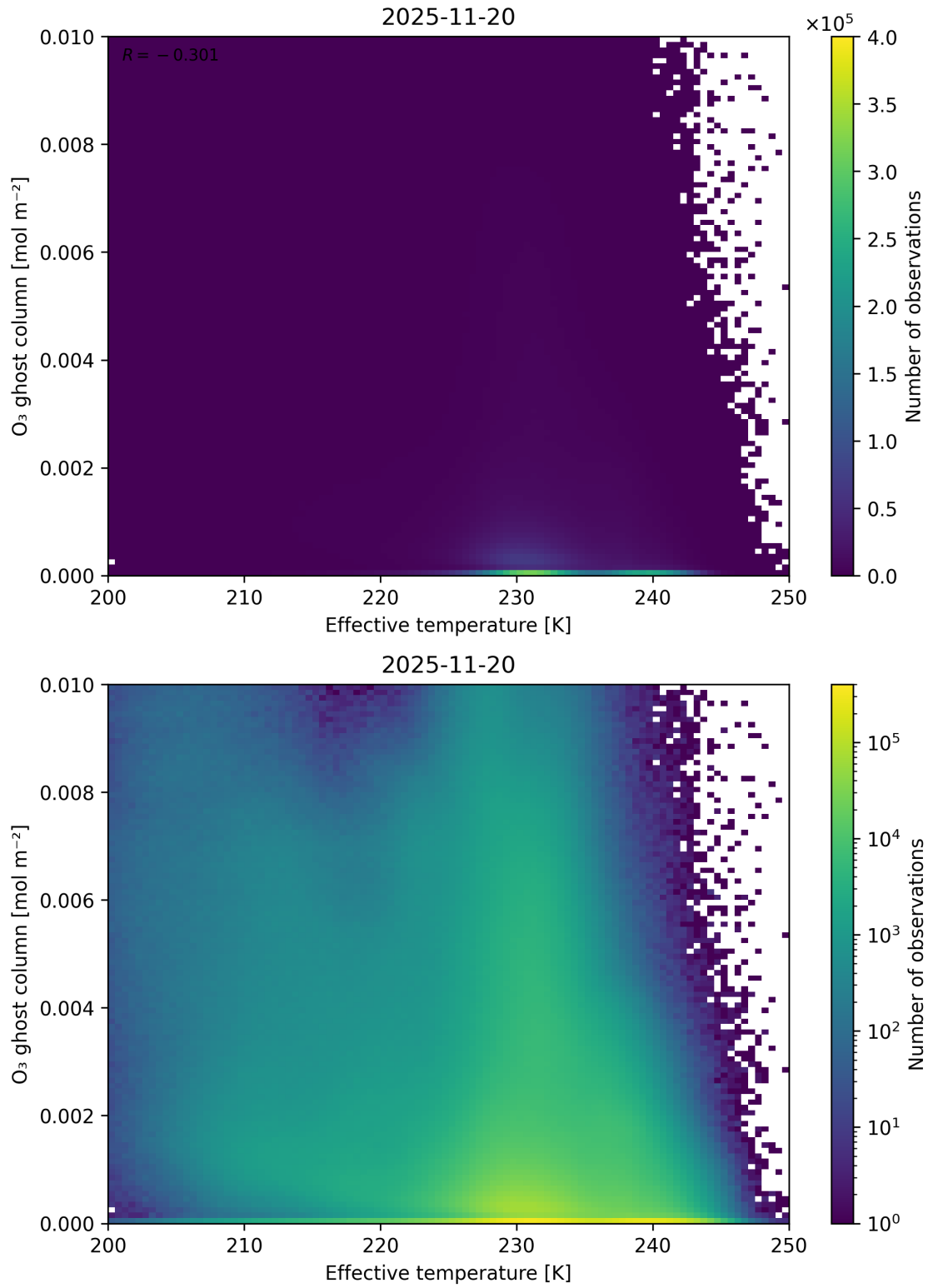
Figure 38: Scatter density plot of “Effective temperature” against “O 3 ghost column” for 2025-11-19 to 2025-11-21.
