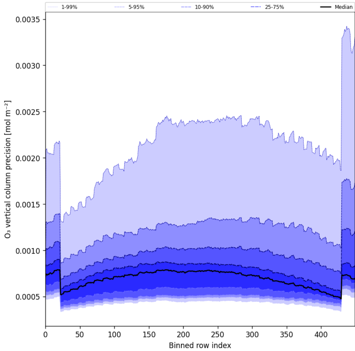
Figure 29: Along track statistics of “O 3 vertical column precision” for 2025-11-19 to 2025-11-21
