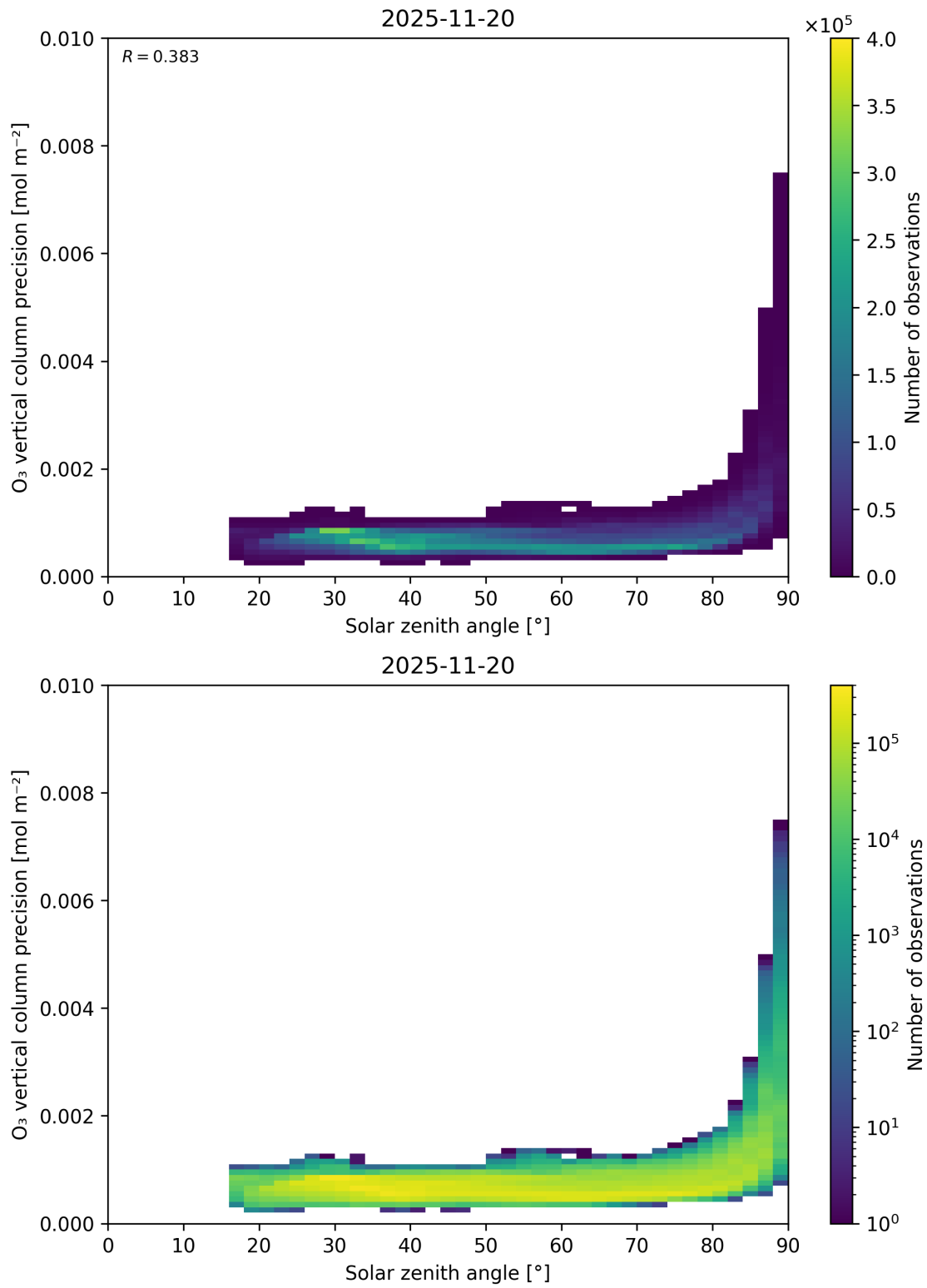
Figure 48: Scatter density plot of “Solar zenith angle” against “O 3 vertical column precision” for 2025-11-19 to 2025-11-21.
