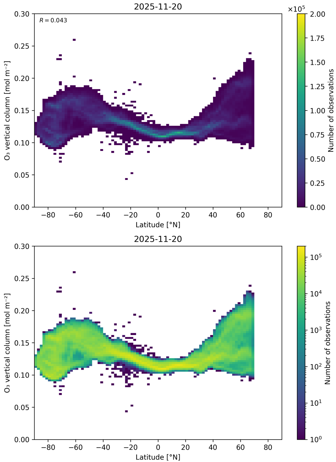
Figure 36: Scatter density plot of “Latitude” against “O 3 vertical column” for 2025-11-19 to 2025-11-21.
