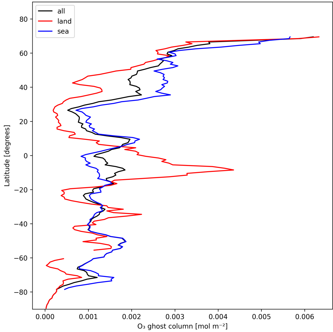
Figure 18: Zonal average of “O 3 ghost column” for 2025-11-19 to 2025-11-21.
