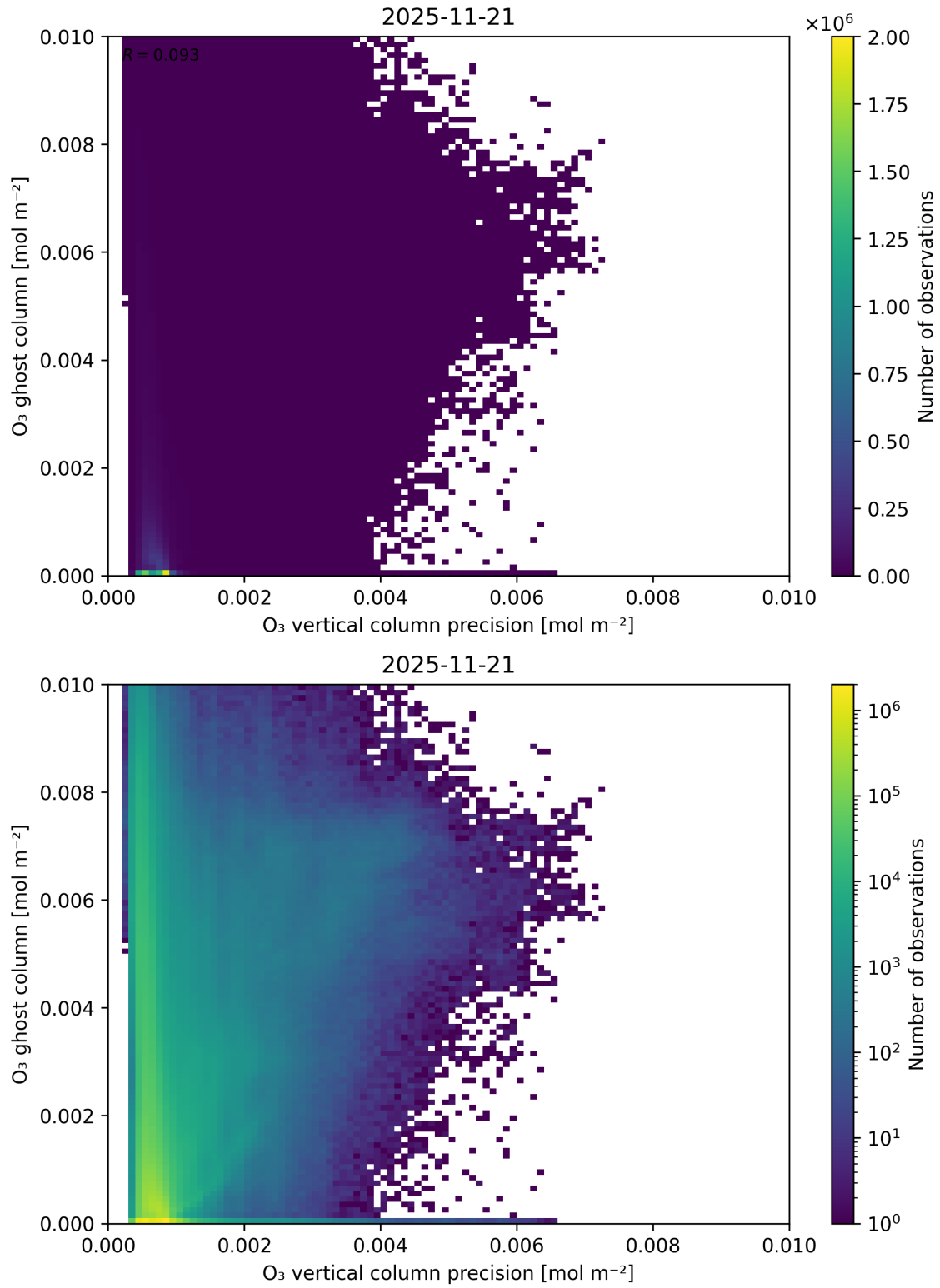
Figure 43: Scatter density plot of “O 3 vertical column precision” against “O 3 ghost column” for 2025-11-20 to 2025-11-22.
