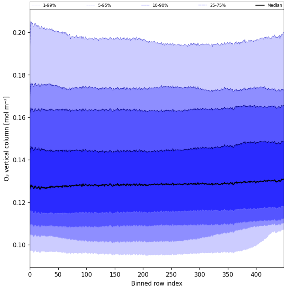
Figure 28: Along track statistics of “O 3 vertical column” for 2025-11-20 to 2025-11-22
