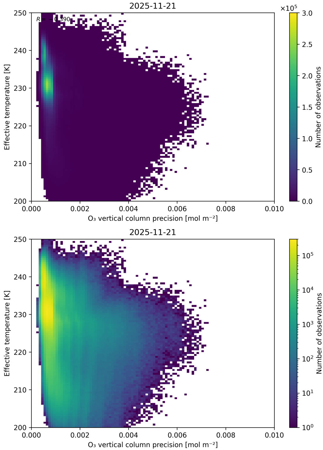
Figure 42: Scatter density plot of “ O_3 vertical column precision” against “Effective temperature” for 2025-11-20 to 2025-11-22.
