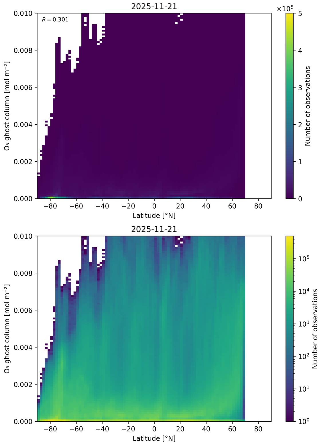
Figure 35: Scatter density plot of “Latitude” against “O 3 ghost column” for 2025-11-20 to 2025-11-22.
