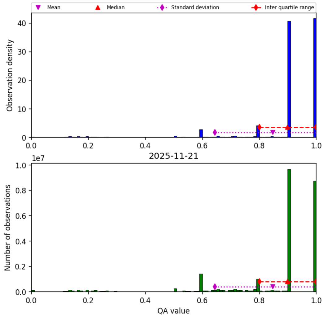
Figure 20: Histogram of “QA value” for 2025-11-20 to 2025-11-22
