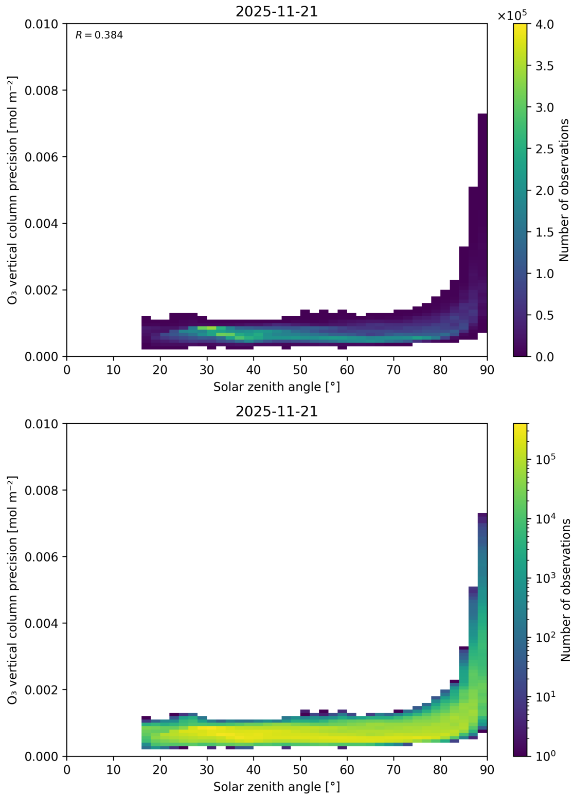
Figure 48: Scatter density plot of “Solar zenith angle” against “O 3 vertical column precision” for 2025-11-20 to 2025-11-22.
