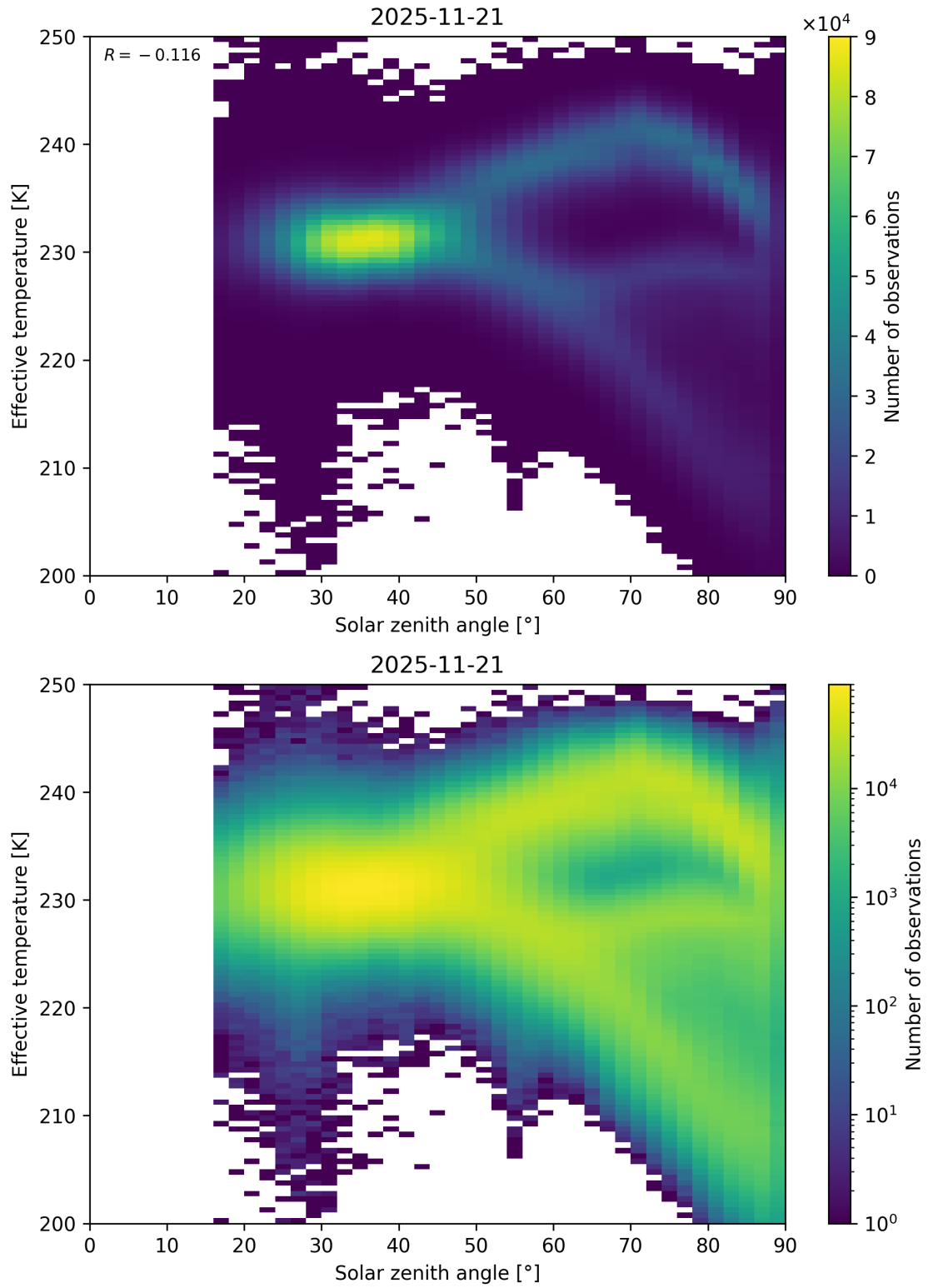
Figure 45: Scatter density plot of “Solar zenith angle” against “Effective temperature” for 2025-11-20 to 2025-11-22.
