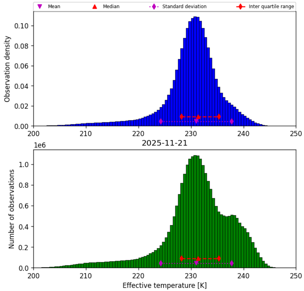
Figure 24: Histogram of “Effective temperature” for 2025-11-20 to 2025-11-22
