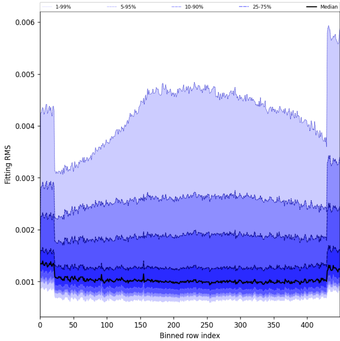
Figure 30: Along track statistics of “Fitting RMS” for 2025-11-20 to 2025-11-22
