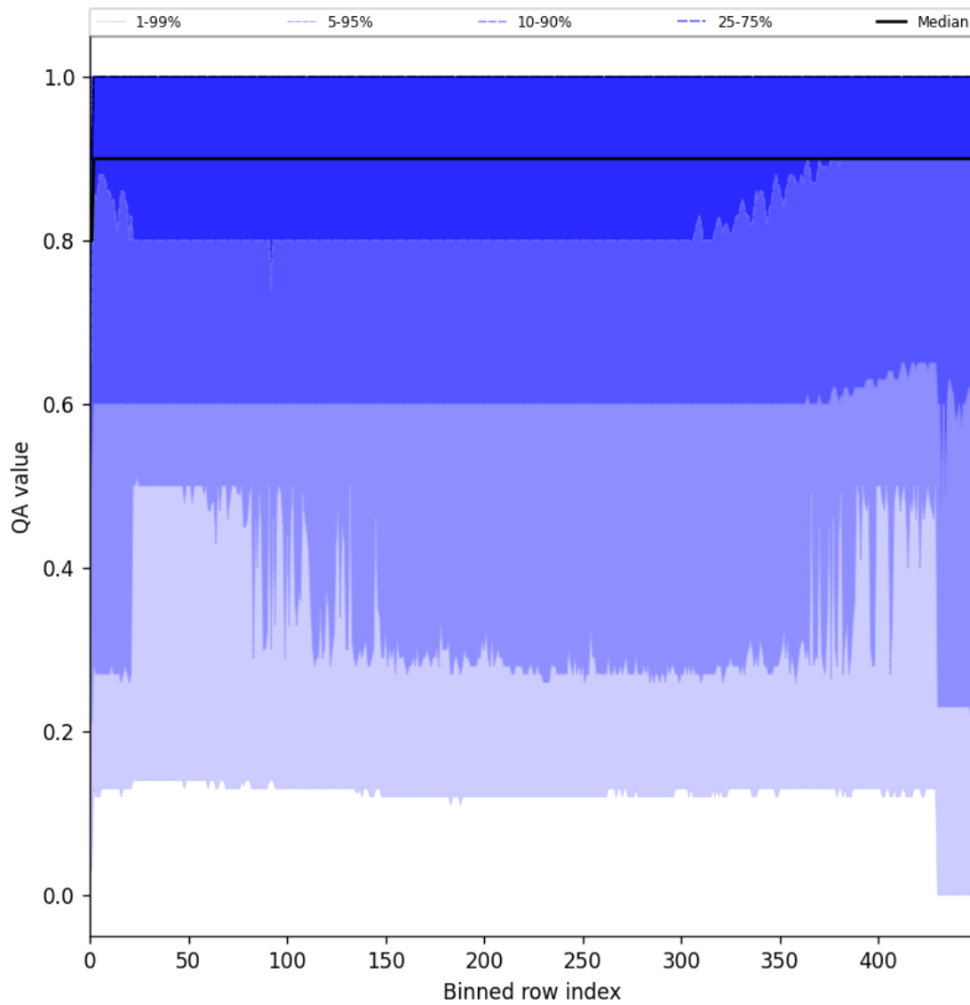
Figure 27: Along track statistics of “QA value” for 2025-11-20 to 2025-11-22
