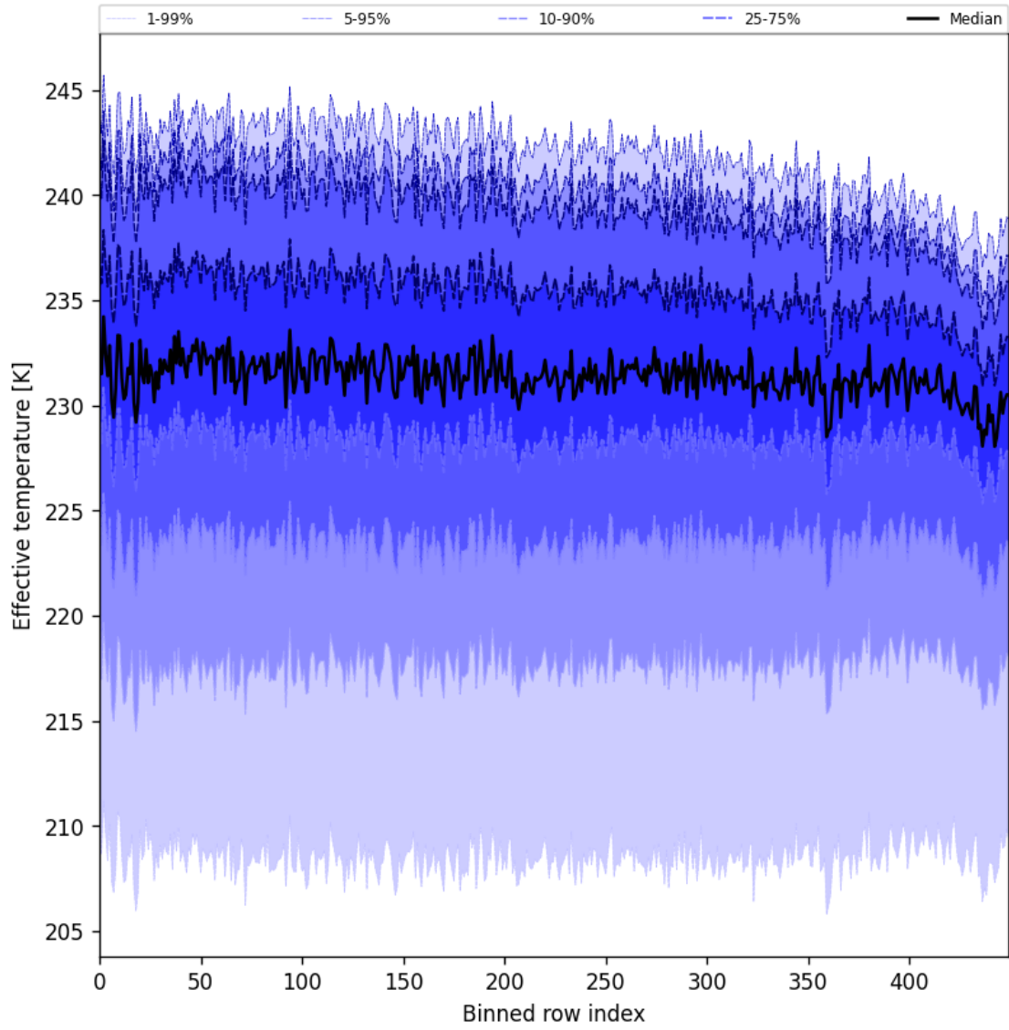
Figure 31: Along track statistics of "Effective temperature" for 2025-11-20 to 2025-11-22
