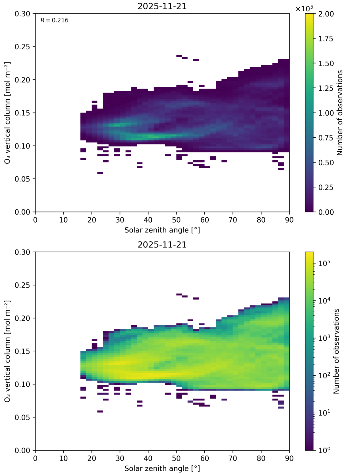
Figure 47: Scatter density plot of “Solar zenith angle” against “O 3 vertical column” for 2025-11-20 to 2025-11-22.
