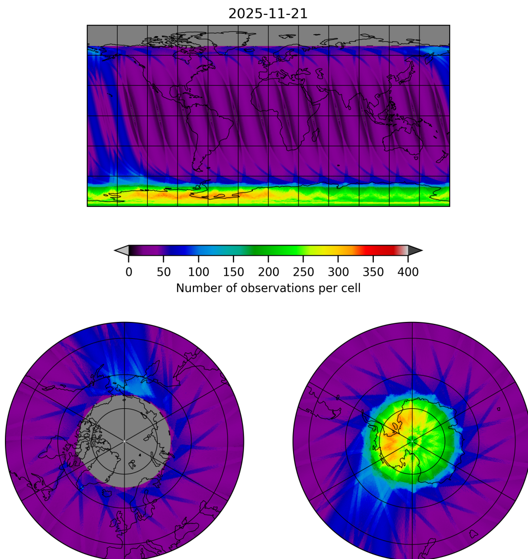
Figure 12: Map of the number of observations for 2025-11-20 to 2025-11-22
