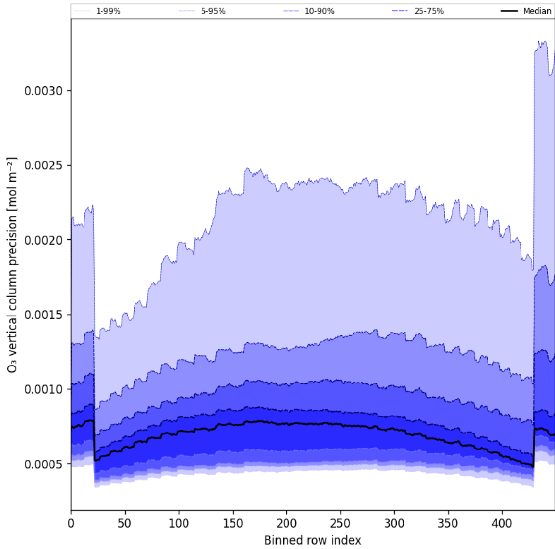
Figure 29: Along track statistics of “O 3 vertical column precision” for 2025-11-20 to 2025-11-22
