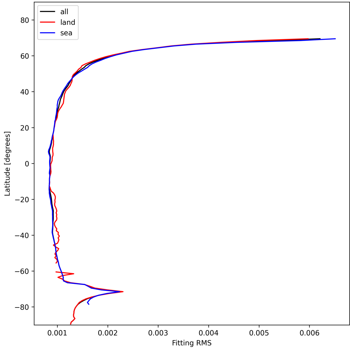
Figure 16: Zonal average of “Fitting RMS” for 2025-11-20 to 2025-11-22.
