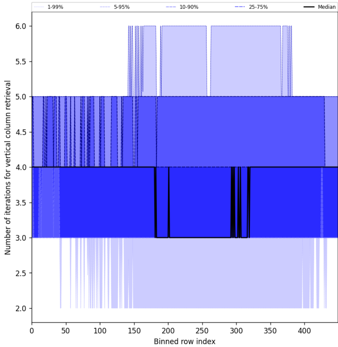
Figure 33: Along track statistics of “Number of iterations for vertical column retrieval” for 2025-11-20 to 2025-11-22
