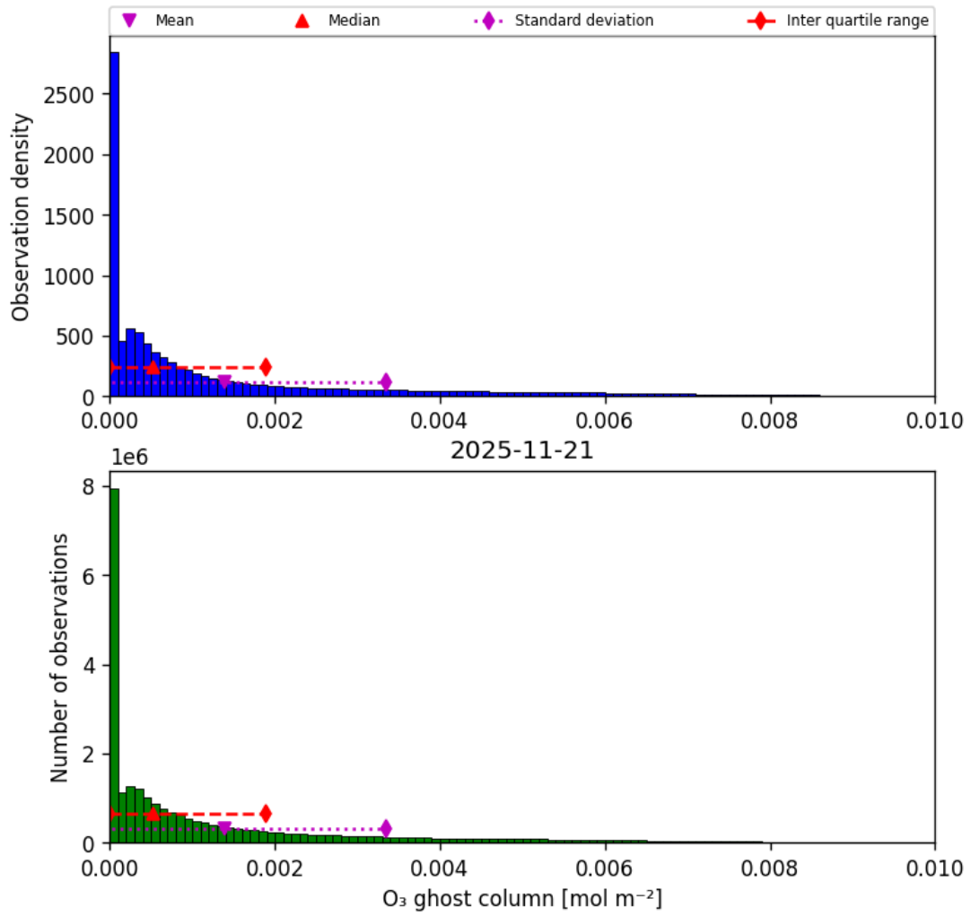
Figure 25: Histogram of “O 3 ghost column” for 2025-11-20 to 2025-11-22
