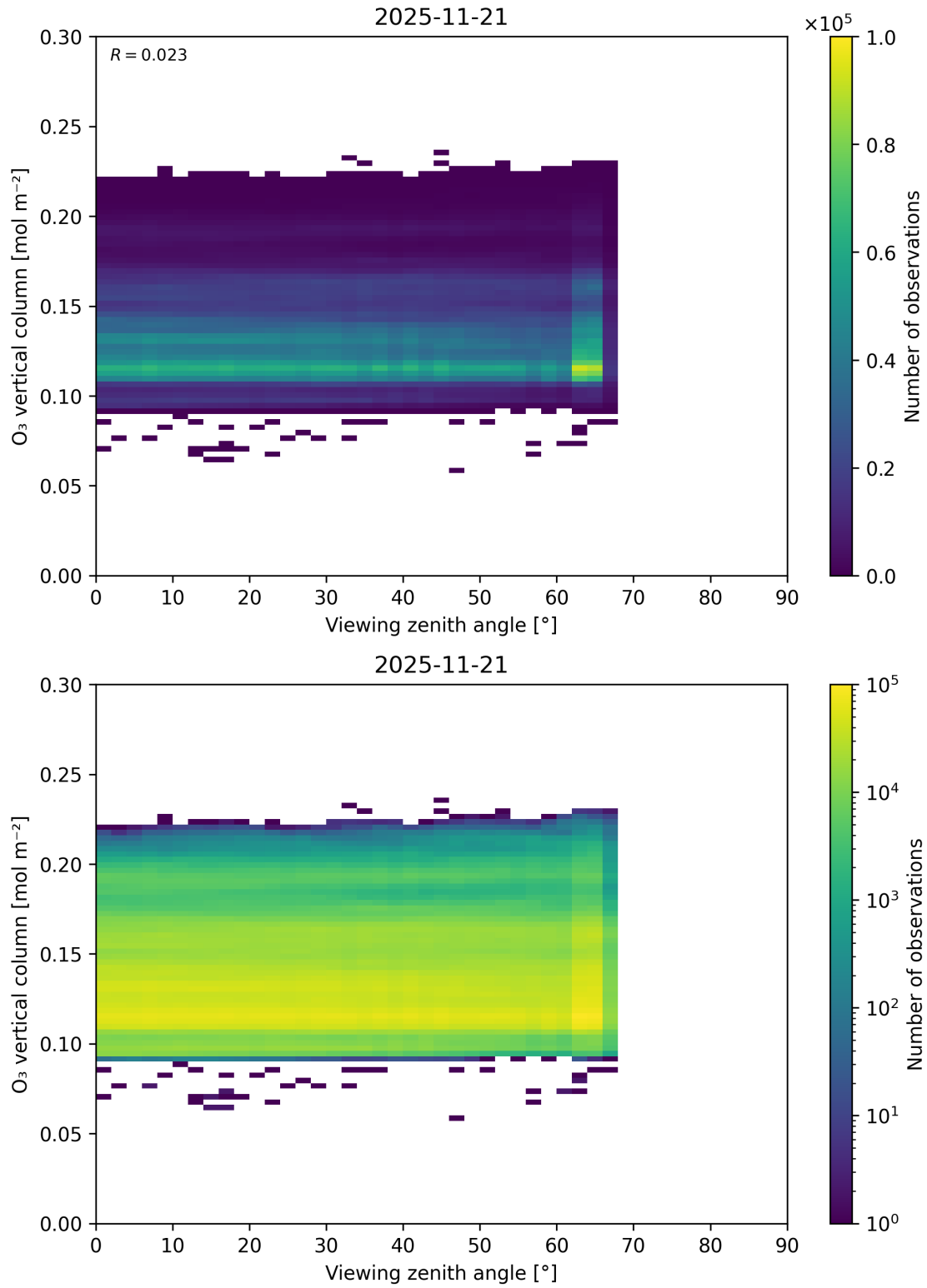
Figure 52: Scatter density plot of “Viewing zenith angle” against “O 3 vertical column” for 2025-11-20 to 2025-11-22.
