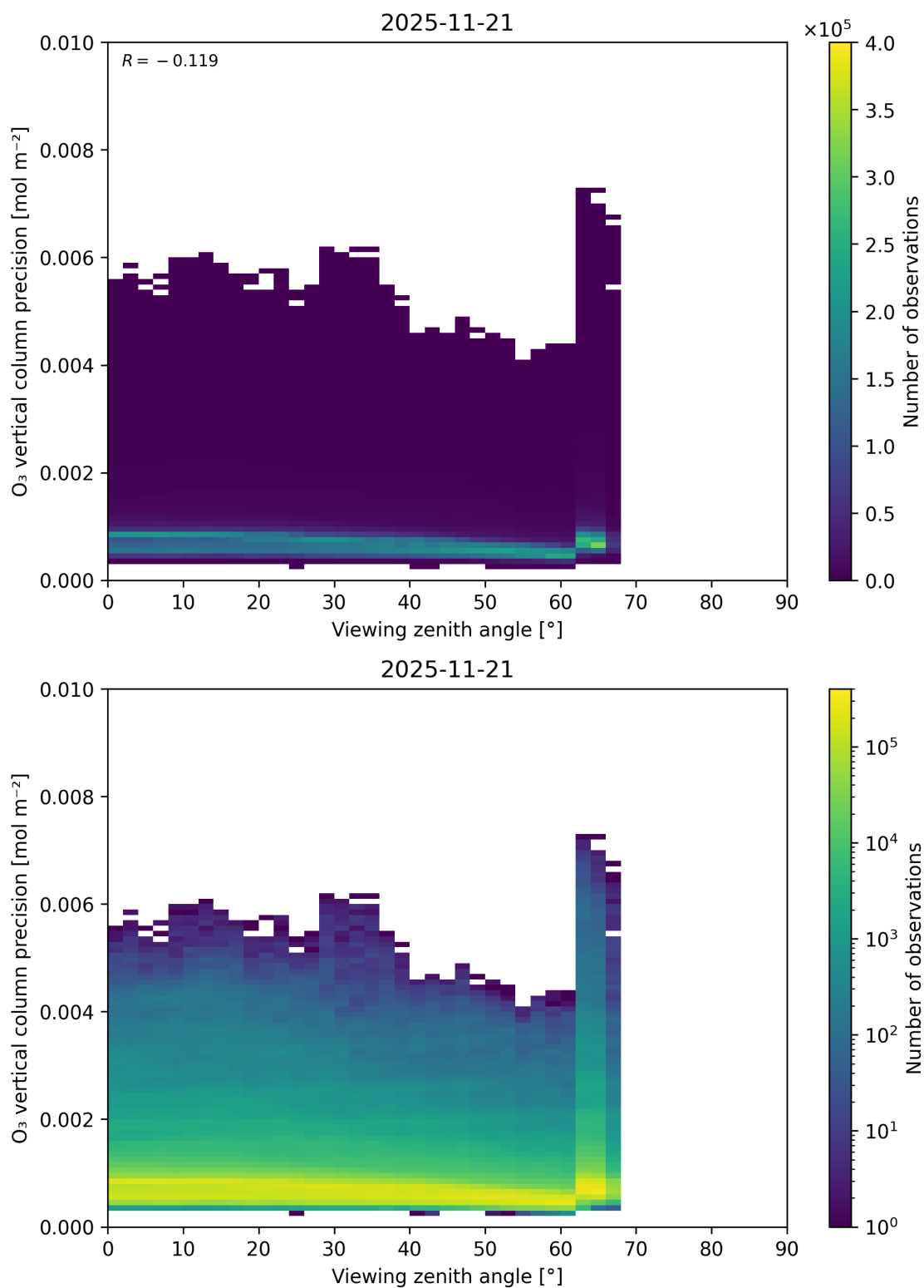
Figure 53: Scatter density plot of “Viewing zenith angle” against “O 3 vertical column precision” for 2025-11-20 to 2025-11-22.
