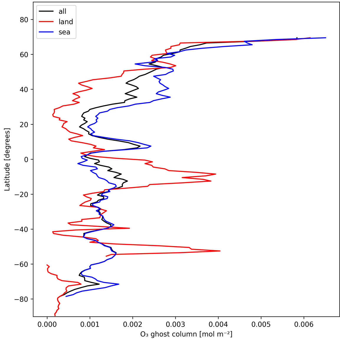
Figure 18: Zonal average of “O 3 ghost column” for 2025-11-20 to 2025-11-22.
