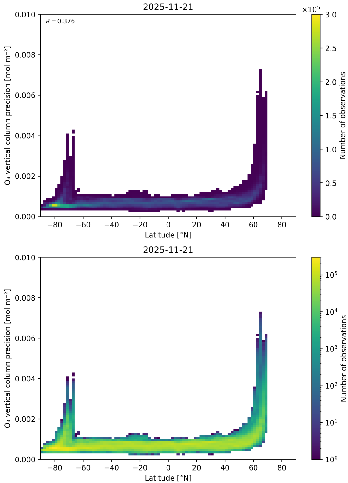
Figure 37: Scatter density plot of “Latitude” against “O 3 vertical column precision” for 2025-11-20 to 2025-11-22.
