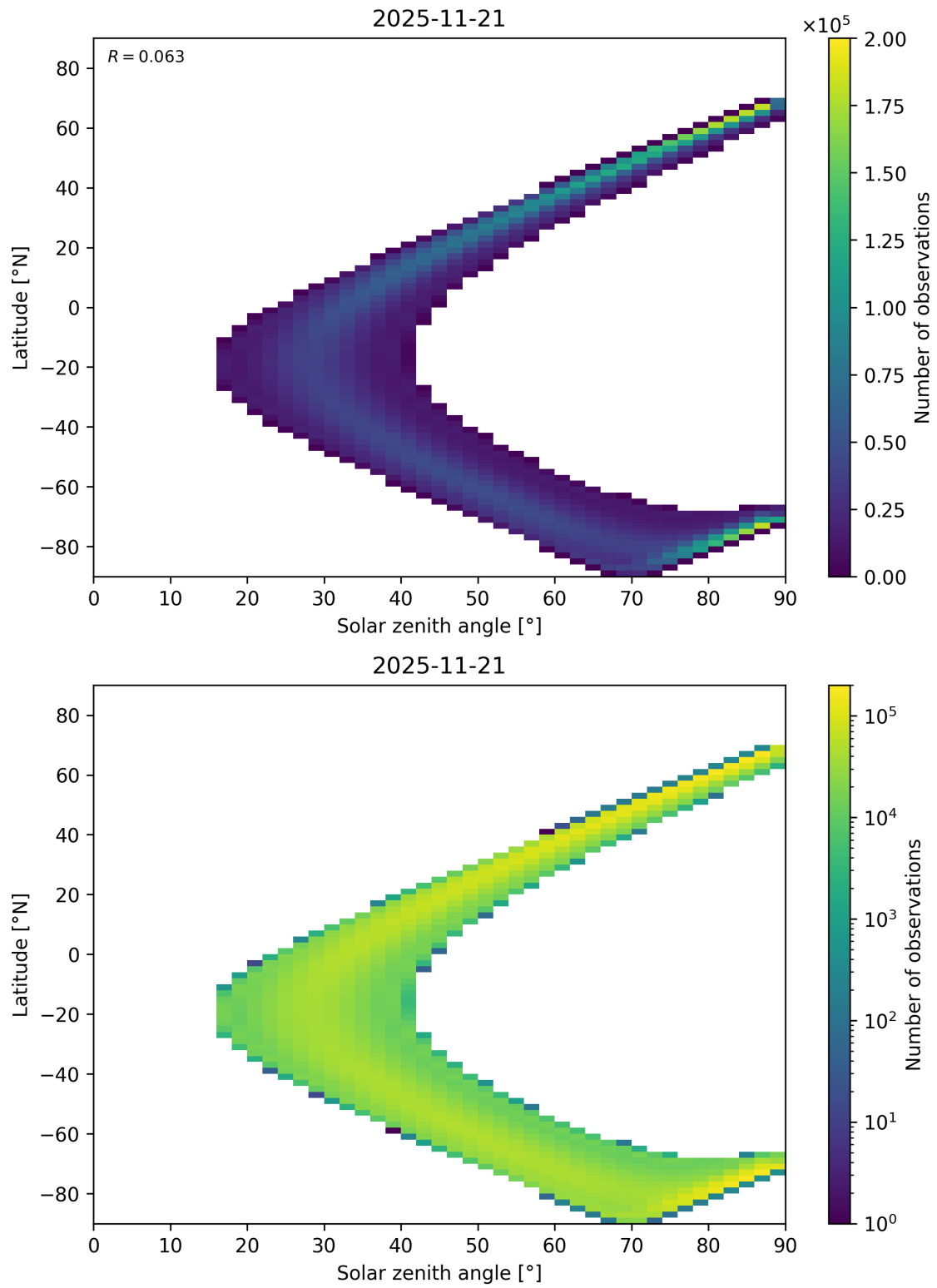
Figure 44: Scatter density plot of “Solar zenith angle” against “Latitude” for 2025-11-20 to 2025-11-22.
