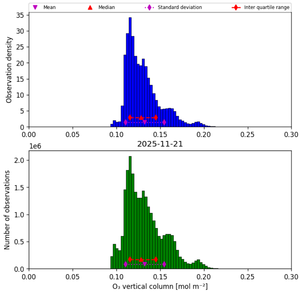
Figure 21: Histogram of “O 3 vertical column” for 2025-11-20 to 2025-11-22
