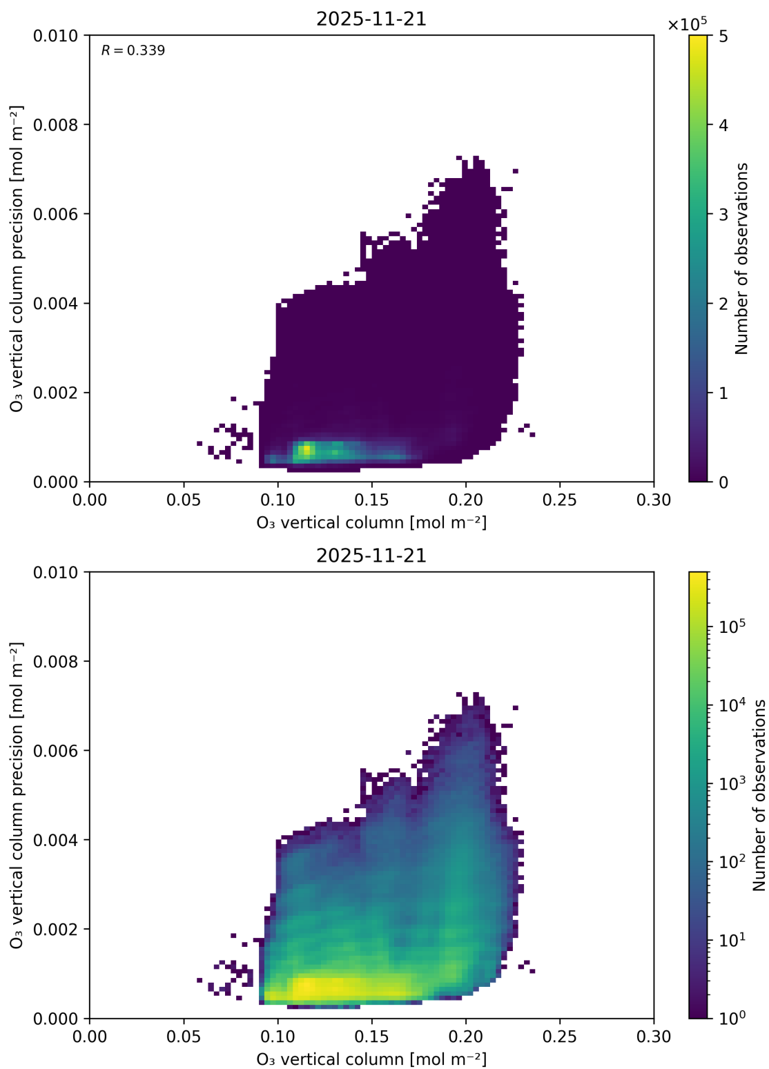
Figure 41: Scatter density plot of “O 3 vertical column” against “O 3 vertical column precision” for 2025-11-20 to 2025-11-22.
