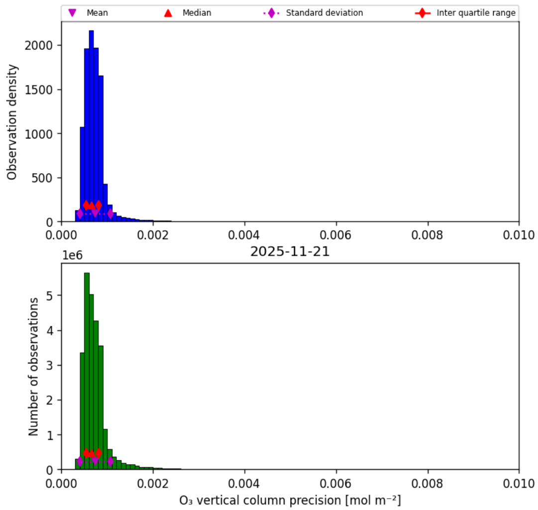
Figure 22: Histogram of “O 3 vertical column precision” for 2025-11-20 to 2025-11-22
