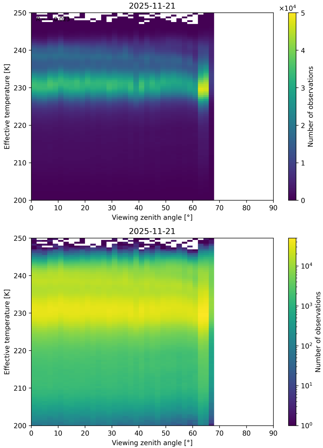
Figure 50: Scatter density plot of “Viewing zenith angle” against “Effective temperature” for 2025-11-20 to 2025-11-22.
