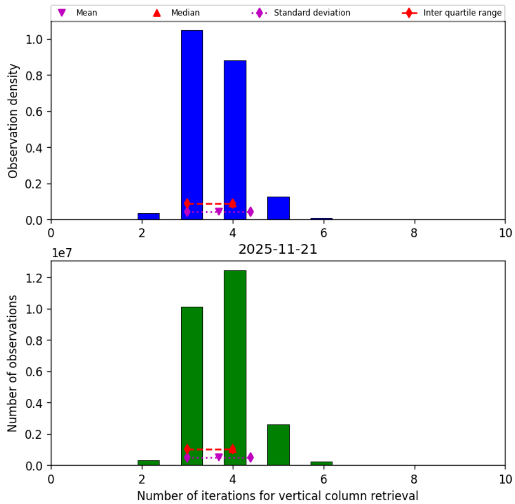
Figure 26: Histogram of “Number of iterations for vertical column retrieval” for 2025-11-20 to 2025-11-22
