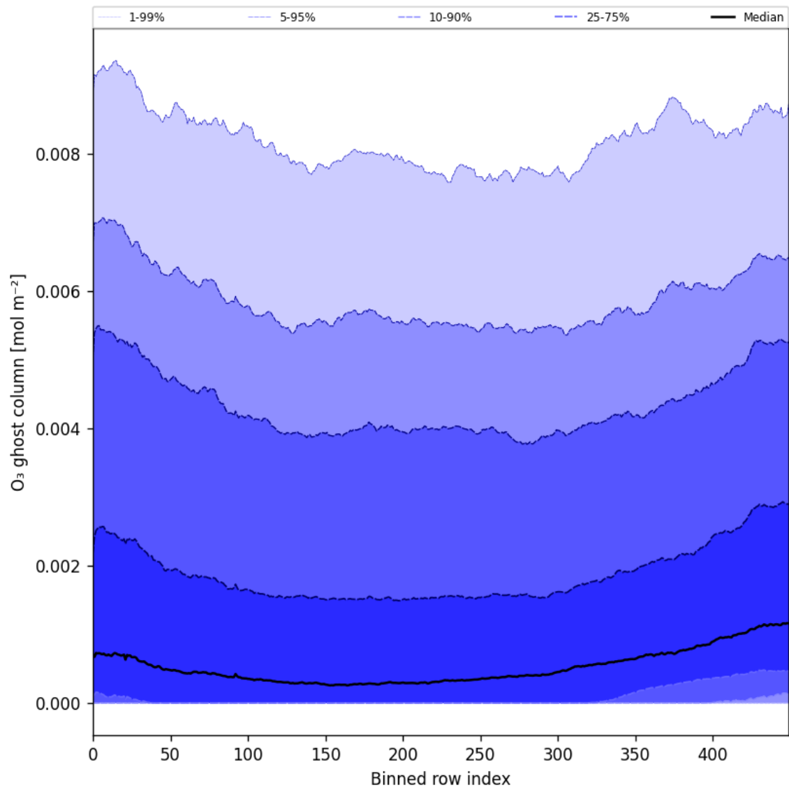
Figure 32: Along track statistics of “O 3 ghost column” for 2025-11-20 to 2025-11-22
