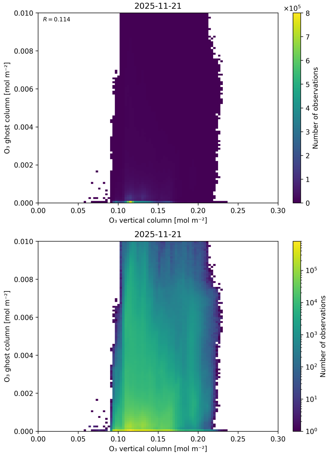
Figure 40: Scatter density plot of “O 3 vertical column” against “O 3 ghost column” for 2025-11-20 to 2025-11-22.
