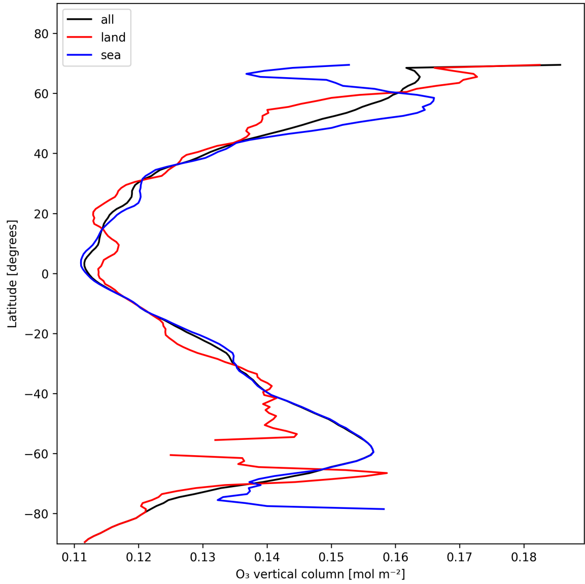
Figure 14: Zonal average of “O 3 vertical column” for 2025-11-20 to 2025-11-22.
