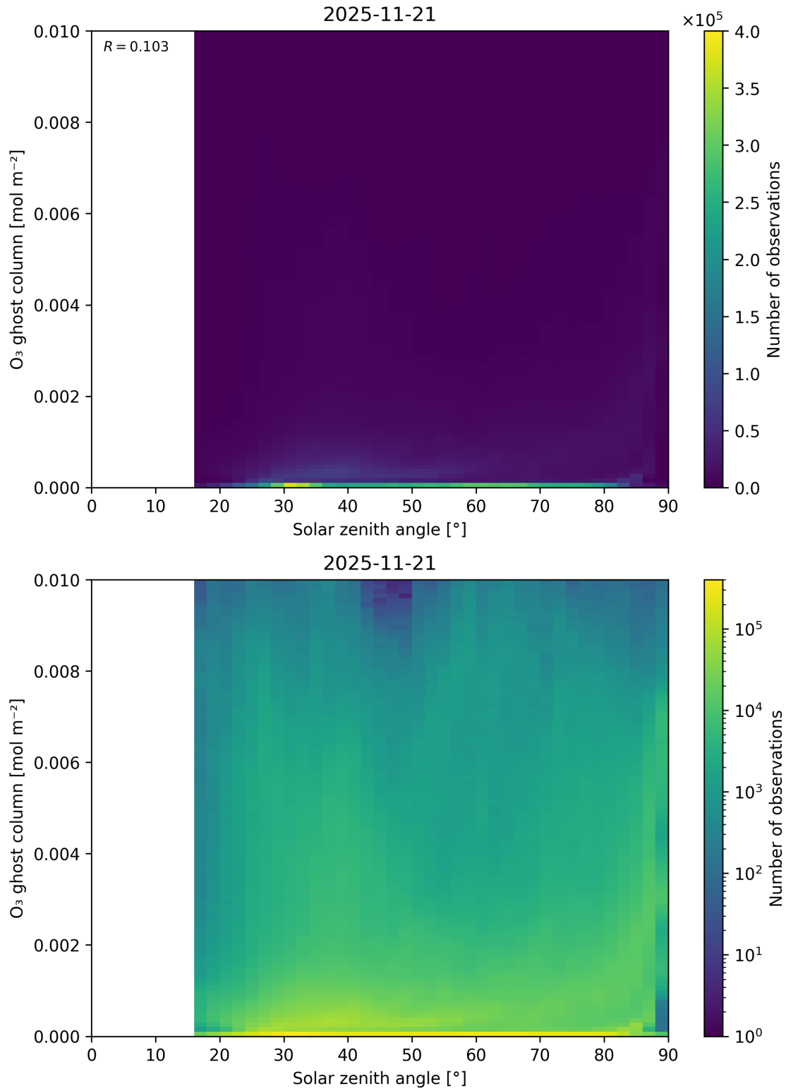
Figure 46: Scatter density plot of “Solar zenith angle” against “O 3 ghost column” for 2025-11-20 to 2025-11-22.
