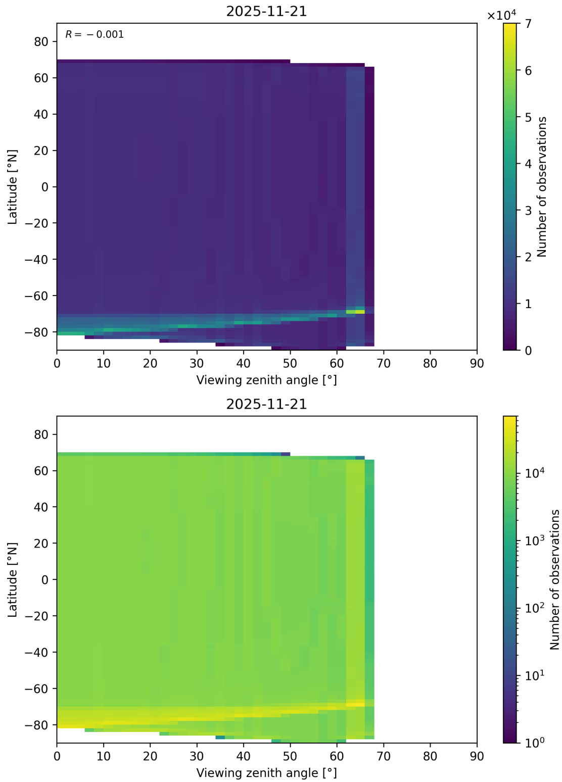
Figure 49: Scatter density plot of “Viewing zenith angle” against “Latitude” for 2025-11-20 to 2025-11-22.
