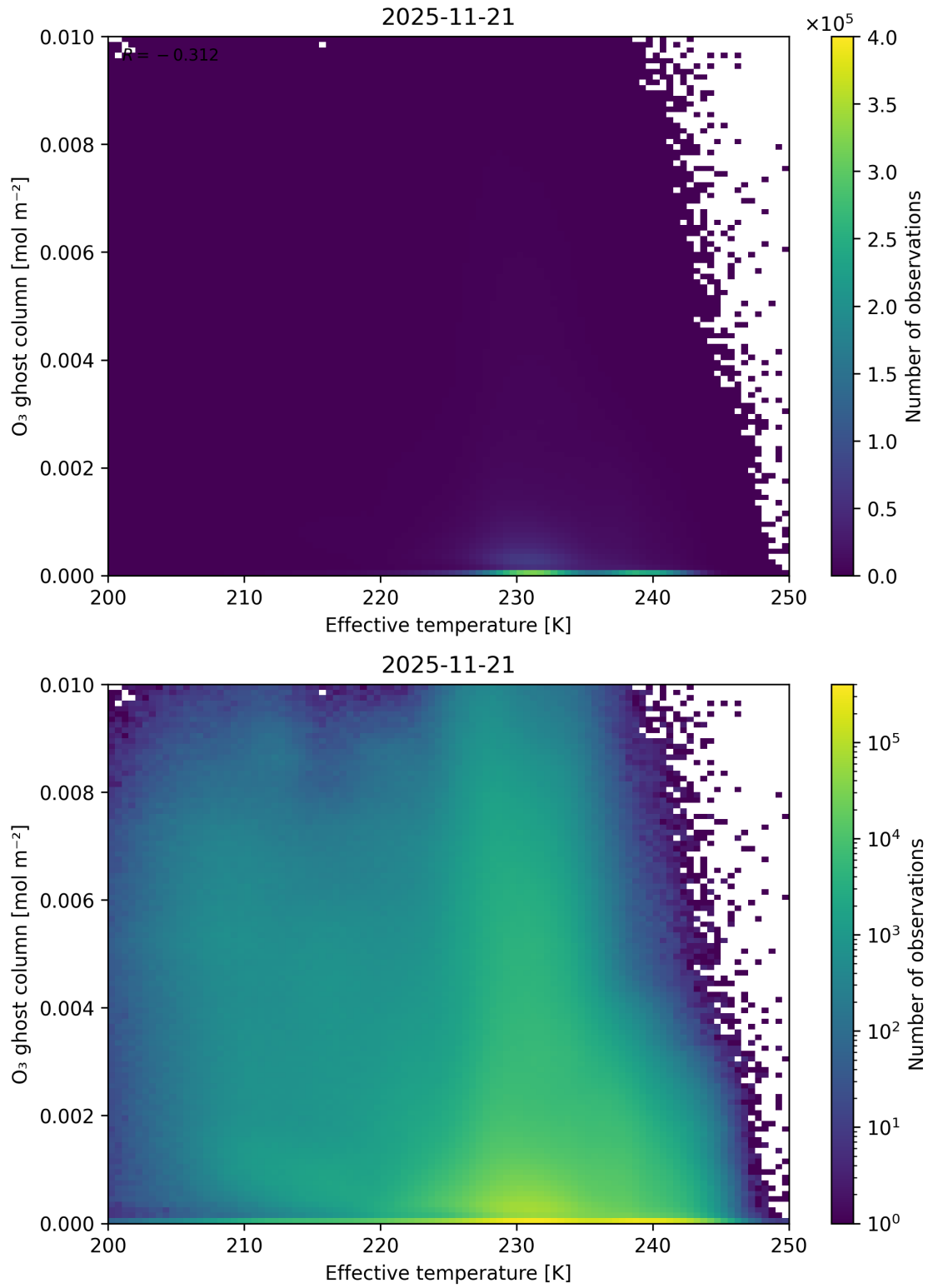
Figure 38: Scatter density plot of “Effective temperature” against “O 3 ghost column” for 2025-11-20 to 2025-11-22.
