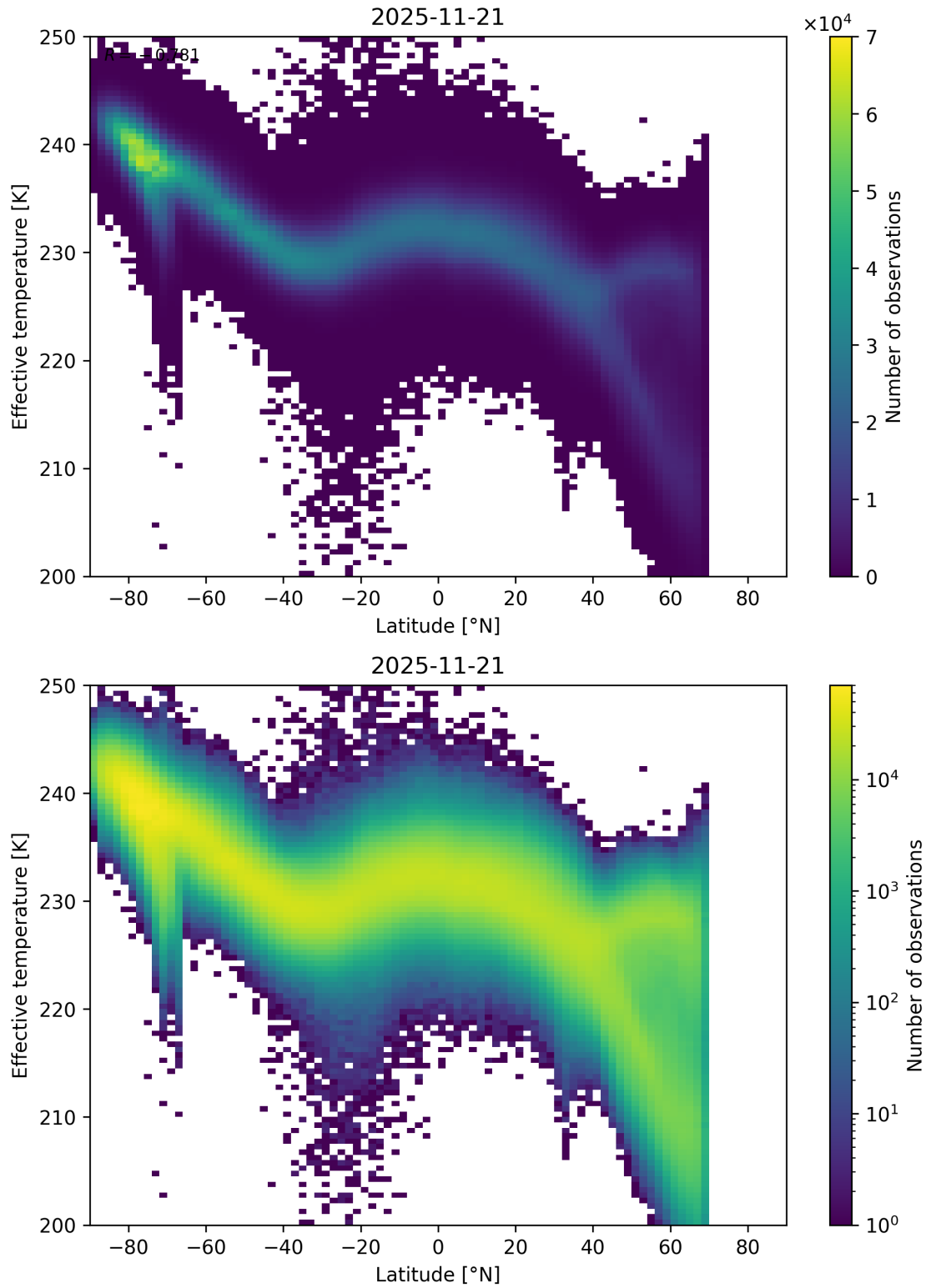
Figure 34: Scatter density plot of “Latitude” against “Effective temperature” for 2025-11-20 to 2025-11-22.
