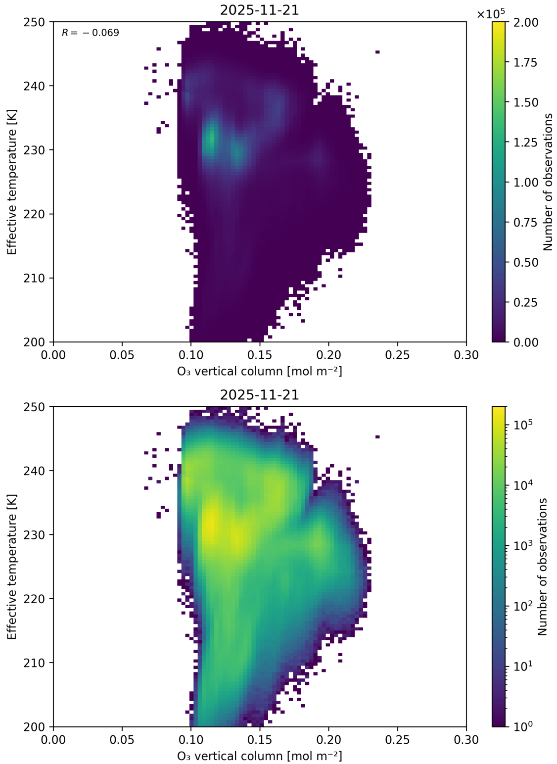
Figure 39: Scatter density plot of “O 3 vertical column” against “Effective temperature” for 2025-11-20 to 2025-11-22.
