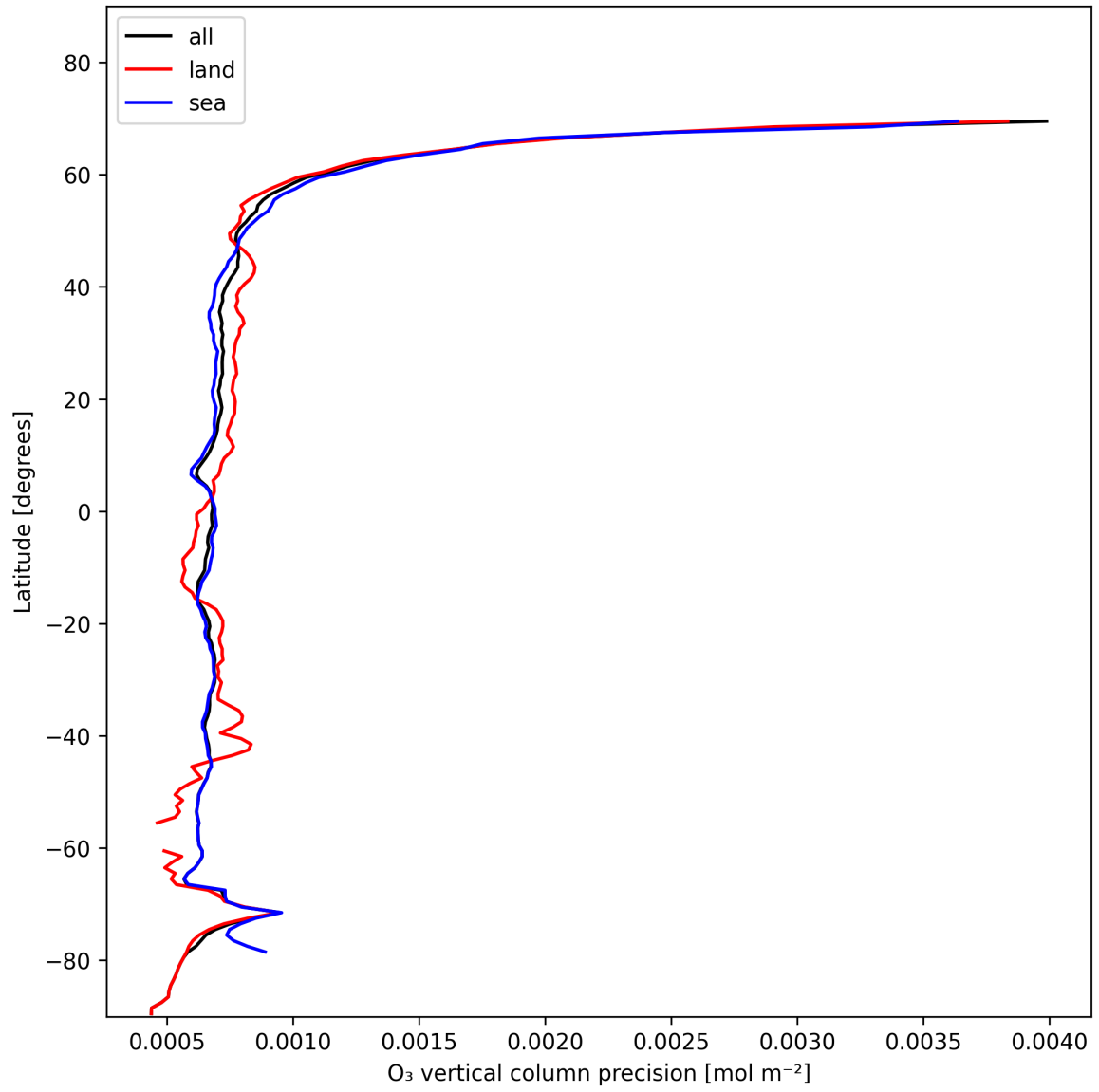
Figure 15: Zonal average of “O 3 vertical column precision” for 2025-11-20 to 2025-11-22.
