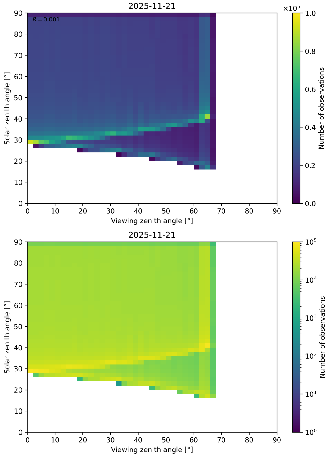
Figure 54: Scatter density plot of “Viewing zenith angle” against “Solar zenith angle” for 2025-11-20 to 2025-11-22.
