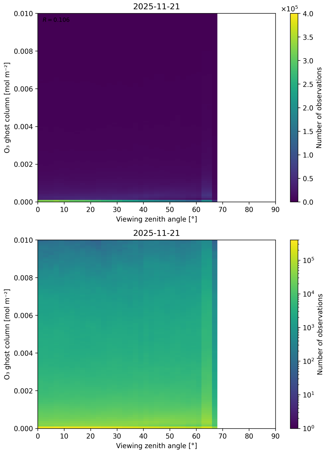
Figure 51: Scatter density plot of “Viewing zenith angle” against “O 3 ghost column” for 2025-11-20 to 2025-11-22.
