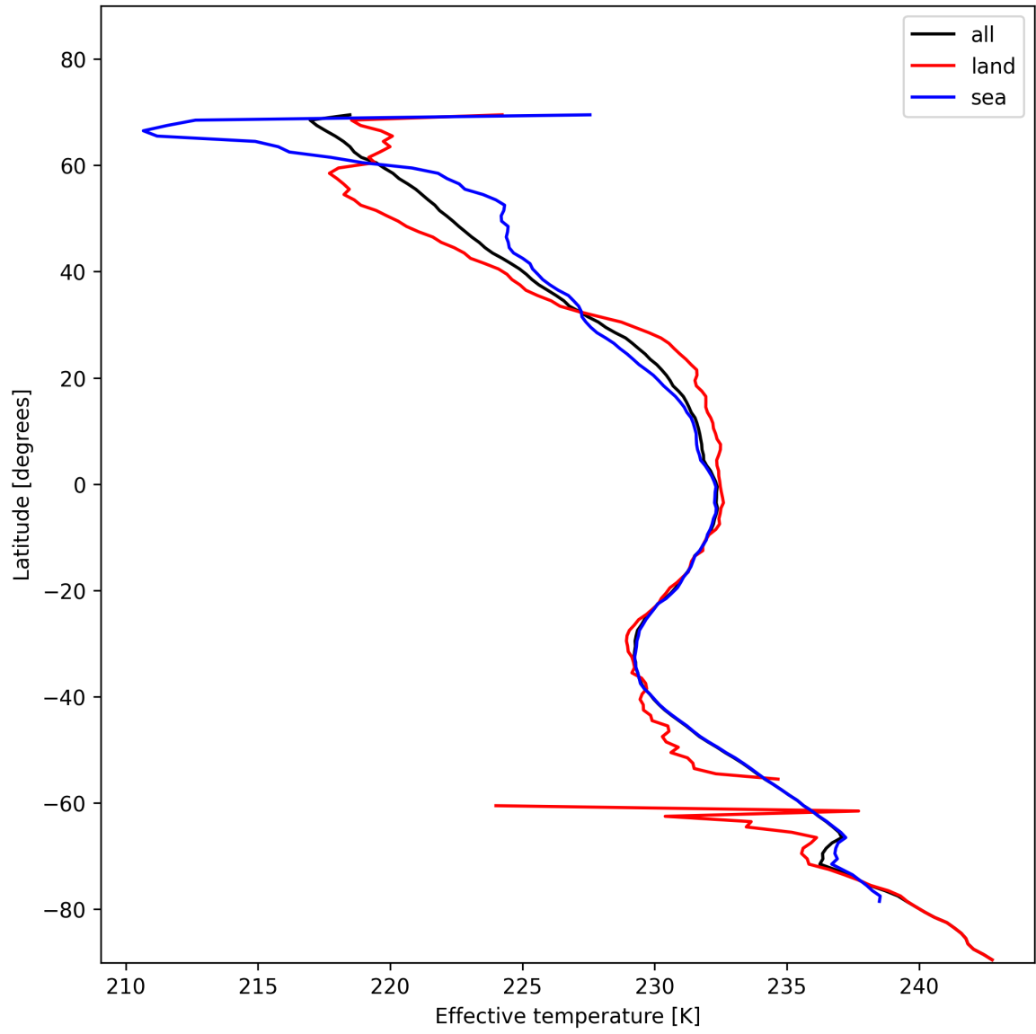
Figure 17: Zonal average of "Effective temperature" for 2025-11-20 to 2025-11-22.
