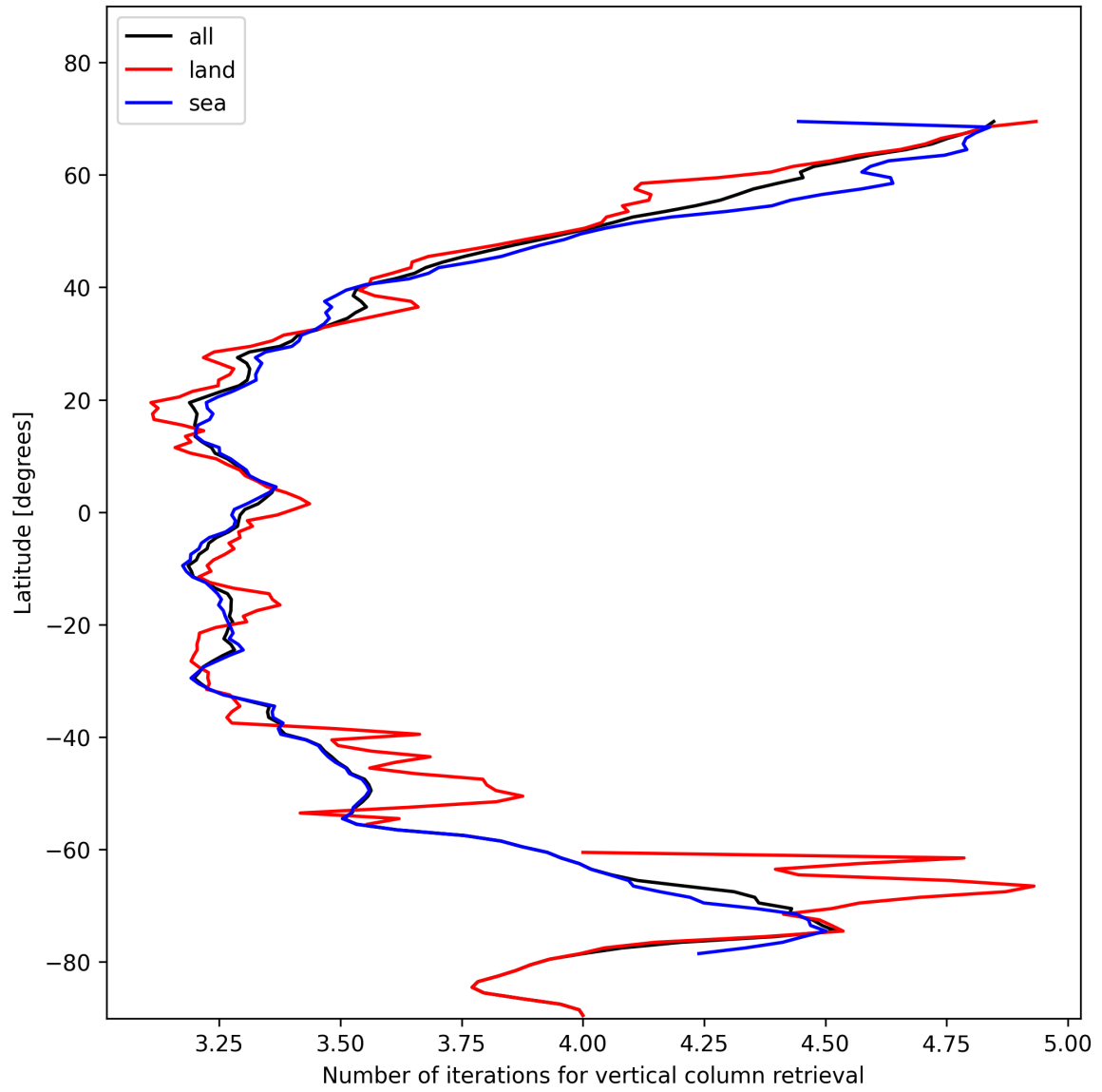
Figure 19: Zonal average of “Number of iterations for vertical column retrieval” for 2025-11-20 to 2025-11-22.
