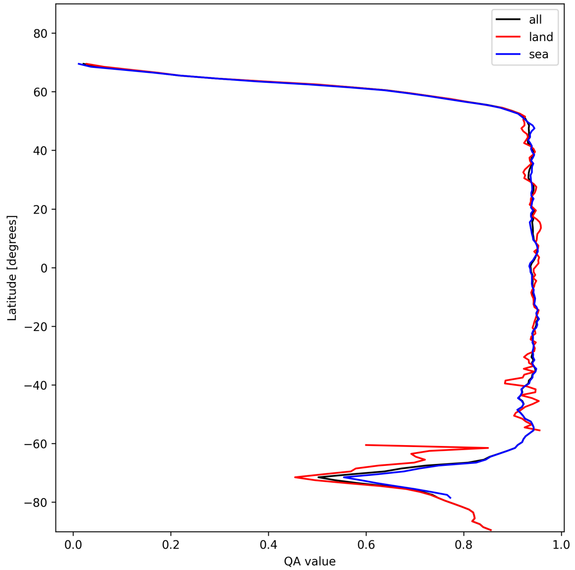
Figure 13: Zonal average of “QA value” for 2025-11-20 to 2025-11-22.
