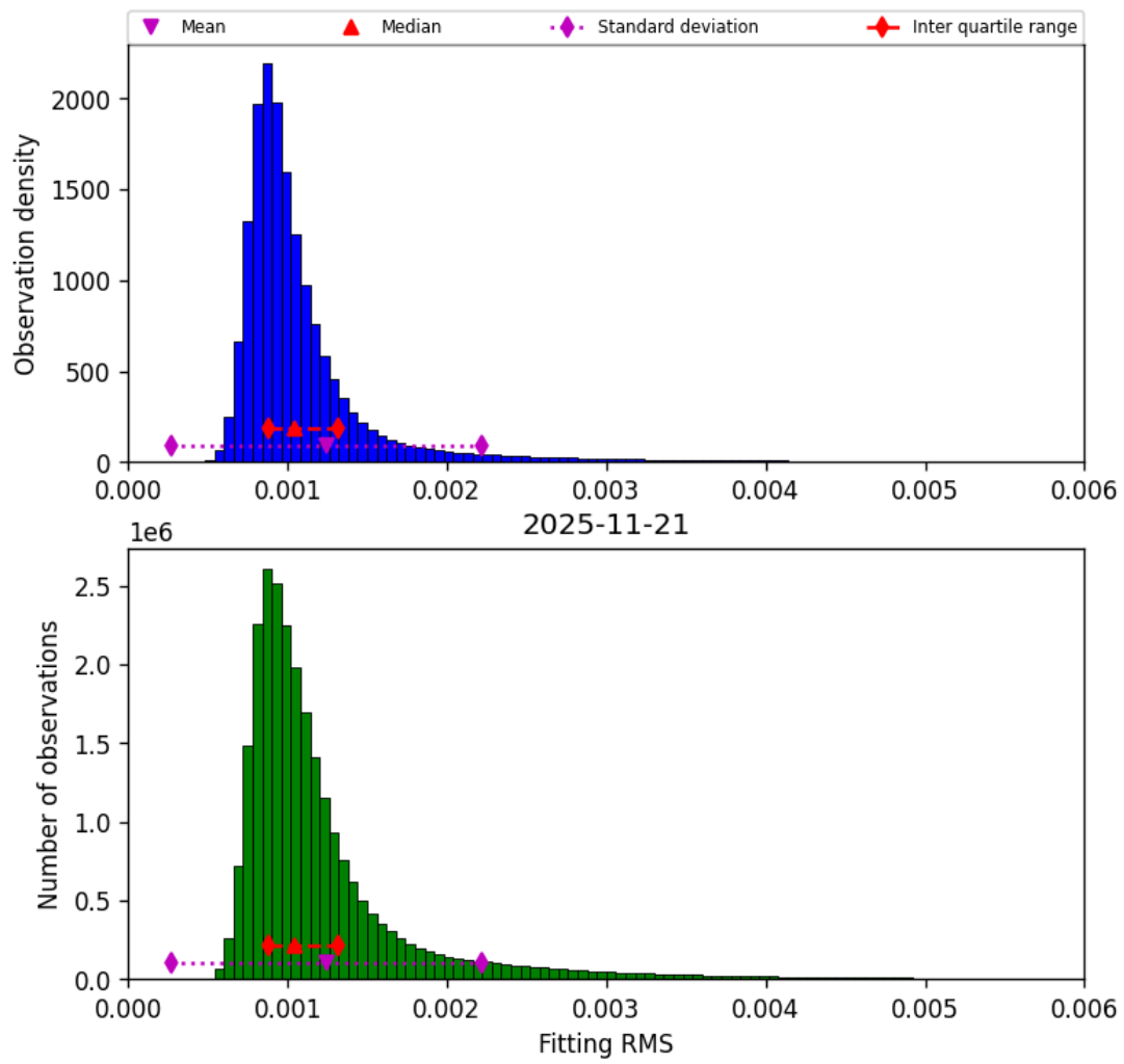
Figure 23: Histogram of “Fitting RMS” for 2025-11-20 to 2025-11-22
