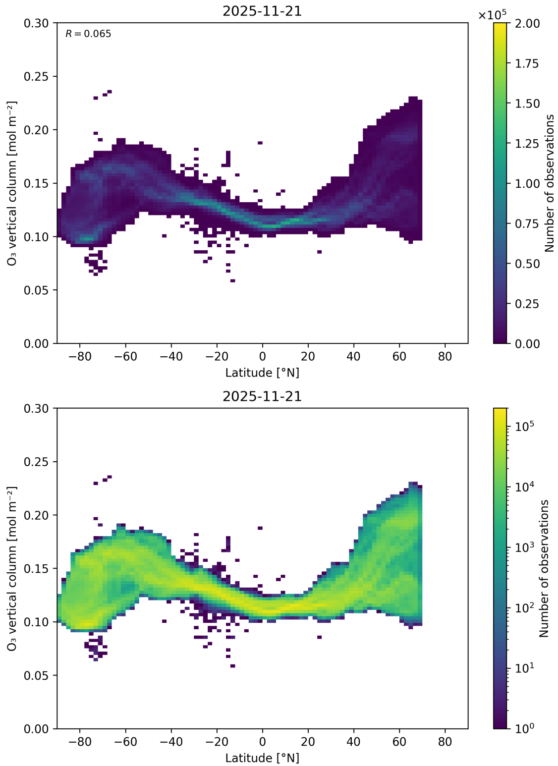
Figure 36: Scatter density plot of “Latitude” against “O 3 vertical column” for 2025-11-20 to 2025-11-22.
