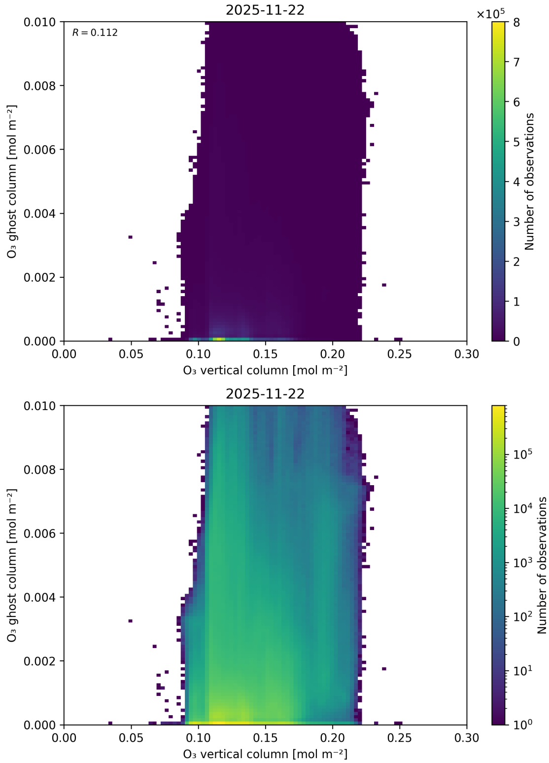
Figure 40: Scatter density plot of “O 3 vertical column” against “O 3 ghost column” for 2025-11-21 to 2025-11-23.
