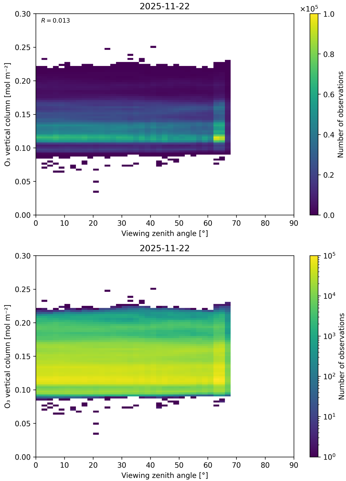
Figure 52: Scatter density plot of “Viewing zenith angle” against “O 3 vertical column” for 2025-11-21 to 2025-11-23.
