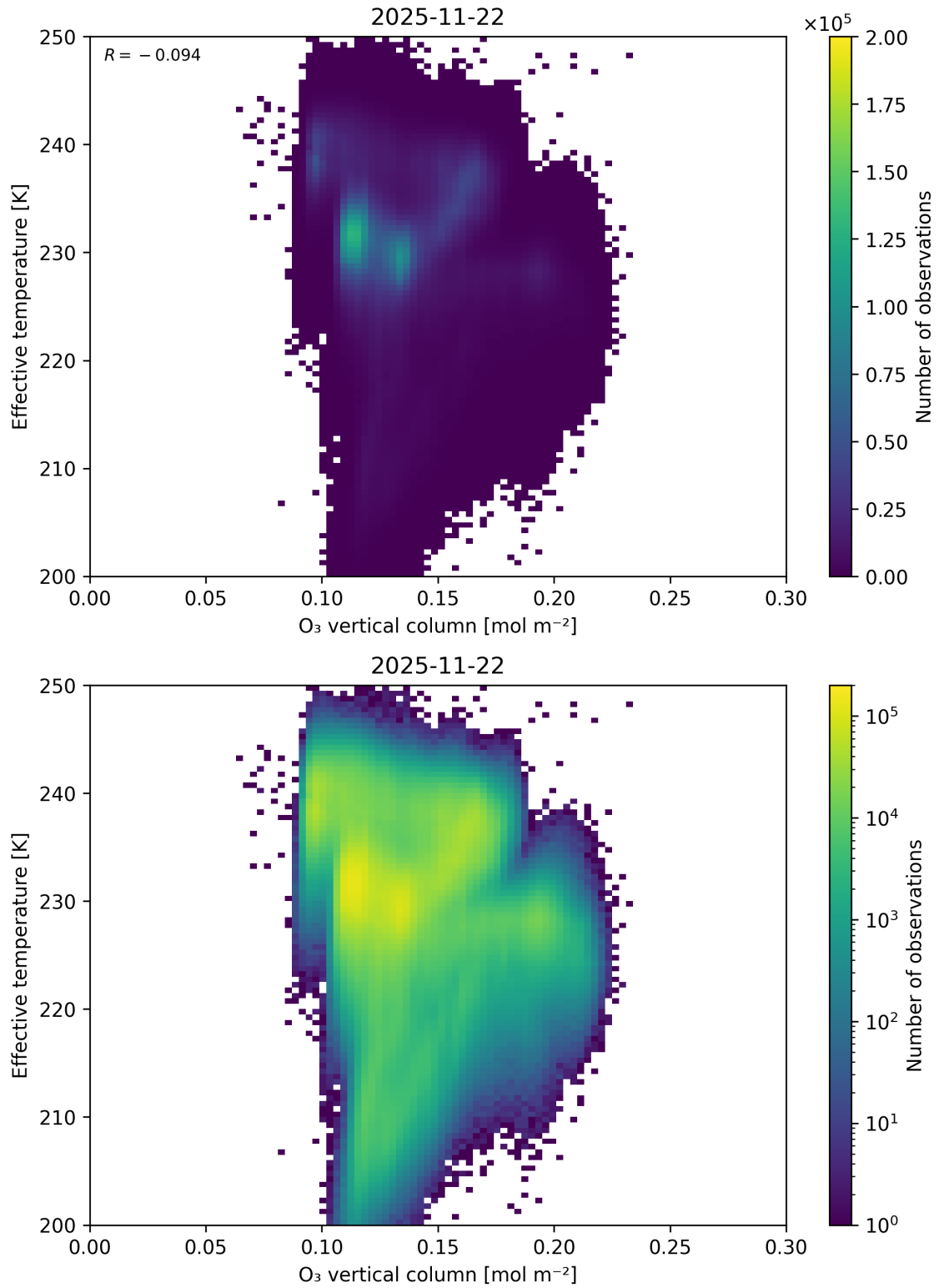
Figure 39: Scatter density plot of “O 3 vertical column” against “Effective temperature” for 2025-11-21 to 2025-11-23.
