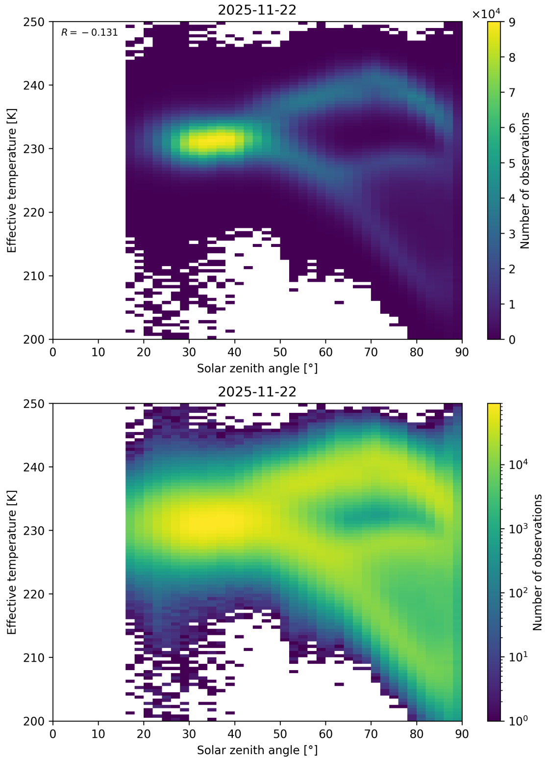
Figure 45: Scatter density plot of “Solar zenith angle” against “Effective temperature” for 2025-11-21 to 2025-11-23.
