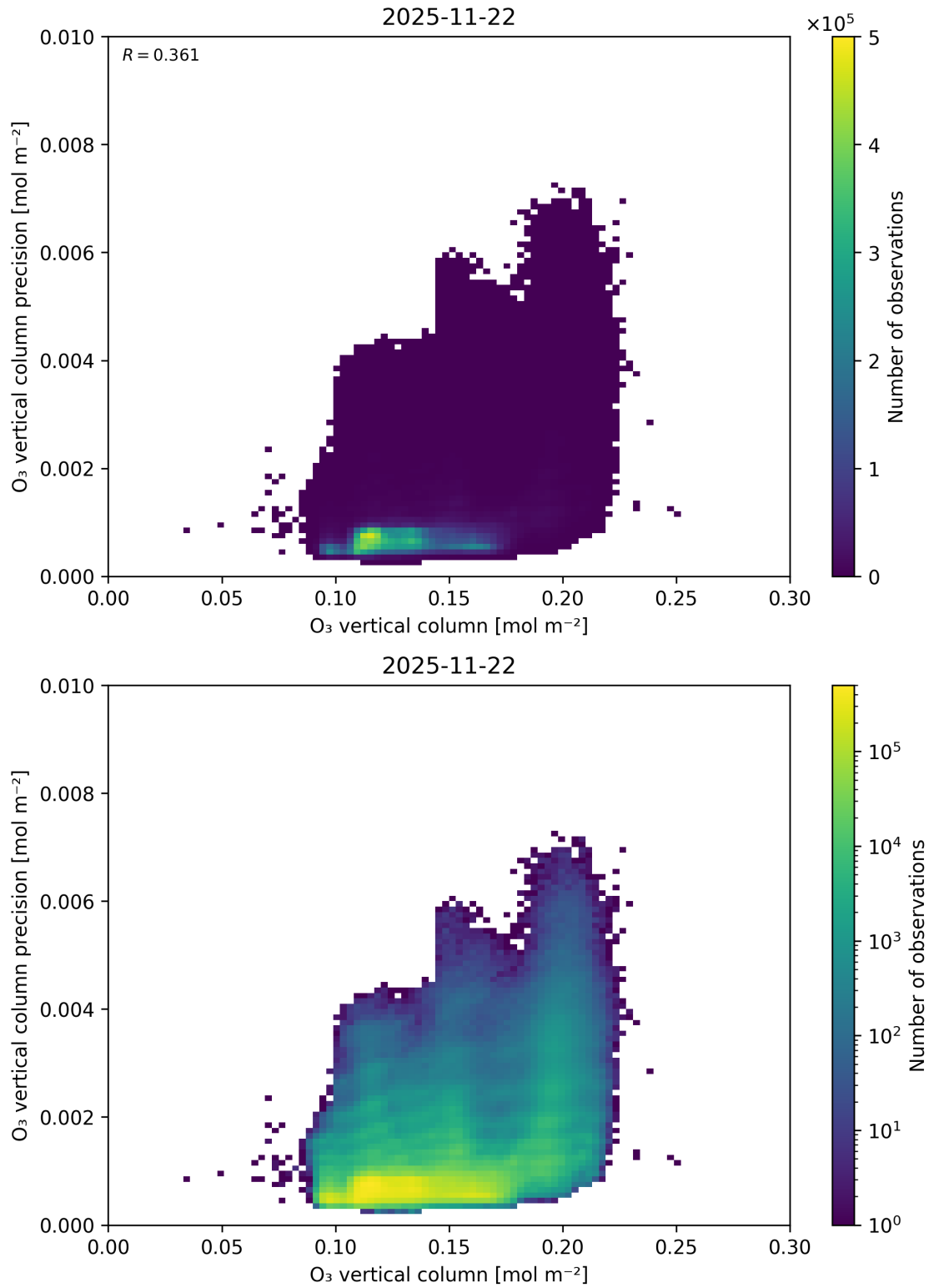
Figure 41: Scatter density plot of “O 3 vertical column” against “O 3 vertical column precision” for 2025-11-21 to 2025-11-23.
