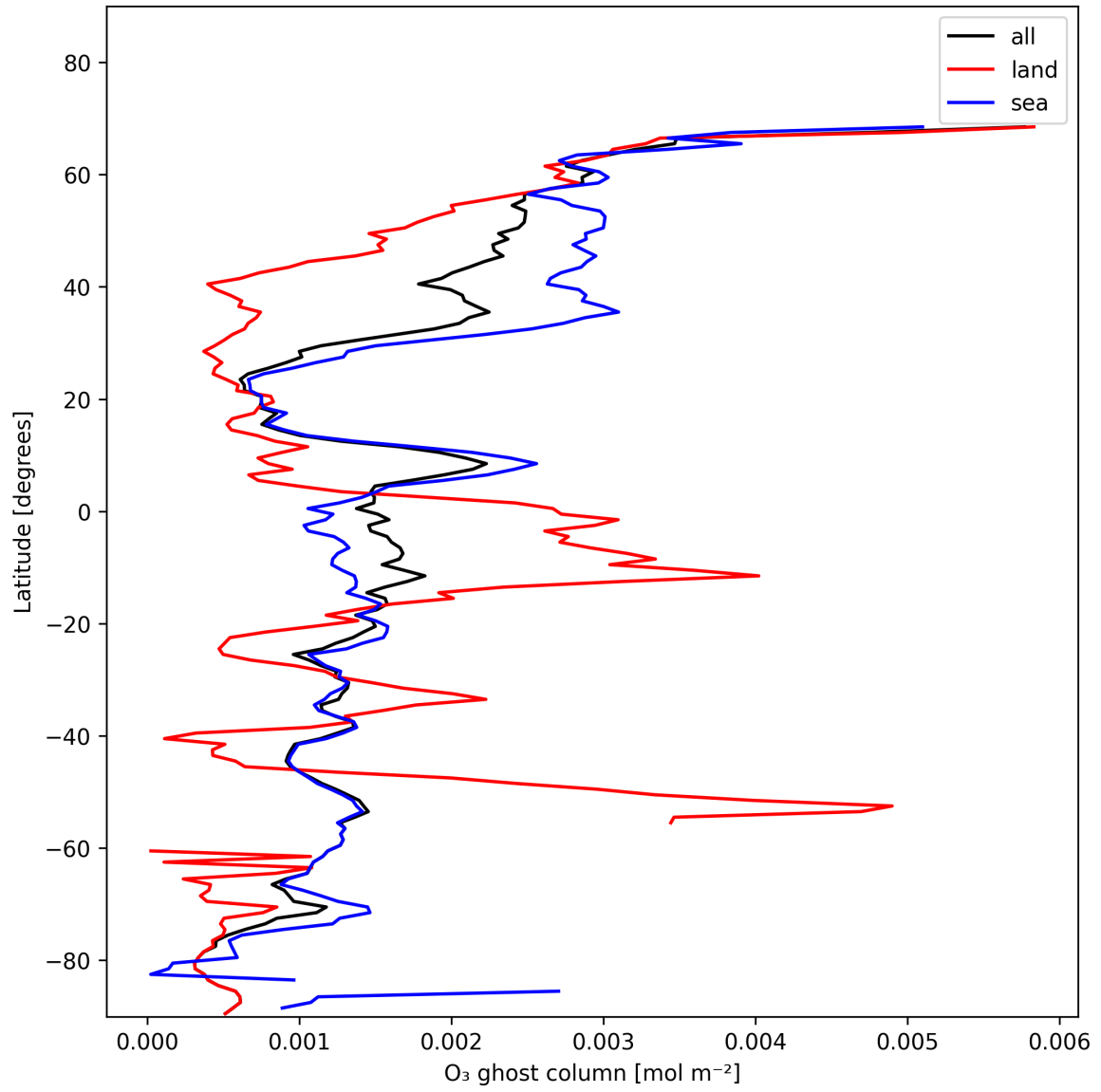
Figure 18: Zonal average of “O 3 ghost column” for 2025-11-21 to 2025-11-23.
