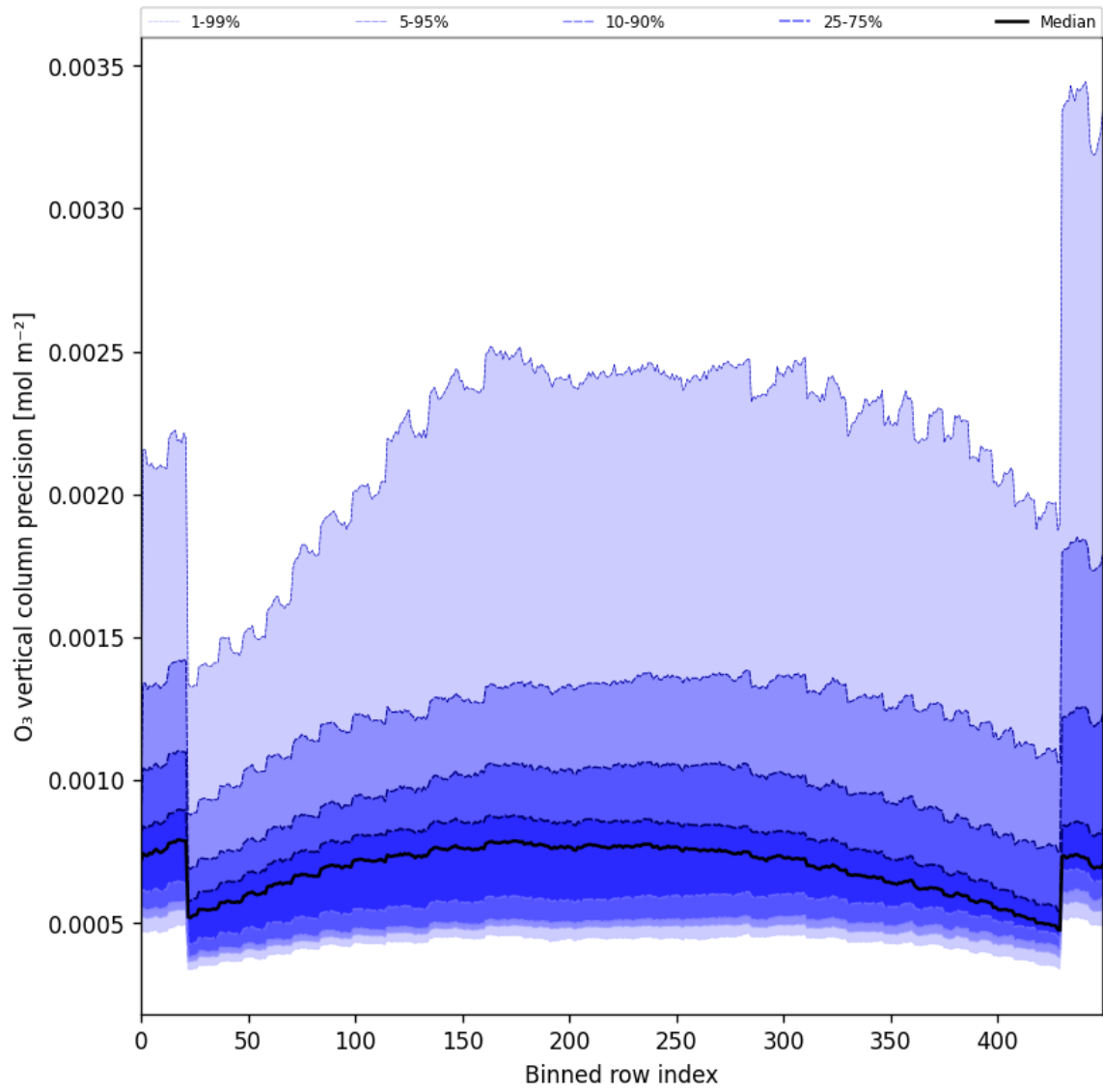
Figure 29: Along track statistics of “O 3 vertical column precision” for 2025-11-21 to 2025-11-23
