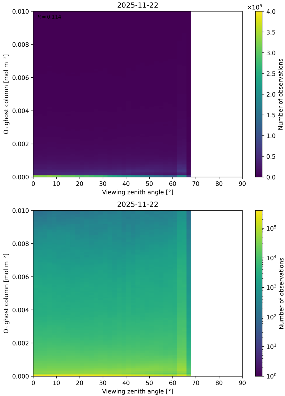
Figure 51: Scatter density plot of “Viewing zenith angle” against “O 3 ghost column” for 2025-11-21 to 2025-11-23.
