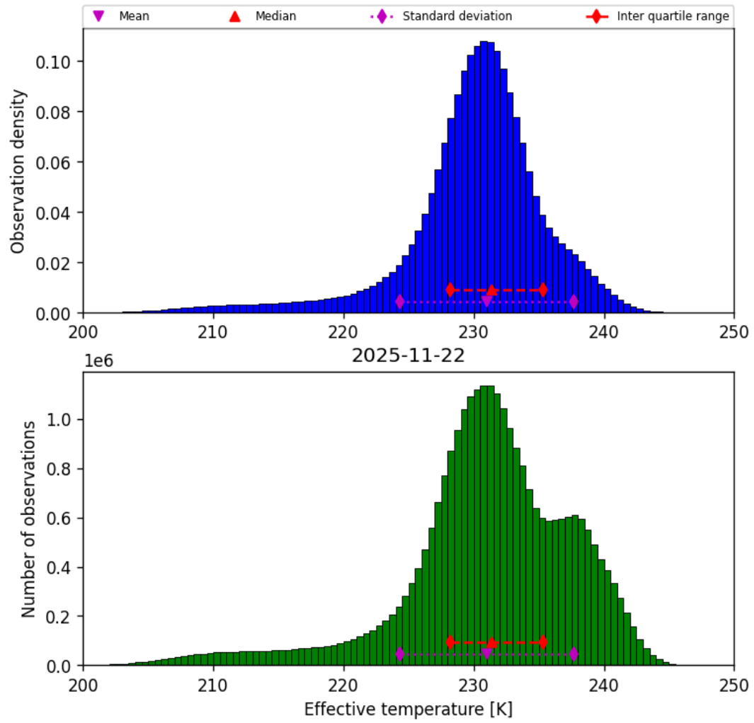
Figure 24: Histogram of “Effective temperature” for 2025-11-21 to 2025-11-23
