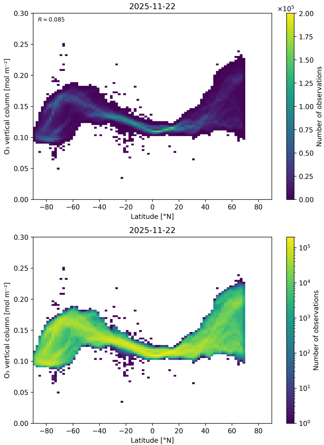
Figure 36: Scatter density plot of “Latitude” against “O 3 vertical column” for 2025-11-21 to 2025-11-23.
