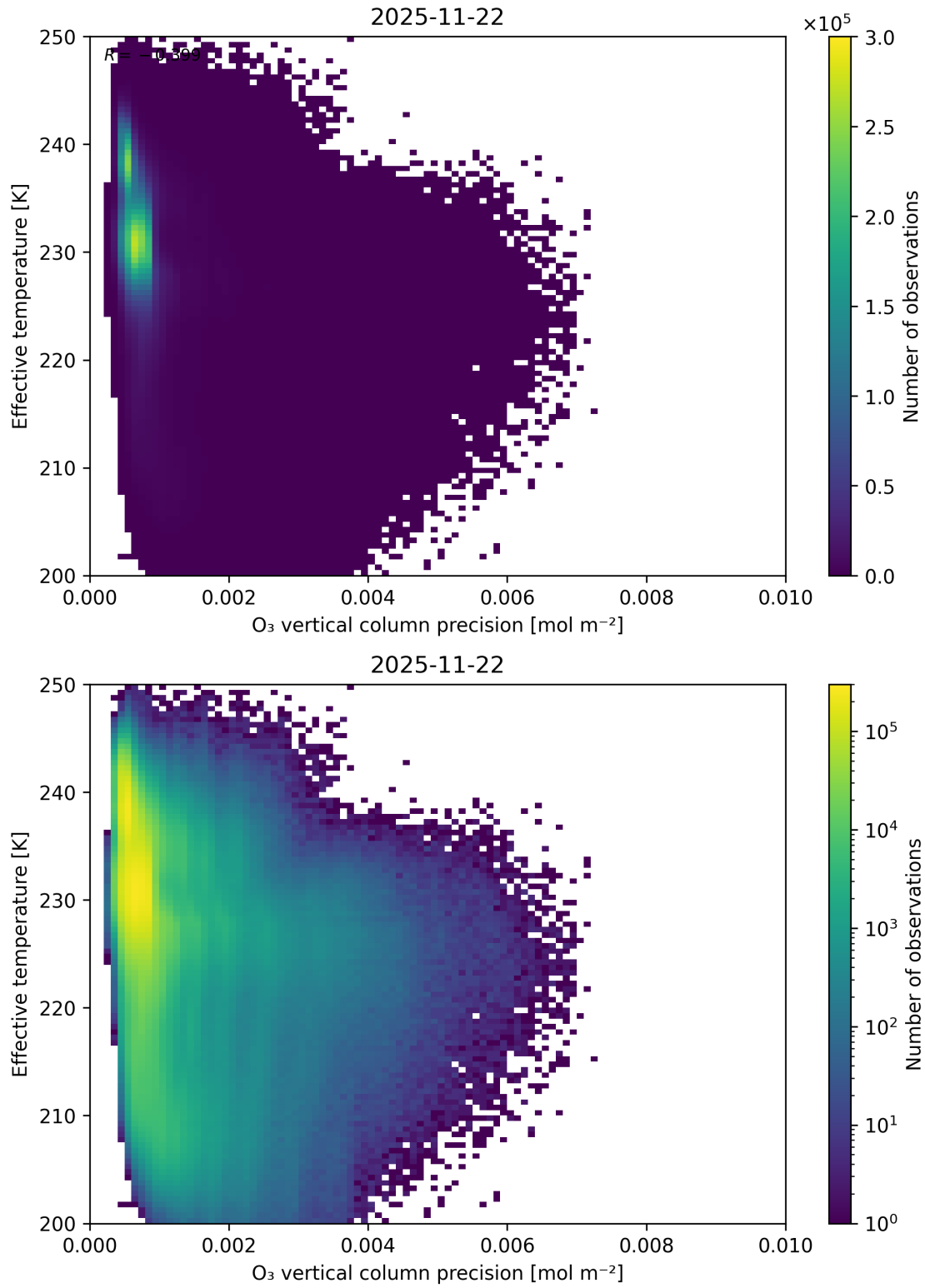
Figure 42: Scatter density plot of “O 3 vertical column precision” against “Effective temperature” for 2025-11-21 to 2025-11-23.
