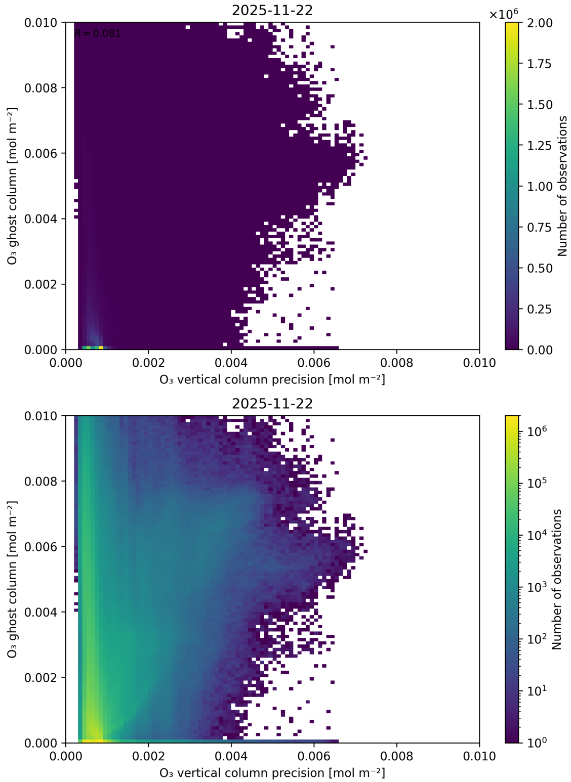
Figure 43: Scatter density plot of “ O_3 vertical column precision” against “ O_3 ghost column” for 2025-11-21 to 2025-11-23.
