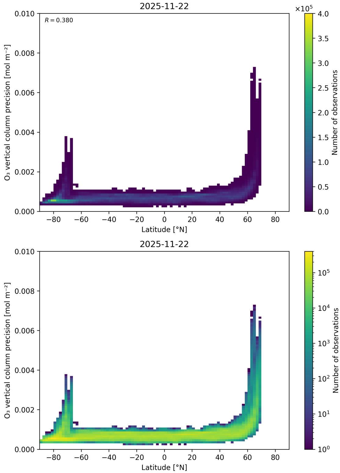
Figure 37: Scatter density plot of “Latitude” against “O 3 vertical column precision” for 2025-11-21 to 2025-11-23.
