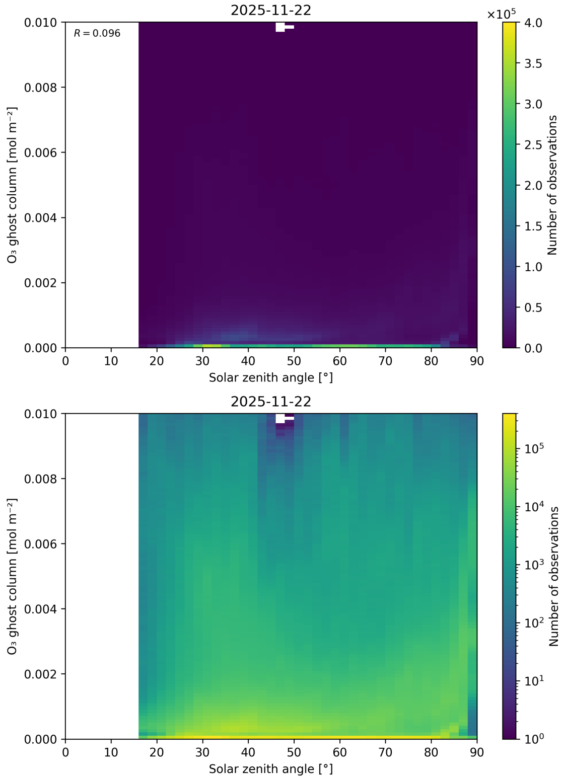
Figure 46: Scatter density plot of “Solar zenith angle” against “O 3 ghost column” for 2025-11-21 to 2025-11-23.
