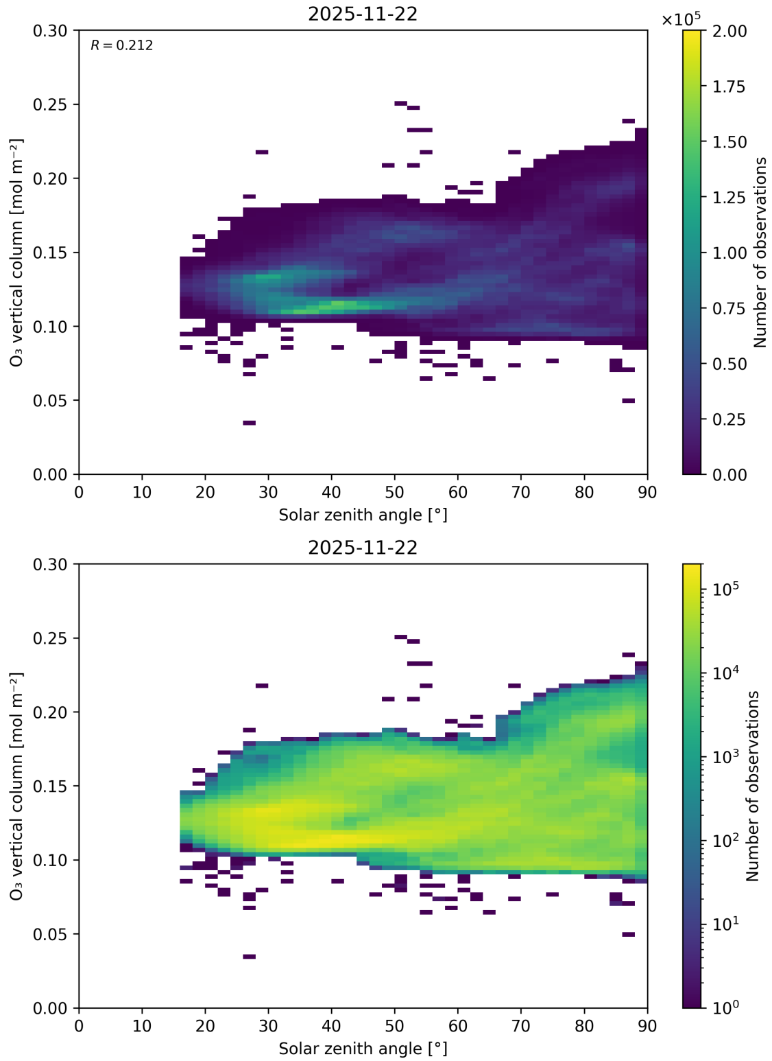
Figure 47: Scatter density plot of “Solar zenith angle” against “O 3 vertical column” for 2025-11-21 to 2025-11-23.
