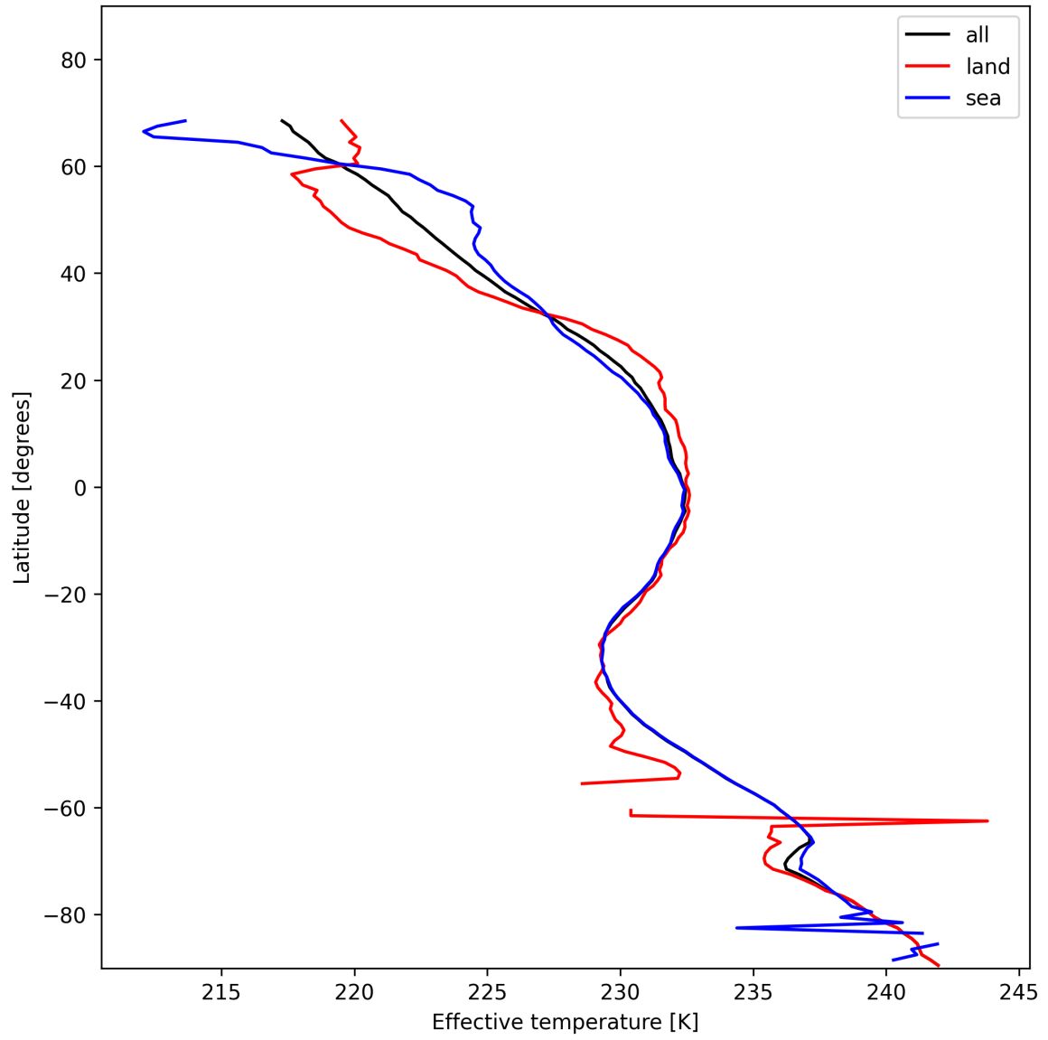
Figure 17: Zonal average of “Effective temperature” for 2025-11-21 to 2025-11-23.
