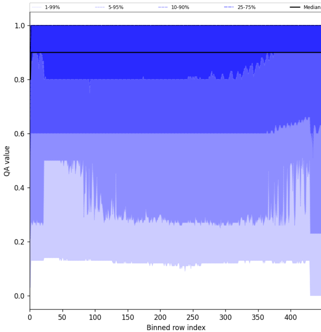
Figure 27: Along track statistics of “QA value” for 2025-11-21 to 2025-11-23
