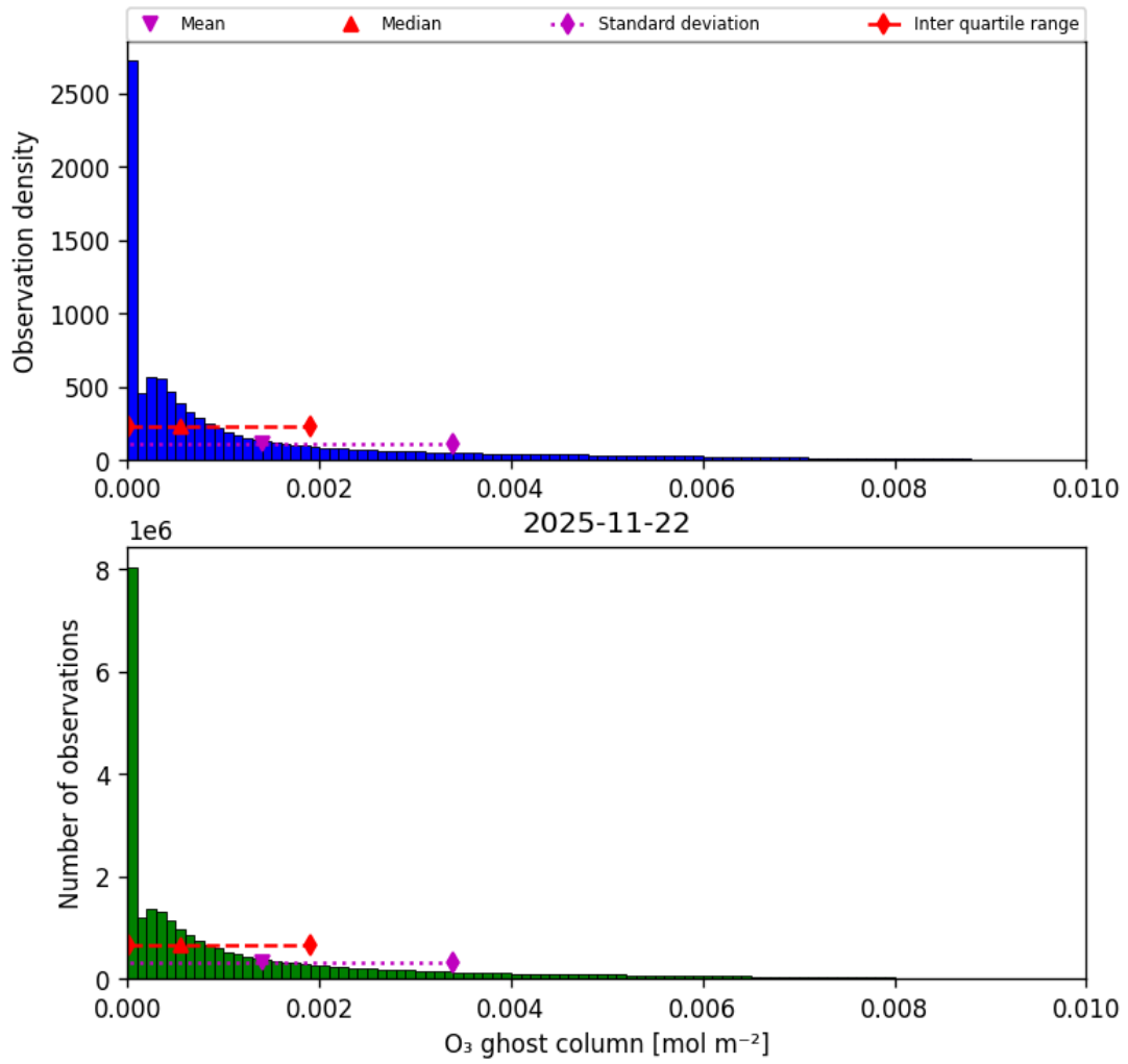
Figure 25: Histogram of “O 3 ghost column” for 2025-11-21 to 2025-11-23
