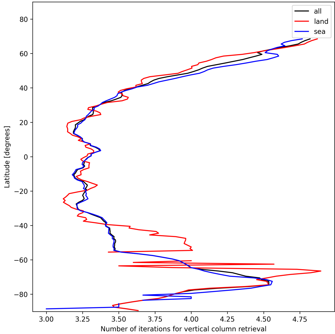
Figure 19: Zonal average of “Number of iterations for vertical column retrieval” for 2025-11-21 to 2025-11-23.
