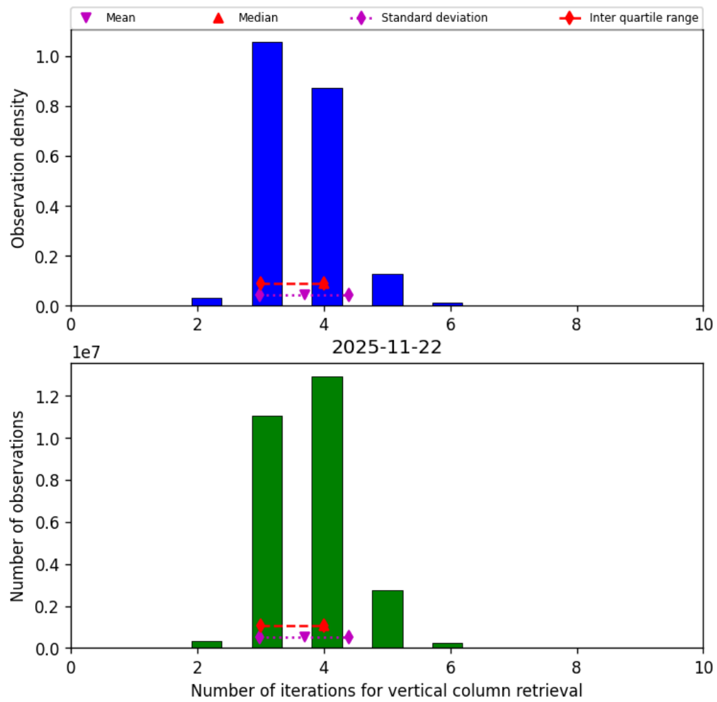
Figure 26: Histogram of “Number of iterations for vertical column retrieval” for 2025-11-21 to 2025-11-23
