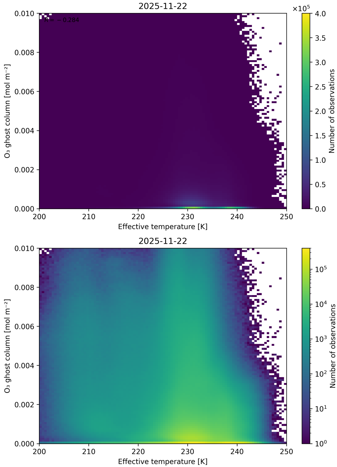
Figure 38: Scatter density plot of “Effective temperature” against “O 3 ghost column” for 2025-11-21 to 2025-11-23.
