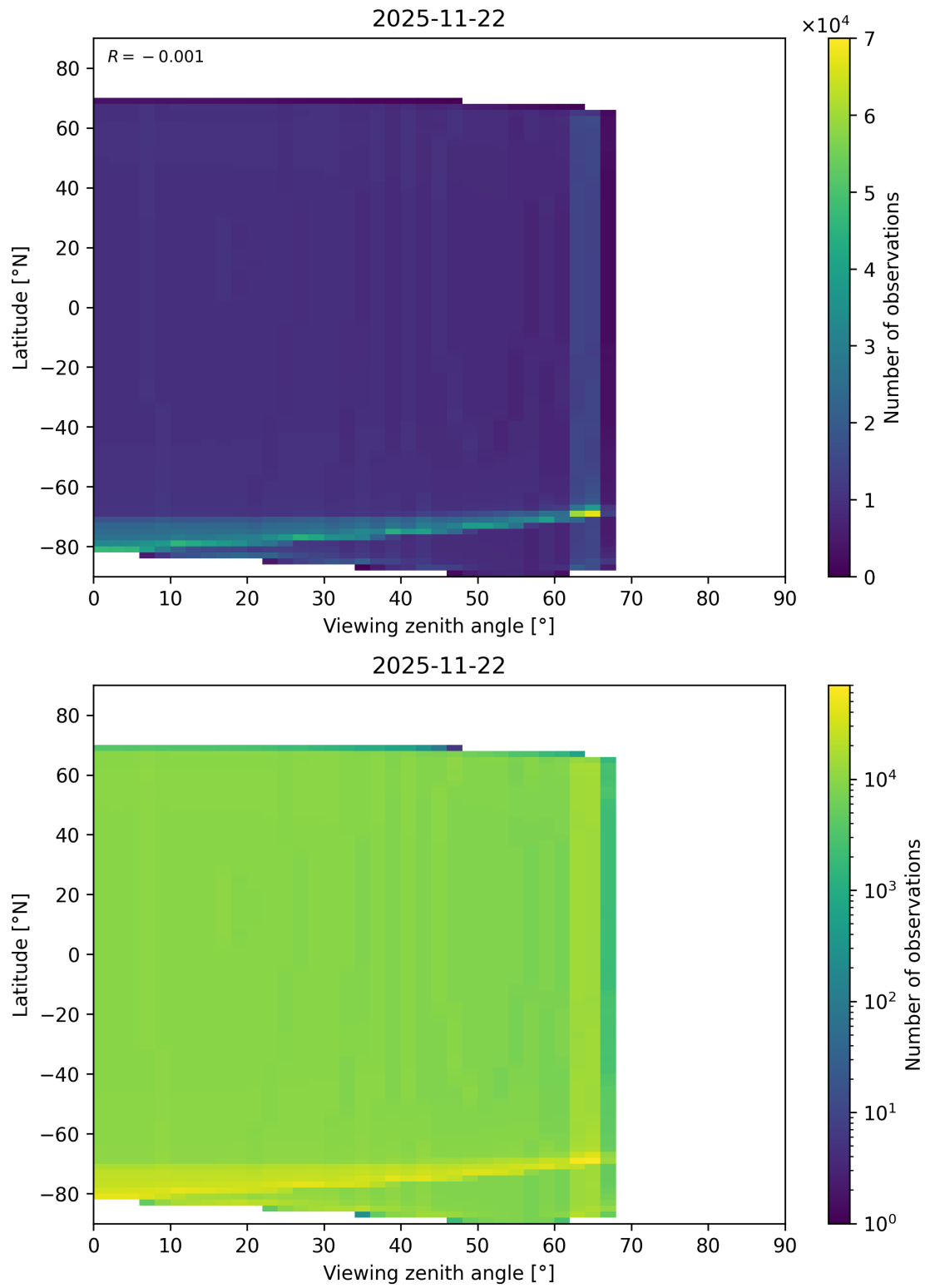
Figure 49: Scatter density plot of “Viewing zenith angle” against “Latitude” for 2025-11-21 to 2025-11-23.
