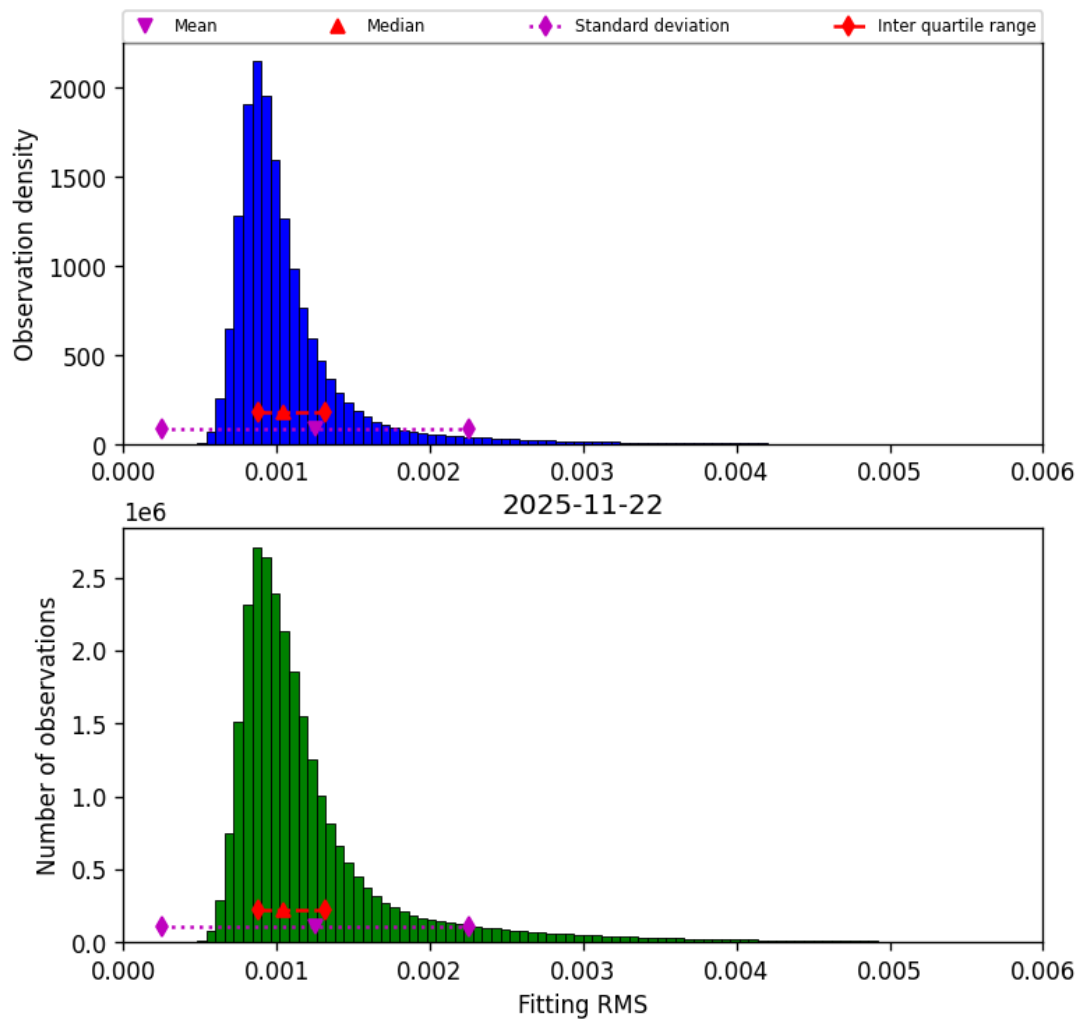
Figure 23: Histogram of “Fitting RMS” for 2025-11-21 to 2025-11-23
