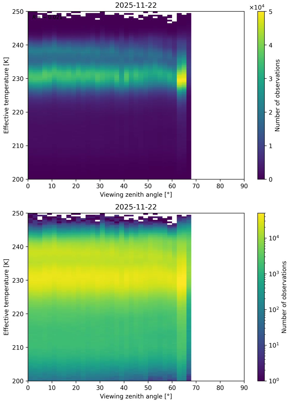
Figure 50: Scatter density plot of “Viewing zenith angle” against “Effective temperature” for 2025-11-21 to 2025-11-23.
