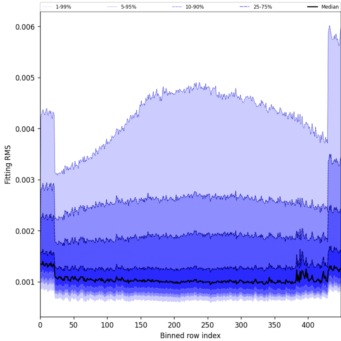
Figure 30: Along track statistics of “Fitting RMS” for 2025-11-21 to 2025-11-23
