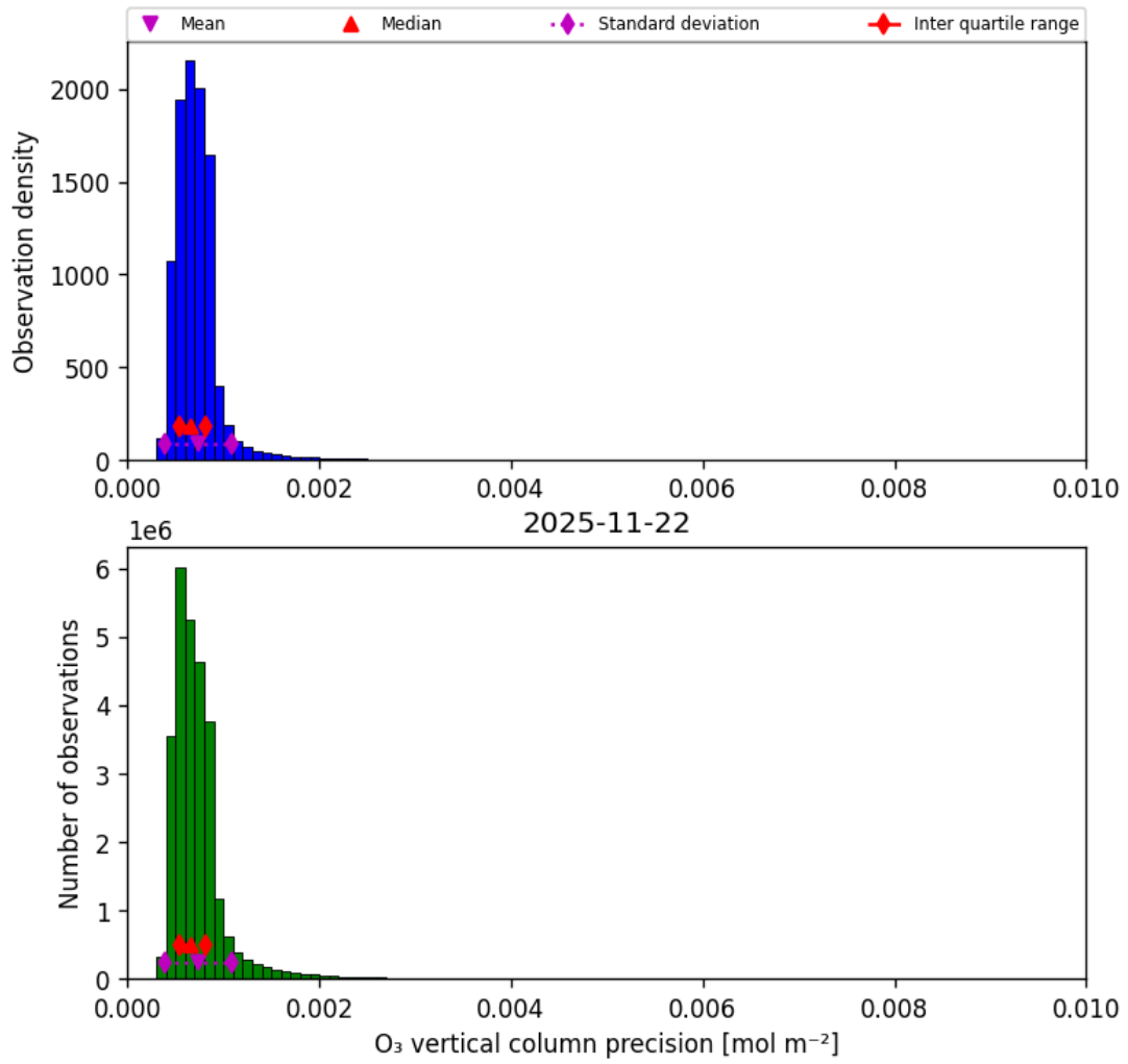
Figure 22: Histogram of “O 3 vertical column precision” for 2025-11-21 to 2025-11-23
