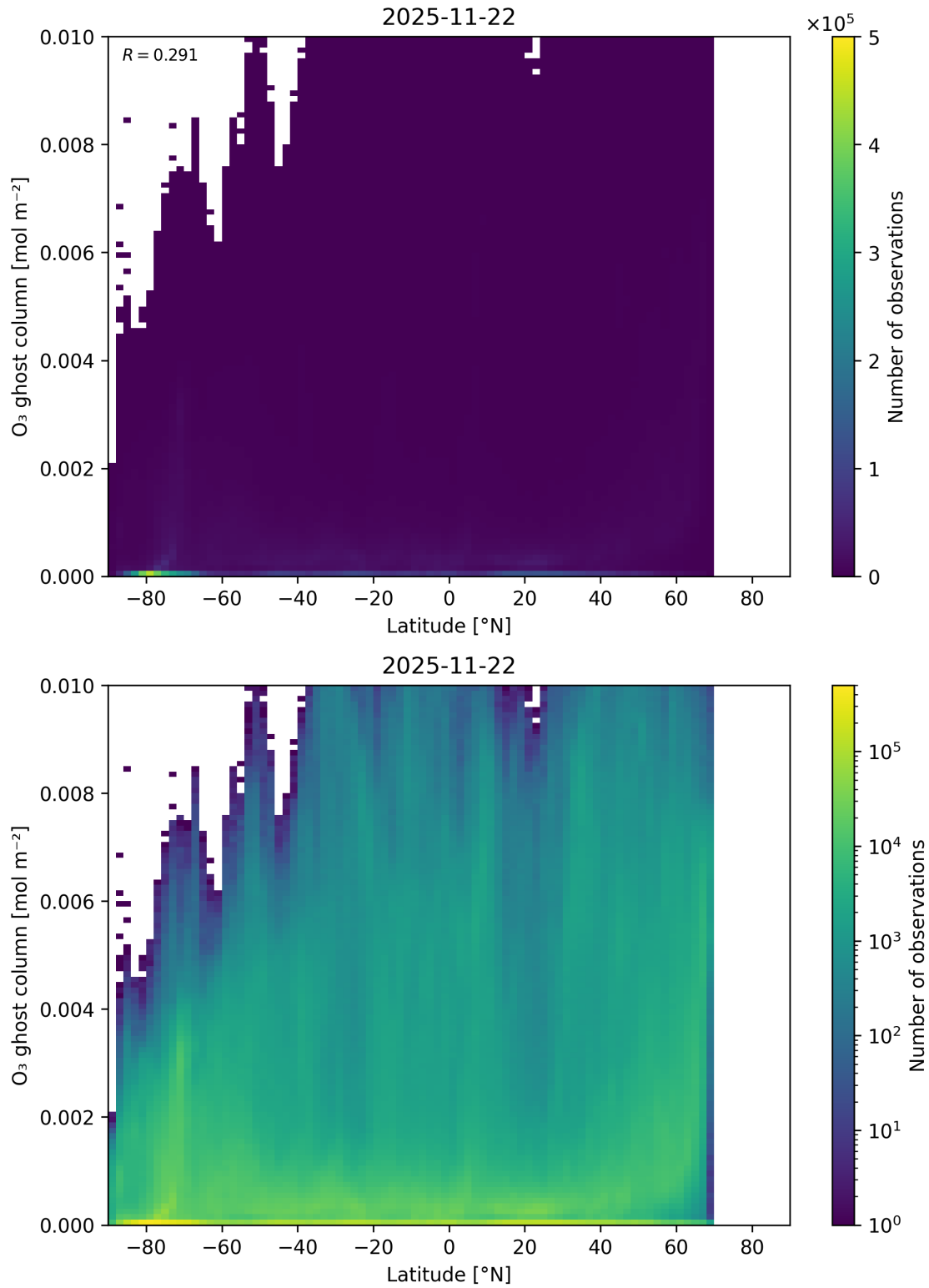
Figure 35: Scatter density plot of “Latitude” against “O 3 ghost column” for 2025-11-21 to 2025-11-23.
