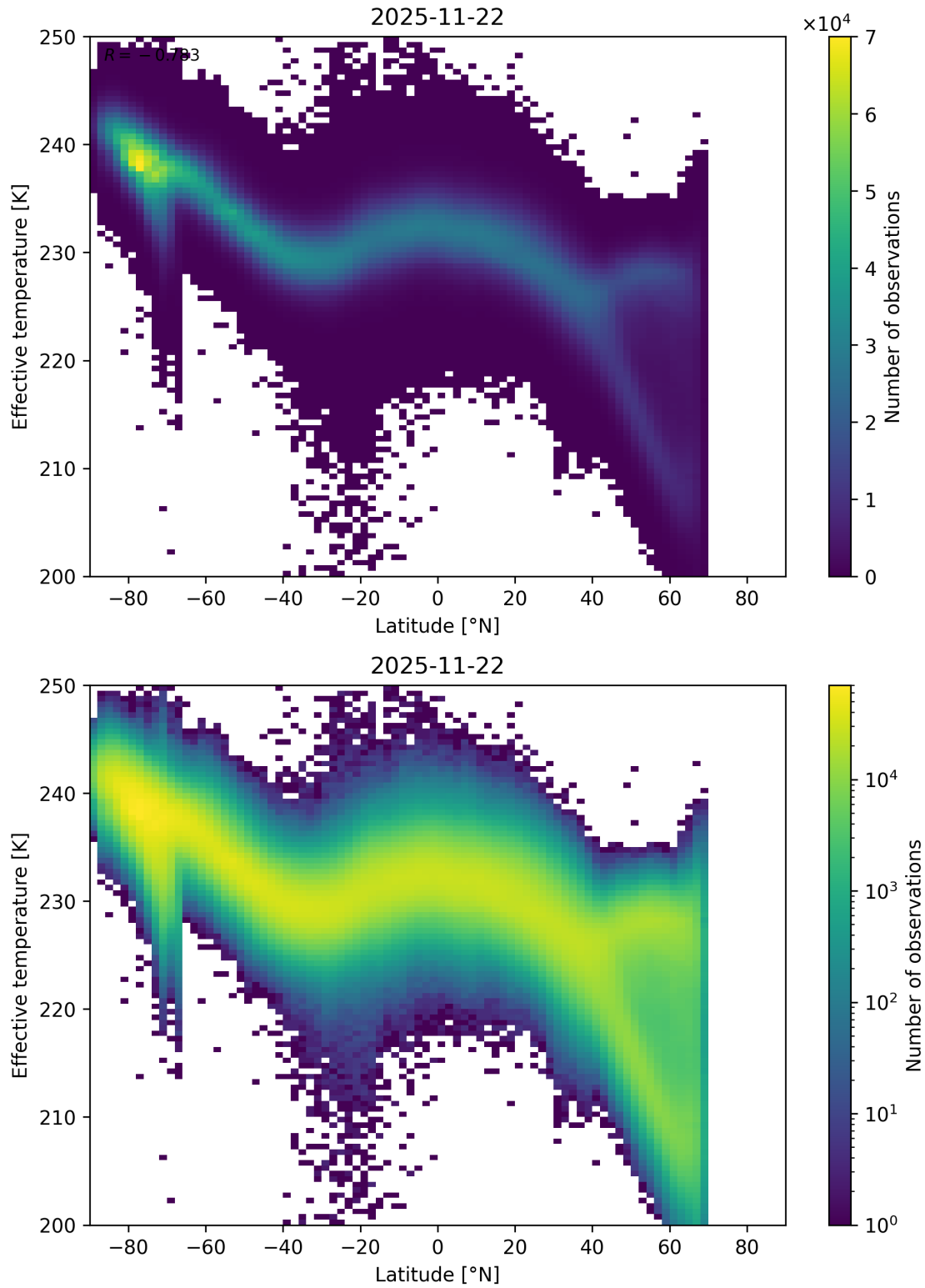
Figure 34: Scatter density plot of “Latitude” against “Effective temperature” for 2025-11-21 to 2025-11-23.
