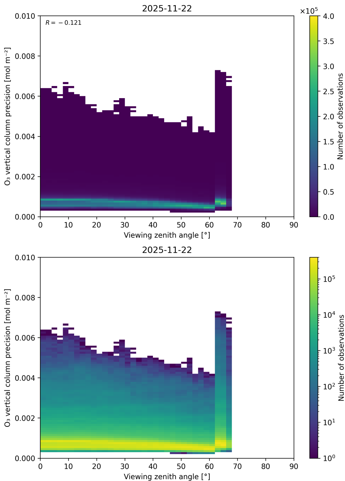
Figure 53: Scatter density plot of “Viewing zenith angle” against “O 3 vertical column precision” for 2025-11-21 to 2025-11-23.
