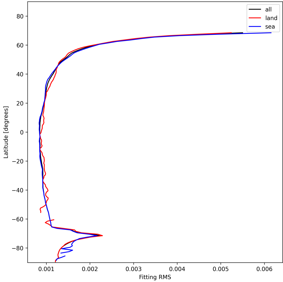
Figure 16: Zonal average of “Fitting RMS” for 2025-11-21 to 2025-11-23.
