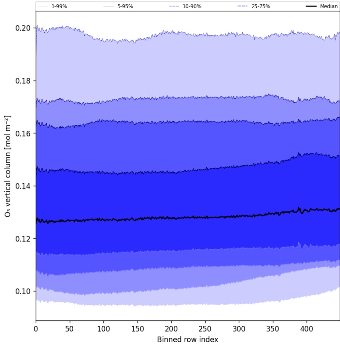
Figure 28: Along track statistics of “ O_3 vertical column” for 2025-11-21 to 2025-11-23
