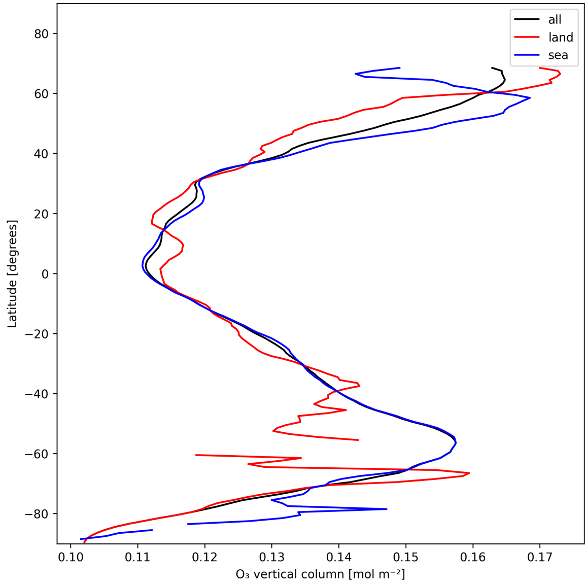
Figure 14: Zonal average of “O 3 vertical column” for 2025-11-21 to 2025-11-23.
