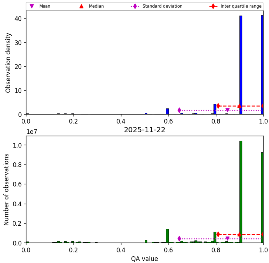
Figure 20: Histogram of “QA value” for 2025-11-21 to 2025-11-23
