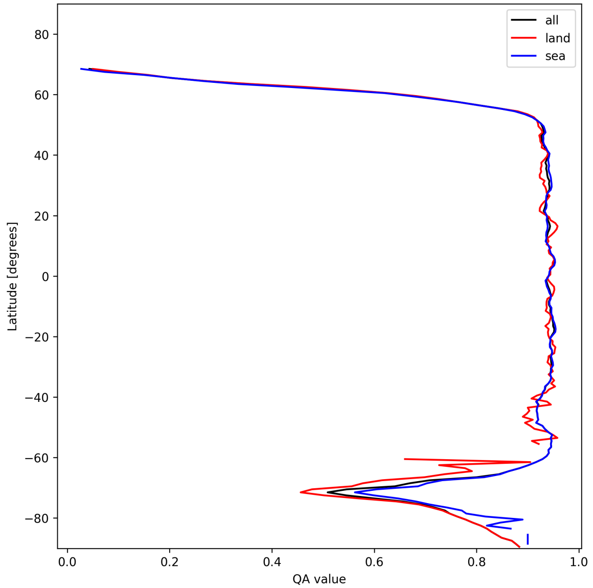
Figure 13: Zonal average of “QA value” for 2025-11-21 to 2025-11-23.
