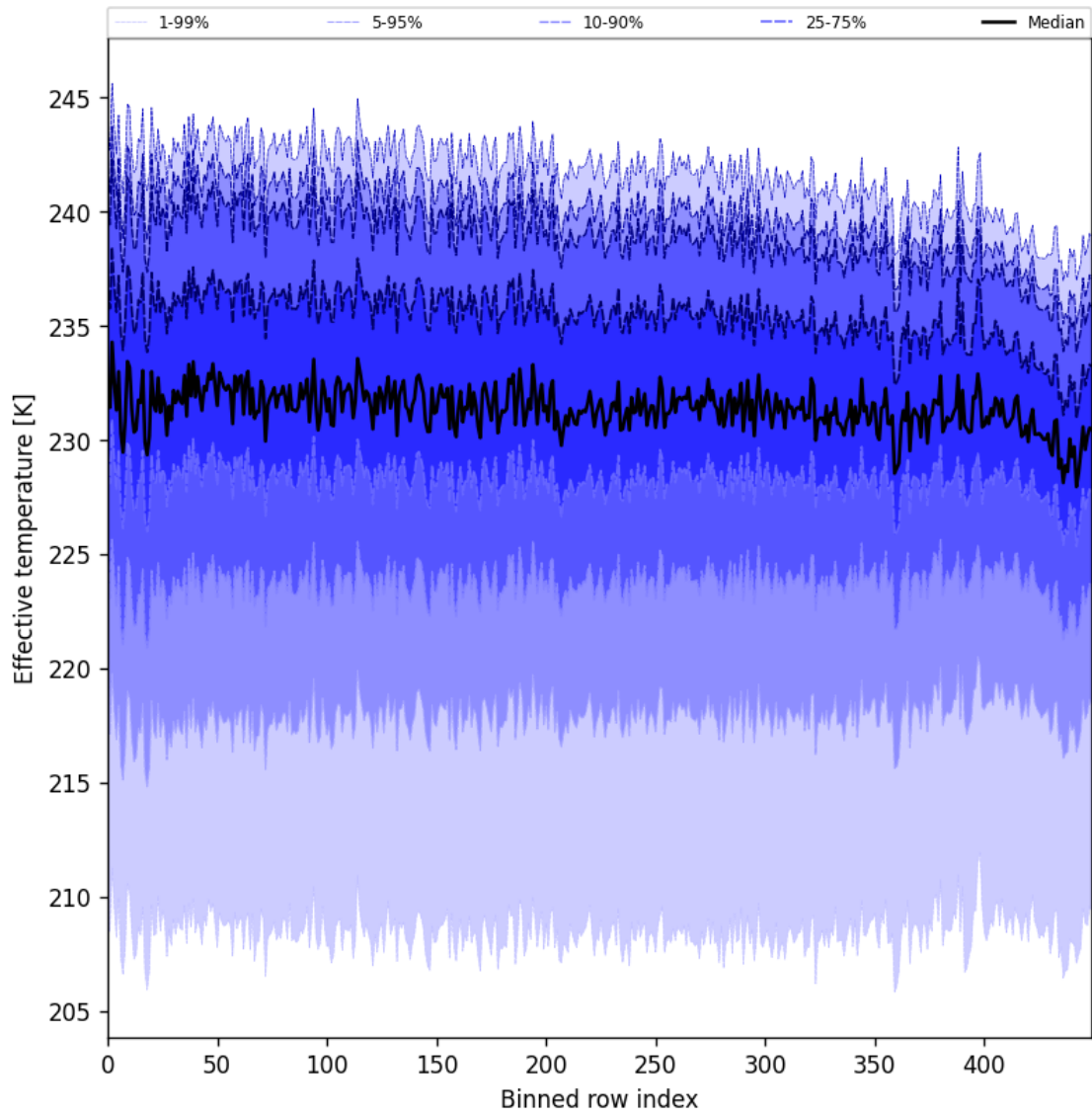
Figure 31: Along track statistics of “Effective temperature” for 2025-11-21 to 2025-11-23
