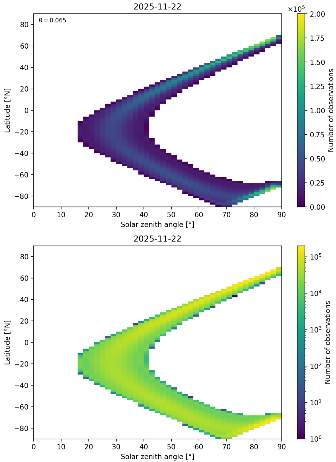
Figure 44: Scatter density plot of “Solar zenith angle” against “Latitude” for 2025-11-21 to 2025-11-23.
