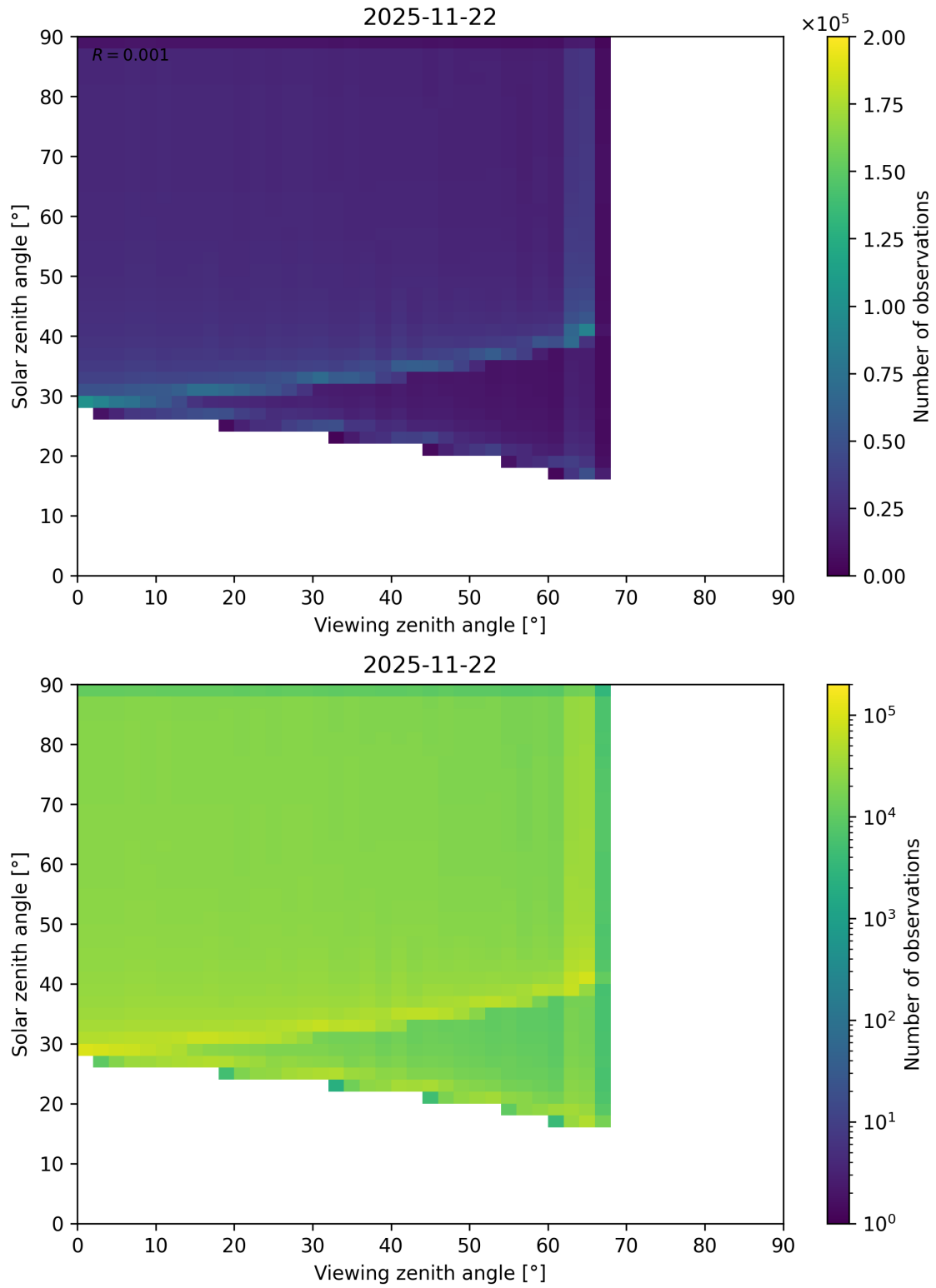
Figure 54: Scatter density plot of “Viewing zenith angle” against “Solar zenith angle” for 2025-11-21 to 2025-11-23.
