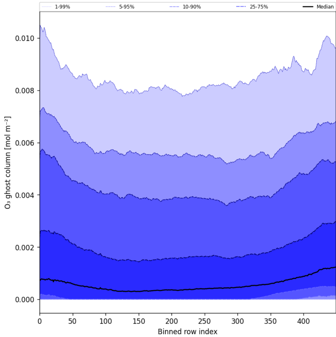
Figure 32: Along track statistics of “O 3 ghost column” for 2025-11-21 to 2025-11-23
