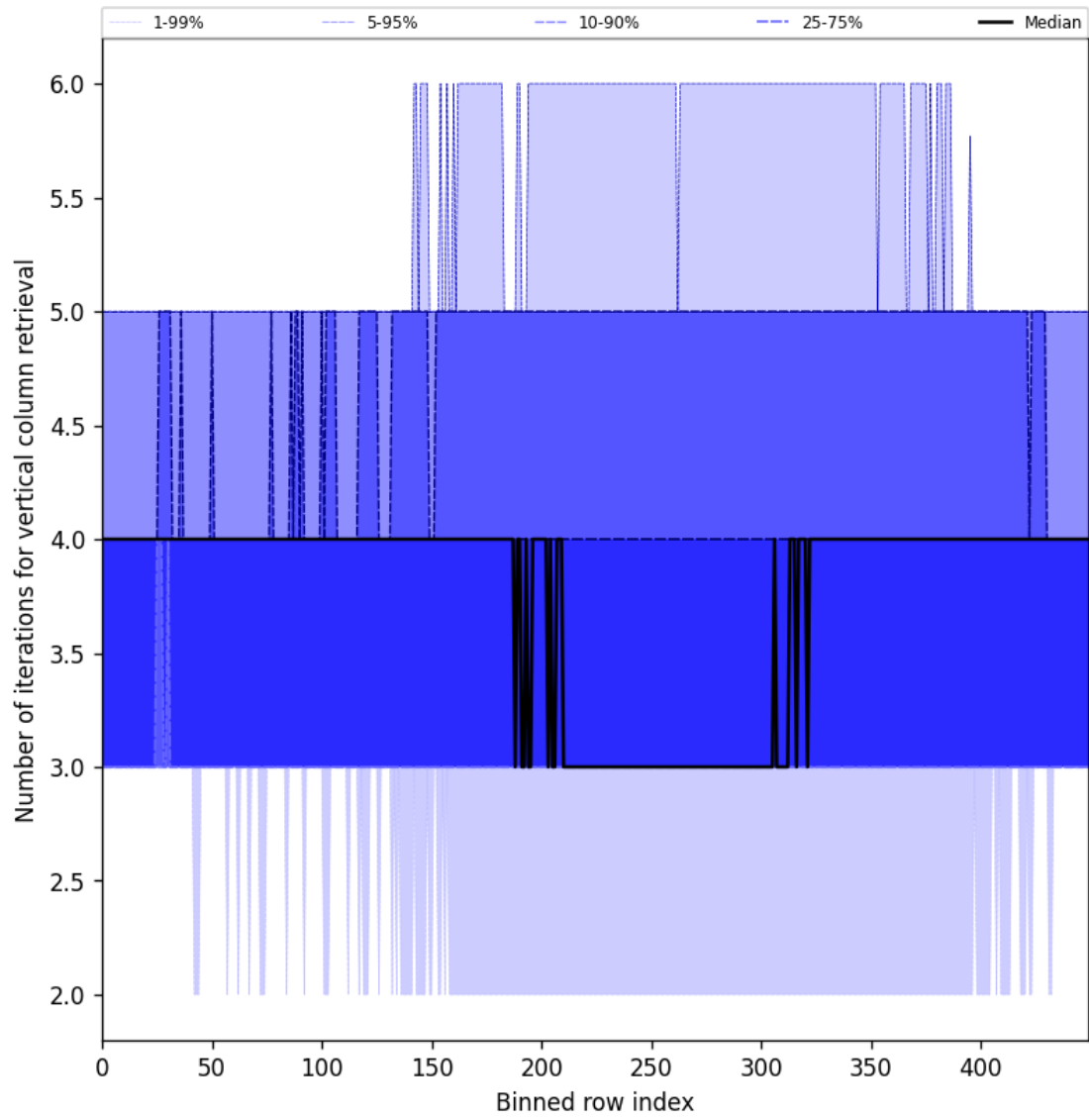
Figure 33: Along track statistics of “Number of iterations for vertical column retrieval” for 2025-11-21 to 2025-11-23
