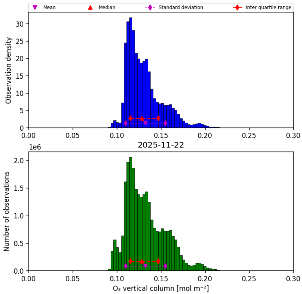
Figure 21: Histogram of “O 3 vertical column” for 2025-11-21 to 2025-11-23
