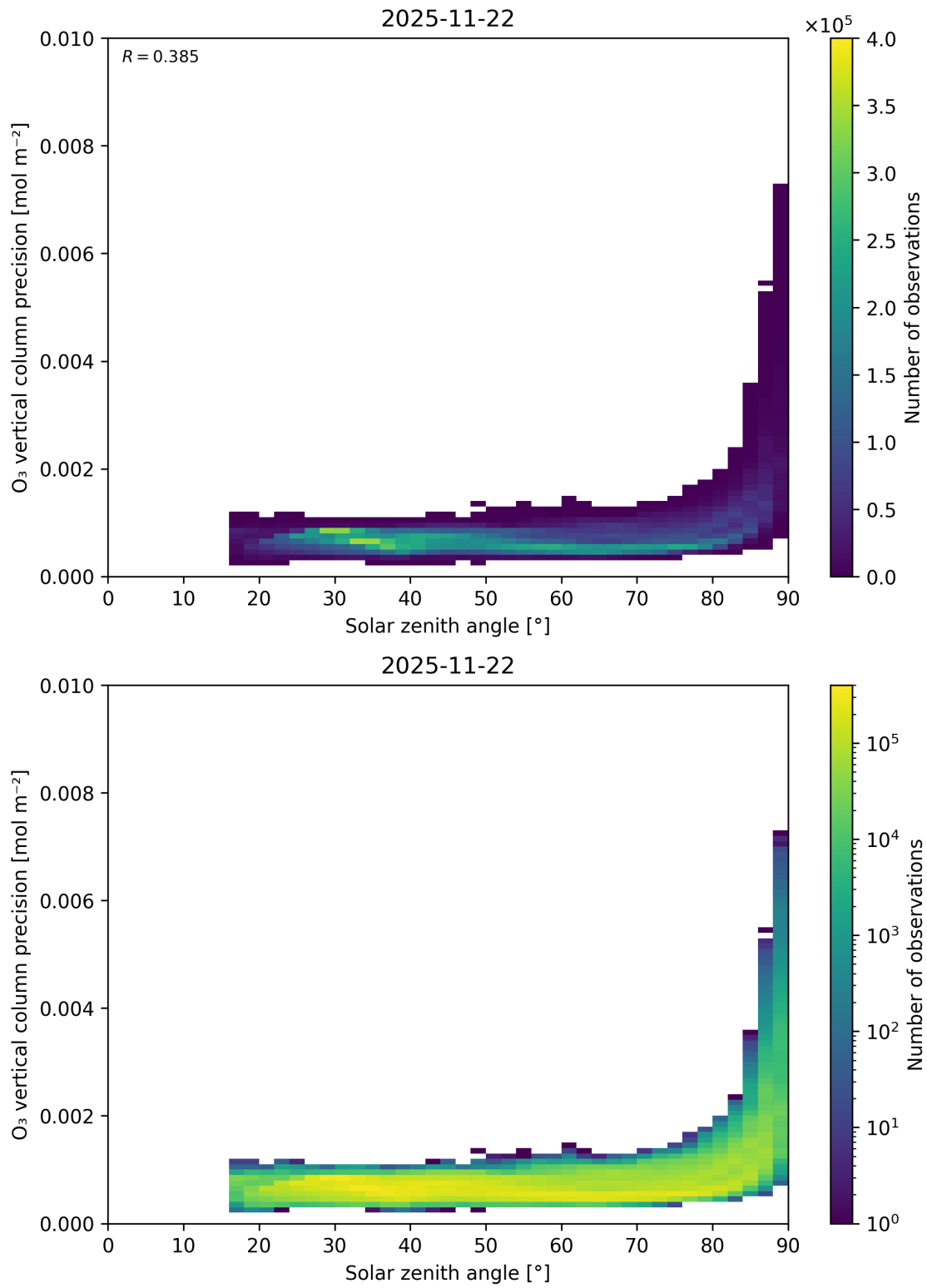
Figure 48: Scatter density plot of “Solar zenith angle” against “O 3 vertical column precision” for 2025-11-21 to 2025-11-23.
