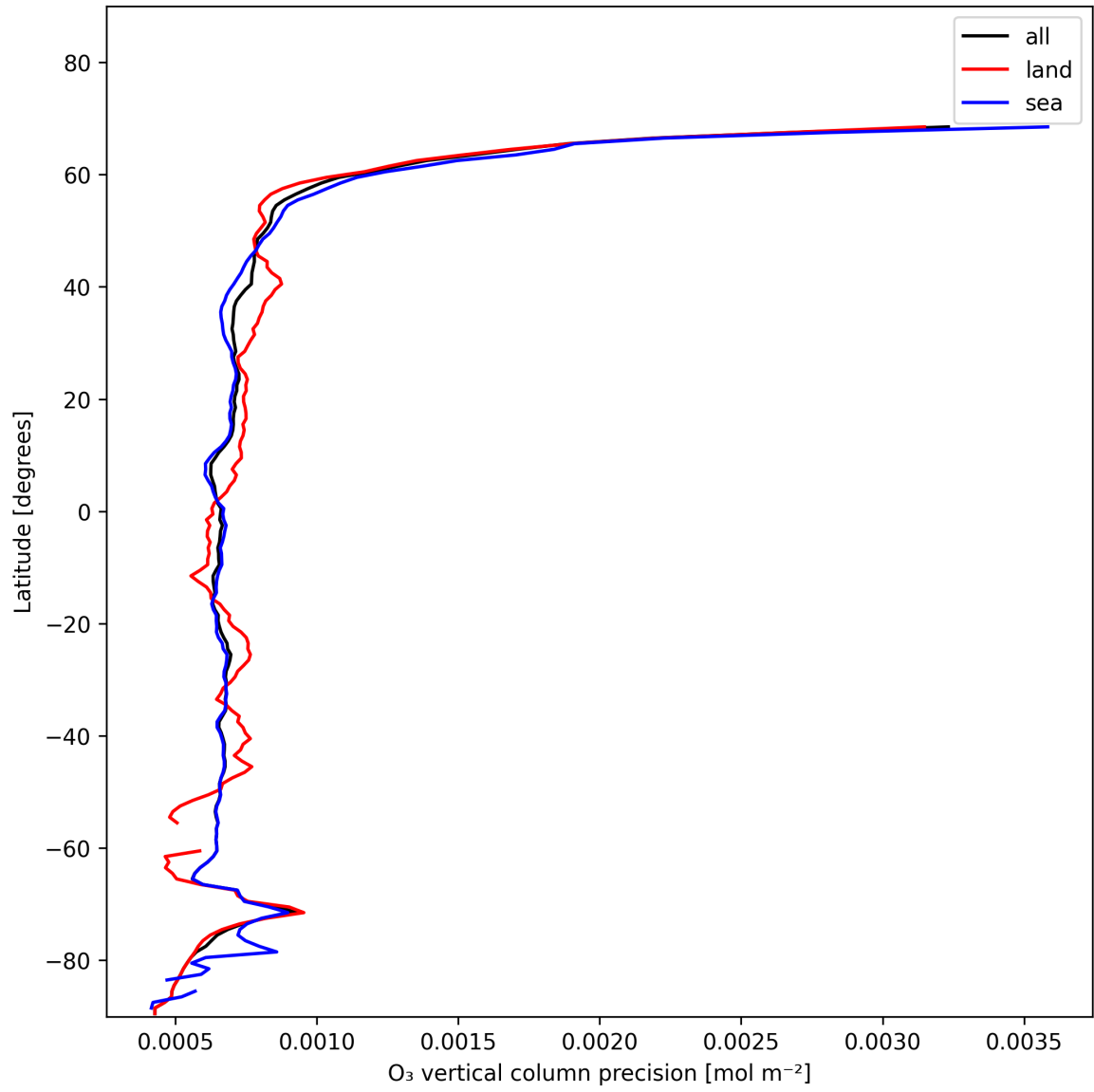
Figure 15: Zonal average of “O 3 vertical column precision” for 2025-11-21 to 2025-11-23.
