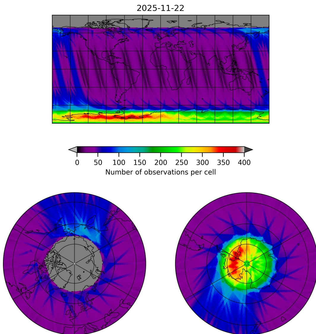
Figure 12: Map of the number of observations for 2025-11-21 to 2025-11-23
