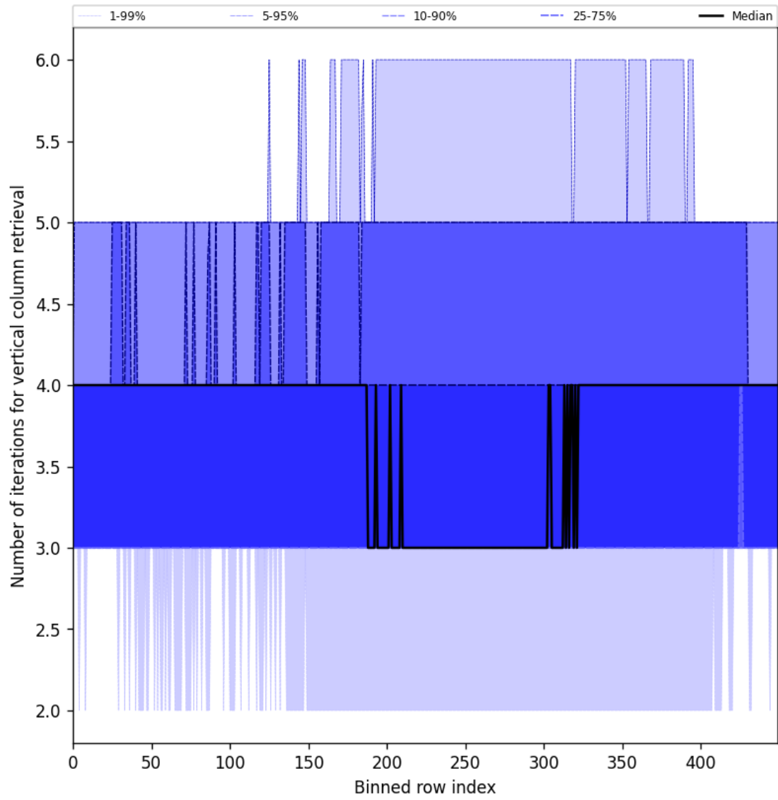
Figure 33: Along track statistics of “Number of iterations for vertical column retrieval” for 2025-11-23 to 2025-11-24
