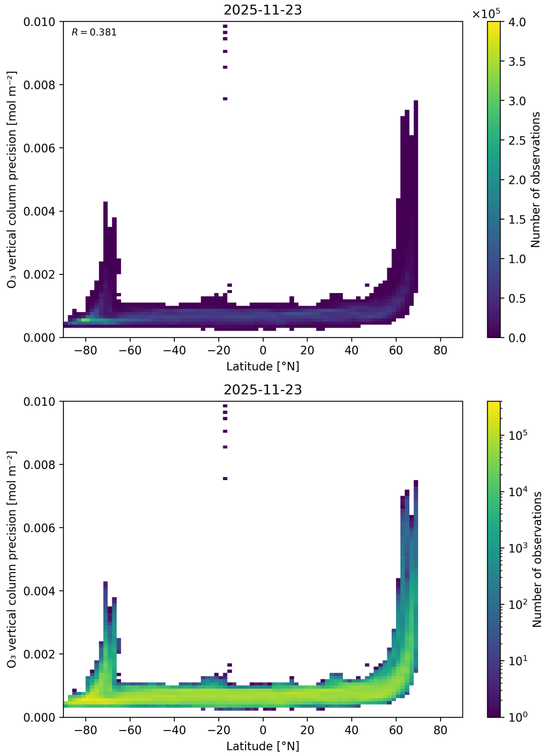
Figure 37: Scatter density plot of “Latitude” against “O 3 vertical column precision” for 2025-11-23 to 2025-11-24.
