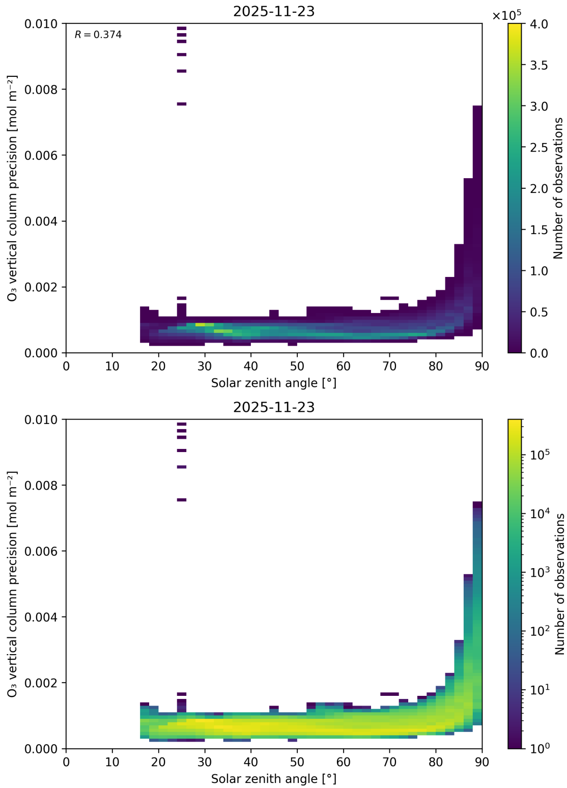
Figure 48: Scatter density plot of “Solar zenith angle” against “O 3 vertical column precision” for 2025-11-23 to 2025-11-24.
