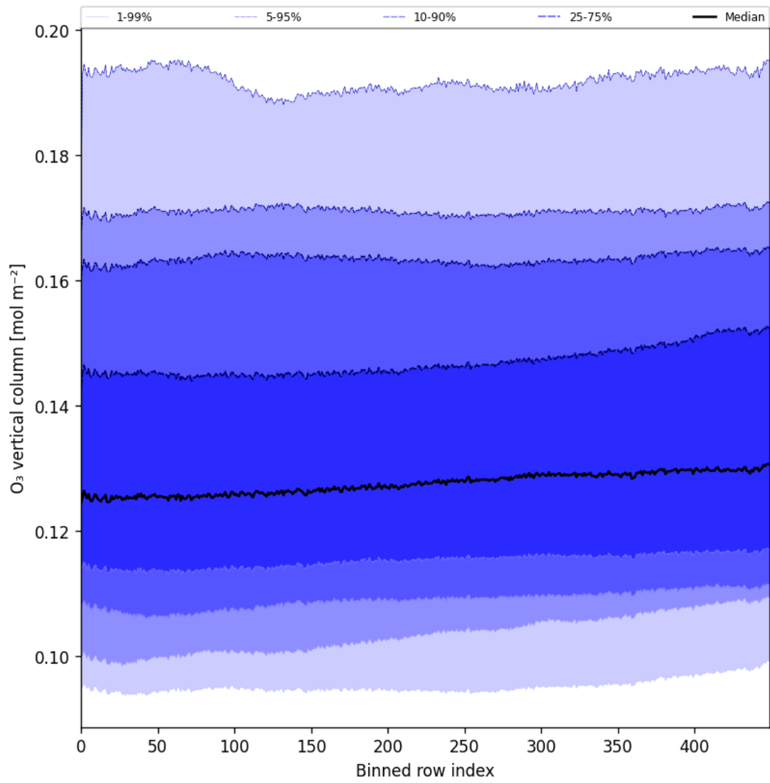
Figure 28: Along track statistics of “O 3 vertical column” for 2025-11-23 to 2025-11-24
