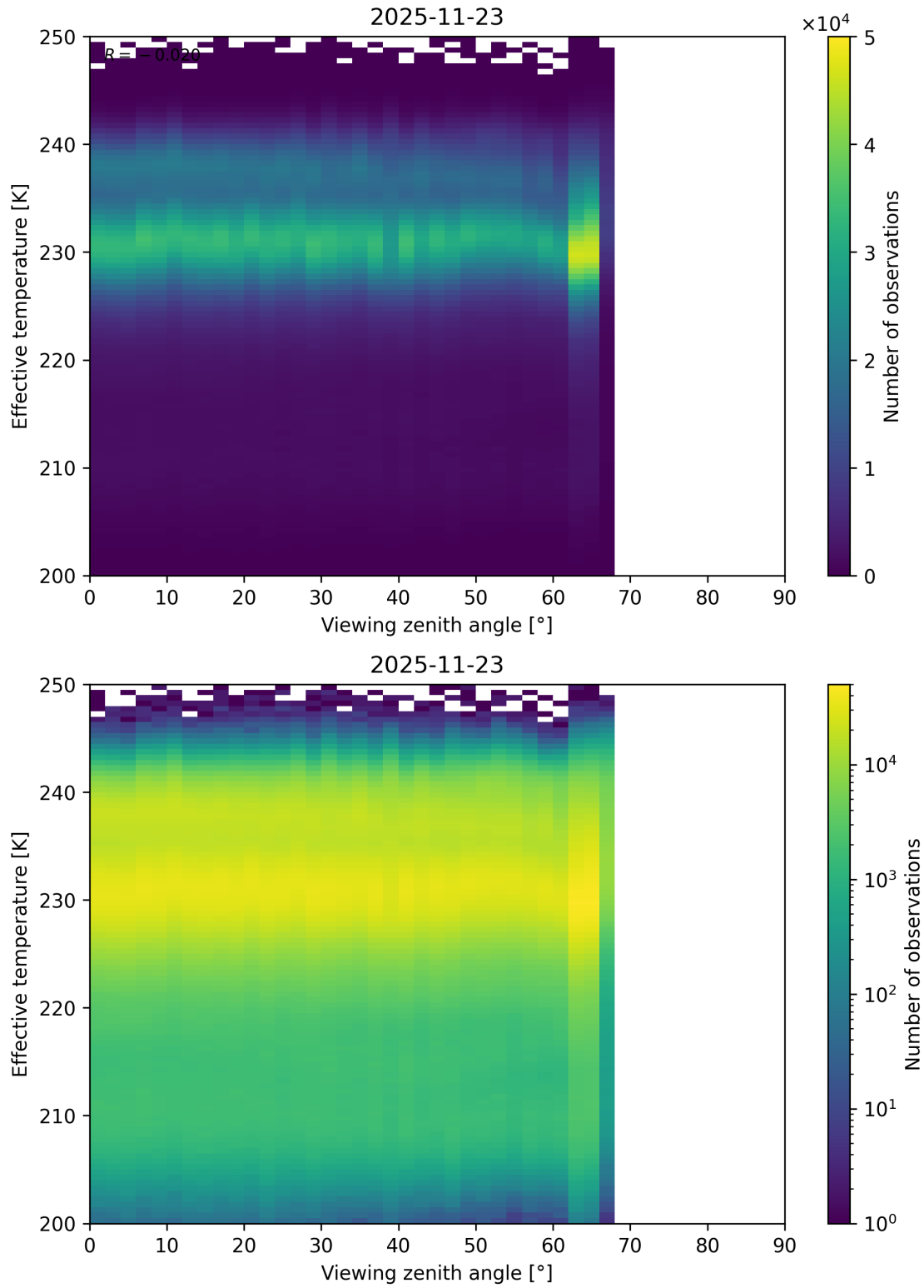
Figure 50: Scatter density plot of “Viewing zenith angle” against “Effective temperature” for 2025-11-23 to 2025-11-24.
