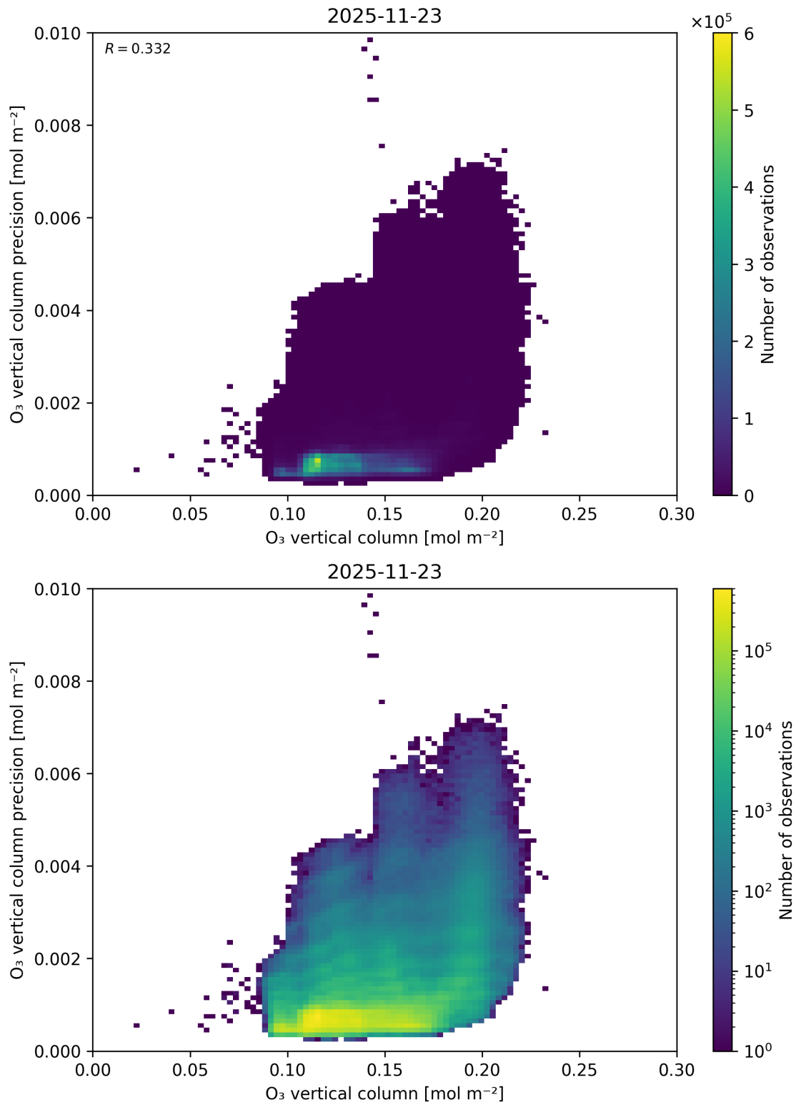
Figure 41: Scatter density plot of “O 3 vertical column” against “O 3 vertical column precision” for 2025-11-23 to 2025-11-24.
