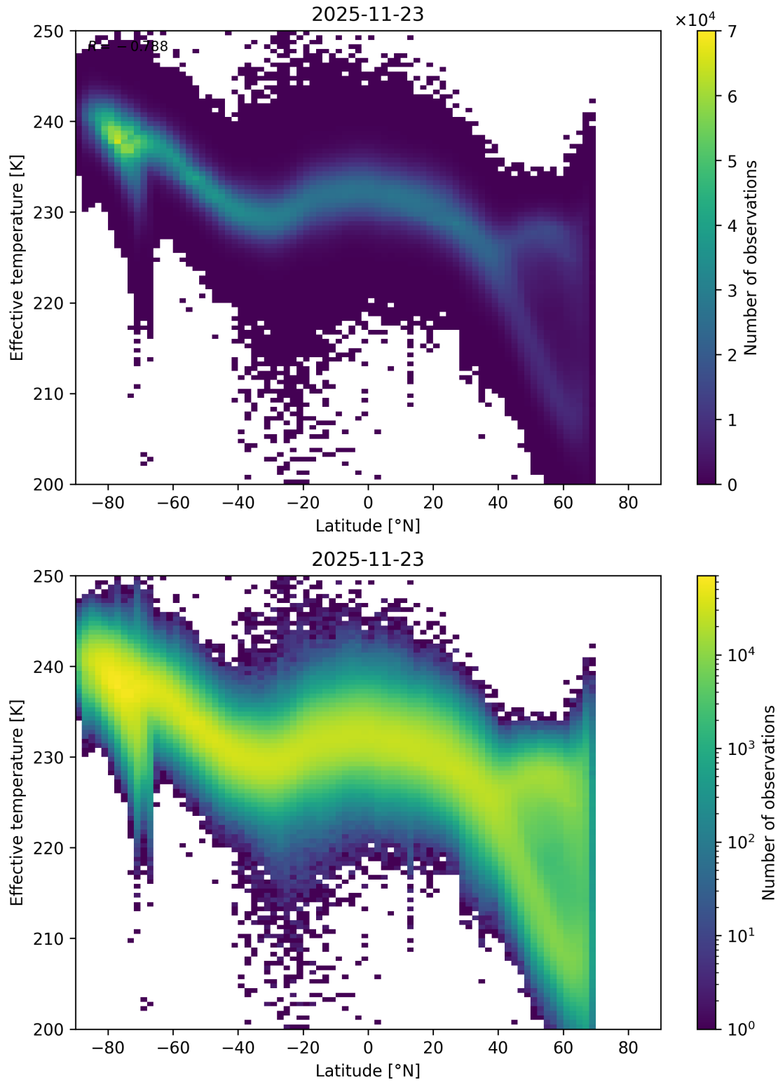
Figure 34: Scatter density plot of “Latitude” against “Effective temperature” for 2025-11-23 to 2025-11-24.
