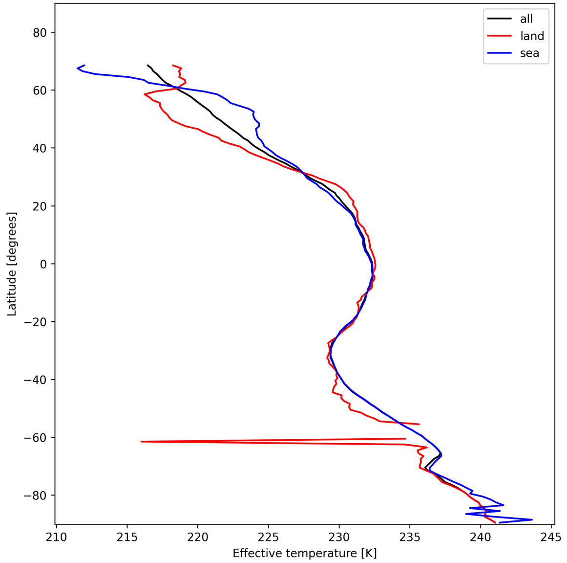
Figure 17: Zonal average of “Effective temperature” for 2025-11-23 to 2025-11-24.
