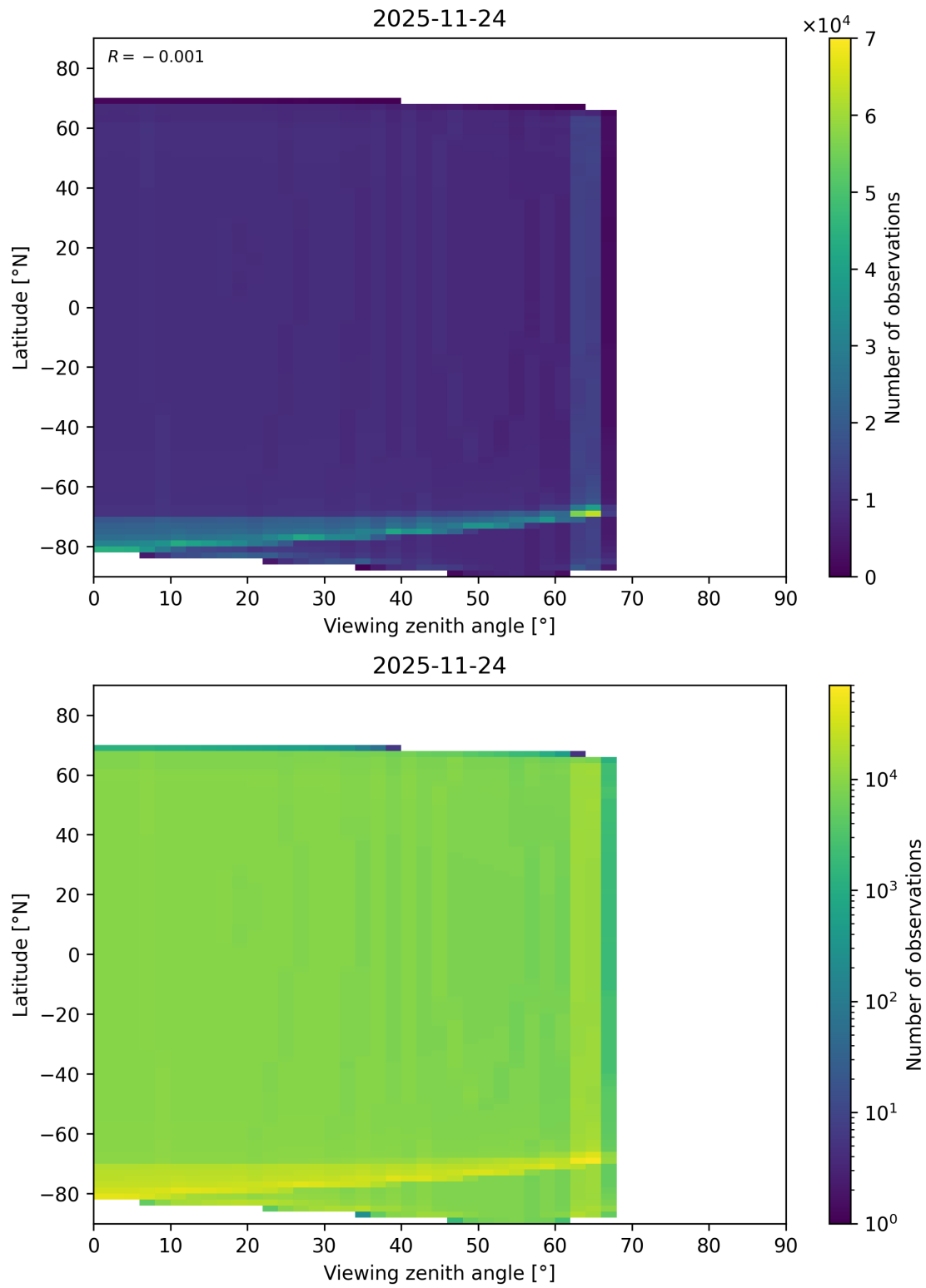
Figure 49: Scatter density plot of “Viewing zenith angle” against “Latitude” for 2025-11-23 to 2025-11-25.
