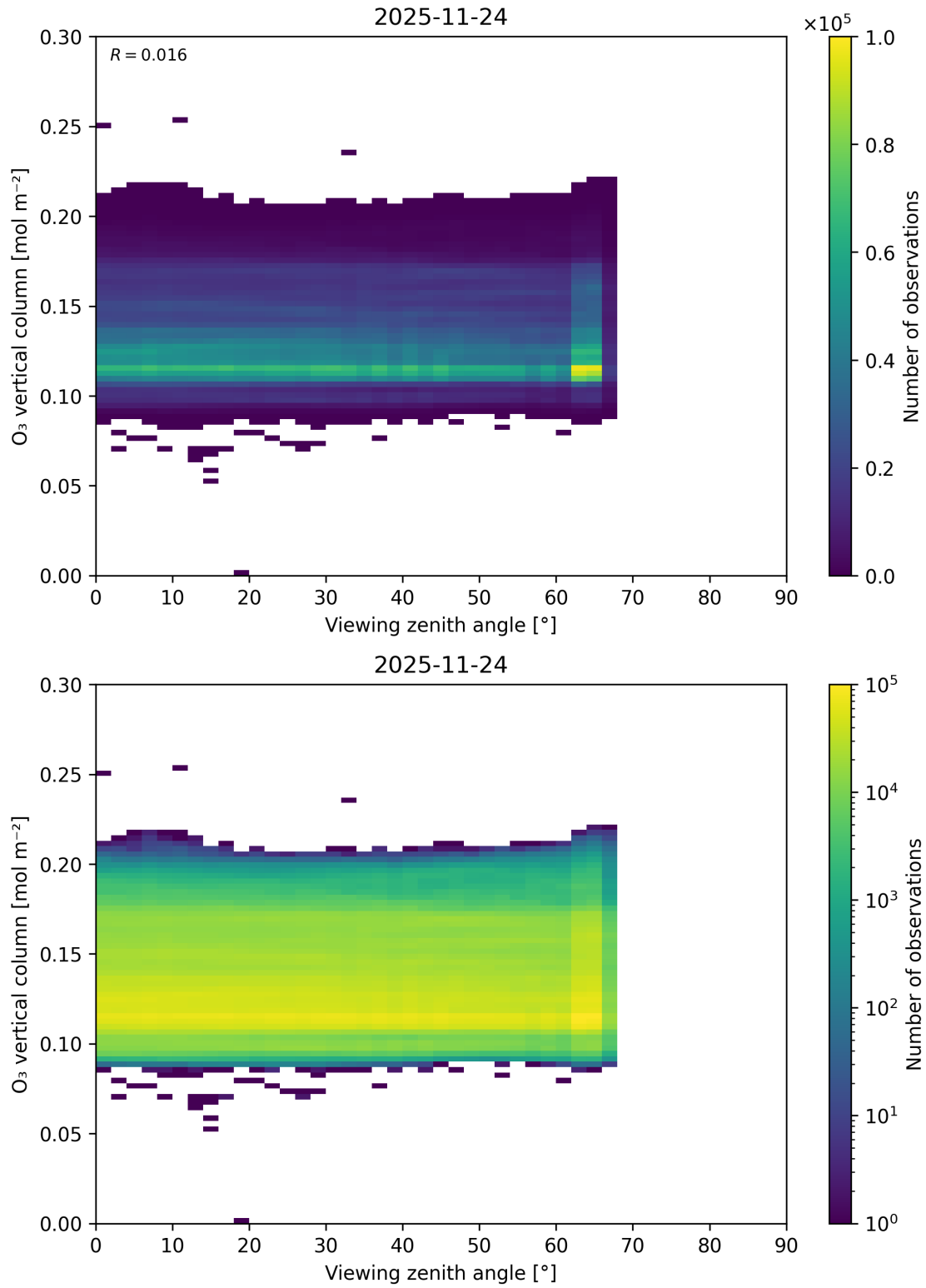
Figure 52: Scatter density plot of “Viewing zenith angle” against “O 3 vertical column” for 2025-11-23 to 2025-11-25.
