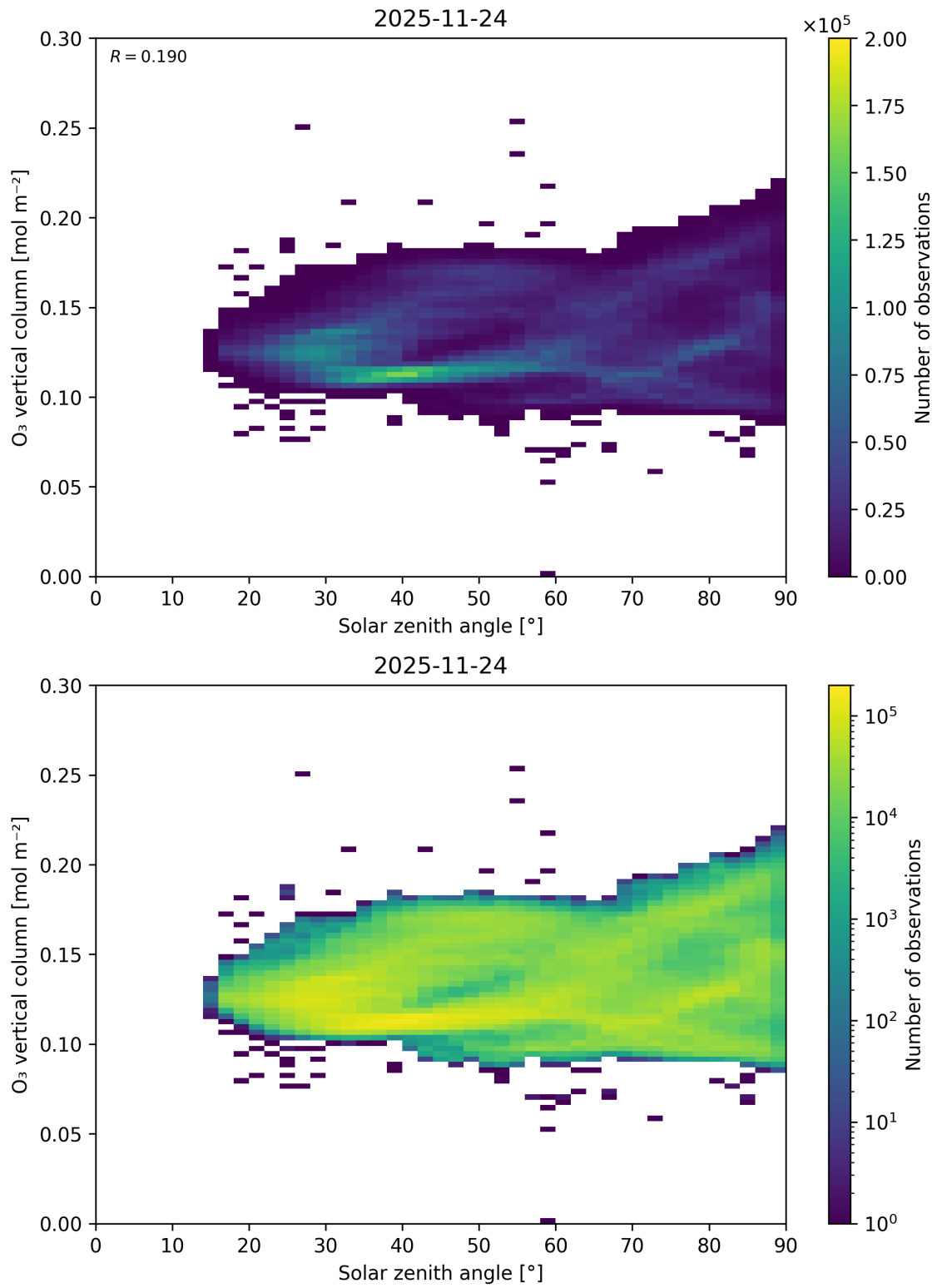
Figure 47: Scatter density plot of “Solar zenith angle” against “O 3 vertical column” for 2025-11-23 to 2025-11-25.
