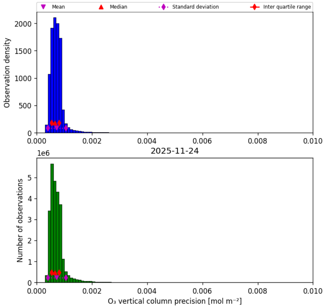
Figure 22: Histogram of “O 3 vertical column precision” for 2025-11-23 to 2025-11-25
