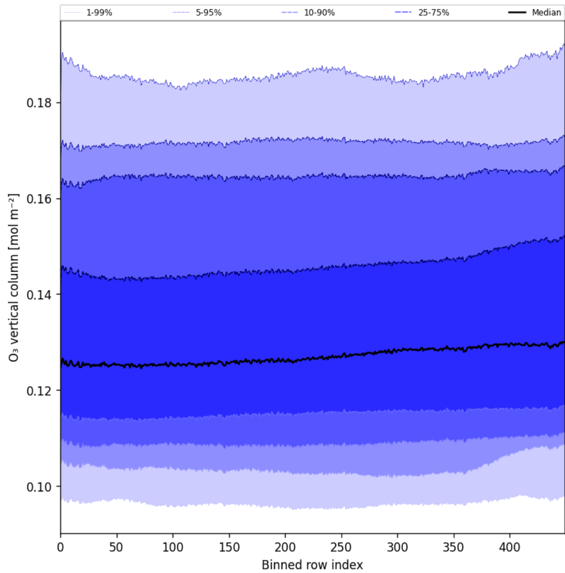
Figure 28: Along track statistics of “O 3 vertical column” for 2025-11-23 to 2025-11-25
