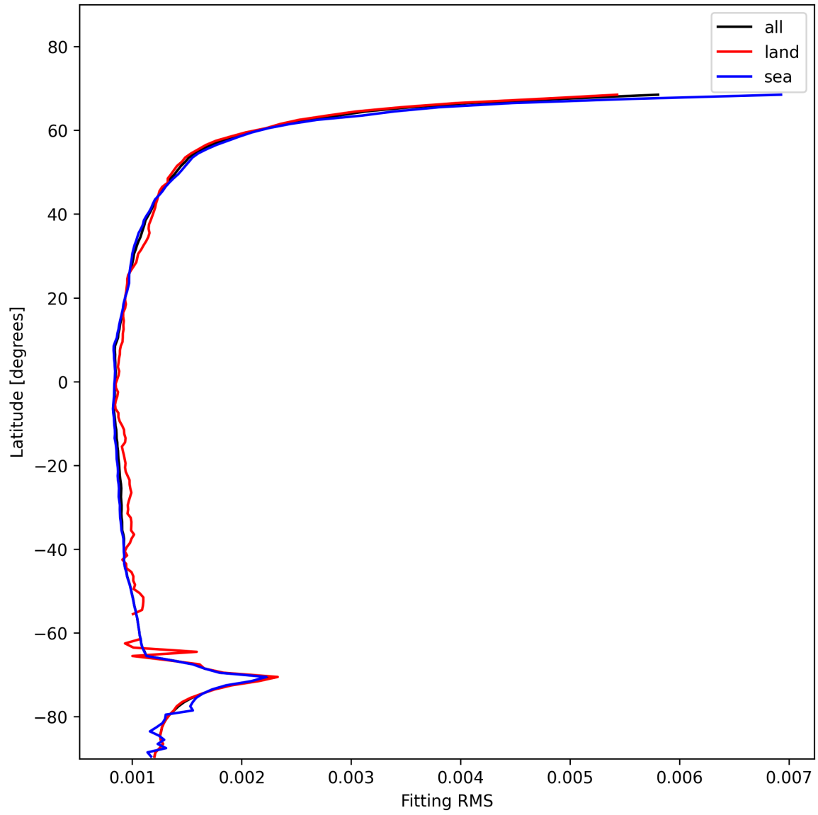
Figure 16: Zonal average of “Fitting RMS” for 2025-11-23 to 2025-11-25.
