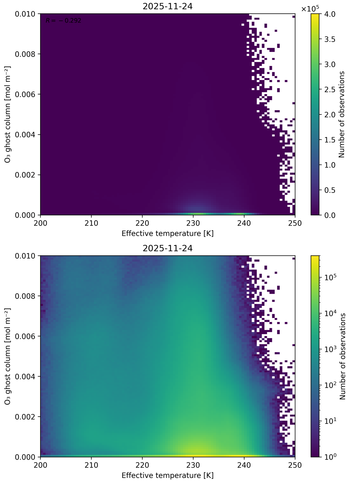
Figure 38: Scatter density plot of “Effective temperature” against “O 3 ghost column” for 2025-11-23 to 2025-11-25.
