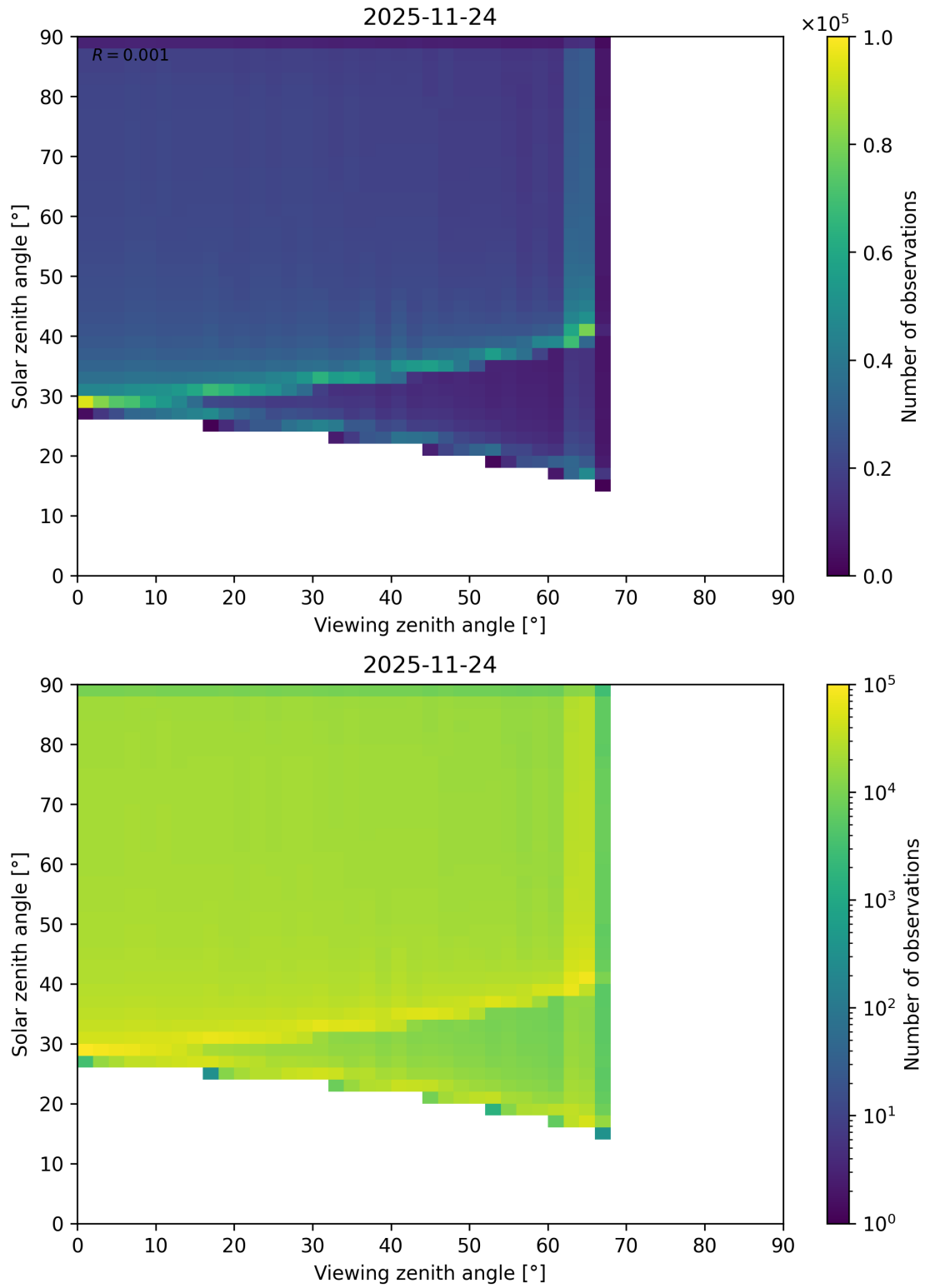
Figure 54: Scatter density plot of “Viewing zenith angle” against “Solar zenith angle” for 2025-11-23 to 2025-11-25.
