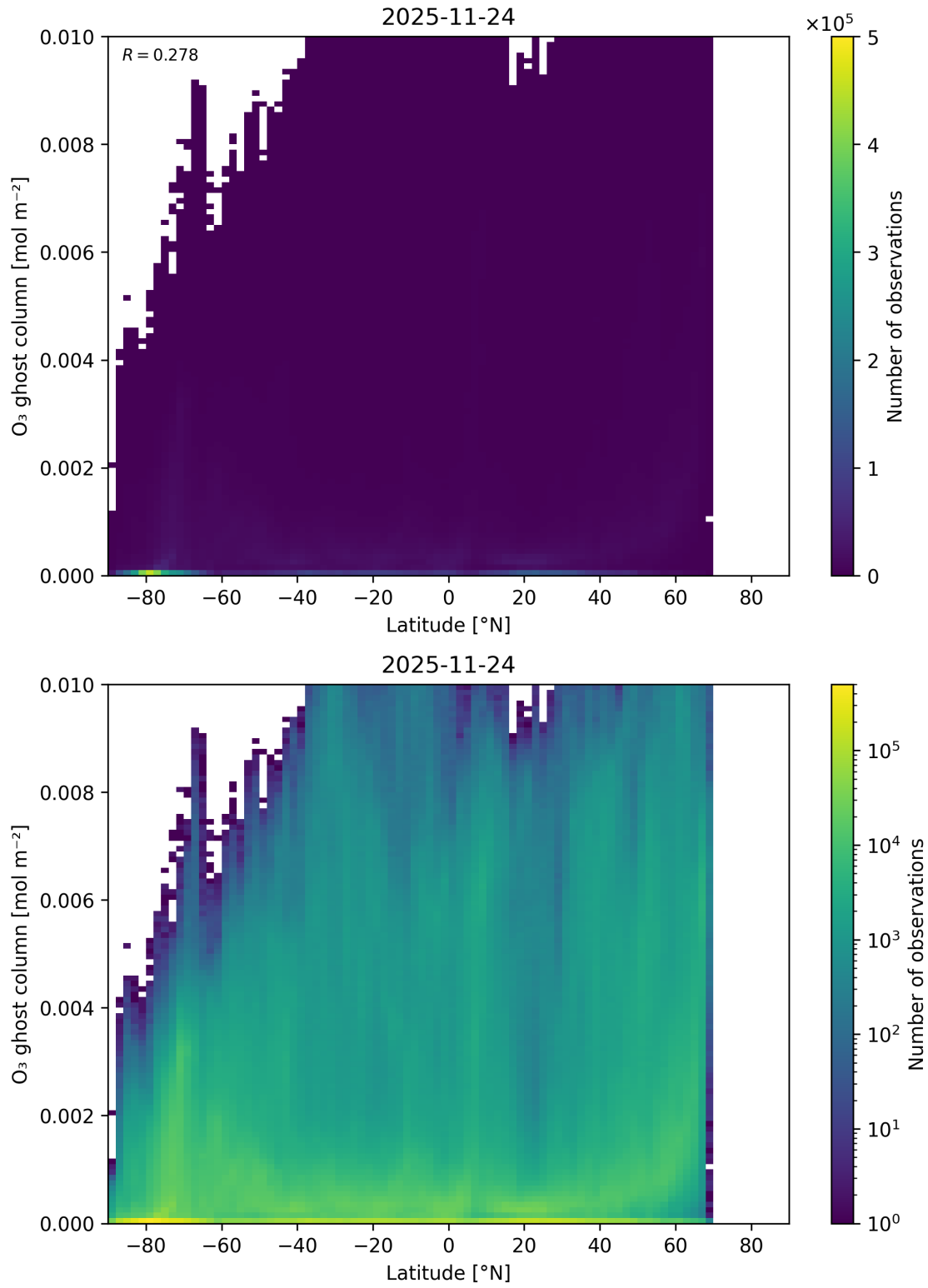
Figure 35: Scatter density plot of “Latitude” against “O 3 ghost column” for 2025-11-23 to 2025-11-25.
