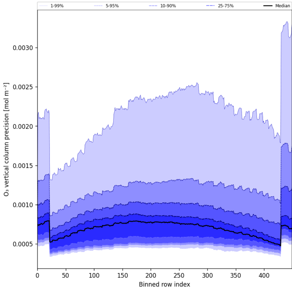
Figure 29: Along track statistics of “O 3 vertical column precision” for 2025-11-23 to 2025-11-25
