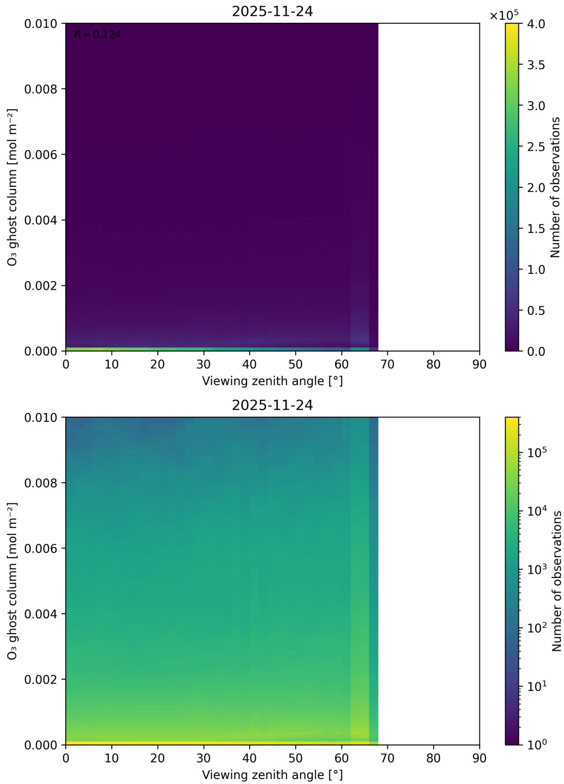
Figure 51: Scatter density plot of “Viewing zenith angle” against “O 3 ghost column” for 2025-11-23 to 2025-11-25.
