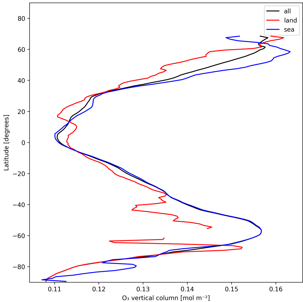
Figure 14: Zonal average of “O 3 vertical column” for 2025-11-23 to 2025-11-25.
