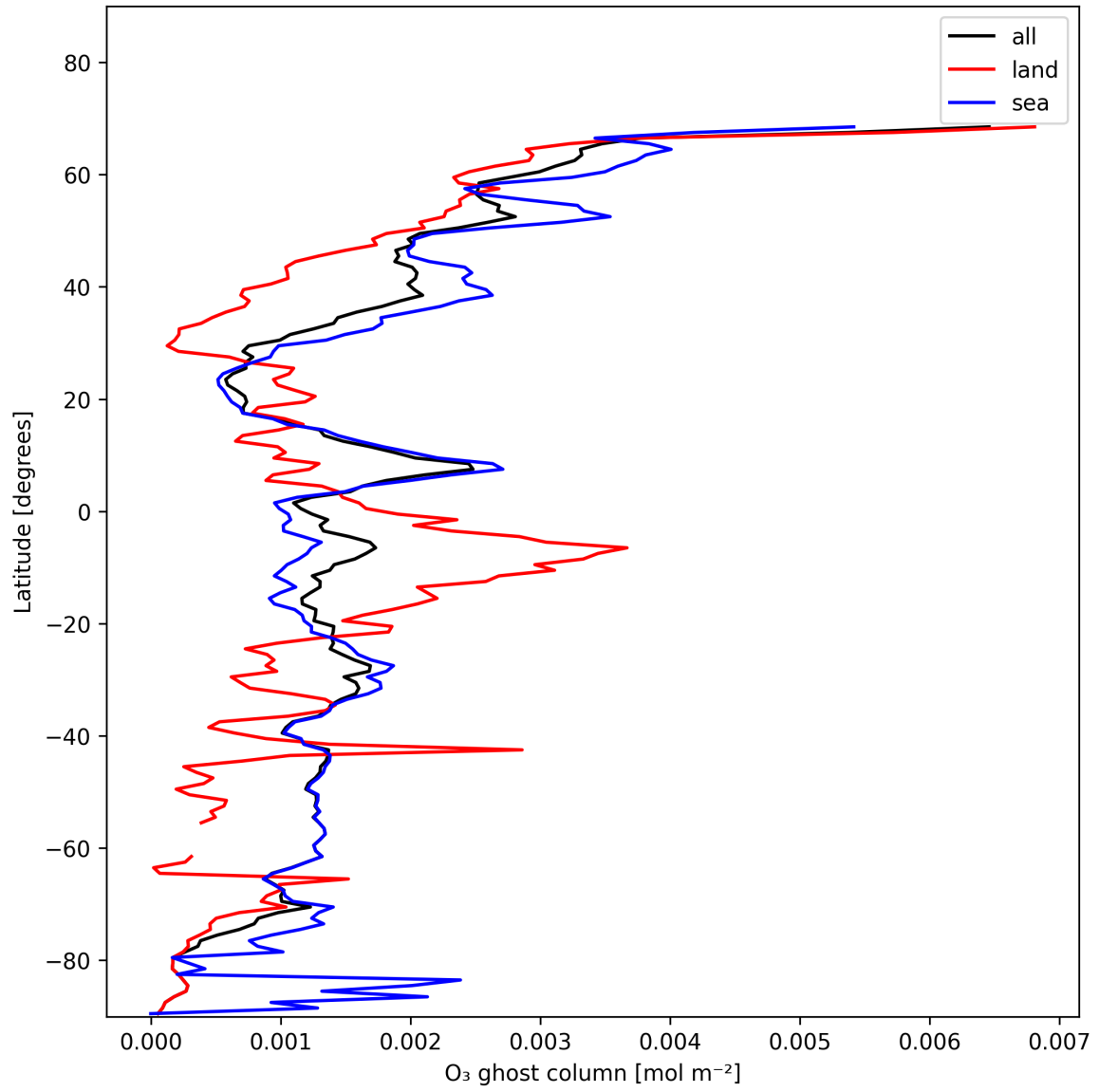
Figure 18: Zonal average of “O 3 ghost column” for 2025-11-23 to 2025-11-25.
