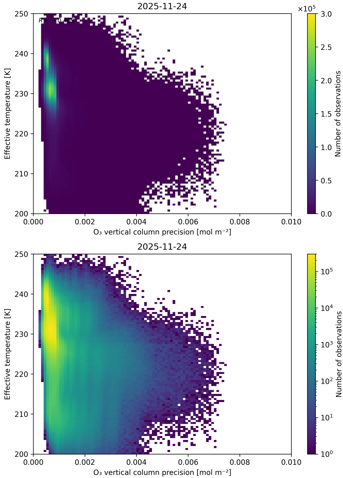
Figure 42: Scatter density plot of “O 3 vertical column precision” against “Effective temperature” for 2025-11-23 to 2025-11-25.
