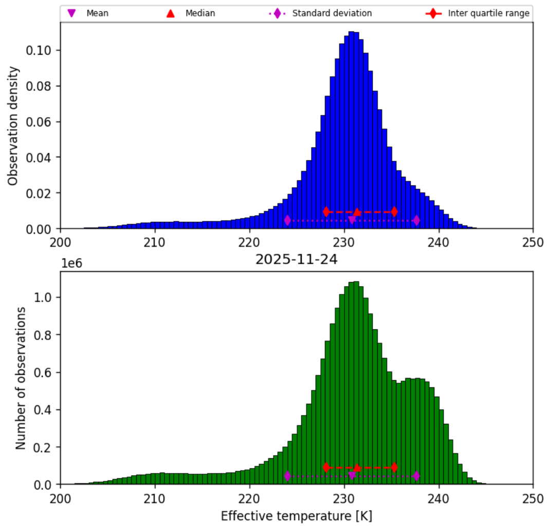
Figure 24: Histogram of “Effective temperature” for 2025-11-23 to 2025-11-25
