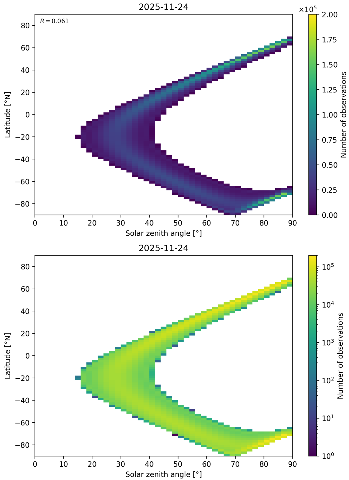
Figure 44: Scatter density plot of “Solar zenith angle” against “Latitude” for 2025-11-23 to 2025-11-25.
