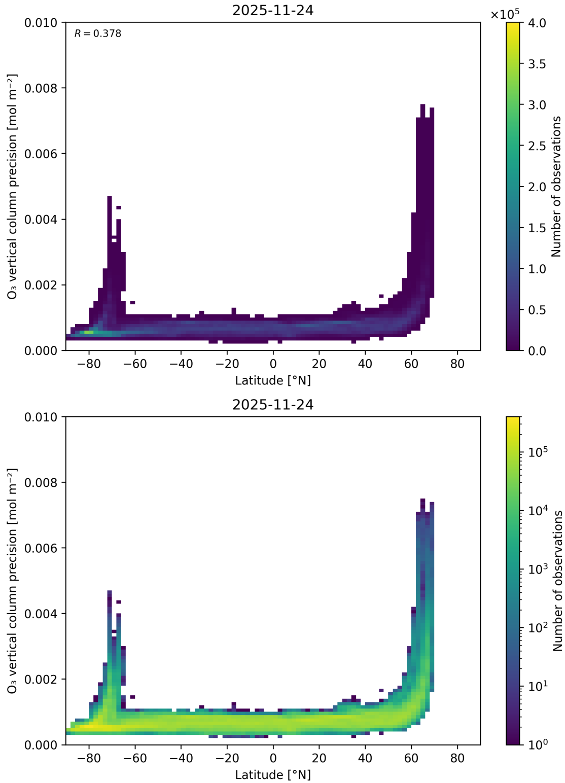
Figure 37: Scatter density plot of “Latitude” against “O 3 vertical column precision” for 2025-11-23 to 2025-11-25.
