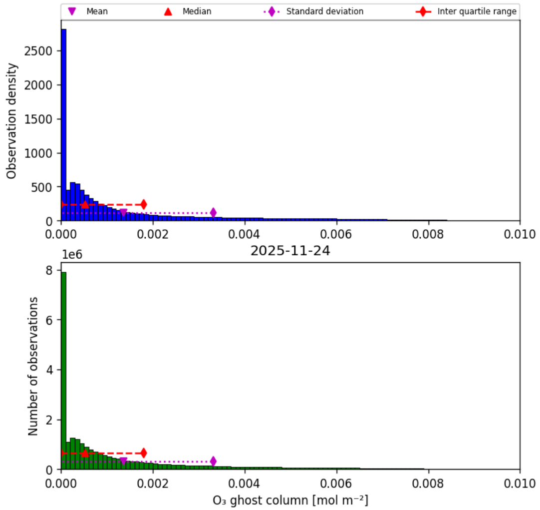
Figure 25: Histogram of “O 3 ghost column” for 2025-11-23 to 2025-11-25
