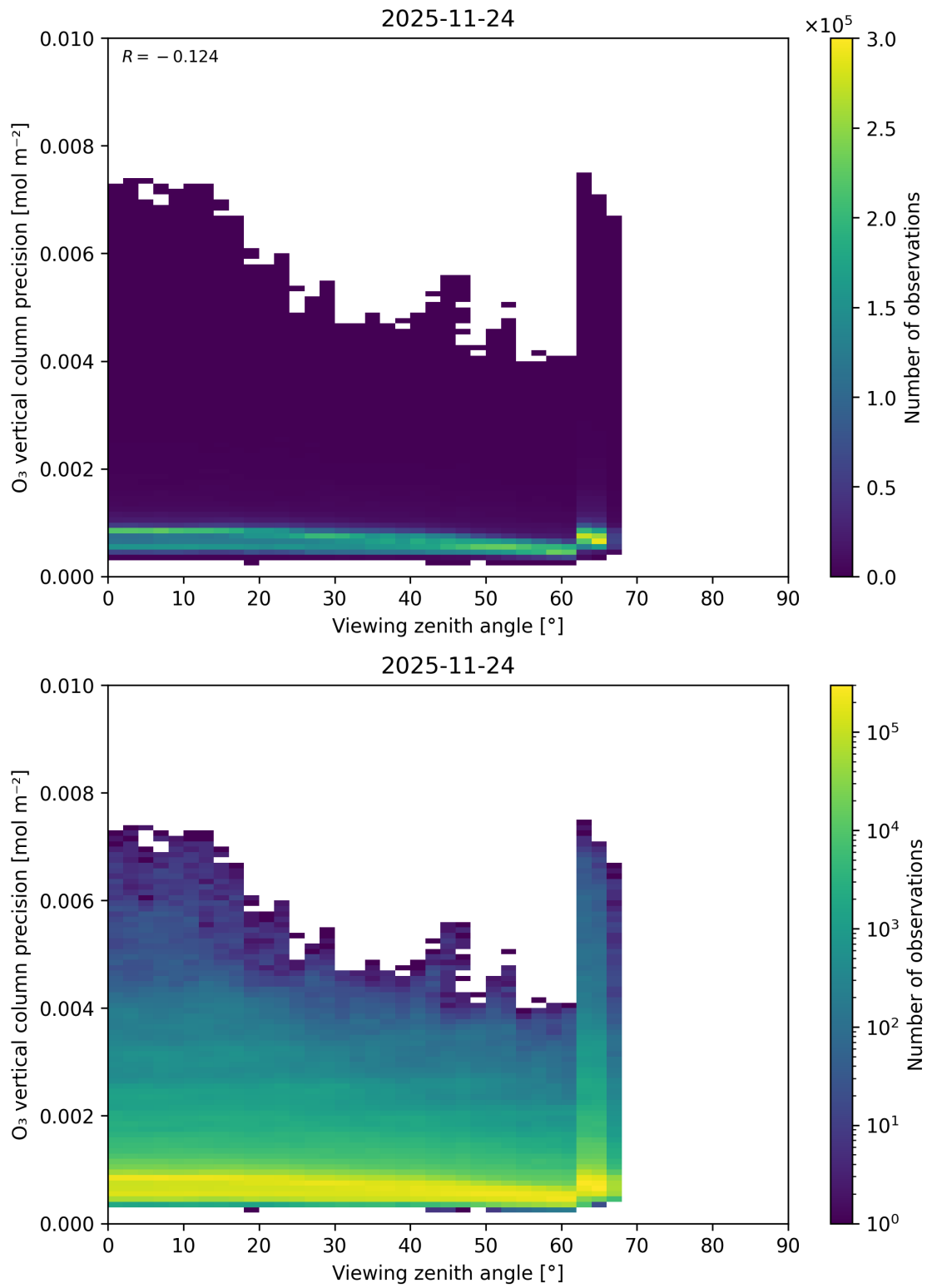
Figure 53: Scatter density plot of “Viewing zenith angle” against “O 3 vertical column precision” for 2025-11-23 to 2025-11-25.
