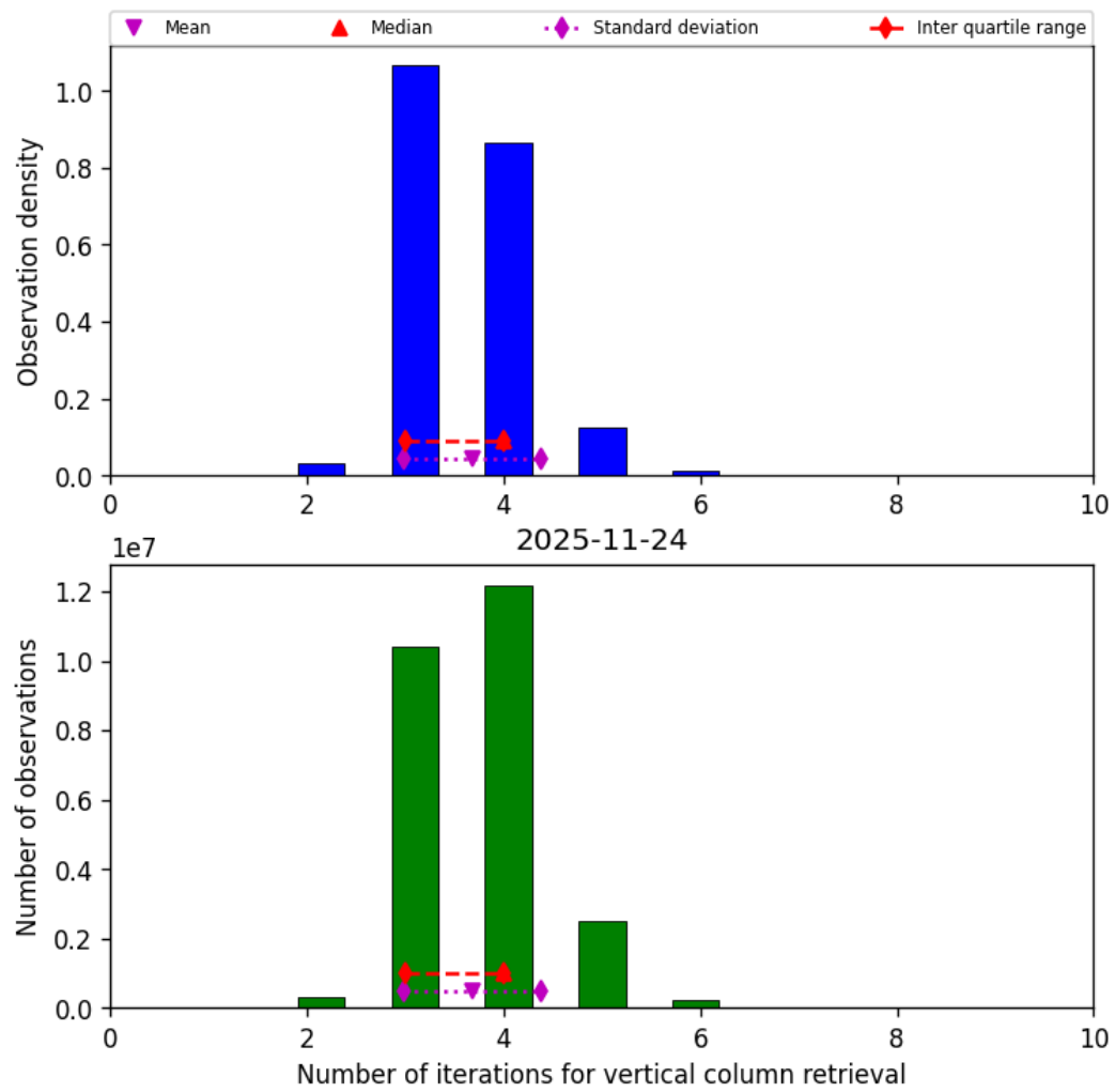
Figure 26: Histogram of “Number of iterations for vertical column retrieval” for 2025-11-23 to 2025-11-25
