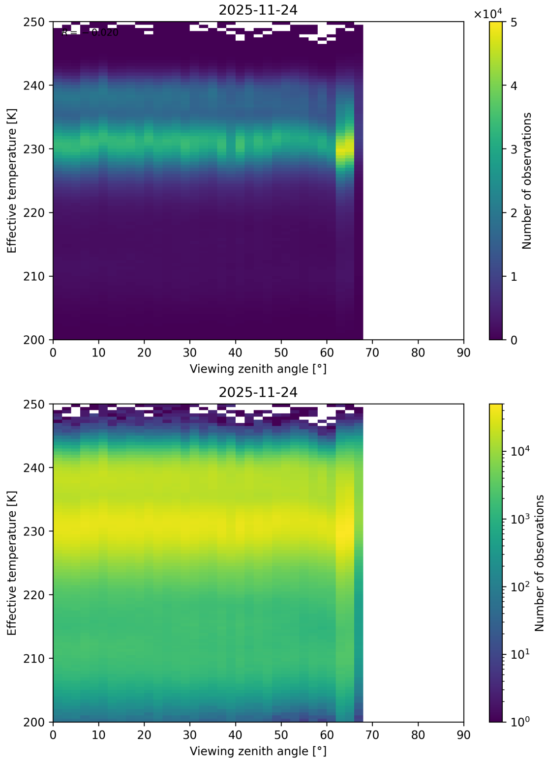
Figure 50: Scatter density plot of “Viewing zenith angle” against “Effective temperature” for 2025-11-23 to 2025-11-25.
