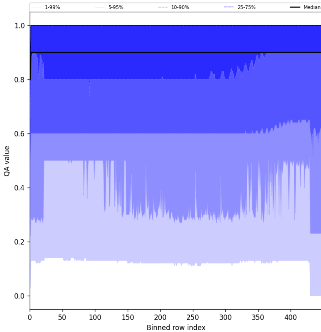
Figure 27: Along track statistics of “QA value” for 2025-11-23 to 2025-11-25
