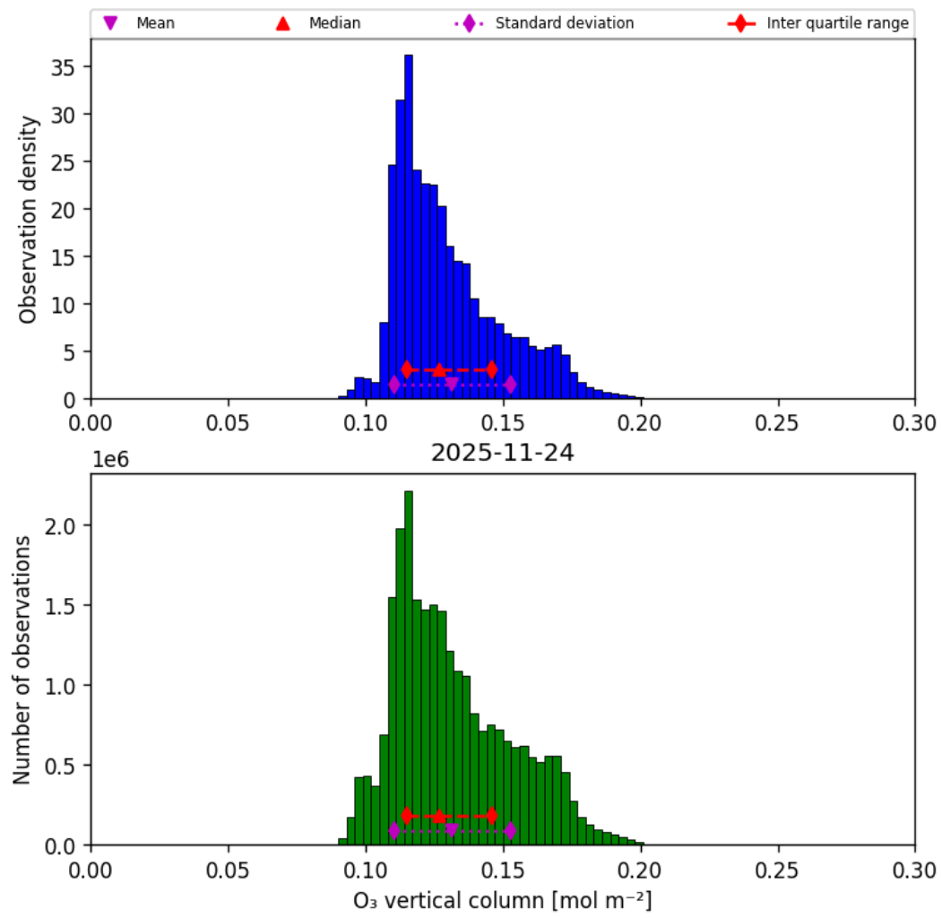
Figure 21: Histogram of “O 3 vertical column” for 2025-11-23 to 2025-11-25
