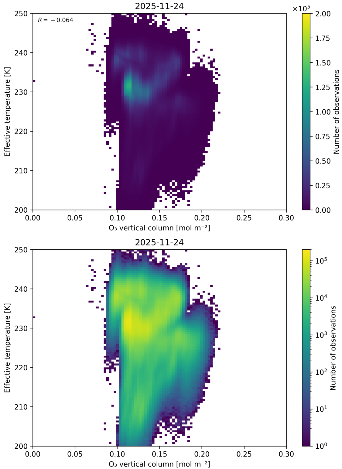
Figure 39: Scatter density plot of “O 3 vertical column” against “Effective temperature” for 2025-11-23 to 2025-11-25.
