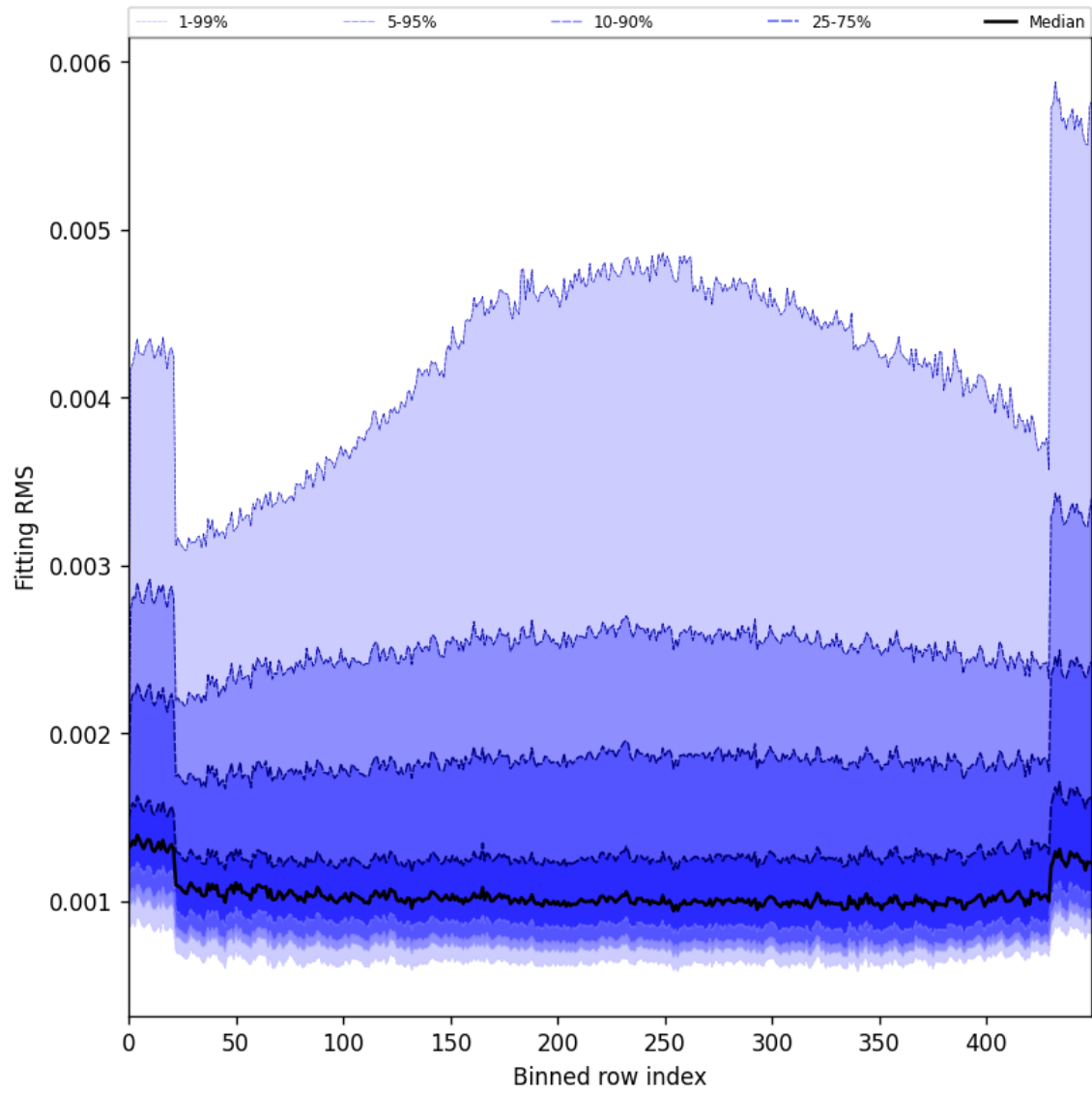
Figure 30: Along track statistics of “Fitting RMS” for 2025-11-23 to 2025-11-25
