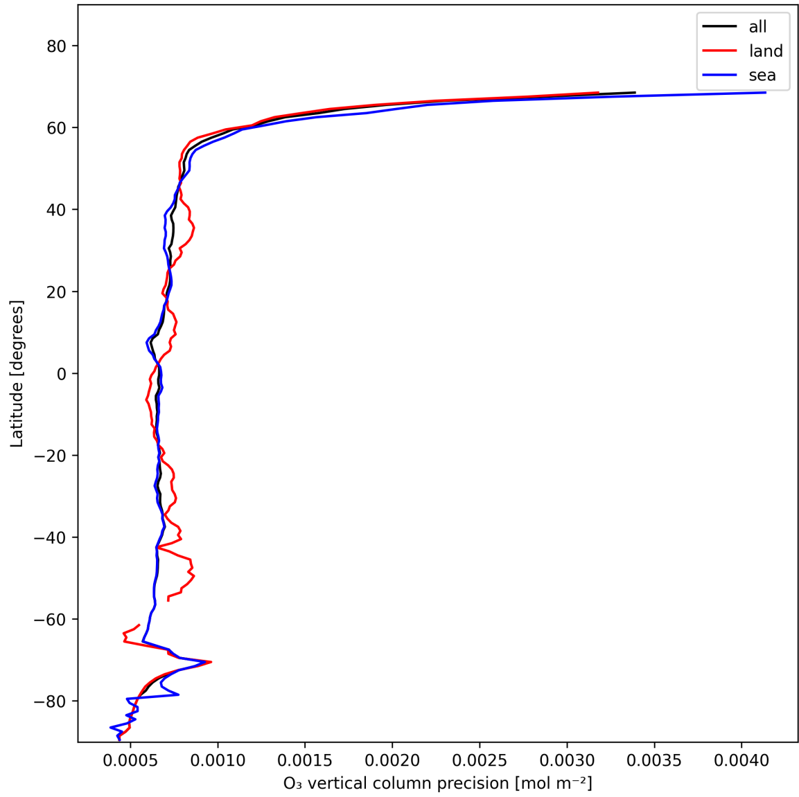
Figure 15: Zonal average of “O 3 vertical column precision” for 2025-11-23 to 2025-11-25.
