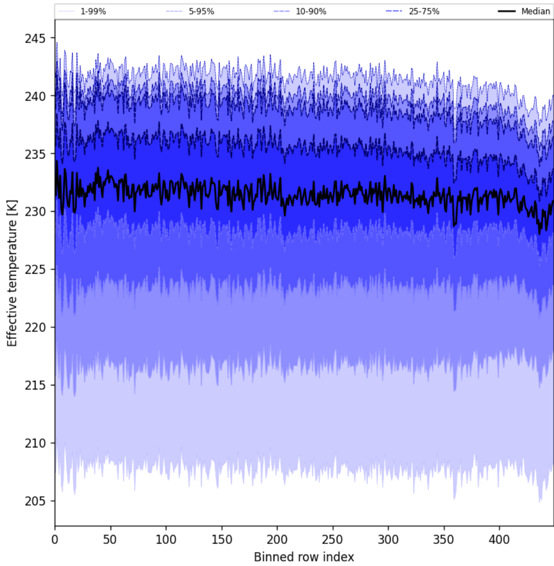
Figure 31: Along track statistics of “Effective temperature” for 2025-11-23 to 2025-11-25
