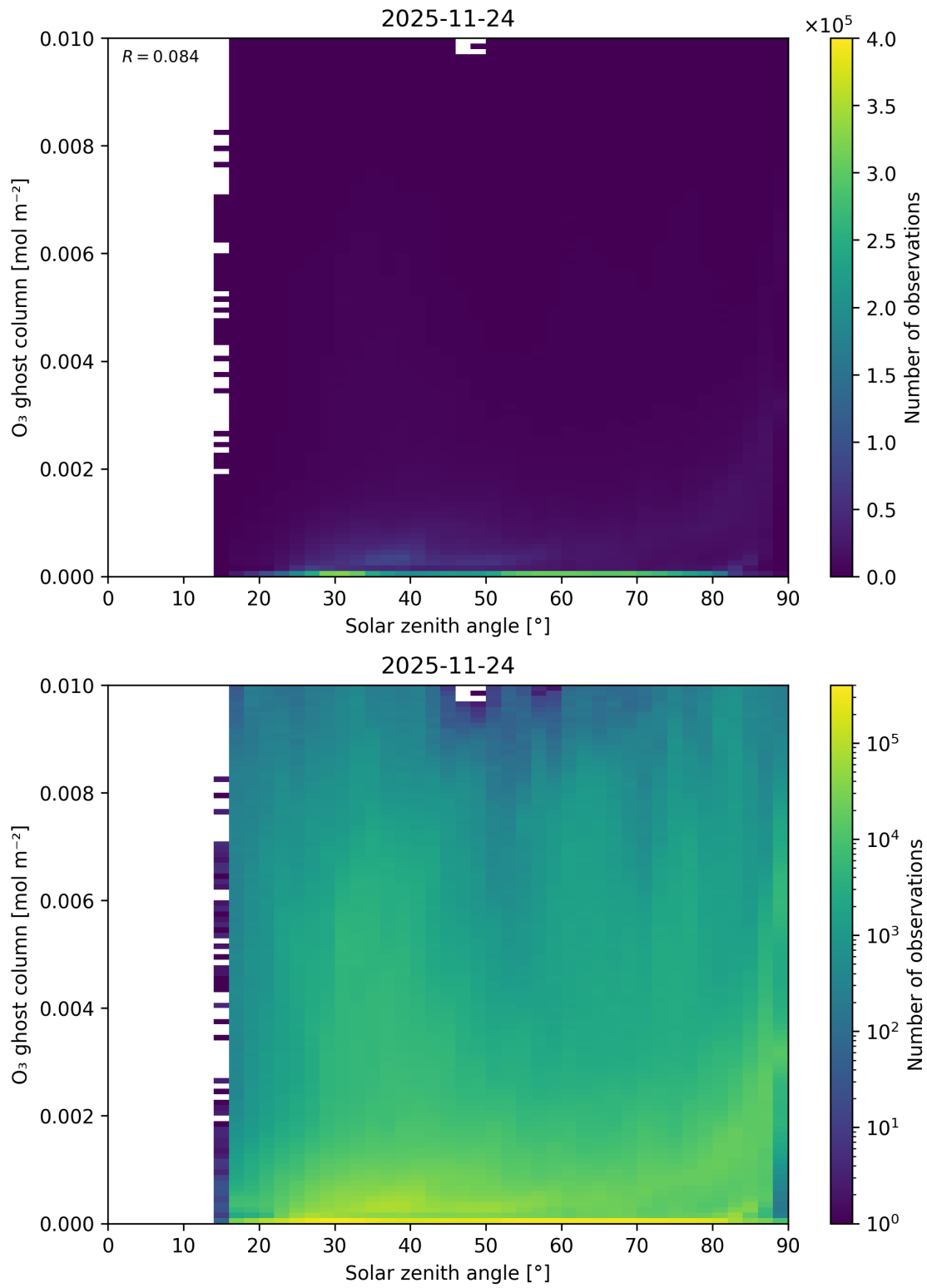
Figure 46: Scatter density plot of “Solar zenith angle” against “O 3 ghost column” for 2025-11-23 to 2025-11-25.
