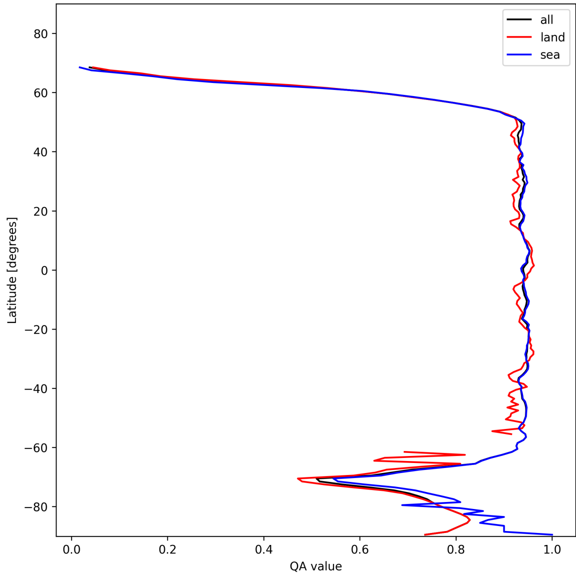
Figure 13: Zonal average of “QA value” for 2025-11-23 to 2025-11-25.
