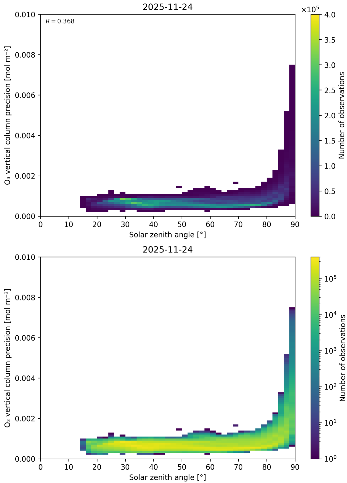
Figure 48: Scatter density plot of “Solar zenith angle” against “O 3 vertical column precision” for 2025-11-23 to 2025-11-25.
