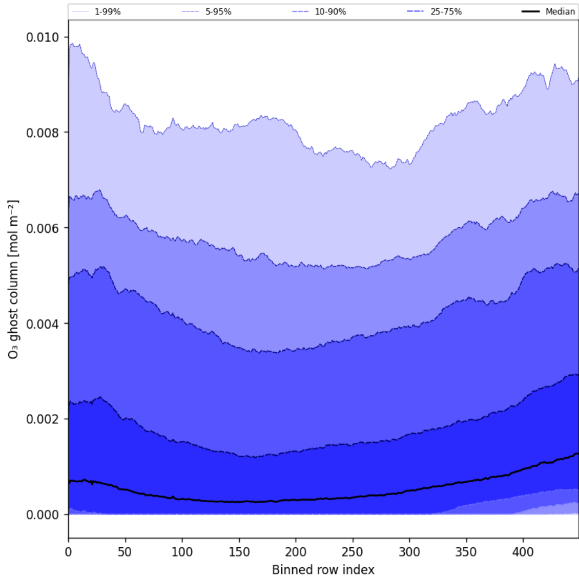
Figure 32: Along track statistics of "O 3 ghost column" for 2025-11-23 to 2025-11-25
