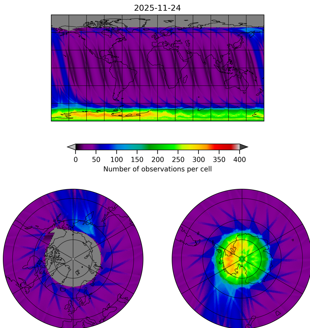
Figure 12: Map of the number of observations for 2025-11-23 to 2025-11-25
