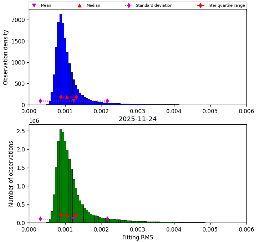
Figure 23: Histogram of “Fitting RMS” for 2025-11-23 to 2025-11-25
