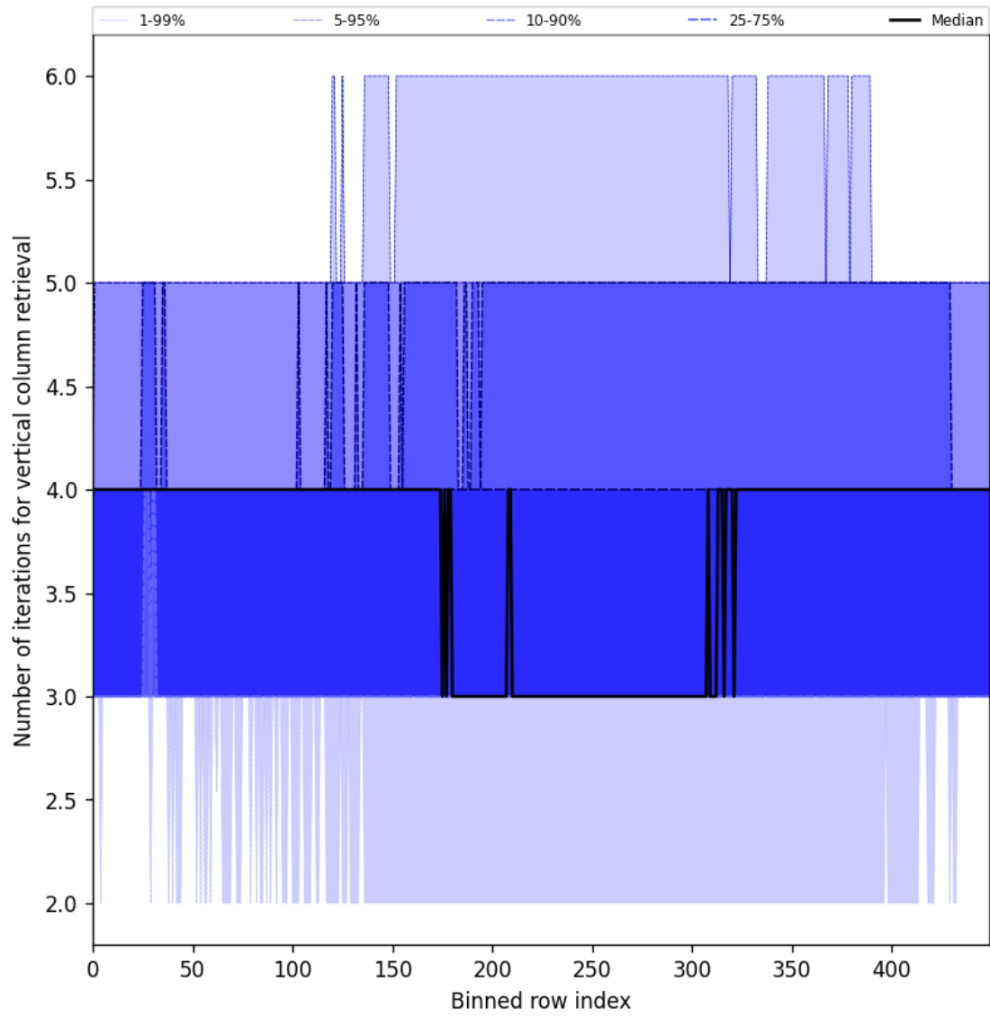
Figure 33: Along track statistics of “Number of iterations for vertical column retrieval” for 2025-11-23 to 2025-11-25
