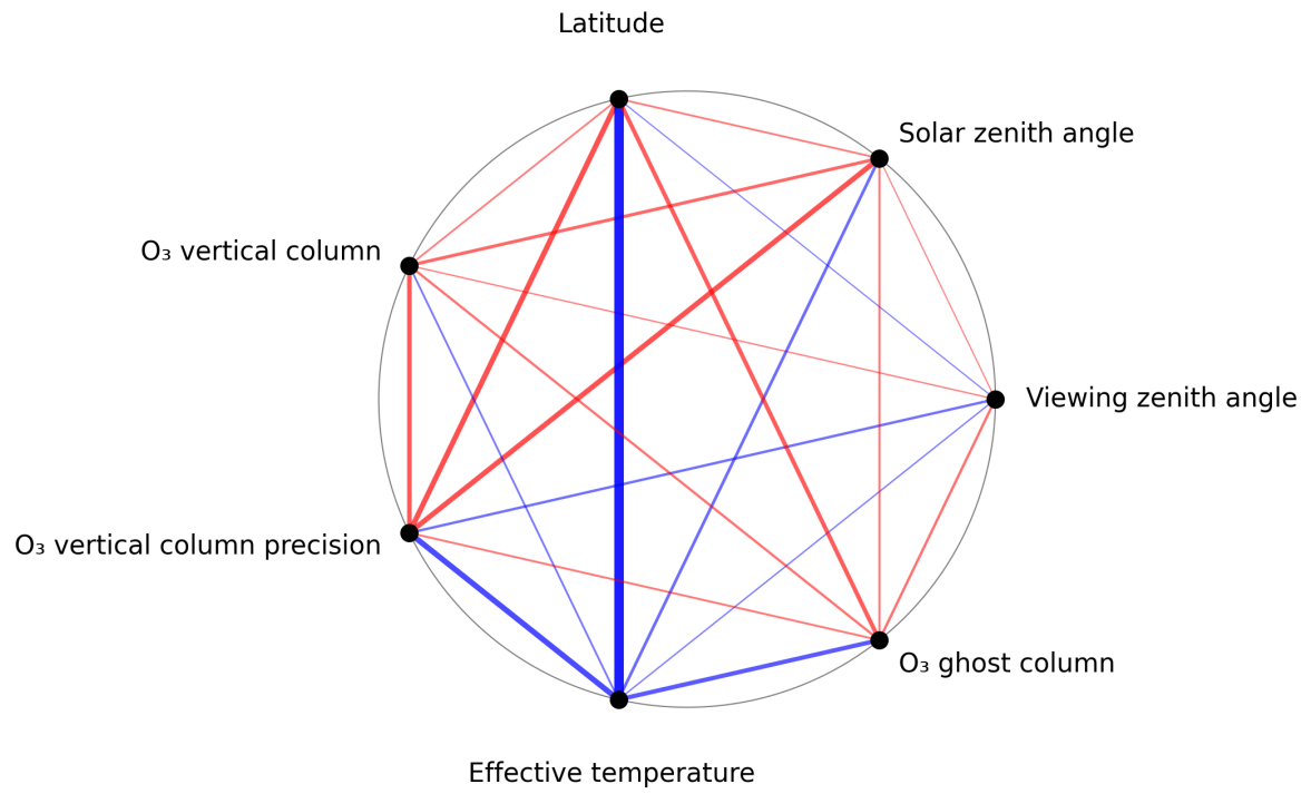
Figure 1: Map of correlation graph for 2025-11-23 to 2025-11-25.
