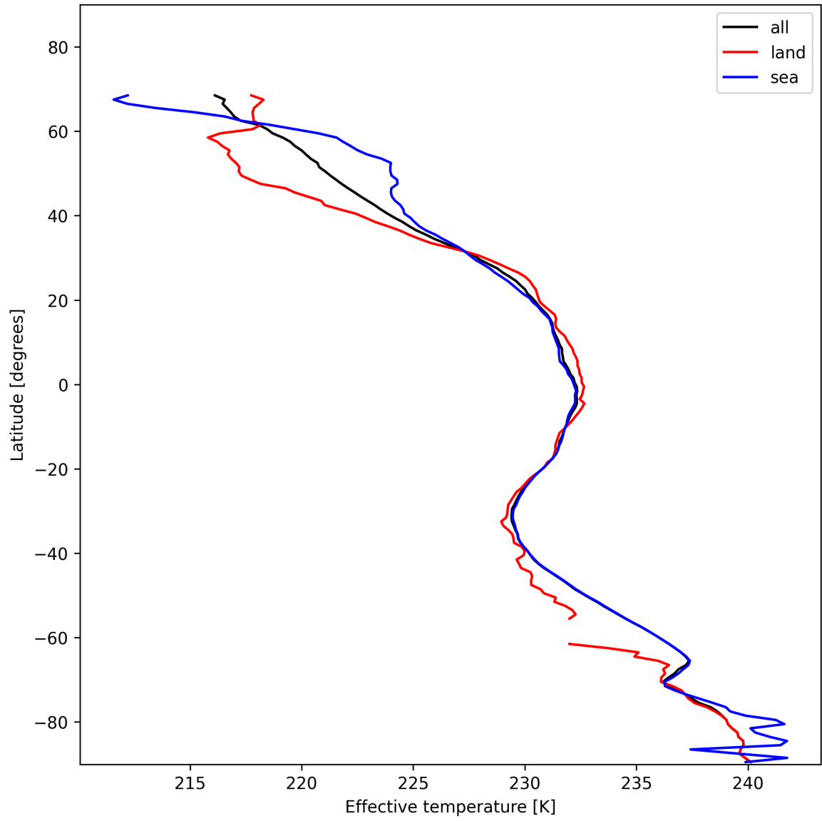
Figure 17: Zonal average of “Effective temperature” for 2025-11-23 to 2025-11-25.
