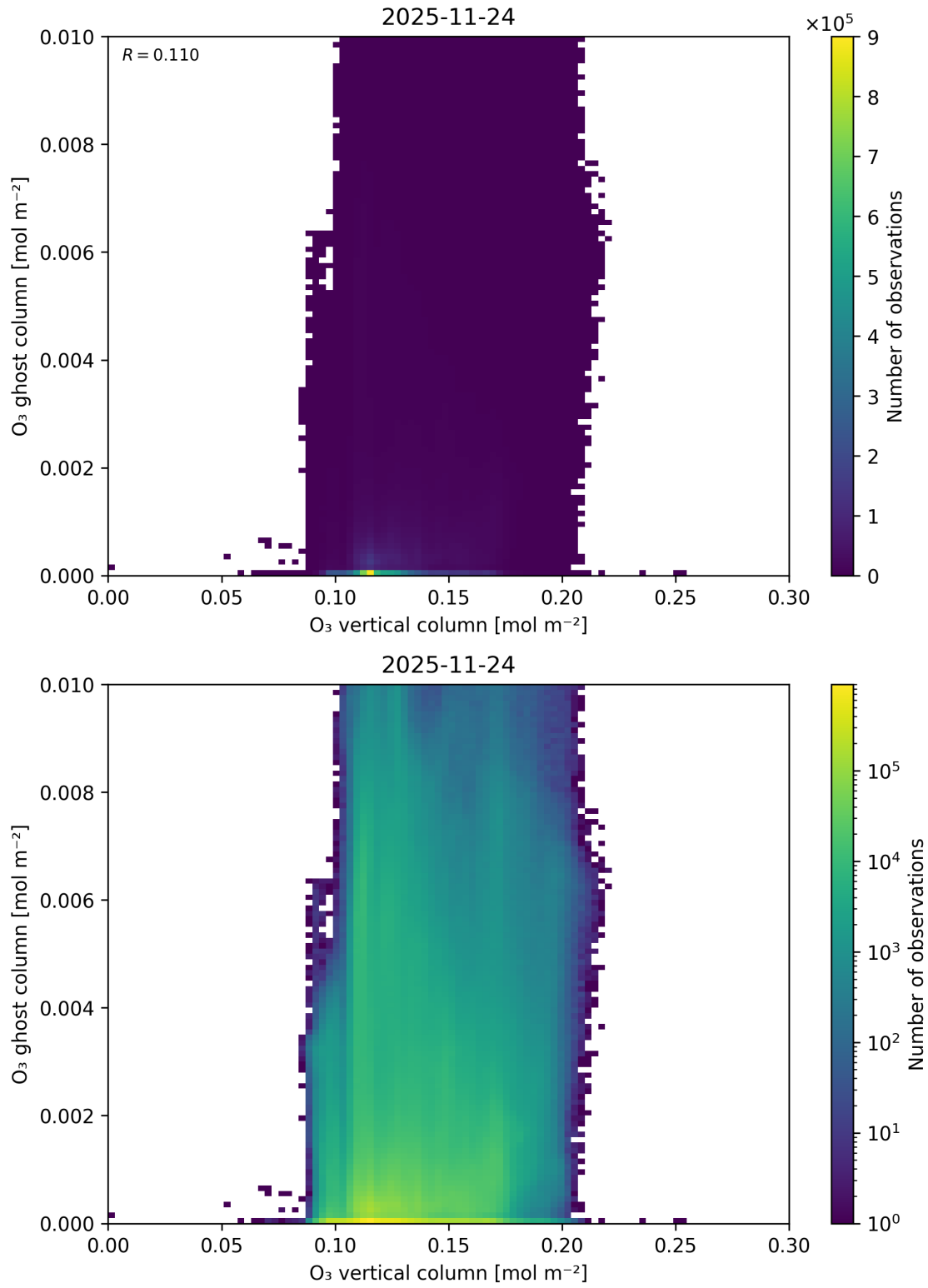
Figure 40: Scatter density plot of “O 3 vertical column” against “O 3 ghost column” for 2025-11-23 to 2025-11-25.
