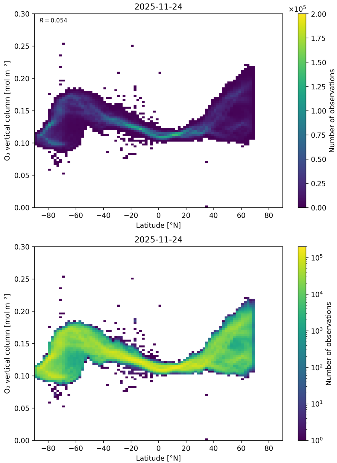
Figure 36: Scatter density plot of “Latitude” against “O 3 vertical column” for 2025-11-23 to 2025-11-25.
