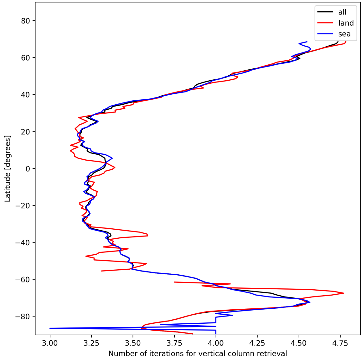
Figure 19: Zonal average of “Number of iterations for vertical column retrieval” for 2025-11-23 to 2025-11-25.
