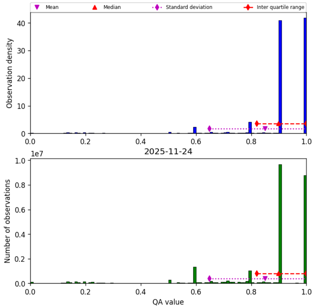
Figure 20: Histogram of “QA value” for 2025-11-23 to 2025-11-25
