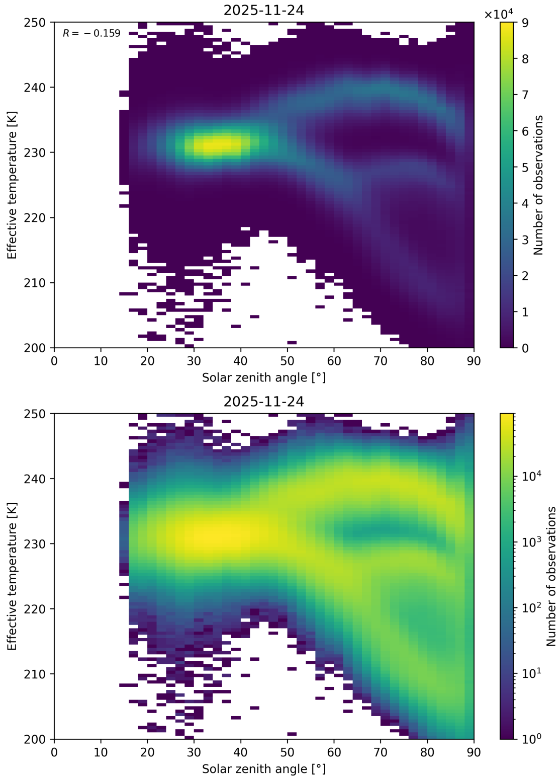
Figure 45: Scatter density plot of “Solar zenith angle” against “Effective temperature” for 2025-11-23 to 2025-11-25.
