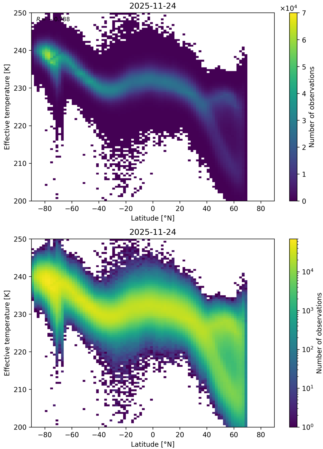
Figure 34: Scatter density plot of “Latitude” against “Effective temperature” for 2025-11-23 to 2025-11-25.
