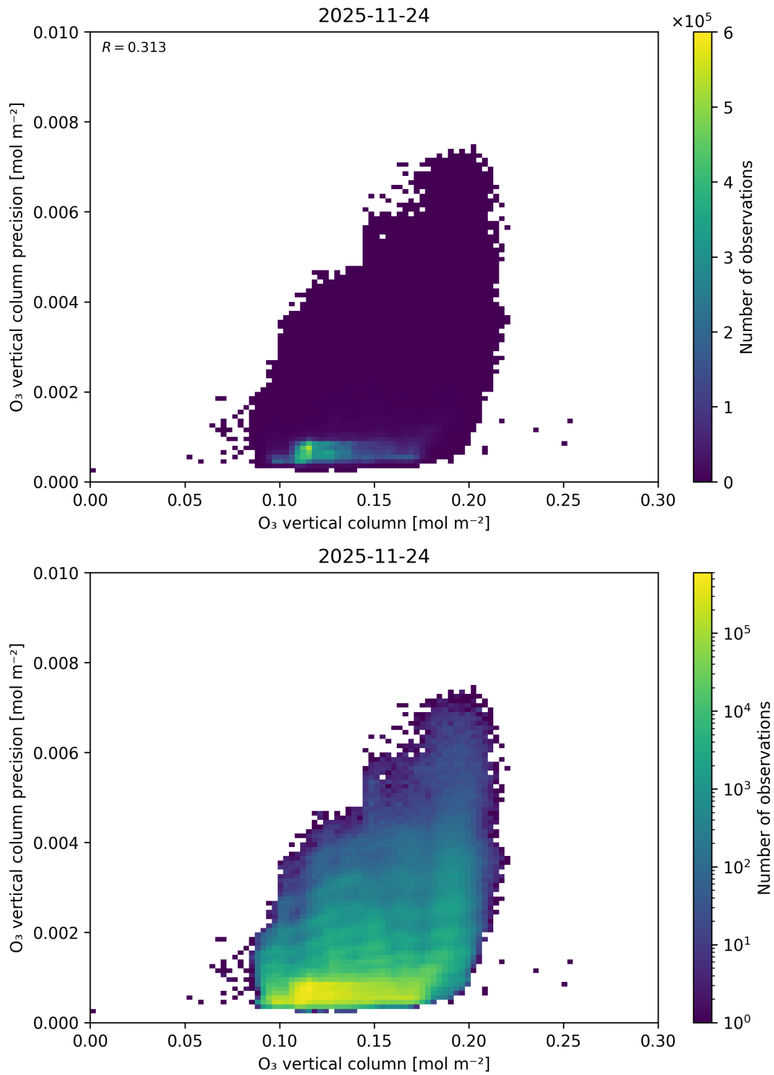
Figure 41: Scatter density plot of “O 3 vertical column” against “O 3 vertical column precision” for 2025-11-23 to 2025-11-25.
