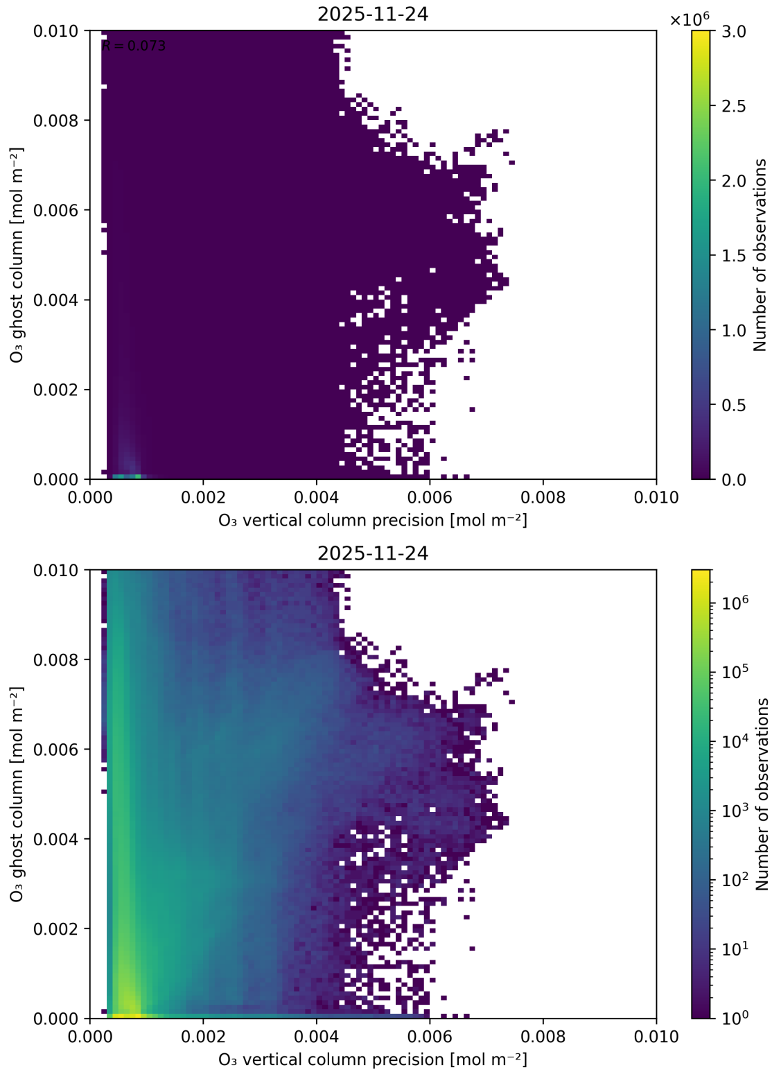
Figure 43: Scatter density plot of “ O_3 vertical column precision” against “ O_3 ghost column” for 2025-11-23 to 2025-11-25.
