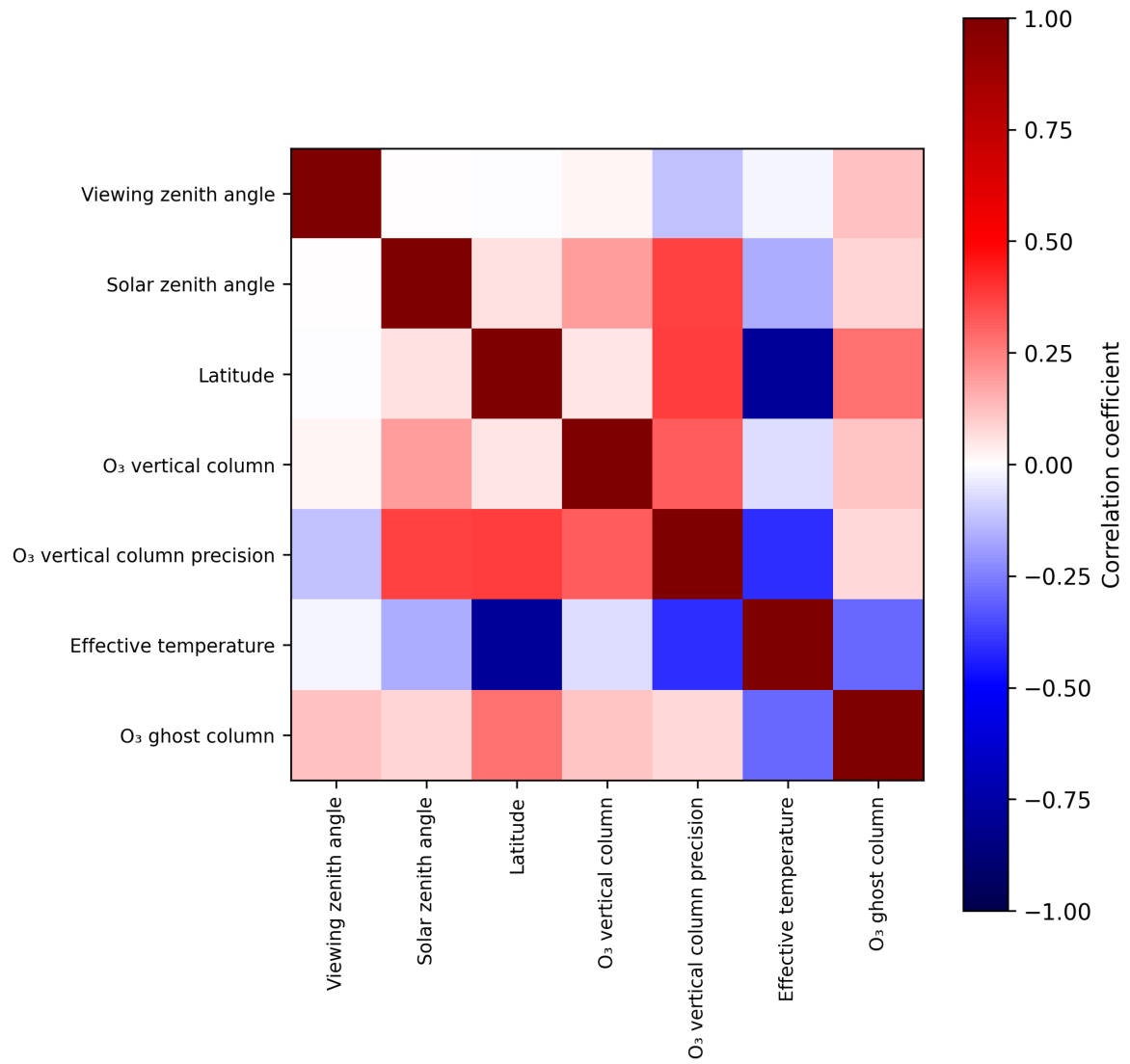
Figure 2: Map of correlation matrix for 2025-11-23 to 2025-11-25.
