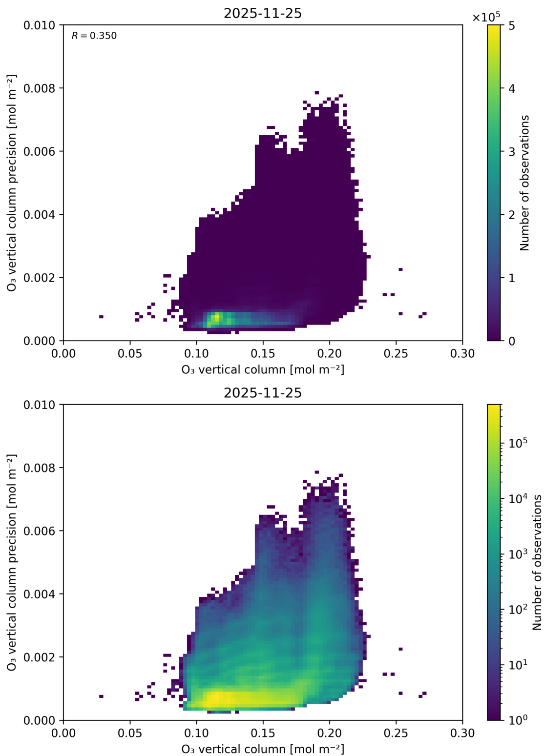
Figure 41: Scatter density plot of “O 3 vertical column” against “O 3 vertical column precision” for 2025-11-24 to 2025-11-26.
