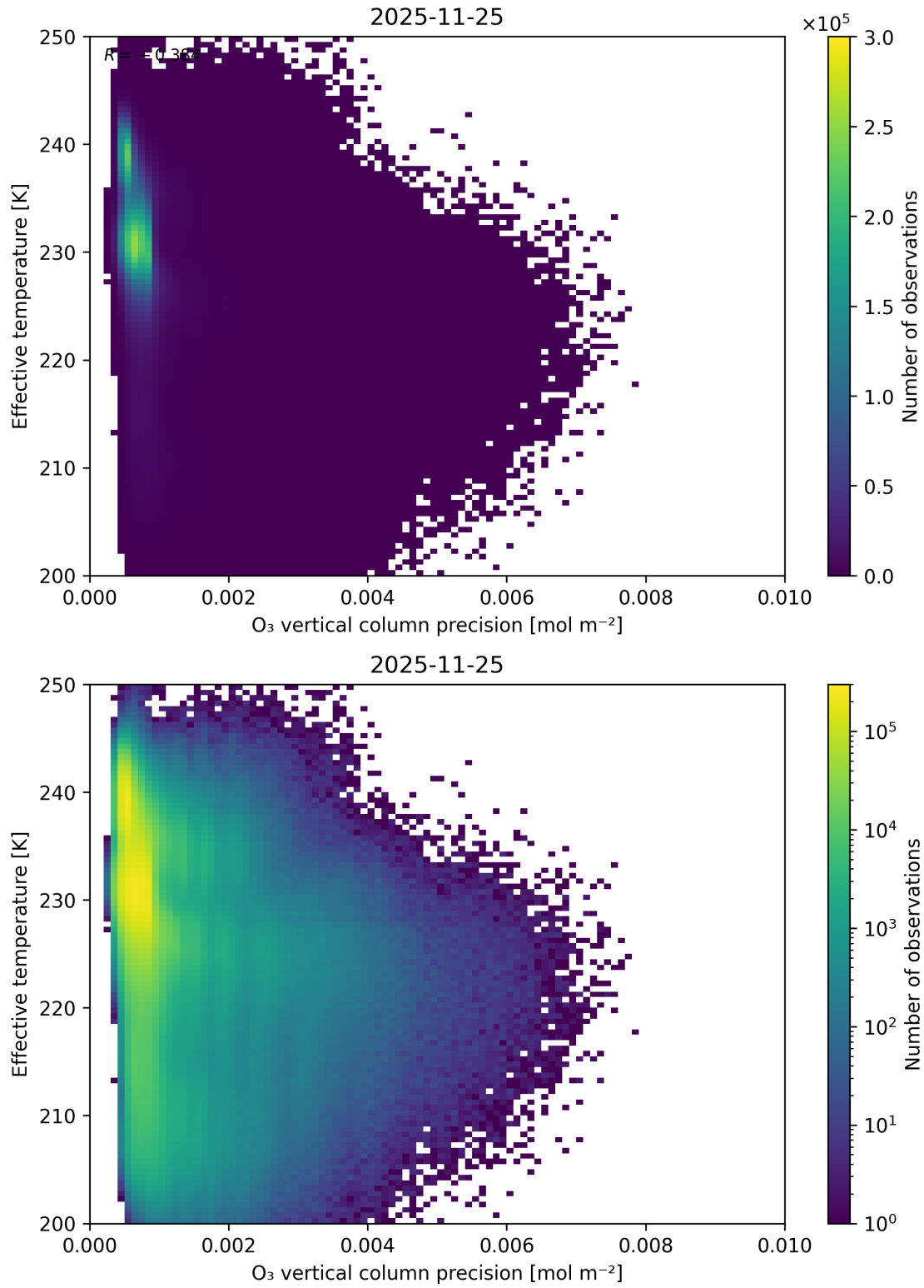
Figure 42: Scatter density plot of “O 3 vertical column precision” against “Effective temperature” for 2025-11-24 to 2025-11-26.
