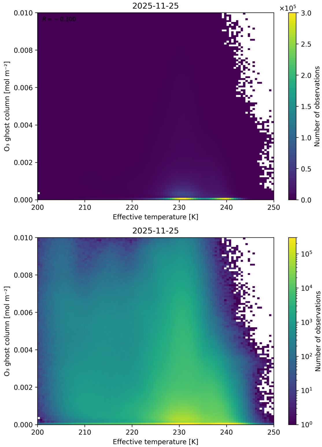
Figure 38: Scatter density plot of “Effective temperature” against “O 3 ghost column” for 2025-11-24 to 2025-11-26.
