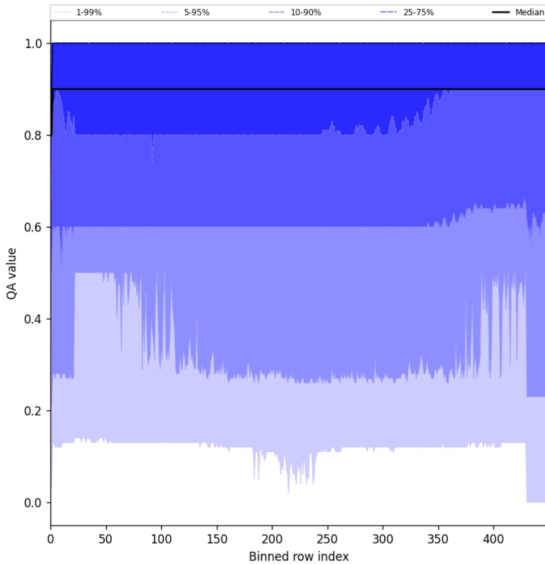
Figure 27: Along track statistics of “QA value” for 2025-11-24 to 2025-11-26
