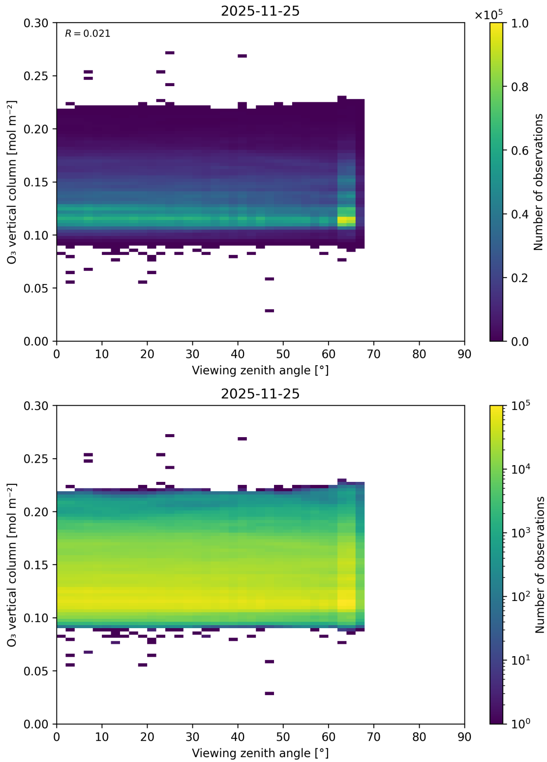
Figure 52: Scatter density plot of “Viewing zenith angle” against “O 3 vertical column” for 2025-11-24 to 2025-11-26.
