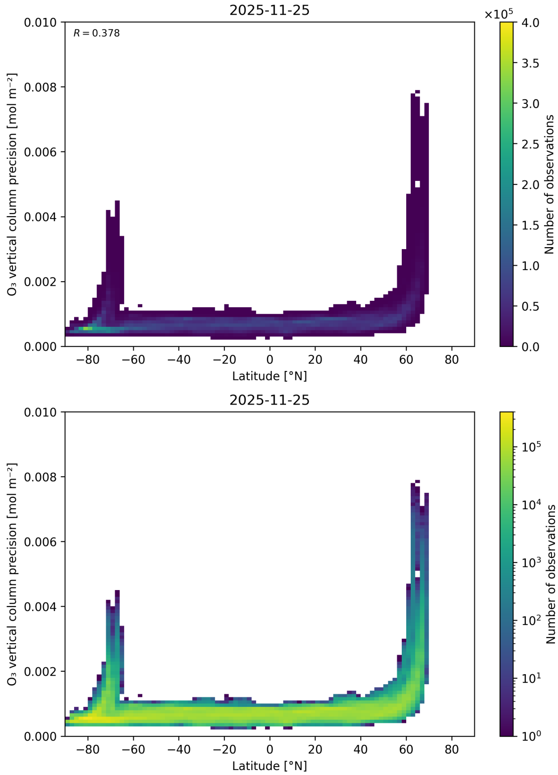
Figure 37: Scatter density plot of “Latitude” against “O 3 vertical column precision” for 2025-11-24 to 2025-11-26.
