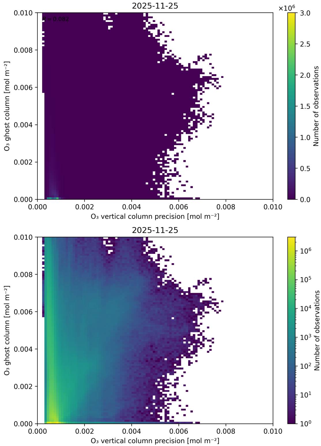
Figure 43: Scatter density plot of “ \text{O}_3 vertical column precision” against “ \text{O}_3 ghost column” for 2025-11-24 to 2025-11-26.
