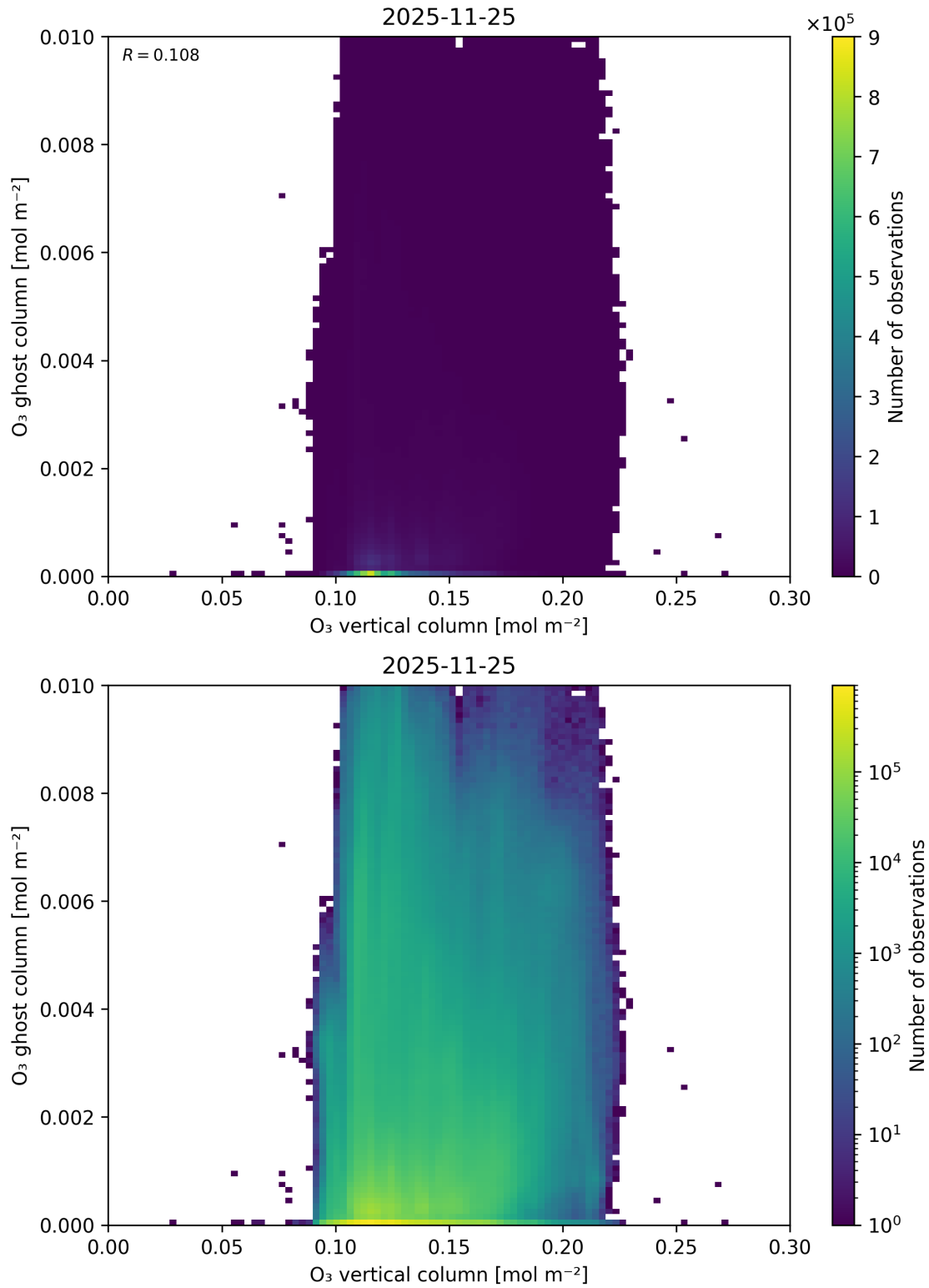
Figure 40: Scatter density plot of “O 3 vertical column” against “O 3 ghost column” for 2025-11-24 to 2025-11-26.
