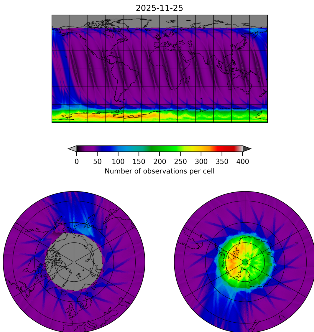
Figure 12: Map of the number of observations for 2025-11-24 to 2025-11-26
