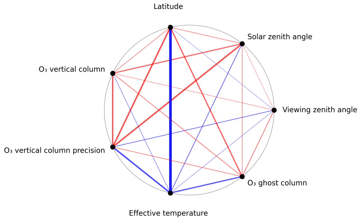
Figure 1: Map of correlation graph for 2025-11-24 to 2025-11-26.
