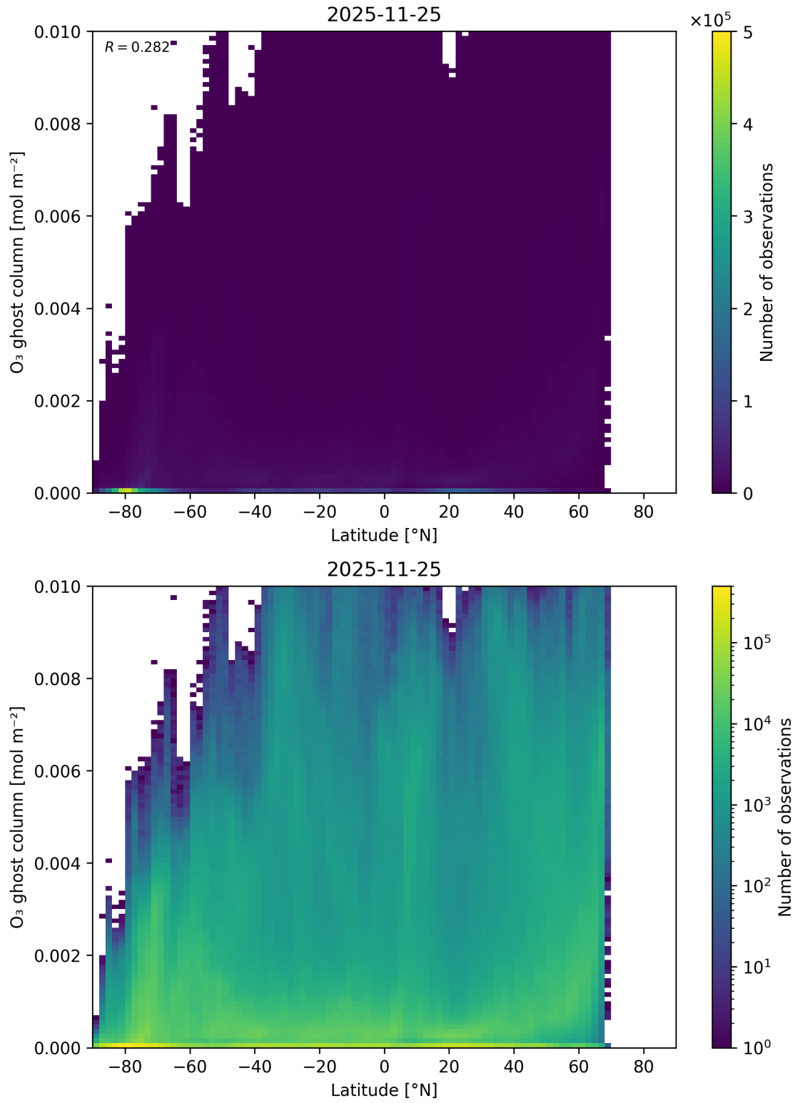
Figure 35: Scatter density plot of “Latitude” against “O 3 ghost column” for 2025-11-24 to 2025-11-26.
