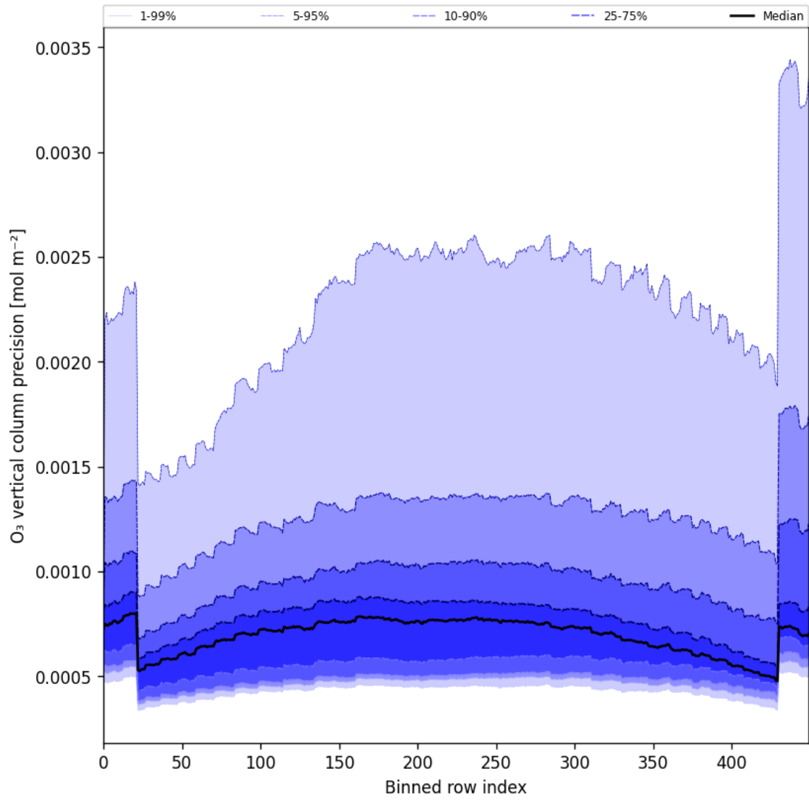
Figure 29: Along track statistics of “O 3 vertical column precision” for 2025-11-24 to 2025-11-26
