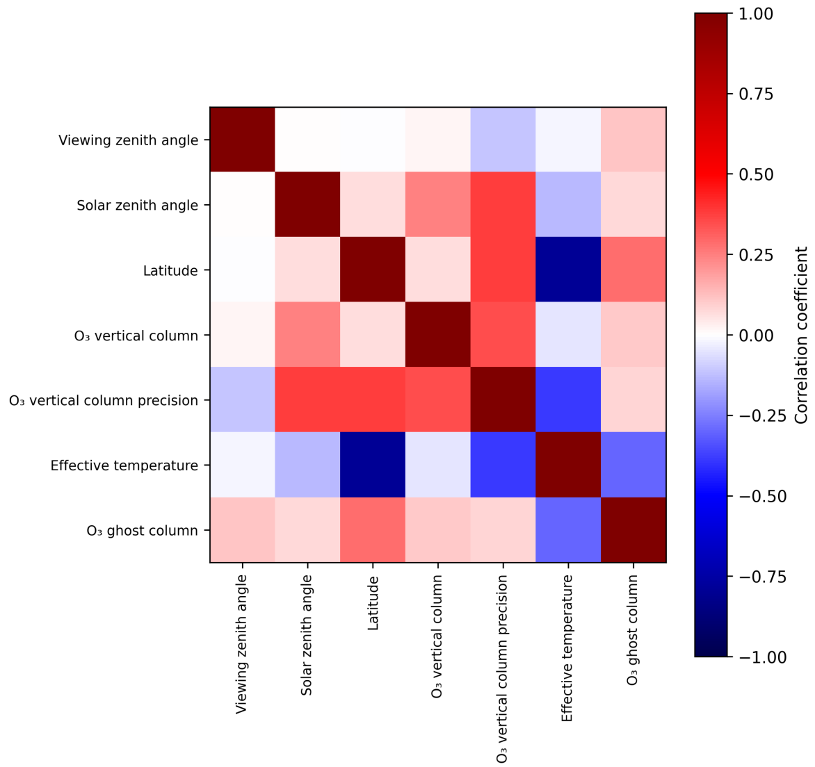
Figure 2: Map of correlation matrix for 2025-11-24 to 2025-11-26.
