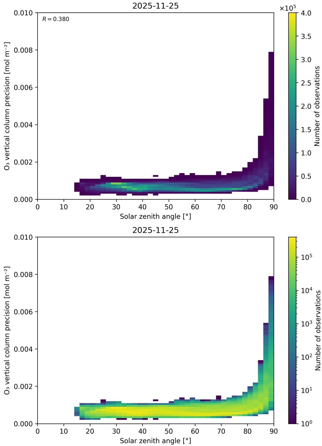
Figure 48: Scatter density plot of “Solar zenith angle” against “O 3 vertical column precision” for 2025-11-24 to 2025-11-26.
