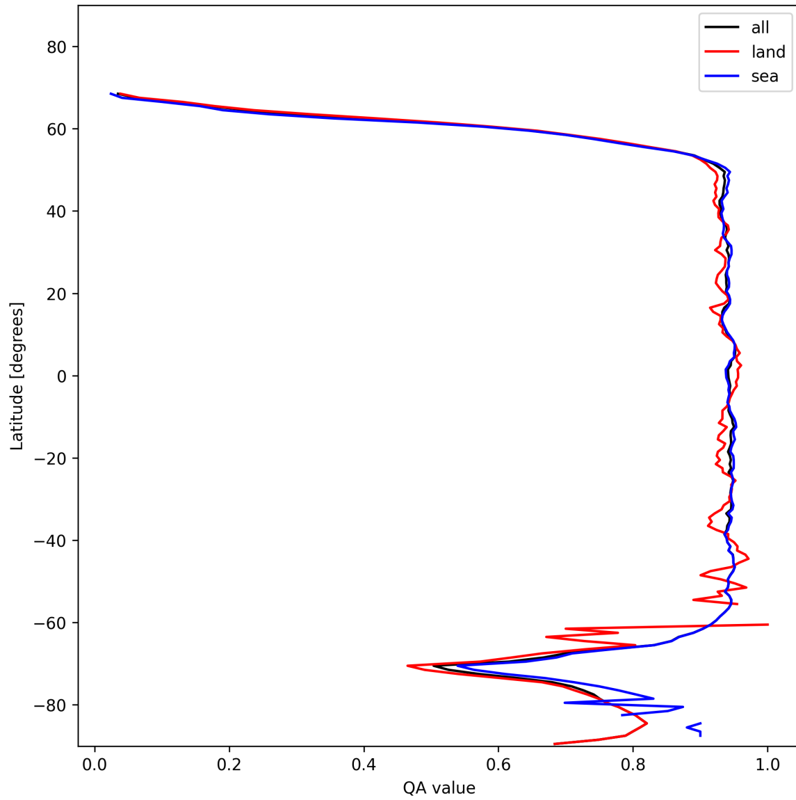
Figure 13: Zonal average of “QA value” for 2025-11-24 to 2025-11-26.
