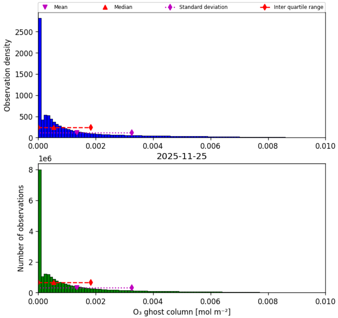
Figure 25: Histogram of “O 3 ghost column” for 2025-11-24 to 2025-11-26
