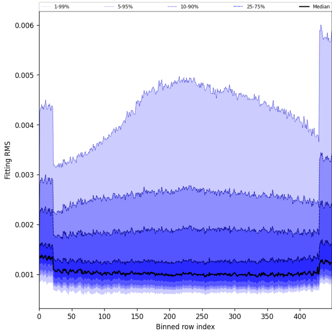
Figure 30: Along track statistics of “Fitting RMS” for 2025-11-24 to 2025-11-26
