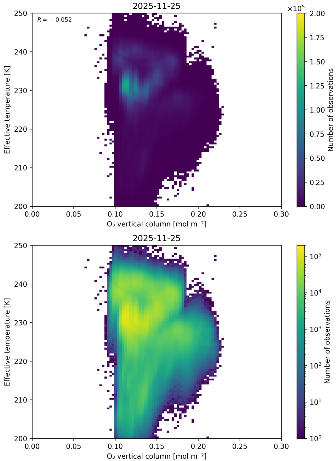
Figure 39: Scatter density plot of “O 3 vertical column” against “Effective temperature” for 2025-11-24 to 2025-11-26.
