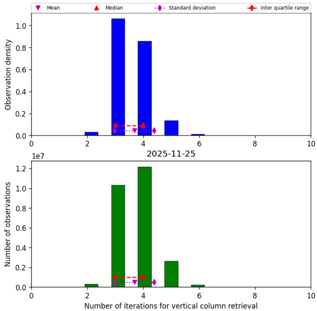
Figure 26: Histogram of “Number of iterations for vertical column retrieval” for 2025-11-24 to 2025-11-26
