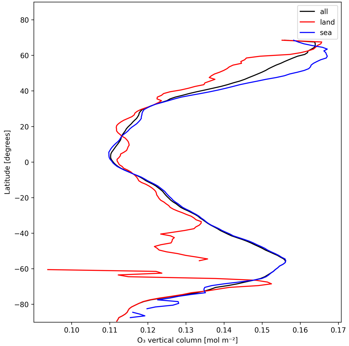
Figure 14: Zonal average of “O 3 vertical column” for 2025-11-24 to 2025-11-26.
