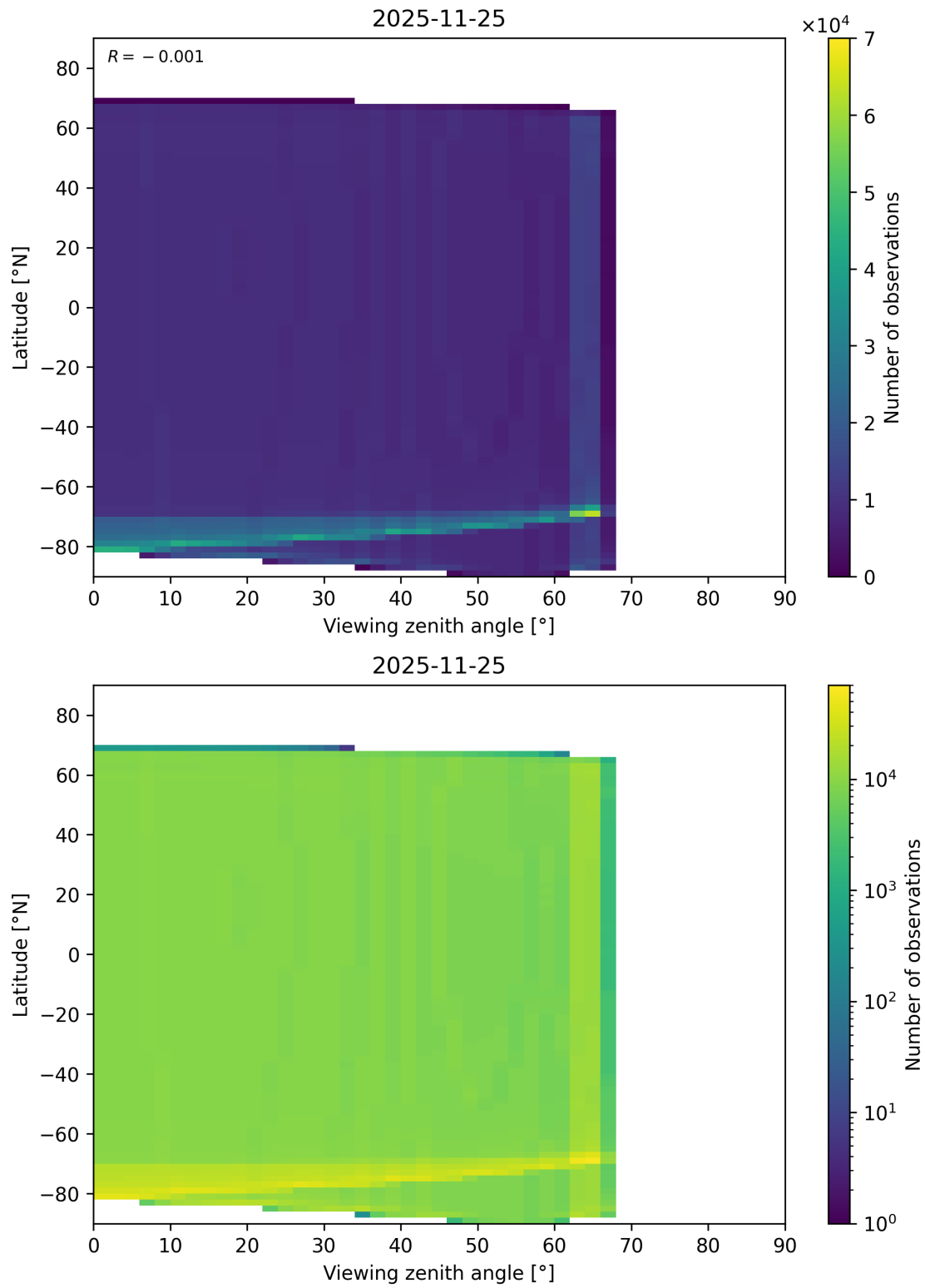
Figure 49: Scatter density plot of “Viewing zenith angle” against “Latitude” for 2025-11-24 to 2025-11-26.
