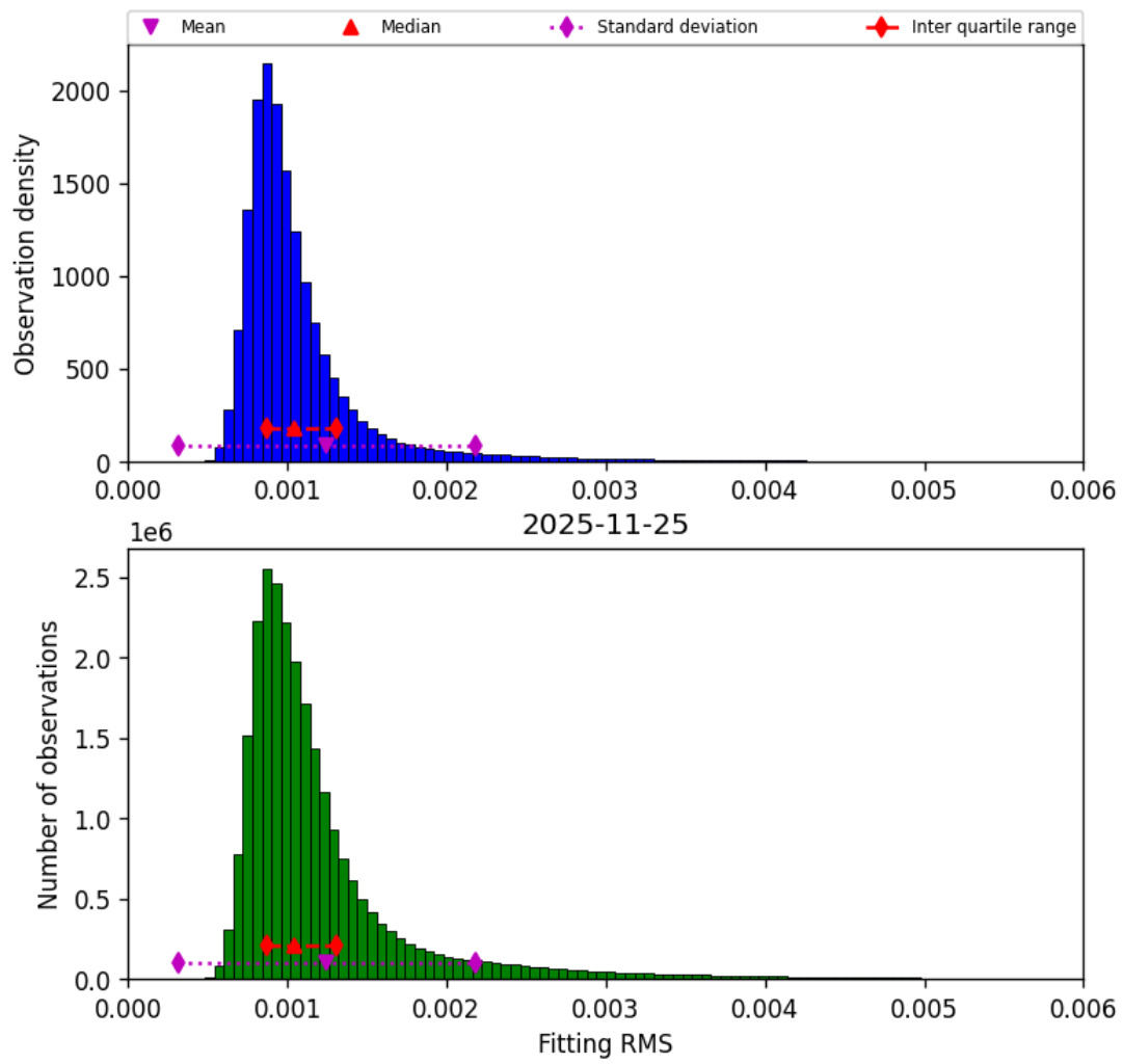
Figure 23: Histogram of “Fitting RMS” for 2025-11-24 to 2025-11-26
