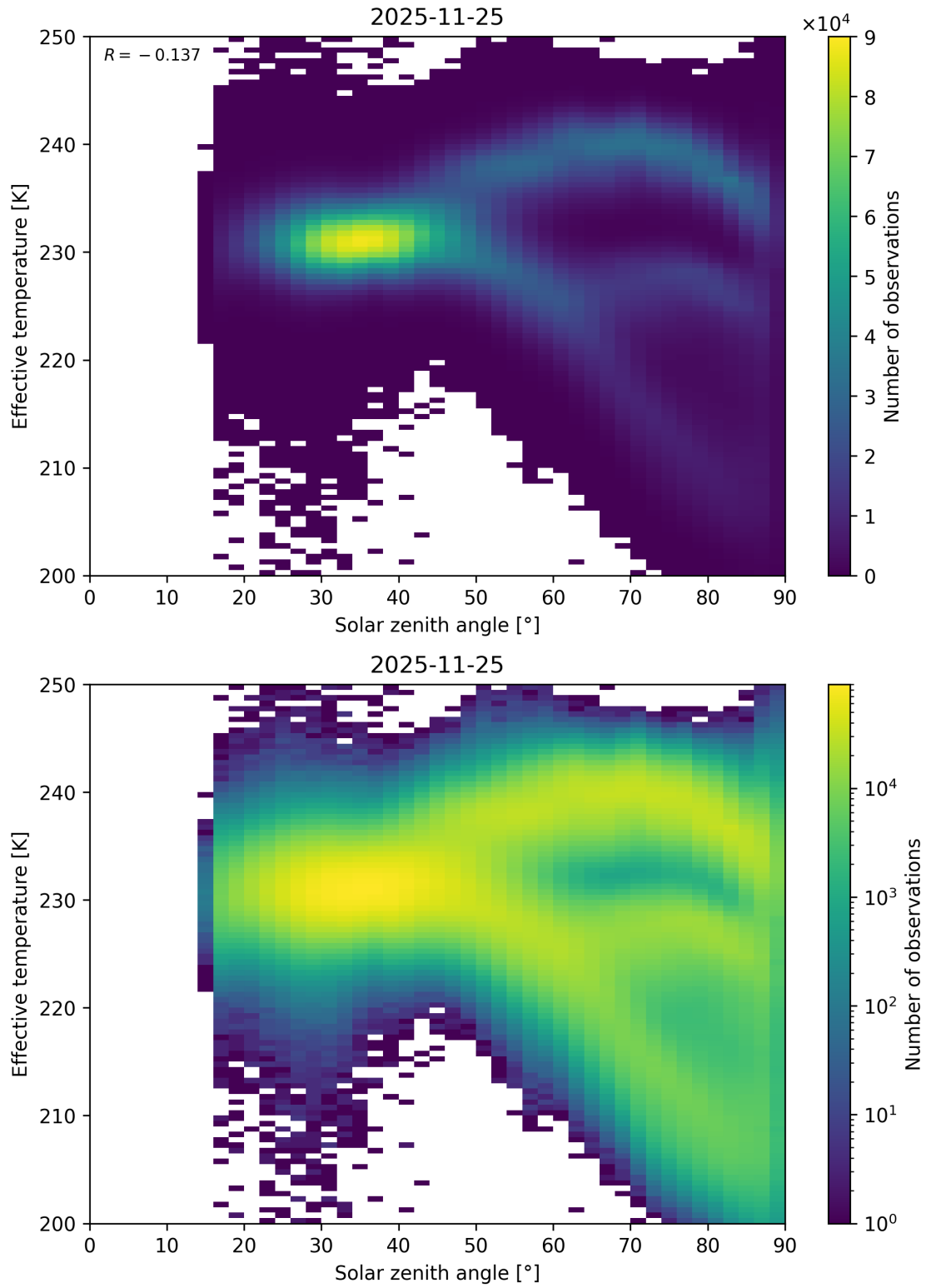
Figure 45: Scatter density plot of “Solar zenith angle” against “Effective temperature” for 2025-11-24 to 2025-11-26.
