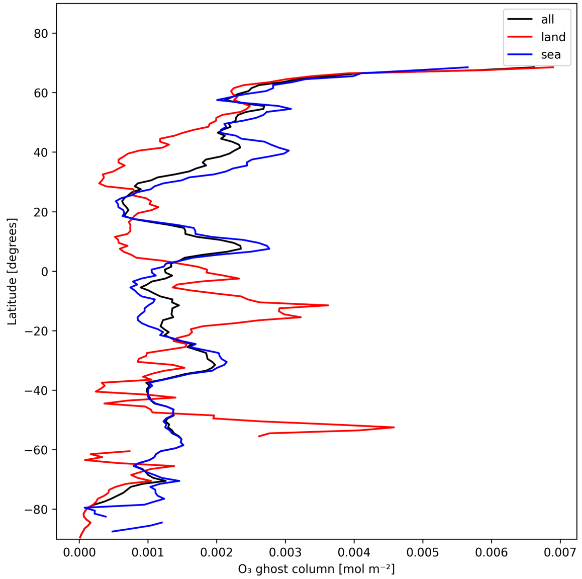
Figure 18: Zonal average of “O 3 ghost column” for 2025-11-24 to 2025-11-26.
