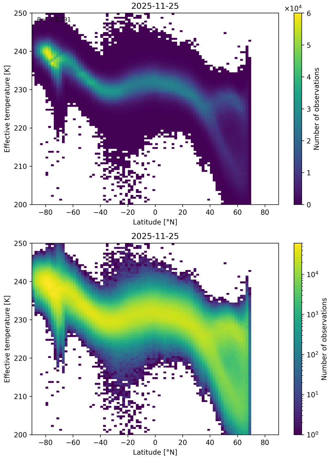
Figure 34: Scatter density plot of “Latitude” against “Effective temperature” for 2025-11-24 to 2025-11-26.
