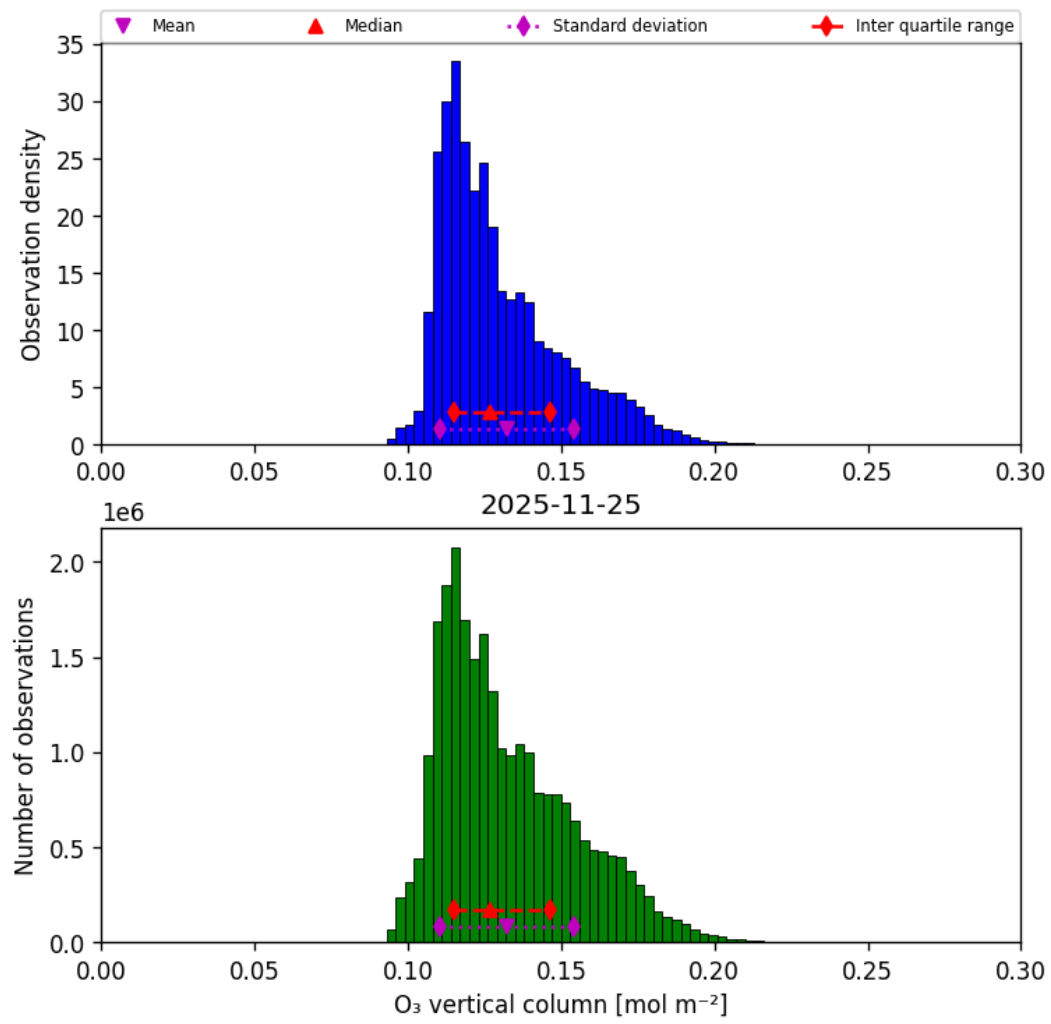
Figure 21: Histogram of “O 3 vertical column” for 2025-11-24 to 2025-11-26
