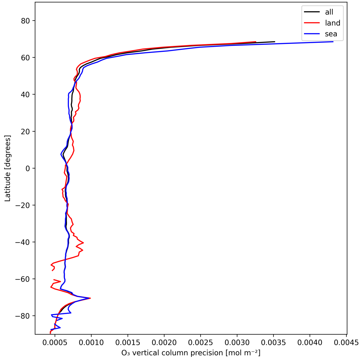
Figure 15: Zonal average of “O 3 vertical column precision” for 2025-11-24 to 2025-11-26.
