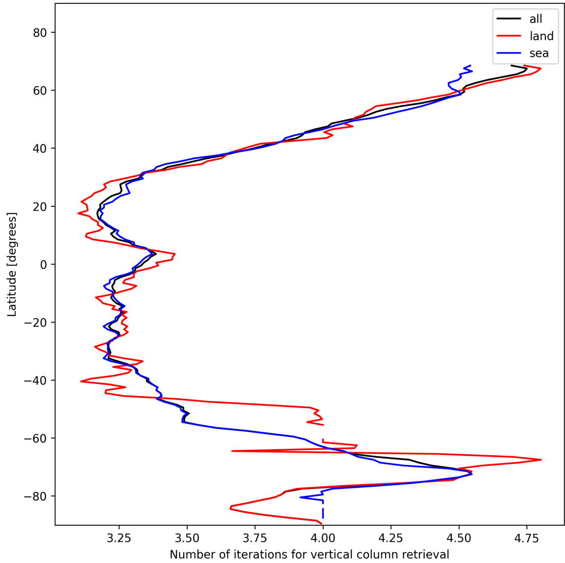
Figure 19: Zonal average of “Number of iterations for vertical column retrieval” for 2025-11-24 to 2025-11-26.
