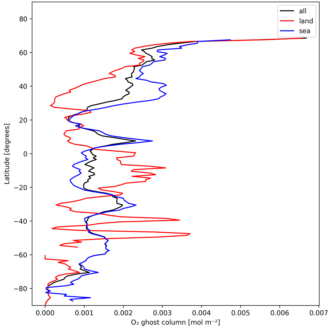
Figure 18: Zonal average of "O 3 ghost column" for 2025-11-25 to 2025-11-27.
