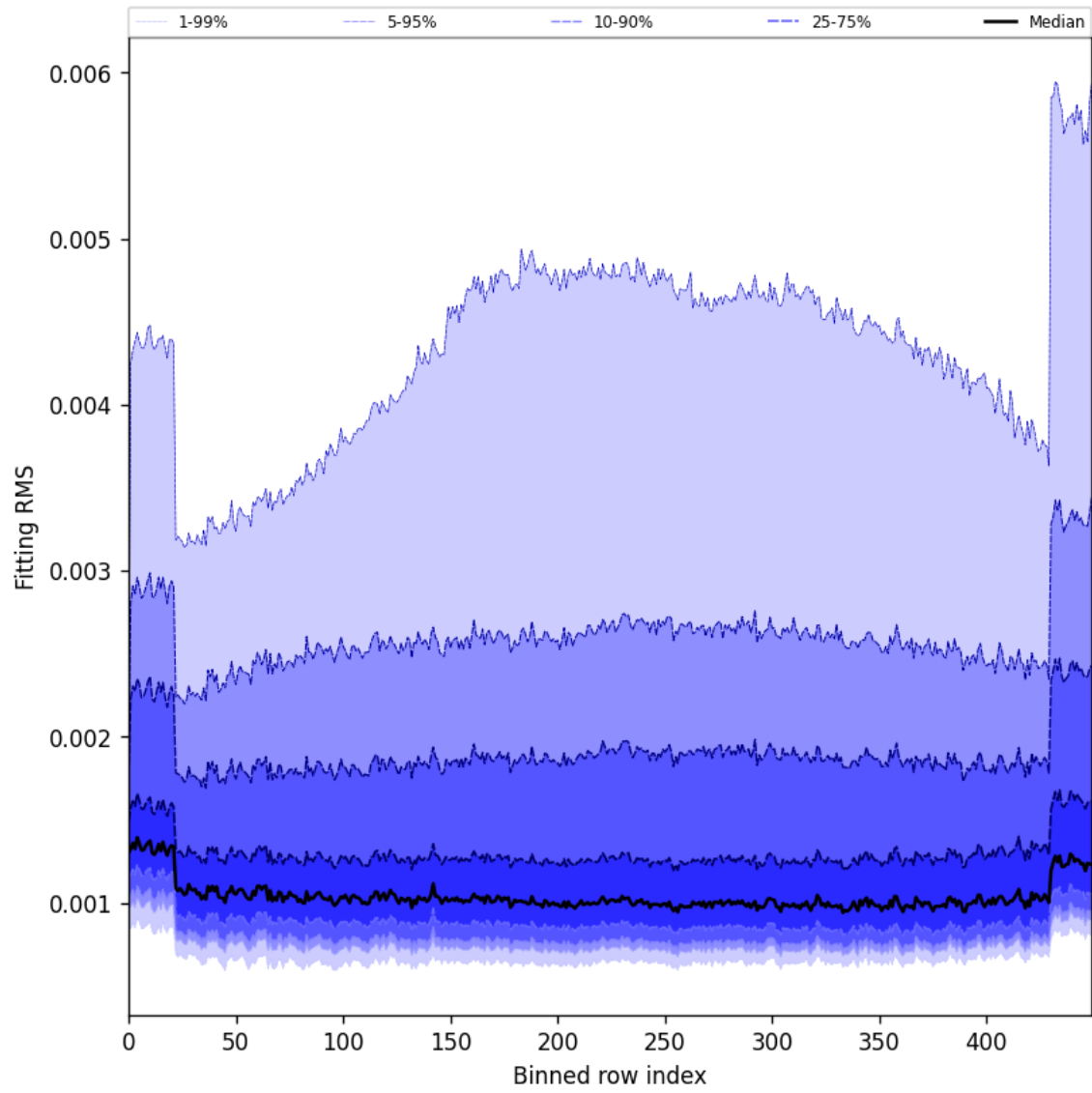
Figure 30: Along track statistics of “Fitting RMS” for 2025-11-25 to 2025-11-27
