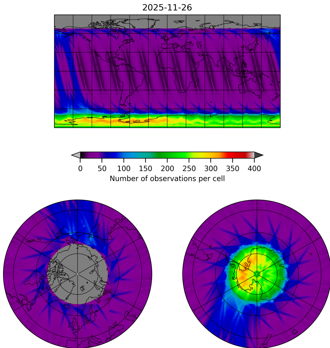
Figure 12: Map of the number of observations for 2025-11-25 to 2025-11-27
