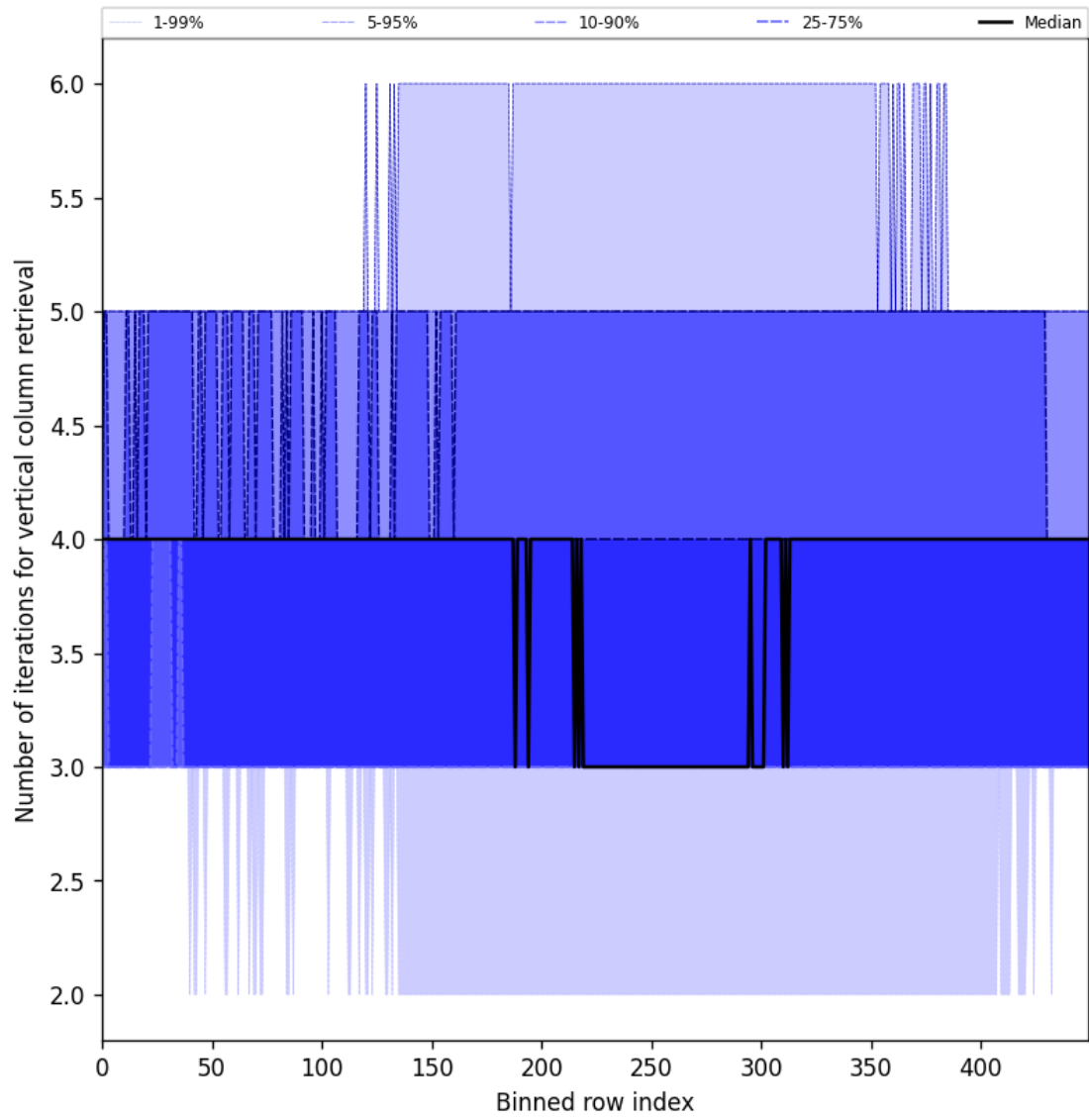
Figure 33: Along track statistics of “Number of iterations for vertical column retrieval” for 2025-11-25 to 2025-11-27
