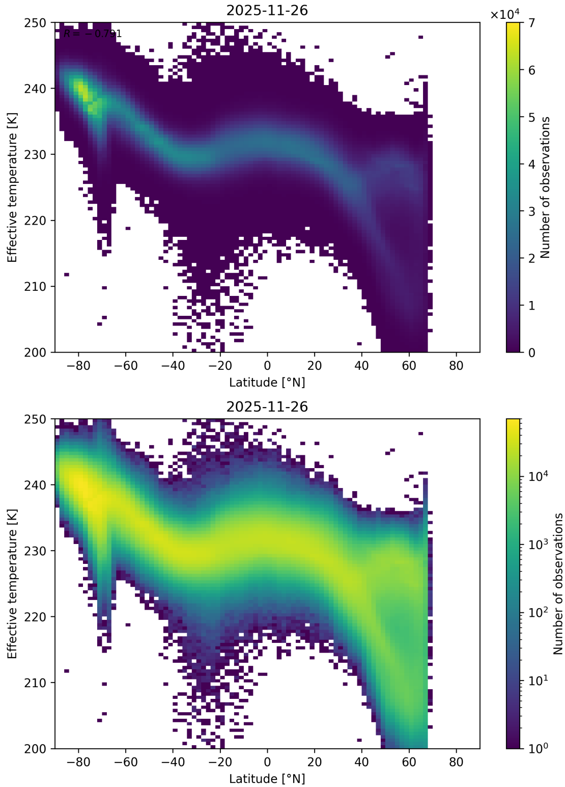
Figure 34: Scatter density plot of “Latitude” against “Effective temperature” for 2025-11-25 to 2025-11-27.
