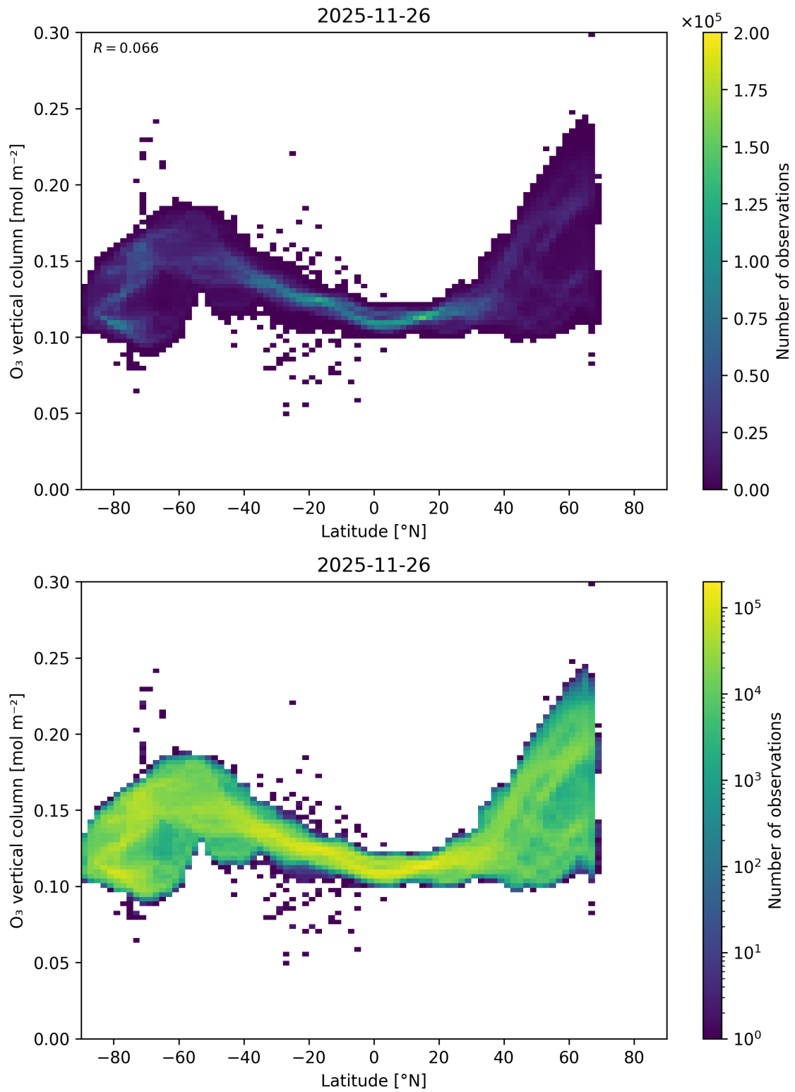
Figure 36: Scatter density plot of “Latitude” against “O 3 vertical column” for 2025-11-25 to 2025-11-27.
