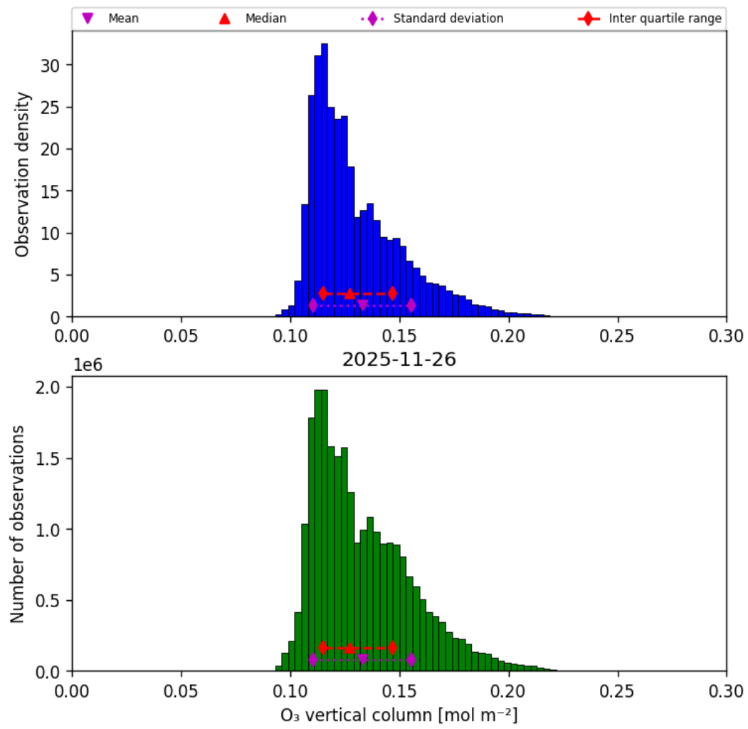
Figure 21: Histogram of “O 3 vertical column” for 2025-11-25 to 2025-11-27
