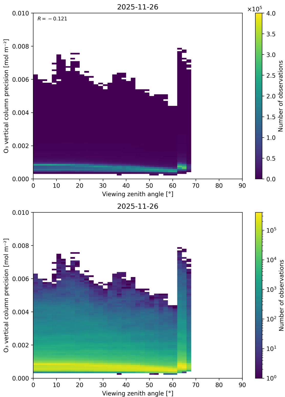
Figure 53: Scatter density plot of “Viewing zenith angle” against “O 3 vertical column precision” for 2025-11-25 to 2025-11-27.
