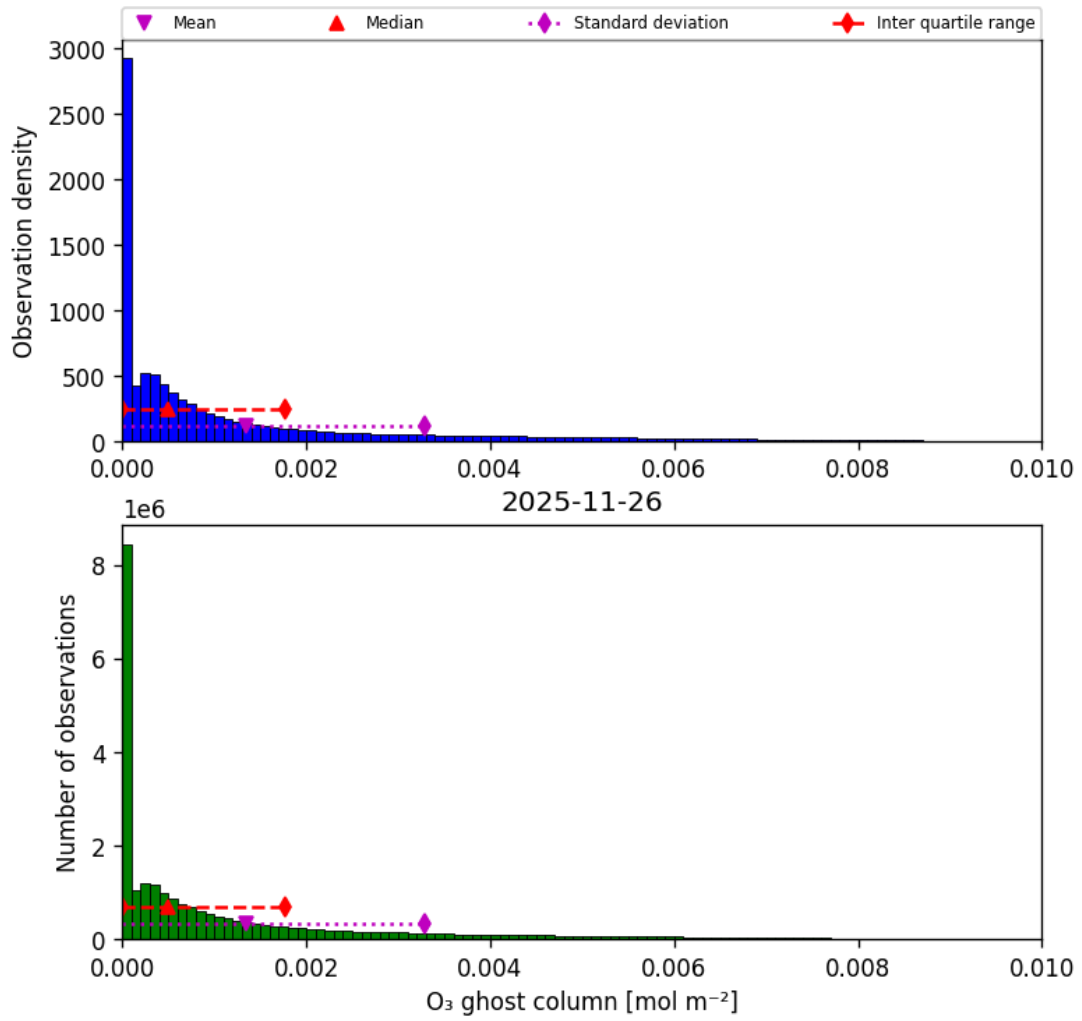
Figure 25: Histogram of “O 3 ghost column” for 2025-11-25 to 2025-11-27
