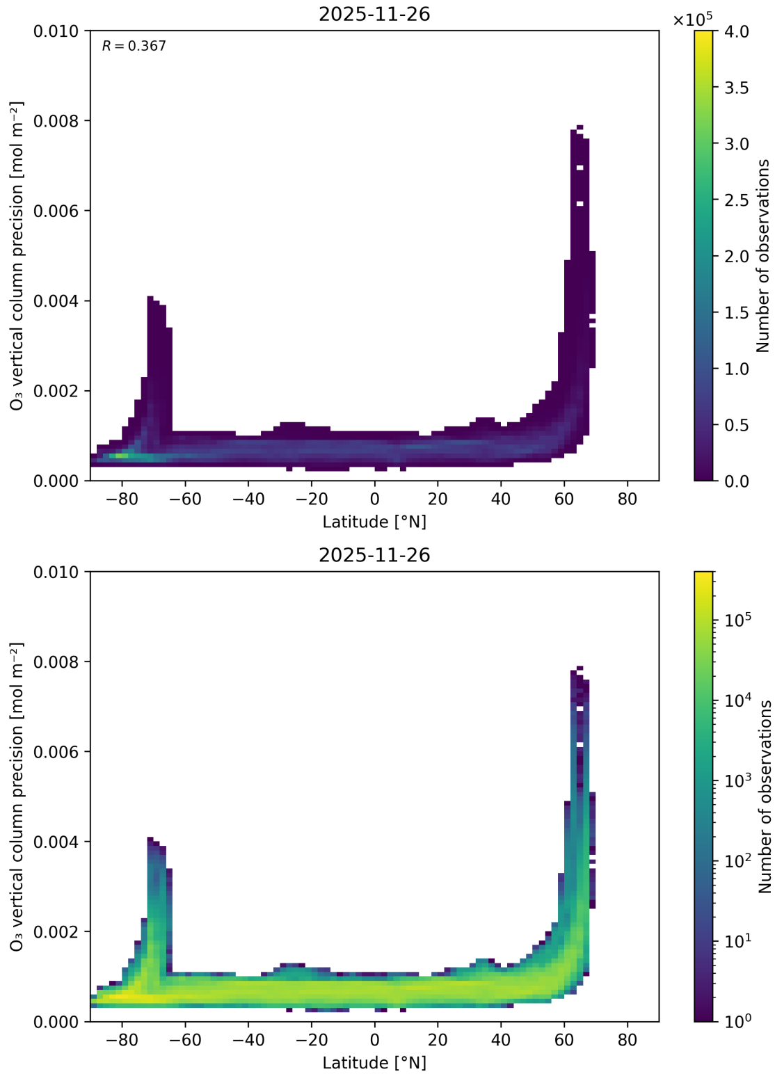
Figure 37: Scatter density plot of “Latitude” against “O 3 vertical column precision” for 2025-11-25 to 2025-11-27.
