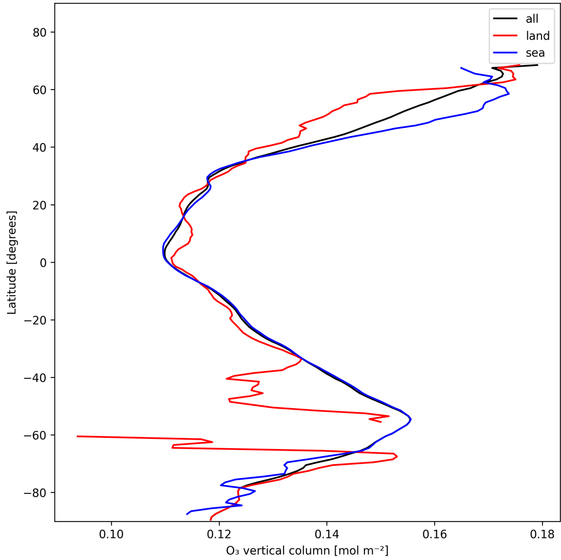
Figure 14: Zonal average of “O 3 vertical column” for 2025-11-25 to 2025-11-27.
