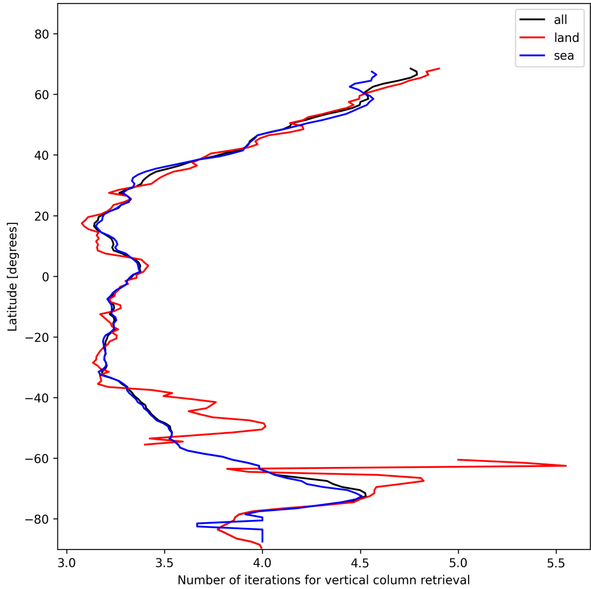
Figure 19: Zonal average of “Number of iterations for vertical column retrieval” for 2025-11-25 to 2025-11-27.
