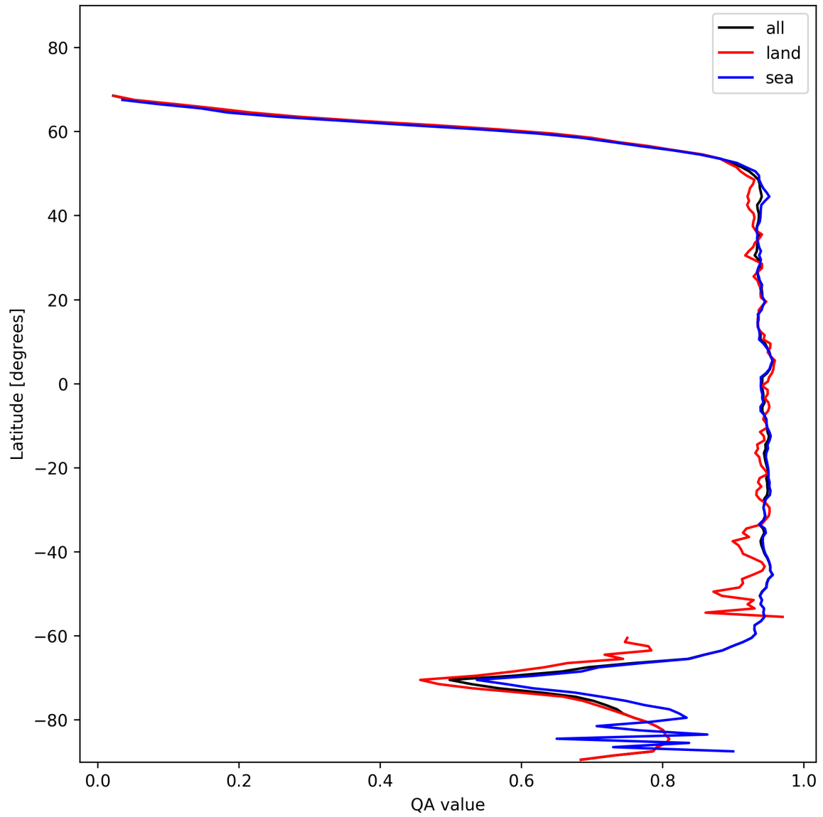
Figure 13: Zonal average of “QA value” for 2025-11-25 to 2025-11-27.
