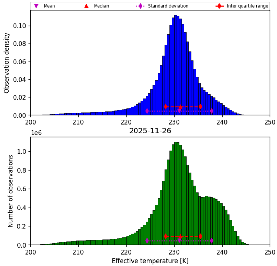
Figure 24: Histogram of “Effective temperature” for 2025-11-25 to 2025-11-27
