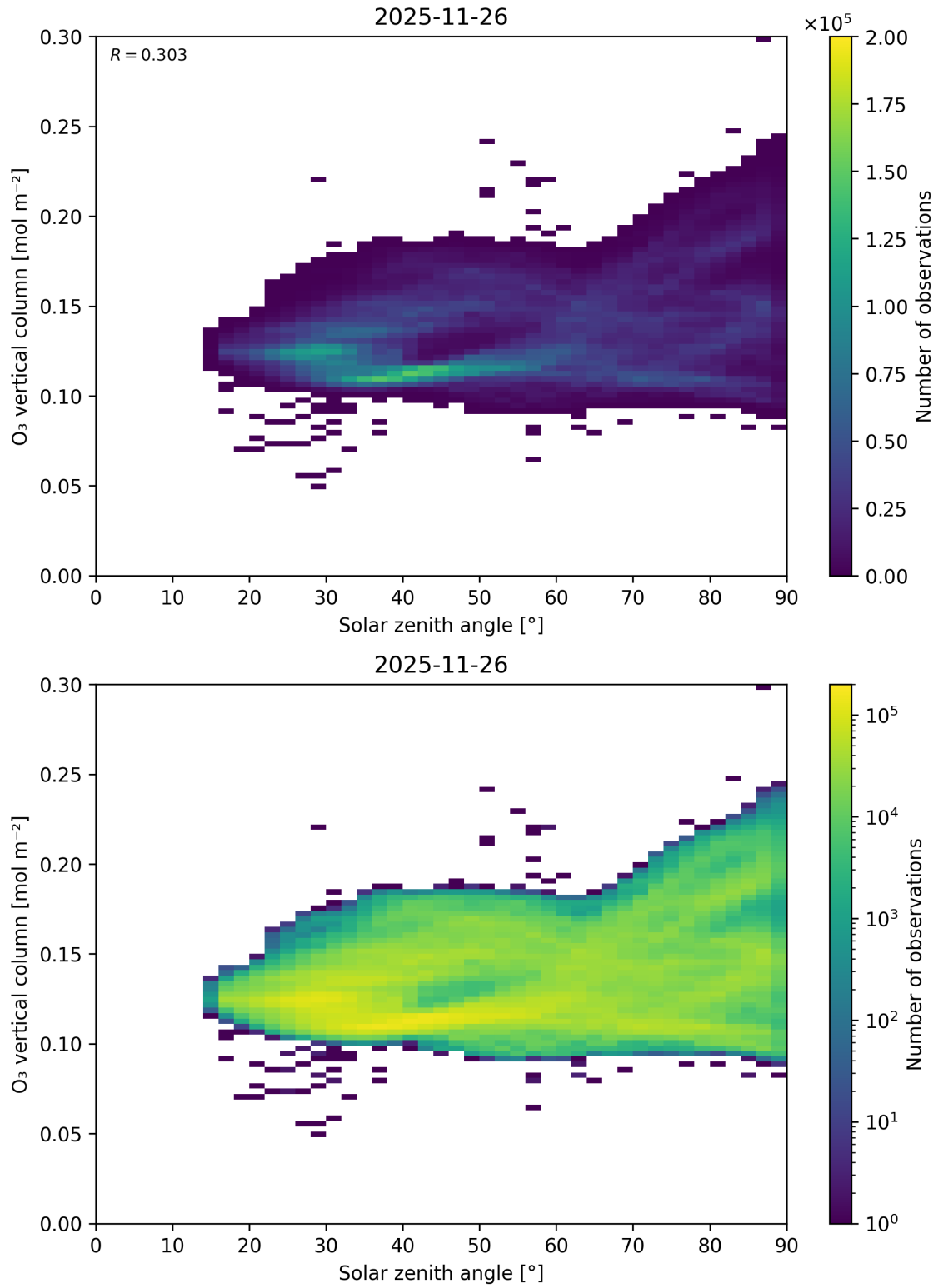
Figure 47: Scatter density plot of “Solar zenith angle” against “O 3 vertical column” for 2025-11-25 to 2025-11-27.
