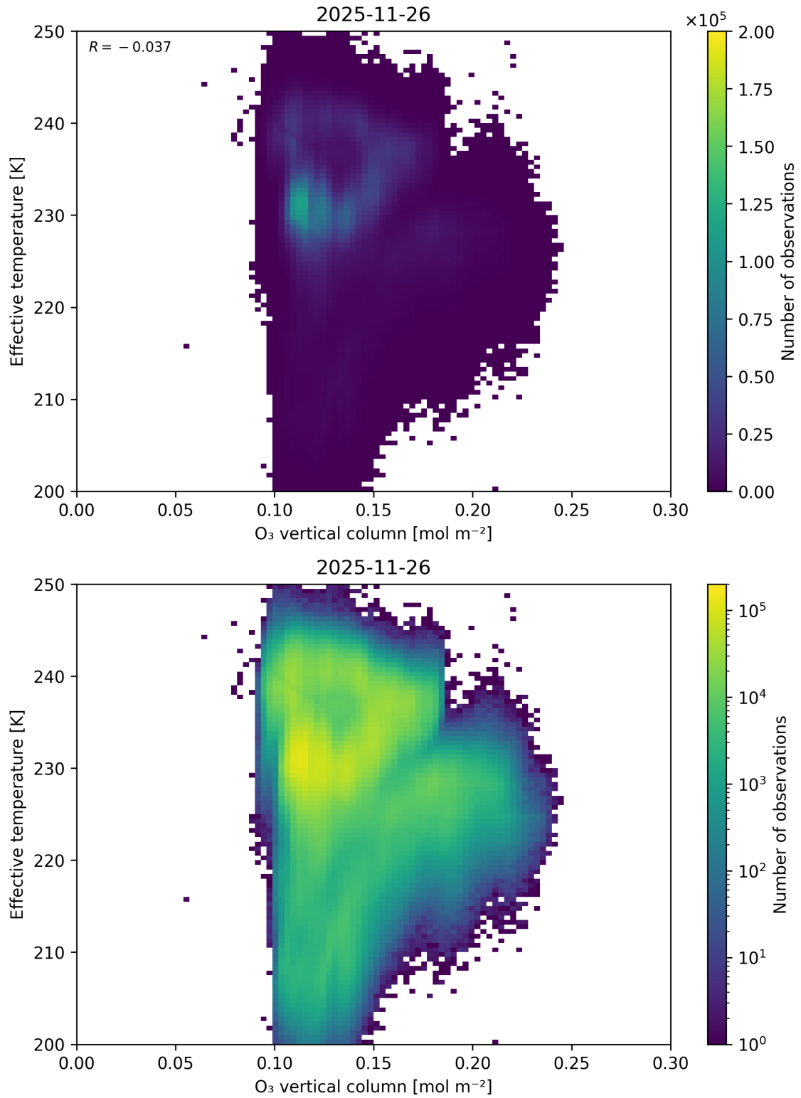
Figure 39: Scatter density plot of “O 3 vertical column” against “Effective temperature” for 2025-11-25 to 2025-11-27.
