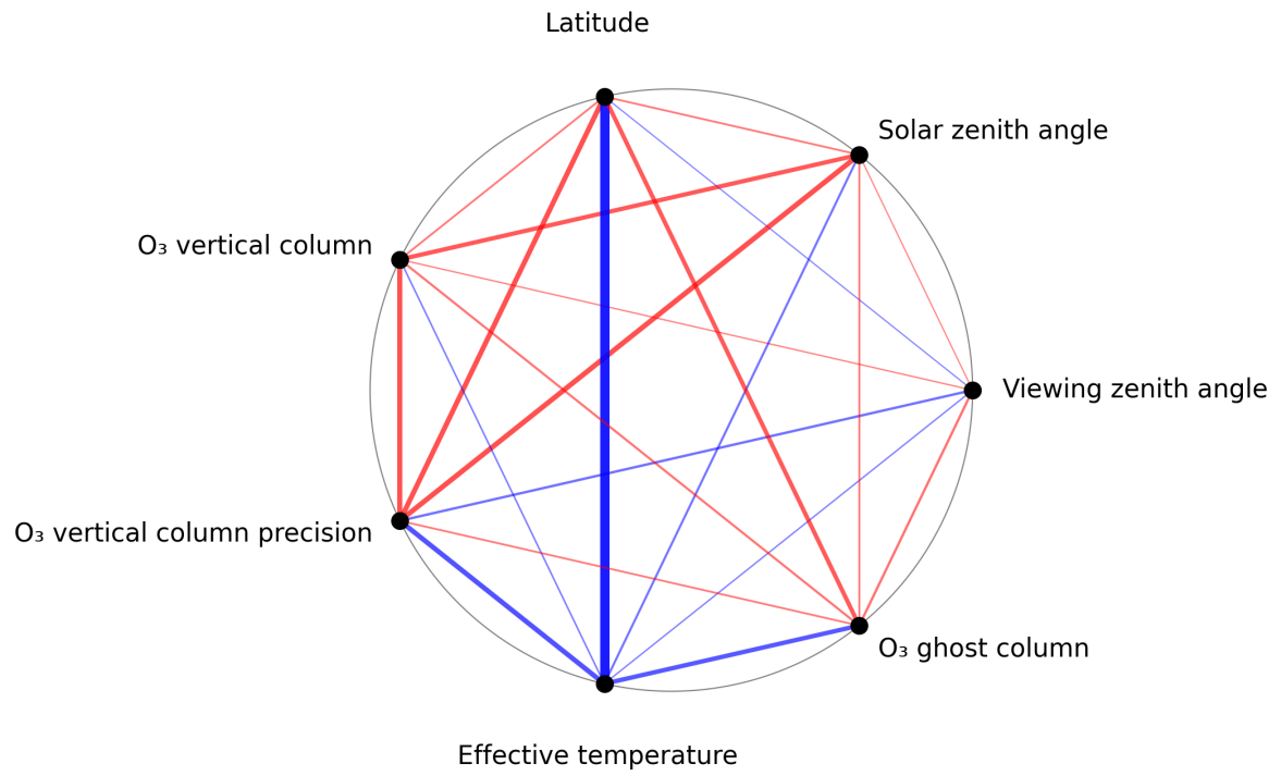
Figure 1: Map of correlation graph for 2025-11-25 to 2025-11-27.
