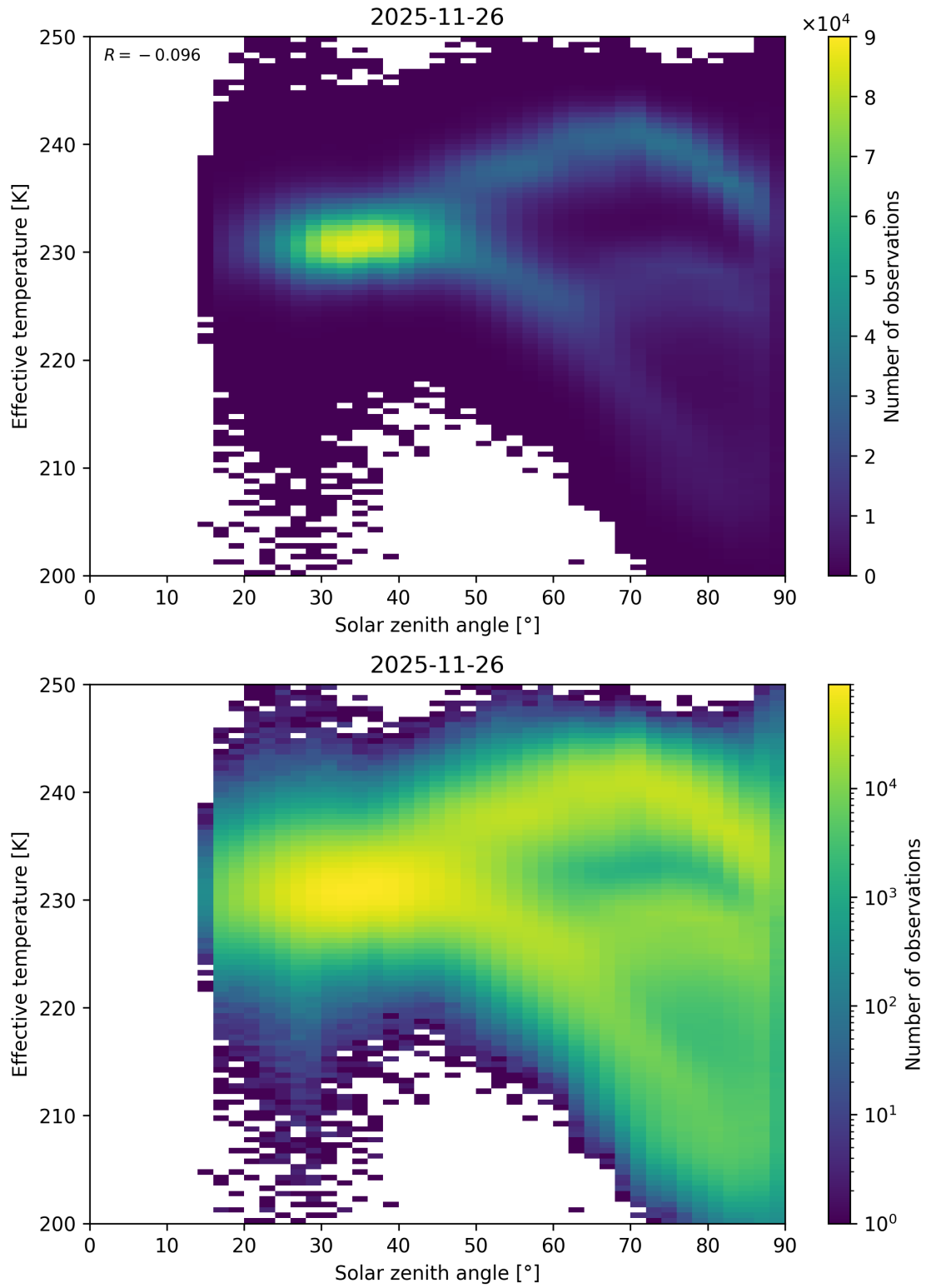
Figure 45: Scatter density plot of “Solar zenith angle” against “Effective temperature” for 2025-11-25 to 2025-11-27.
