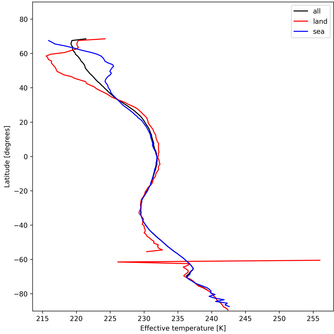
Figure 17: Zonal average of "Effective temperature" for 2025-11-25 to 2025-11-27.
