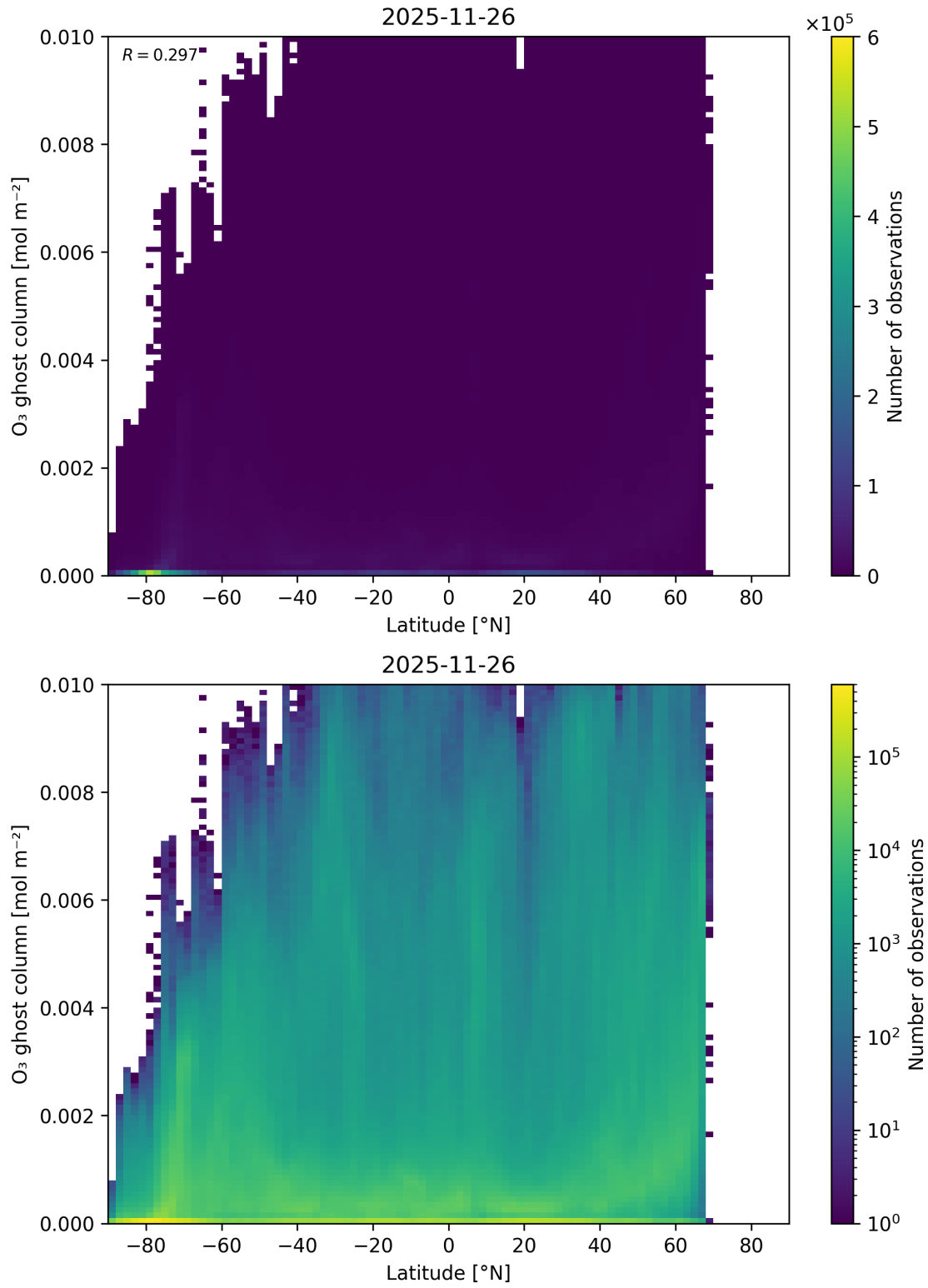
Figure 35: Scatter density plot of “Latitude” against “O 3 ghost column” for 2025-11-25 to 2025-11-27.
