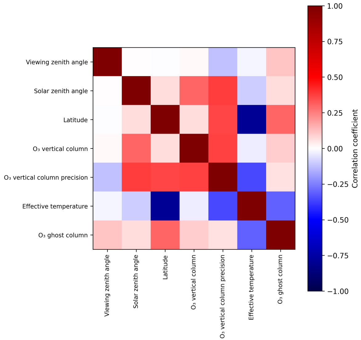
Figure 2: Map of correlation matrix for 2025-11-25 to 2025-11-27.
