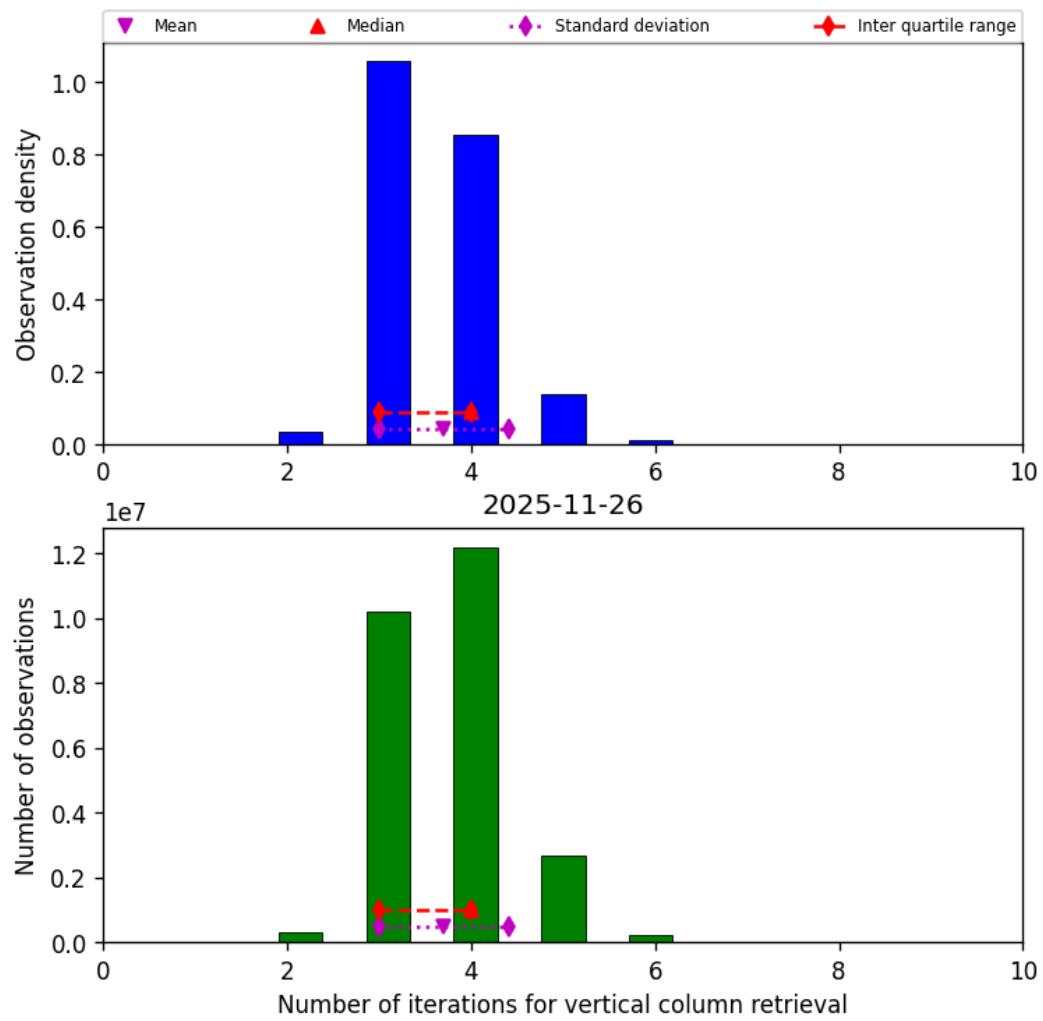
Figure 26: Histogram of “Number of iterations for vertical column retrieval” for 2025-11-25 to 2025-11-27
