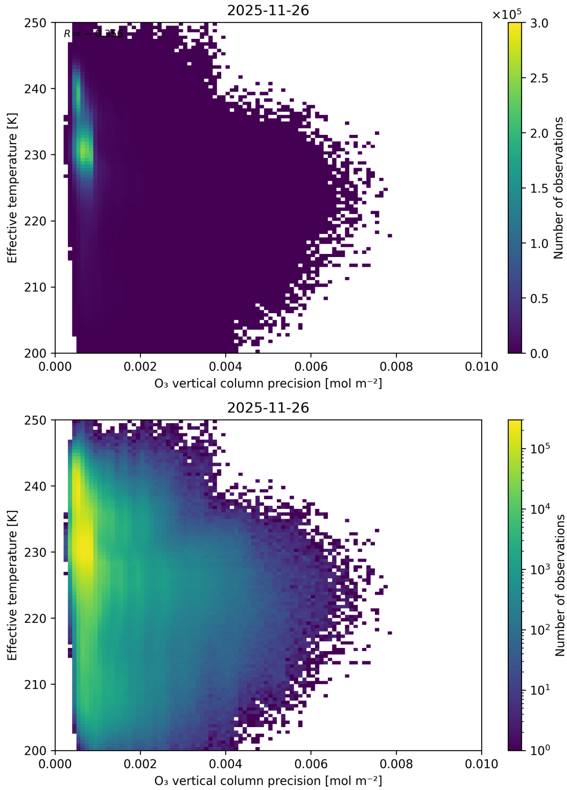
Figure 42: Scatter density plot of “O 3 vertical column precision” against “Effective temperature” for 2025-11-25 to 2025-11-27.
