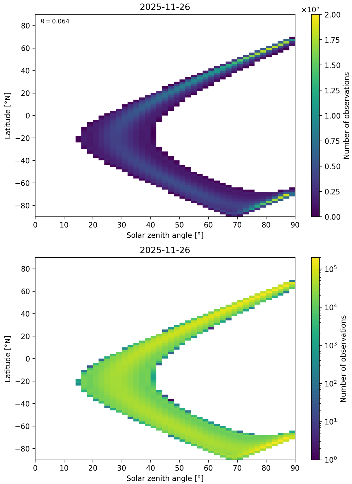
Figure 44: Scatter density plot of “Solar zenith angle” against “Latitude” for 2025-11-25 to 2025-11-27.
