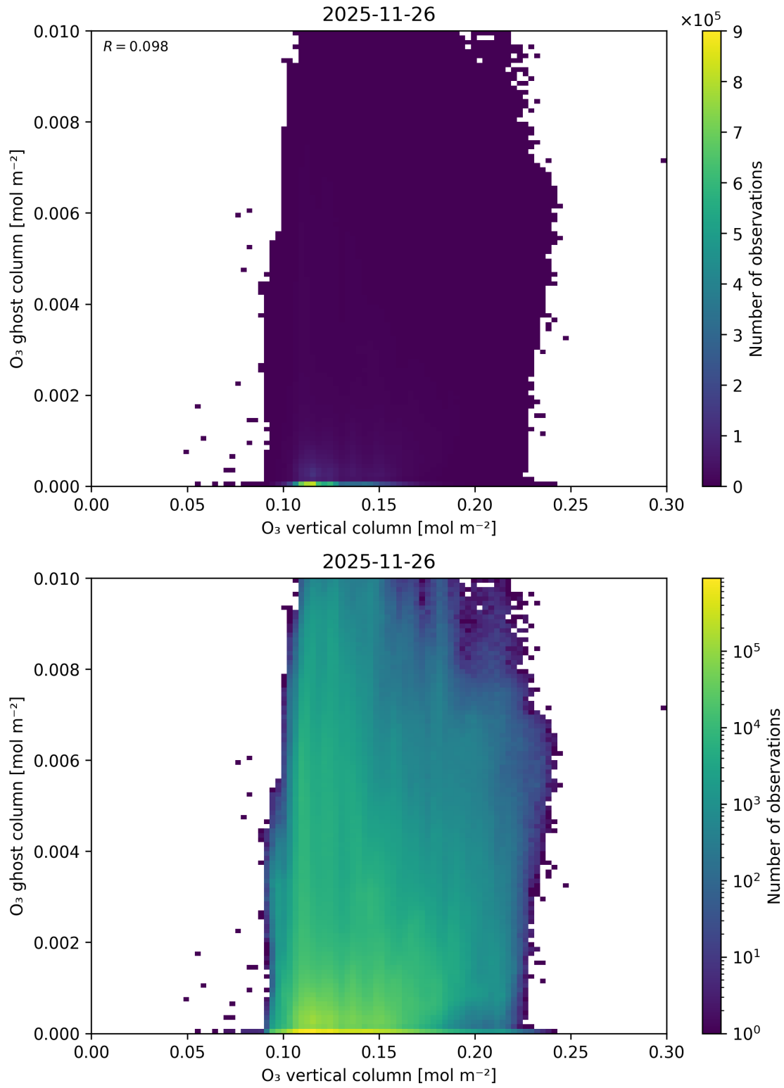
Figure 40: Scatter density plot of “O 3 vertical column” against “O 3 ghost column” for 2025-11-25 to 2025-11-27.
