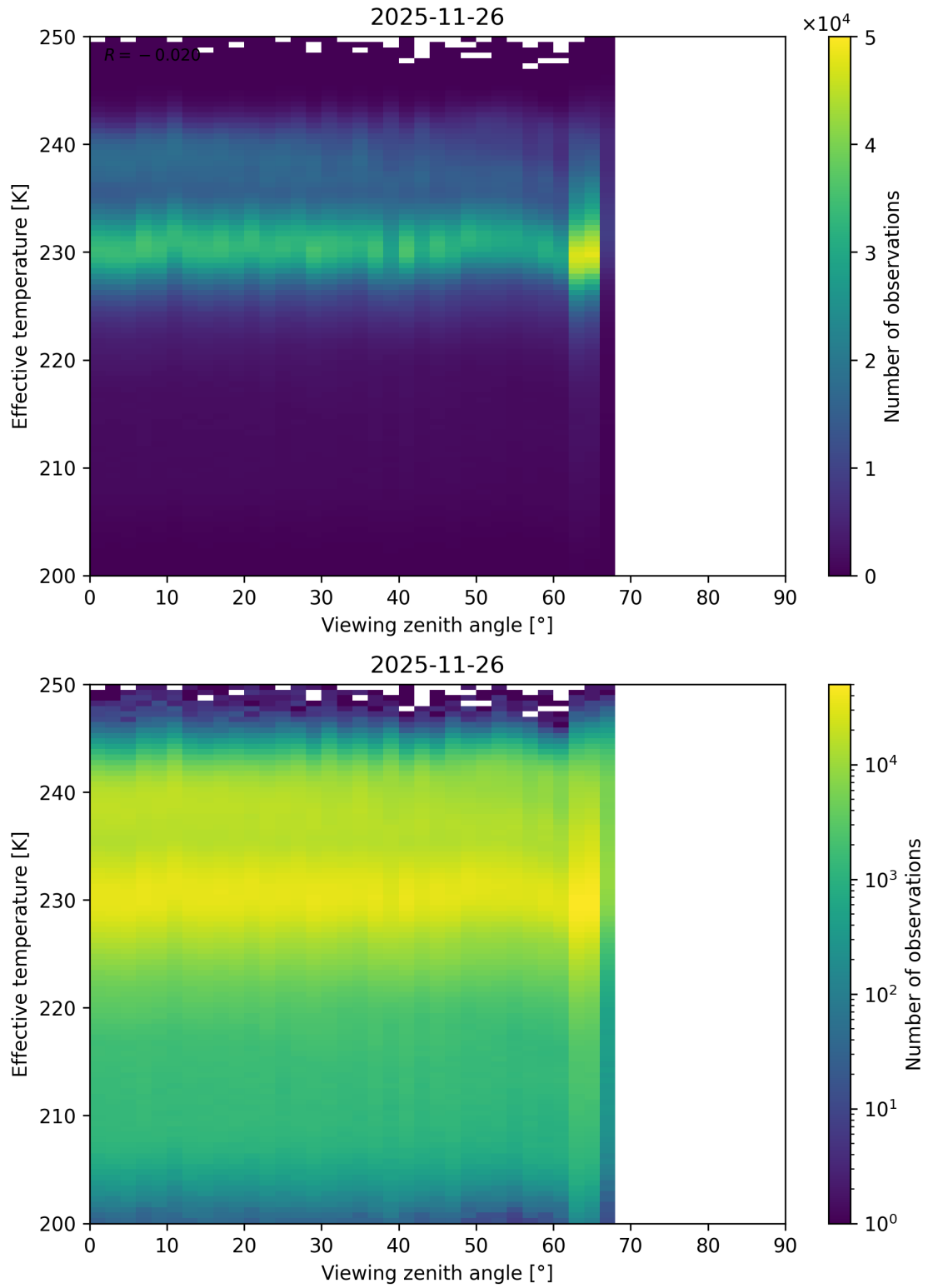
Figure 50: Scatter density plot of “Viewing zenith angle” against “Effective temperature” for 2025-11-25 to 2025-11-27.
