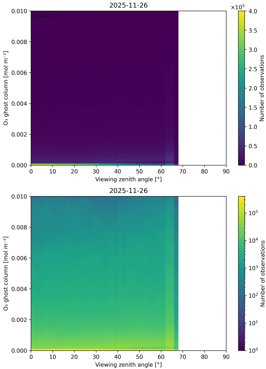
Figure 51: Scatter density plot of “Viewing zenith angle” against “O 3 ghost column” for 2025-11-25 to 2025-11-27.
