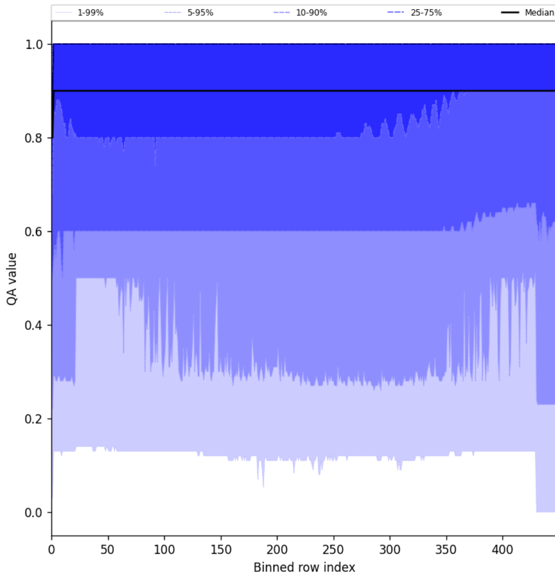
Figure 27: Along track statistics of “QA value” for 2025-11-25 to 2025-11-27
