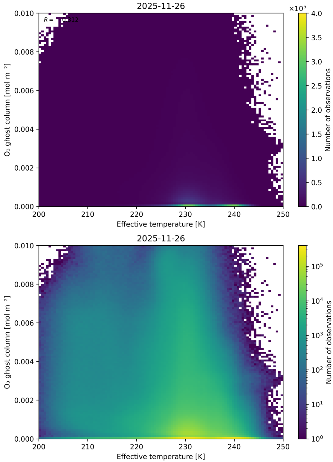
Figure 38: Scatter density plot of “Effective temperature” against “O 3 ghost column” for 2025-11-25 to 2025-11-27.
