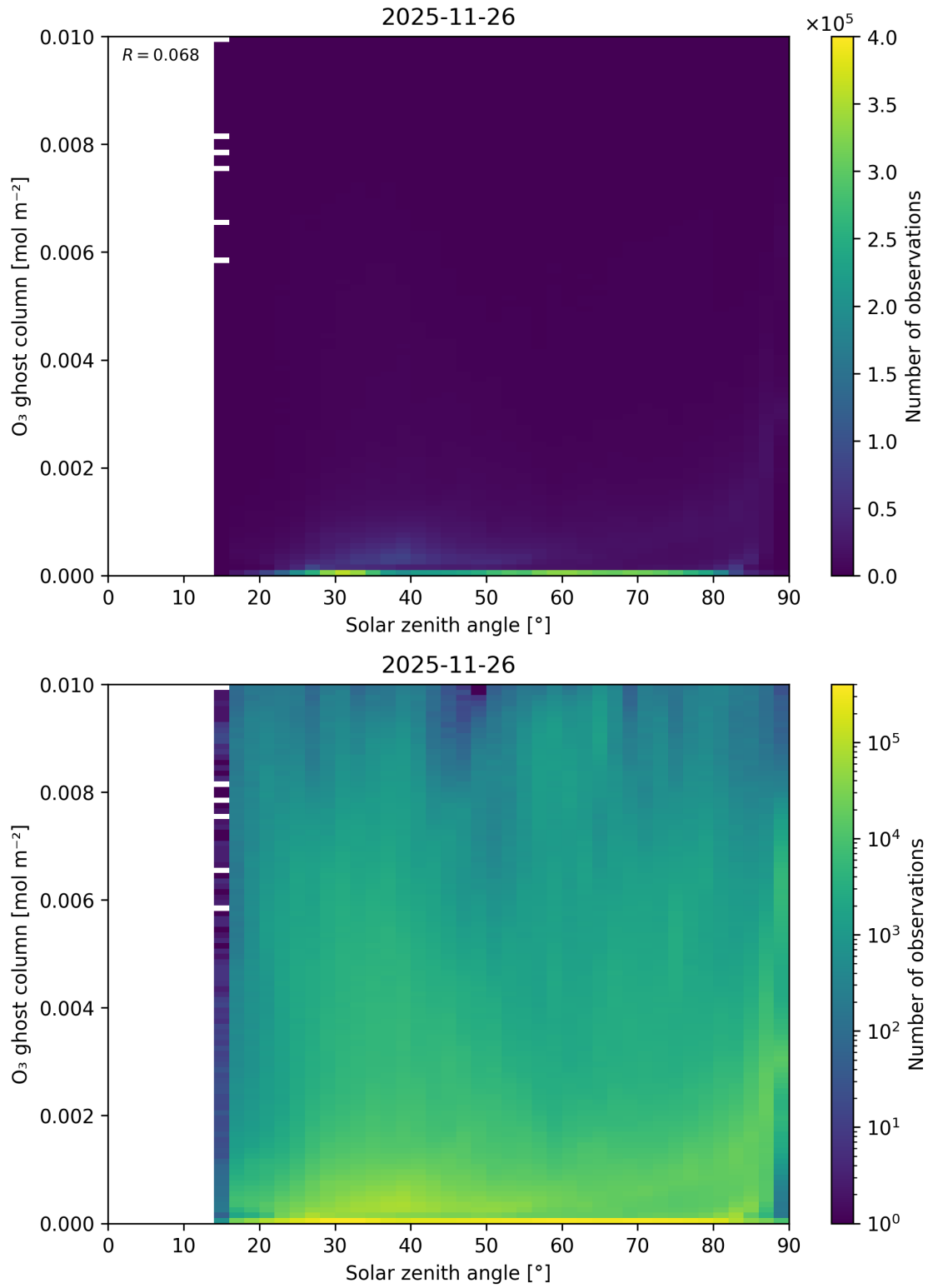
Figure 46: Scatter density plot of “Solar zenith angle” against “O 3 ghost column” for 2025-11-25 to 2025-11-27.
