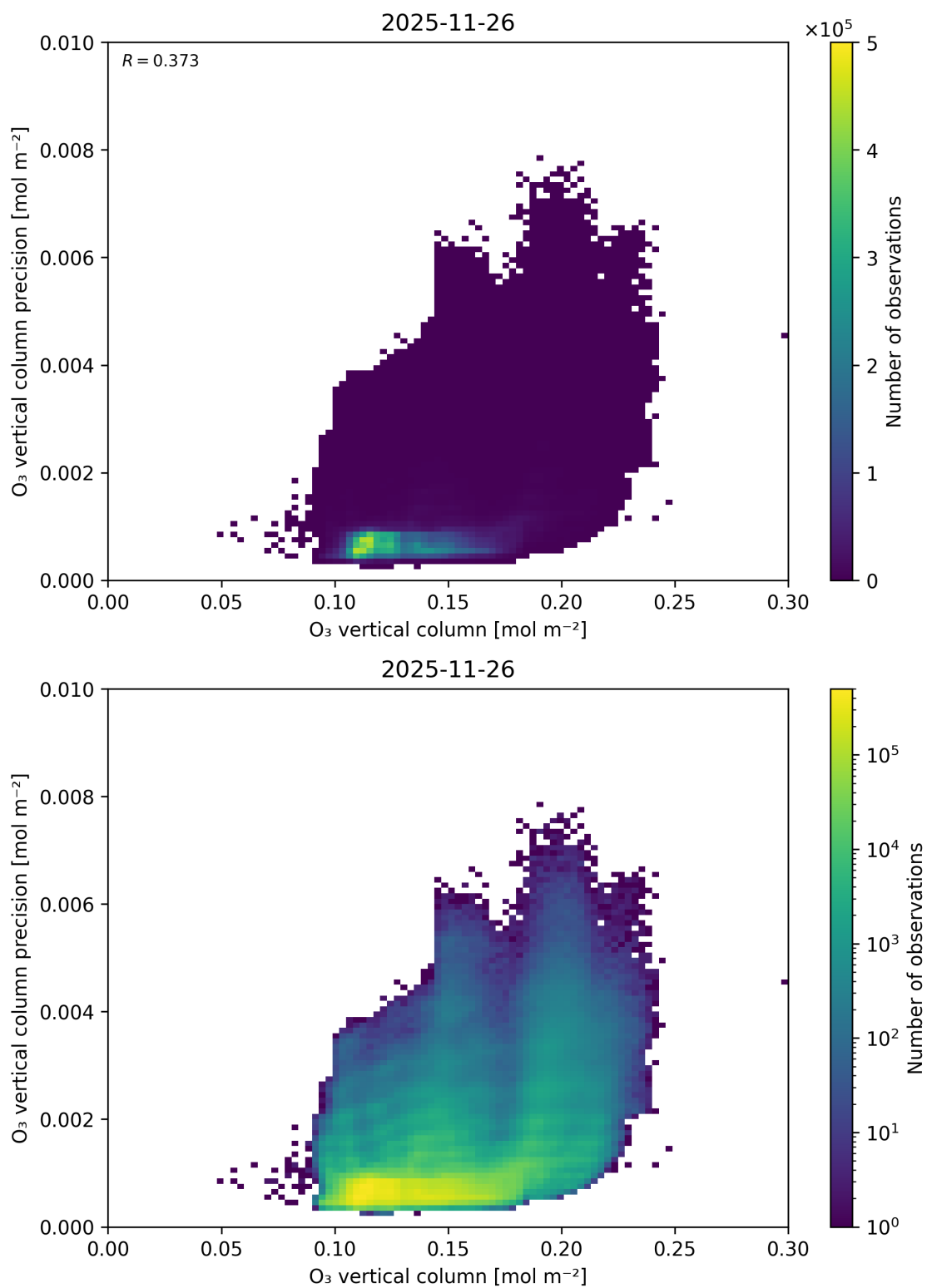
Figure 41: Scatter density plot of “O 3 vertical column” against “O 3 vertical column precision” for 2025-11-25 to 2025-11-27.
