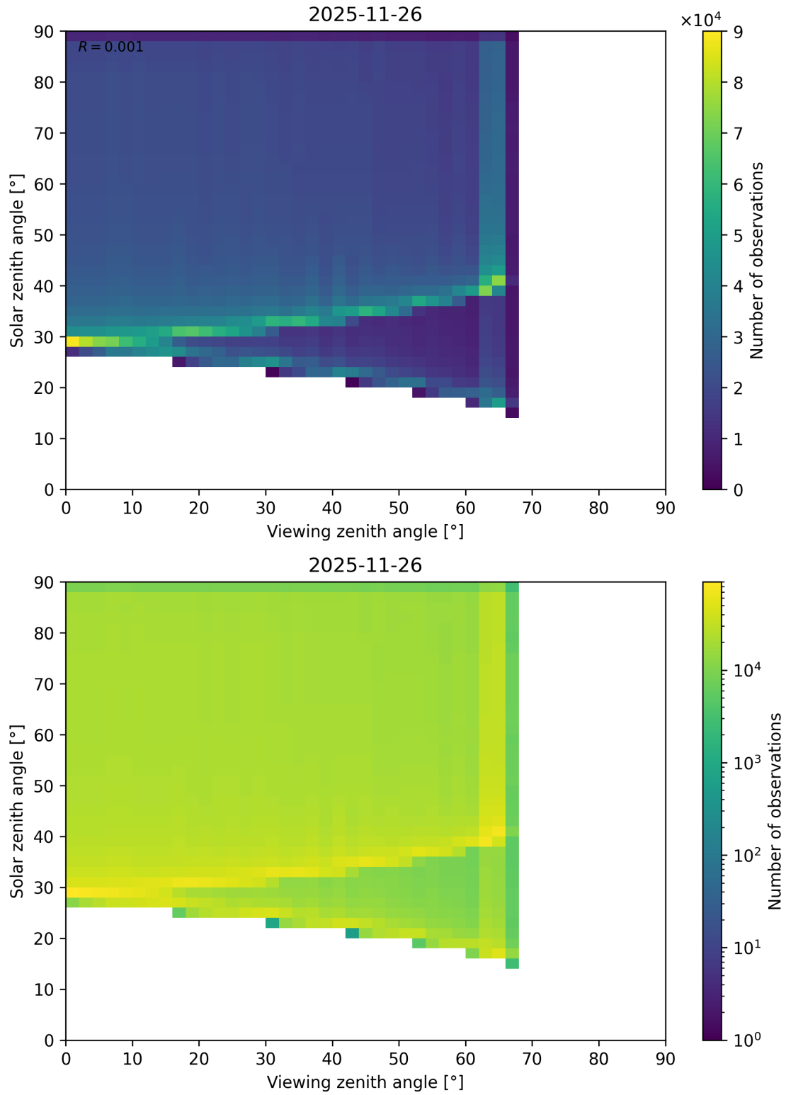
Figure 54: Scatter density plot of “Viewing zenith angle” against “Solar zenith angle” for 2025-11-25 to 2025-11-27.
