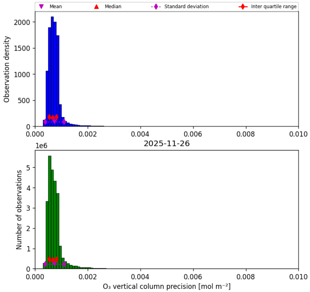
Figure 22: Histogram of “O 3 vertical column precision” for 2025-11-25 to 2025-11-27
