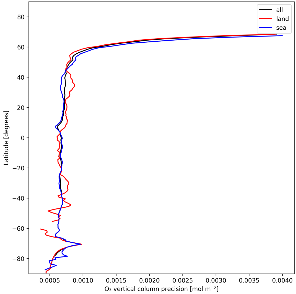
Figure 15: Zonal average of “O 3 vertical column precision” for 2025-11-25 to 2025-11-27.
