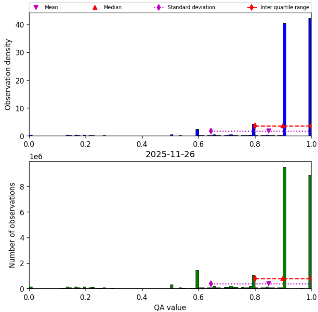
Figure 20: Histogram of “QA value” for 2025-11-25 to 2025-11-27
