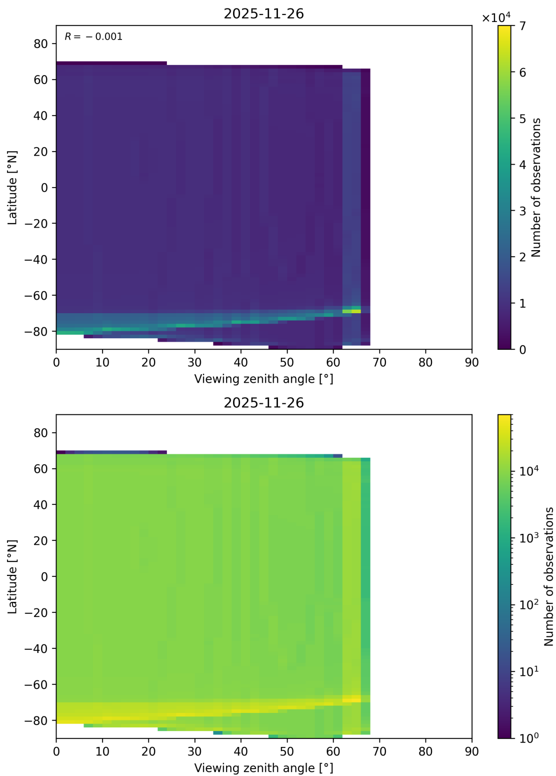
Figure 49: Scatter density plot of “Viewing zenith angle” against “Latitude” for 2025-11-25 to 2025-11-27.
