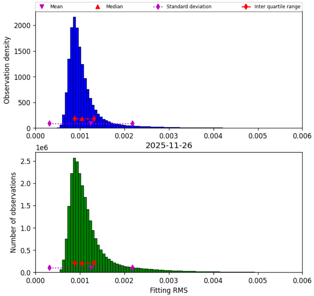
Figure 23: Histogram of “Fitting RMS” for 2025-11-25 to 2025-11-27
