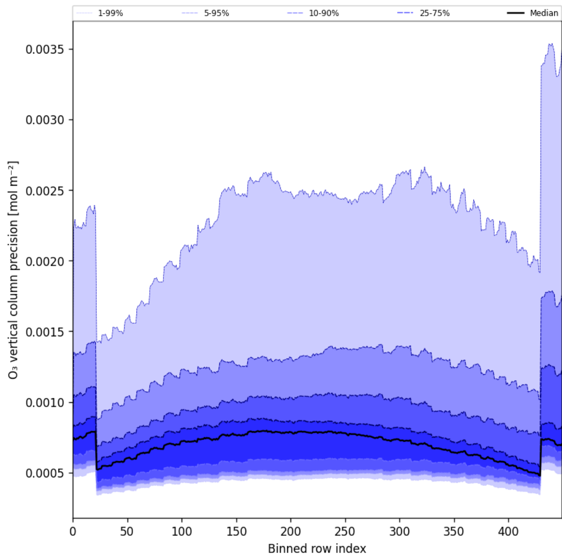
Figure 29: Along track statistics of “O 3 vertical column precision” for 2025-11-25 to 2025-11-27
