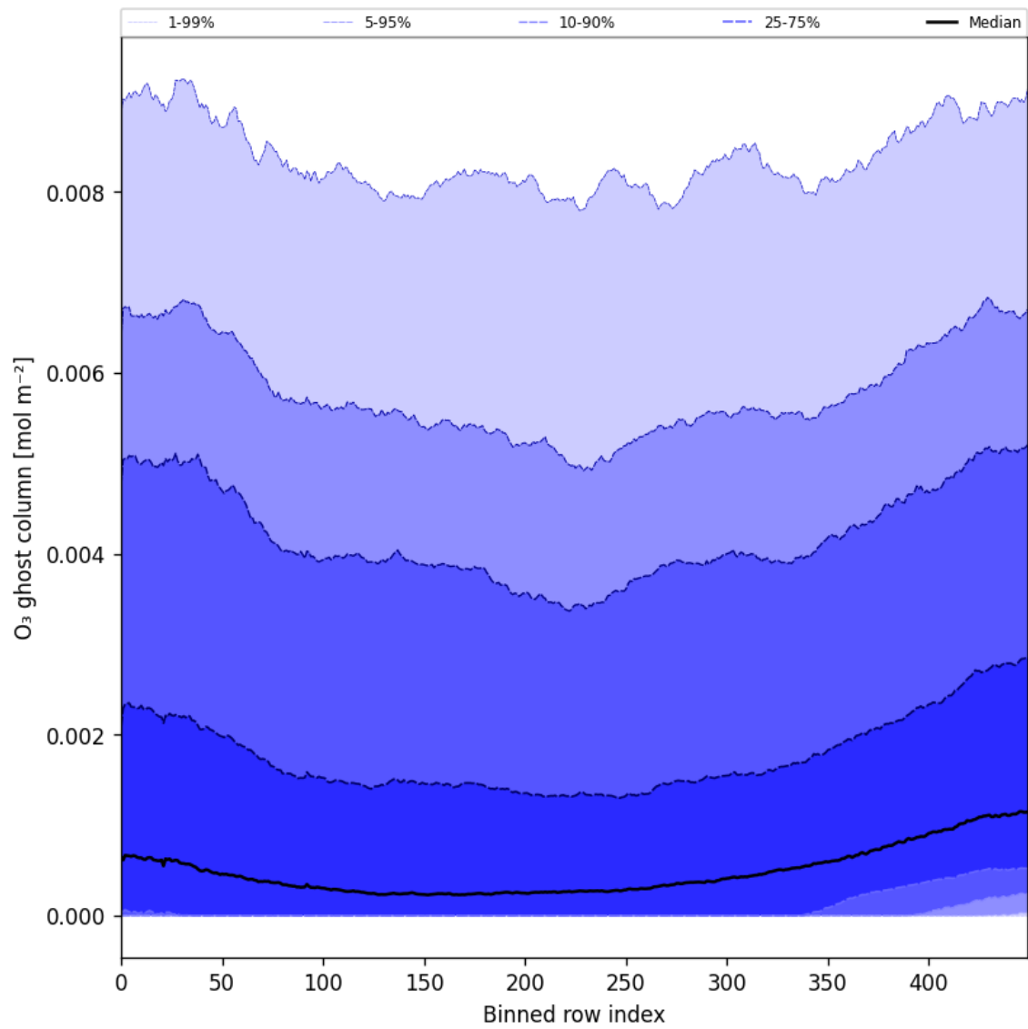
Figure 32: Along track statistics of “O 3 ghost column” for 2025-11-25 to 2025-11-27
