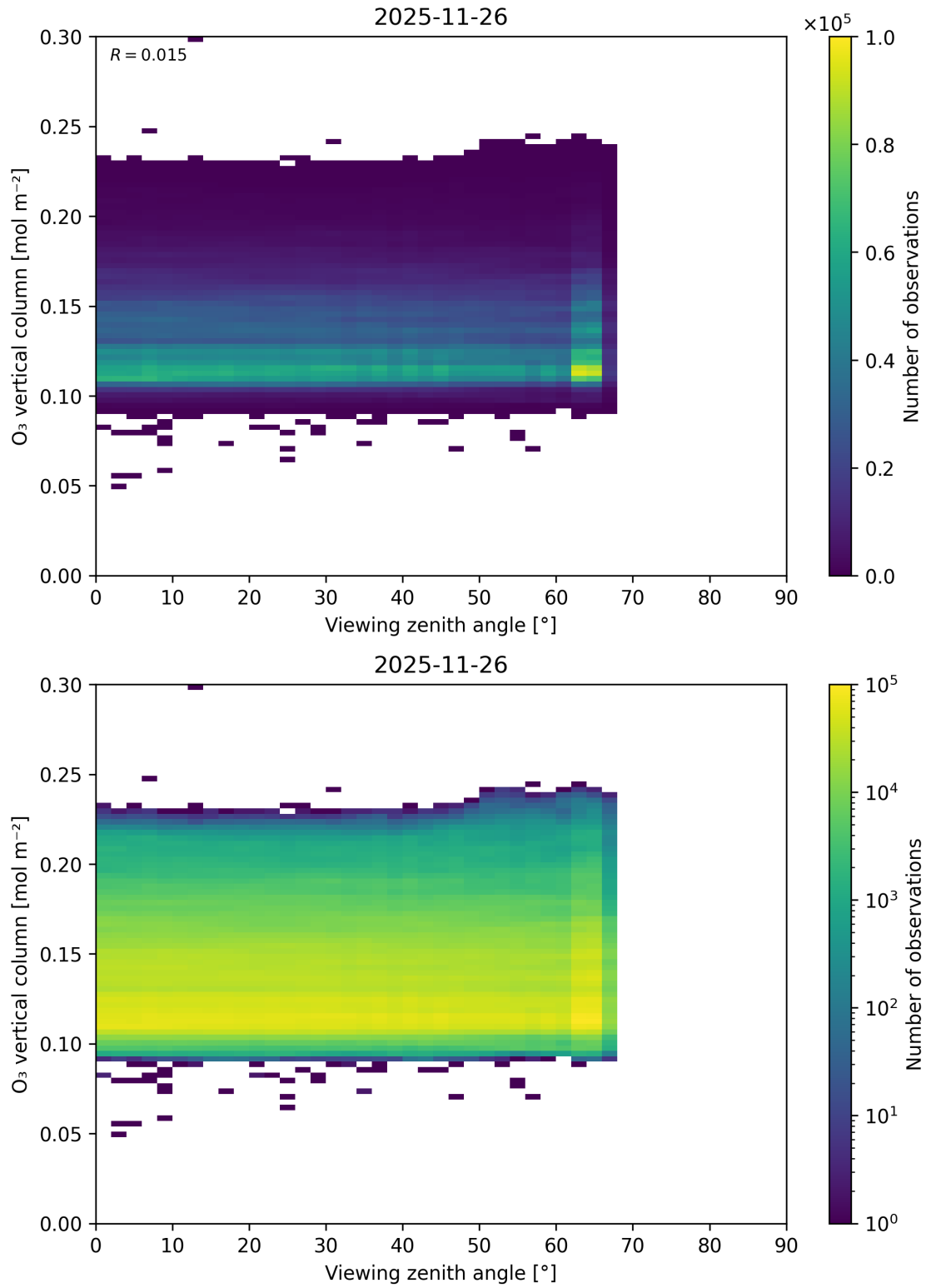
Figure 52: Scatter density plot of “Viewing zenith angle” against “O 3 vertical column” for 2025-11-25 to 2025-11-27.
