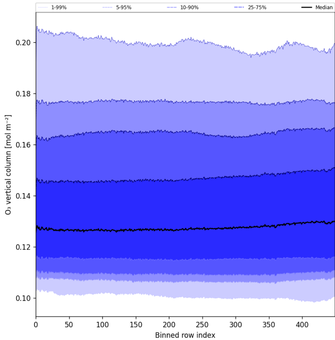
Figure 28: Along track statistics of “O 3 vertical column” for 2025-11-25 to 2025-11-27
