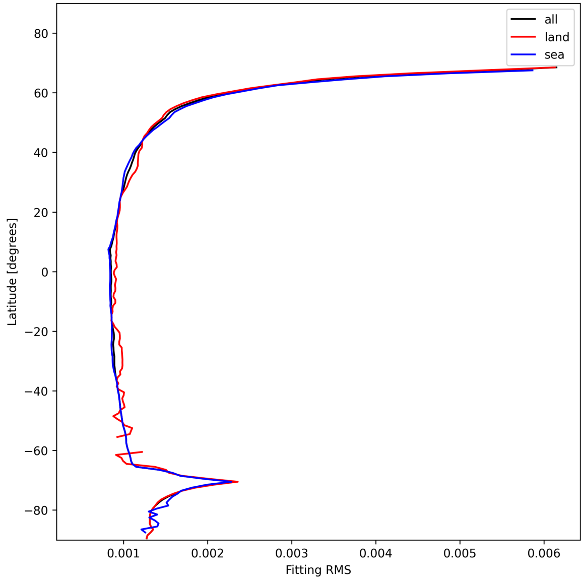
Figure 16: Zonal average of “Fitting RMS” for 2025-11-25 to 2025-11-27.
