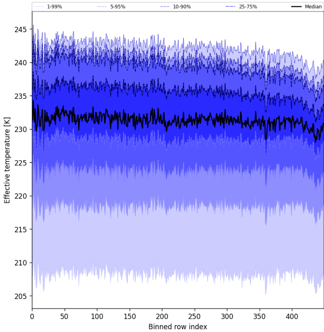
Figure 31: Along track statistics of “Effective temperature” for 2025-11-25 to 2025-11-27
