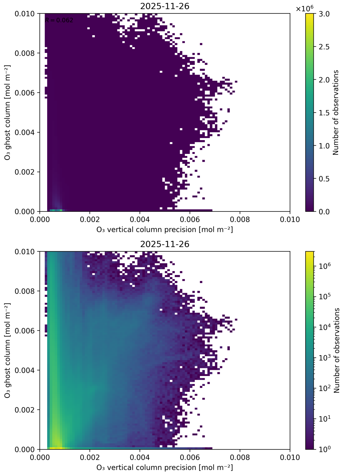
Figure 43: Scatter density plot of “ O_3 vertical column precision” against “ O_3 ghost column” for 2025-11-25 to 2025-11-27.
