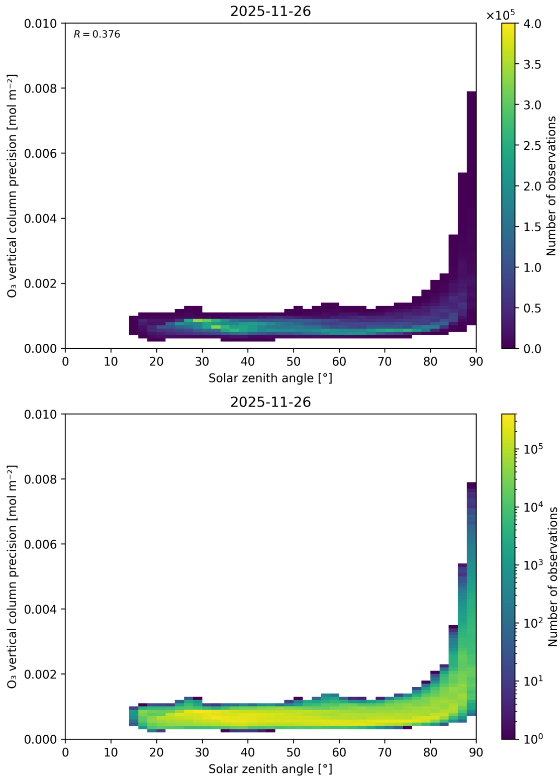
Figure 48: Scatter density plot of “Solar zenith angle” against “O 3 vertical column precision” for 2025-11-25 to 2025-11-27.
