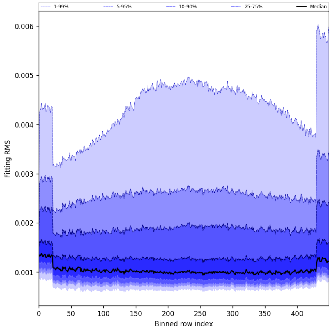
Figure 30: Along track statistics of “Fitting RMS” for 2025-11-26 to 2025-11-28
