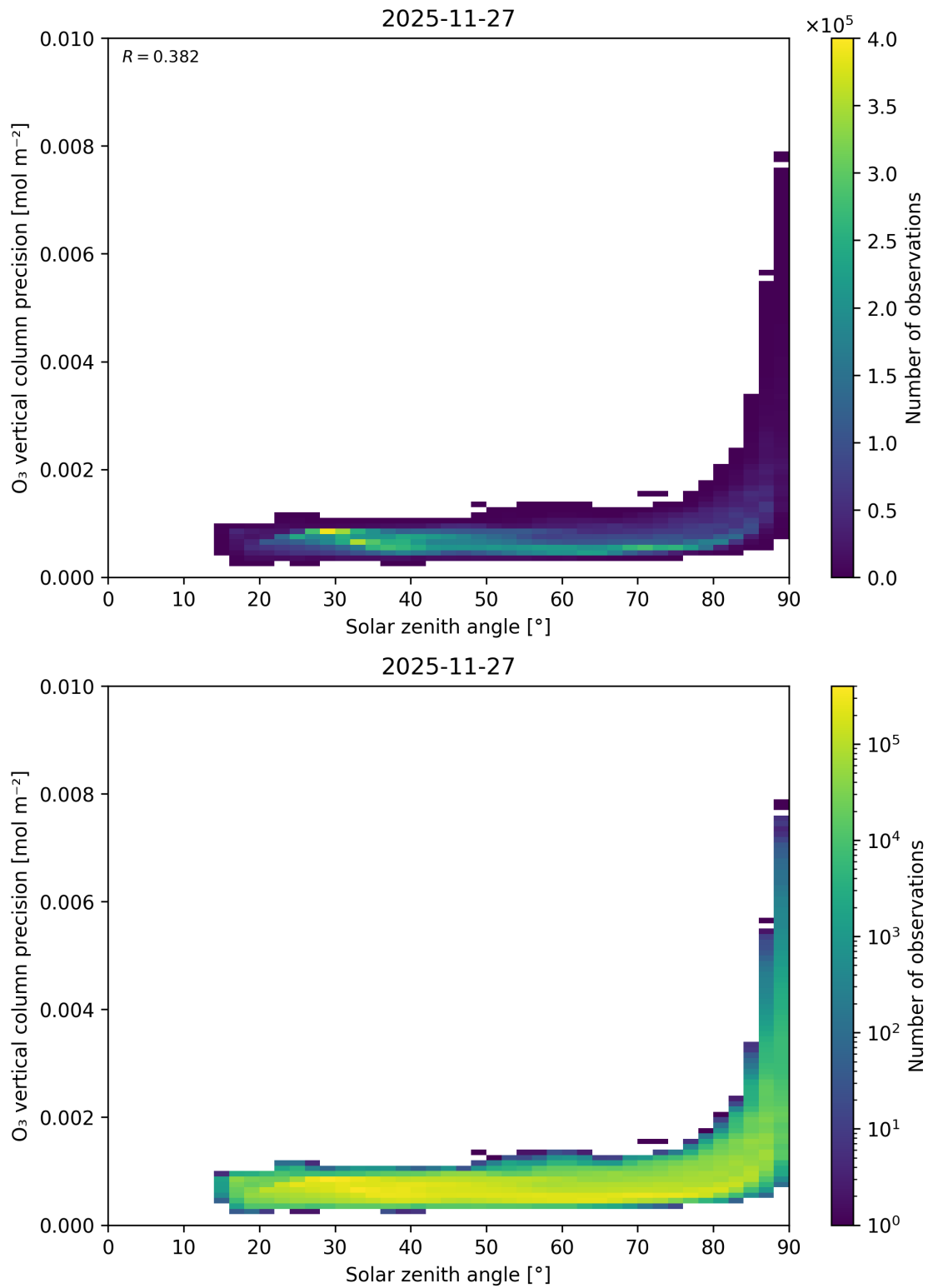
Figure 48: Scatter density plot of “Solar zenith angle” against “O 3 vertical column precision” for 2025-11-26 to 2025-11-28.
