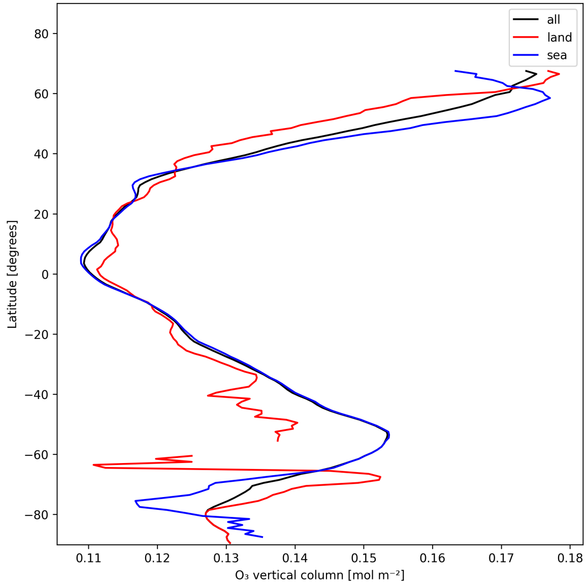
Figure 14: Zonal average of “O 3 vertical column” for 2025-11-26 to 2025-11-28.
