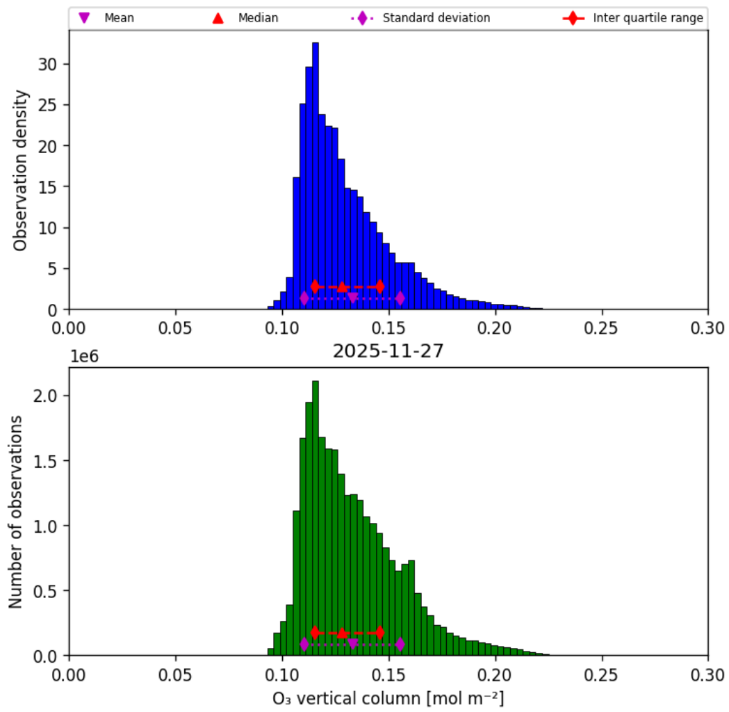
Figure 21: Histogram of “O 3 vertical column” for 2025-11-26 to 2025-11-28
