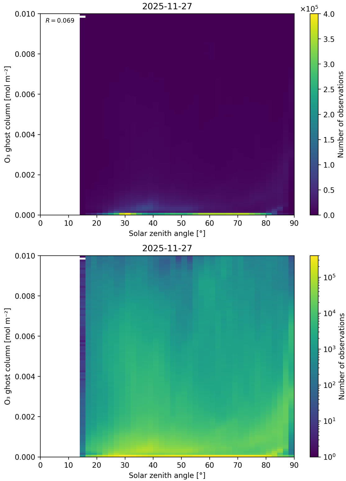
Figure 46: Scatter density plot of “Solar zenith angle” against “O 3 ghost column” for 2025-11-26 to 2025-11-28.
