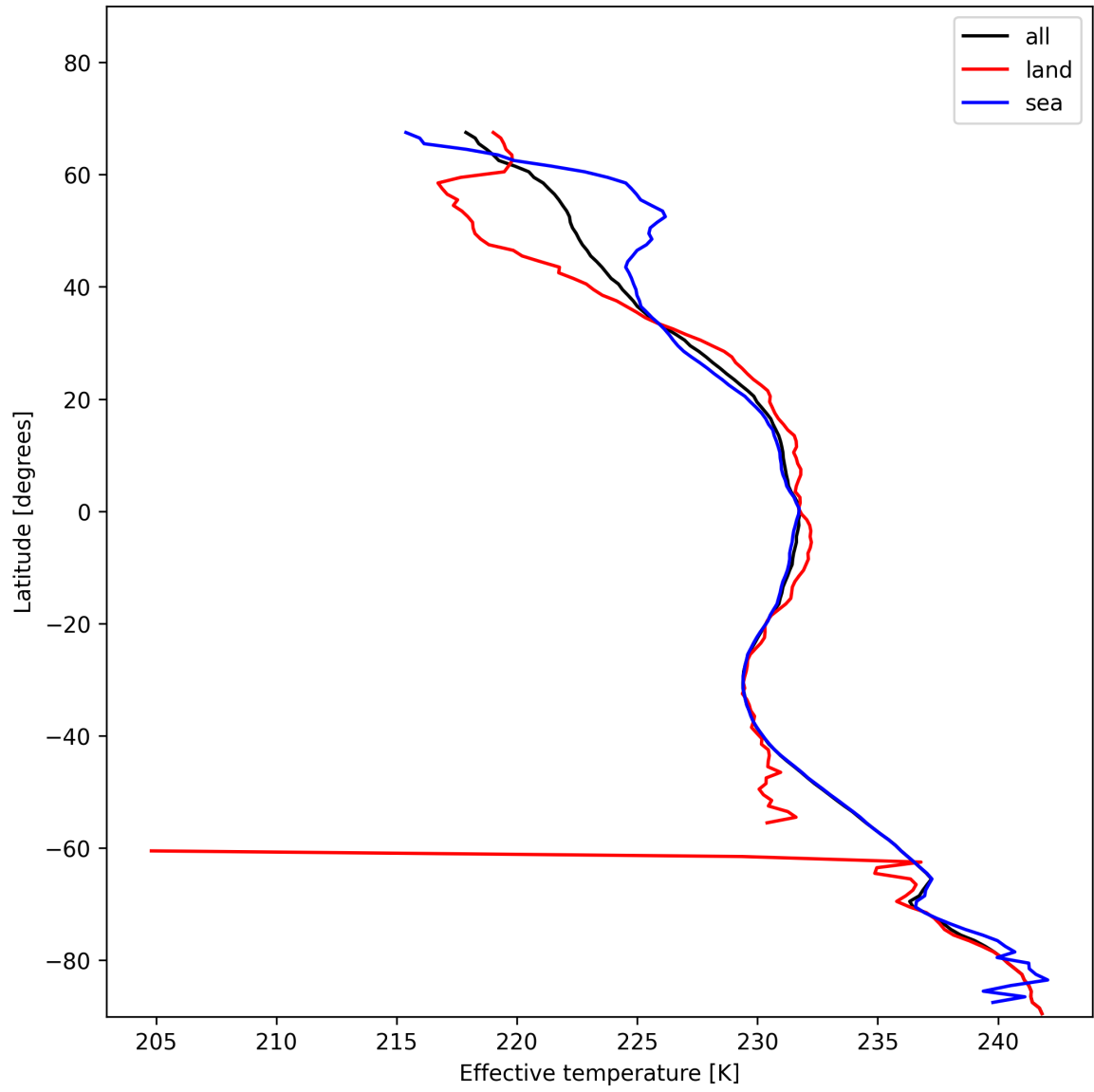
Figure 17: Zonal average of "Effective temperature" for 2025-11-26 to 2025-11-28.
