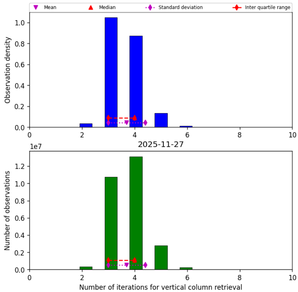
Figure 26: Histogram of “Number of iterations for vertical column retrieval” for 2025-11-26 to 2025-11-28
