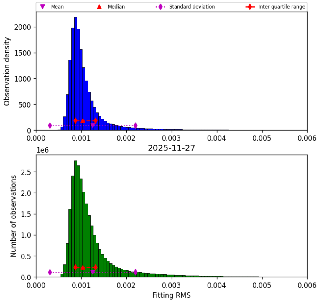
Figure 23: Histogram of “Fitting RMS” for 2025-11-26 to 2025-11-28
