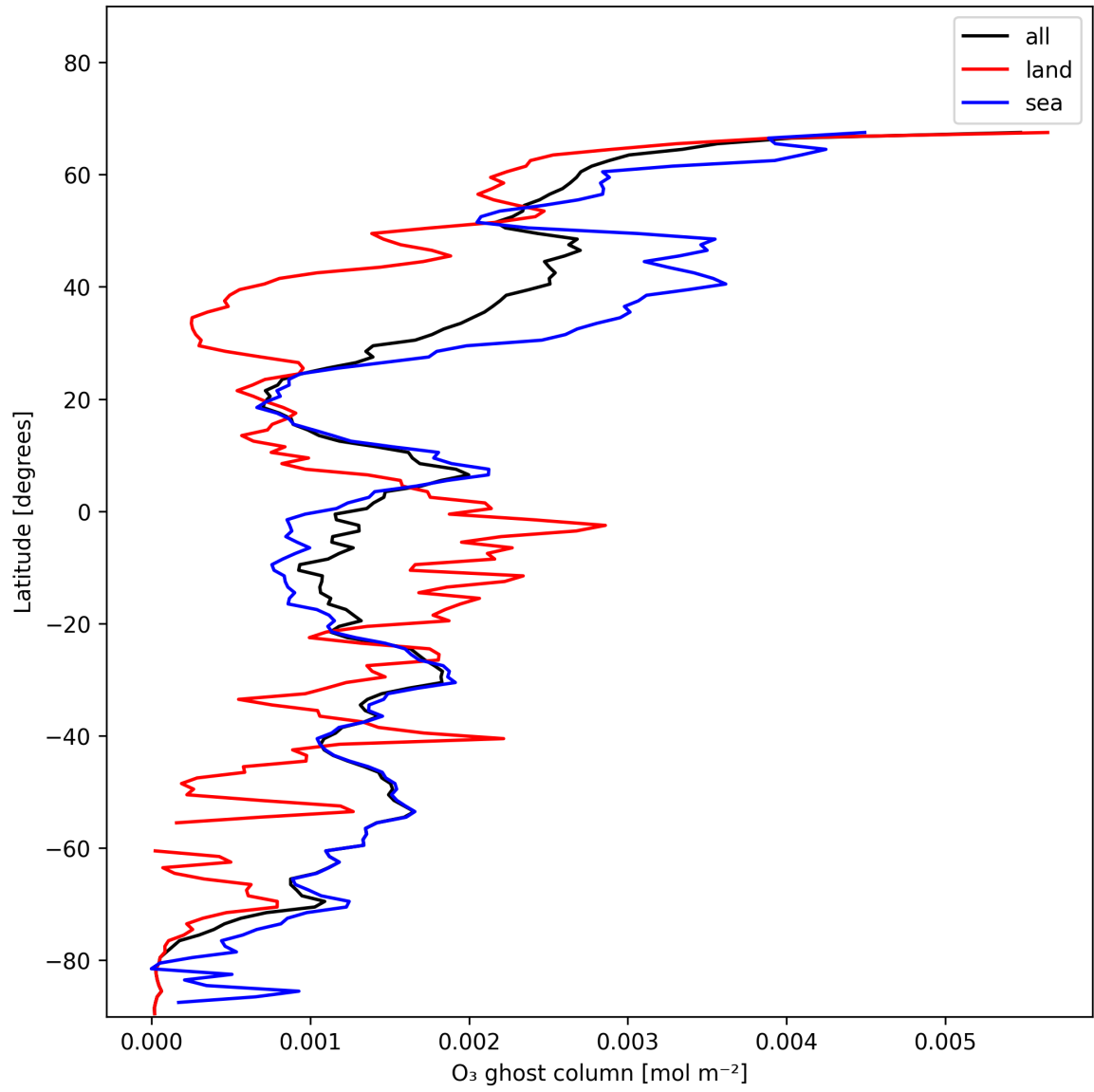
Figure 18: Zonal average of “O 3 ghost column” for 2025-11-26 to 2025-11-28.
