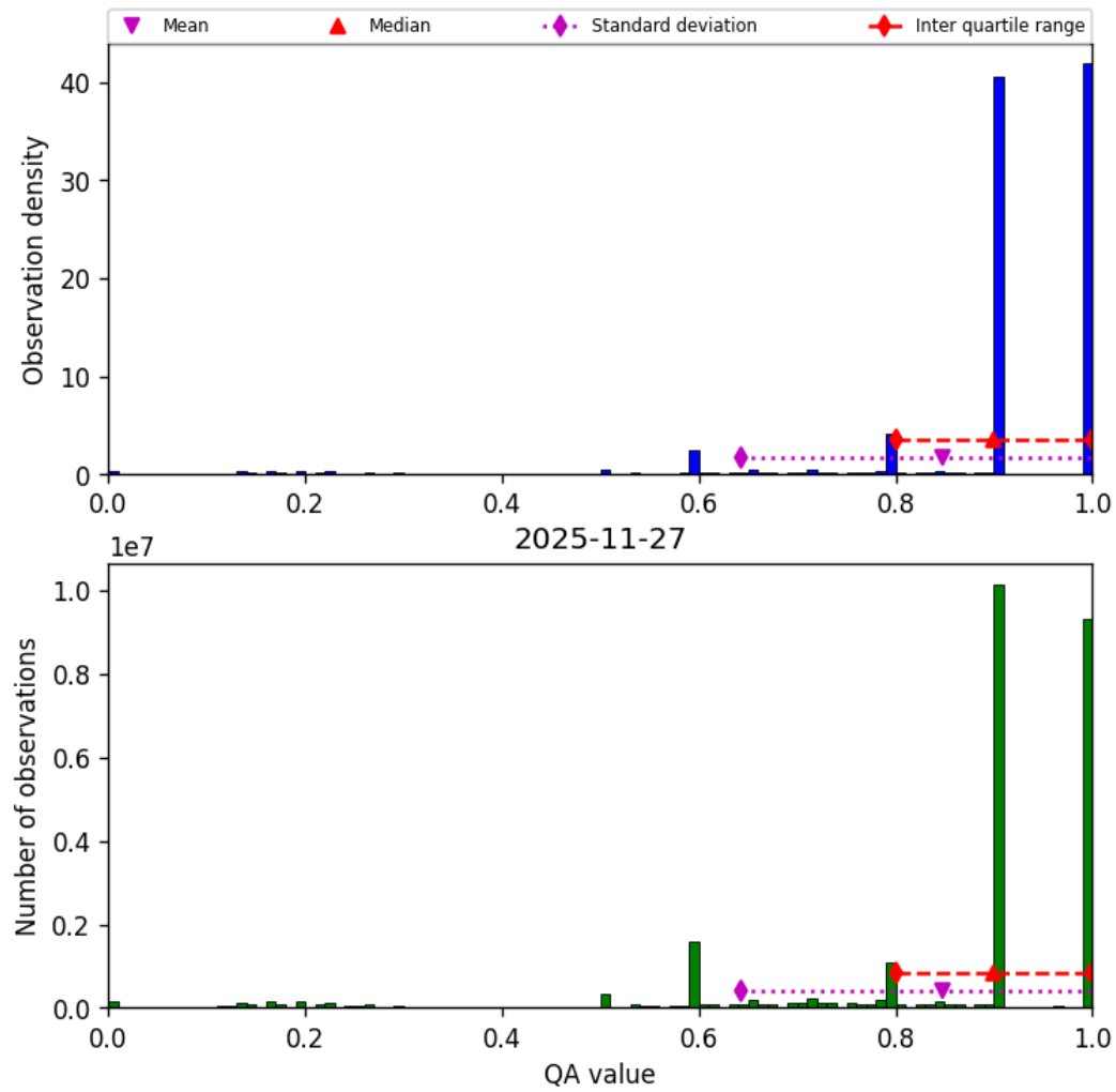
Figure 20: Histogram of “QA value” for 2025-11-26 to 2025-11-28
