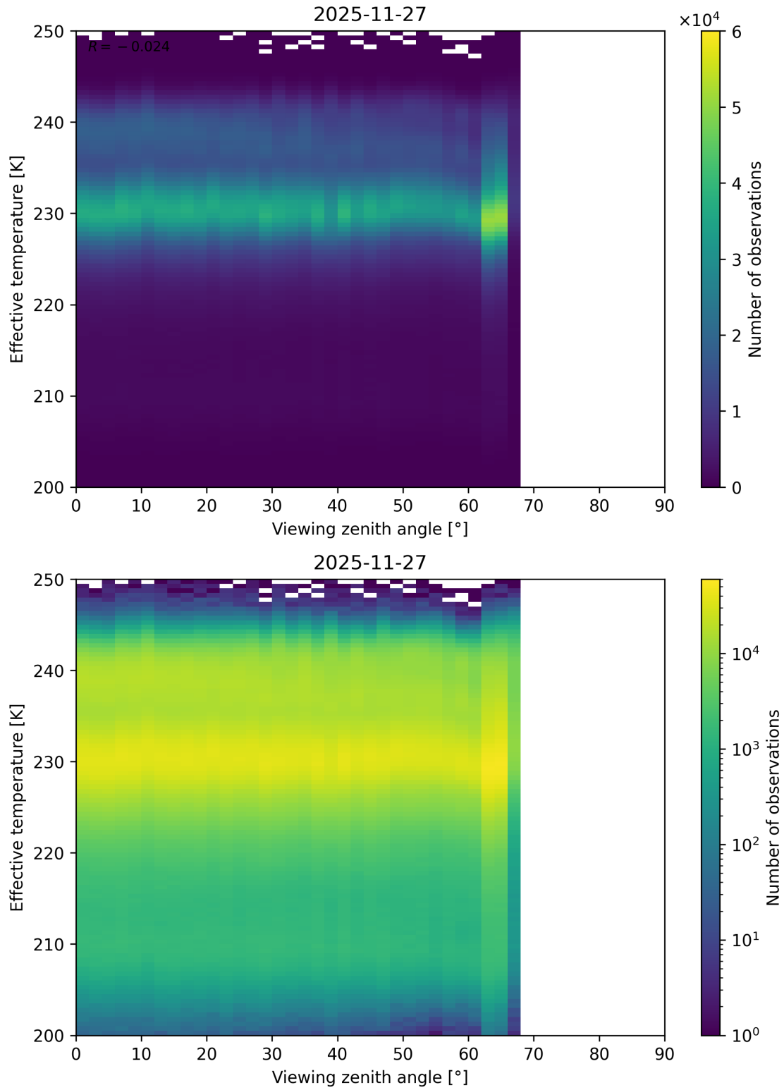
Figure 50: Scatter density plot of “Viewing zenith angle” against “Effective temperature” for 2025-11-26 to 2025-11-28.
