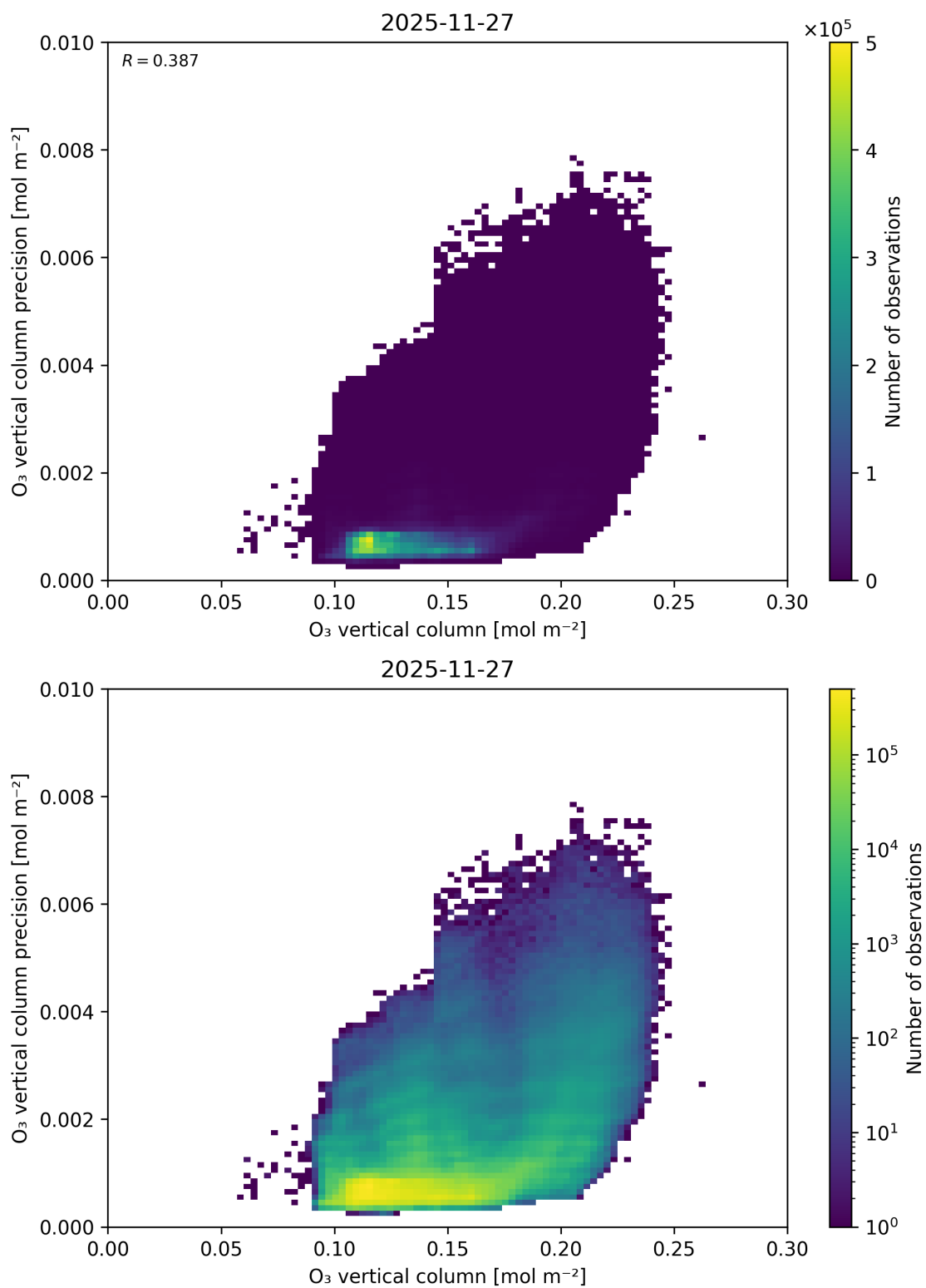
Figure 41: Scatter density plot of “O 3 vertical column” against “O 3 vertical column precision” for 2025-11-26 to 2025-11-28.
