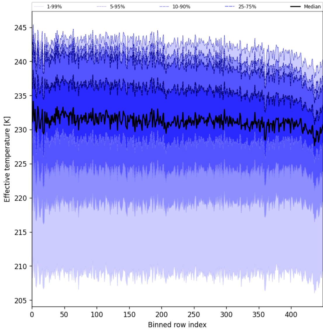
Figure 31: Along track statistics of “Effective temperature” for 2025-11-26 to 2025-11-28
