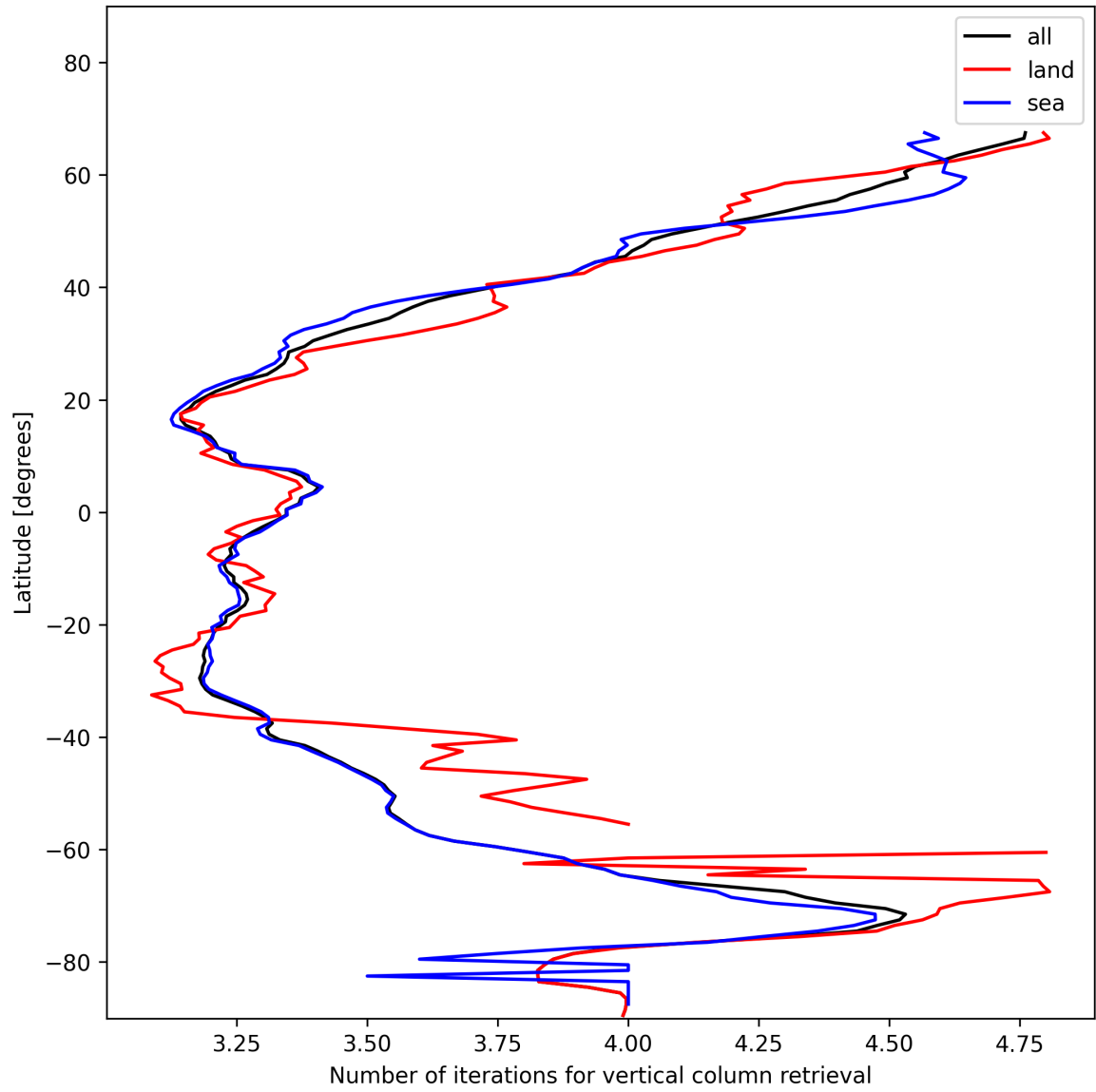
Figure 19: Zonal average of “Number of iterations for vertical column retrieval” for 2025-11-26 to 2025-11-28.
