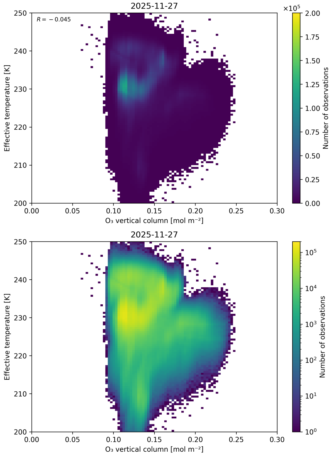
Figure 39: Scatter density plot of “O 3 vertical column” against “Effective temperature” for 2025-11-26 to 2025-11-28.
