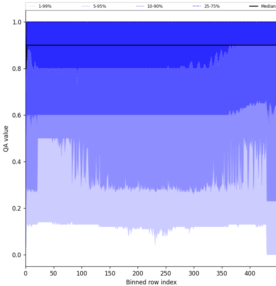
Figure 27: Along track statistics of “QA value” for 2025-11-26 to 2025-11-28
