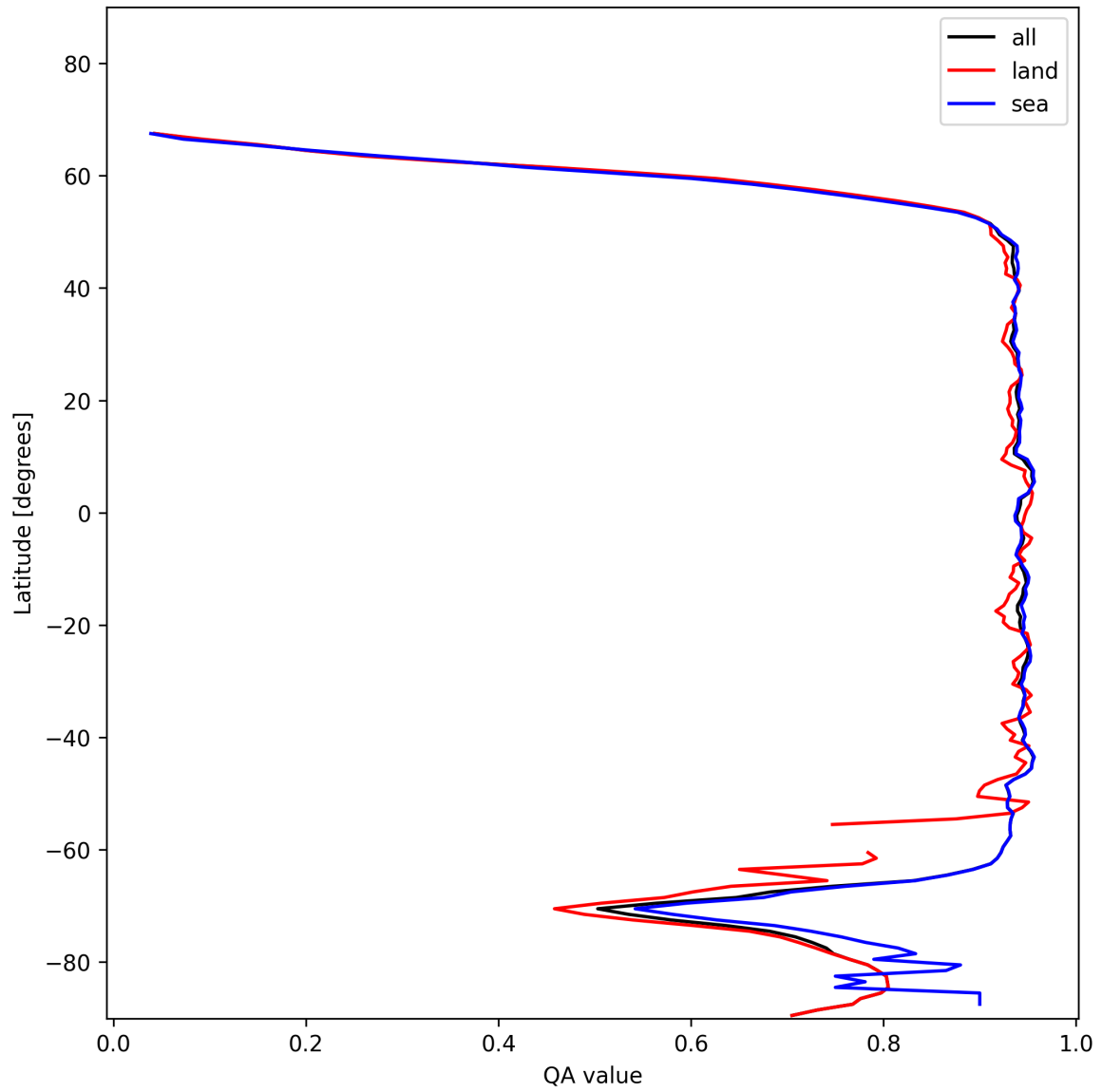
Figure 13: Zonal average of “QA value” for 2025-11-26 to 2025-11-28.
