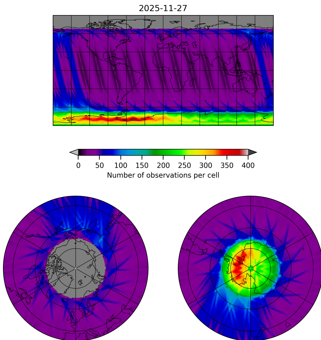
Figure 12: Map of the number of observations for 2025-11-26 to 2025-11-28
