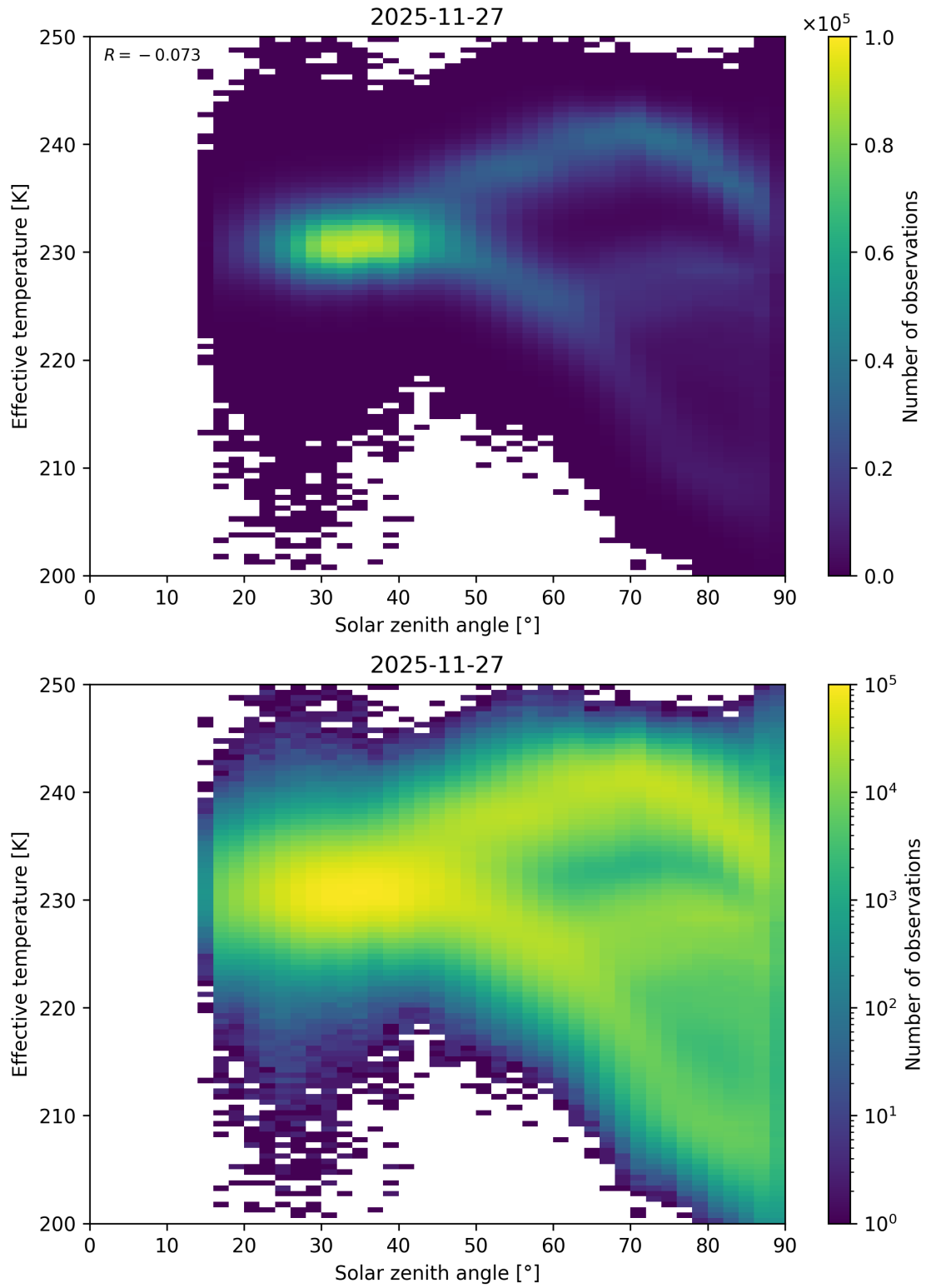
Figure 45: Scatter density plot of “Solar zenith angle” against “Effective temperature” for 2025-11-26 to 2025-11-28.
