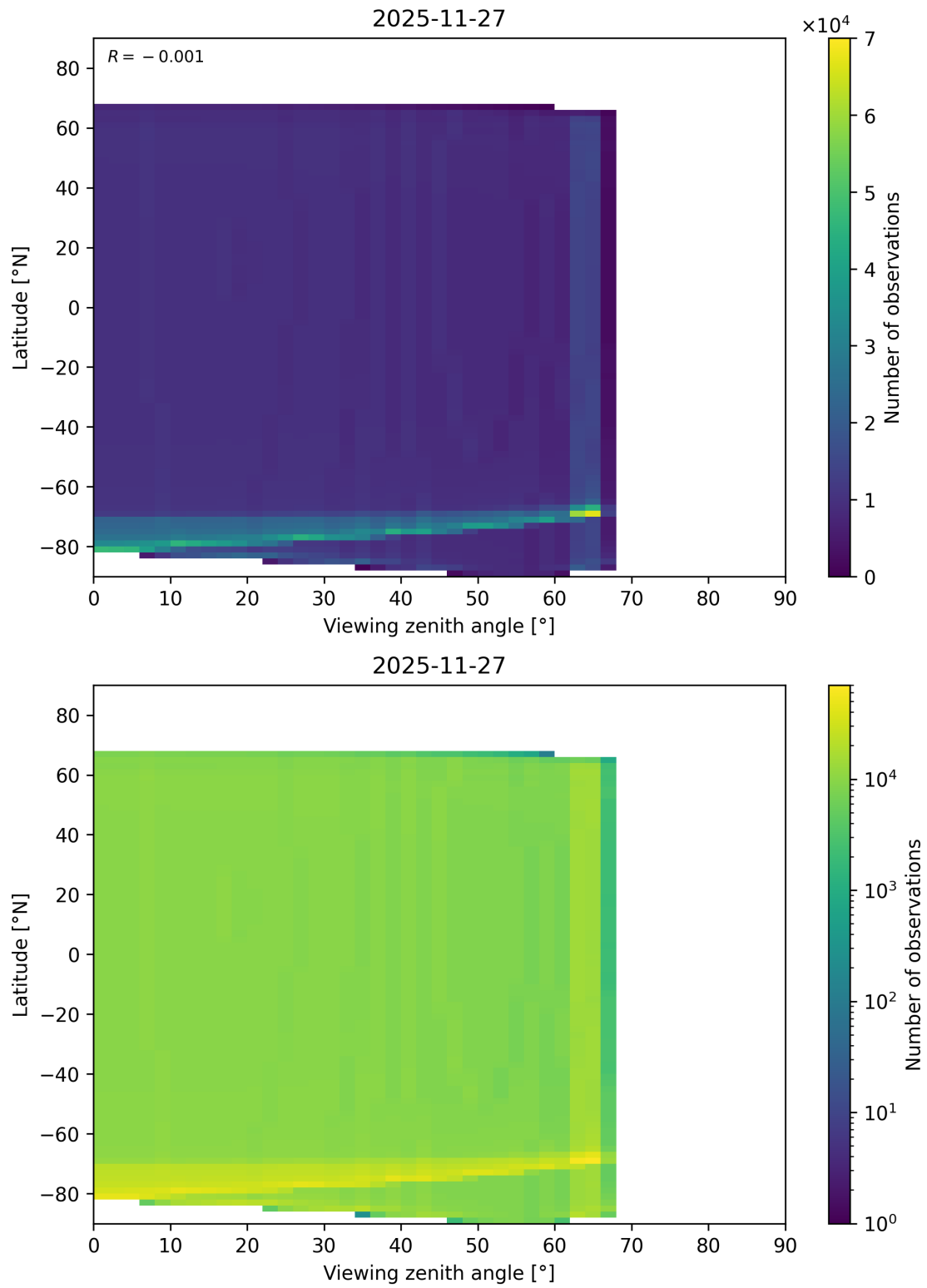
Figure 49: Scatter density plot of “Viewing zenith angle” against “Latitude” for 2025-11-26 to 2025-11-28.
