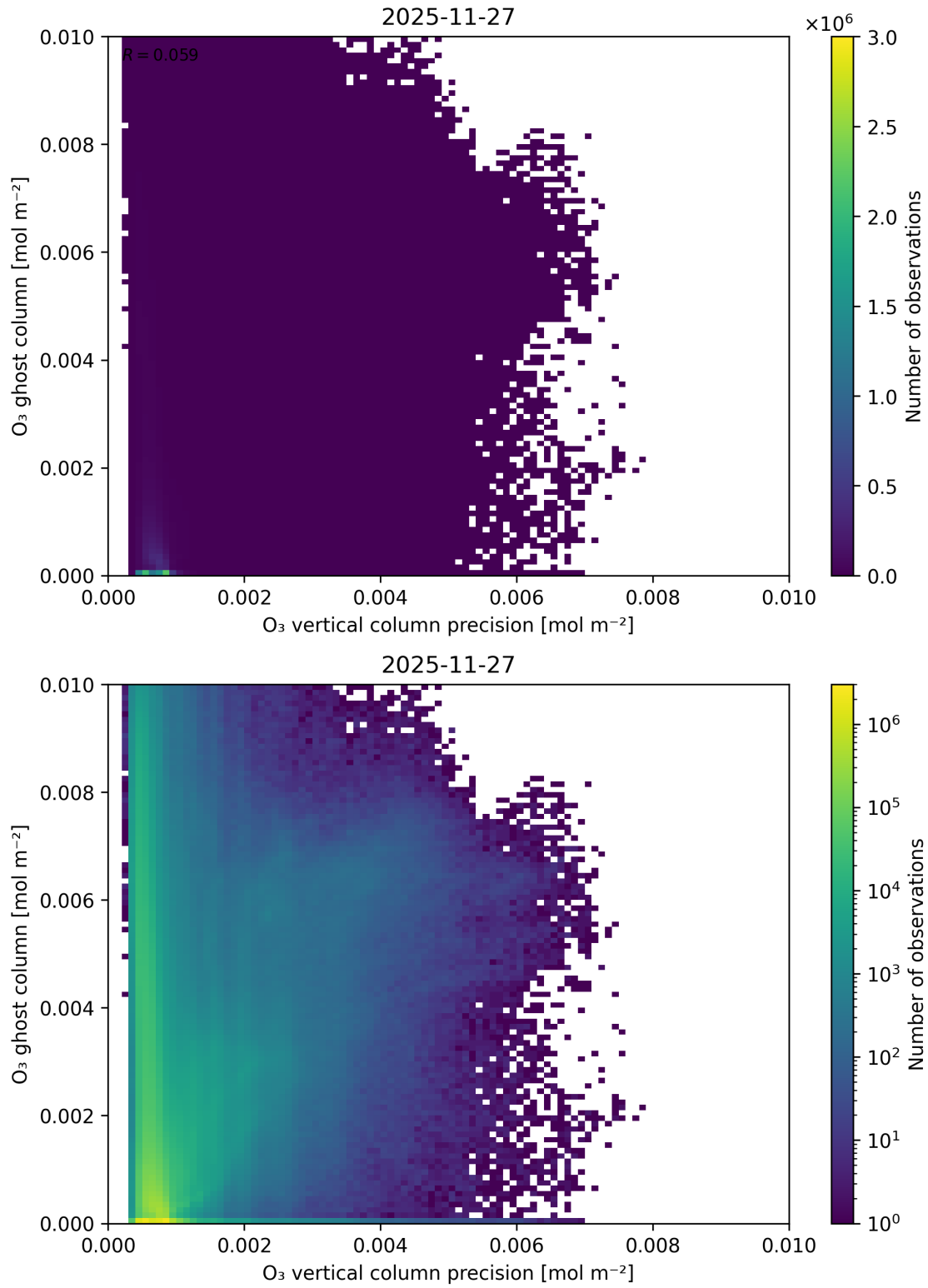
Figure 43: Scatter density plot of “O 3 vertical column precision” against “O 3 ghost column” for 2025-11-26 to 2025-11-28.
