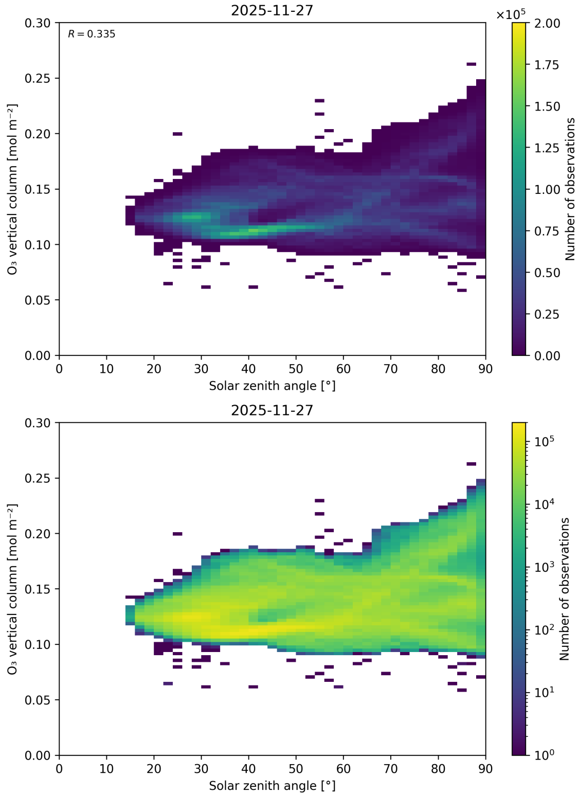
Figure 47: Scatter density plot of “Solar zenith angle” against “O 3 vertical column” for 2025-11-26 to 2025-11-28.
