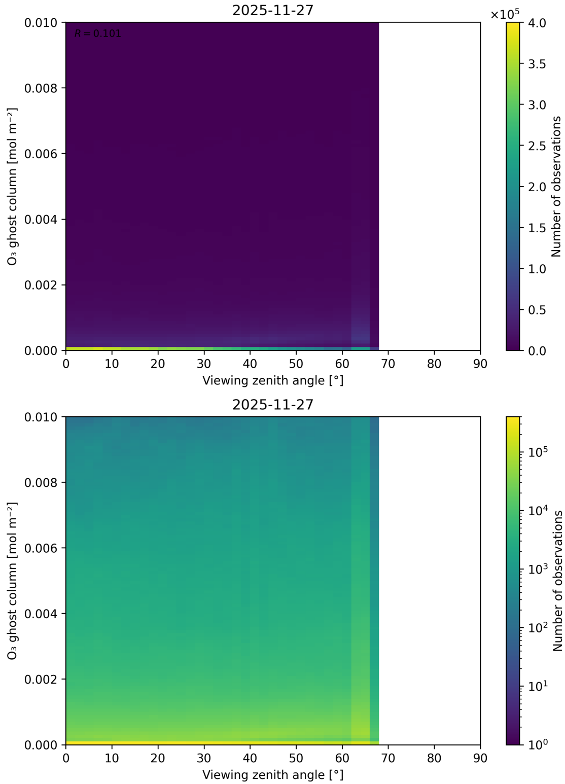
Figure 51: Scatter density plot of “Viewing zenith angle” against “O 3 ghost column” for 2025-11-26 to 2025-11-28.
