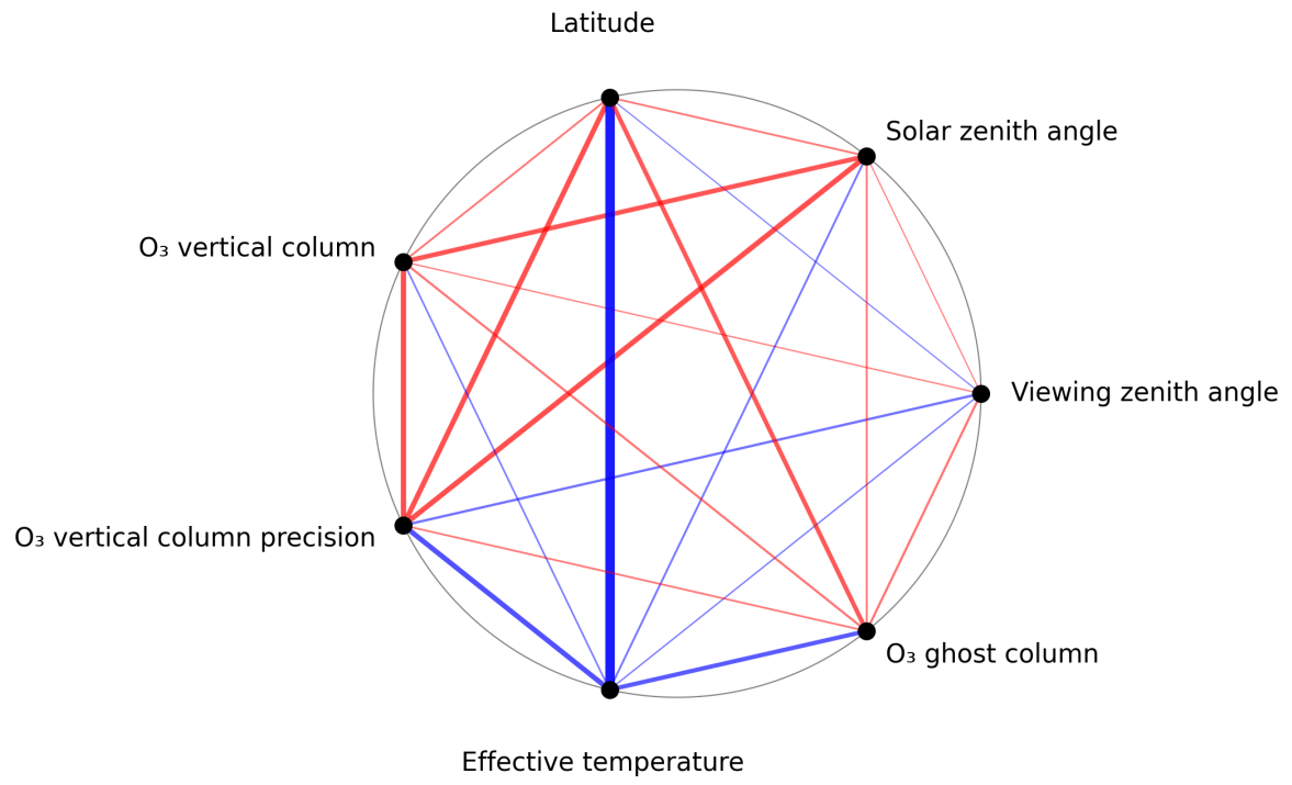
Figure 1: Map of correlation graph for 2025-11-26 to 2025-11-28.
