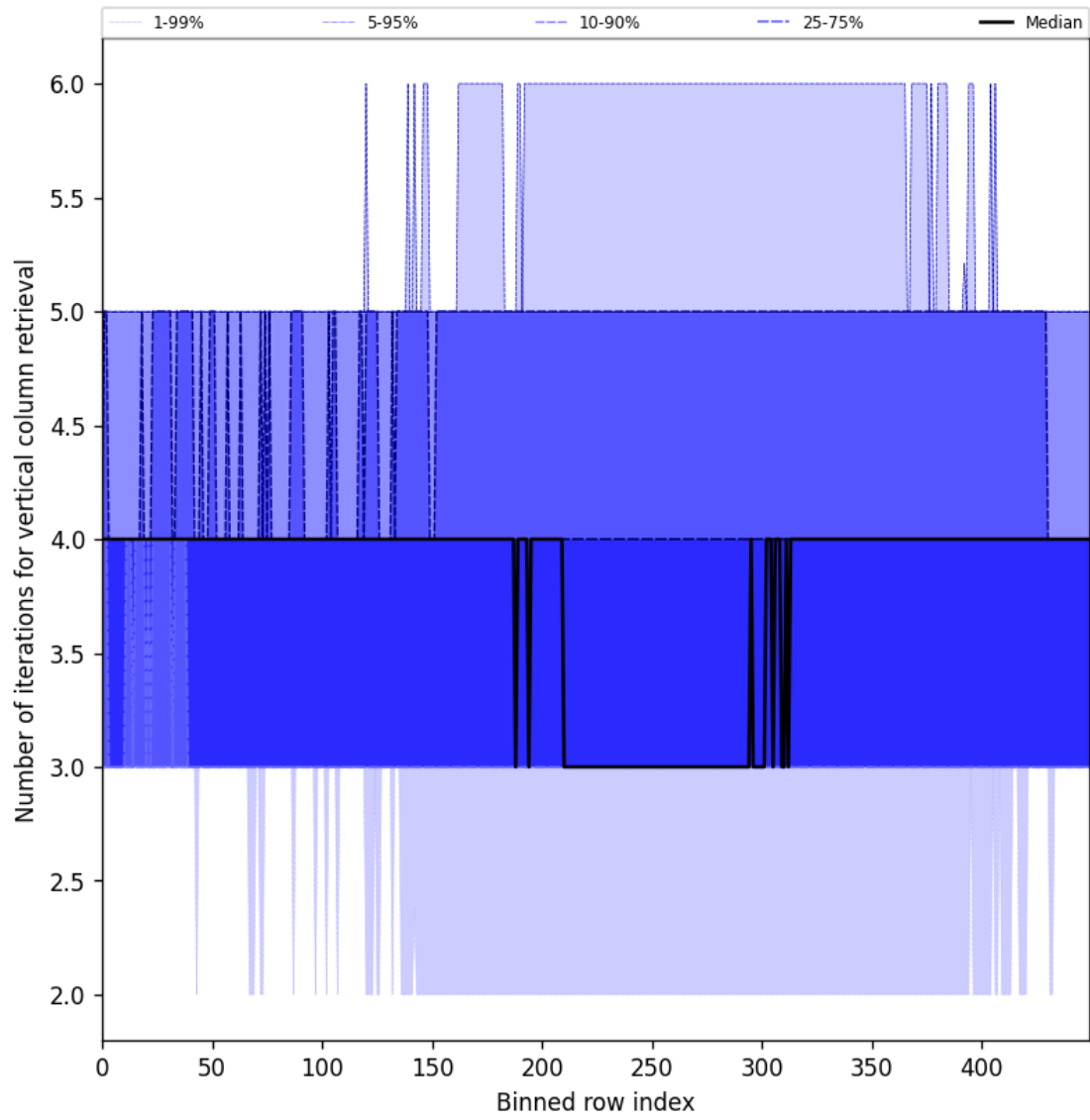
Figure 33: Along track statistics of “Number of iterations for vertical column retrieval” for 2025-11-26 to 2025-11-28
