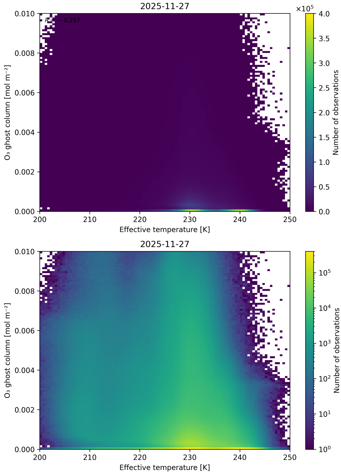
Figure 38: Scatter density plot of “Effective temperature” against “O 3 ghost column” for 2025-11-26 to 2025-11-28.
