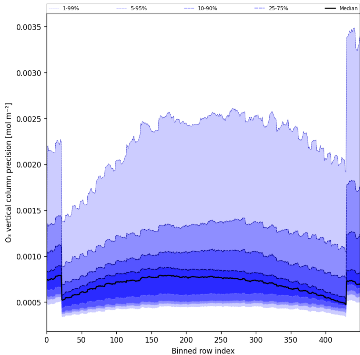
Figure 29: Along track statistics of “O 3 vertical column precision” for 2025-11-26 to 2025-11-28
