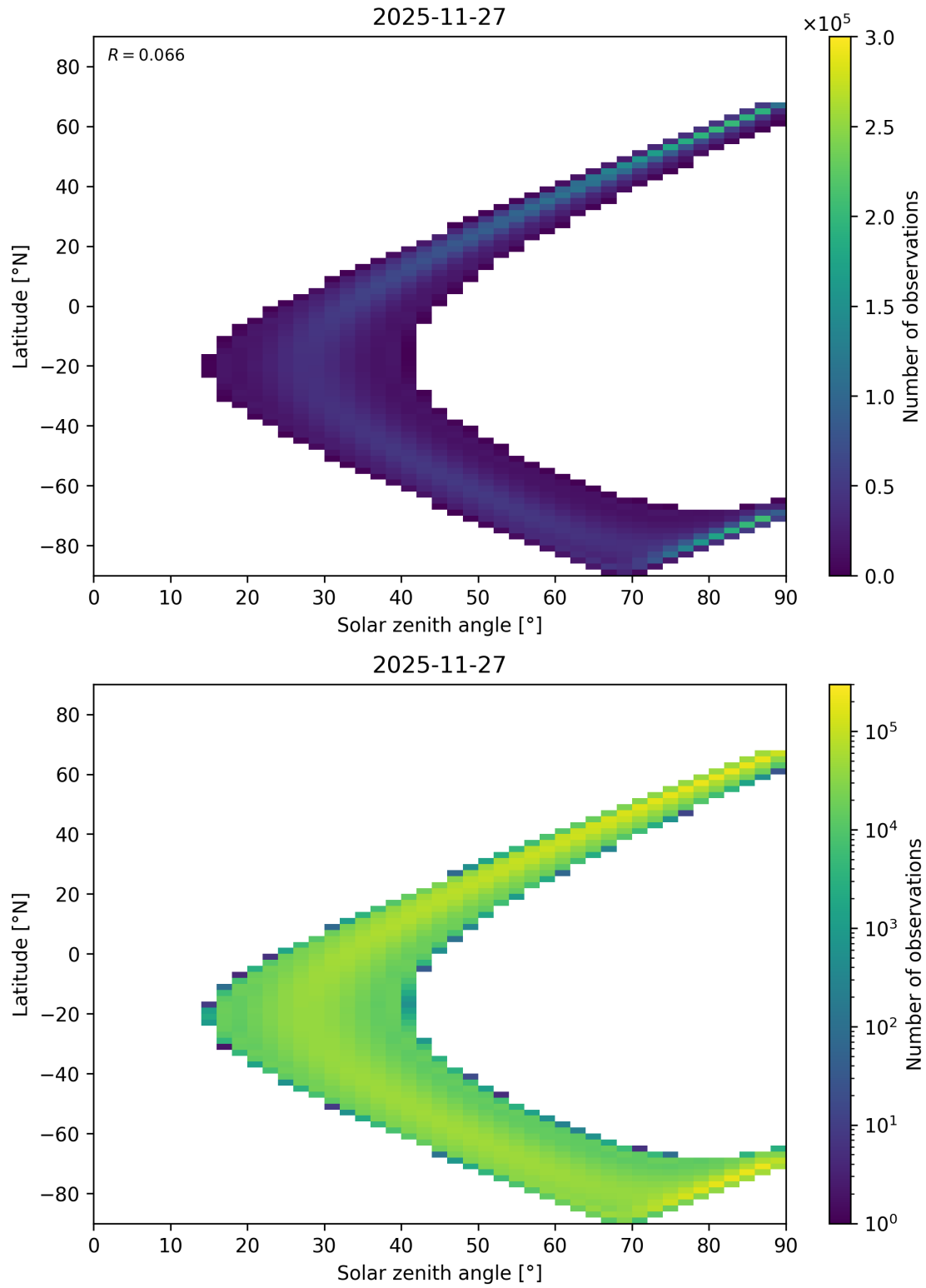
Figure 44: Scatter density plot of “Solar zenith angle” against “Latitude” for 2025-11-26 to 2025-11-28.
