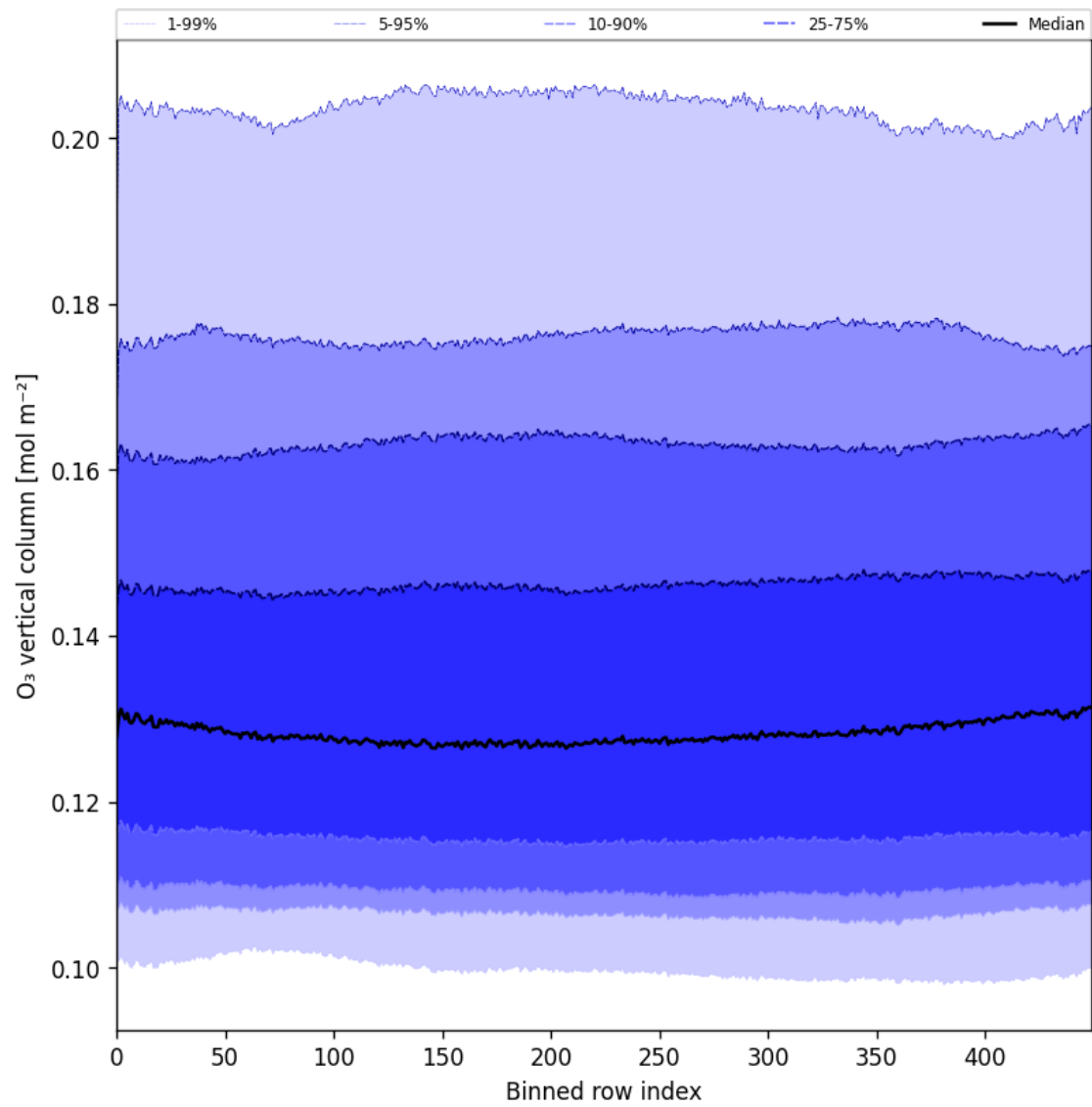
Figure 28: Along track statistics of “O 3 vertical column” for 2025-11-26 to 2025-11-28
