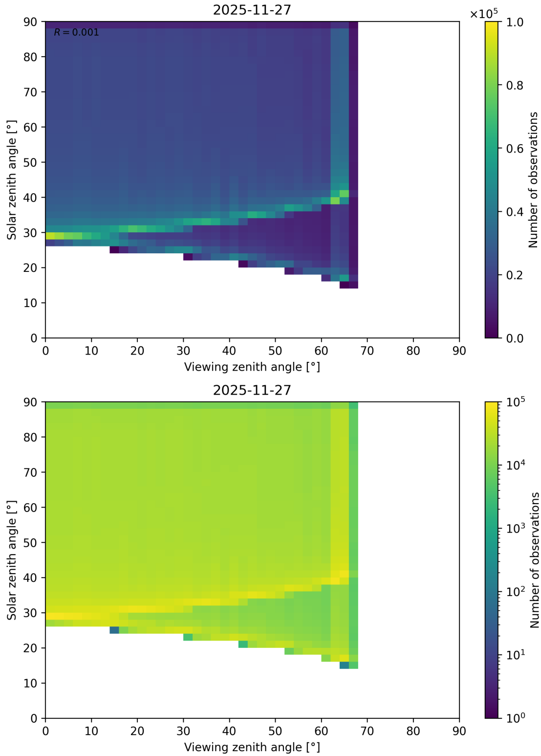
Figure 54: Scatter density plot of “Viewing zenith angle” against “Solar zenith angle” for 2025-11-26 to 2025-11-28.
