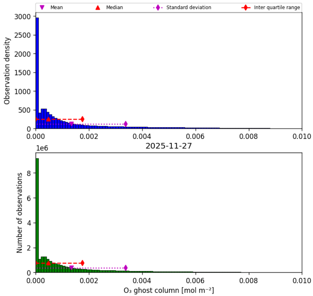
Figure 25: Histogram of “O 3 ghost column” for 2025-11-26 to 2025-11-28
