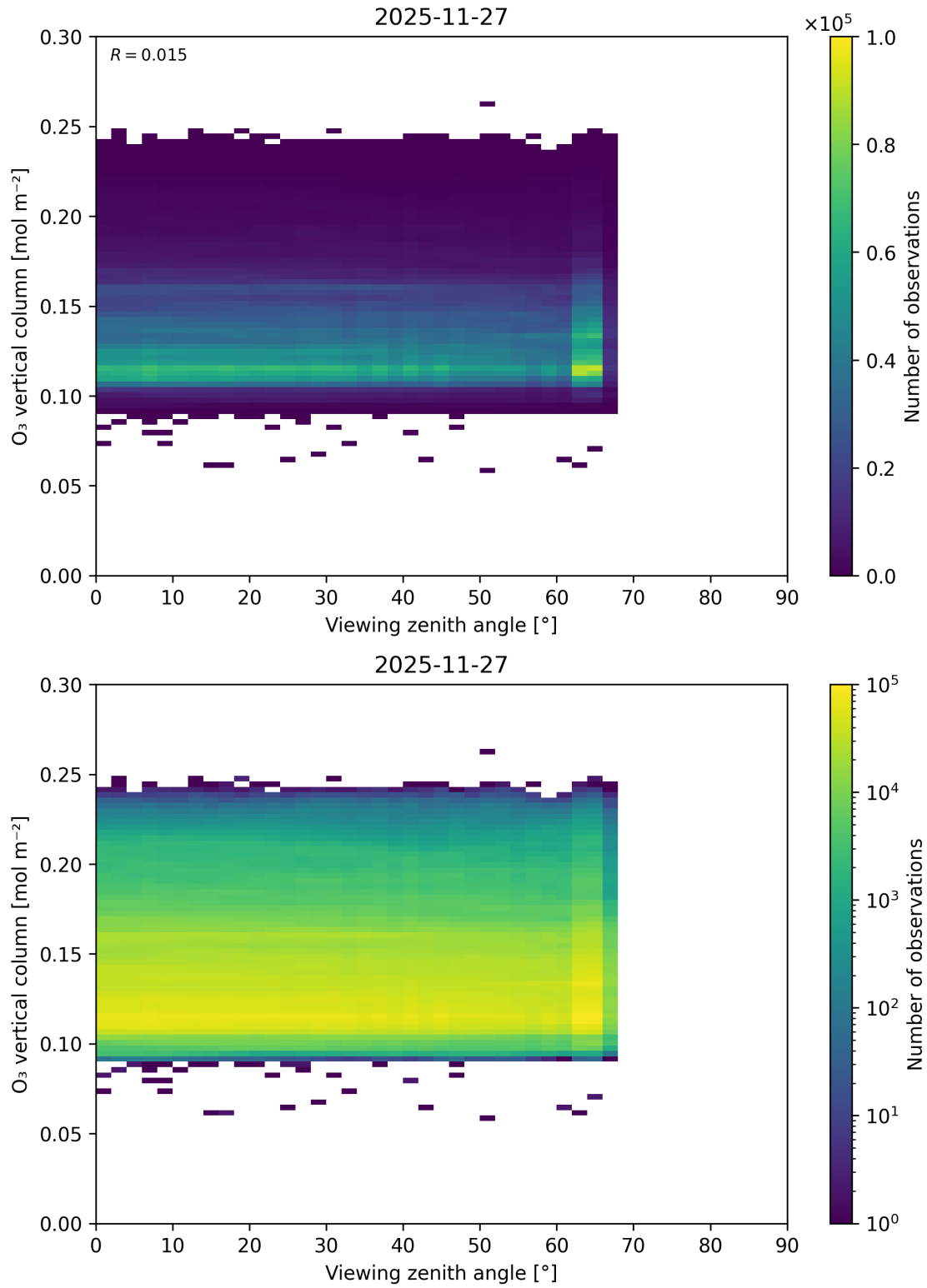
Figure 52: Scatter density plot of “Viewing zenith angle” against “O 3 vertical column” for 2025-11-26 to 2025-11-28.
