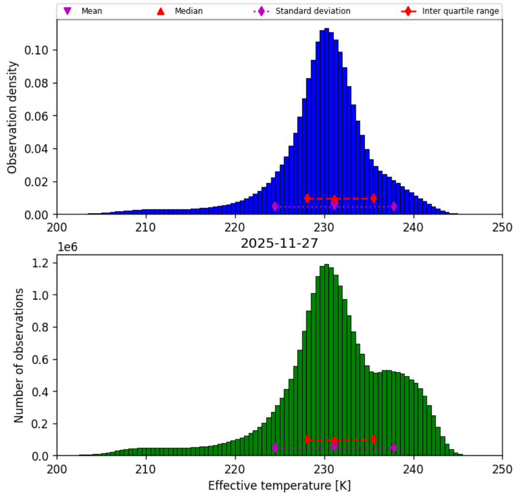
Figure 24: Histogram of “Effective temperature” for 2025-11-26 to 2025-11-28
