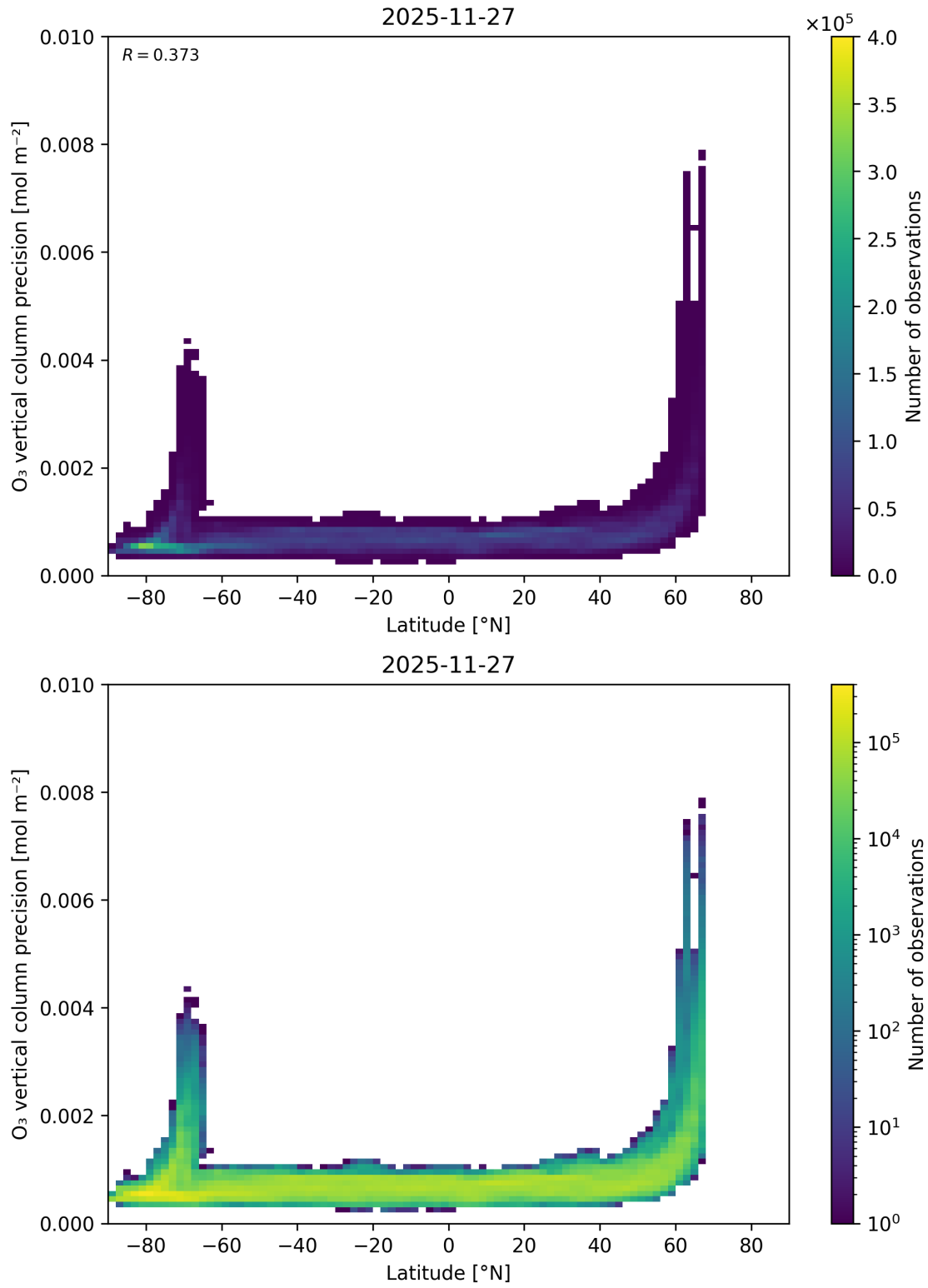
Figure 37: Scatter density plot of “Latitude” against “O 3 vertical column precision” for 2025-11-26 to 2025-11-28.
