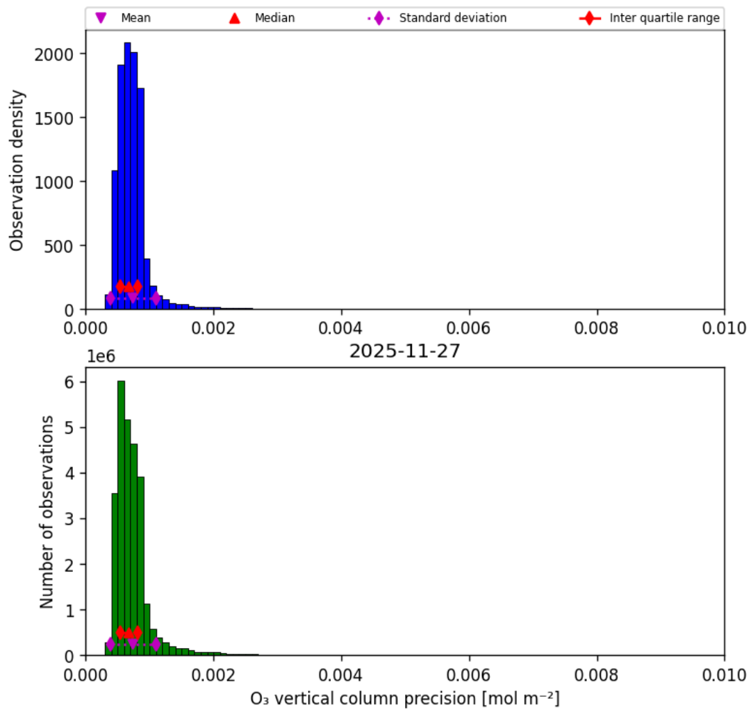
Figure 22: Histogram of “O 3 vertical column precision” for 2025-11-26 to 2025-11-28
