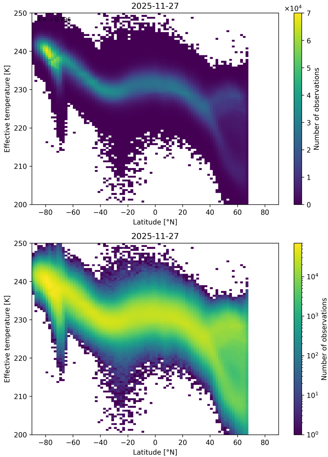
Figure 34: Scatter density plot of “Latitude” against “Effective temperature” for 2025-11-26 to 2025-11-28.
