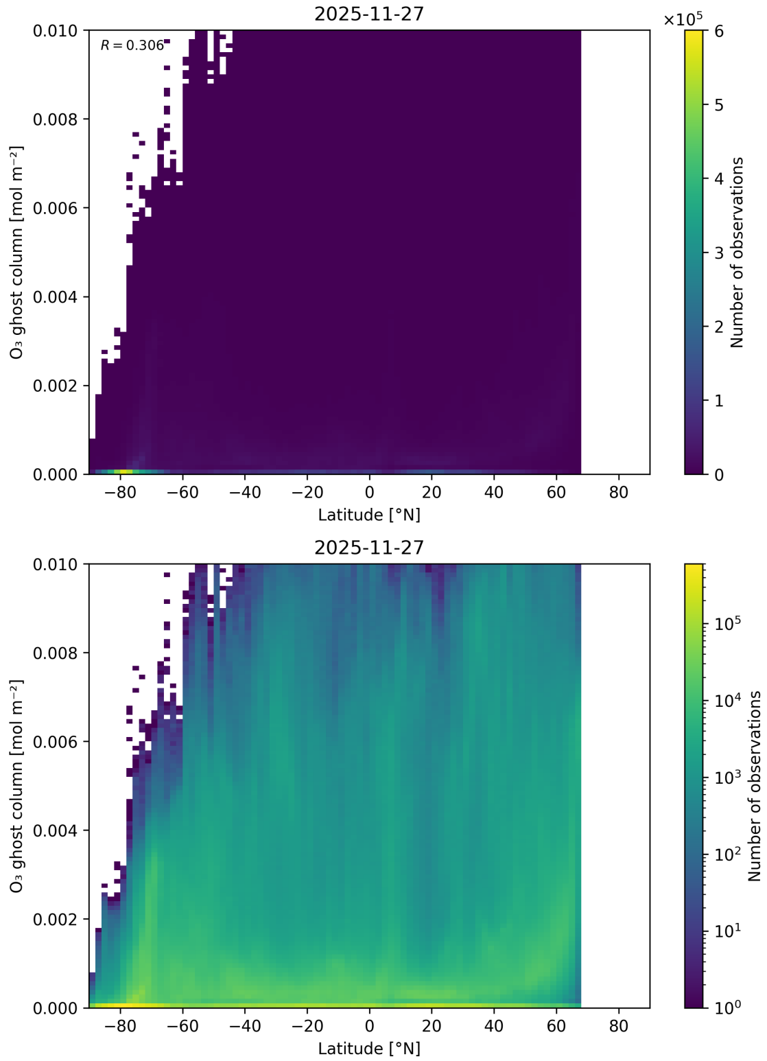
Figure 35: Scatter density plot of “Latitude” against “O 3 ghost column” for 2025-11-26 to 2025-11-28.
