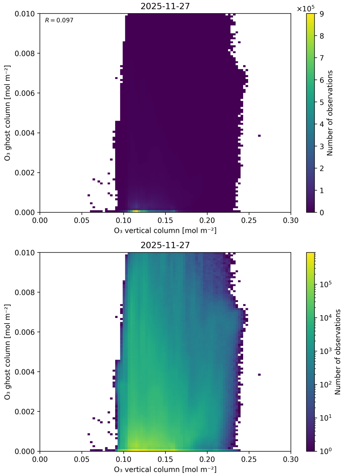
Figure 40: Scatter density plot of “O 3 vertical column” against “O 3 ghost column” for 2025-11-26 to 2025-11-28.
