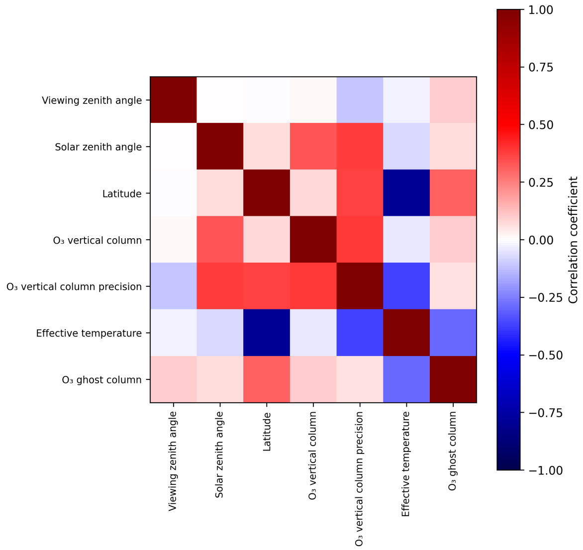
Figure 2: Map of correlation matrix for 2025-11-26 to 2025-11-28.
