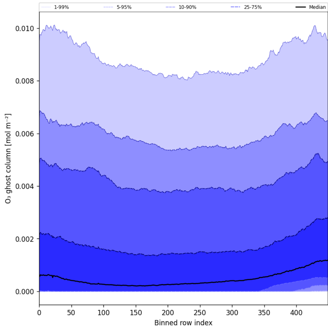
Figure 32: Along track statistics of “O 3 ghost column” for 2025-11-26 to 2025-11-28
