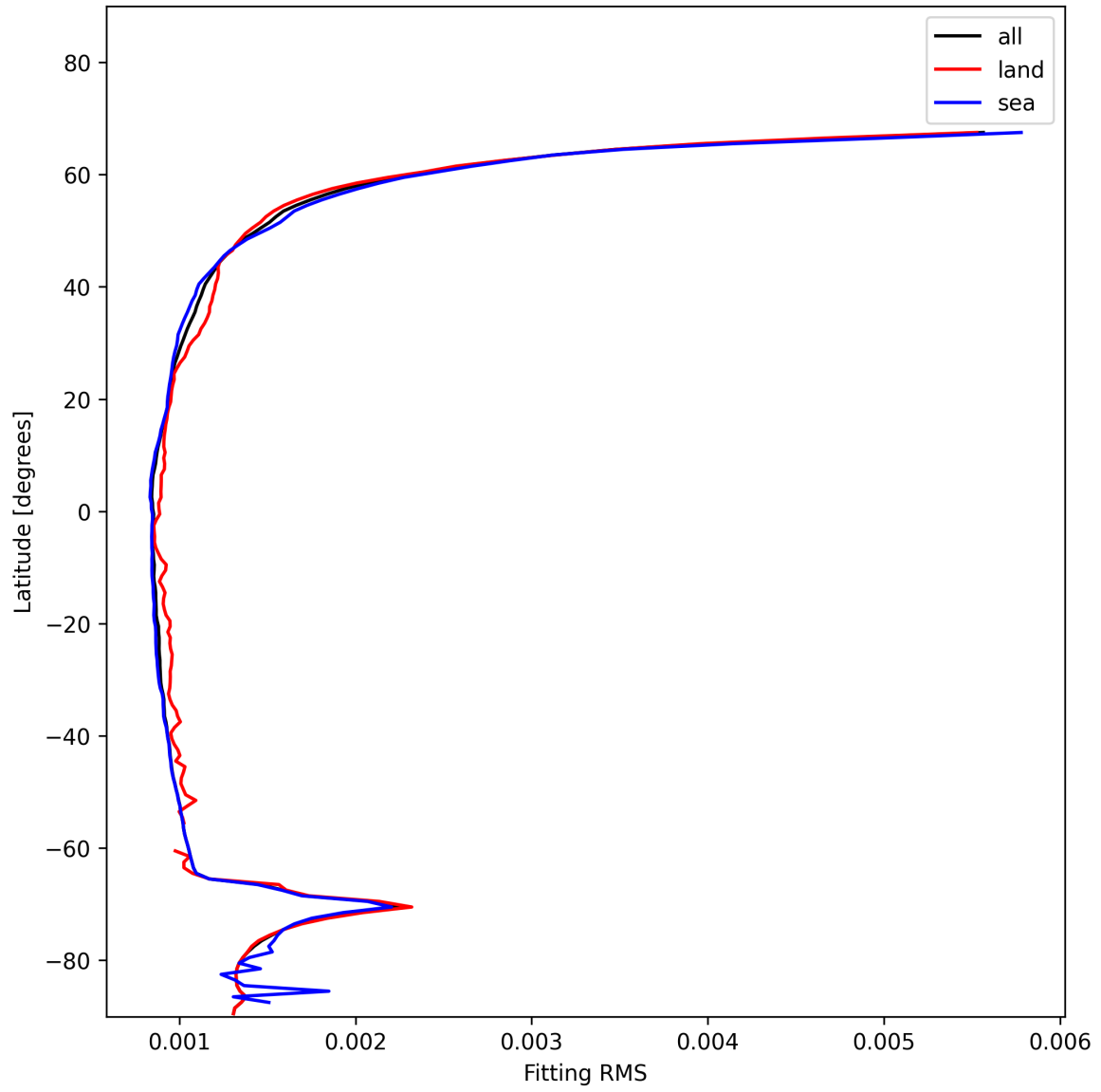
Figure 16: Zonal average of “Fitting RMS” for 2025-11-26 to 2025-11-28.
