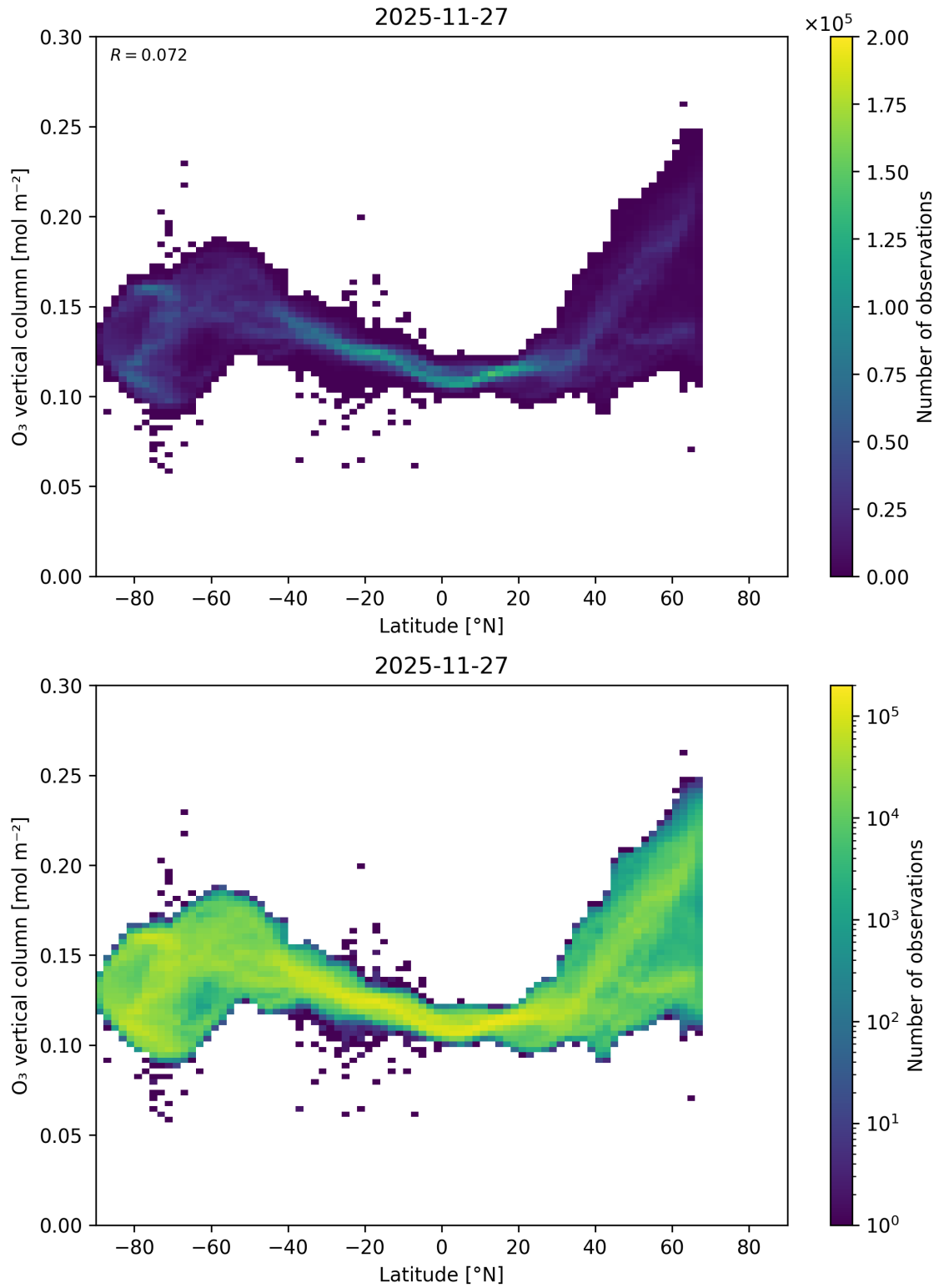
Figure 36: Scatter density plot of “Latitude” against “O 3 vertical column” for 2025-11-26 to 2025-11-28.
