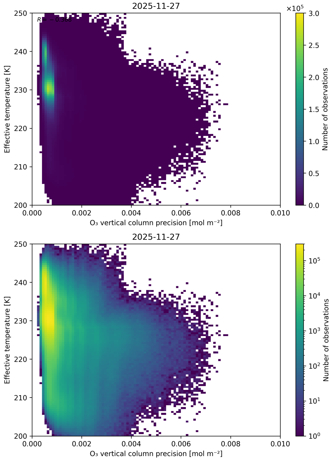
Figure 42: Scatter density plot of “O 3 vertical column precision” against “Effective temperature” for 2025-11-26 to 2025-11-28.
