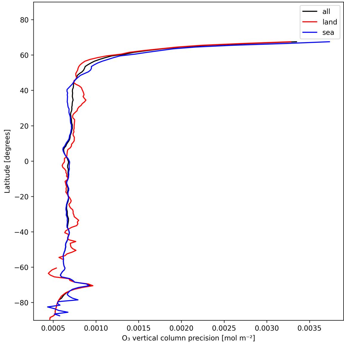
Figure 15: Zonal average of “O 3 vertical column precision” for 2025-11-26 to 2025-11-28.
