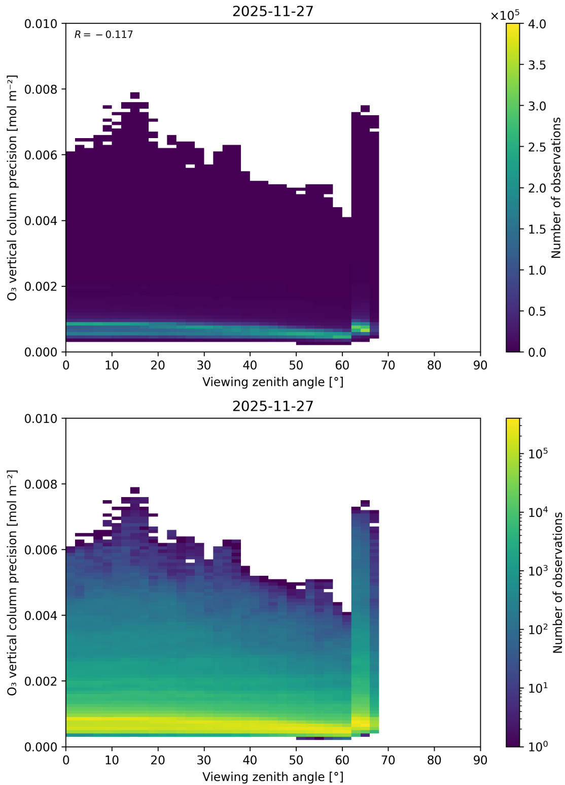
Figure 53: Scatter density plot of “Viewing zenith angle” against “O 3 vertical column precision” for 2025-11-26 to 2025-11-28.
