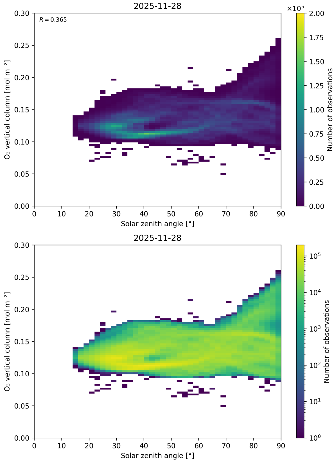
Figure 47: Scatter density plot of “Solar zenith angle” against “O 3 vertical column” for 2025-11-28 to 2025-11-29.
