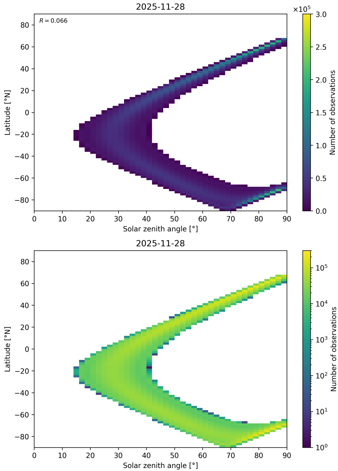
Figure 44: Scatter density plot of “Solar zenith angle” against “Latitude” for 2025-11-28 to 2025-11-29.
