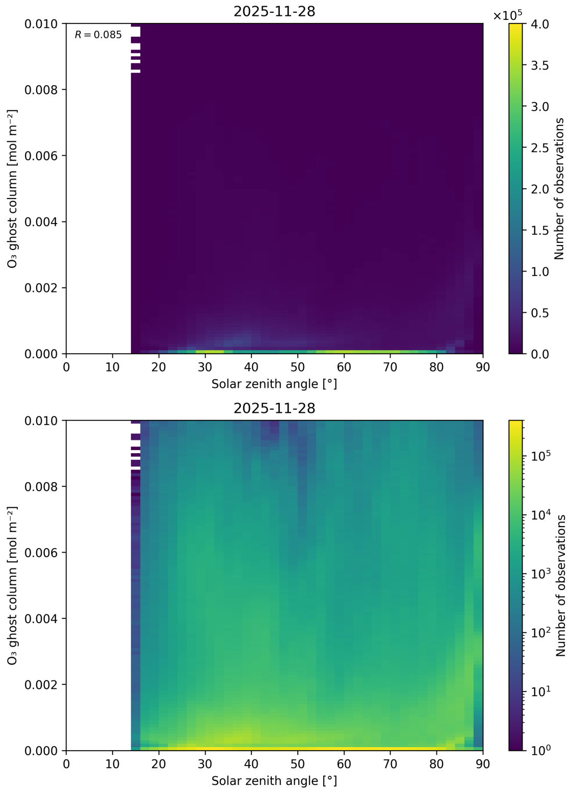
Figure 46: Scatter density plot of “Solar zenith angle” against “O 3 ghost column” for 2025-11-28 to 2025-11-29.
