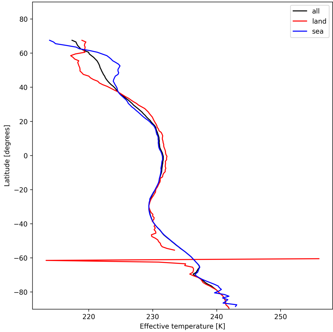
Figure 17: Zonal average of “Effective temperature” for 2025-11-28 to 2025-11-29.
