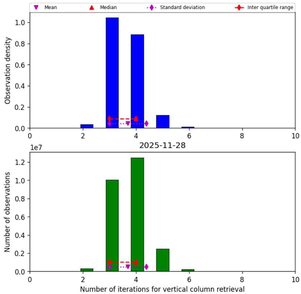
Figure 26: Histogram of “Number of iterations for vertical column retrieval” for 2025-11-28 to 2025-11-29
