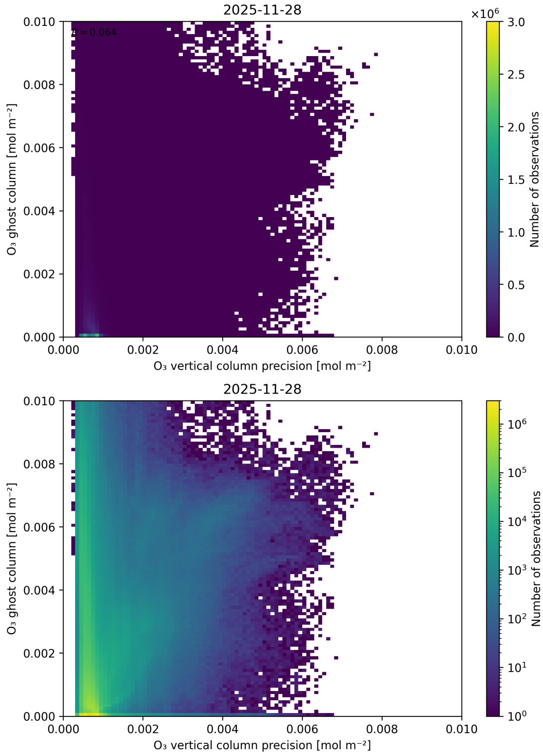
Figure 43: Scatter density plot of “O 3 vertical column precision” against “O 3 ghost column” for 2025-11-28 to 2025-11-29.
