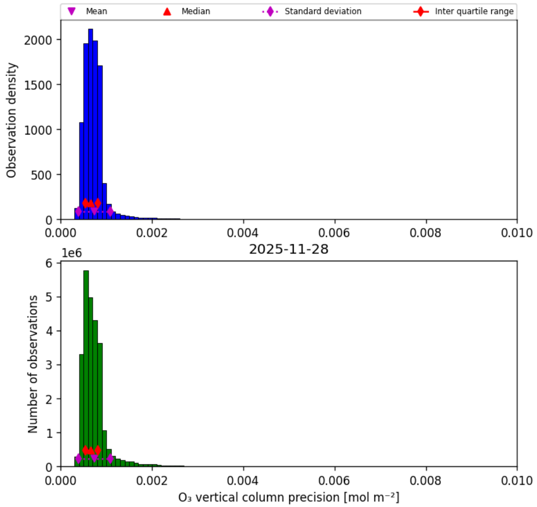
Figure 22: Histogram of "O 3 vertical column precision" for 2025-11-28 to 2025-11-29
