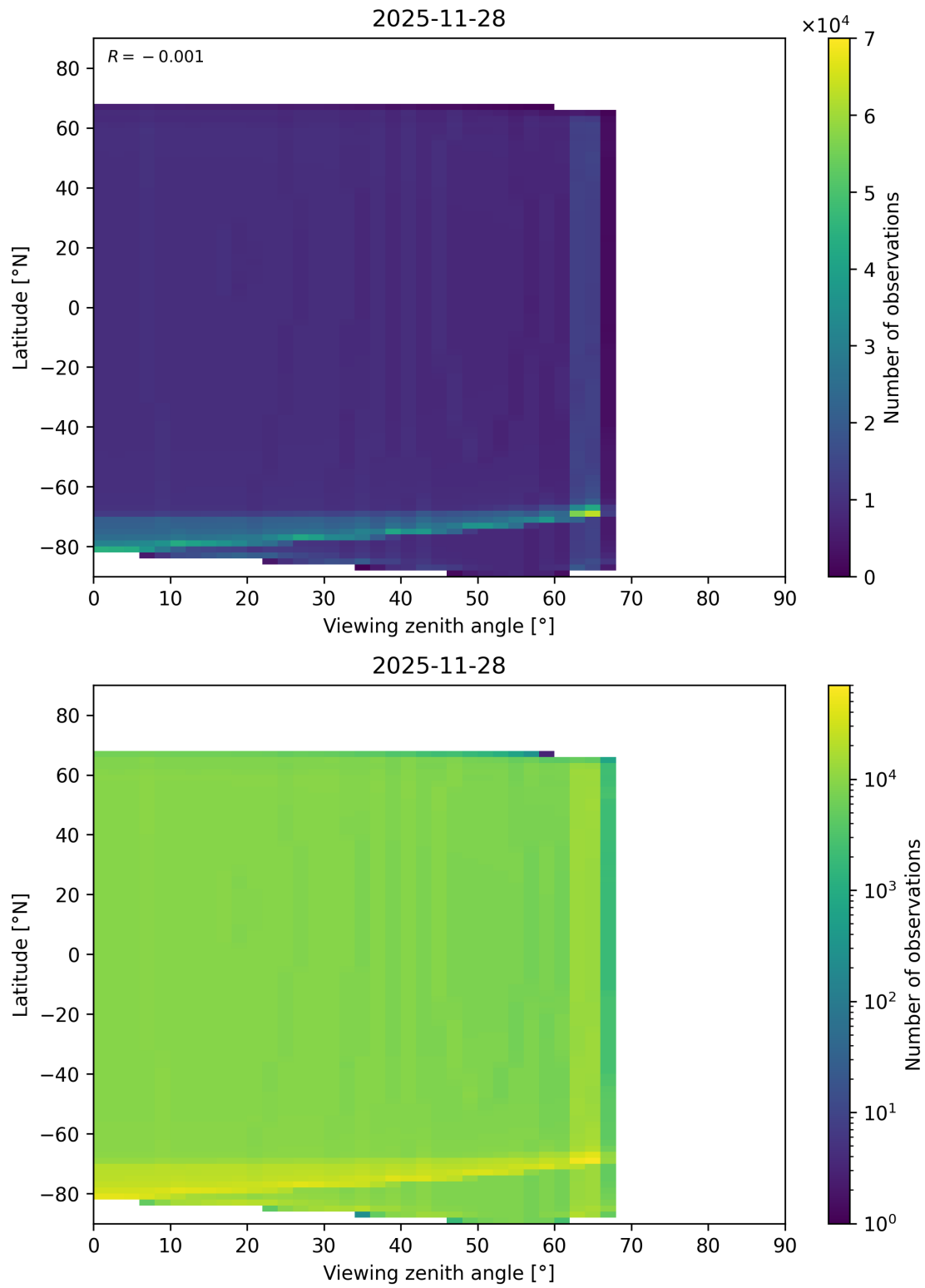
Figure 49: Scatter density plot of “Viewing zenith angle” against “Latitude” for 2025-11-28 to 2025-11-29.
