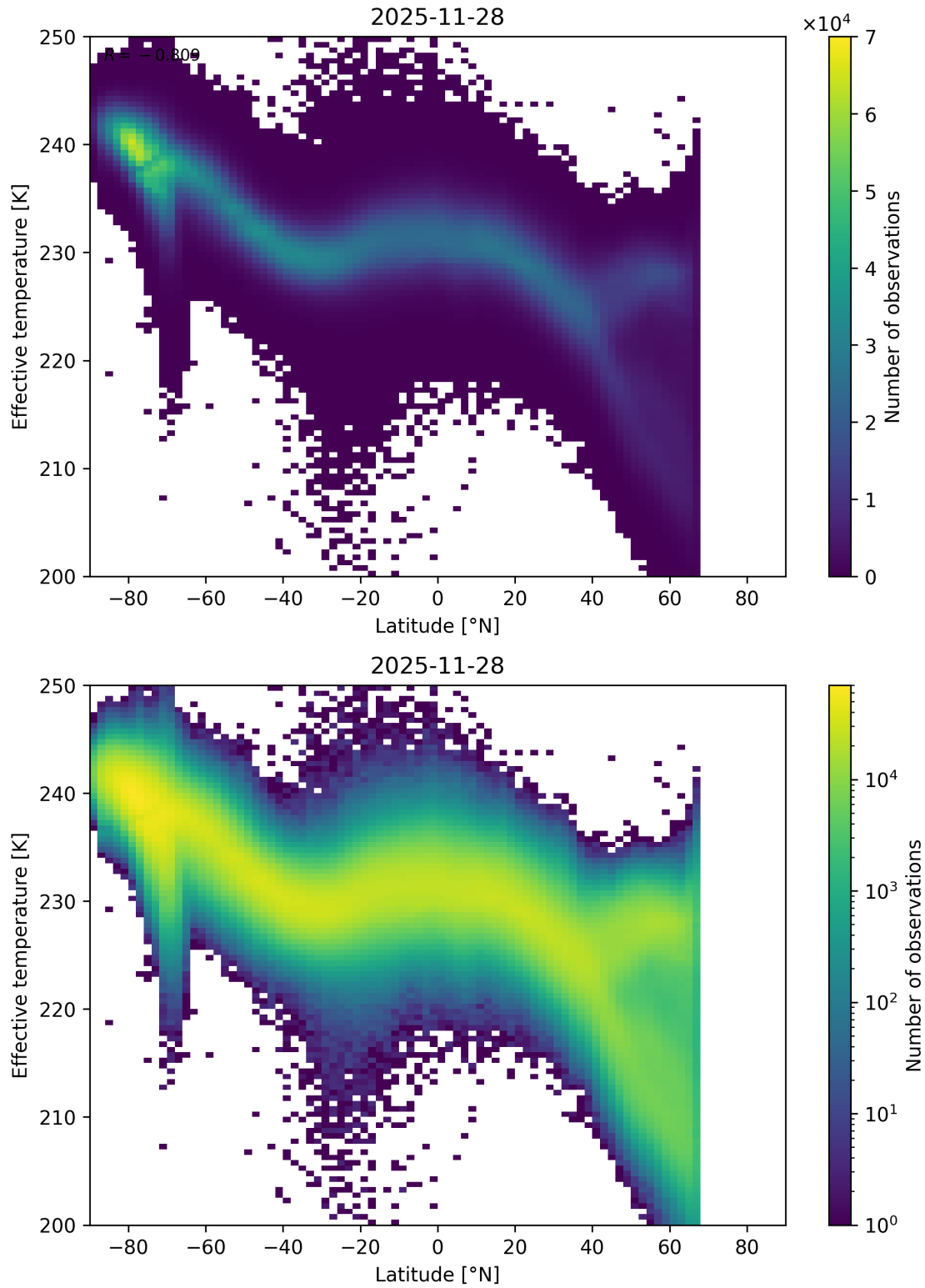
Figure 34: Scatter density plot of “Latitude” against “Effective temperature” for 2025-11-28 to 2025-11-29.
