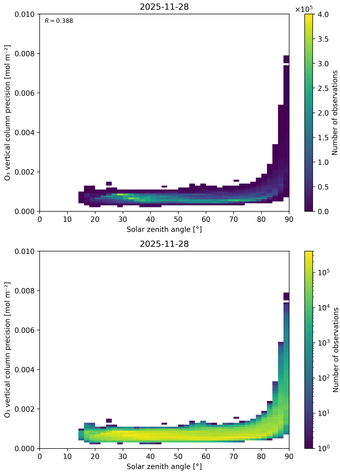
Figure 48: Scatter density plot of “Solar zenith angle” against “O 3 vertical column precision” for 2025-11-28 to 2025-11-29.
