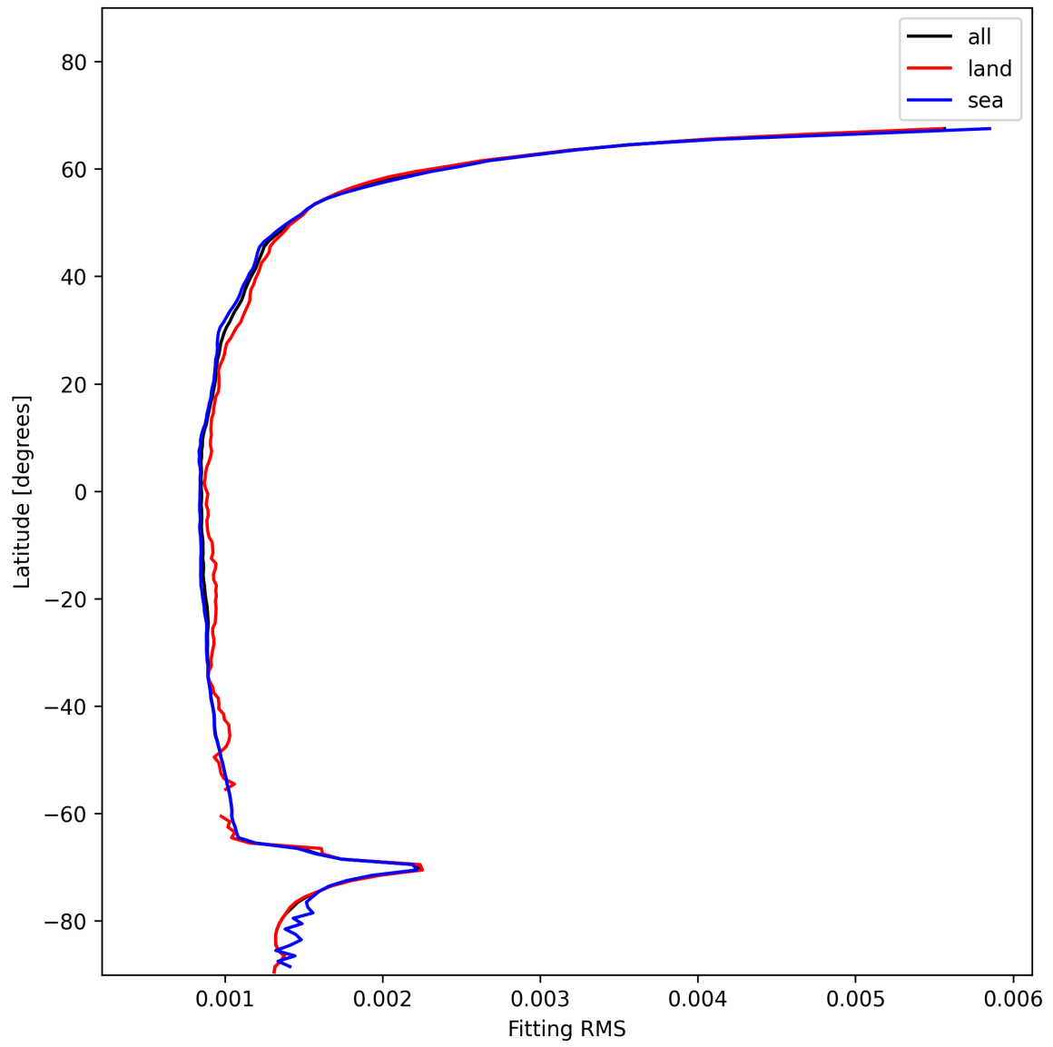
Figure 16: Zonal average of “Fitting RMS” for 2025-11-28 to 2025-11-29.
