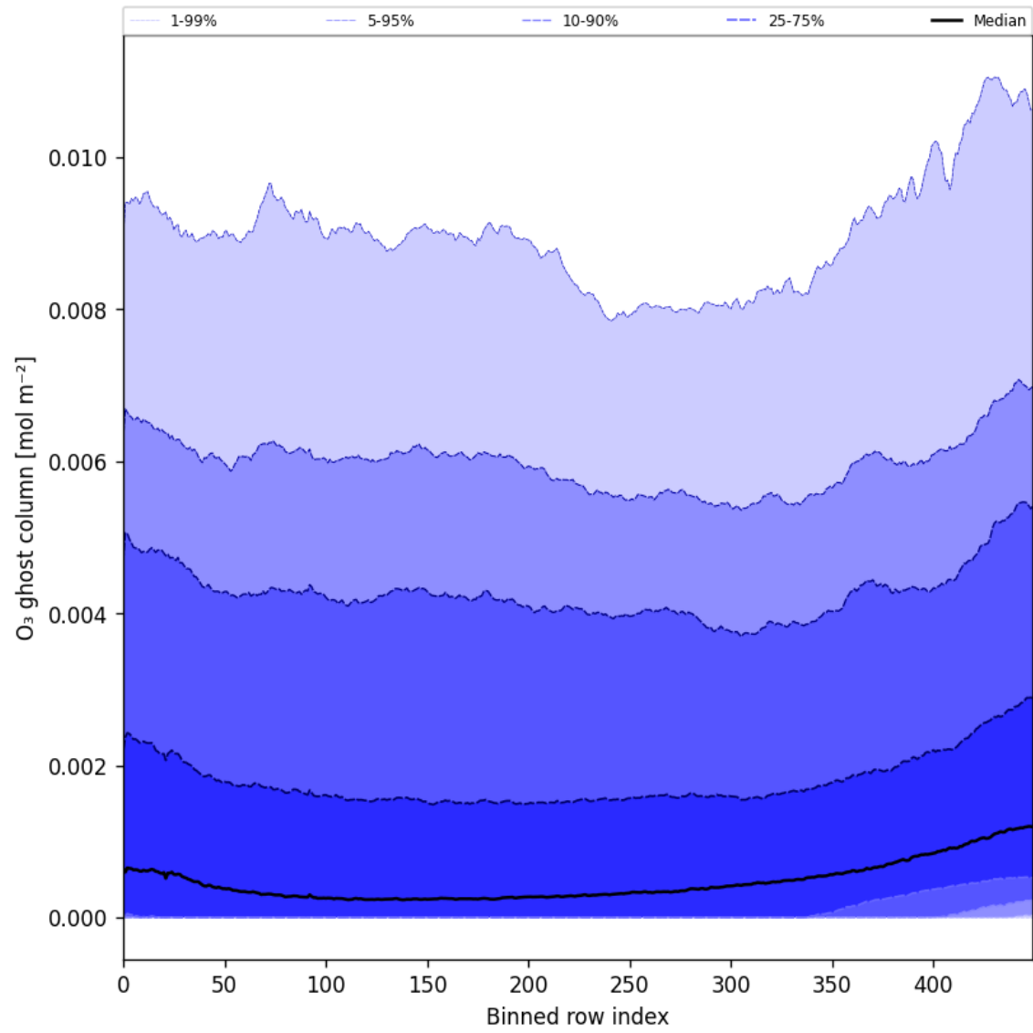
Figure 32: Along track statistics of “O 3 ghost column” for 2025-11-28 to 2025-11-29
