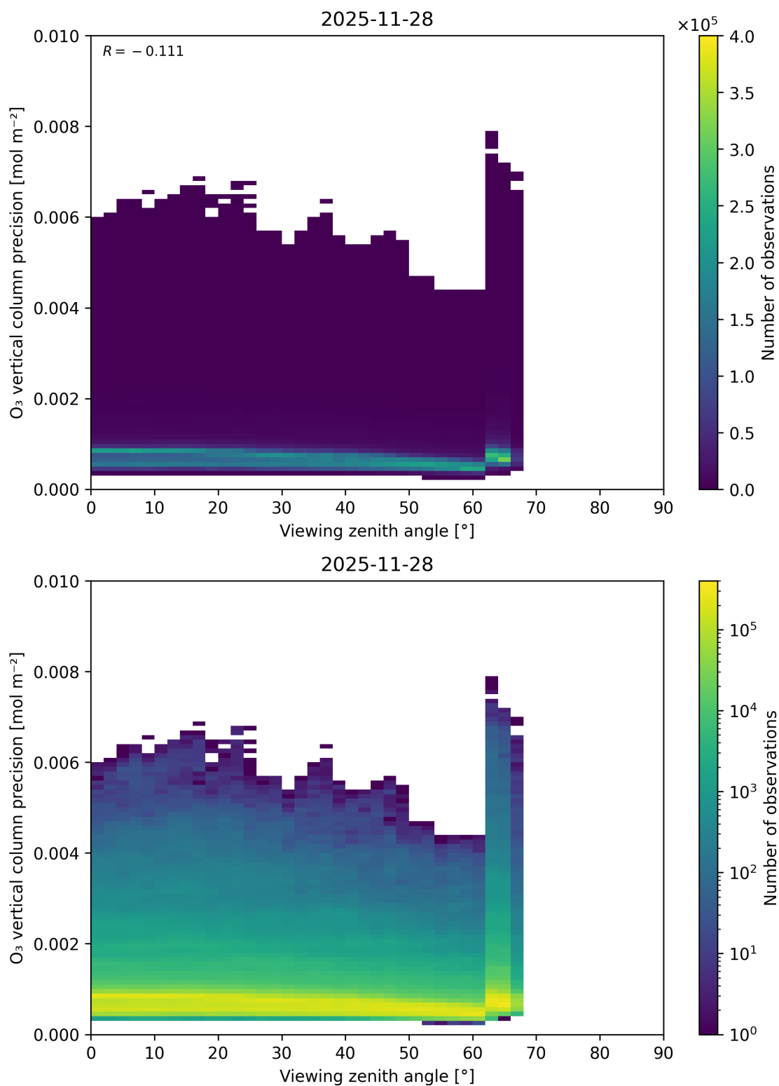
Figure 53: Scatter density plot of “Viewing zenith angle” against “O 3 vertical column precision” for 2025-11-28 to 2025-11-29.
