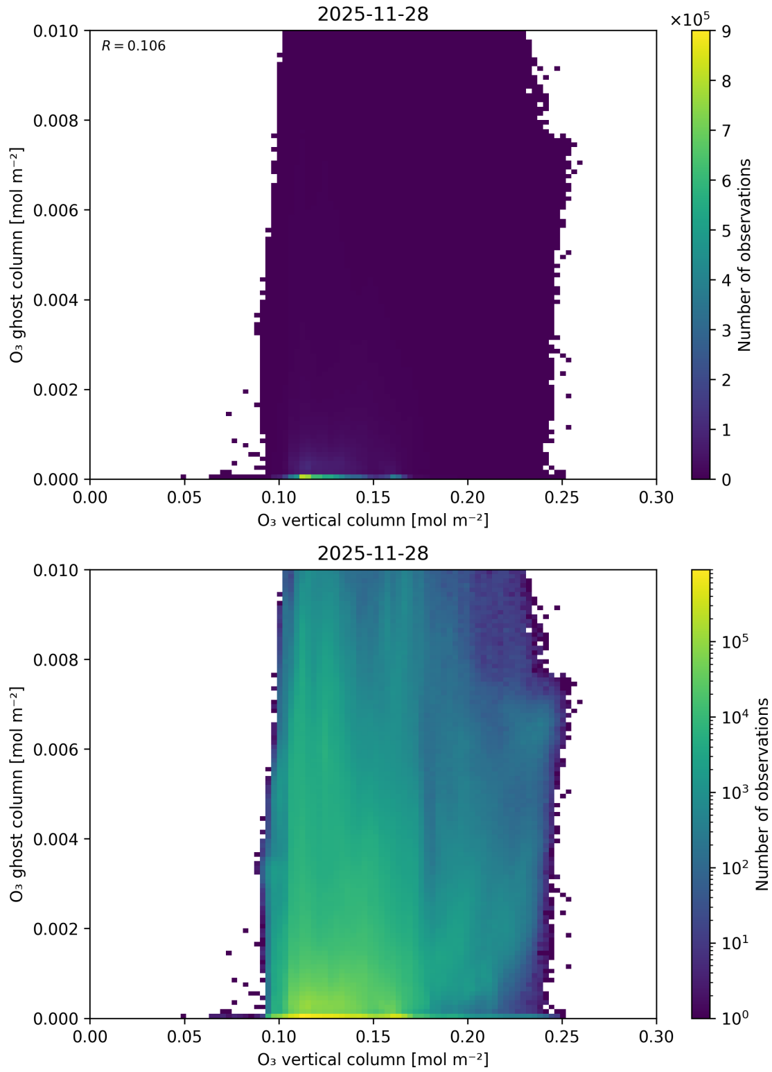
Figure 40: Scatter density plot of “O 3 vertical column” against “O 3 ghost column” for 2025-11-28 to 2025-11-29.
