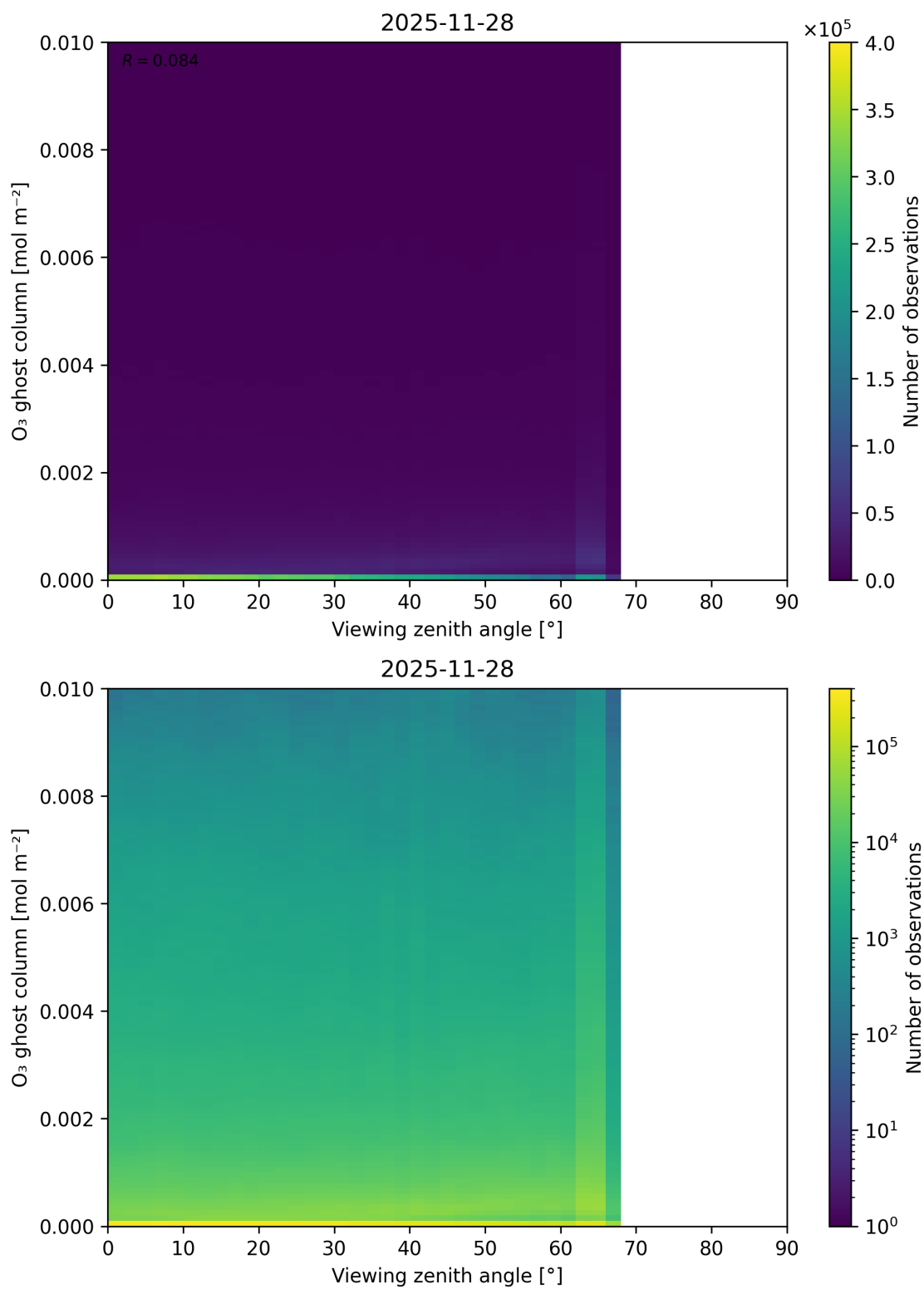
Figure 51: Scatter density plot of “Viewing zenith angle” against “O 3 ghost column” for 2025-11-28 to 2025-11-29.
