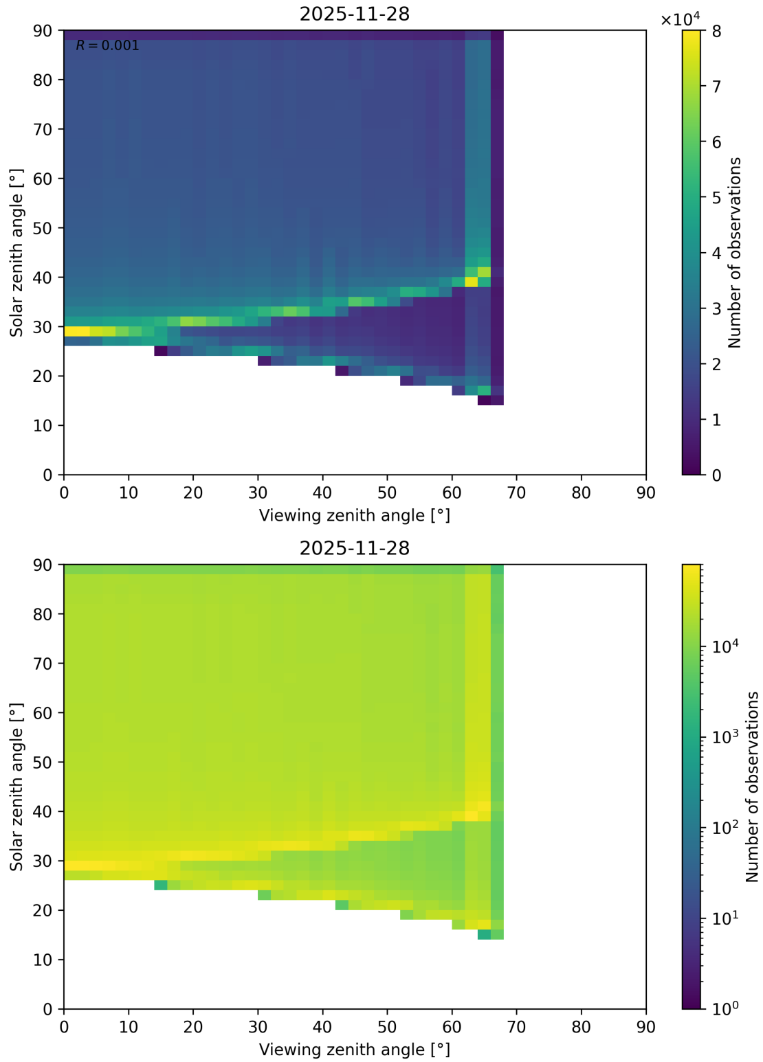
Figure 54: Scatter density plot of “Viewing zenith angle” against “Solar zenith angle” for 2025-11-28 to 2025-11-29.
