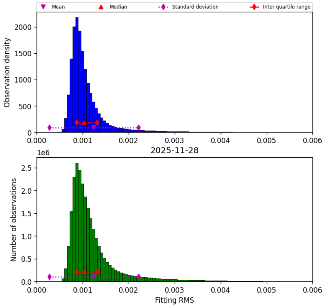
Figure 23: Histogram of “Fitting RMS” for 2025-11-28 to 2025-11-29
