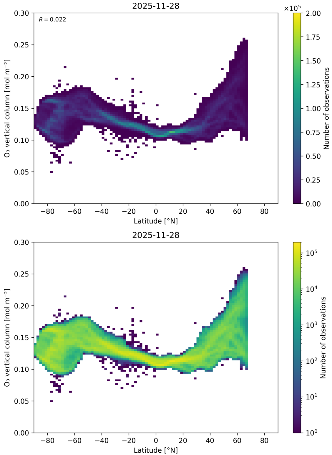
Figure 36: Scatter density plot of “Latitude” against “O 3 vertical column” for 2025-11-28 to 2025-11-29.
