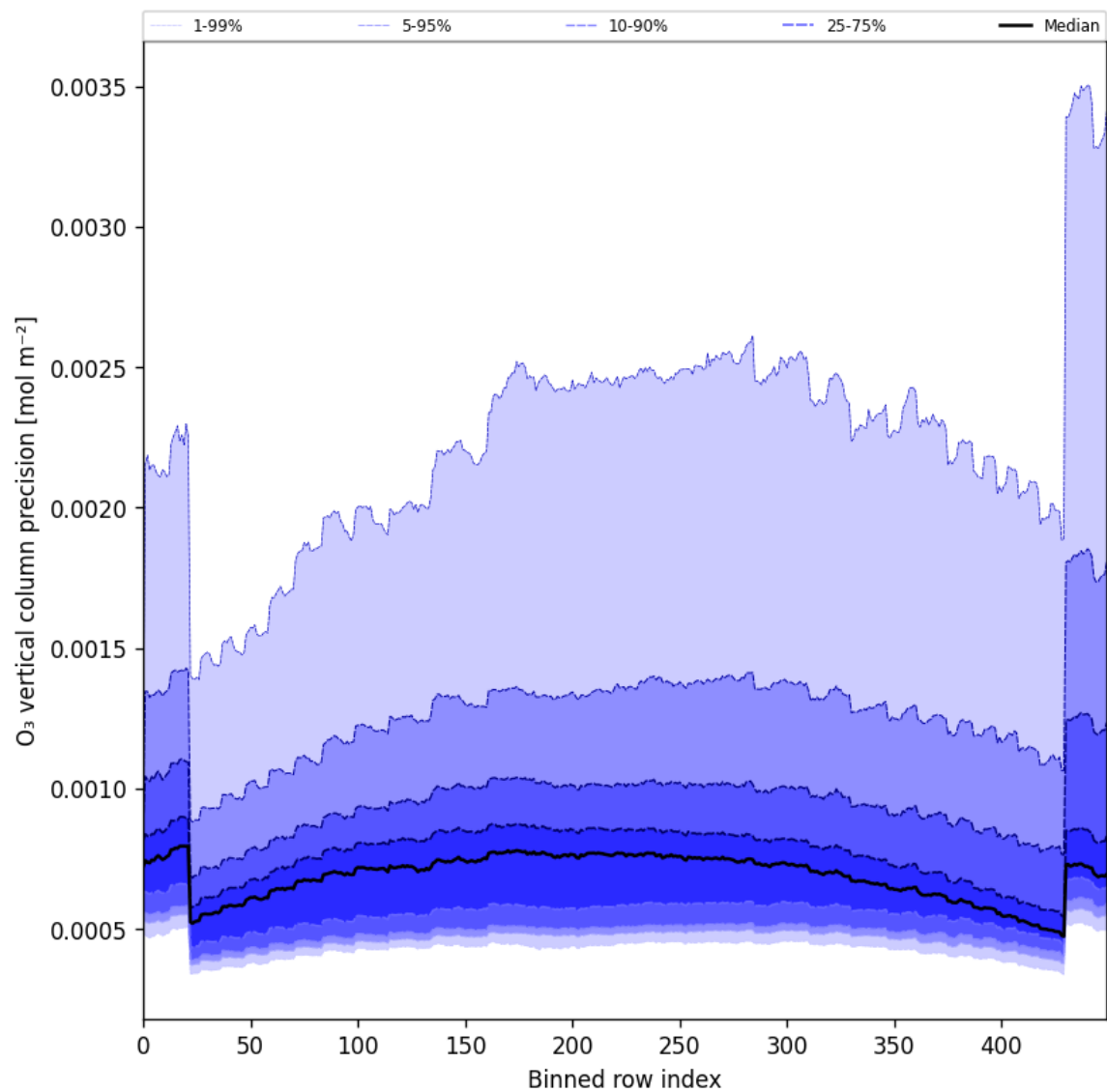
Figure 29: Along track statistics of “O 3 vertical column precision” for 2025-11-28 to 2025-11-29
