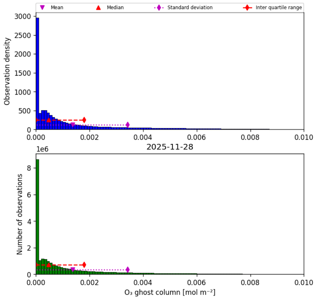
Figure 25: Histogram of "O 3 ghost column" for 2025-11-28 to 2025-11-29
