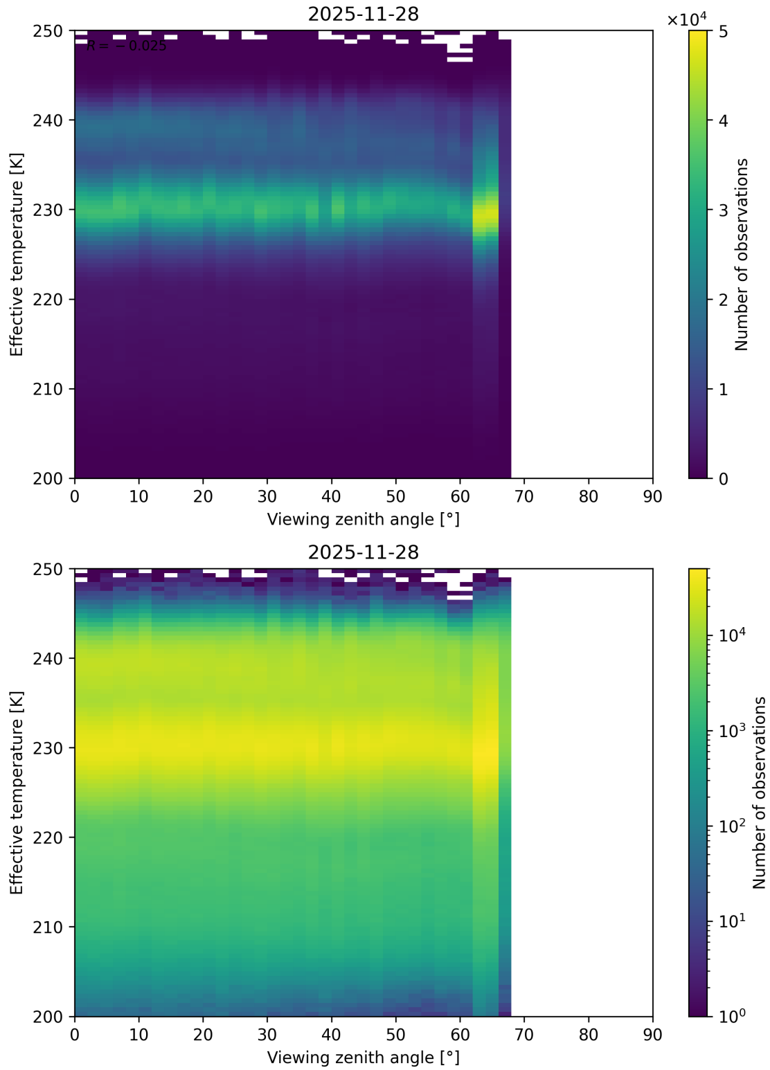
Figure 50: Scatter density plot of “Viewing zenith angle” against “Effective temperature” for 2025-11-28 to 2025-11-29.
