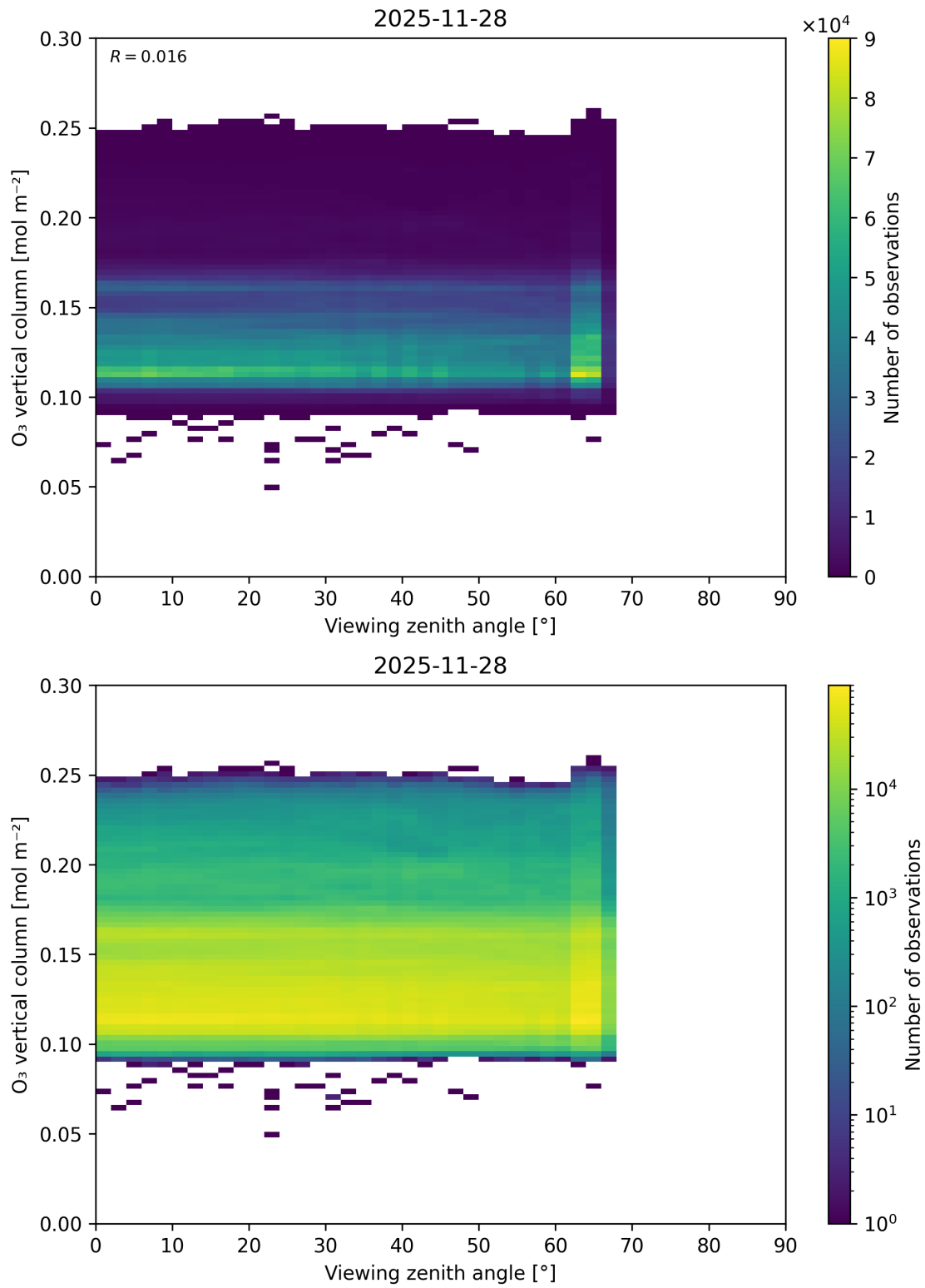
Figure 52: Scatter density plot of “Viewing zenith angle” against “O 3 vertical column” for 2025-11-28 to 2025-11-29.
