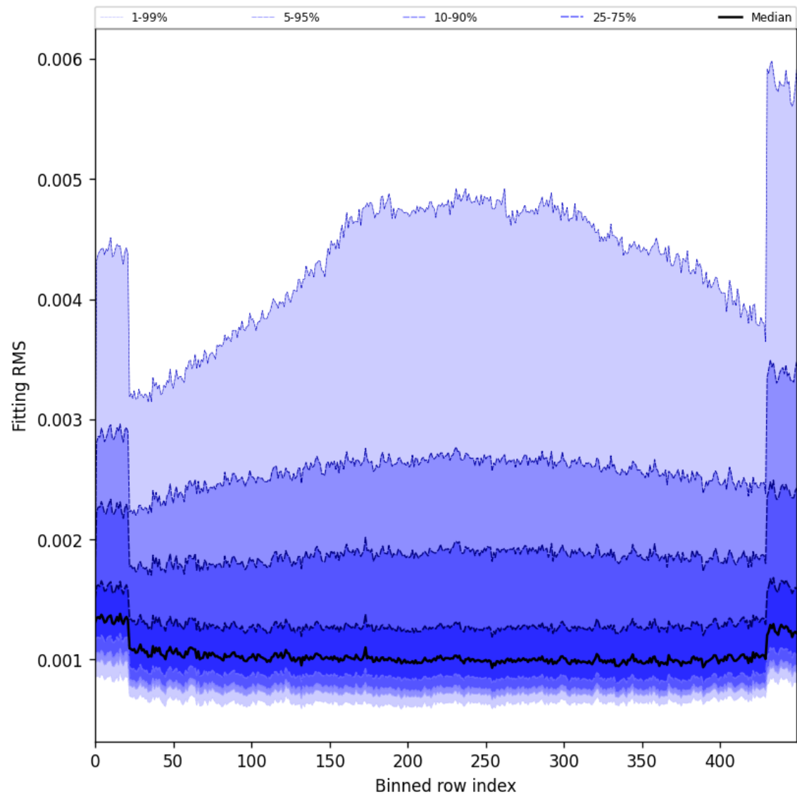
Figure 30: Along track statistics of “Fitting RMS” for 2025-11-28 to 2025-11-29
