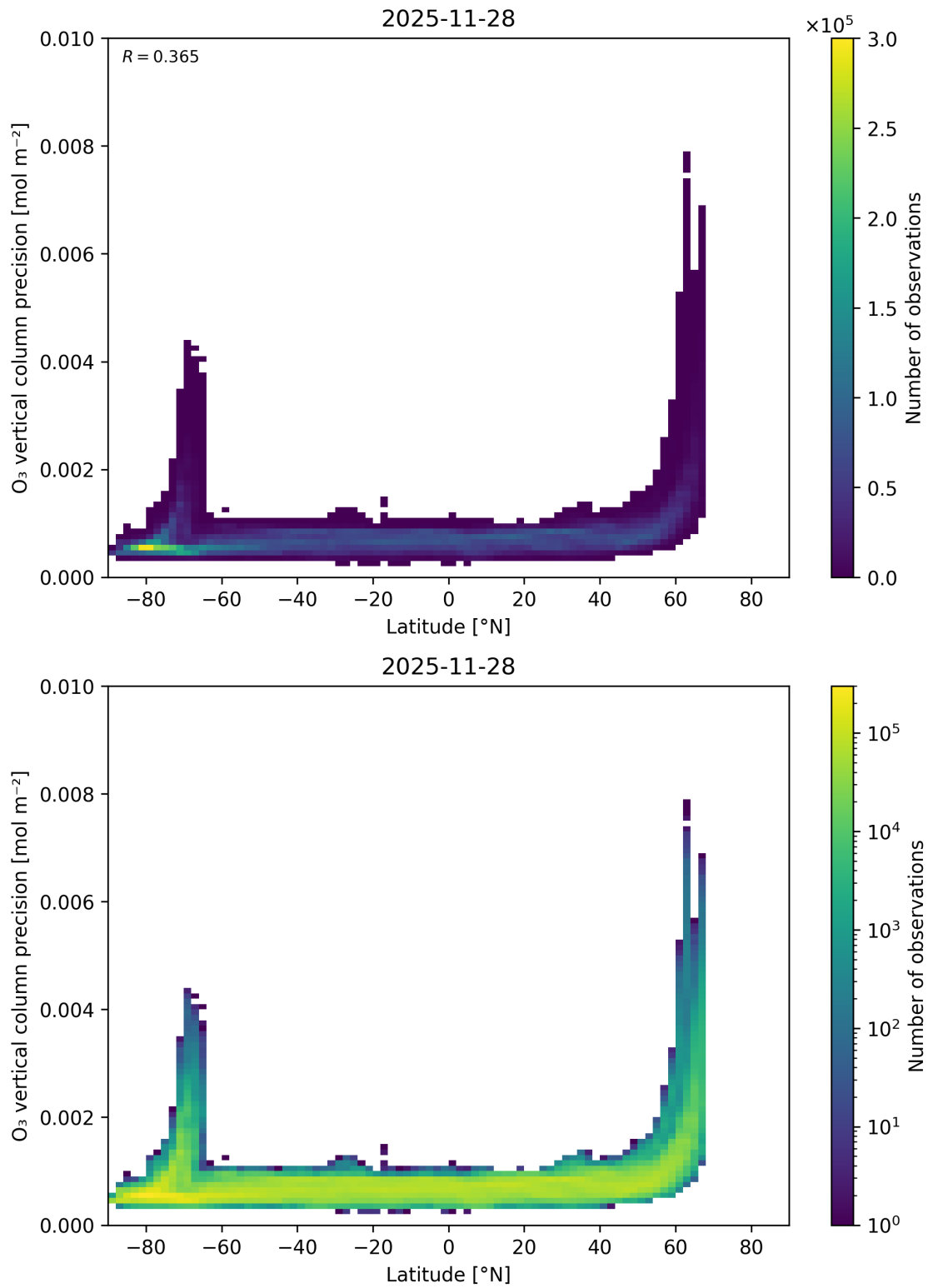
Figure 37: Scatter density plot of “Latitude” against “O 3 vertical column precision” for 2025-11-28 to 2025-11-29.
