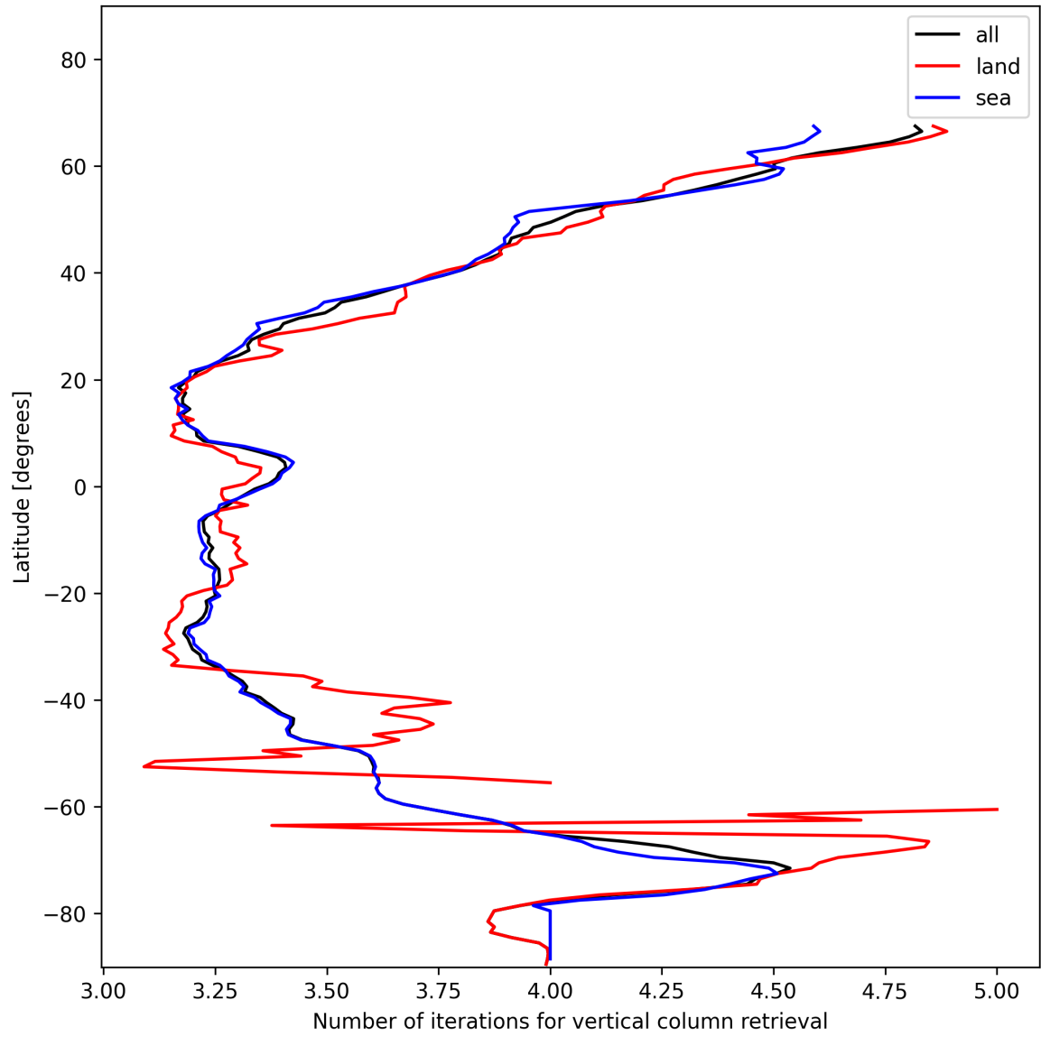
Figure 19: Zonal average of “Number of iterations for vertical column retrieval” for 2025-11-28 to 2025-11-29.
