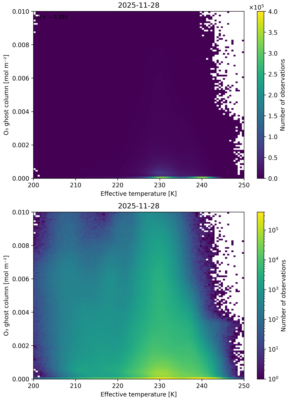
Figure 38: Scatter density plot of “Effective temperature” against “O 3 ghost column” for 2025-11-28 to 2025-11-29.
