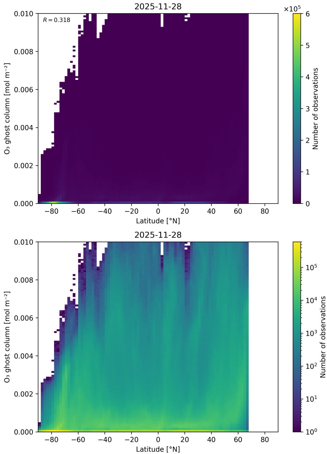
Figure 35: Scatter density plot of “Latitude” against “O 3 ghost column” for 2025-11-28 to 2025-11-29.
