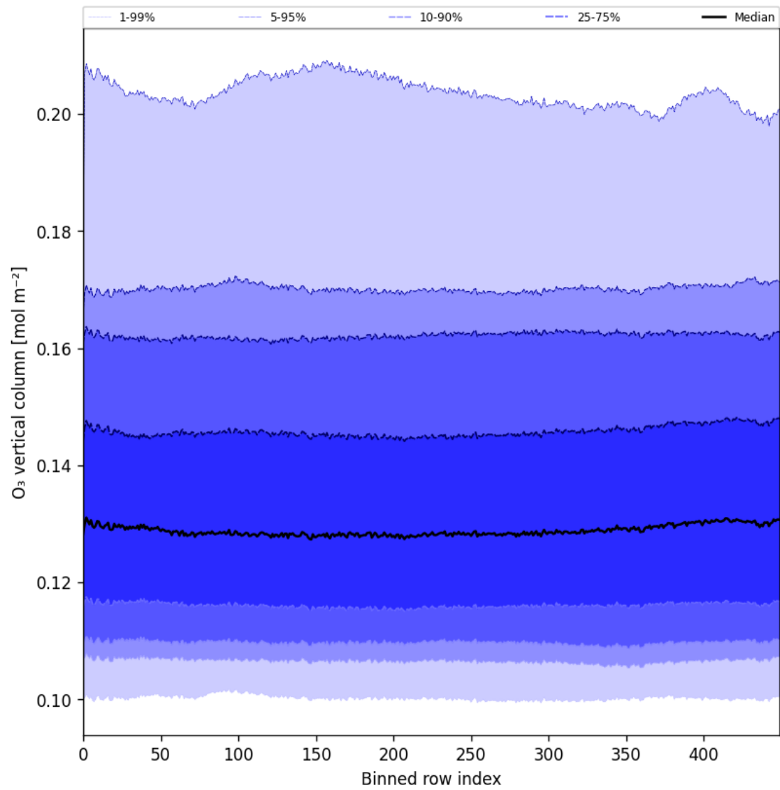
Figure 28: Along track statistics of “O 3 vertical column” for 2025-11-28 to 2025-11-29
