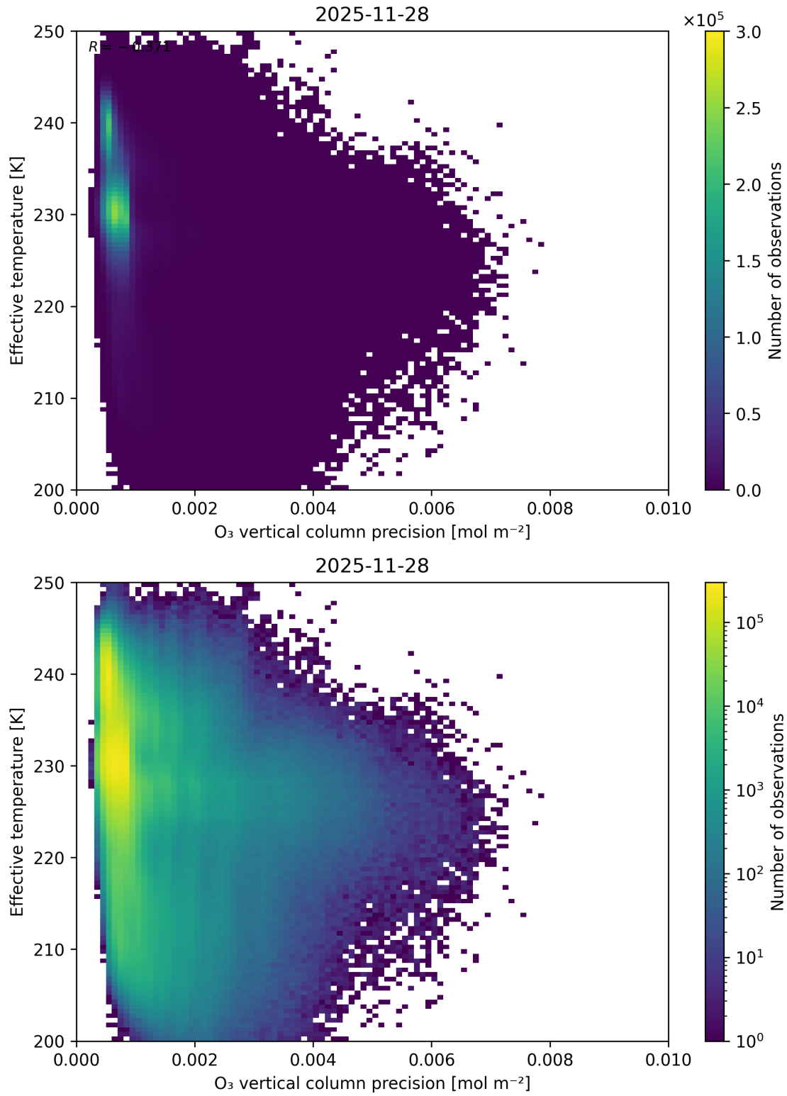
Figure 42: Scatter density plot of “O 3 vertical column precision” against “Effective temperature” for 2025-11-28 to 2025-11-29.
