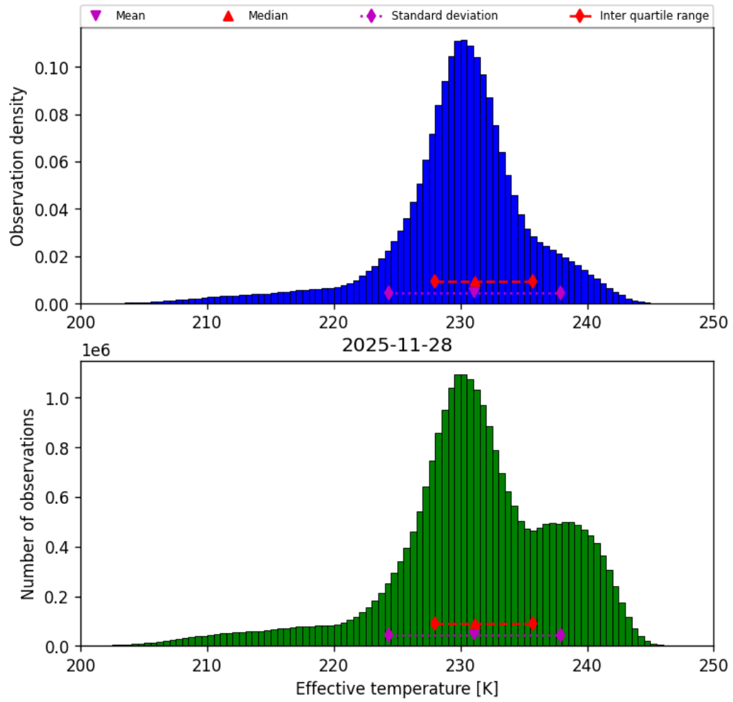
Figure 24: Histogram of “Effective temperature” for 2025-11-28 to 2025-11-29
