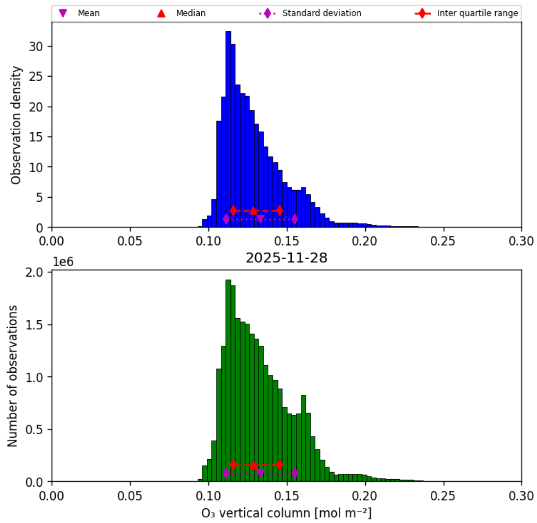
Figure 21: Histogram of “O 3 vertical column” for 2025-11-28 to 2025-11-29
