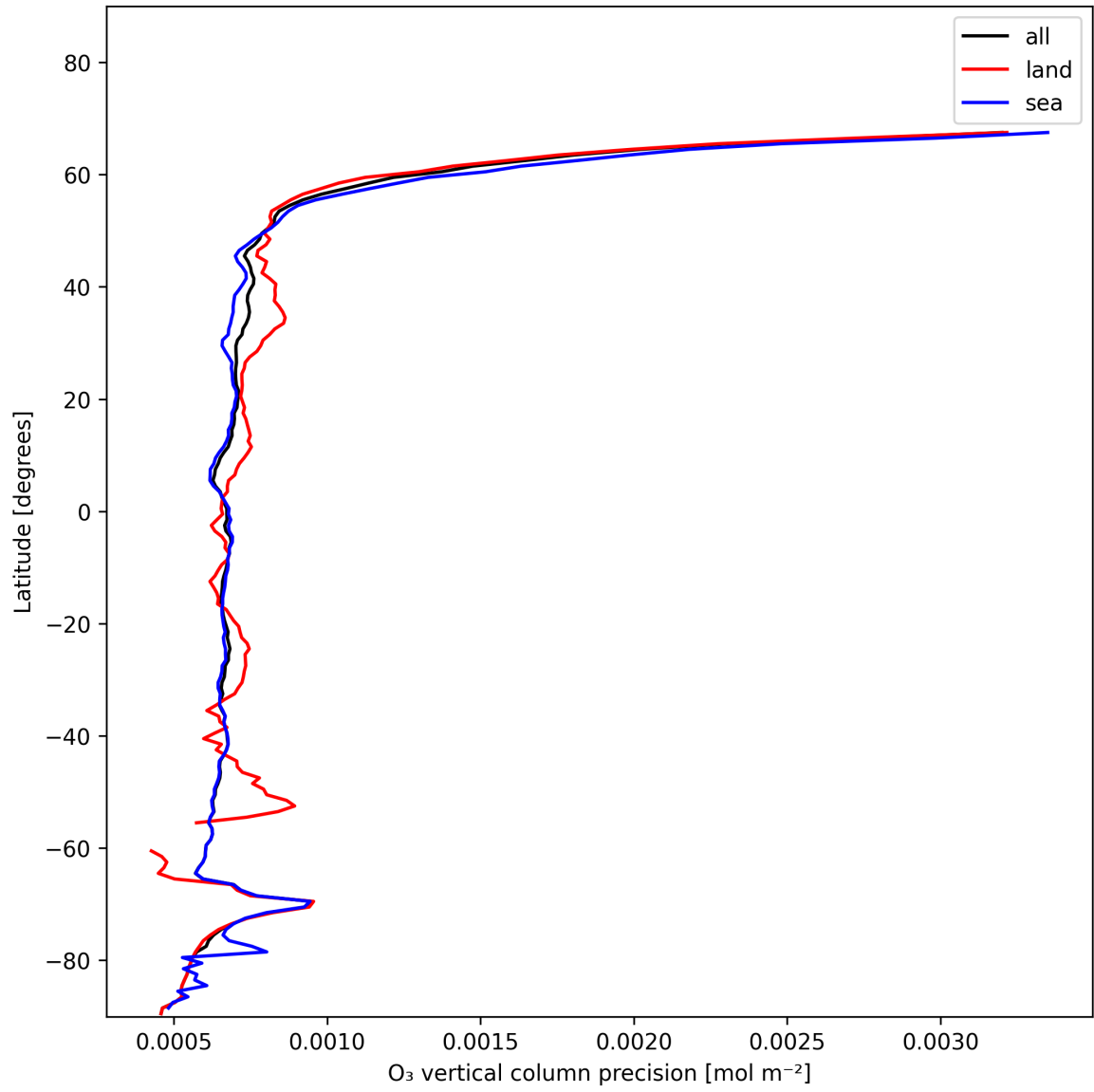
Figure 15: Zonal average of “O 3 vertical column precision” for 2025-11-28 to 2025-11-29.
