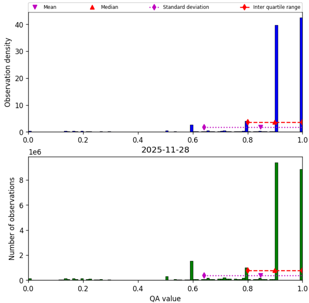
Figure 20: Histogram of “QA value” for 2025-11-28 to 2025-11-29
