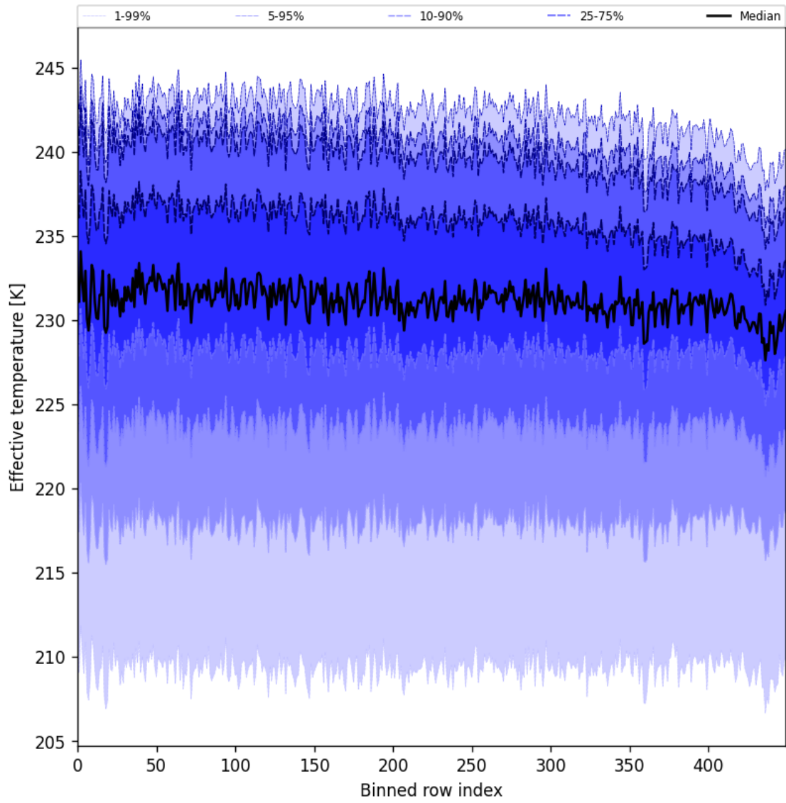
Figure 31: Along track statistics of “Effective temperature” for 2025-11-28 to 2025-11-29
