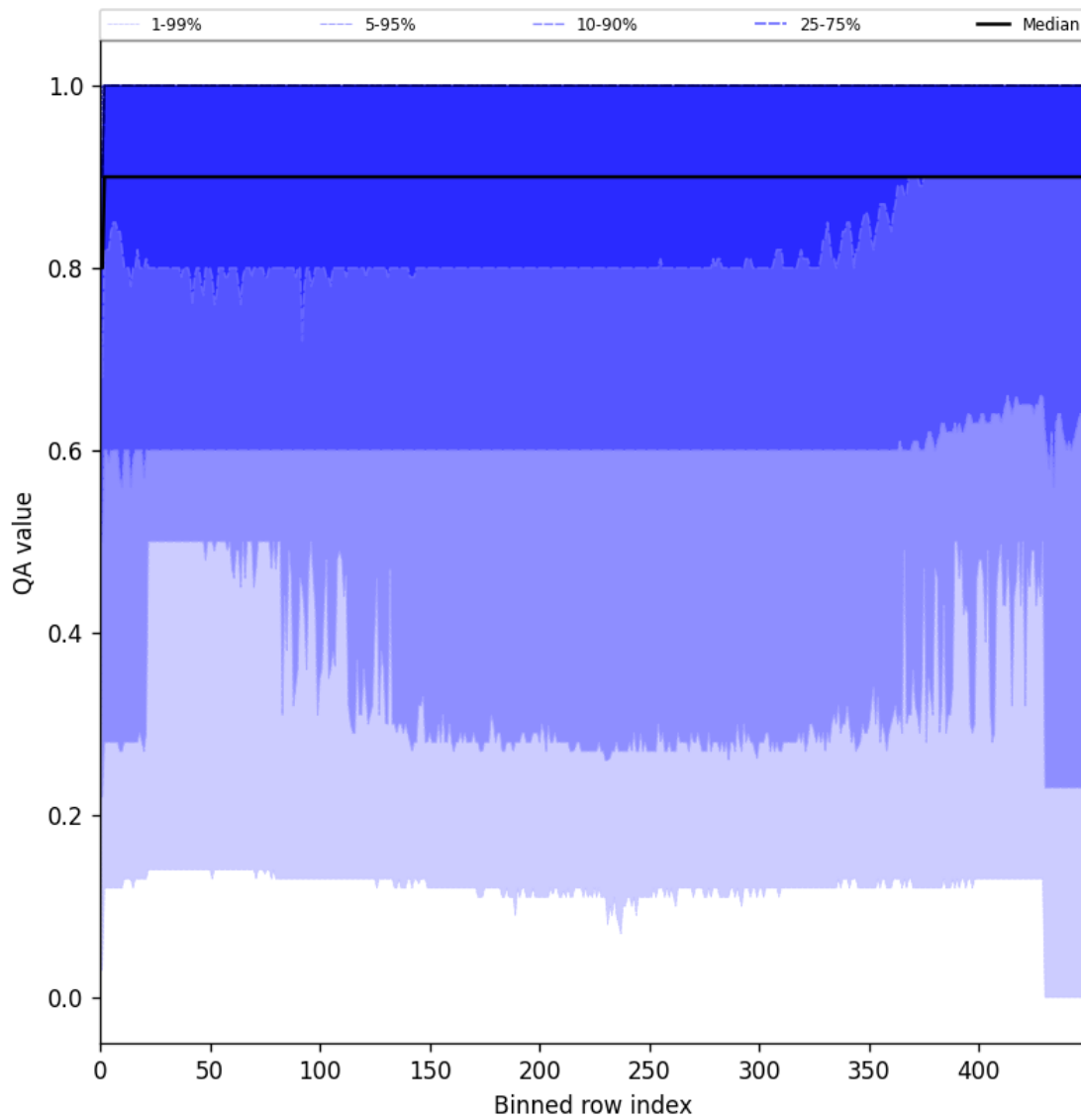
Figure 27: Along track statistics of “QA value” for 2025-11-28 to 2025-11-29
