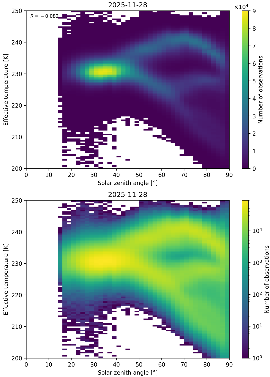
Figure 45: Scatter density plot of “Solar zenith angle” against “Effective temperature” for 2025-11-28 to 2025-11-29.
