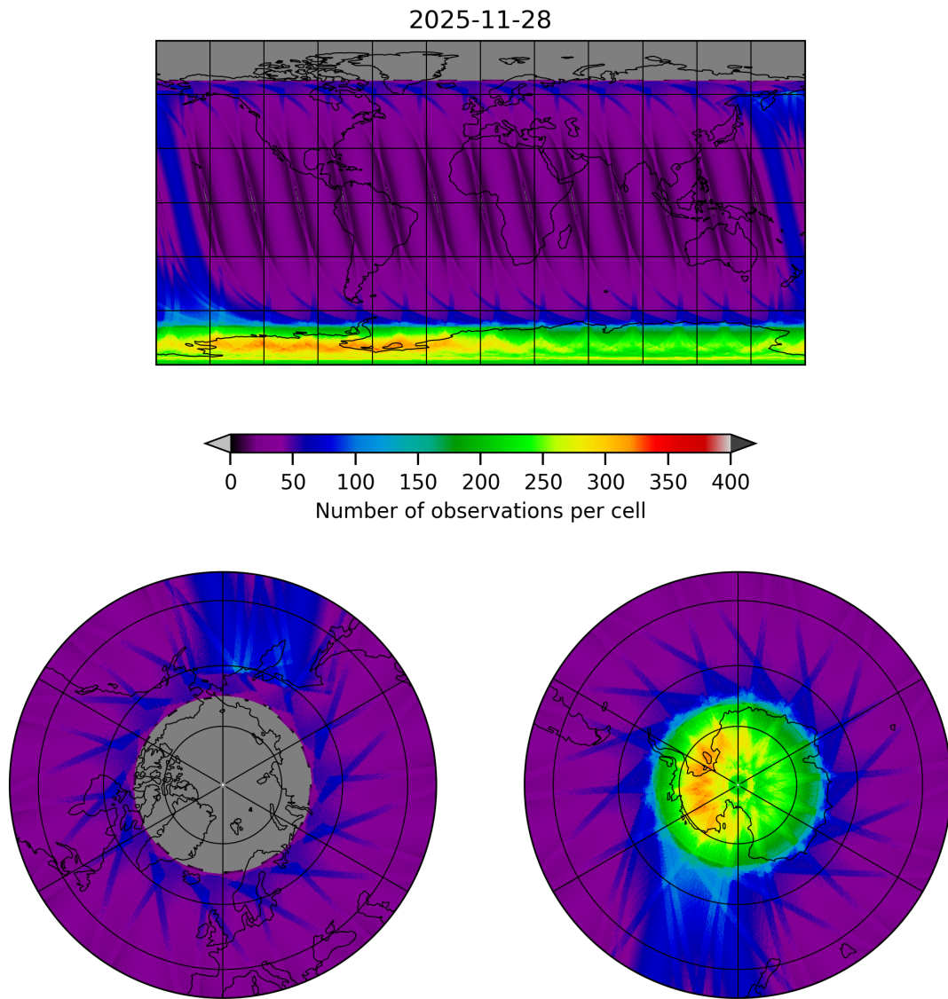
Figure 12: Map of the number of observations for 2025-11-28 to 2025-11-29
