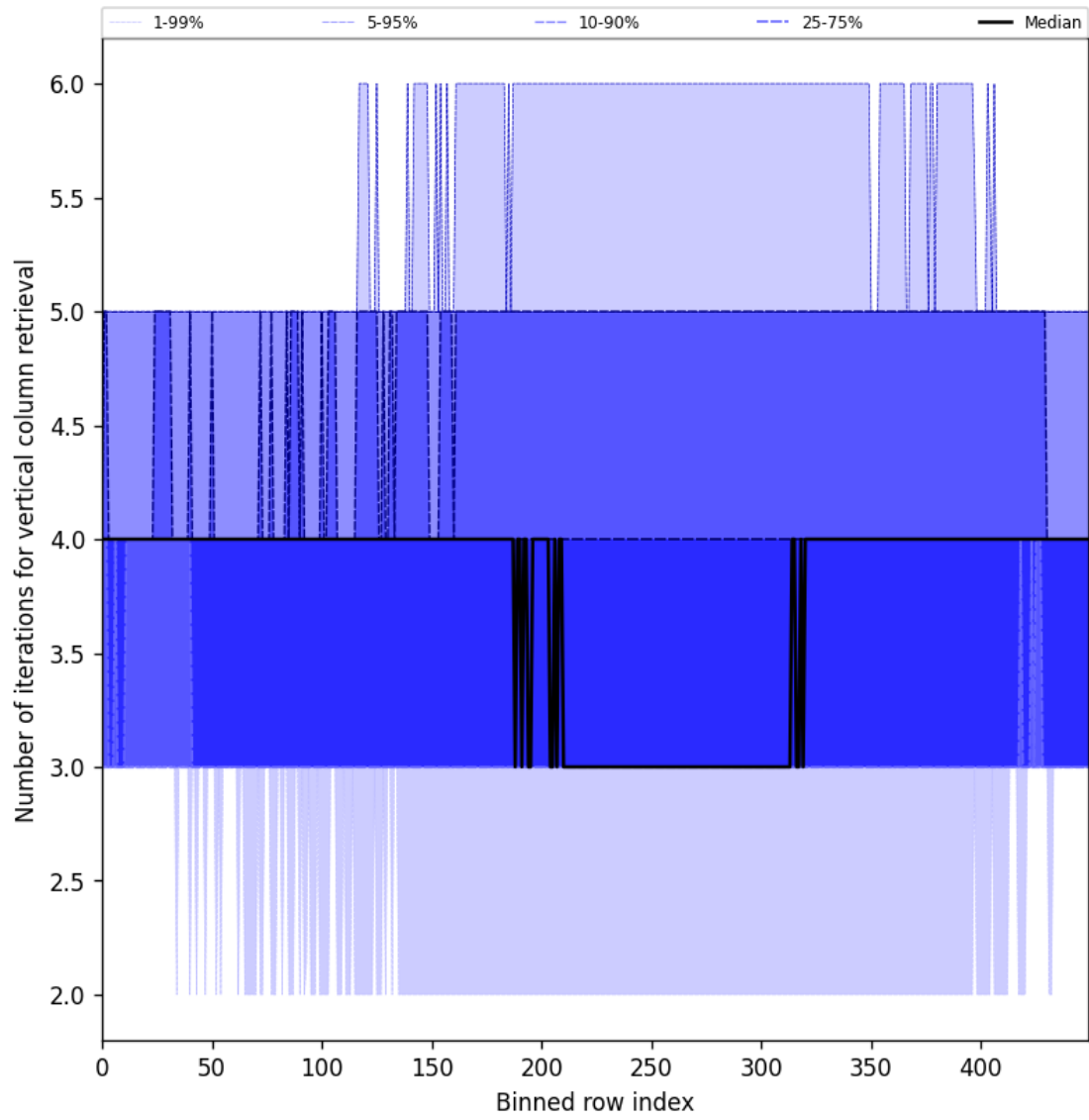
Figure 33: Along track statistics of “Number of iterations for vertical column retrieval” for 2025-11-28 to 2025-11-29
