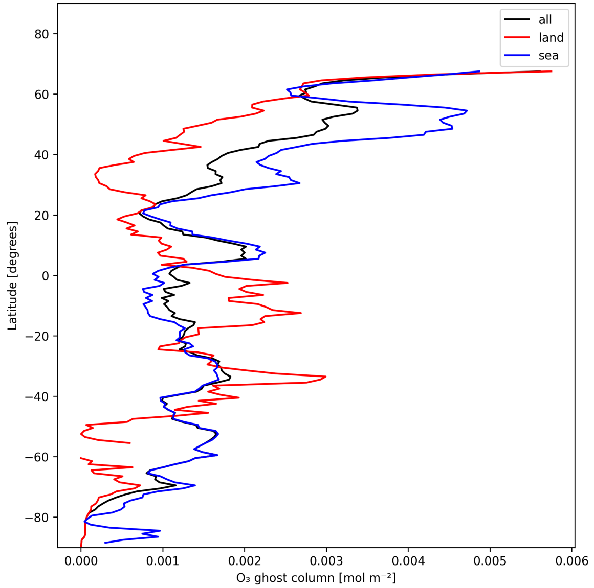
Figure 18: Zonal average of “O 3 ghost column” for 2025-11-28 to 2025-11-29.
