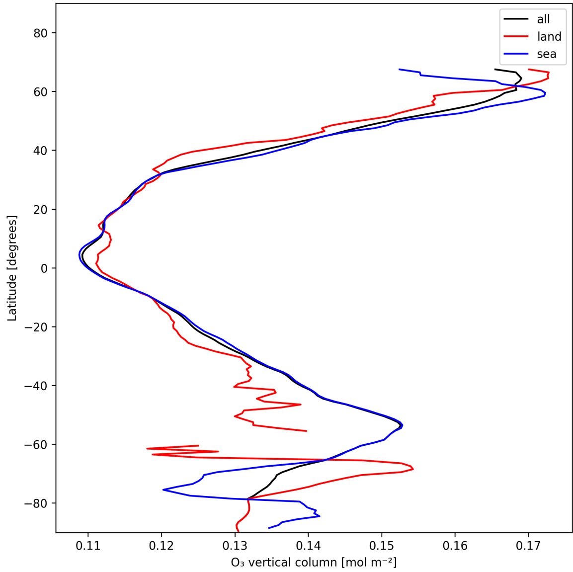
Figure 14: Zonal average of “O 3 vertical column” for 2025-11-28 to 2025-11-29.
