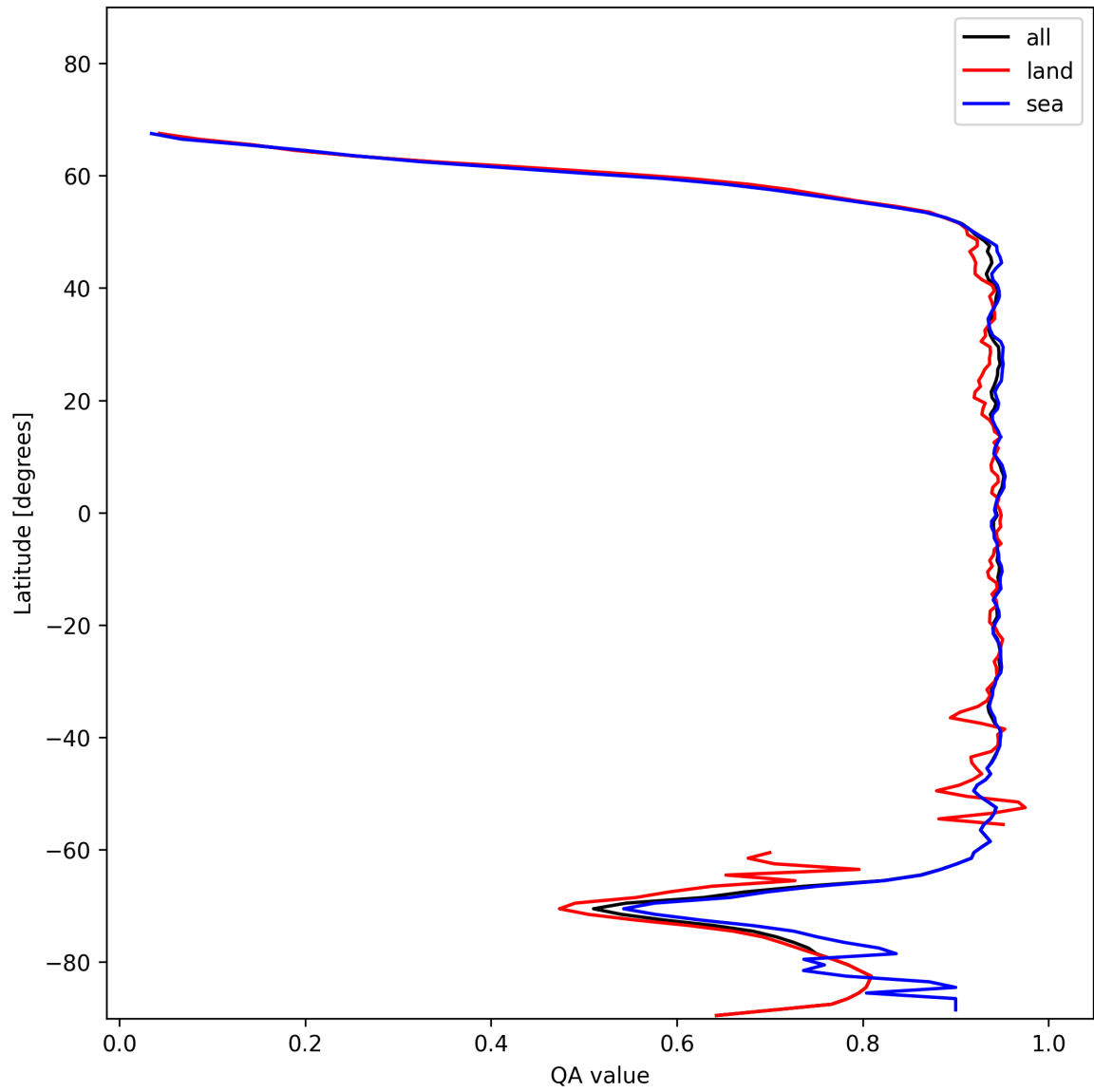
Figure 13: Zonal average of “QA value” for 2025-11-28 to 2025-11-29.
