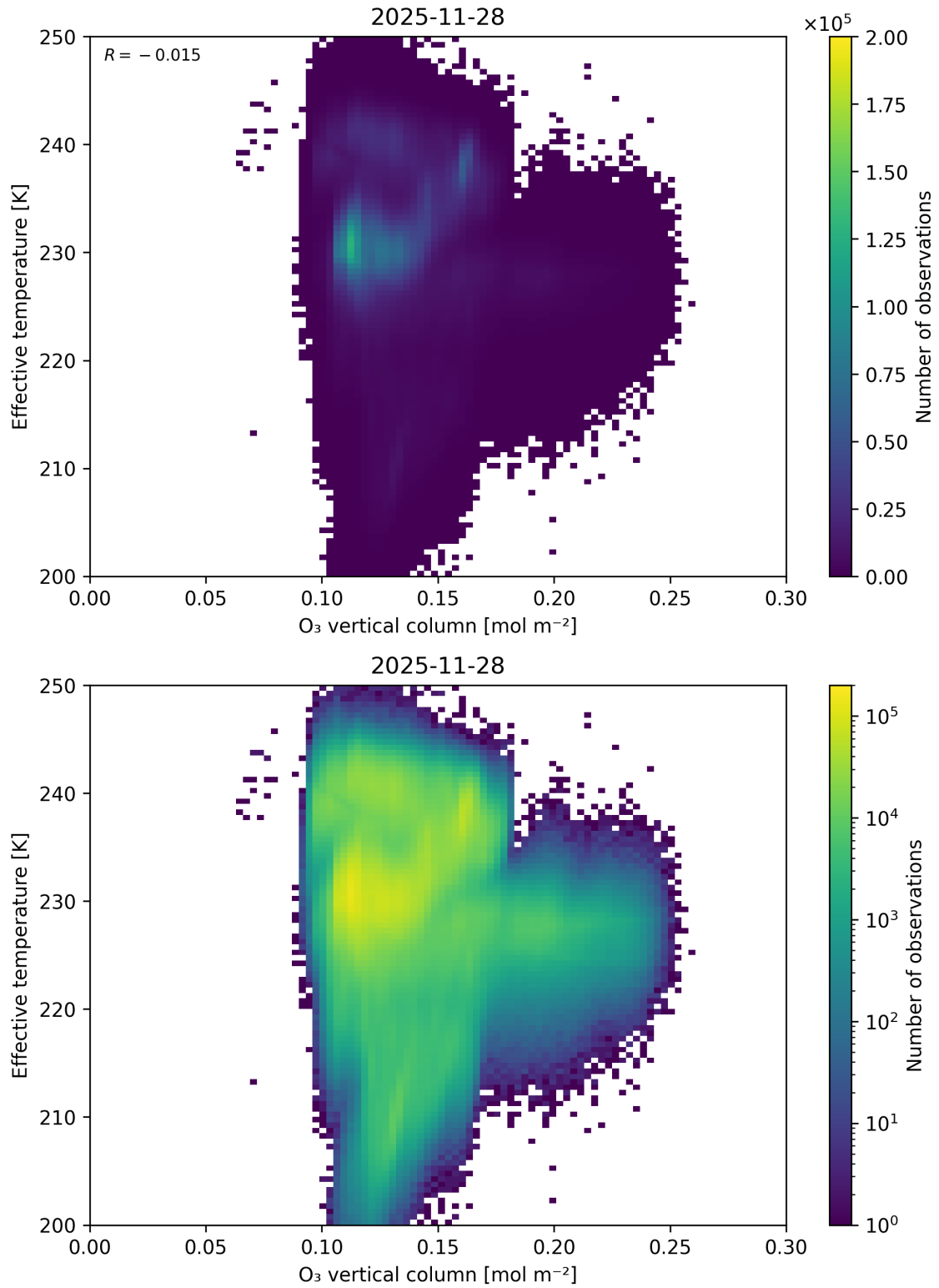
Figure 39: Scatter density plot of “O 3 vertical column” against “Effective temperature” for 2025-11-28 to 2025-11-29.
