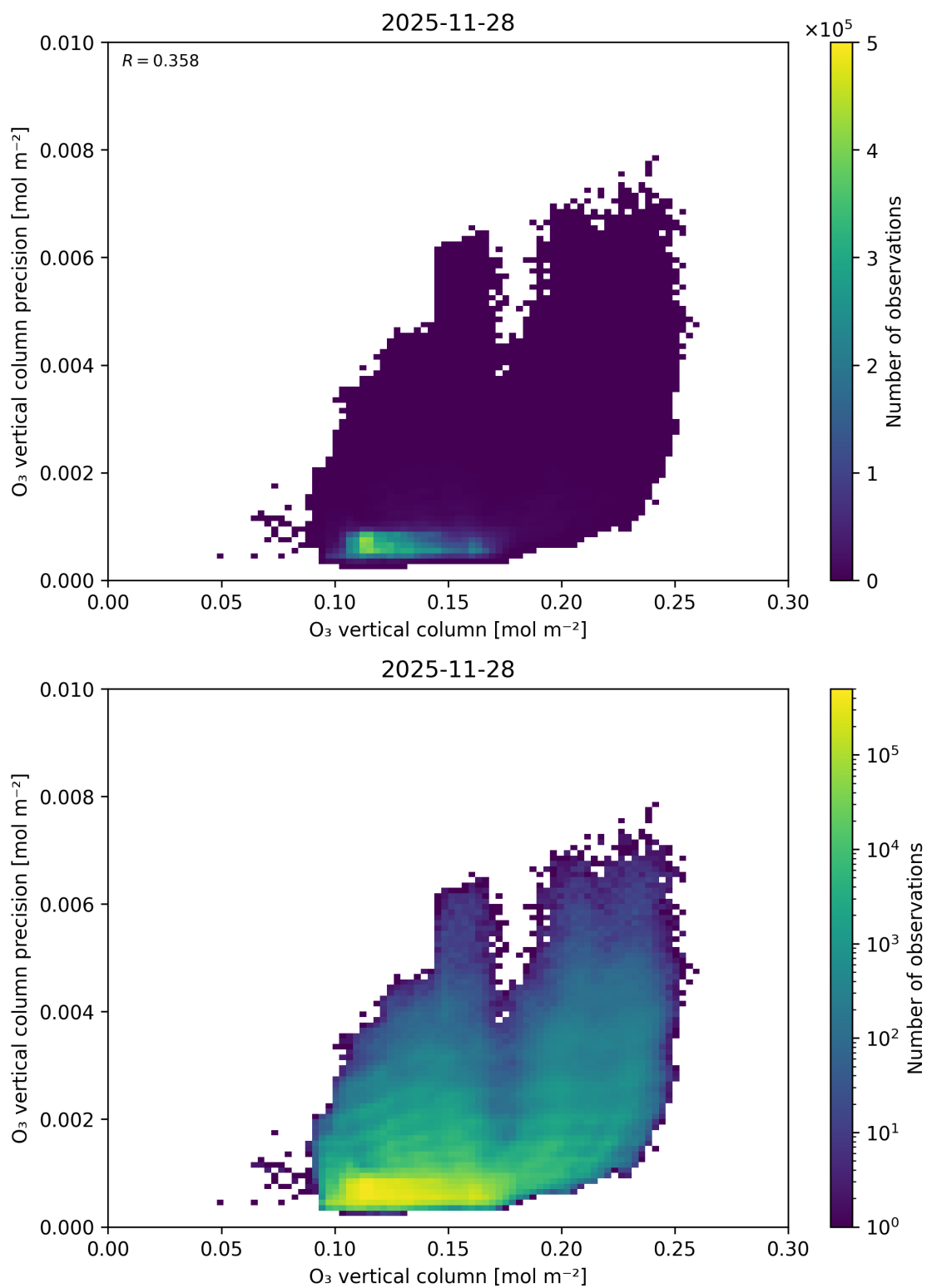
Figure 41: Scatter density plot of “O 3 vertical column” against “O 3 vertical column precision” for 2025-11-28 to 2025-11-29.
