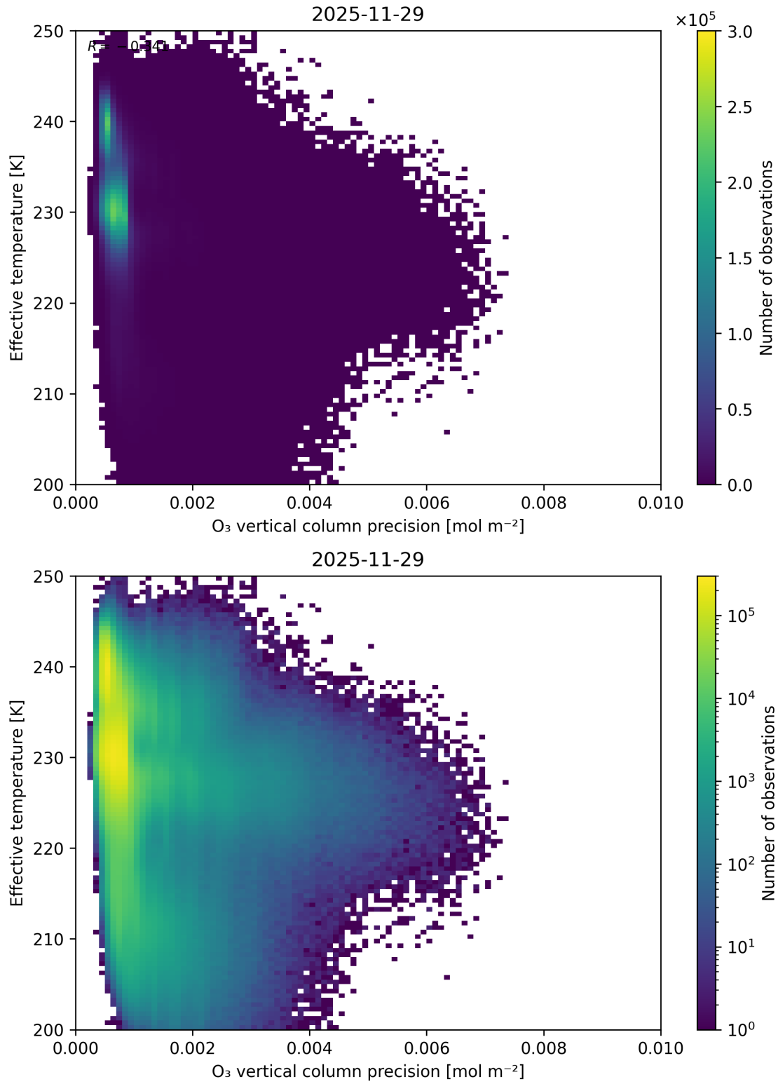
Figure 42: Scatter density plot of “O 3 vertical column precision” against “Effective temperature” for 2025-11-28 to 2025-11-30.
