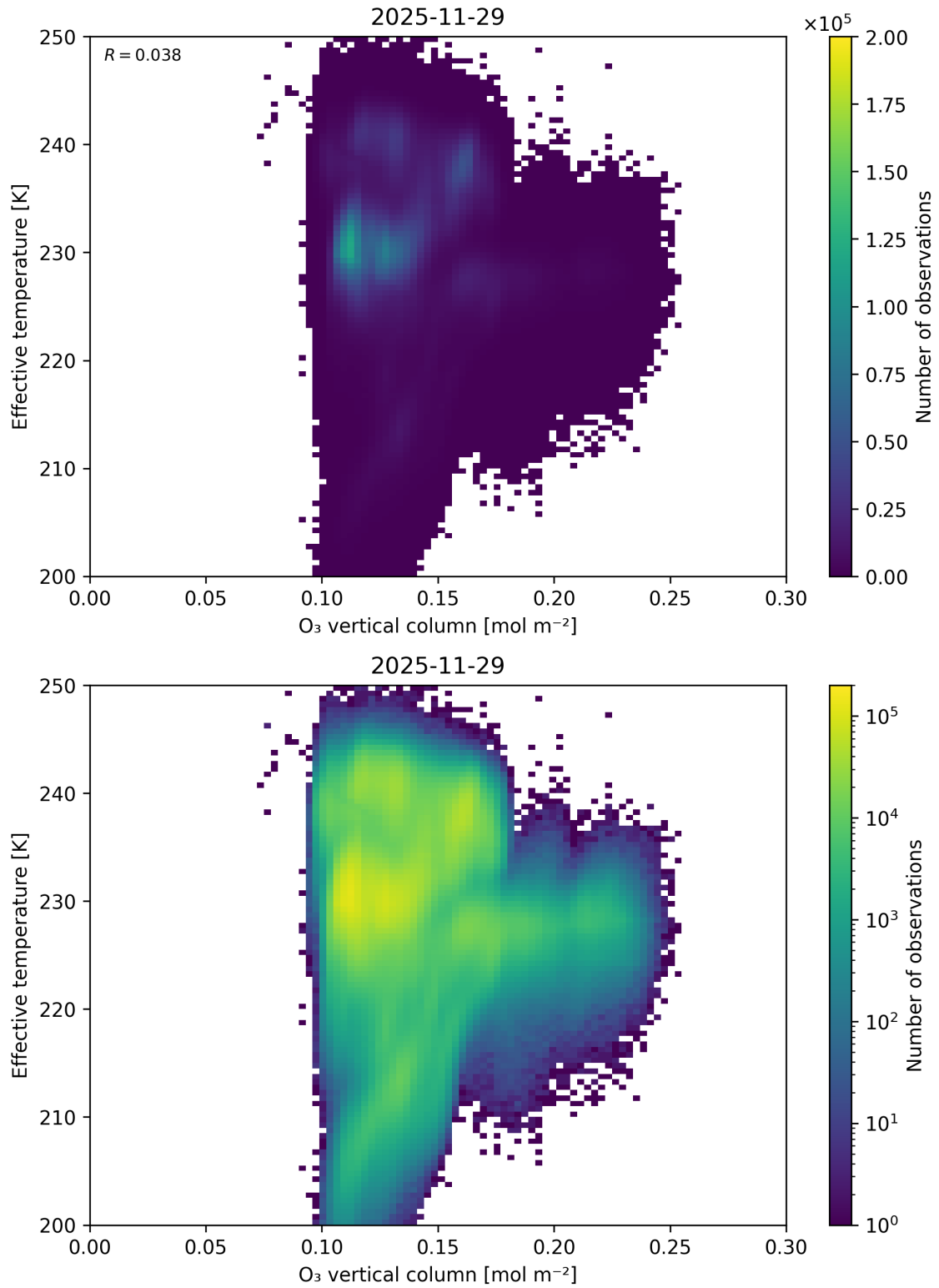
Figure 39: Scatter density plot of “O 3 vertical column” against “Effective temperature” for 2025-11-28 to 2025-11-30.
