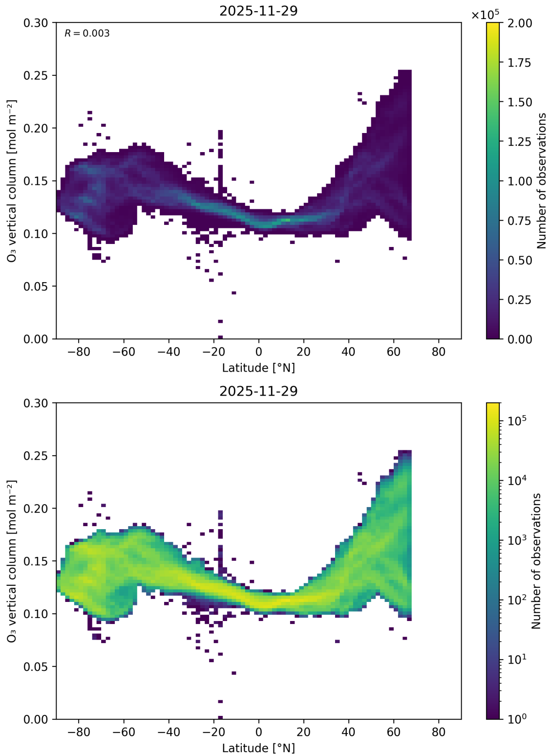
Figure 36: Scatter density plot of “Latitude” against “O 3 vertical column” for 2025-11-28 to 2025-11-30.
