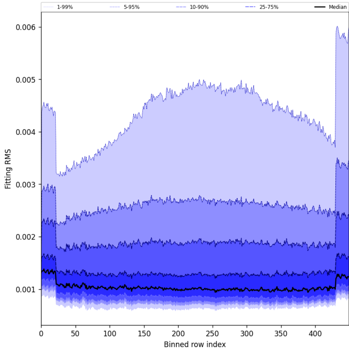
Figure 30: Along track statistics of “Fitting RMS” for 2025-11-28 to 2025-11-30
