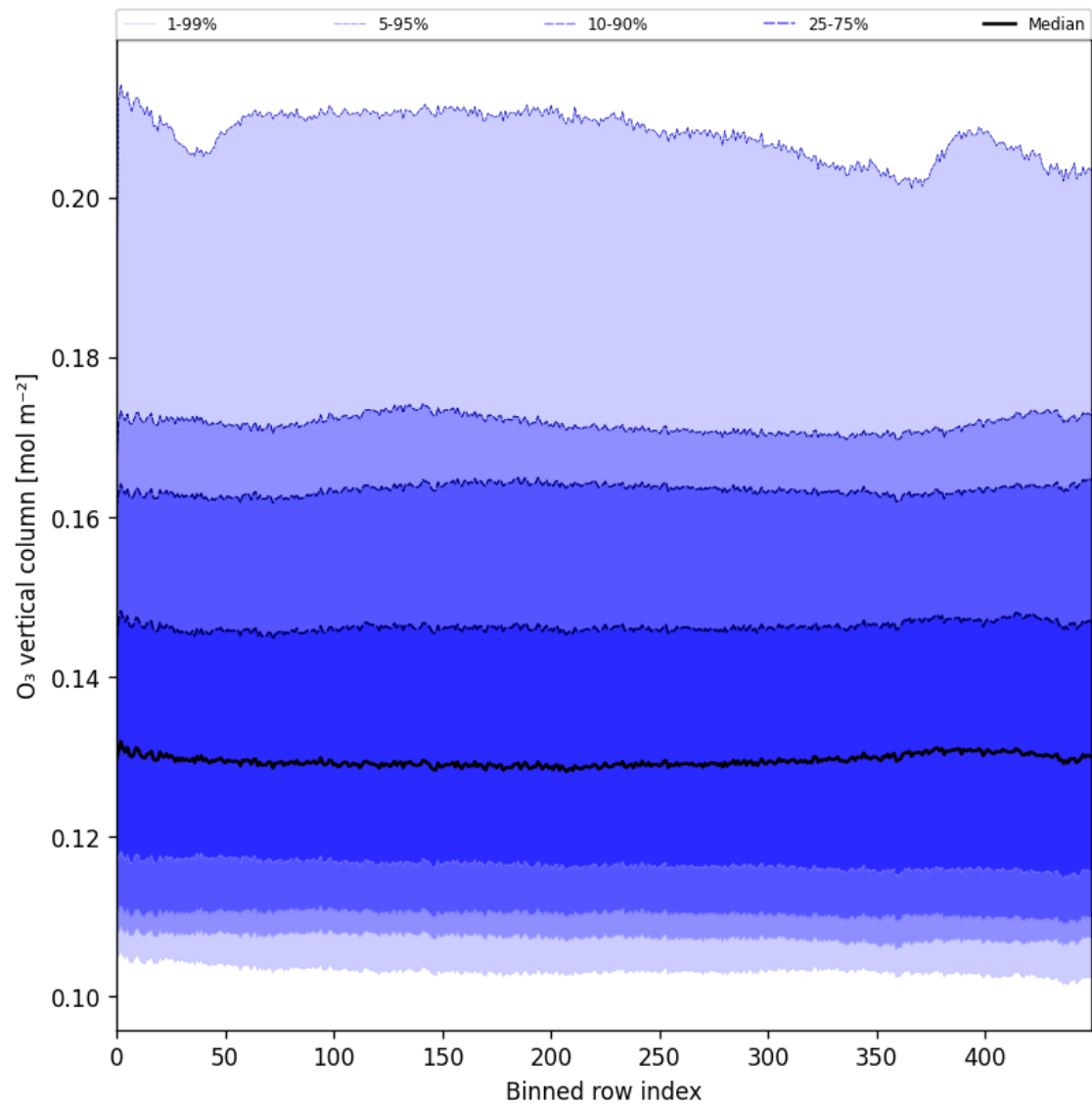
Figure 28: Along track statistics of “O 3 vertical column” for 2025-11-28 to 2025-11-30
