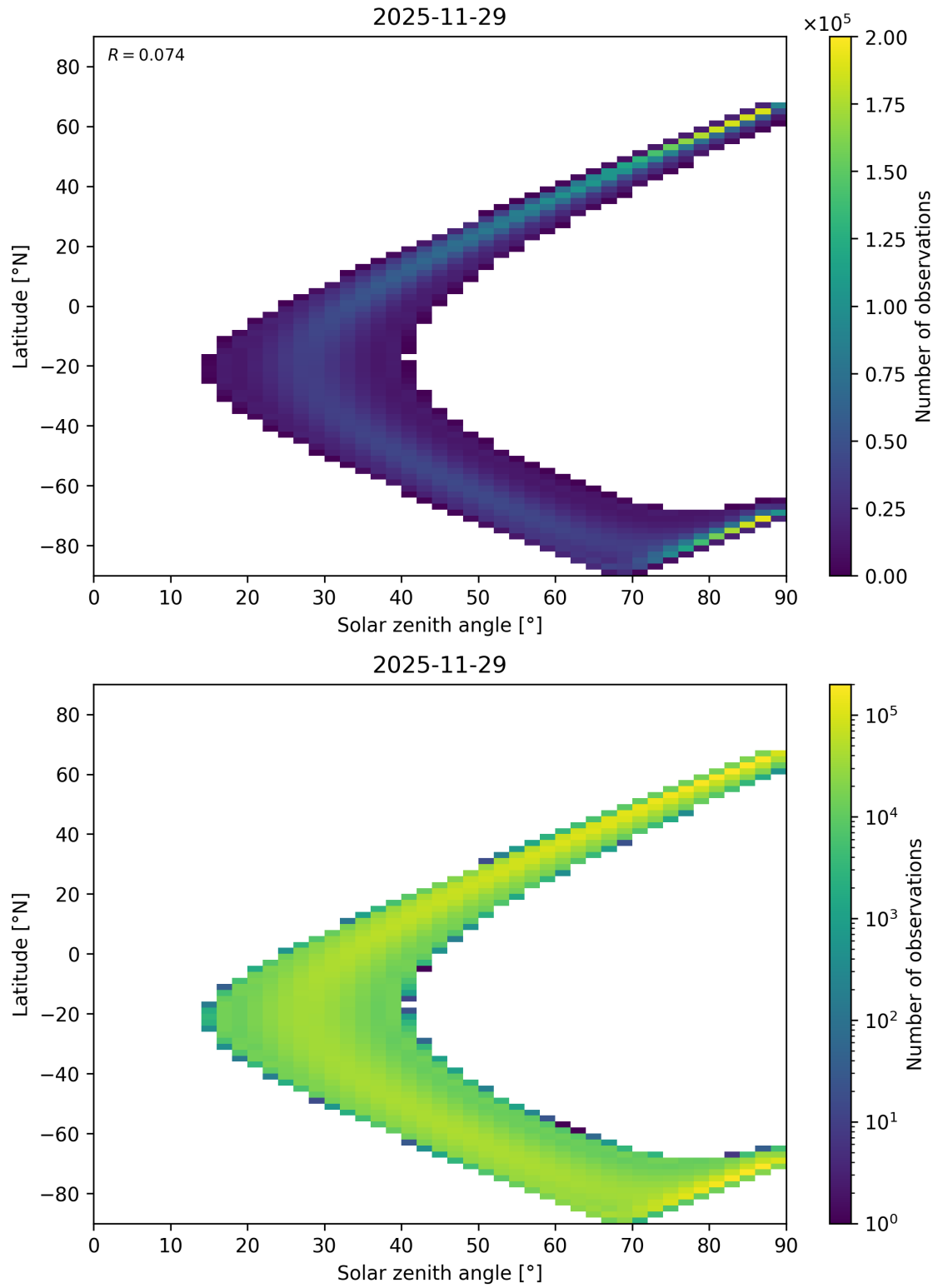
Figure 44: Scatter density plot of “Solar zenith angle” against “Latitude” for 2025-11-28 to 2025-11-30.
