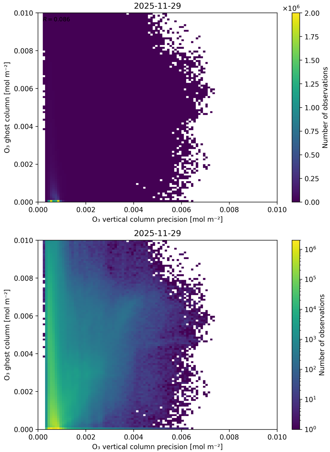
Figure 43: Scatter density plot of “ \text{O}_3 vertical column precision” against “ \text{O}_3 ghost column” for 2025-11-28 to 2025-11-30.
