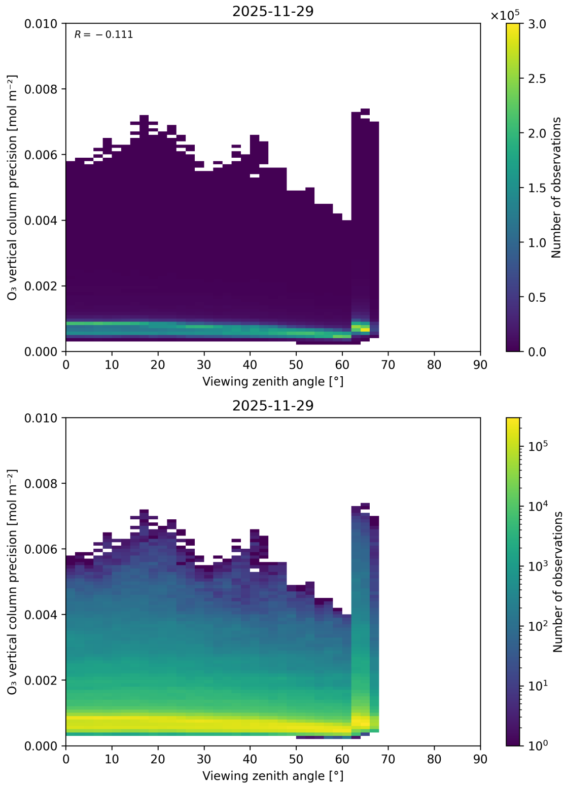
Figure 53: Scatter density plot of “Viewing zenith angle” against “O 3 vertical column precision” for 2025-11-28 to 2025-11-30.
