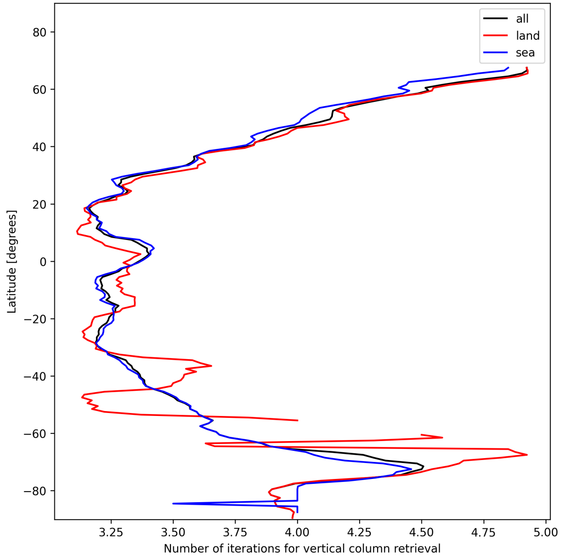
Figure 19: Zonal average of “Number of iterations for vertical column retrieval” for 2025-11-28 to 2025-11-30.
