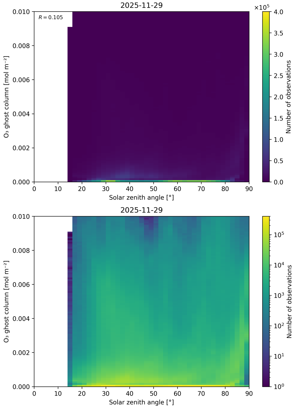
Figure 46: Scatter density plot of “Solar zenith angle” against “O 3 ghost column” for 2025-11-28 to 2025-11-30.
