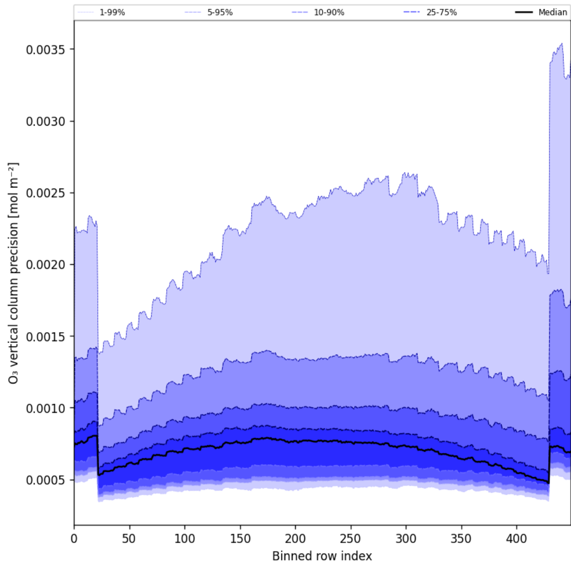
Figure 29: Along track statistics of “O 3 vertical column precision” for 2025-11-28 to 2025-11-30
