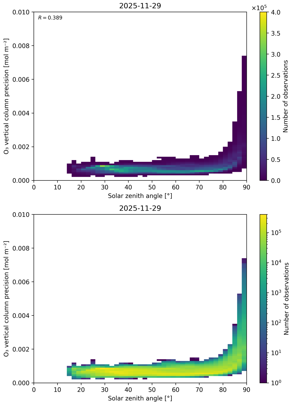
Figure 48: Scatter density plot of “Solar zenith angle” against “O 3 vertical column precision” for 2025-11-28 to 2025-11-30.
