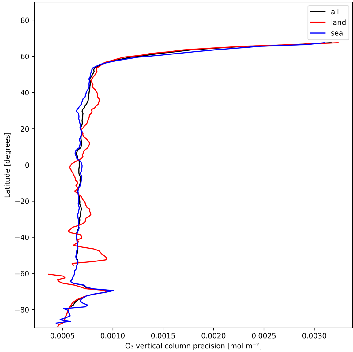
Figure 15: Zonal average of “O 3 vertical column precision” for 2025-11-28 to 2025-11-30.
