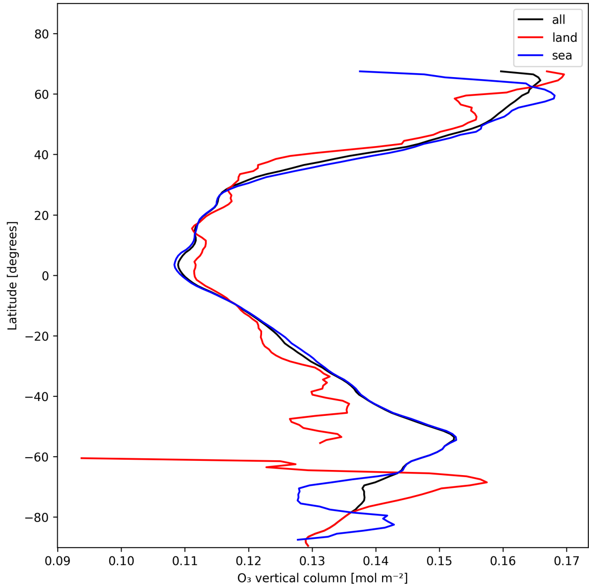
Figure 14: Zonal average of “O 3 vertical column” for 2025-11-28 to 2025-11-30.
