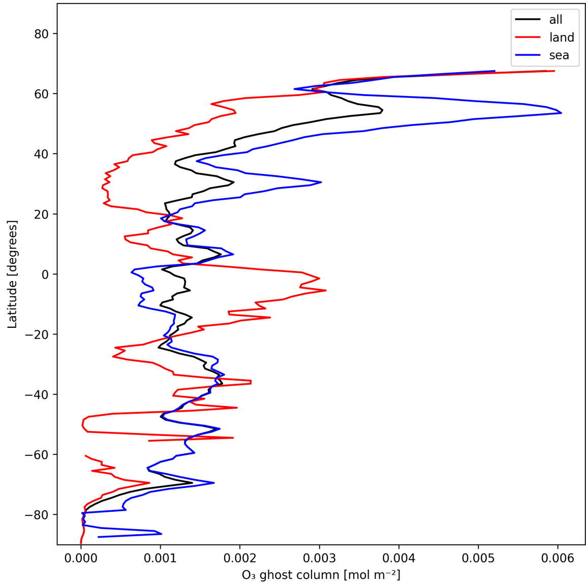
Figure 18: Zonal average of “O 3 ghost column” for 2025-11-28 to 2025-11-30.
