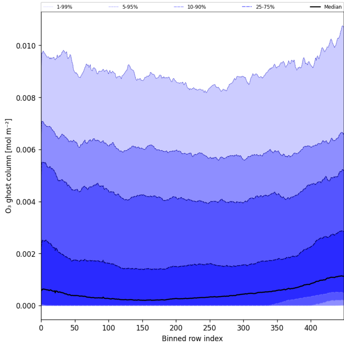
Figure 32: Along track statistics of "O 3 ghost column" for 2025-11-28 to 2025-11-30
