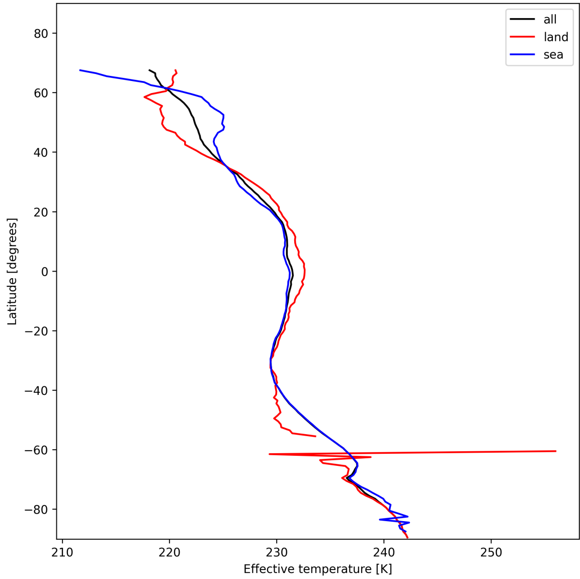
Figure 17: Zonal average of "Effective temperature" for 2025-11-28 to 2025-11-30.
