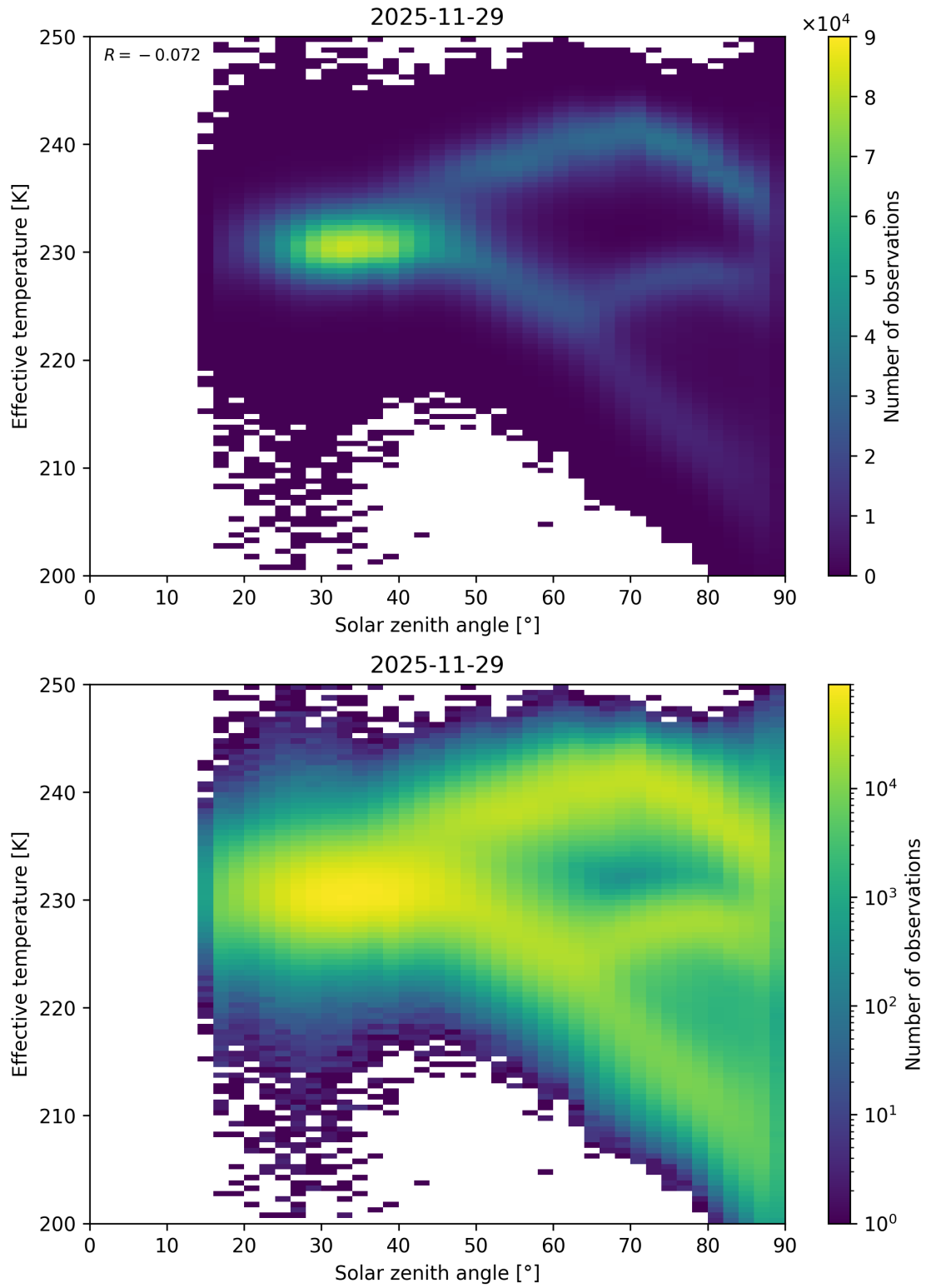
Figure 45: Scatter density plot of “Solar zenith angle” against “Effective temperature” for 2025-11-28 to 2025-11-30.
