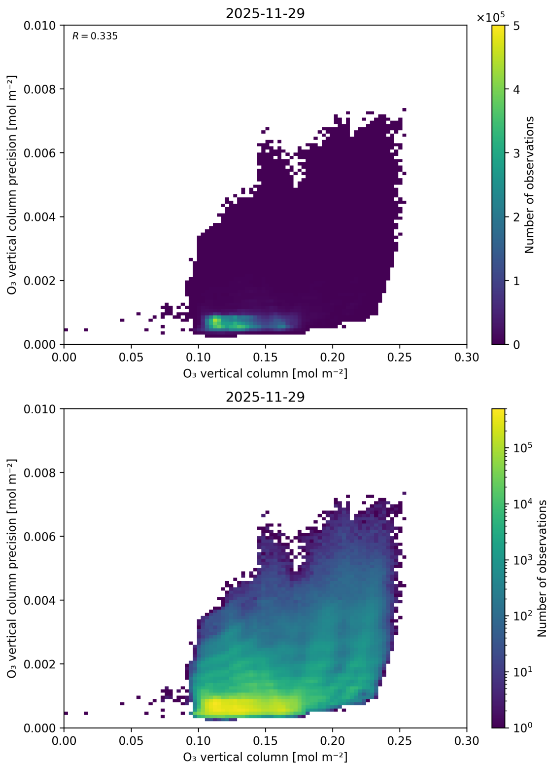
Figure 41: Scatter density plot of “O 3 vertical column” against “O 3 vertical column precision” for 2025-11-28 to 2025-11-30.
