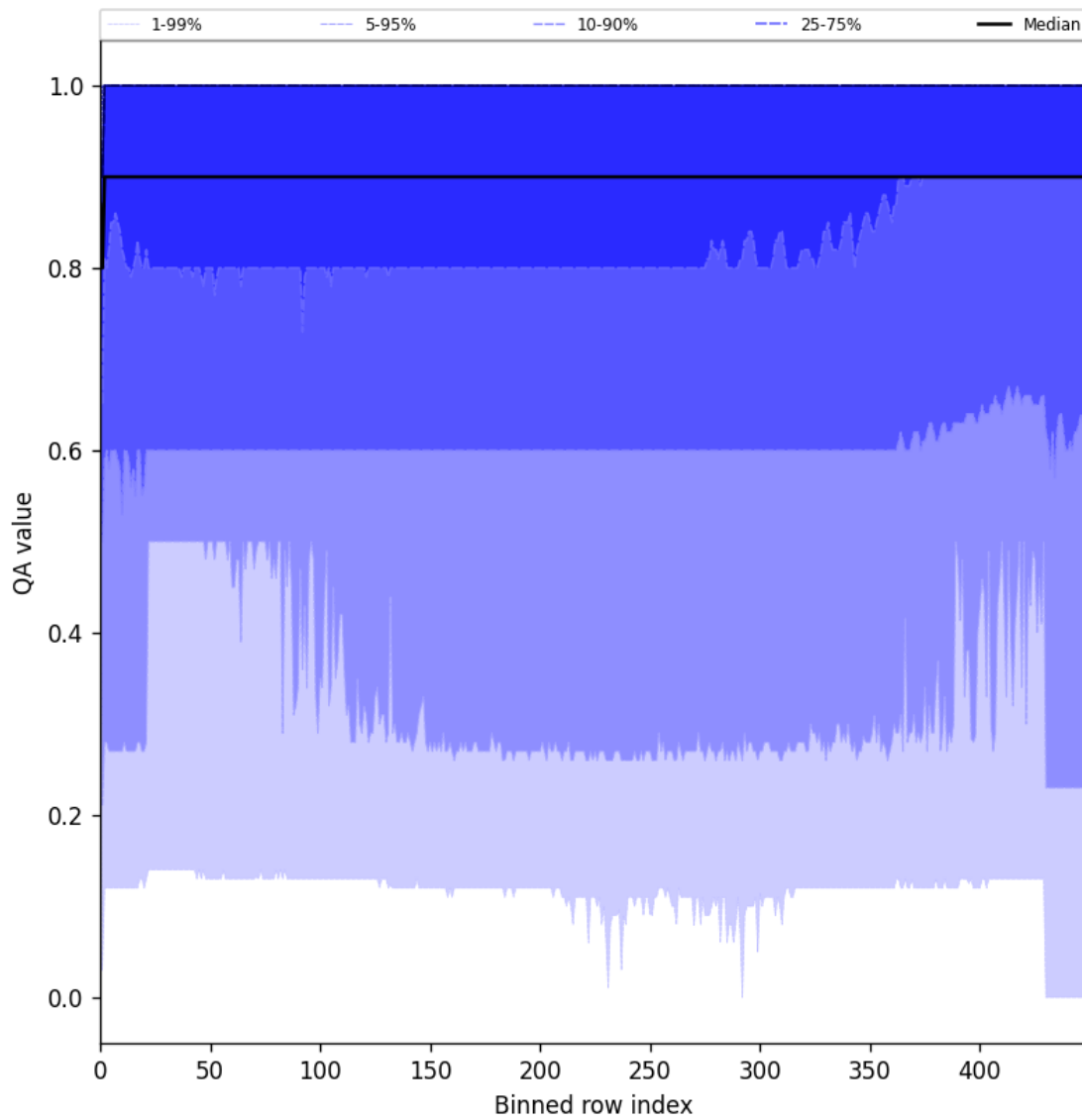
Figure 27: Along track statistics of “QA value” for 2025-11-28 to 2025-11-30
