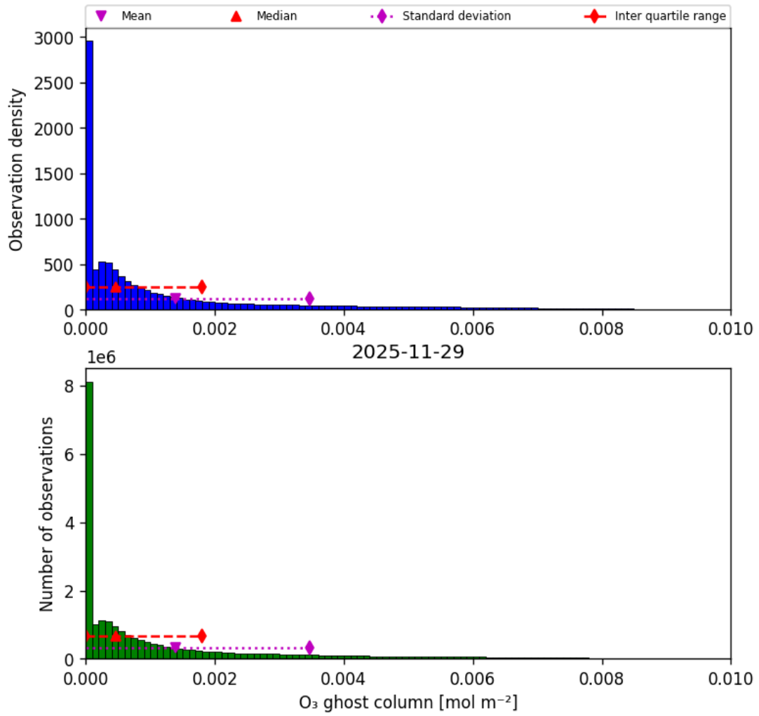
Figure 25: Histogram of “O 3 ghost column” for 2025-11-28 to 2025-11-30
