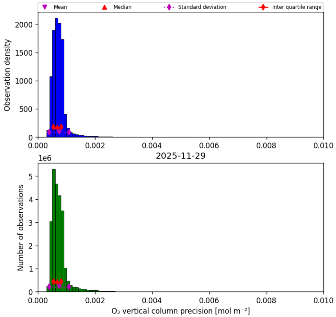
Figure 22: Histogram of “O 3 vertical column precision” for 2025-11-28 to 2025-11-30
