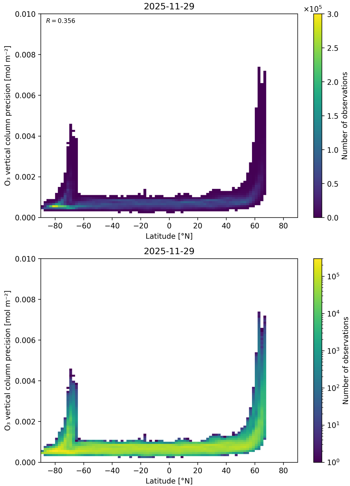
Figure 37: Scatter density plot of “Latitude” against “O 3 vertical column precision” for 2025-11-28 to 2025-11-30.
