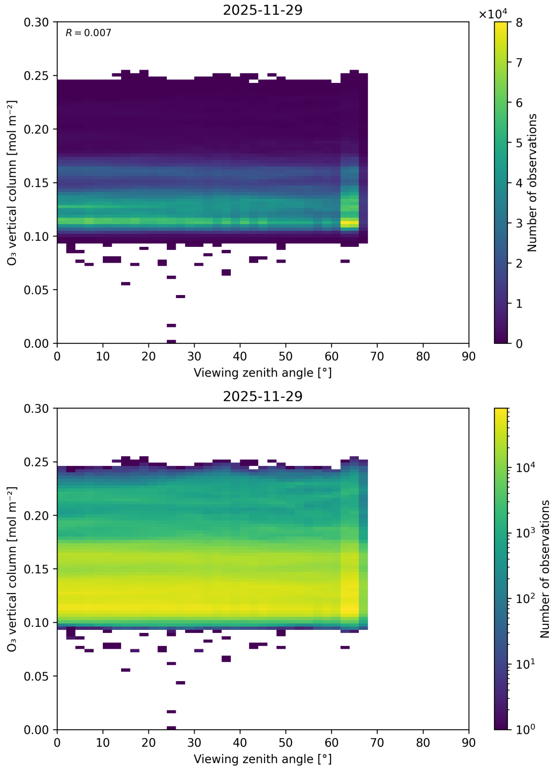
Figure 52: Scatter density plot of “Viewing zenith angle” against “O 3 vertical column” for 2025-11-28 to 2025-11-30.
