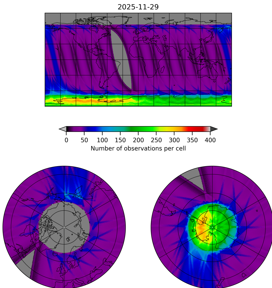
Figure 12: Map of the number of observations for 2025-11-28 to 2025-11-30
