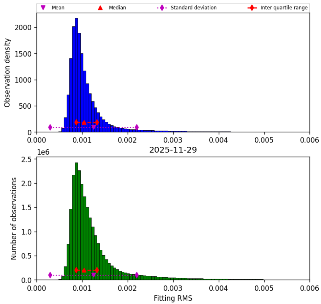
Figure 23: Histogram of “Fitting RMS” for 2025-11-28 to 2025-11-30
