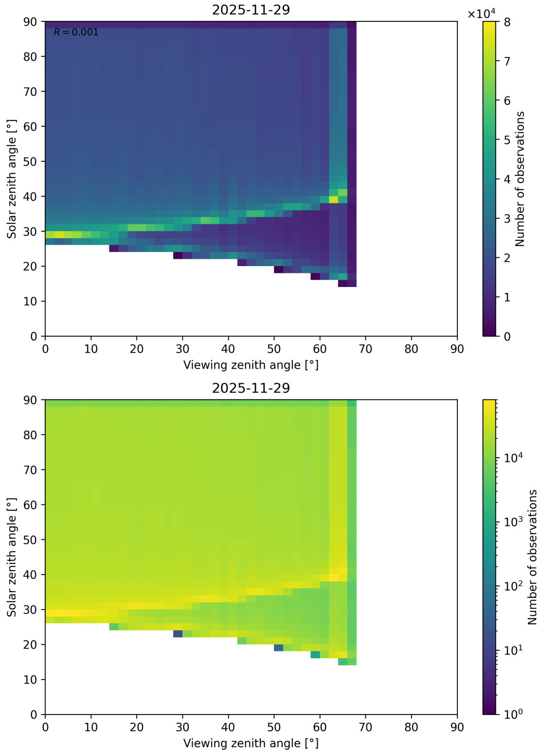
Figure 54: Scatter density plot of “Viewing zenith angle” against “Solar zenith angle” for 2025-11-28 to 2025-11-30.
