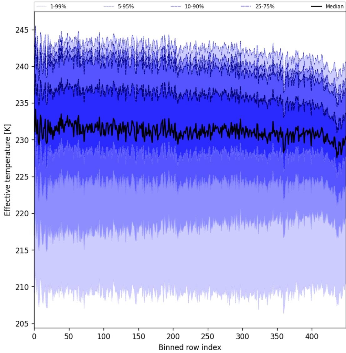
Figure 31: Along track statistics of “Effective temperature” for 2025-11-28 to 2025-11-30
