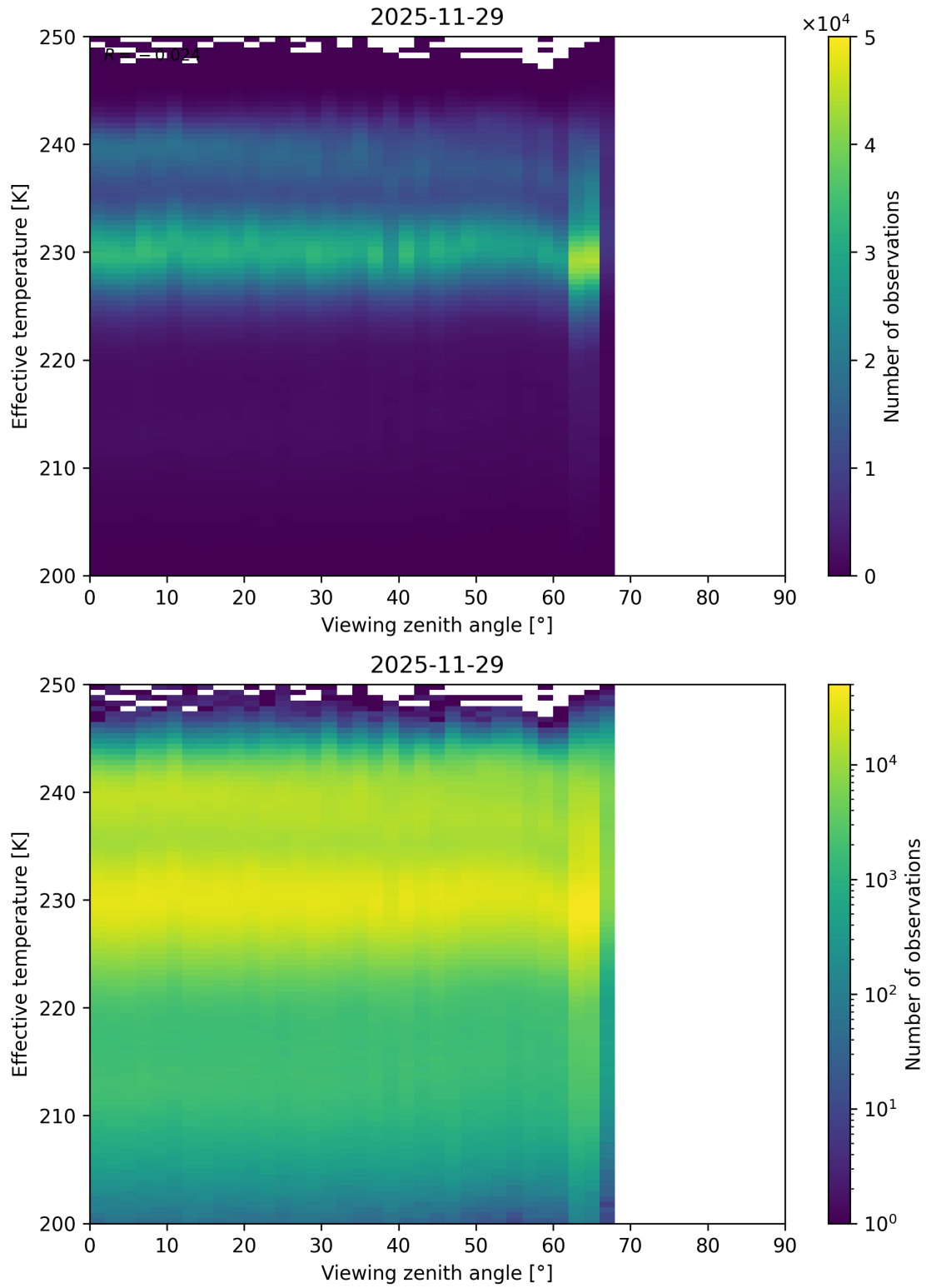
Figure 50: Scatter density plot of “Viewing zenith angle” against “Effective temperature” for 2025-11-28 to 2025-11-30.
