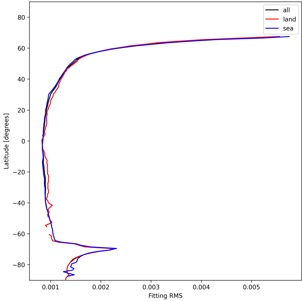
Figure 16: Zonal average of “Fitting RMS” for 2025-11-28 to 2025-11-30.
