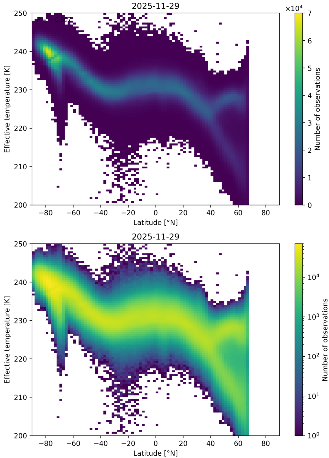
Figure 34: Scatter density plot of “Latitude” against “Effective temperature” for 2025-11-28 to 2025-11-30.
