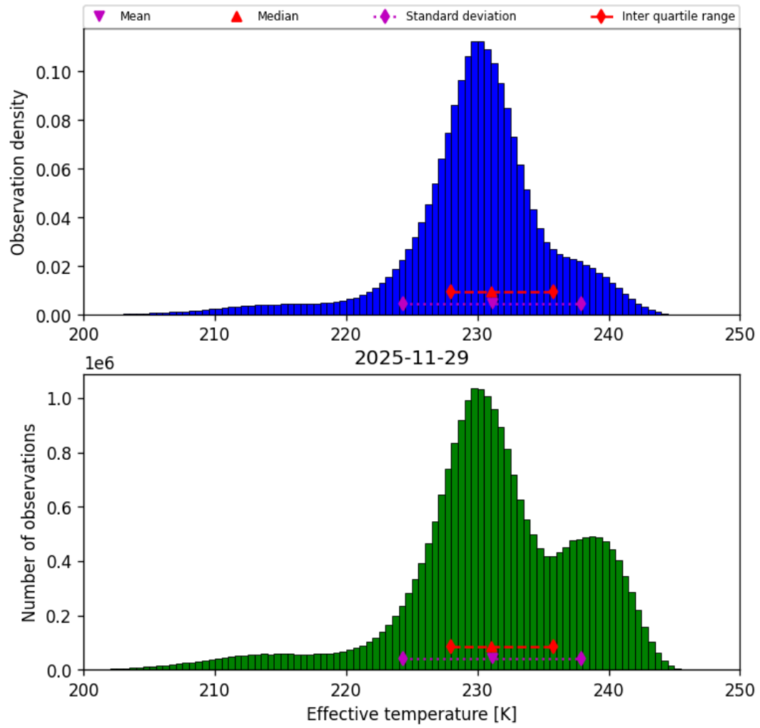
Figure 24: Histogram of “Effective temperature” for 2025-11-28 to 2025-11-30
