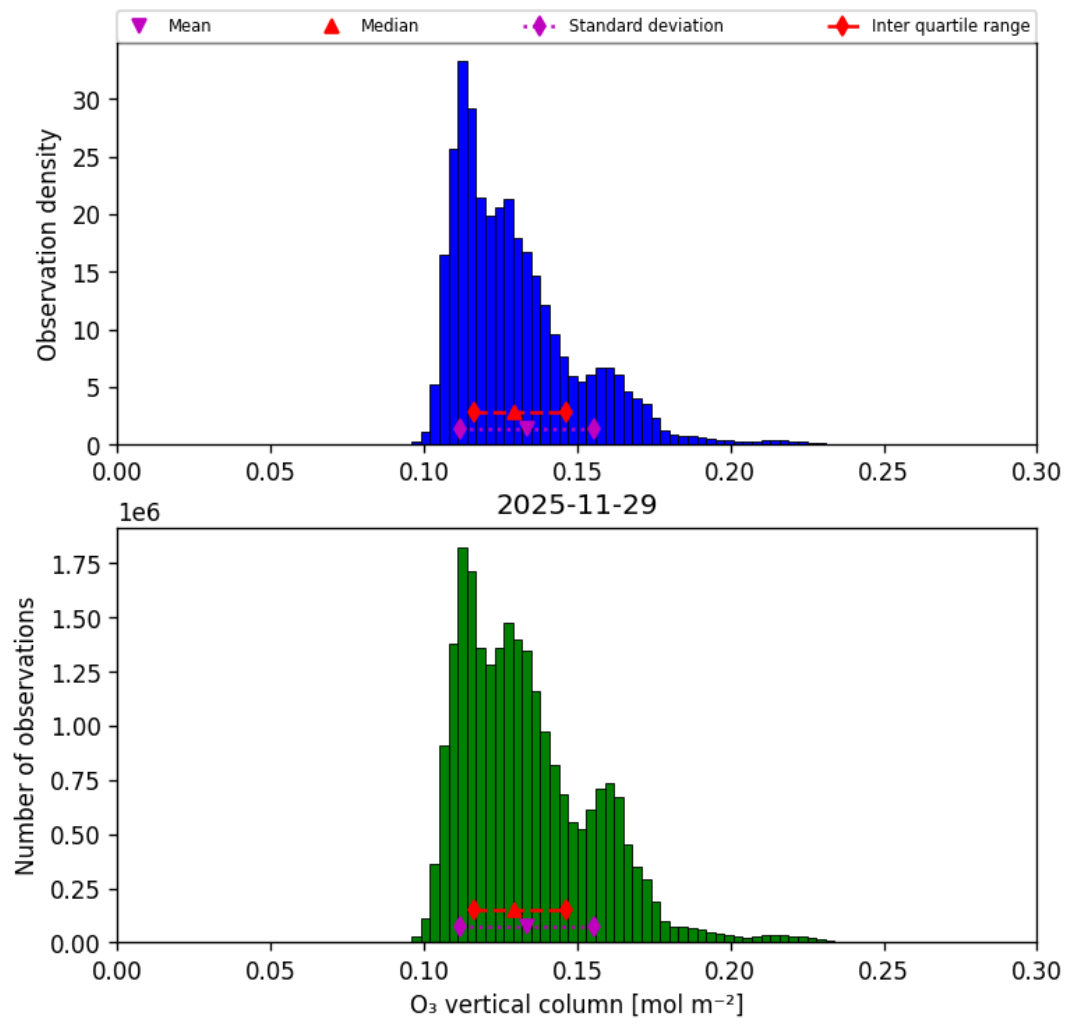
Figure 21: Histogram of “O 3 vertical column” for 2025-11-28 to 2025-11-30
