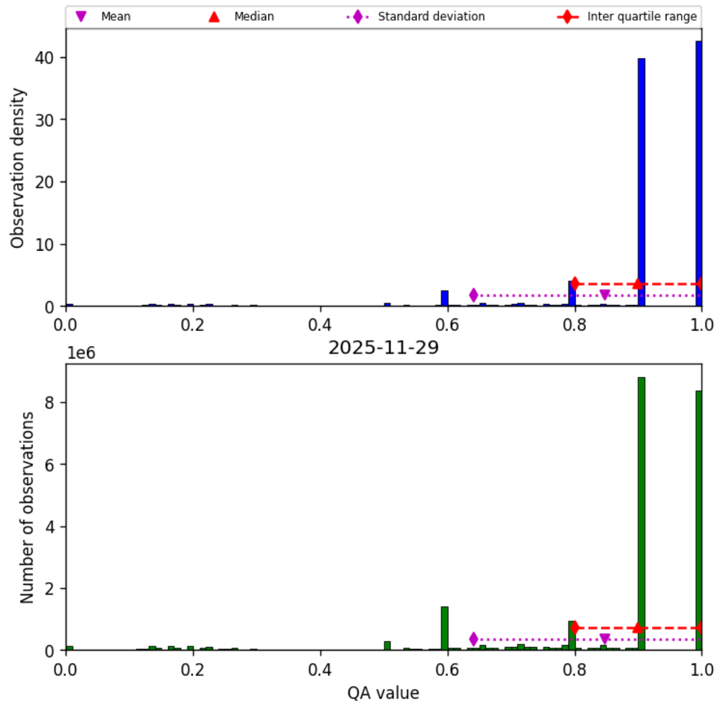
Figure 20: Histogram of “QA value” for 2025-11-28 to 2025-11-30
