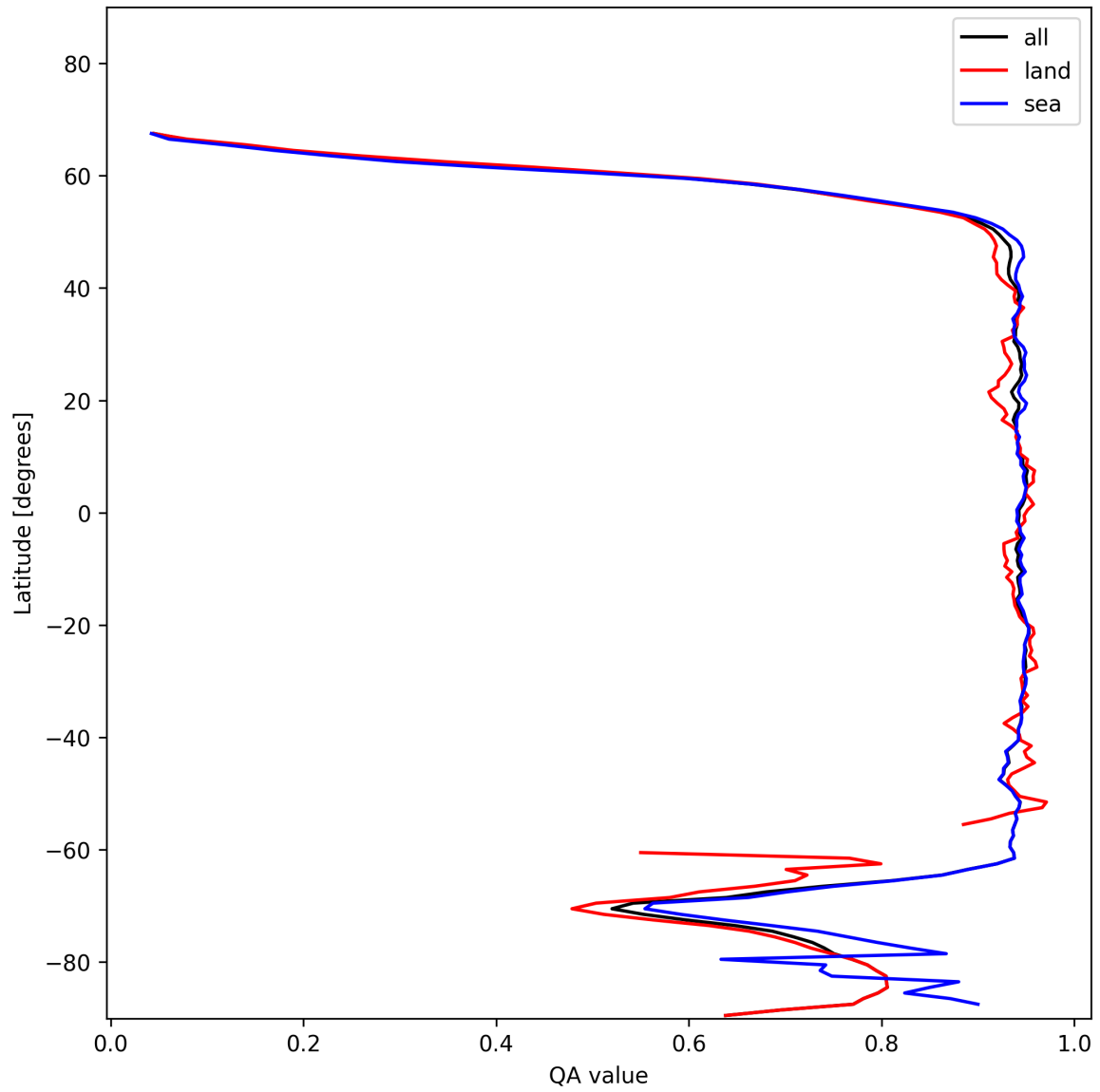
Figure 13: Zonal average of “QA value” for 2025-11-28 to 2025-11-30.
