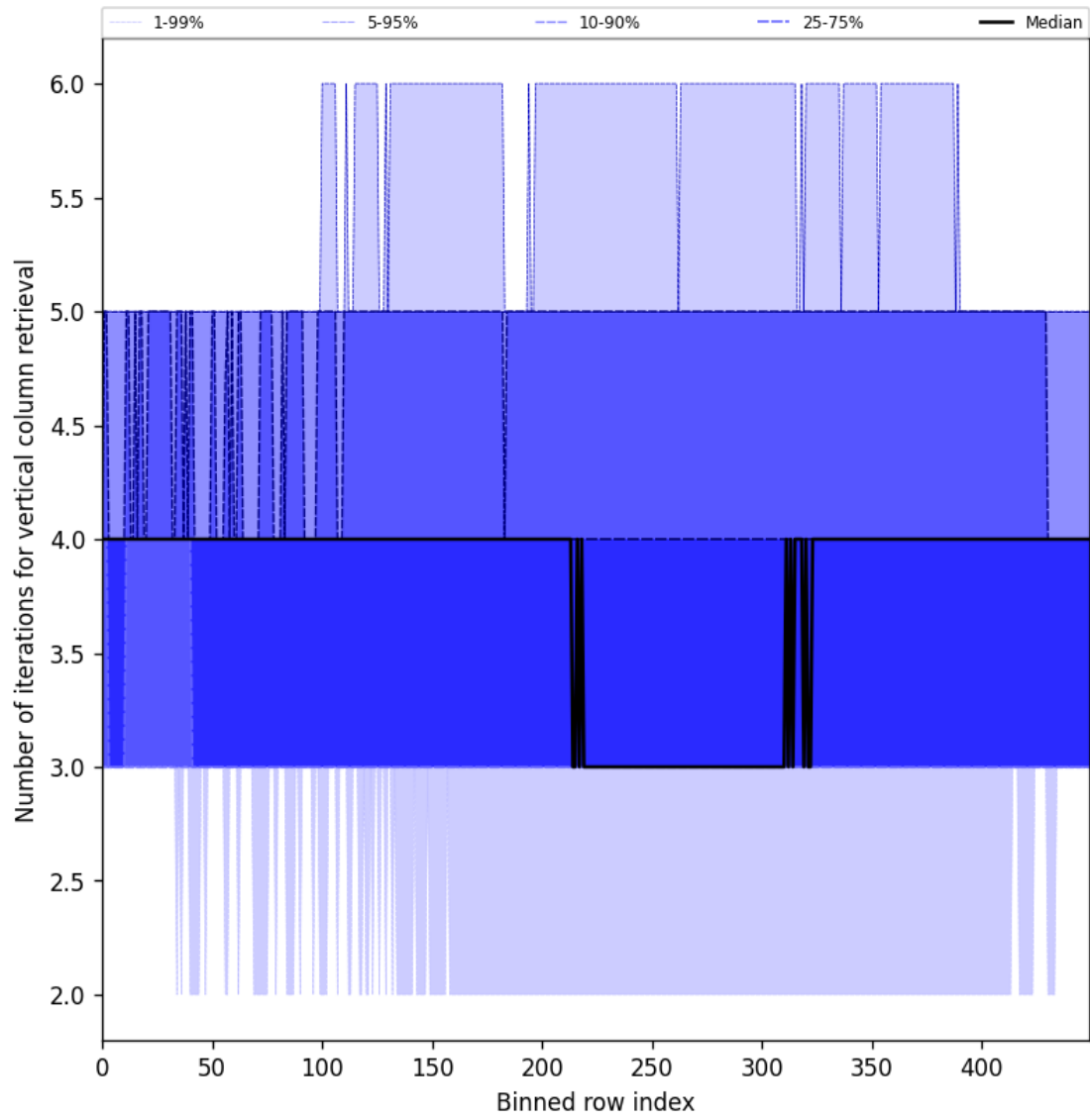
Figure 33: Along track statistics of “Number of iterations for vertical column retrieval” for 2025-11-28 to 2025-11-30
