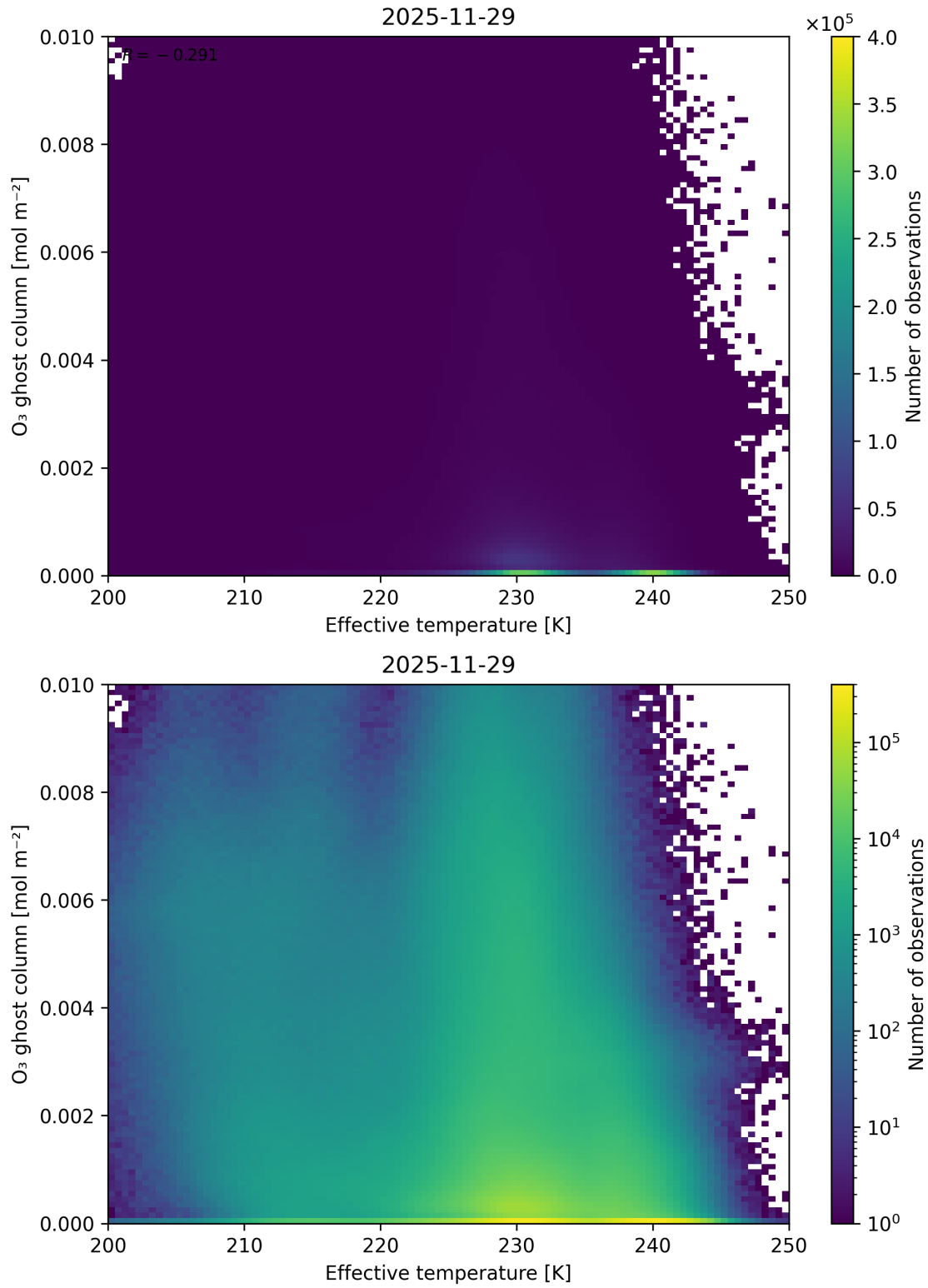
Figure 38: Scatter density plot of “Effective temperature” against “O 3 ghost column” for 2025-11-28 to 2025-11-30.
