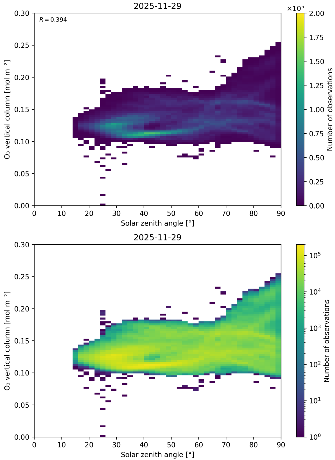
Figure 47: Scatter density plot of “Solar zenith angle” against “O 3 vertical column” for 2025-11-28 to 2025-11-30.
