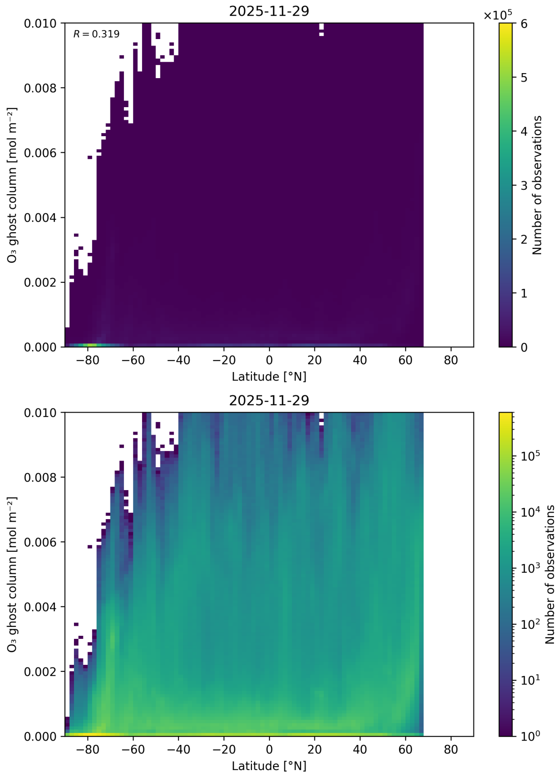
Figure 35: Scatter density plot of “Latitude” against “O 3 ghost column” for 2025-11-28 to 2025-11-30.
