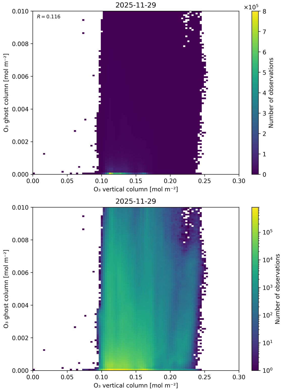
Figure 40: Scatter density plot of “O 3 vertical column” against “O 3 ghost column” for 2025-11-28 to 2025-11-30.
