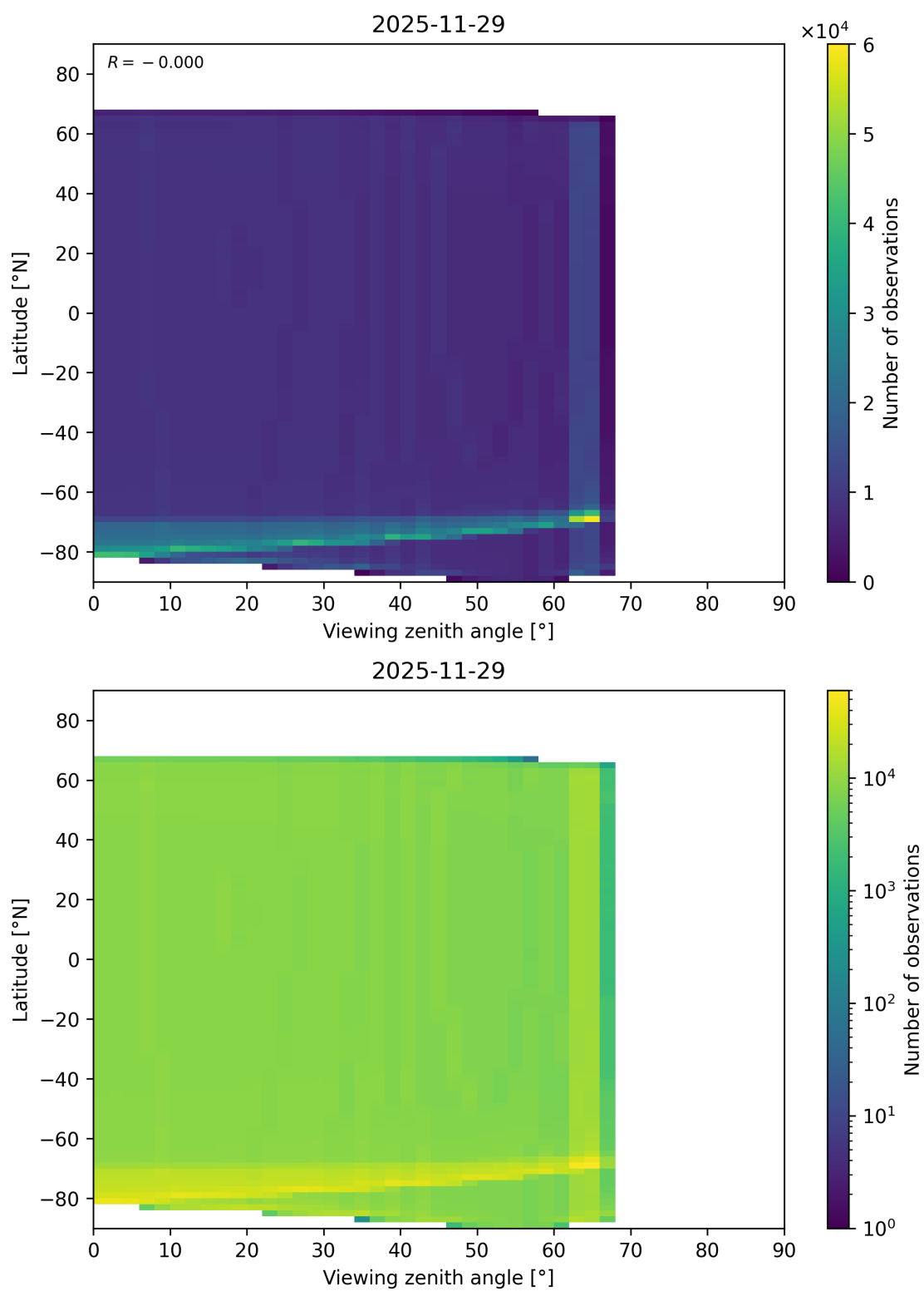
Figure 49: Scatter density plot of “Viewing zenith angle” against “Latitude” for 2025-11-28 to 2025-11-30.
