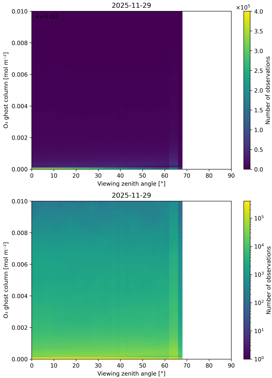
Figure 51: Scatter density plot of “Viewing zenith angle” against “O 3 ghost column” for 2025-11-28 to 2025-11-30.
