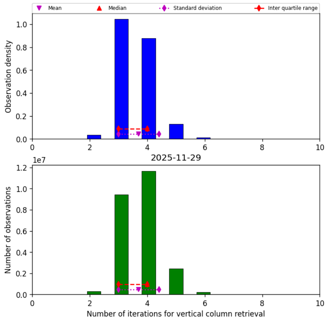
Figure 26: Histogram of “Number of iterations for vertical column retrieval” for 2025-11-28 to 2025-11-30
