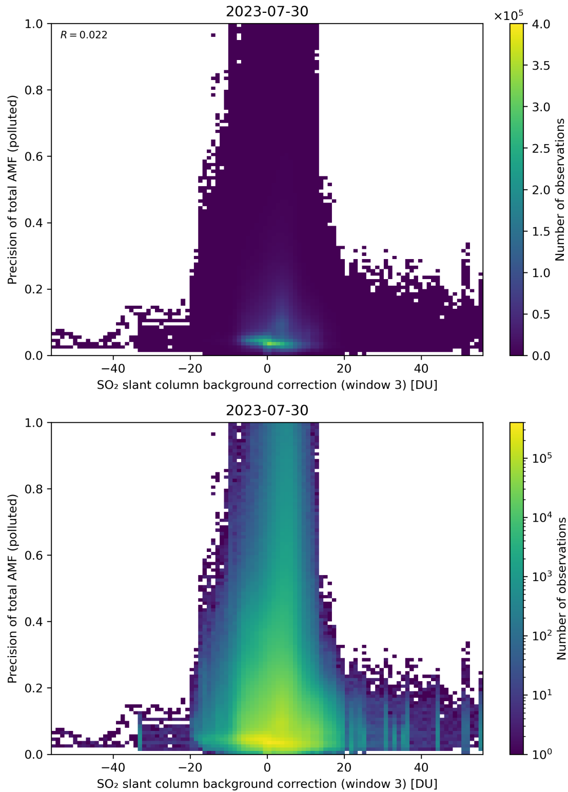
Figure 126: Scatter density plot of “SO 2 slant column background correction (window 3)” against “Precision of total AMF (polluted)” for 2023-07-29 to 2023-07-31.
