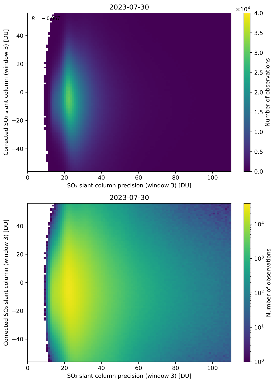
Figure 262: Scatter density plot of “SO 2 slant column precision (window 3)” against “Corrected SO 2 slant column (window 3)” for 2023-07-29 to 2023-07-31.
