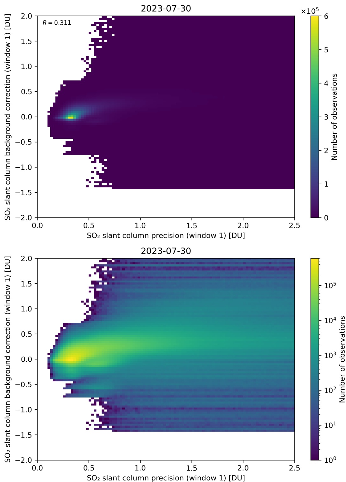
Figure 218: Scatter density plot of “SO 2 slant column precision (window 1)” against “SO 2 slant column background correction (window 1)” for 2023-07-29 to 2023-07-31.
