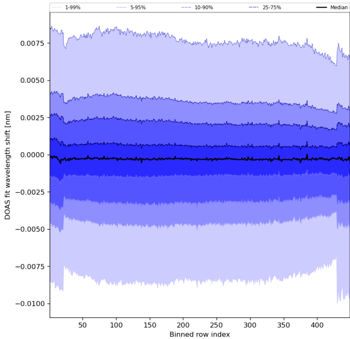
Figure 91: Along track statistics of “DOAS fit wavelength shift” for 2023-07-29 to 2023-07-31
