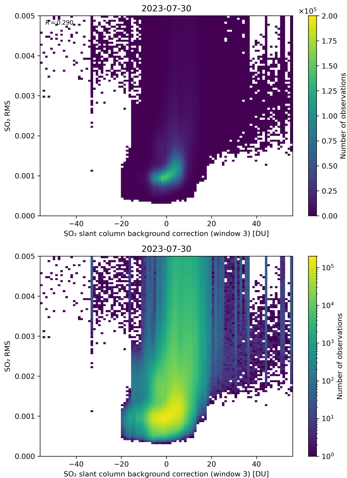
Figure 123: Scatter density plot of “SO 2 slant column background correction (window 3)” against “SO 2 RMS” for 2023-07-29 to 2023-07-31.
