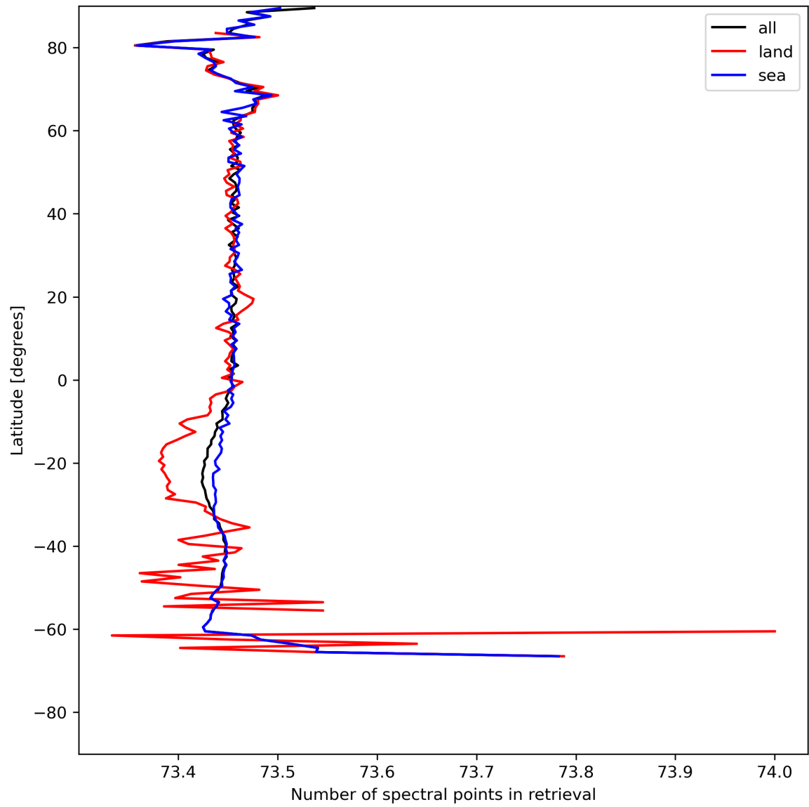
Figure 51: Zonal average of “Number of spectral points in retrieval” for 2023-07-29 to 2023-07-31.
