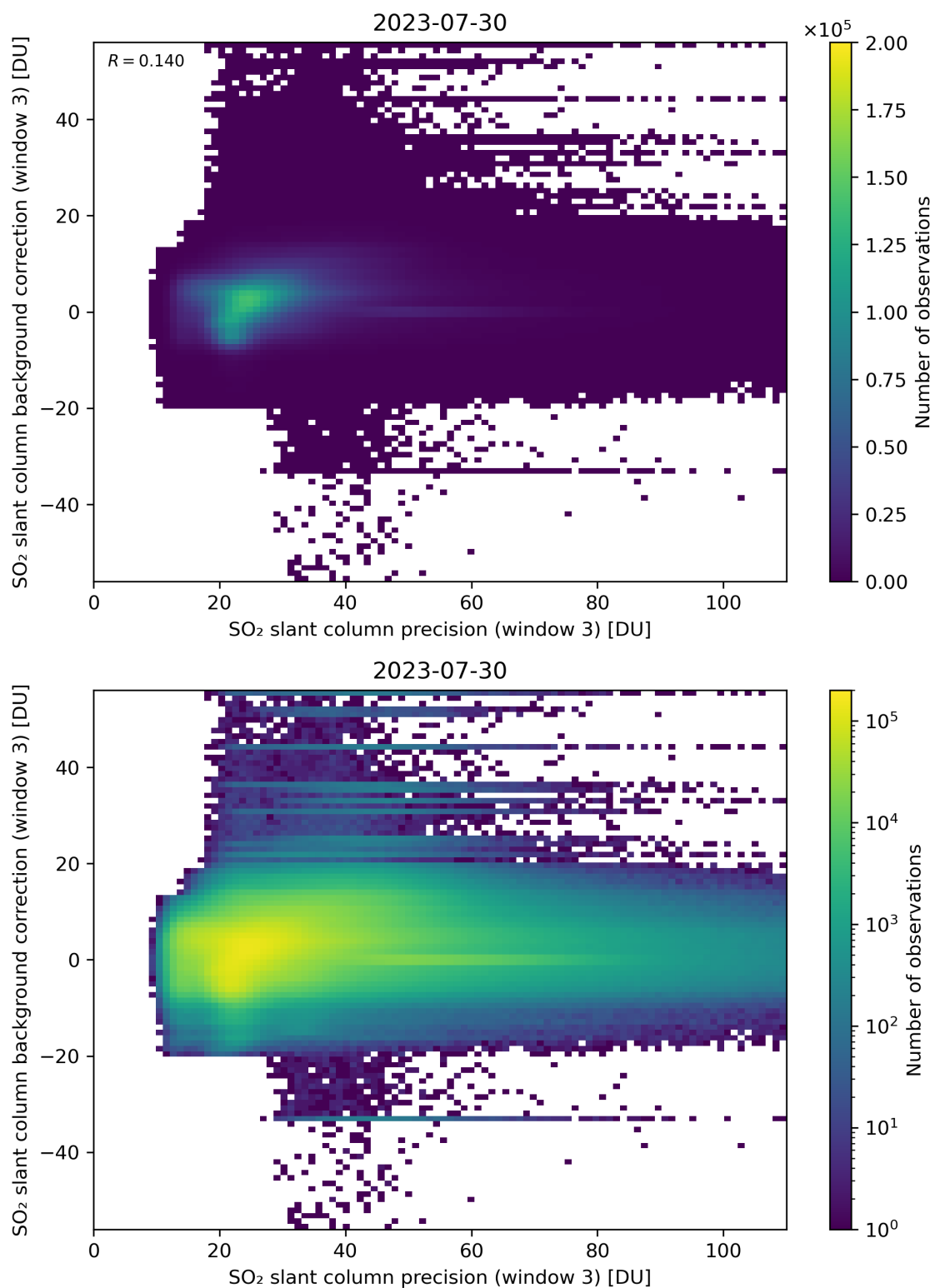
Figure 257: Scatter density plot of “SO 2 slant column precision (window 3)” against “SO 2 slant column background correction (window 3)” for 2023-07-29 to 2023-07-31.
