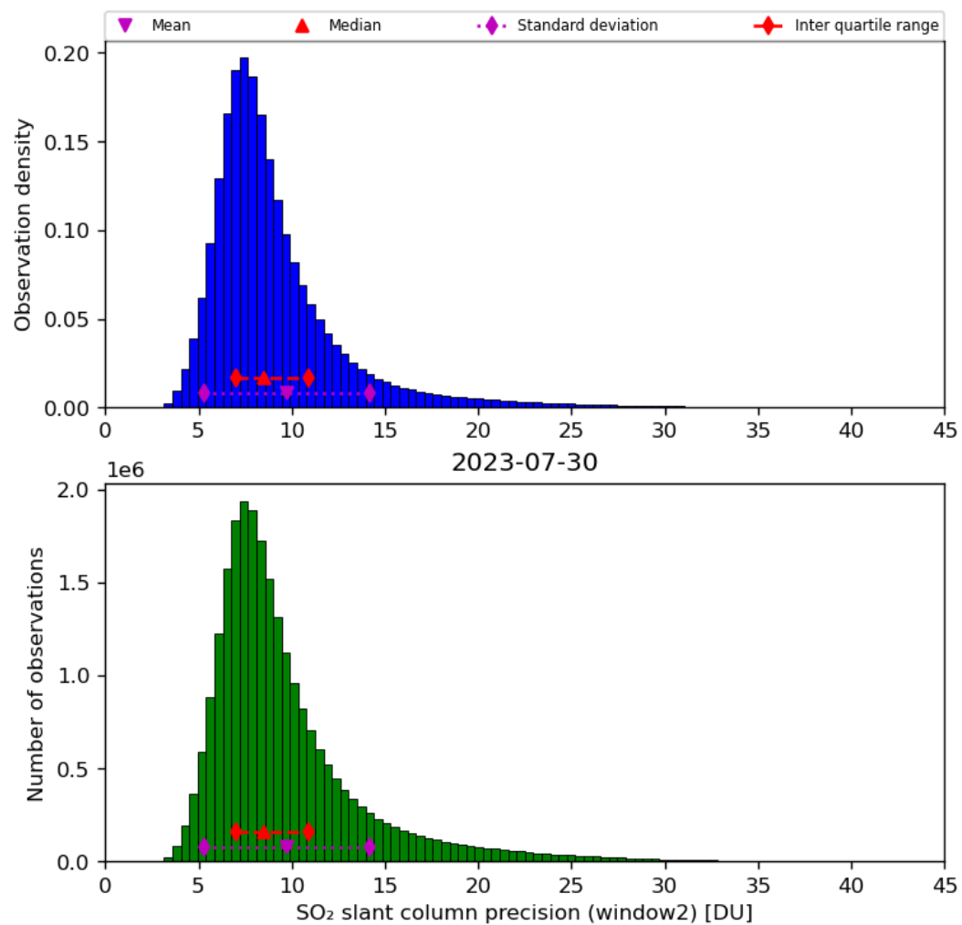
Figure 61: Histogram of “SO 2 slant column precision (window2)” for 2023-07-29 to 2023-07-31
