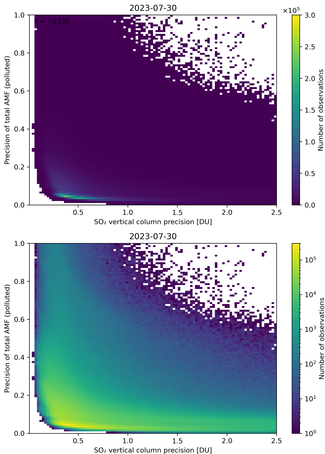
Figure 295: Scatter density plot of “SO 2 vertical column precision” against “Precision of total AMF (polluted)” for 2023-07-29 to 2023-07-31.
