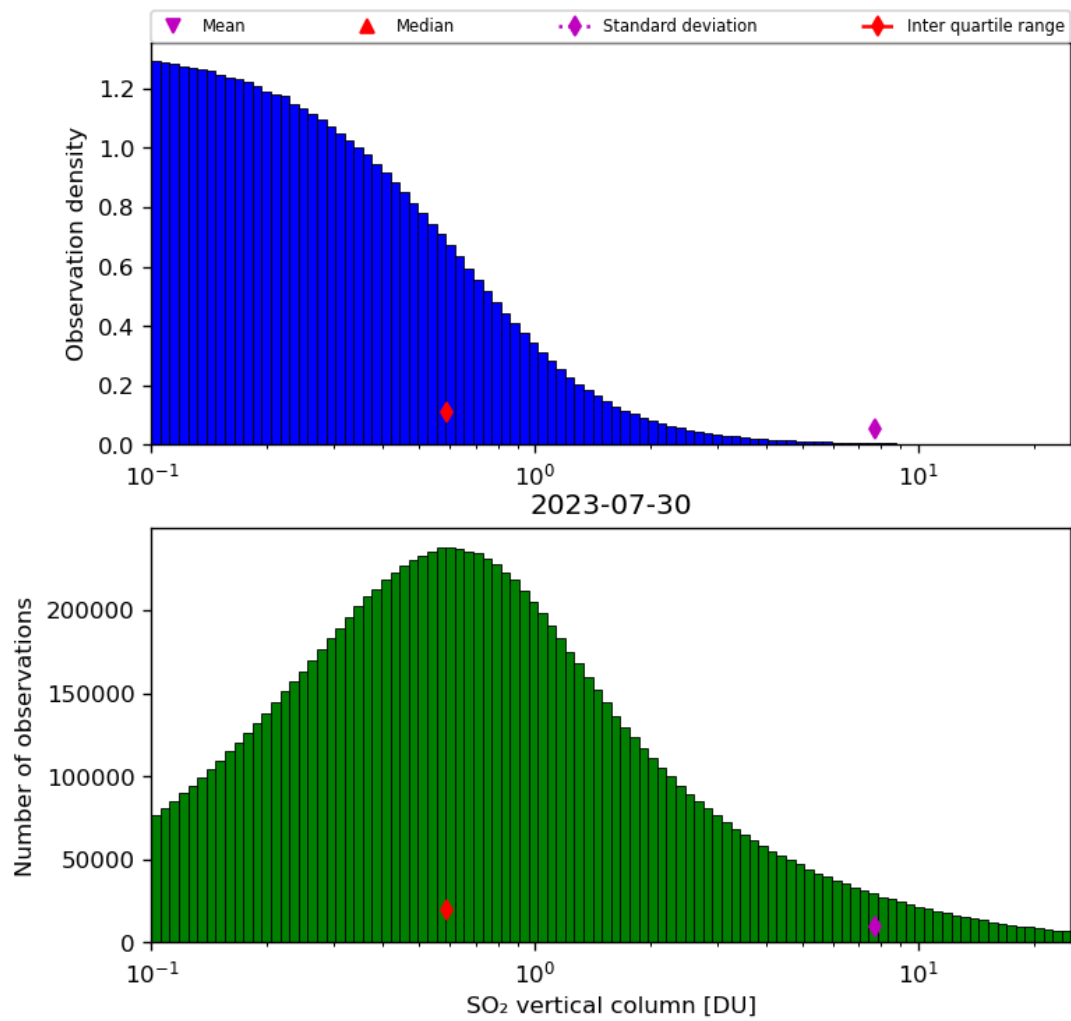
Figure 53: Histogram of “SO 2 vertical column” for 2023-07-29 to 2023-07-31
