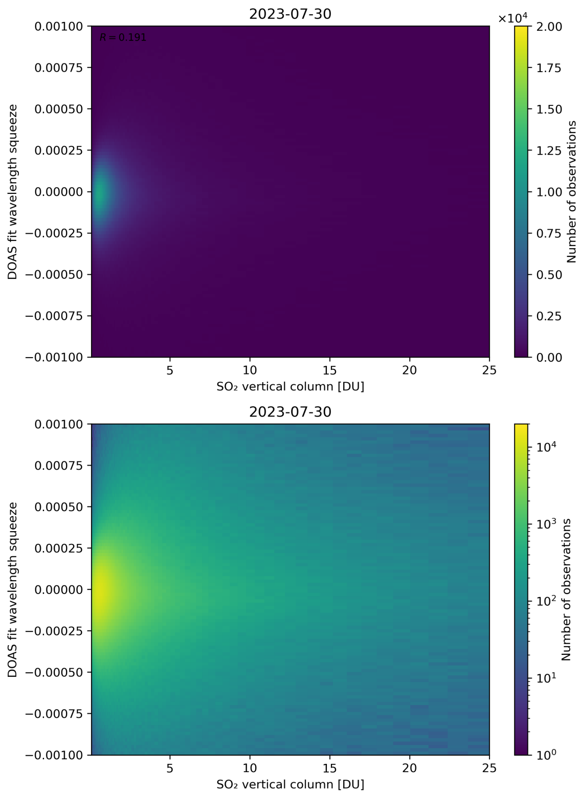
Figure 277: Scatter density plot of “SO 2 vertical column” against “DOAS fit wavelength squeeze” for 2023-07-29 to 2023-07-31.
