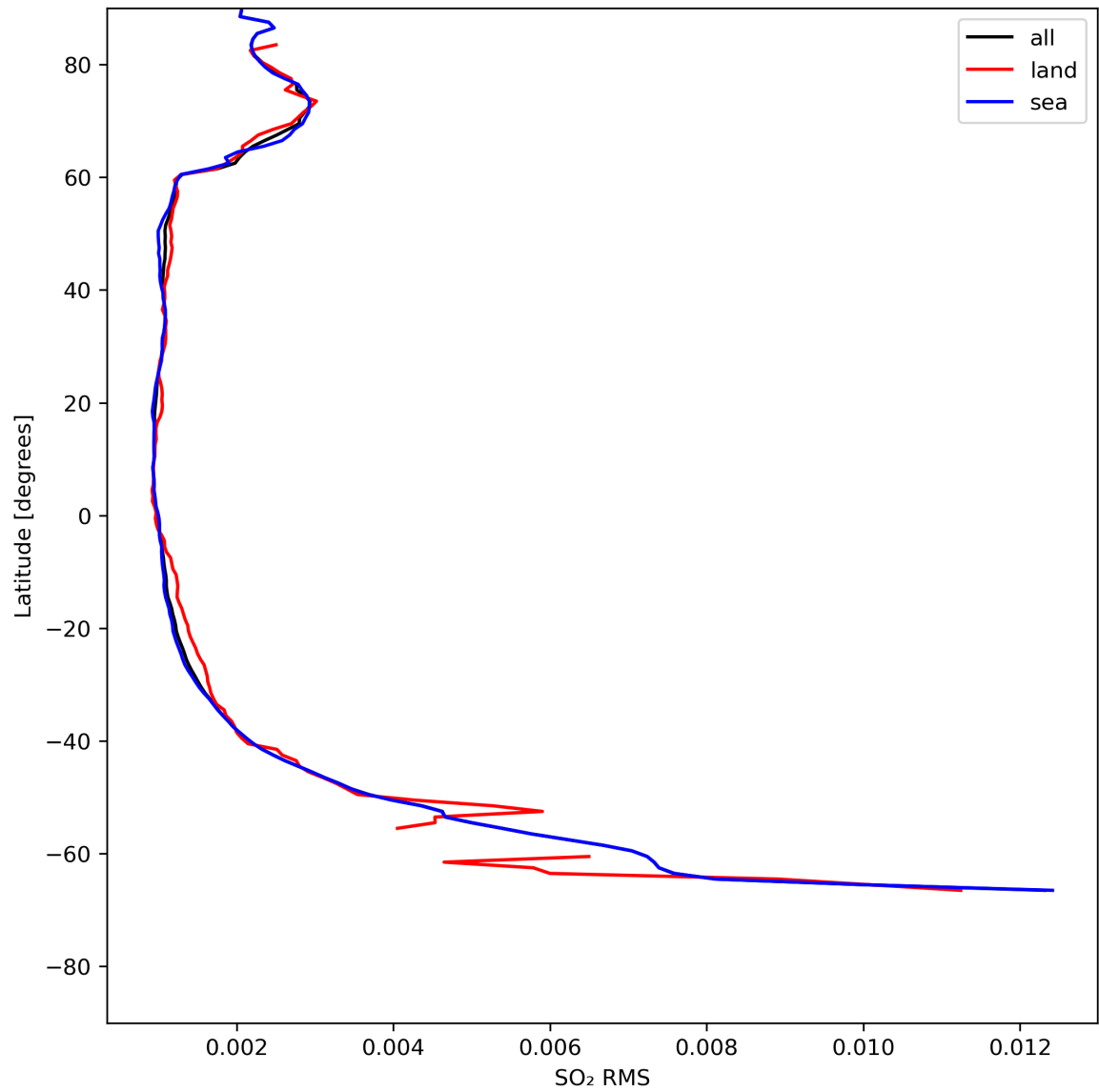
Figure 47: Zonal average of “SO 2 RMS” for 2023-07-29 to 2023-07-31.
