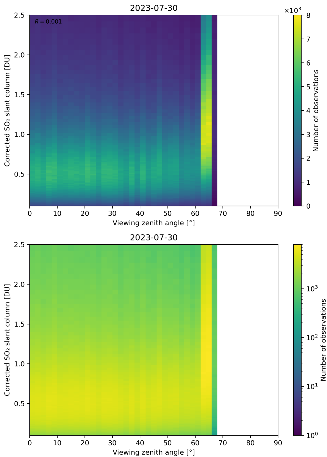
Figure 317: Scatter density plot of “Viewing zenith angle” against “Corrected SO 2 slant column” for 2023-07-29 to 2023-07-31.
