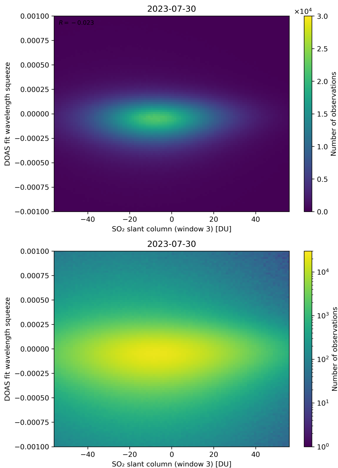
Figure 255: Scatter density plot of “SO 2 slant column (window 3)” against “DOAS fit wavelength squeeze” for 2023-07-29 to 2023-07-31.
