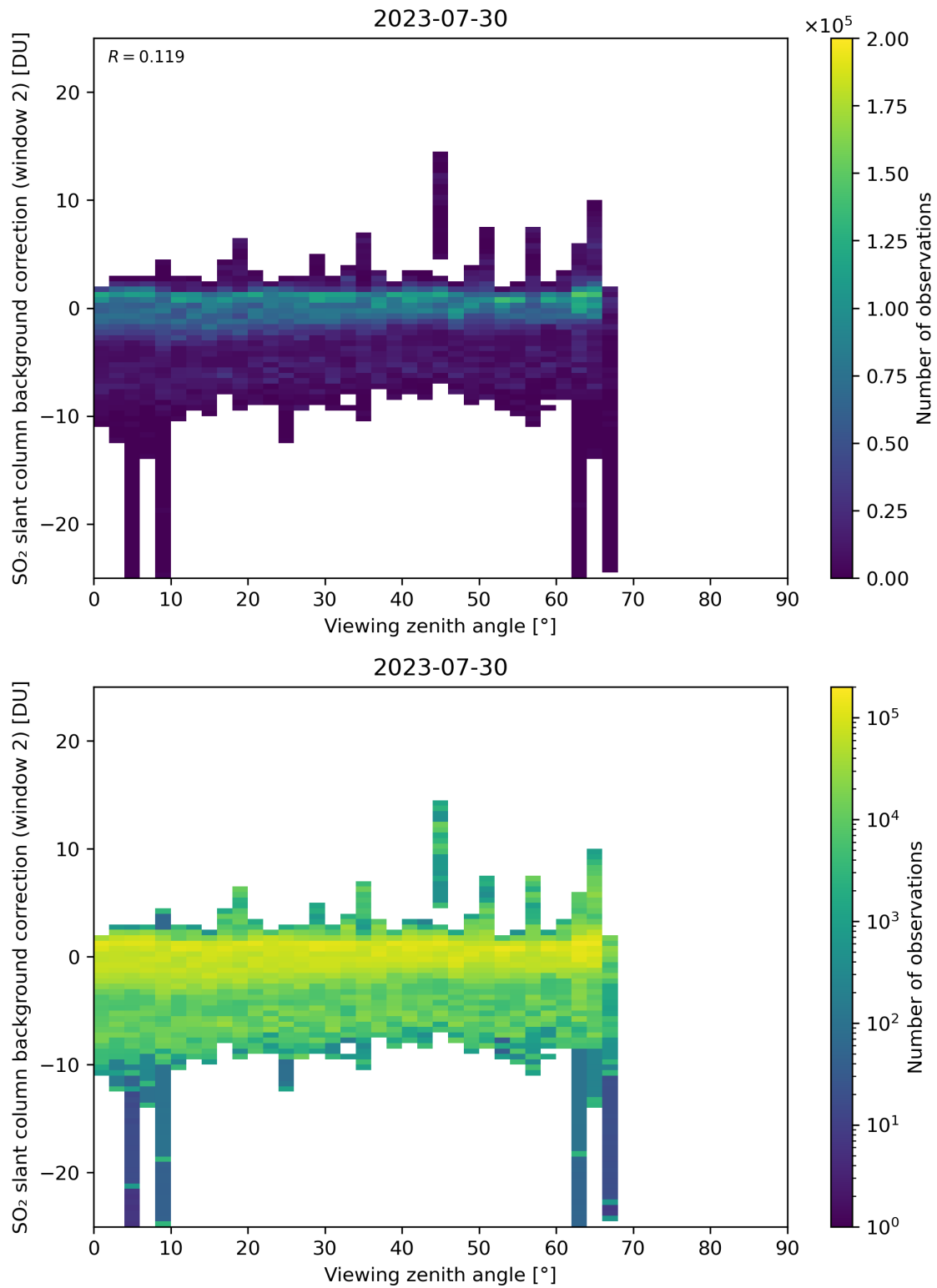
Figure 309: Scatter density plot of “Viewing zenith angle” against “SO 2 slant column background correction (window 2)” for 2023-07-29 to 2023-07-31.
