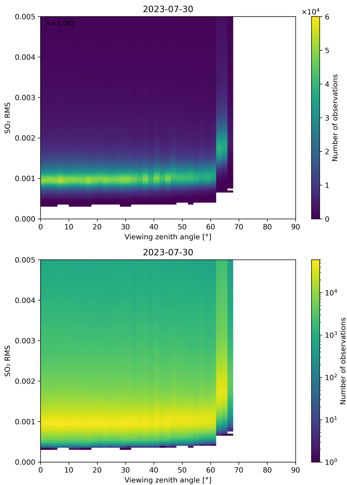
Figure 313: Scatter density plot of “Viewing zenith angle” against “SO 2 RMS” for 2023-07-29 to 2023-07-31.
