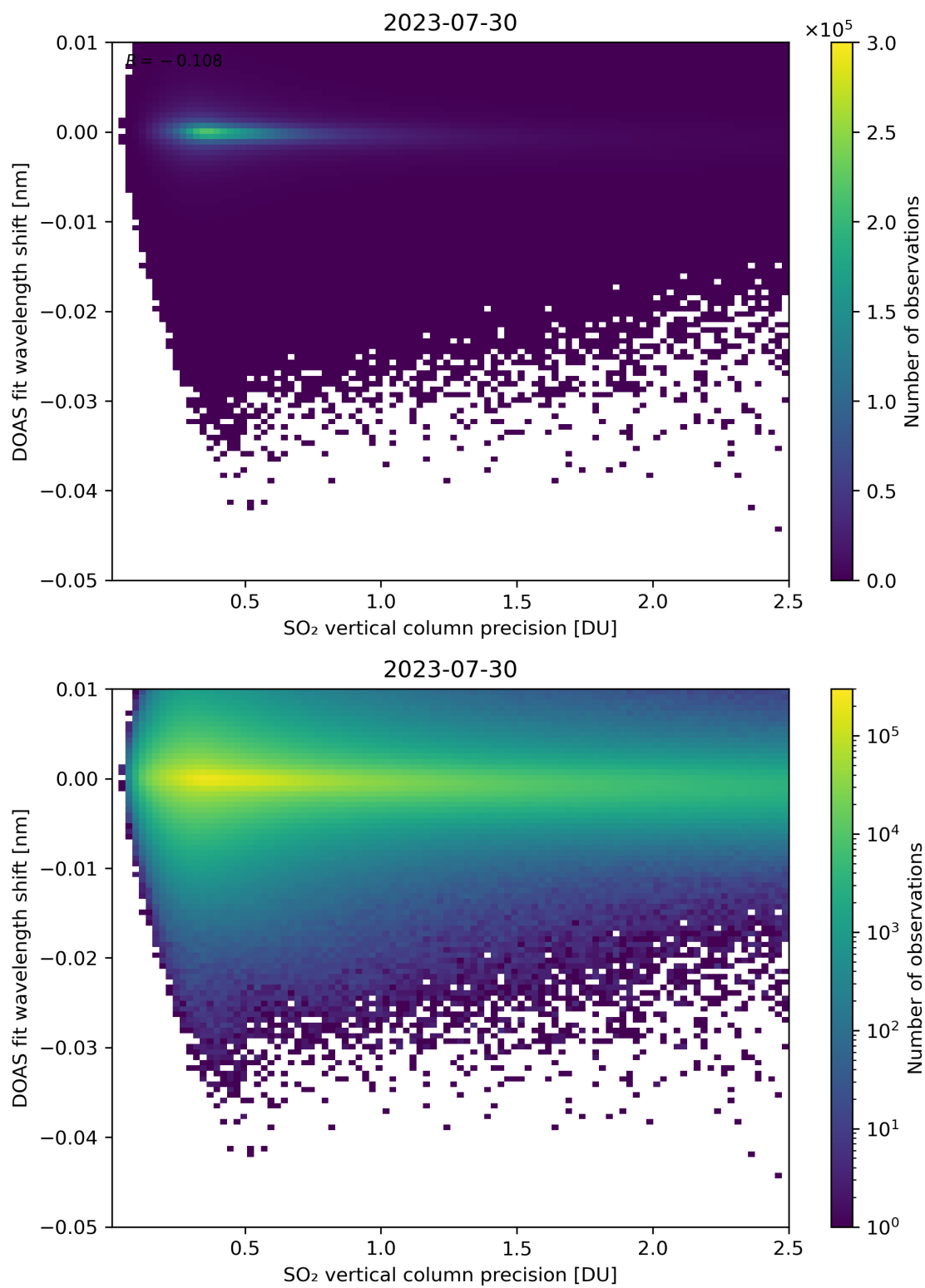
Figure 282: Scatter density plot of “SO 2 vertical column precision” against “DOAS fit wavelength shift” for 2023-07-29 to 2023-07-31.
