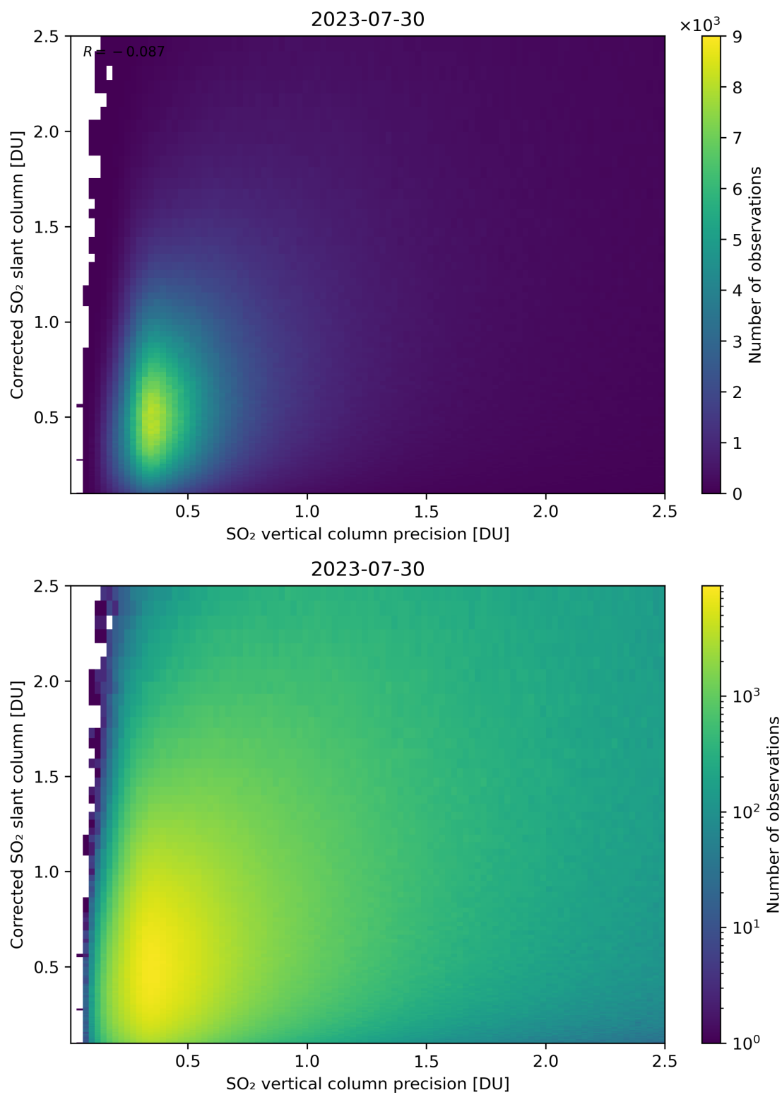
Figure 286: Scatter density plot of “SO 2 vertical column precision” against “Corrected SO 2 slant column” for 2023-07-29 to 2023-07-31.
