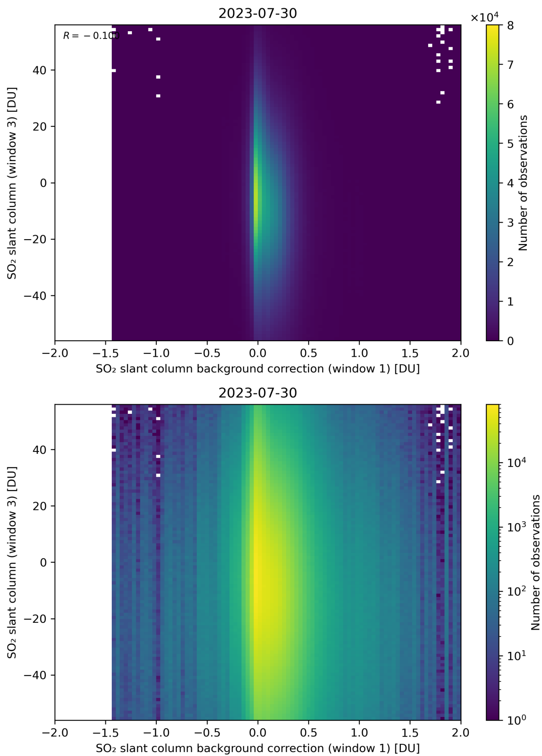
Figure 107: Scatter density plot of “SO 2 slant column background correction (window 1)” against “SO 2 slant column (window 3)” for 2023-07-29 to 2023-07-31.
