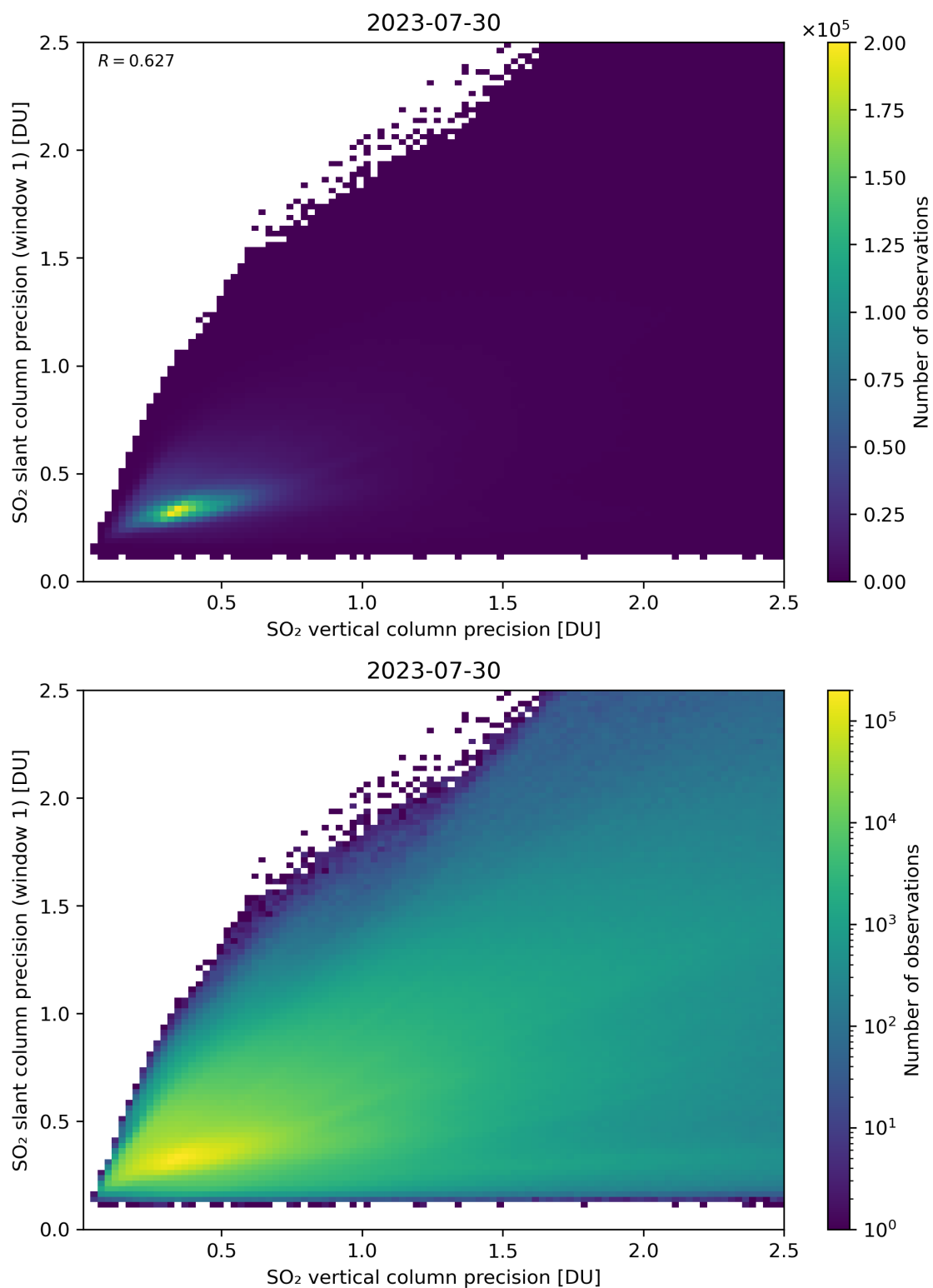
Figure 290: Scatter density plot of “SO 2 vertical column precision” against “SO 2 slant column precision (window 1)” for 2023-07-29 to 2023-07-31.
