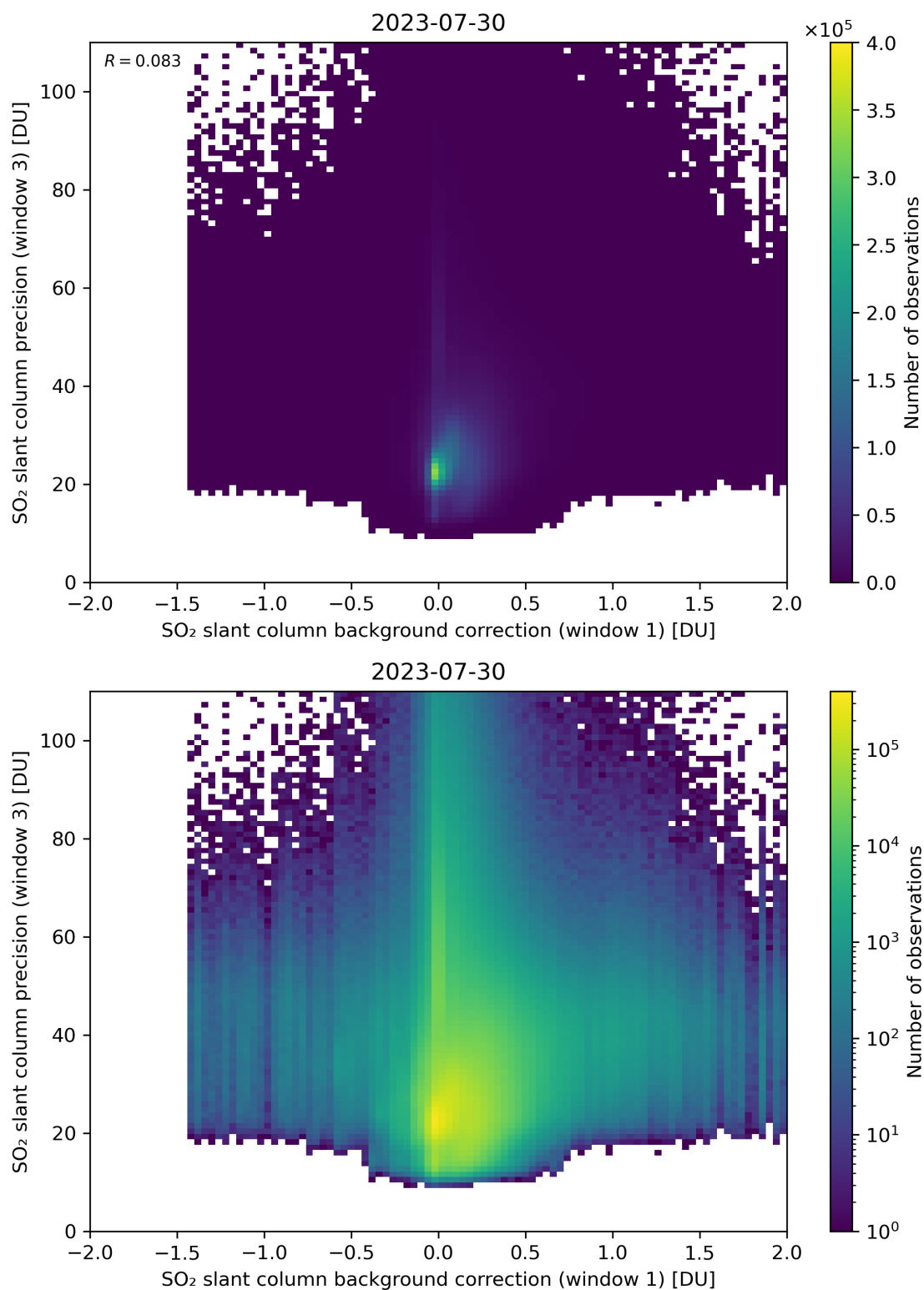
Figure 108: Scatter density plot of “SO 2 slant column background correction (window 1)” against “SO 2 slant column precision (window 3)” for 2023-07-29 to 2023-07-31.
