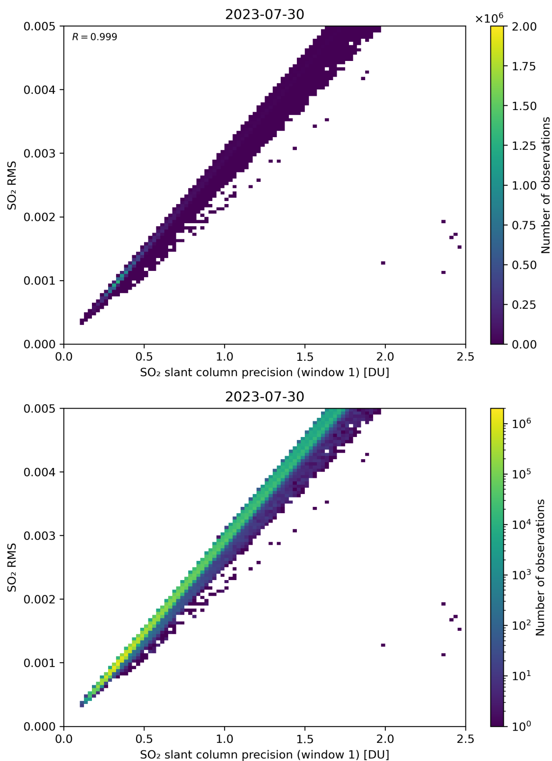
Figure 223: Scatter density plot of “SO 2 slant column precision (window 1)” against “SO 2 RMS” for 2023-07-29 to 2023-07-31.
