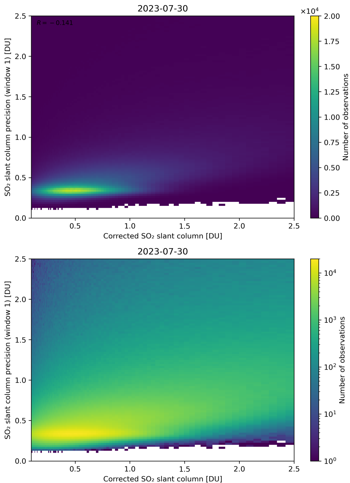
Figure 188: Scatter density plot of “Corrected SO 2 slant column” against “SO 2 slant column precision (window 1)” for 2023-07-29 to 2023-07-31.
