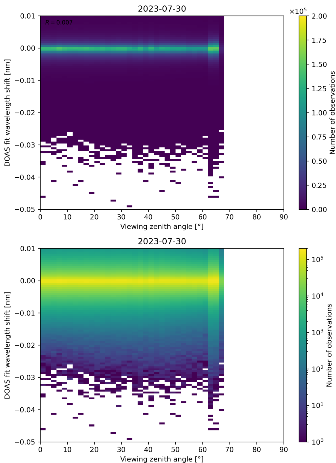
Figure 311: Scatter density plot of “Viewing zenith angle” against “DOAS fit wavelength shift” for 2023-07-29 to 2023-07-31.
