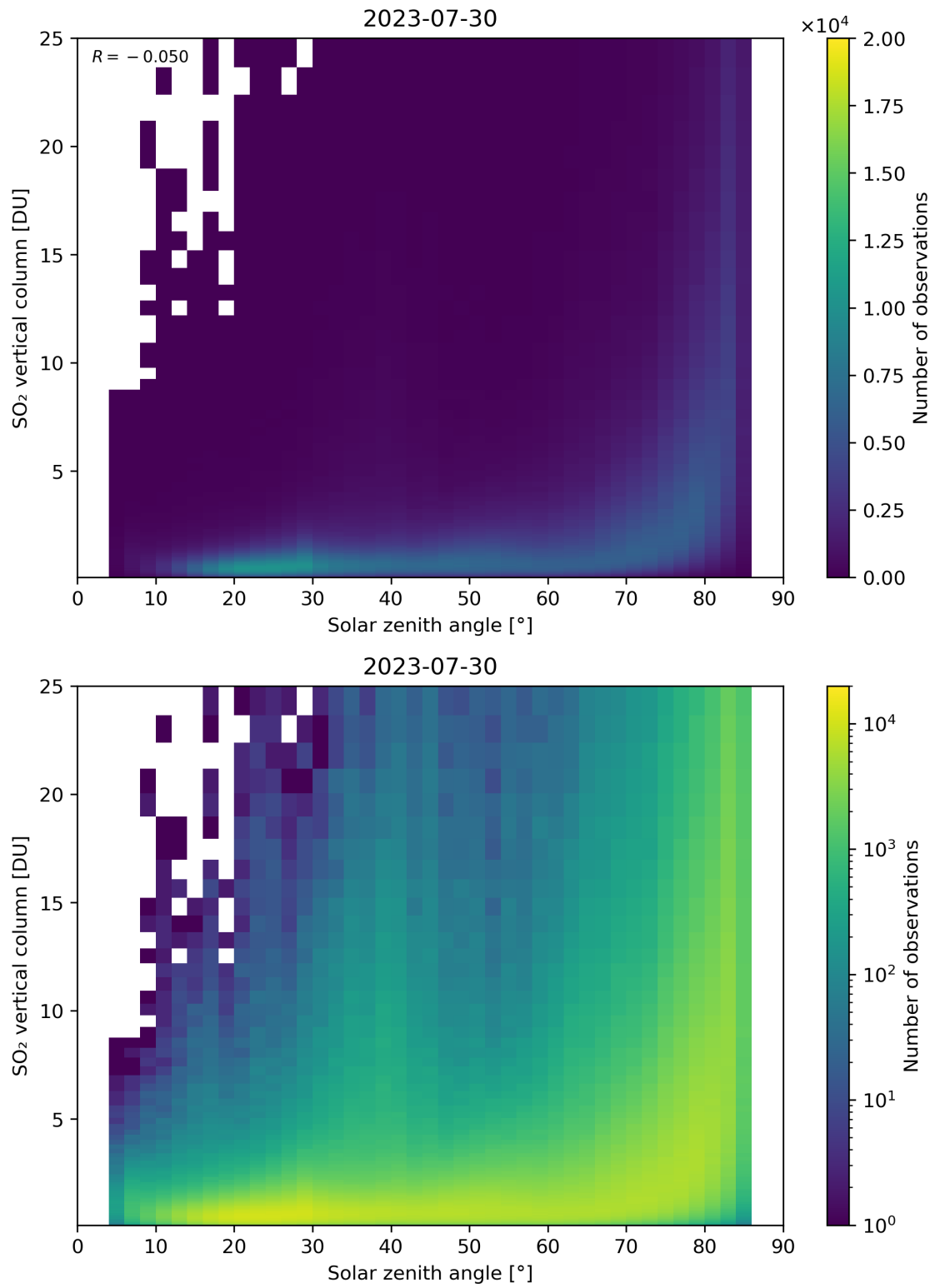
Figure 176: Scatter density plot of “Solar zenith angle” against “SO 2 vertical column” for 2023-07-29 to 2023-07-31.
