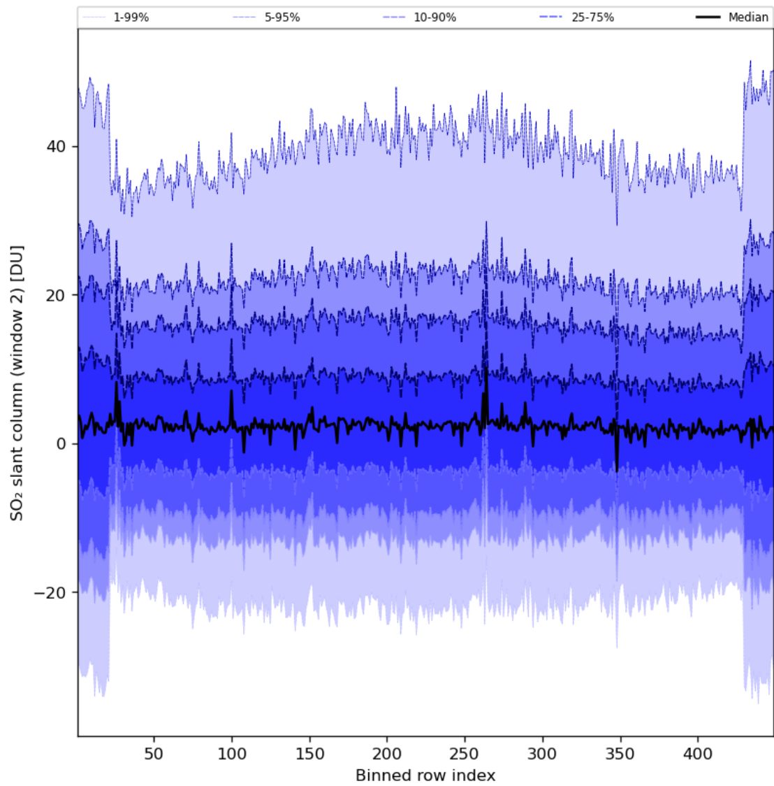
Figure 83: Along track statistics of “SO 2 slant column (window 2)” for 2023-07-29 to 2023-07-31
