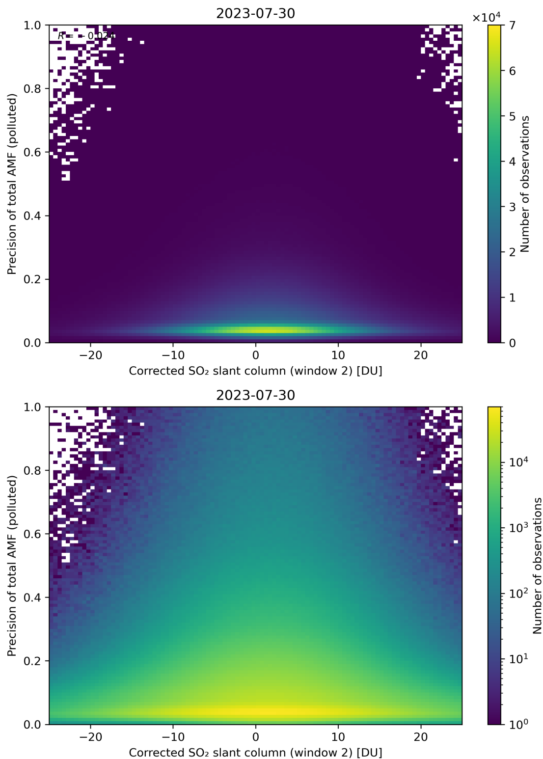
Figure 204: Scatter density plot of “Corrected SO 2 slant column (window 2)” against “Precision of total AMF (polluted)” for 2023-07-29 to 2023-07-31.
