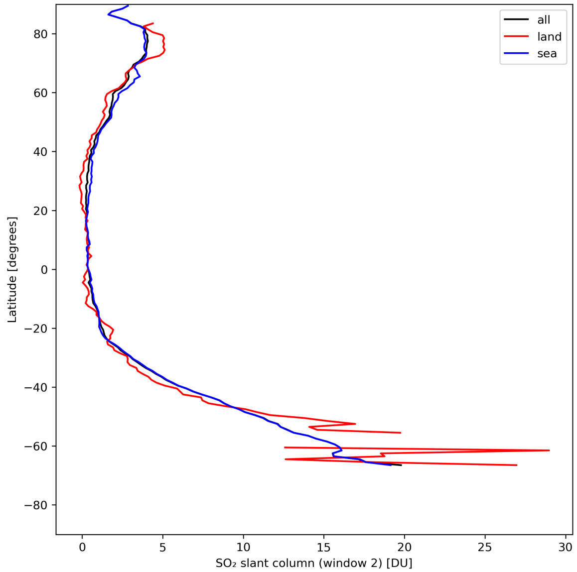
Figure 37: Zonal average of “SO 2 slant column (window 2)” for 2023-07-29 to 2023-07-31.
