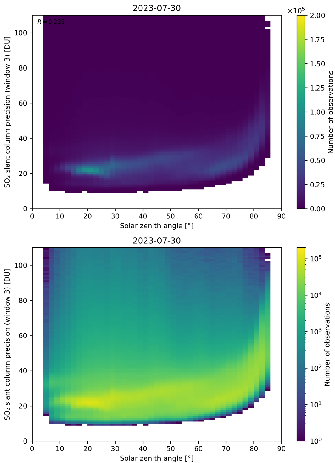
Figure 173: Scatter density plot of “Solar zenith angle” against “SO 2 slant column precision (window 3)” for 2023-07-29 to 2023-07-31.
