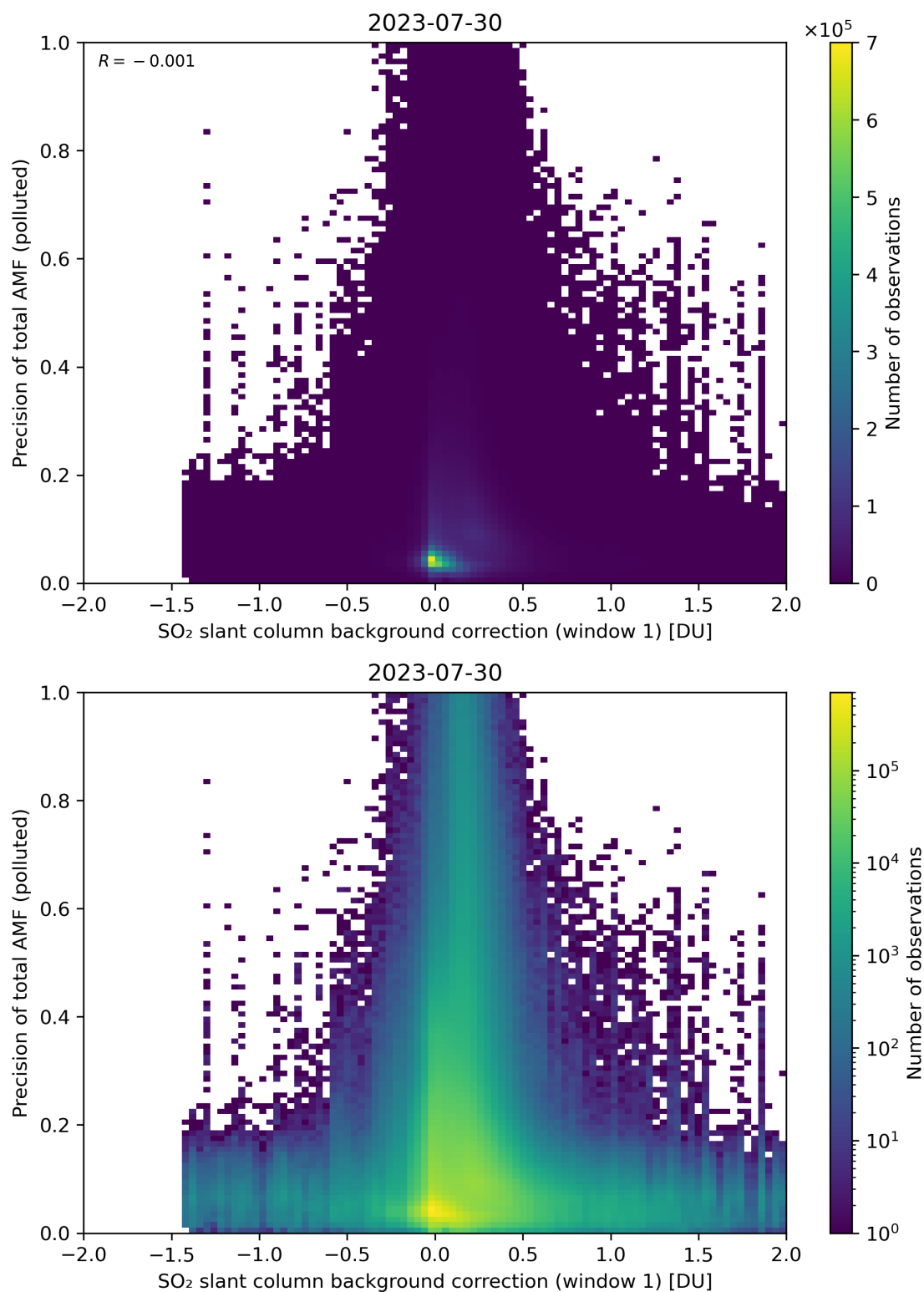
Figure 110: Scatter density plot of “SO 2 slant column background correction (window 1)” against “Precision of total AMF (polluted)” for 2023-07-29 to 2023-07-31.
