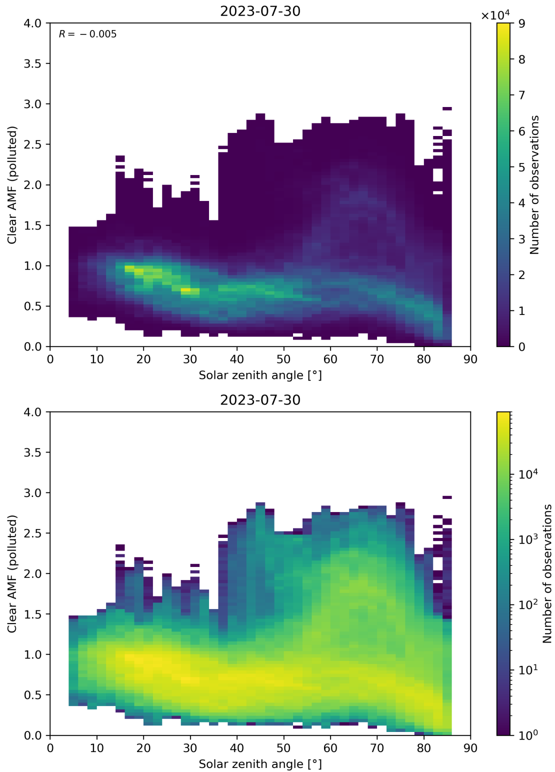
Figure 165: Scatter density plot of “Solar zenith angle” against “Clear AMF (polluted)” for 2023-07-29 to 2023-07-31.
