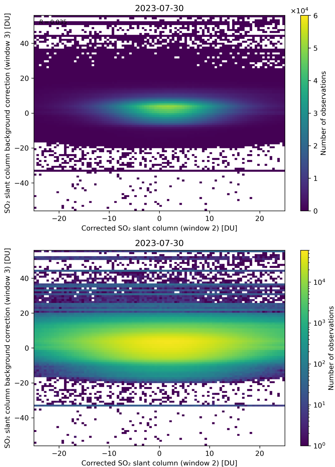
Figure 195: Scatter density plot of “Corrected SO 2 slant column (window 2)” against “SO 2 slant column background correction (window 3)” for 2023-07-29 to 2023-07-31.
