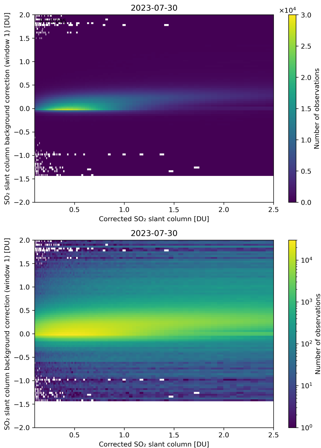
Figure 178: Scatter density plot of “Corrected SO 2 slant column” against “SO 2 slant column background correction (window 1)” for 2023-07-29 to 2023-07-31.
