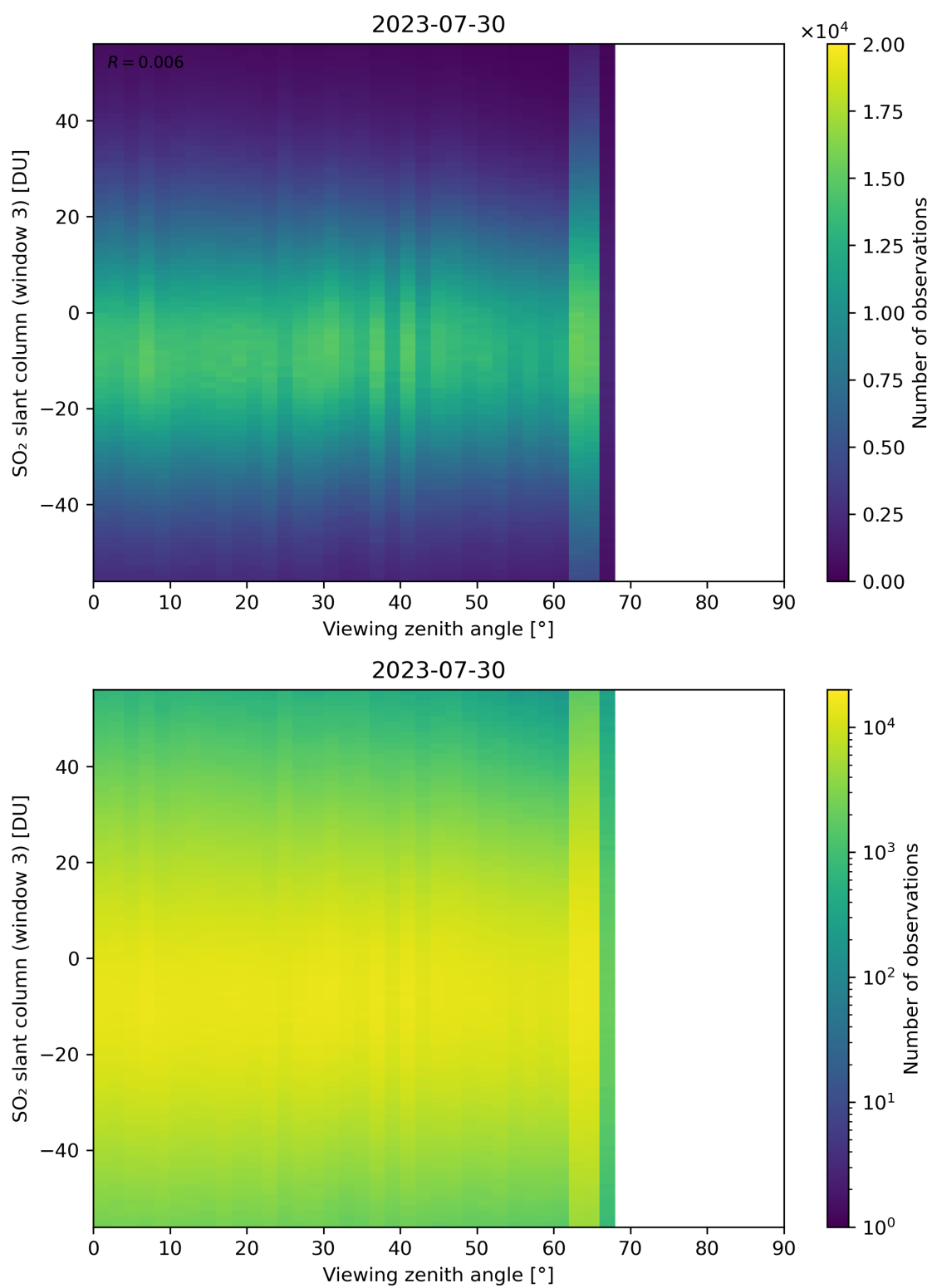
Figure 323: Scatter density plot of “Viewing zenith angle” against “SO 2 slant column (window 3)” for 2023-07-29 to 2023-07-31.
