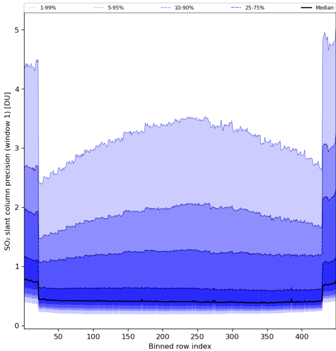
Figure 80: Along track statistics of “SO 2 slant column precision (window 1)” for 2023-07-29 to 2023-07-31
