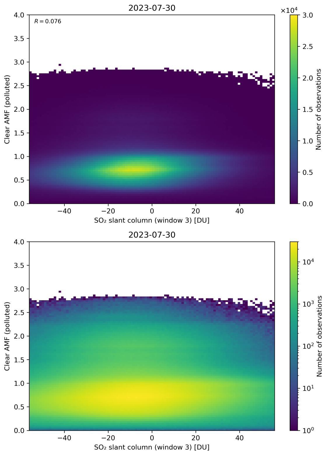
Figure 265: Scatter density plot of “SO 2 slant column (window 3)” against “Clear AMF (polluted)” for 2023-07-29 to 2023-07-31.
