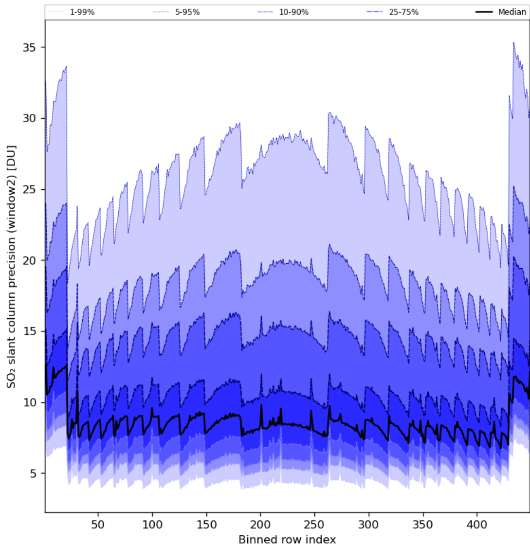
Figure 84: Along track statistics of “SO 2 slant column precision (window2)” for 2023-07-29 to 2023-07-31
