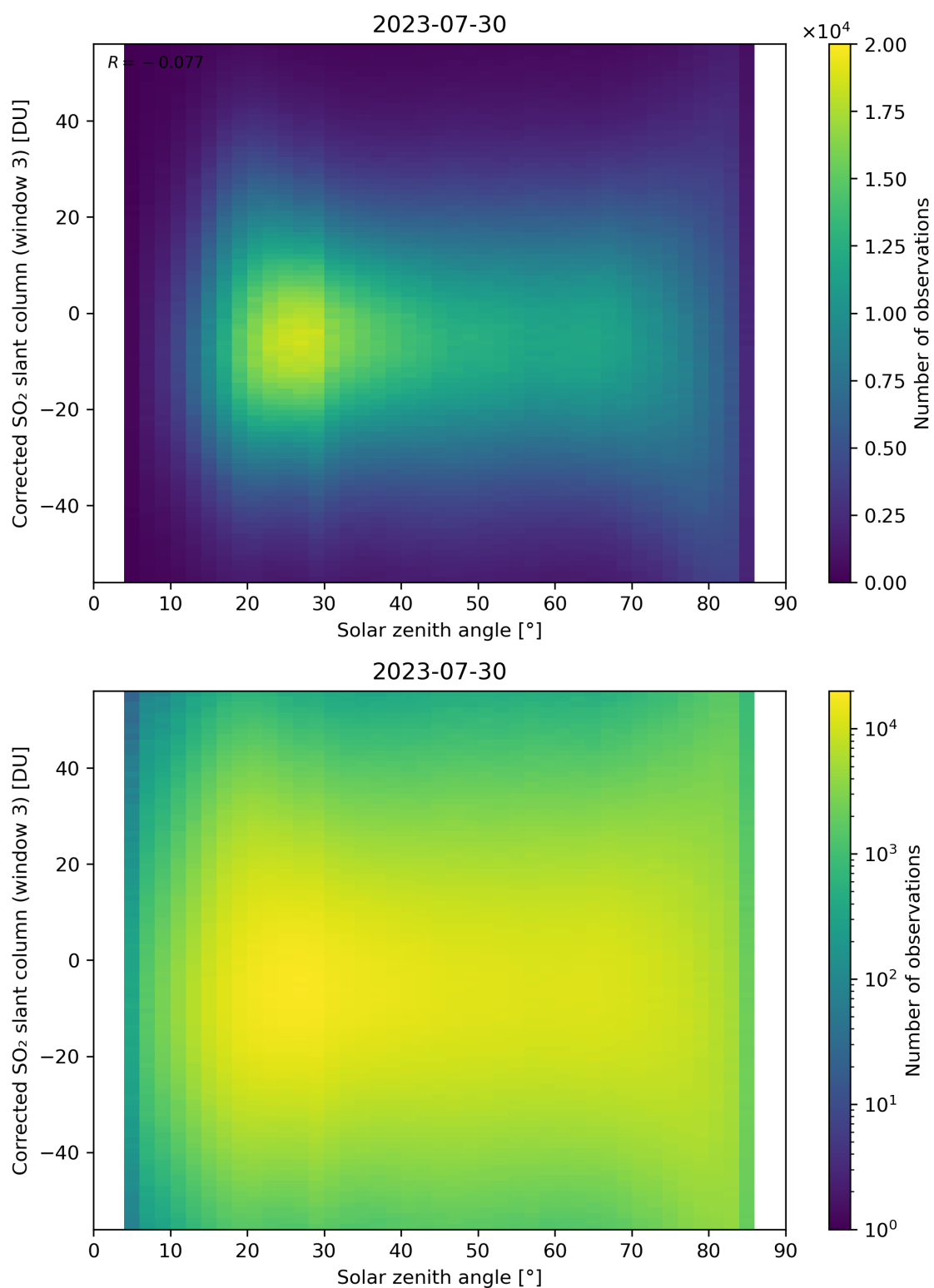
Figure 168: Scatter density plot of “Solar zenith angle” against “Corrected SO 2 slant column (window 3)” for 2023-07-29 to 2023-07-31.
