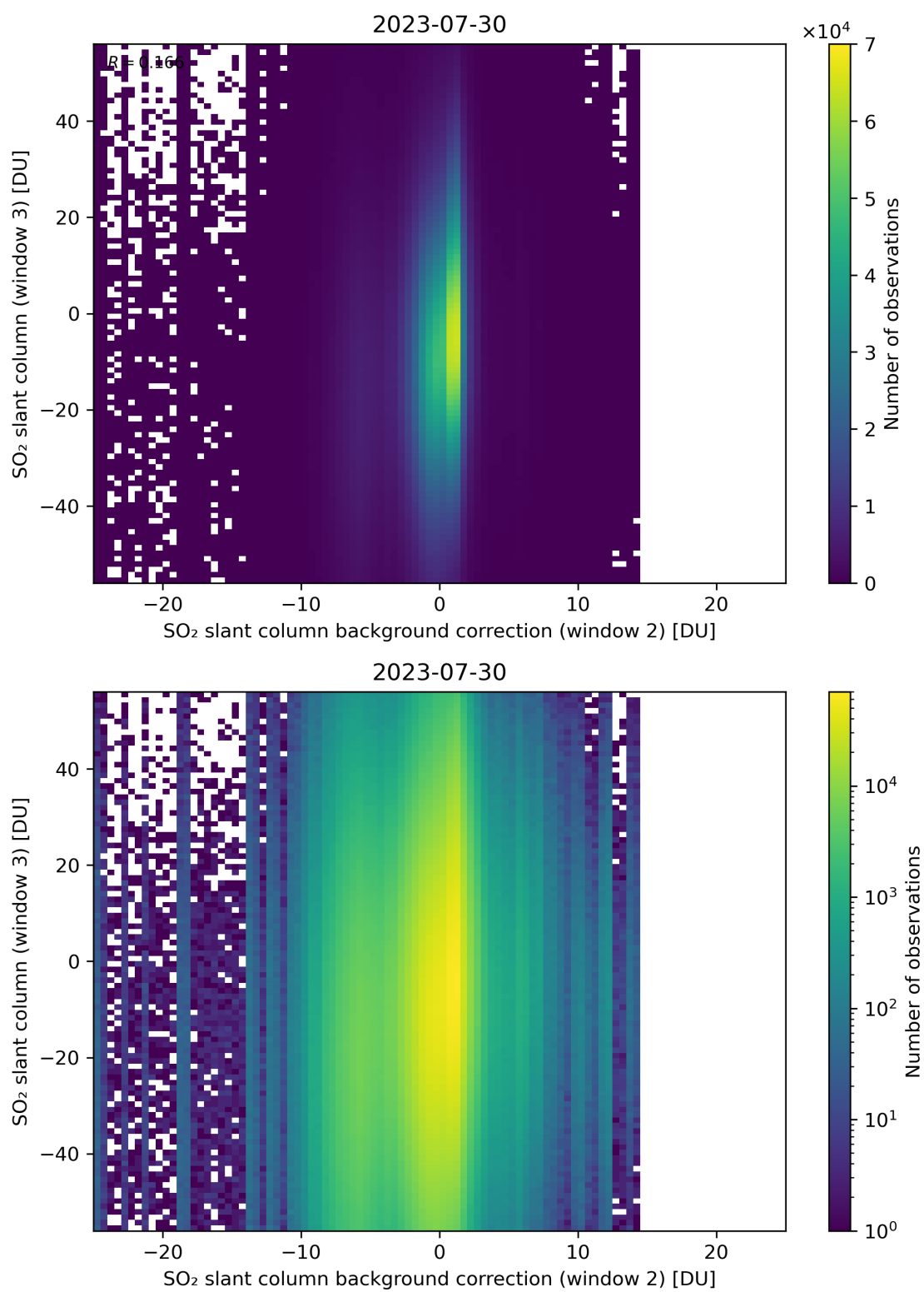
Figure 117: Scatter density plot of “SO 2 slant column background correction (window 2)” against “SO 2 slant column (window 3)” for 2023-07-29 to 2023-07-31.
