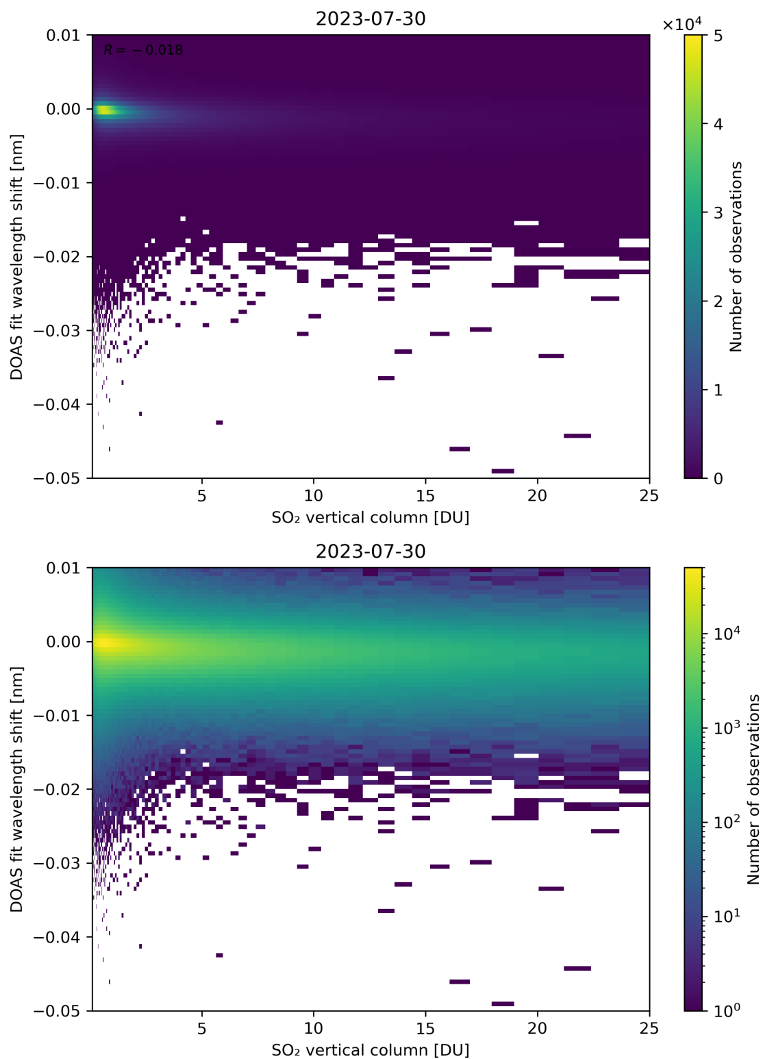
Figure 276: Scatter density plot of “SO 2 vertical column” against “DOAS fit wavelength shift” for 2023-07-29 to 2023-07-31.
