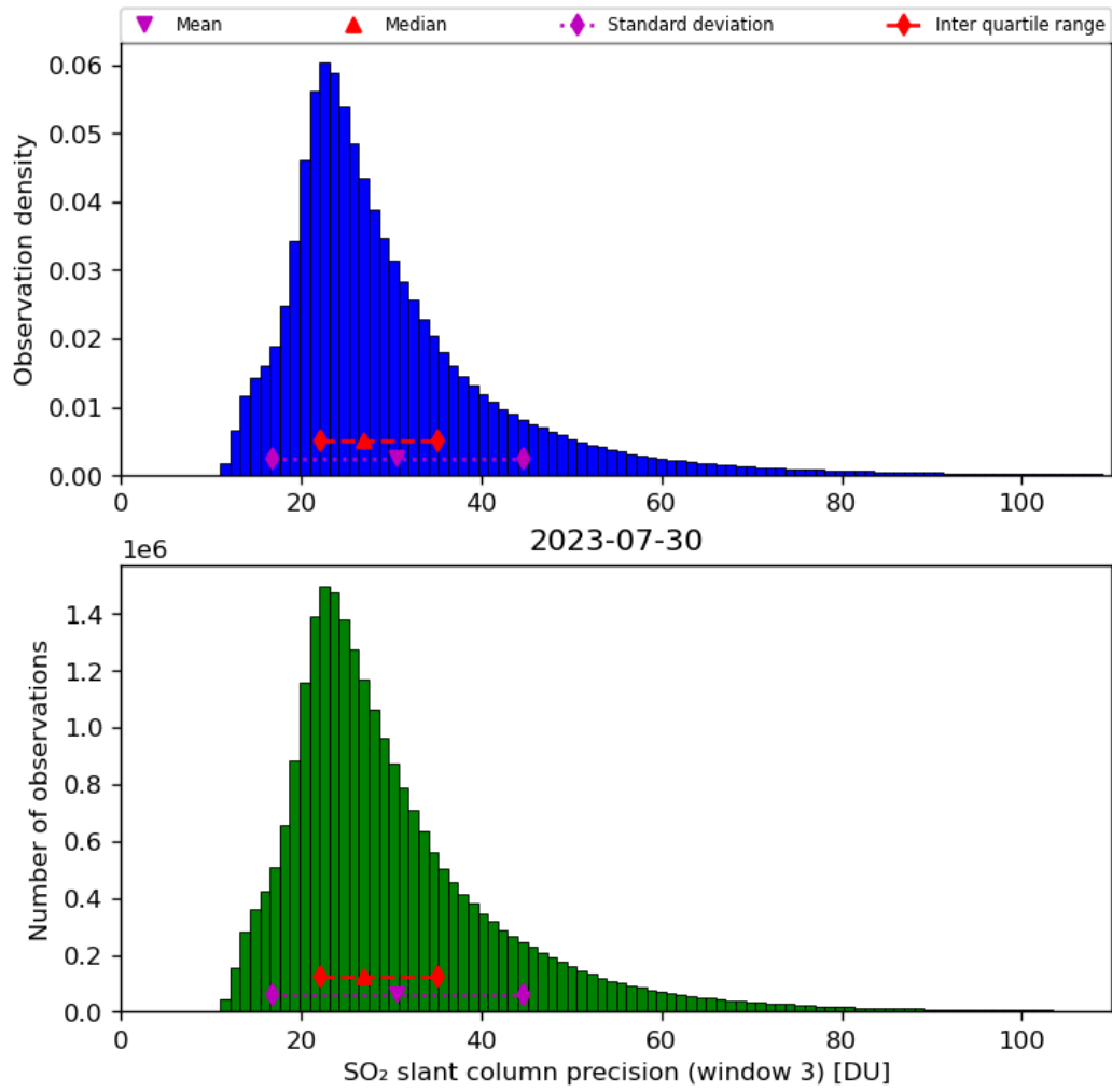
Figure 65: Histogram of “SO 2 slant column precision (window 3)” for 2023-07-29 to 2023-07-31
