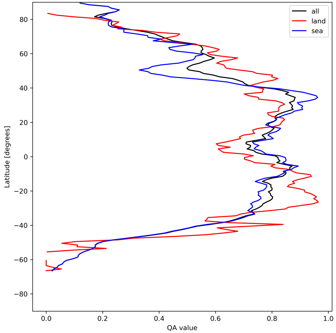
Figure 29: Zonal average of “QA value” for 2023-07-29 to 2023-07-31.
