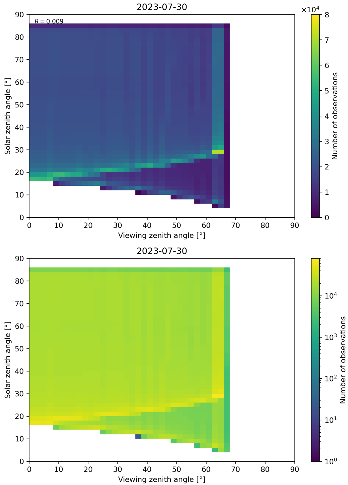
Figure 315: Scatter density plot of “Viewing zenith angle” against “Solar zenith angle” for 2023-07-29 to 2023-07-31.
