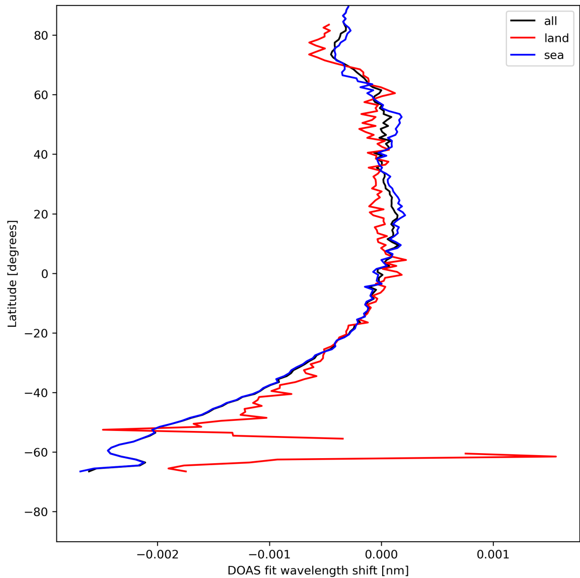
Figure 45: Zonal average of “DOAS fit wavelength shift” for 2023-07-29 to 2023-07-31.
