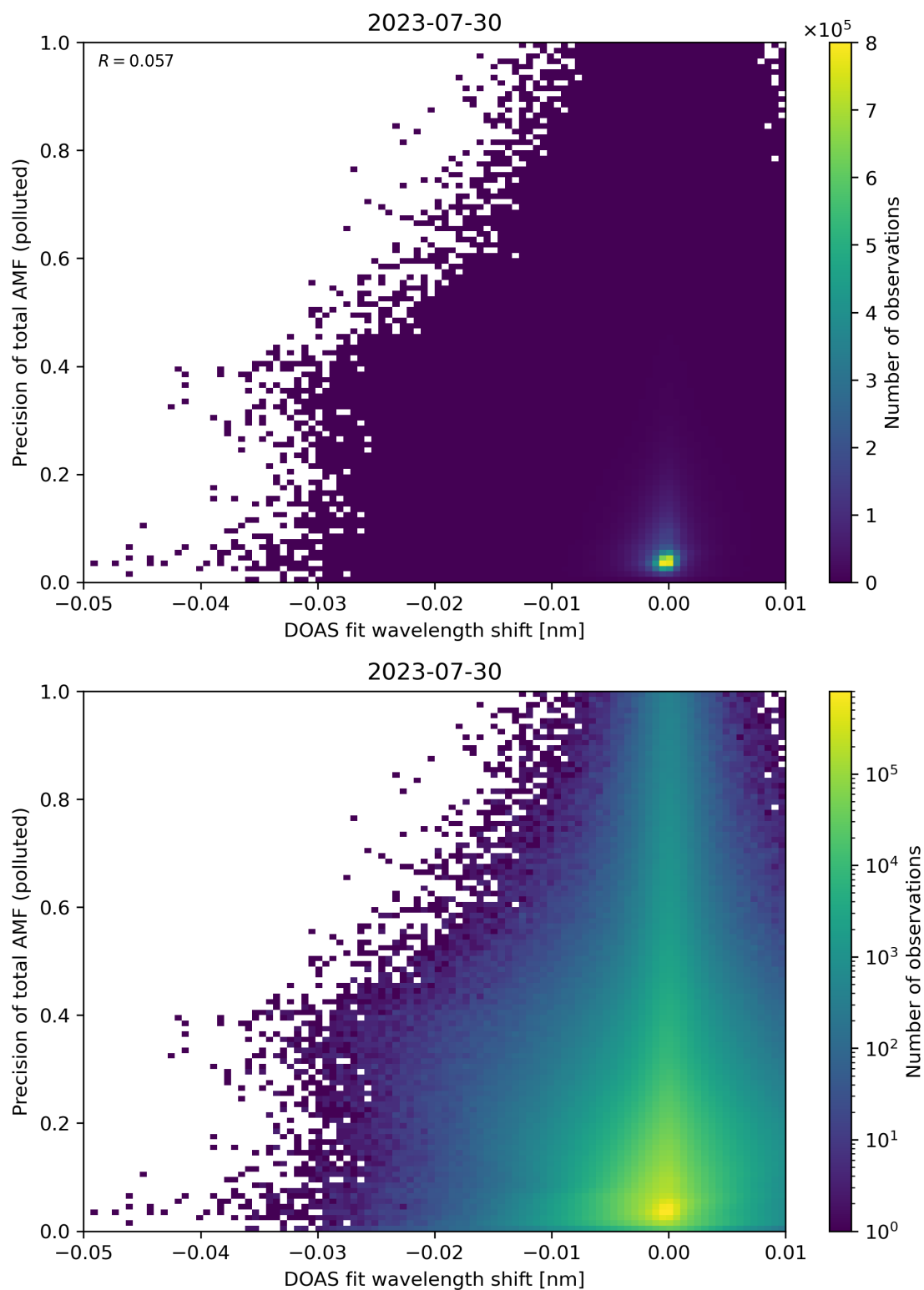
Figure 131: Scatter density plot of “DOAS fit wavelength shift” against “Precision of total AMF (polluted)” for 2023-07-29 to 2023-07-31.
