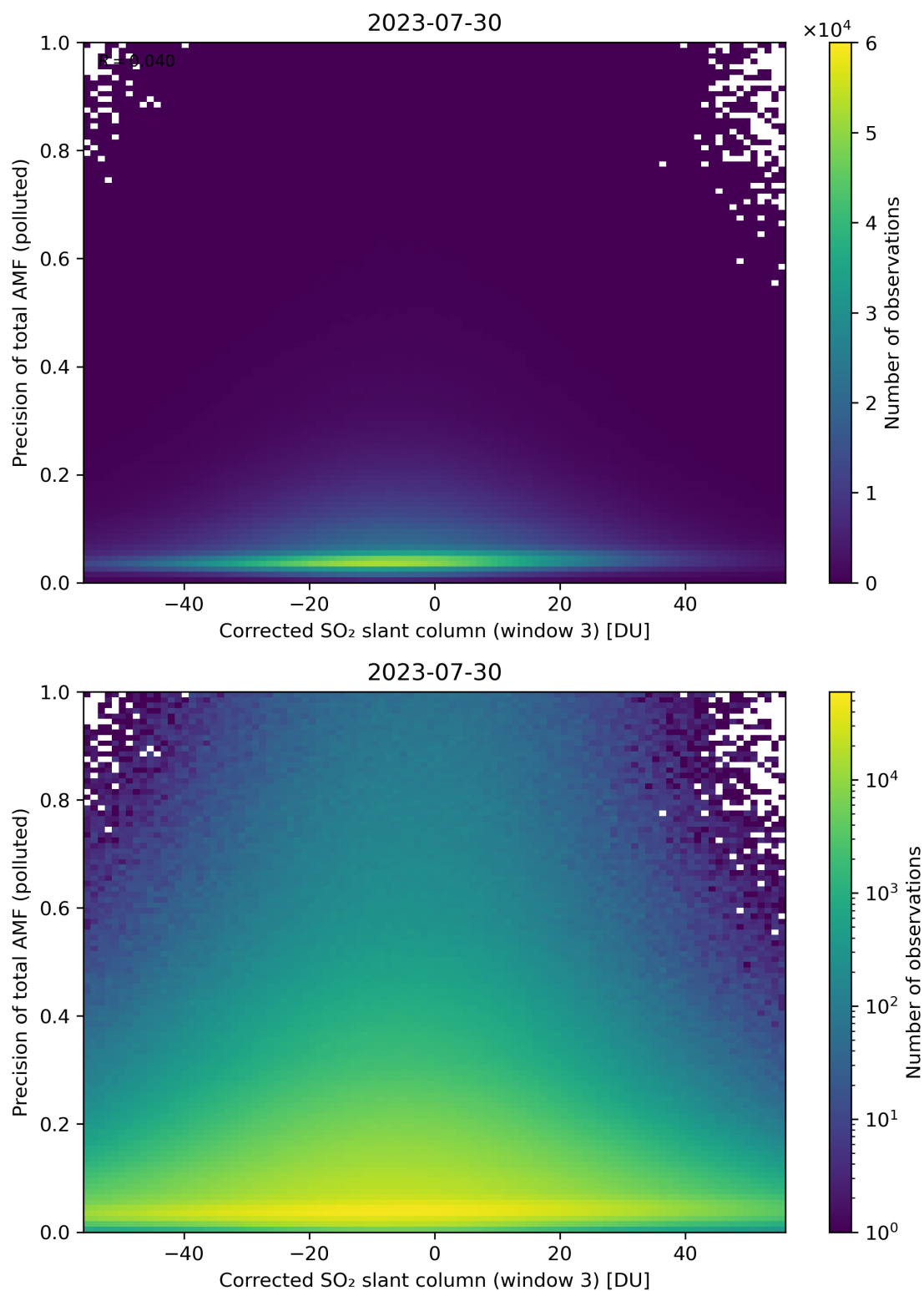
Figure 211: Scatter density plot of “Corrected SO 2 slant column (window 3)” against “Precision of total AMF (polluted)” for 2023-07-29 to 2023-07-31.
