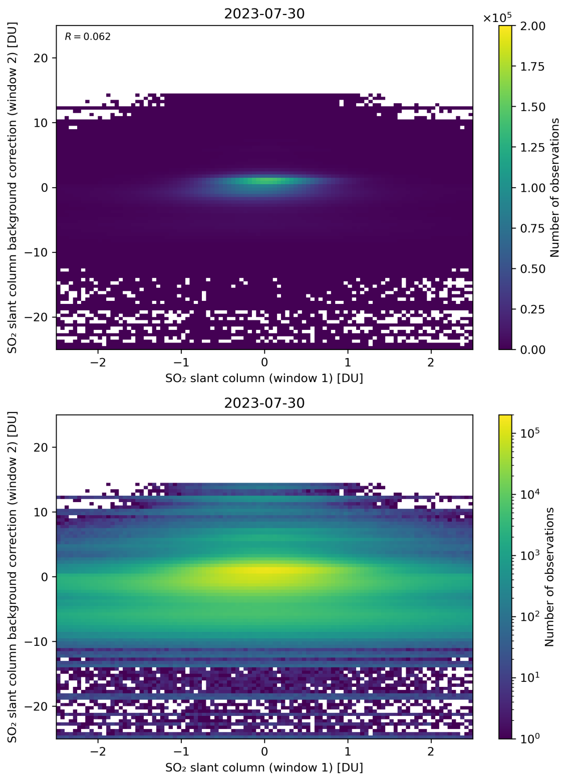
Figure 213: Scatter density plot of “SO 2 slant column (window 1)” against “SO 2 slant column background correction (window 2)” for 2023-07-29 to 2023-07-31.
