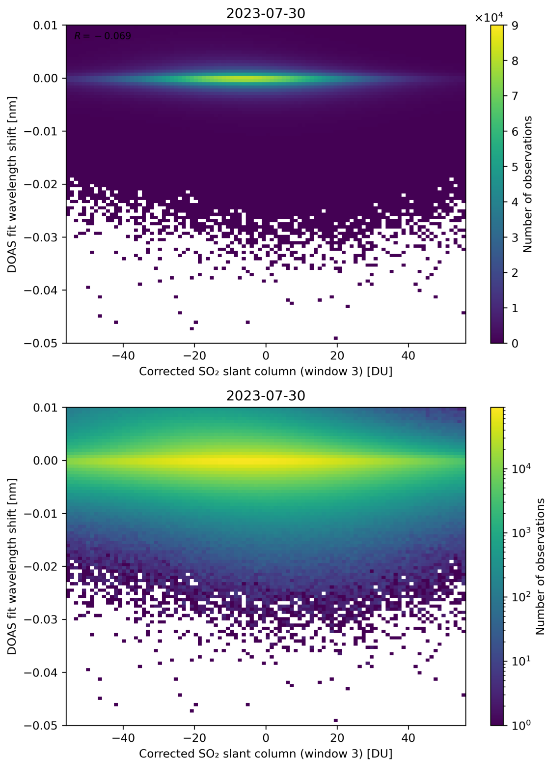
Figure 206: Scatter density plot of “Corrected SO 2 slant column (window 3)” against “DOAS fit wavelength shift” for 2023-07-29 to 2023-07-31.
