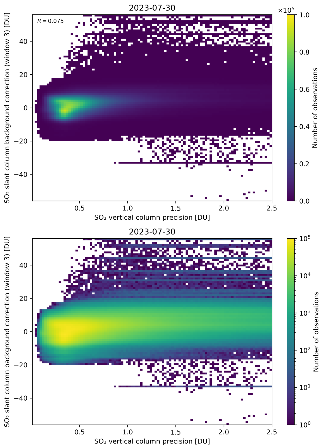
Figure 281: Scatter density plot of “SO 2 vertical column precision” against “SO 2 slant column background correction (window 3)” for 2023-07-29 to 2023-07-31.
