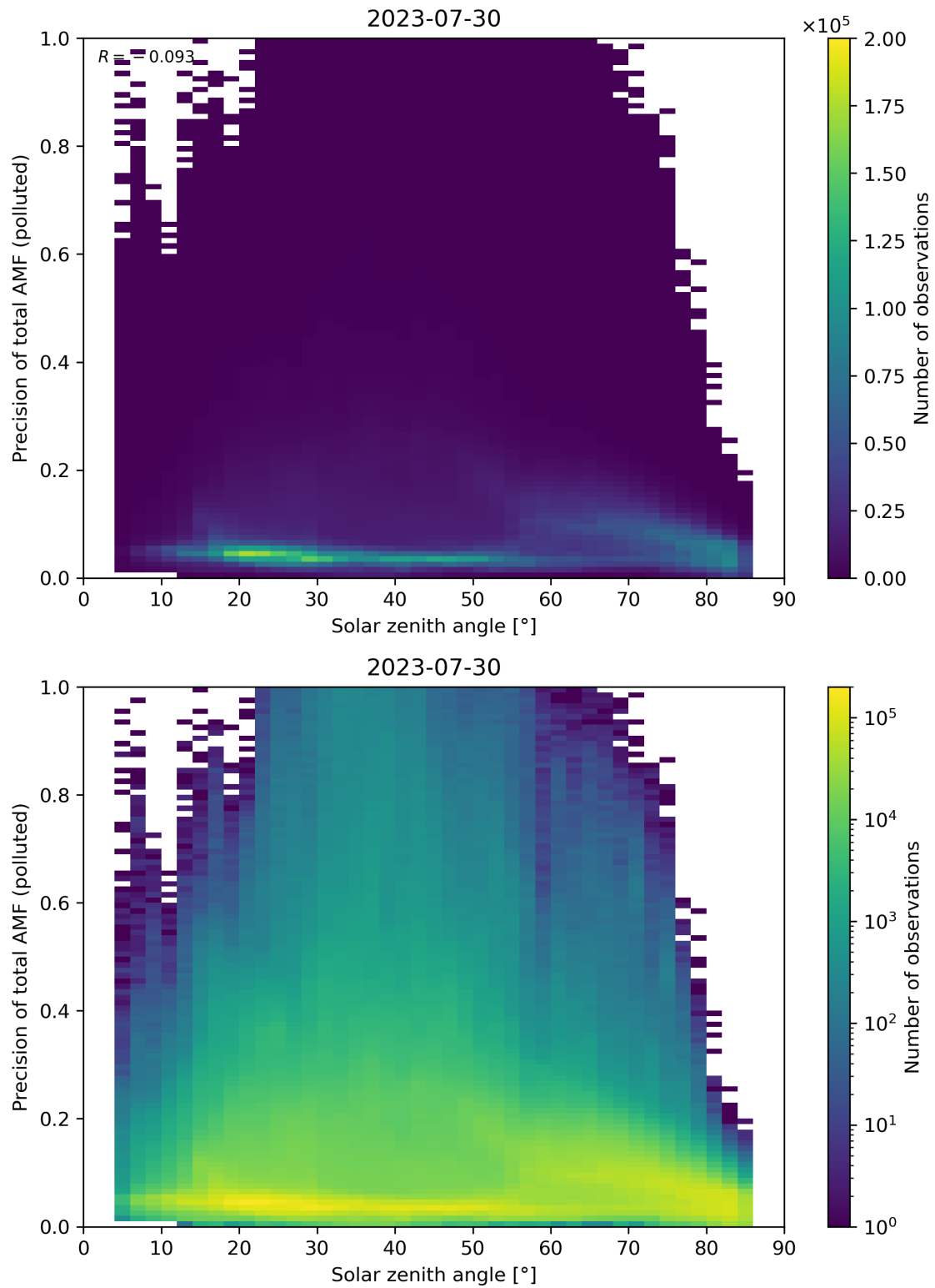
Figure 175: Scatter density plot of “Solar zenith angle” against “Precision of total AMF (polluted)” for 2023-07-29 to 2023-07-31.
