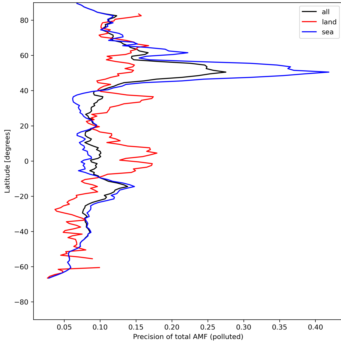
Figure 49: Zonal average of “Precision of total AMF (polluted)” for 2023-07-29 to 2023-07-31.
