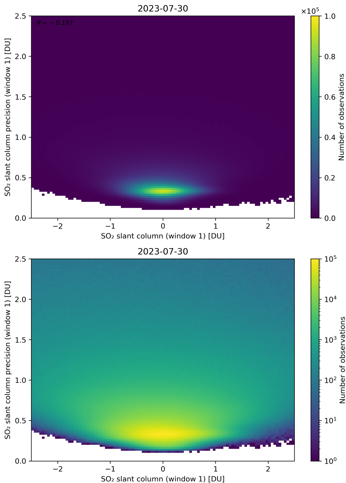
Figure 235: Scatter density plot of “SO 2 slant column (window 1)” against “SO 2 slant column precision (window 1)” for 2023-07-29 to 2023-07-31.
