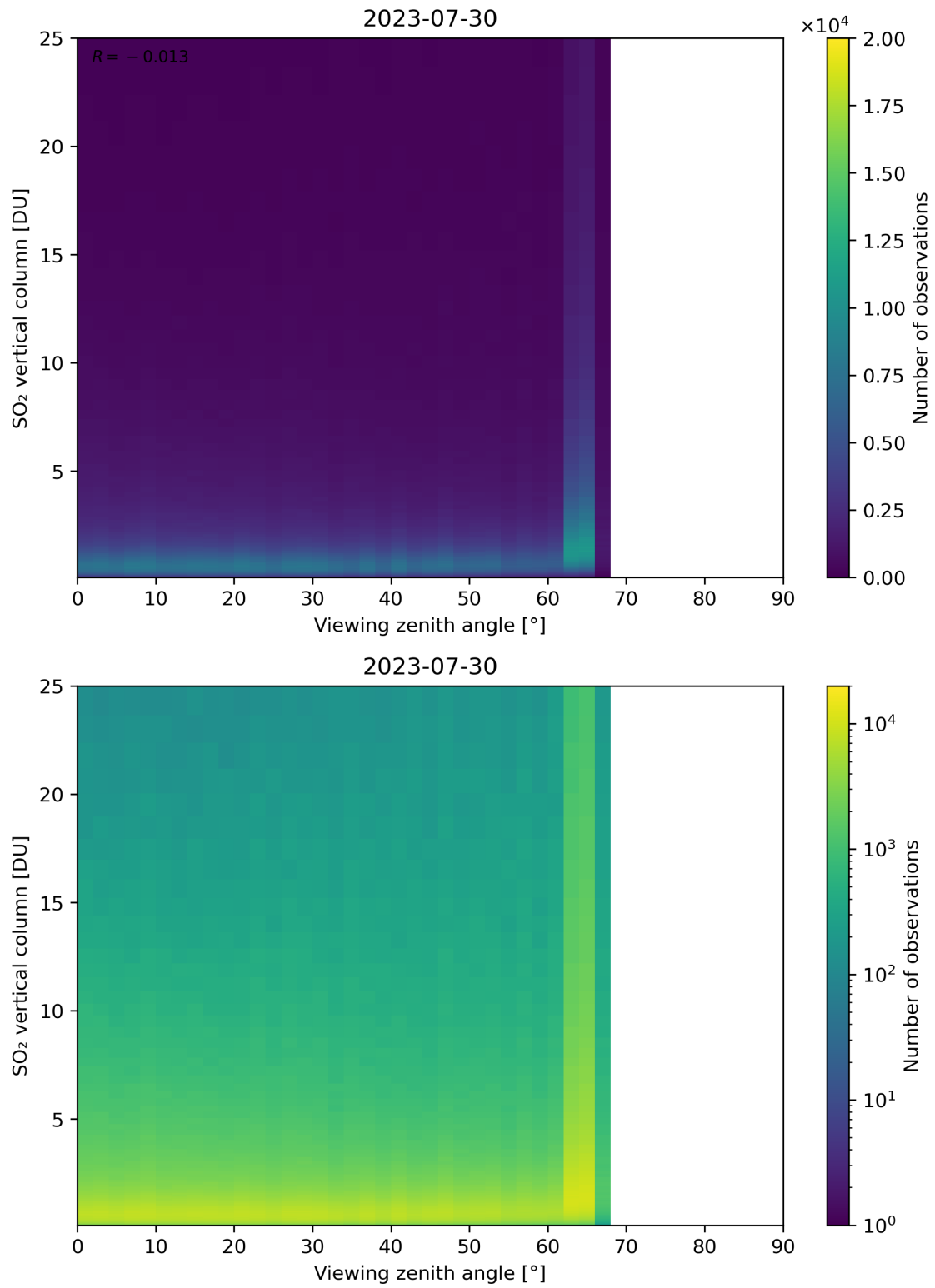
Figure 327: Scatter density plot of “Viewing zenith angle” against “SO 2 vertical column” for 2023-07-29 to 2023-07-31.
