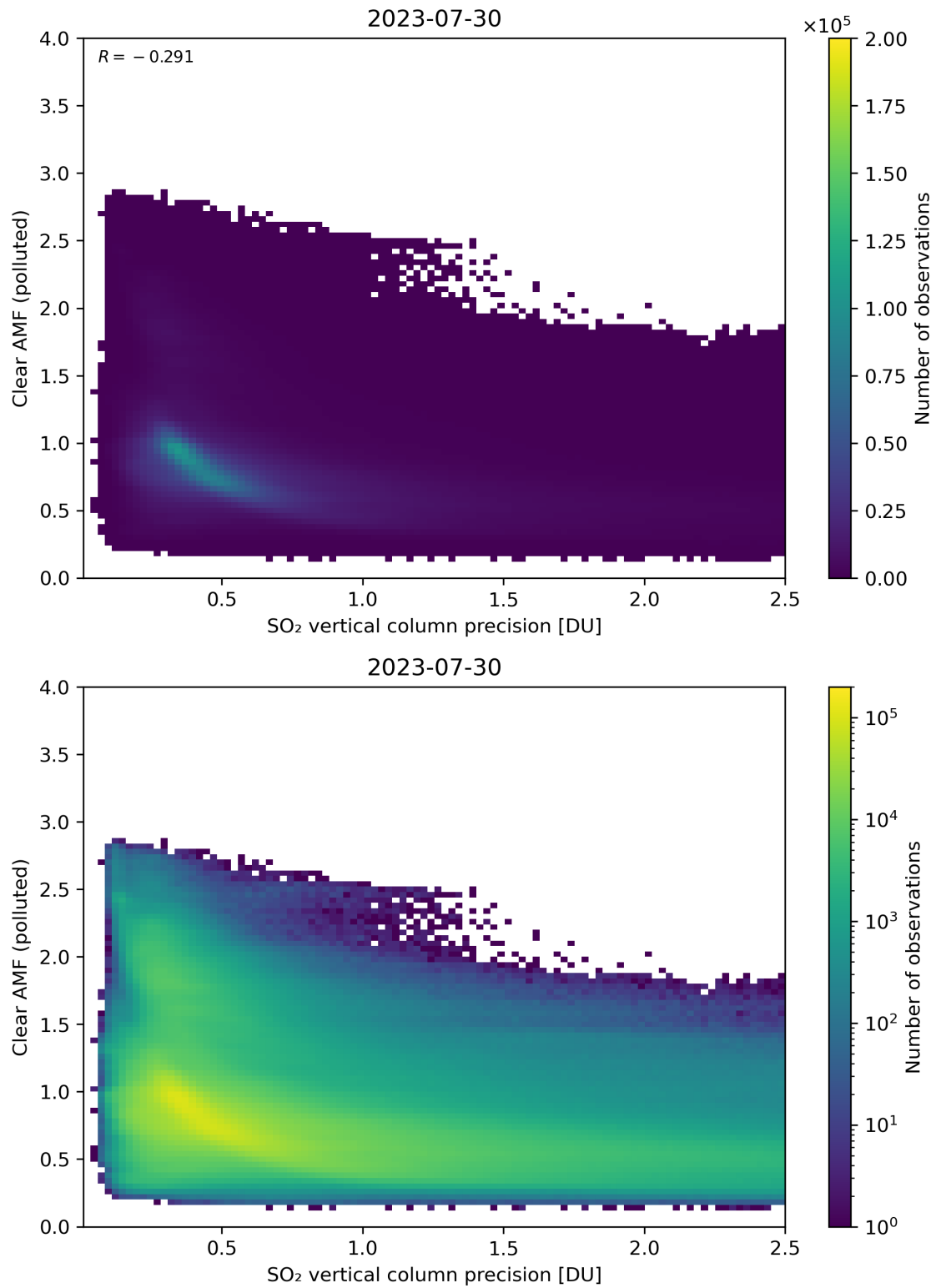
Figure 285: Scatter density plot of “SO 2 vertical column precision” against “Clear AMF (polluted)” for 2023-07-29 to 2023-07-31.
