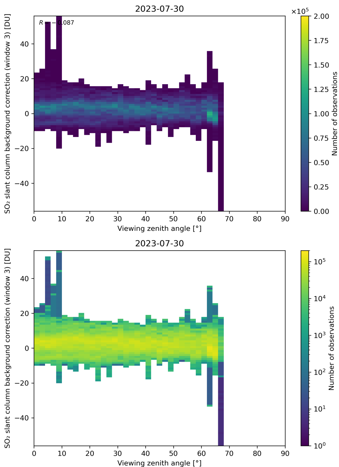
Figure 310: Scatter density plot of “Viewing zenith angle” against “SO 2 slant column background correction (window 3)” for 2023-07-29 to 2023-07-31.
