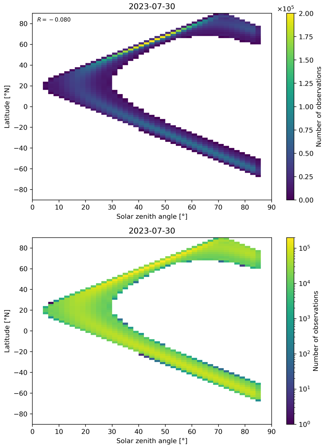
Figure 164: Scatter density plot of “Solar zenith angle” against “Latitude” for 2023-07-29 to 2023-07-31.
