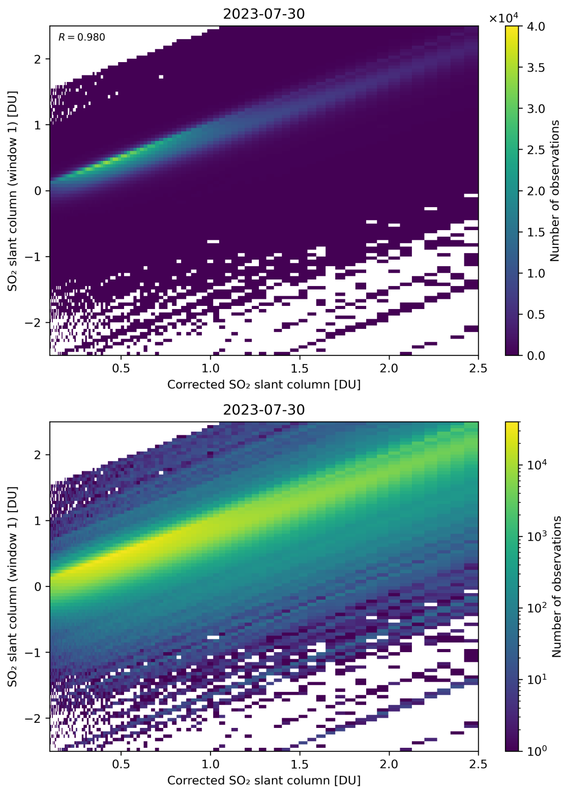
Figure 187: Scatter density plot of “Corrected SO 2 slant column” against “SO 2 slant column (window 1)” for 2023-07-29 to 2023-07-31.
