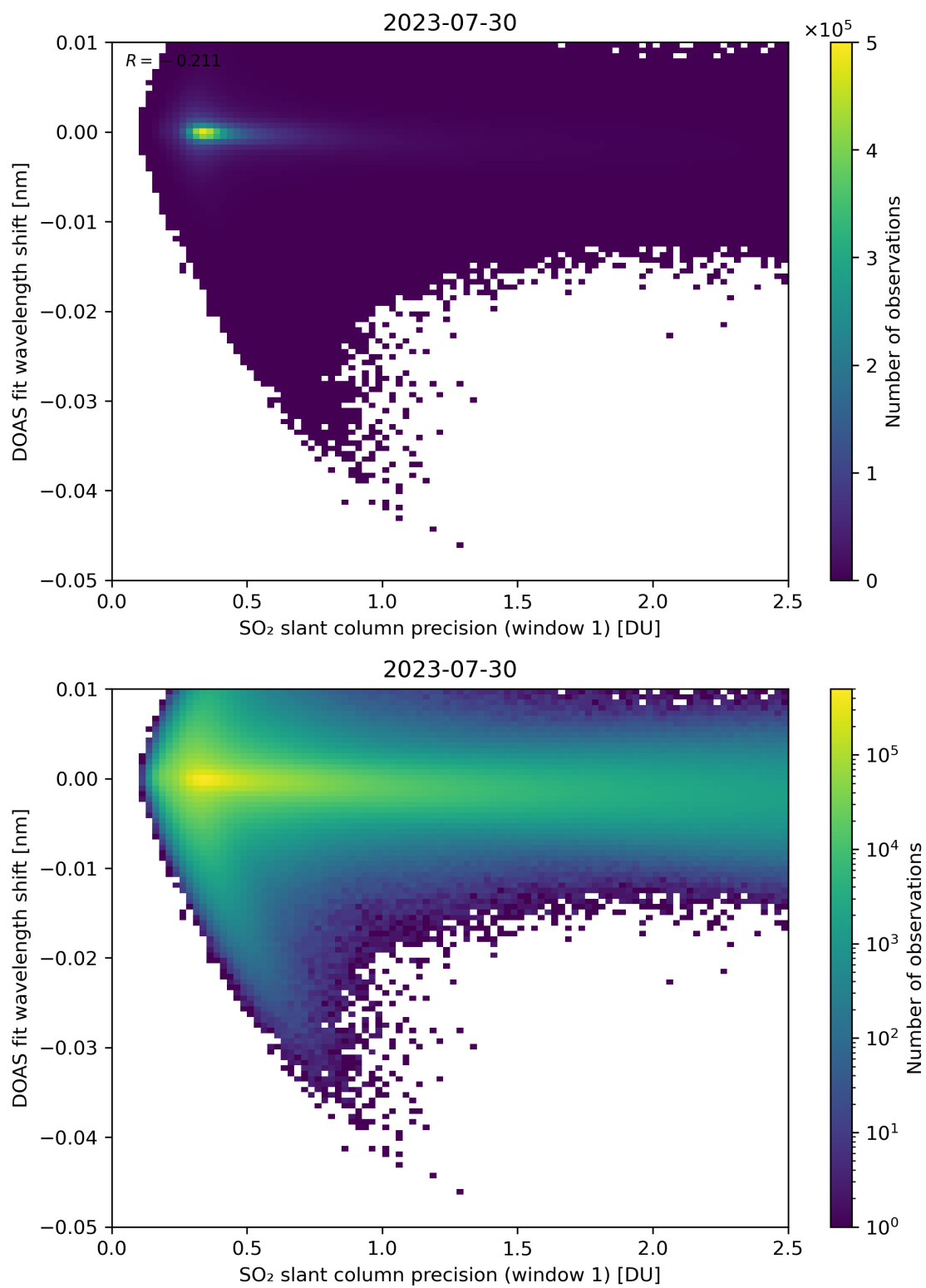
Figure 221: Scatter density plot of “SO 2 slant column precision (window 1)” against “DOAS fit wavelength shift” for 2023-07-29 to 2023-07-31.
