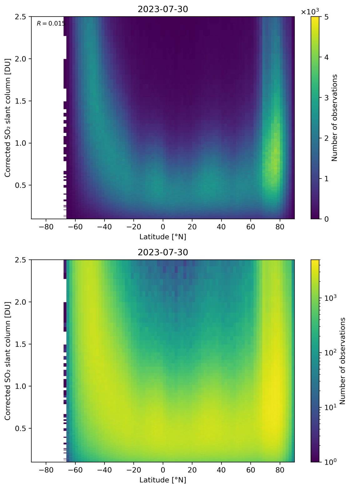
Figure 146: Scatter density plot of “Latitude” against “Corrected SO 2 slant column” for 2023-07-29 to 2023-07-31.
