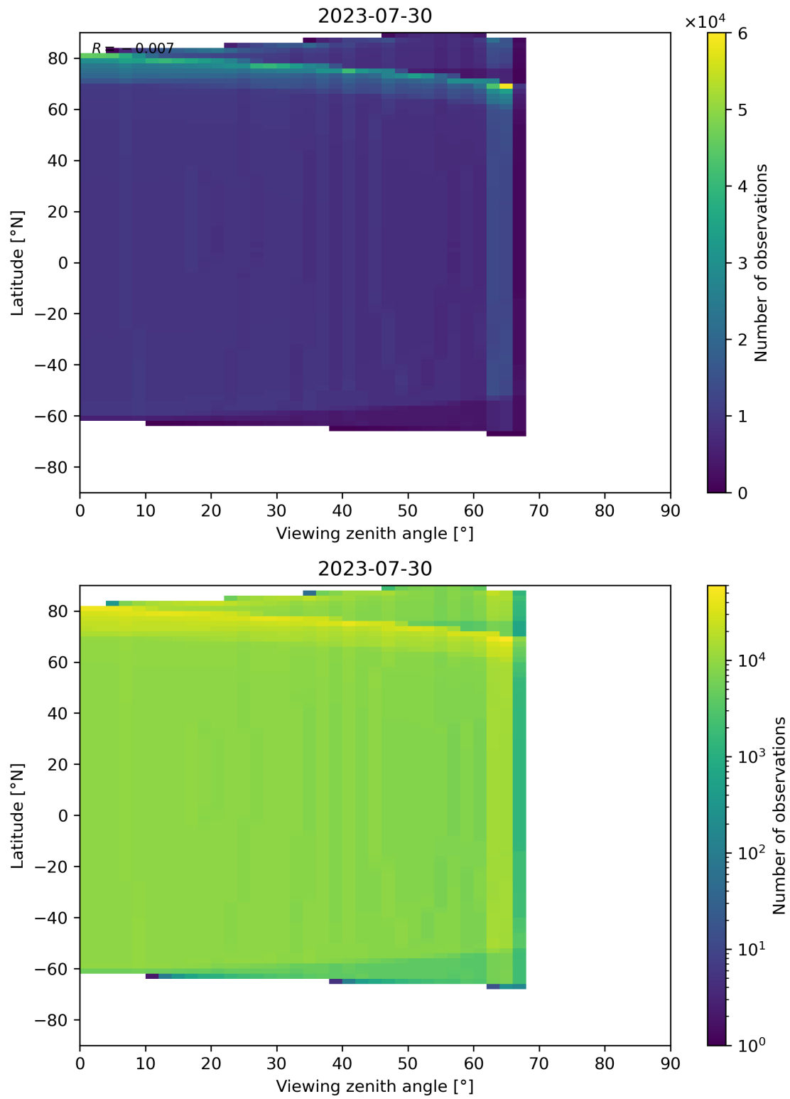
Figure 314: Scatter density plot of “Viewing zenith angle” against “Latitude” for 2023-07-29 to 2023-07-31.
