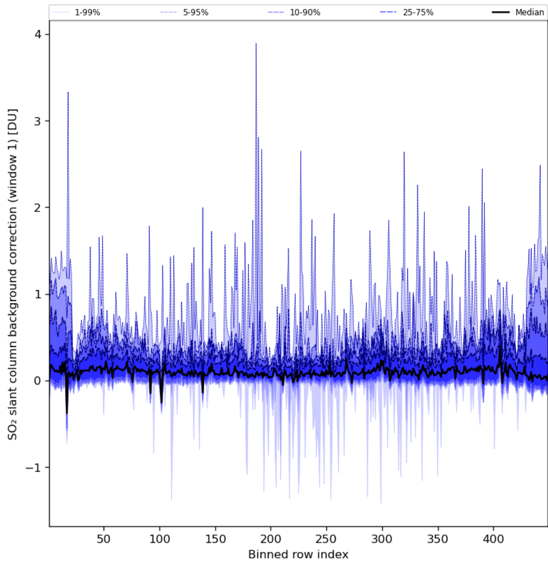
Figure 82: Along track statistics of “SO 2 slant column background correction (window 1)” for 2023-07-29 to 2023-07-31
