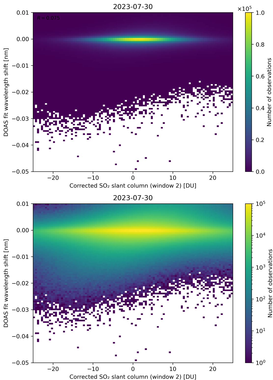
Figure 196: Scatter density plot of “Corrected SO 2 slant column (window 2)” against “DOAS fit wavelength shift” for 2023-07-29 to 2023-07-31.
