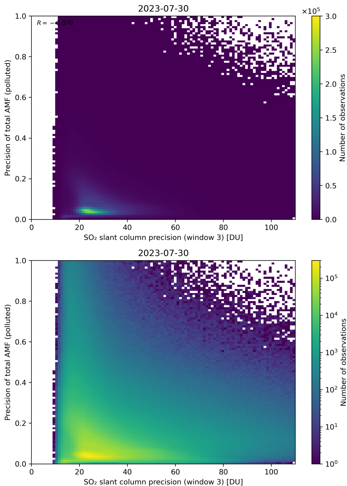
Figure 264: Scatter density plot of “SO 2 slant column precision (window 3)” against “Precision of total AMF (polluted)” for 2023-07-29 to 2023-07-31.
