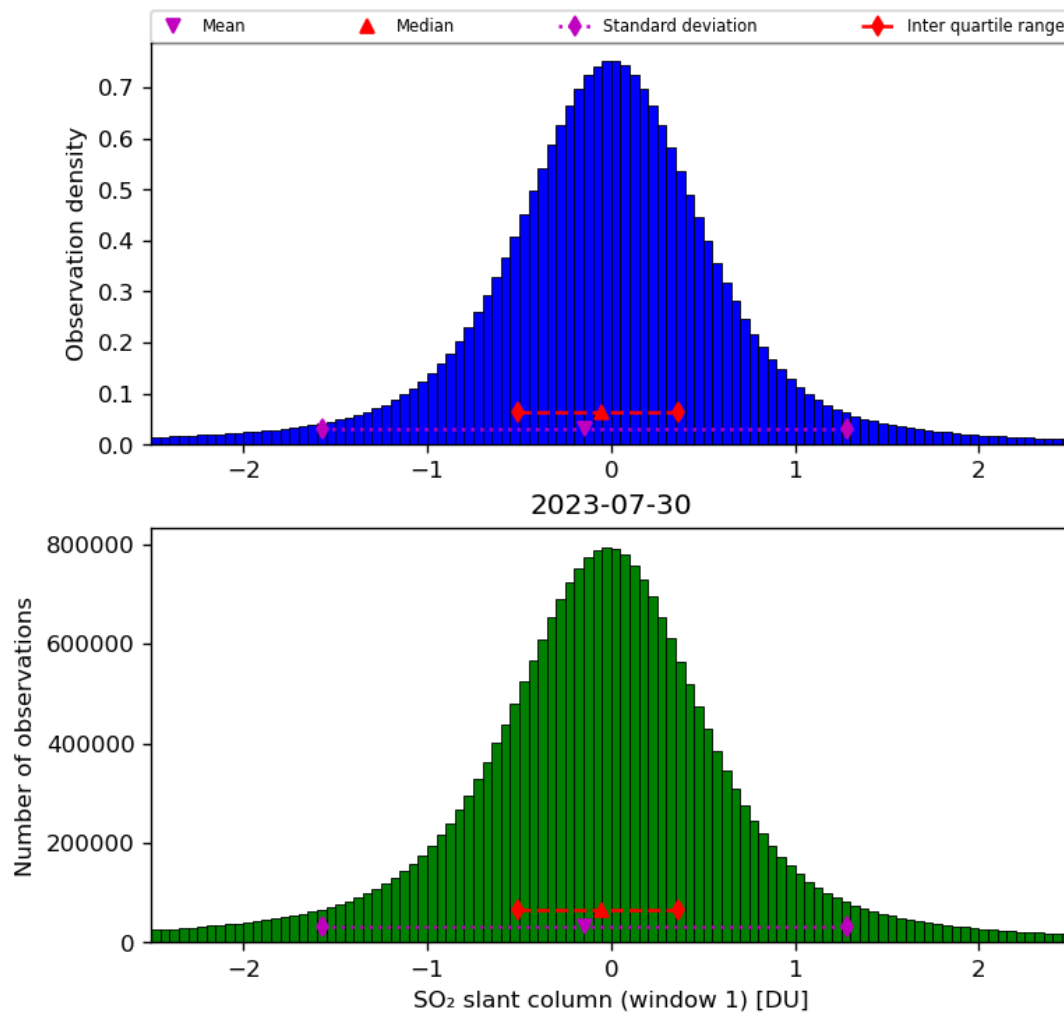
Figure 56: Histogram of “SO 2 slant column (window 1)” for 2023-07-29 to 2023-07-31
