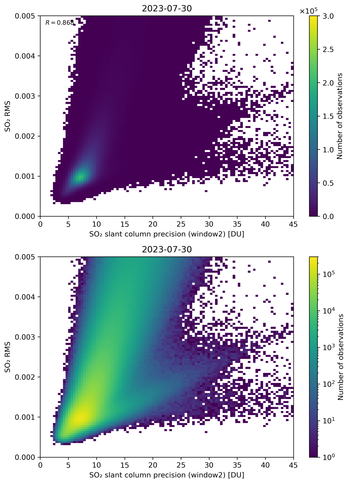
Figure 245: Scatter density plot of “SO 2 slant column precision (window2)” against “SO 2 RMS” for 2023-07-29 to 2023-07-31.
