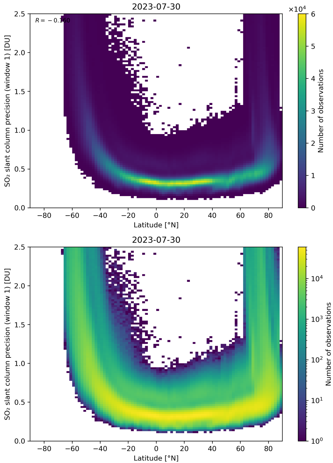
Figure 150: Scatter density plot of “Latitude” against “SO 2 slant column precision (window 1)” for 2023-07-29 to 2023-07-31.
