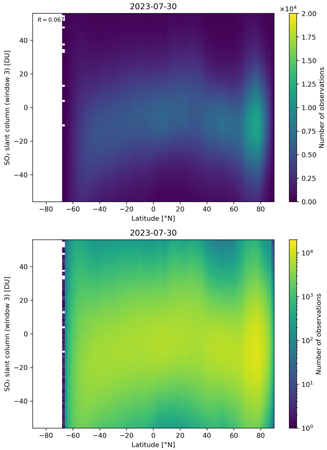
Figure 152: Scatter density plot of “Latitude” against “SO 2 slant column (window 3)” for 2023-07-29 to 2023-07-31.
