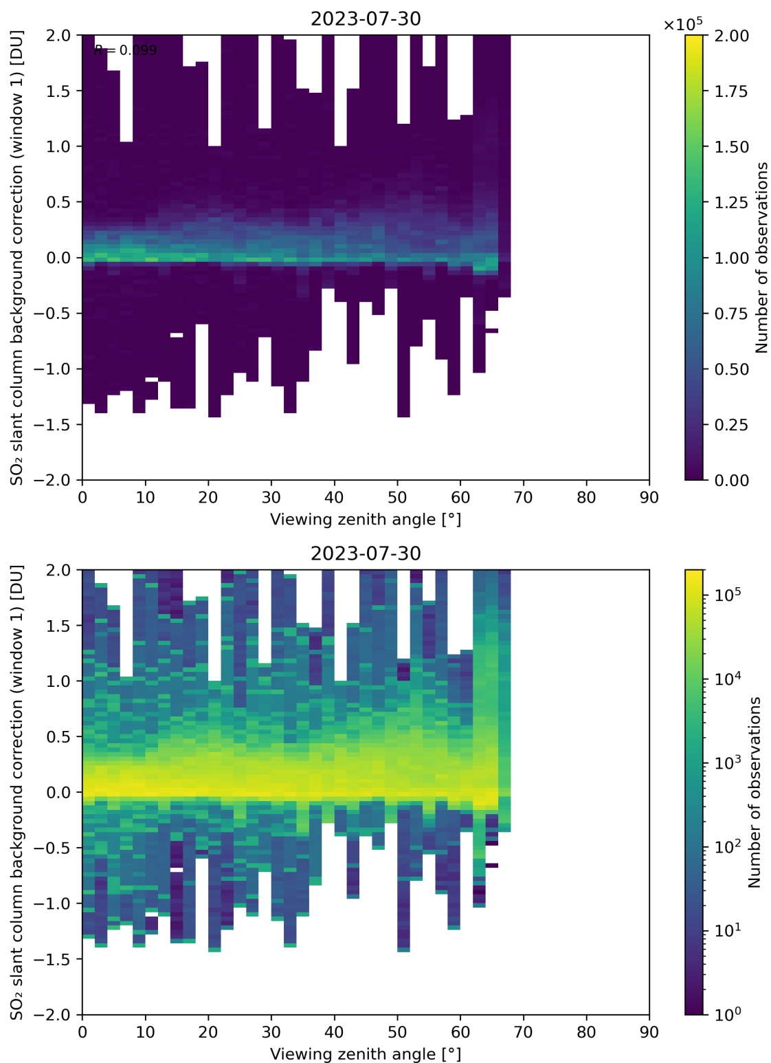
Figure 308: Scatter density plot of “Viewing zenith angle” against “SO 2 slant column background correction (window 1)” for 2023-07-29 to 2023-07-31.
