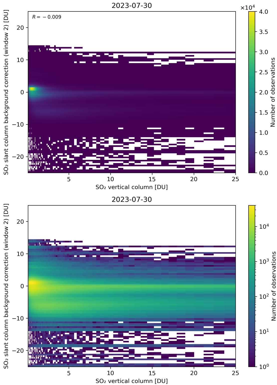
Figure 274: Scatter density plot of “SO 2 vertical column” against “SO 2 slant column background correction (window 2)” for 2023-07-29 to 2023-07-31.
