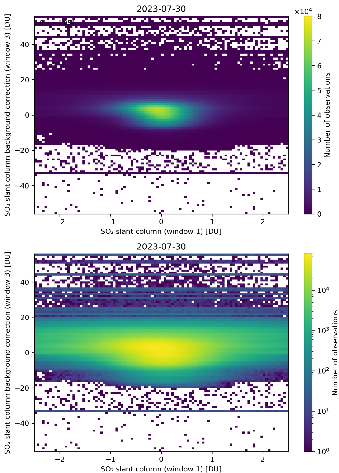
Figure 214: Scatter density plot of “SO 2 slant column (window 1)” against “SO 2 slant column background correction (window 3)” for 2023-07-29 to 2023-07-31.
