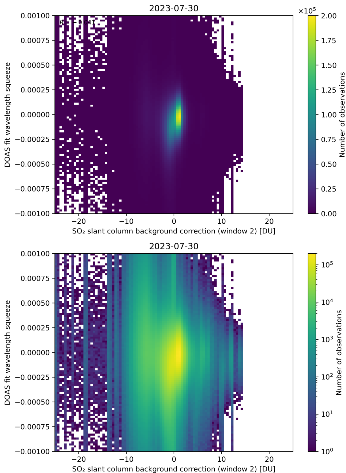
Figure 113: Scatter density plot of “SO 2 slant column background correction (window 2)” against “DOAS fit wavelength squeeze” for 2023-07-29 to 2023-07-31.
