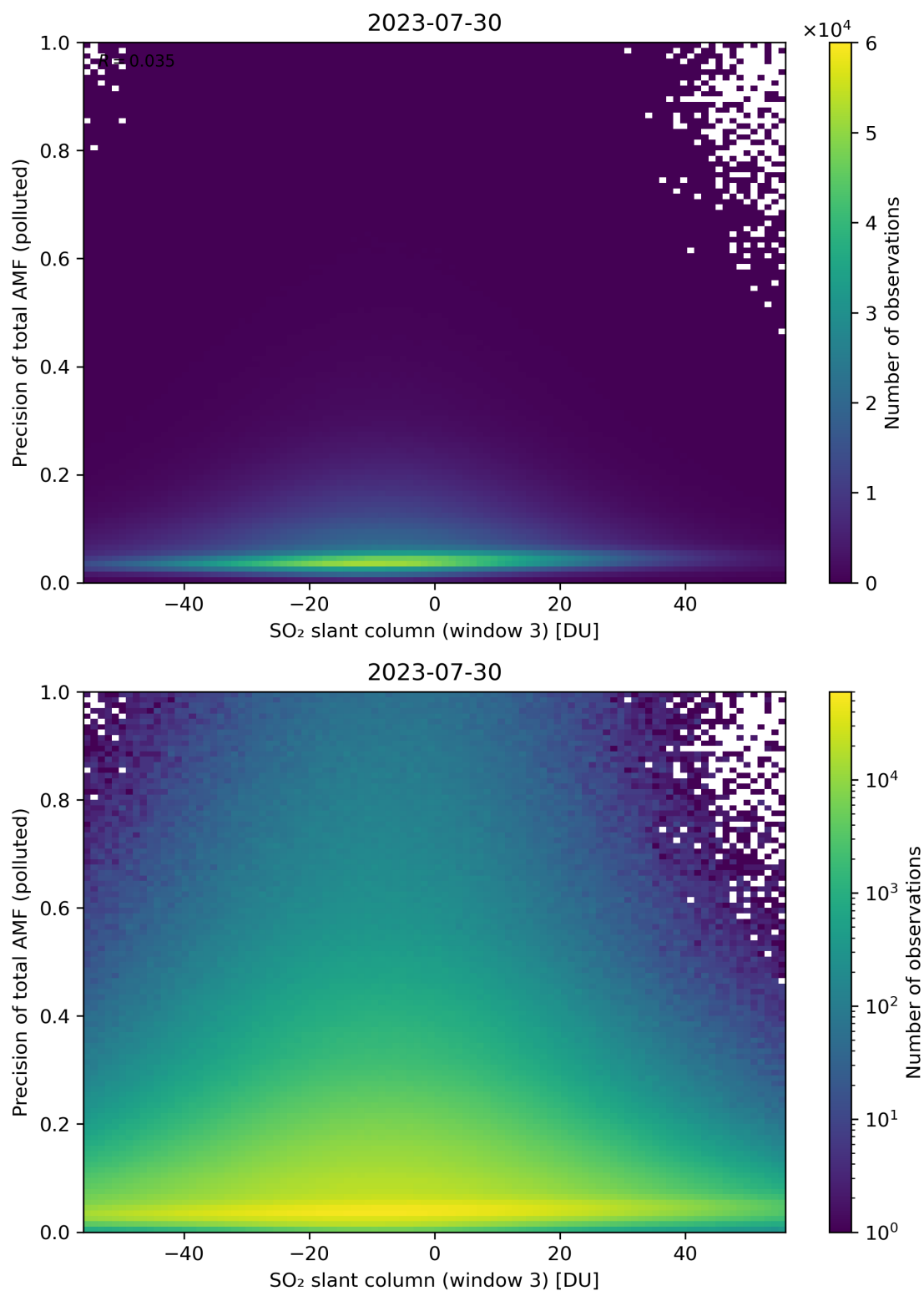
Figure 269: Scatter density plot of “SO 2 slant column (window 3)” against “Precision of total AMF (polluted)” for 2023-07-29 to 2023-07-31.
