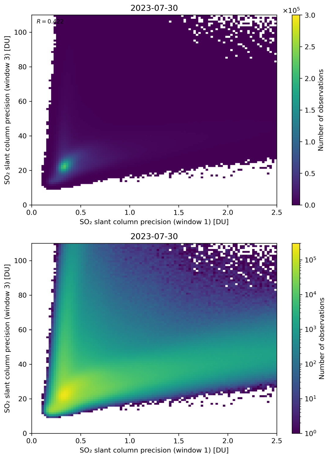
Figure 229: Scatter density plot of “SO 2 slant column precision (window 1)” against “SO 2 slant column precision (window 3)” for 2023-07-29 to 2023-07-31.
