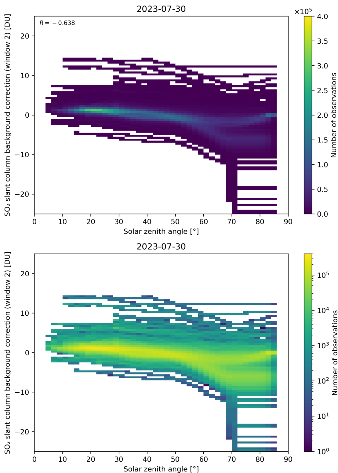
Figure 159: Scatter density plot of “Solar zenith angle” against “SO 2 slant column background correction (window 2)” for 2023-07-29 to 2023-07-31.
