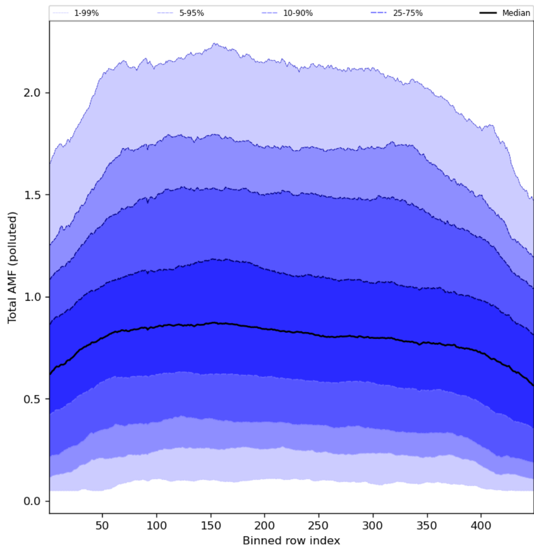
Figure 94: Along track statistics of “Total AMF (polluted)” for 2023-07-29 to 2023-07-31
