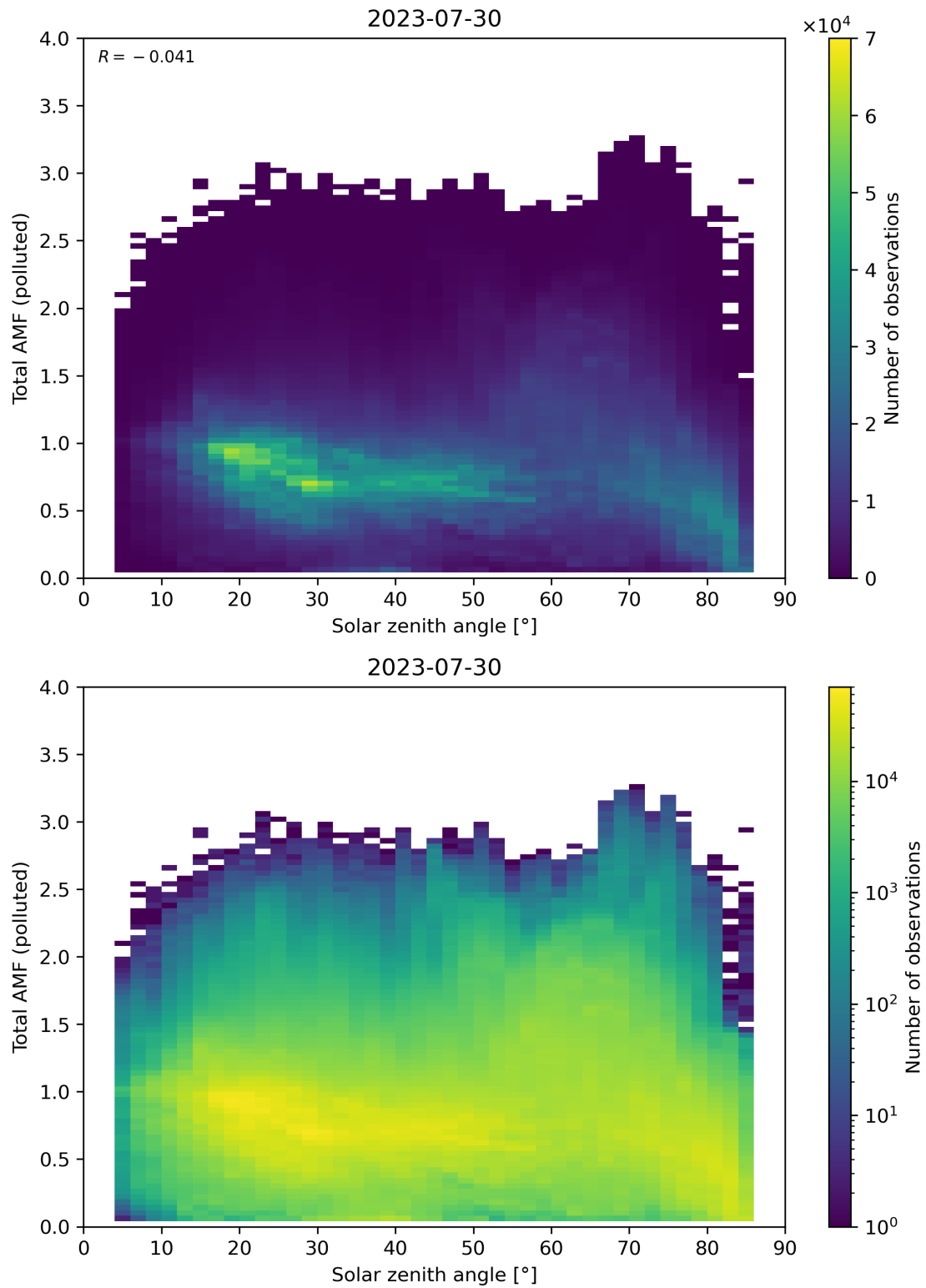
Figure 174: Scatter density plot of “Solar zenith angle” against “Total AMF (polluted)” for 2023-07-29 to 2023-07-31.
