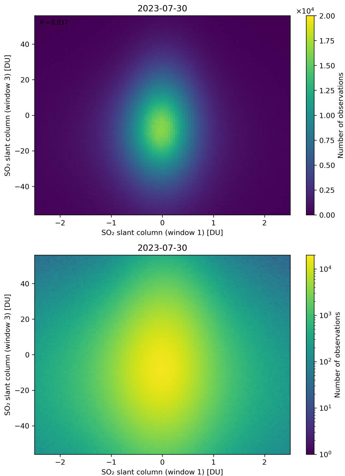
Figure 237: Scatter density plot of “SO 2 slant column (window 1)” against “SO 2 slant column (window 3)” for 2023-07-29 to 2023-07-31.
