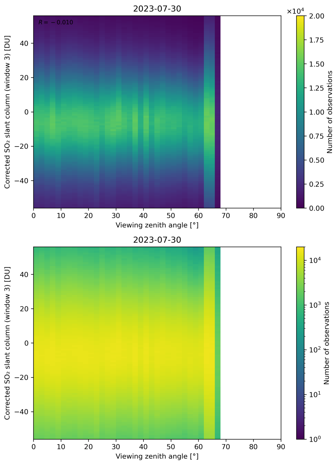
Figure 319: Scatter density plot of “Viewing zenith angle” against “Corrected SO 2 slant column (window 3)” for 2023-07-29 to 2023-07-31.
