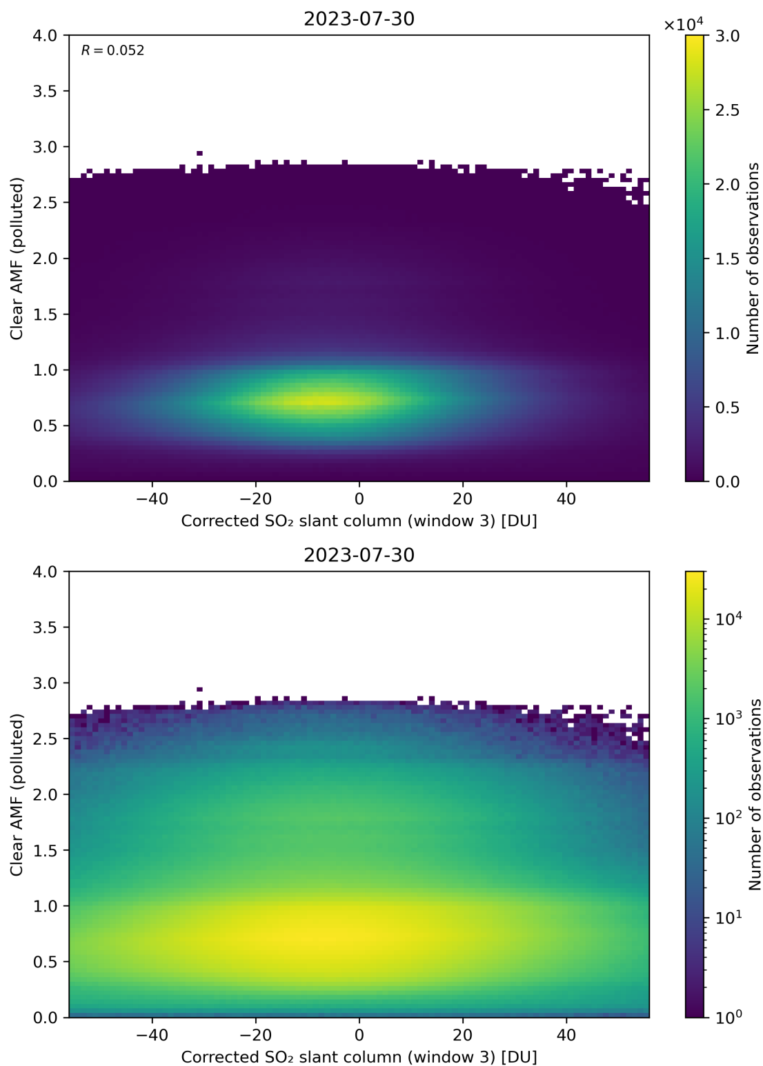
Figure 209: Scatter density plot of “Corrected SO 2 slant column (window 3)” against “Clear AMF (polluted)” for 2023-07-29 to 2023-07-31.
