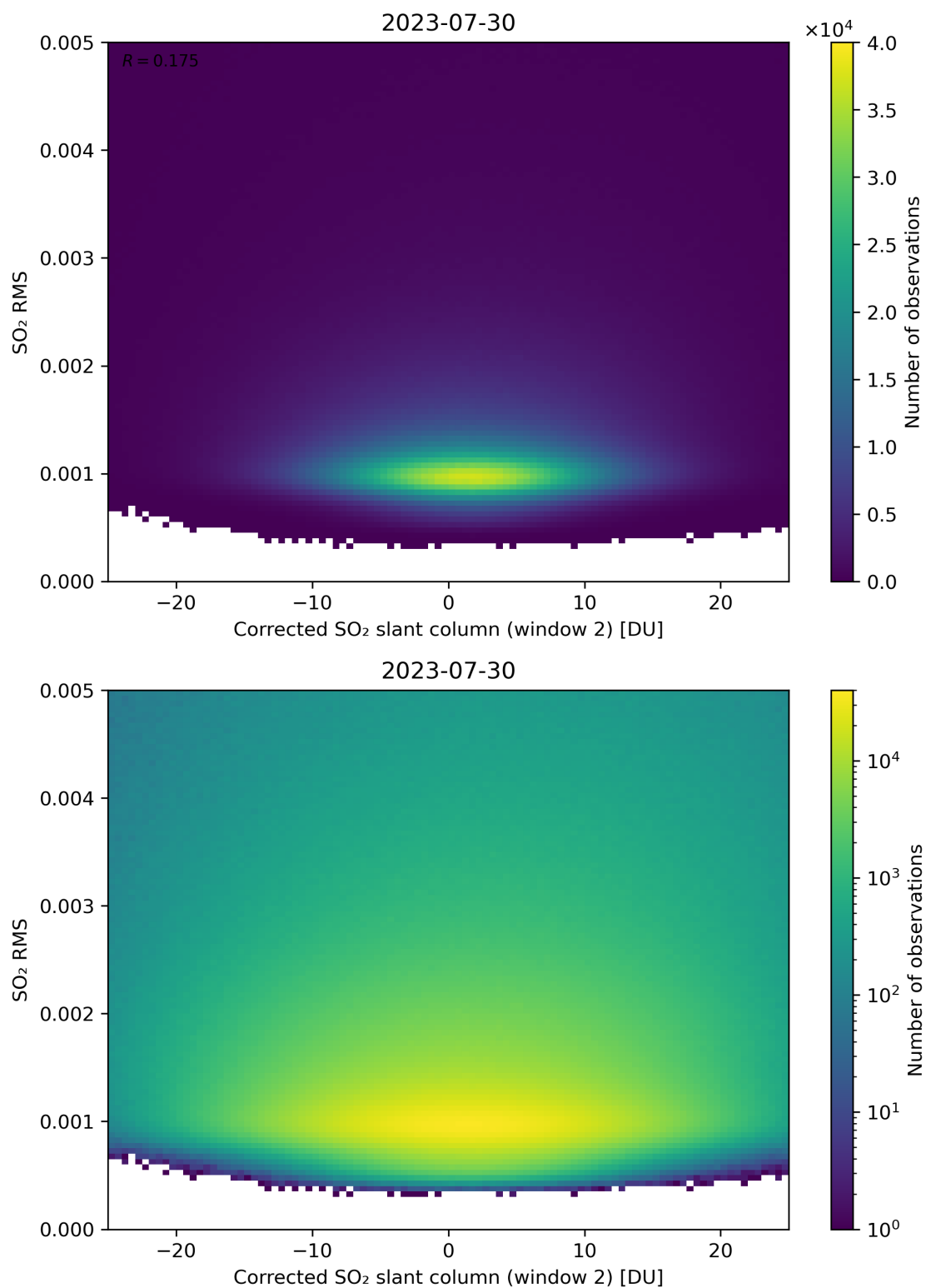
Figure 198: Scatter density plot of “Corrected SO 2 slant column (window 2)” against “SO 2 RMS” for 2023-07-29 to 2023-07-31.
