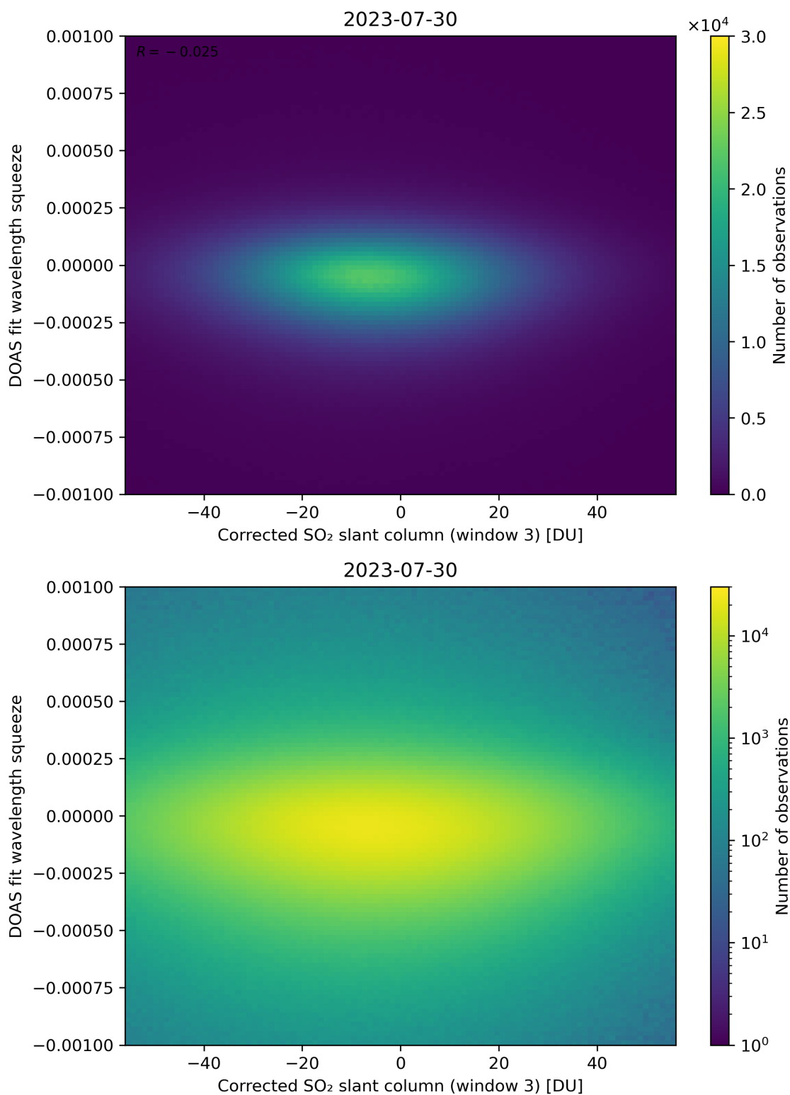
Figure 207: Scatter density plot of “Corrected SO 2 slant column (window 3)” against “DOAS fit wavelength squeeze” for 2023-07-29 to 2023-07-31.
