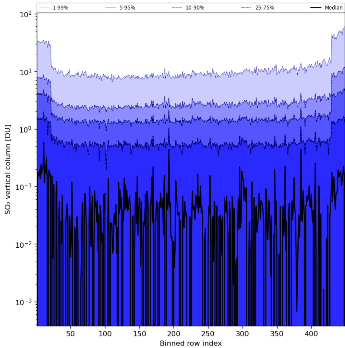
Figure 76: Along track statistics of “SO 2 vertical column” for 2023-07-29 to 2023-07-31
