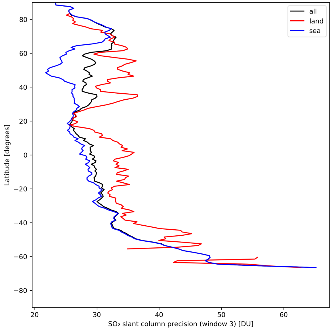
Figure 42: Zonal average of "SO 2 slant column precision (window 3)" for 2023-07-29 to 2023-07-31.
