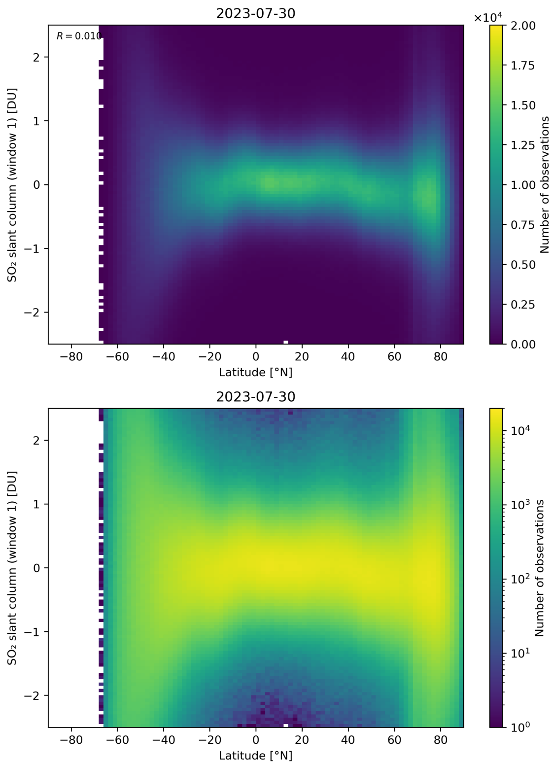
Figure 149: Scatter density plot of “Latitude” against “SO 2 slant column (window 1)” for 2023-07-29 to 2023-07-31.
