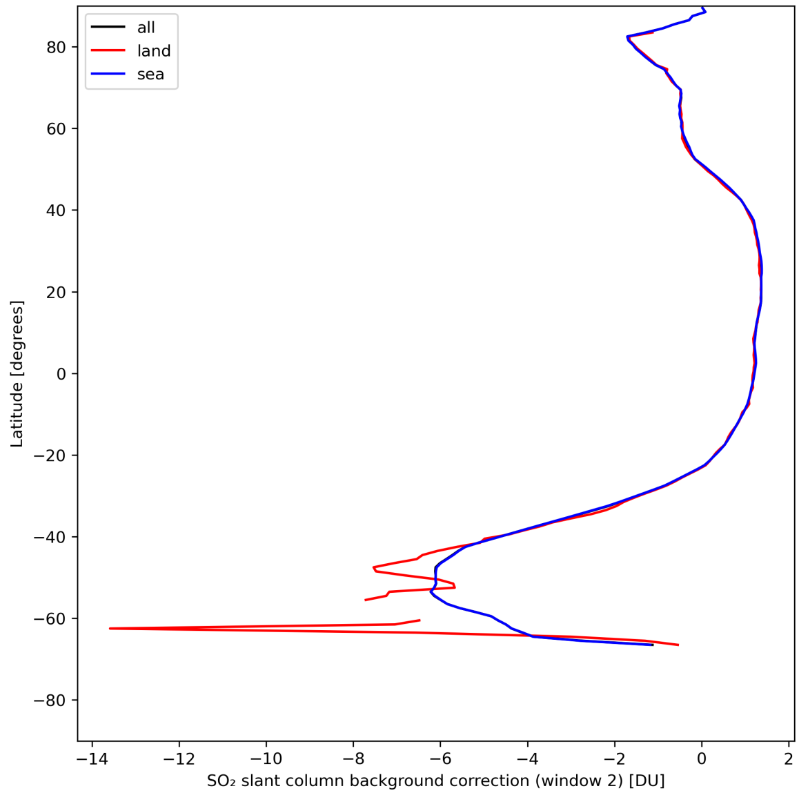
Figure 40: Zonal average of “SO 2 slant column background correction (window 2)” for 2023-07-29 to 2023-07-31.
