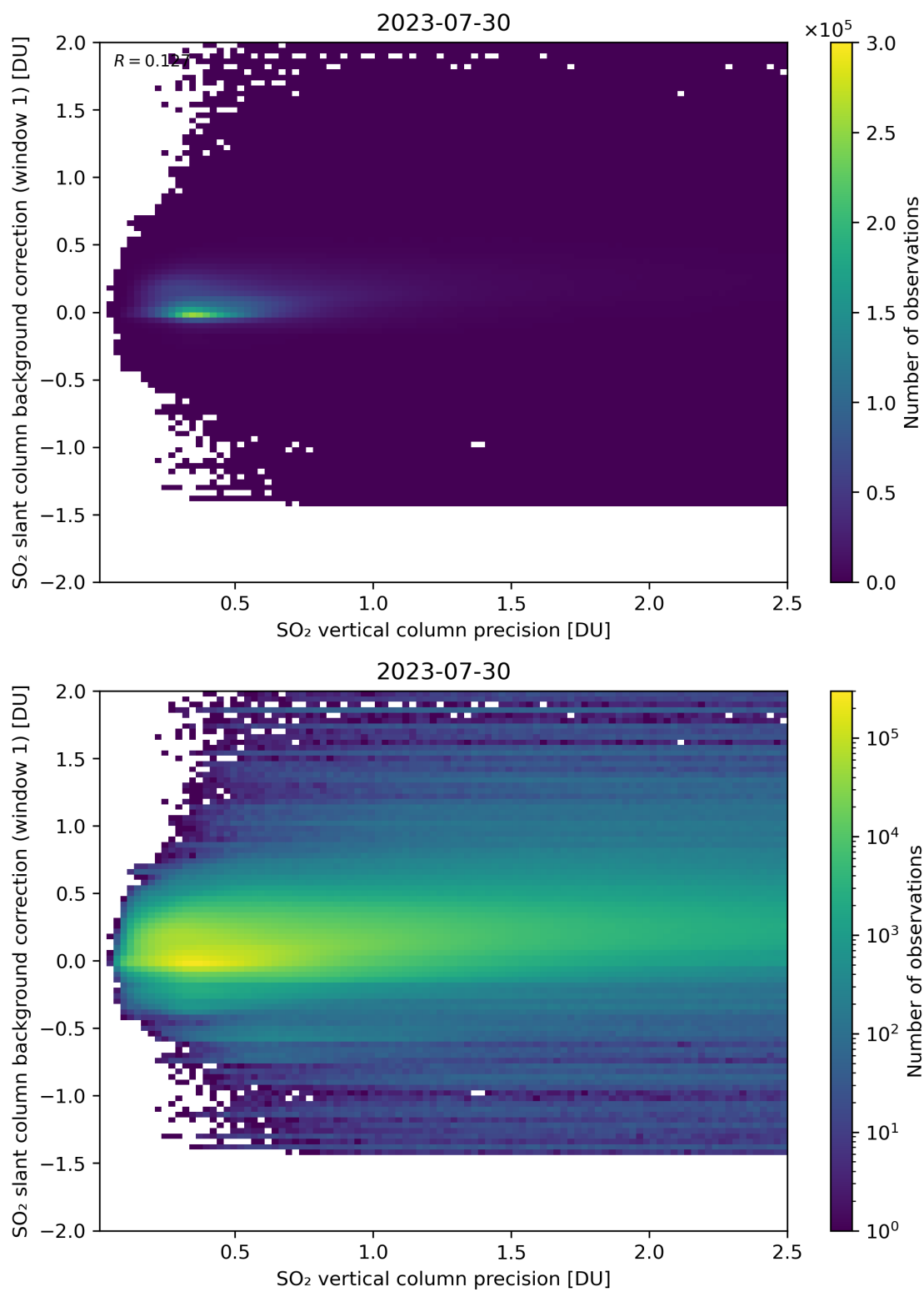
Figure 279: Scatter density plot of “SO 2 vertical column precision” against “SO 2 slant column background correction (window 1)” for 2023-07-29 to 2023-07-31.
