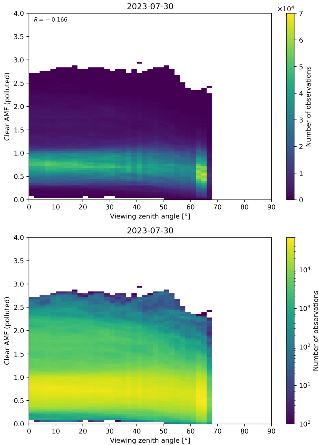
Figure 316: Scatter density plot of “Viewing zenith angle” against “Clear AMF (polluted)” for 2023-07-29 to 2023-07-31.
