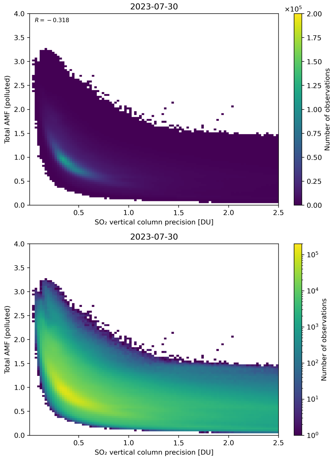
Figure 294: Scatter density plot of “SO 2 vertical column precision” against “Total AMF (polluted)” for 2023-07-29 to 2023-07-31.
