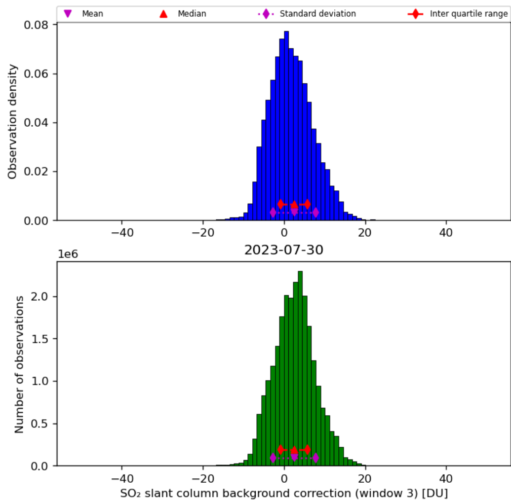
Figure 67: Histogram of “SO 2 slant column background correction (window 3)” for 2023-07-29 to 2023-07-31
