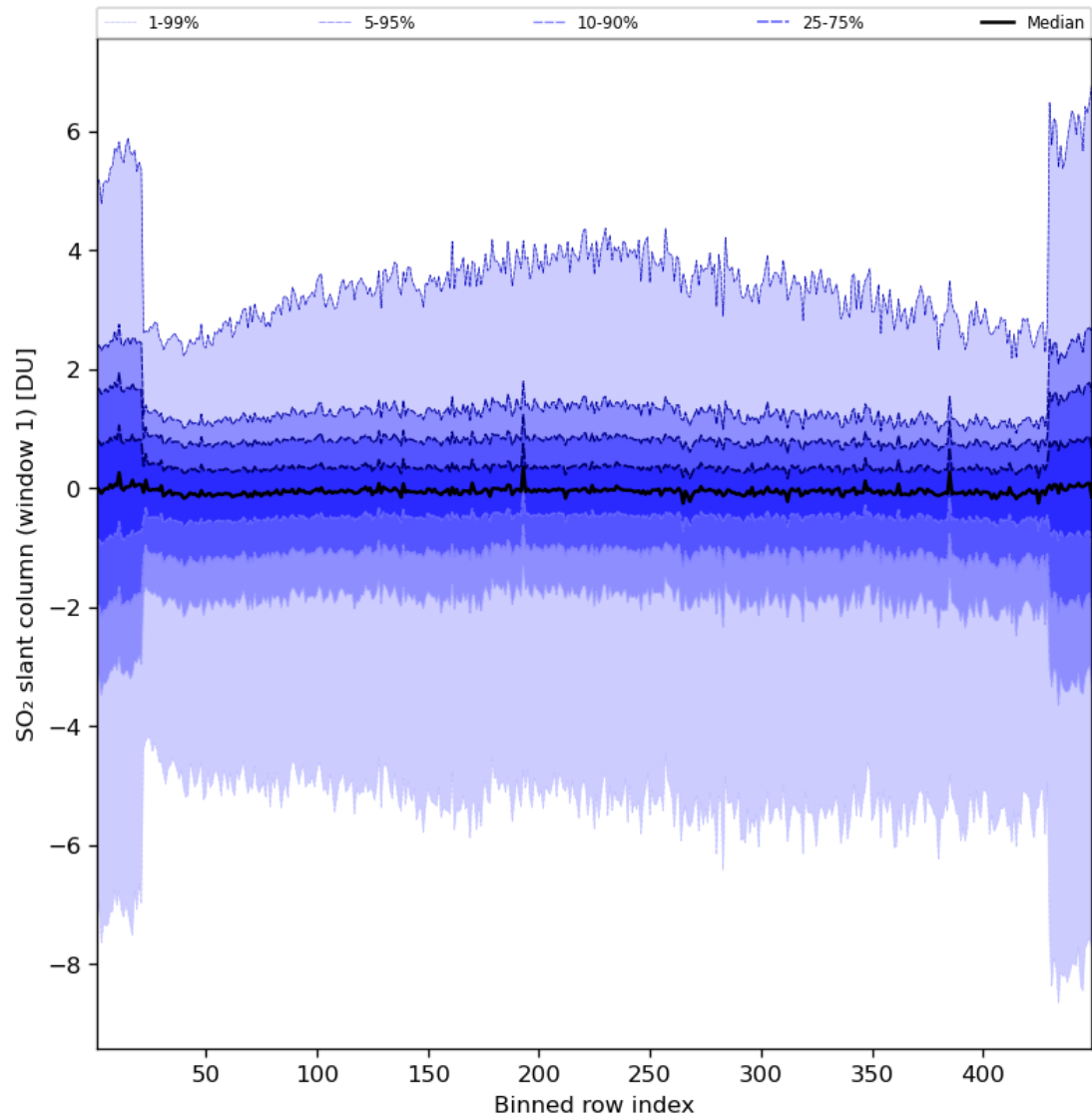
Figure 79: Along track statistics of “SO 2 slant column (window 1)” for 2023-07-29 to 2023-07-31
