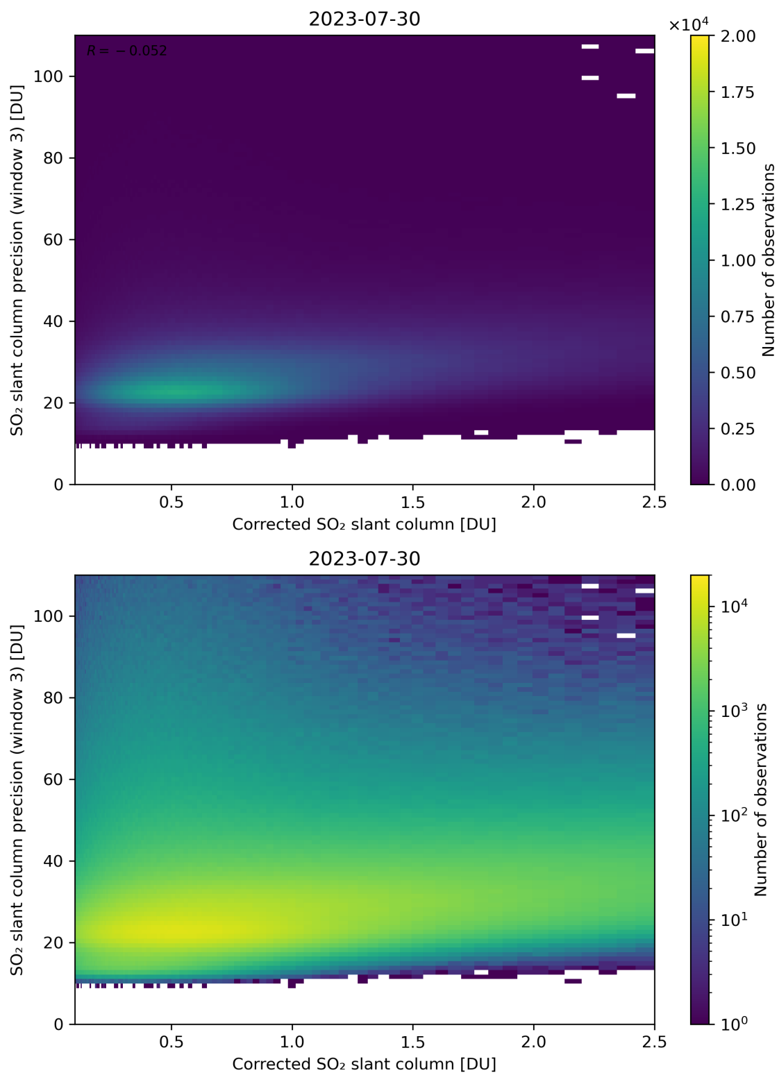
Figure 191: Scatter density plot of “Corrected SO 2 slant column” against “SO 2 slant column precision (window 3)” for 2023-07-29 to 2023-07-31.
