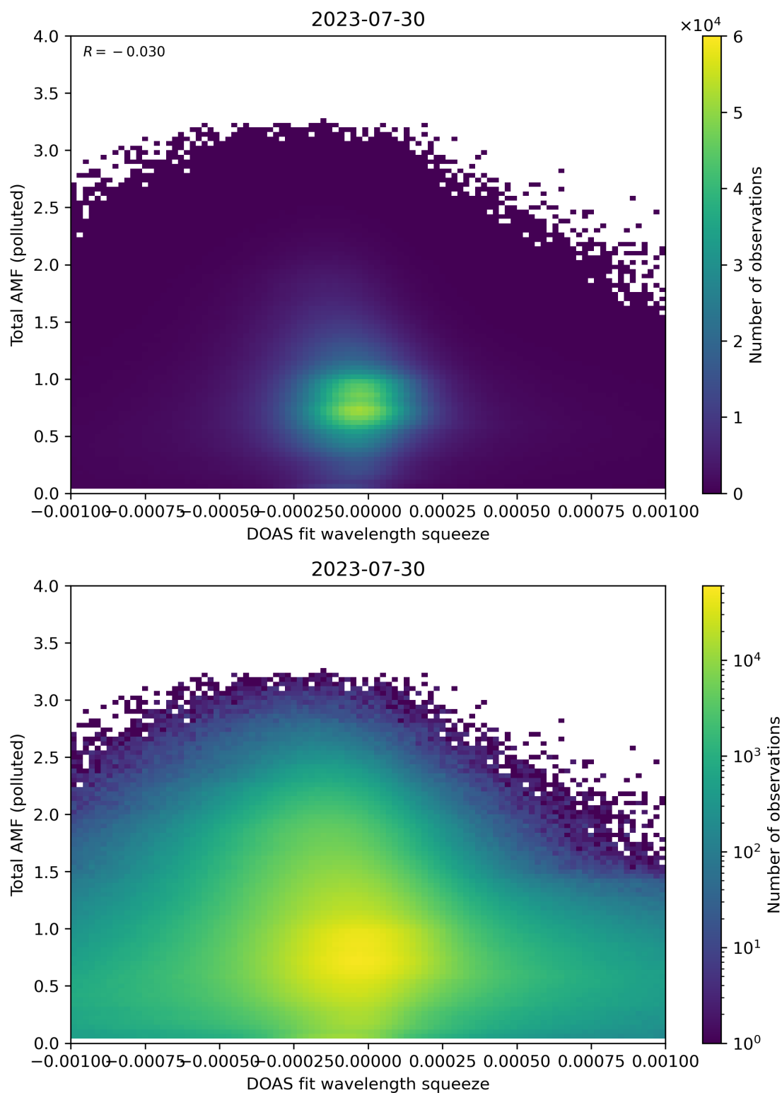
Figure 134: Scatter density plot of “DOAS fit wavelength squeeze” against “Total AMF (polluted)” for 2023-07-29 to 2023-07-31.
