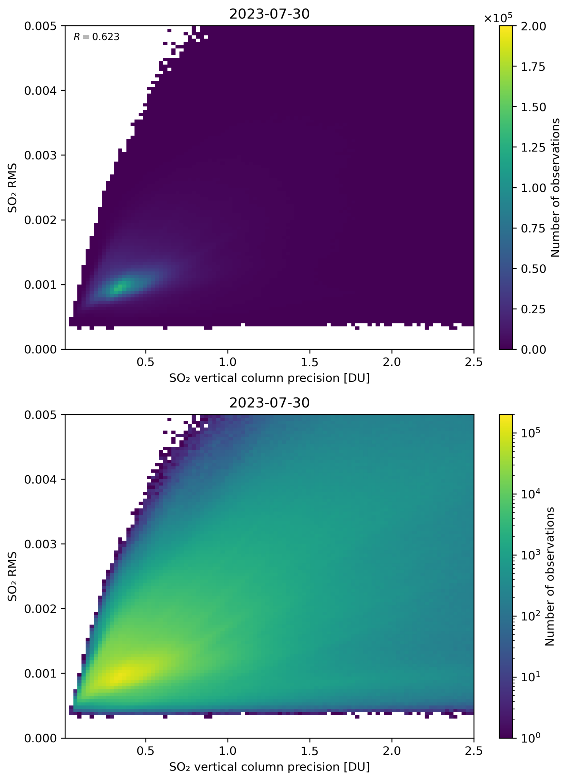
Figure 284: Scatter density plot of “SO 2 vertical column precision” against “SO 2 RMS” for 2023-07-29 to 2023-07-31.
