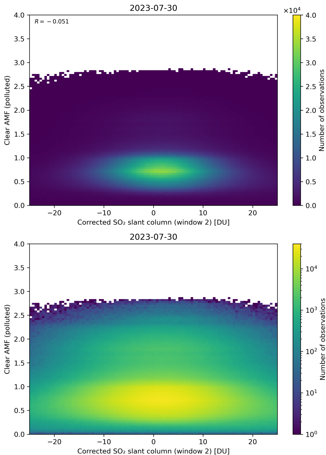
Figure 199: Scatter density plot of “Corrected SO 2 slant column (window 2)” against “Clear AMF (polluted)” for 2023-07-29 to 2023-07-31.
