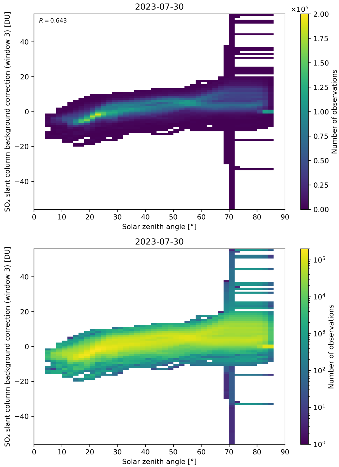
Figure 160: Scatter density plot of “Solar zenith angle” against “SO 2 slant column background correction (window 3)” for 2023-07-29 to 2023-07-31.
