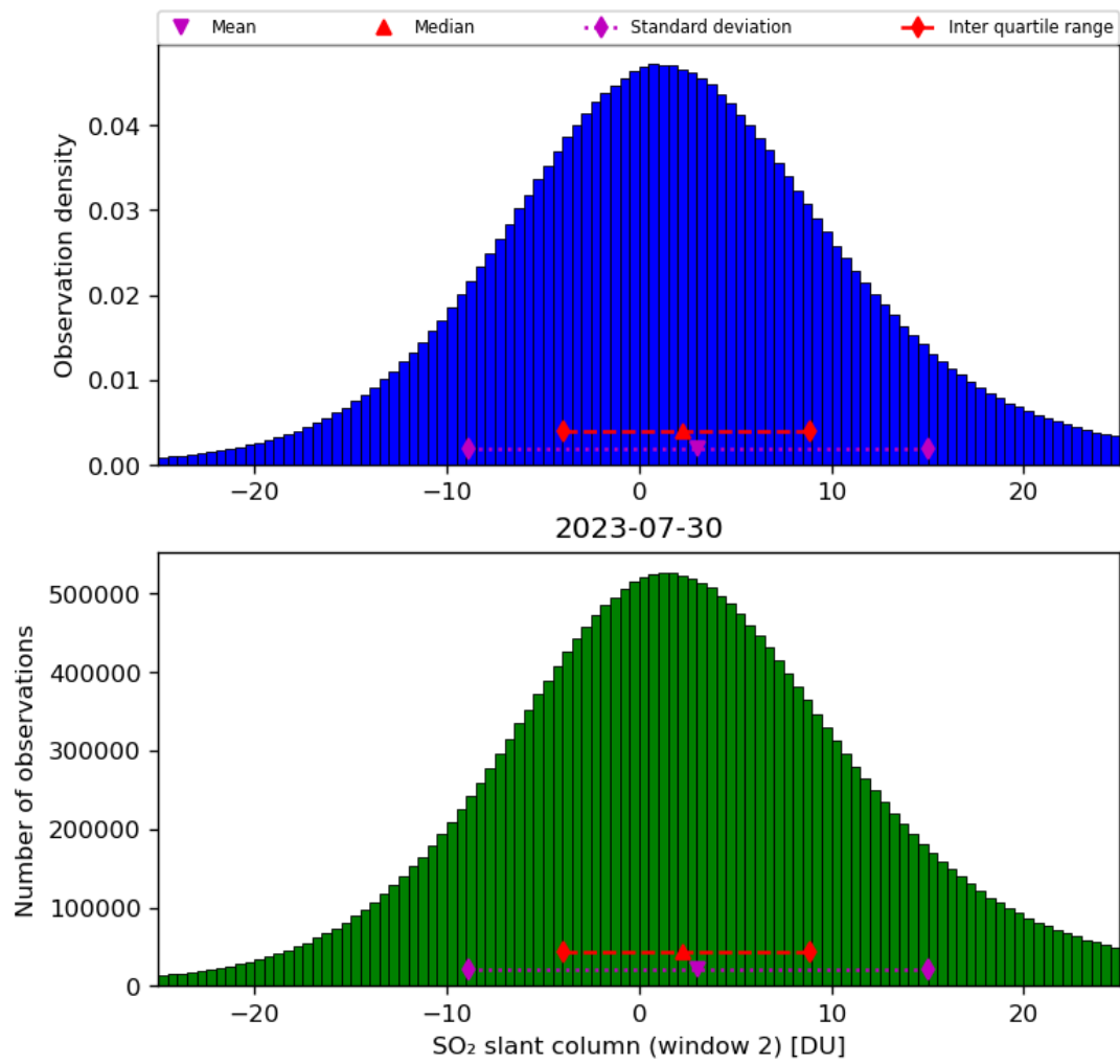
Figure 60: Histogram of “SO 2 slant column (window 2)” for 2023-07-29 to 2023-07-31
