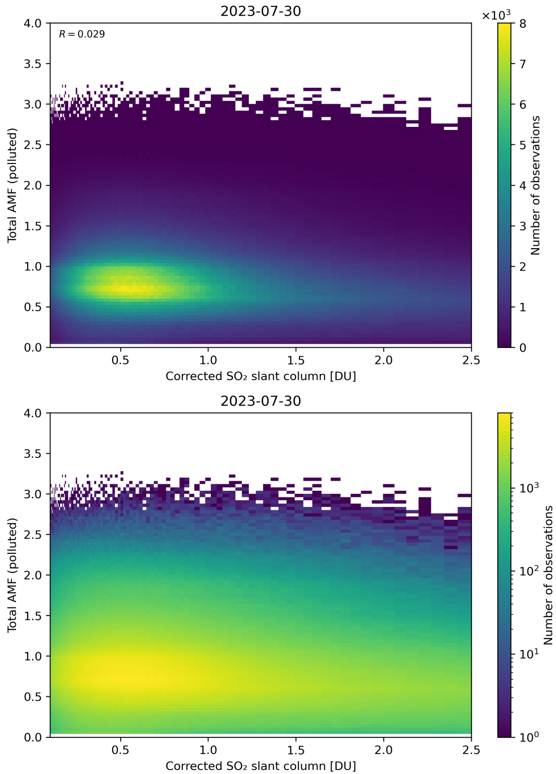
Figure 192: Scatter density plot of “Corrected SO 2 slant column” against “Total AMF (polluted)” for 2023-07-29 to 2023-07-31.
