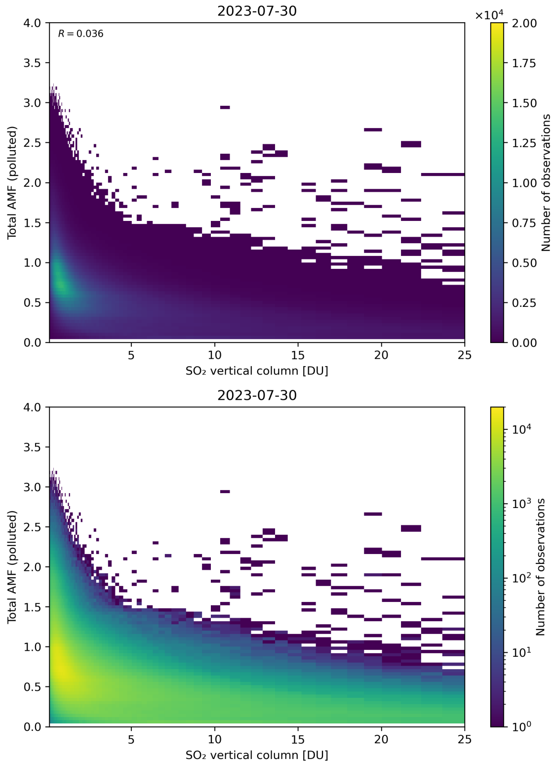
Figure 305: Scatter density plot of “SO 2 vertical column” against “Total AMF (polluted)” for 2023-07-29 to 2023-07-31.
