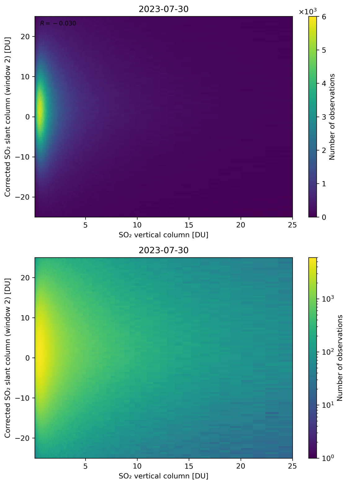
Figure 298: Scatter density plot of “SO 2 vertical column” against “Corrected SO 2 slant column (window 2)” for 2023-07-29 to 2023-07-31.
