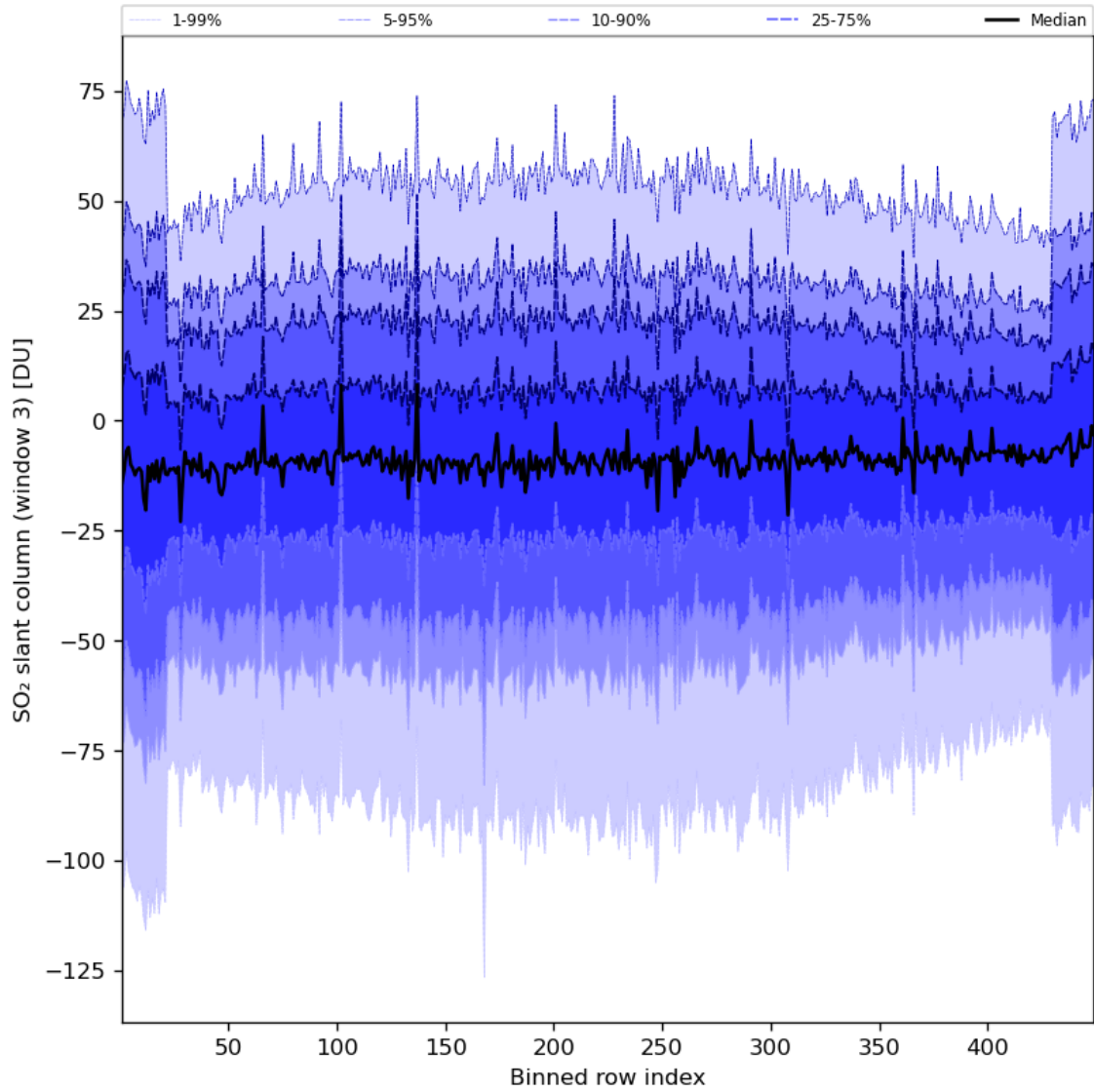
Figure 87: Along track statistics of “SO 2 slant column (window 3)” for 2023-07-29 to 2023-07-31
