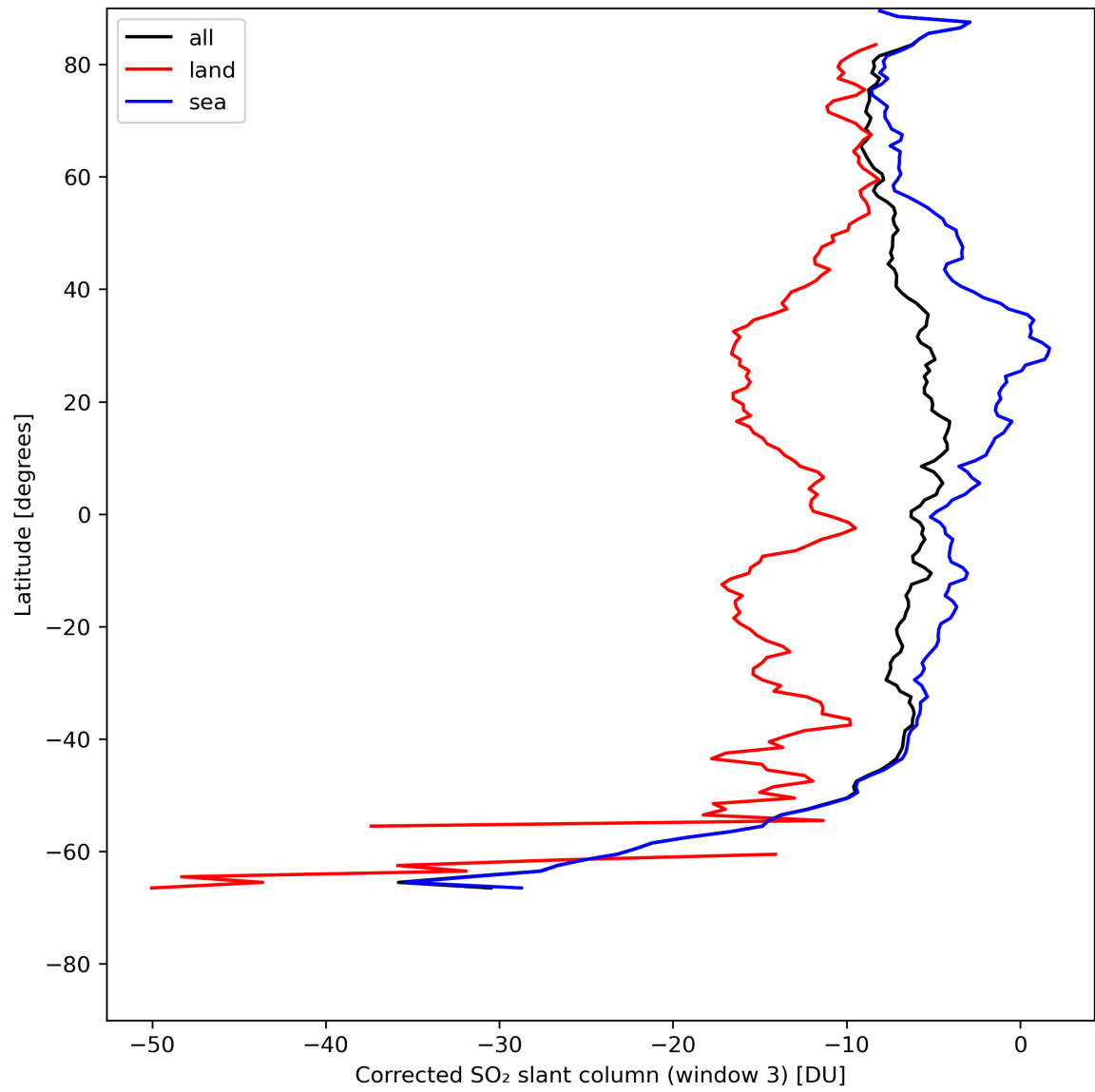
Figure 43: Zonal average of “Corrected SO 2 slant column (window 3)” for 2023-07-29 to 2023-07-31.
