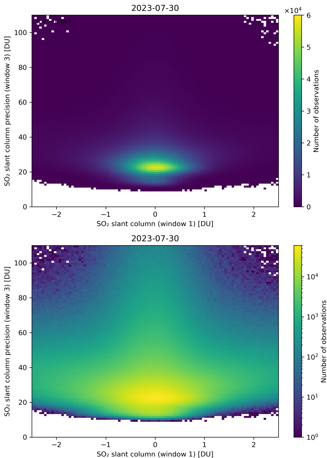
Figure 238: Scatter density plot of “SO 2 slant column (window 1)” against “SO 2 slant column precision (window 3)” for 2023-07-29 to 2023-07-31.
