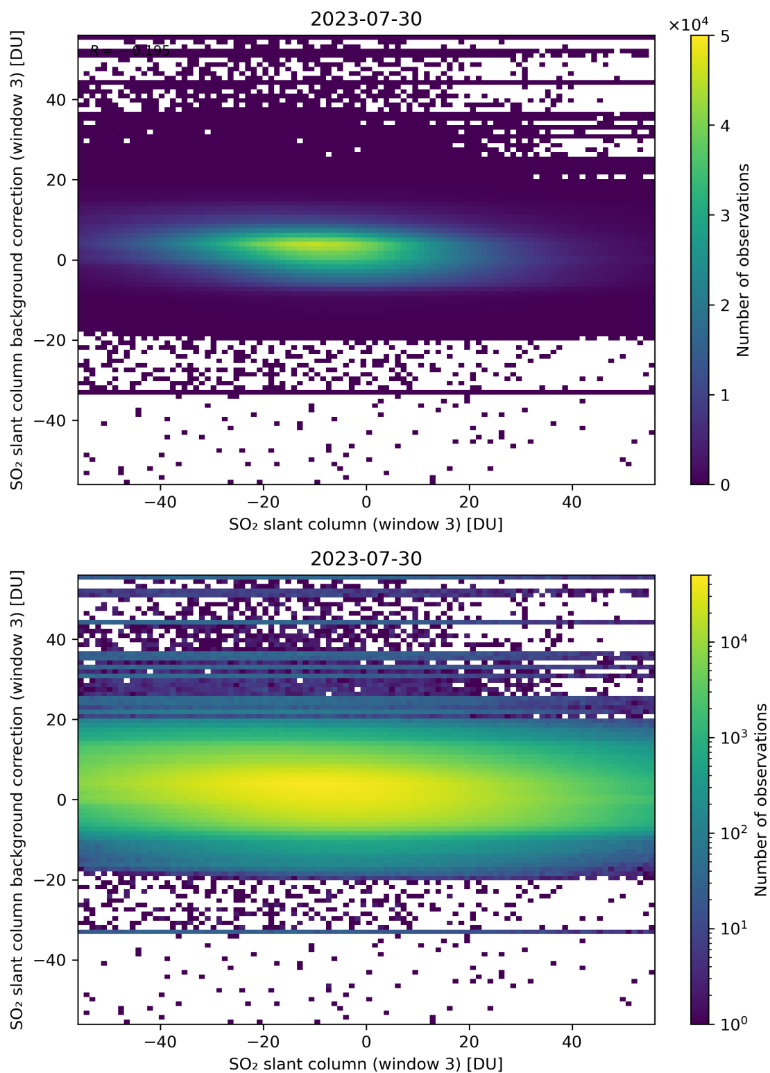
Figure 253: Scatter density plot of “SO 2 slant column (window 3)” against “SO 2 slant column background correction (window 3)” for 2023-07-29 to 2023-07-31.
