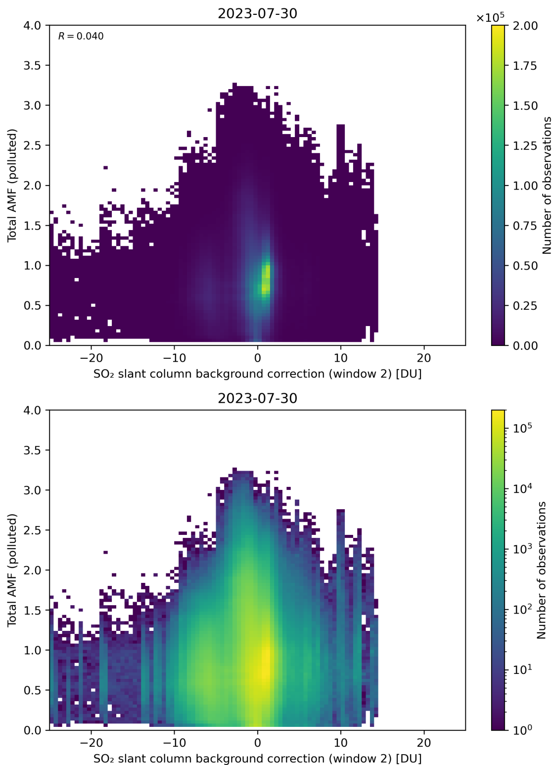
Figure 119: Scatter density plot of “SO 2 slant column background correction (window 2)” against “Total AMF (polluted)” for 2023-07-29 to 2023-07-31.
