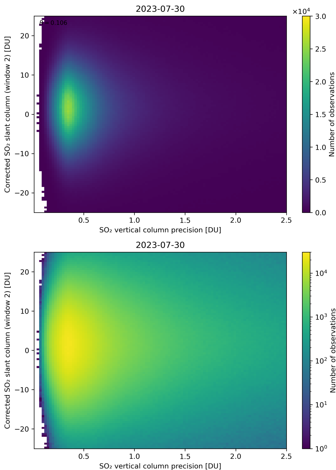
Figure 287: Scatter density plot of “SO 2 vertical column precision” against “Corrected SO 2 slant column (window 2)” for 2023-07-29 to 2023-07-31.
