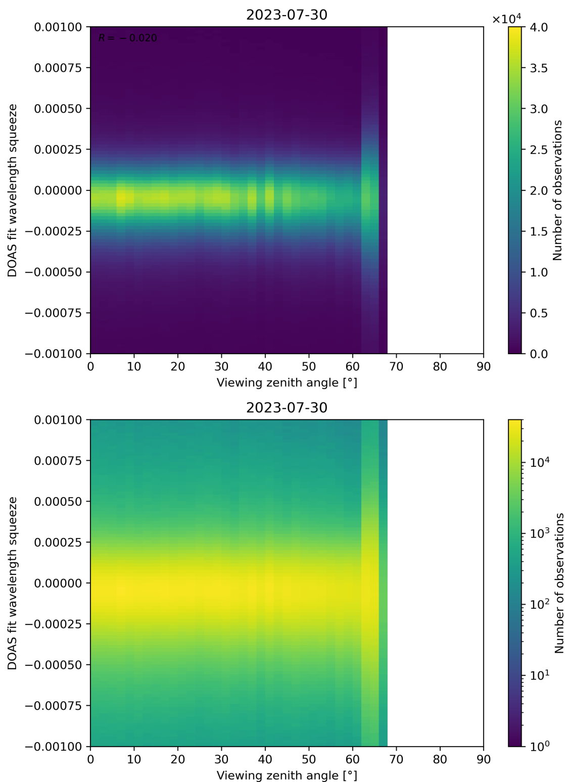
Figure 312: Scatter density plot of “Viewing zenith angle” against “DOAS fit wavelength squeeze” for 2023-07-29 to 2023-07-31.
