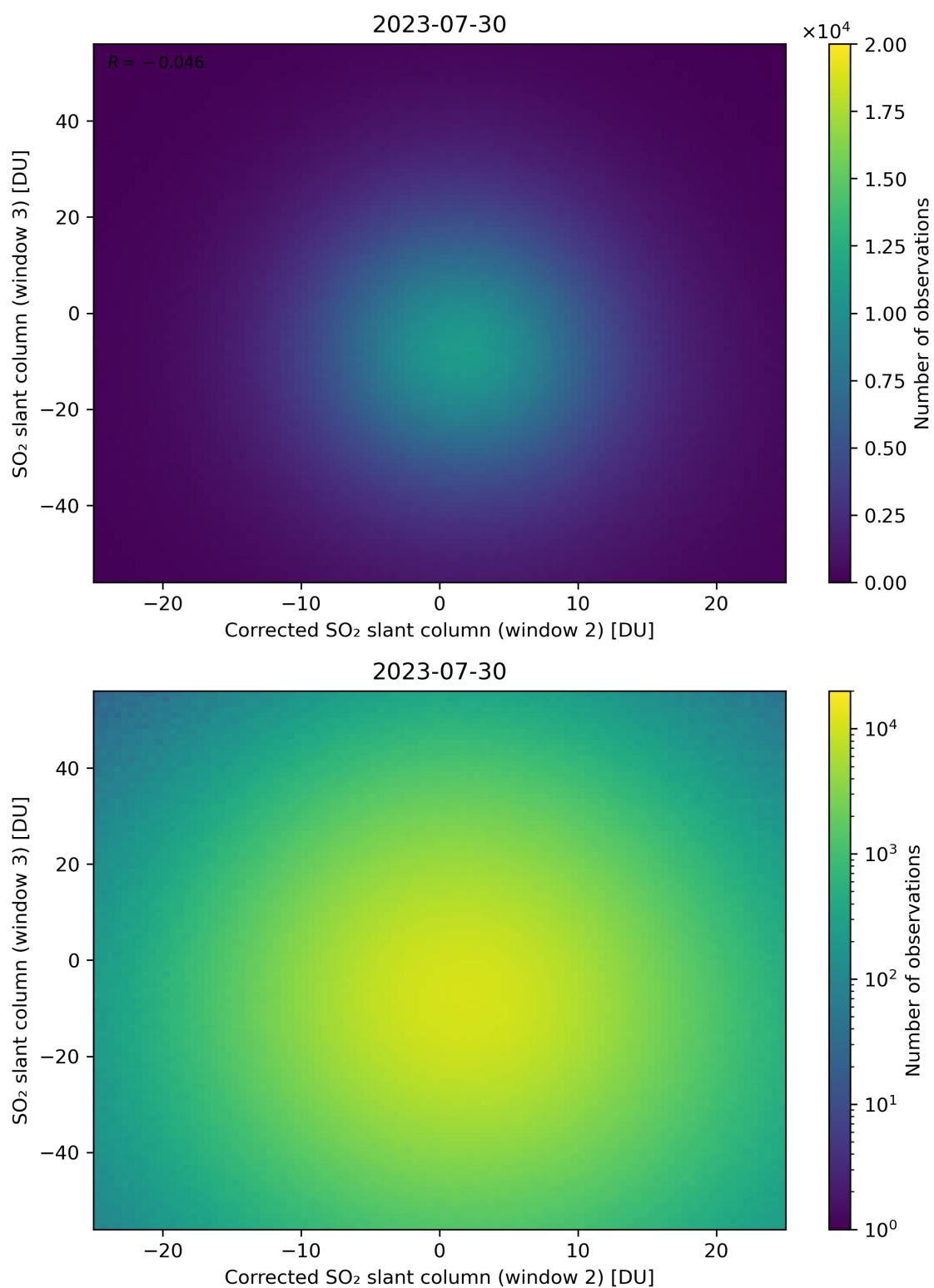
Figure 201: Scatter density plot of “Corrected SO 2 slant column (window 2)” against “SO 2 slant column (window 3)” for 2023-07-29 to 2023-07-31.
