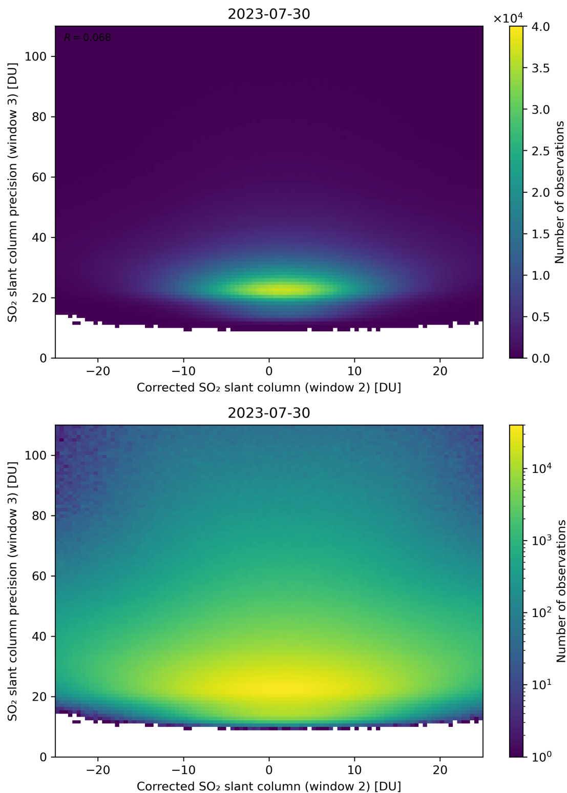
Figure 202: Scatter density plot of “Corrected SO 2 slant column (window 2)” against “SO 2 slant column precision (window 3)” for 2023-07-29 to 2023-07-31.
