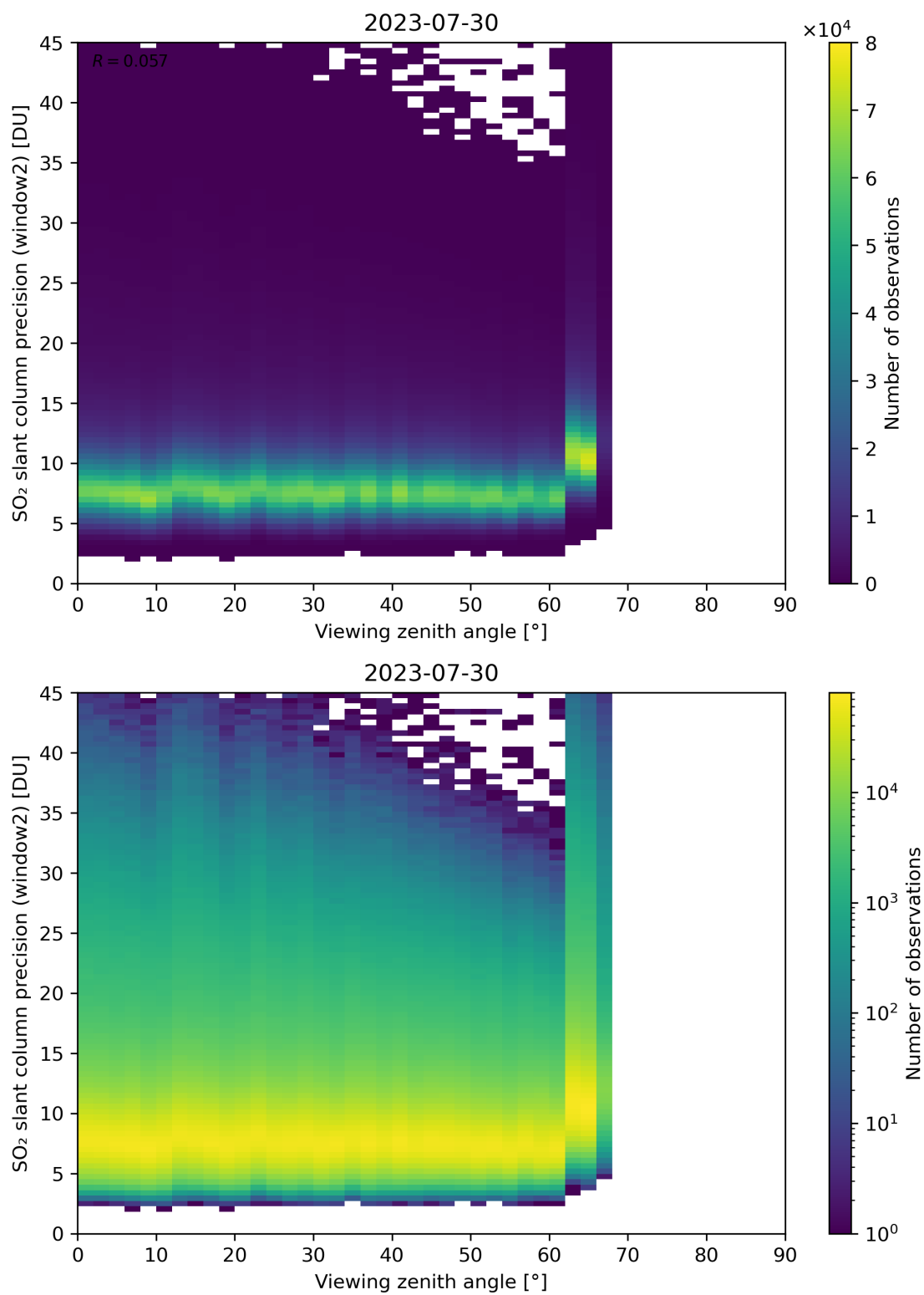
Figure 322: Scatter density plot of “Viewing zenith angle” against “SO 2 slant column precision (window2)” for 2023-07-29 to 2023-07-31.
