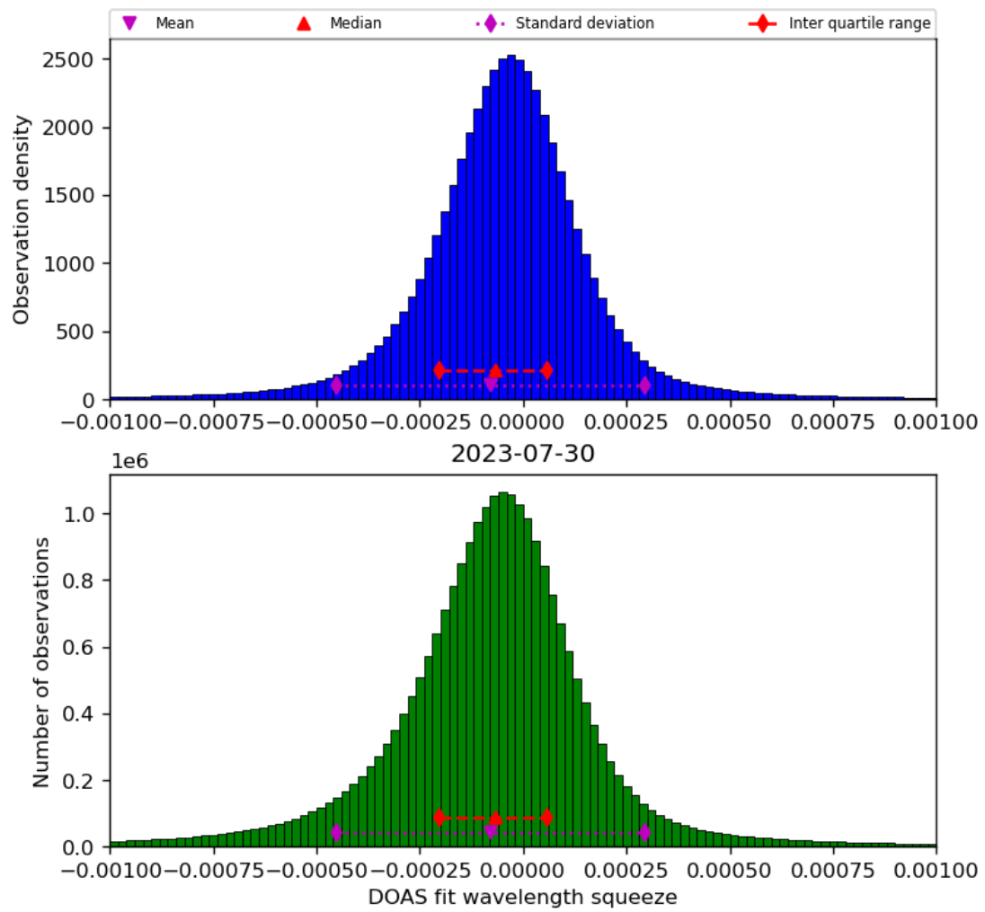
Figure 69: Histogram of “DOAS fit wavelength squeeze” for 2023-07-29 to 2023-07-31
