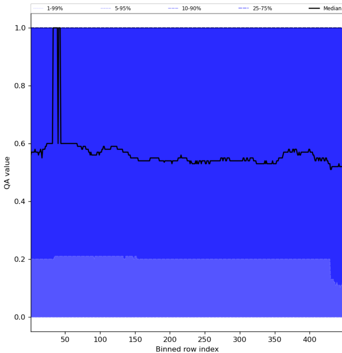
Figure 75: Along track statistics of “QA value” for 2023-07-29 to 2023-07-31
