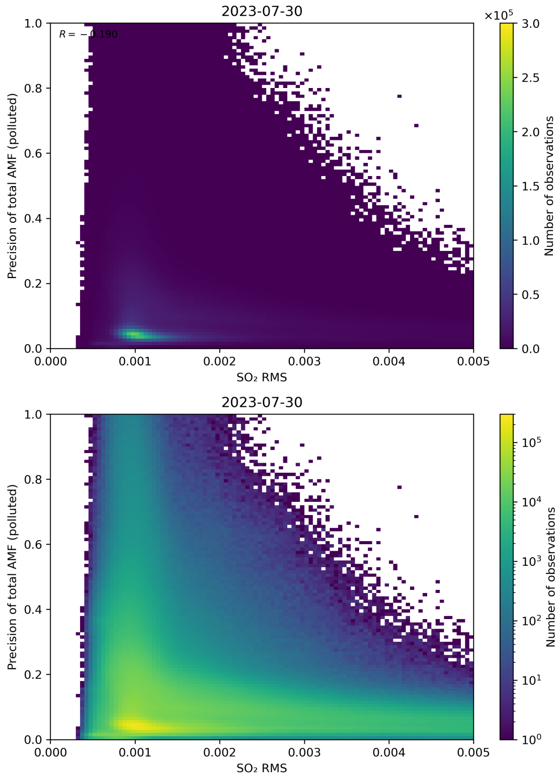
Figure 138: Scatter density plot of “SO 2 RMS” against “Precision of total AMF (polluted)” for 2023-07-29 to 2023-07-31.
