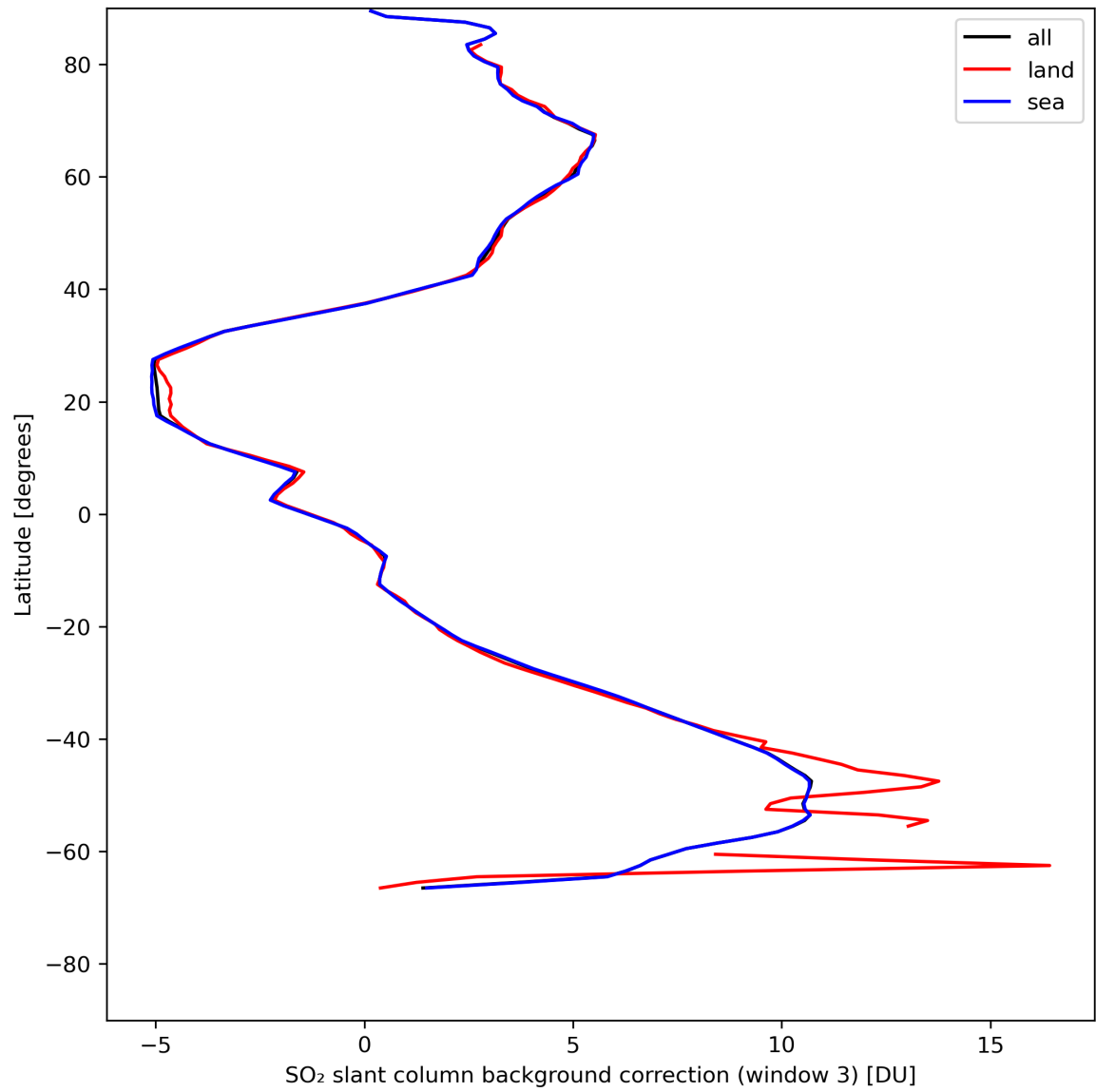
Figure 44: Zonal average of “SO 2 slant column background correction (window 3)” for 2023-07-29 to 2023-07-31.
