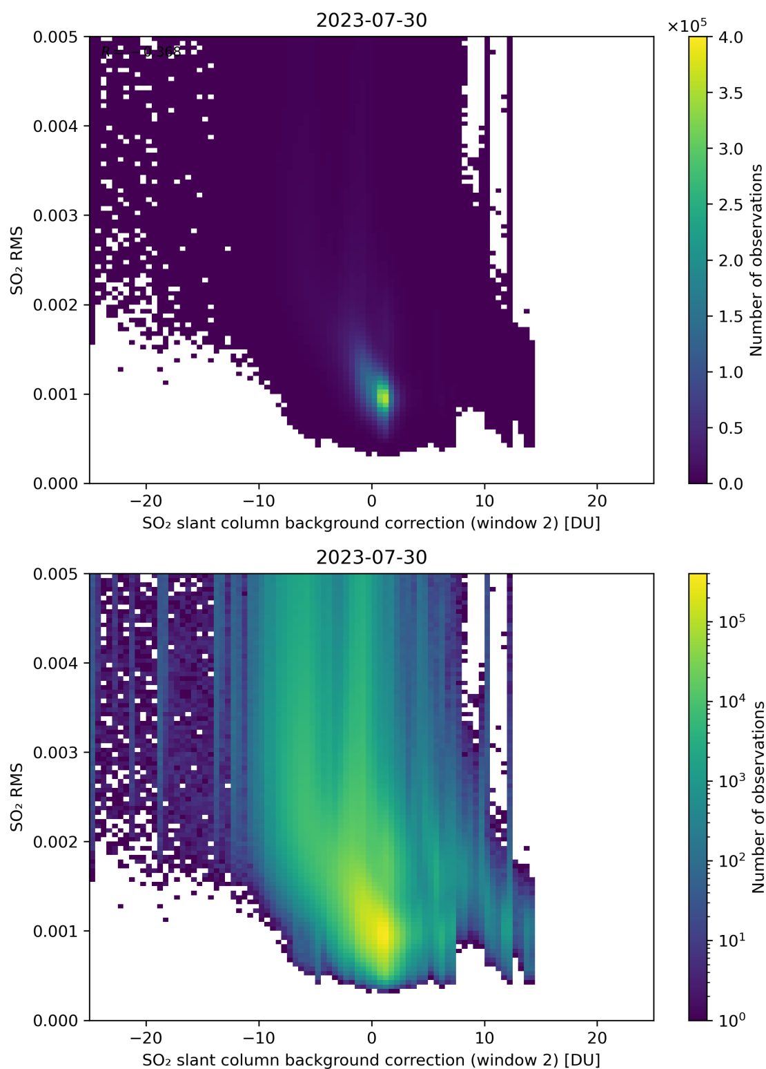
Figure 114: Scatter density plot of “SO 2 slant column background correction (window 2)” against “SO 2 RMS” for 2023-07-29 to 2023-07-31.
