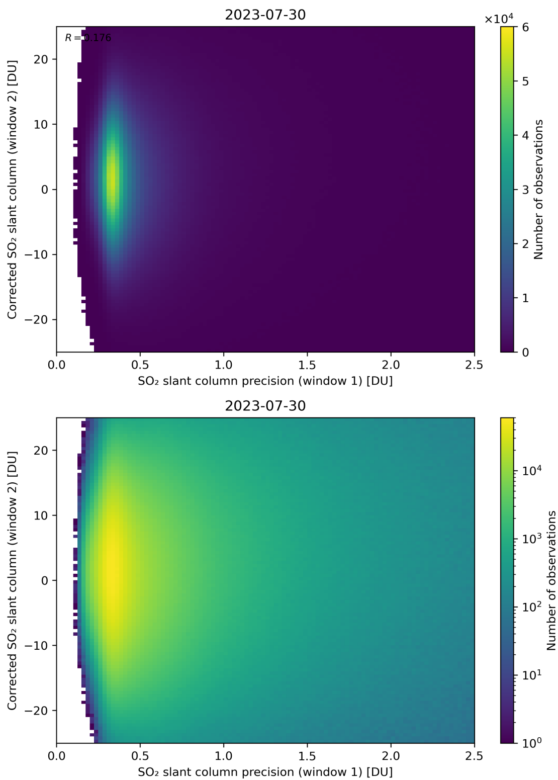
Figure 225: Scatter density plot of “SO 2 slant column precision (window 1)” against “Corrected SO 2 slant column (window 2)” for 2023-07-29 to 2023-07-31.
