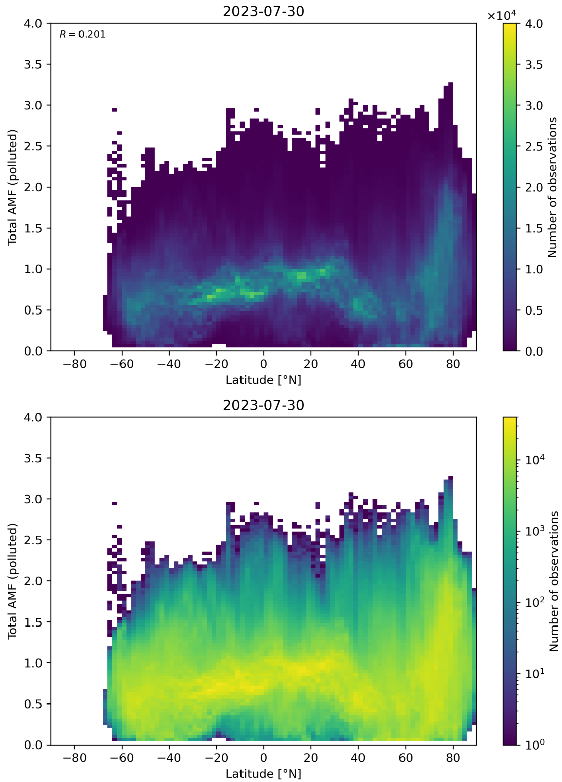
Figure 154: Scatter density plot of “Latitude” against “Total AMF (polluted)” for 2023-07-29 to 2023-07-31.
