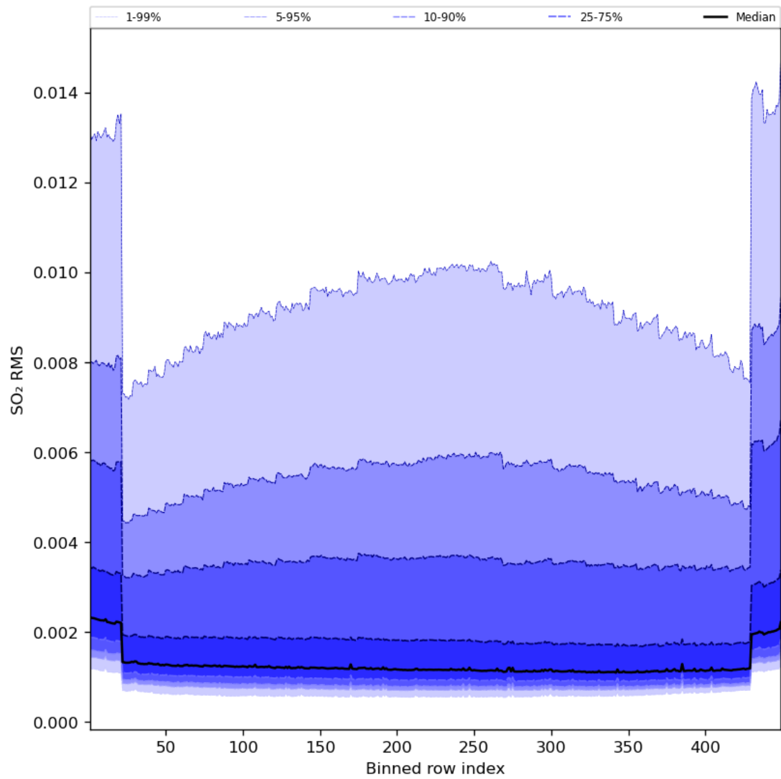
Figure 93: Along track statistics of “SO 2 RMS” for 2023-07-29 to 2023-07-31
