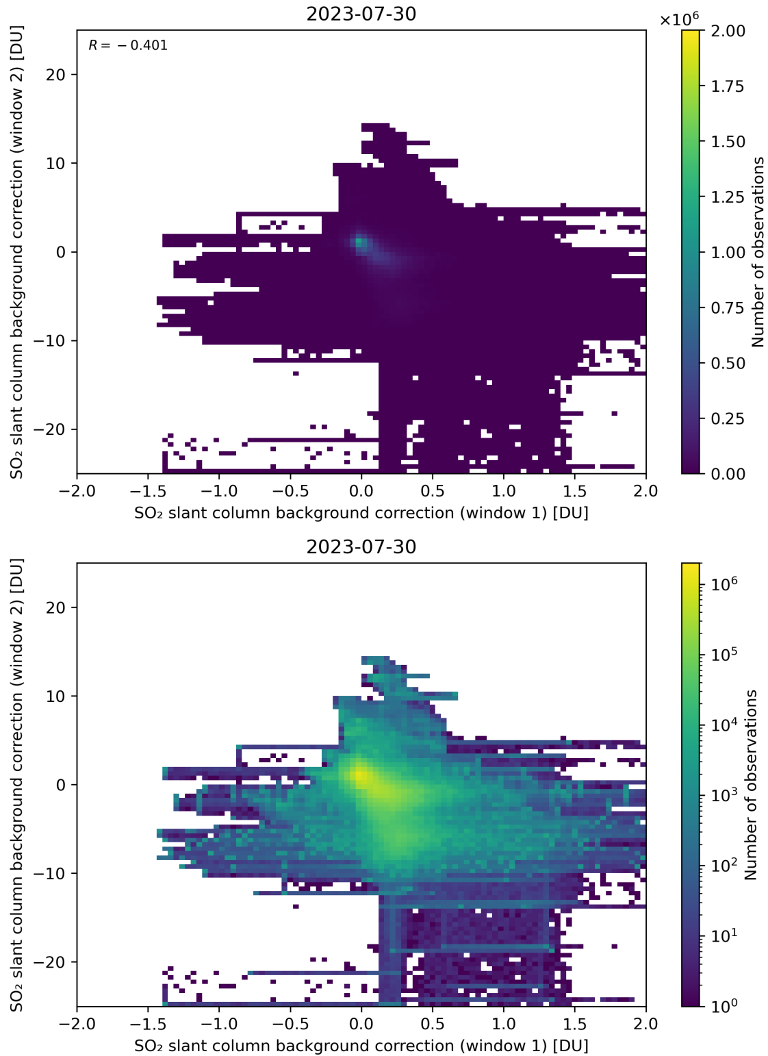
Figure 98: Scatter density plot of “SO 2 slant column background correction (window 1)” against “SO 2 slant column background correction (window 2)” for 2023-07-29 to 2023-07-31.
