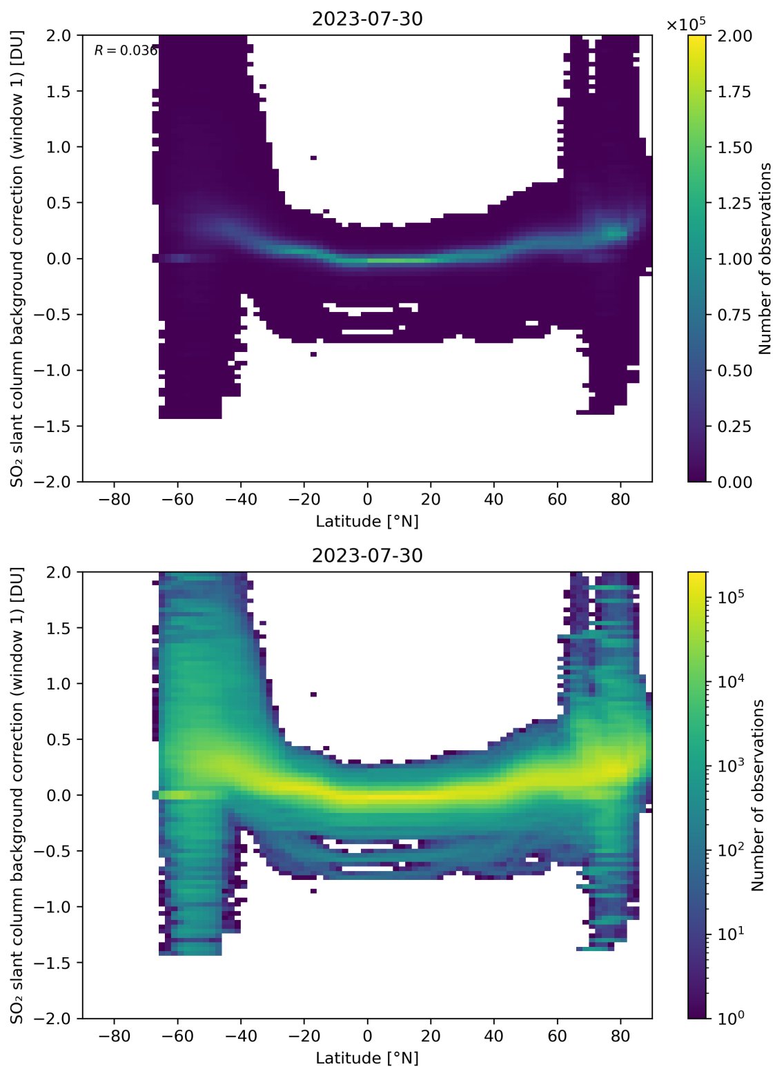
Figure 139: Scatter density plot of “Latitude” against “SO 2 slant column background correction (window 1)” for 2023-07-29 to 2023-07-31.
