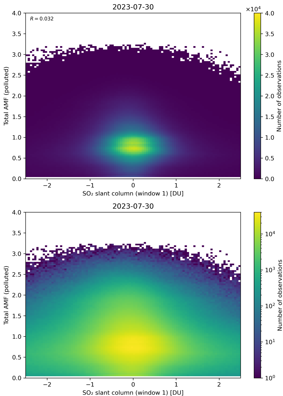
Figure 239: Scatter density plot of “SO 2 slant column (window 1)” against “Total AMF (polluted)” for 2023-07-29 to 2023-07-31.
