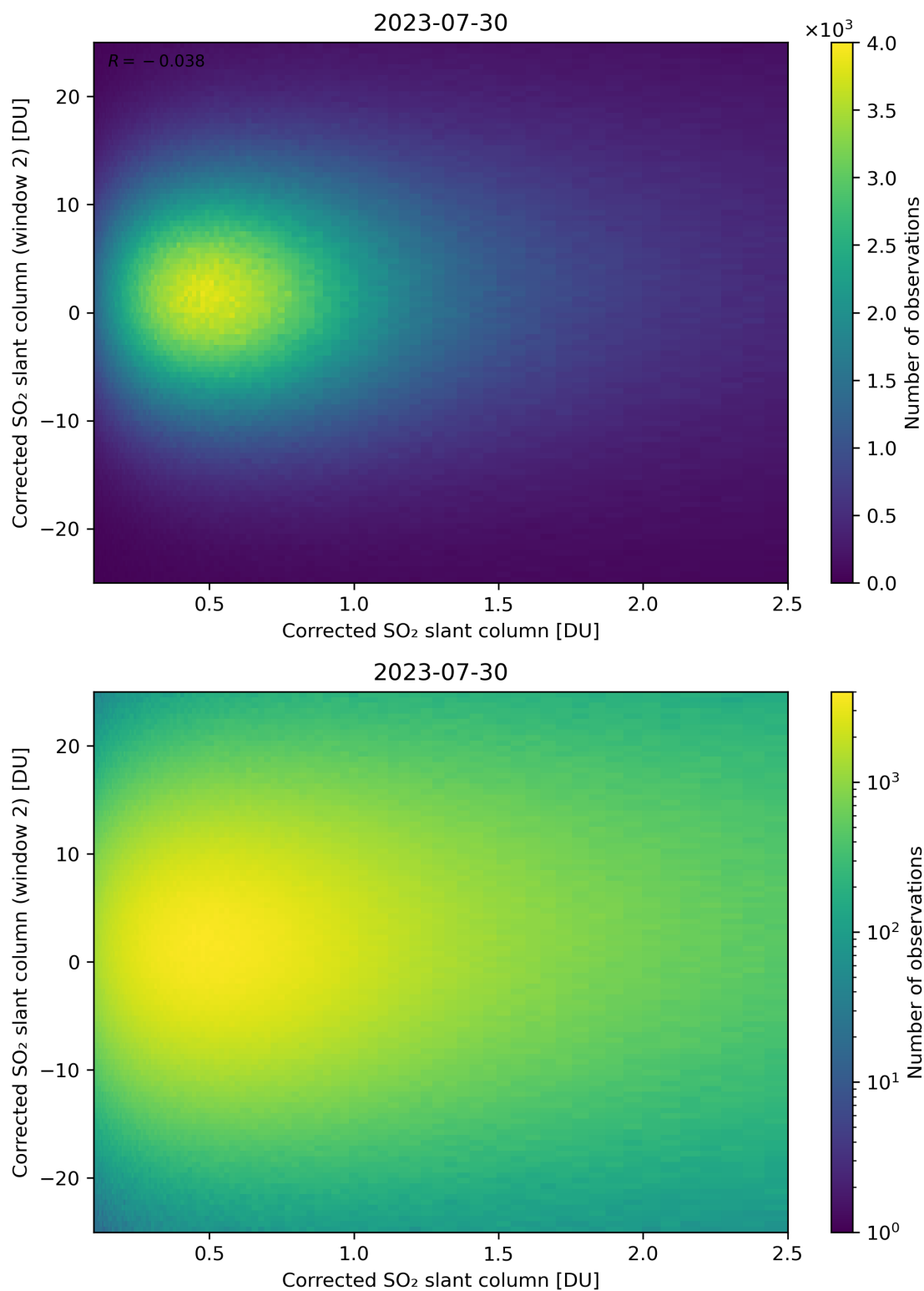
Figure 185: Scatter density plot of “Corrected SO 2 slant column” against “Corrected SO 2 slant column (window 2)” for 2023-07-29 to 2023-07-31.
