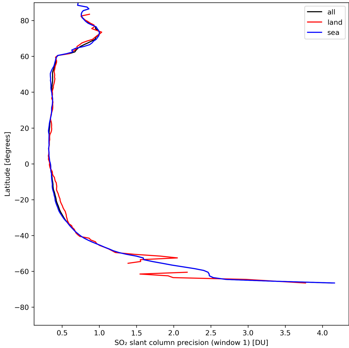
Figure 34: Zonal average of “SO 2 slant column precision (window 1)” for 2023-07-29 to 2023-07-31.
