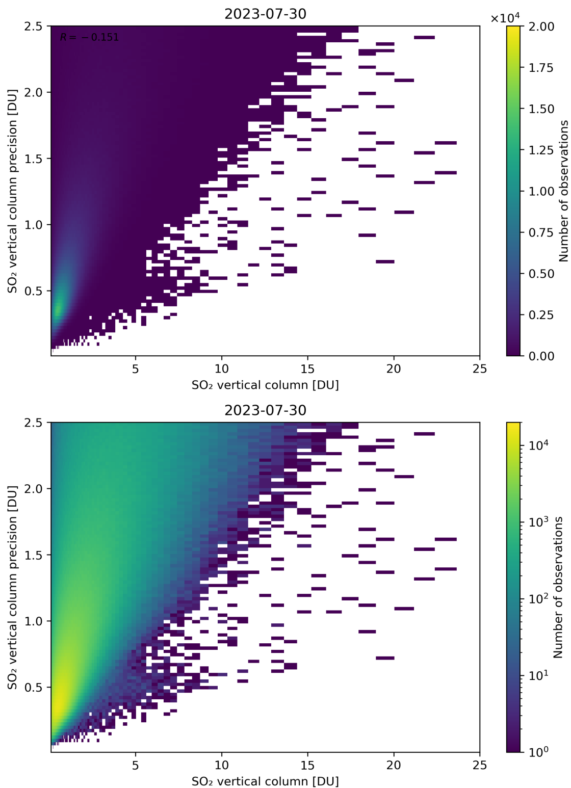
Figure 307: Scatter density plot of “SO 2 vertical column” against “SO 2 vertical column precision” for 2023-07-29 to 2023-07-31.
