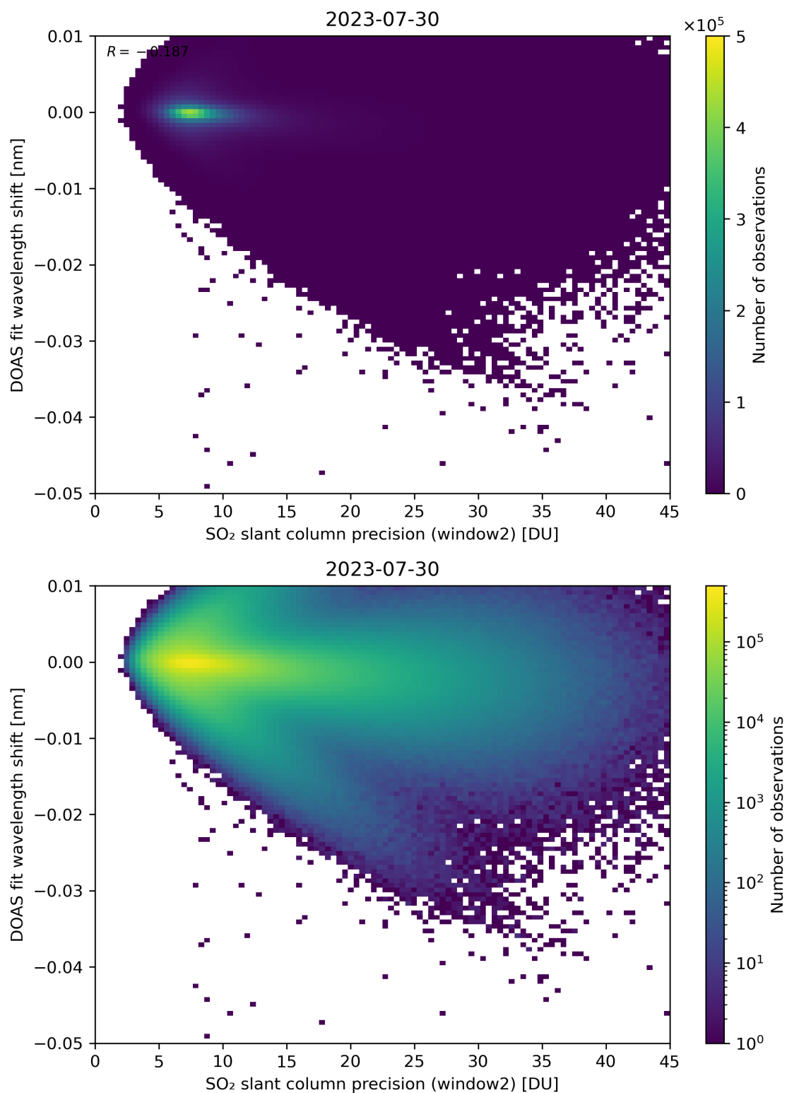
Figure 243: Scatter density plot of “SO 2 slant column precision (window2)” against “DOAS fit wavelength shift” for 2023-07-29 to 2023-07-31.
