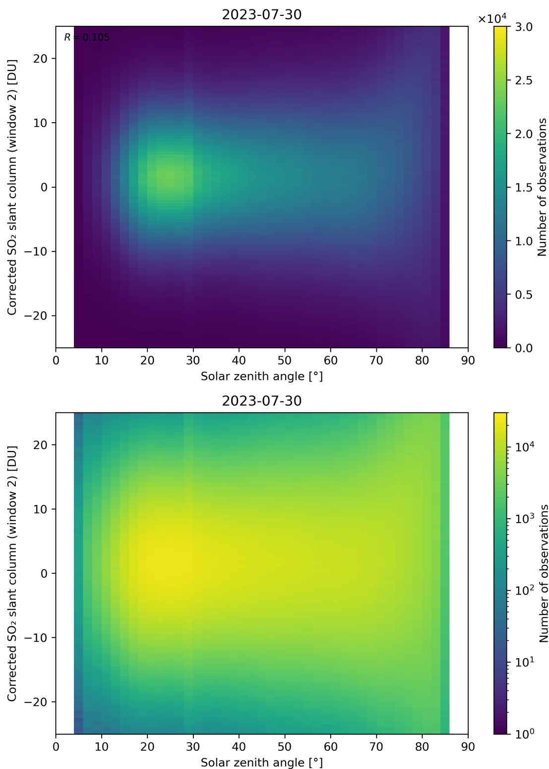
Figure 167: Scatter density plot of “Solar zenith angle” against “Corrected SO 2 slant column (window 2)” for 2023-07-29 to 2023-07-31.
