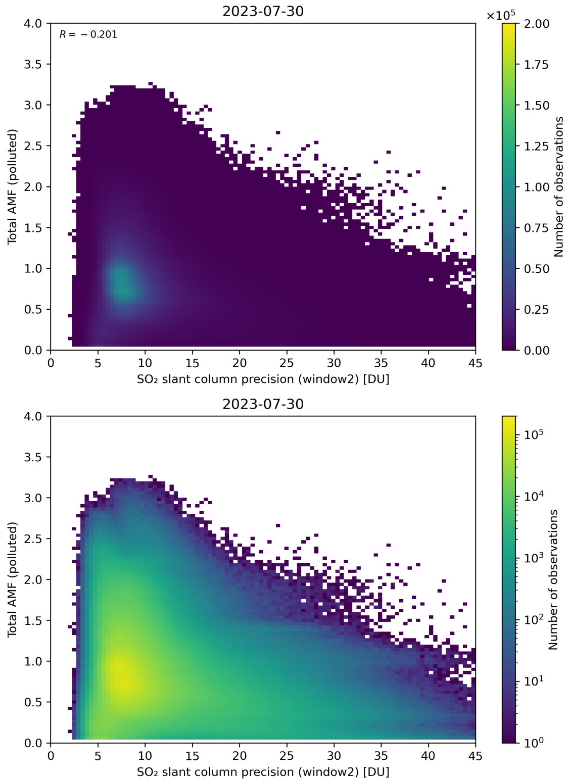
Figure 251: Scatter density plot of “SO 2 slant column precision (window2)” against “Total AMF (polluted)” for 2023-07-29 to 2023-07-31.
