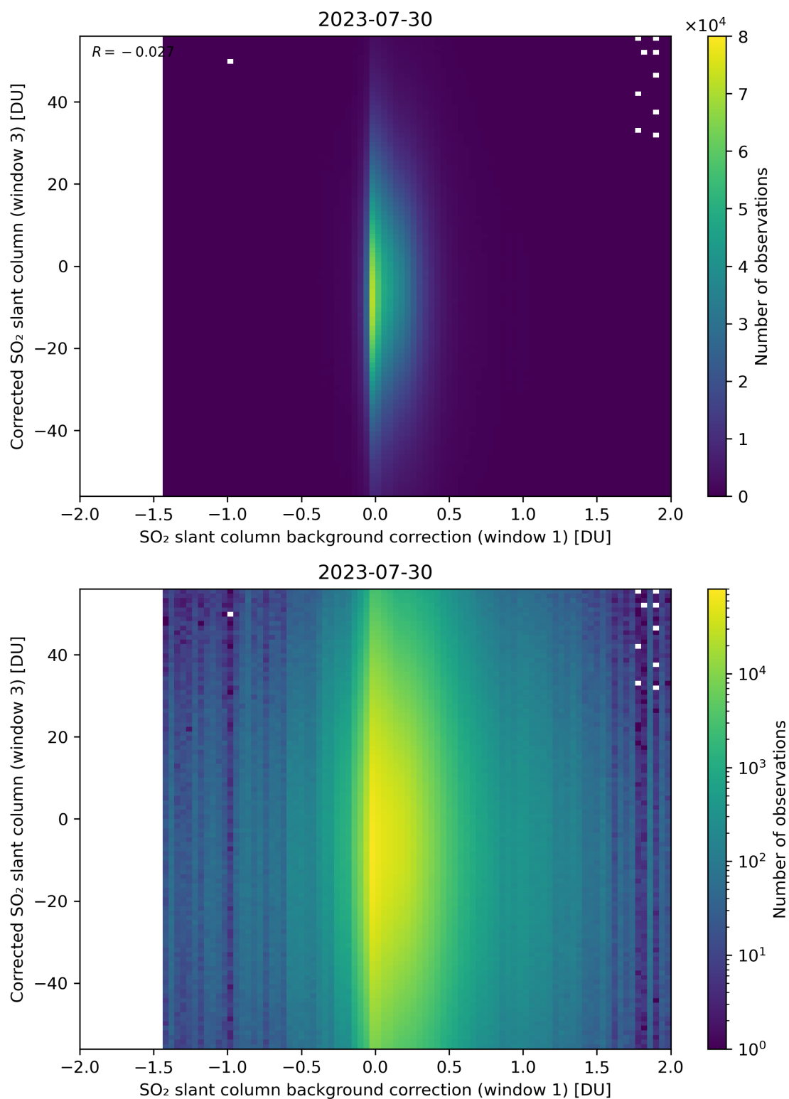
Figure 105: Scatter density plot of “SO 2 slant column background correction (window 1)” against “Corrected SO 2 slant column (window 3)” for 2023-07-29 to 2023-07-31.
