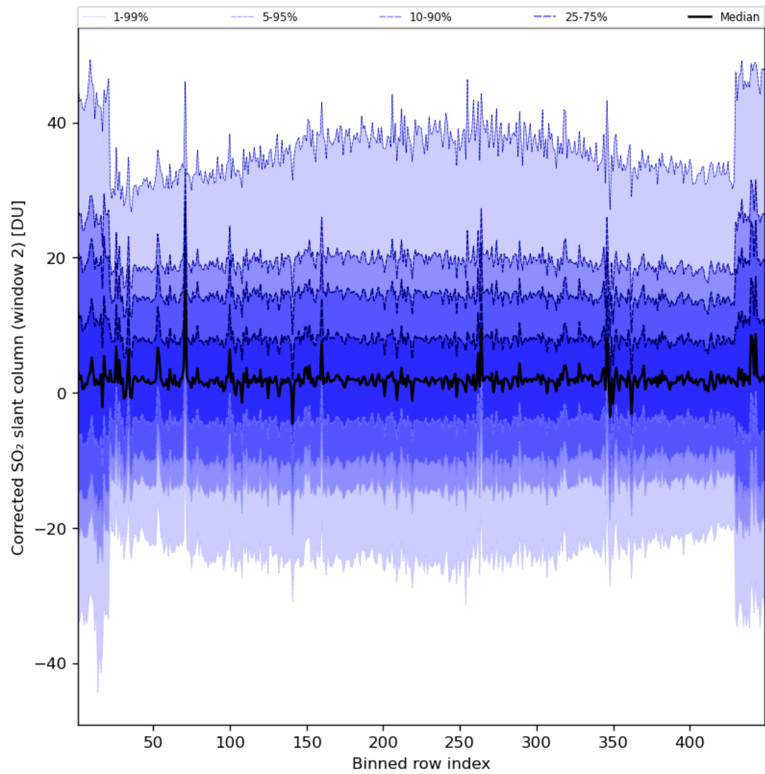
Figure 85: Along track statistics of “Corrected SO 2 slant column (window 2)” for 2023-07-29 to 2023-07-31
