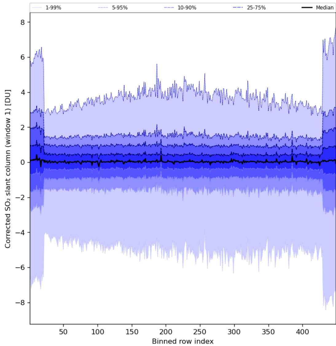
Figure 81: Along track statistics of “Corrected SO 2 slant column (window 1)” for 2023-07-29 to 2023-07-31
