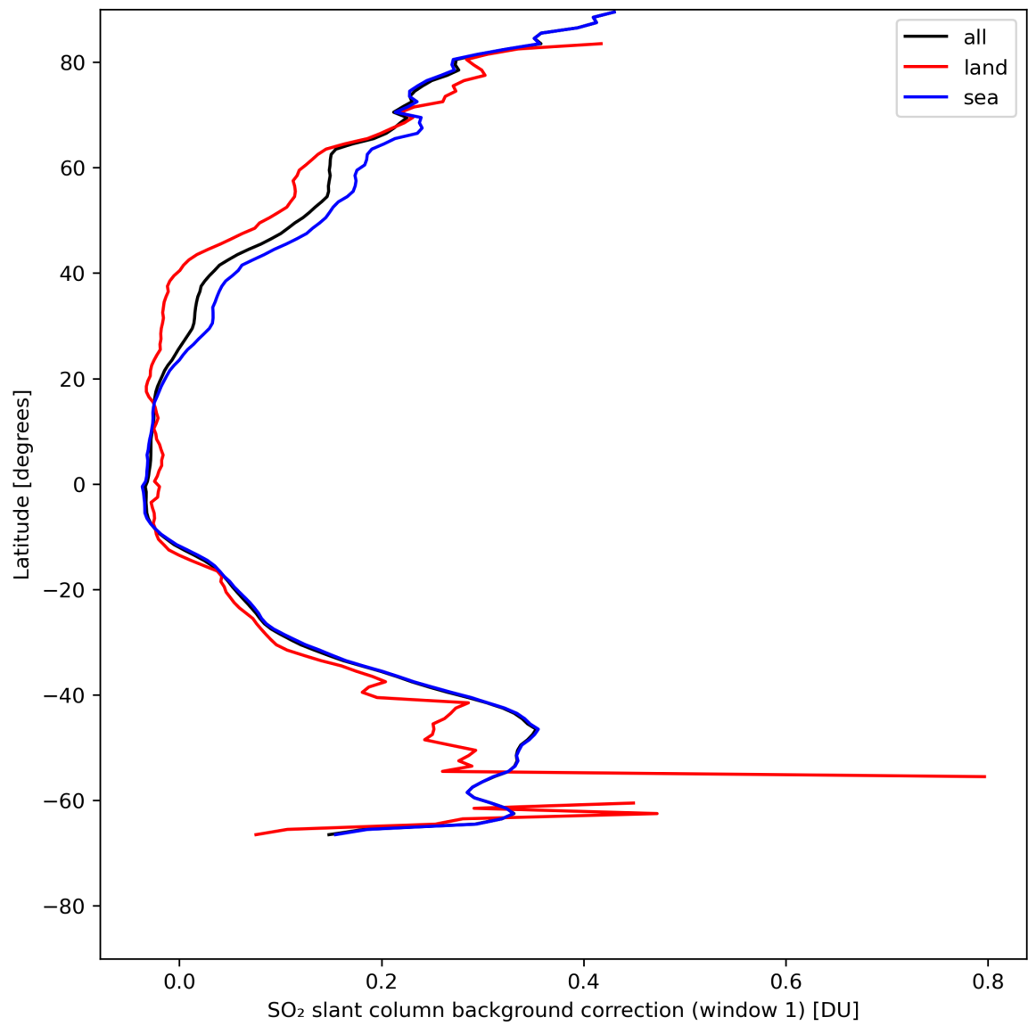
Figure 36: Zonal average of "SO 2 slant column background correction (window 1)" for 2023-07-29 to 2023-07-31.
