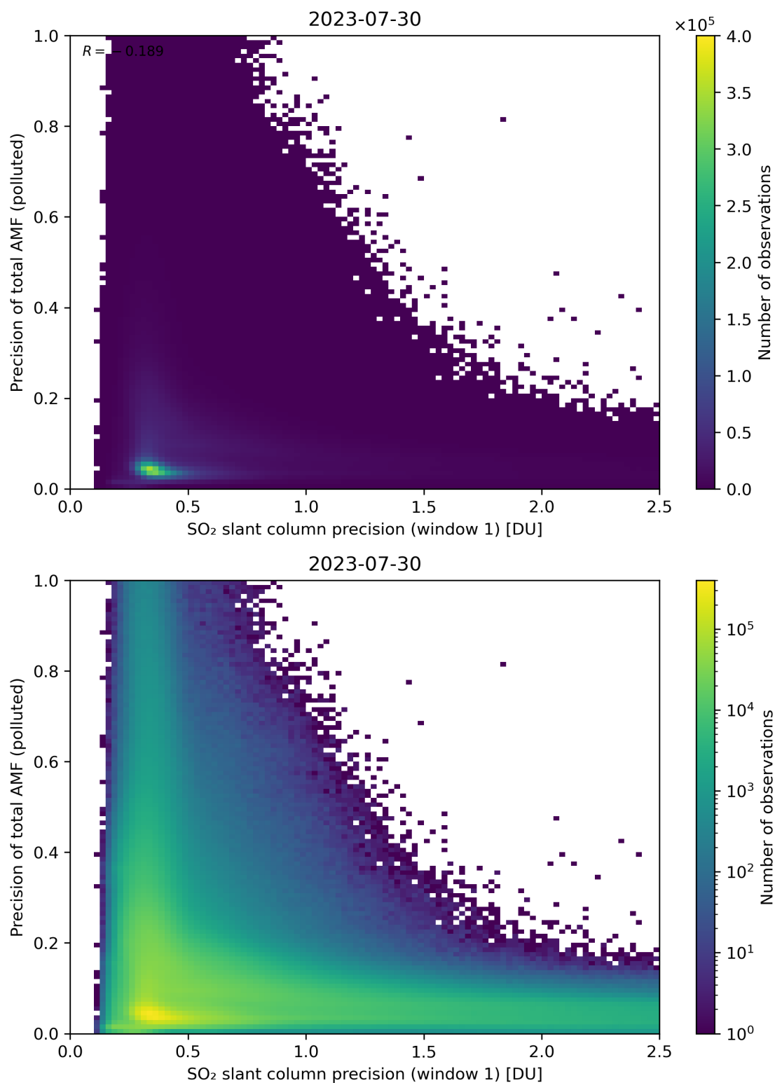
Figure 231: Scatter density plot of “SO 2 slant column precision (window 1)” against “Precision of total AMF (polluted)” for 2023-07-29 to 2023-07-31.
