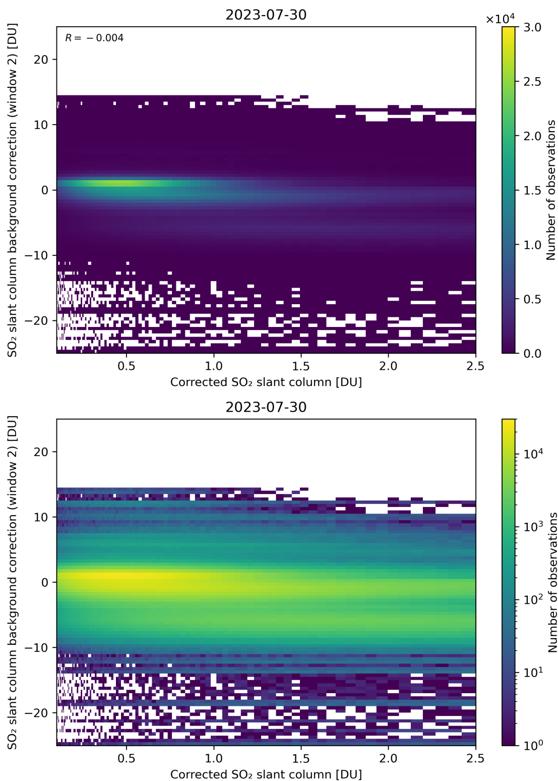
Figure 179: Scatter density plot of “Corrected SO 2 slant column” against “SO 2 slant column background correction (window 2)” for 2023-07-29 to 2023-07-31.
