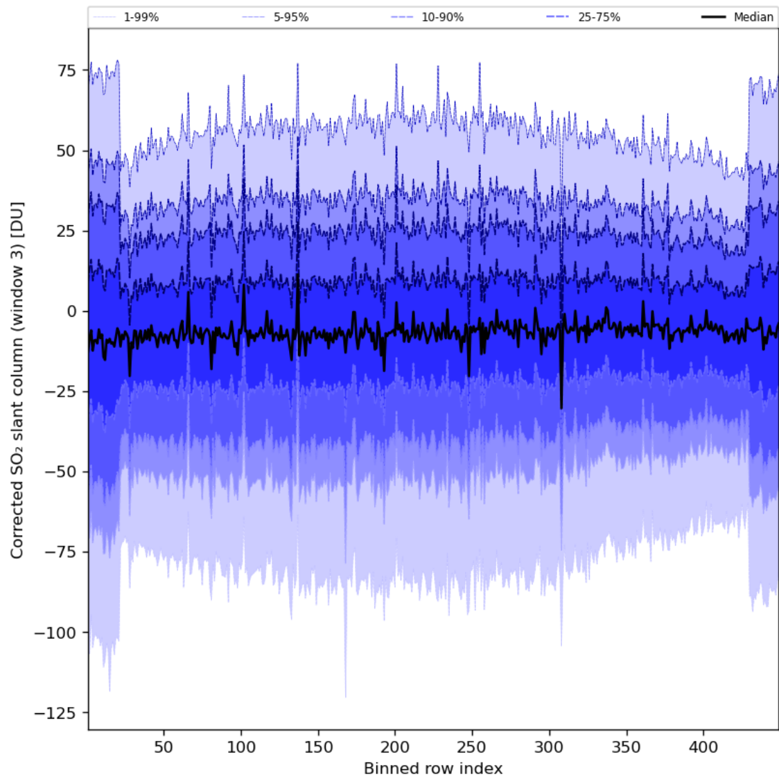
Figure 89: Along track statistics of “Corrected SO 2 slant column (window 3)” for 2023-07-29 to 2023-07-31
