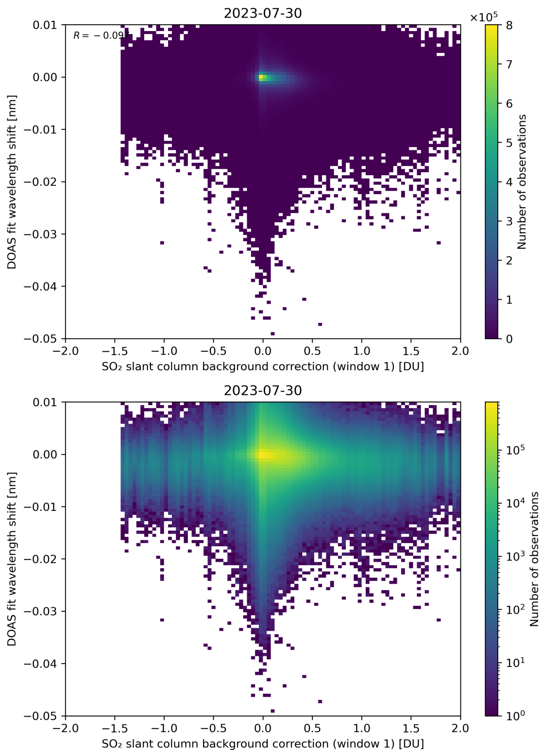
Figure 100: Scatter density plot of “SO 2 slant column background correction (window 1)” against “DOAS fit wavelength shift” for 2023-07-29 to 2023-07-31.
