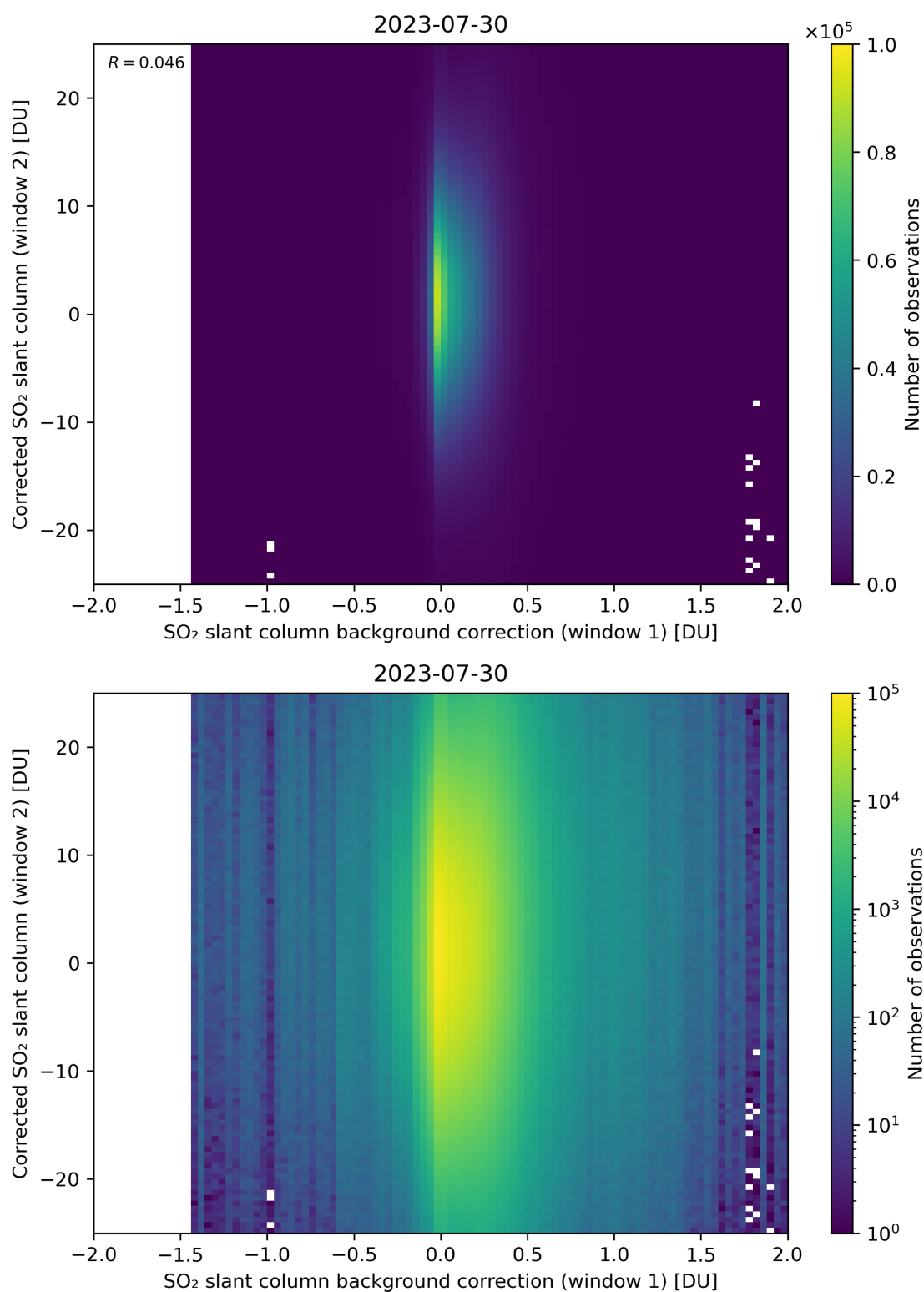
Figure 104: Scatter density plot of “SO 2 slant column background correction (window 1)” against “Corrected SO 2 slant column (window 2)” for 2023-07-29 to 2023-07-31.
