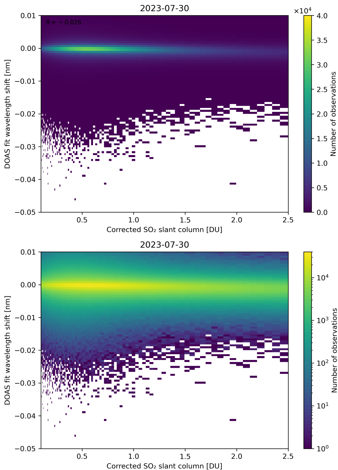
Figure 181: Scatter density plot of “Corrected SO 2 slant column” against “DOAS fit wavelength shift” for 2023-07-29 to 2023-07-31.
