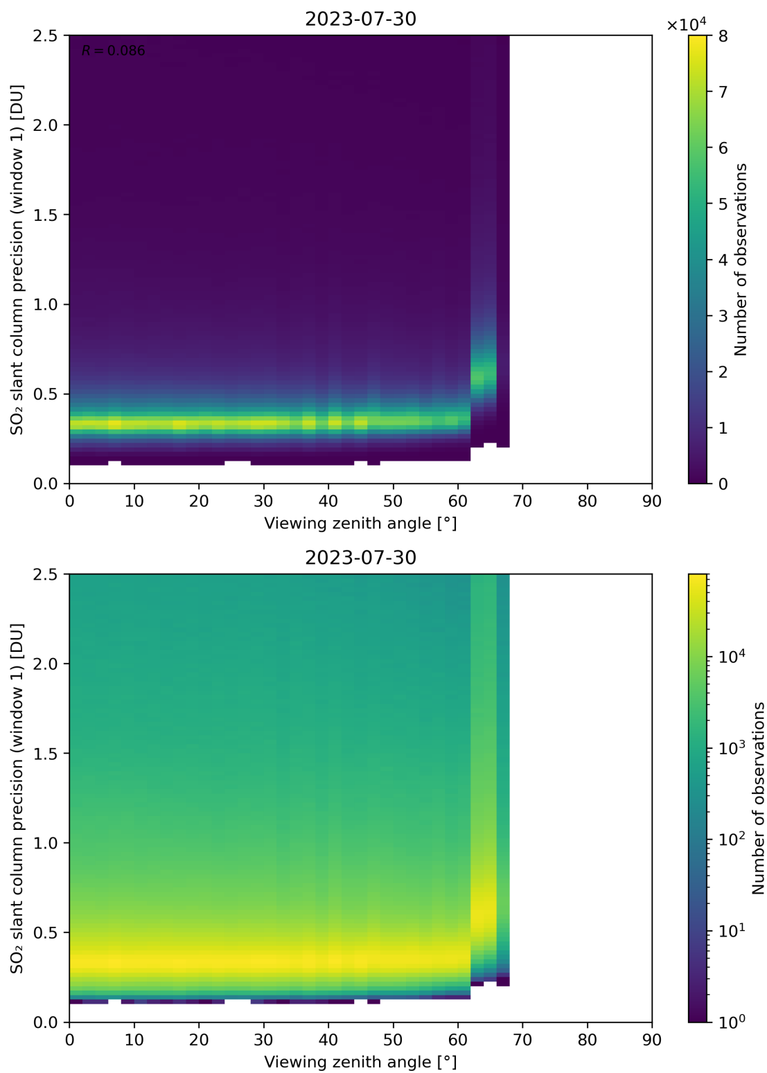
Figure 321: Scatter density plot of “Viewing zenith angle” against “SO 2 slant column precision (window 1)” for 2023-07-29 to 2023-07-31.
