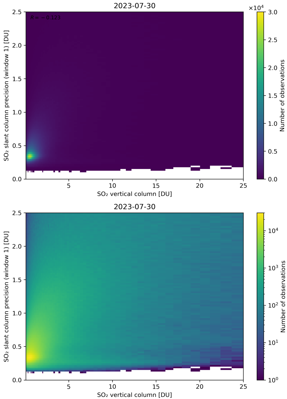
Figure 301: Scatter density plot of “SO 2 vertical column” against “SO 2 slant column precision (window 1)” for 2023-07-29 to 2023-07-31.
