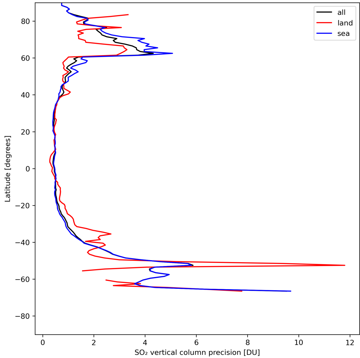
Figure 31: Zonal average of “SO 2 vertical column precision” for 2023-07-29 to 2023-07-31.
