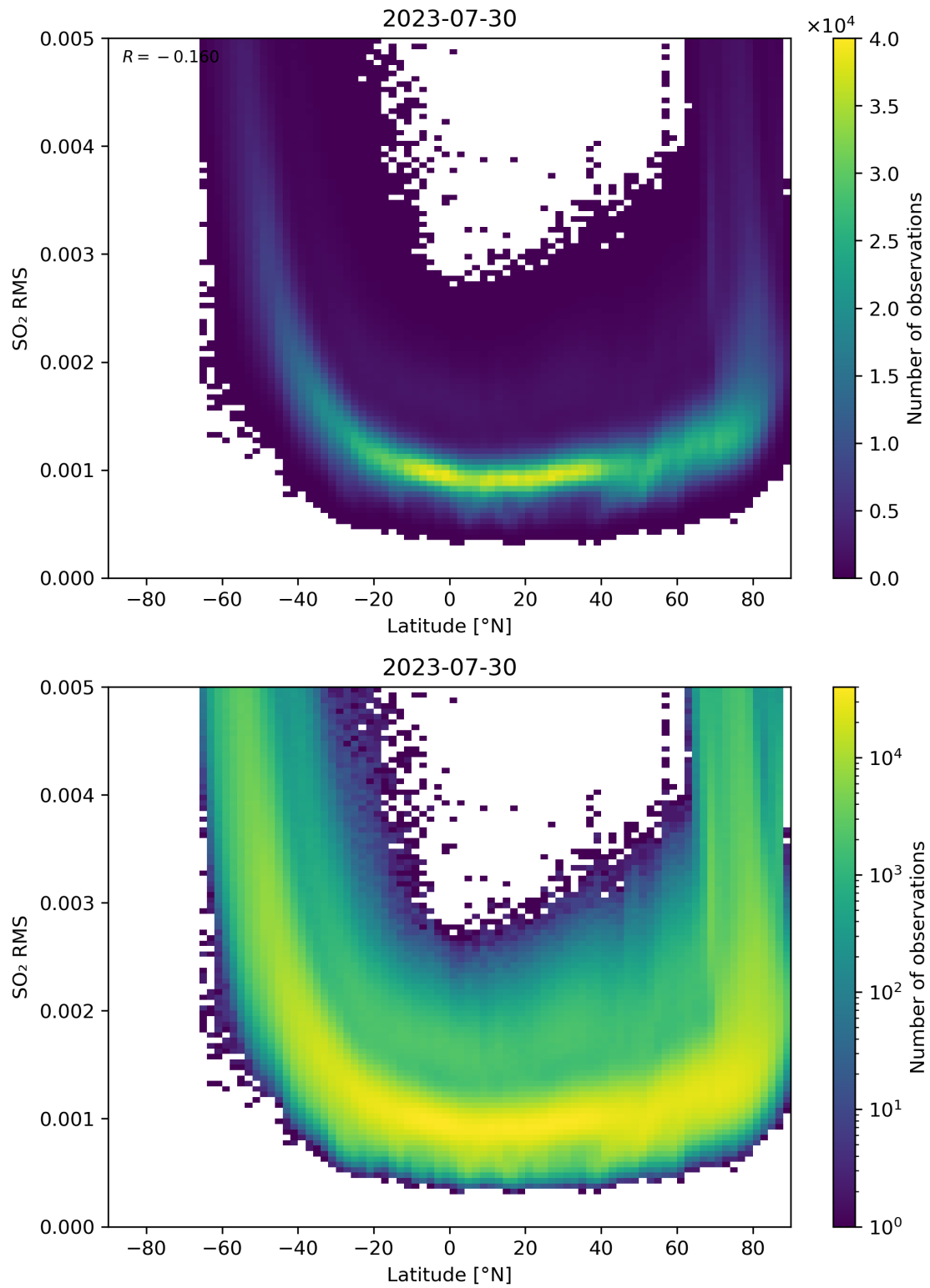
Figure 144: Scatter density plot of “Latitude” against “SO 2 RMS” for 2023-07-29 to 2023-07-31.
