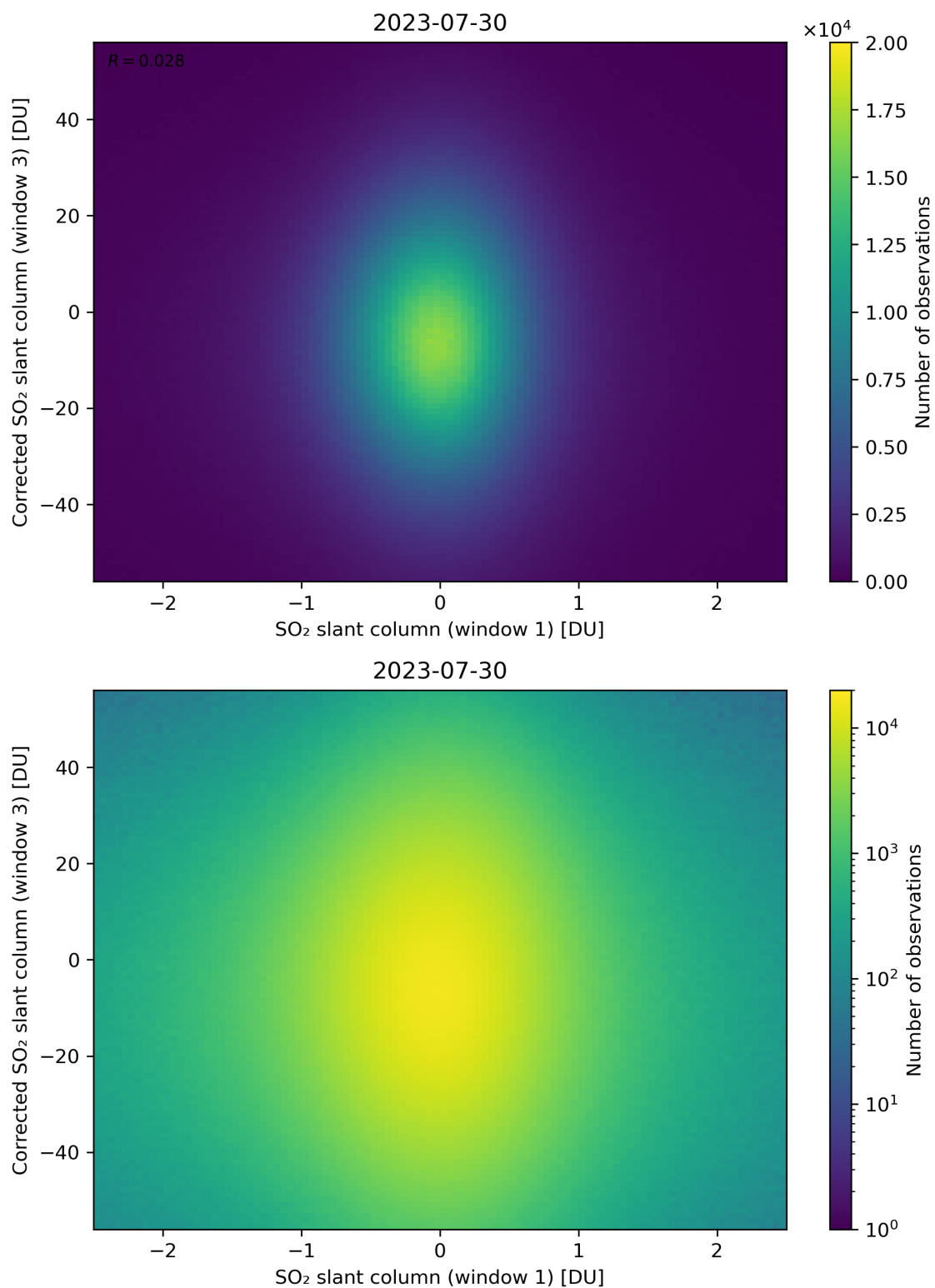
Figure 234: Scatter density plot of “SO 2 slant column (window 1)” against “Corrected SO 2 slant column (window 3)” for 2023-07-29 to 2023-07-31.
