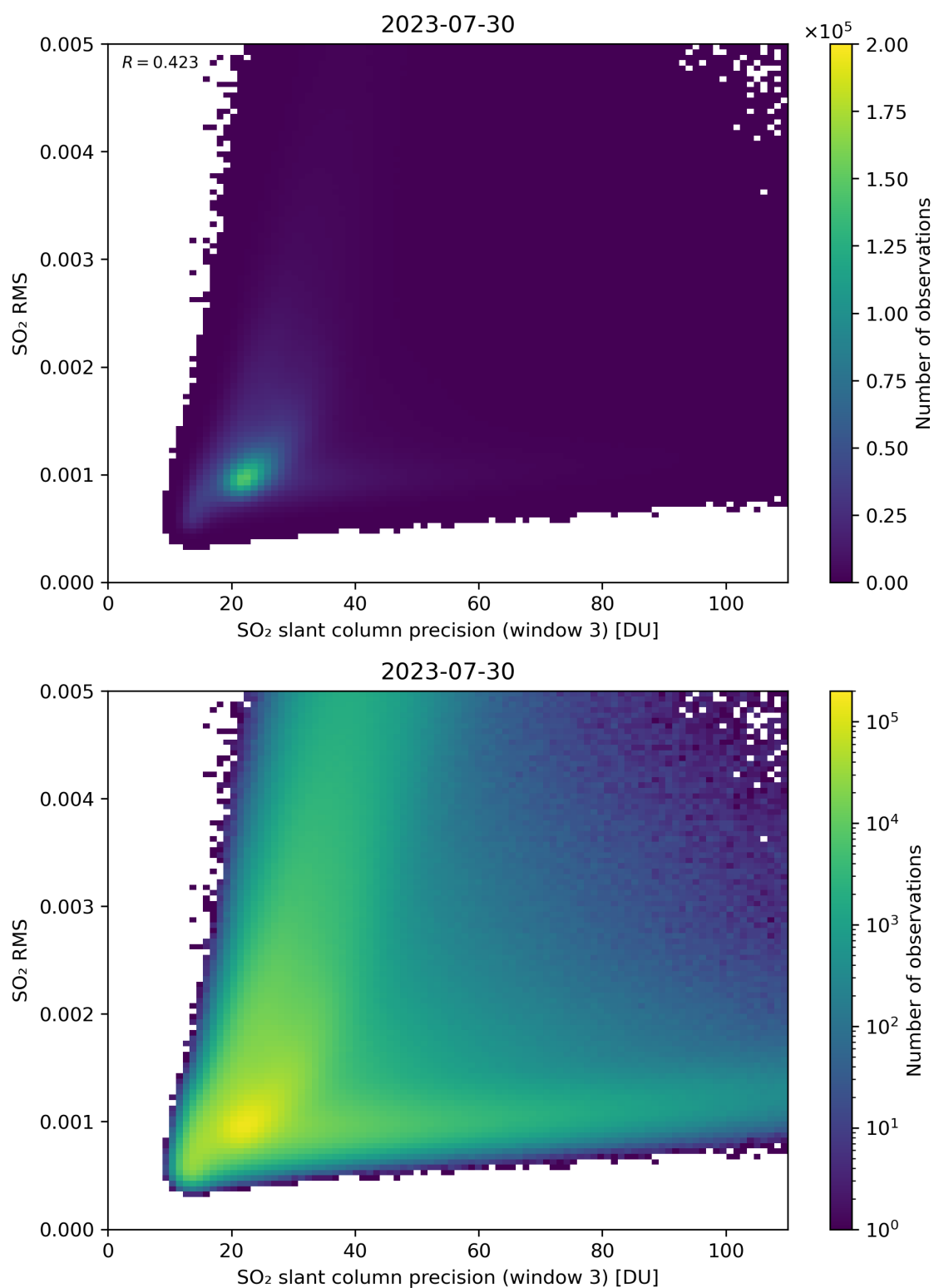
Figure 260: Scatter density plot of “SO 2 slant column precision (window 3)” against “SO 2 RMS” for 2023-07-29 to 2023-07-31.
