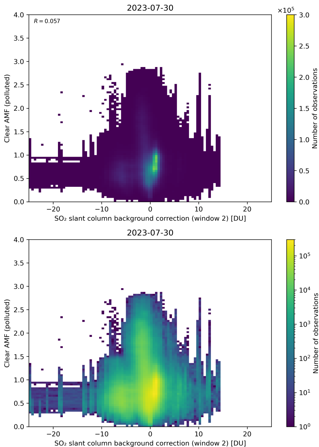
Figure 115: Scatter density plot of “SO 2 slant column background correction (window 2)” against “Clear AMF (polluted)” for 2023-07-29 to 2023-07-31.
