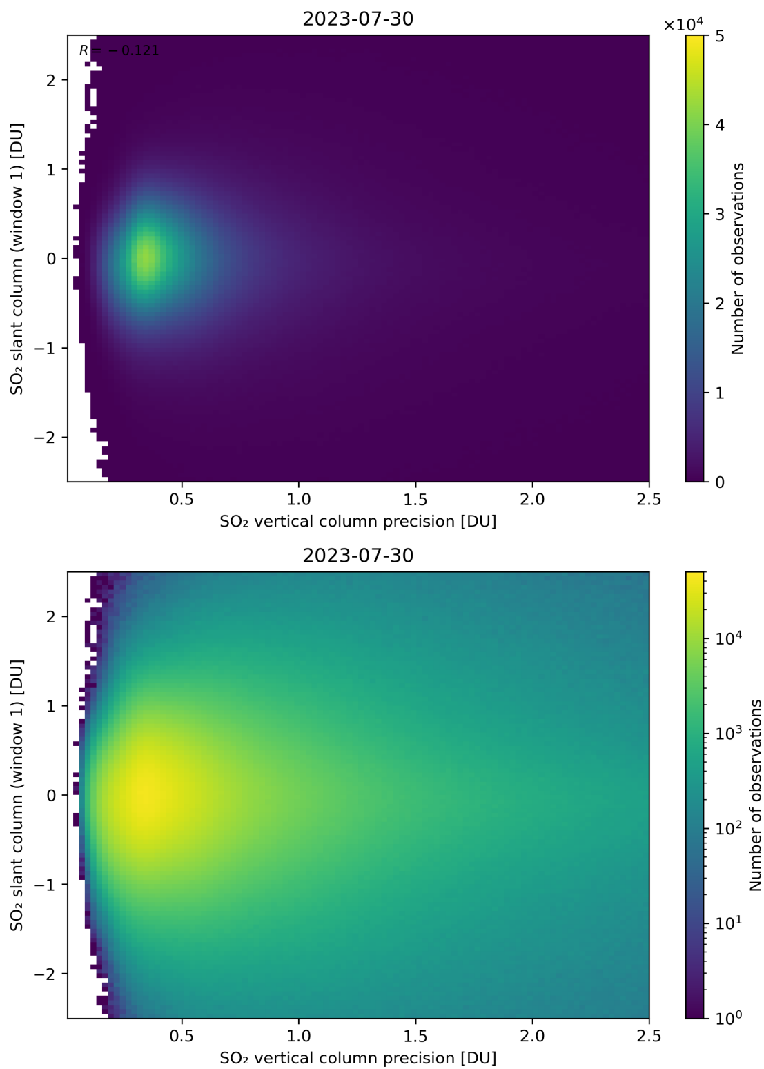
Figure 289: Scatter density plot of “SO 2 vertical column precision” against “SO 2 slant column (window 1)” for 2023-07-29 to 2023-07-31.
