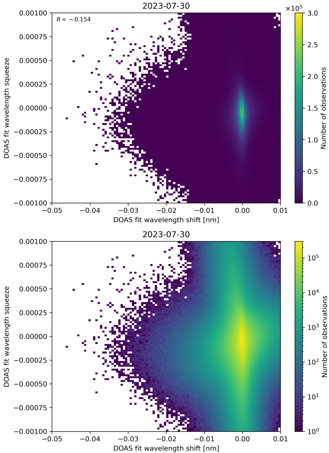
Figure 127: Scatter density plot of “DOAS fit wavelength shift” against “DOAS fit wavelength squeeze” for 2023-07-29 to 2023-07-31.
