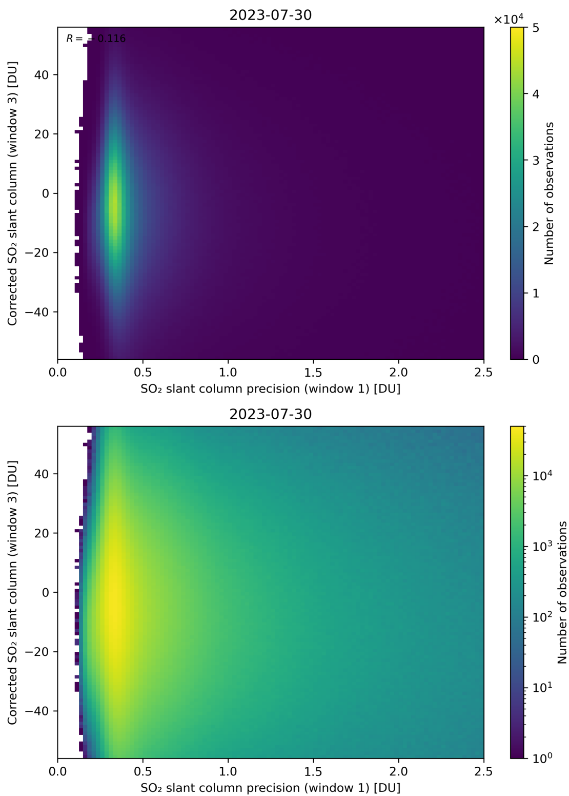
Figure 226: Scatter density plot of “SO 2 slant column precision (window 1)” against “Corrected SO 2 slant column (window 3)” for 2023-07-29 to 2023-07-31.
