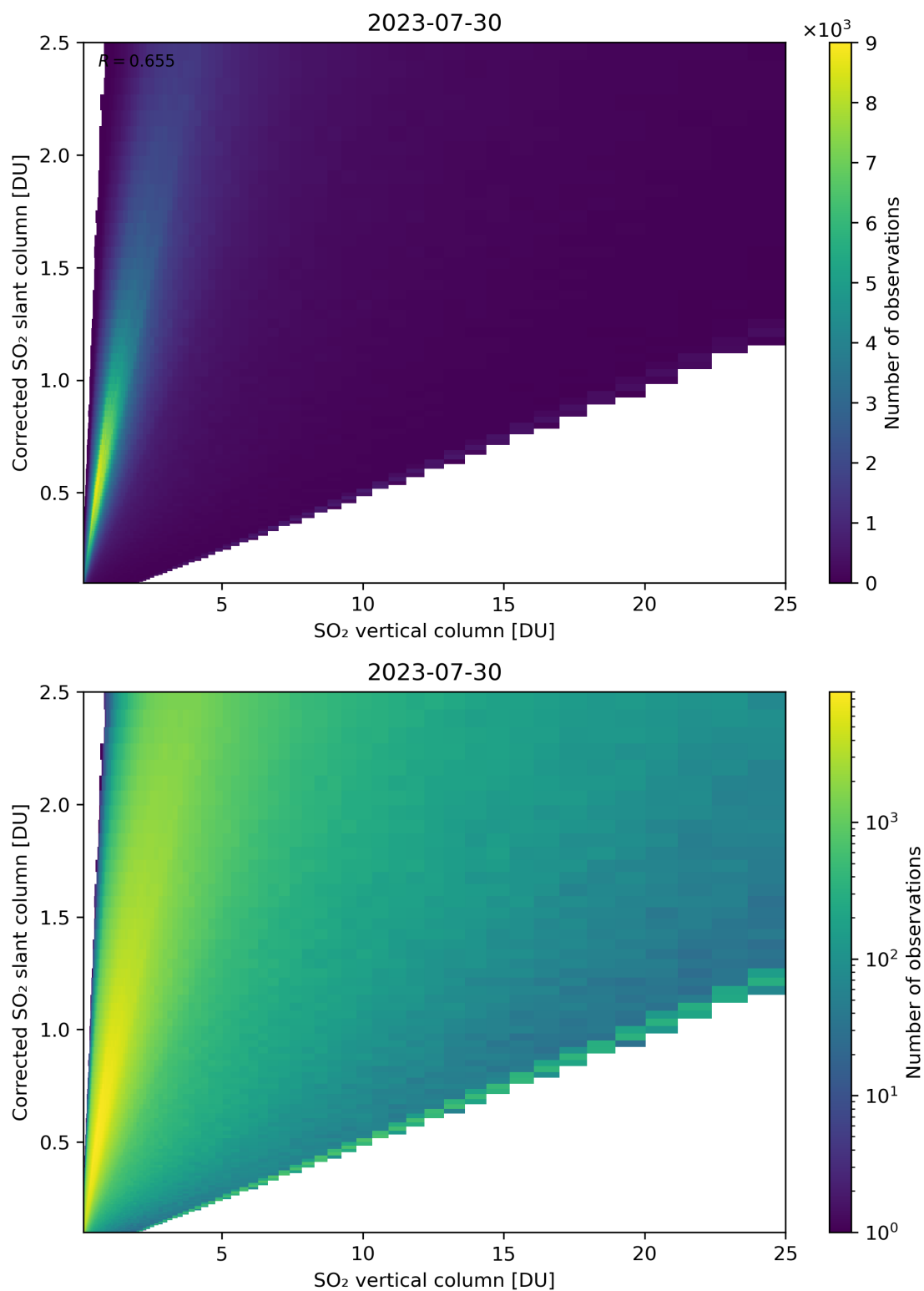
Figure 297: Scatter density plot of “SO 2 vertical column” against “Corrected SO 2 slant column” for 2023-07-29 to 2023-07-31.
