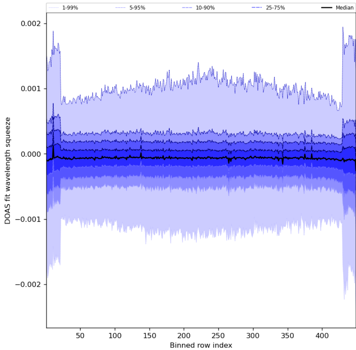
Figure 92: Along track statistics of “DOAS fit wavelength squeeze” for 2023-07-29 to 2023-07-31
