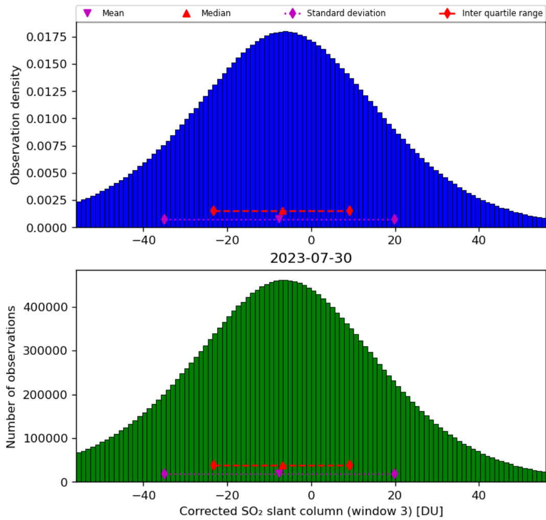
Figure 66: Histogram of “Corrected SO 2 slant column (window 3)” for 2023-07-29 to 2023-07-31
