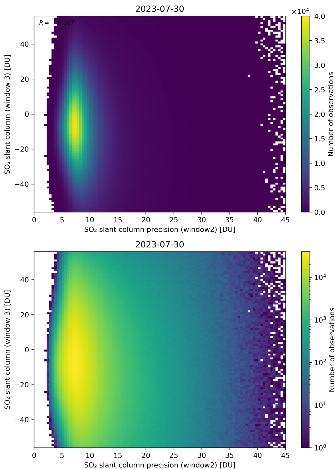
Figure 249: Scatter density plot of “SO 2 slant column precision (window2)” against “SO 2 slant column (window 3)” for 2023-07-29 to 2023-07-31.
