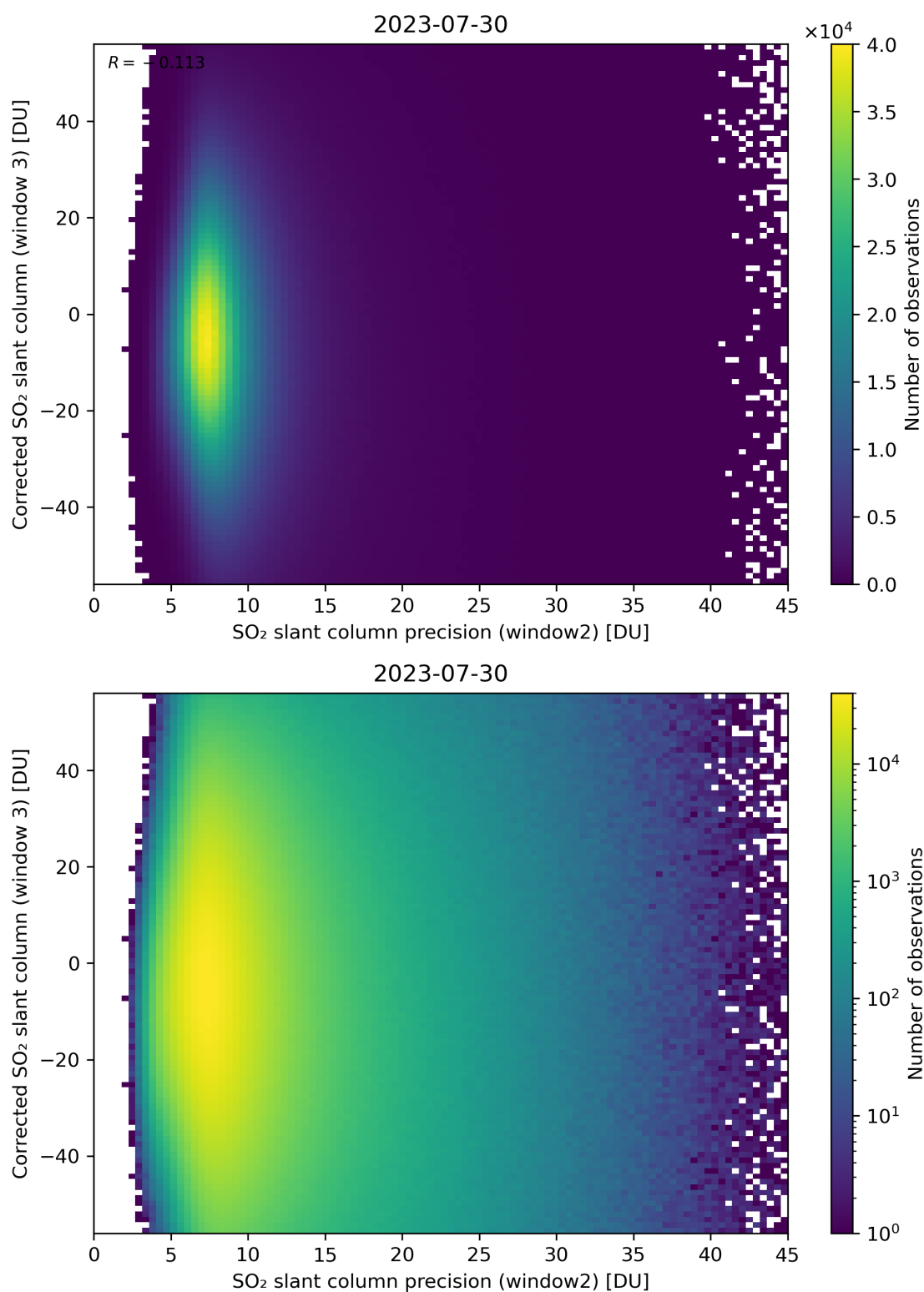
Figure 248: Scatter density plot of “SO 2 slant column precision (window2)” against “Corrected SO 2 slant column (window 3)” for 2023-07-29 to 2023-07-31.
