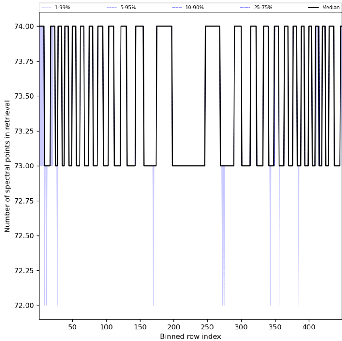
Figure 97: Along track statistics of “Number of spectral points in retrieval” for 2023-07-29 to 2023-07-31
