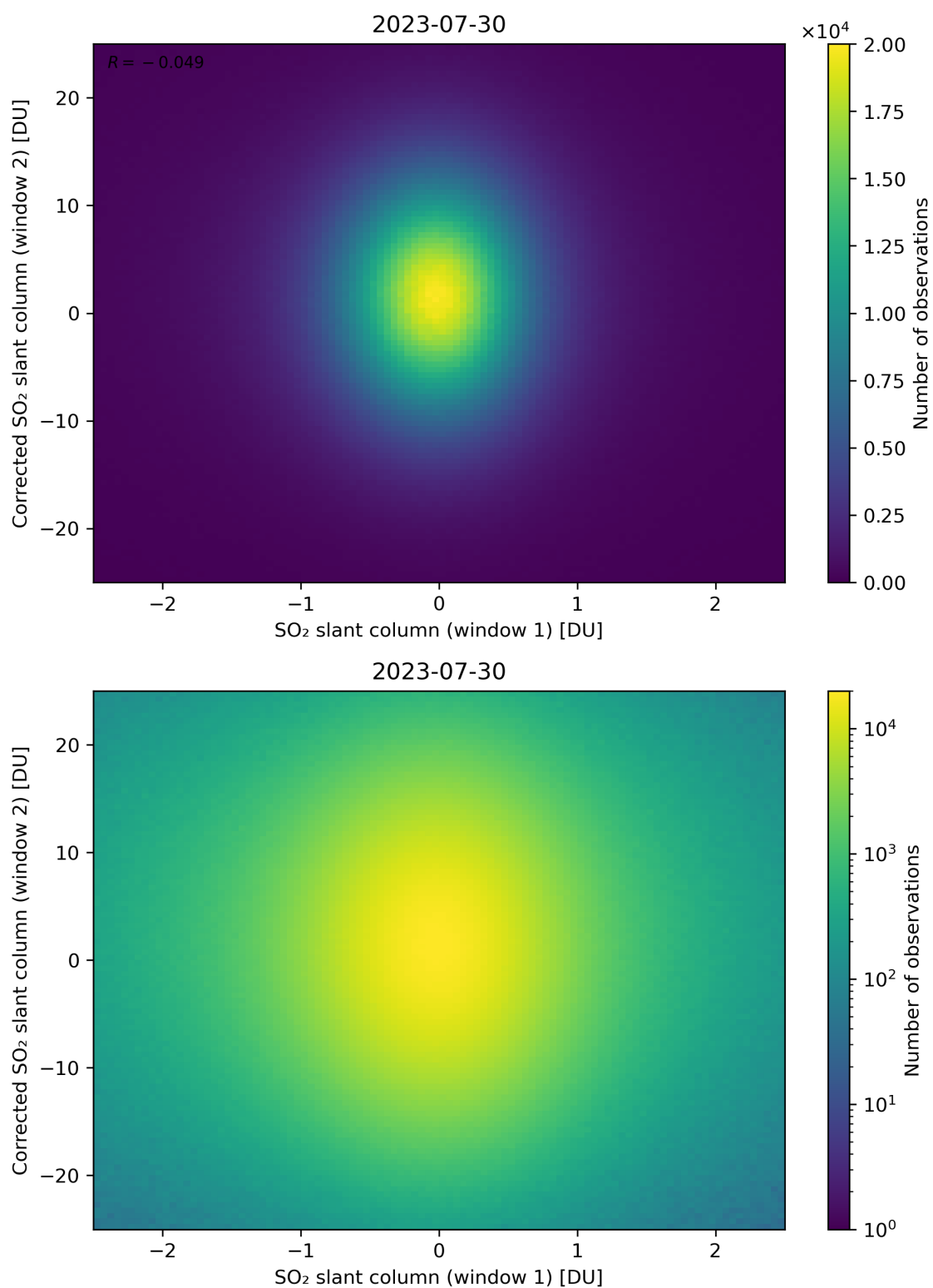
Figure 233: Scatter density plot of “SO 2 slant column (window 1)” against “Corrected SO 2 slant column (window 2)” for 2023-07-29 to 2023-07-31.
