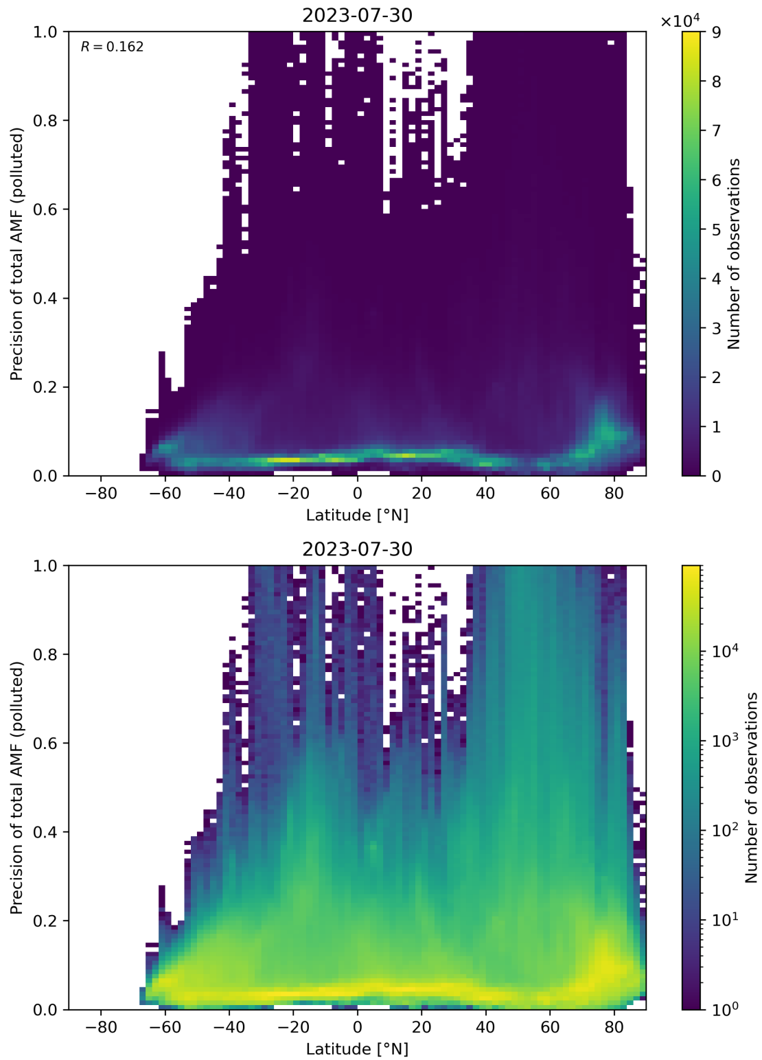
Figure 155: Scatter density plot of “Latitude” against “Precision of total AMF (polluted)” for 2023-07-29 to 2023-07-31.
