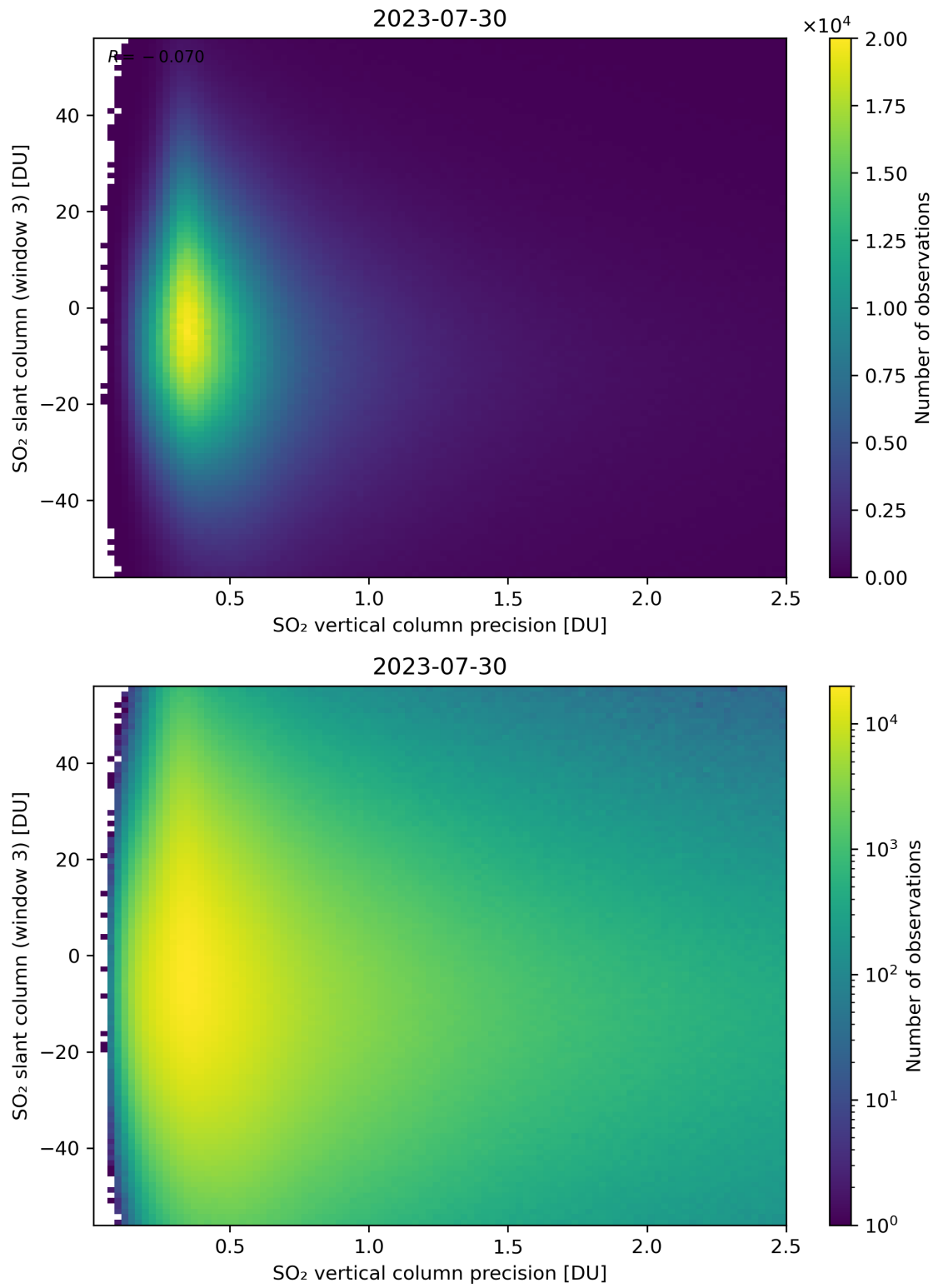
Figure 292: Scatter density plot of “SO 2 vertical column precision” against “SO 2 slant column (window 3)” for 2023-07-29 to 2023-07-31.
