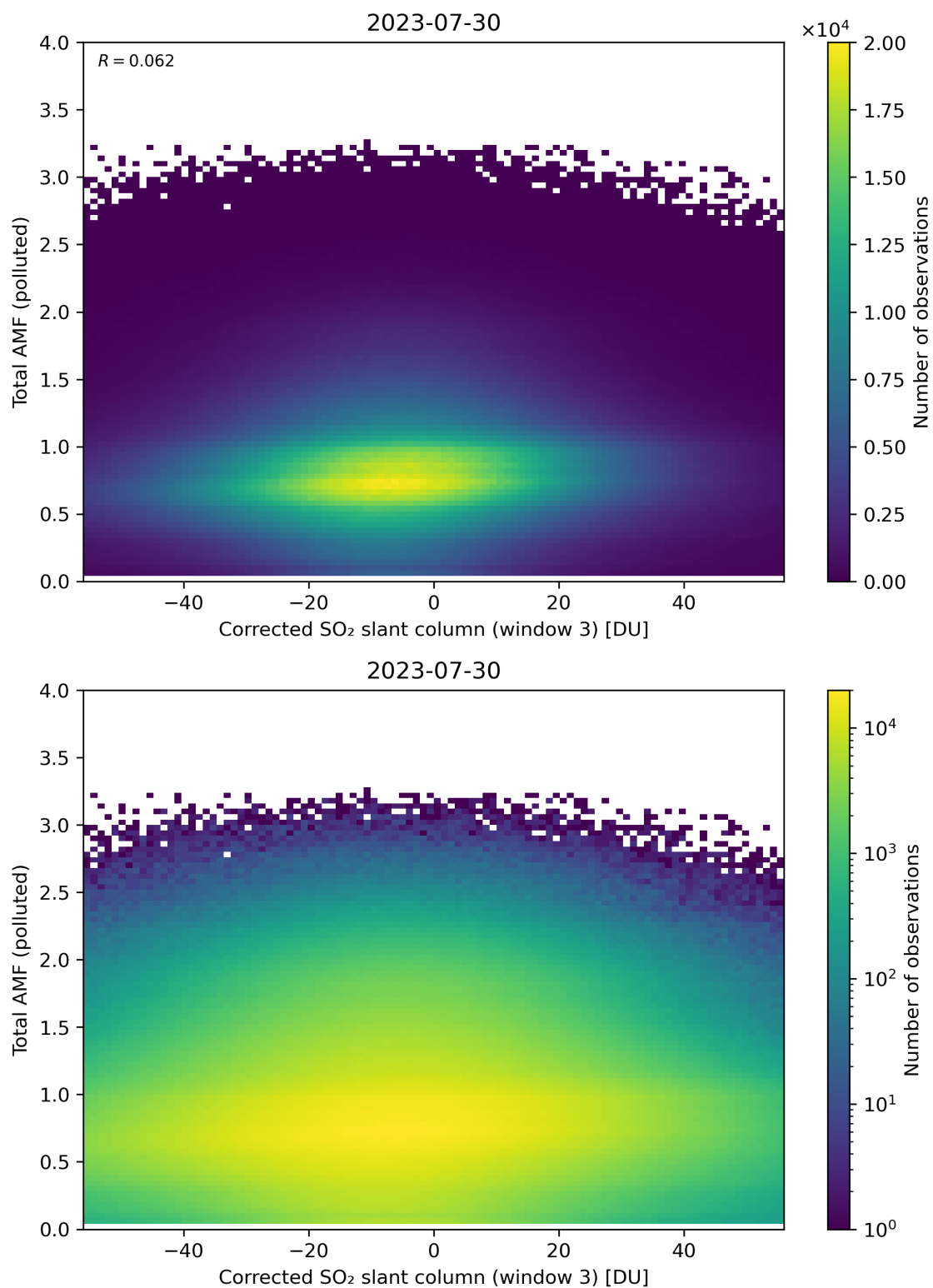
Figure 210: Scatter density plot of “Corrected SO 2 slant column (window 3)” against “Total AMF (polluted)” for 2023-07-29 to 2023-07-31.
