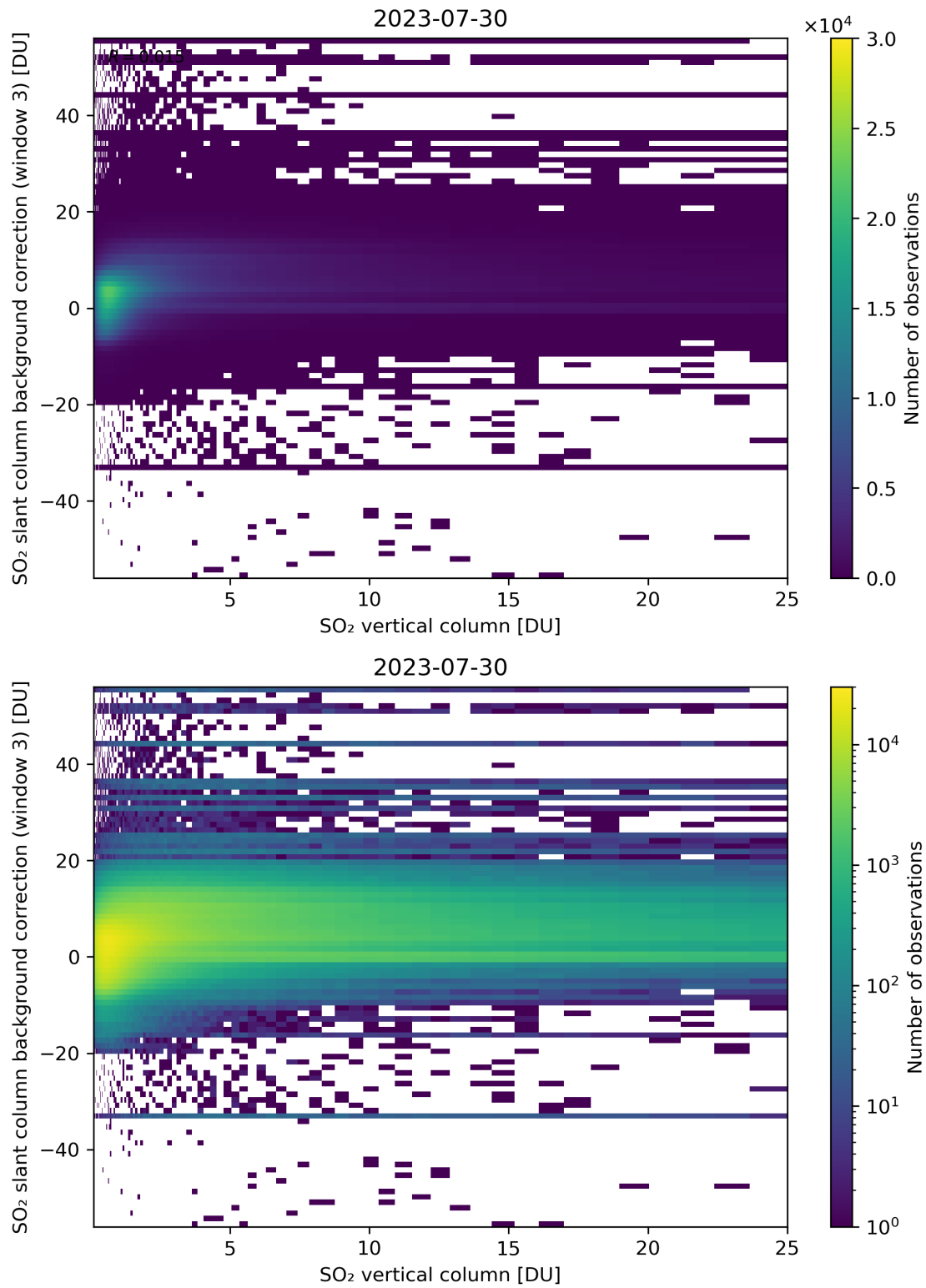
Figure 275: Scatter density plot of “SO 2 vertical column” against “SO 2 slant column background correction (window 3)” for 2023-07-29 to 2023-07-31.
