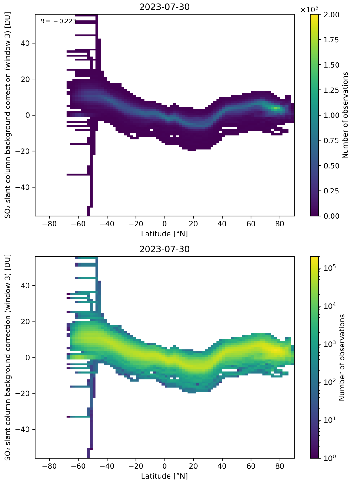
Figure 141: Scatter density plot of “Latitude” against “SO 2 slant column background correction (window 3)” for 2023-07-29 to 2023-07-31.
