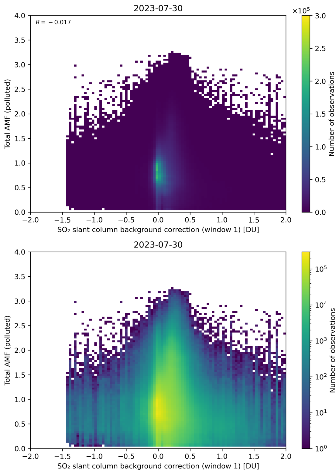
Figure 109: Scatter density plot of “SO 2 slant column background correction (window 1)” against “Total AMF (polluted)” for 2023-07-29 to 2023-07-31.
