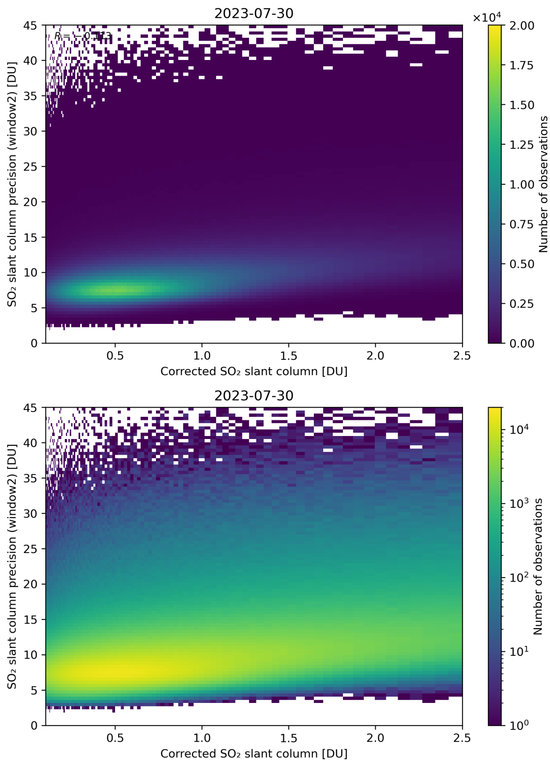
Figure 189: Scatter density plot of “Corrected SO 2 slant column” against “SO 2 slant column precision (window2)” for 2023-07-29 to 2023-07-31.
