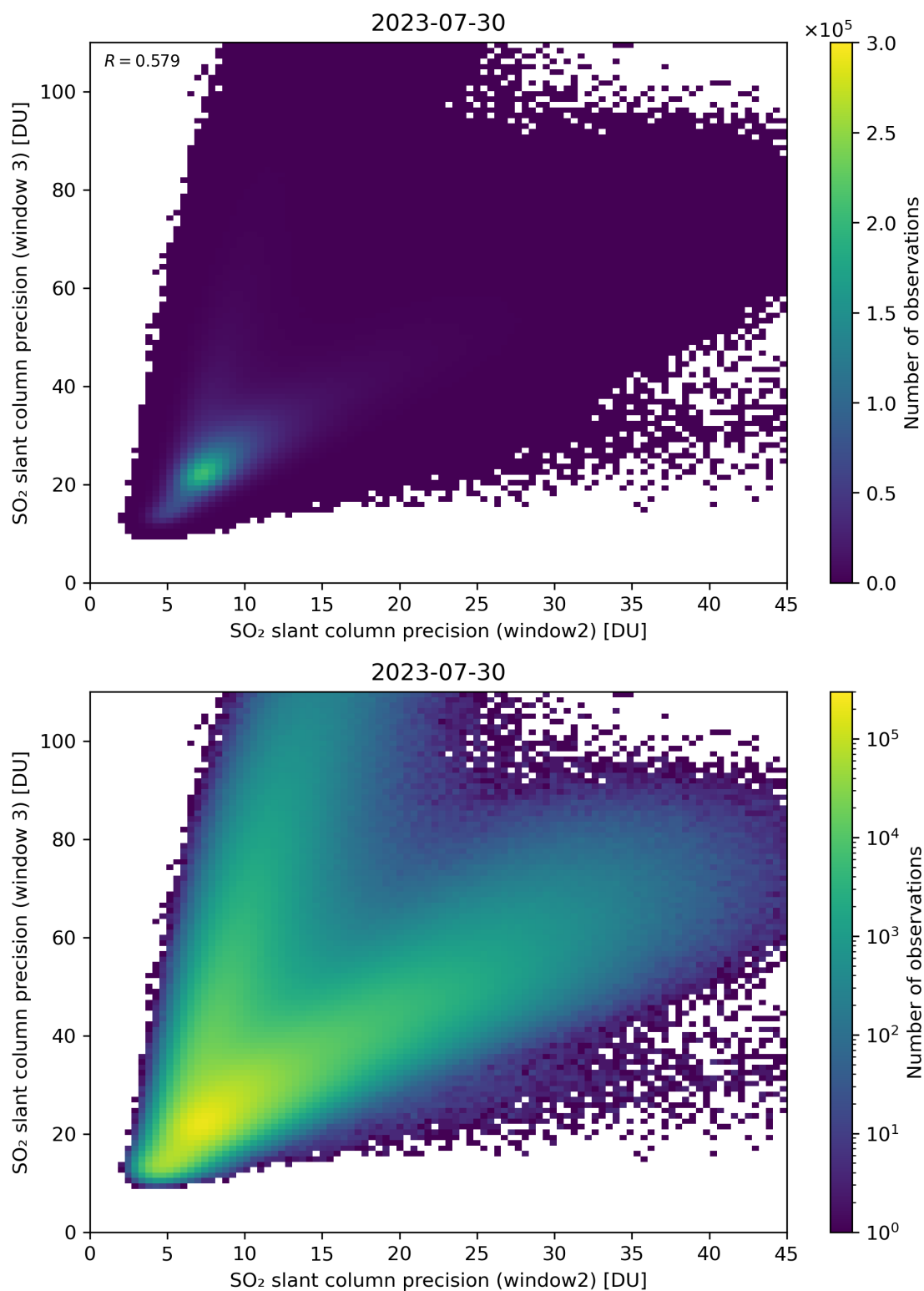
Figure 250: Scatter density plot of “SO 2 slant column precision (window2)” against “SO 2 slant column precision (window 3)” for 2023-07-29 to 2023-07-31.
