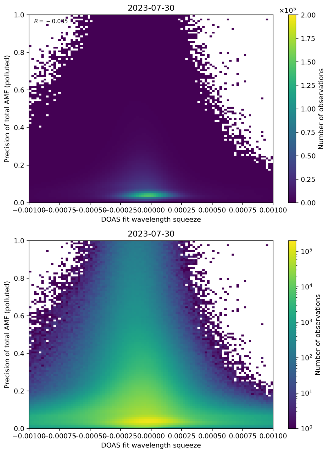
Figure 135: Scatter density plot of “DOAS fit wavelength squeeze” against “Precision of total AMF (polluted)” for 2023-07-29 to 2023-07-31.
