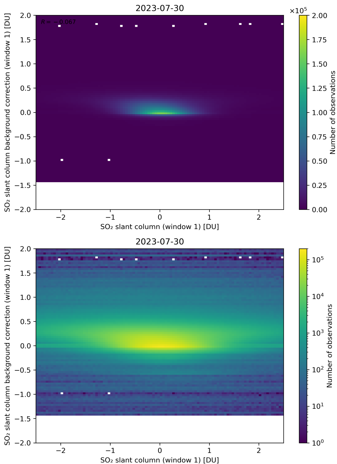
Figure 212: Scatter density plot of “SO 2 slant column (window 1)” against “SO 2 slant column background correction (window 1)” for 2023-07-29 to 2023-07-31.
