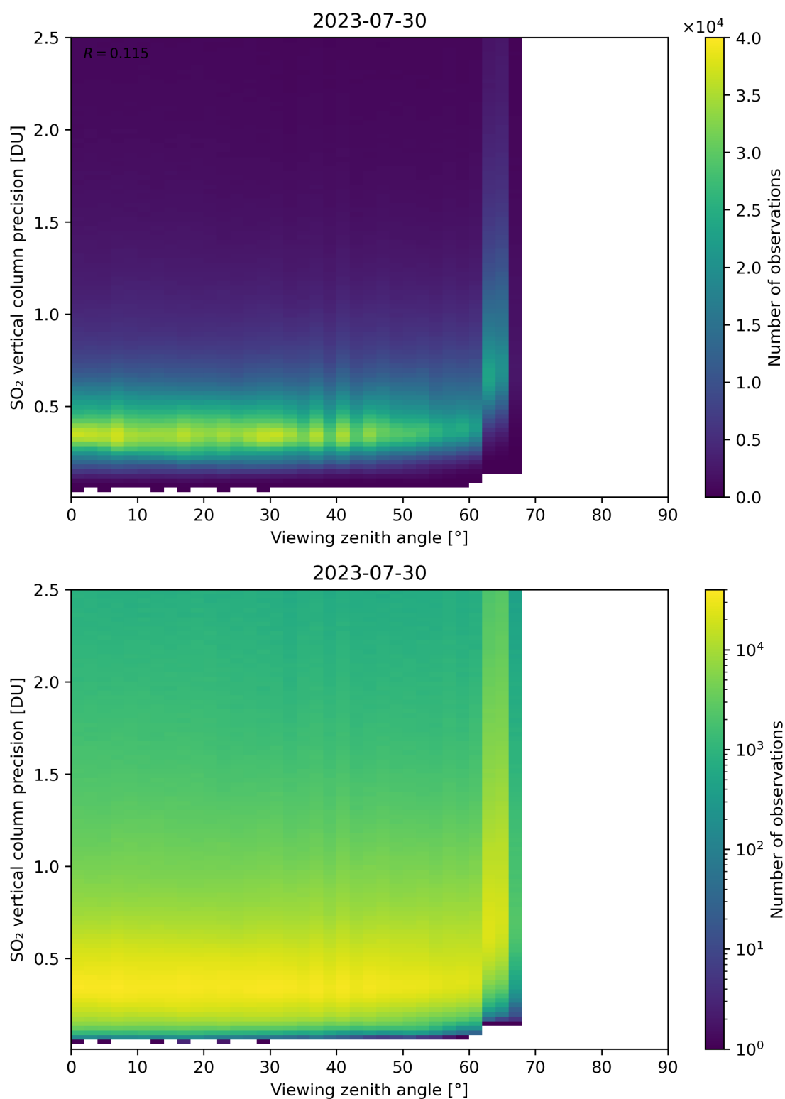
Figure 328: Scatter density plot of “Viewing zenith angle” against “SO 2 vertical column precision” for 2023-07-29 to 2023-07-31.
