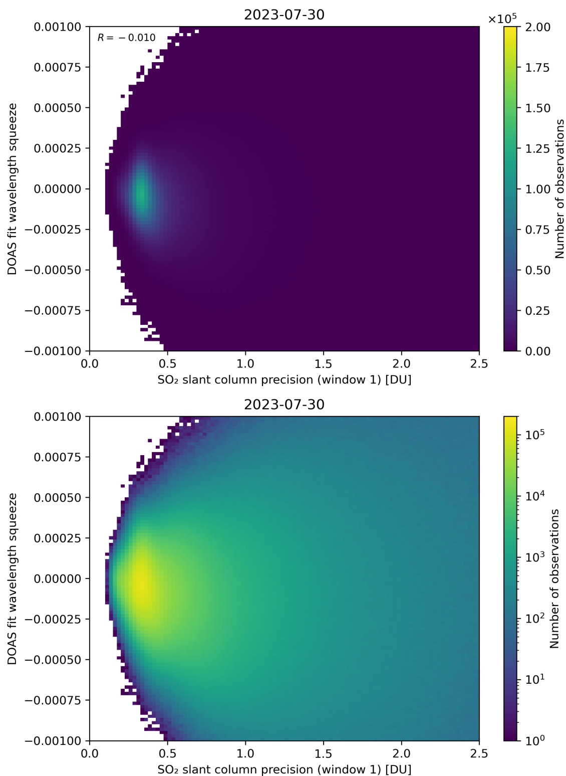
Figure 222: Scatter density plot of “SO 2 slant column precision (window 1)” against “DOAS fit wavelength squeeze” for 2023-07-29 to 2023-07-31.
