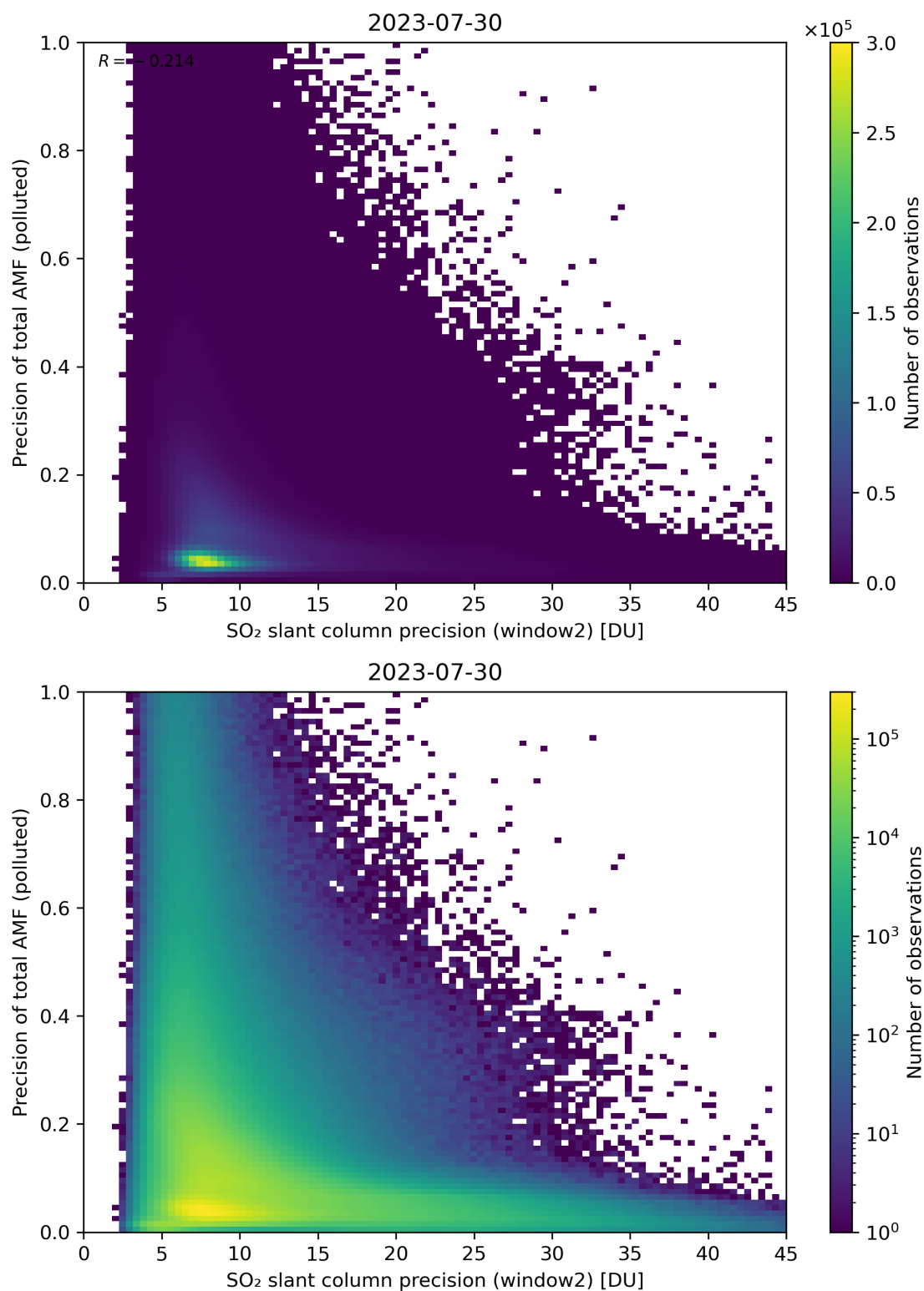
Figure 252: Scatter density plot of “SO 2 slant column precision (window2)” against “Precision of total AMF (polluted)” for 2023-07-29 to 2023-07-31.
