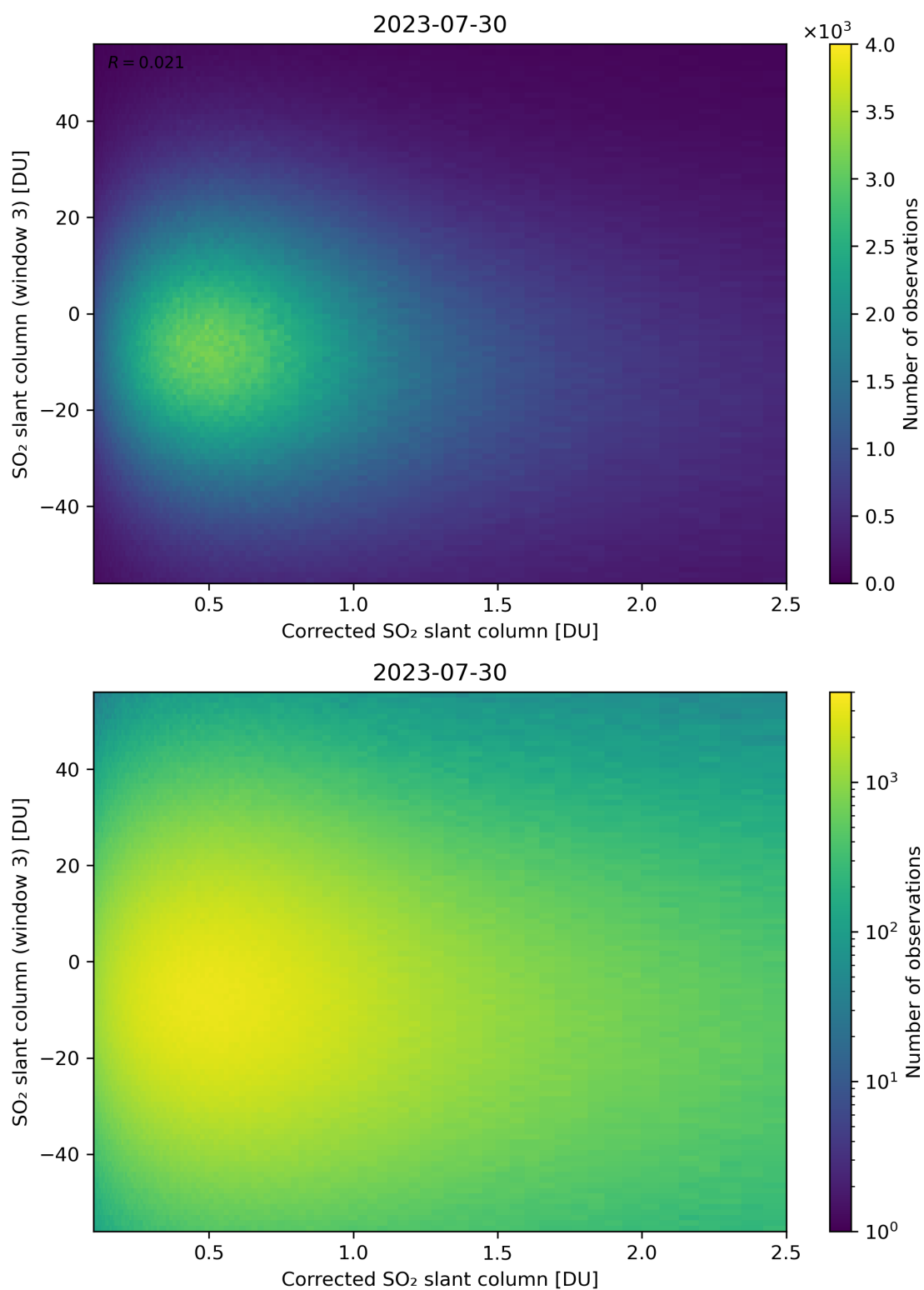
Figure 190: Scatter density plot of “Corrected SO 2 slant column” against “SO 2 slant column (window 3)” for 2023-07-29 to 2023-07-31.
