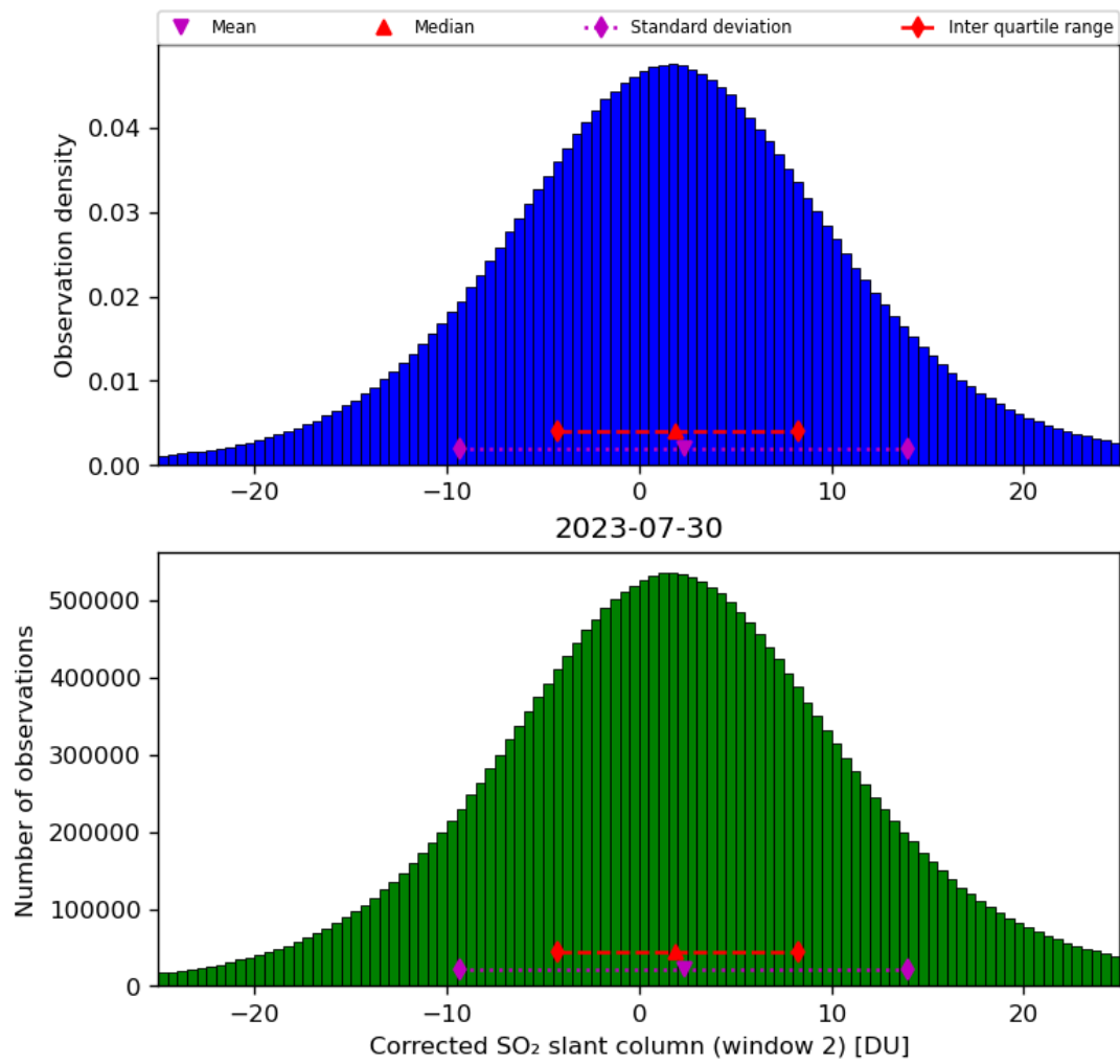
Figure 62: Histogram of “Corrected SO 2 slant column (window 2)” for 2023-07-29 to 2023-07-31
