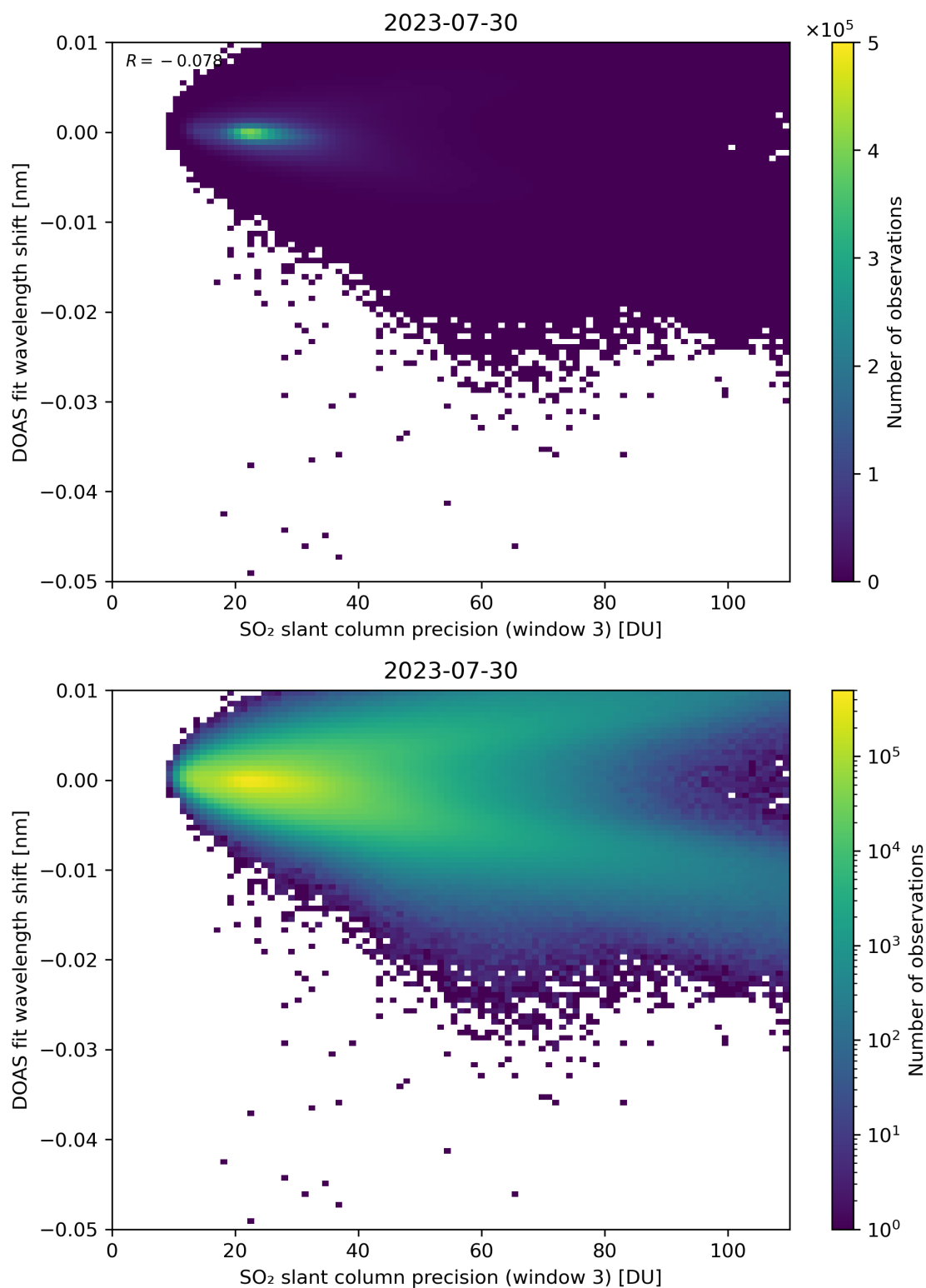
Figure 258: Scatter density plot of “SO 2 slant column precision (window 3)” against “DOAS fit wavelength shift” for 2023-07-29 to 2023-07-31.
