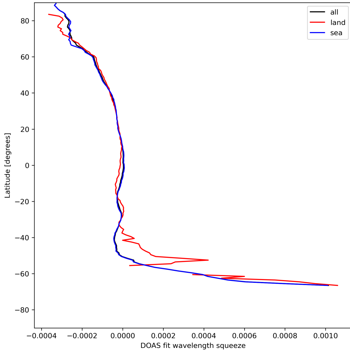
Figure 46: Zonal average of “DOAS fit wavelength squeeze” for 2023-07-29 to 2023-07-31.
