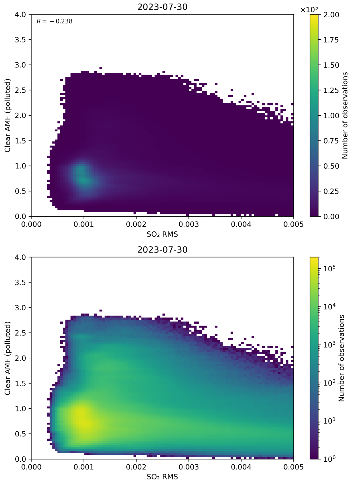
Figure 136: Scatter density plot of “SO 2 RMS” against “Clear AMF (polluted)” for 2023-07-29 to 2023-07-31.
