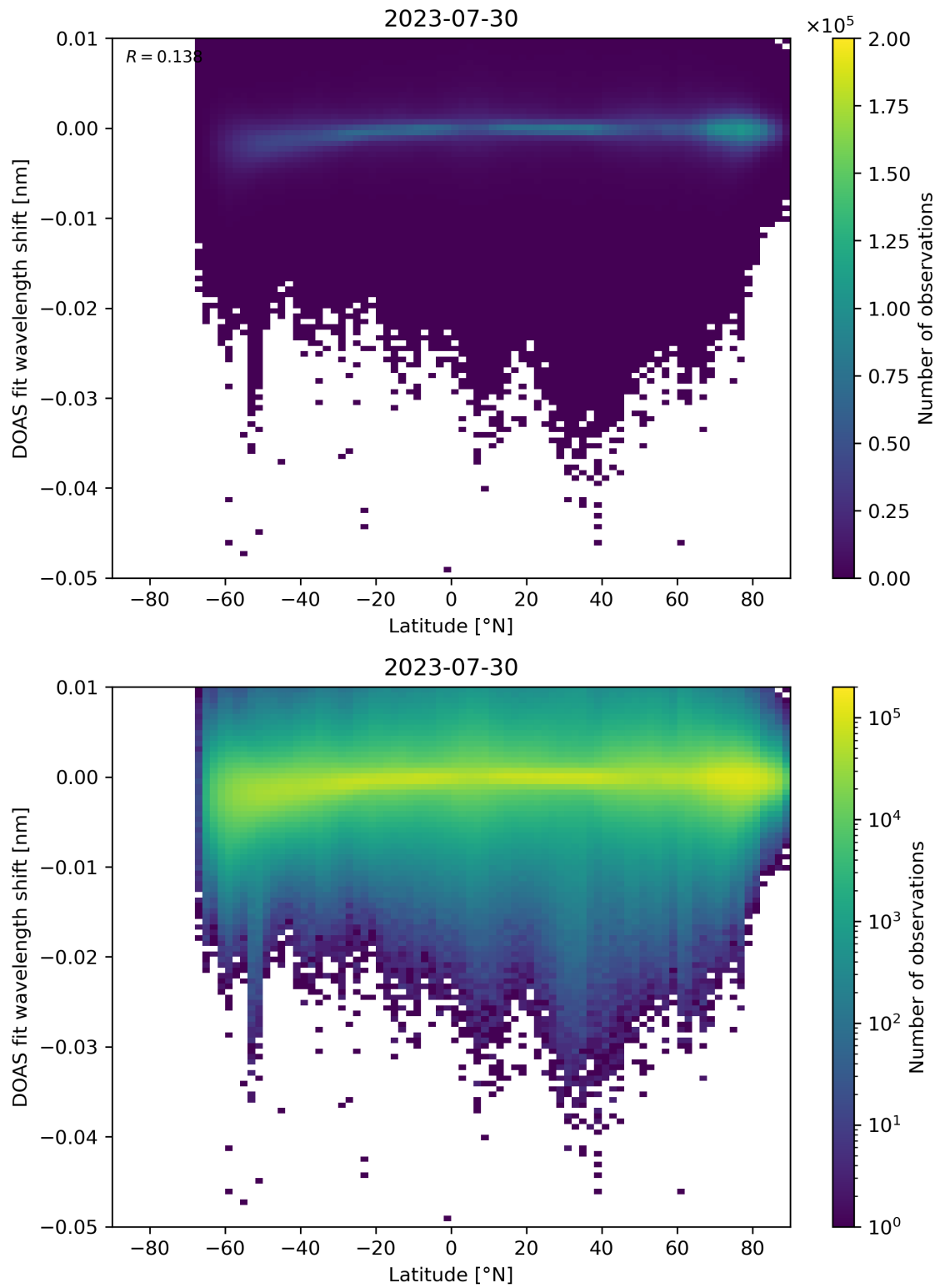
Figure 142: Scatter density plot of “Latitude” against “DOAS fit wavelength shift” for 2023-07-29 to 2023-07-31.
