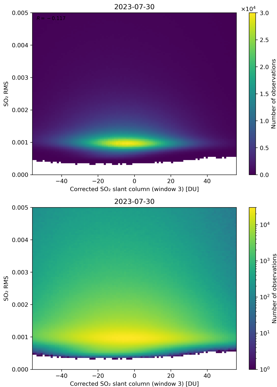
Figure 208: Scatter density plot of “Corrected SO 2 slant column (window 3)” against “SO 2 RMS” for 2023-07-29 to 2023-07-31.
