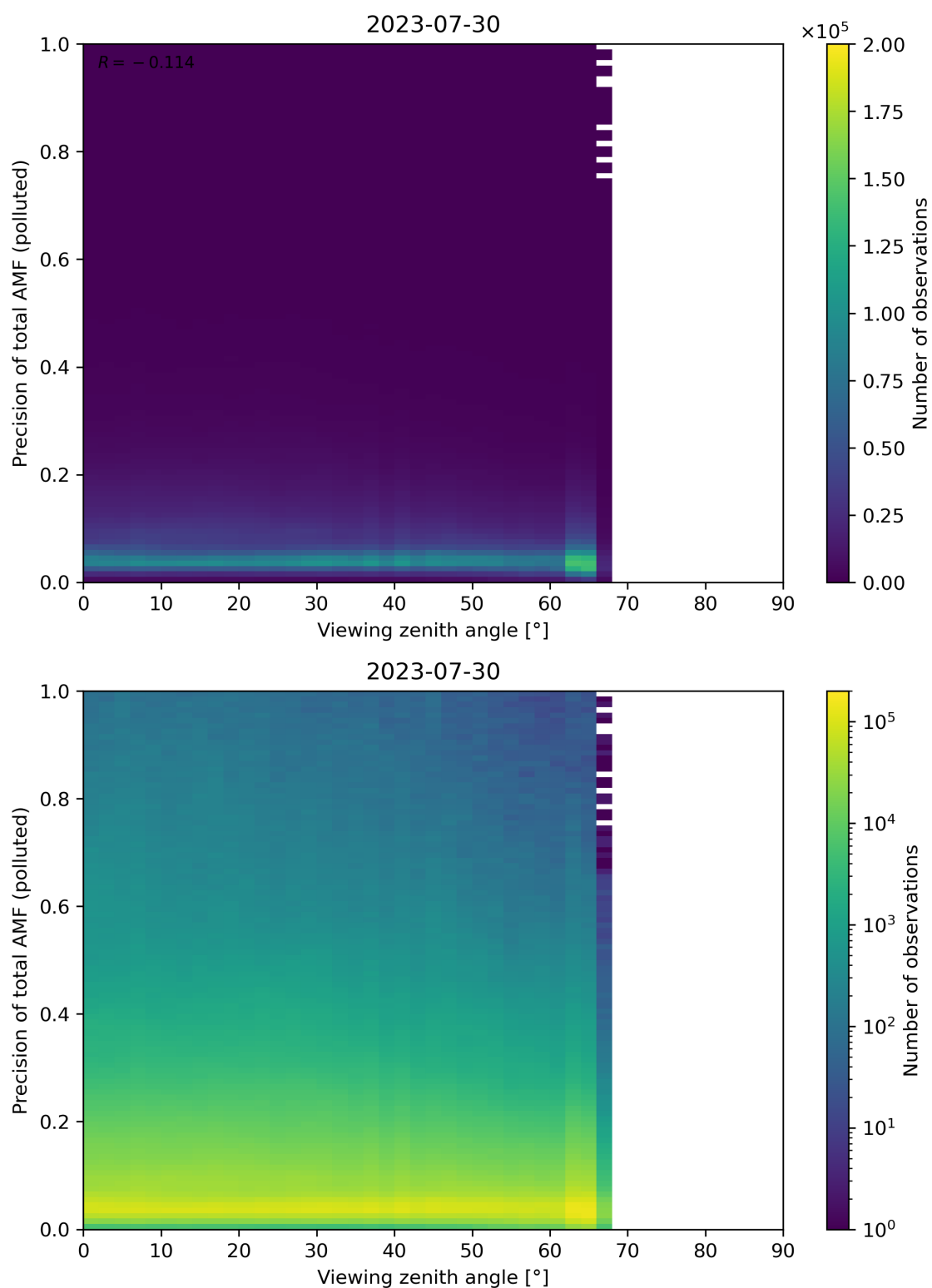
Figure 326: Scatter density plot of “Viewing zenith angle” against “Precision of total AMF (polluted)” for 2023-07-29 to 2023-07-31.
