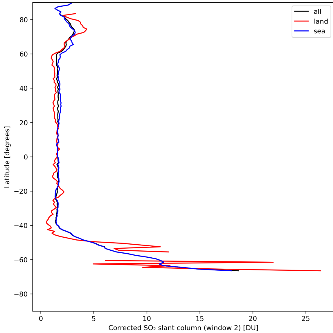
Figure 39: Zonal average of “Corrected SO 2 slant column (window 2)” for 2023-07-29 to 2023-07-31.
