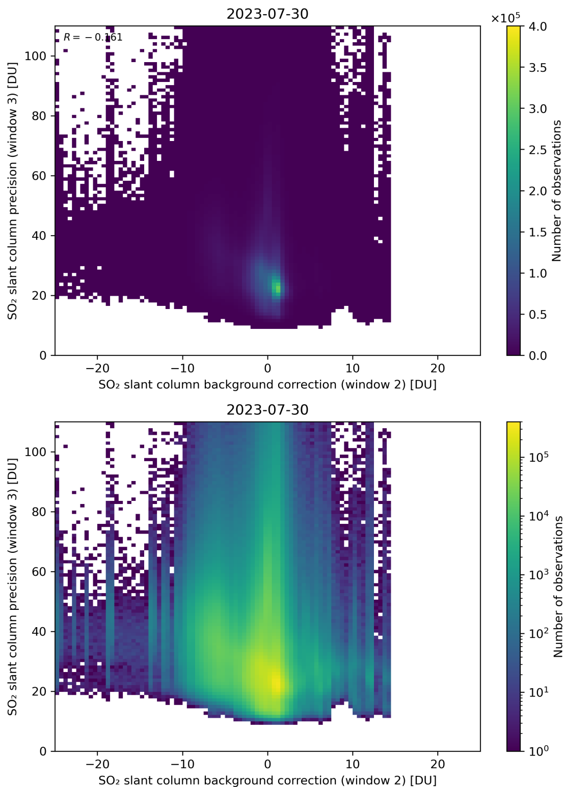
Figure 118: Scatter density plot of “SO 2 slant column background correction (window 2)” against “SO 2 slant column precision (window 3)” for 2023-07-29 to 2023-07-31.
