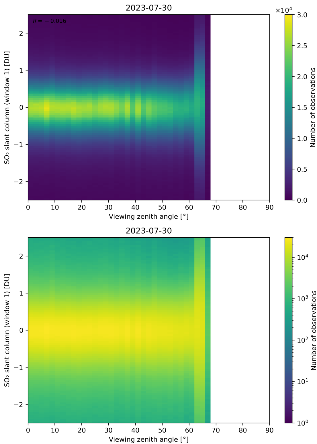
Figure 320: Scatter density plot of “Viewing zenith angle” against “SO 2 slant column (window 1)” for 2023-07-29 to 2023-07-31.
