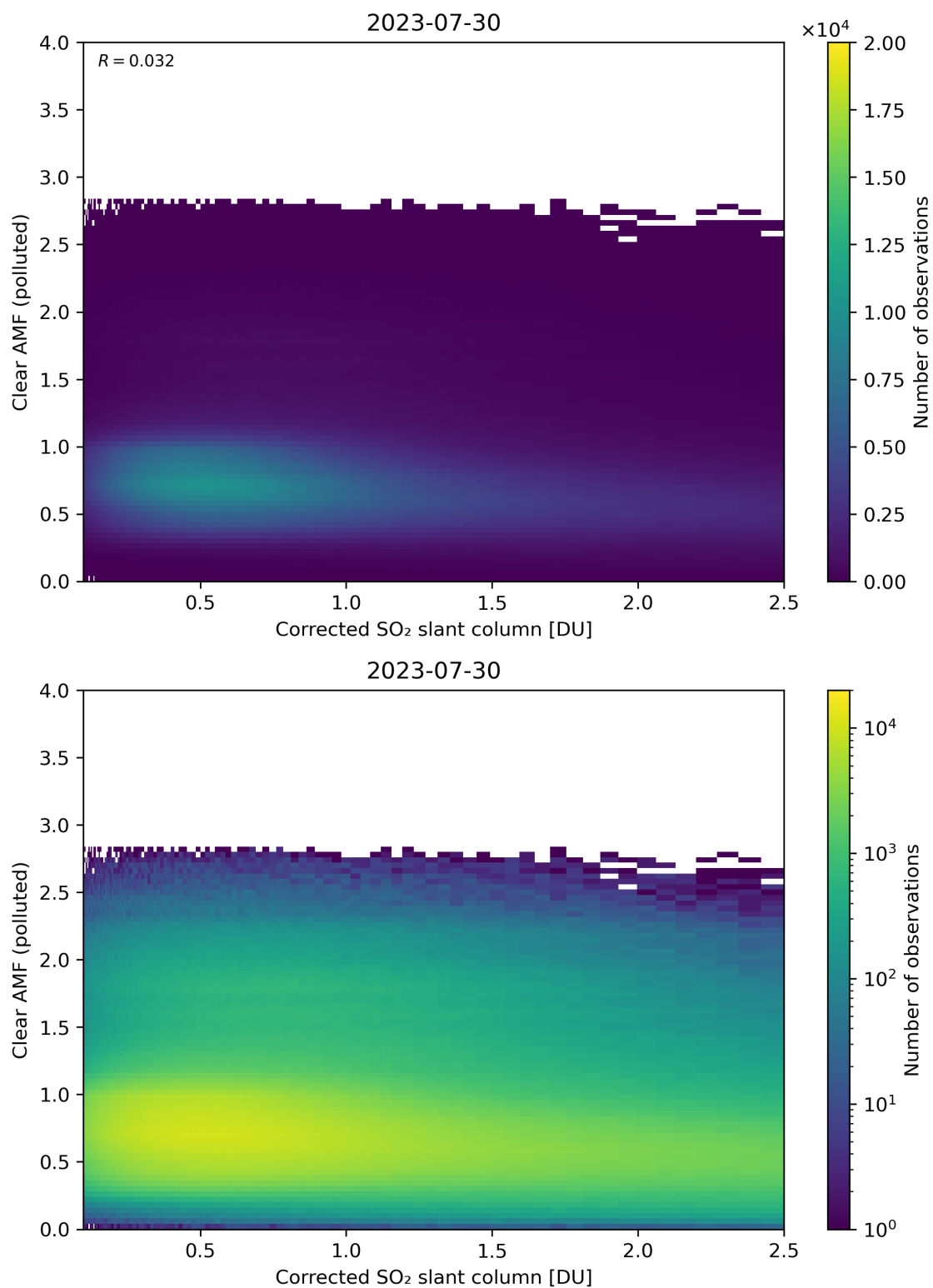
Figure 184: Scatter density plot of “Corrected SO 2 slant column” against “Clear AMF (polluted)” for 2023-07-29 to 2023-07-31.
