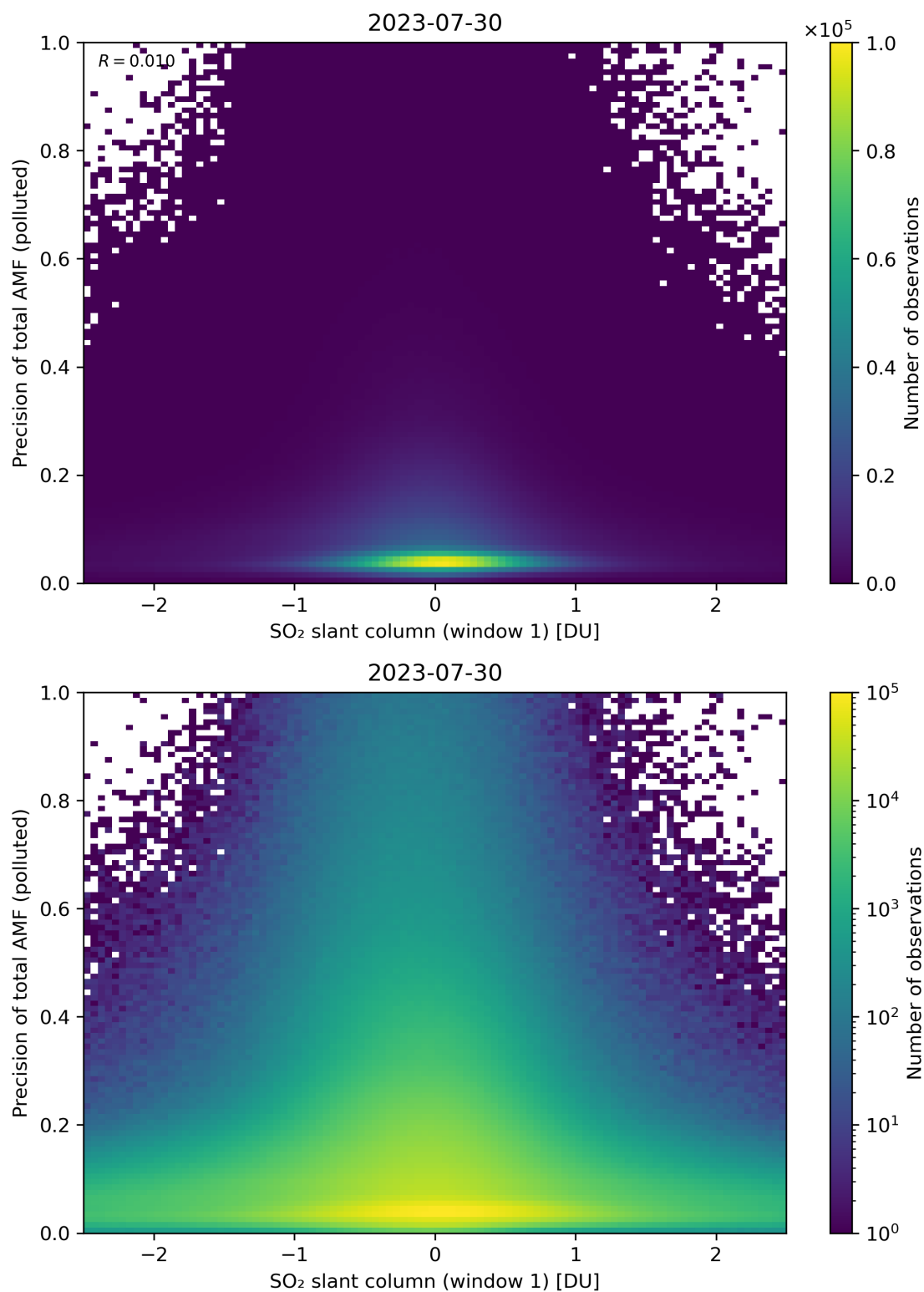
Figure 240: Scatter density plot of “SO 2 slant column (window 1)” against “Precision of total AMF (polluted)” for 2023-07-29 to 2023-07-31.
