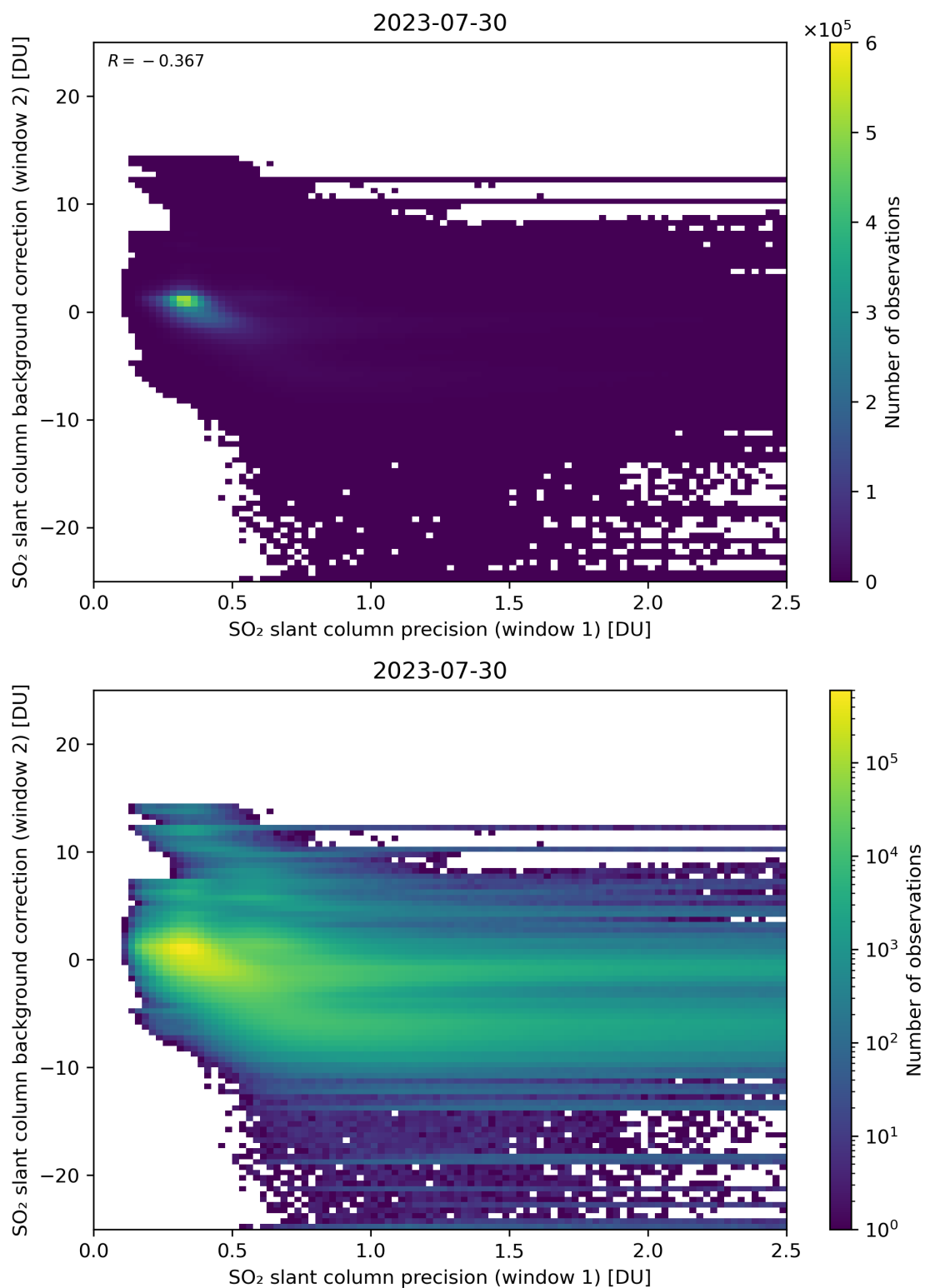
Figure 219: Scatter density plot of “SO 2 slant column precision (window 1)” against “SO 2 slant column background correction (window 2)” for 2023-07-29 to 2023-07-31.
