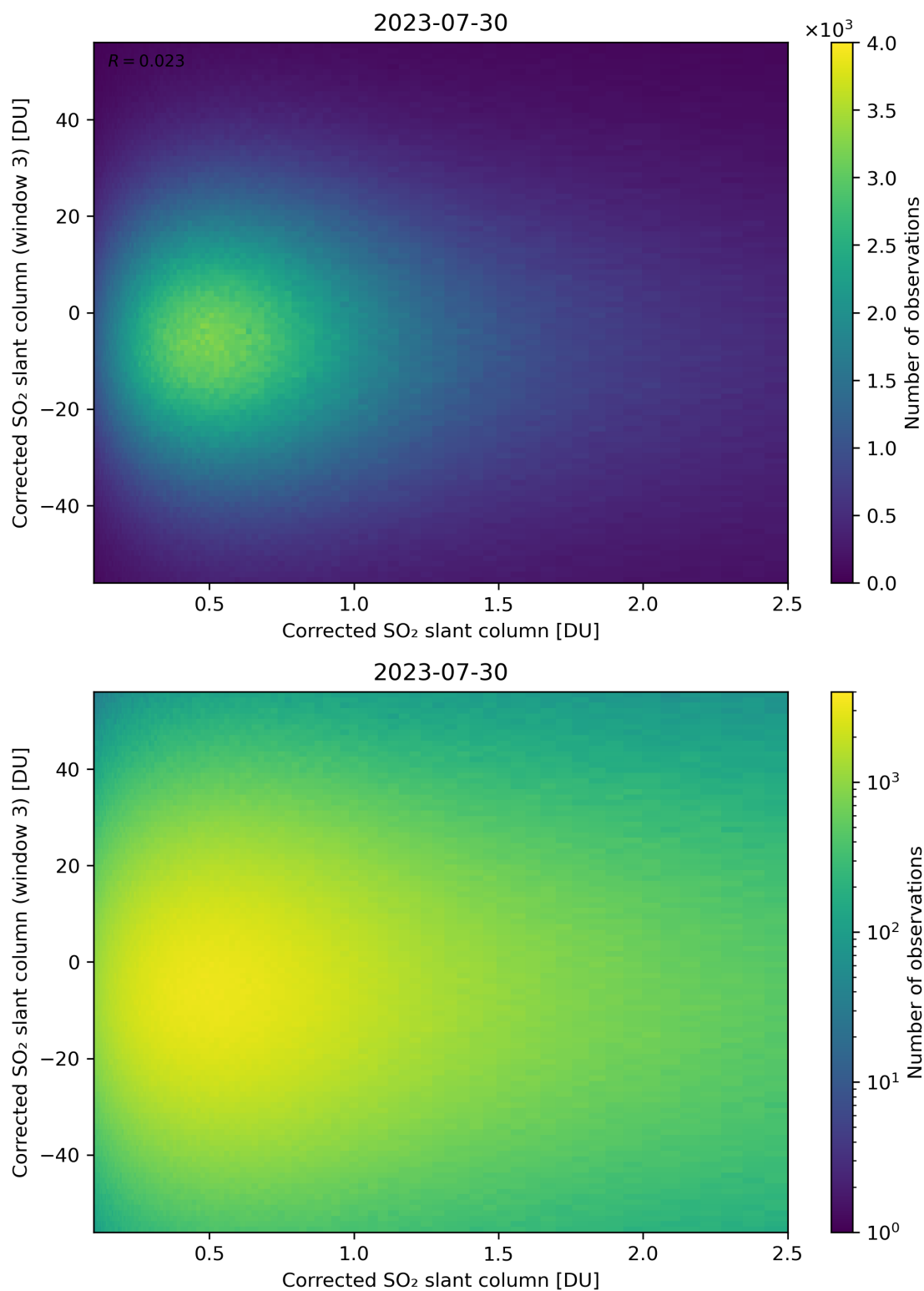
Figure 186: Scatter density plot of “Corrected SO 2 slant column” against “Corrected SO 2 slant column (window 3)” for 2023-07-29 to 2023-07-31.
