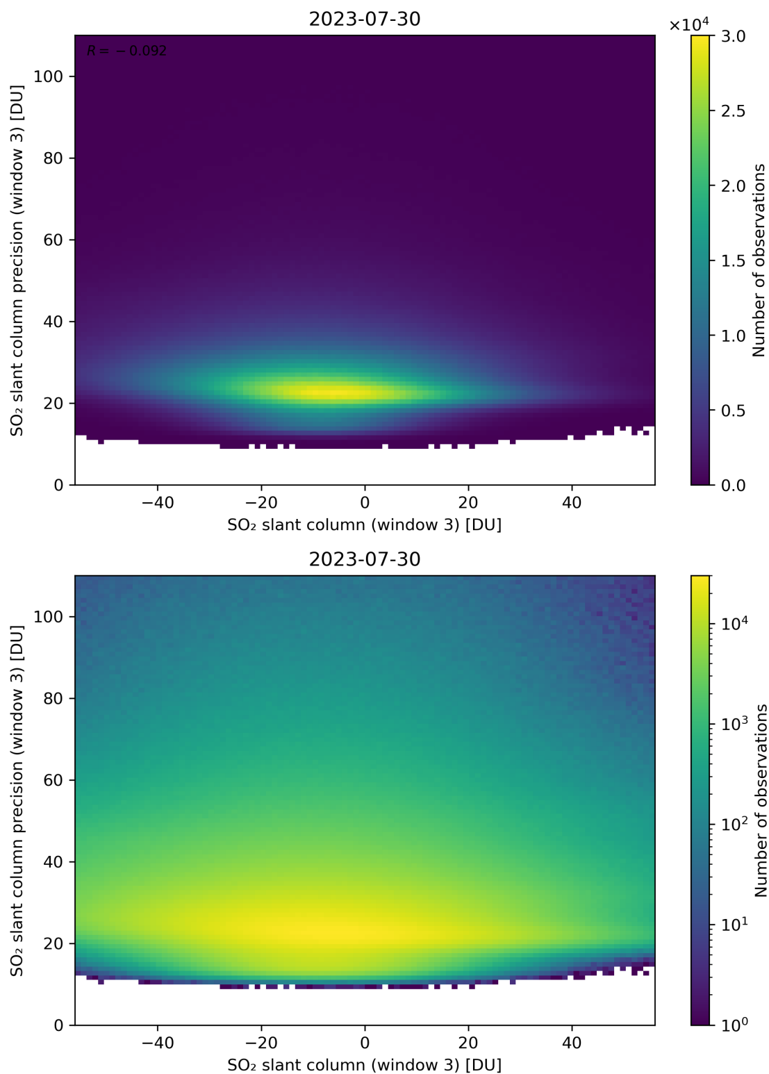
Figure 267: Scatter density plot of “SO 2 slant column (window 3)” against “SO 2 slant column precision (window 3)” for 2023-07-29 to 2023-07-31.
