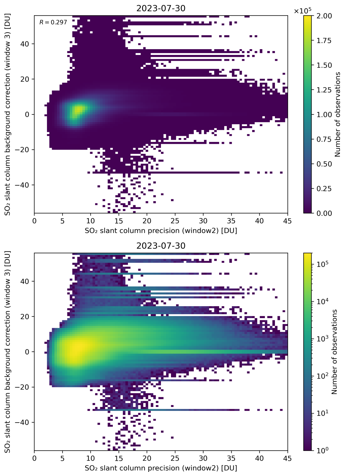
Figure 242: Scatter density plot of “SO 2 slant column precision (window2)” against “SO 2 slant column background correction (window 3)” for 2023-07-29 to 2023-07-31.
