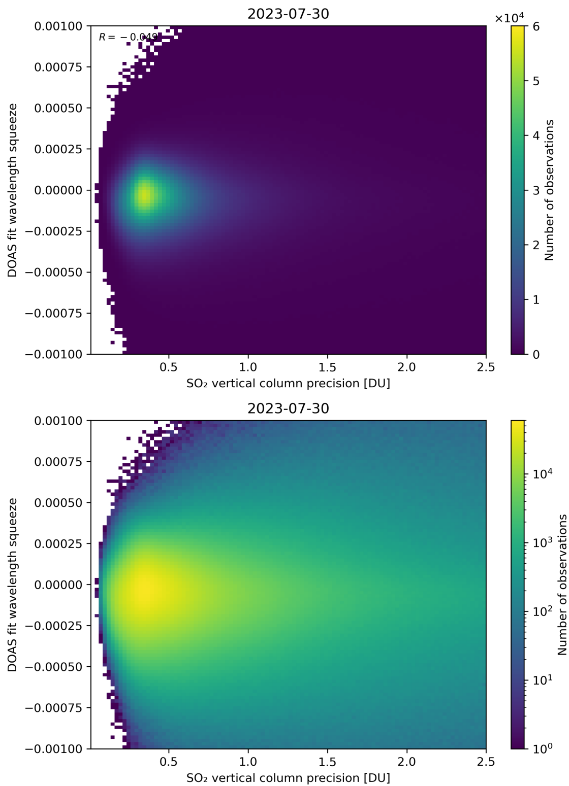
Figure 283: Scatter density plot of “SO 2 vertical column precision” against “DOAS fit wavelength squeeze” for 2023-07-29 to 2023-07-31.
