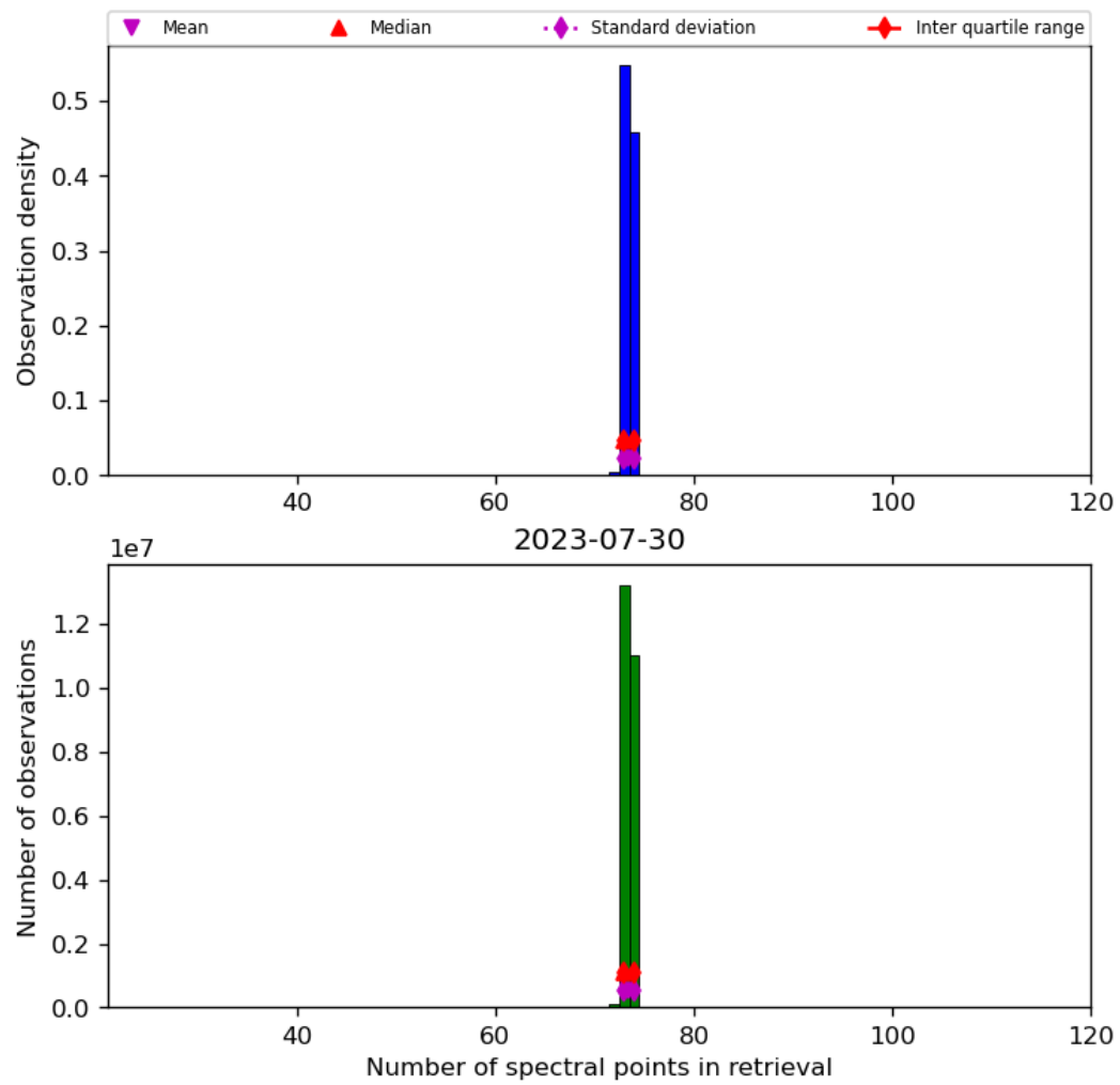
Figure 74: Histogram of “Number of spectral points in retrieval” for 2023-07-29 to 2023-07-31
