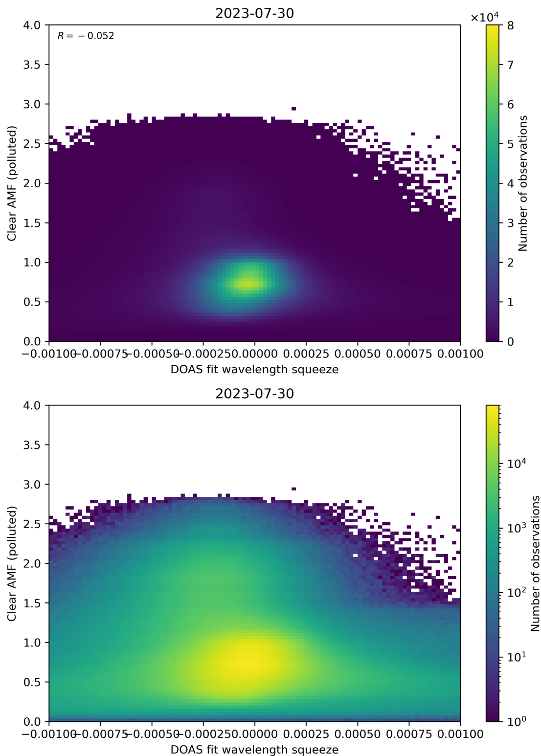
Figure 133: Scatter density plot of “DOAS fit wavelength squeeze” against “Clear AMF (polluted)” for 2023-07-29 to 2023-07-31.
