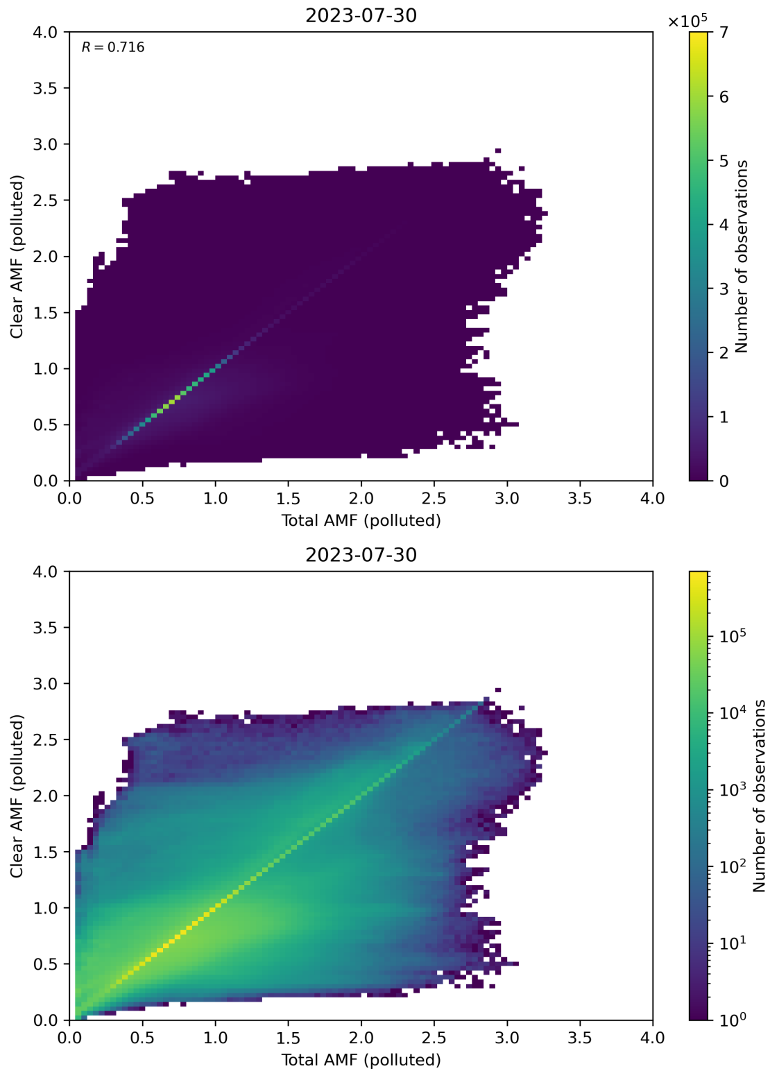
Figure 271: Scatter density plot of “Total AMF (polluted)” against “Clear AMF (polluted)” for 2023-07-29 to 2023-07-31.
