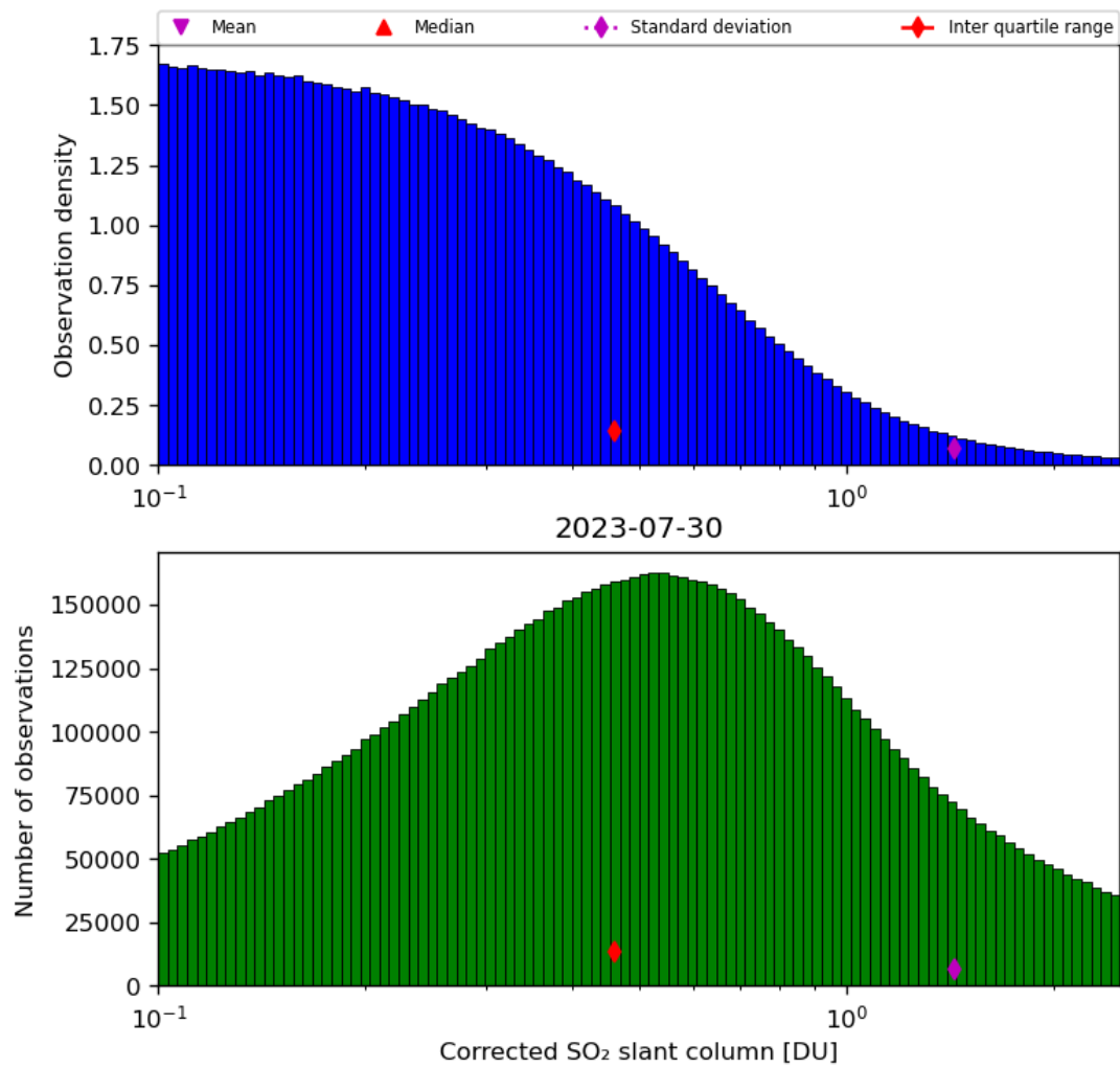
Figure 55: Histogram of “Corrected SO 2 slant column” for 2023-07-29 to 2023-07-31
