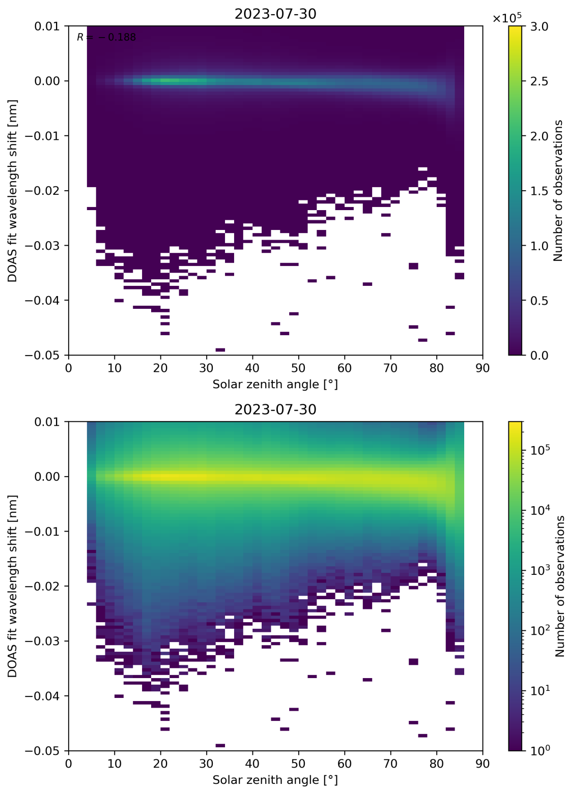
Figure 161: Scatter density plot of “Solar zenith angle” against “DOAS fit wavelength shift” for 2023-07-29 to 2023-07-31.
