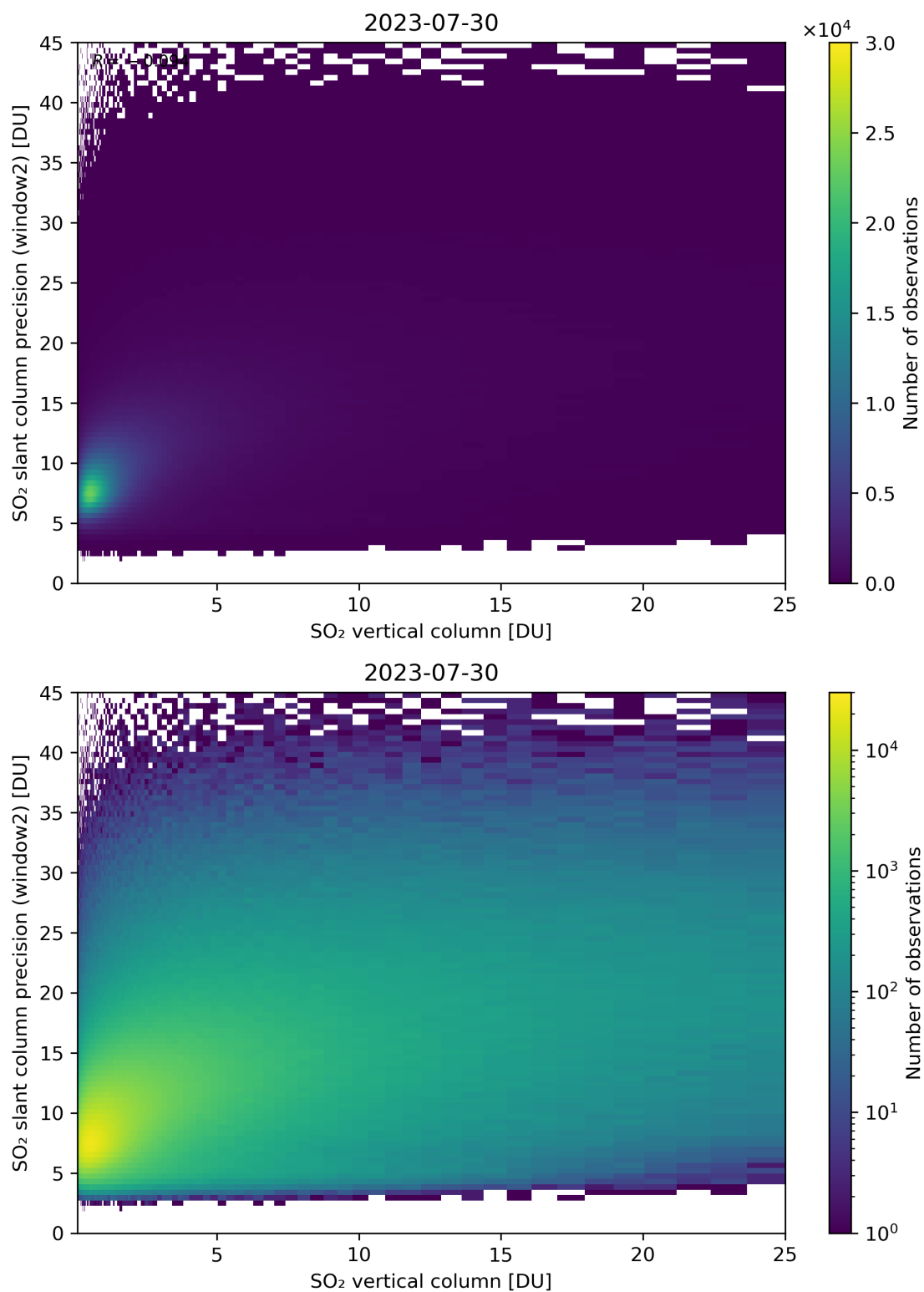
Figure 302: Scatter density plot of “SO 2 vertical column” against “SO 2 slant column precision (window2)” for 2023-07-29 to 2023-07-31.
