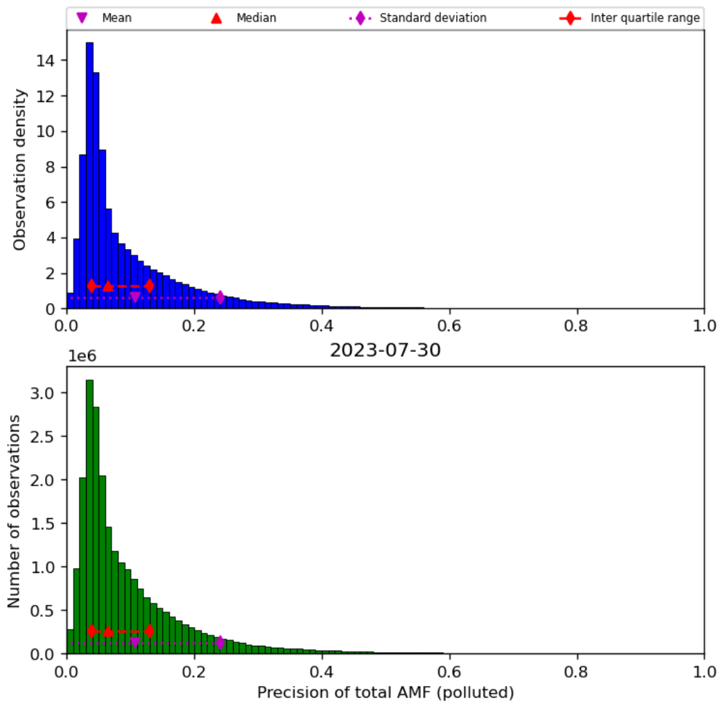
Figure 72: Histogram of “Precision of total AMF (polluted)” for 2023-07-29 to 2023-07-31
