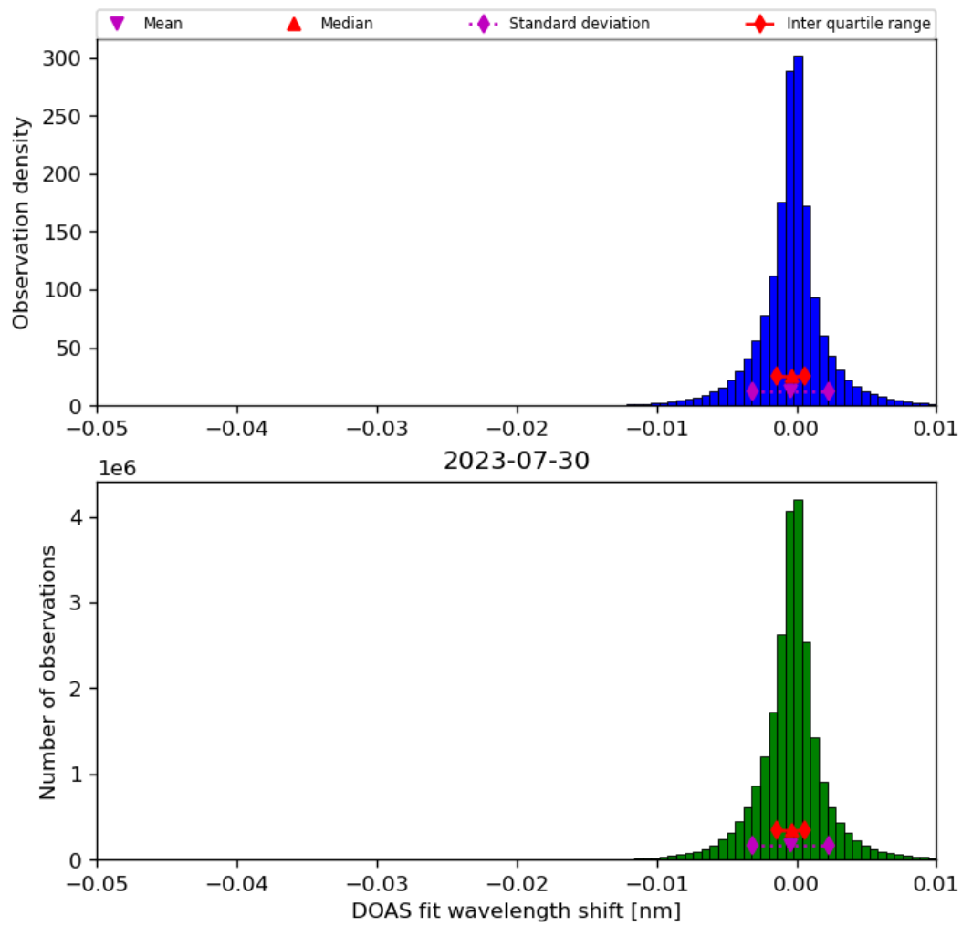
Figure 68: Histogram of “DOAS fit wavelength shift” for 2023-07-29 to 2023-07-31
