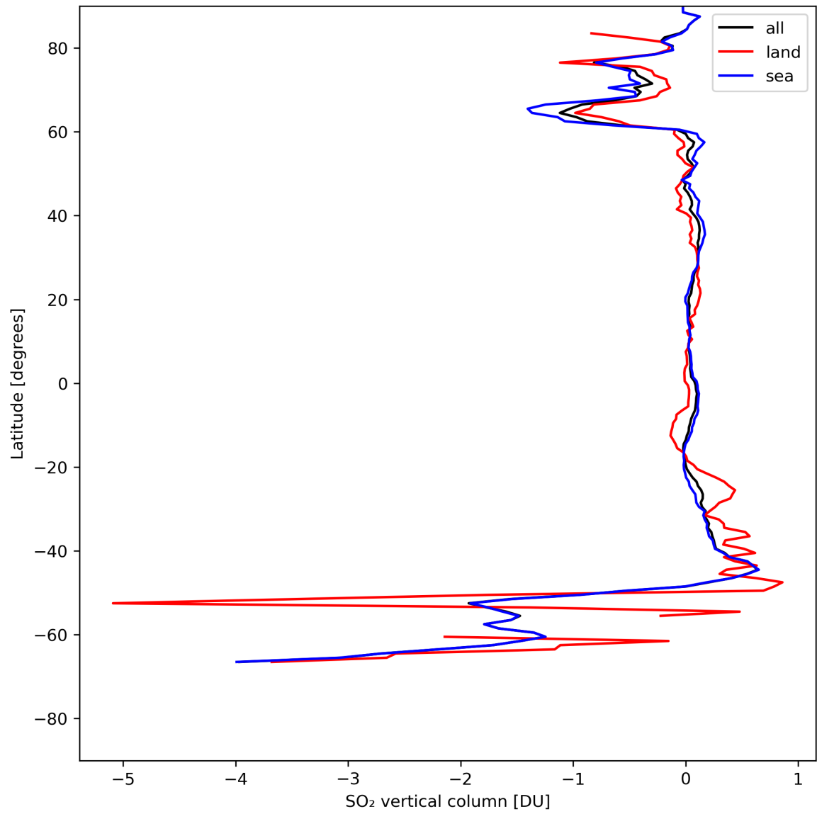
Figure 30: Zonal average of “SO 2 vertical column” for 2023-07-29 to 2023-07-31.
