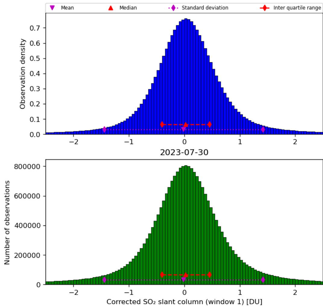
Figure 58: Histogram of “Corrected SO 2 slant column (window 1)” for 2023-07-29 to 2023-07-31
