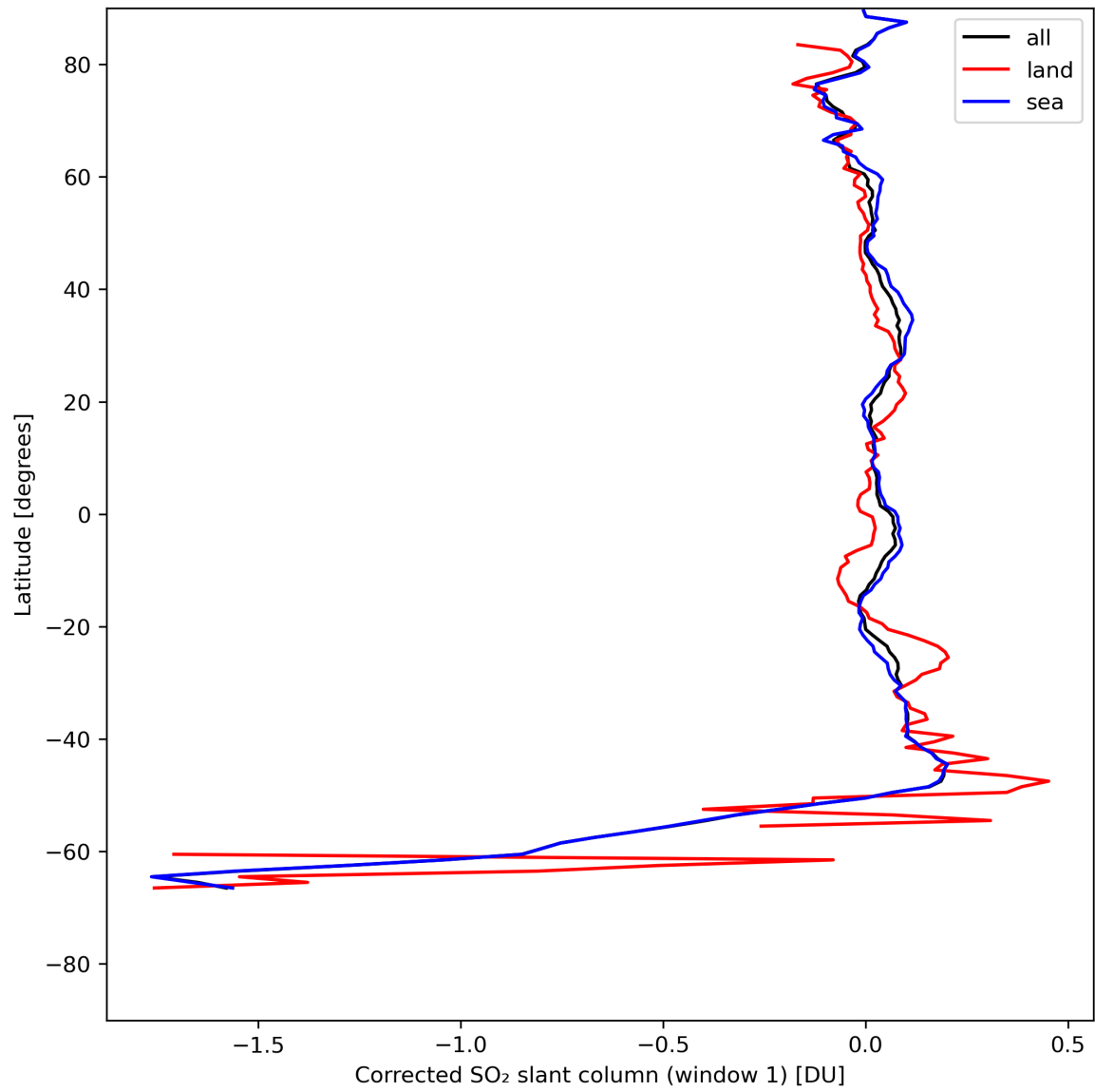
Figure 35: Zonal average of “Corrected SO 2 slant column (window 1)” for 2023-07-29 to 2023-07-31.
