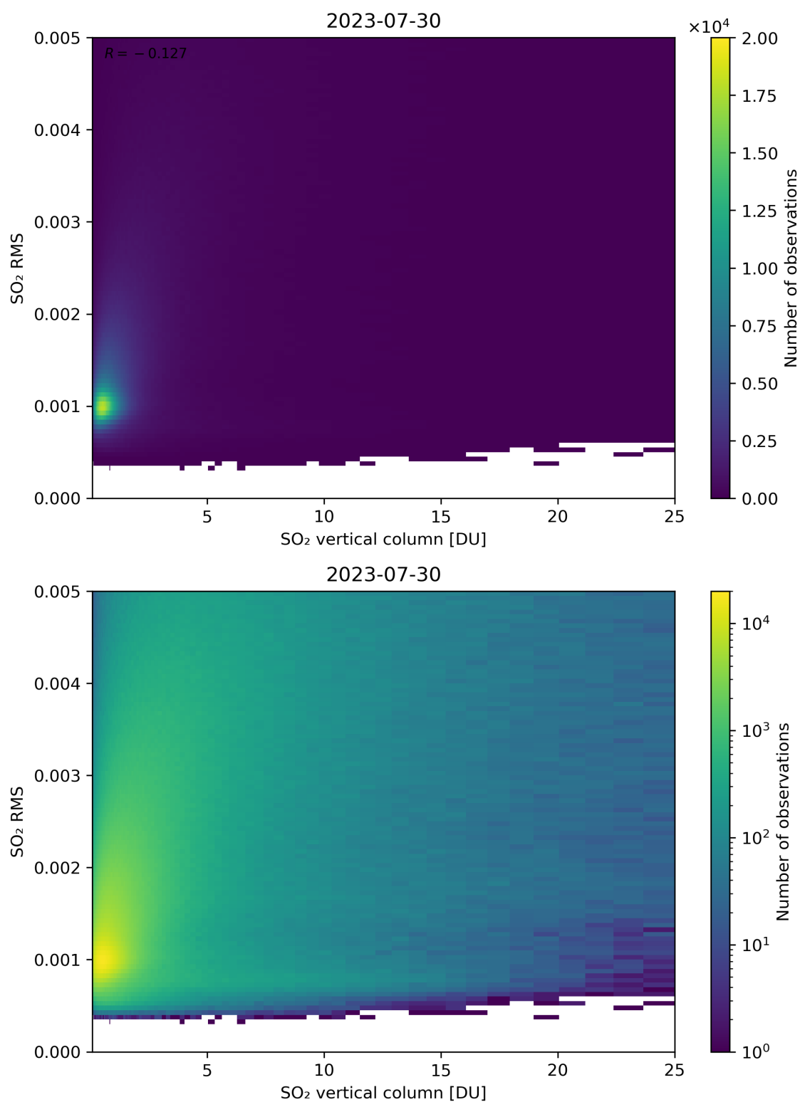
Figure 278: Scatter density plot of “SO 2 vertical column” against “SO 2 RMS” for 2023-07-29 to 2023-07-31.
