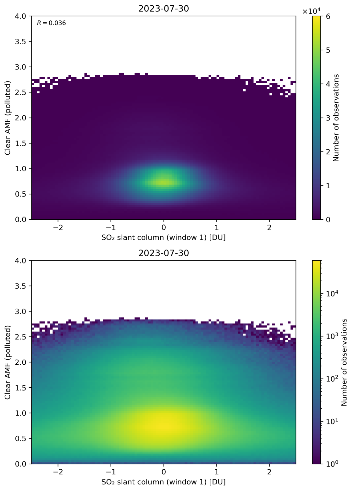
Figure 232: Scatter density plot of “SO 2 slant column (window 1)” against “Clear AMF (polluted)” for 2023-07-29 to 2023-07-31.
