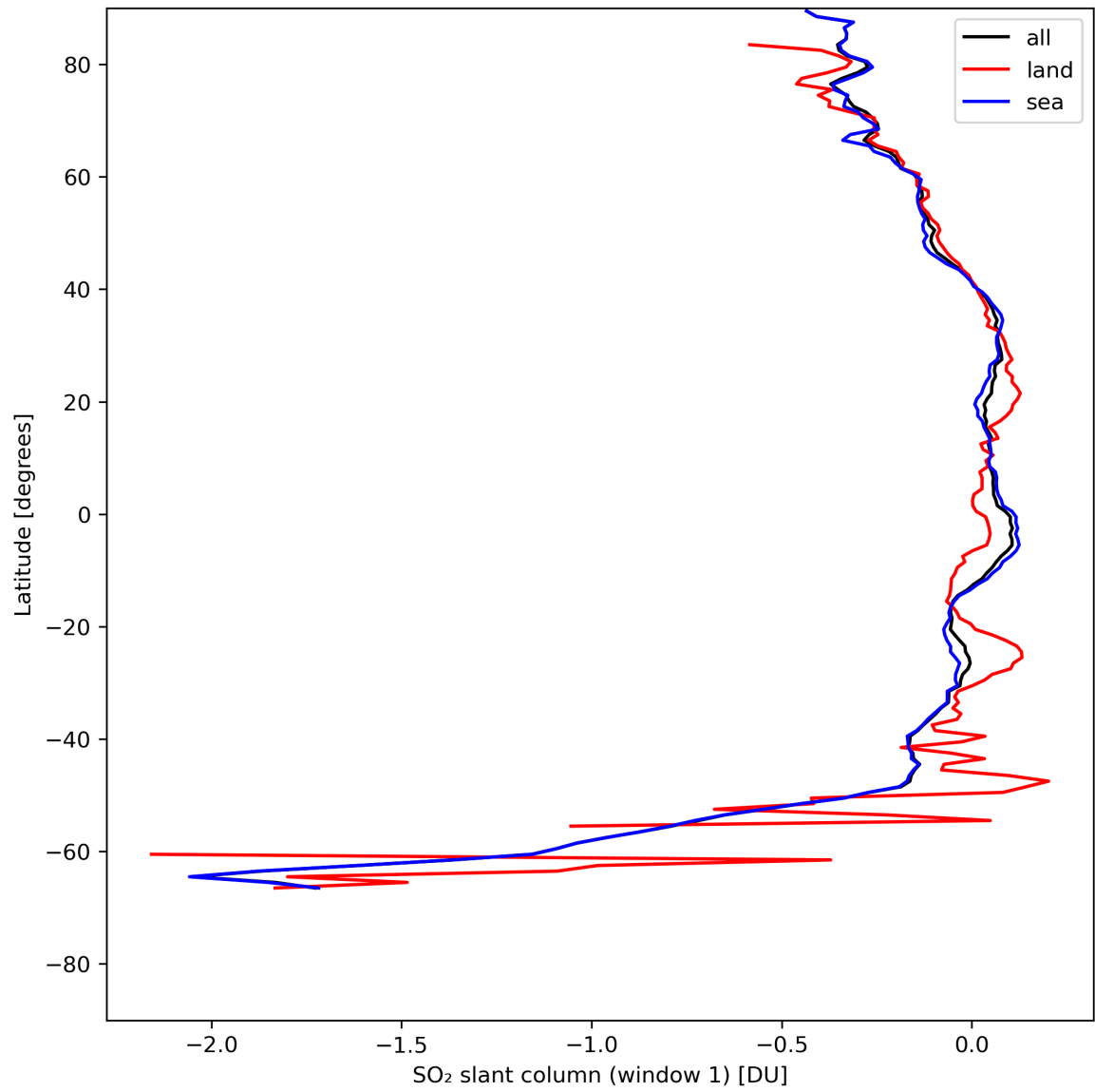
Figure 33: Zonal average of “SO 2 slant column (window 1)” for 2023-07-29 to 2023-07-31.
