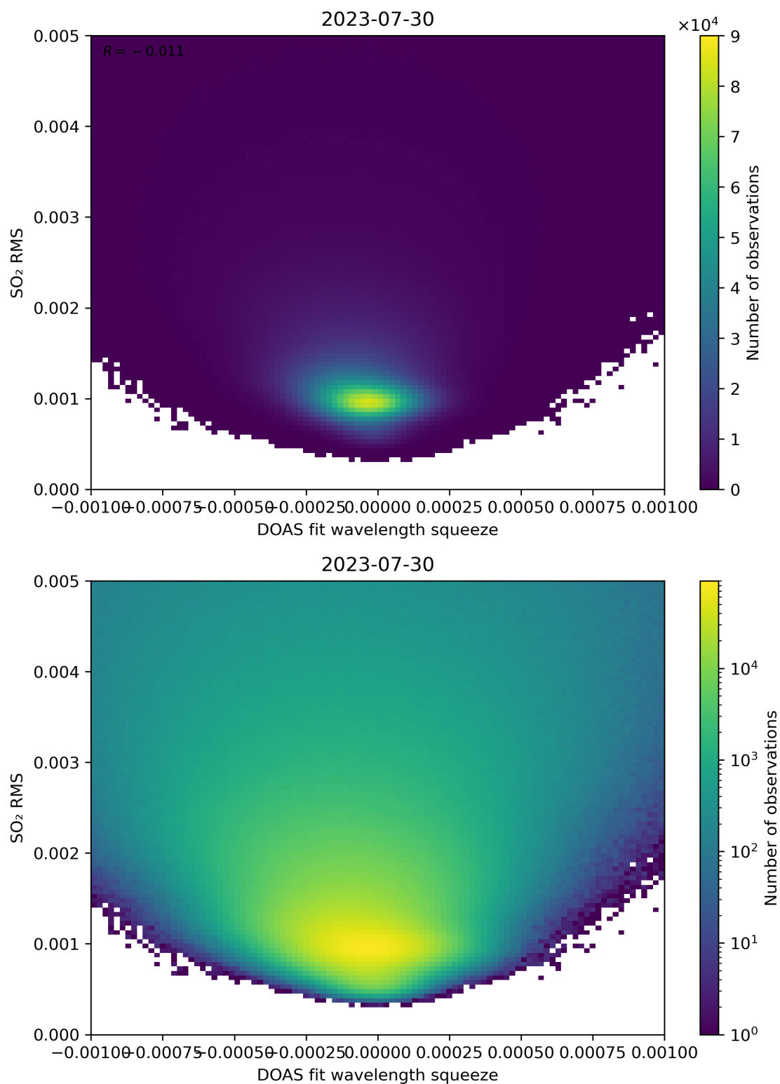
Figure 132: Scatter density plot of “DOAS fit wavelength squeeze” against “SO 2 RMS” for 2023-07-29 to 2023-07-31.
