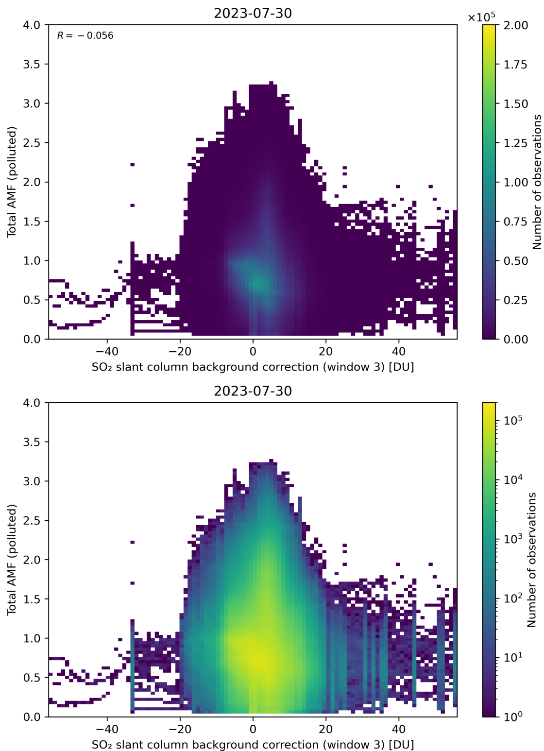
Figure 125: Scatter density plot of “SO 2 slant column background correction (window 3)” against “Total AMF (polluted)” for 2023-07-29 to 2023-07-31.
