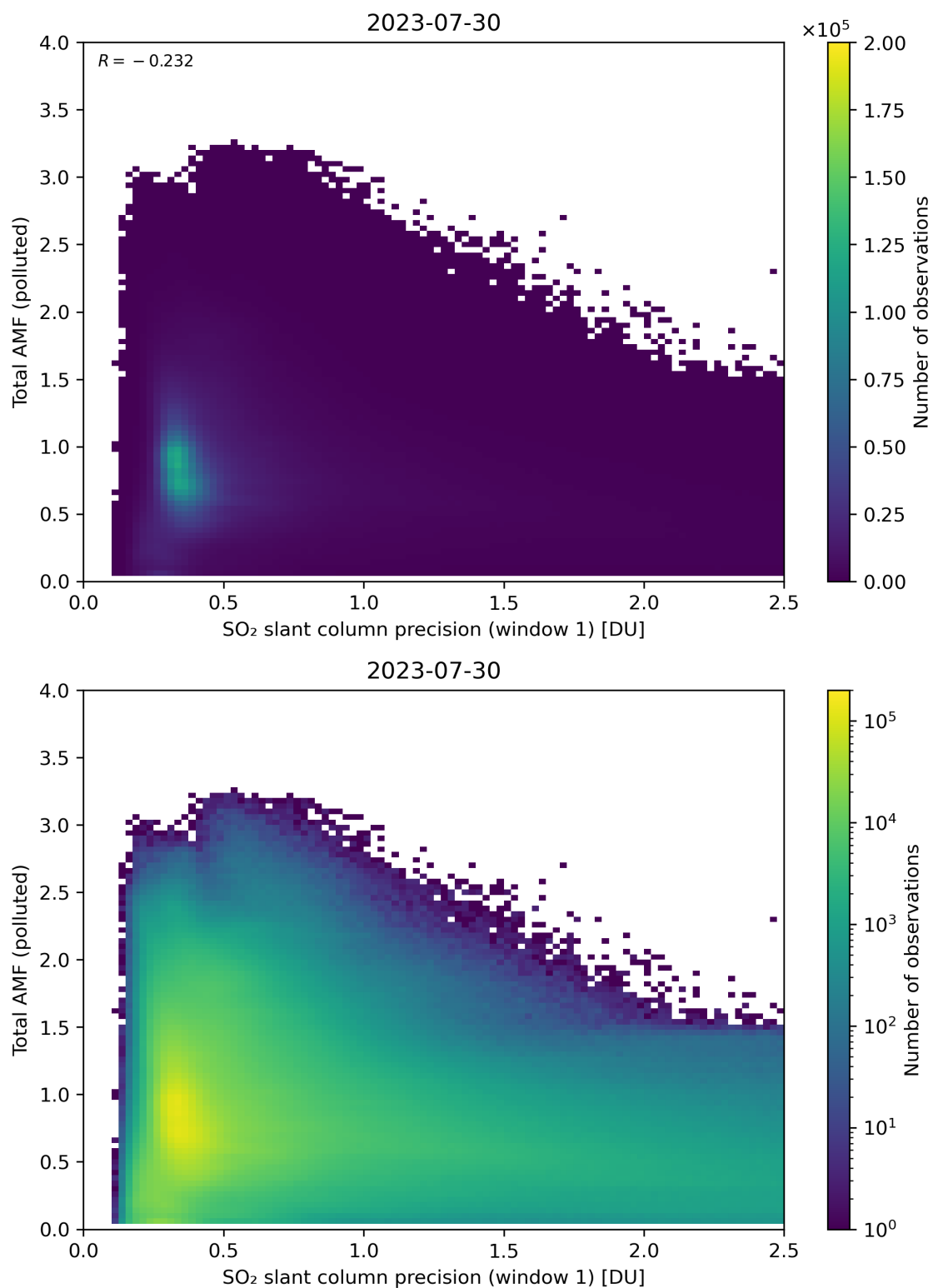
Figure 230: Scatter density plot of “SO 2 slant column precision (window 1)” against “Total AMF (polluted)” for 2023-07-29 to 2023-07-31.
