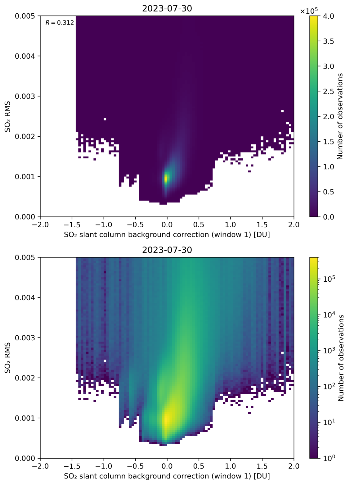
Figure 102: Scatter density plot of “SO 2 slant column background correction (window 1)” against “SO 2 RMS” for 2023-07-29 to 2023-07-31.
