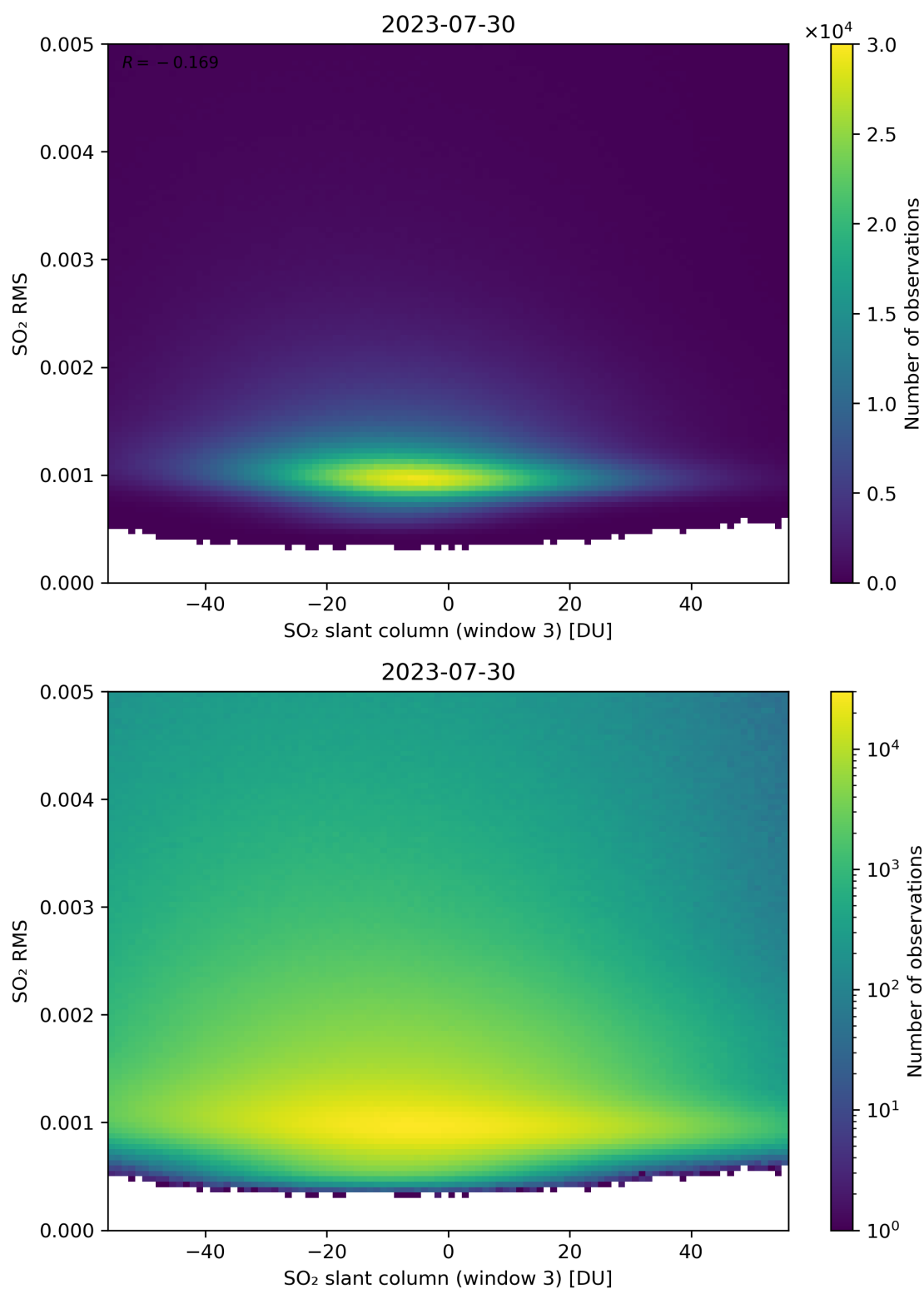
Figure 256: Scatter density plot of “SO 2 slant column (window 3)” against “SO 2 RMS” for 2023-07-29 to 2023-07-31.
