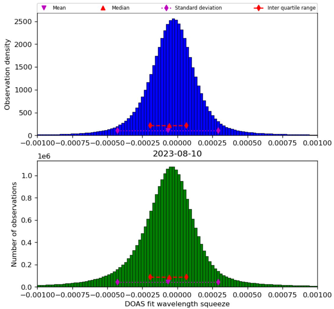
Figure 69: Histogram of “DOAS fit wavelength squeeze” for 2023-08-09 to 2023-08-11
