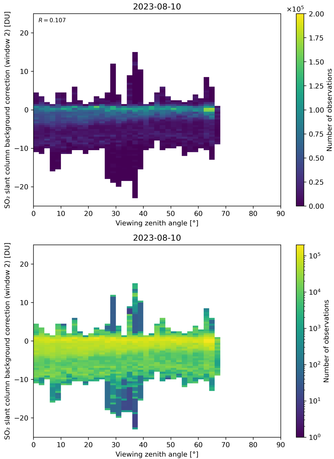
Figure 309: Scatter density plot of “Viewing zenith angle” against “SO 2 slant column background correction (window 2)” for 2023-08-09 to 2023-08-11.
