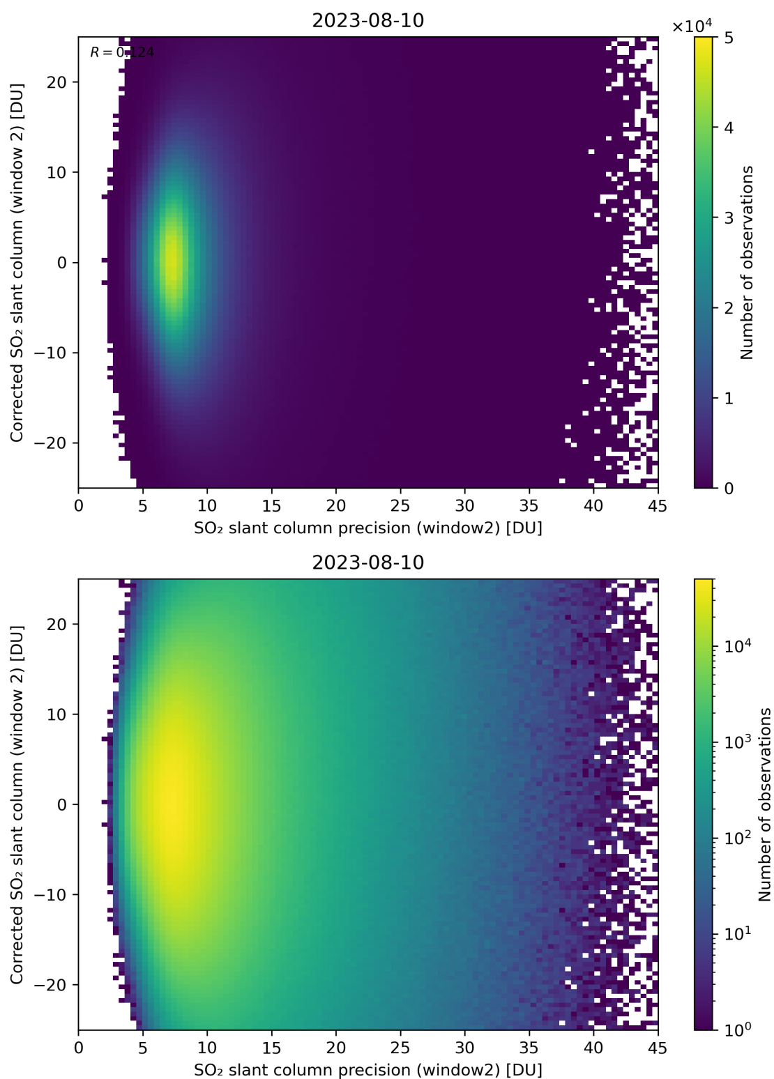
Figure 247: Scatter density plot of “SO 2 slant column precision (window2)” against “Corrected SO 2 slant column (window 2)” for 2023-08-09 to 2023-08-11.
