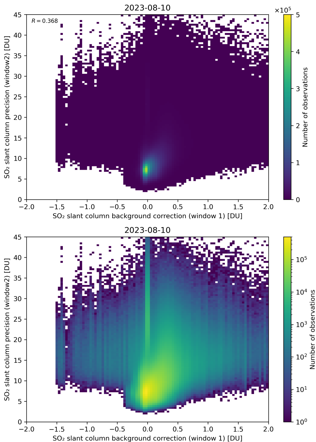
Figure 106: Scatter density plot of “SO 2 slant column background correction (window 1)” against “SO 2 slant column precision (window2)” for 2023-08-09 to 2023-08-11.
