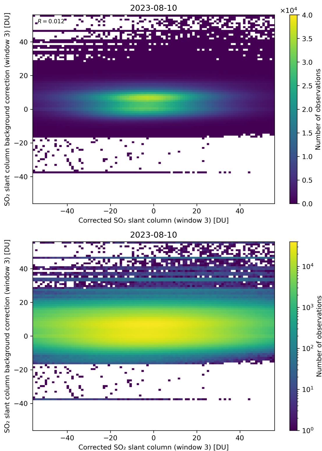
Figure 205: Scatter density plot of “Corrected SO 2 slant column (window 3)” against “SO 2 slant column background correction (window 3)” for 2023-08-09 to 2023-08-11.
