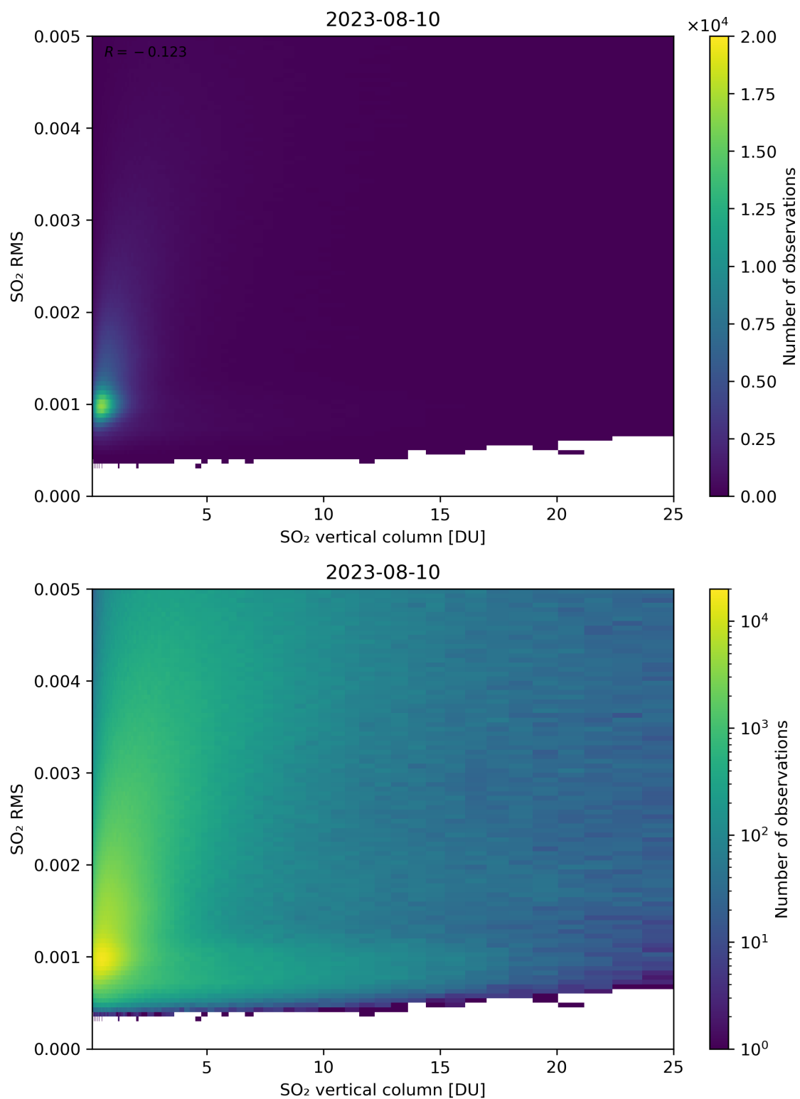
Figure 278: Scatter density plot of “SO 2 vertical column” against “SO 2 RMS” for 2023-08-09 to 2023-08-11.
