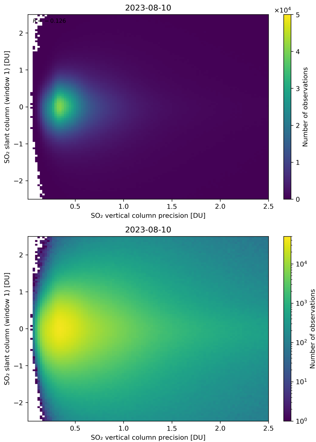
Figure 289: Scatter density plot of “SO 2 vertical column precision” against “SO 2 slant column (window 1)” for 2023-08-09 to 2023-08-11.
