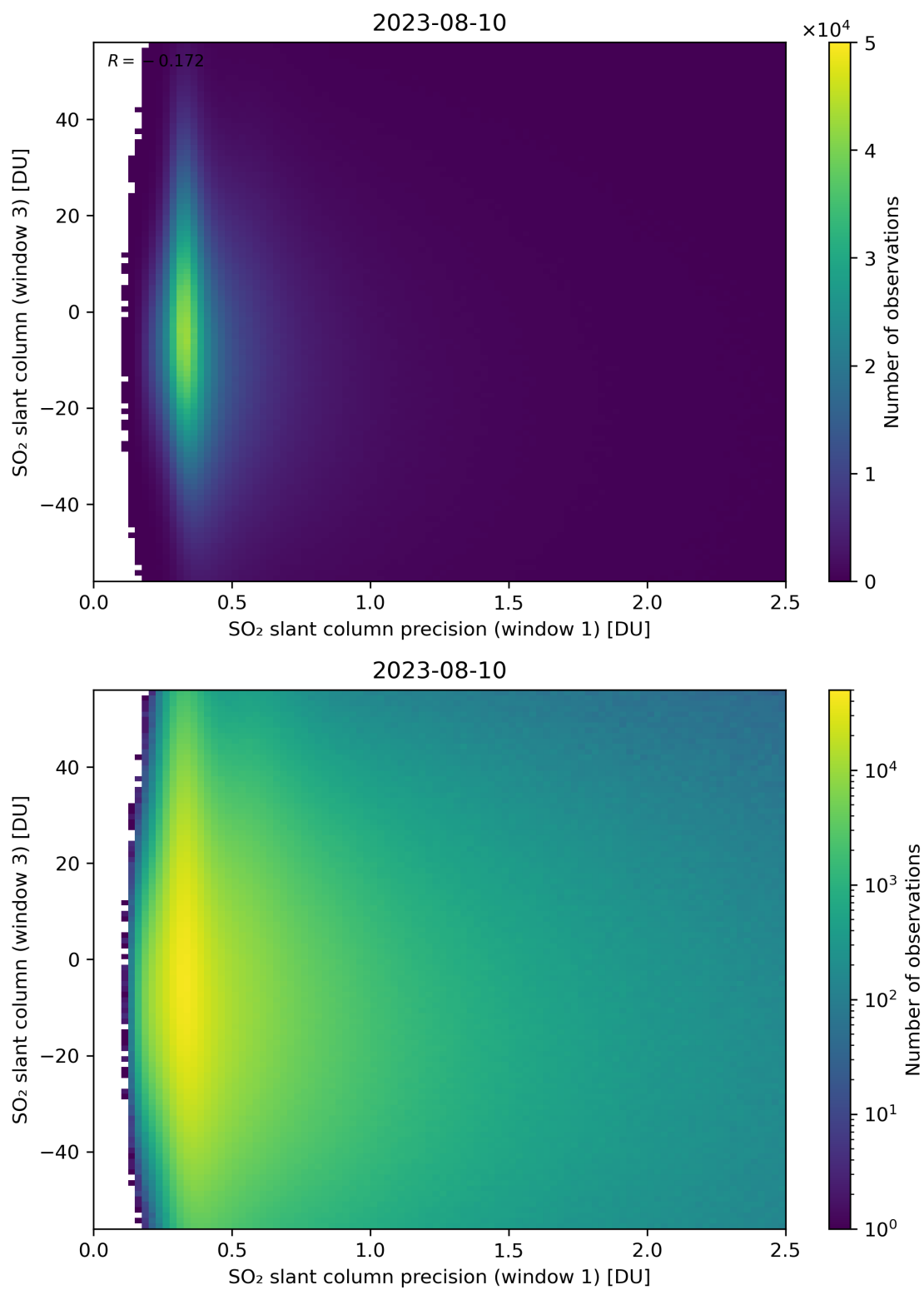
Figure 228: Scatter density plot of “SO 2 slant column precision (window 1)” against “SO 2 slant column (window 3)” for 2023-08-09 to 2023-08-11.
