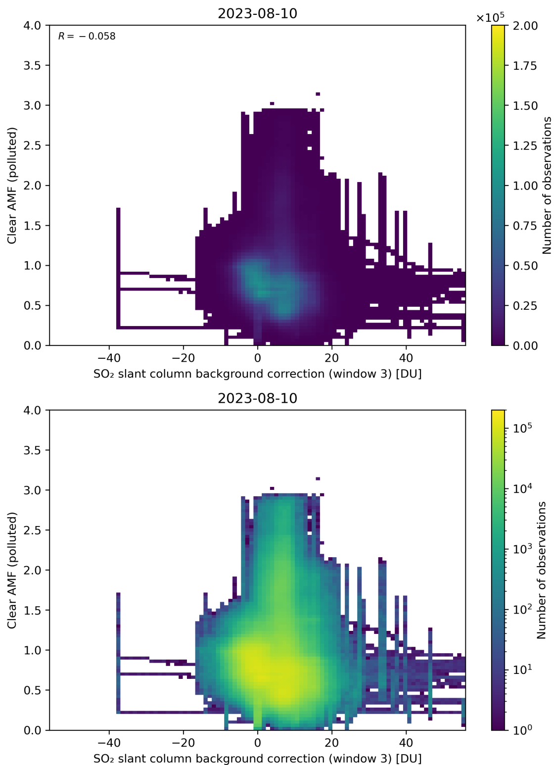
Figure 124: Scatter density plot of “SO 2 slant column background correction (window 3)” against “Clear AMF (polluted)” for 2023-08-09 to 2023-08-11.
