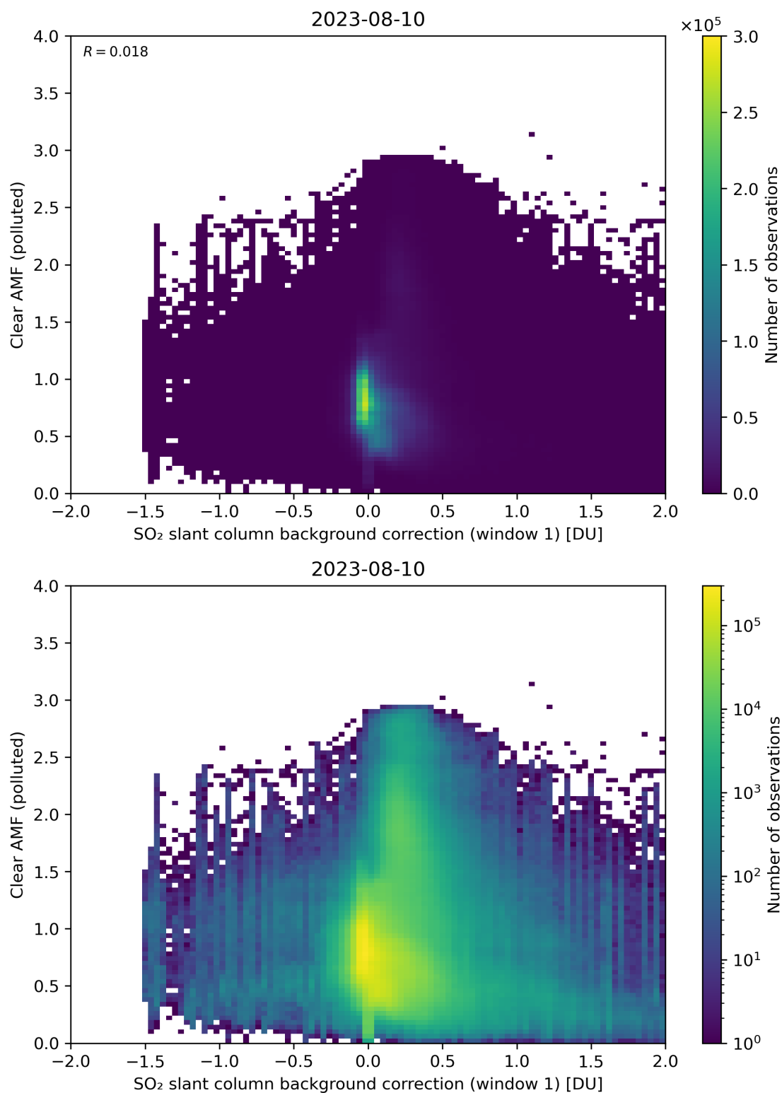
Figure 103: Scatter density plot of “SO 2 slant column background correction (window 1)” against “Clear AMF (polluted)” for 2023-08-09 to 2023-08-11.
