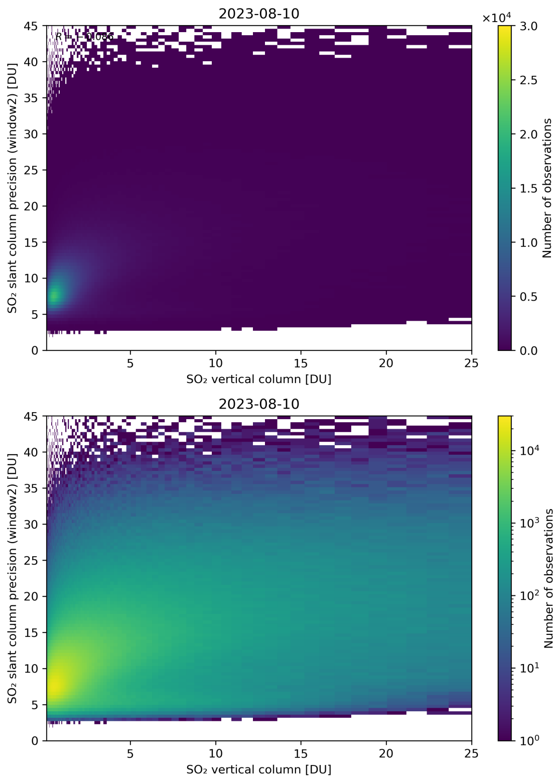
Figure 302: Scatter density plot of “SO 2 vertical column” against “SO 2 slant column precision (window2)” for 2023-08-09 to 2023-08-11.
