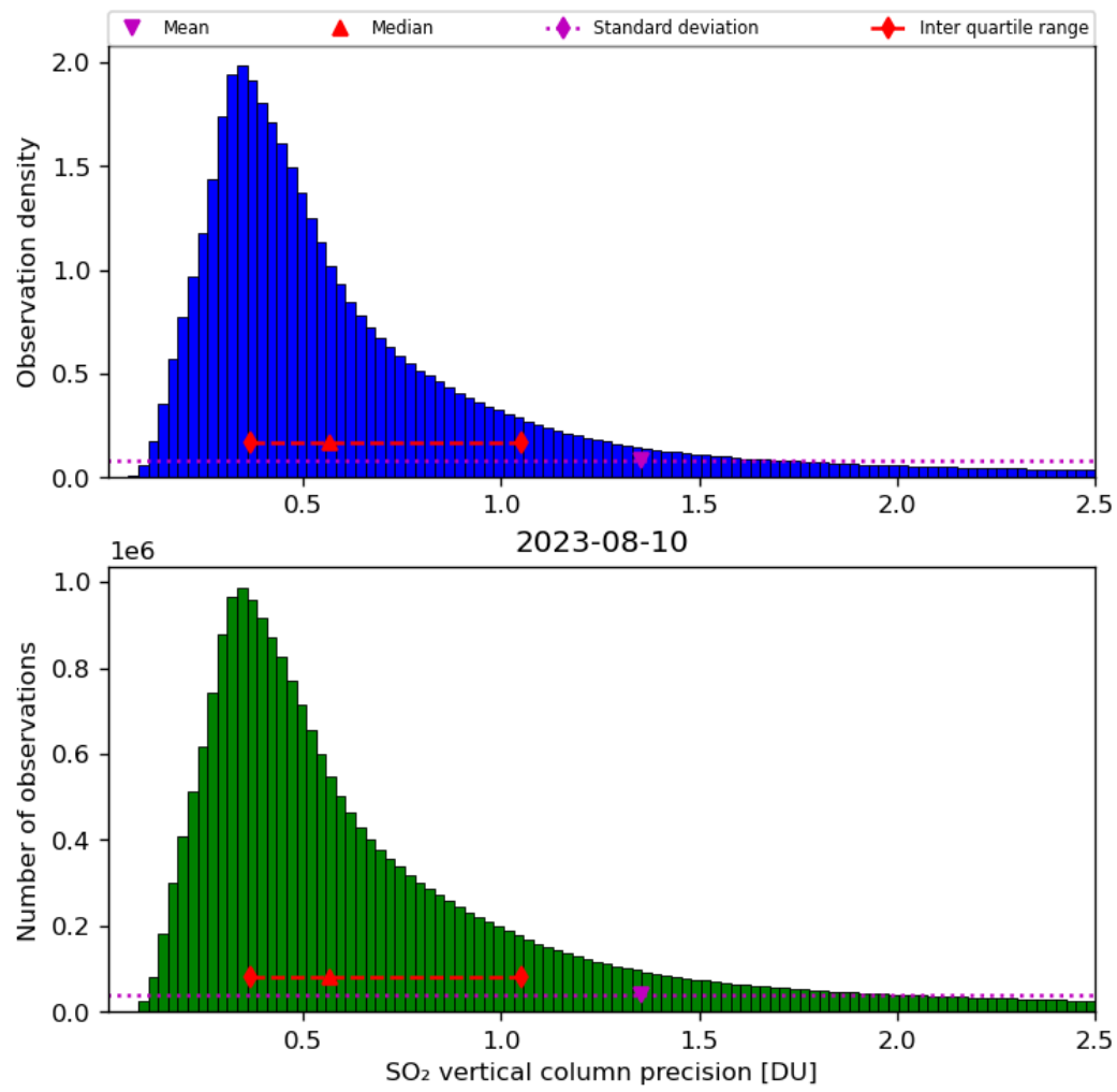
Figure 54: Histogram of “SO 2 vertical column precision” for 2023-08-09 to 2023-08-11
