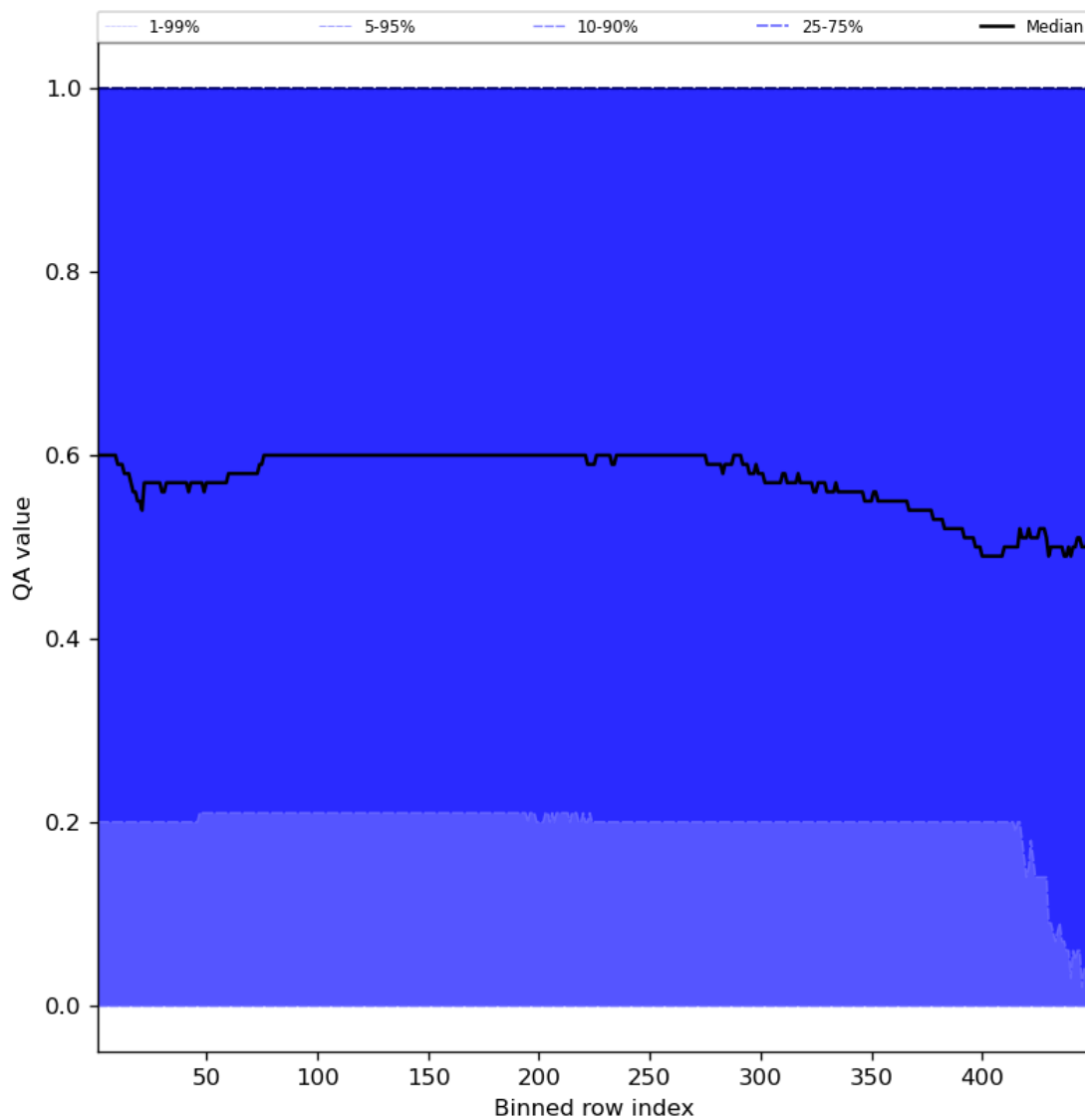
Figure 75: Along track statistics of “QA value” for 2023-08-09 to 2023-08-11
