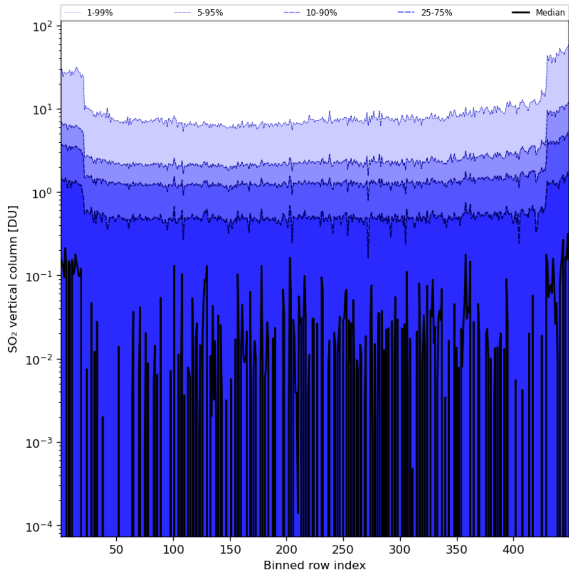
Figure 76: Along track statistics of “SO 2 vertical column” for 2023-08-09 to 2023-08-11
