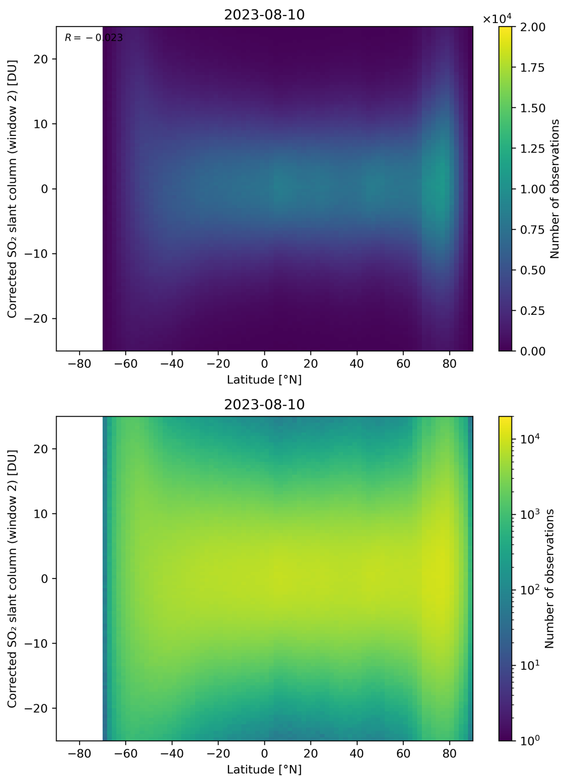
Figure 147: Scatter density plot of “Latitude” against “Corrected SO 2 slant column (window 2)” for 2023-08-09 to 2023-08-11.
