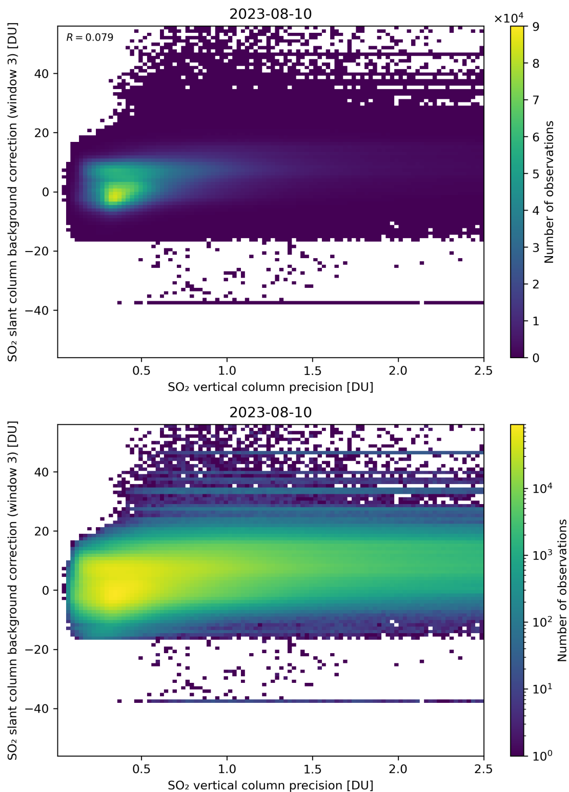
Figure 281: Scatter density plot of “SO 2 vertical column precision” against “SO 2 slant column background correction (window 3)” for 2023-08-09 to 2023-08-11.
