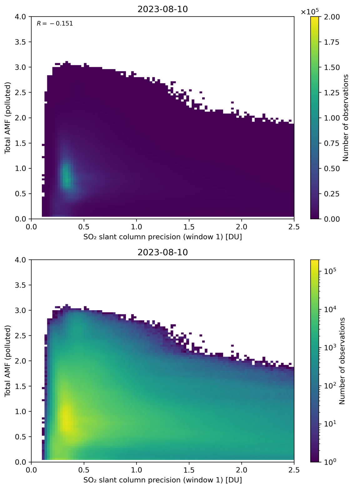
Figure 230: Scatter density plot of “SO 2 slant column precision (window 1)” against “Total AMF (polluted)” for 2023-08-09 to 2023-08-11.
