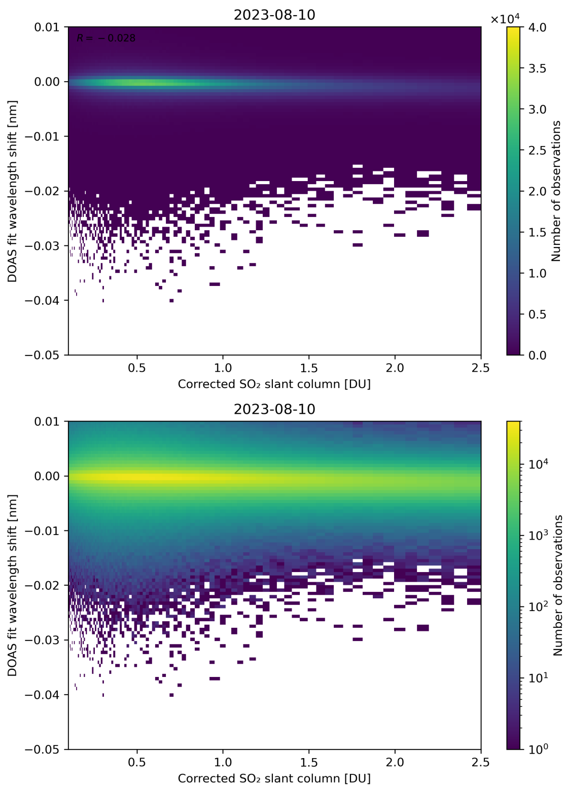
Figure 181: Scatter density plot of “Corrected SO 2 slant column” against “DOAS fit wavelength shift” for 2023-08-09 to 2023-08-11.
