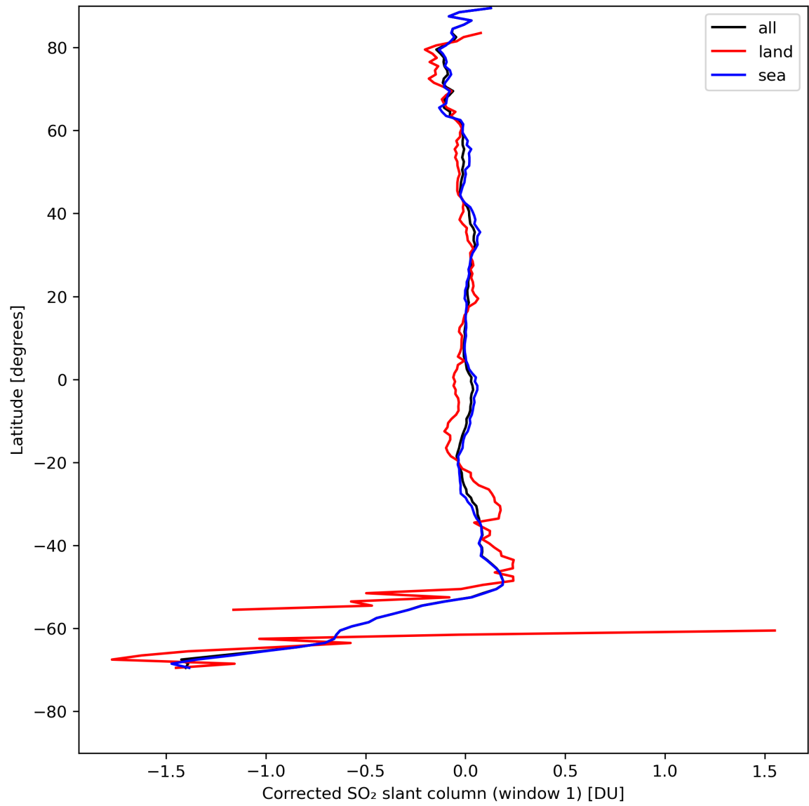
Figure 35: Zonal average of “Corrected SO 2 slant column (window 1)” for 2023-08-09 to 2023-08-11.
