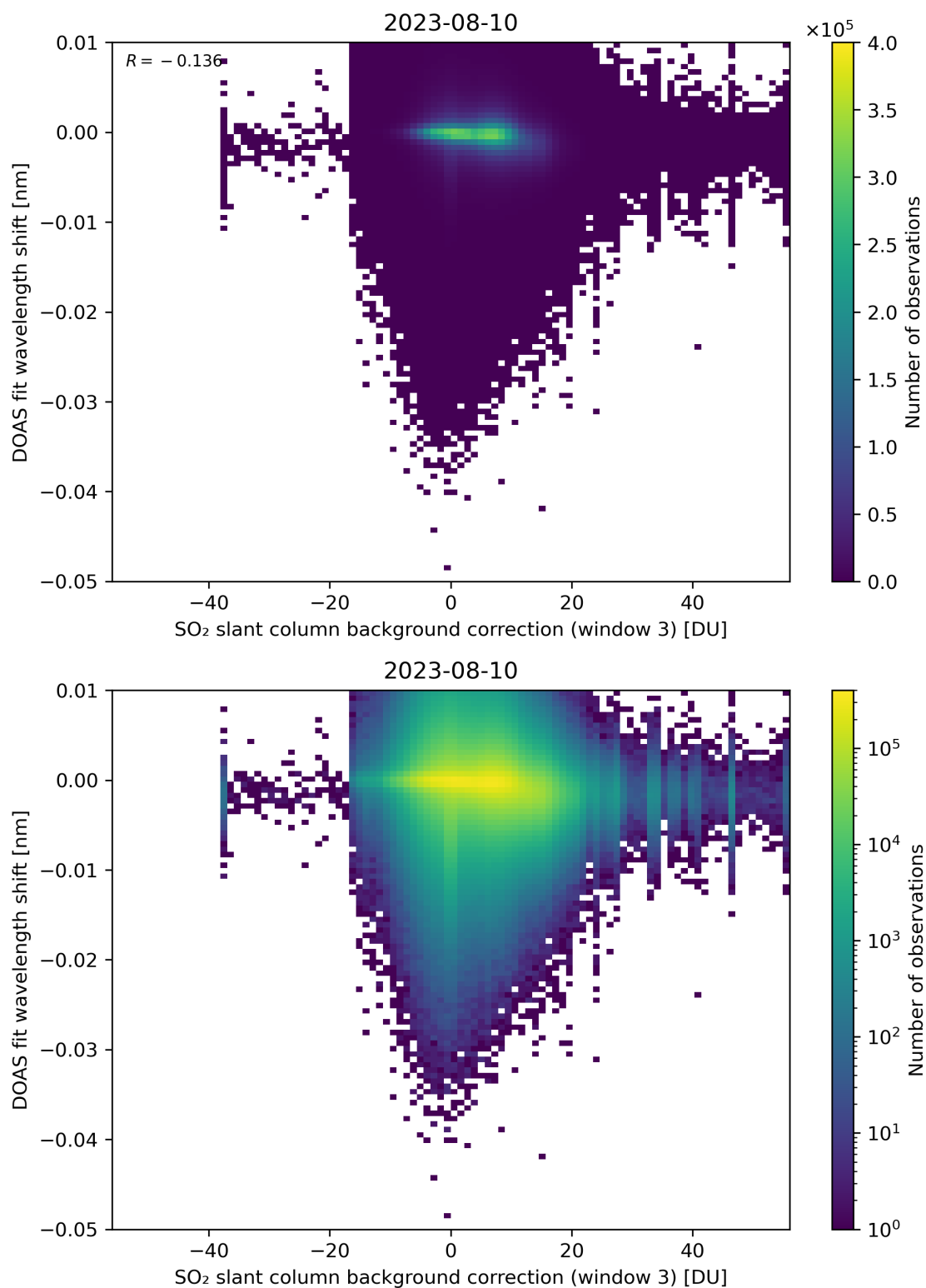
Figure 121: Scatter density plot of “SO 2 slant column background correction (window 3)” against “DOAS fit wavelength shift” for 2023-08-09 to 2023-08-11.
