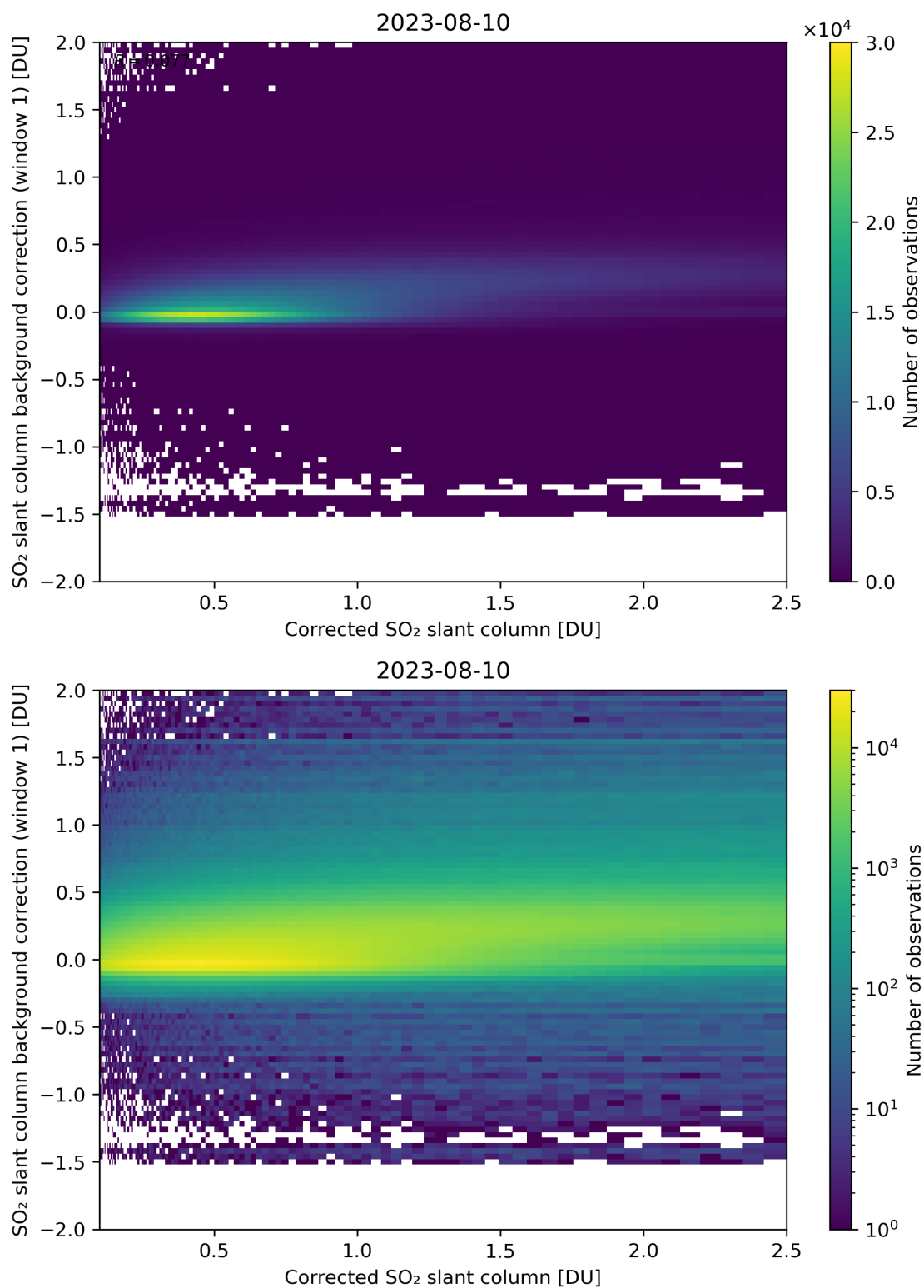
Figure 178: Scatter density plot of “Corrected SO 2 slant column” against “SO 2 slant column background correction (window 1)” for 2023-08-09 to 2023-08-11.
