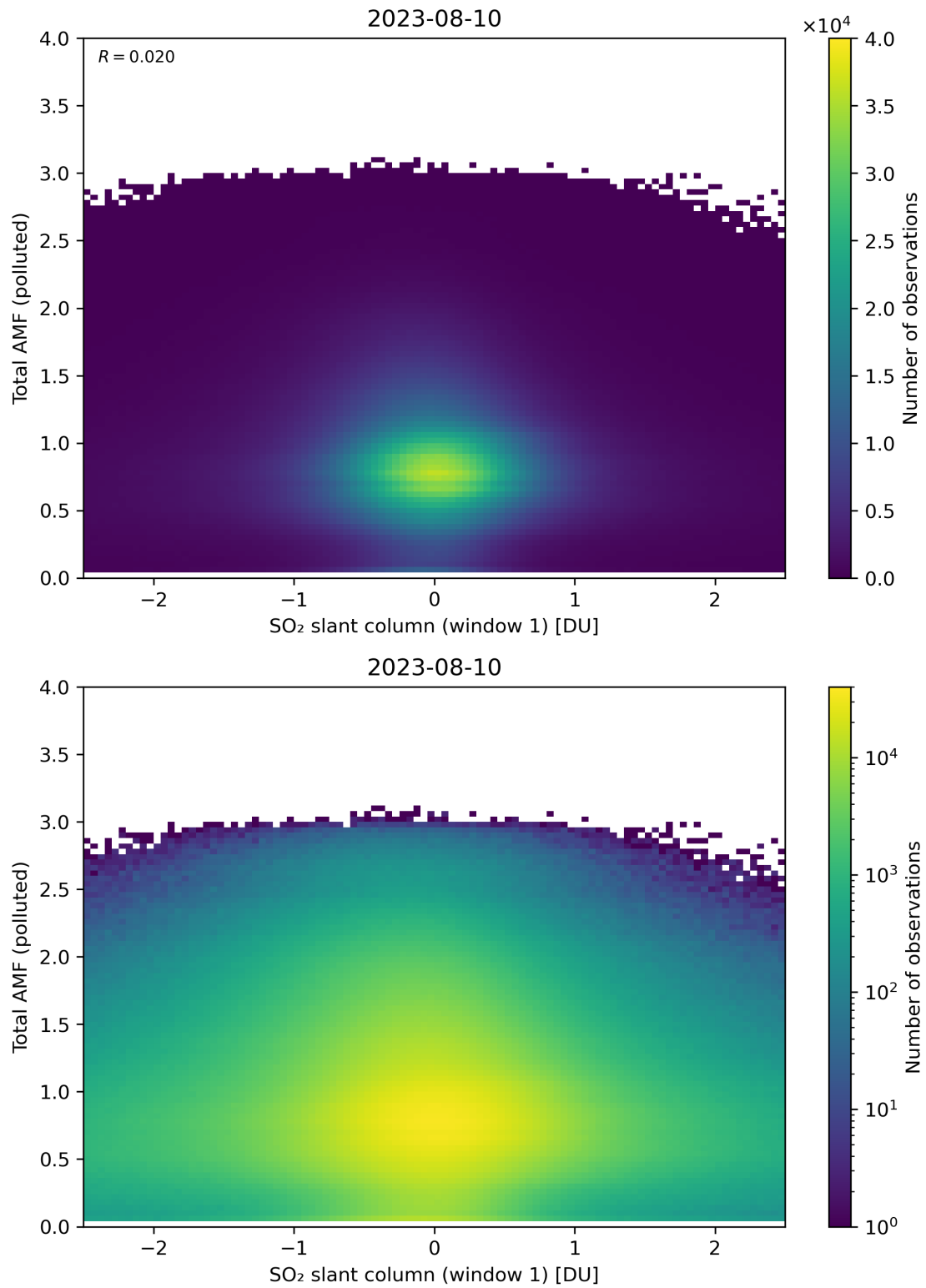
Figure 239: Scatter density plot of “SO 2 slant column (window 1)” against “Total AMF (polluted)” for 2023-08-09 to 2023-08-11.
