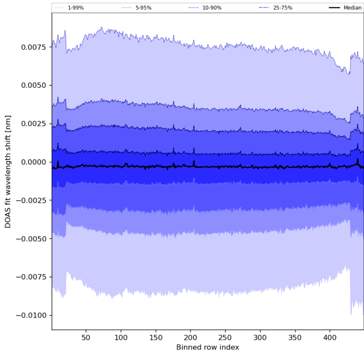
Figure 91: Along track statistics of “DOAS fit wavelength shift” for 2023-08-09 to 2023-08-11
