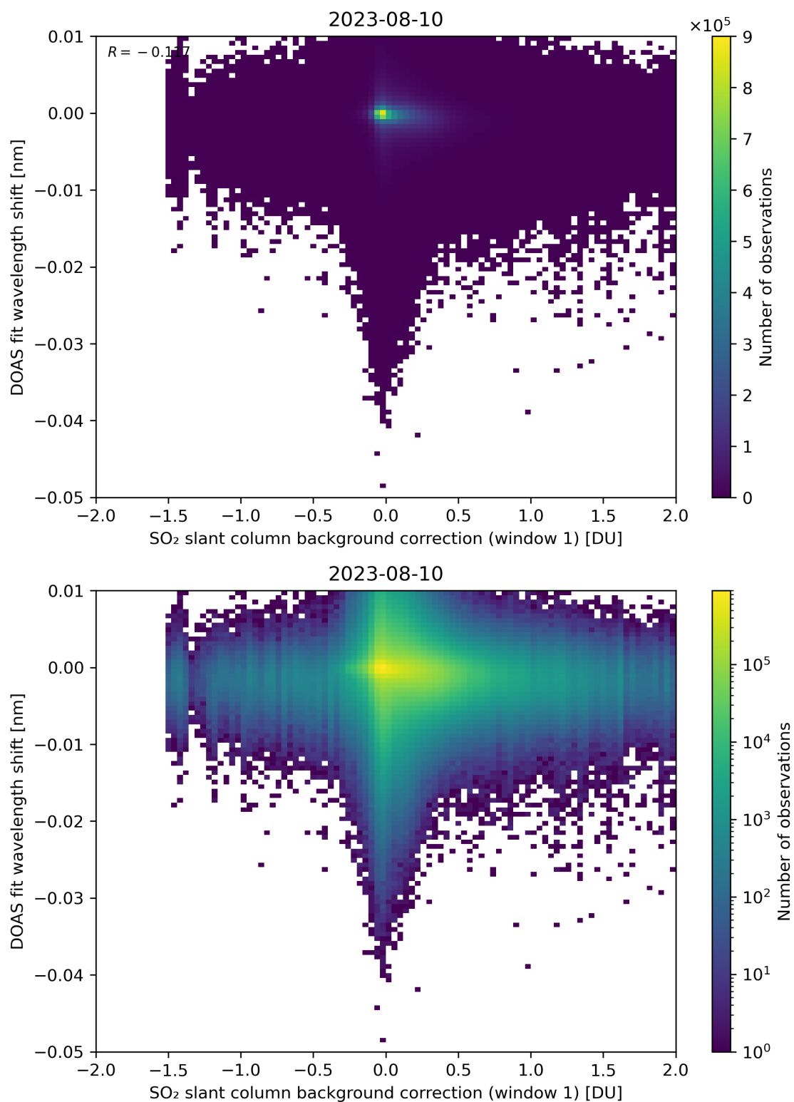
Figure 100: Scatter density plot of “SO 2 slant column background correction (window 1)” against “DOAS fit wavelength shift” for 2023-08-09 to 2023-08-11.
