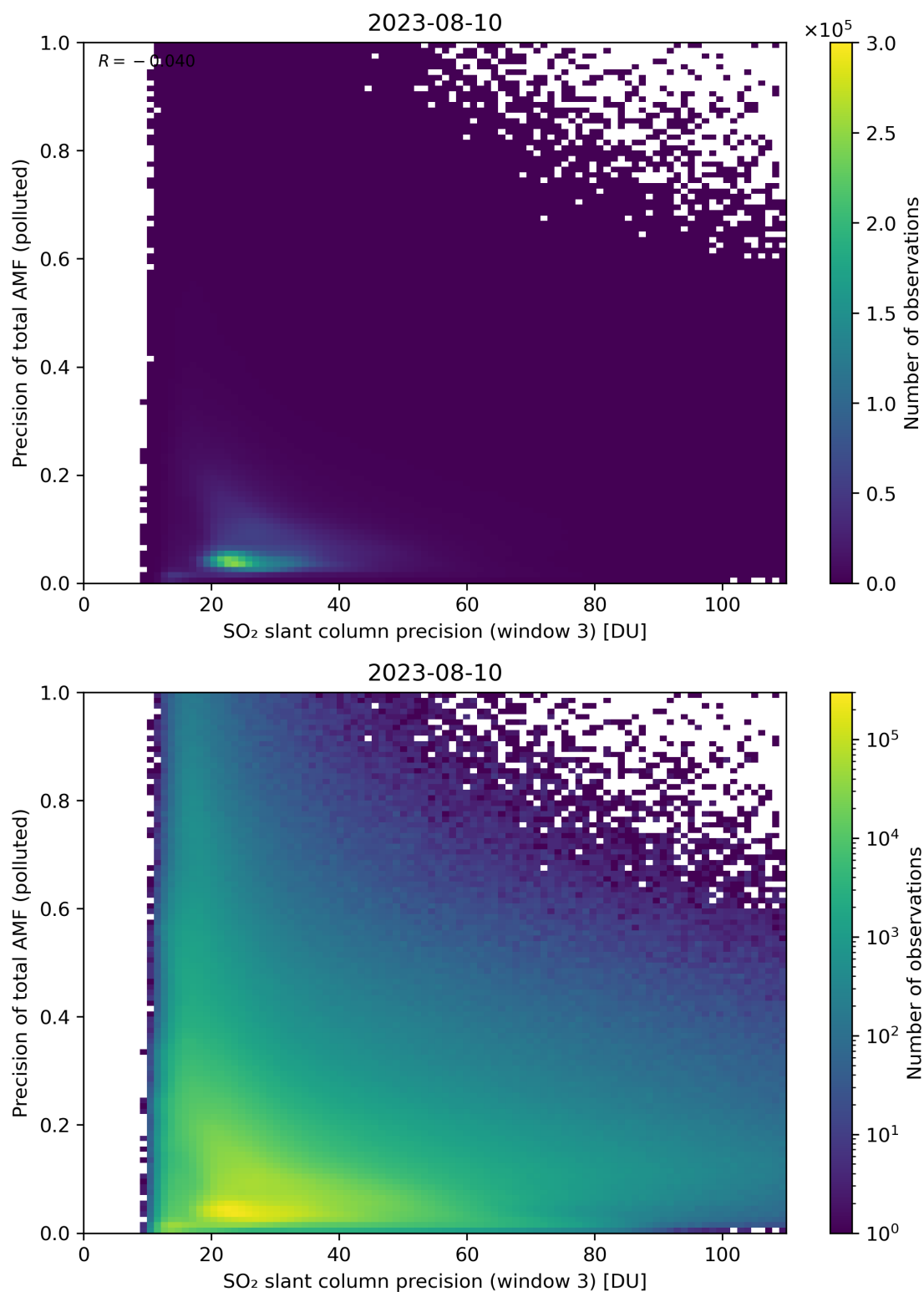
Figure 264: Scatter density plot of “SO 2 slant column precision (window 3)” against “Precision of total AMF (polluted)” for 2023-08-09 to 2023-08-11.
