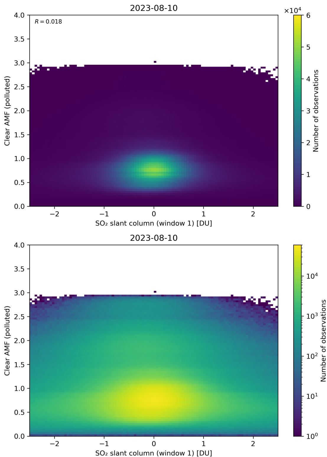
Figure 232: Scatter density plot of “SO 2 slant column (window 1)” against “Clear AMF (polluted)” for 2023-08-09 to 2023-08-11.
