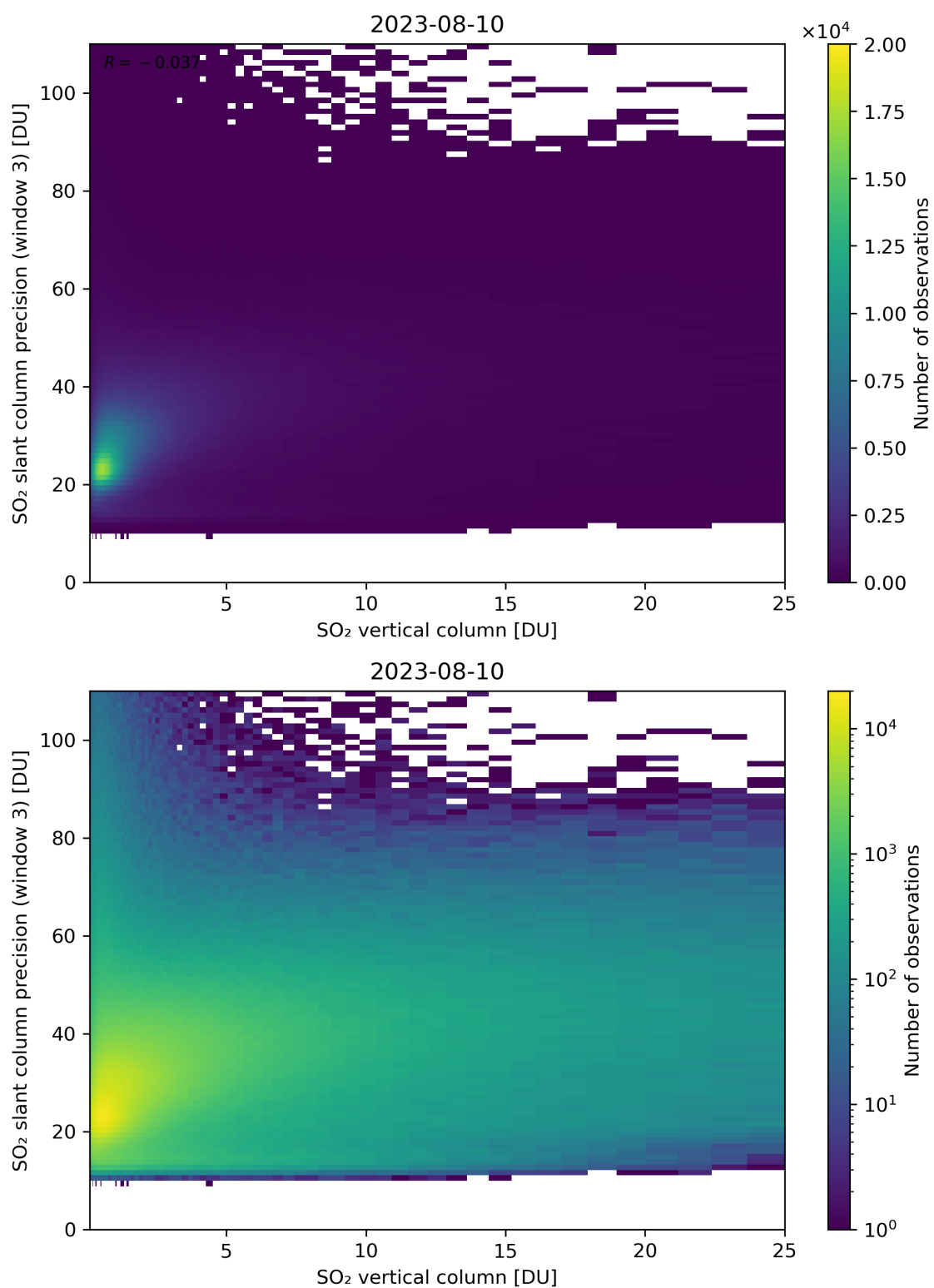
Figure 304: Scatter density plot of “SO 2 vertical column” against “SO 2 slant column precision (window 3)” for 2023-08-09 to 2023-08-11.
