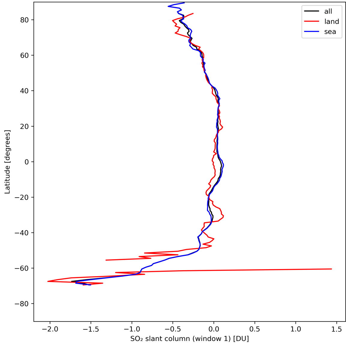
Figure 33: Zonal average of “SO 2 slant column (window 1)” for 2023-08-09 to 2023-08-11.
