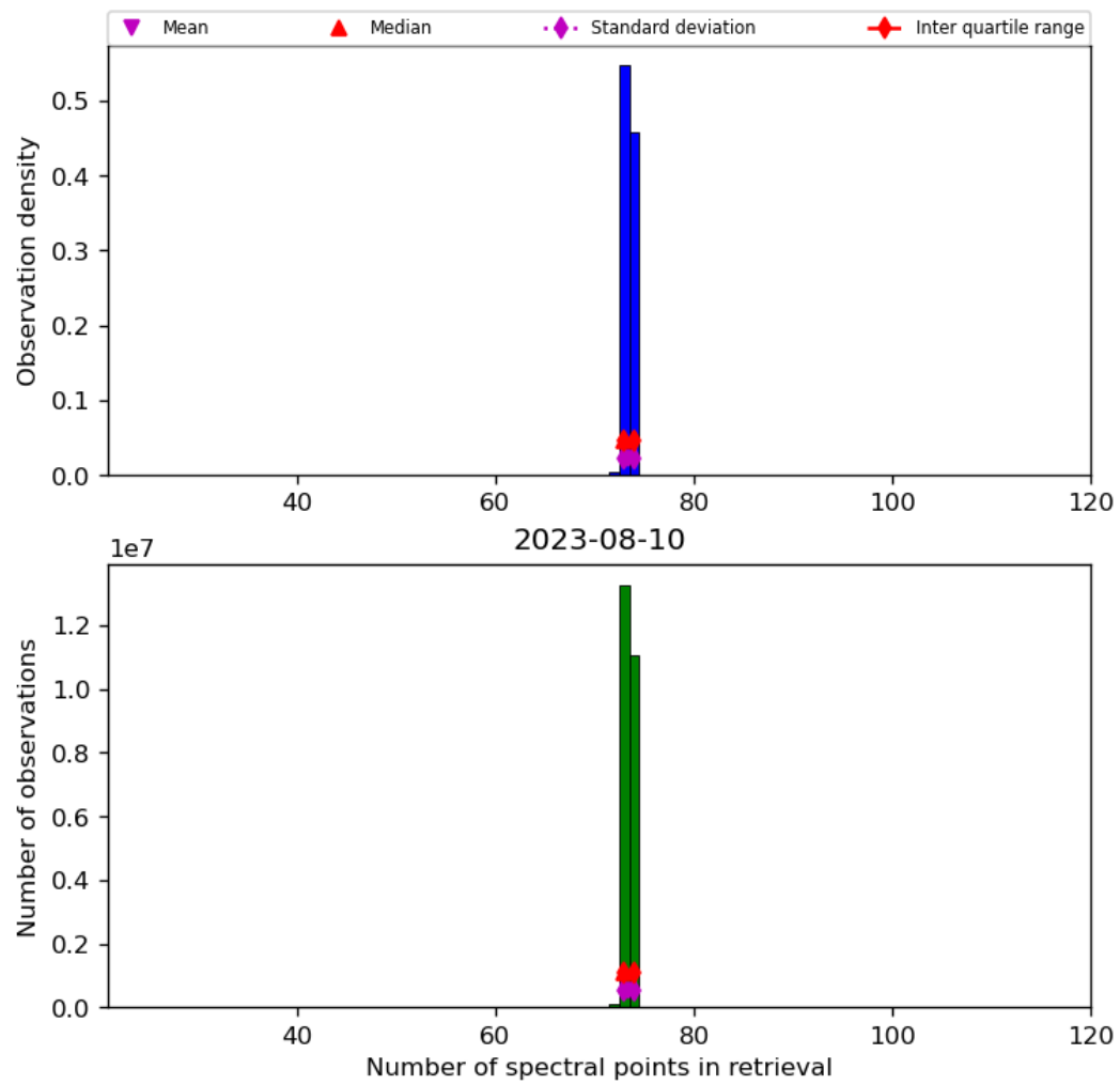
Figure 74: Histogram of “Number of spectral points in retrieval” for 2023-08-09 to 2023-08-11
