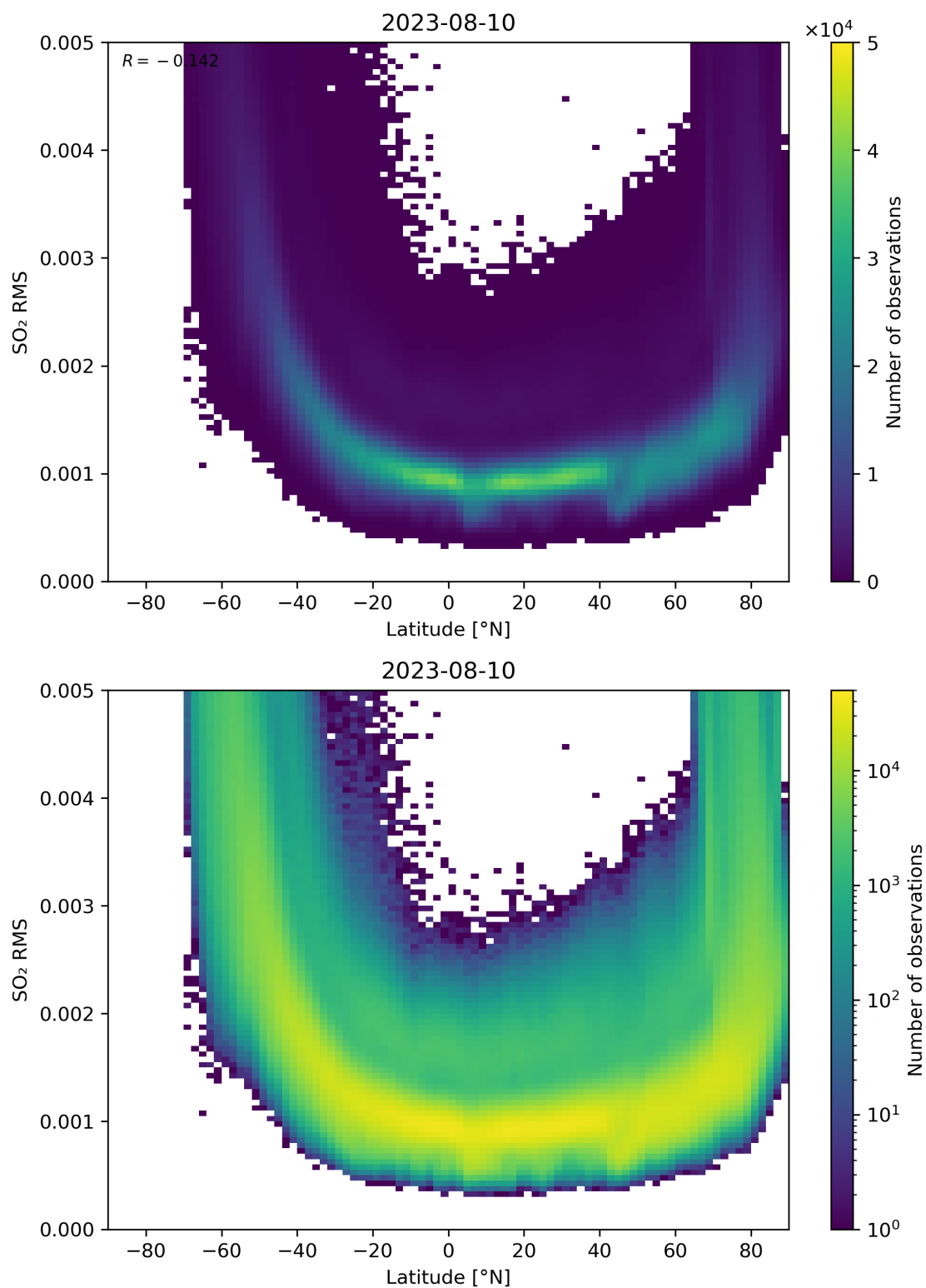
Figure 144: Scatter density plot of “Latitude” against “SO 2 RMS” for 2023-08-09 to 2023-08-11.
