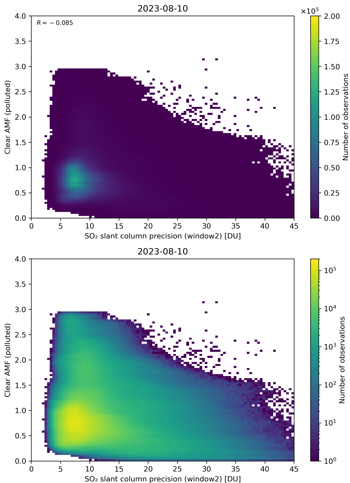
Figure 246: Scatter density plot of “SO 2 slant column precision (window2)” against “Clear AMF (polluted)” for 2023-08-09 to 2023-08-11.
