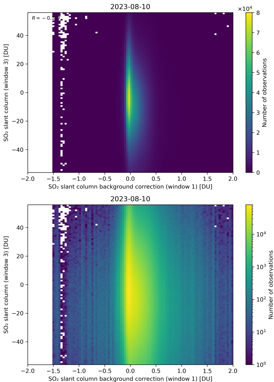
Figure 107: Scatter density plot of “SO 2 slant column background correction (window 1)” against “SO 2 slant column (window 3)” for 2023-08-09 to 2023-08-11.
