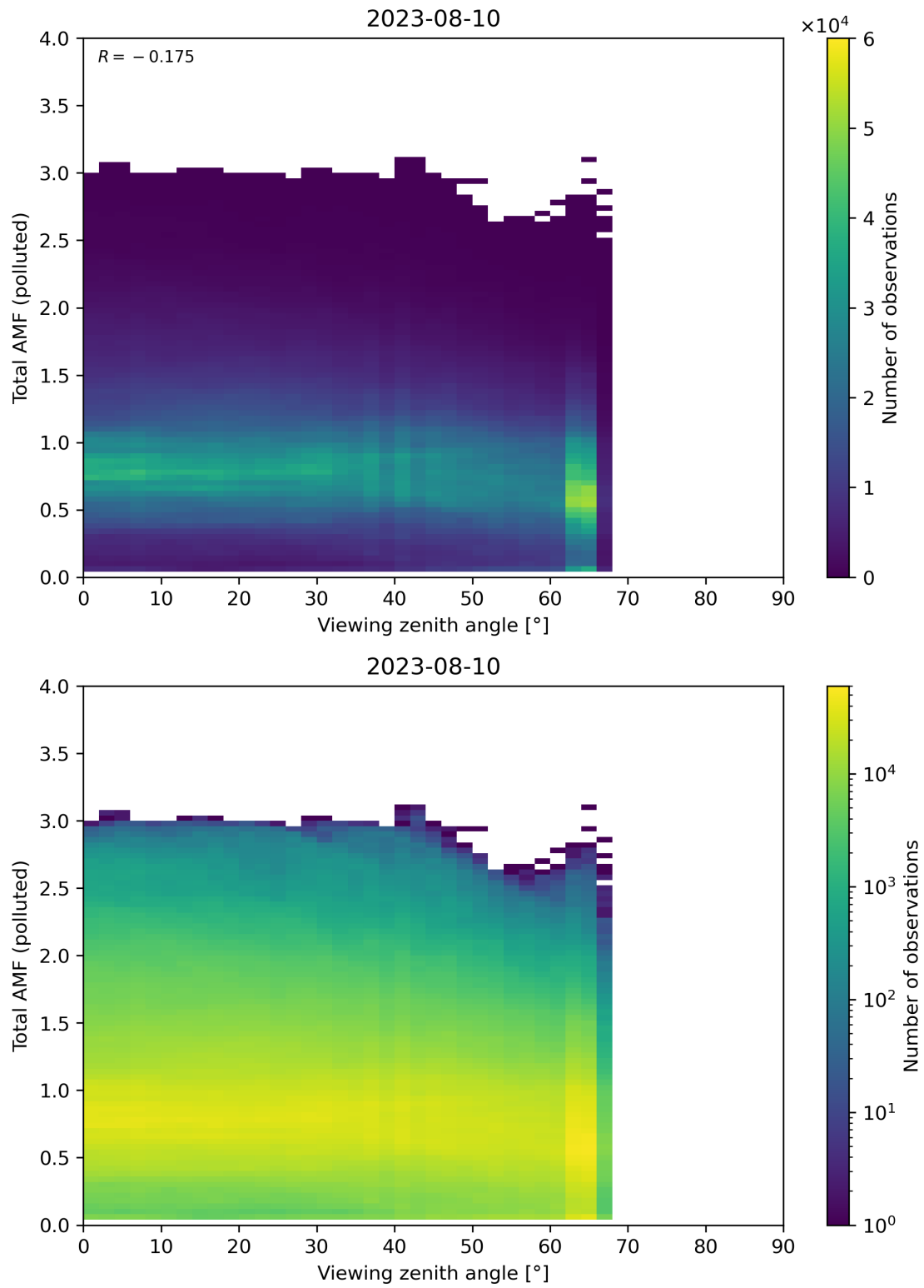
Figure 325: Scatter density plot of “Viewing zenith angle” against “Total AMF (polluted)” for 2023-08-09 to 2023-08-11.
