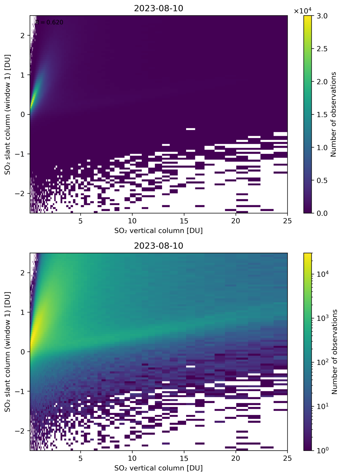
Figure 300: Scatter density plot of “SO 2 vertical column” against “SO 2 slant column (window 1)” for 2023-08-09 to 2023-08-11.
