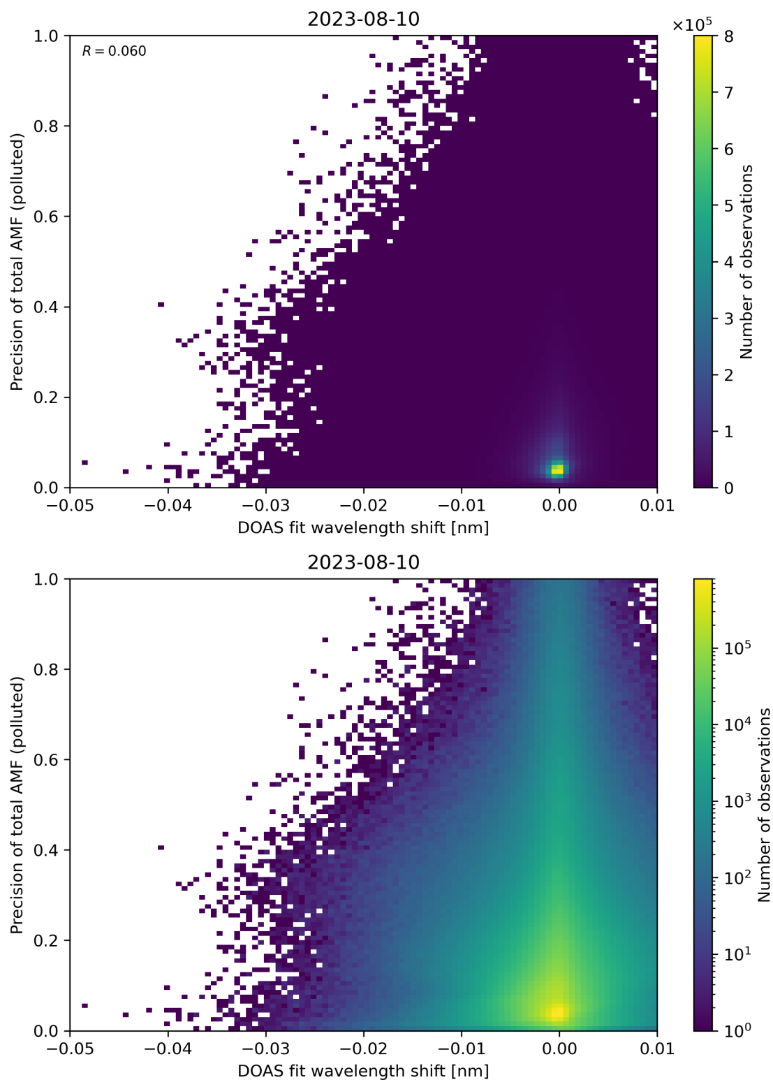
Figure 131: Scatter density plot of “DOAS fit wavelength shift” against “Precision of total AMF (polluted)” for 2023-08-09 to 2023-08-11.
