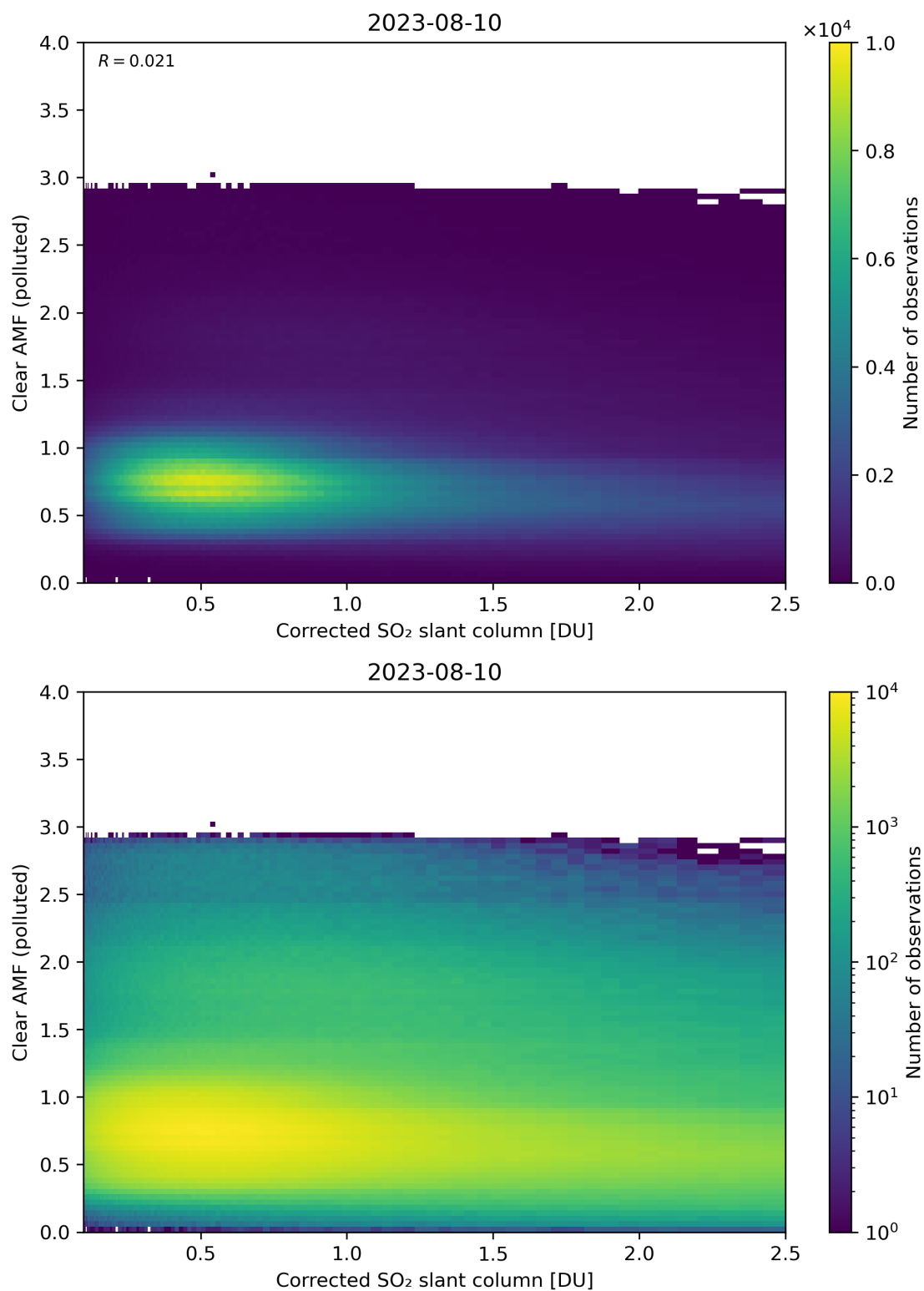
Figure 184: Scatter density plot of “Corrected SO 2 slant column” against “Clear AMF (polluted)” for 2023-08-09 to 2023-08-11.
