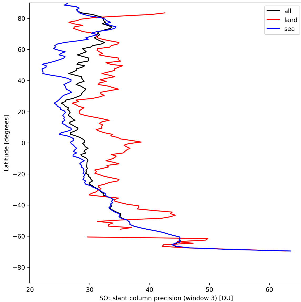
Figure 42: Zonal average of “SO 2 slant column precision (window 3)” for 2023-08-09 to 2023-08-11.
