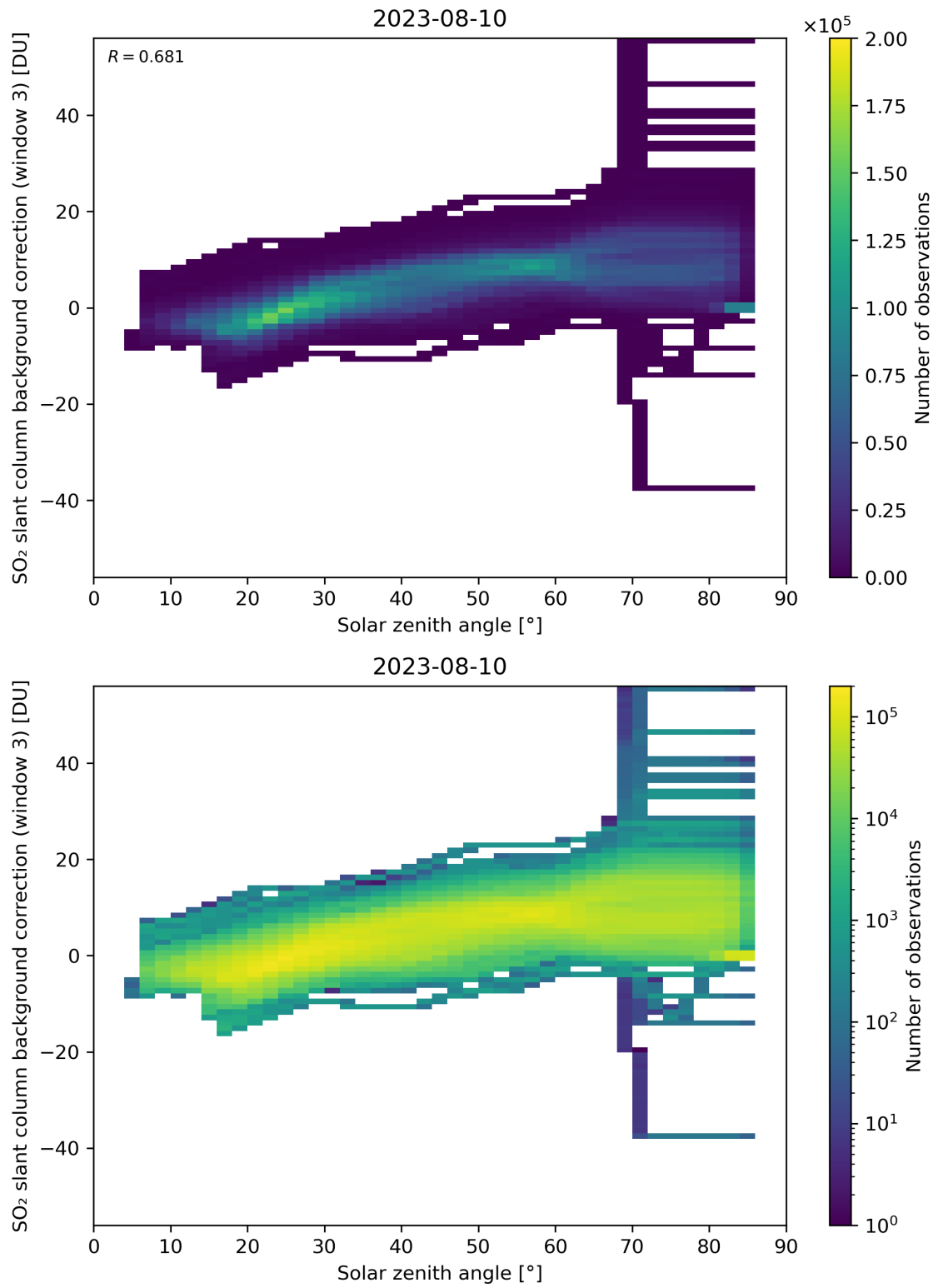
Figure 160: Scatter density plot of “Solar zenith angle” against “SO 2 slant column background correction (window 3)” for 2023-08-09 to 2023-08-11.
