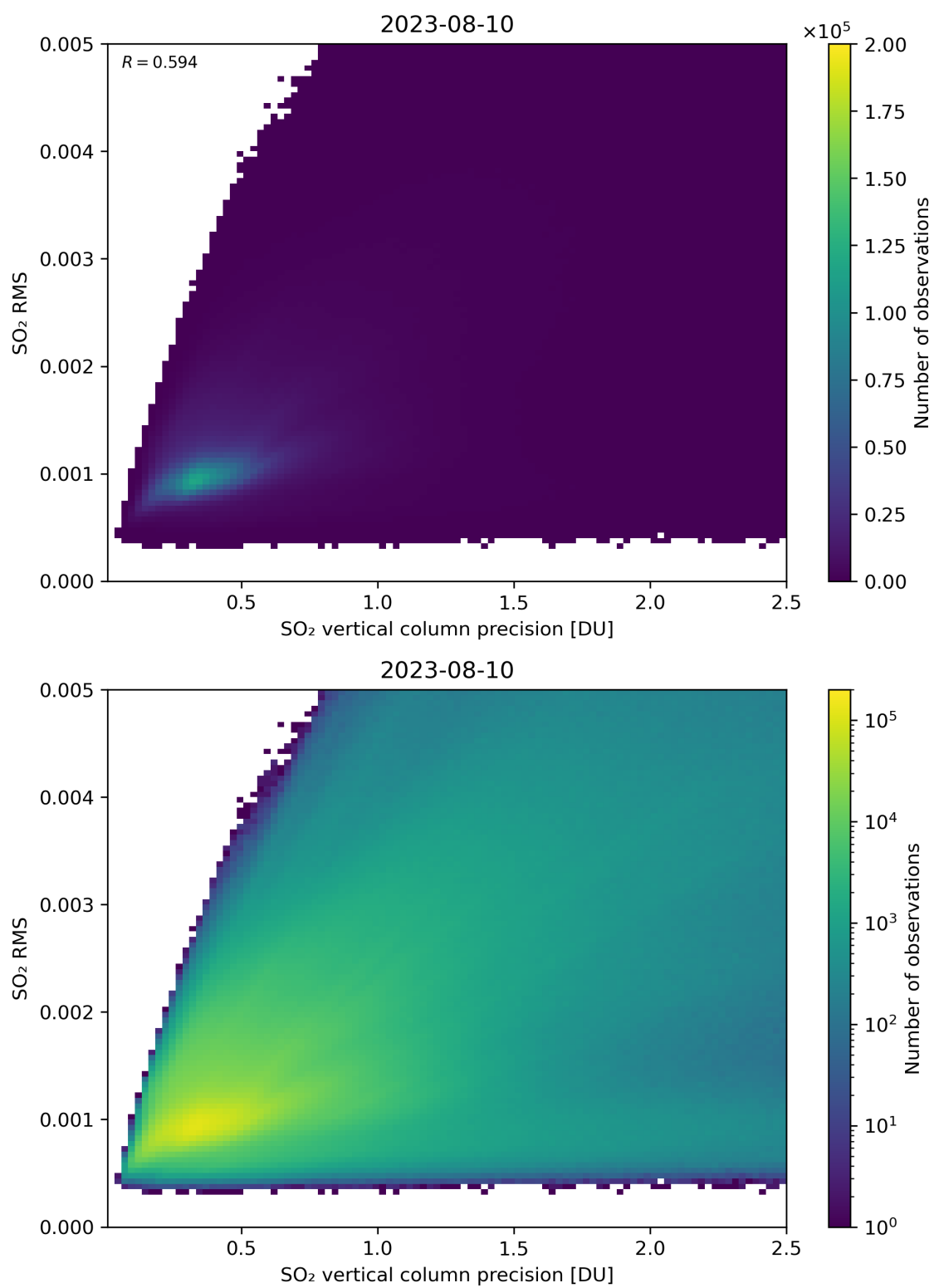
Figure 284: Scatter density plot of “SO 2 vertical column precision” against “SO 2 RMS” for 2023-08-09 to 2023-08-11.
