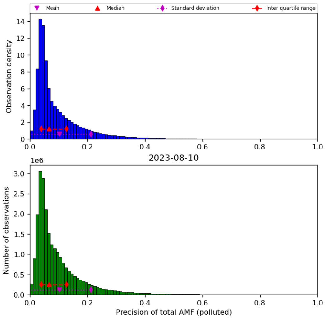
Figure 72: Histogram of “Precision of total AMF (polluted)” for 2023-08-09 to 2023-08-11
