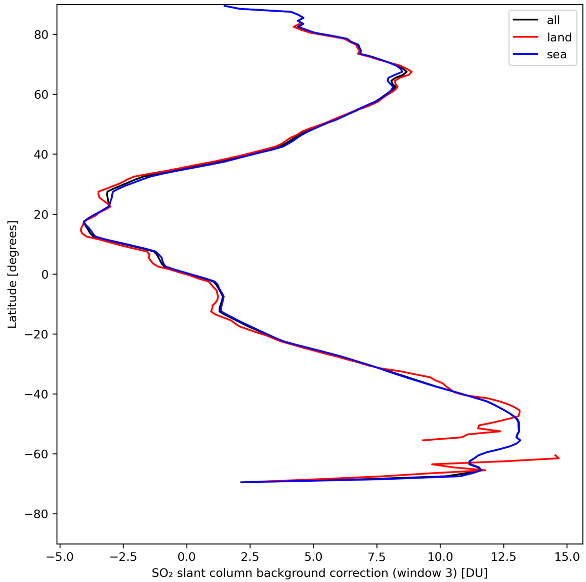
Figure 44: Zonal average of “SO 2 slant column background correction (window 3)” for 2023-08-09 to 2023-08-11.
