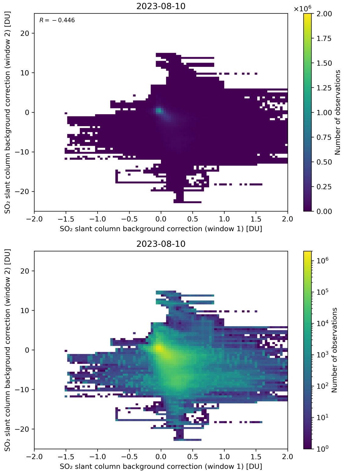
Figure 98: Scatter density plot of “SO 2 slant column background correction (window 1)” against “SO 2 slant column background correction (window 2)” for 2023-08-09 to 2023-08-11.
