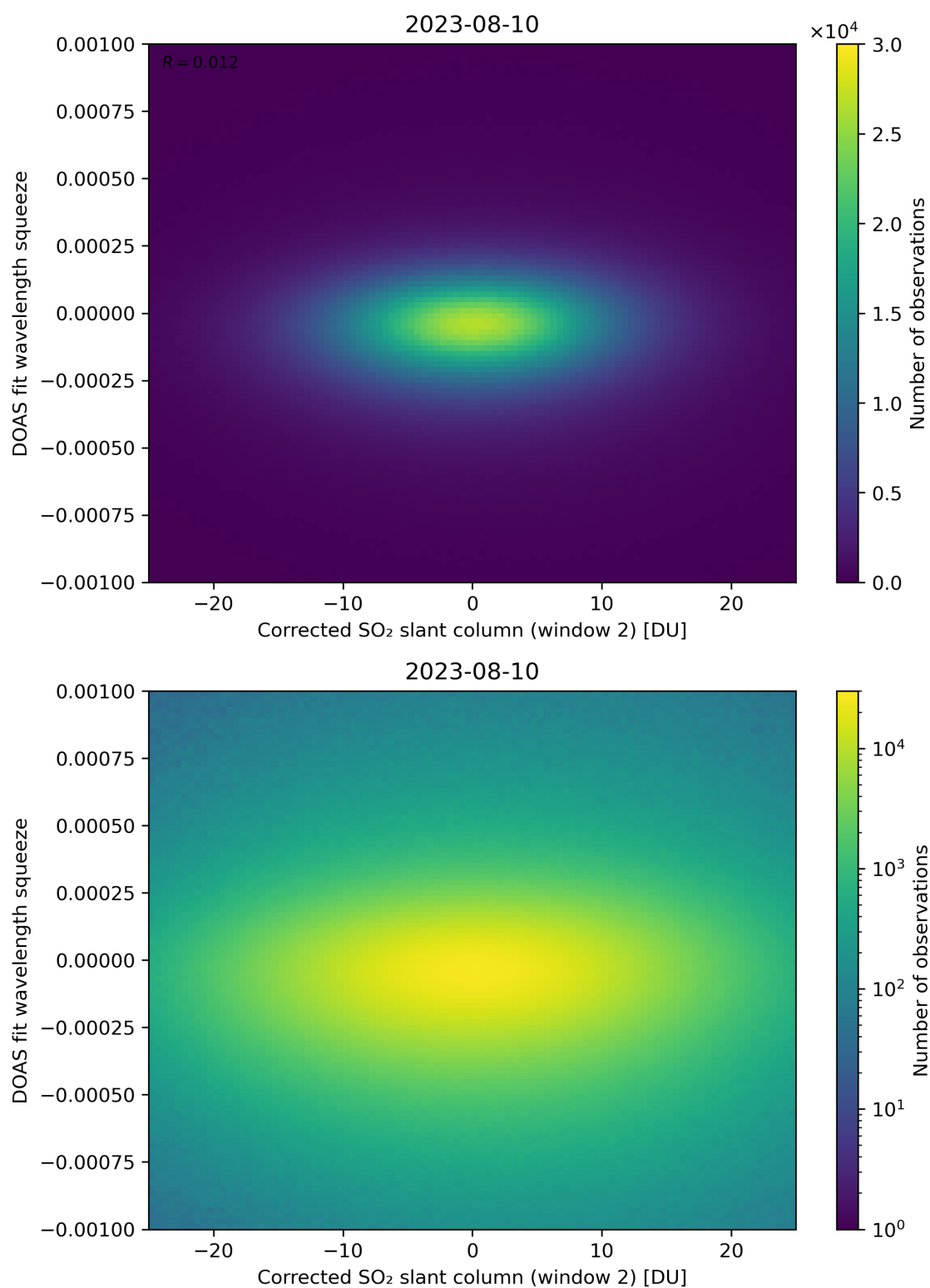
Figure 197: Scatter density plot of “Corrected SO 2 slant column (window 2)” against “DOAS fit wavelength squeeze” for 2023-08-09 to 2023-08-11.
