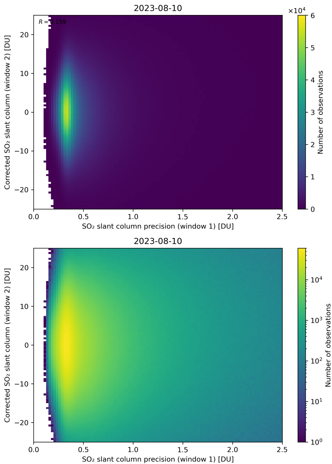
Figure 225: Scatter density plot of “SO 2 slant column precision (window 1)” against “Corrected SO 2 slant column (window 2)” for 2023-08-09 to 2023-08-11.
