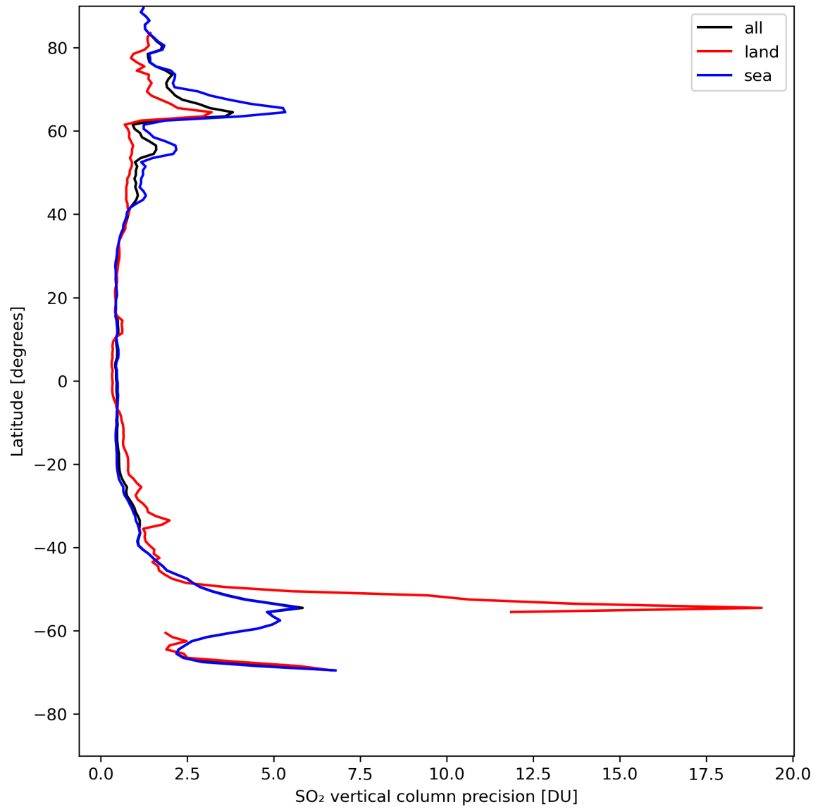
Figure 31: Zonal average of “SO 2 vertical column precision” for 2023-08-09 to 2023-08-11.
