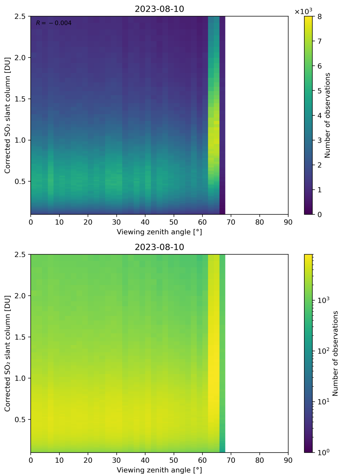
Figure 317: Scatter density plot of “Viewing zenith angle” against “Corrected SO 2 slant column” for 2023-08-09 to 2023-08-11.
