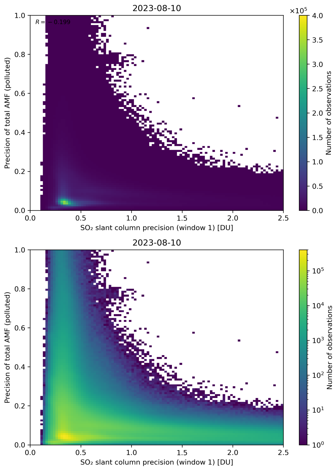
Figure 231: Scatter density plot of “SO 2 slant column precision (window 1)” against “Precision of total AMF (polluted)” for 2023-08-09 to 2023-08-11.
