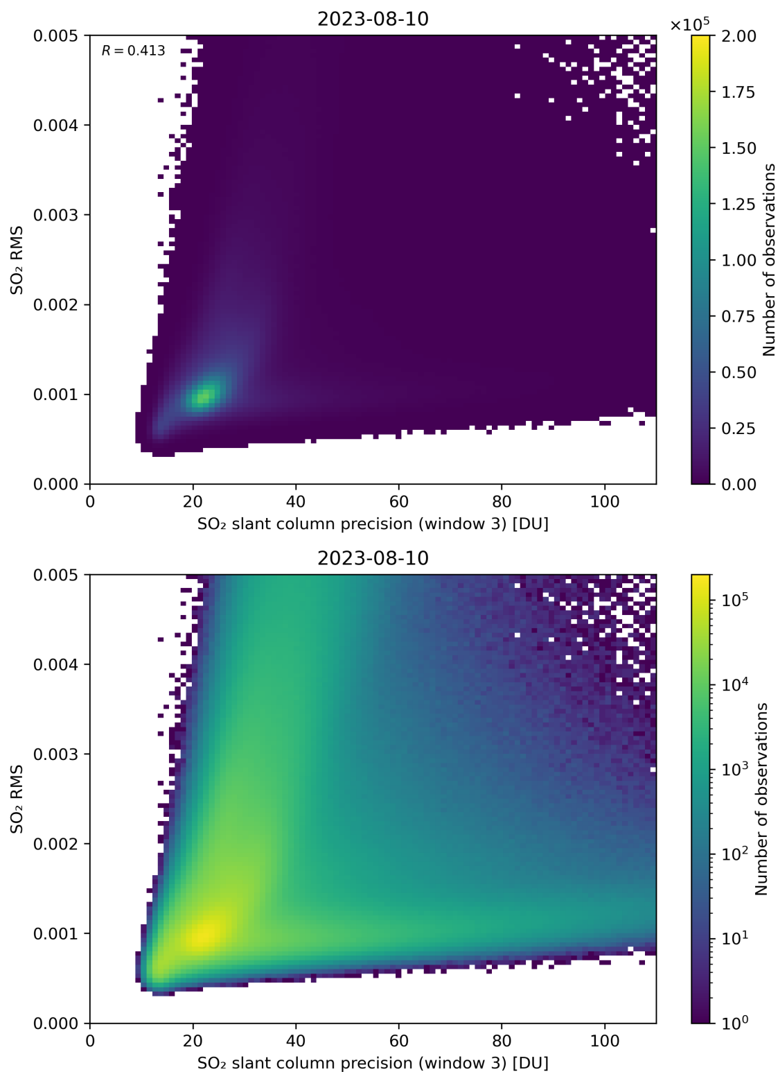
Figure 260: Scatter density plot of “SO 2 slant column precision (window 3)” against “SO 2 RMS” for 2023-08-09 to 2023-08-11.
