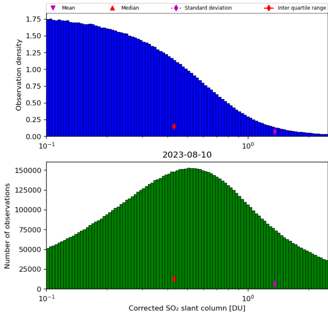
Figure 55: Histogram of “Corrected SO 2 slant column” for 2023-08-09 to 2023-08-11
