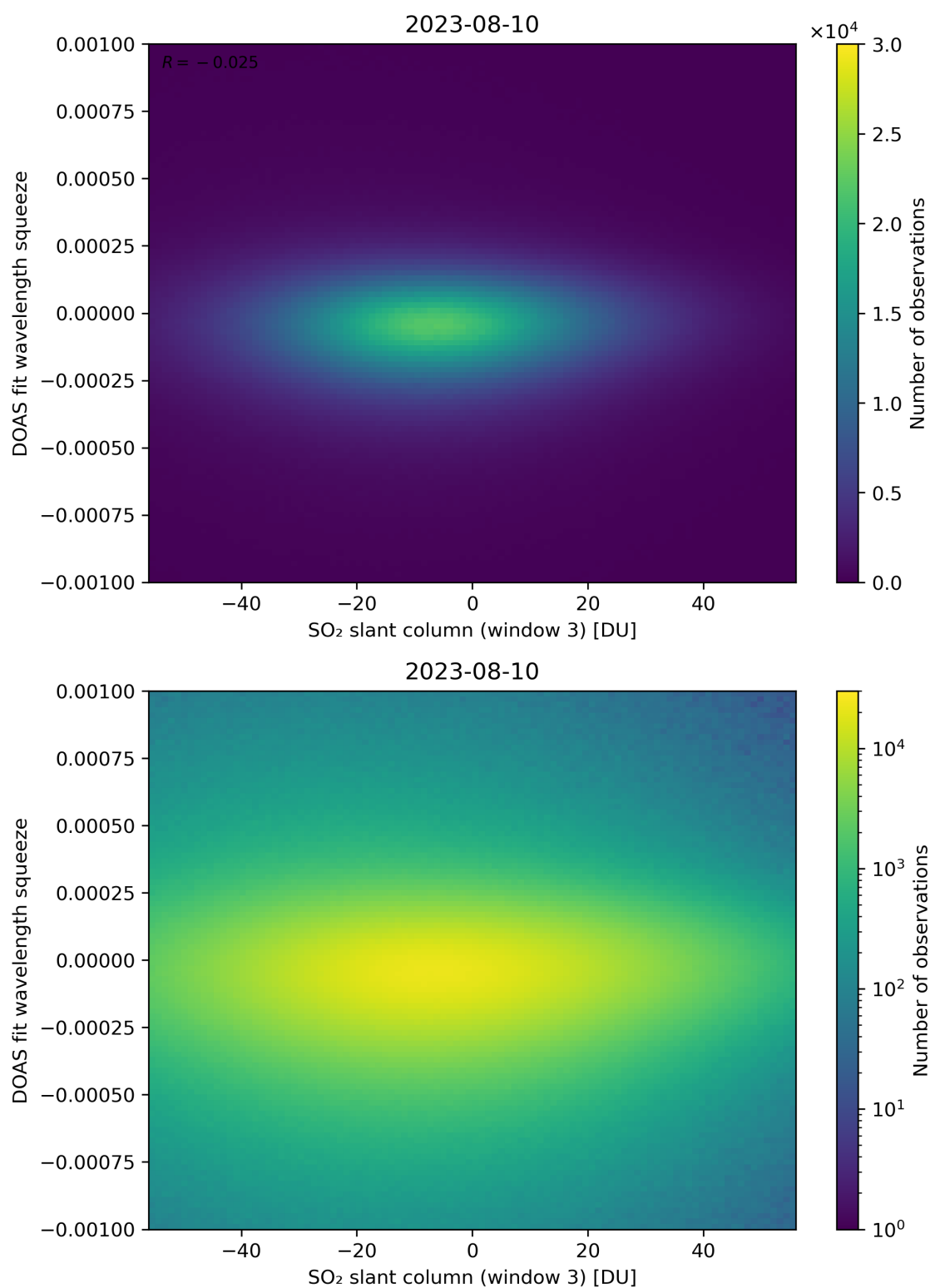
Figure 255: Scatter density plot of “SO 2 slant column (window 3)” against “DOAS fit wavelength squeeze” for 2023-08-09 to 2023-08-11.
