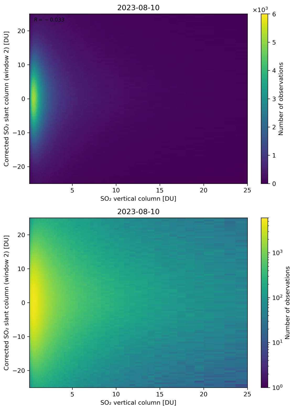
Figure 298: Scatter density plot of “SO 2 vertical column” against “Corrected SO 2 slant column (window 2)” for 2023-08-09 to 2023-08-11.
