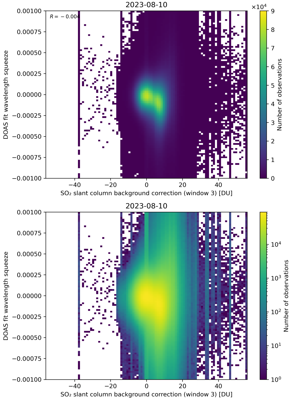
Figure 122: Scatter density plot of “SO 2 slant column background correction (window 3)” against “DOAS fit wavelength squeeze” for 2023-08-09 to 2023-08-11.
