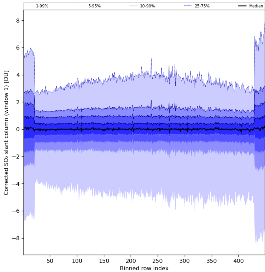
Figure 81: Along track statistics of “Corrected SO 2 slant column (window 1)” for 2023-08-09 to 2023-08-11
