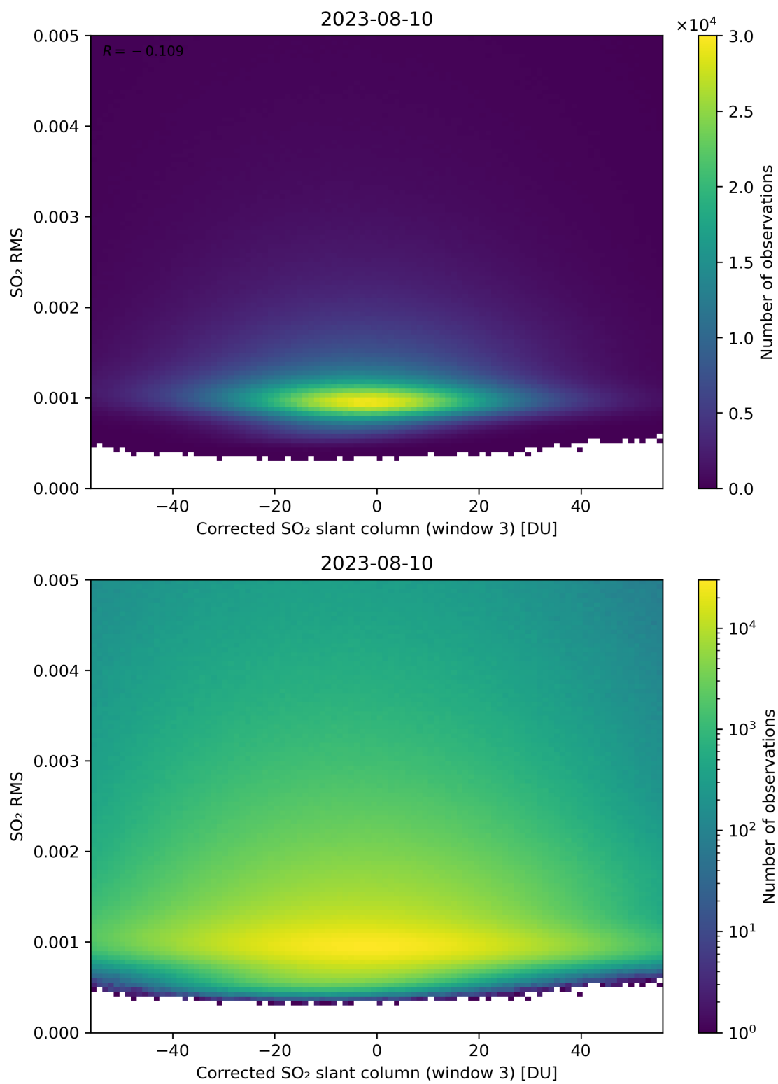
Figure 208: Scatter density plot of “Corrected SO 2 slant column (window 3)” against “SO 2 RMS” for 2023-08-09 to 2023-08-11.
