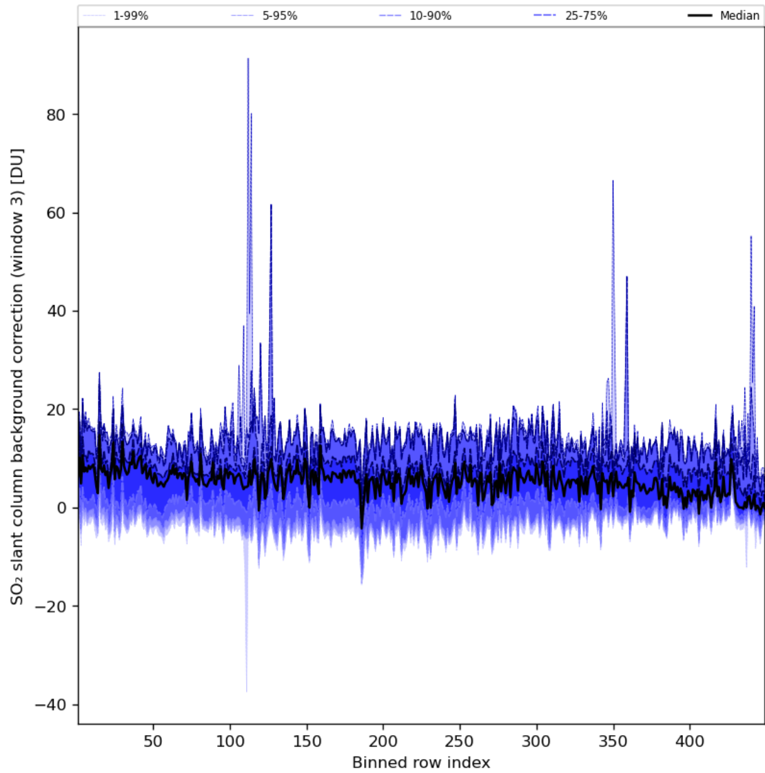
Figure 90: Along track statistics of “SO 2 slant column background correction (window 3)” for 2023-08-09 to 2023-08-11
