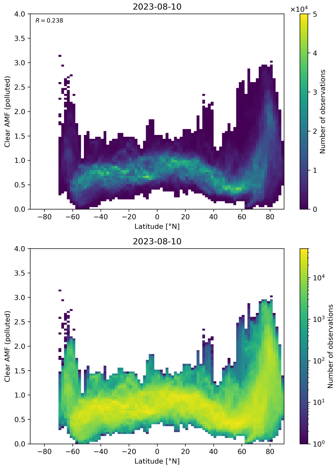
Figure 145: Scatter density plot of “Latitude” against “Clear AMF (polluted)” for 2023-08-09 to 2023-08-11.
