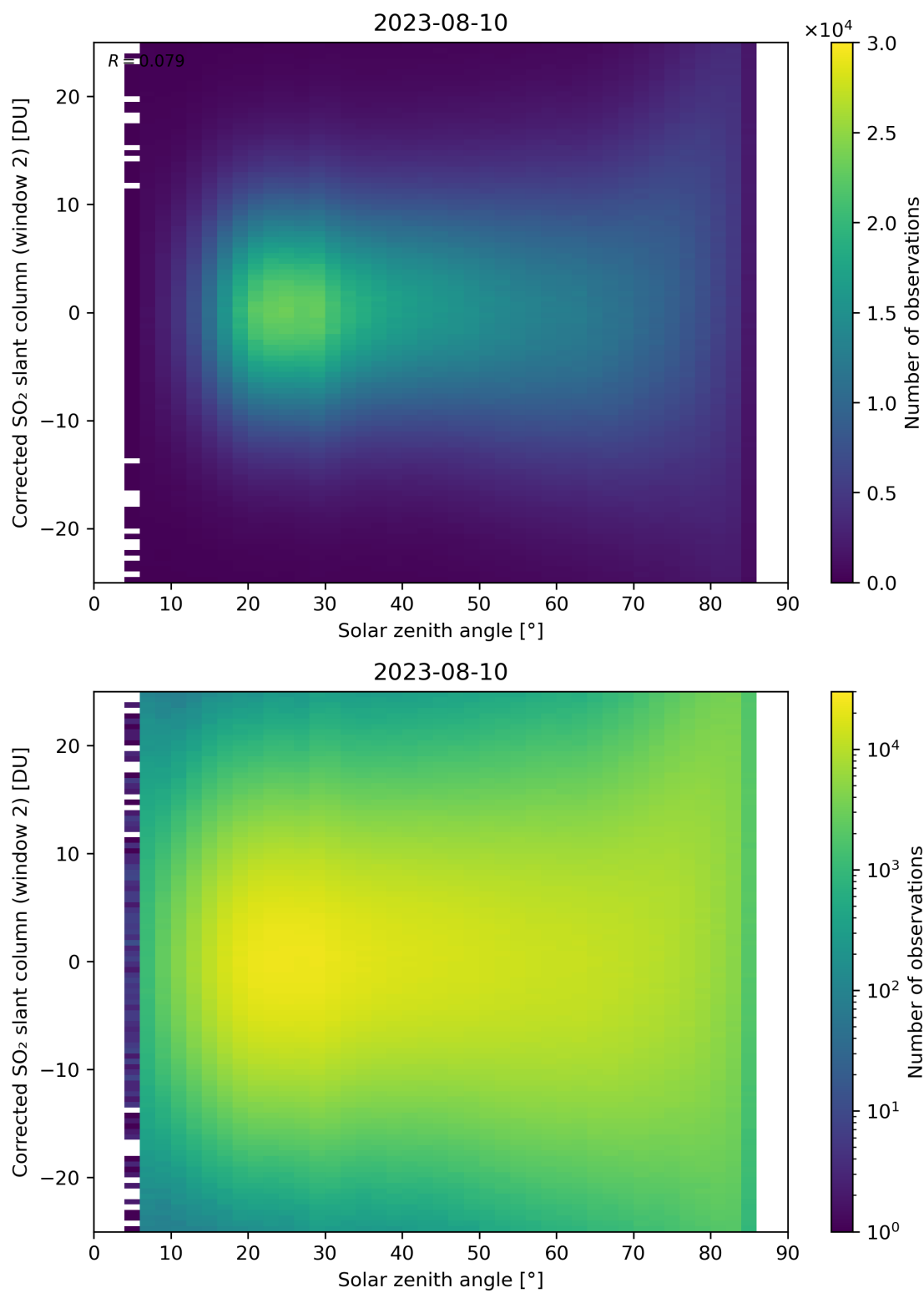
Figure 167: Scatter density plot of “Solar zenith angle” against “Corrected SO 2 slant column (window 2)” for 2023-08-09 to 2023-08-11.
