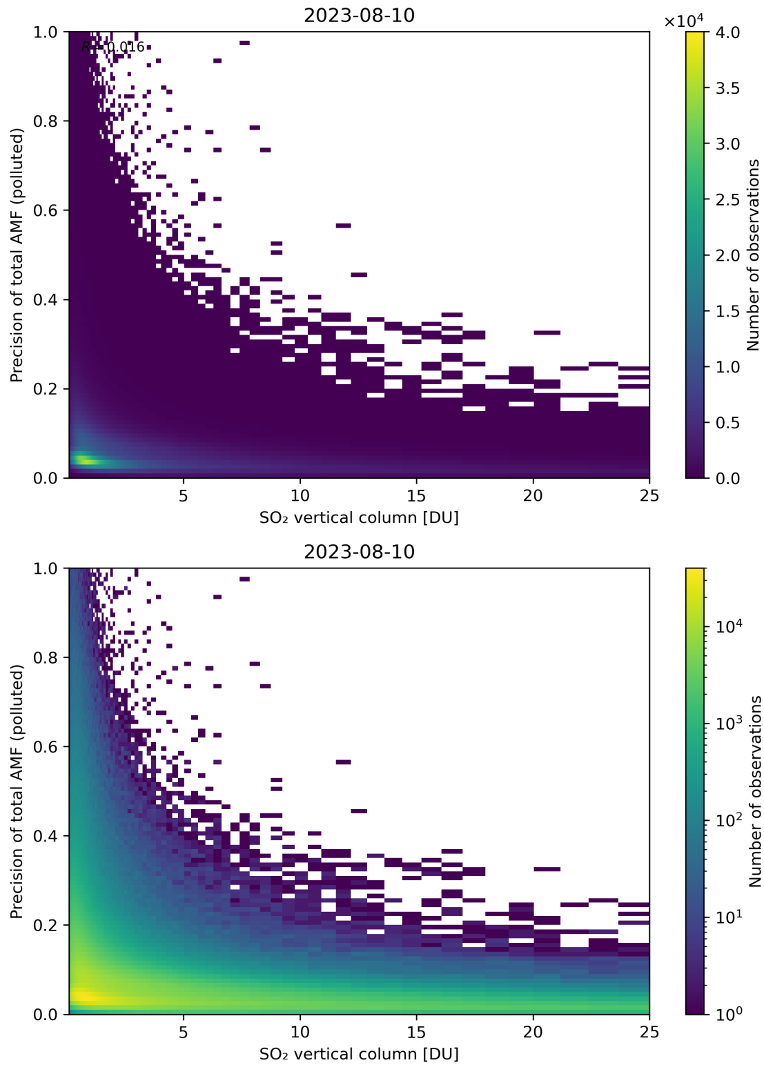
Figure 306: Scatter density plot of “SO 2 vertical column” against “Precision of total AMF (polluted)” for 2023-08-09 to 2023-08-11.
