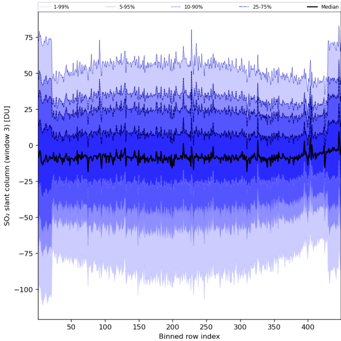
Figure 87: Along track statistics of "SO 2 slant column (window 3)" for 2023-08-09 to 2023-08-11
