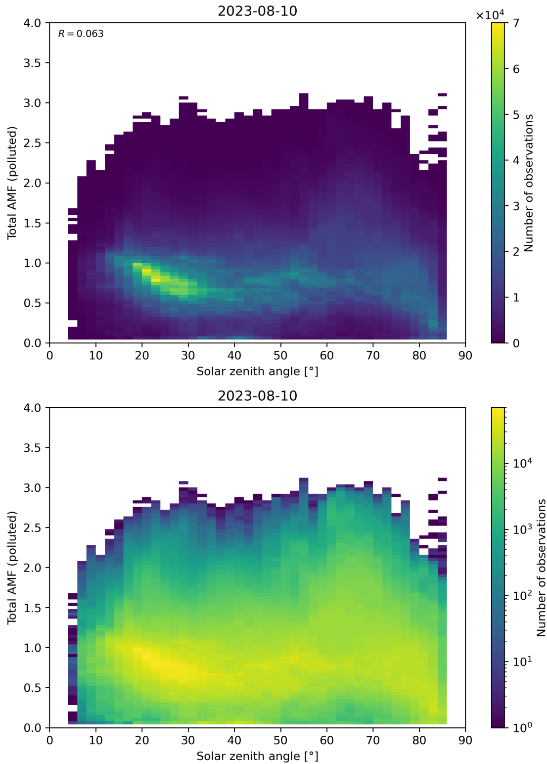
Figure 174: Scatter density plot of “Solar zenith angle” against “Total AMF (polluted)” for 2023-08-09 to 2023-08-11.
