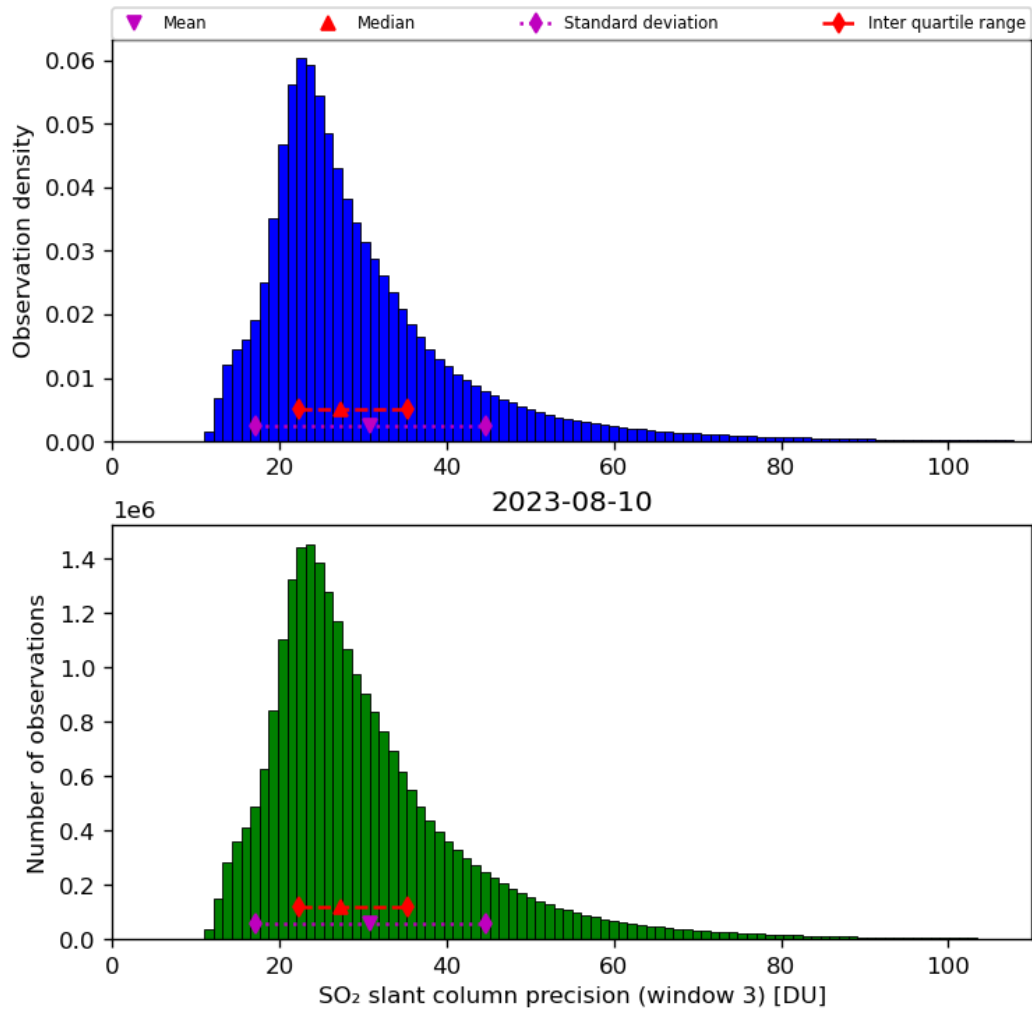
Figure 65: Histogram of “SO 2 slant column precision (window 3)” for 2023-08-09 to 2023-08-11
