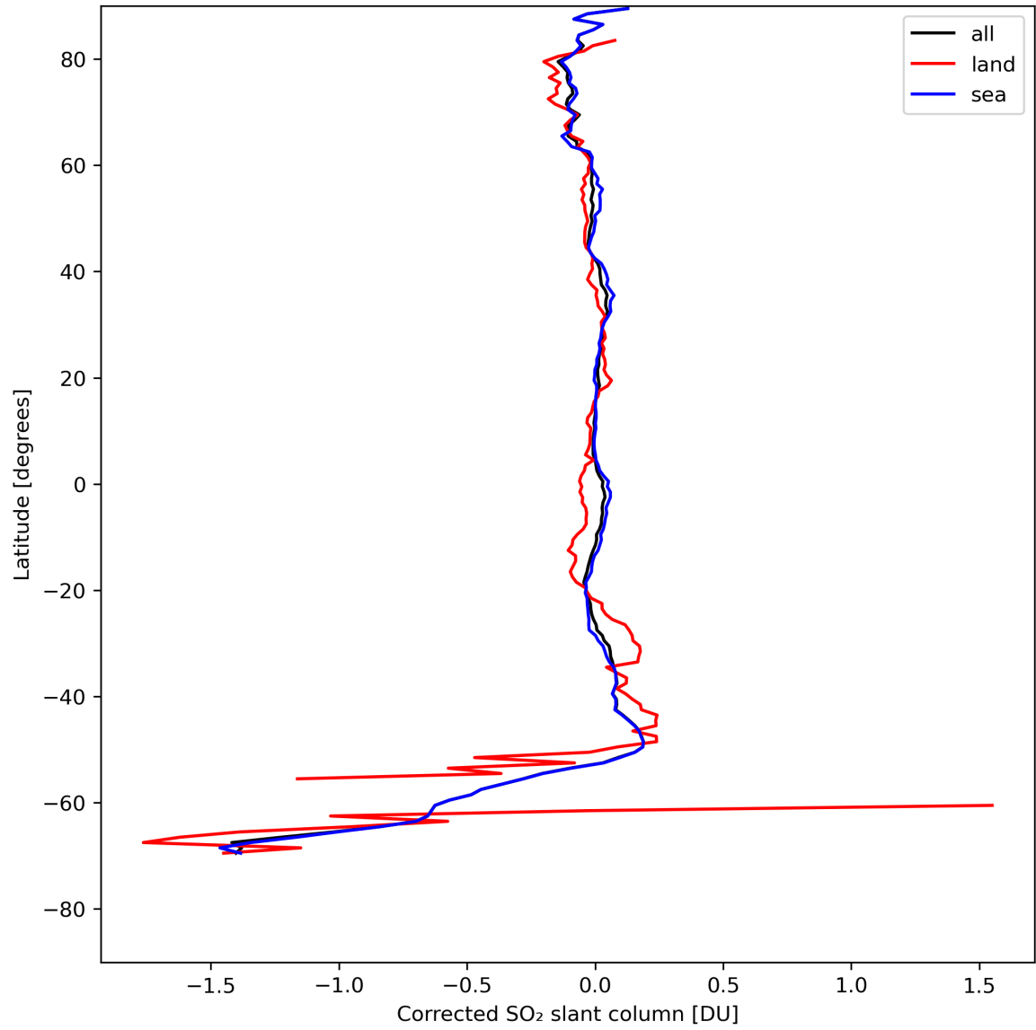
Figure 32: Zonal average of “Corrected SO 2 slant column” for 2023-08-09 to 2023-08-11.
