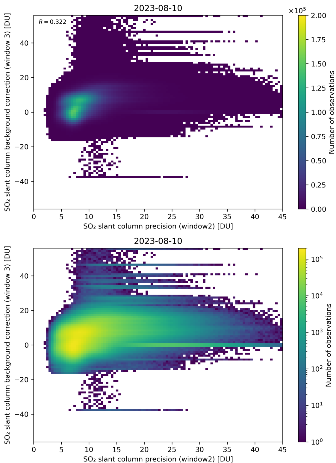
Figure 242: Scatter density plot of “SO 2 slant column precision (window2)” against “SO 2 slant column background correction (window 3)” for 2023-08-09 to 2023-08-11.
