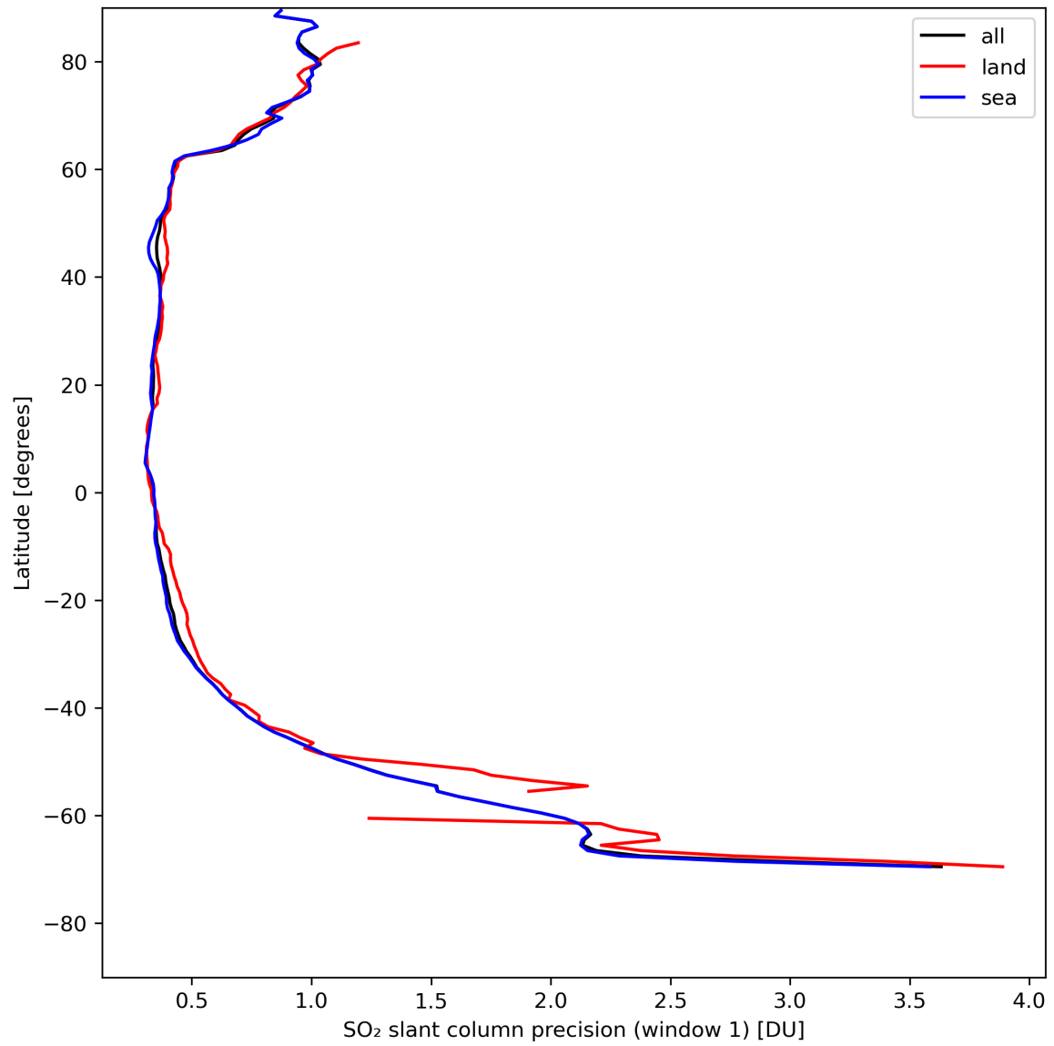
Figure 34: Zonal average of “SO 2 slant column precision (window 1)” for 2023-08-09 to 2023-08-11.
