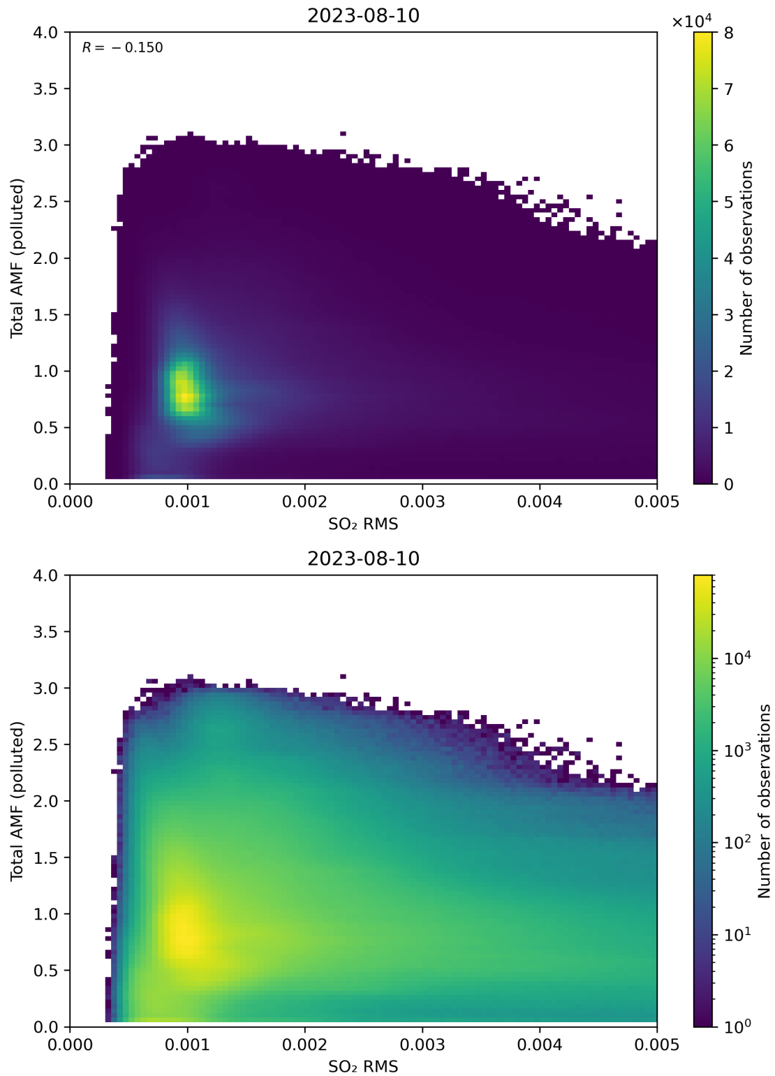
Figure 137: Scatter density plot of “SO 2 RMS” against “Total AMF (polluted)” for 2023-08-09 to 2023-08-11.
