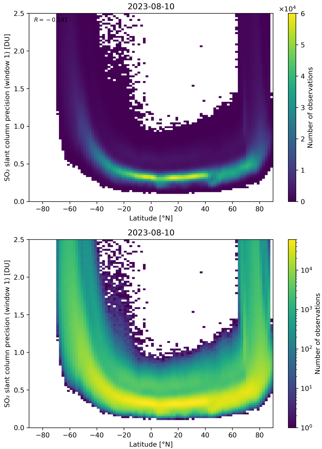
Figure 150: Scatter density plot of “Latitude” against “SO 2 slant column precision (window 1)” for 2023-08-09 to 2023-08-11.
