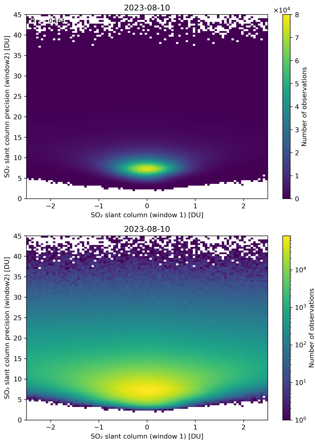
Figure 236: Scatter density plot of “SO 2 slant column (window 1)” against “SO 2 slant column precision (window2)” for 2023-08-09 to 2023-08-11.
