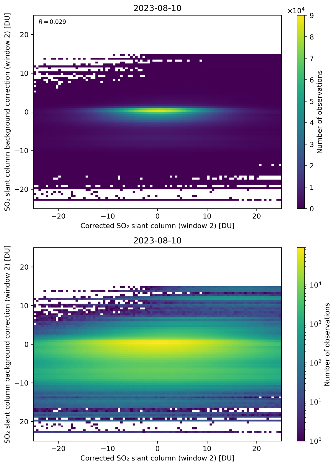
Figure 194: Scatter density plot of “Corrected SO 2 slant column (window 2)” against “SO 2 slant column background correction (window 2)” for 2023-08-09 to 2023-08-11.
