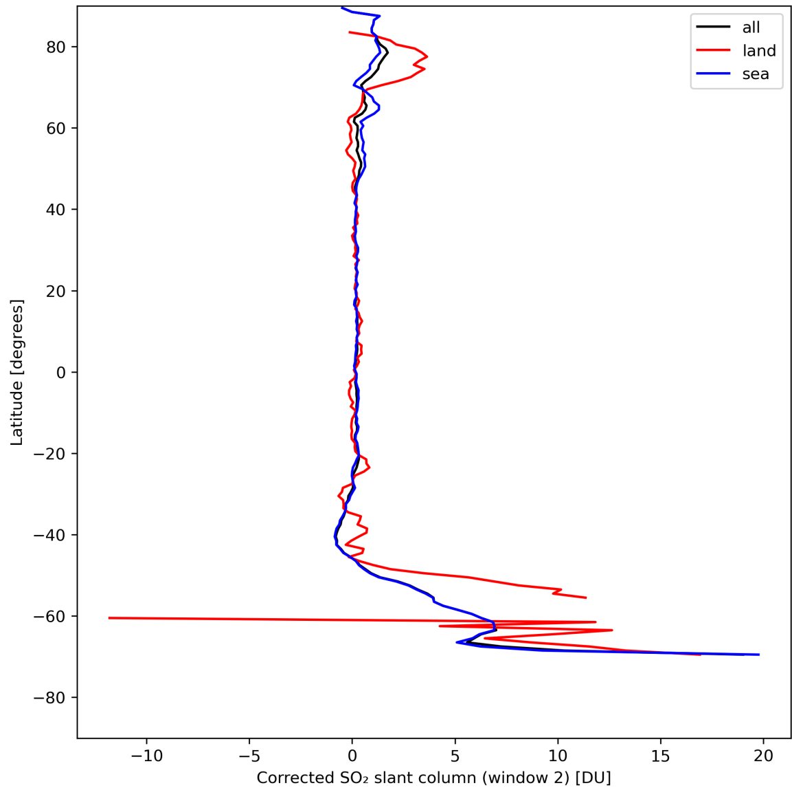
Figure 39: Zonal average of “Corrected SO 2 slant column (window 2)” for 2023-08-09 to 2023-08-11.
