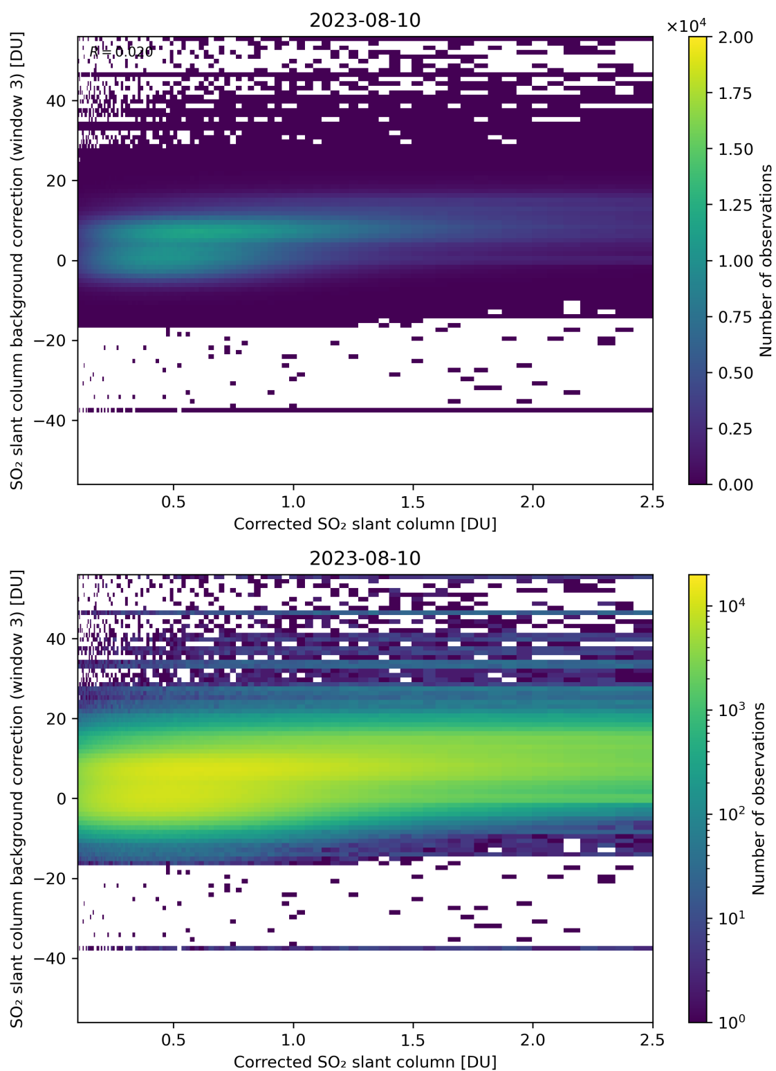
Figure 180: Scatter density plot of “Corrected SO 2 slant column” against “SO 2 slant column background correction (window 3)” for 2023-08-09 to 2023-08-11.
