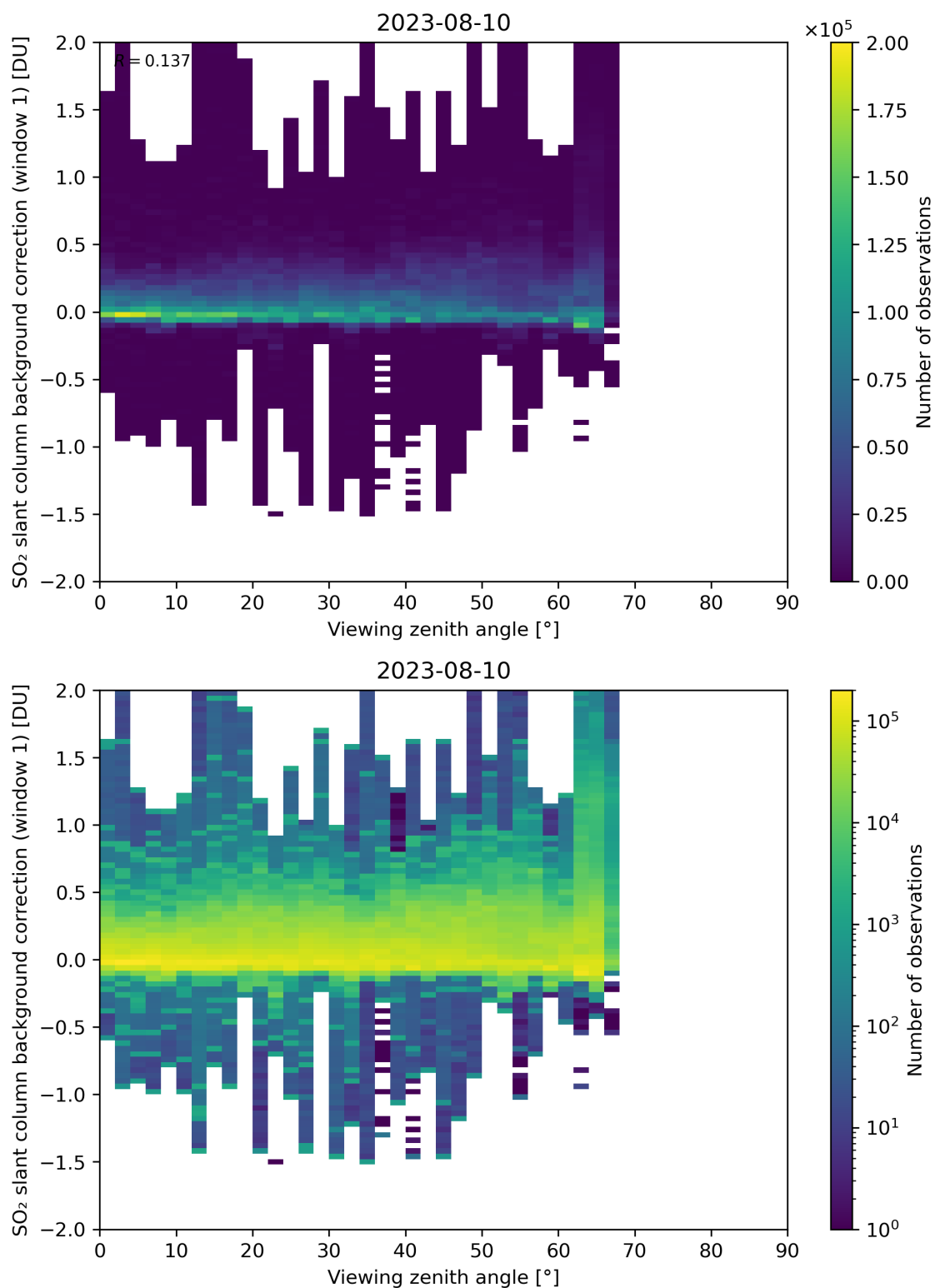
Figure 308: Scatter density plot of “Viewing zenith angle” against “SO 2 slant column background correction (window 1)” for 2023-08-09 to 2023-08-11.
