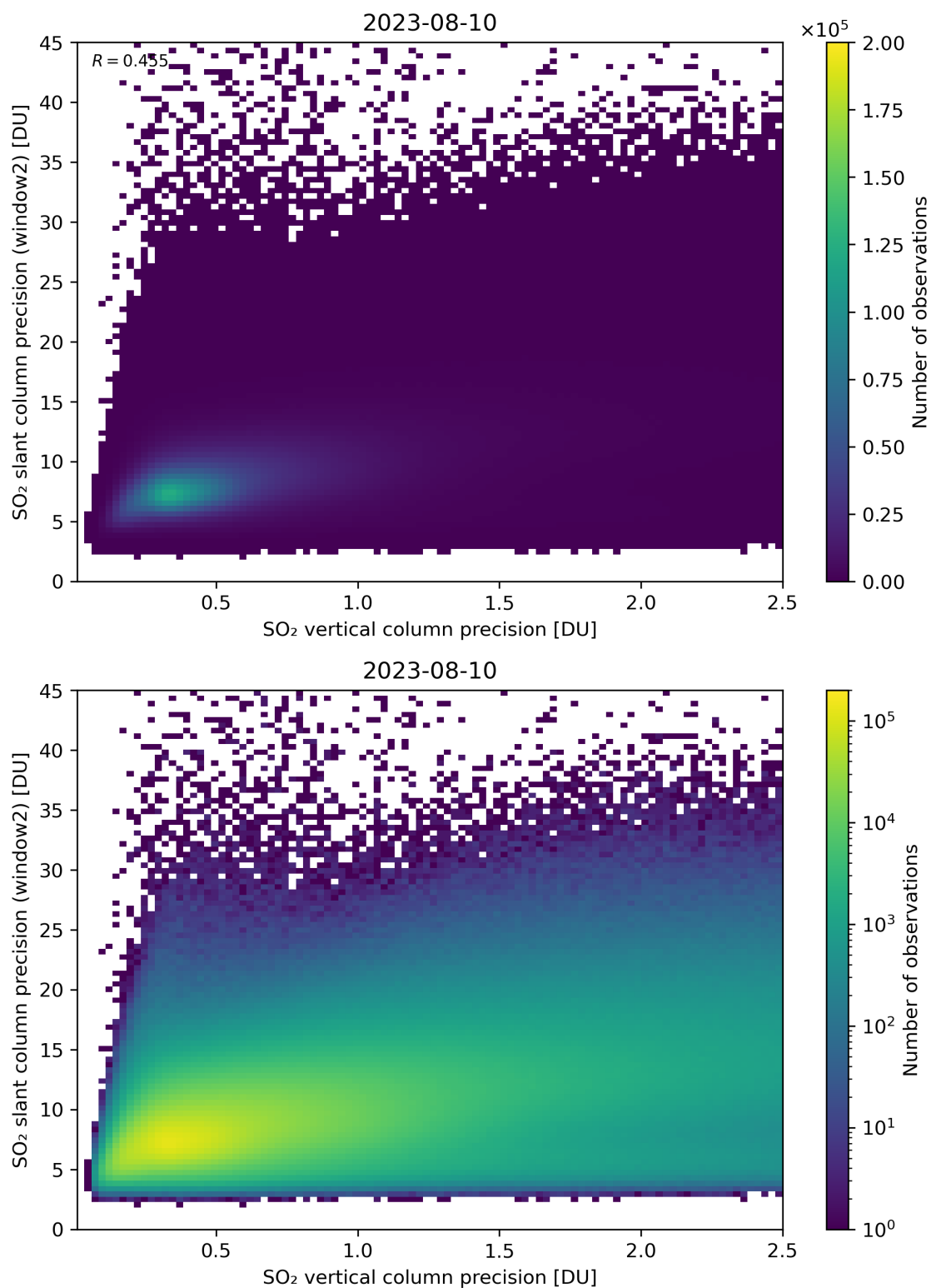
Figure 291: Scatter density plot of “SO 2 vertical column precision” against “SO 2 slant column precision (window2)” for 2023-08-09 to 2023-08-11.
