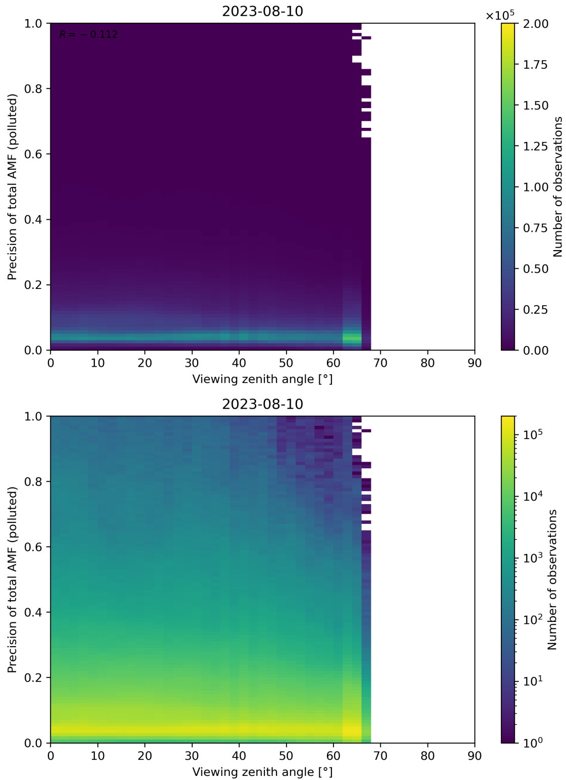
Figure 326: Scatter density plot of “Viewing zenith angle” against “Precision of total AMF (polluted)” for 2023-08-09 to 2023-08-11.
