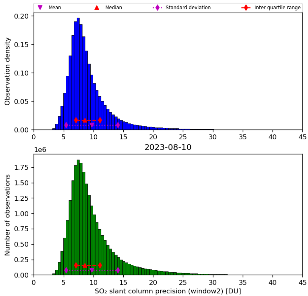
Figure 61: Histogram of “SO 2 slant column precision (window2)” for 2023-08-09 to 2023-08-11
