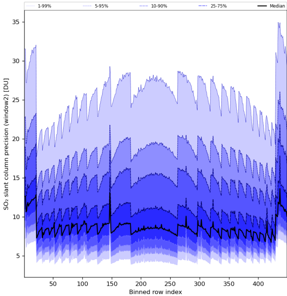
Figure 84: Along track statistics of “SO 2 slant column precision (window2)” for 2023-08-09 to 2023-08-11
