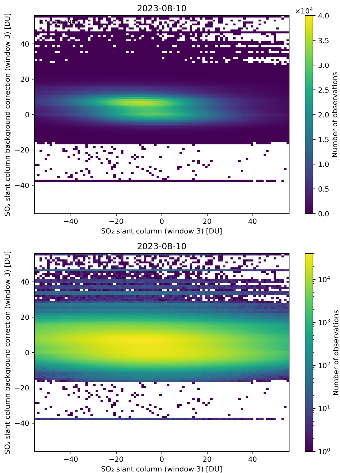
Figure 253: Scatter density plot of “SO 2 slant column (window 3)” against “SO 2 slant column background correction (window 3)” for 2023-08-09 to 2023-08-11.
