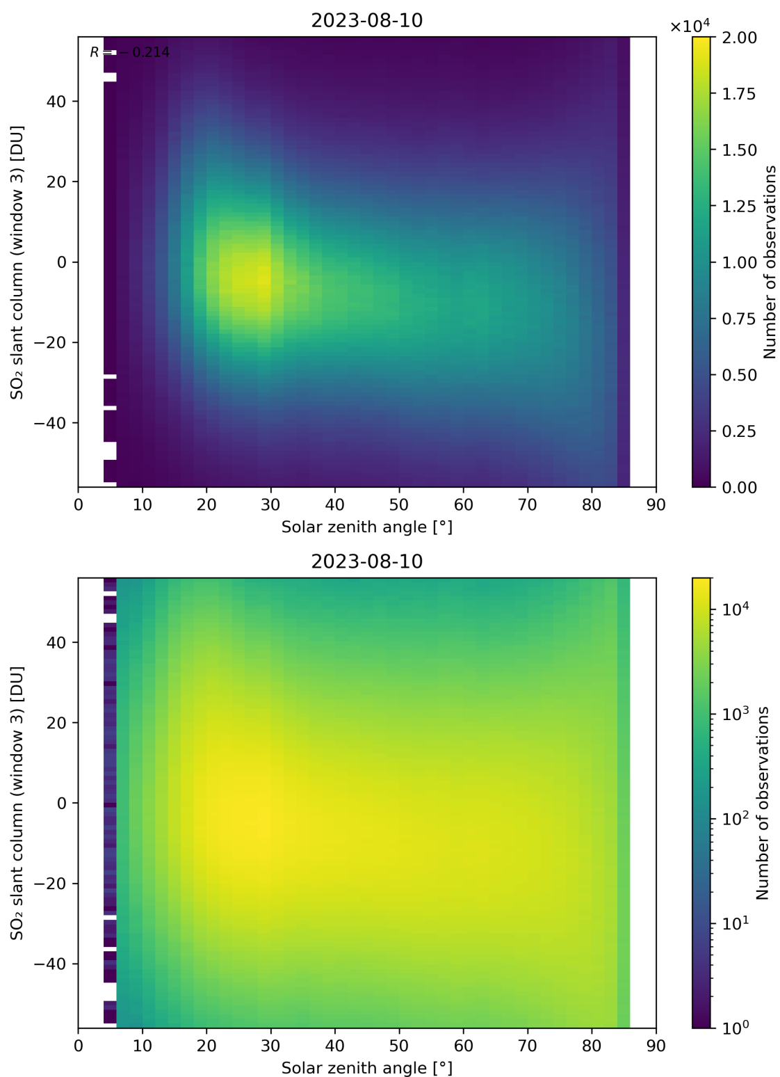
Figure 172: Scatter density plot of “Solar zenith angle” against “SO 2 slant column (window 3)” for 2023-08-09 to 2023-08-11.
