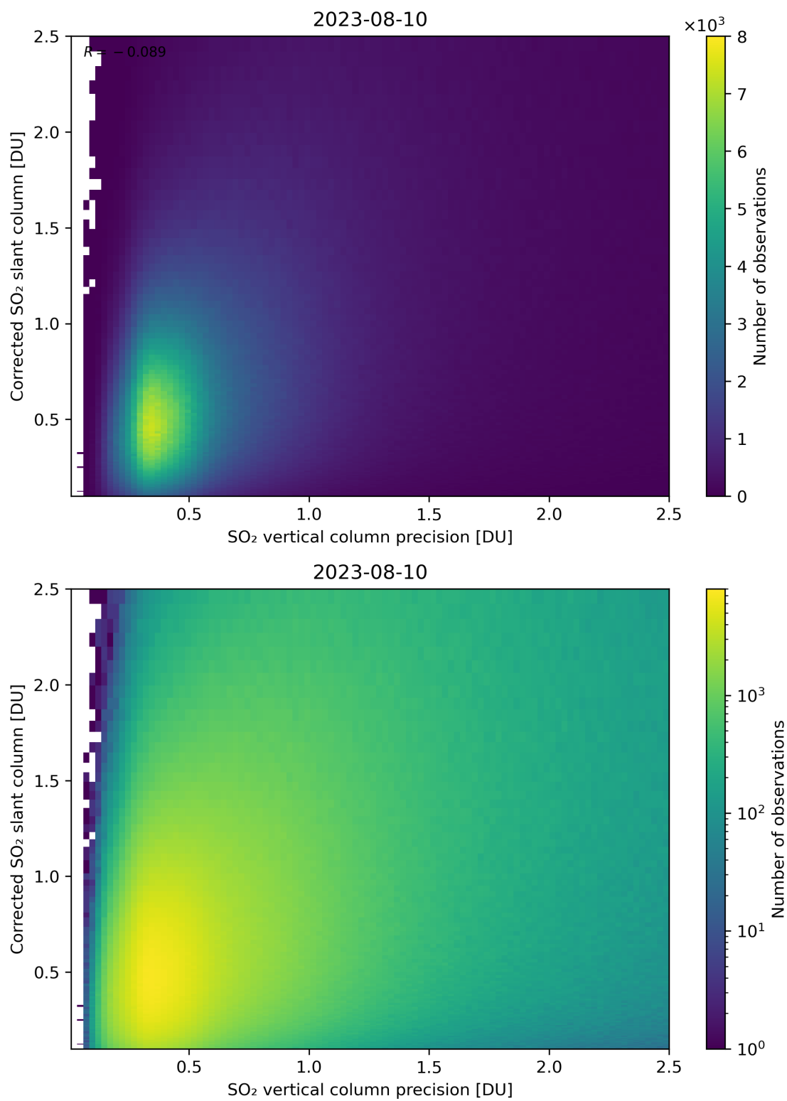
Figure 286: Scatter density plot of “SO 2 vertical column precision” against “Corrected SO 2 slant column” for 2023-08-09 to 2023-08-11.
