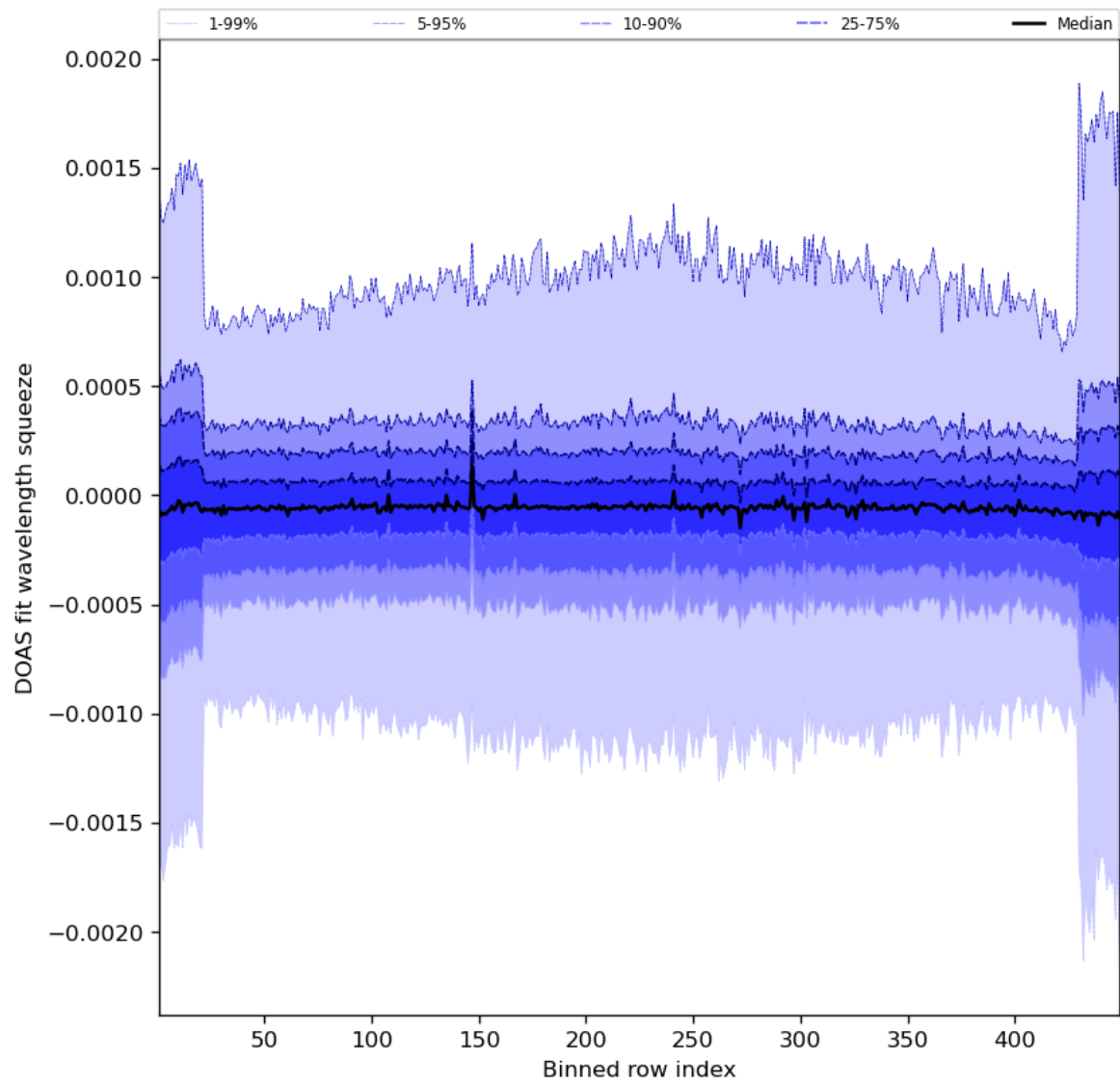
Figure 92: Along track statistics of “DOAS fit wavelength squeeze” for 2023-08-09 to 2023-08-11
