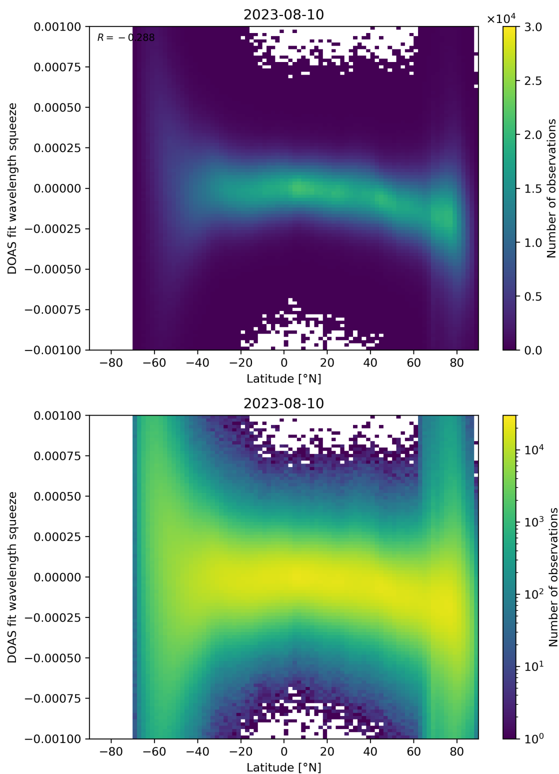
Figure 143: Scatter density plot of “Latitude” against “DOAS fit wavelength squeeze” for 2023-08-09 to 2023-08-11.
