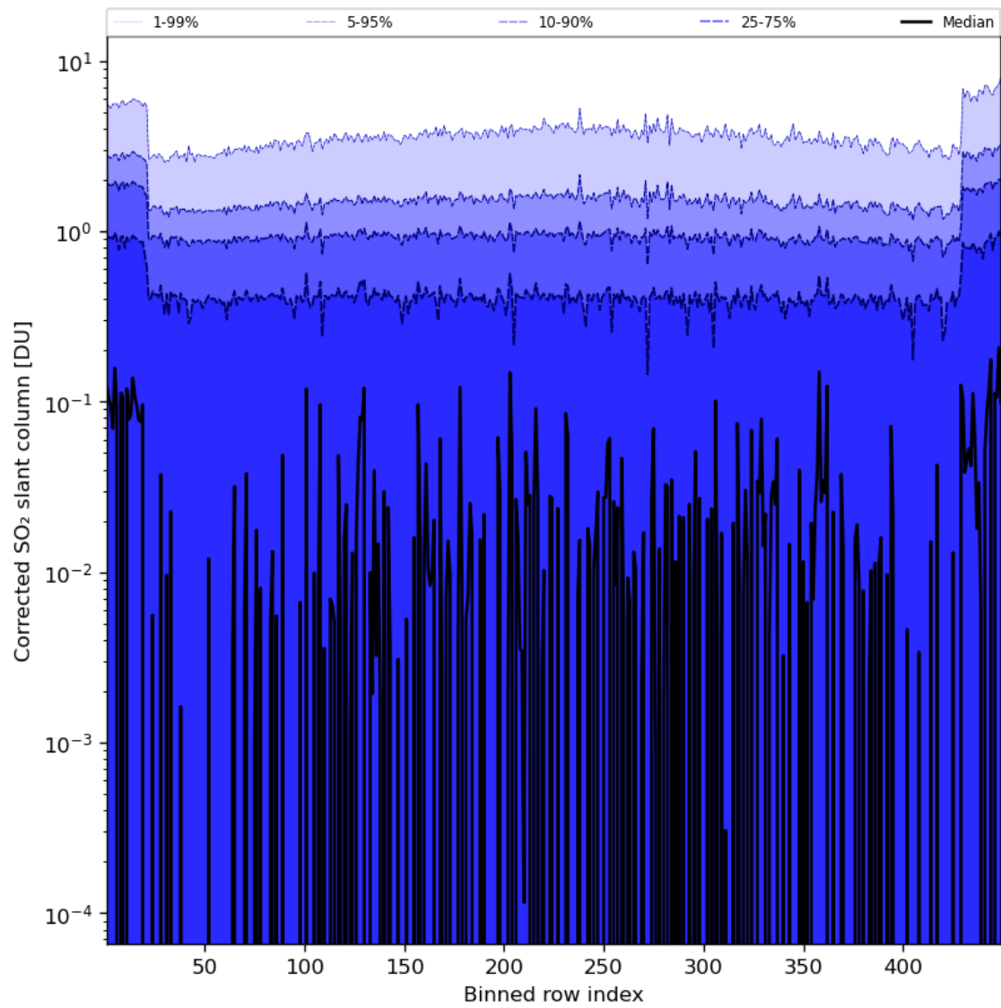
Figure 78: Along track statistics of “Corrected SO 2 slant column” for 2023-08-09 to 2023-08-11
