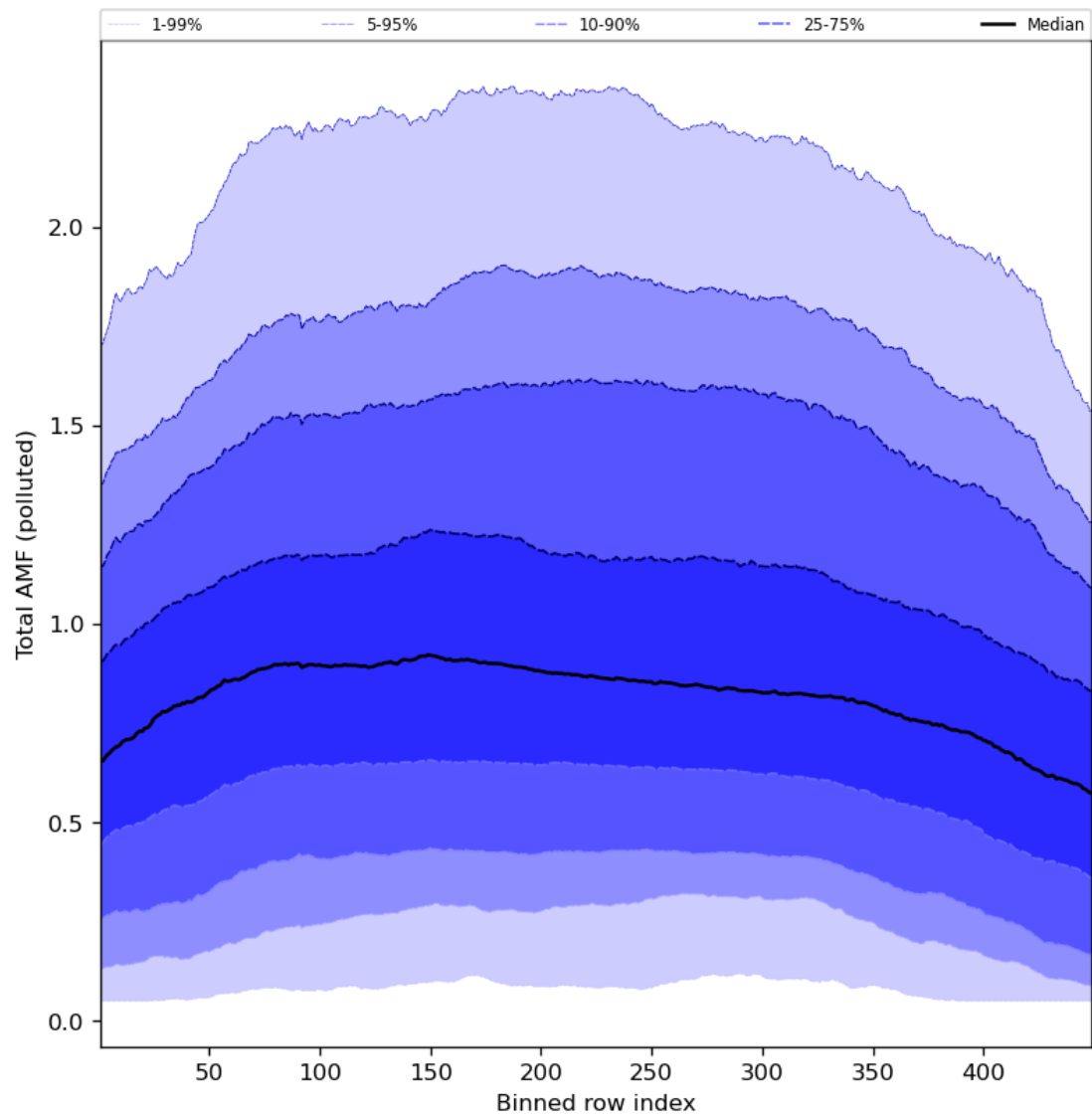
Figure 94: Along track statistics of “Total AMF (polluted)” for 2023-08-09 to 2023-08-11
