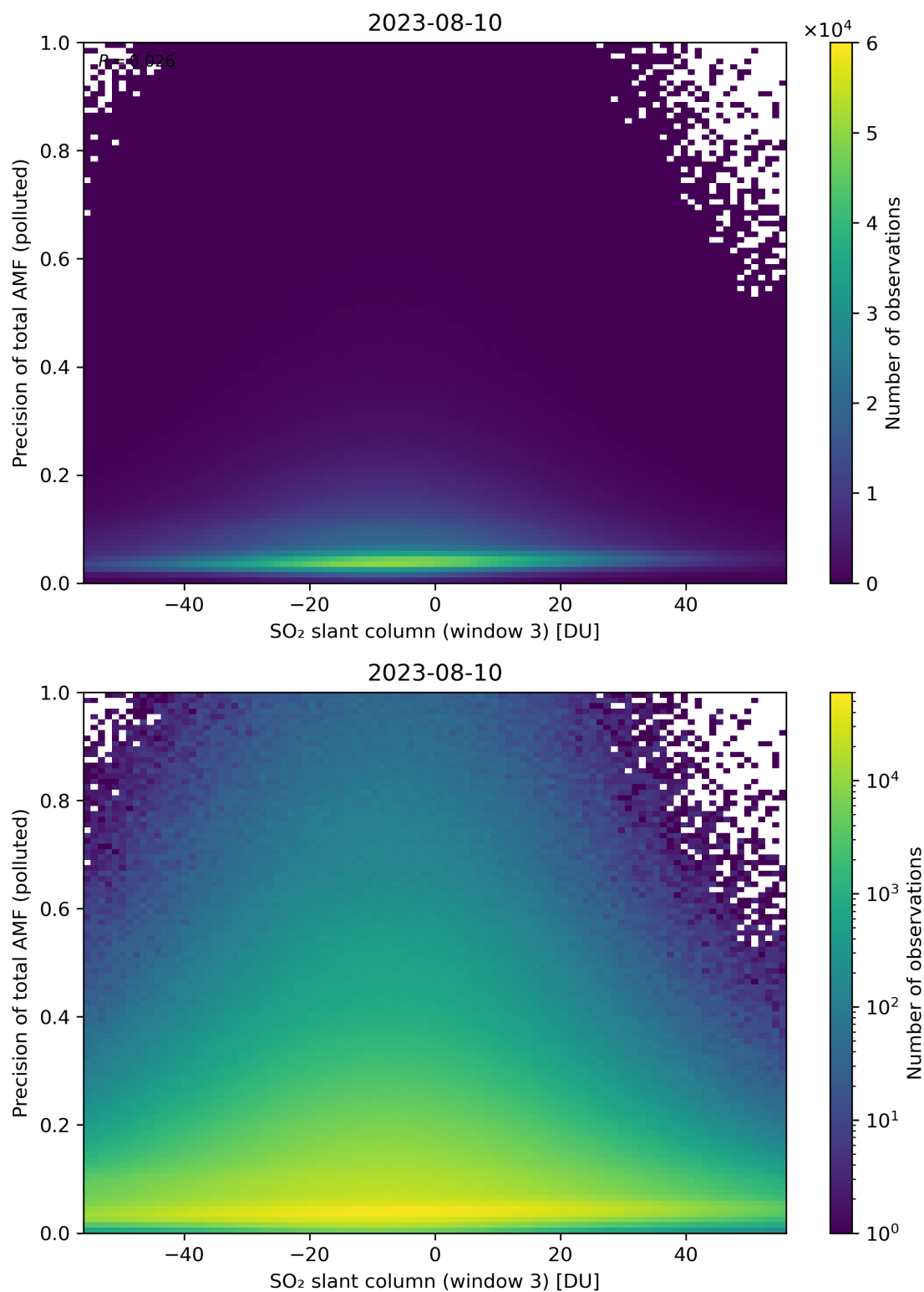
Figure 269: Scatter density plot of “SO 2 slant column (window 3)” against “Precision of total AMF (polluted)” for 2023-08-09 to 2023-08-11.
