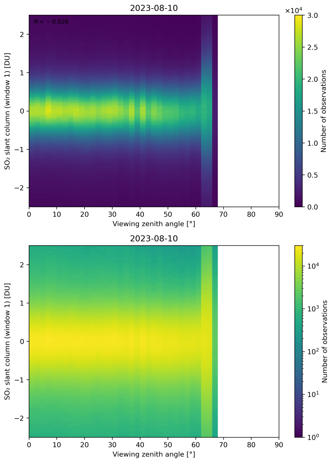
Figure 320: Scatter density plot of “Viewing zenith angle” against “SO 2 slant column (window 1)” for 2023-08-09 to 2023-08-11.
