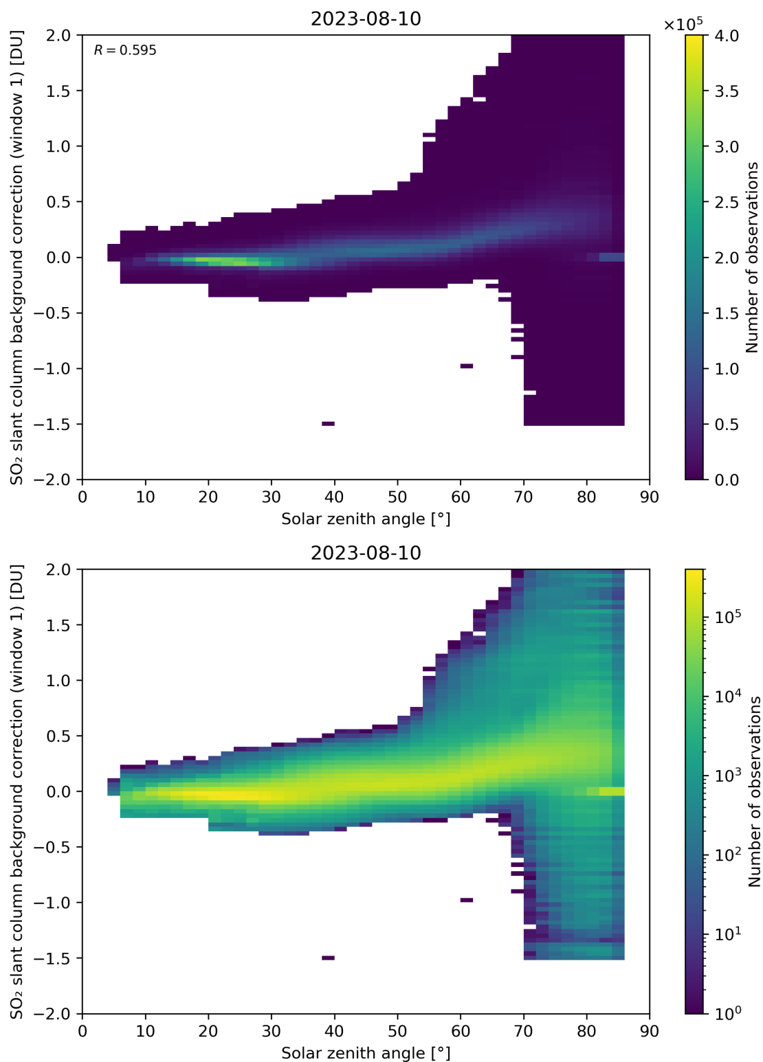
Figure 158: Scatter density plot of “Solar zenith angle” against “SO 2 slant column background correction (window 1)” for 2023-08-09 to 2023-08-11.
