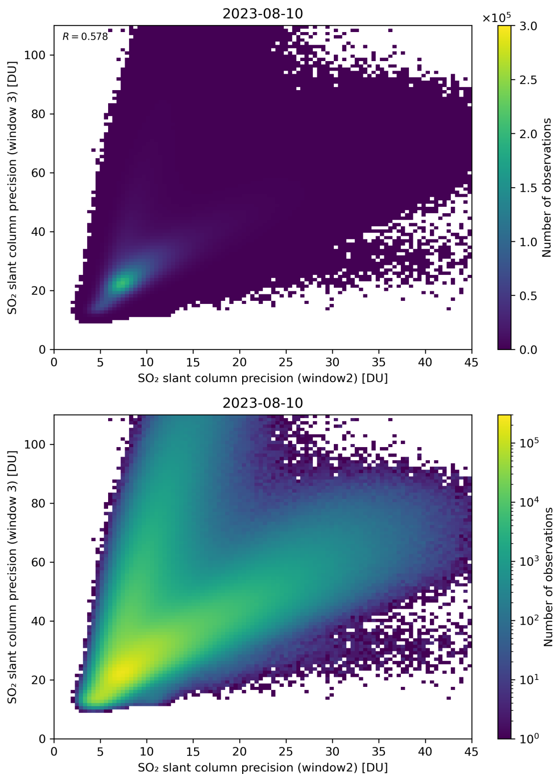
Figure 250: Scatter density plot of “SO 2 slant column precision (window2)” against “SO 2 slant column precision (window 3)” for 2023-08-09 to 2023-08-11.
