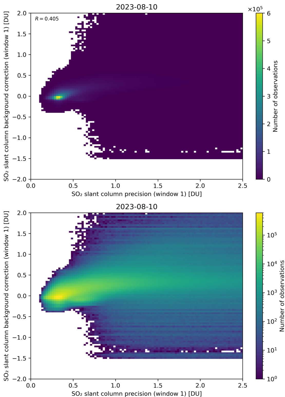
Figure 218: Scatter density plot of “SO 2 slant column precision (window 1)” against “SO 2 slant column background correction (window 1)” for 2023-08-09 to 2023-08-11.
