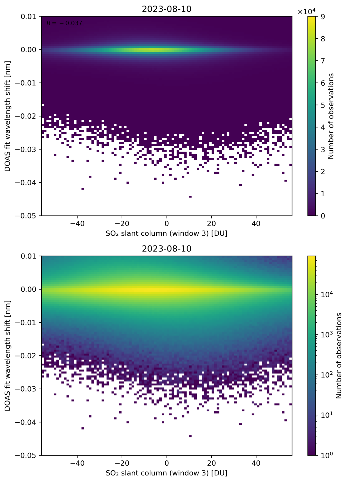
Figure 254: Scatter density plot of “SO 2 slant column (window 3)” against “DOAS fit wavelength shift” for 2023-08-09 to 2023-08-11.
