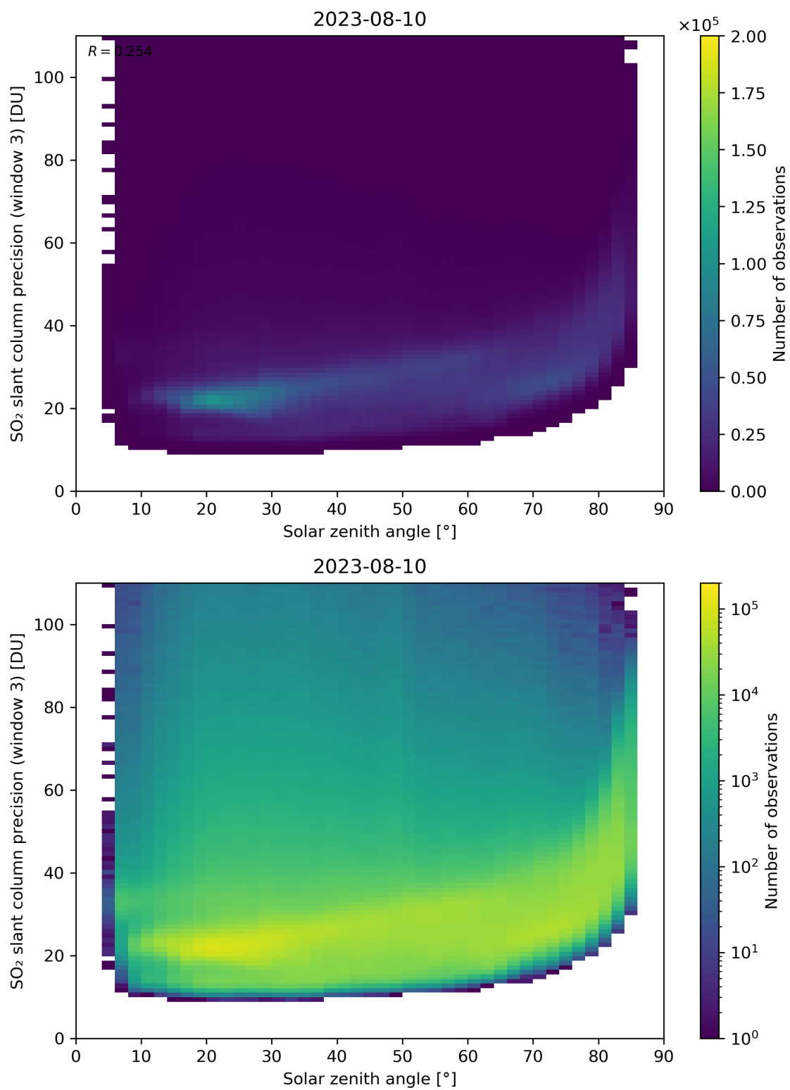
Figure 173: Scatter density plot of “Solar zenith angle” against “SO 2 slant column precision (window 3)” for 2023-08-09 to 2023-08-11.
