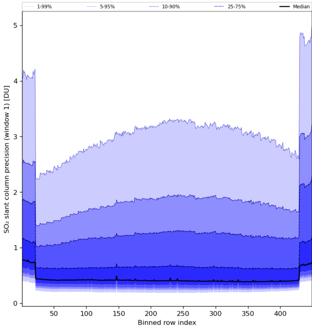
Figure 80: Along track statistics of “SO 2 slant column precision (window 1)” for 2023-08-09 to 2023-08-11
