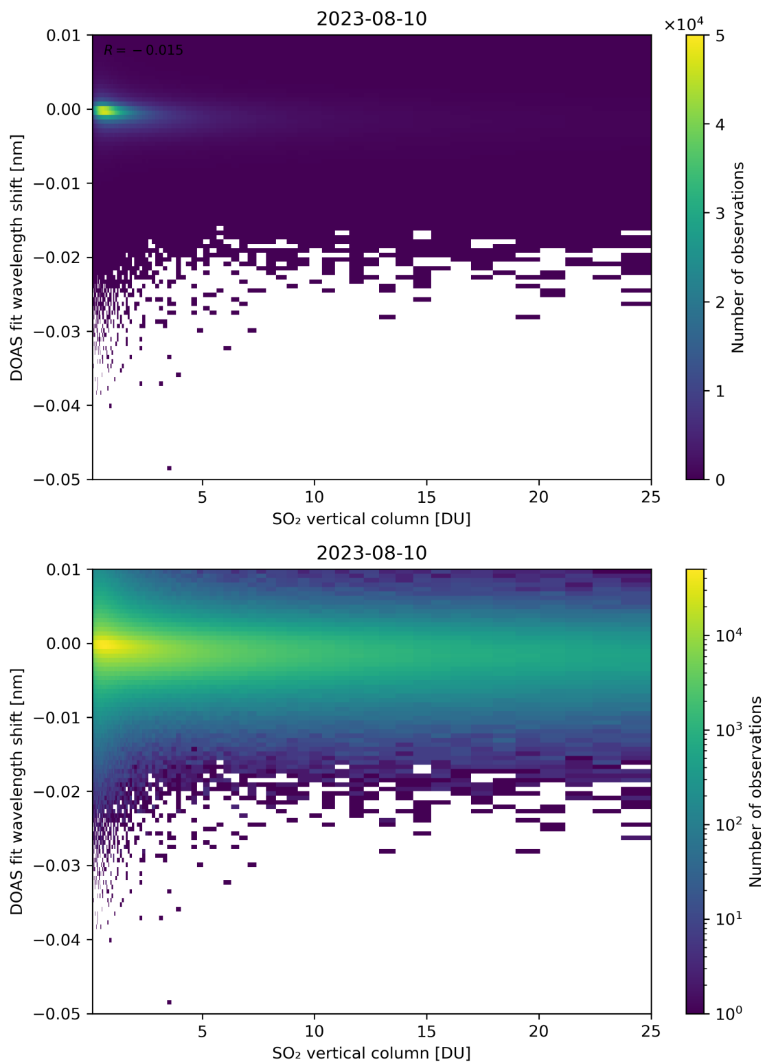
Figure 276: Scatter density plot of “SO 2 vertical column” against “DOAS fit wavelength shift” for 2023-08-09 to 2023-08-11.
