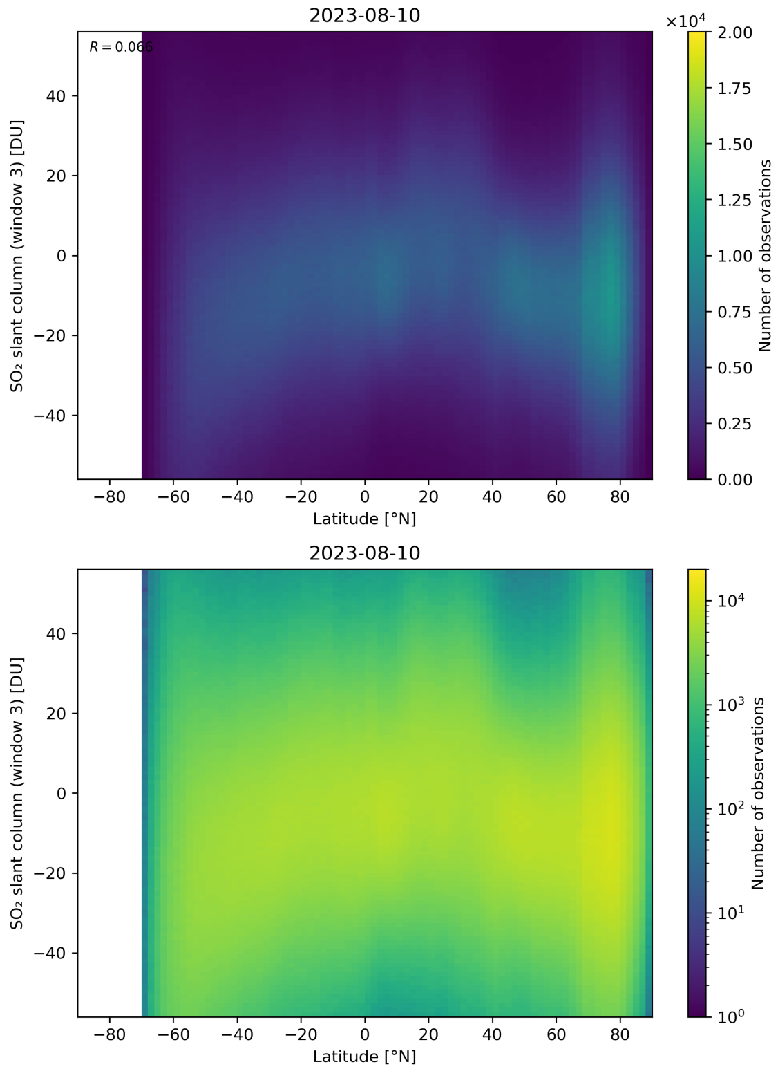
Figure 152: Scatter density plot of “Latitude” against “SO 2 slant column (window 3)” for 2023-08-09 to 2023-08-11.
