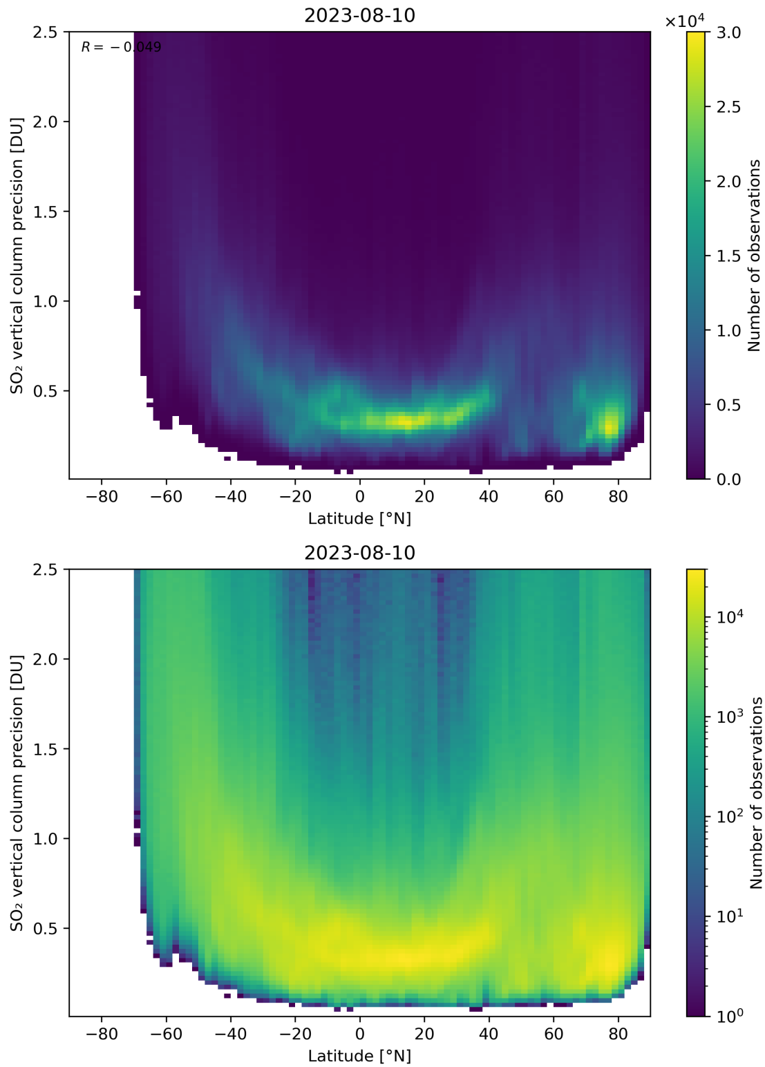
Figure 157: Scatter density plot of “Latitude” against “SO 2 vertical column precision” for 2023-08-09 to 2023-08-11.
