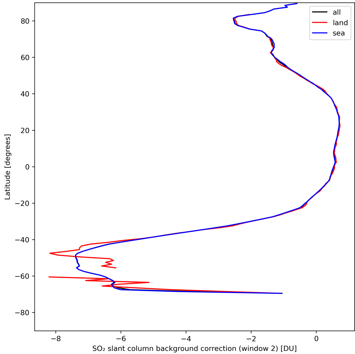
Figure 40: Zonal average of “SO 2 slant column background correction (window 2)” for 2023-08-09 to 2023-08-11.
