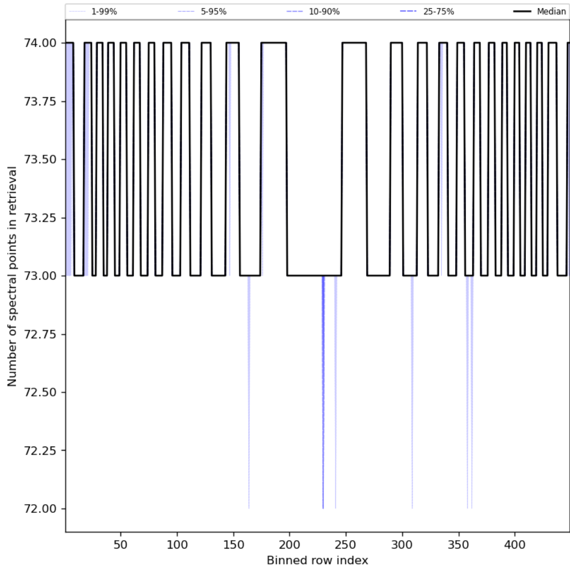
Figure 97: Along track statistics of “Number of spectral points in retrieval” for 2023-08-09 to 2023-08-11
