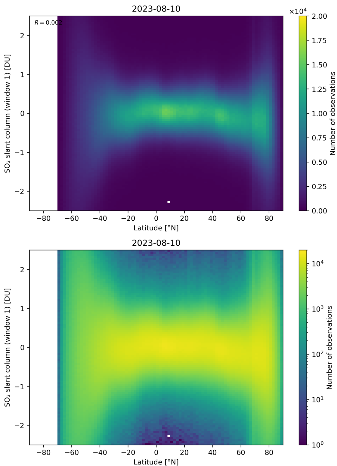
Figure 149: Scatter density plot of “Latitude” against “SO 2 slant column (window 1)” for 2023-08-09 to 2023-08-11.
