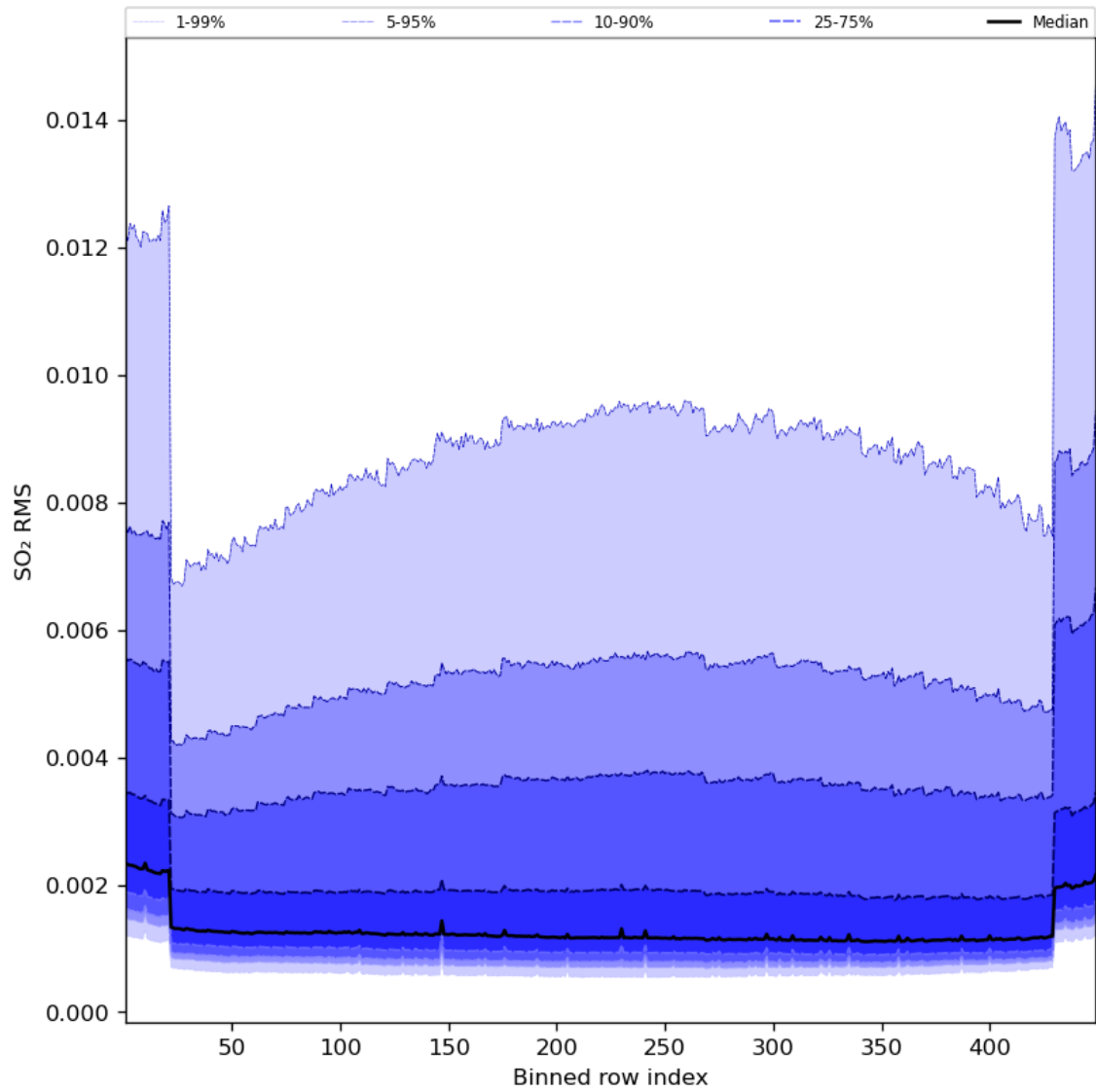
Figure 93: Along track statistics of “SO 2 RMS” for 2023-08-09 to 2023-08-11
