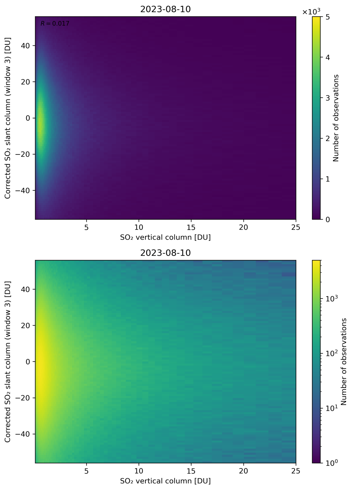
Figure 299: Scatter density plot of “SO 2 vertical column” against “Corrected SO 2 slant column (window 3)” for 2023-08-09 to 2023-08-11.
