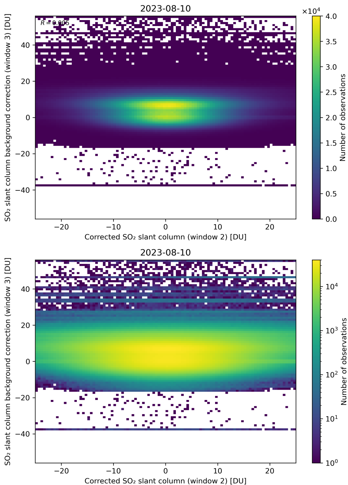
Figure 195: Scatter density plot of “Corrected SO 2 slant column (window 2)” against “SO 2 slant column background correction (window 3)” for 2023-08-09 to 2023-08-11.
