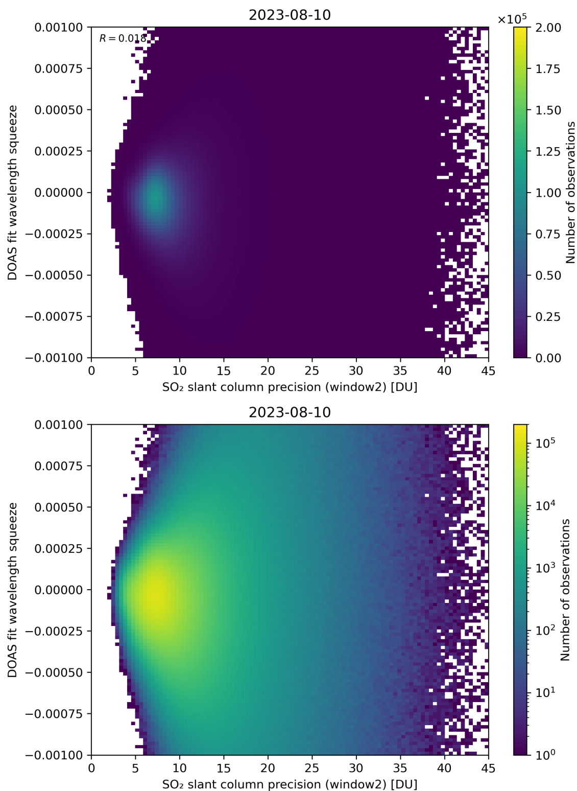
Figure 244: Scatter density plot of “SO 2 slant column precision (window2)” against “DOAS fit wavelength squeeze” for 2023-08-09 to 2023-08-11.
