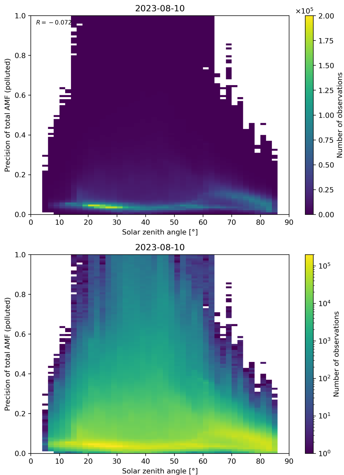
Figure 175: Scatter density plot of “Solar zenith angle” against “Precision of total AMF (polluted)” for 2023-08-09 to 2023-08-11.
