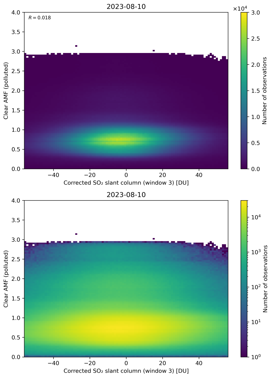
Figure 209: Scatter density plot of “Corrected SO 2 slant column (window 3)” against “Clear AMF (polluted)” for 2023-08-09 to 2023-08-11.
