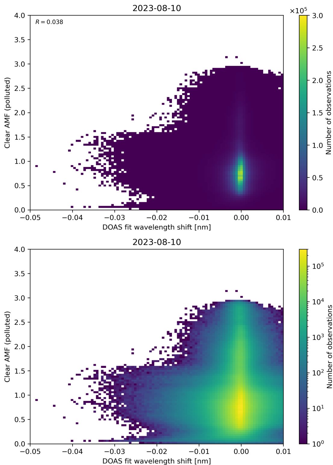
Figure 129: Scatter density plot of “DOAS fit wavelength shift” against “Clear AMF (polluted)” for 2023-08-09 to 2023-08-11.
