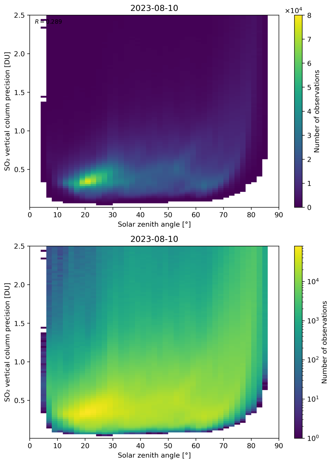
Figure 177: Scatter density plot of “Solar zenith angle” against “SO 2 vertical column precision” for 2023-08-09 to 2023-08-11.
