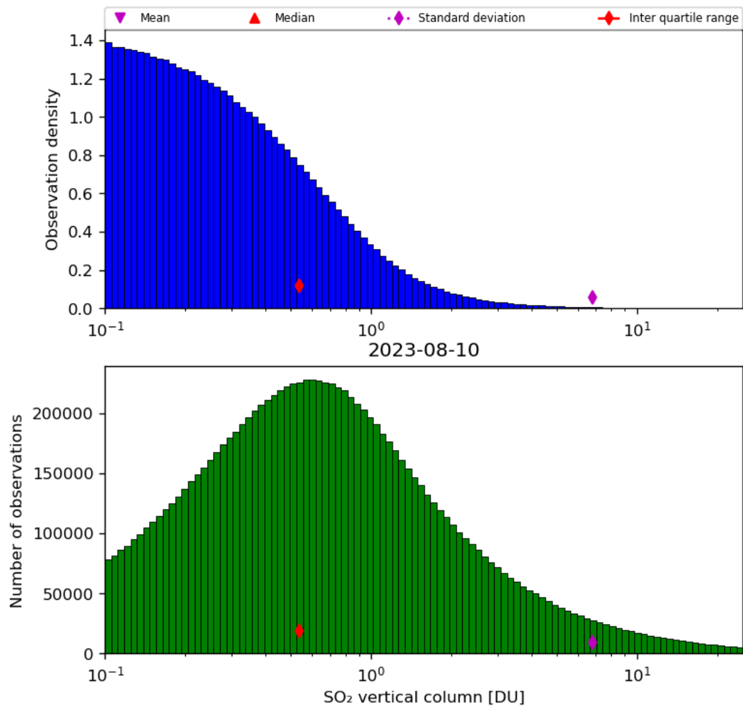
Figure 53: Histogram of “SO 2 vertical column” for 2023-08-09 to 2023-08-11
