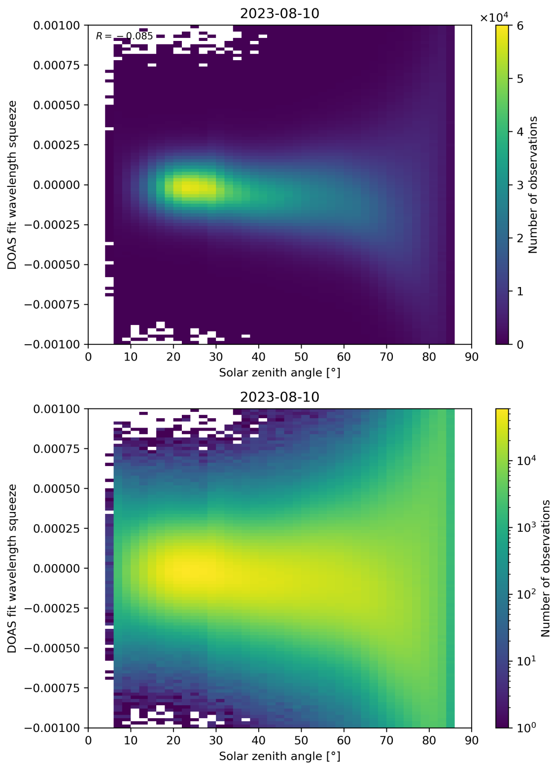
Figure 162: Scatter density plot of “Solar zenith angle” against “DOAS fit wavelength squeeze” for 2023-08-09 to 2023-08-11.
