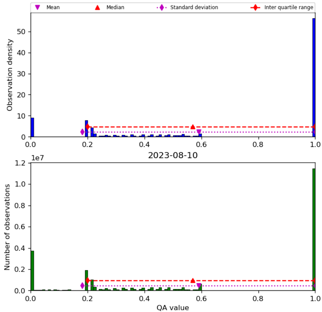
Figure 52: Histogram of “QA value” for 2023-08-09 to 2023-08-11
