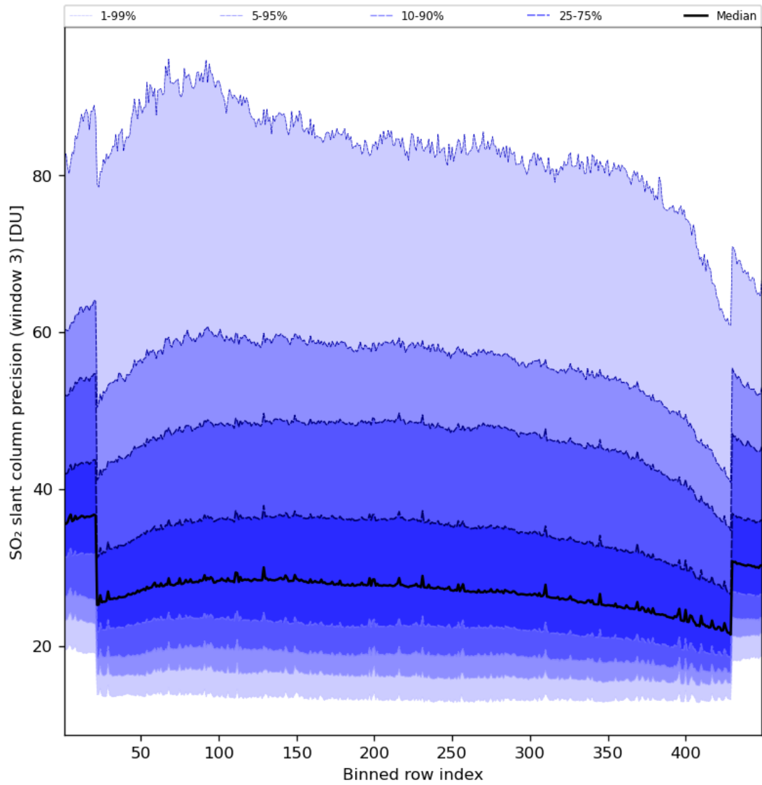
Figure 88: Along track statistics of “SO 2 slant column precision (window 3)” for 2023-08-09 to 2023-08-11
