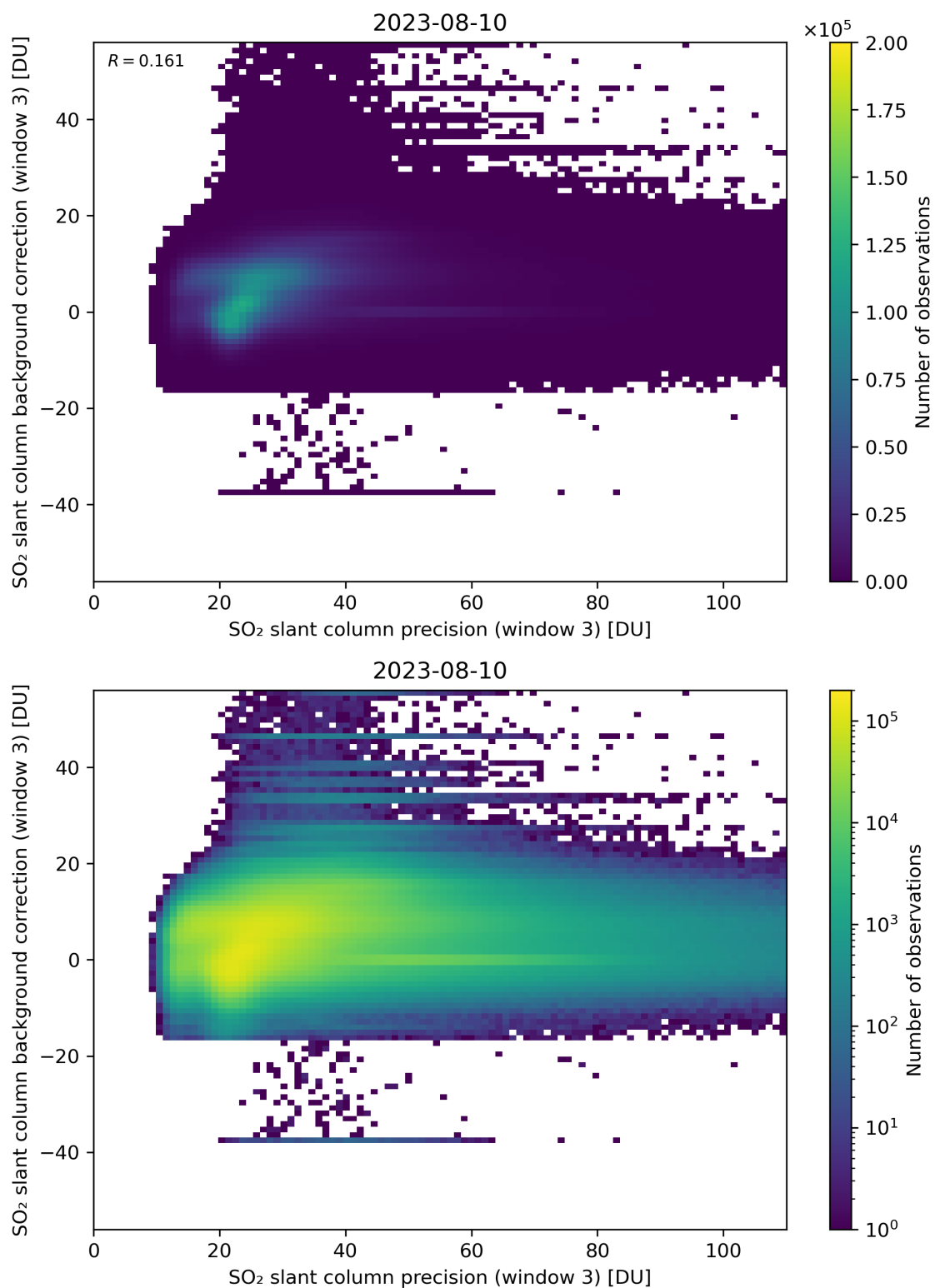
Figure 257: Scatter density plot of “SO 2 slant column precision (window 3)” against “SO 2 slant column background correction (window 3)” for 2023-08-09 to 2023-08-11.
