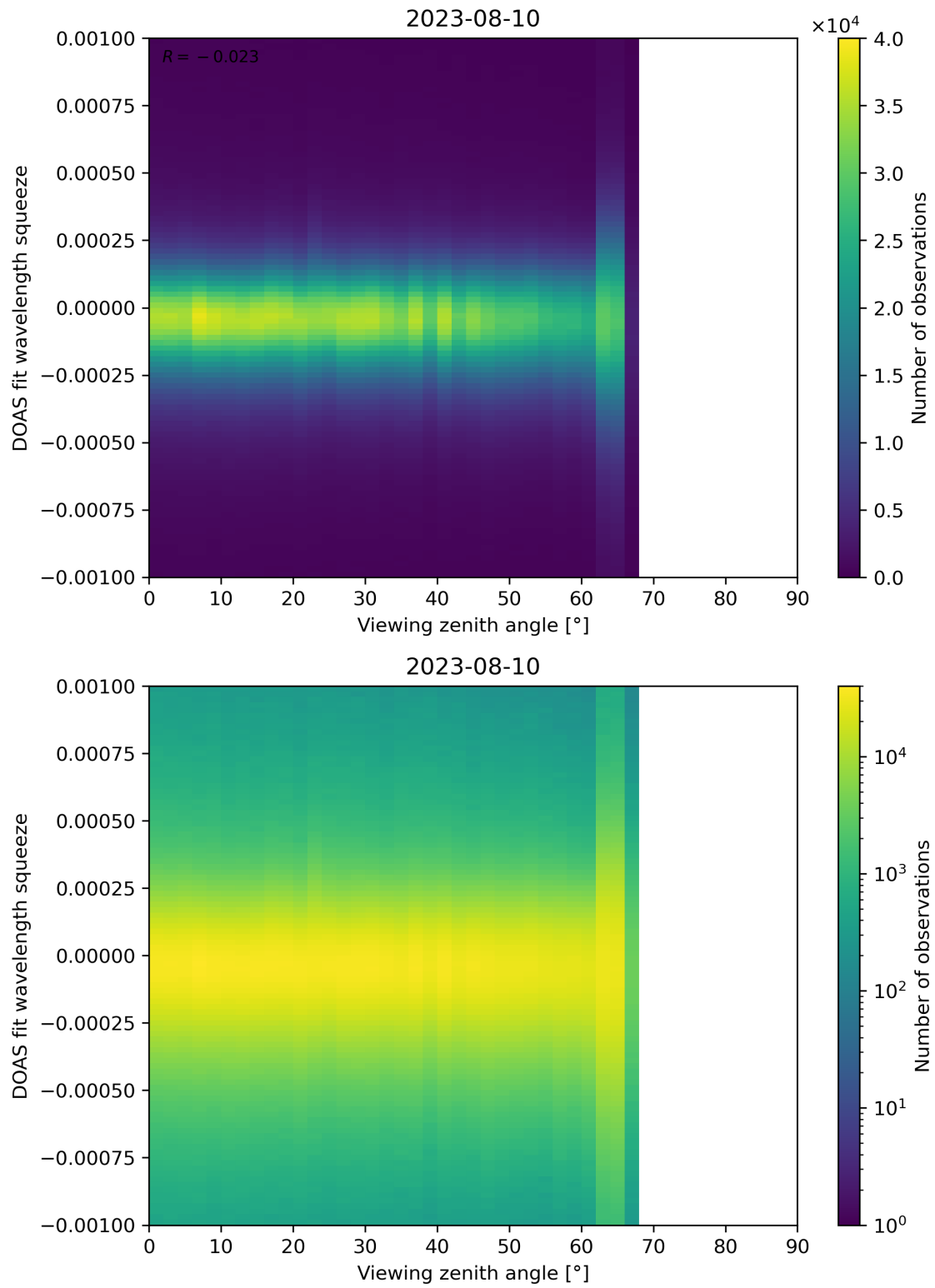
Figure 312: Scatter density plot of “Viewing zenith angle” against “DOAS fit wavelength squeeze” for 2023-08-09 to 2023-08-11.
