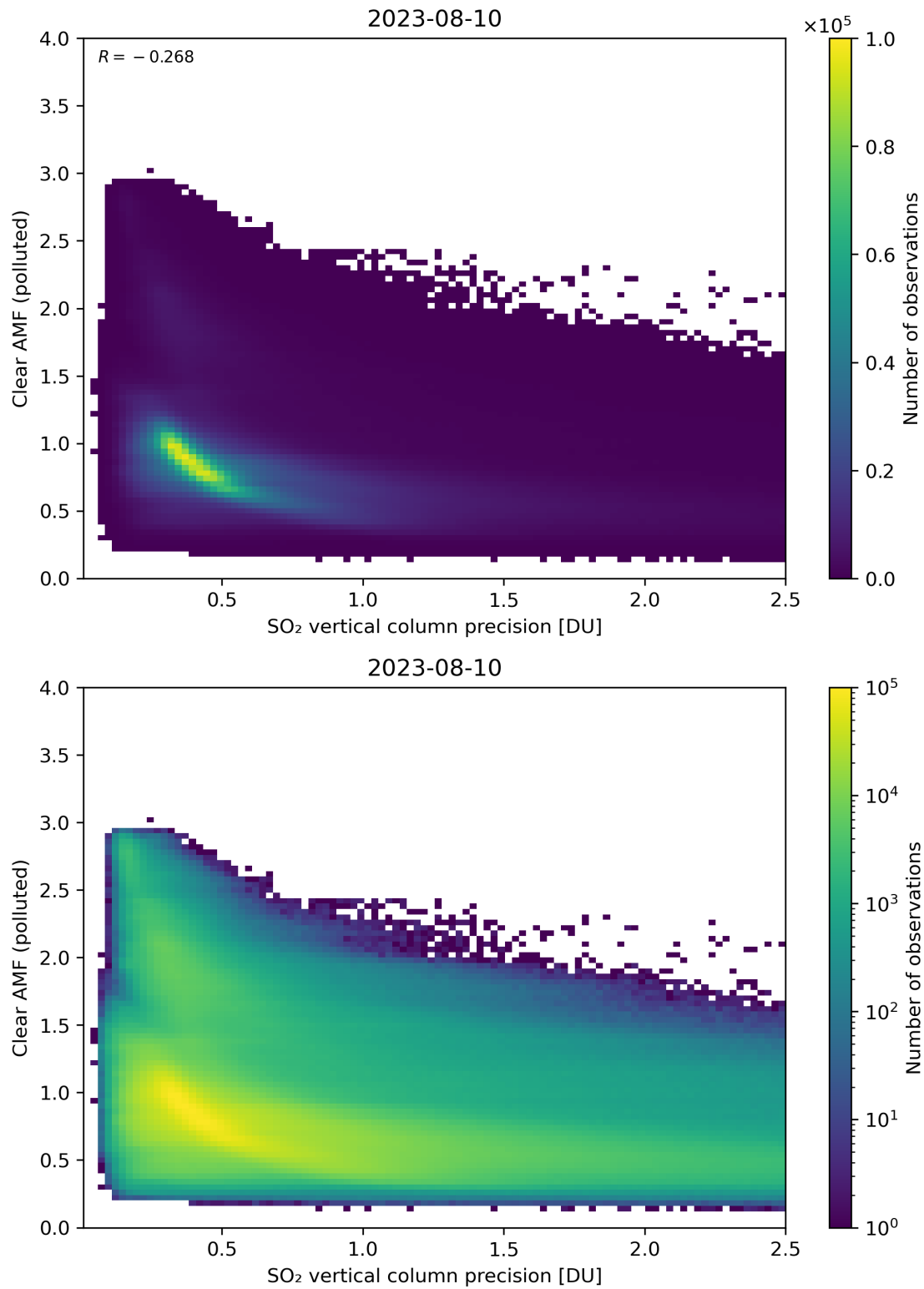
Figure 285: Scatter density plot of “SO 2 vertical column precision” against “Clear AMF (polluted)” for 2023-08-09 to 2023-08-11.
