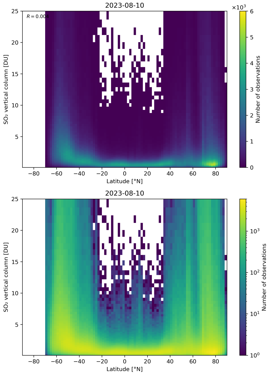
Figure 156: Scatter density plot of “Latitude” against “SO 2 vertical column” for 2023-08-09 to 2023-08-11.
