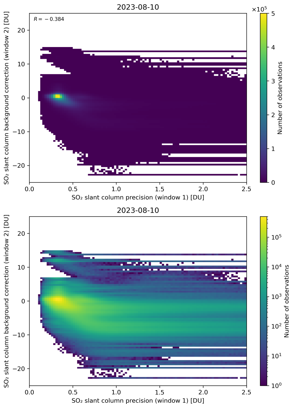
Figure 219: Scatter density plot of “SO 2 slant column precision (window 1)” against “SO 2 slant column background correction (window 2)” for 2023-08-09 to 2023-08-11.
