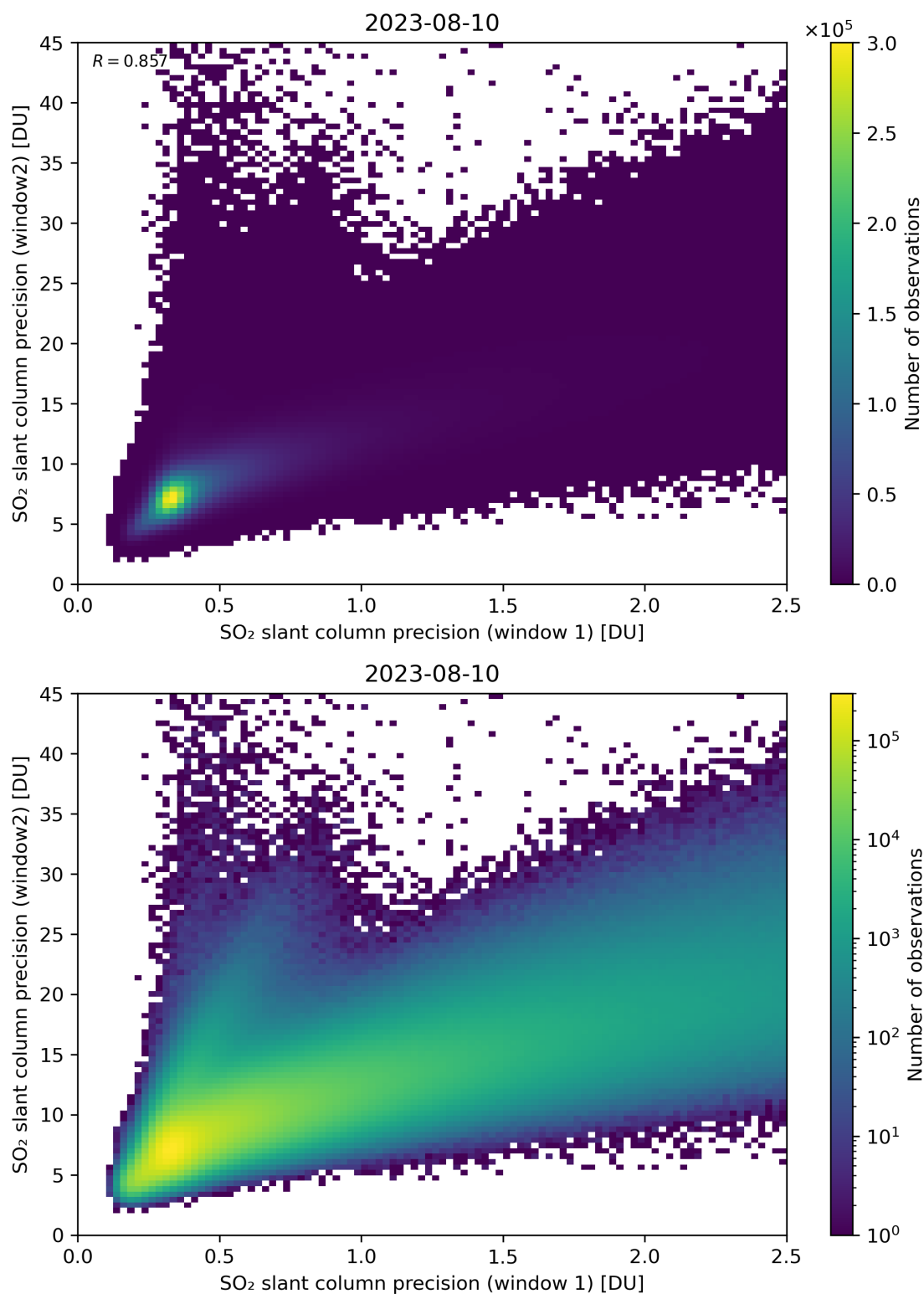
Figure 227: Scatter density plot of “SO 2 slant column precision (window 1)” against “SO 2 slant column precision (window2)” for 2023-08-09 to 2023-08-11.
