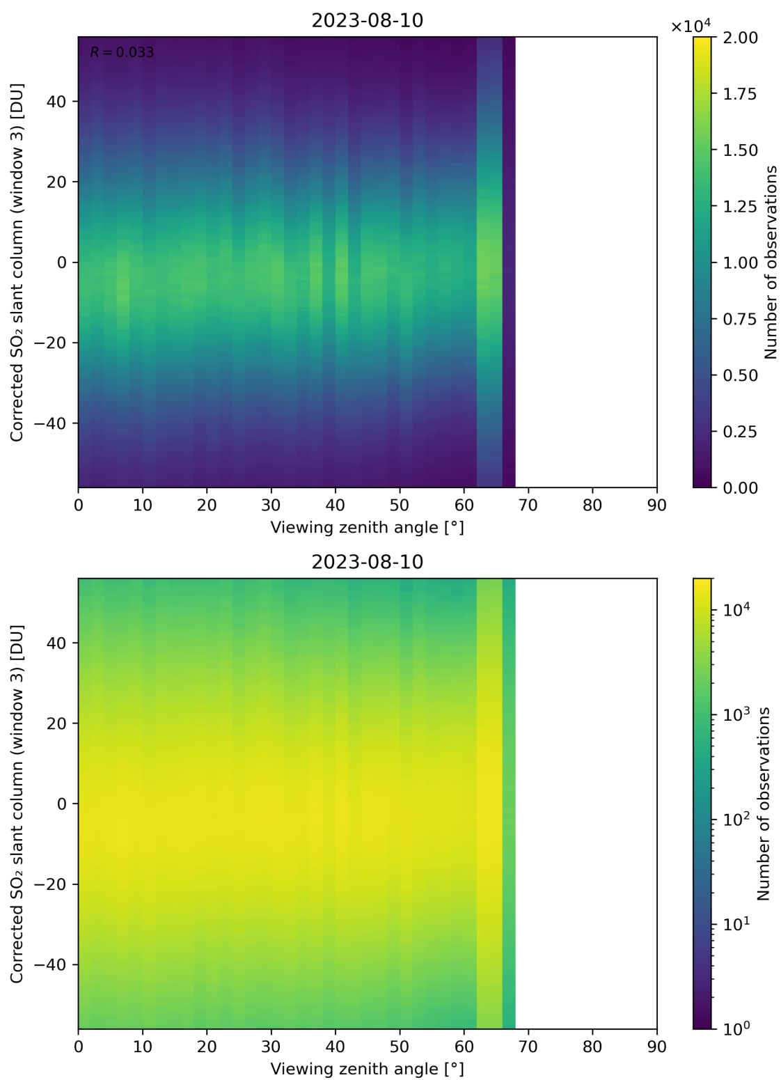
Figure 319: Scatter density plot of “Viewing zenith angle” against “Corrected SO 2 slant column (window 3)” for 2023-08-09 to 2023-08-11.
