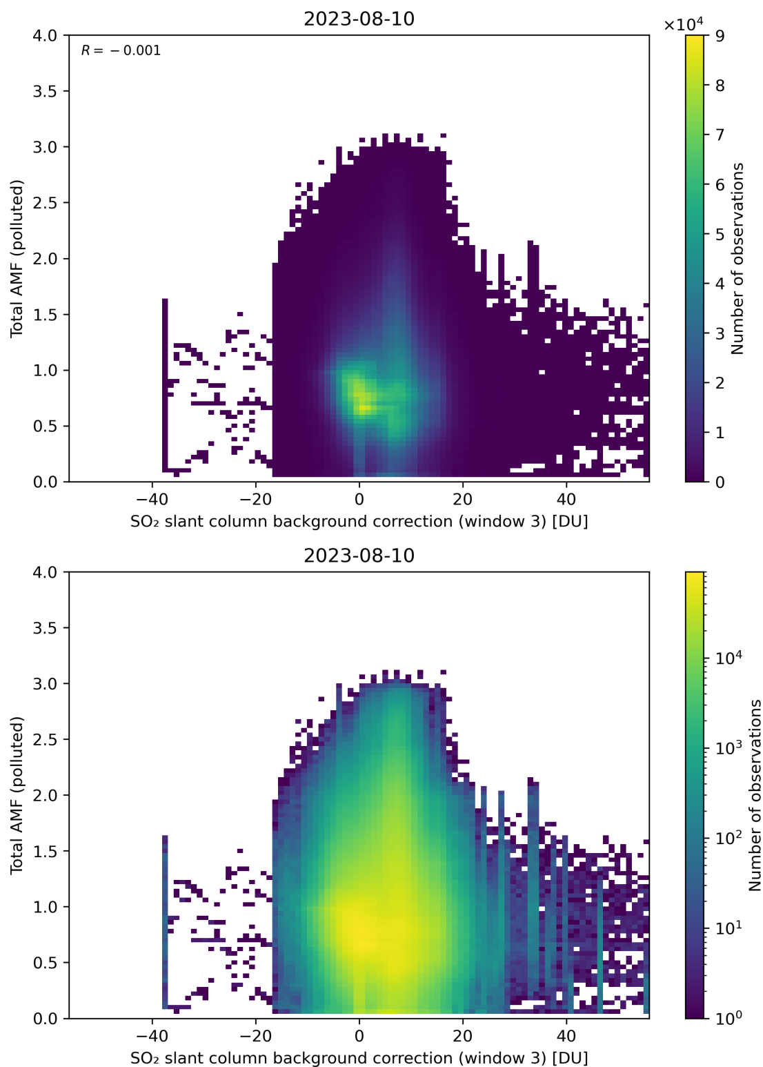
Figure 125: Scatter density plot of “SO 2 slant column background correction (window 3)” against “Total AMF (polluted)” for 2023-08-09 to 2023-08-11.
