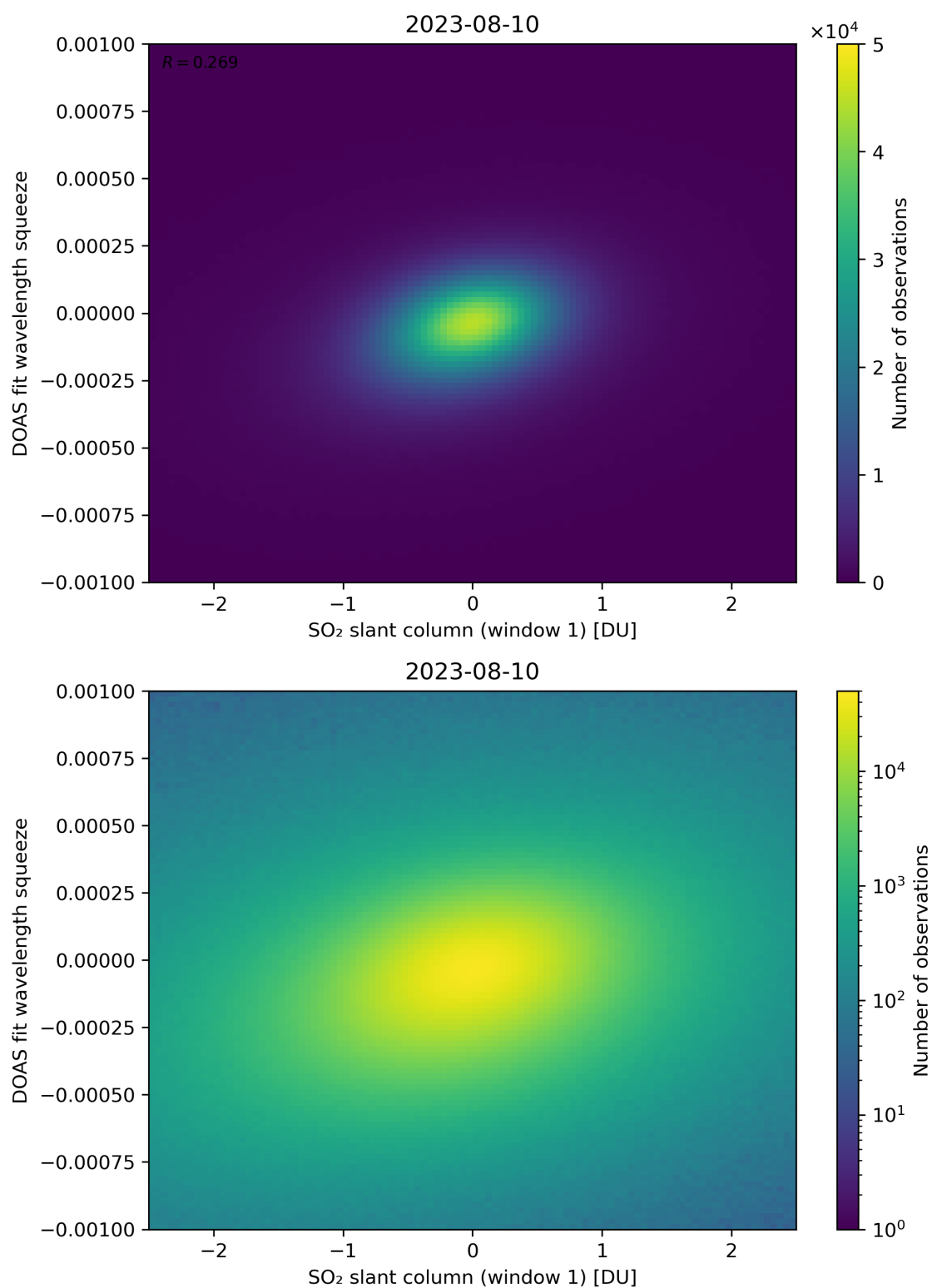
Figure 216: Scatter density plot of “SO 2 slant column (window 1)” against “DOAS fit wavelength squeeze” for 2023-08-09 to 2023-08-11.
