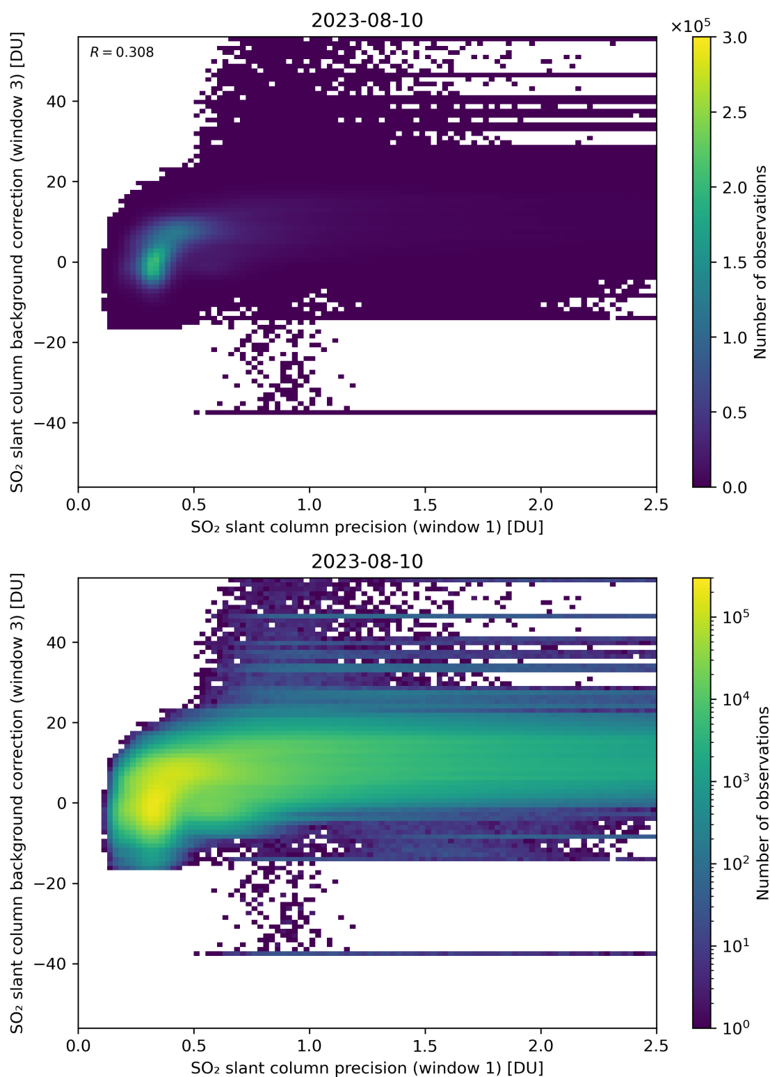
Figure 220: Scatter density plot of “SO 2 slant column precision (window 1)” against “SO 2 slant column background correction (window 3)” for 2023-08-09 to 2023-08-11.
