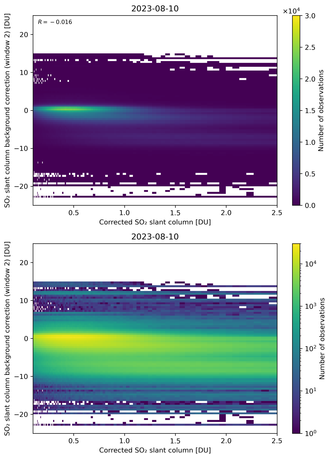
Figure 179: Scatter density plot of “Corrected SO 2 slant column” against “SO 2 slant column background correction (window 2)” for 2023-08-09 to 2023-08-11.
