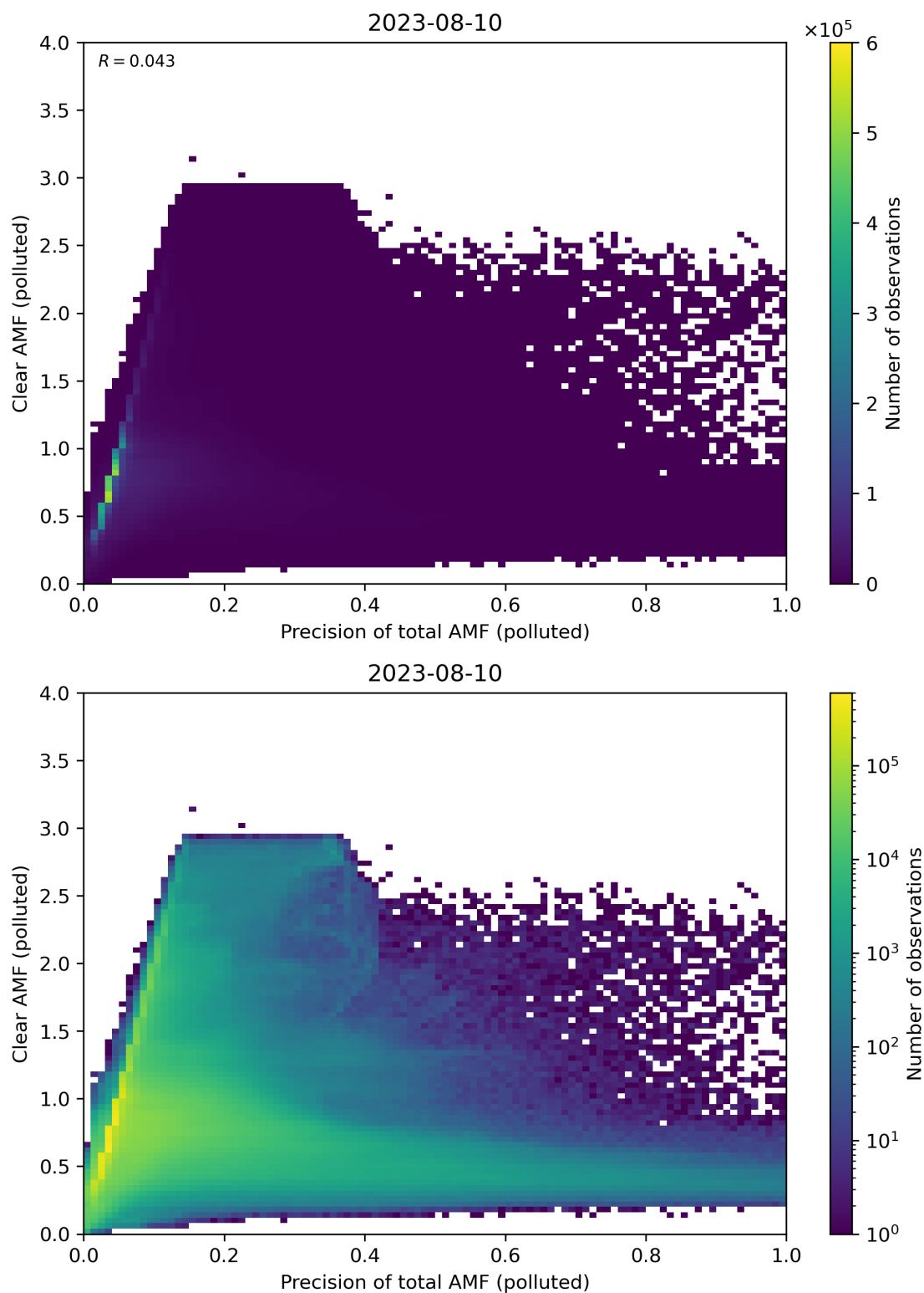
Figure 270: Scatter density plot of “Precision of total AMF (polluted)” against “Clear AMF (polluted)” for 2023-08-09 to 2023-08-11.
