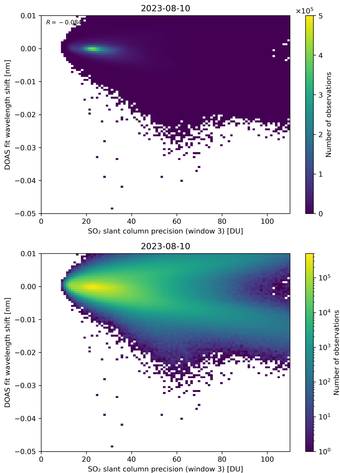
Figure 258: Scatter density plot of “SO 2 slant column precision (window 3)” against “DOAS fit wavelength shift” for 2023-08-09 to 2023-08-11.
