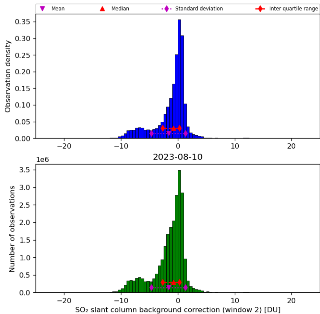
Figure 63: Histogram of “SO 2 slant column background correction (window 2)” for 2023-08-09 to 2023-08-11
