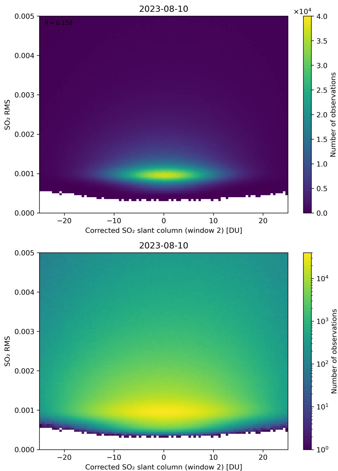
Figure 198: Scatter density plot of “Corrected SO 2 slant column (window 2)” against “SO 2 RMS” for 2023-08-09 to 2023-08-11.
