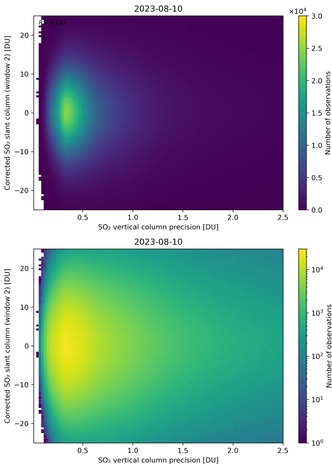
Figure 287: Scatter density plot of “SO 2 vertical column precision” against “Corrected SO 2 slant column (window 2)” for 2023-08-09 to 2023-08-11.
