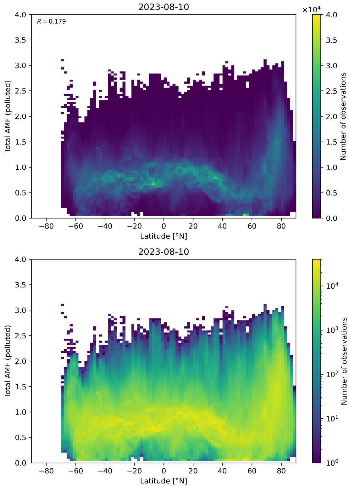
Figure 154: Scatter density plot of “Latitude” against “Total AMF (polluted)” for 2023-08-09 to 2023-08-11.
