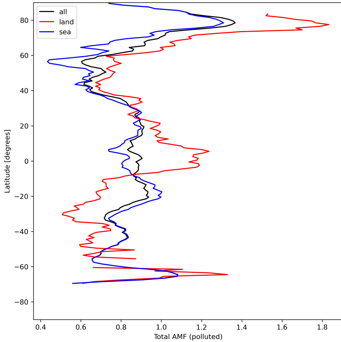
Figure 48: Zonal average of “Total AMF (polluted)” for 2023-08-09 to 2023-08-11.
