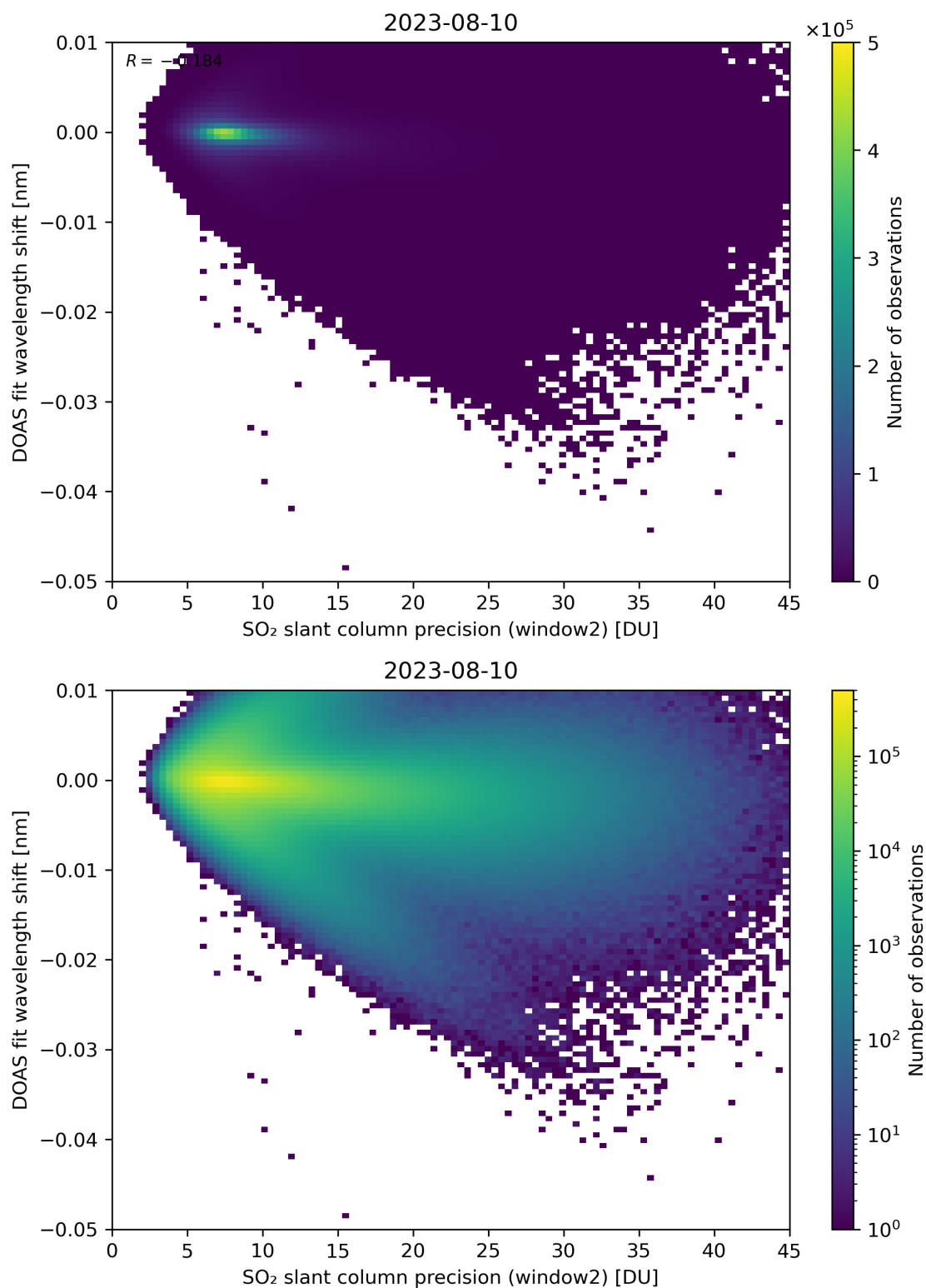
Figure 243: Scatter density plot of “SO 2 slant column precision (window2)” against “DOAS fit wavelength shift” for 2023-08-09 to 2023-08-11.
