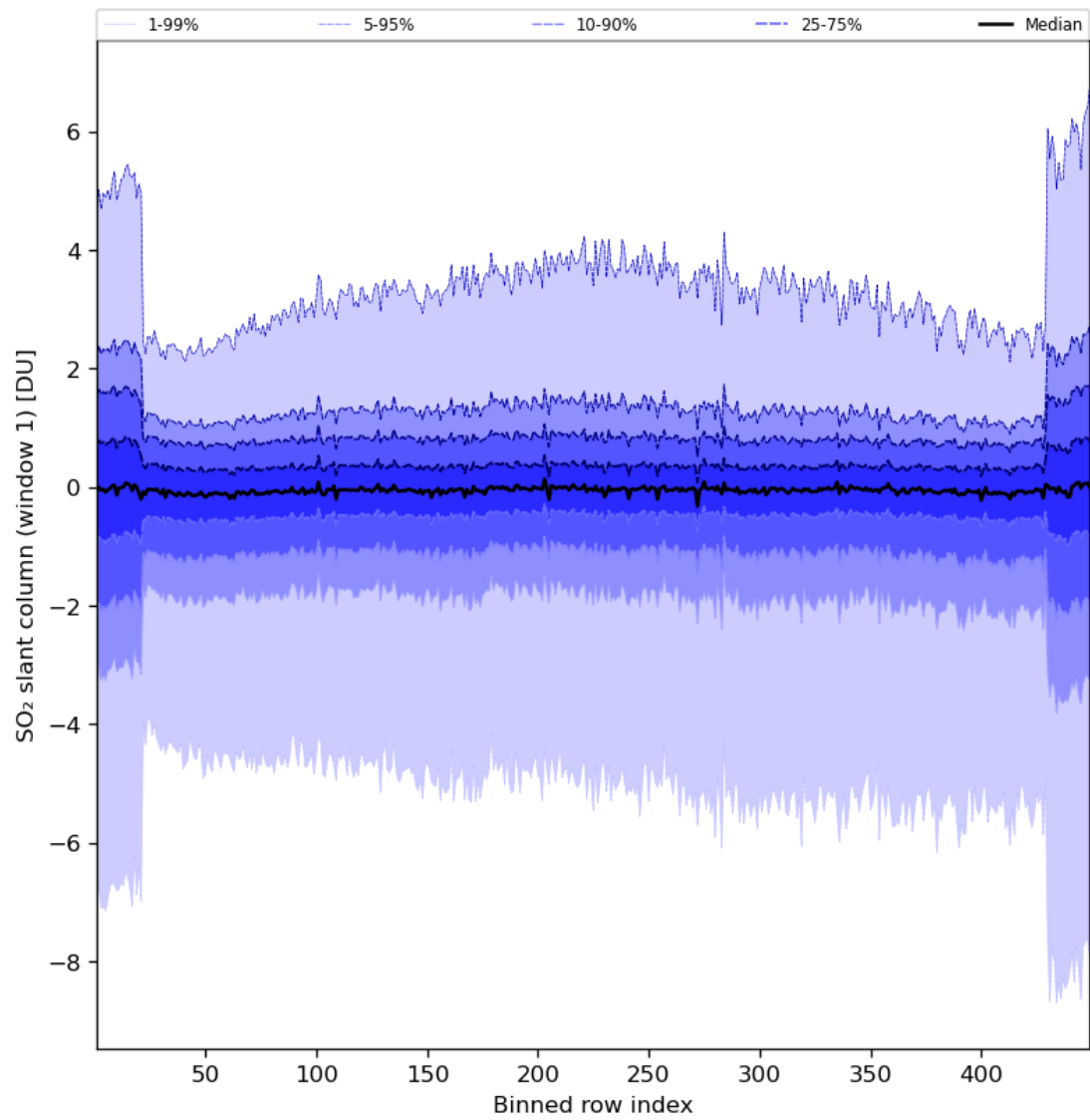
Figure 79: Along track statistics of “SO 2 slant column (window 1)” for 2023-08-09 to 2023-08-11
