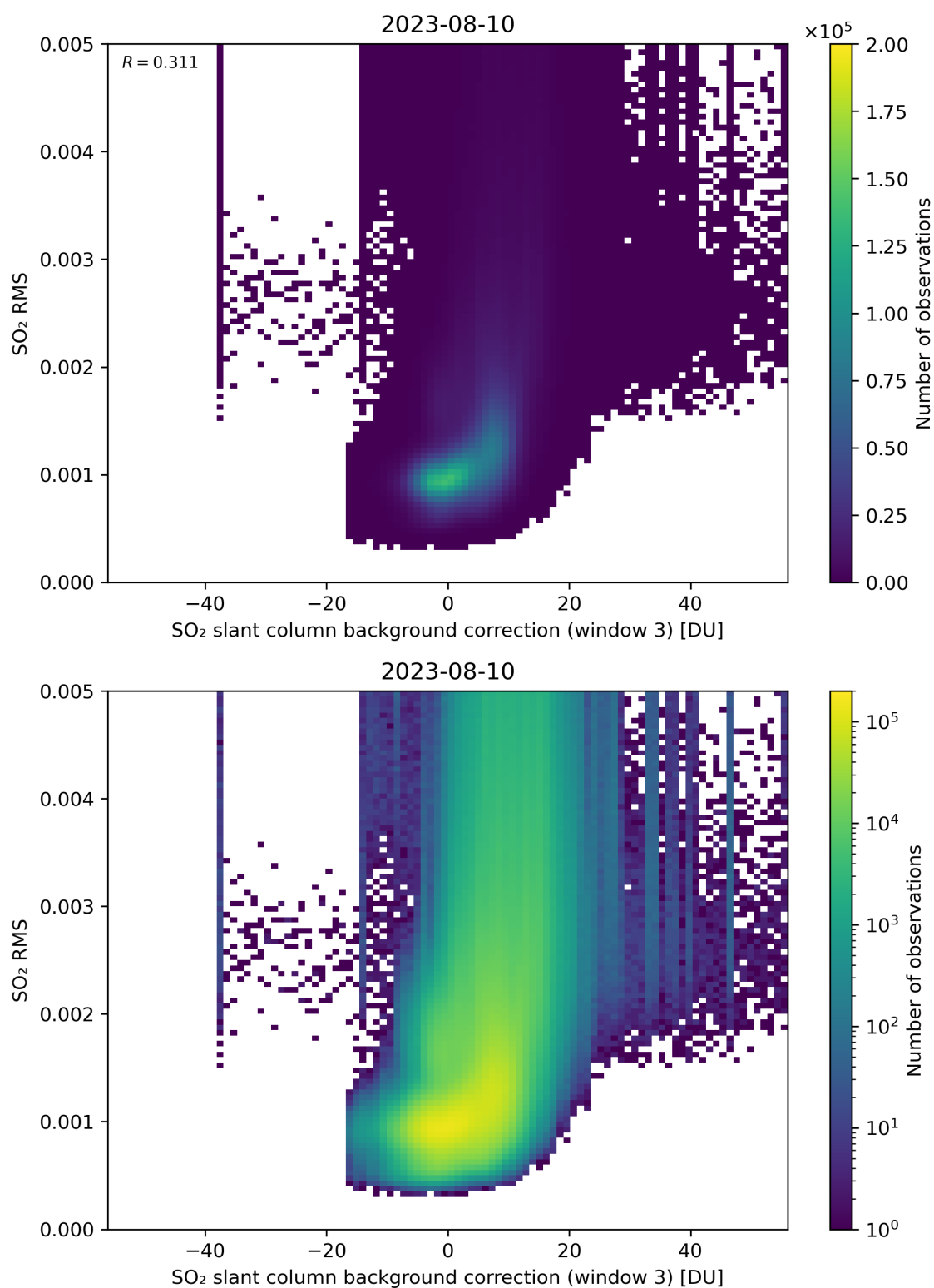
Figure 123: Scatter density plot of “SO 2 slant column background correction (window 3)” against “SO 2 RMS” for 2023-08-09 to 2023-08-11.
