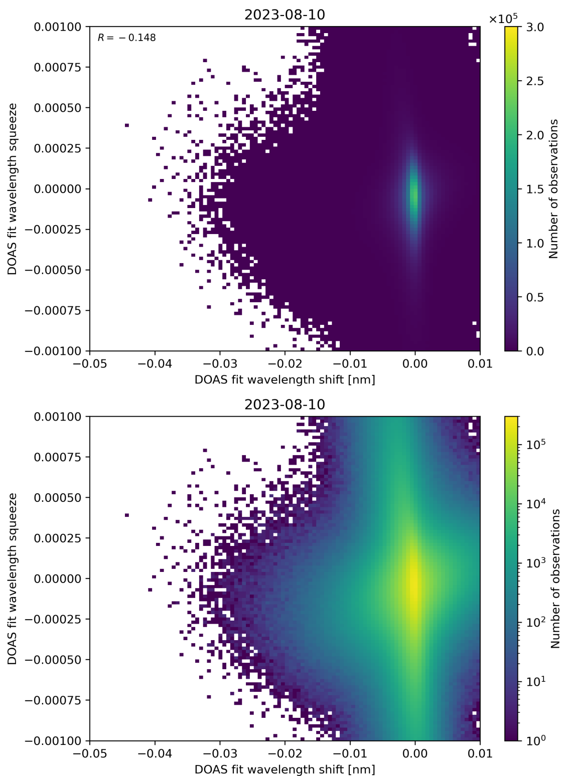
Figure 127: Scatter density plot of “DOAS fit wavelength shift” against “DOAS fit wavelength squeeze” for 2023-08-09 to 2023-08-11.
