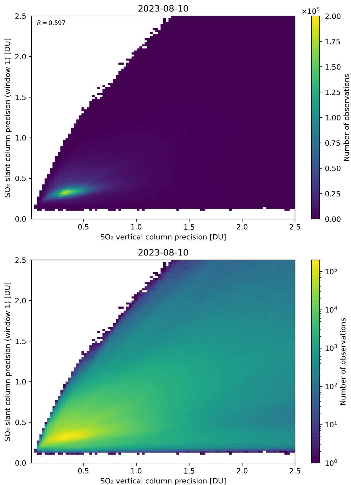
Figure 290: Scatter density plot of “SO 2 vertical column precision” against “SO 2 slant column precision (window 1)” for 2023-08-09 to 2023-08-11.
