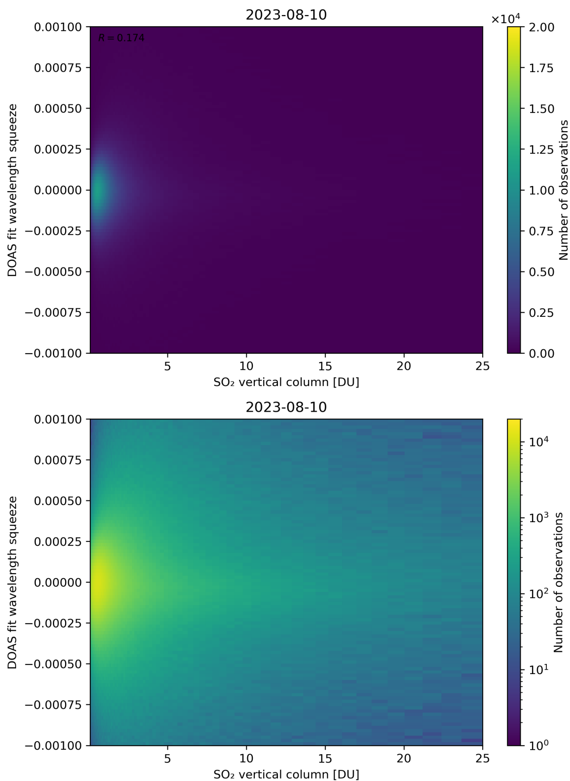
Figure 277: Scatter density plot of “SO 2 vertical column” against “DOAS fit wavelength squeeze” for 2023-08-09 to 2023-08-11.
