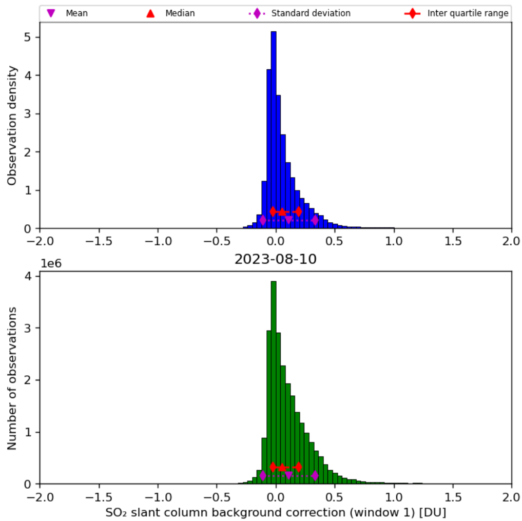
Figure 59: Histogram of “SO 2 slant column background correction (window 1)” for 2023-08-09 to 2023-08-11
