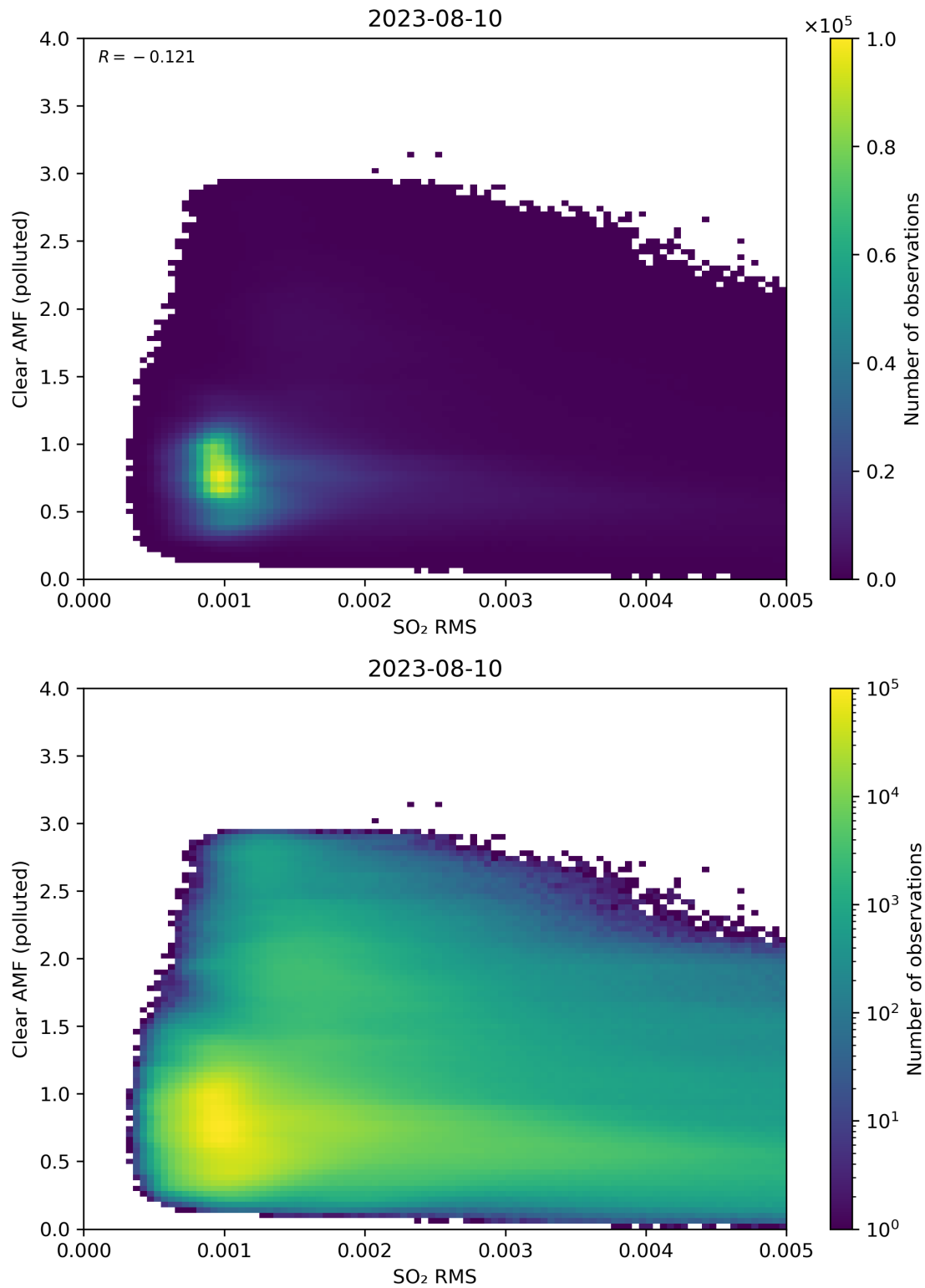
Figure 136: Scatter density plot of “SO 2 RMS” against “Clear AMF (polluted)” for 2023-08-09 to 2023-08-11.
