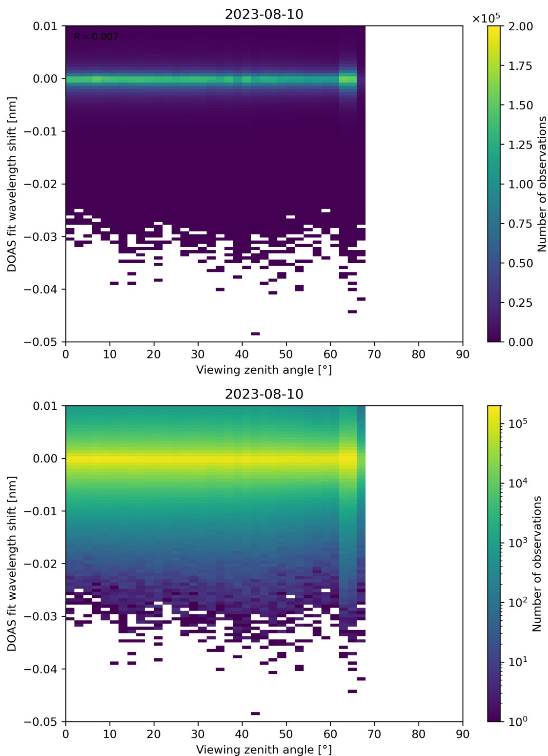
Figure 311: Scatter density plot of “Viewing zenith angle” against “DOAS fit wavelength shift” for 2023-08-09 to 2023-08-11.
