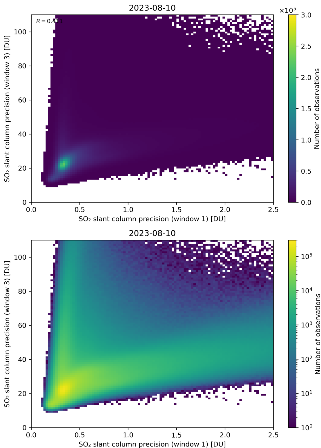
Figure 229: Scatter density plot of “SO 2 slant column precision (window 1)” against “SO 2 slant column precision (window 3)” for 2023-08-09 to 2023-08-11.
