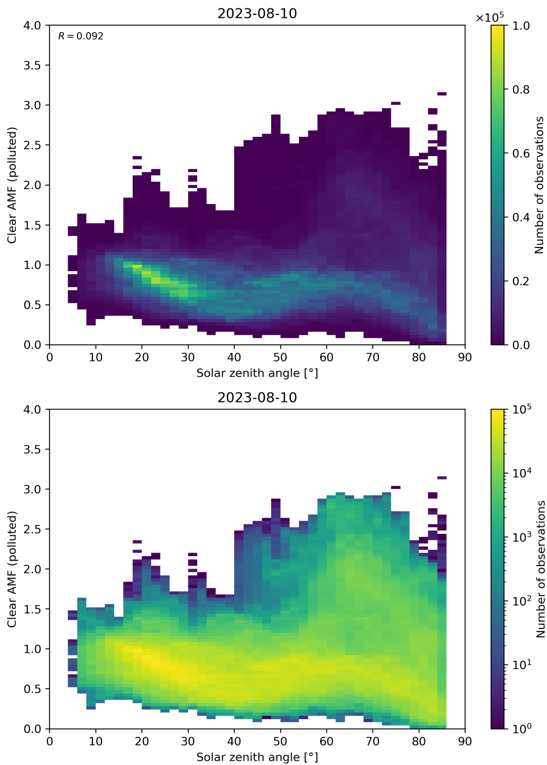
Figure 165: Scatter density plot of “Solar zenith angle” against “Clear AMF (polluted)” for 2023-08-09 to 2023-08-11.
