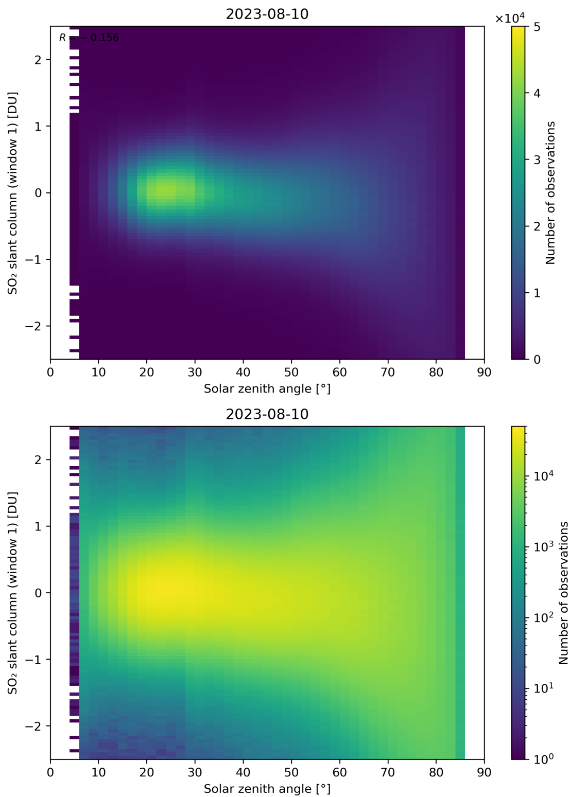
Figure 169: Scatter density plot of “Solar zenith angle” against “SO 2 slant column (window 1)” for 2023-08-09 to 2023-08-11.
