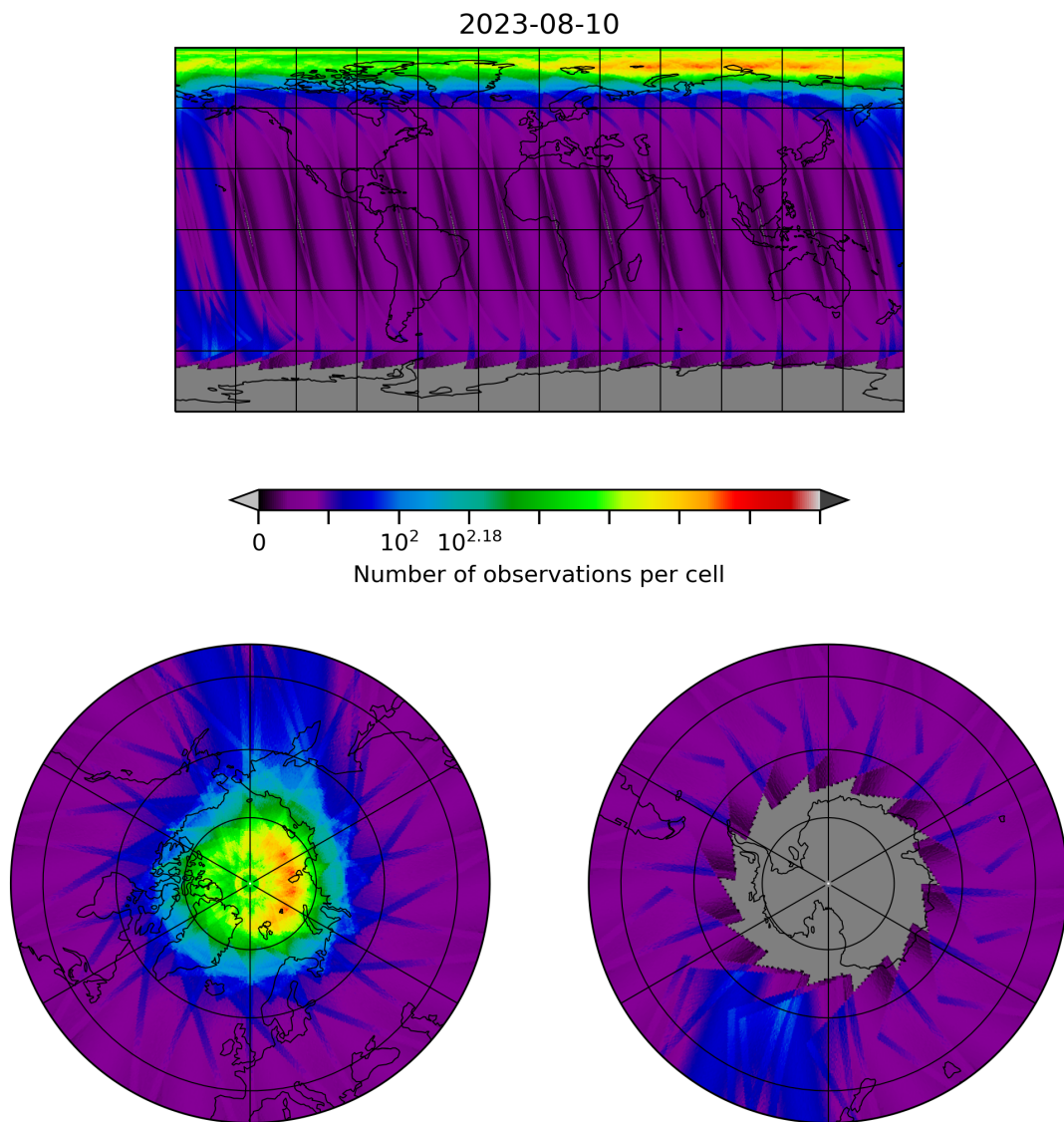
Figure 28: Map of the number of observations for 2023-08-09 to 2023-08-11
