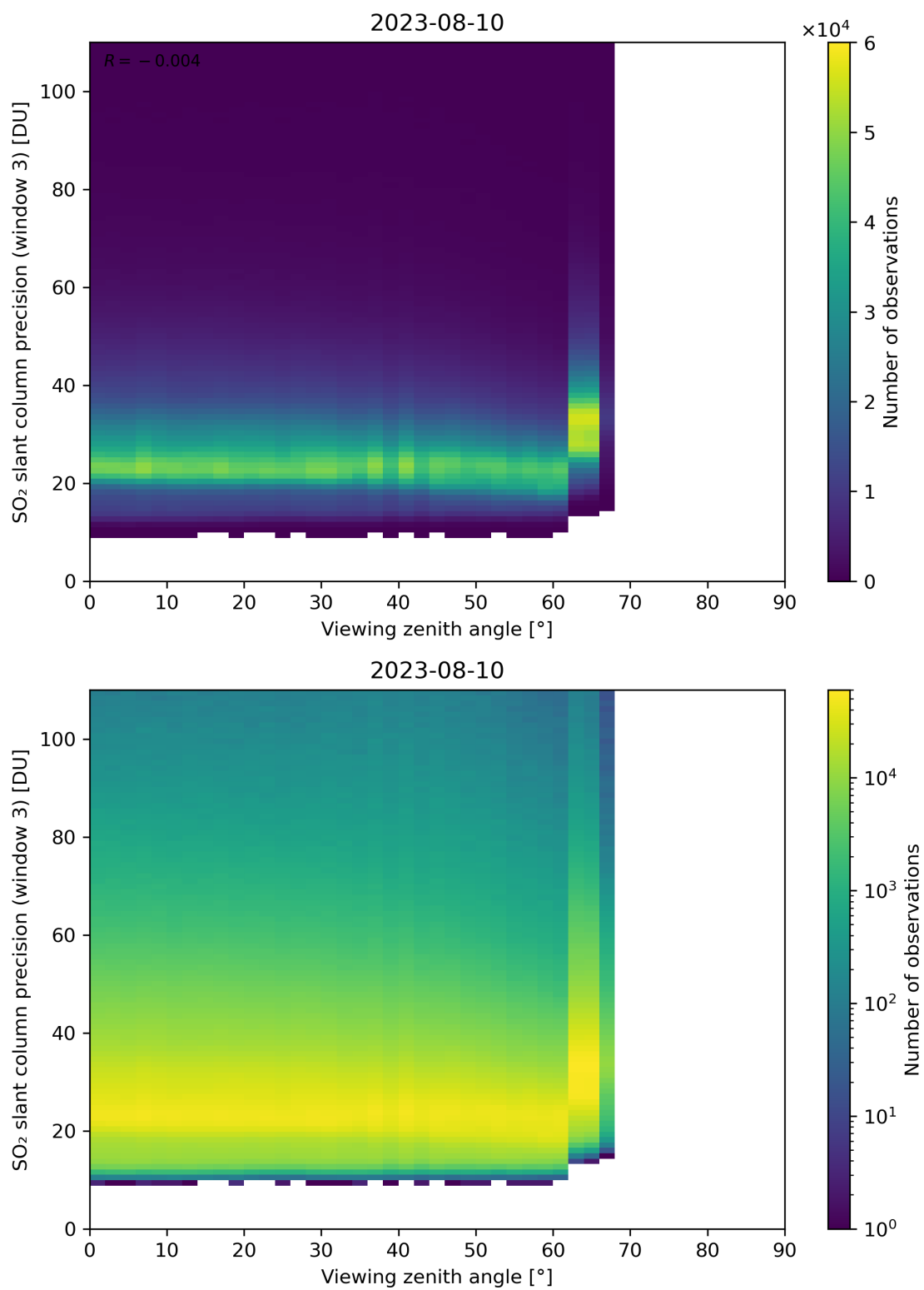
Figure 324: Scatter density plot of “Viewing zenith angle” against “SO 2 slant column precision (window 3)” for 2023-08-09 to 2023-08-11.
