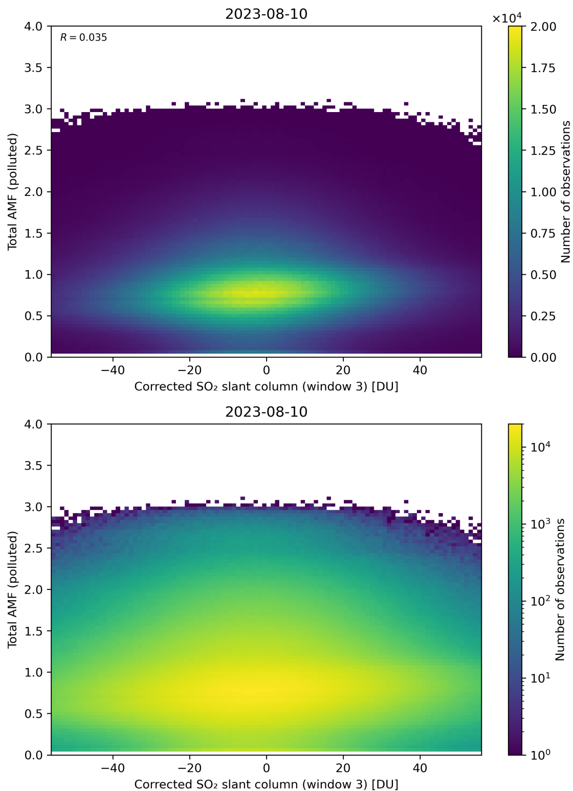
Figure 210: Scatter density plot of “Corrected SO 2 slant column (window 3)” against “Total AMF (polluted)” for 2023-08-09 to 2023-08-11.
