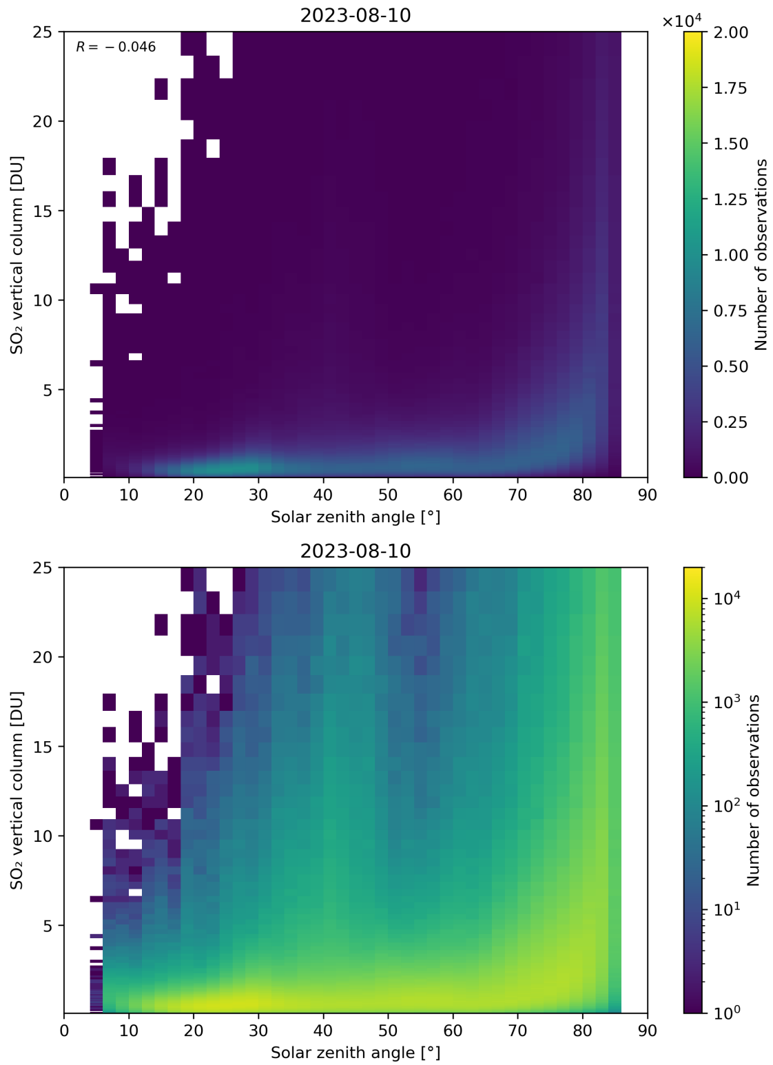
Figure 176: Scatter density plot of “Solar zenith angle” against “SO 2 vertical column” for 2023-08-09 to 2023-08-11.
