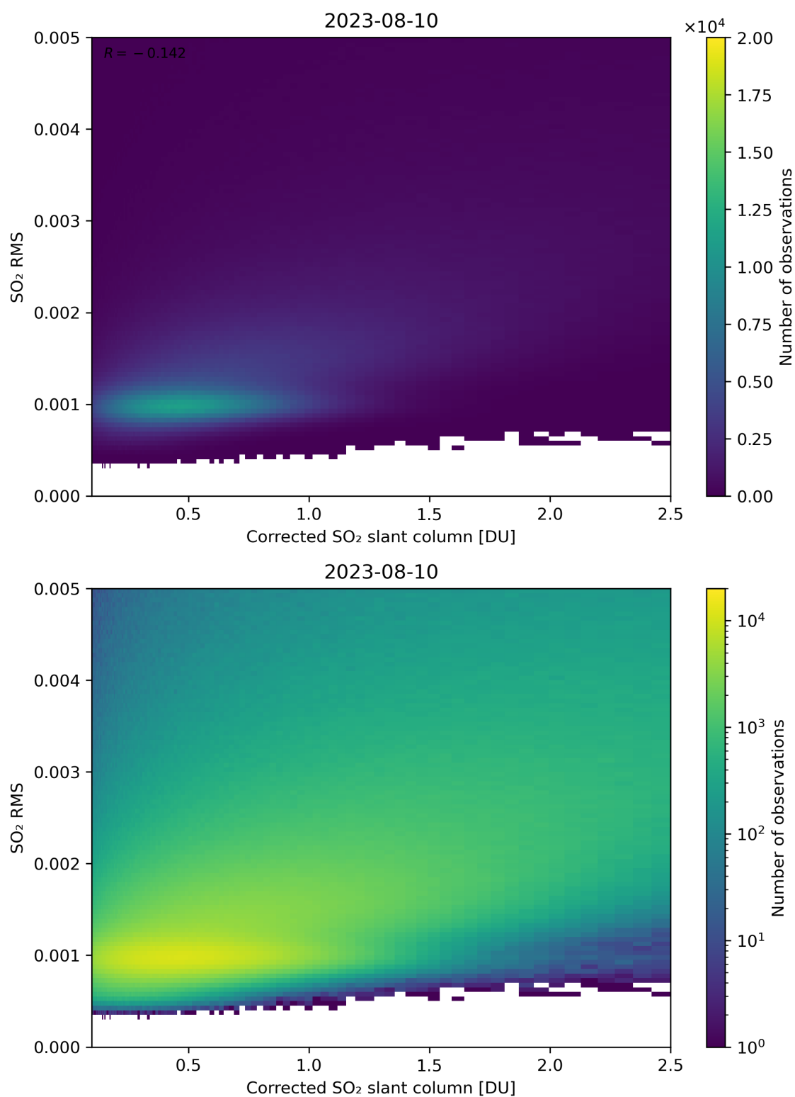
Figure 183: Scatter density plot of “Corrected SO 2 slant column” against “SO 2 RMS” for 2023-08-09 to 2023-08-11.
