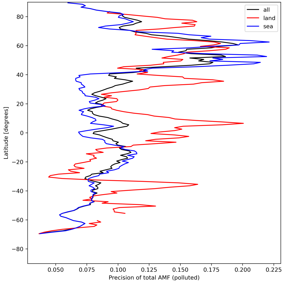
Figure 49: Zonal average of “Precision of total AMF (polluted)” for 2023-08-09 to 2023-08-11.
