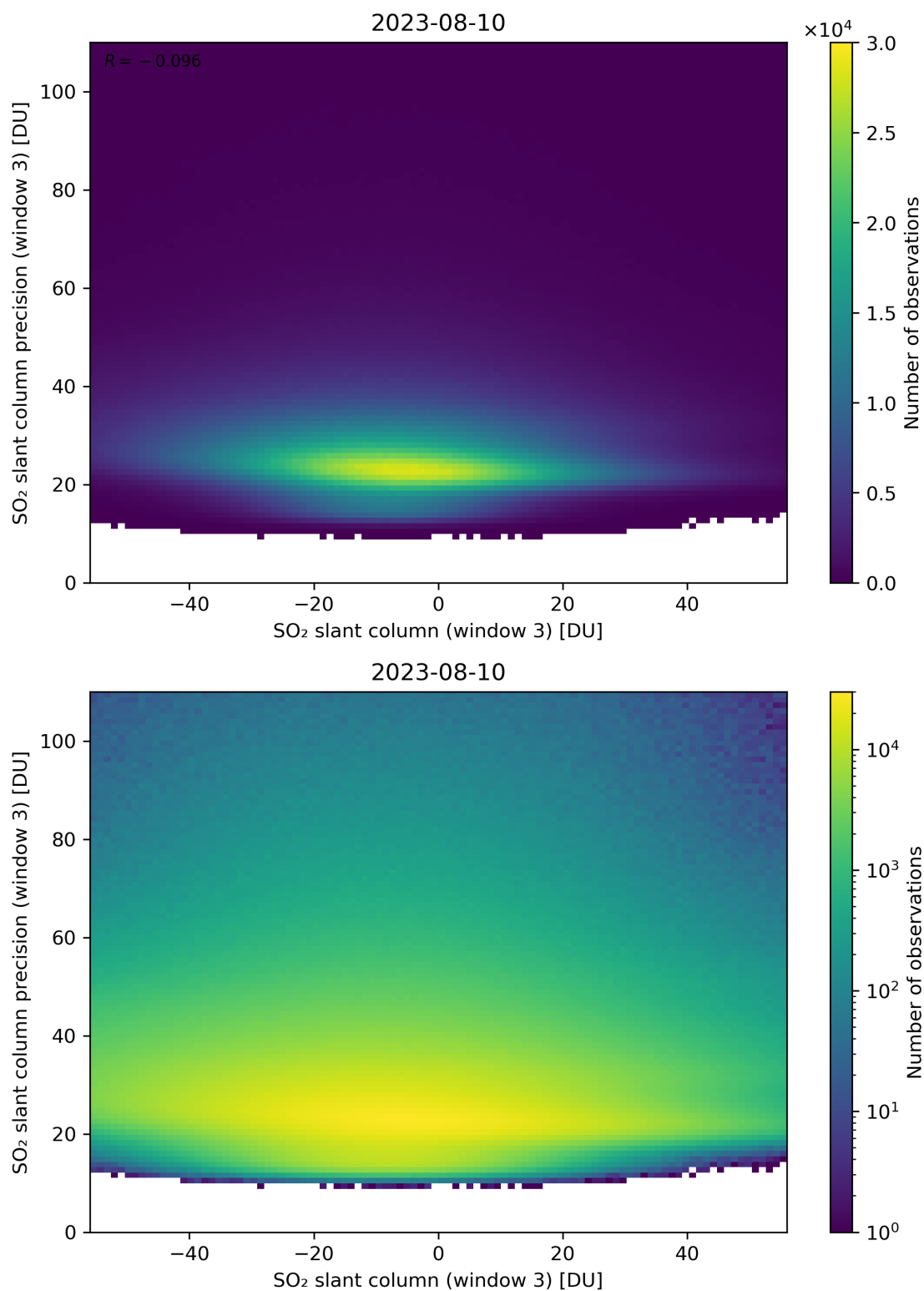
Figure 267: Scatter density plot of “SO 2 slant column (window 3)” against “SO 2 slant column precision (window 3)” for 2023-08-09 to 2023-08-11.
