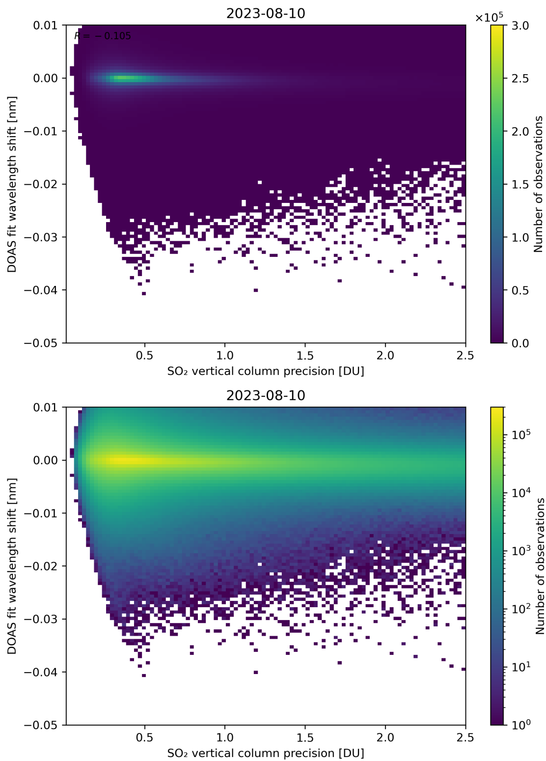
Figure 282: Scatter density plot of “SO 2 vertical column precision” against “DOAS fit wavelength shift” for 2023-08-09 to 2023-08-11.
