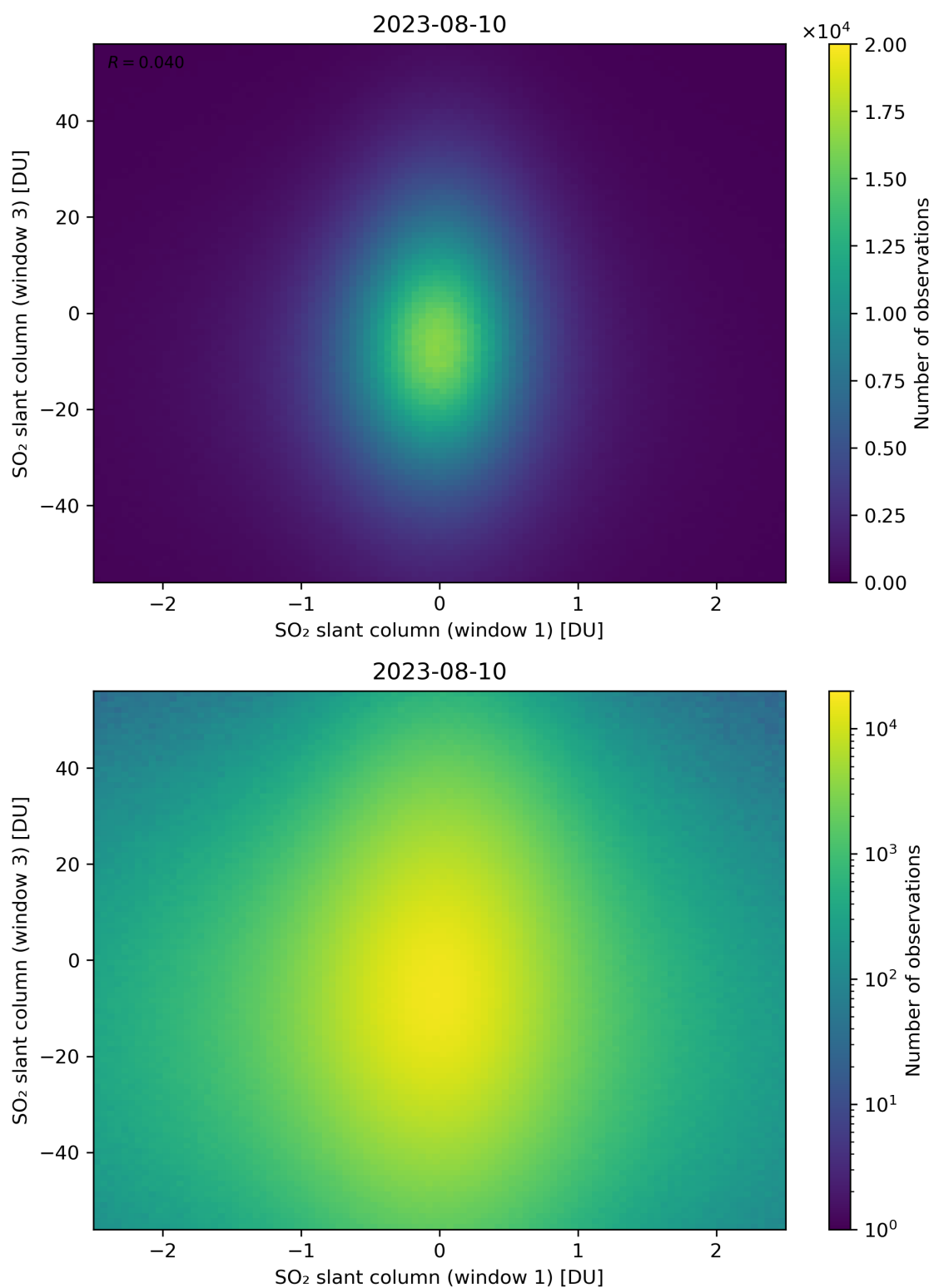
Figure 237: Scatter density plot of “SO 2 slant column (window 1)” against “SO 2 slant column (window 3)” for 2023-08-09 to 2023-08-11.
