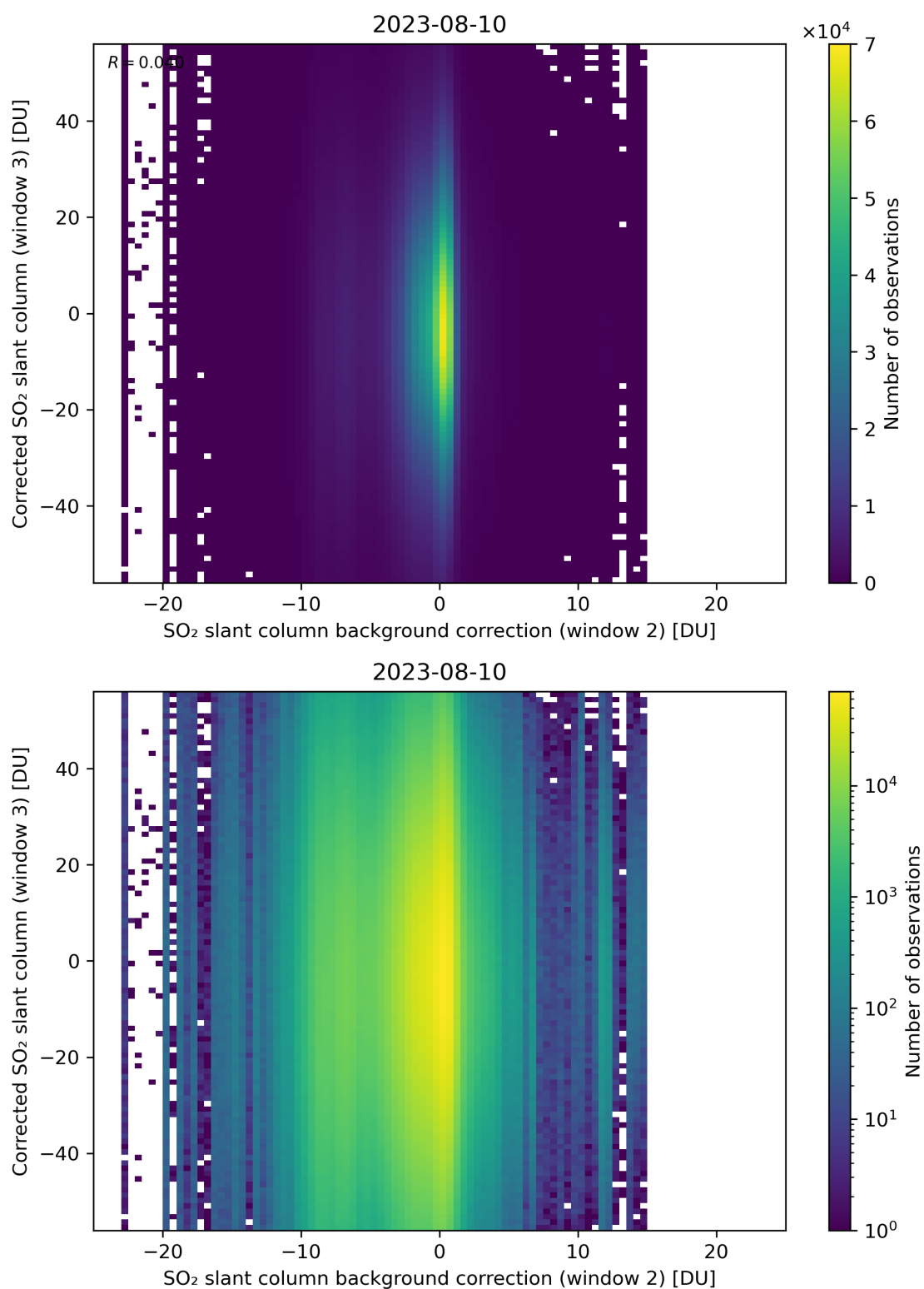
Figure 116: Scatter density plot of “SO 2 slant column background correction (window 2)” against “Corrected SO 2 slant column (window 3)” for 2023-08-09 to 2023-08-11.
