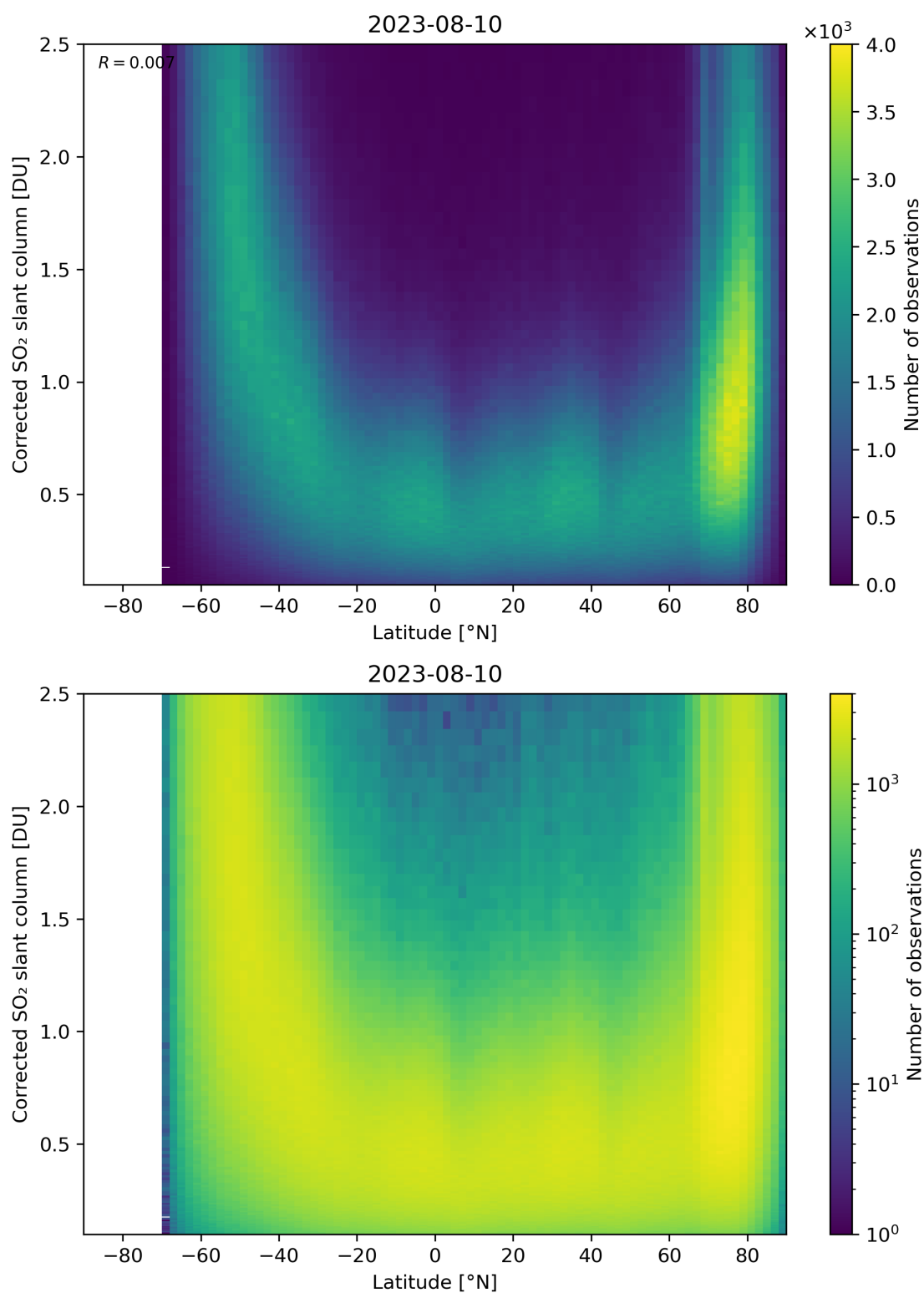
Figure 146: Scatter density plot of “Latitude” against “Corrected SO 2 slant column” for 2023-08-09 to 2023-08-11.
