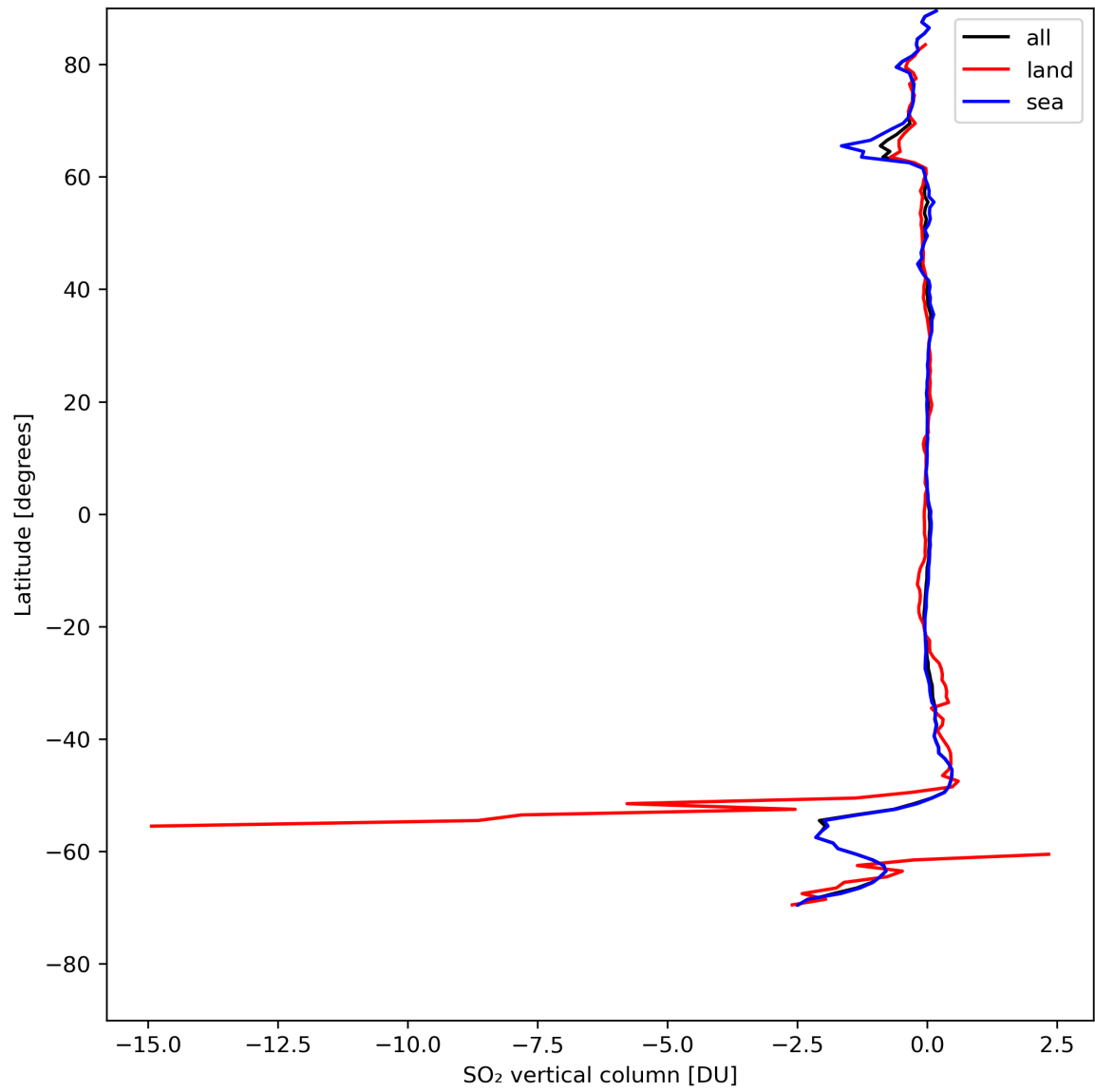
Figure 30: Zonal average of “SO 2 vertical column” for 2023-08-09 to 2023-08-11.
