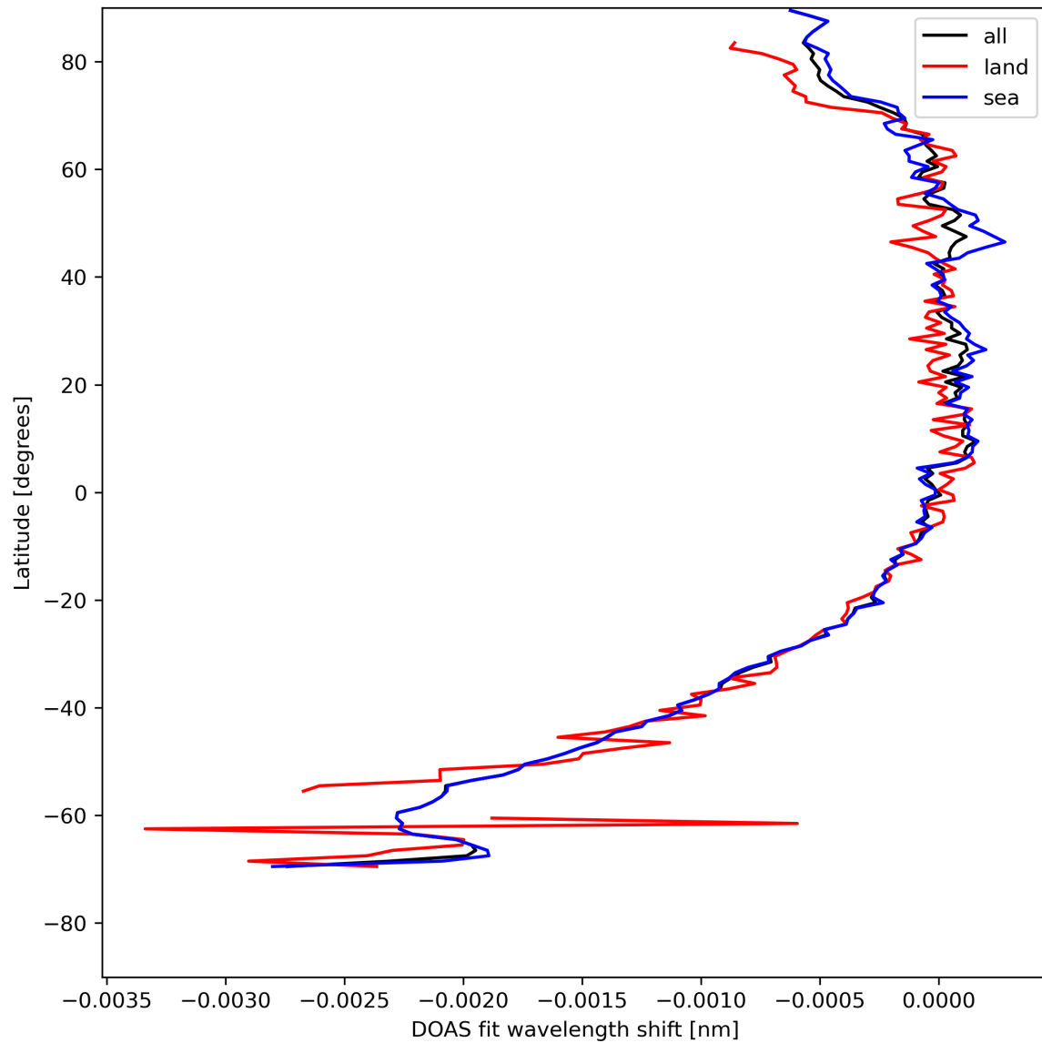
Figure 45: Zonal average of “DOAS fit wavelength shift” for 2023-08-09 to 2023-08-11.
