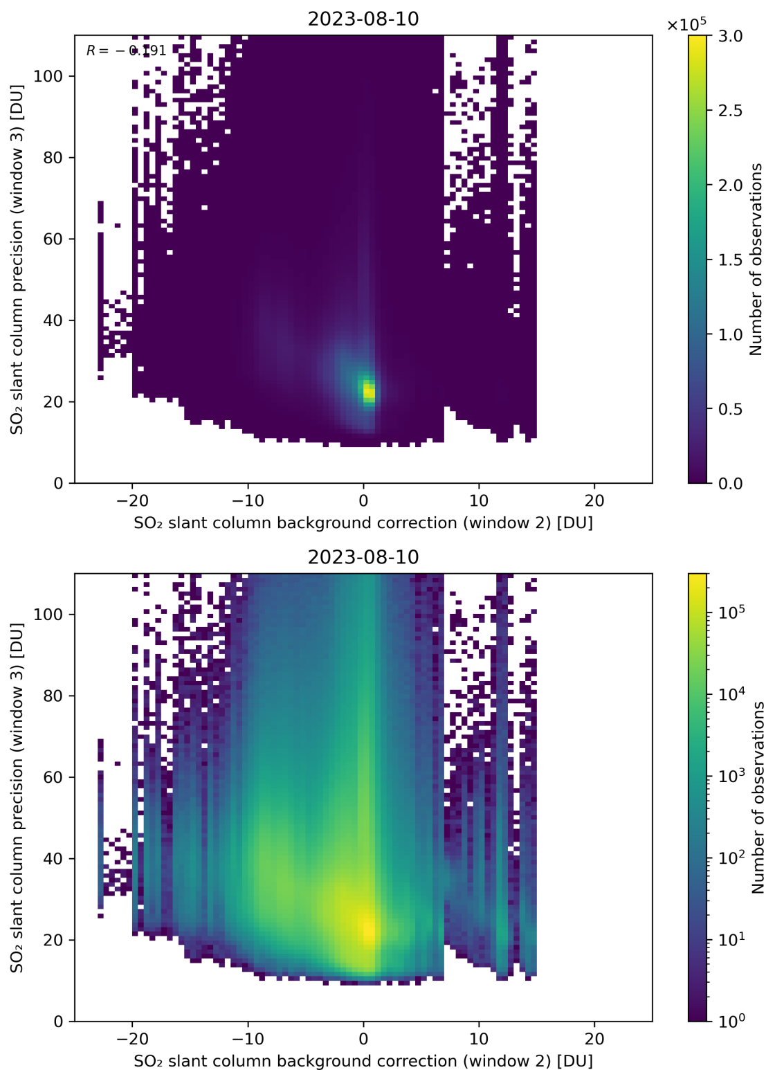
Figure 118: Scatter density plot of “SO 2 slant column background correction (window 2)” against “SO 2 slant column precision (window 3)” for 2023-08-09 to 2023-08-11.
