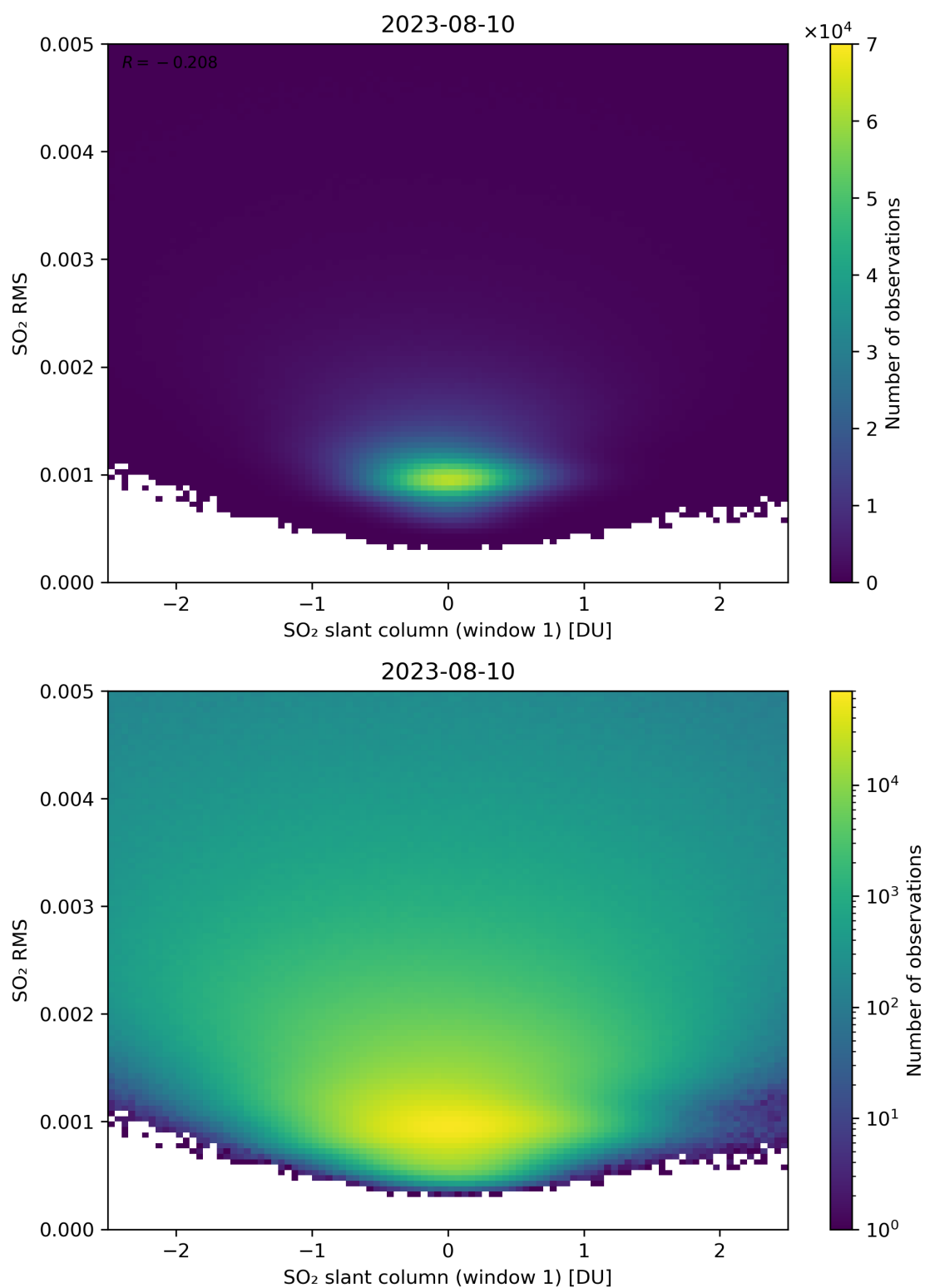
Figure 217: Scatter density plot of “SO 2 slant column (window 1)” against “SO 2 RMS” for 2023-08-09 to 2023-08-11.
