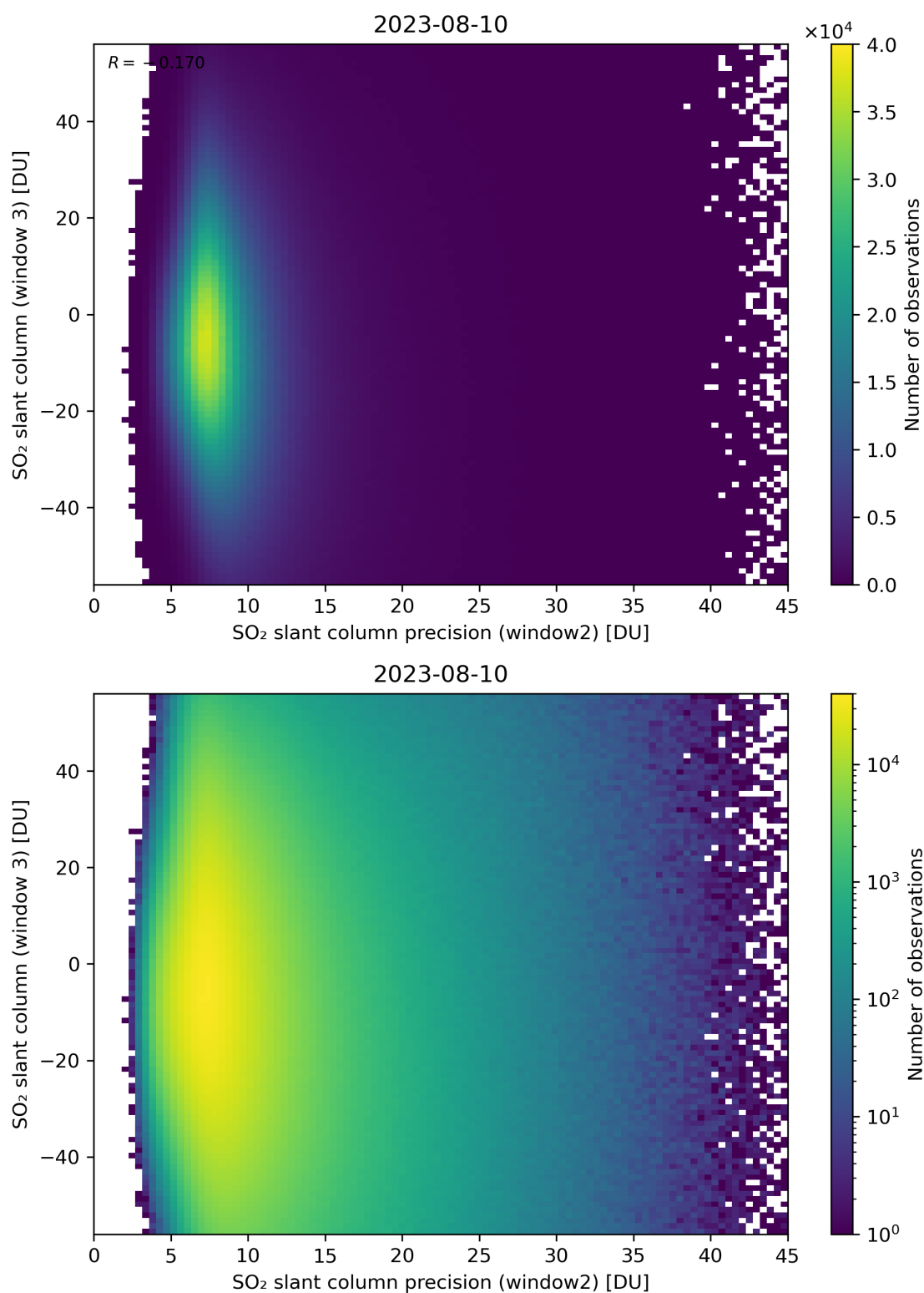
Figure 249: Scatter density plot of “SO 2 slant column precision (window2)” against “SO 2 slant column (window 3)” for 2023-08-09 to 2023-08-11.
