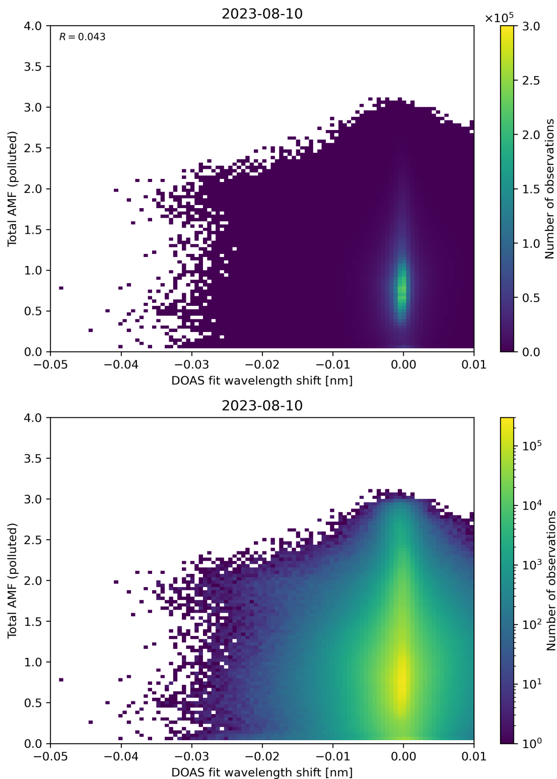
Figure 130: Scatter density plot of “DOAS fit wavelength shift” against “Total AMF (polluted)” for 2023-08-09 to 2023-08-11.
