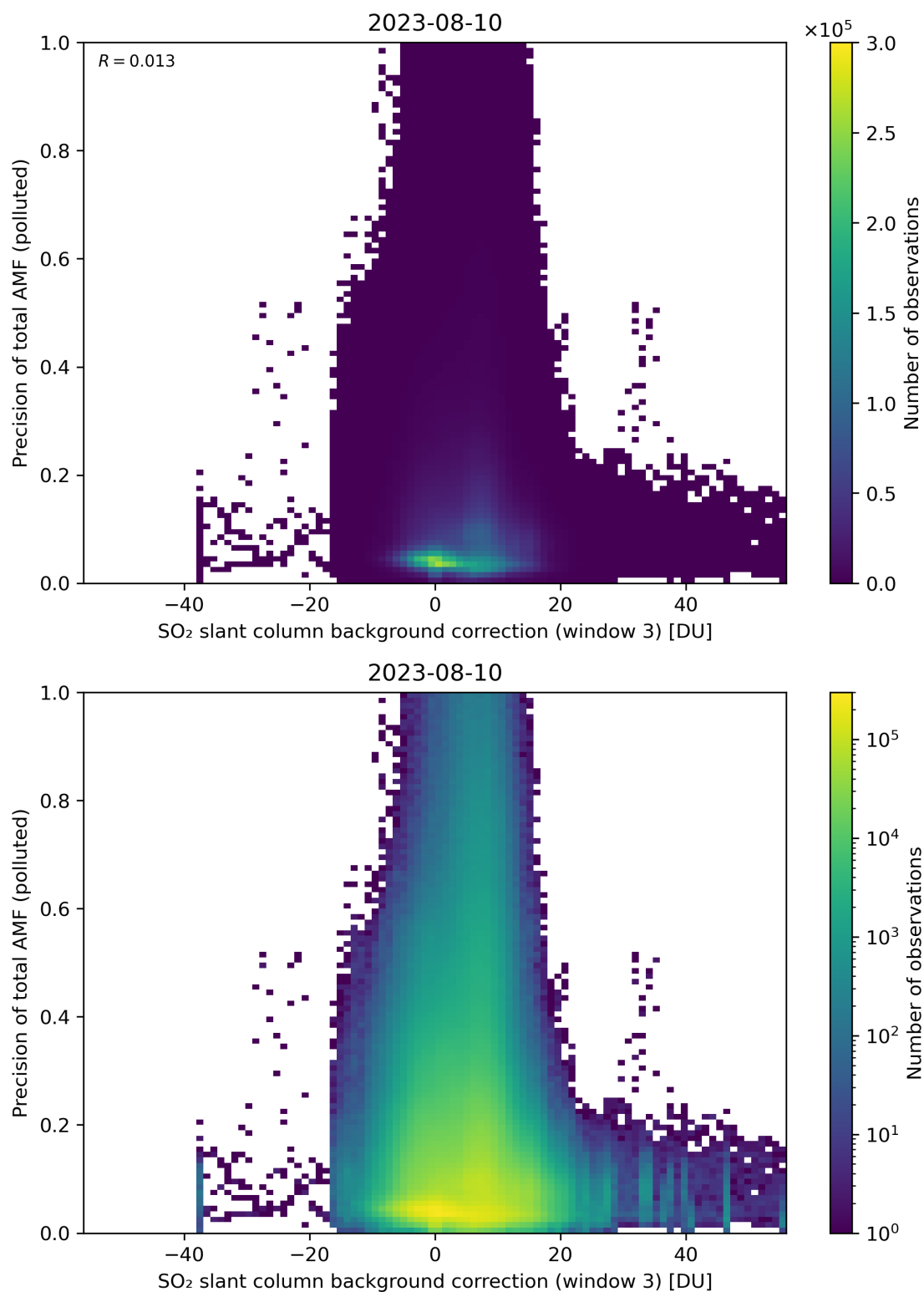
Figure 126: Scatter density plot of “SO 2 slant column background correction (window 3)” against “Precision of total AMF (polluted)” for 2023-08-09 to 2023-08-11.
