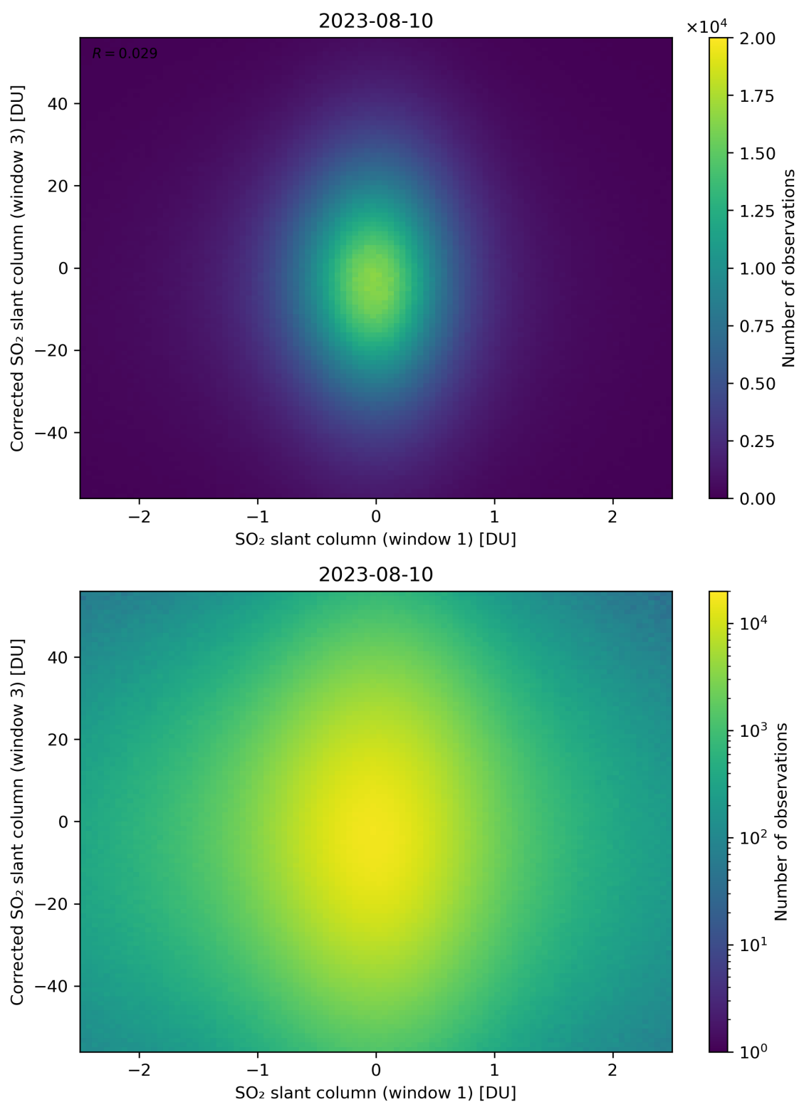
Figure 234: Scatter density plot of “SO 2 slant column (window 1)” against “Corrected SO 2 slant column (window 3)” for 2023-08-09 to 2023-08-11.
