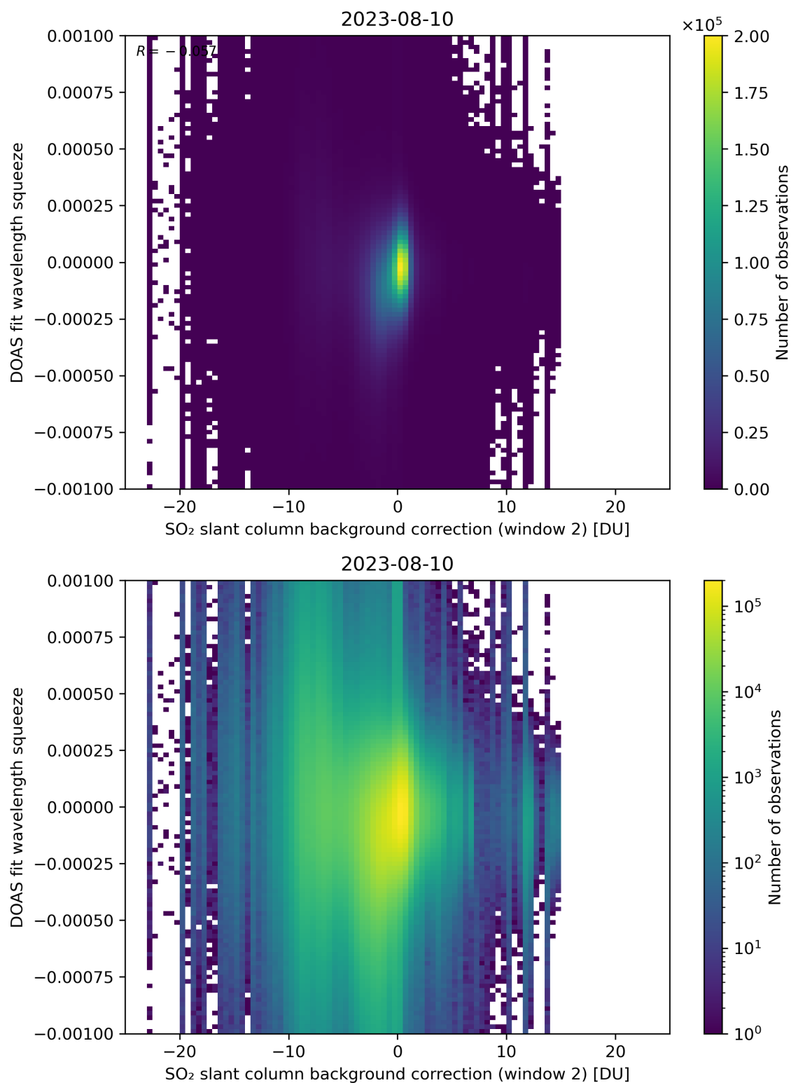
Figure 113: Scatter density plot of “SO 2 slant column background correction (window 2)” against “DOAS fit wavelength squeeze” for 2023-08-09 to 2023-08-11.
