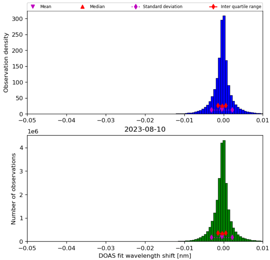
Figure 68: Histogram of “DOAS fit wavelength shift” for 2023-08-09 to 2023-08-11
