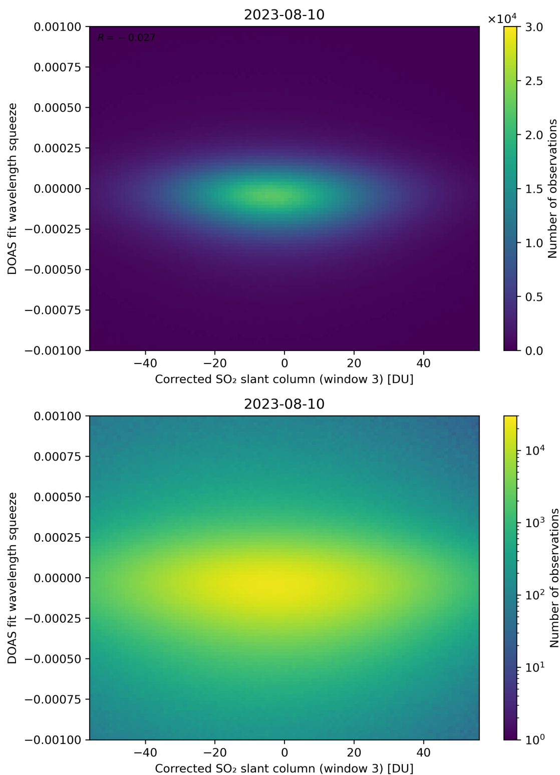
Figure 207: Scatter density plot of “Corrected SO 2 slant column (window 3)” against “DOAS fit wavelength squeeze” for 2023-08-09 to 2023-08-11.
