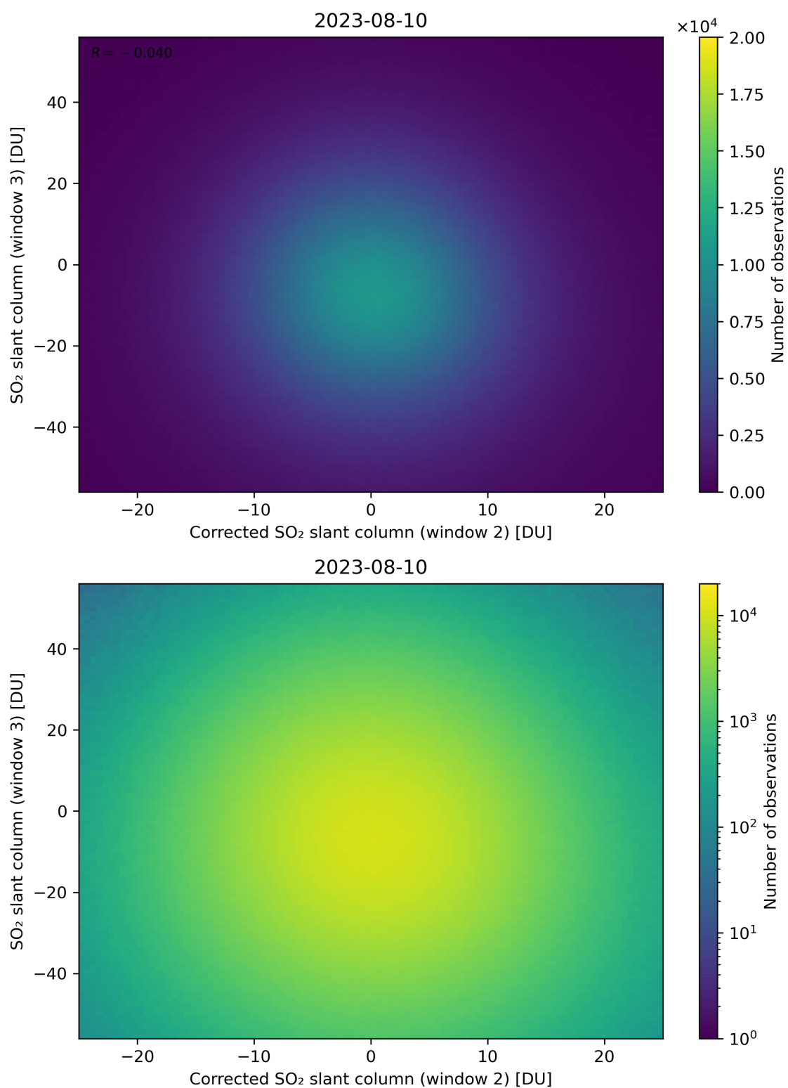
Figure 201: Scatter density plot of “Corrected SO 2 slant column (window 2)” against “SO 2 slant column (window 3)” for 2023-08-09 to 2023-08-11.
