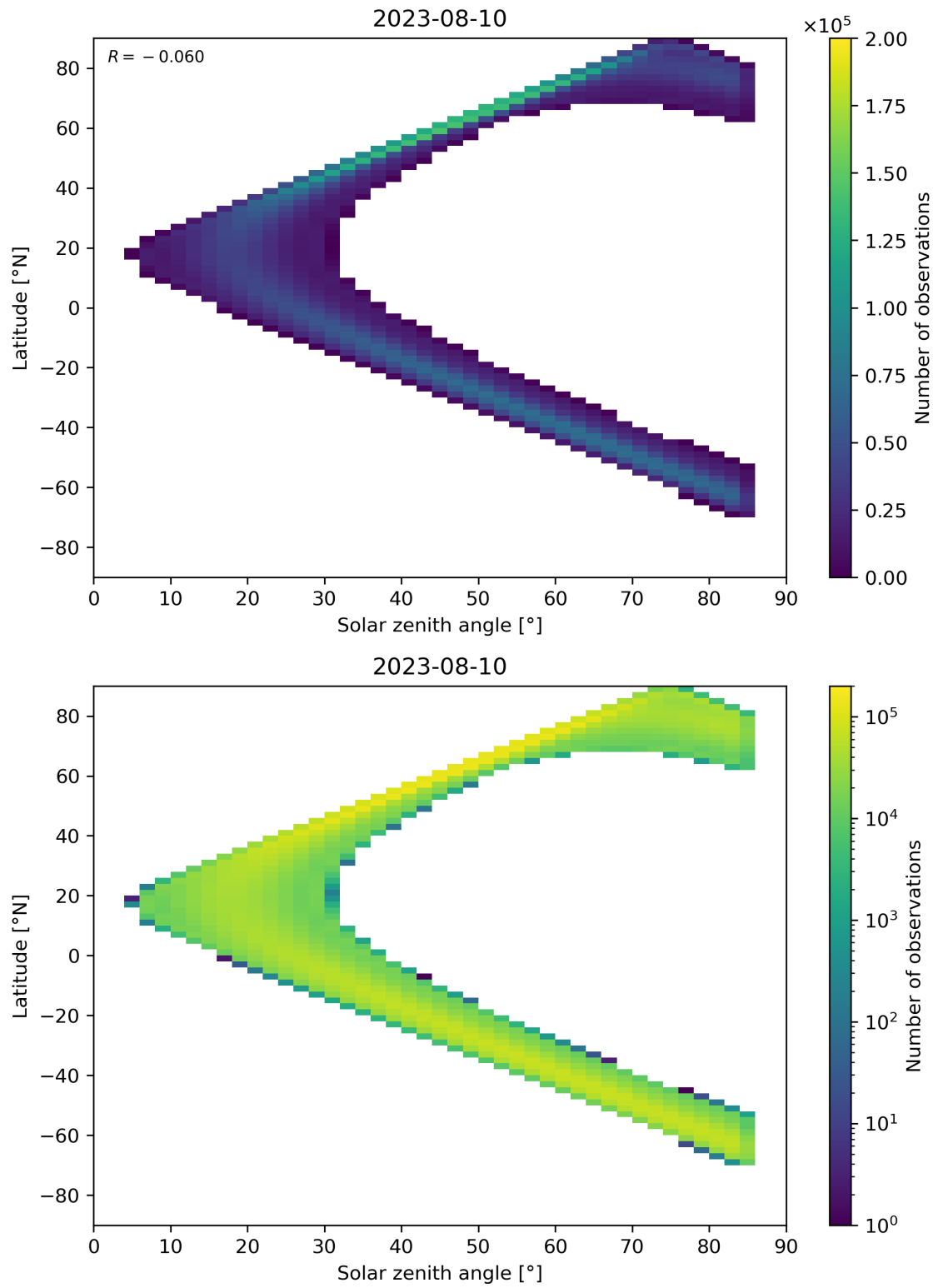
Figure 164: Scatter density plot of “Solar zenith angle” against “Latitude” for 2023-08-09 to 2023-08-11.
