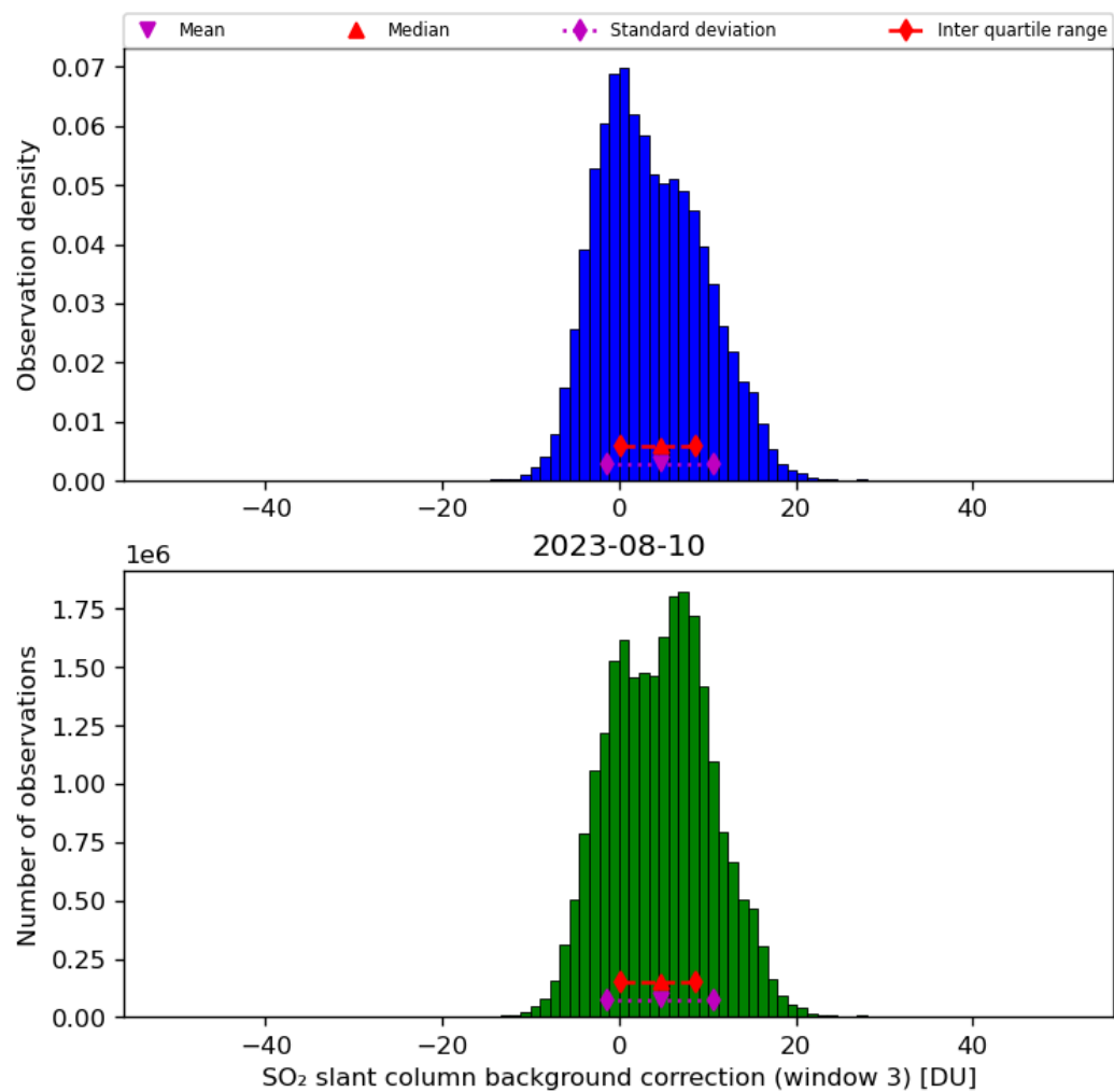
Figure 67: Histogram of “SO 2 slant column background correction (window 3)” for 2023-08-09 to 2023-08-11
