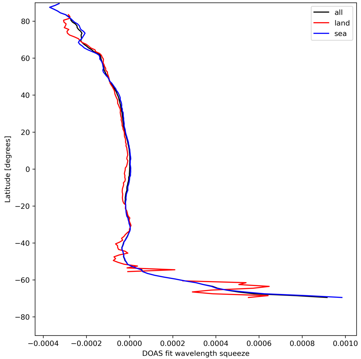
Figure 46: Zonal average of “DOAS fit wavelength squeeze” for 2023-08-09 to 2023-08-11.
