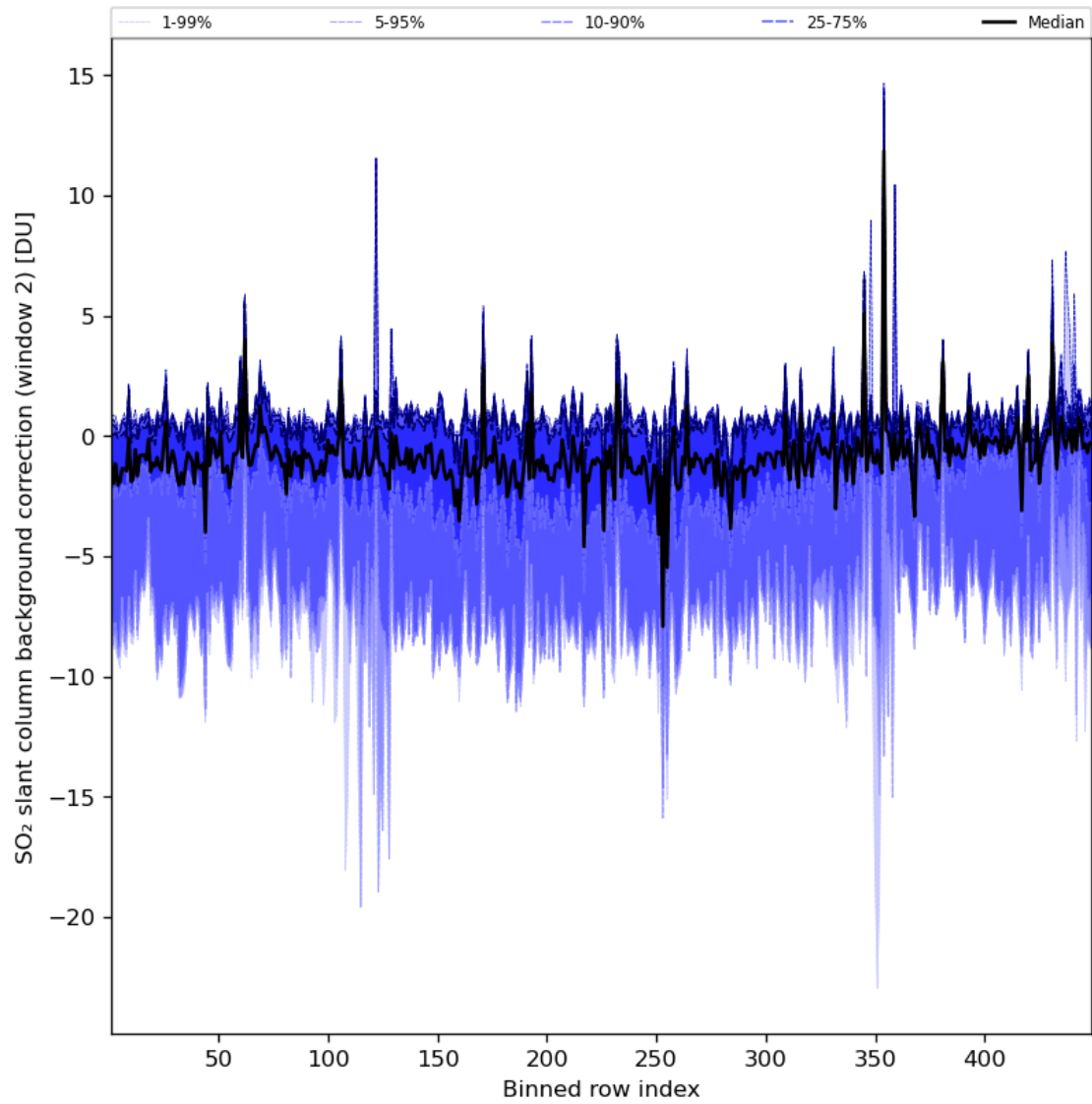
Figure 86: Along track statistics of “SO 2 slant column background correction (window 2)” for 2023-08-09 to 2023-08-11
