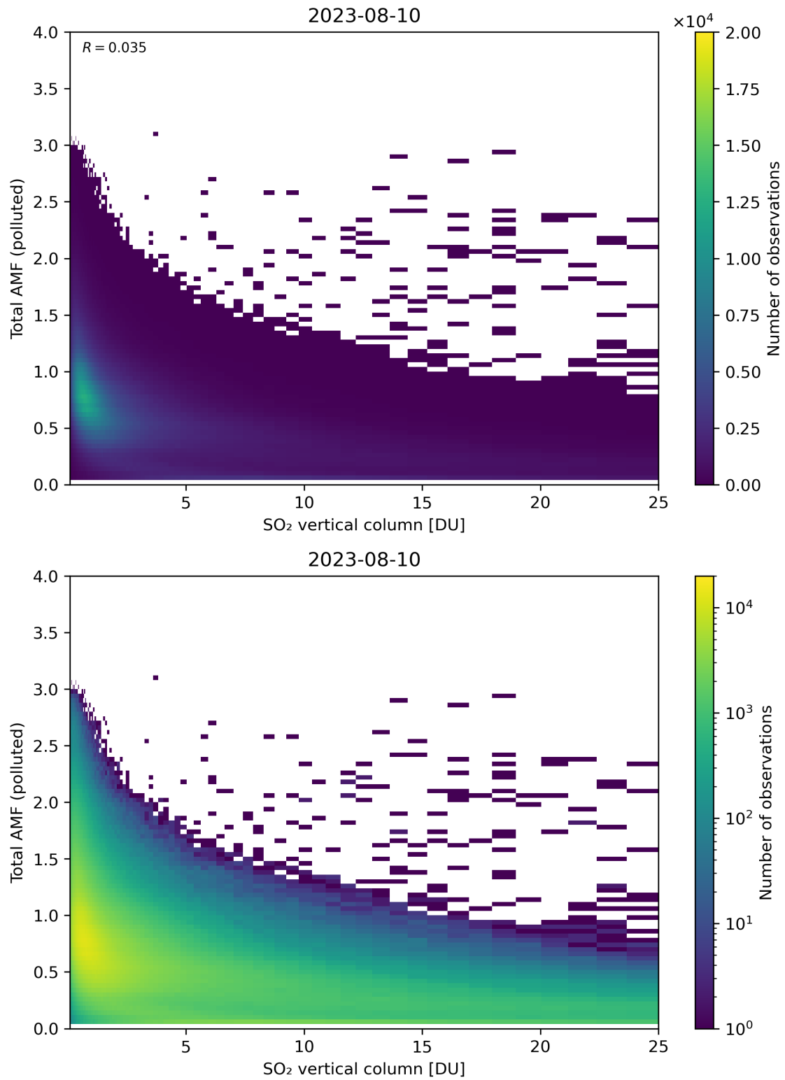
Figure 305: Scatter density plot of “SO 2 vertical column” against “Total AMF (polluted)” for 2023-08-09 to 2023-08-11.
