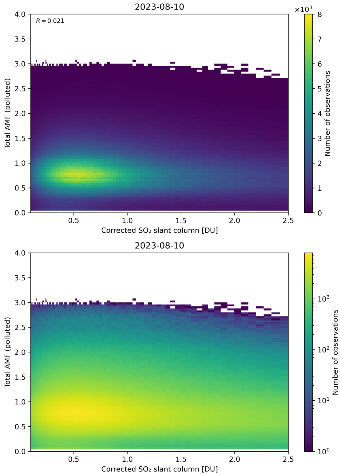
Figure 192: Scatter density plot of “Corrected SO 2 slant column” against “Total AMF (polluted)” for 2023-08-09 to 2023-08-11.
