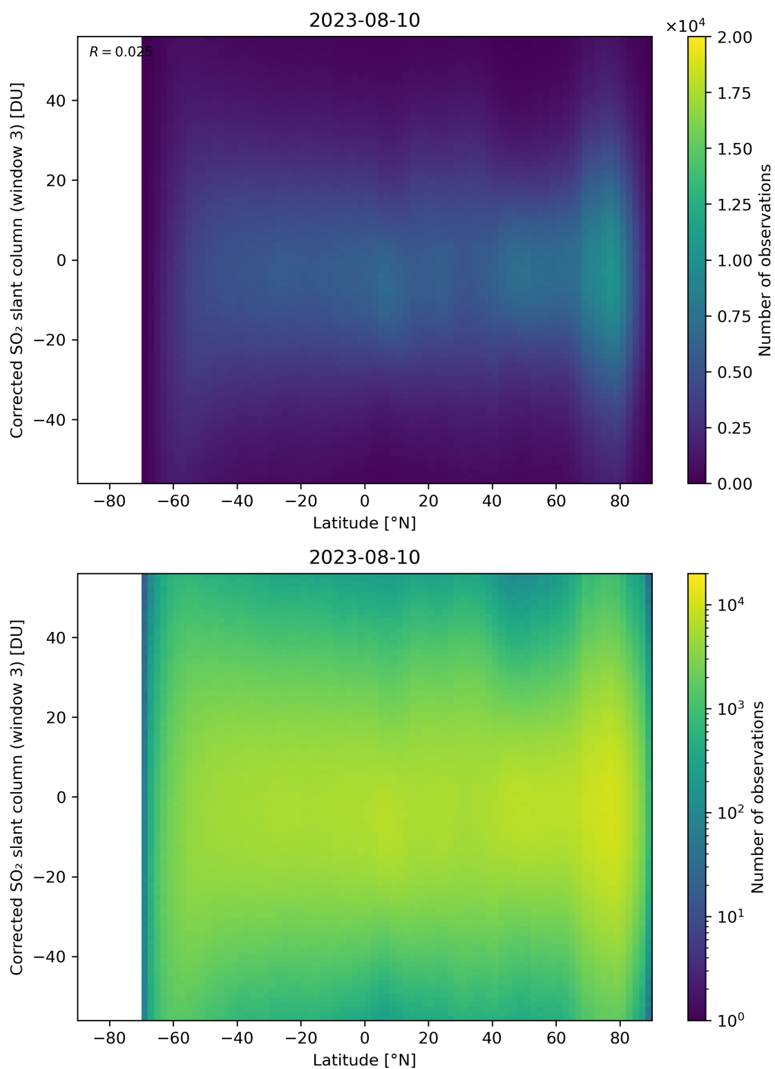
Figure 148: Scatter density plot of “Latitude” against “Corrected SO 2 slant column (window 3)” for 2023-08-09 to 2023-08-11.
