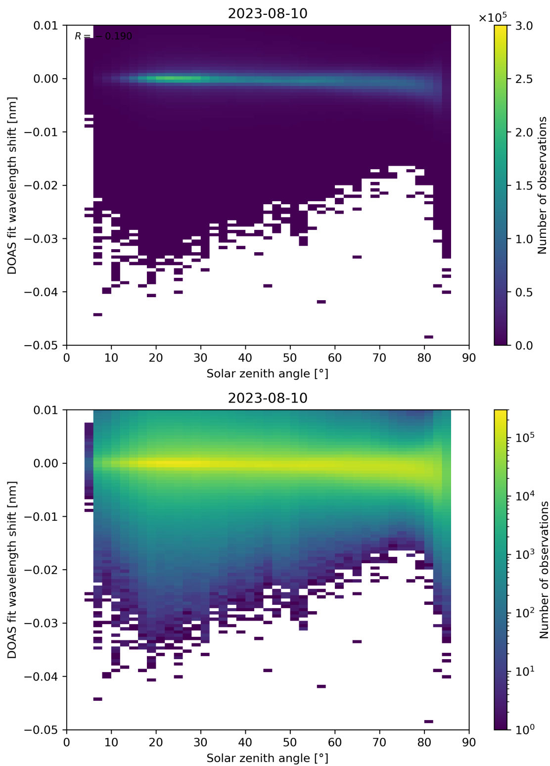
Figure 161: Scatter density plot of “Solar zenith angle” against “DOAS fit wavelength shift” for 2023-08-09 to 2023-08-11.
