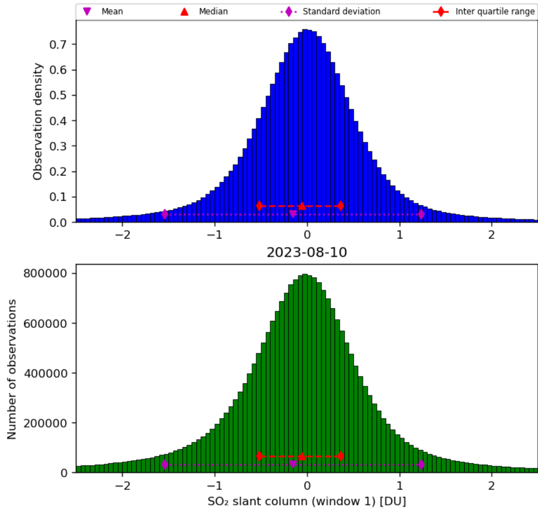
Figure 56: Histogram of “SO 2 slant column (window 1)” for 2023-08-09 to 2023-08-11
