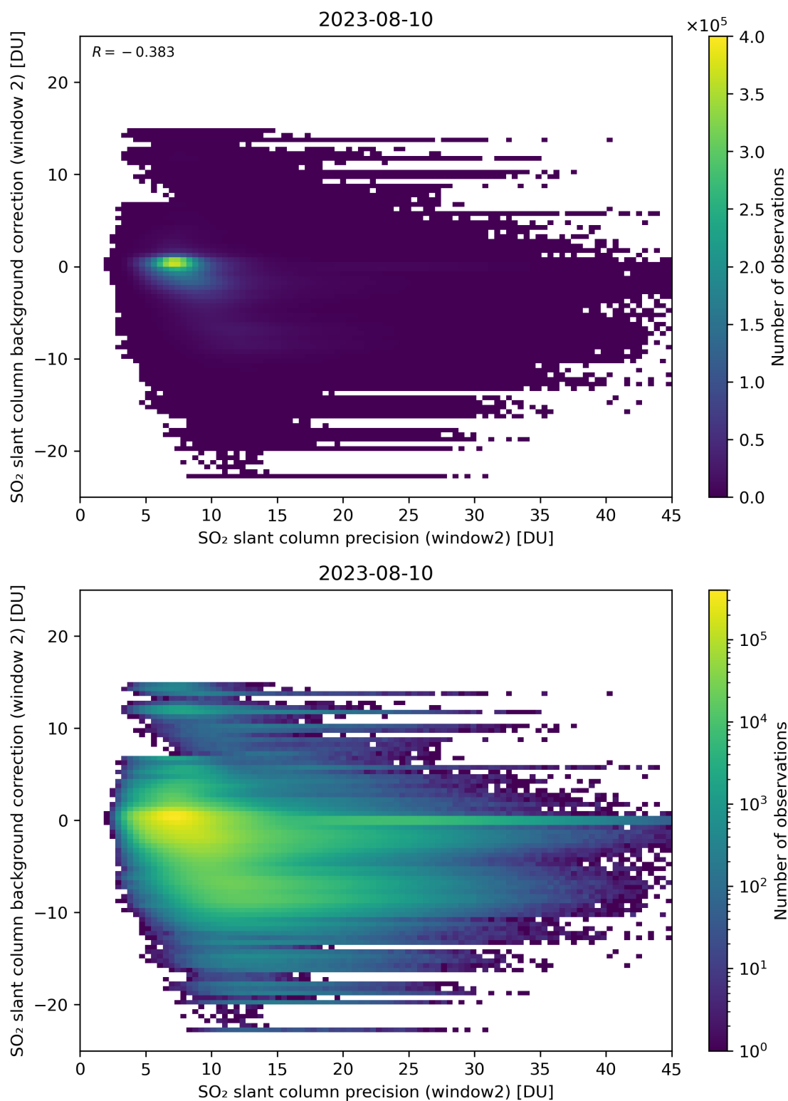
Figure 241: Scatter density plot of “SO 2 slant column precision (window2)” against “SO 2 slant column background correction (window 2)” for 2023-08-09 to 2023-08-11.
