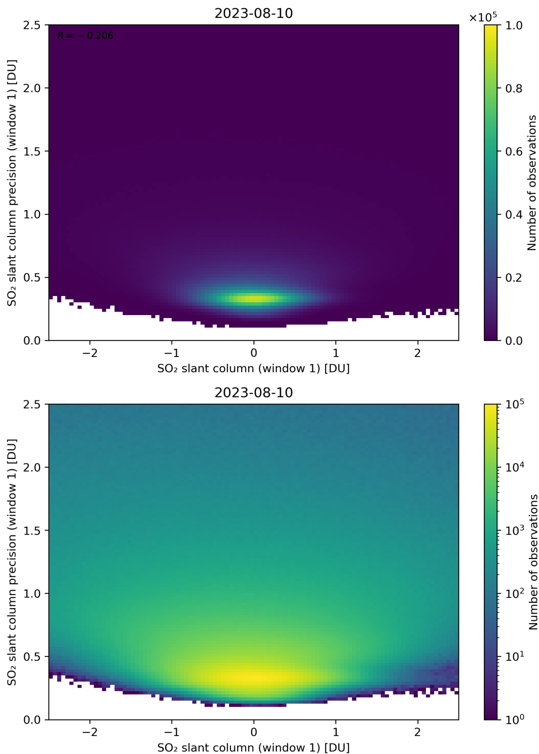
Figure 235: Scatter density plot of “SO 2 slant column (window 1)” against “SO 2 slant column precision (window 1)” for 2023-08-09 to 2023-08-11.
