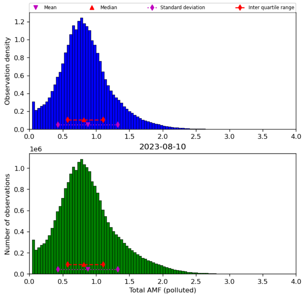
Figure 71: Histogram of “Total AMF (polluted)” for 2023-08-09 to 2023-08-11
