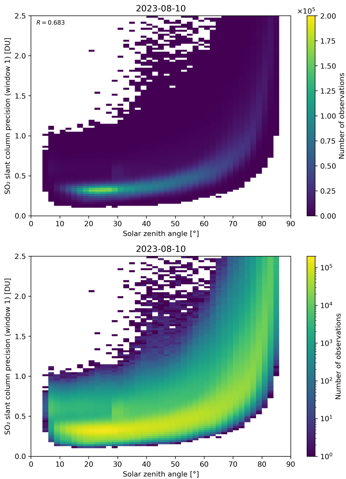
Figure 170: Scatter density plot of “Solar zenith angle” against “SO 2 slant column precision (window 1)” for 2023-08-09 to 2023-08-11.
