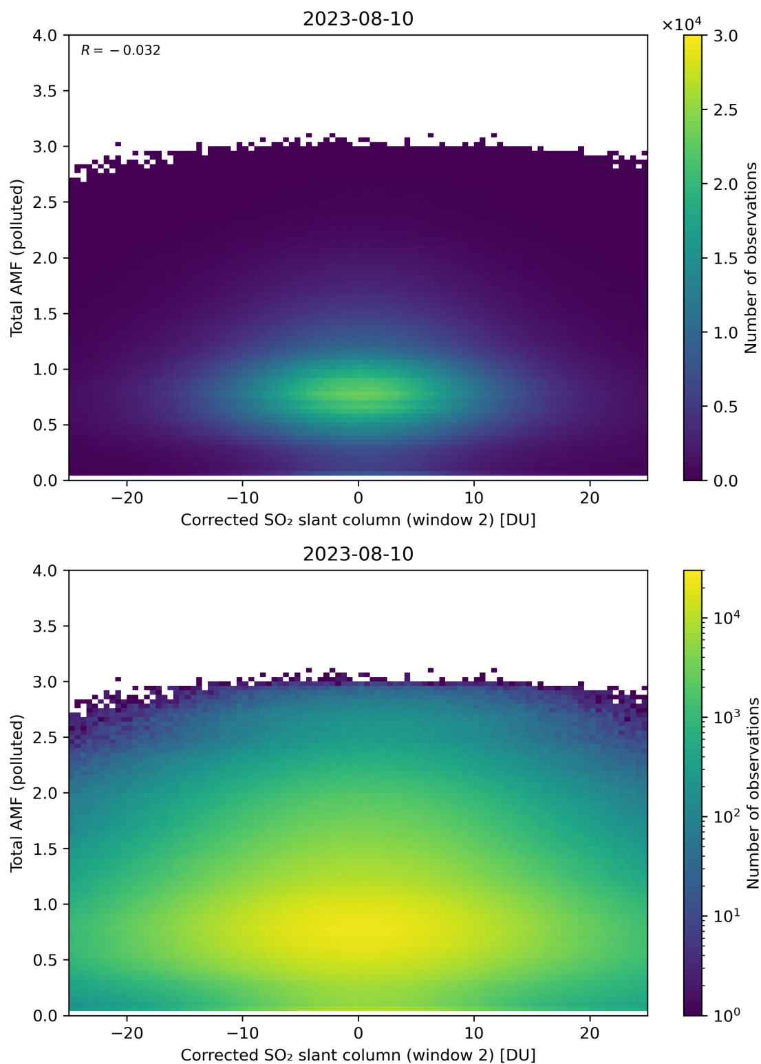
Figure 203: Scatter density plot of “Corrected SO 2 slant column (window 2)” against “Total AMF (polluted)” for 2023-08-09 to 2023-08-11.
