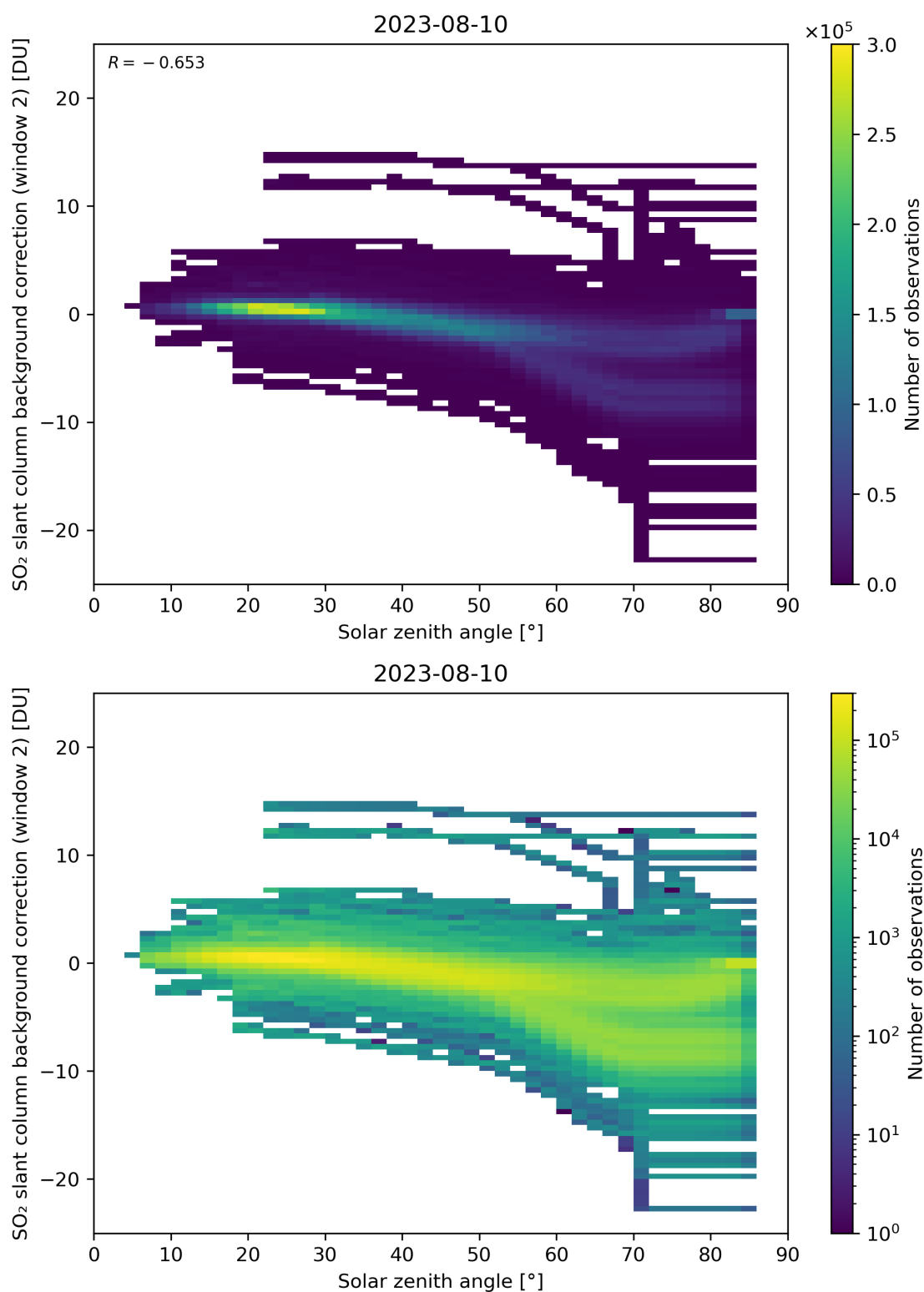
Figure 159: Scatter density plot of “Solar zenith angle” against “SO 2 slant column background correction (window 2)” for 2023-08-09 to 2023-08-11.
