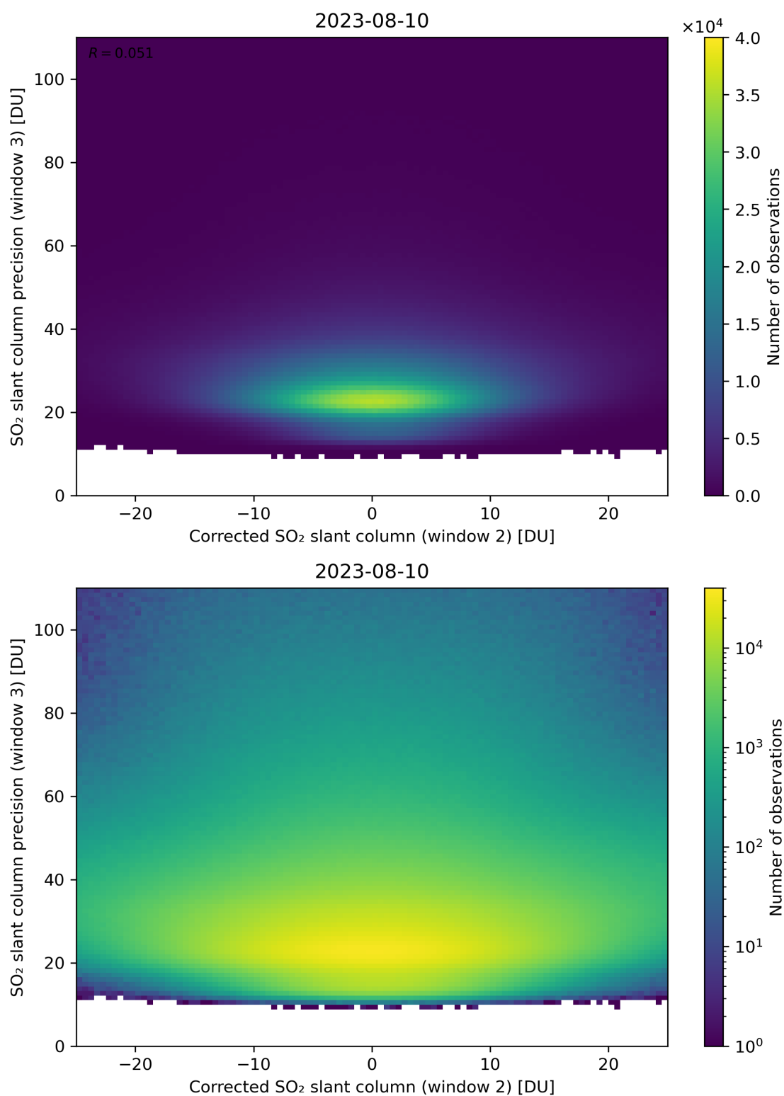
Figure 202: Scatter density plot of “Corrected SO 2 slant column (window 2)” against “SO 2 slant column precision (window 3)” for 2023-08-09 to 2023-08-11.
