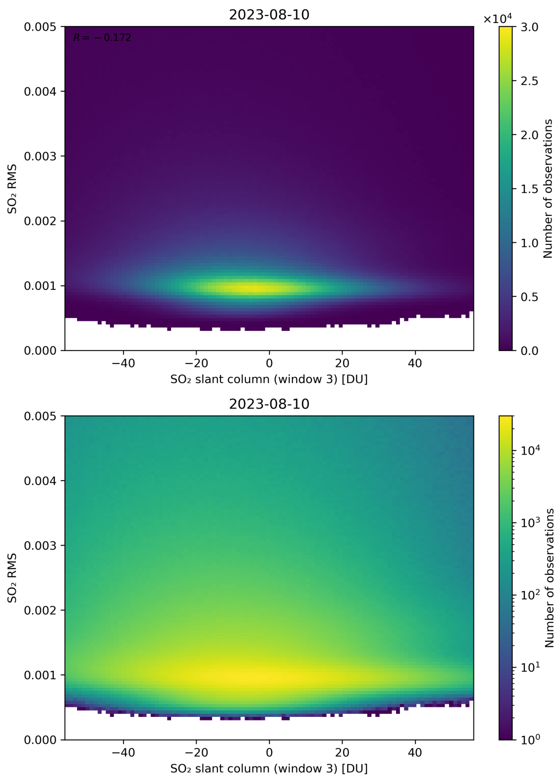
Figure 256: Scatter density plot of “SO 2 slant column (window 3)” against “SO 2 RMS” for 2023-08-09 to 2023-08-11.
