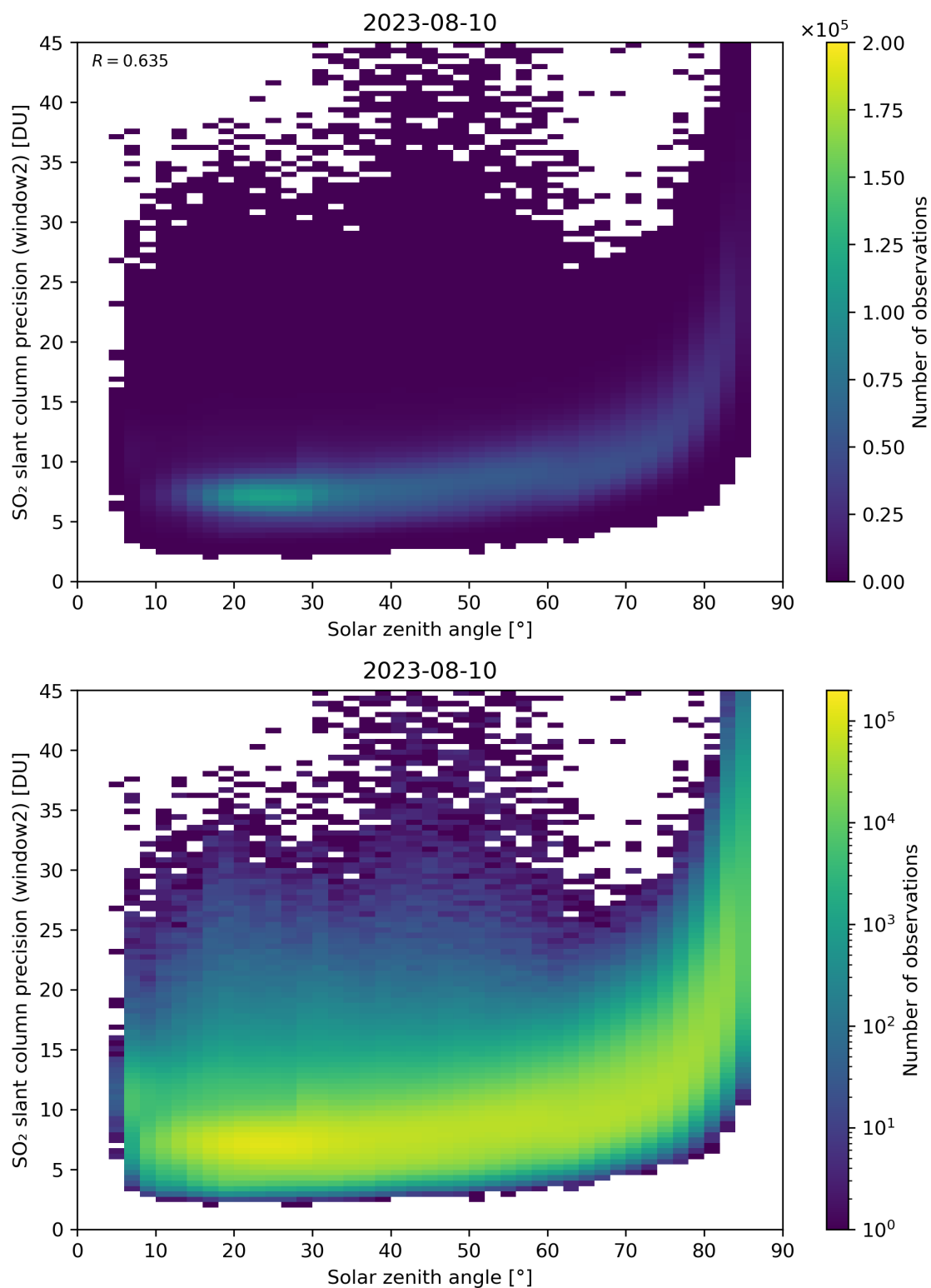
Figure 171: Scatter density plot of “Solar zenith angle” against “SO 2 slant column precision (window2)” for 2023-08-09 to 2023-08-11.
