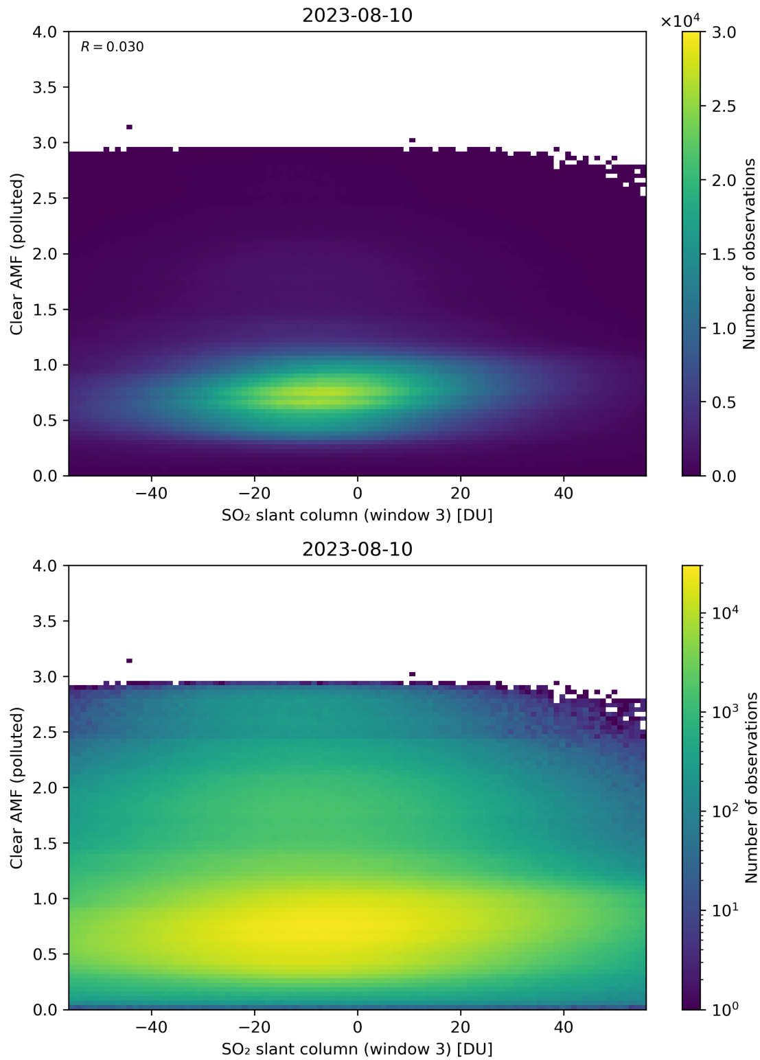
Figure 265: Scatter density plot of “SO 2 slant column (window 3)” against “Clear AMF (polluted)” for 2023-08-09 to 2023-08-11.
