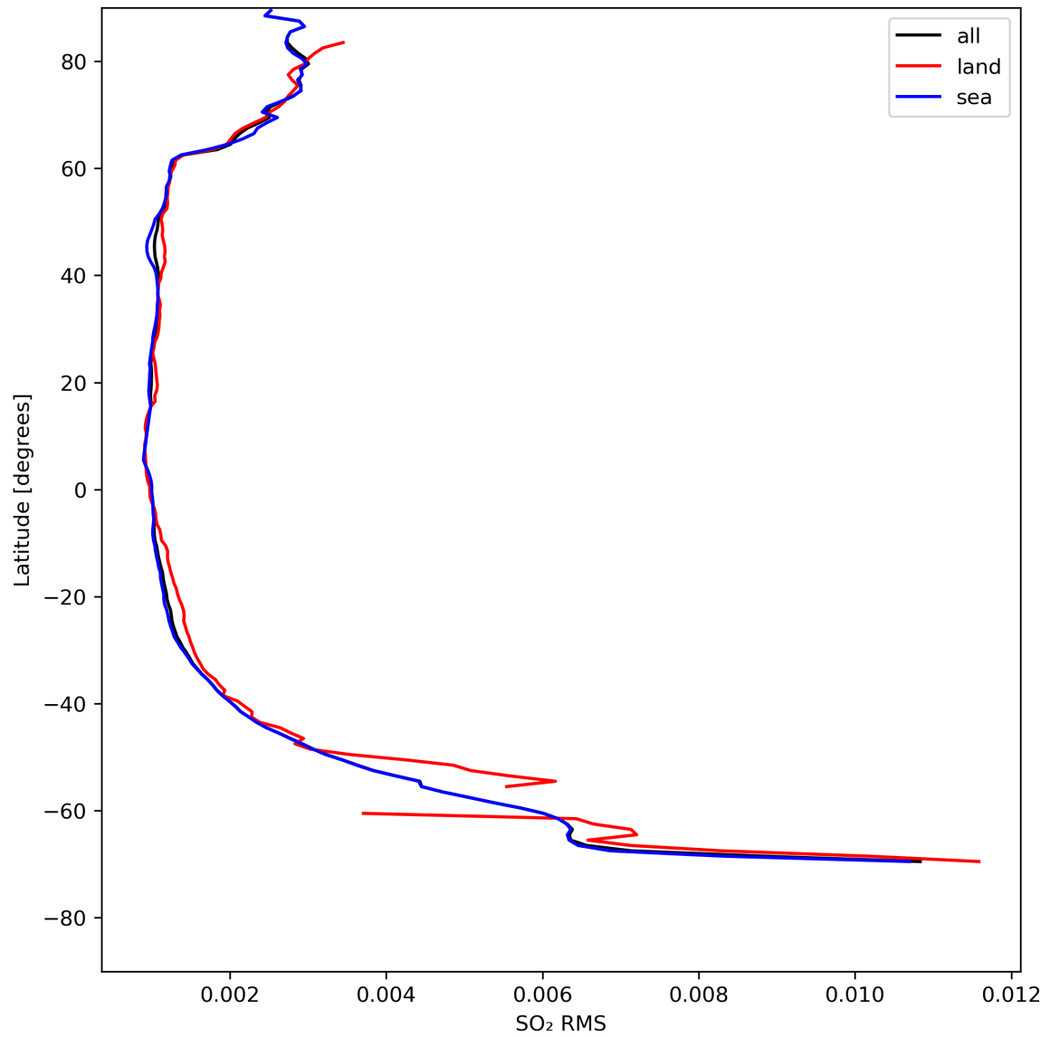
Figure 47: Zonal average of “SO 2 RMS” for 2023-08-09 to 2023-08-11.
