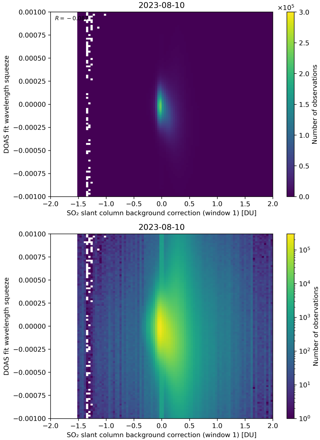
Figure 101: Scatter density plot of “SO 2 slant column background correction (window 1)” against “DOAS fit wavelength squeeze” for 2023-08-09 to 2023-08-11.
