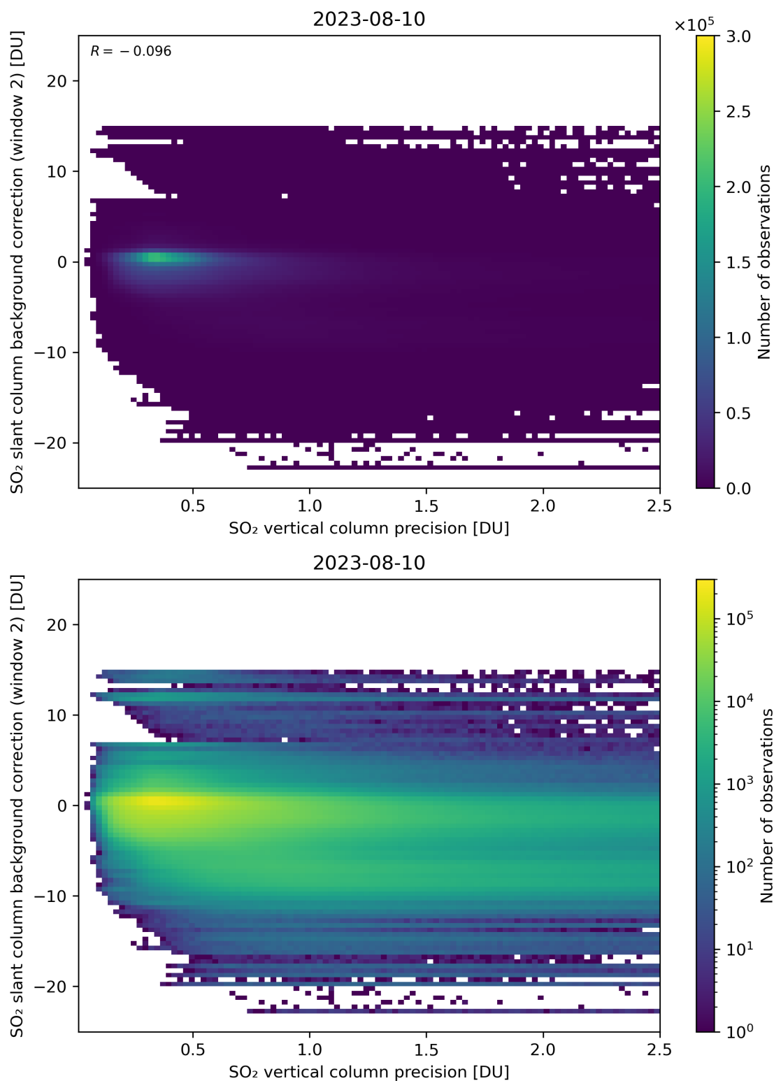
Figure 280: Scatter density plot of “SO 2 vertical column precision” against “SO 2 slant column background correction (window 2)” for 2023-08-09 to 2023-08-11.
