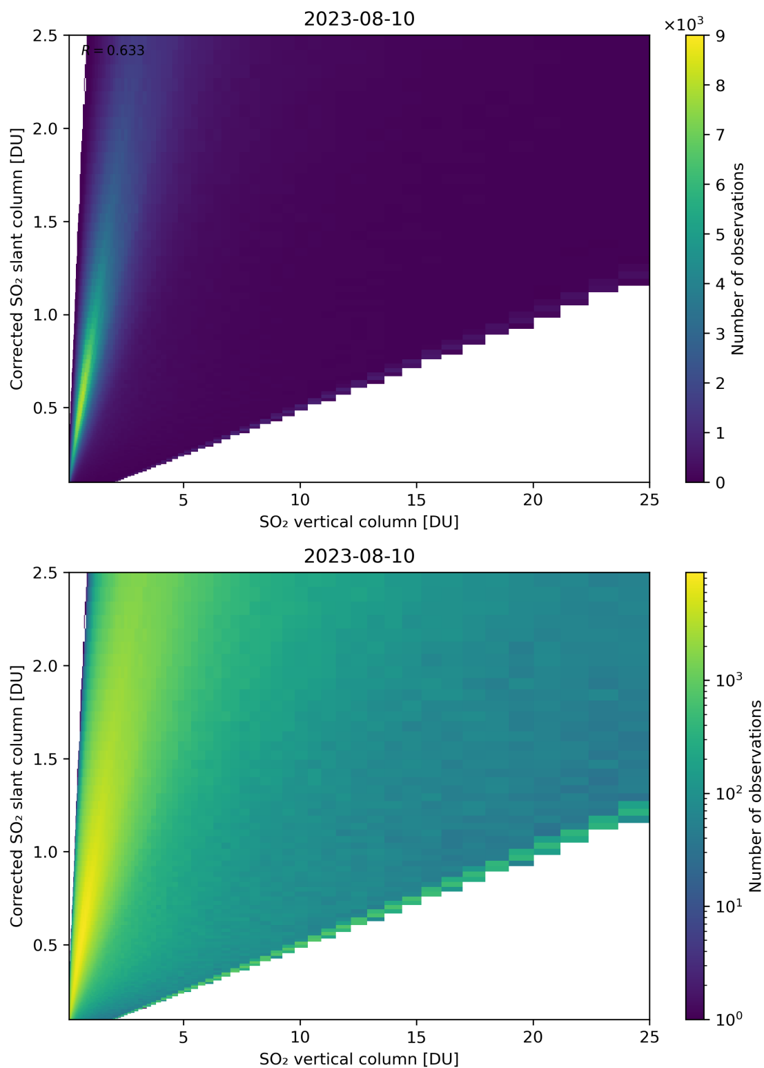
Figure 297: Scatter density plot of “SO 2 vertical column” against “Corrected SO 2 slant column” for 2023-08-09 to 2023-08-11.
