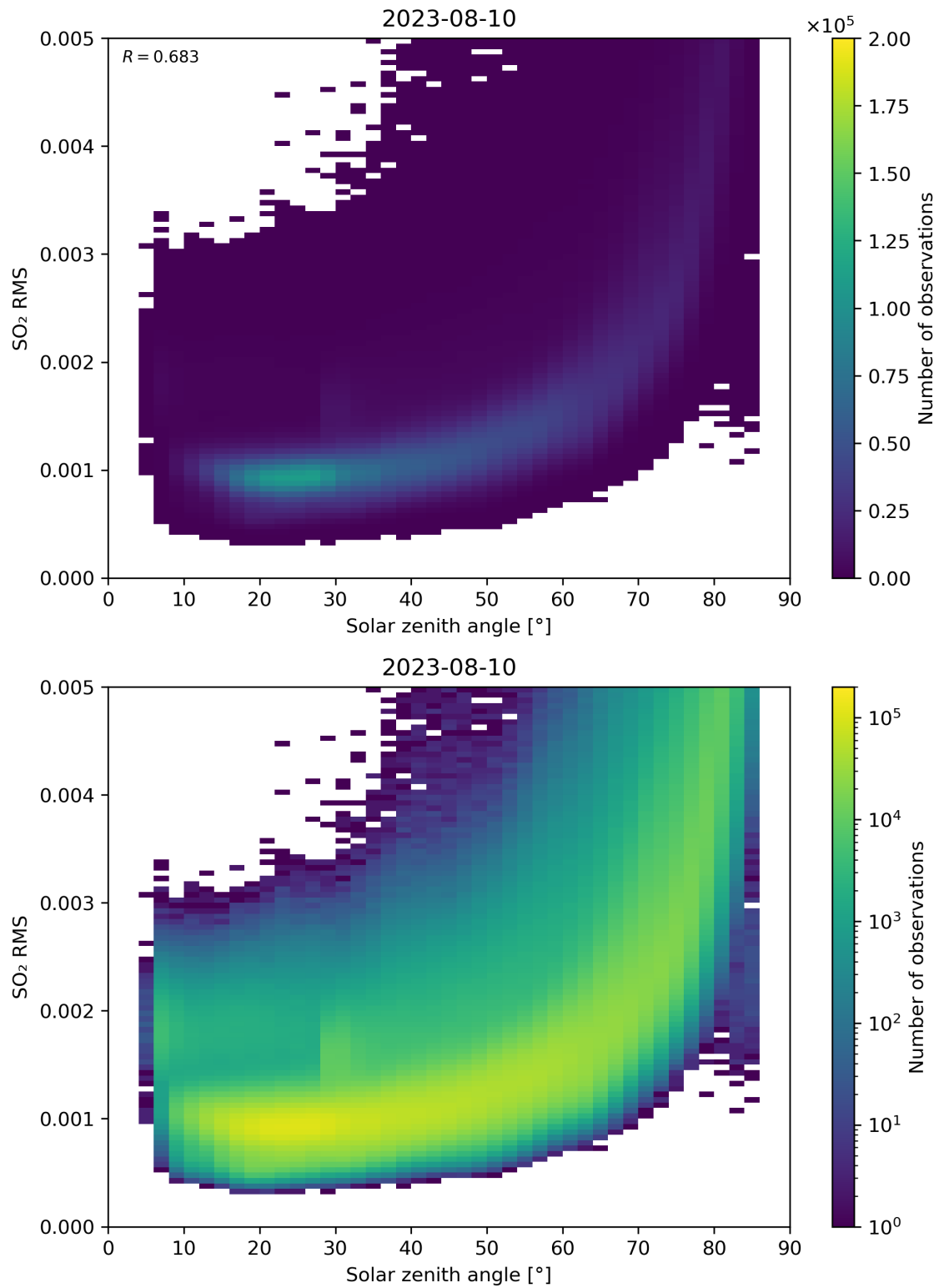
Figure 163: Scatter density plot of “Solar zenith angle” against “SO 2 RMS” for 2023-08-09 to 2023-08-11.
