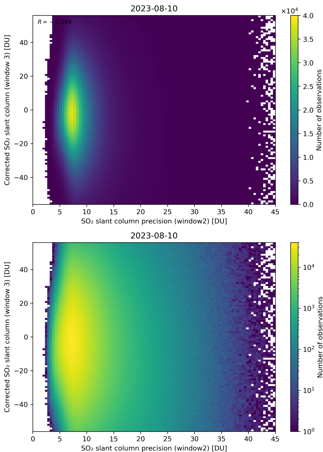
Figure 248: Scatter density plot of “SO 2 slant column precision (window2)” against “Corrected SO 2 slant column (window 3)” for 2023-08-09 to 2023-08-11.
