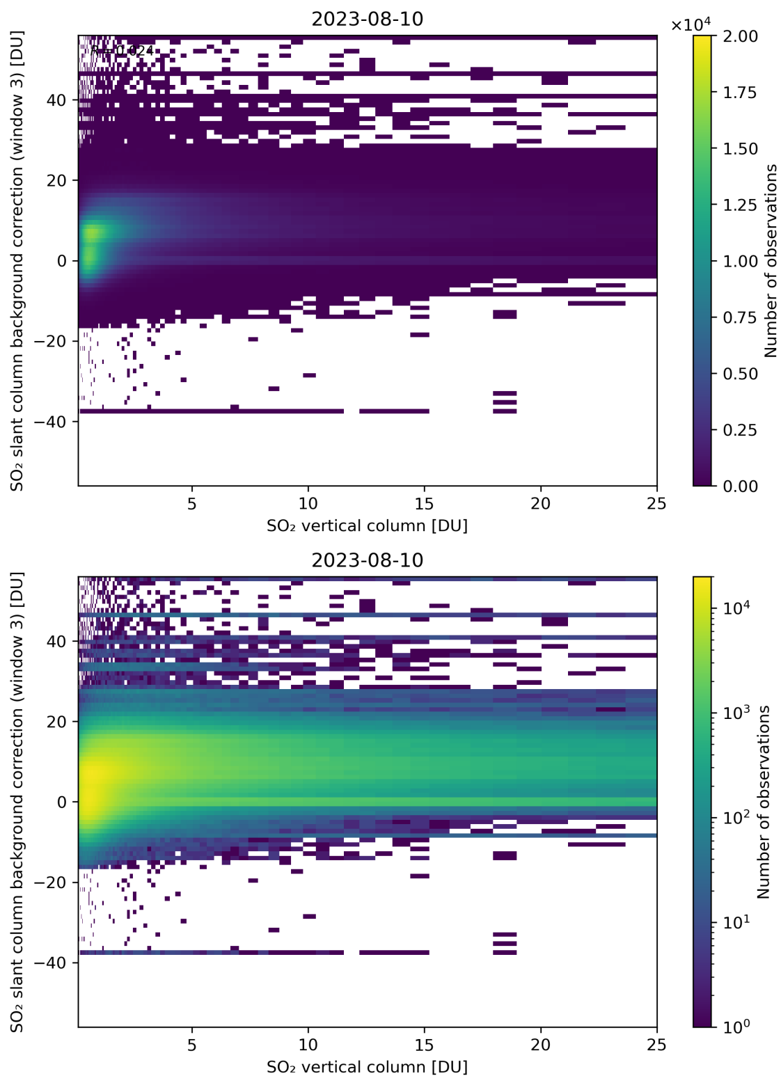
Figure 275: Scatter density plot of “SO 2 vertical column” against “SO 2 slant column background correction (window 3)” for 2023-08-09 to 2023-08-11.
