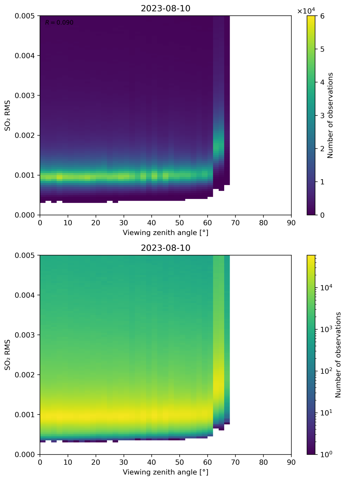
Figure 313: Scatter density plot of “Viewing zenith angle” against “SO 2 RMS” for 2023-08-09 to 2023-08-11.
