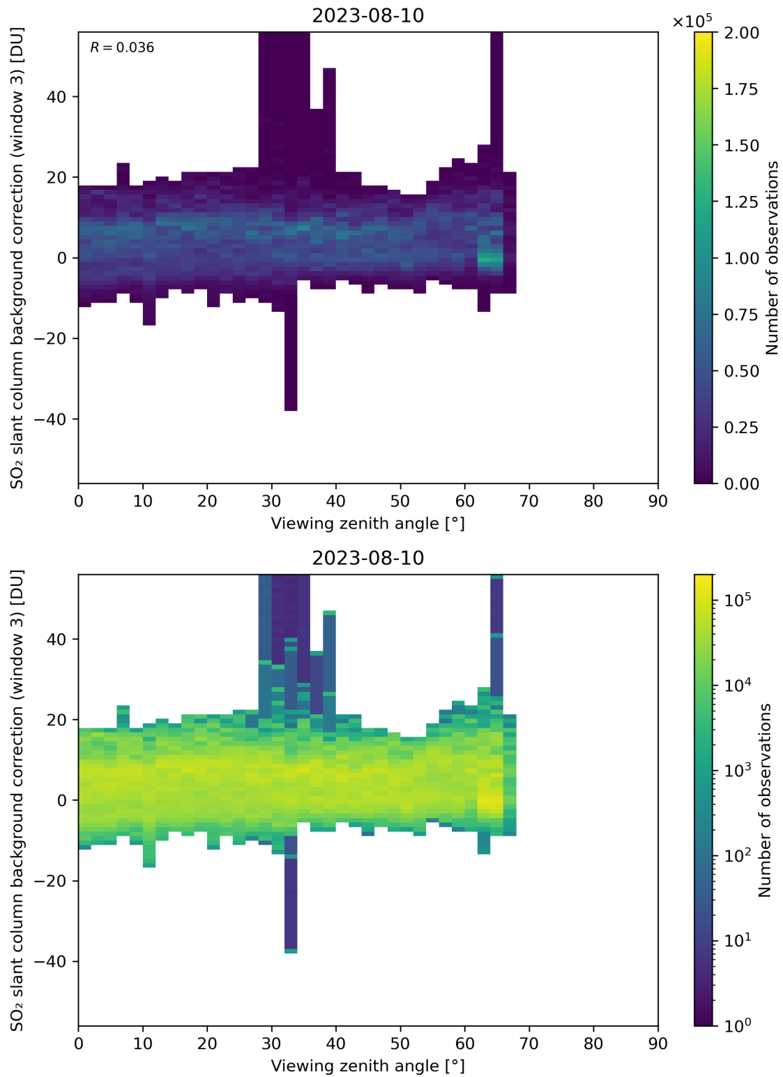
Figure 310: Scatter density plot of “Viewing zenith angle” against “SO 2 slant column background correction (window 3)” for 2023-08-09 to 2023-08-11.
