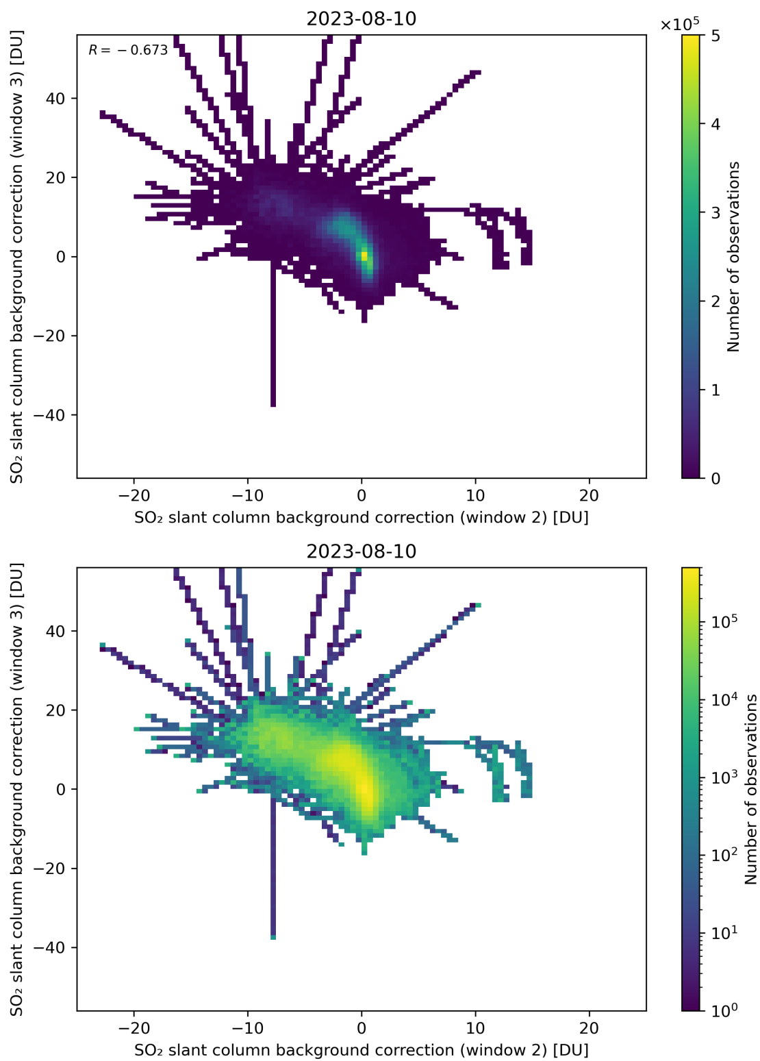
Figure 111: Scatter density plot of “SO 2 slant column background correction (window 2)” against “SO 2 slant column background correction (window 3)” for 2023-08-09 to 2023-08-11.
