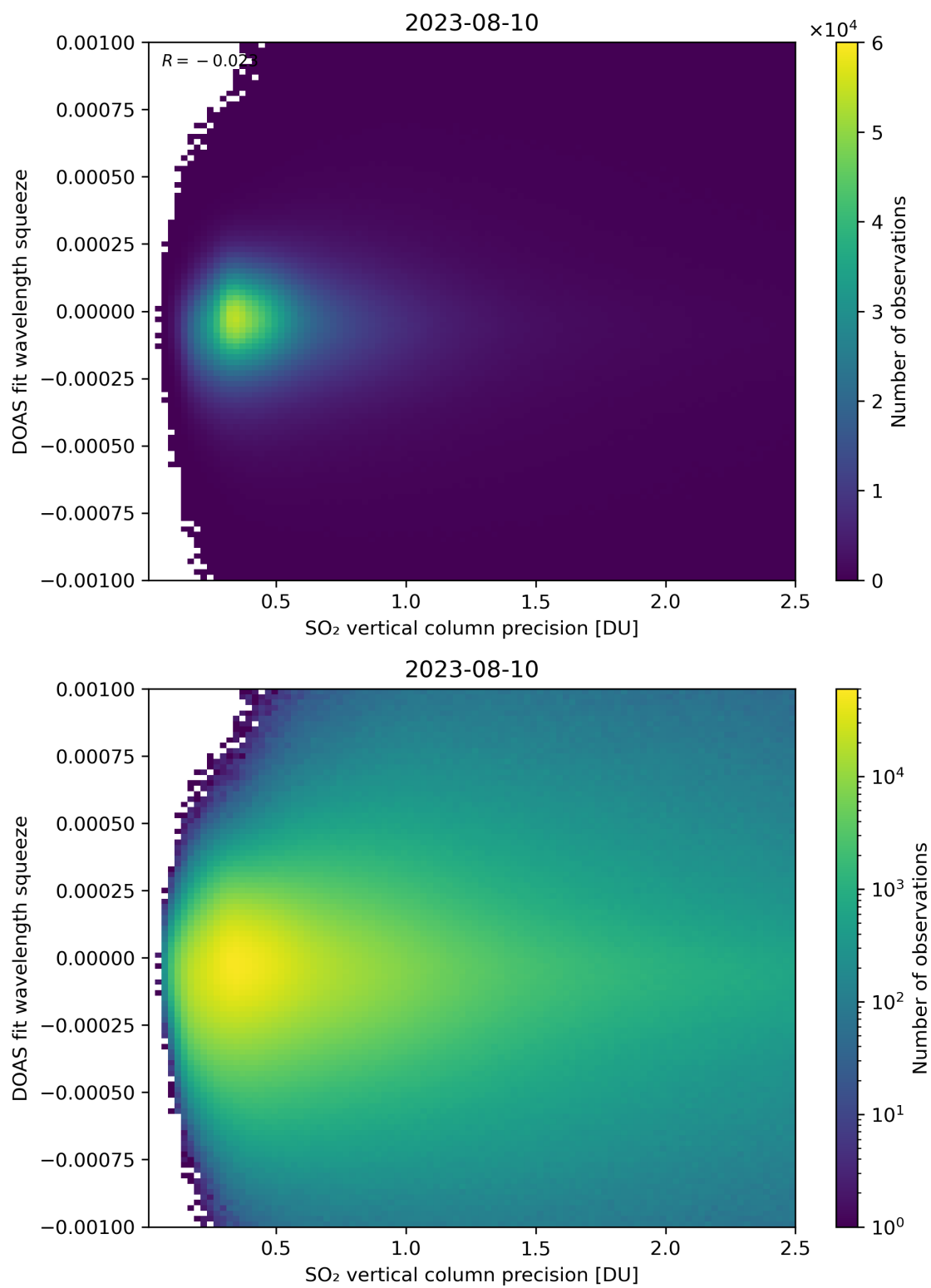
Figure 283: Scatter density plot of “SO 2 vertical column precision” against “DOAS fit wavelength squeeze” for 2023-08-09 to 2023-08-11.
