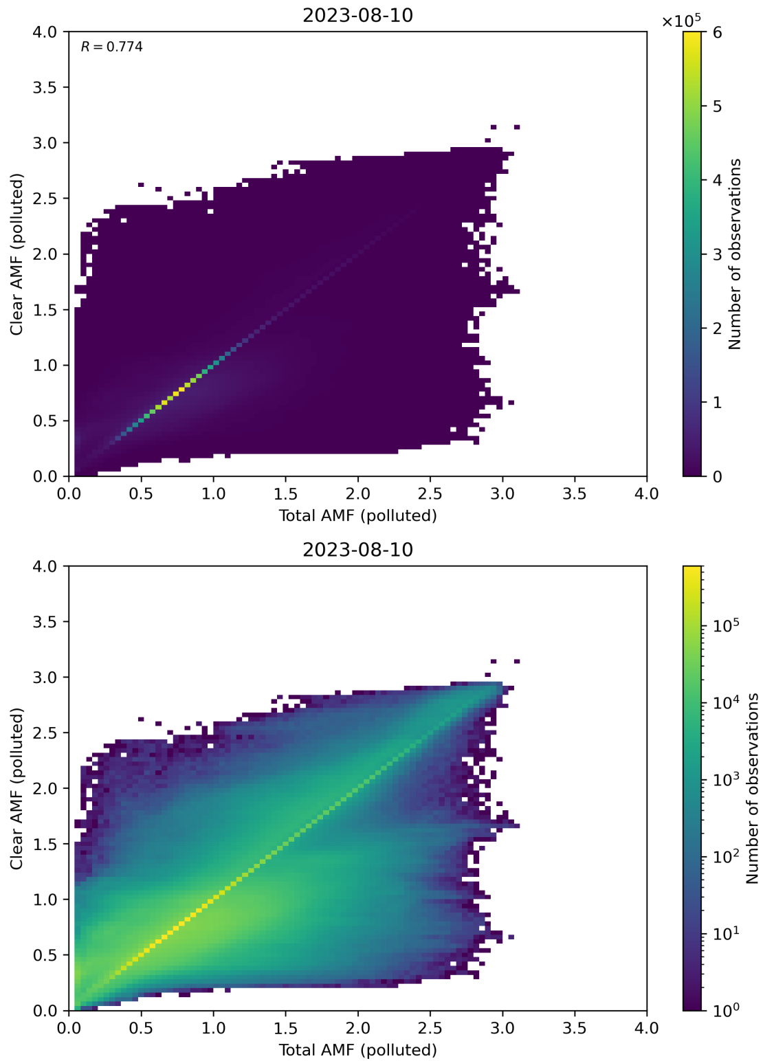
Figure 271: Scatter density plot of “Total AMF (polluted)” against “Clear AMF (polluted)” for 2023-08-09 to 2023-08-11.
