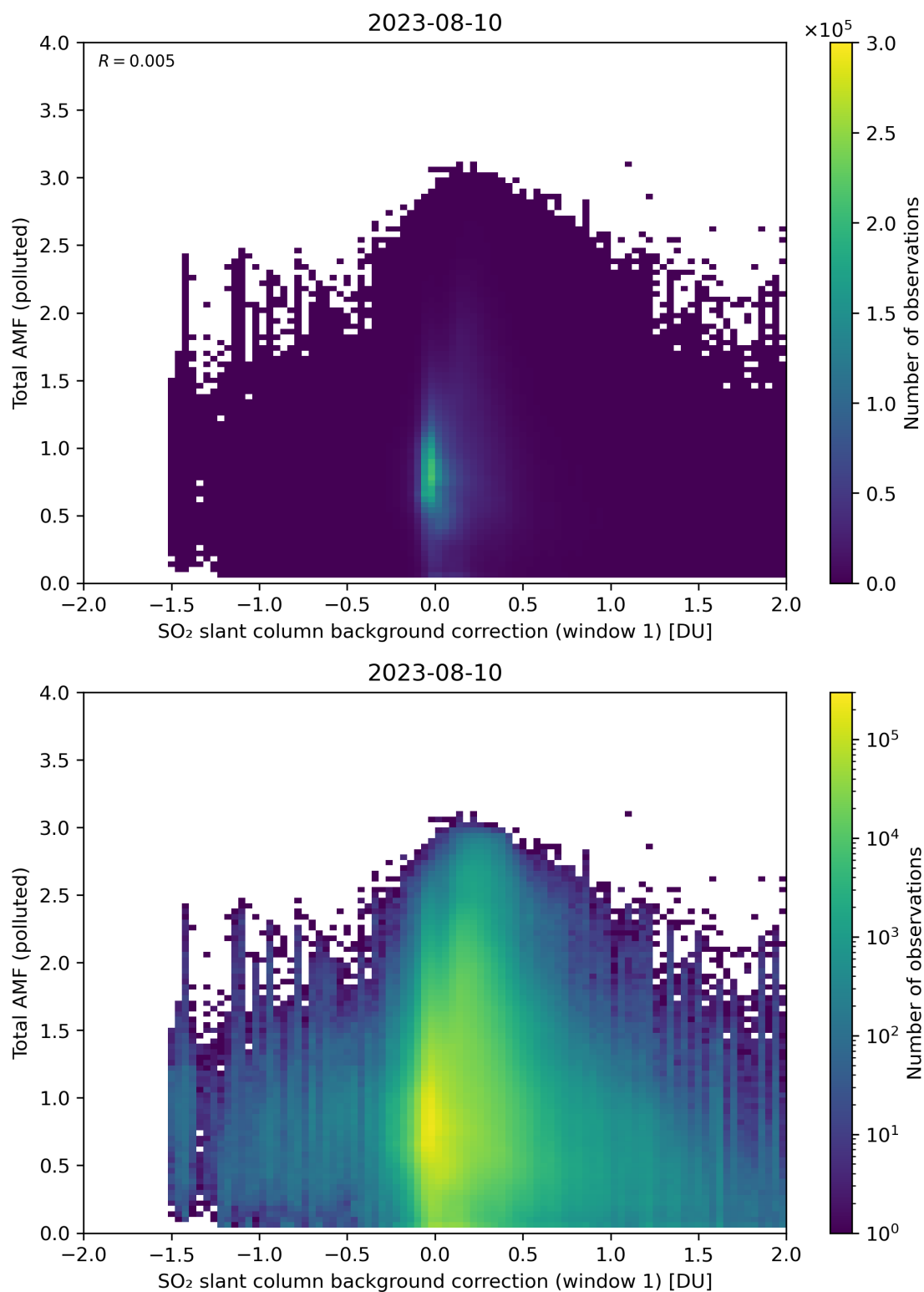
Figure 109: Scatter density plot of “SO 2 slant column background correction (window 1)” against “Total AMF (polluted)” for 2023-08-09 to 2023-08-11.
