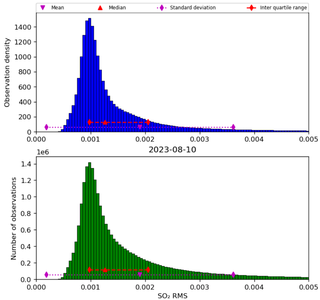
Figure 70: Histogram of “SO 2 RMS” for 2023-08-09 to 2023-08-11
