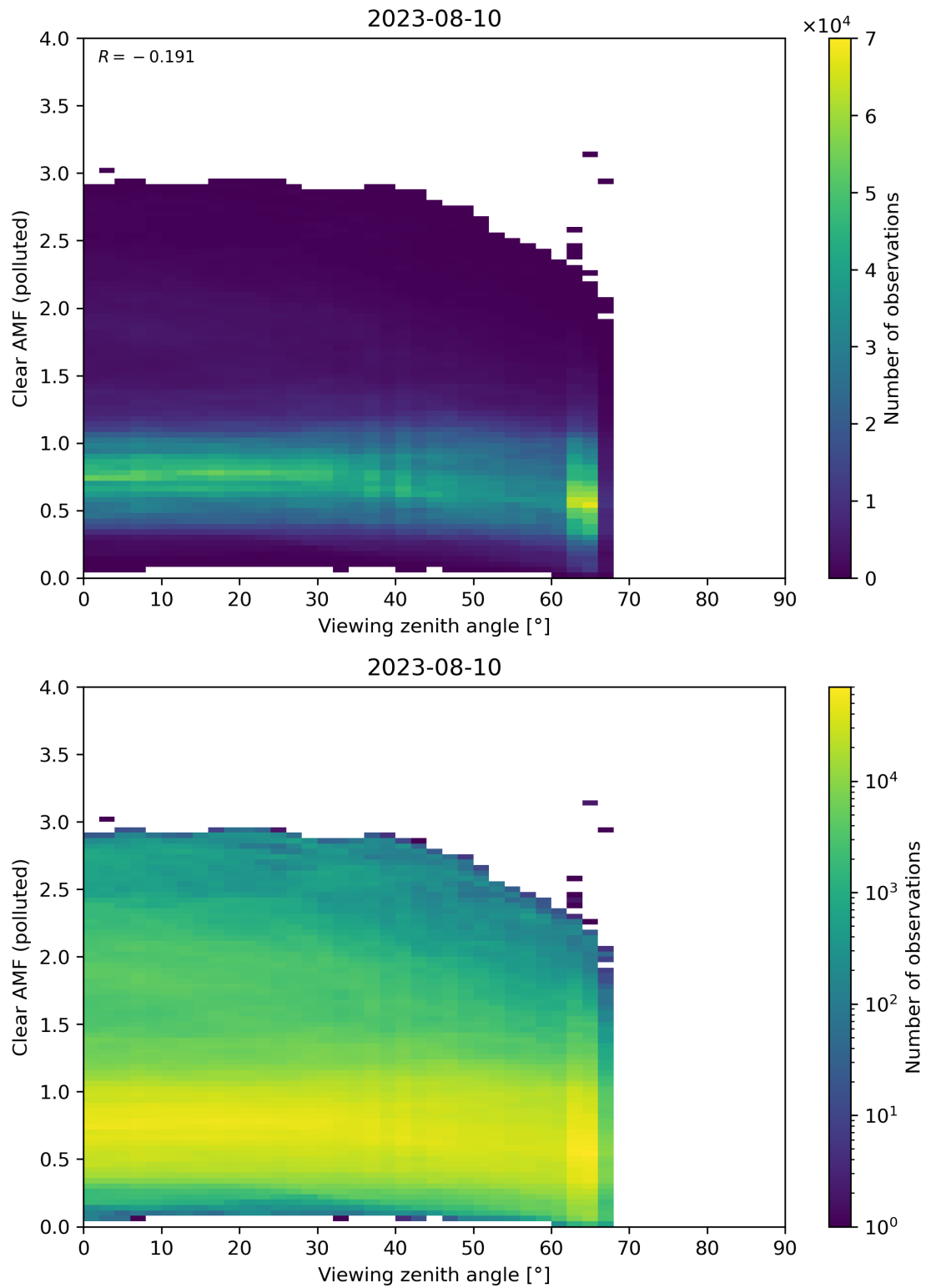
Figure 316: Scatter density plot of “Viewing zenith angle” against “Clear AMF (polluted)” for 2023-08-09 to 2023-08-11.
