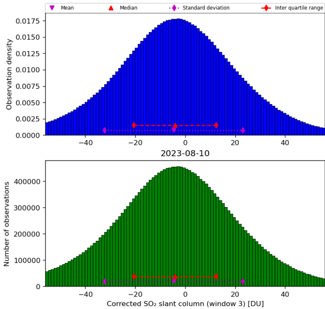
Figure 66: Histogram of “Corrected SO 2 slant column (window 3)” for 2023-08-09 to 2023-08-11
