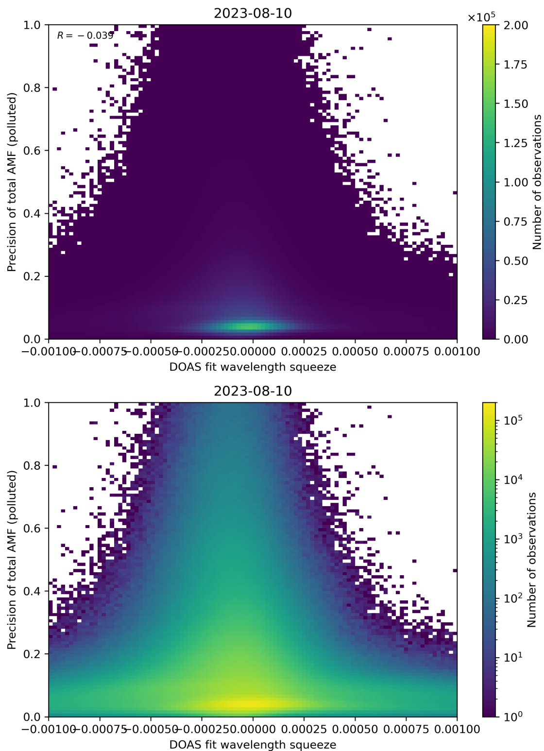
Figure 135: Scatter density plot of “DOAS fit wavelength squeeze” against “Precision of total AMF (polluted)” for 2023-08-09 to 2023-08-11.
