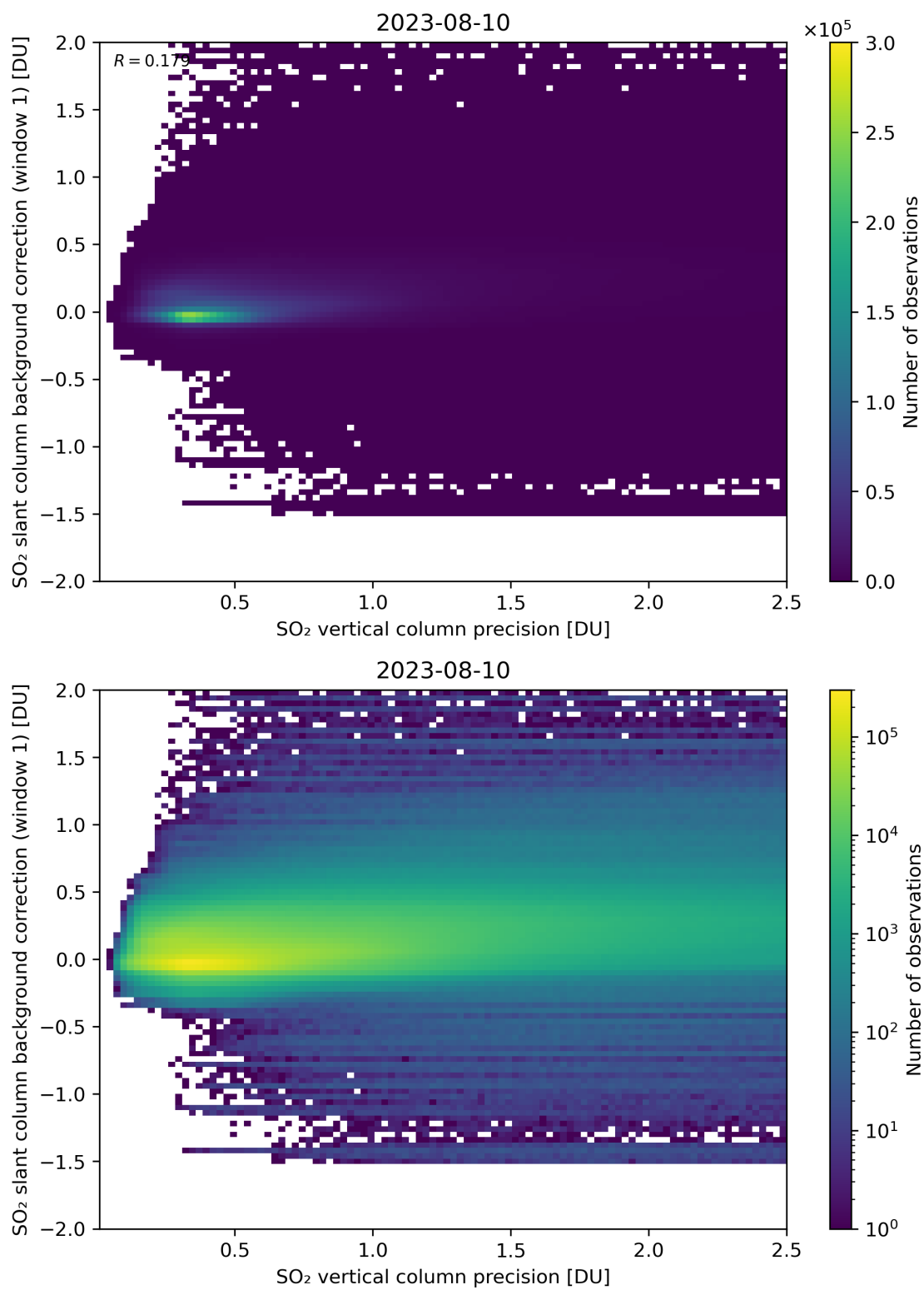
Figure 279: Scatter density plot of “SO 2 vertical column precision” against “SO 2 slant column background correction (window 1)” for 2023-08-09 to 2023-08-11.
