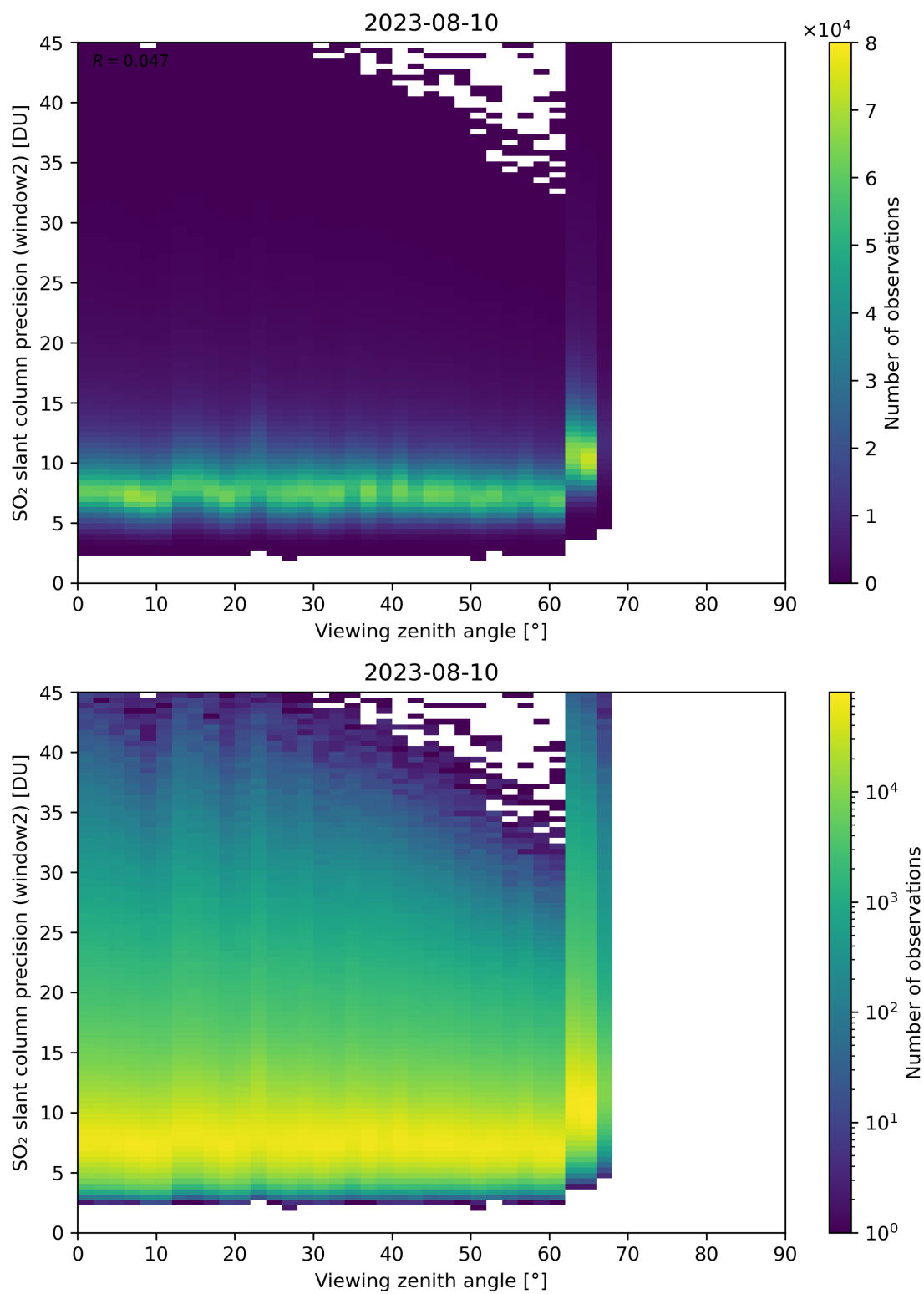
Figure 322: Scatter density plot of “Viewing zenith angle” against “SO 2 slant column precision (window2)” for 2023-08-09 to 2023-08-11.
