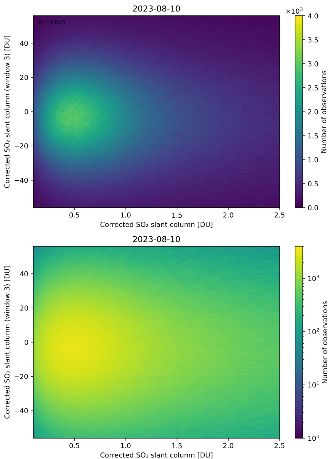
Figure 186: Scatter density plot of “Corrected SO 2 slant column” against “Corrected SO 2 slant column (window 3)” for 2023-08-09 to 2023-08-11.
