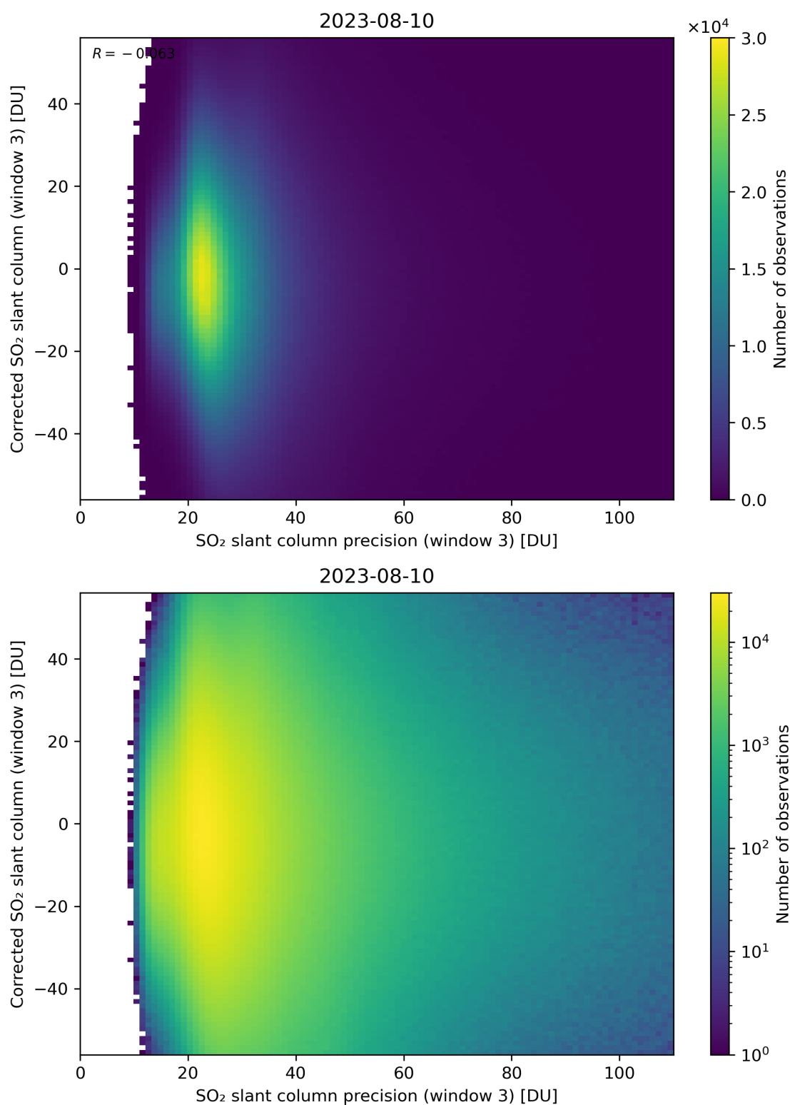
Figure 262: Scatter density plot of “SO 2 slant column precision (window 3)” against “Corrected SO 2 slant column (window 3)” for 2023-08-09 to 2023-08-11.
