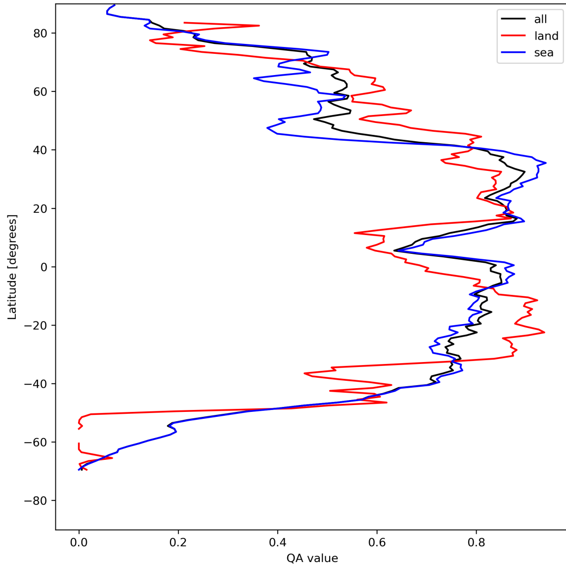
Figure 29: Zonal average of “QA value” for 2023-08-09 to 2023-08-11.
