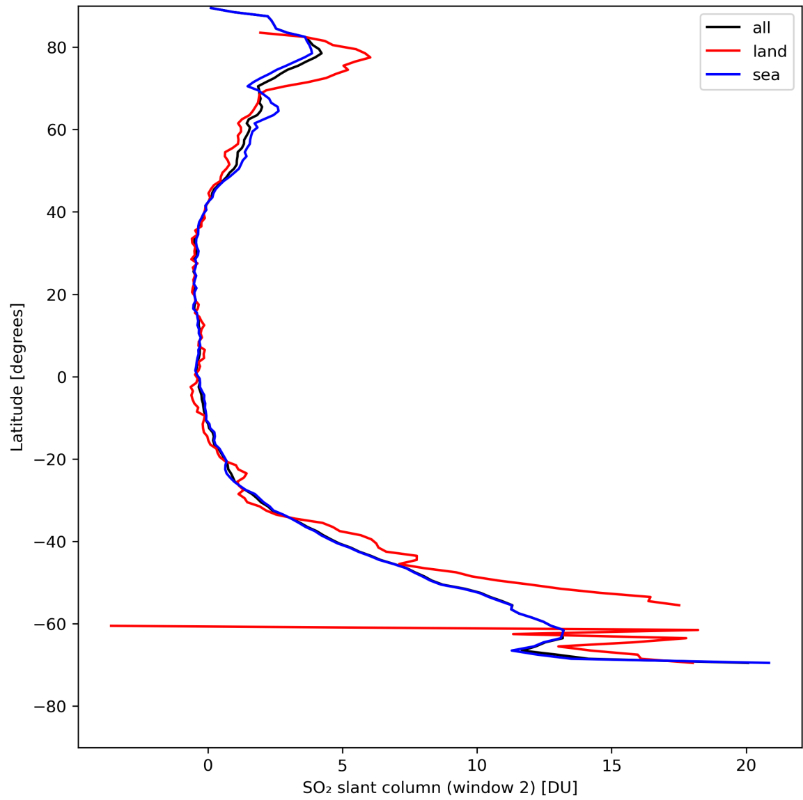
Figure 37: Zonal average of “SO 2 slant column (window 2)” for 2023-08-09 to 2023-08-11.
