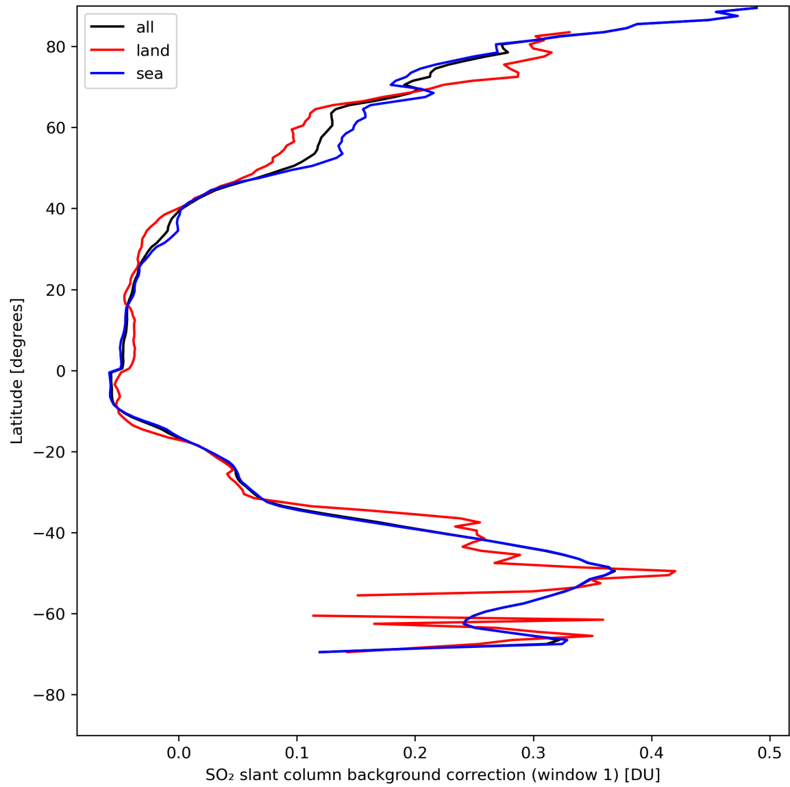
Figure 36: Zonal average of “SO 2 slant column background correction (window 1)” for 2023-08-09 to 2023-08-11.
