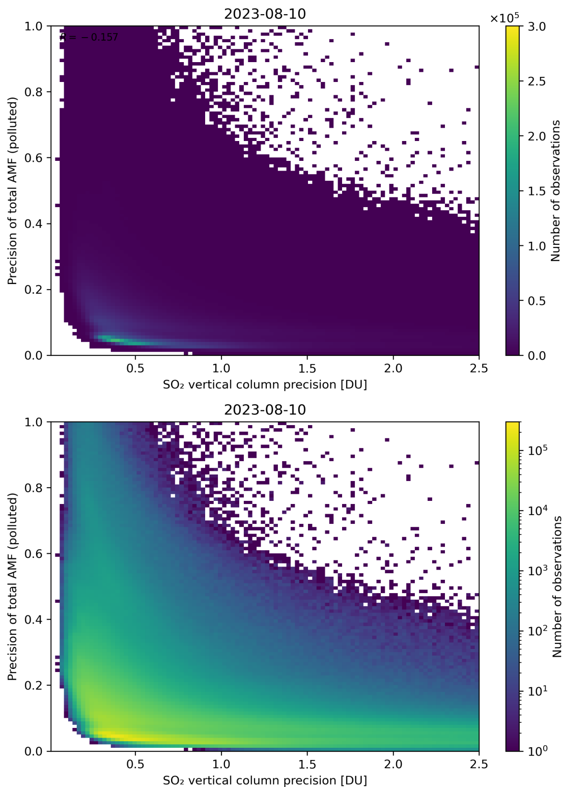
Figure 295: Scatter density plot of “SO 2 vertical column precision” against “Precision of total AMF (polluted)” for 2023-08-09 to 2023-08-11.
