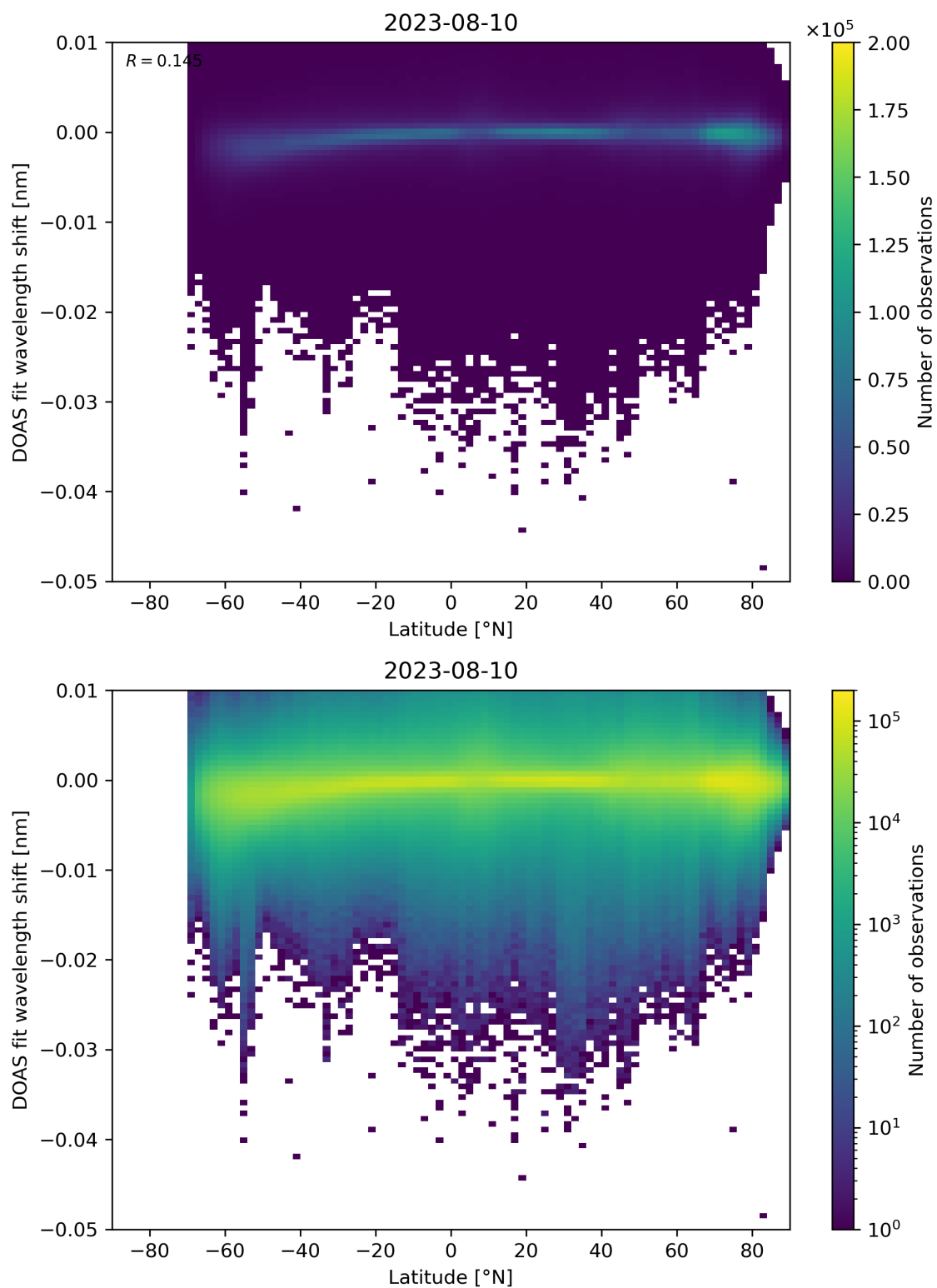
Figure 142: Scatter density plot of “Latitude” against “DOAS fit wavelength shift” for 2023-08-09 to 2023-08-11.
