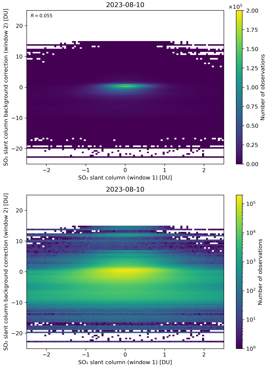
Figure 213: Scatter density plot of “SO 2 slant column (window 1)” against “SO 2 slant column background correction (window 2)” for 2023-08-09 to 2023-08-11.
