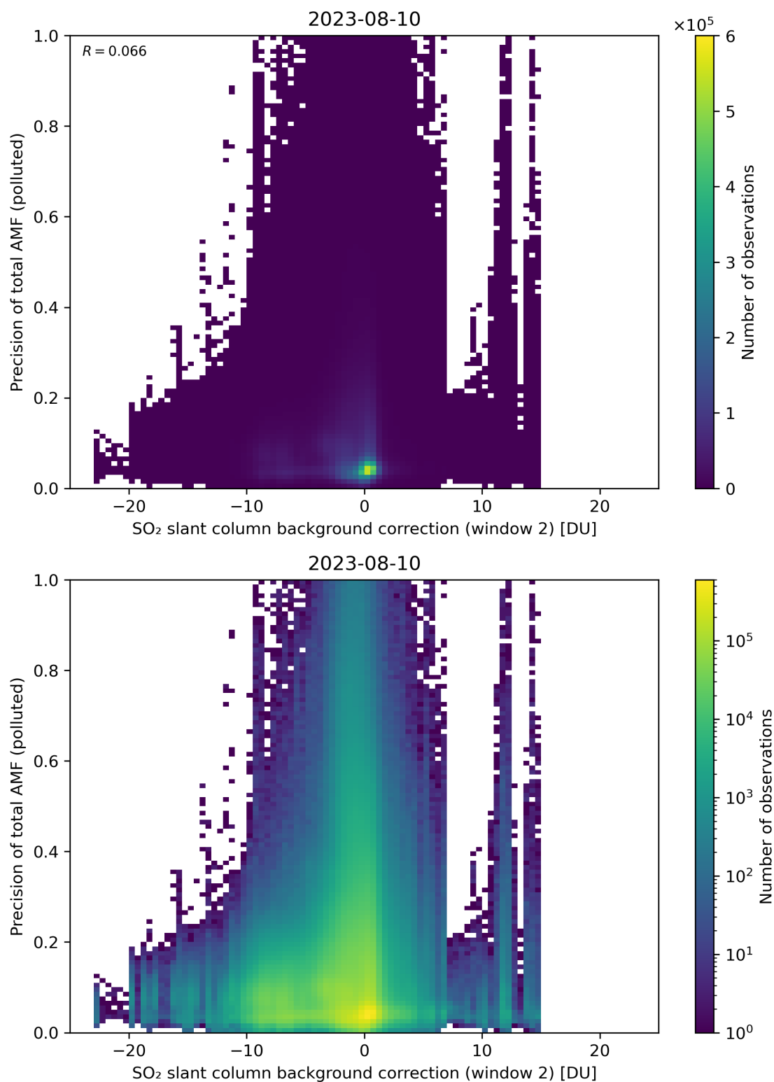
Figure 120: Scatter density plot of “SO 2 slant column background correction (window 2)” against “Precision of total AMF (polluted)” for 2023-08-09 to 2023-08-11.
