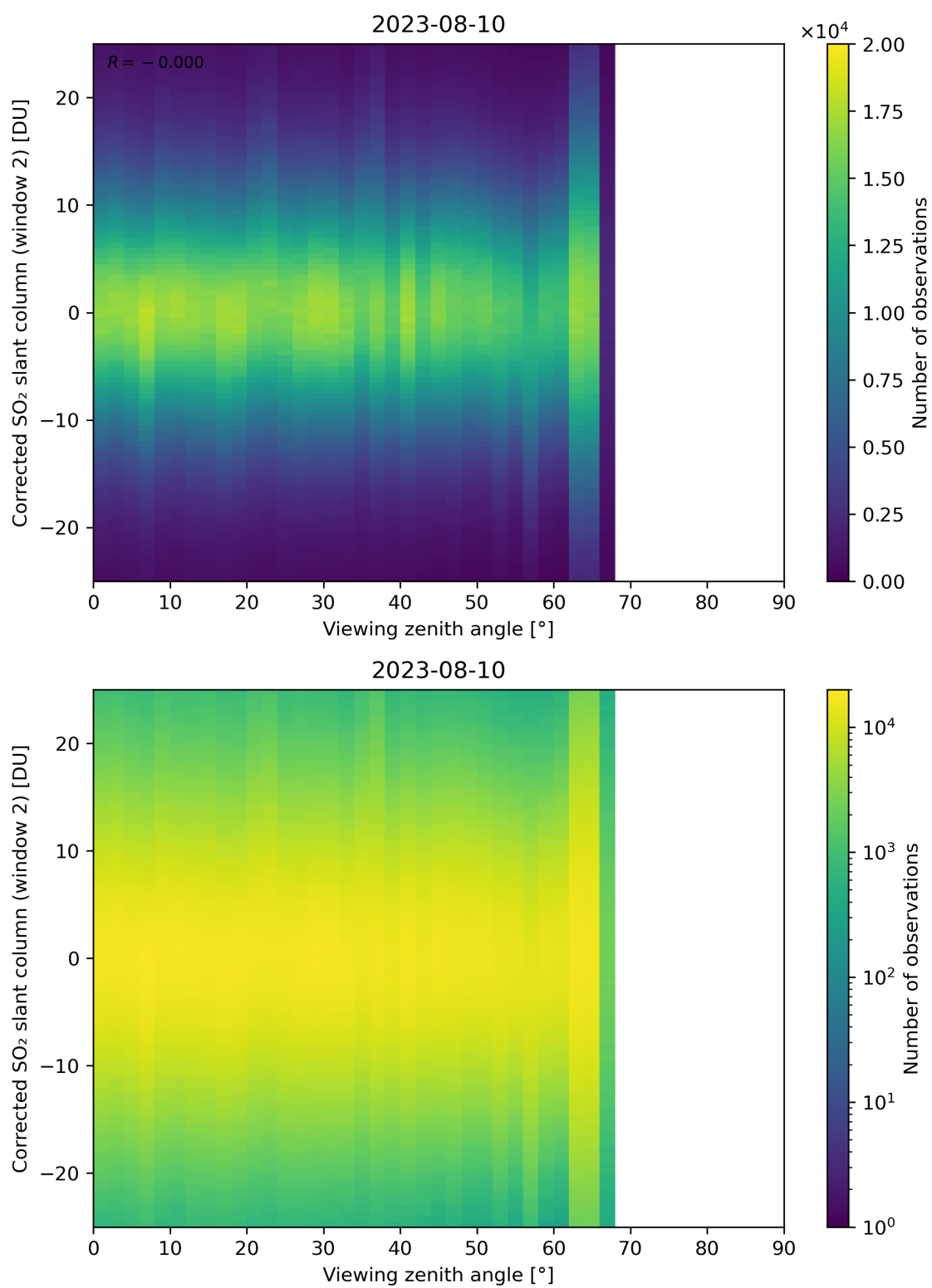
Figure 318: Scatter density plot of “Viewing zenith angle” against “Corrected SO 2 slant column (window 2)” for 2023-08-09 to 2023-08-11.
