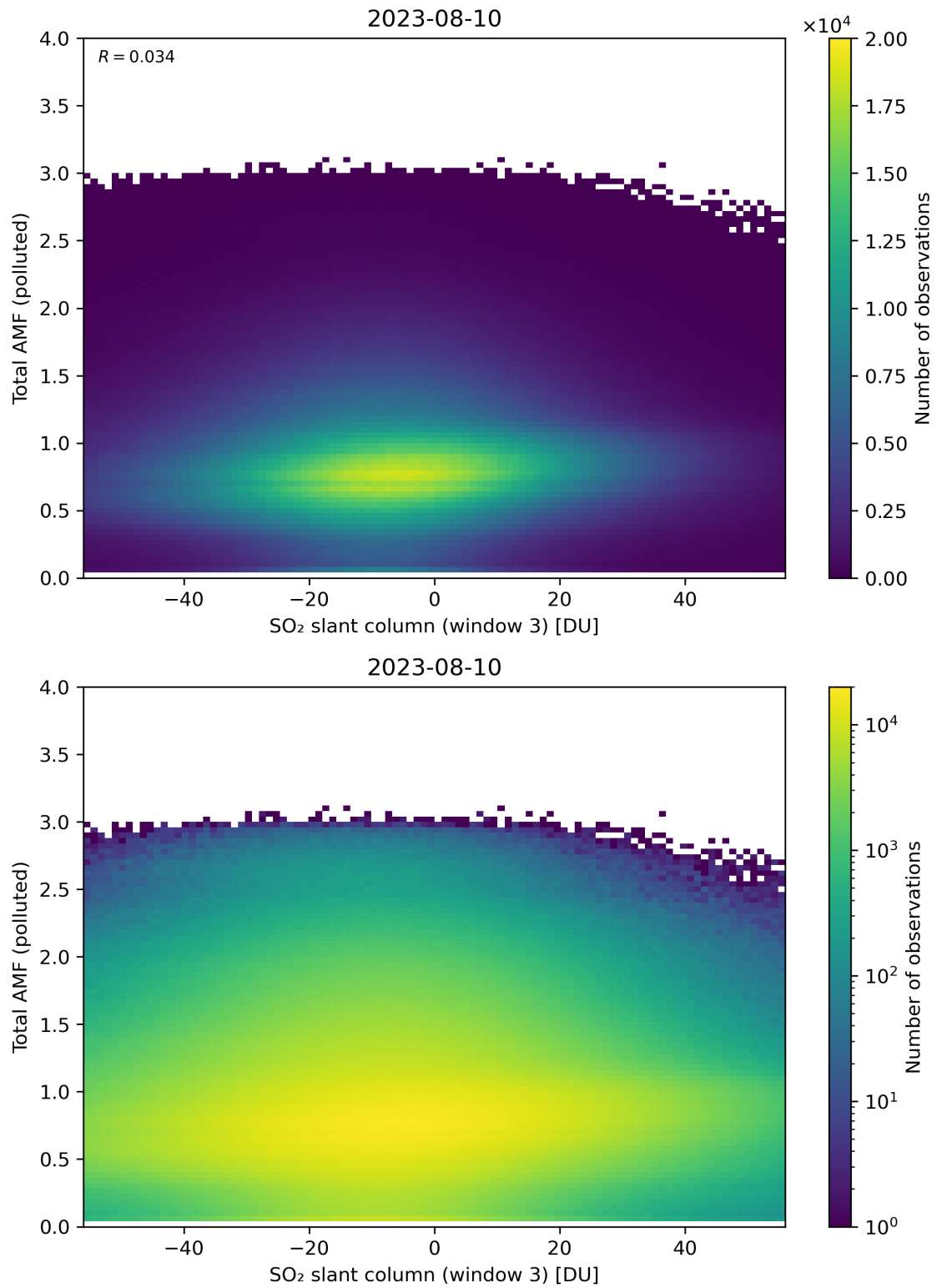
Figure 268: Scatter density plot of “SO 2 slant column (window 3)” against “Total AMF (polluted)” for 2023-08-09 to 2023-08-11.
