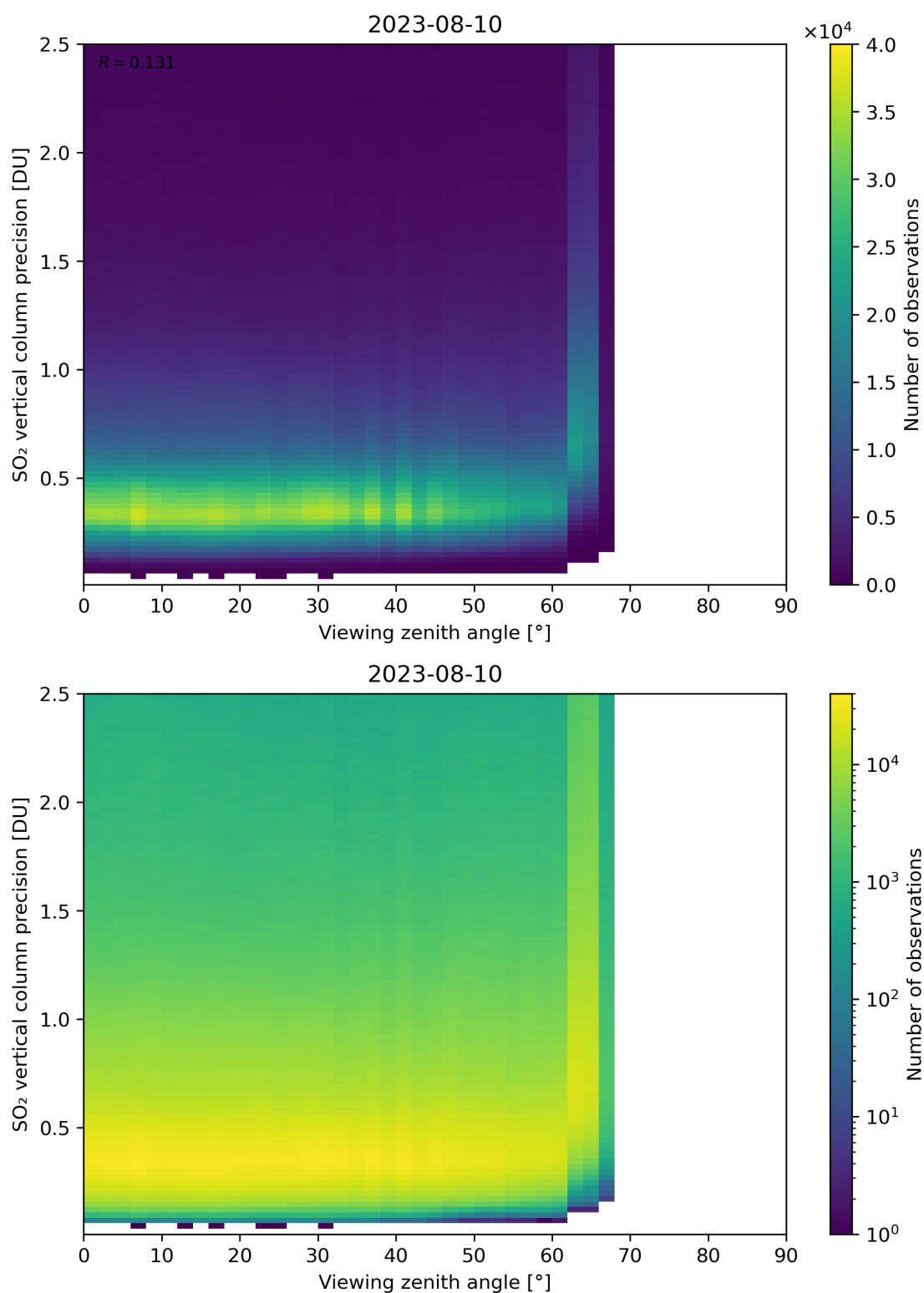
Figure 328: Scatter density plot of “Viewing zenith angle” against “SO 2 vertical column precision” for 2023-08-09 to 2023-08-11.
