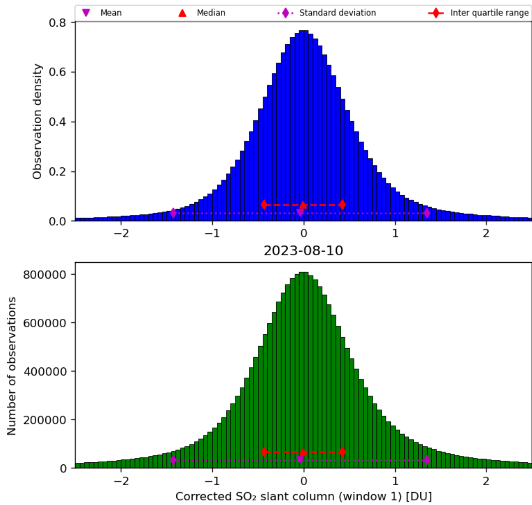
Figure 58: Histogram of “Corrected SO 2 slant column (window 1)” for 2023-08-09 to 2023-08-11
