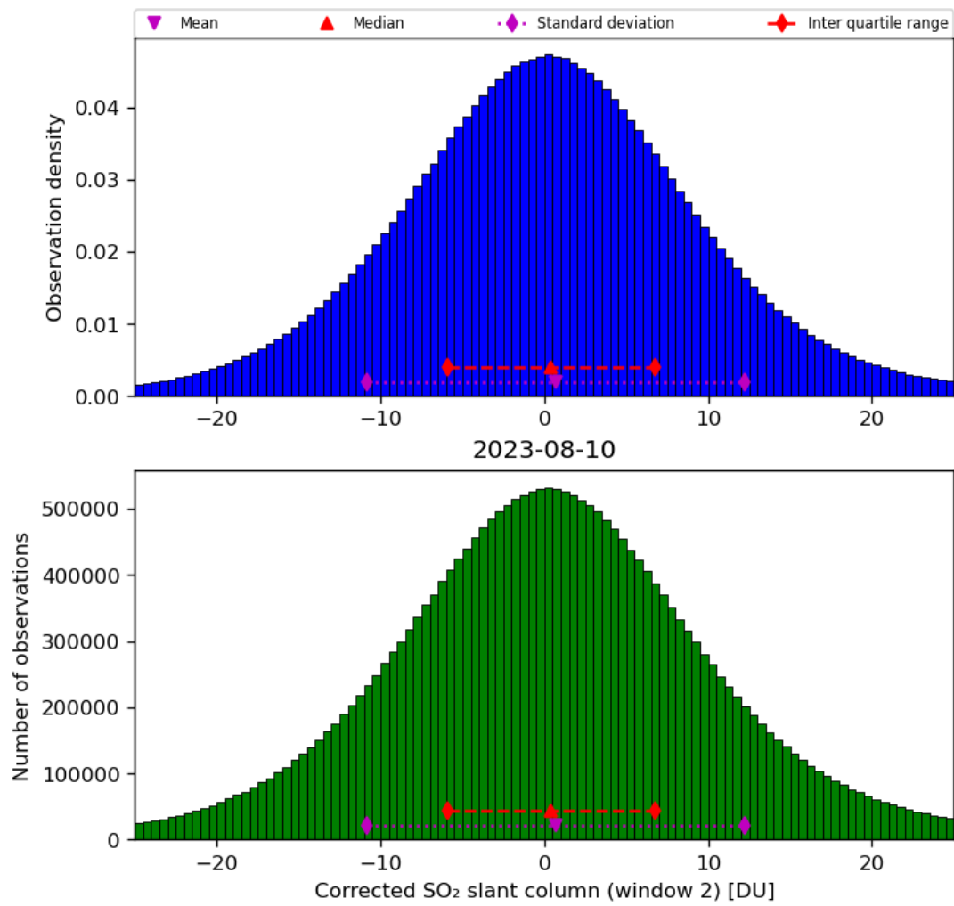
Figure 62: Histogram of “Corrected SO 2 slant column (window 2)” for 2023-08-09 to 2023-08-11
