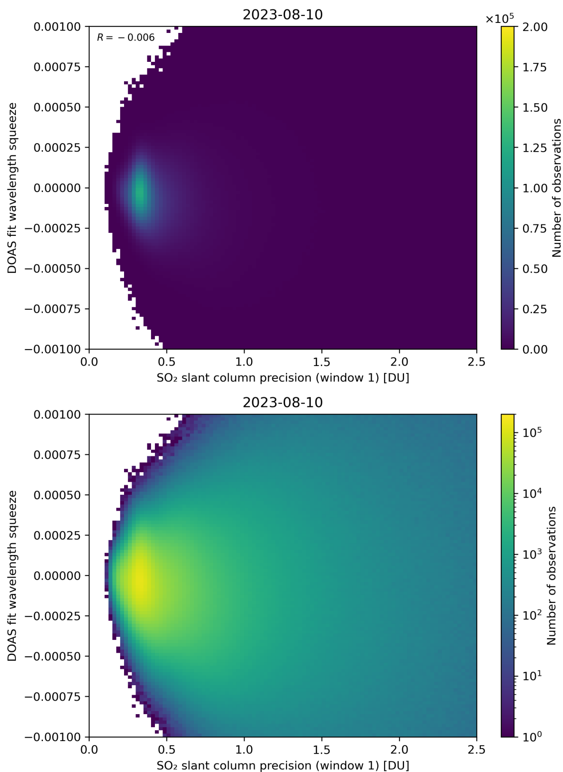
Figure 222: Scatter density plot of “SO 2 slant column precision (window 1)” against “DOAS fit wavelength squeeze” for 2023-08-09 to 2023-08-11.
