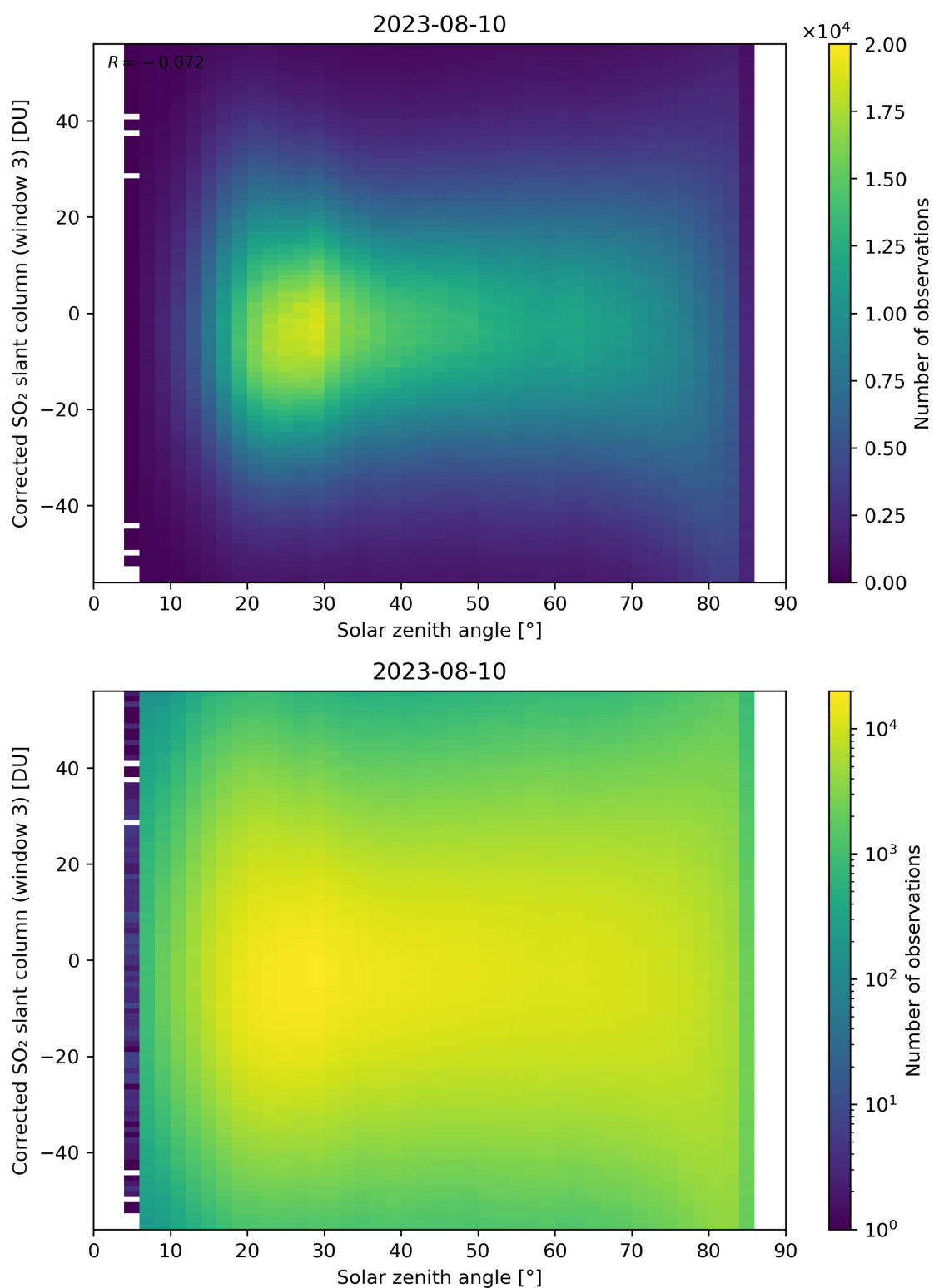
Figure 168: Scatter density plot of “Solar zenith angle” against “Corrected SO 2 slant column (window 3)” for 2023-08-09 to 2023-08-11.
