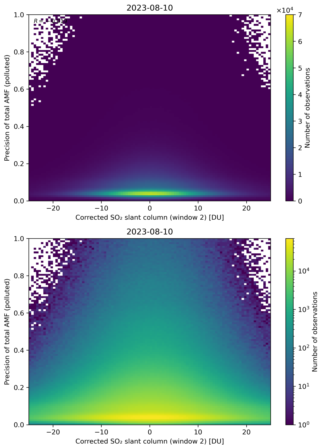
Figure 204: Scatter density plot of “Corrected SO 2 slant column (window 2)” against “Precision of total AMF (polluted)” for 2023-08-09 to 2023-08-11.
