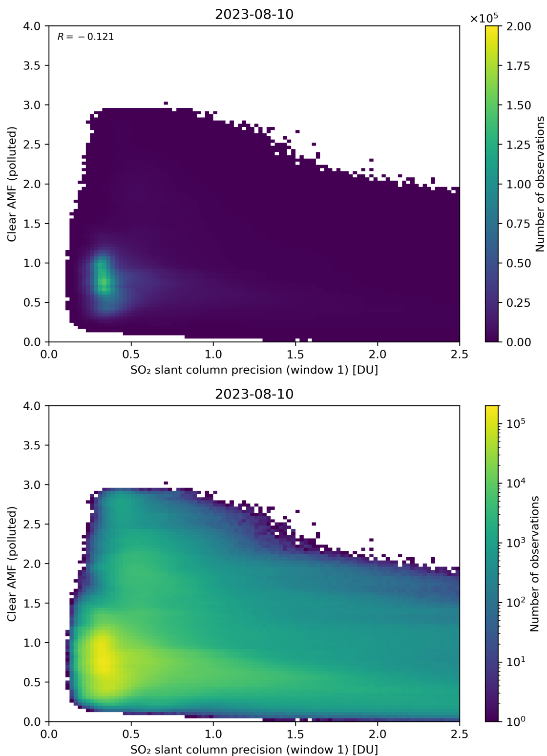
Figure 224: Scatter density plot of “SO 2 slant column precision (window 1)” against “Clear AMF (polluted)” for 2023-08-09 to 2023-08-11.
