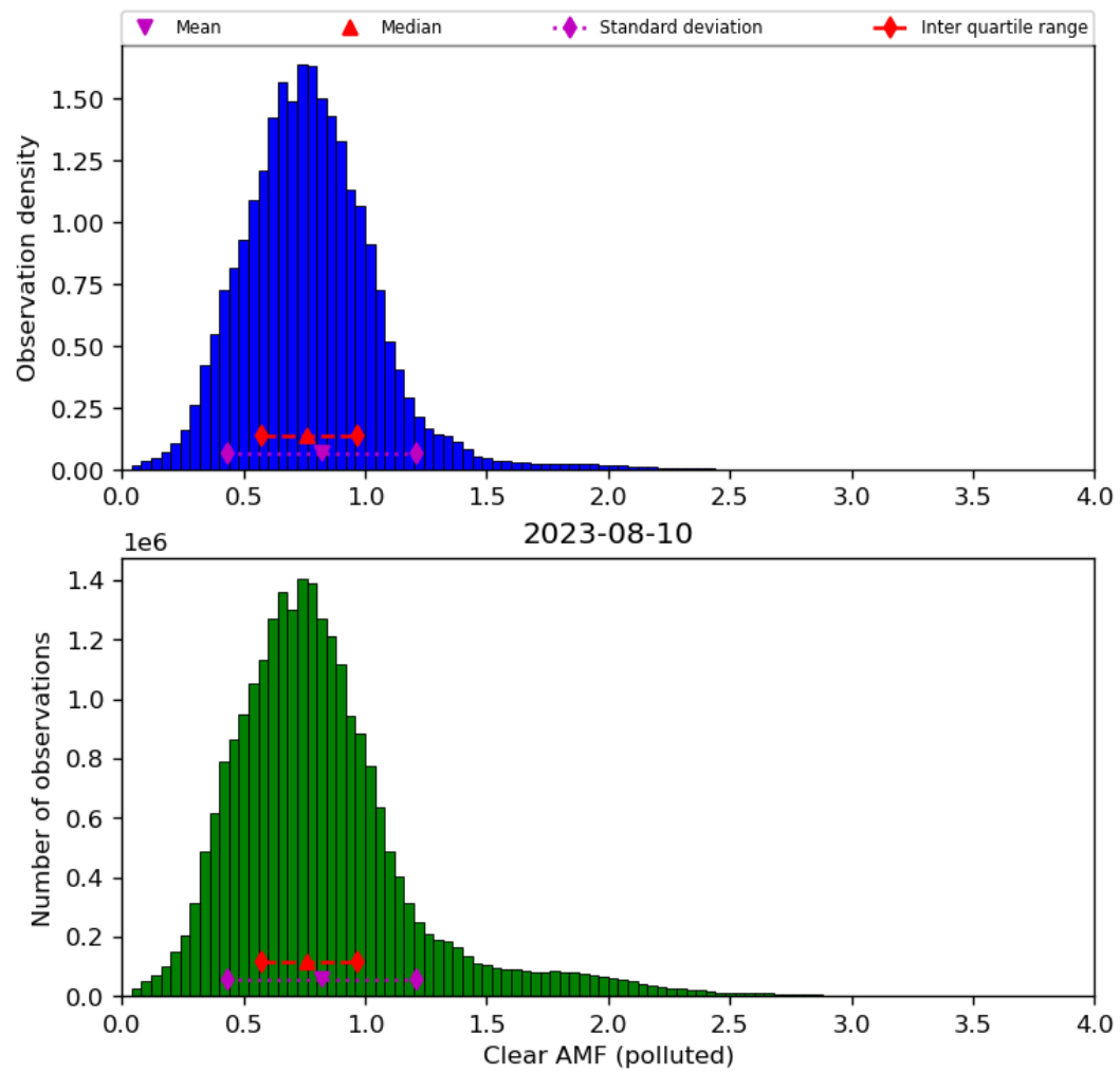
Figure 73: Histogram of “Clear AMF (polluted)” for 2023-08-09 to 2023-08-11
