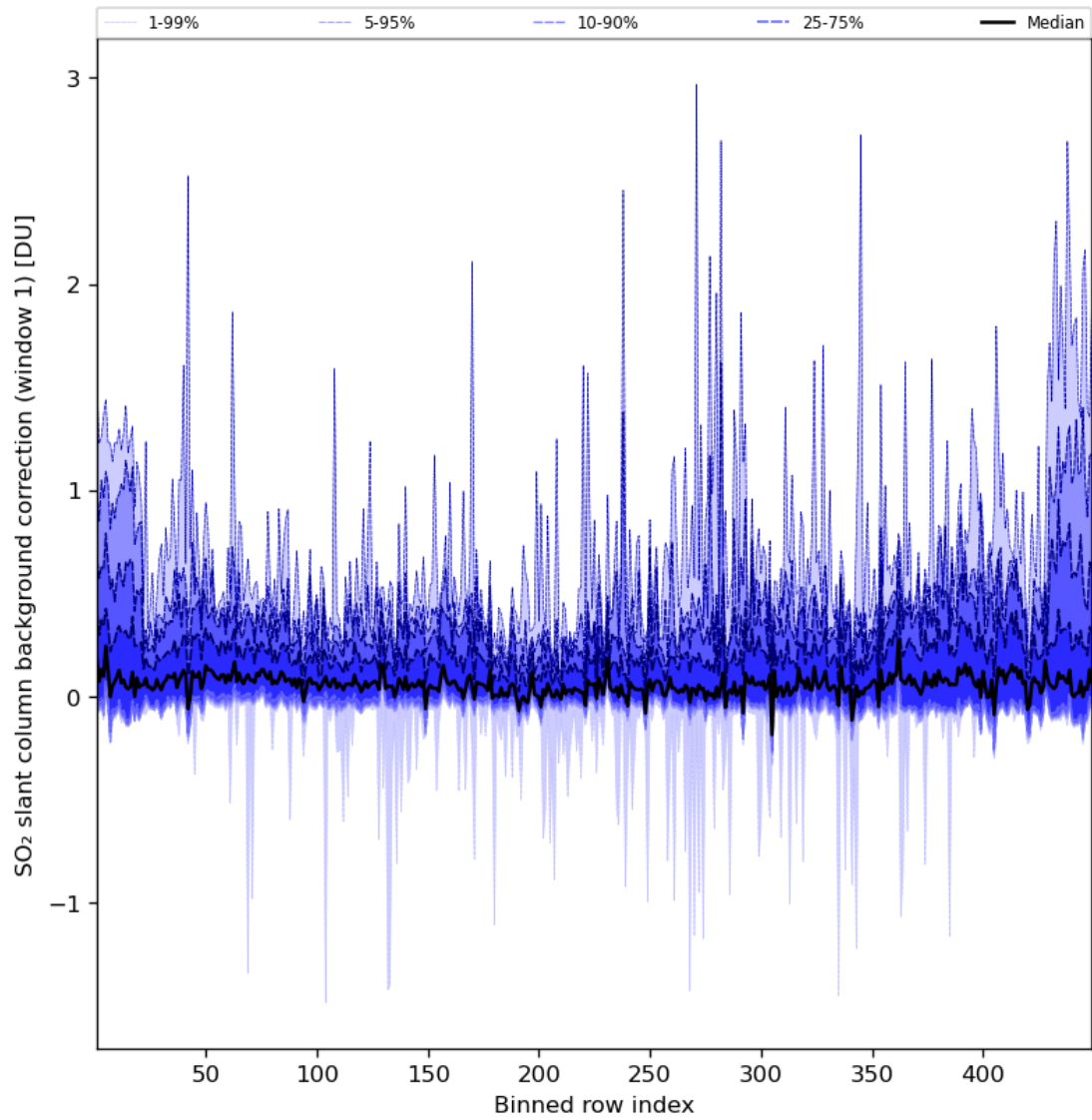
Figure 82: Along track statistics of “SO 2 slant column background correction (window 1)” for 2023-08-09 to 2023-08-11
