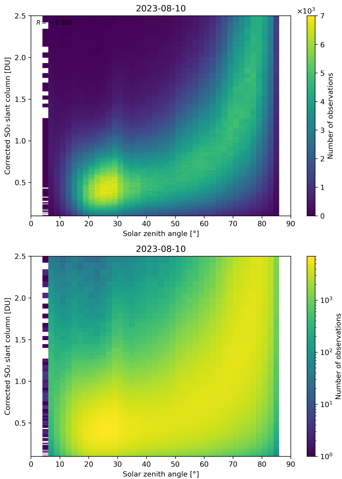
Figure 166: Scatter density plot of “Solar zenith angle” against “Corrected SO 2 slant column” for 2023-08-09 to 2023-08-11.
