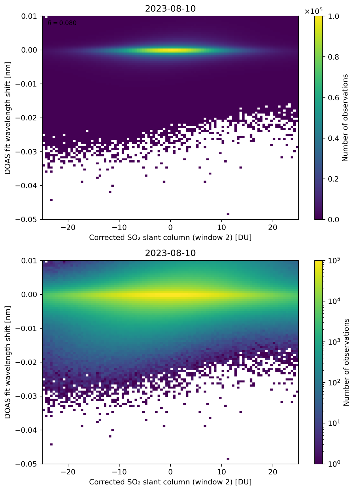
Figure 196: Scatter density plot of “Corrected SO 2 slant column (window 2)” against “DOAS fit wavelength shift” for 2023-08-09 to 2023-08-11.
