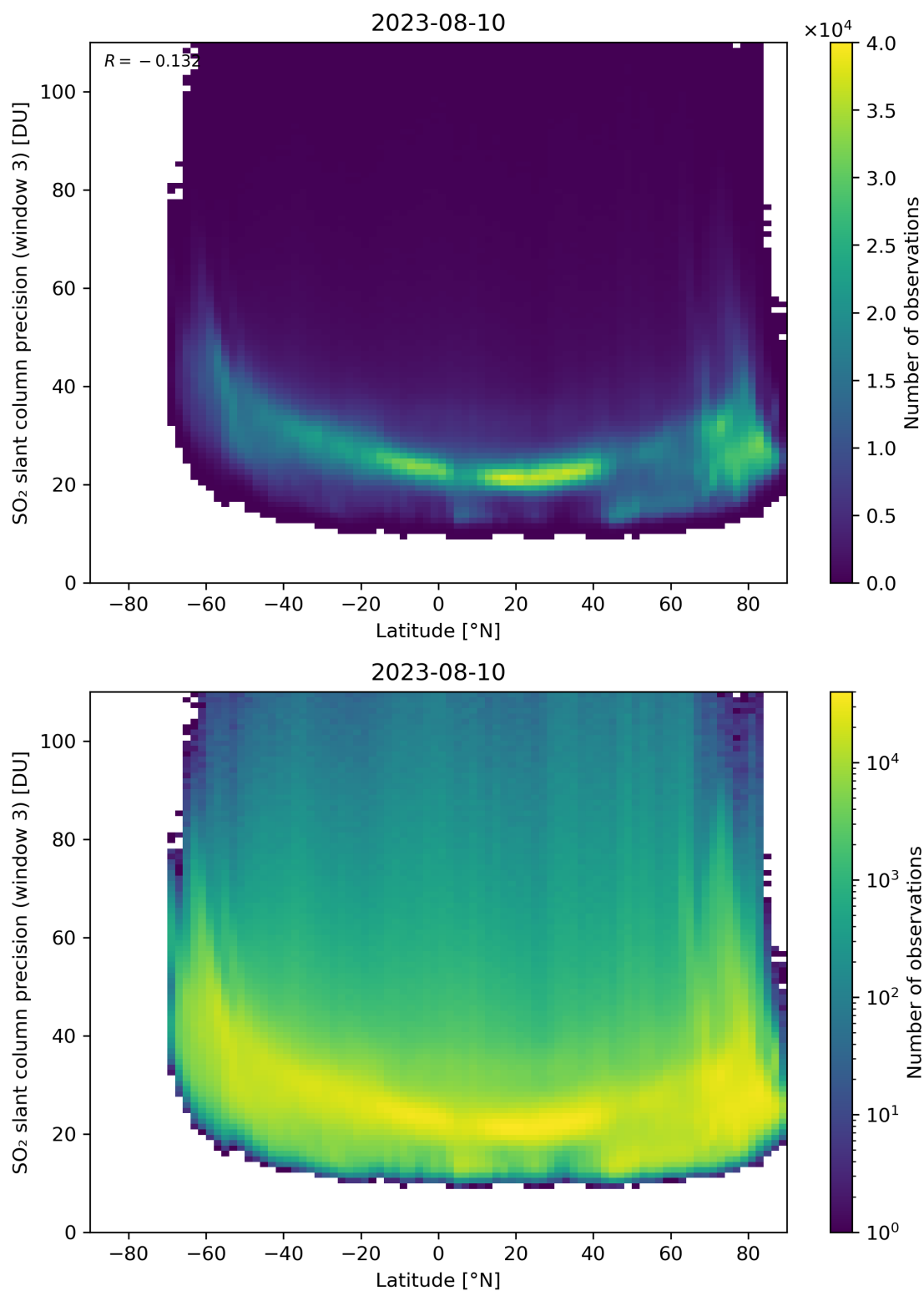
Figure 153: Scatter density plot of “Latitude” against “SO 2 slant column precision (window 3)” for 2023-08-09 to 2023-08-11.
