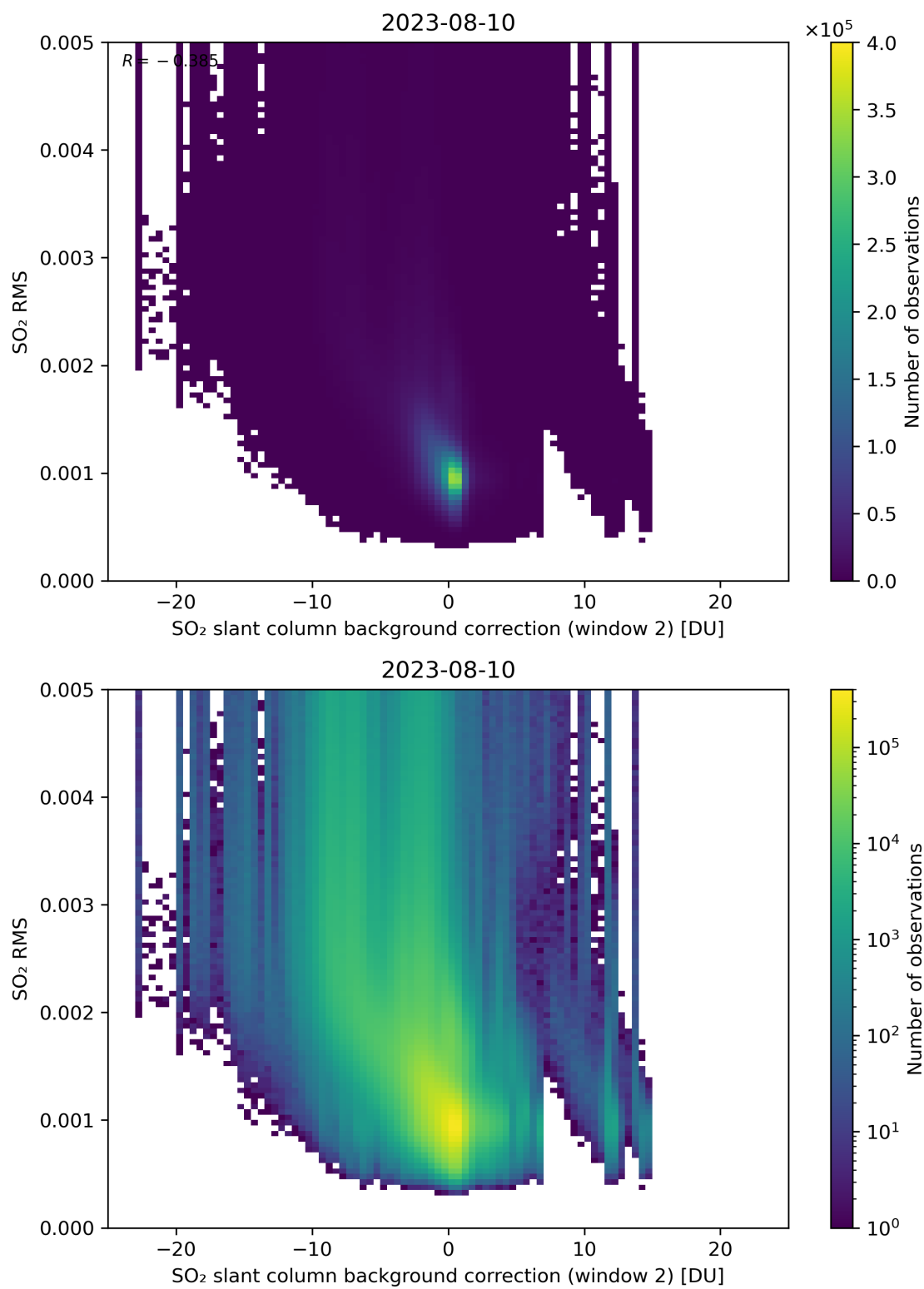
Figure 114: Scatter density plot of “SO 2 slant column background correction (window 2)” against “SO 2 RMS” for 2023-08-09 to 2023-08-11.
