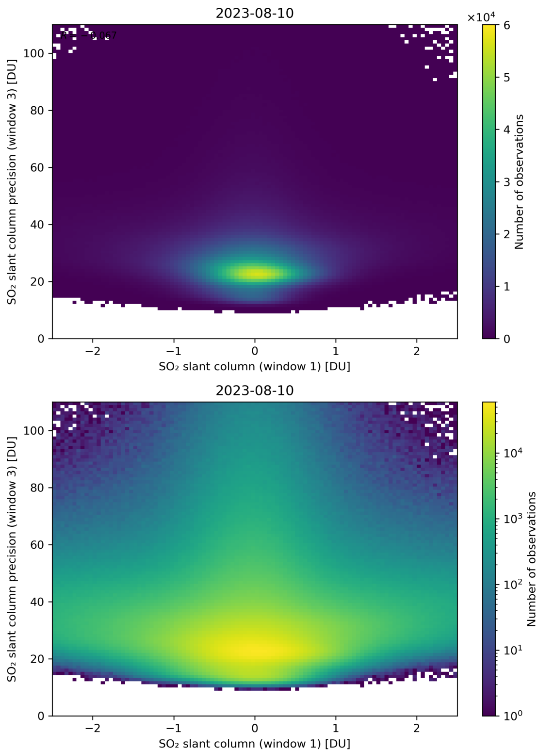
Figure 238: Scatter density plot of “SO 2 slant column (window 1)” against “SO 2 slant column precision (window 3)” for 2023-08-09 to 2023-08-11.
