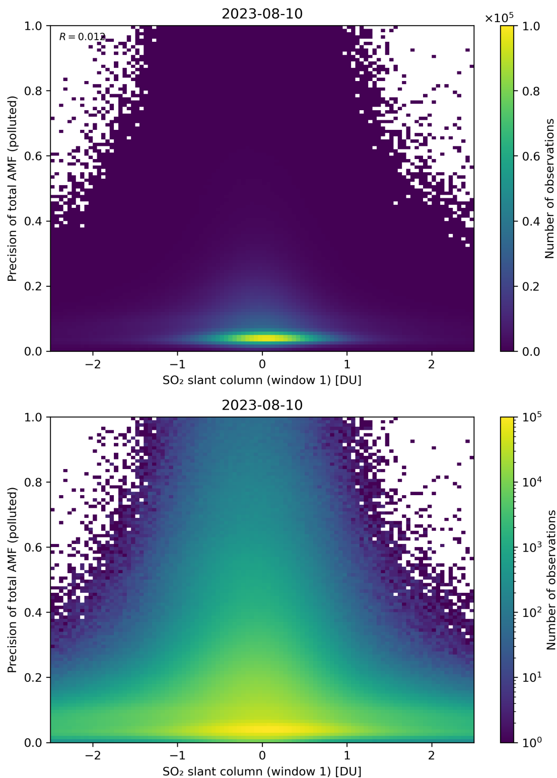
Figure 240: Scatter density plot of “SO 2 slant column (window 1)” against “Precision of total AMF (polluted)” for 2023-08-09 to 2023-08-11.
