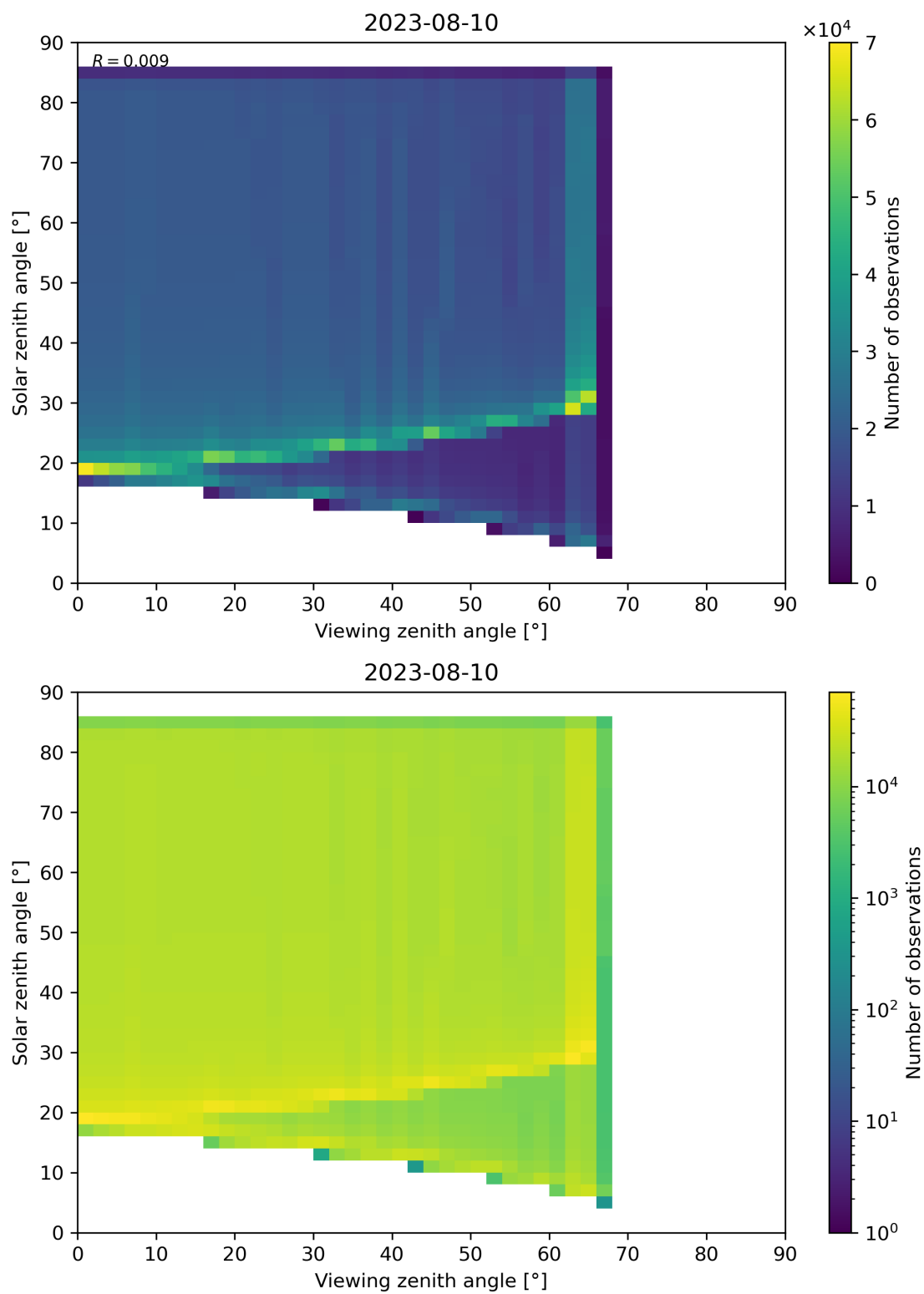
Figure 315: Scatter density plot of “Viewing zenith angle” against “Solar zenith angle” for 2023-08-09 to 2023-08-11.
