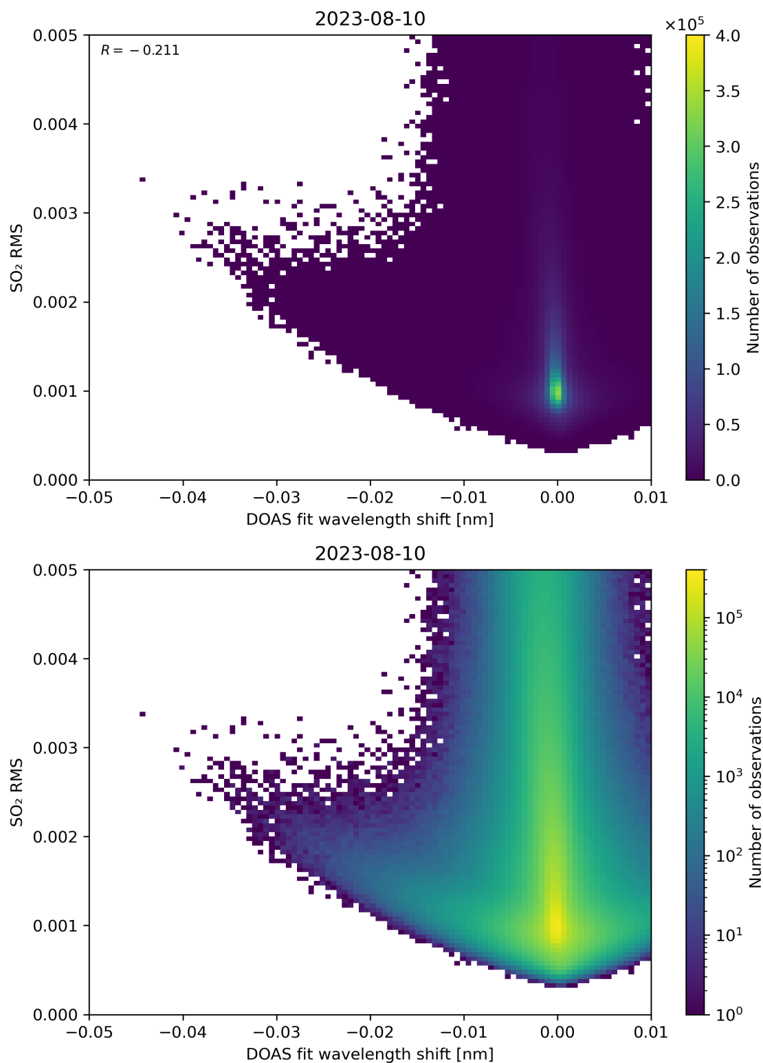
Figure 128: Scatter density plot of “DOAS fit wavelength shift” against “SO 2 RMS” for 2023-08-09 to 2023-08-11.
