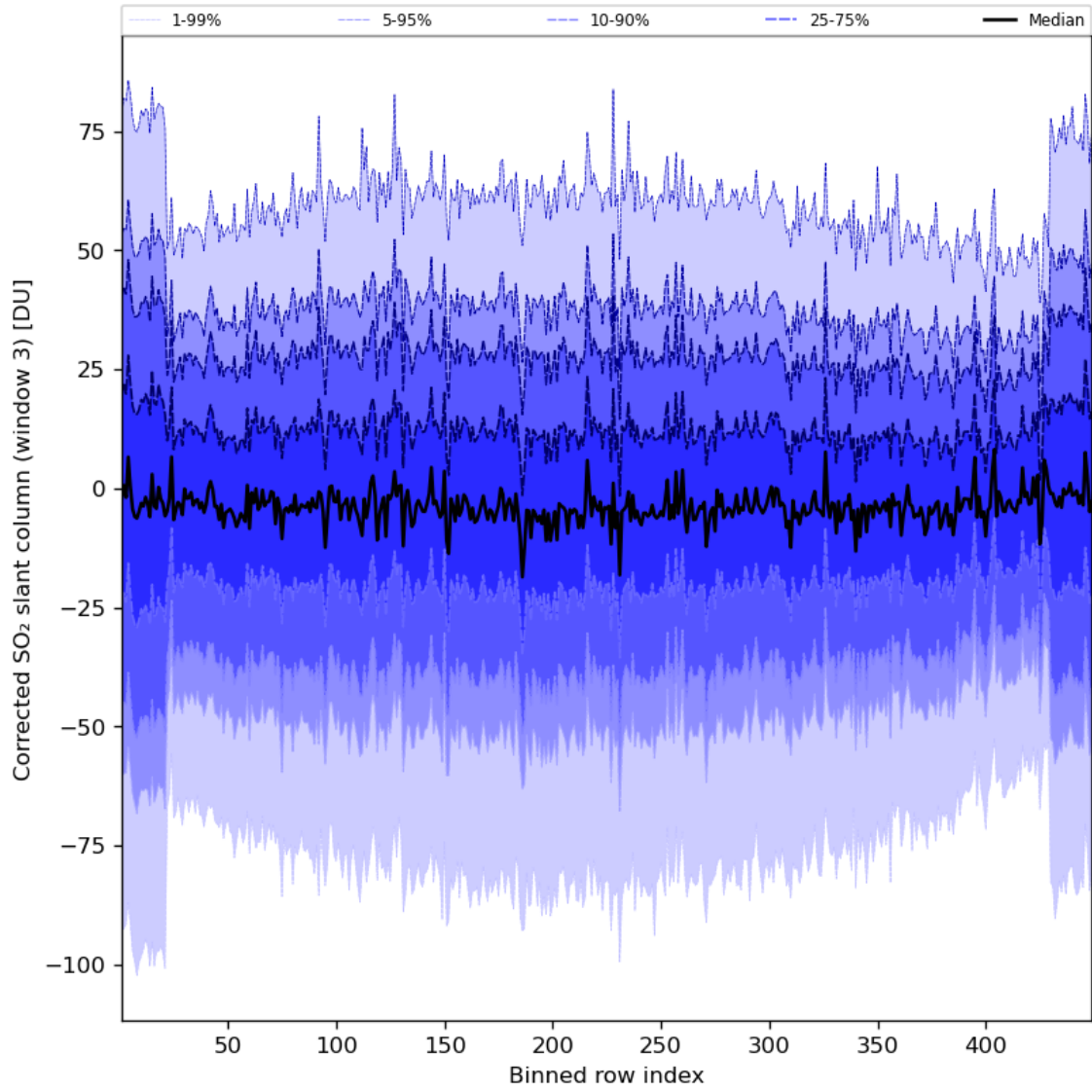
Figure 89: Along track statistics of “Corrected SO 2 slant column (window 3)” for 2023-08-09 to 2023-08-11
