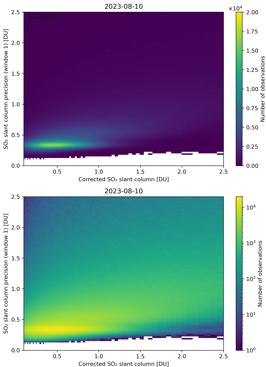
Figure 188: Scatter density plot of “Corrected SO 2 slant column” against “SO 2 slant column precision (window 1)” for 2023-08-09 to 2023-08-11.
