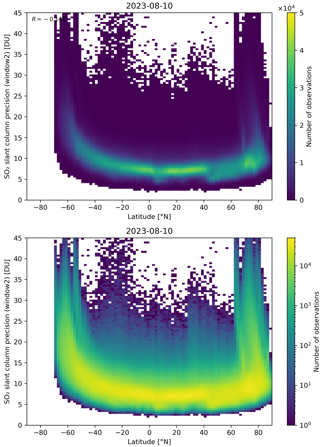
Figure 151: Scatter density plot of “Latitude” against “SO 2 slant column precision (window2)” for 2023-08-09 to 2023-08-11.
