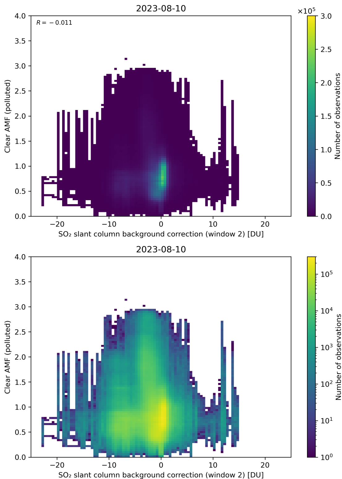
Figure 115: Scatter density plot of “SO 2 slant column background correction (window 2)” against “Clear AMF (polluted)” for 2023-08-09 to 2023-08-11.
