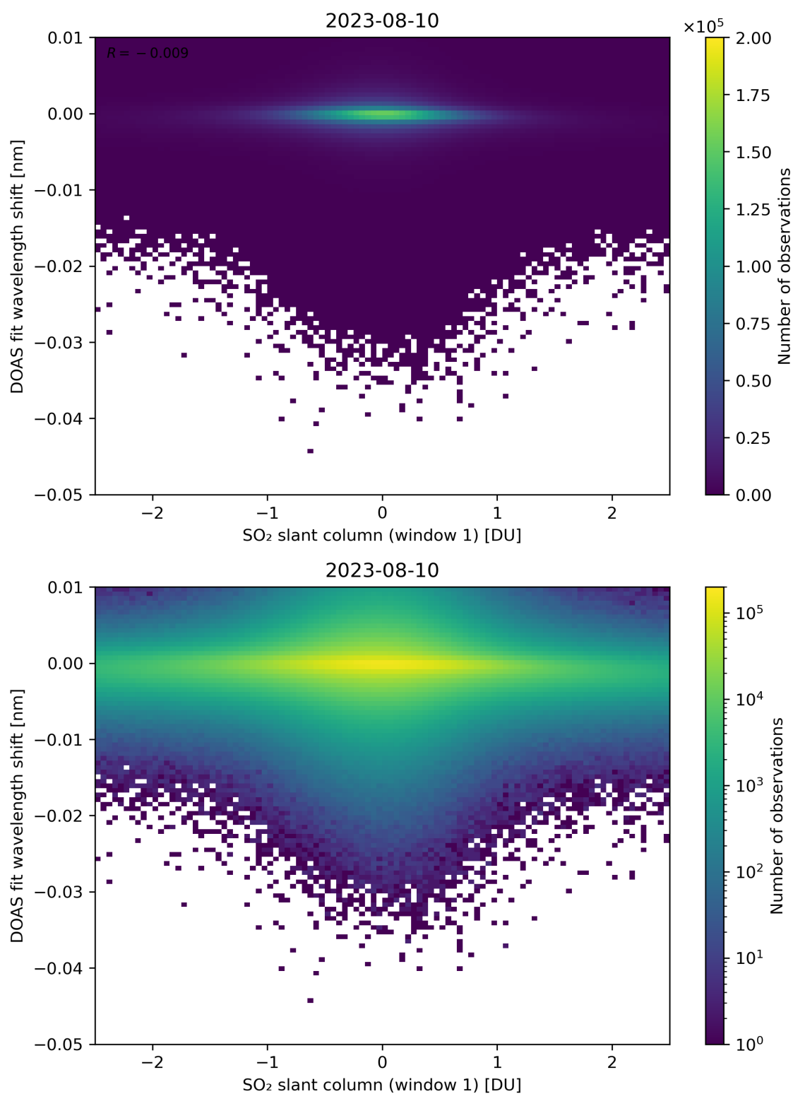
Figure 215: Scatter density plot of “SO 2 slant column (window 1)” against “DOAS fit wavelength shift” for 2023-08-09 to 2023-08-11.
