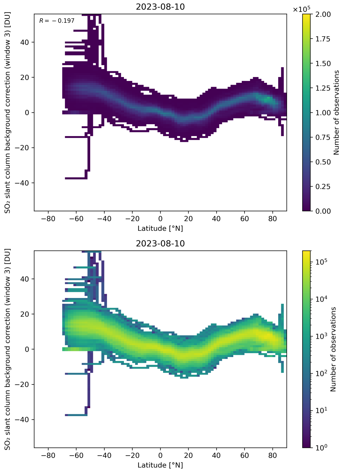
Figure 141: Scatter density plot of “Latitude” against “SO 2 slant column background correction (window 3)” for 2023-08-09 to 2023-08-11.
