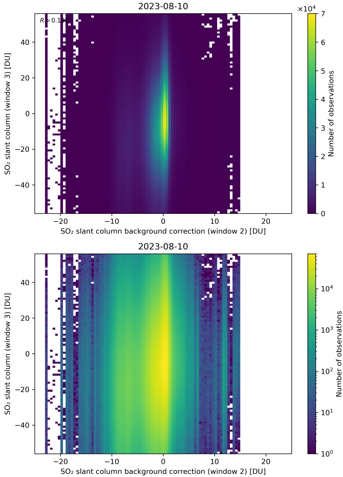
Figure 117: Scatter density plot of “SO 2 slant column background correction (window 2)” against “SO 2 slant column (window 3)” for 2023-08-09 to 2023-08-11.
