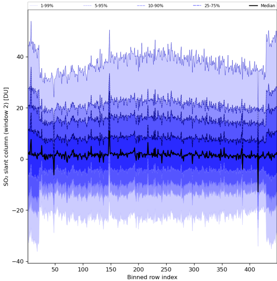
Figure 83: Along track statistics of “SO 2 slant column (window 2)” for 2023-08-09 to 2023-08-11
