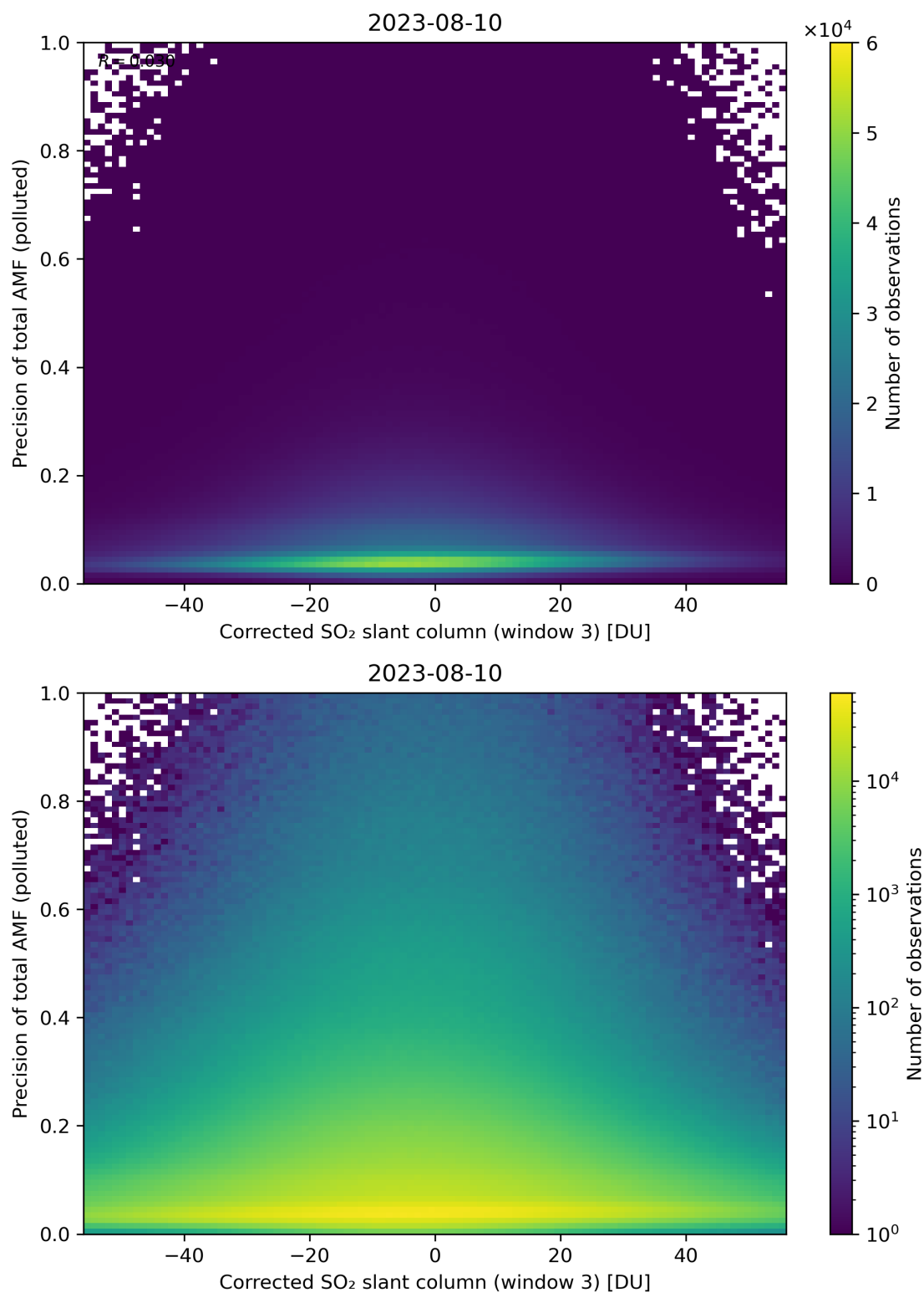
Figure 211: Scatter density plot of “Corrected SO 2 slant column (window 3)” against “Precision of total AMF (polluted)” for 2023-08-09 to 2023-08-11.
