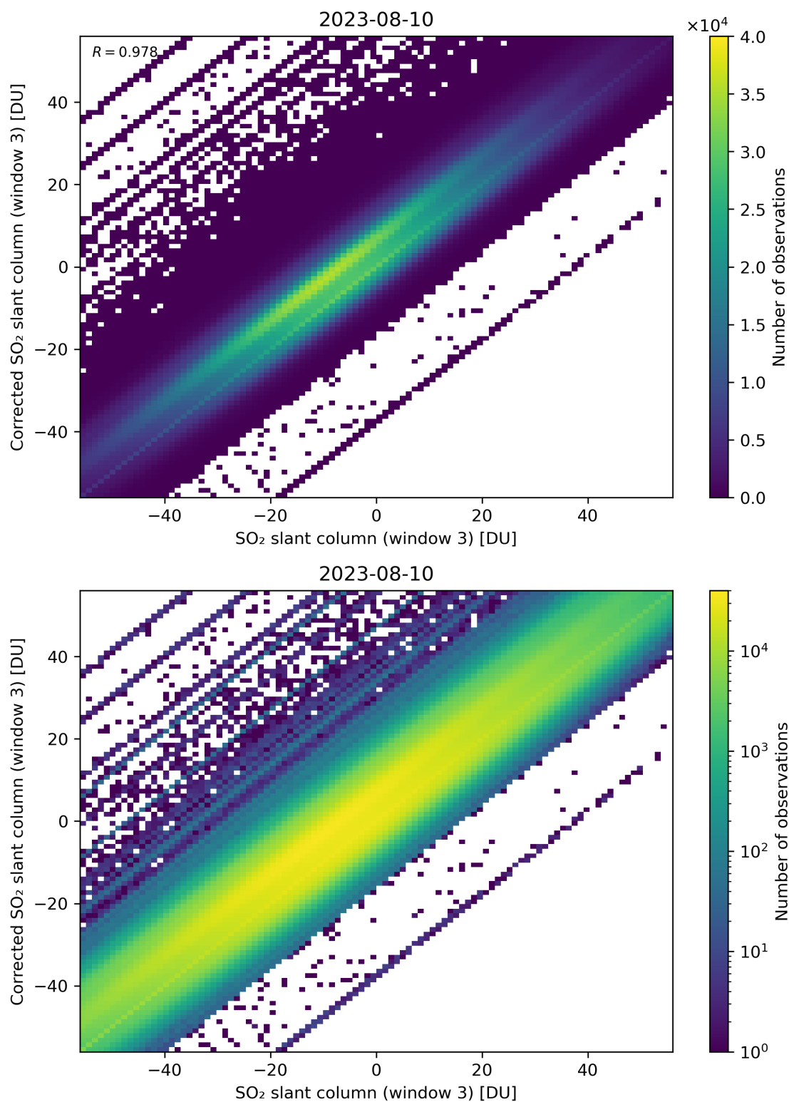
Figure 266: Scatter density plot of “SO 2 slant column (window 3)” against “Corrected SO 2 slant column (window 3)” for 2023-08-09 to 2023-08-11.
