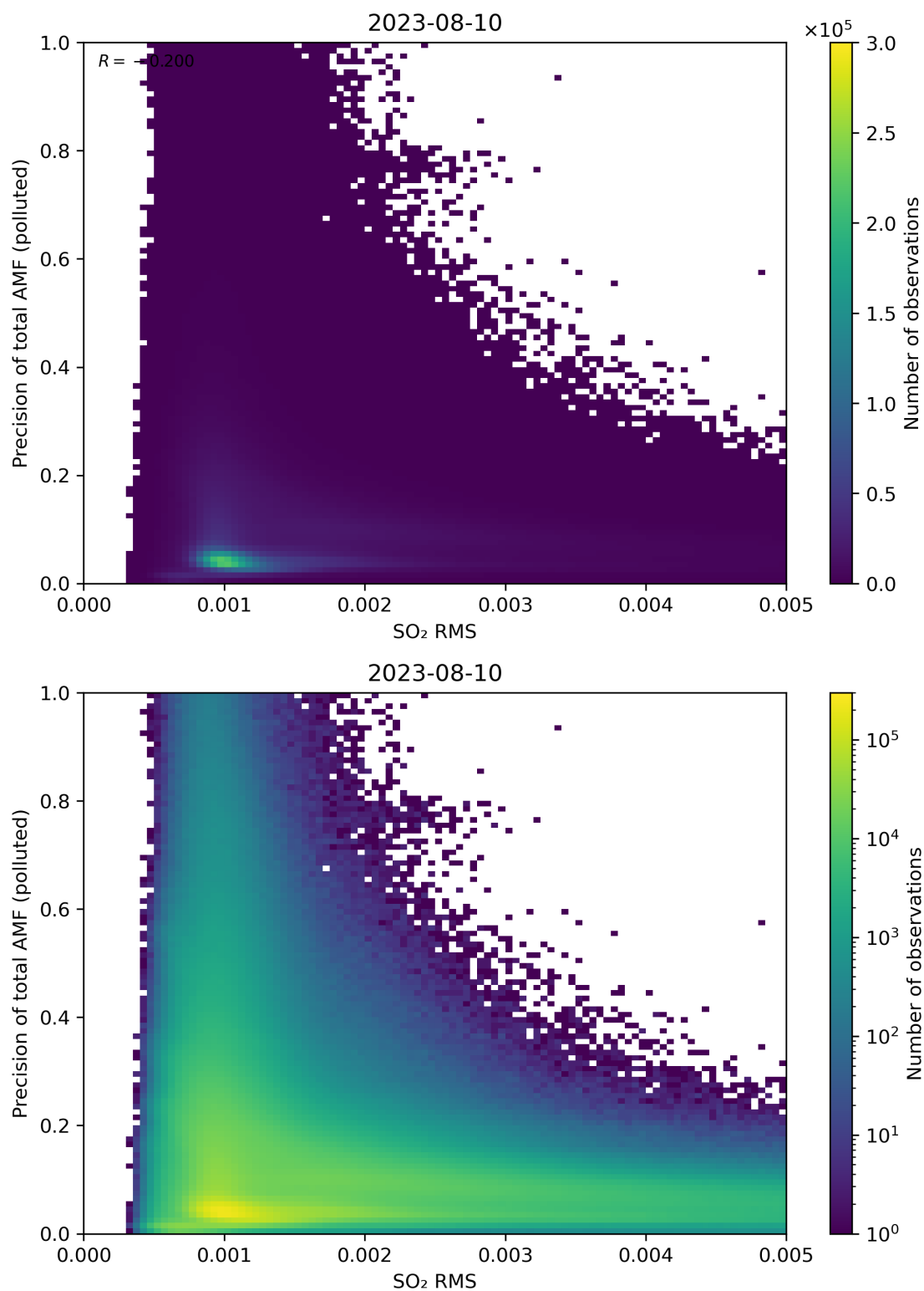
Figure 138: Scatter density plot of “SO 2 RMS” against “Precision of total AMF (polluted)” for 2023-08-09 to 2023-08-11.
