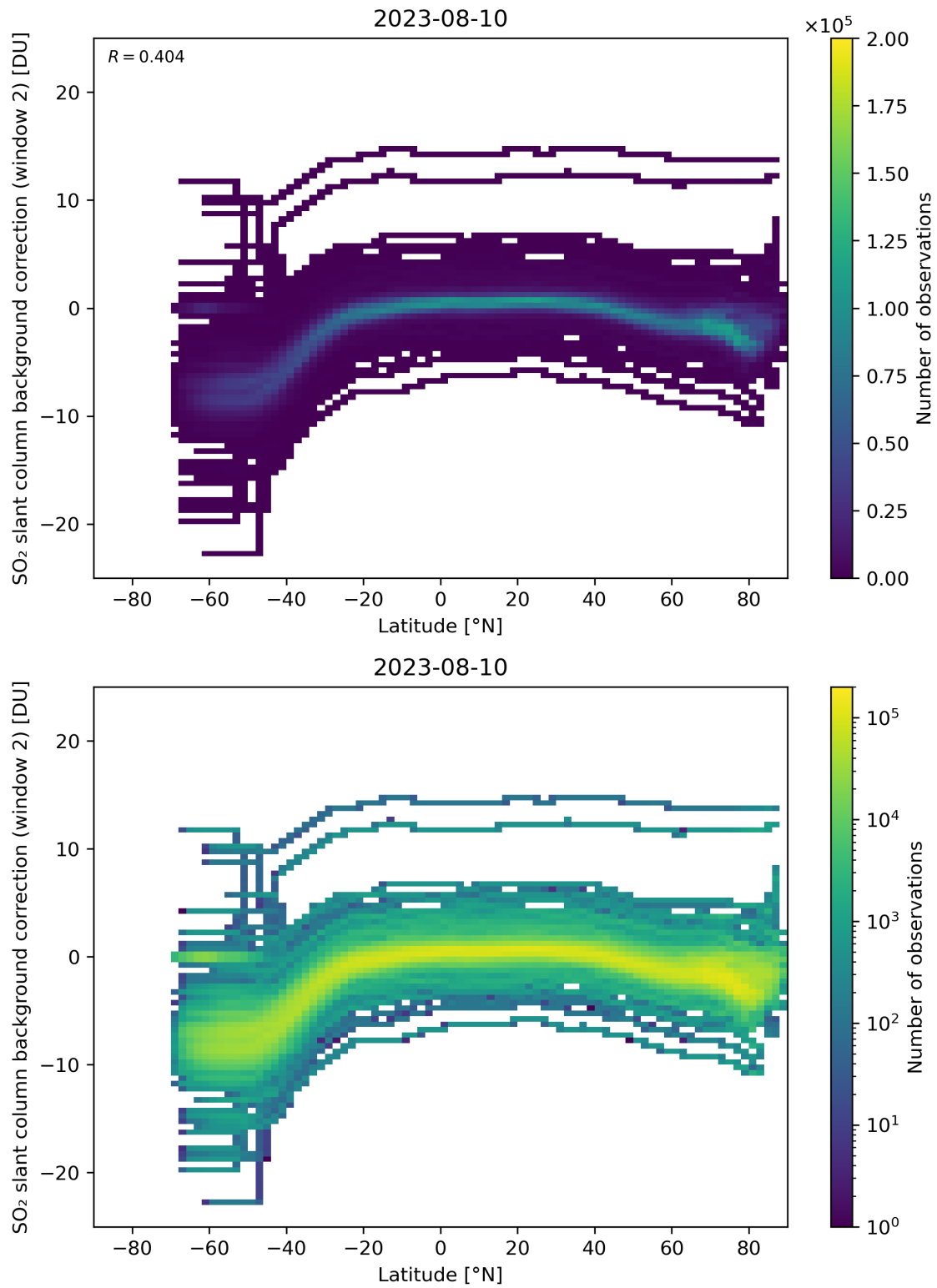
Figure 140: Scatter density plot of “Latitude” against “SO 2 slant column background correction (window 2)” for 2023-08-09 to 2023-08-11.
