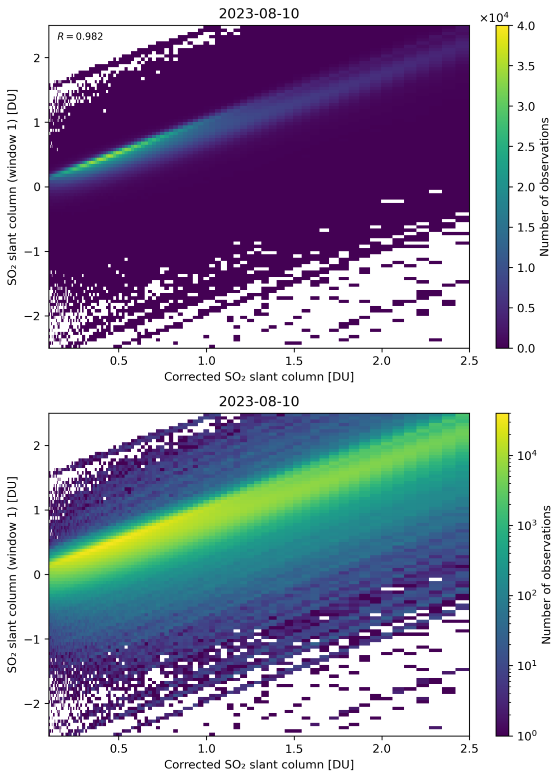
Figure 187: Scatter density plot of “Corrected SO 2 slant column” against “SO 2 slant column (window 1)” for 2023-08-09 to 2023-08-11.
