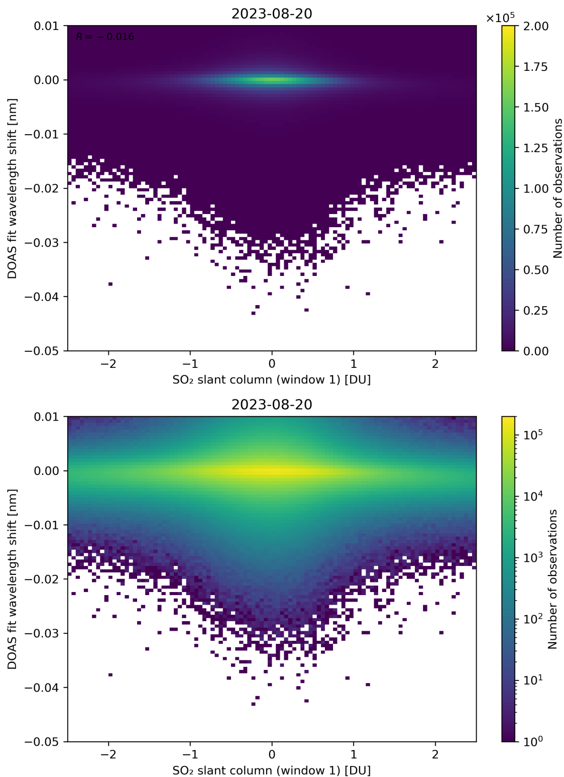
Figure 215: Scatter density plot of “SO 2 slant column (window 1)” against “DOAS fit wavelength shift” for 2023-08-20 to 2023-08-21.
