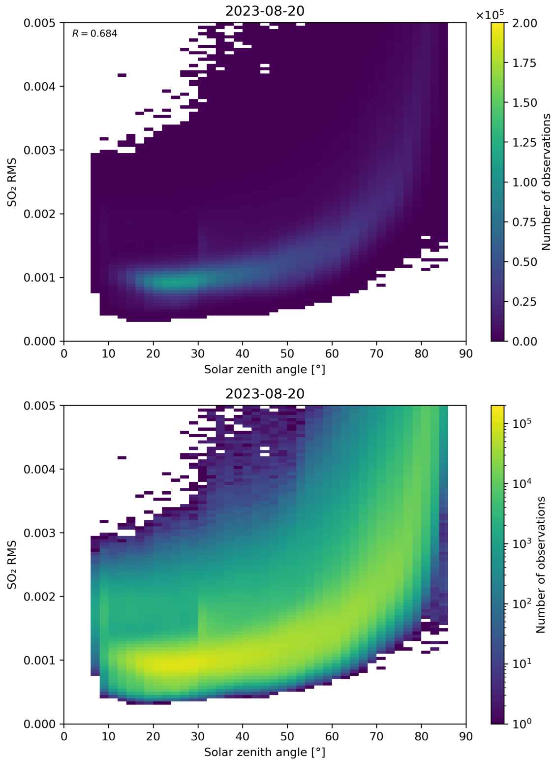
Figure 163: Scatter density plot of “Solar zenith angle” against “SO 2 RMS” for 2023-08-20 to 2023-08-21.
