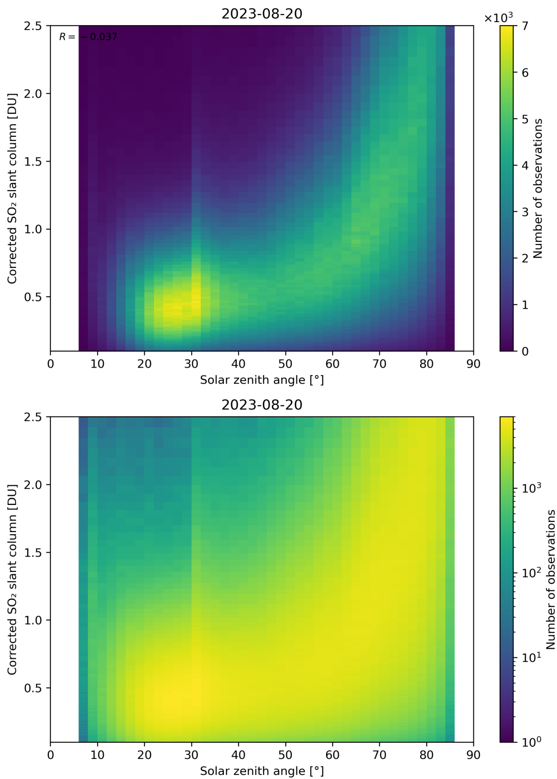
Figure 166: Scatter density plot of “Solar zenith angle” against “Corrected SO 2 slant column” for 2023-08-20 to 2023-08-21.
