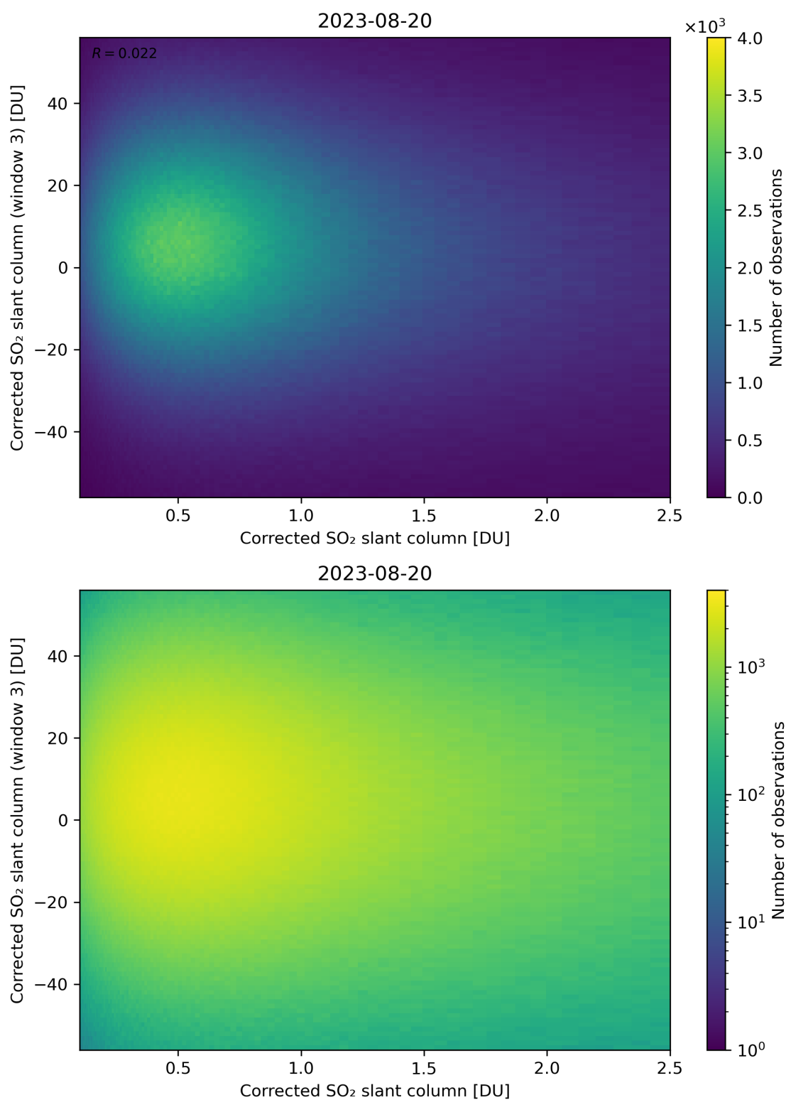
Figure 186: Scatter density plot of “Corrected SO 2 slant column” against “Corrected SO 2 slant column (window 3)” for 2023-08-20 to 2023-08-21.
