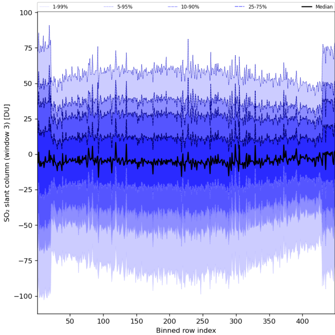
Figure 87: Along track statistics of “SO 2 slant column (window 3)” for 2023-08-20 to 2023-08-21
