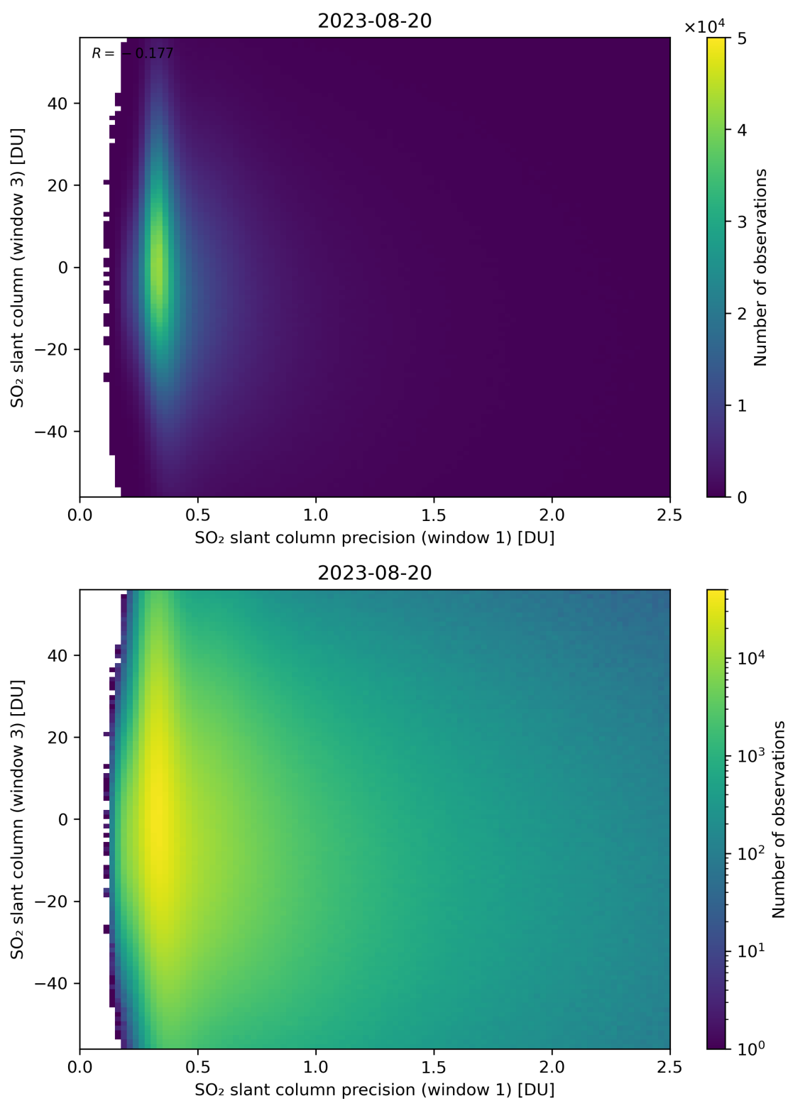
Figure 228: Scatter density plot of “SO 2 slant column precision (window 1)” against “SO 2 slant column (window 3)” for 2023-08-20 to 2023-08-21.
