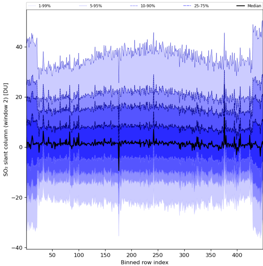
Figure 83: Along track statistics of “SO 2 slant column (window 2)” for 2023-08-20 to 2023-08-21
