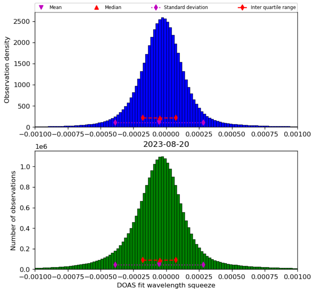
Figure 69: Histogram of “DOAS fit wavelength squeeze” for 2023-08-20 to 2023-08-21
