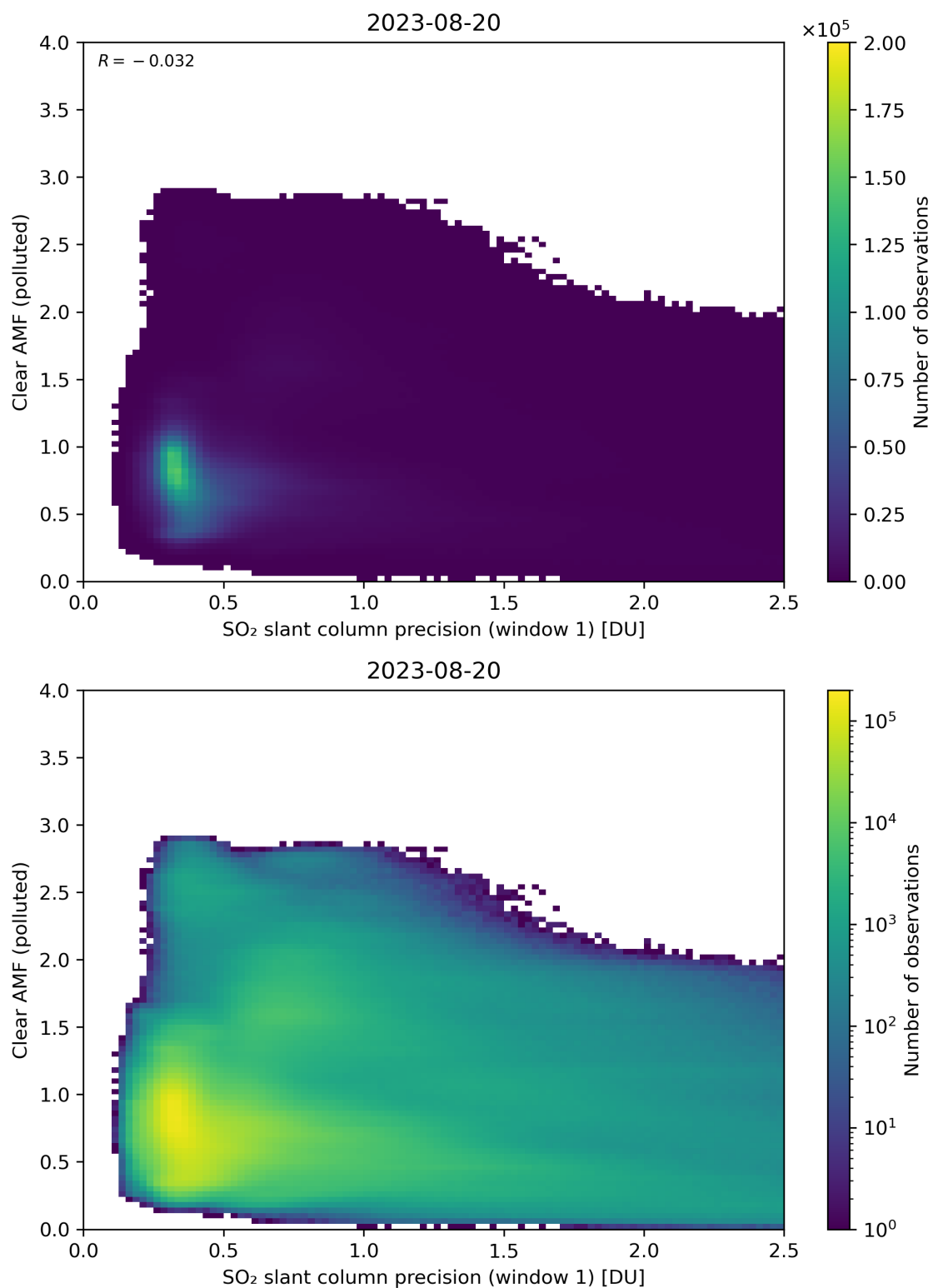
Figure 224: Scatter density plot of “SO 2 slant column precision (window 1)” against “Clear AMF (polluted)” for 2023-08-20 to 2023-08-21.
