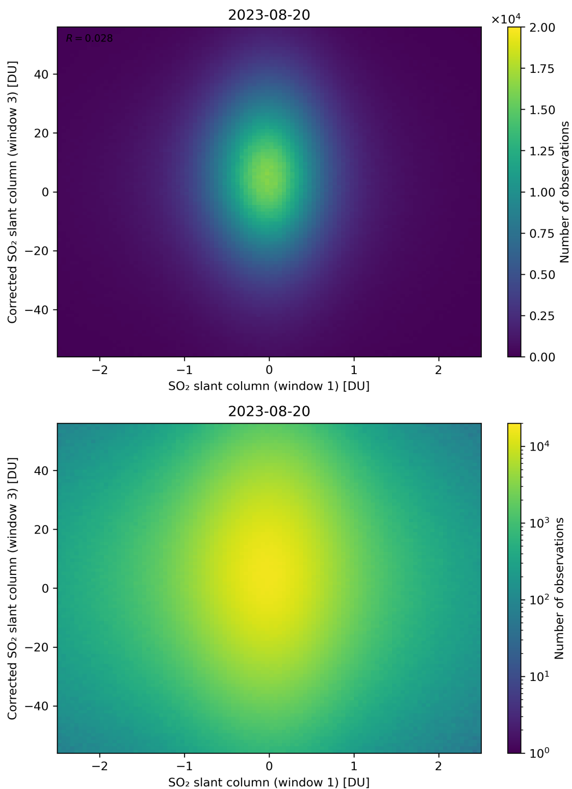
Figure 234: Scatter density plot of “SO 2 slant column (window 1)” against “Corrected SO 2 slant column (window 3)” for 2023-08-20 to 2023-08-21.
