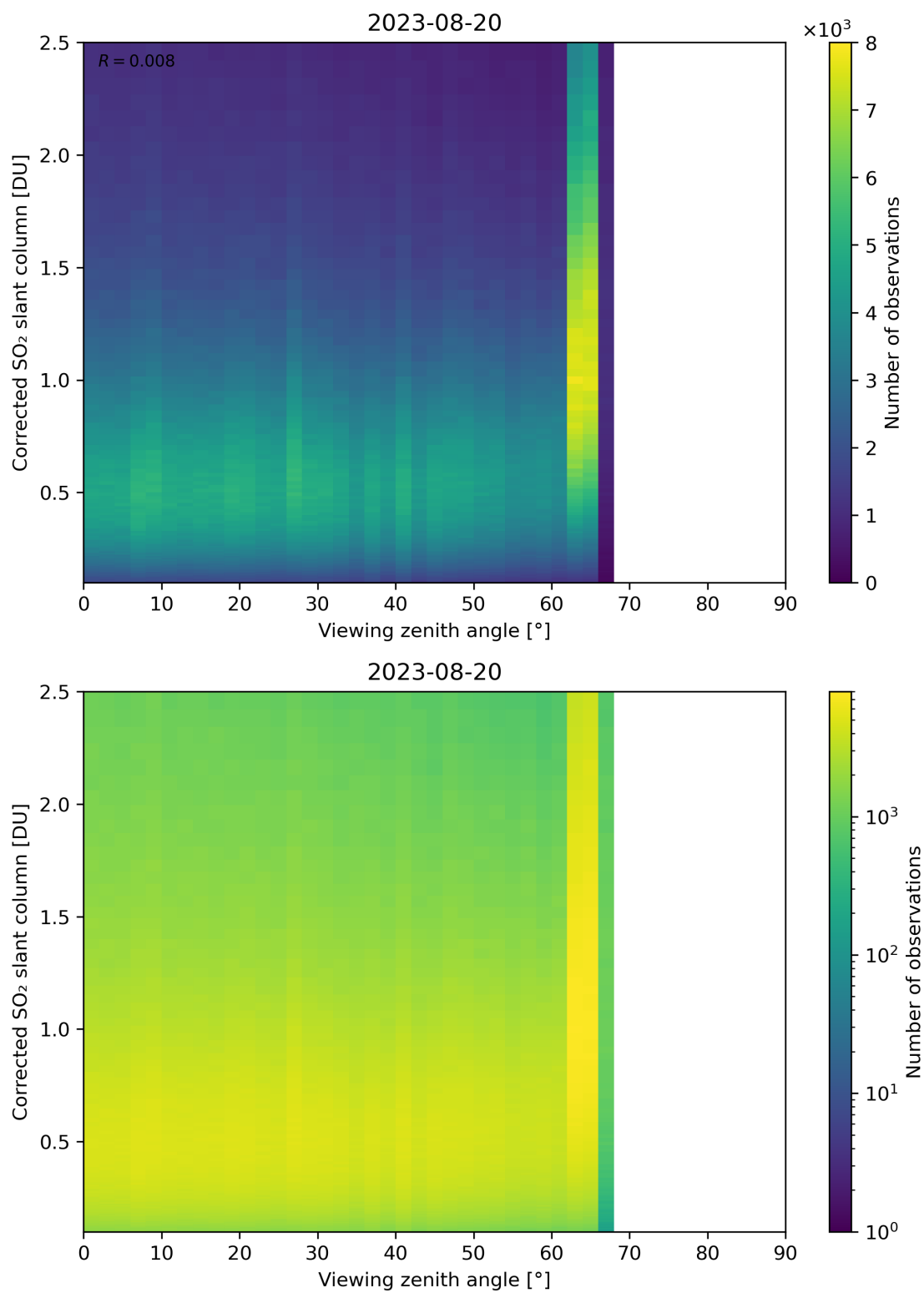
Figure 317: Scatter density plot of “Viewing zenith angle” against “Corrected SO 2 slant column” for 2023-08-20 to 2023-08-21.
