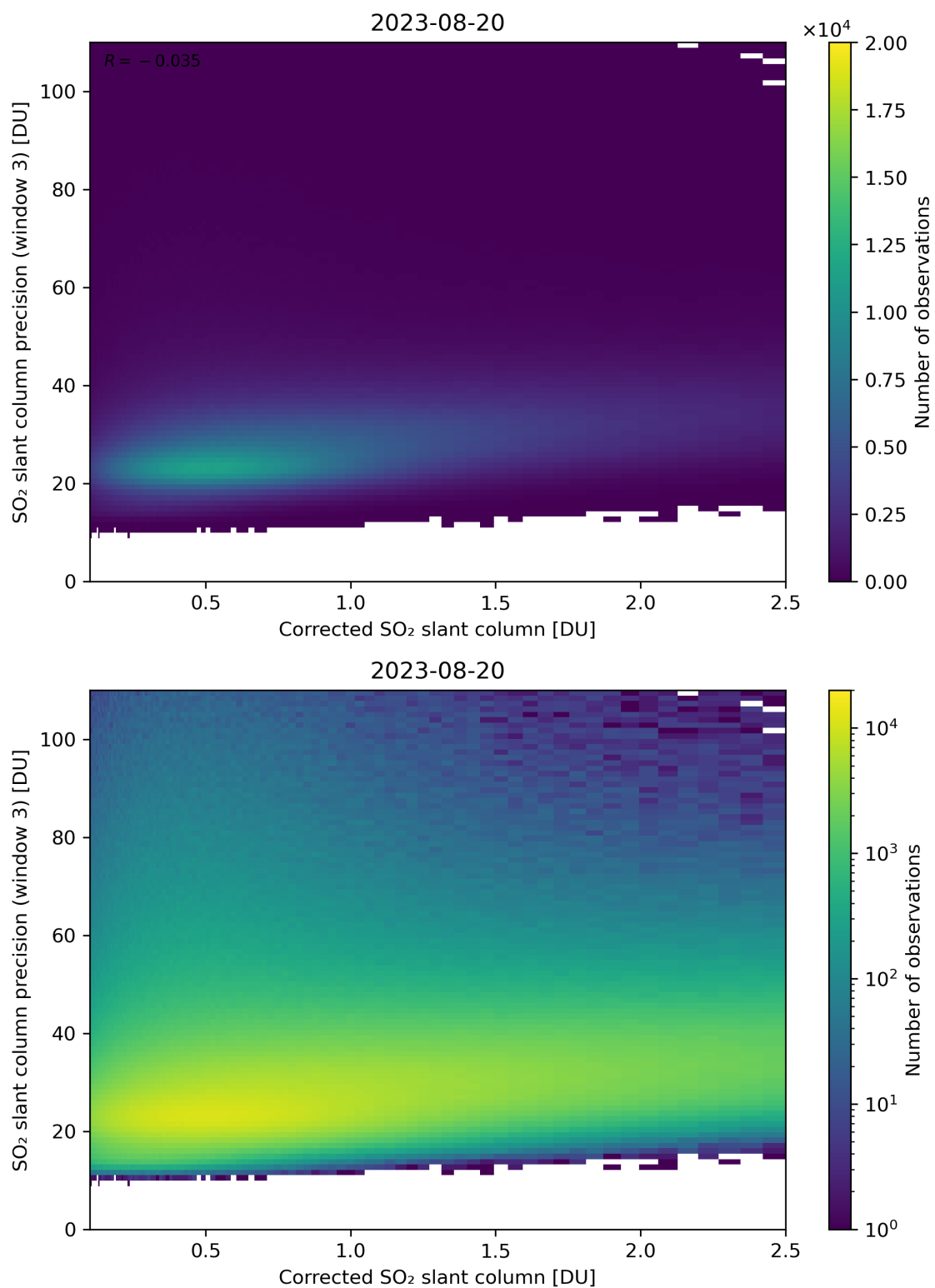
Figure 191: Scatter density plot of “Corrected SO 2 slant column” against “SO 2 slant column precision (window 3)” for 2023-08-20 to 2023-08-21.
