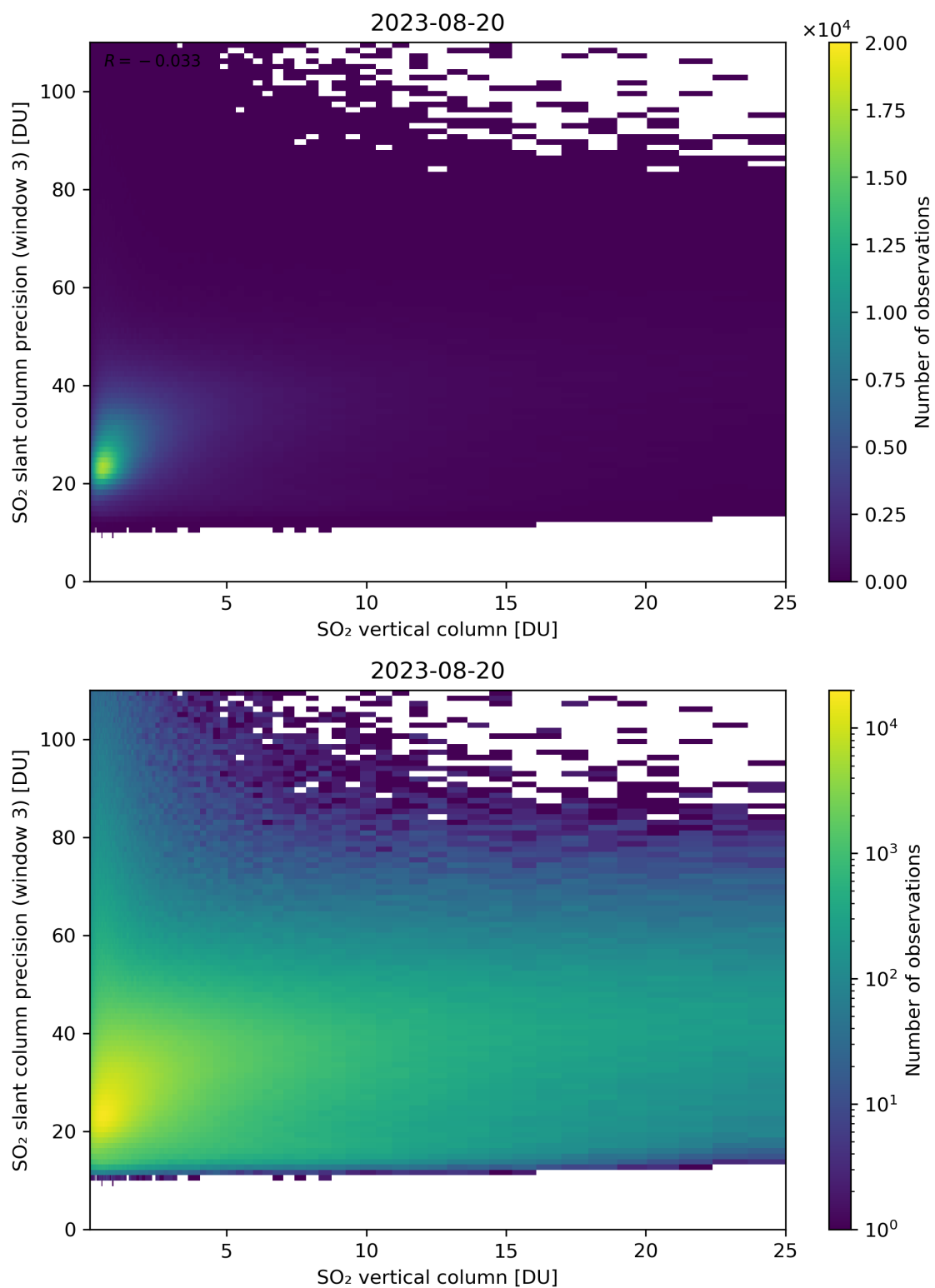
Figure 304: Scatter density plot of “SO 2 vertical column” against “SO 2 slant column precision (window 3)” for 2023-08-20 to 2023-08-21.
