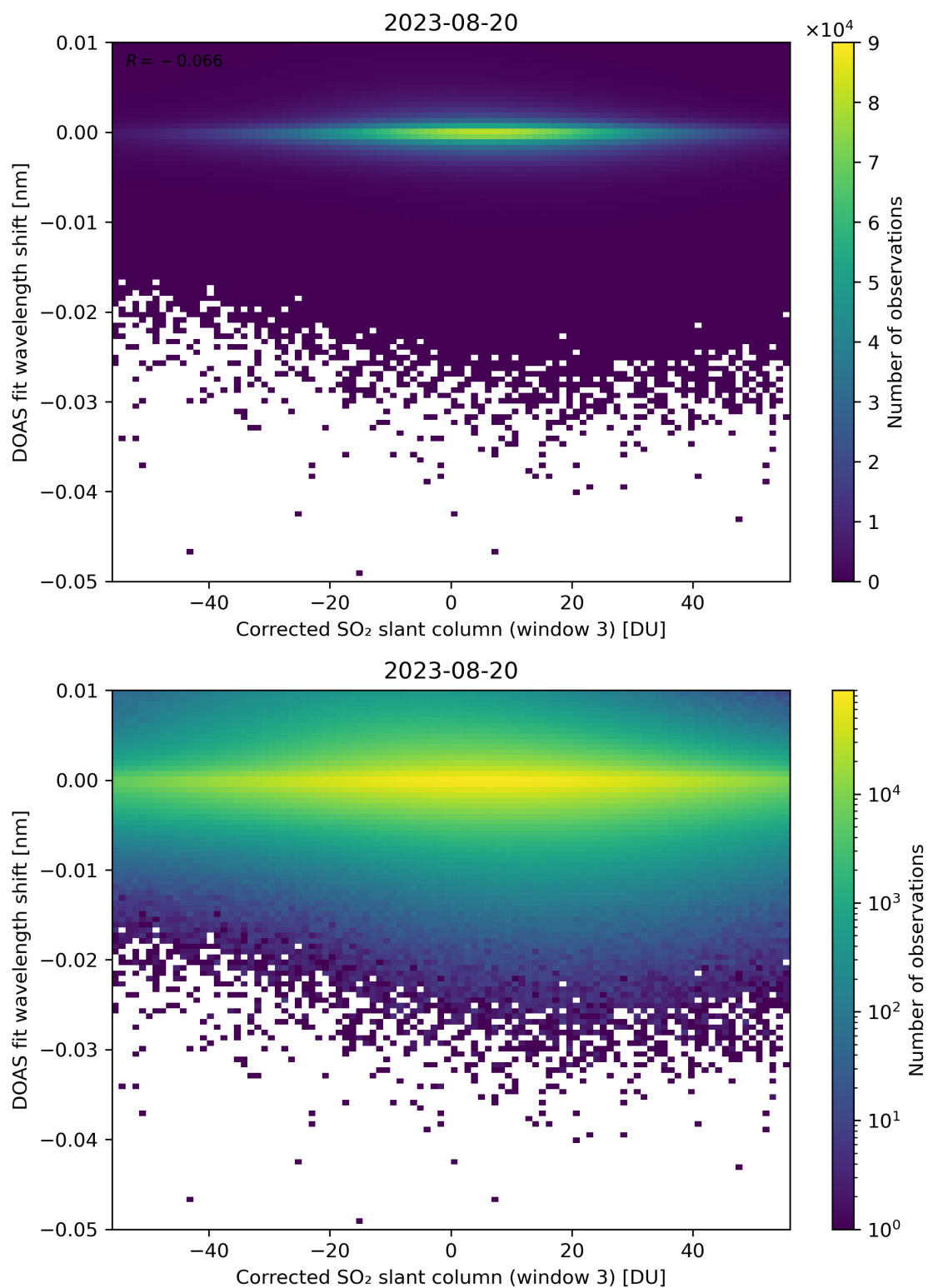
Figure 206: Scatter density plot of “Corrected SO 2 slant column (window 3)” against “DOAS fit wavelength shift” for 2023-08-20 to 2023-08-21.
