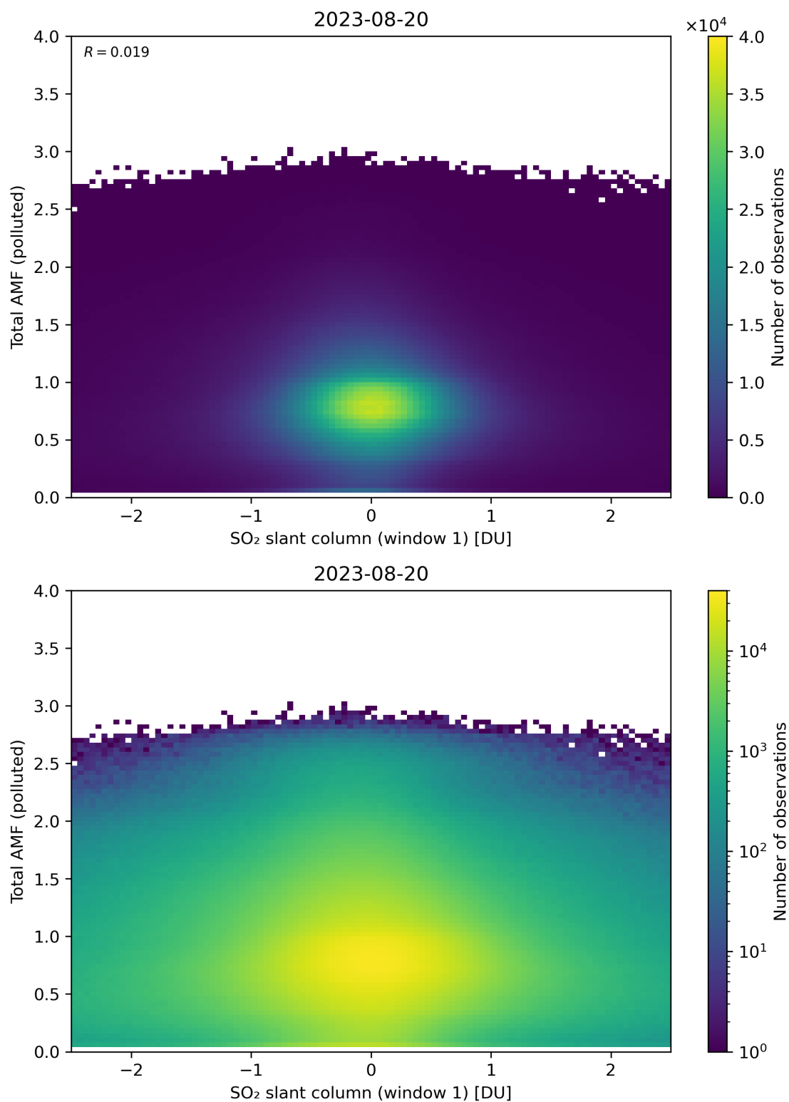
Figure 239: Scatter density plot of “SO 2 slant column (window 1)” against “Total AMF (polluted)” for 2023-08-20 to 2023-08-21.
