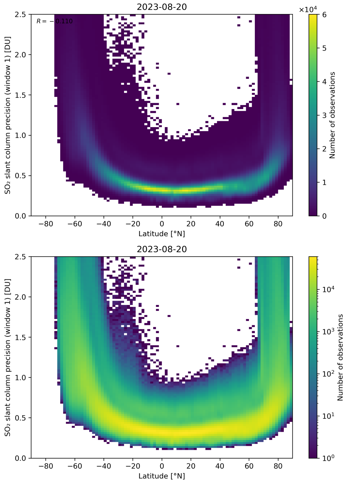
Figure 150: Scatter density plot of “Latitude” against “SO 2 slant column precision (window 1)” for 2023-08-20 to 2023-08-21.
