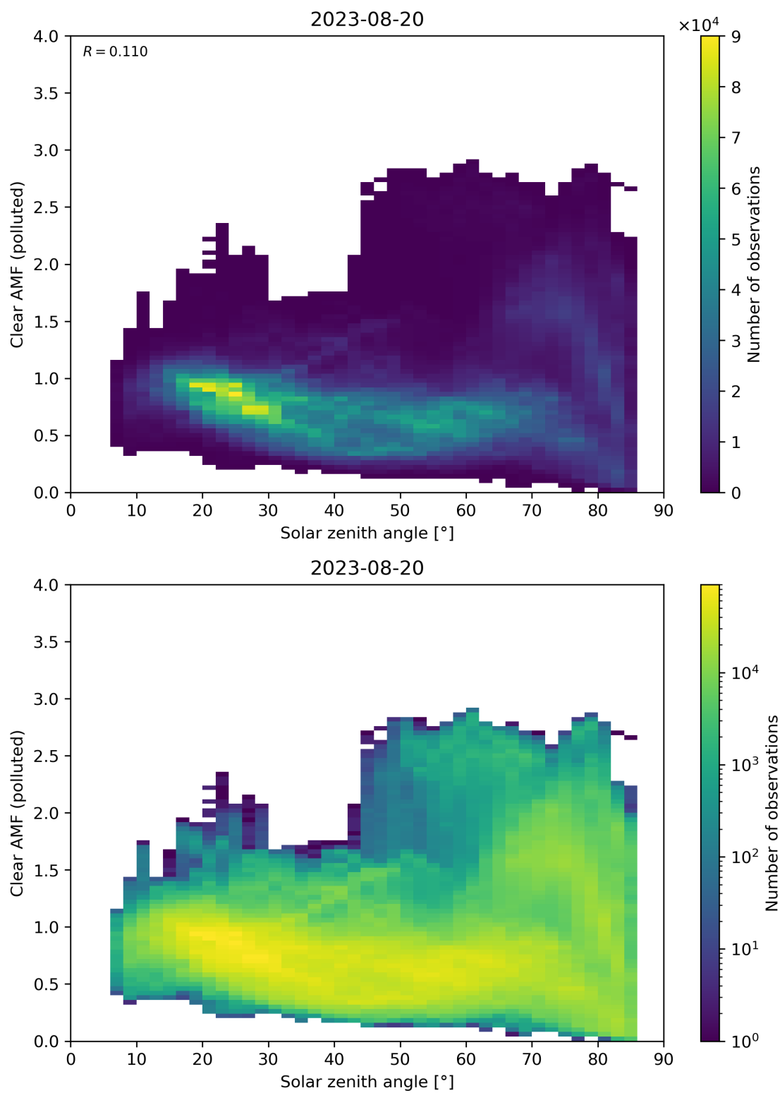
Figure 165: Scatter density plot of “Solar zenith angle” against “Clear AMF (polluted)” for 2023-08-20 to 2023-08-21.
