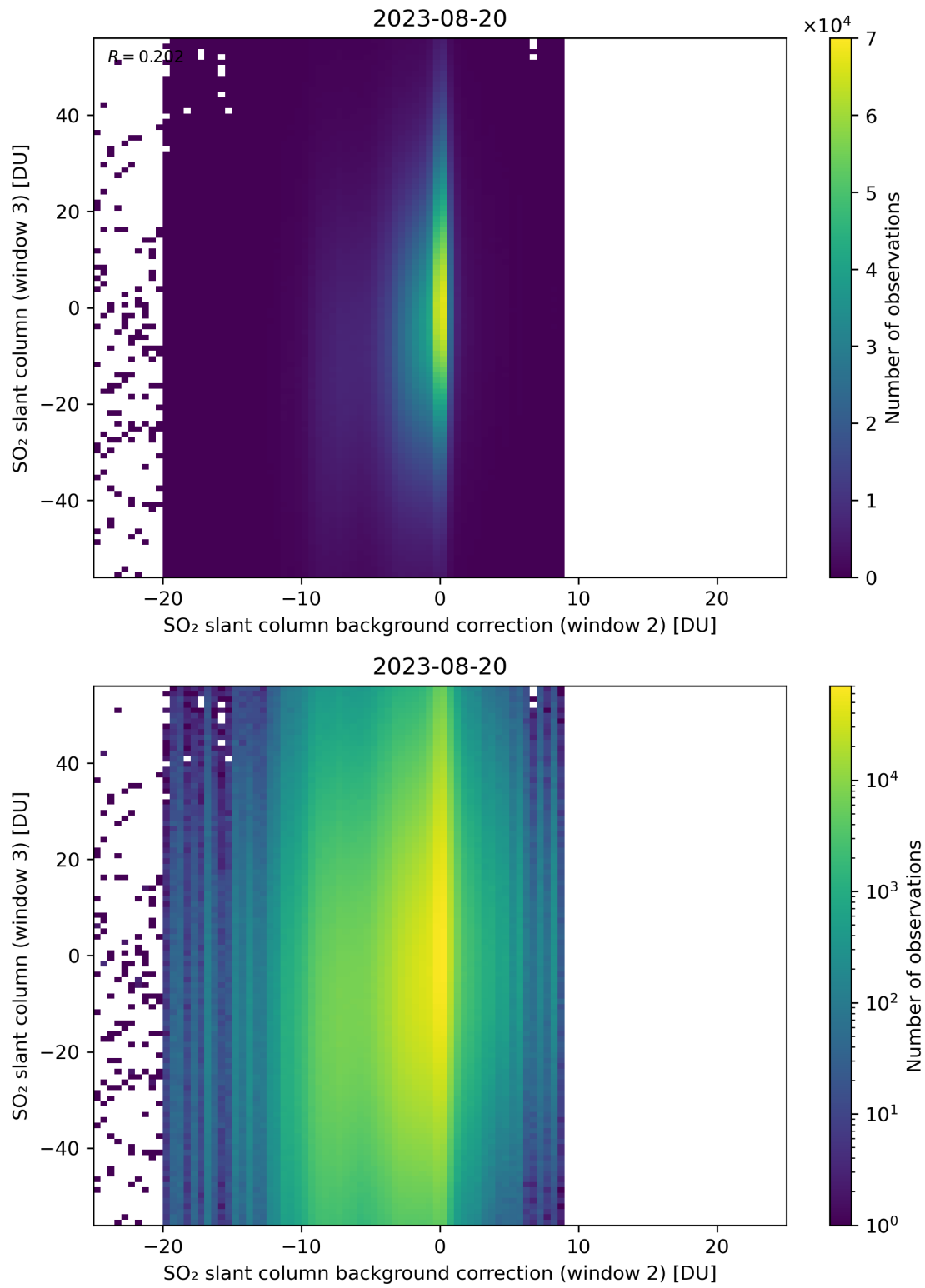
Figure 117: Scatter density plot of “SO 2 slant column background correction (window 2)” against “SO 2 slant column (window 3)” for 2023-08-20 to 2023-08-21.
