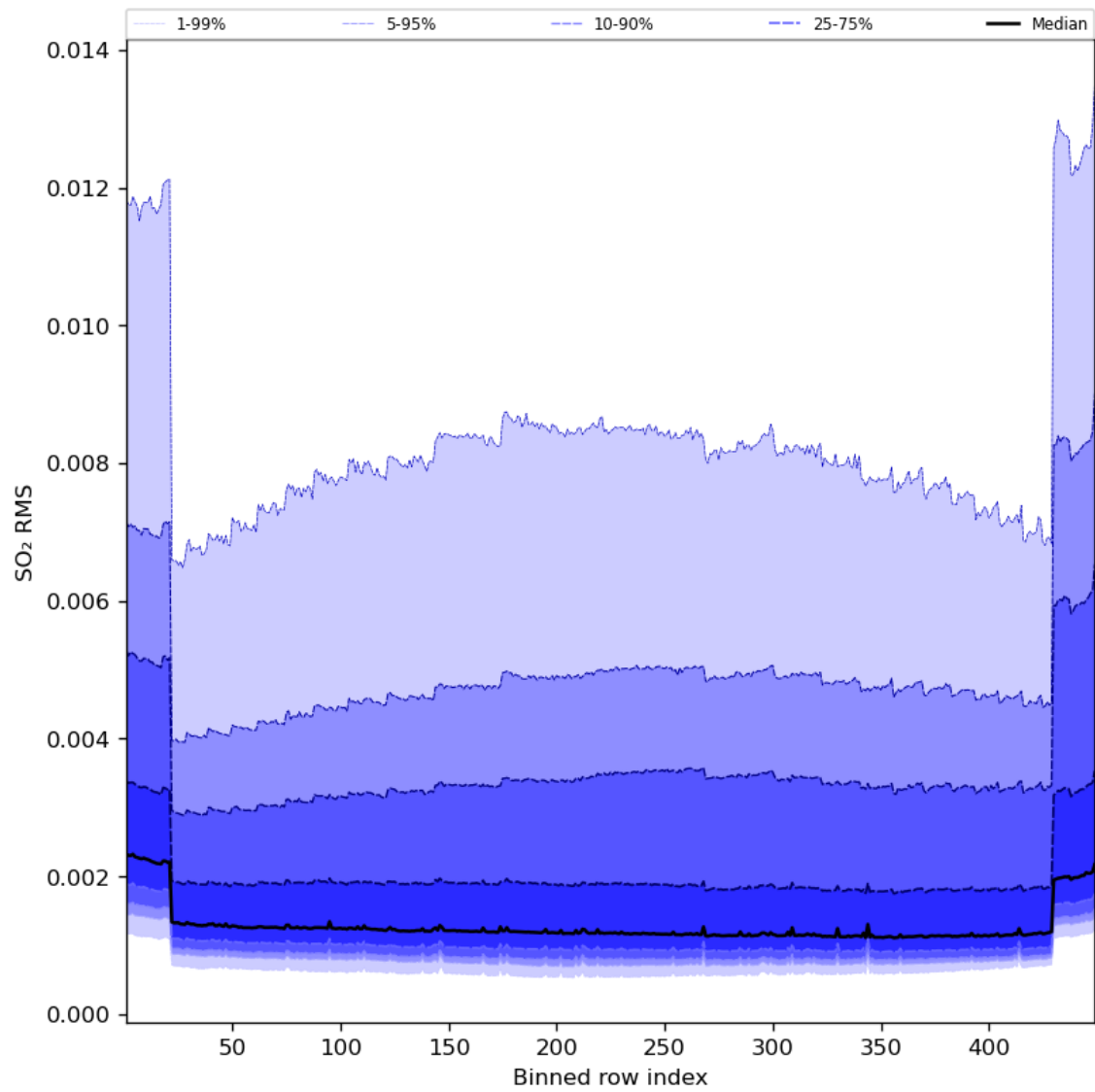
Figure 93: Along track statistics of “SO 2 RMS” for 2023-08-20 to 2023-08-21
