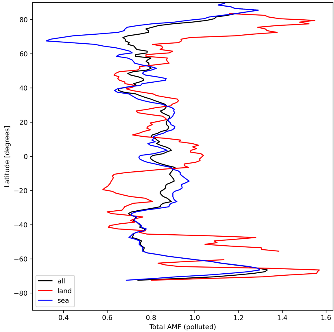
Figure 48: Zonal average of “Total AMF (polluted)” for 2023-08-20 to 2023-08-21.
