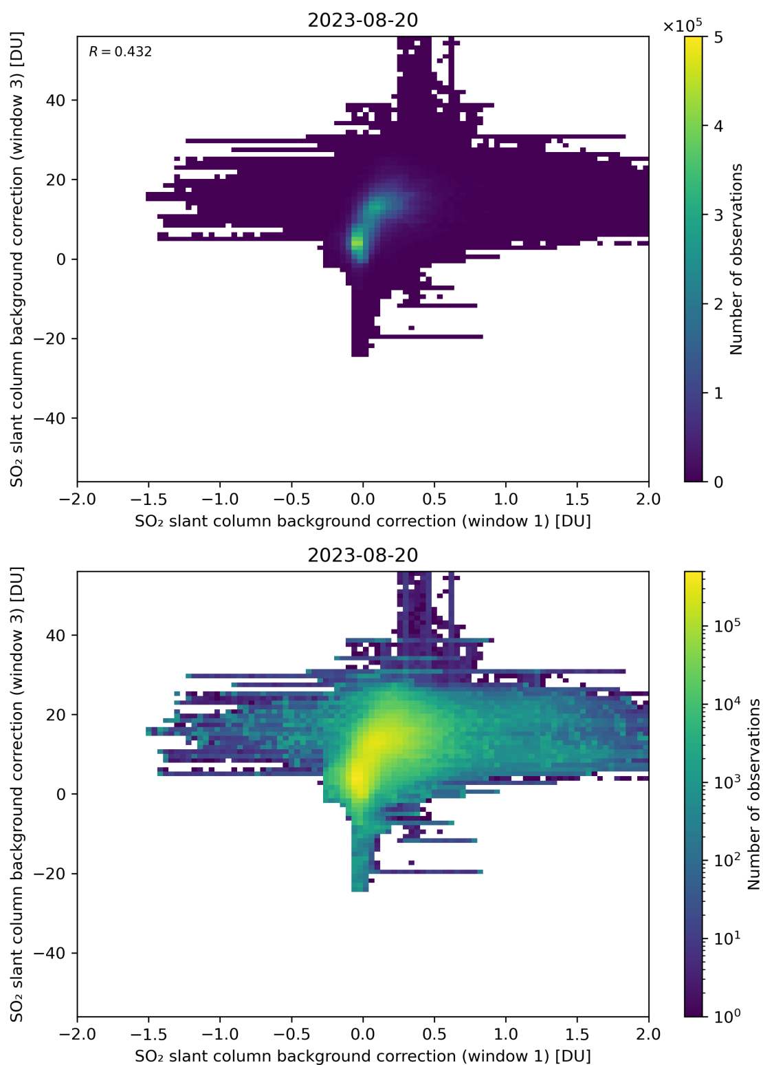
Figure 99: Scatter density plot of “SO 2 slant column background correction (window 1)” against “SO 2 slant column background correction (window 3)” for 2023-08-20 to 2023-08-21.
