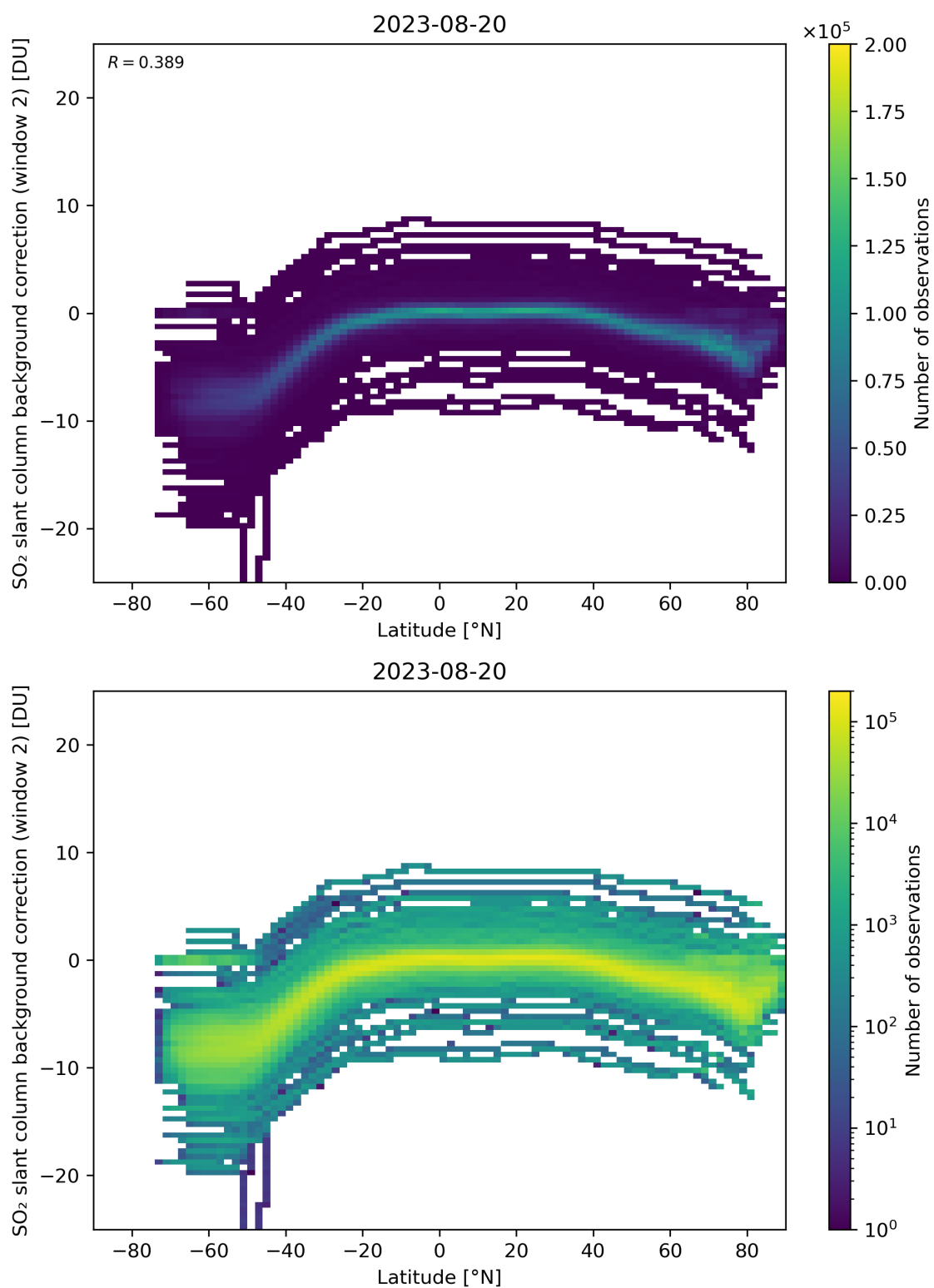
Figure 140: Scatter density plot of “Latitude” against “SO 2 slant column background correction (window 2)” for 2023-08-20 to 2023-08-21.
