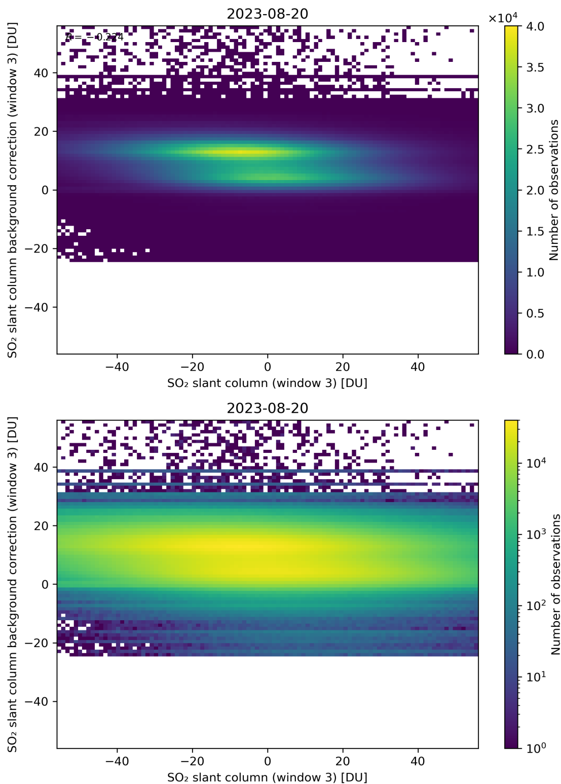
Figure 253: Scatter density plot of “SO 2 slant column (window 3)” against “SO 2 slant column background correction (window 3)” for 2023-08-20 to 2023-08-21.
