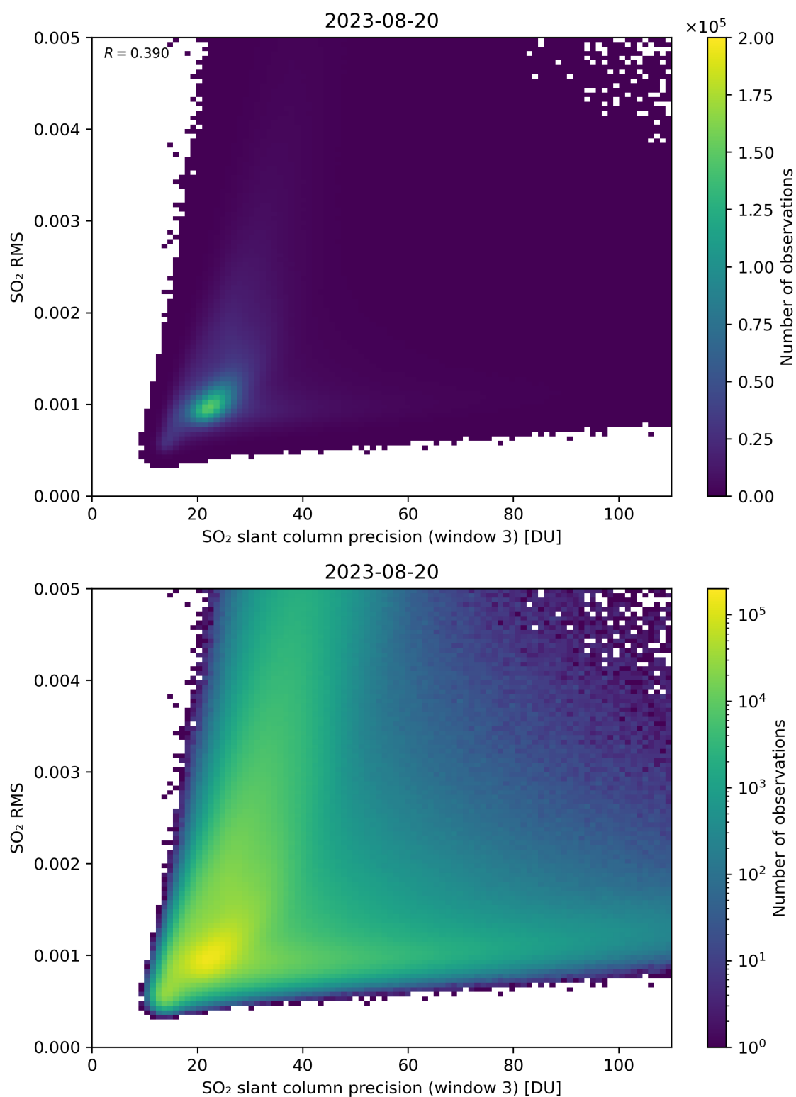
Figure 260: Scatter density plot of “SO 2 slant column precision (window 3)” against “SO 2 RMS” for 2023-08-20 to 2023-08-21.
