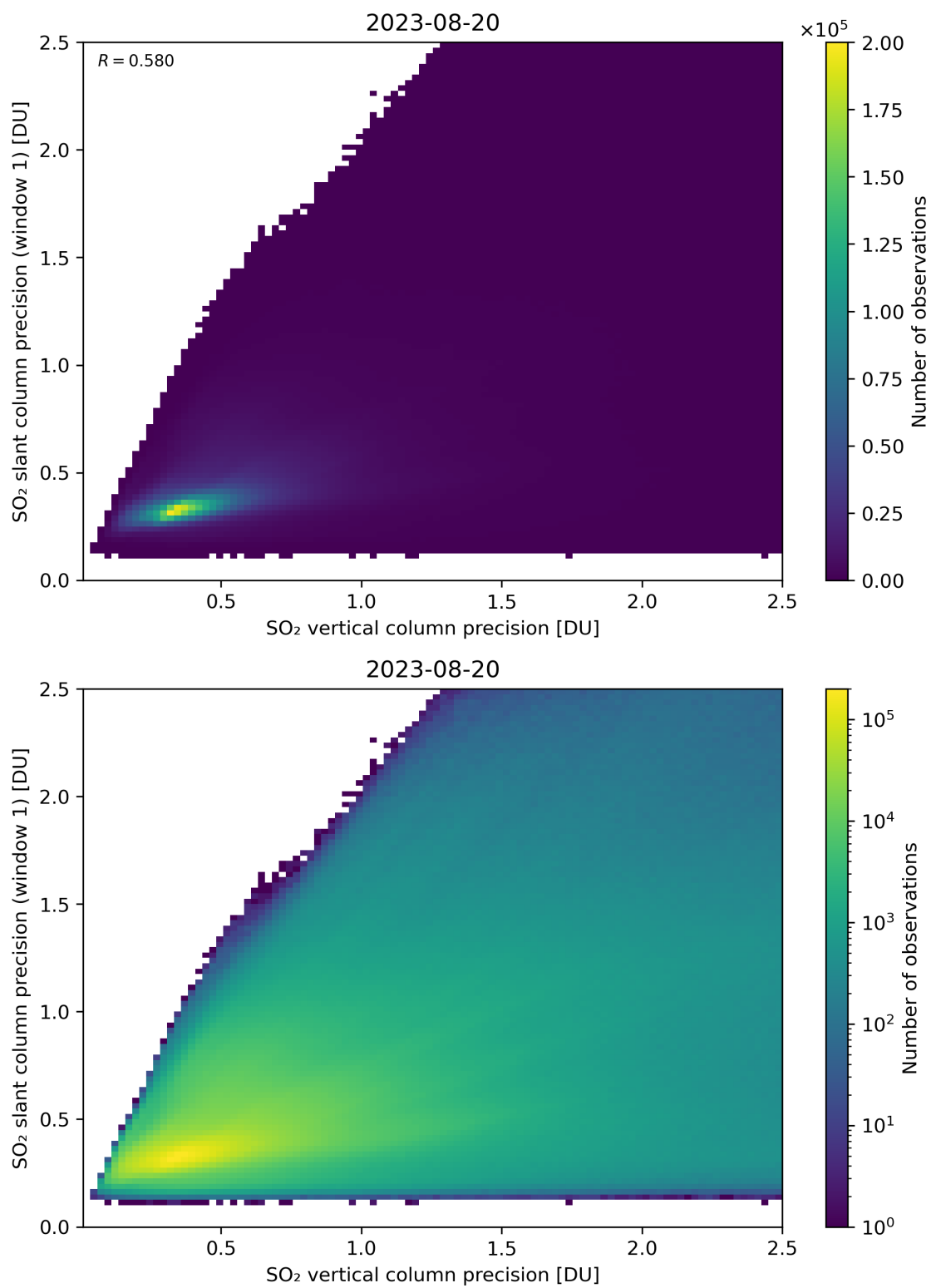
Figure 290: Scatter density plot of “SO 2 vertical column precision” against “SO 2 slant column precision (window 1)” for 2023-08-20 to 2023-08-21.
