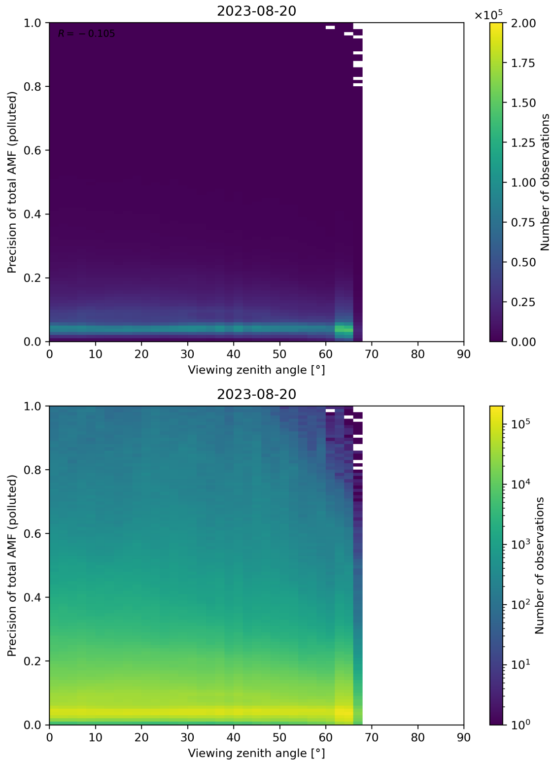
Figure 326: Scatter density plot of “Viewing zenith angle” against “Precision of total AMF (polluted)” for 2023-08-20 to 2023-08-21.
