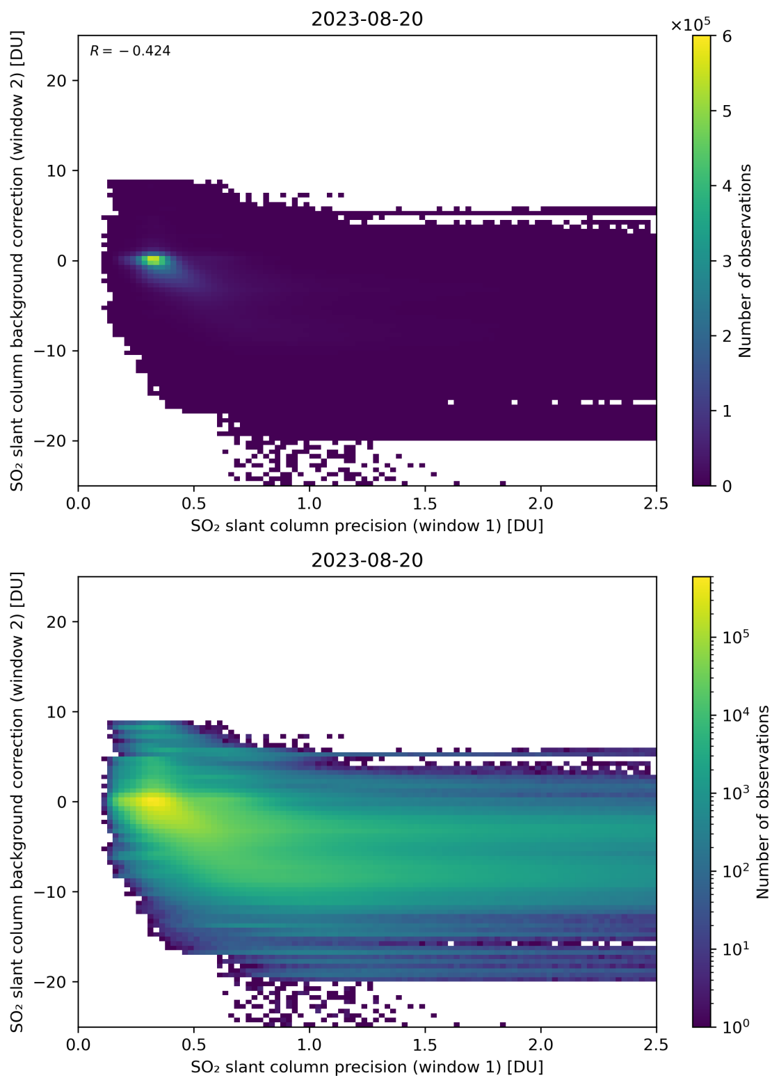
Figure 219: Scatter density plot of “SO 2 slant column precision (window 1)” against “SO 2 slant column background correction (window 2)” for 2023-08-20 to 2023-08-21.
