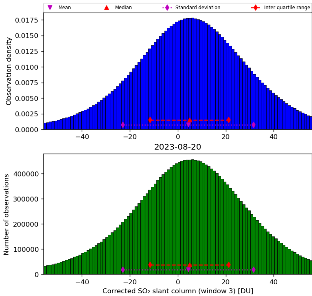
Figure 66: Histogram of “Corrected SO 2 slant column (window 3)” for 2023-08-20 to 2023-08-21
