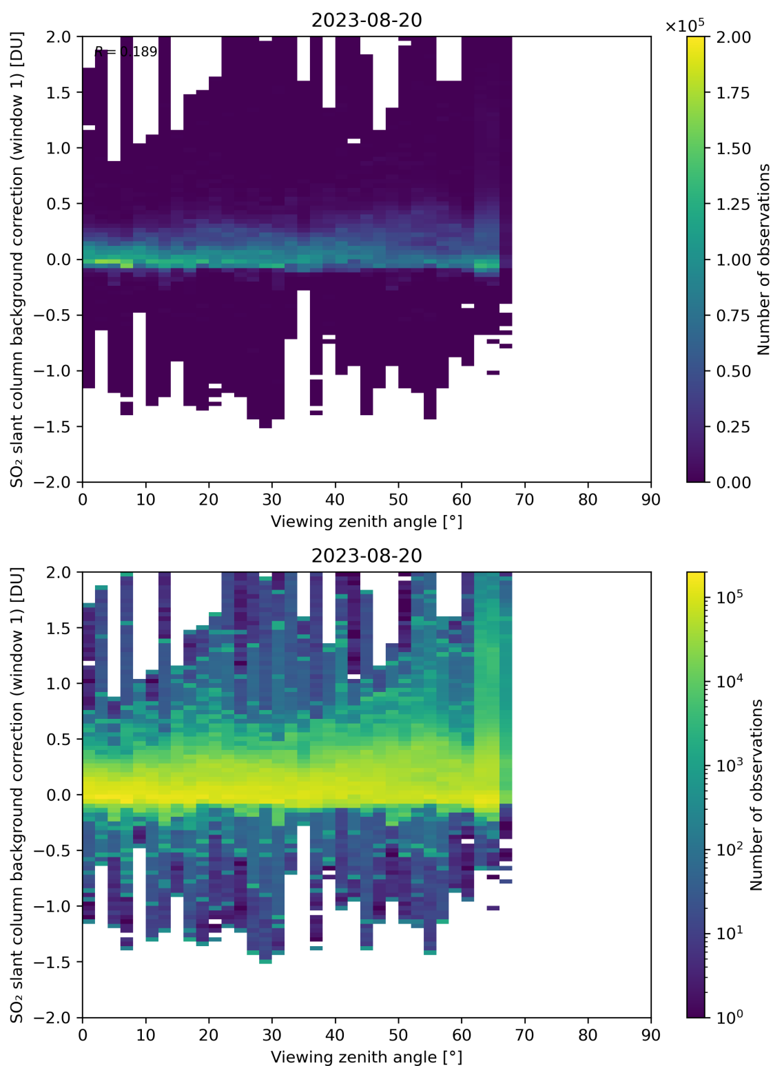
Figure 308: Scatter density plot of “Viewing zenith angle” against “SO 2 slant column background correction (window 1)” for 2023-08-20 to 2023-08-21.
