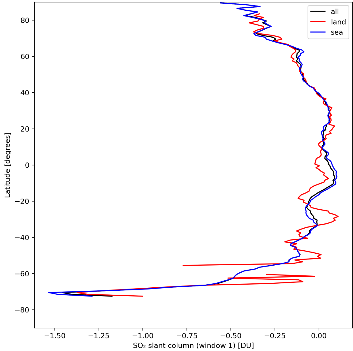
Figure 33: Zonal average of “SO 2 slant column (window 1)” for 2023-08-20 to 2023-08-21.
