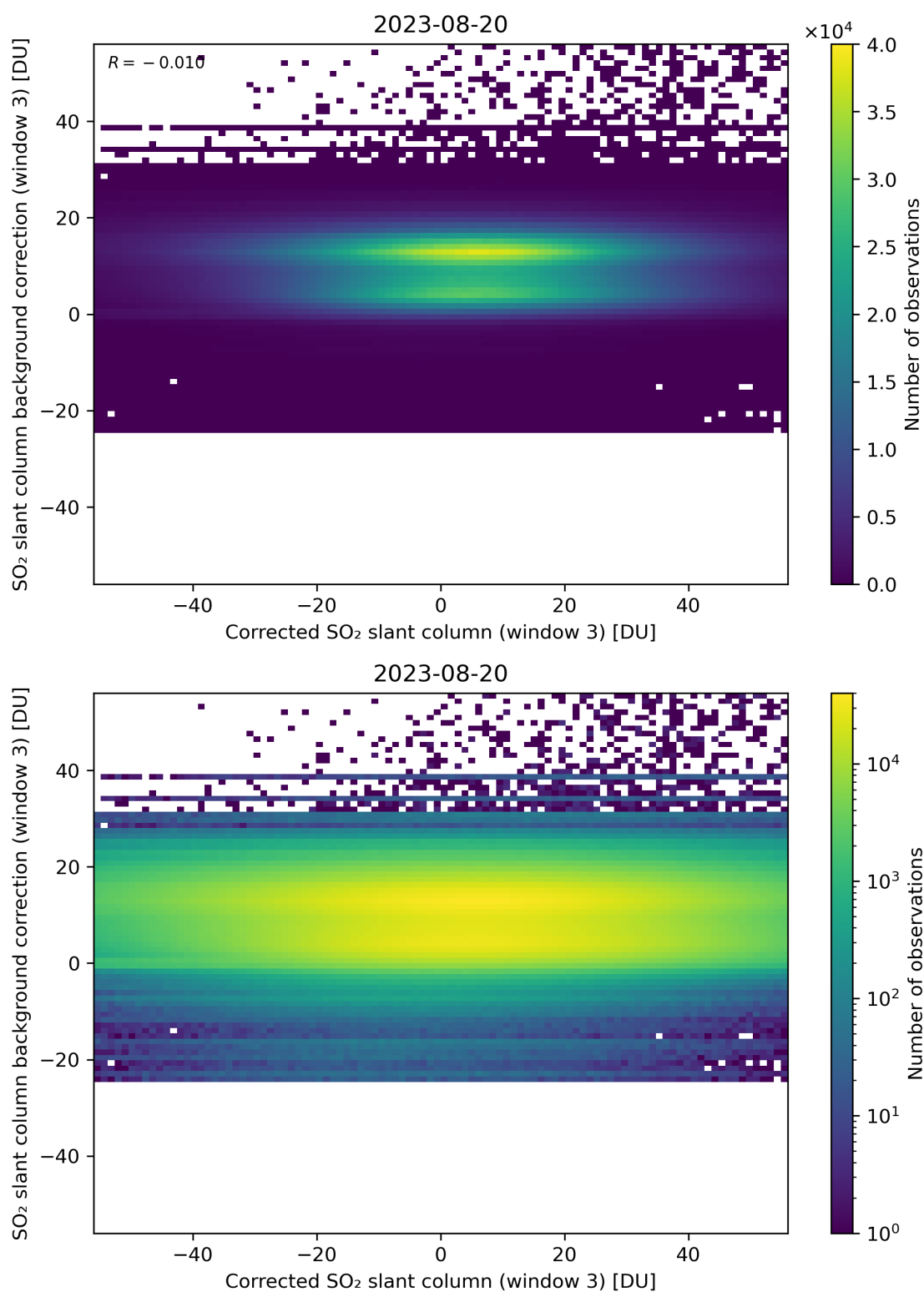
Figure 205: Scatter density plot of “Corrected SO 2 slant column (window 3)” against “SO 2 slant column background correction (window 3)” for 2023-08-20 to 2023-08-21.
