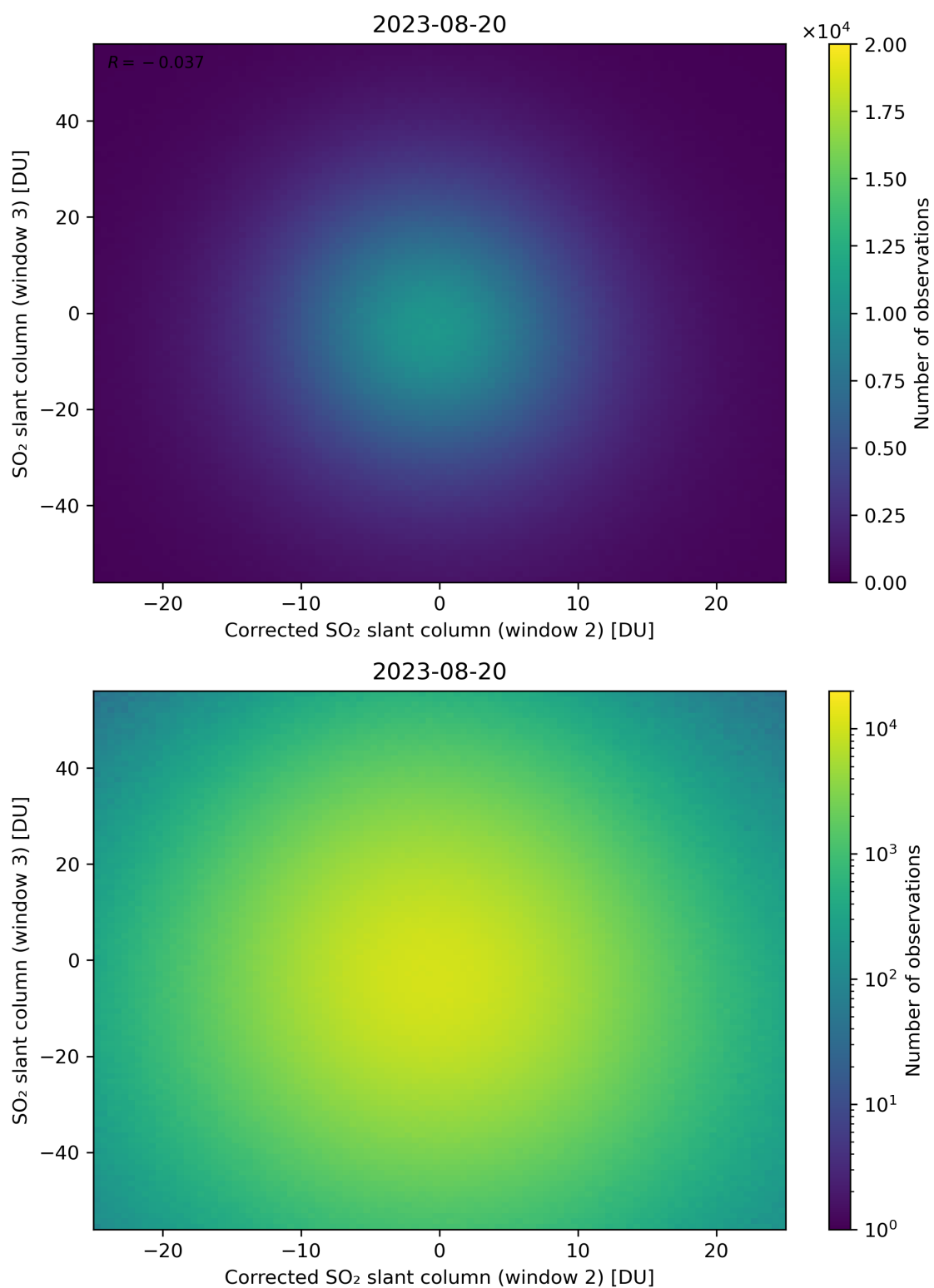
Figure 201: Scatter density plot of “Corrected SO 2 slant column (window 2)” against “SO 2 slant column (window 3)” for 2023-08-20 to 2023-08-21.
