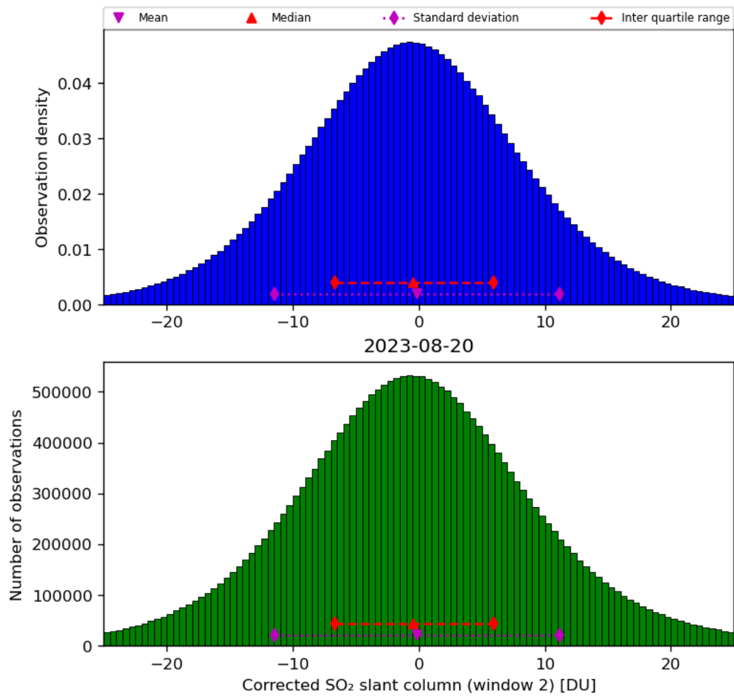
Figure 62: Histogram of “Corrected SO 2 slant column (window 2)” for 2023-08-20 to 2023-08-21
