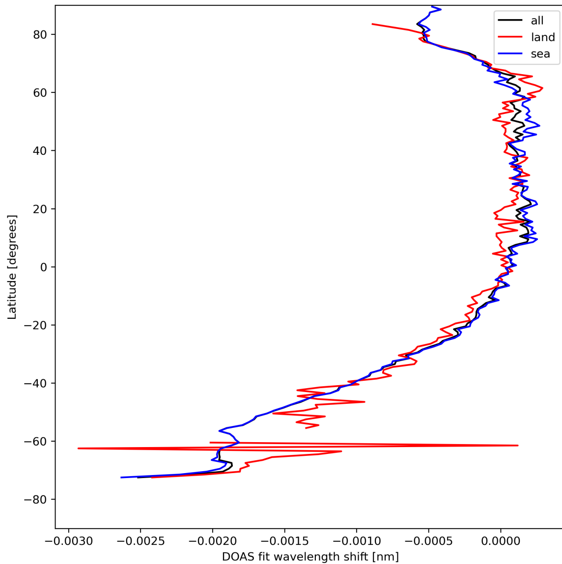
Figure 45: Zonal average of “DOAS fit wavelength shift” for 2023-08-20 to 2023-08-21.
