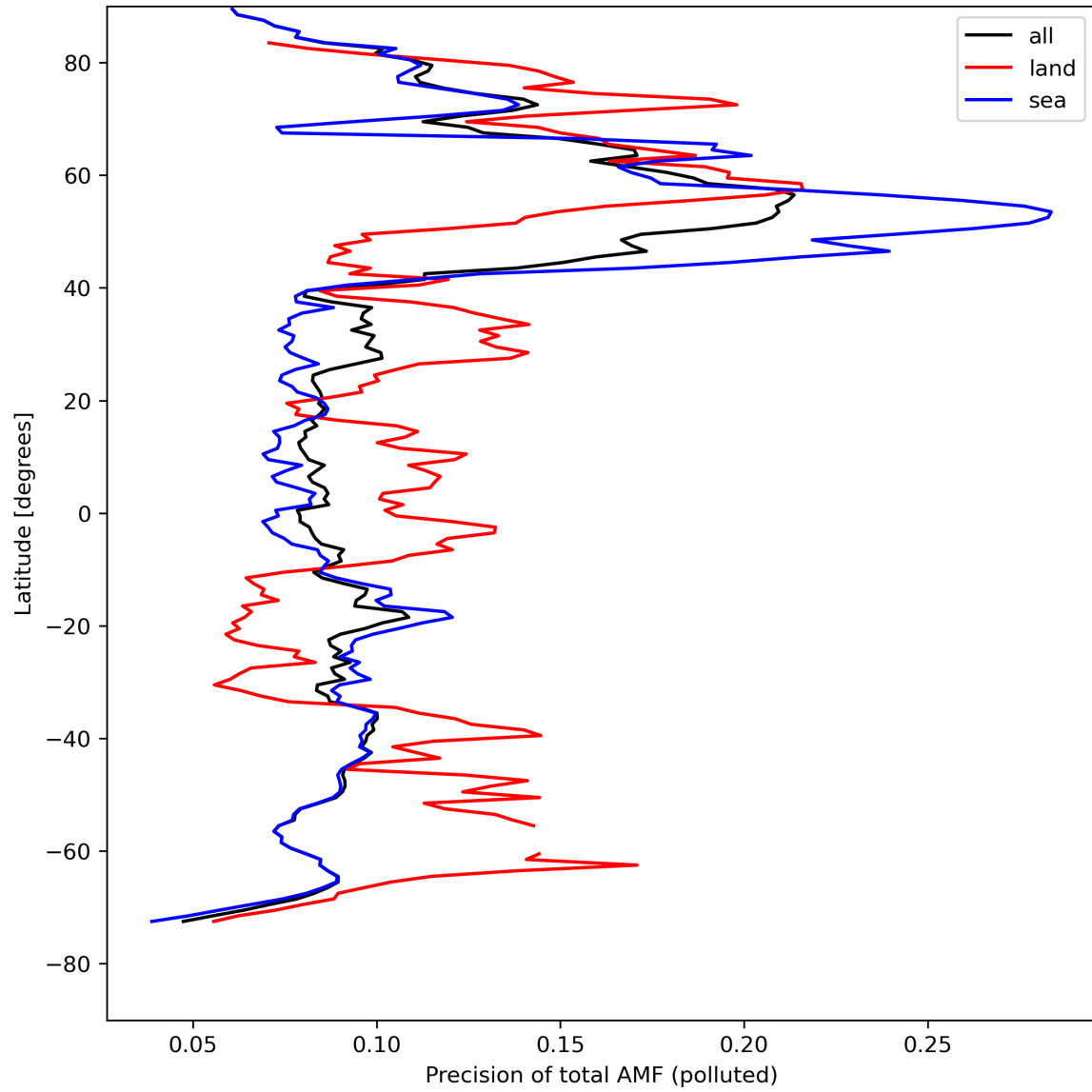
Figure 49: Zonal average of “Precision of total AMF (polluted)” for 2023-08-20 to 2023-08-21.
