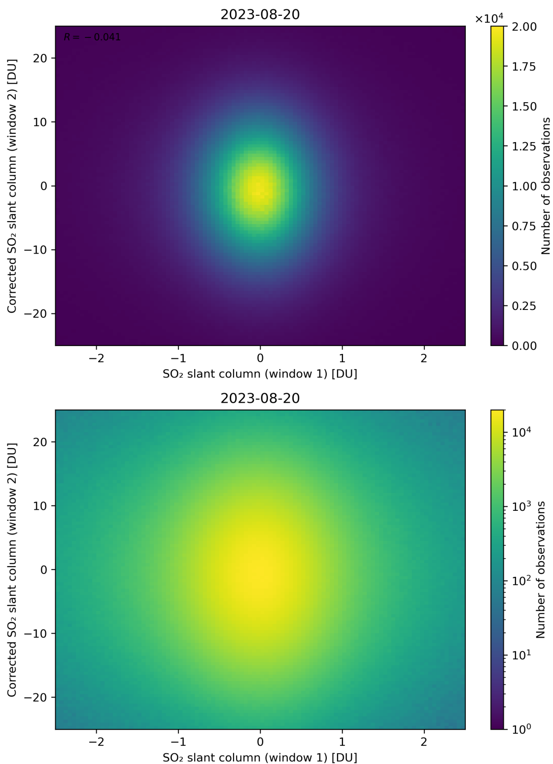
Figure 233: Scatter density plot of “SO 2 slant column (window 1)” against “Corrected SO 2 slant column (window 2)” for 2023-08-20 to 2023-08-21.
