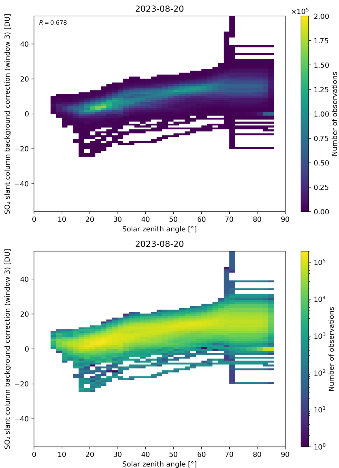
Figure 160: Scatter density plot of “Solar zenith angle” against “SO 2 slant column background correction (window 3)” for 2023-08-20 to 2023-08-21.
