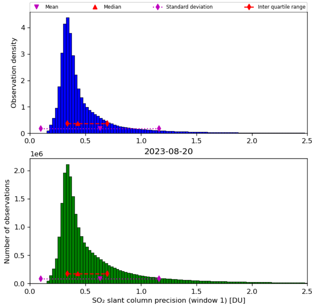
Figure 57: Histogram of “SO 2 slant column precision (window 1)” for 2023-08-20 to 2023-08-21
