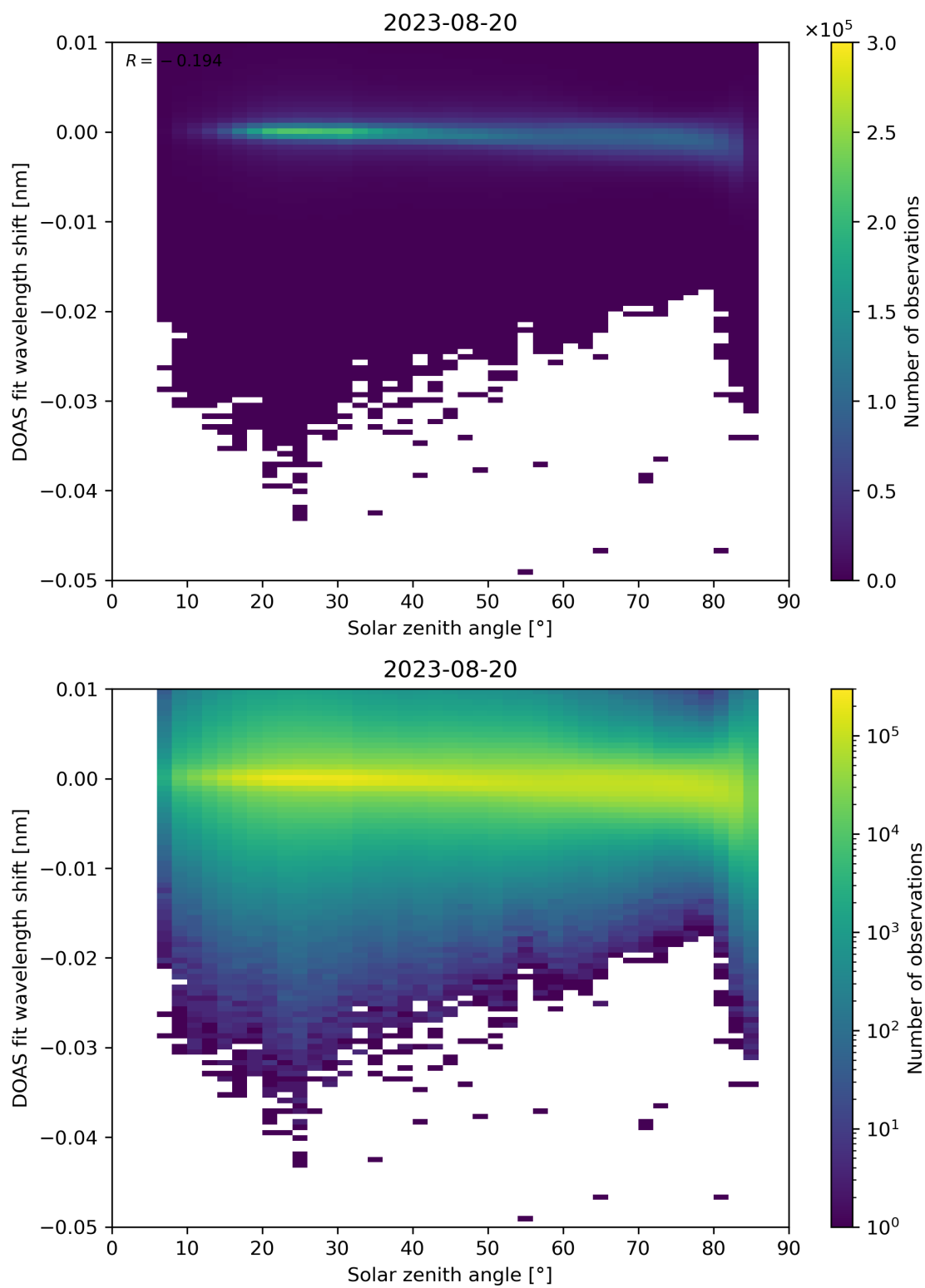
Figure 161: Scatter density plot of “Solar zenith angle” against “DOAS fit wavelength shift” for 2023-08-20 to 2023-08-21.
