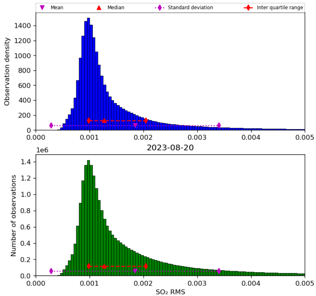
Figure 70: Histogram of “SO 2 RMS” for 2023-08-20 to 2023-08-21
