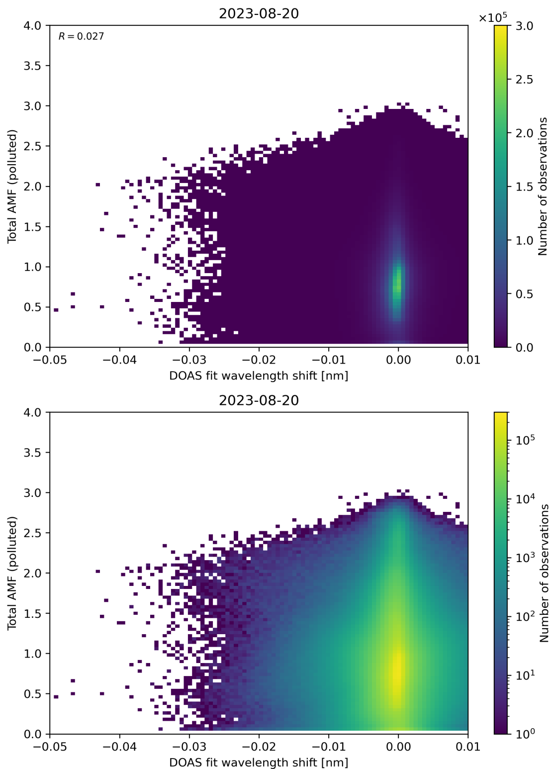
Figure 130: Scatter density plot of “DOAS fit wavelength shift” against “Total AMF (polluted)” for 2023-08-20 to 2023-08-21.
