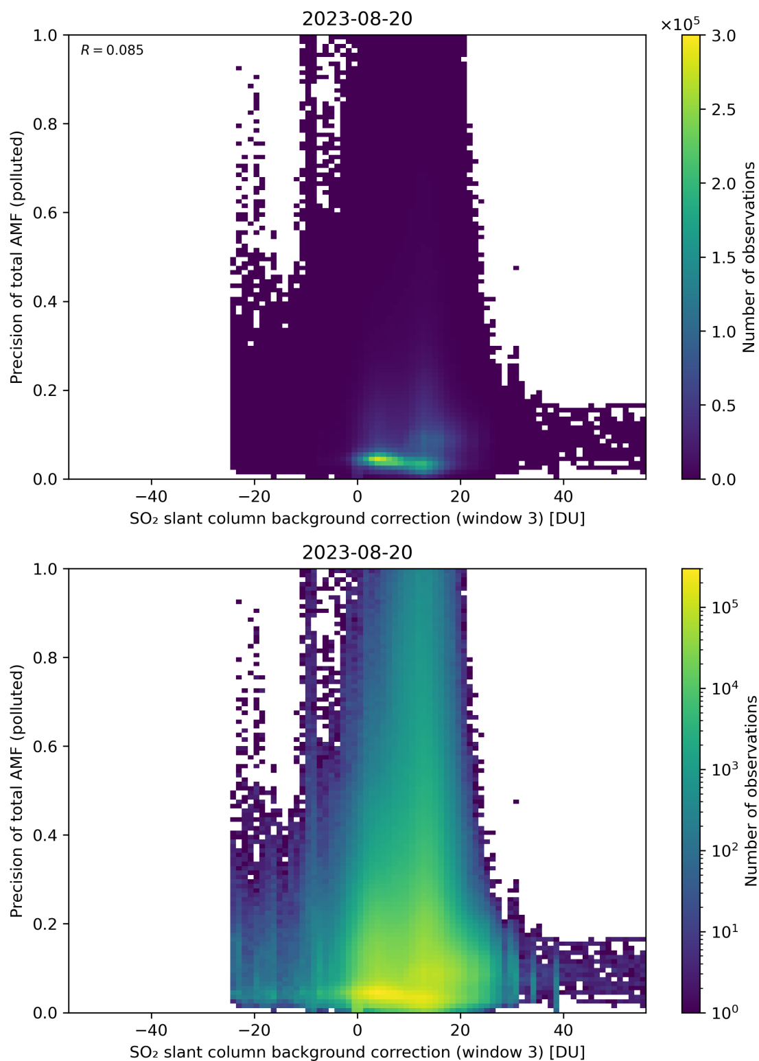
Figure 126: Scatter density plot of “SO 2 slant column background correction (window 3)” against “Precision of total AMF (polluted)” for 2023-08-20 to 2023-08-21.
