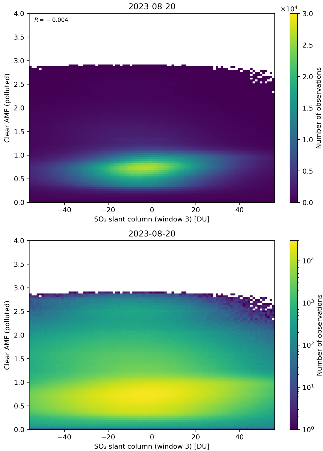
Figure 265: Scatter density plot of “SO 2 slant column (window 3)” against “Clear AMF (polluted)” for 2023-08-20 to 2023-08-21.
