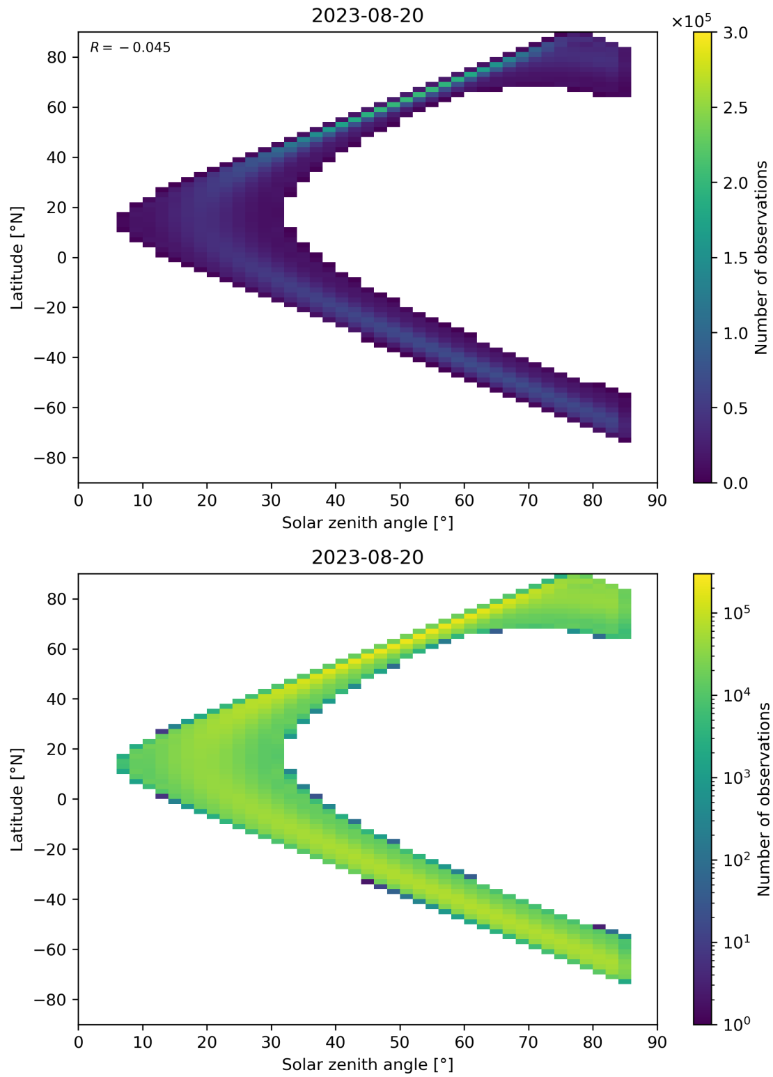
Figure 164: Scatter density plot of “Solar zenith angle” against “Latitude” for 2023-08-20 to 2023-08-21.
