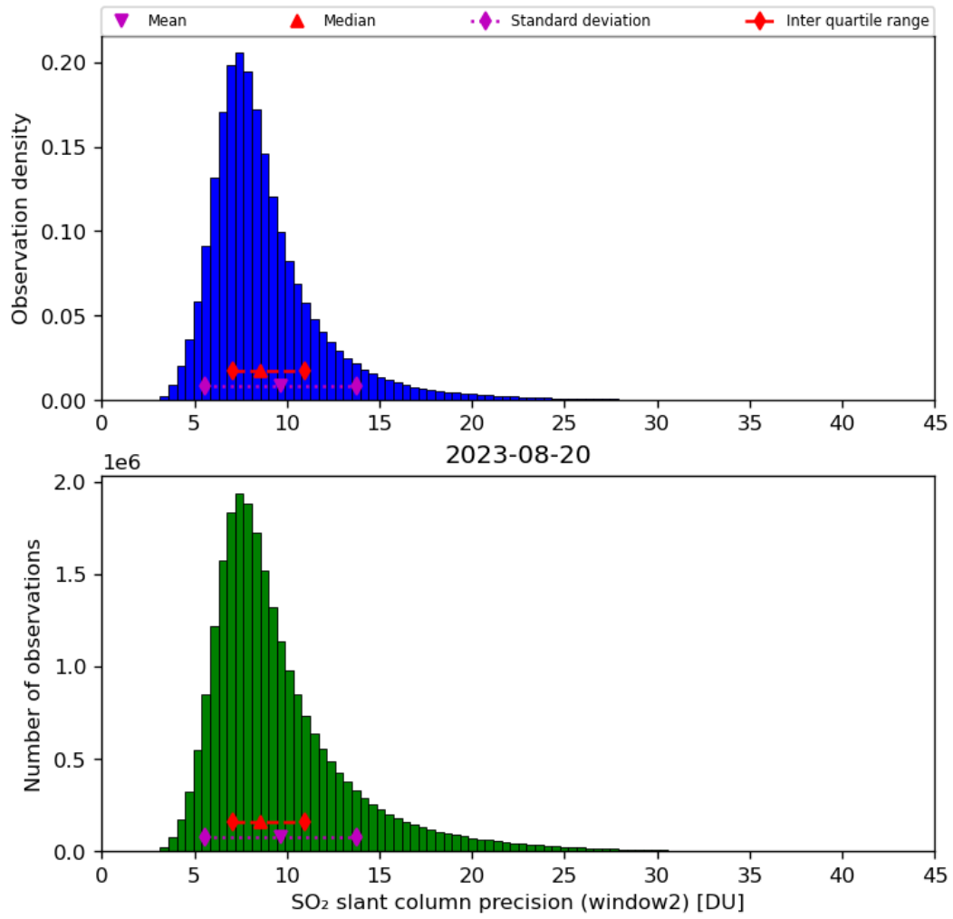
Figure 61: Histogram of “SO 2 slant column precision (window2)” for 2023-08-20 to 2023-08-21
