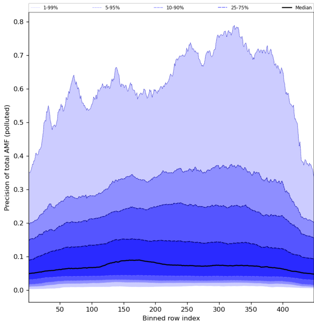
Figure 95: Along track statistics of “Precision of total AMF (polluted)” for 2023-08-20 to 2023-08-21
