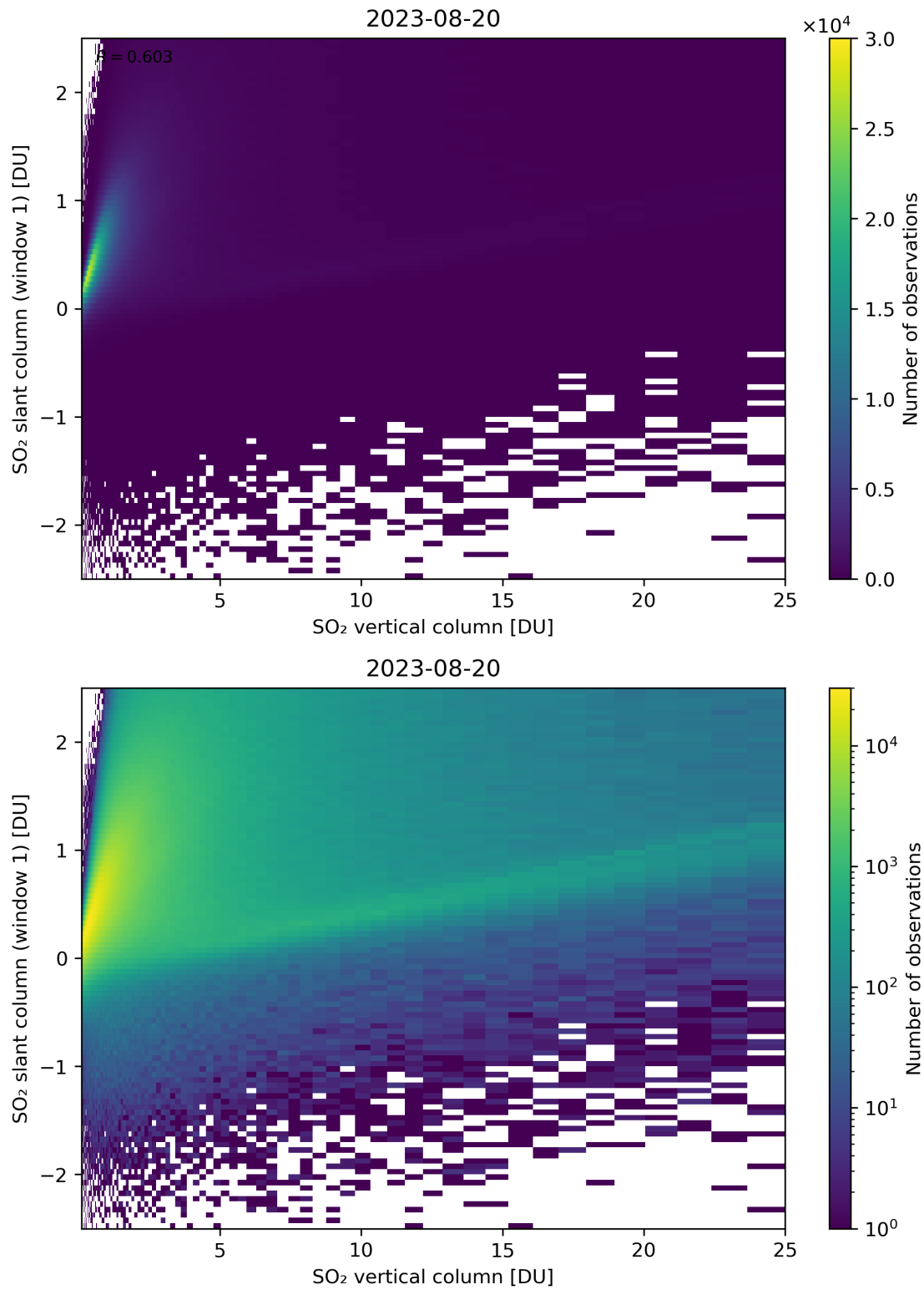
Figure 300: Scatter density plot of “SO 2 vertical column” against “SO 2 slant column (window 1)” for 2023-08-20 to 2023-08-21.
