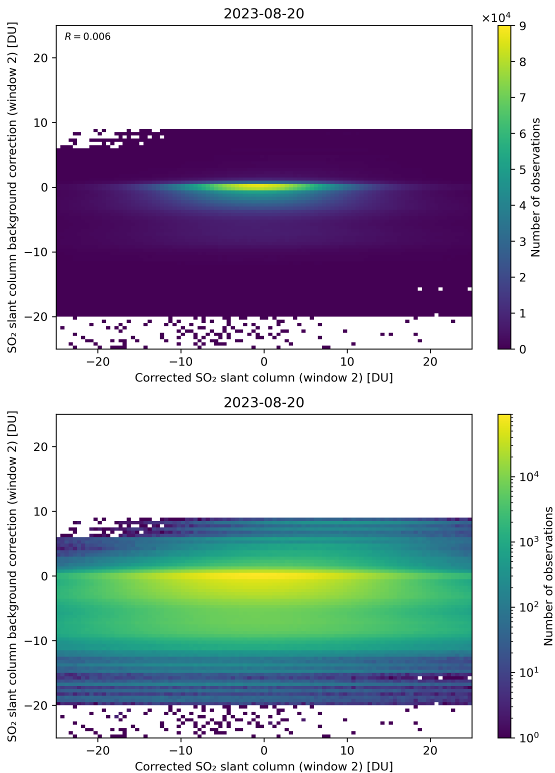
Figure 194: Scatter density plot of “Corrected SO 2 slant column (window 2)” against “SO 2 slant column background correction (window 2)” for 2023-08-20 to 2023-08-21.
