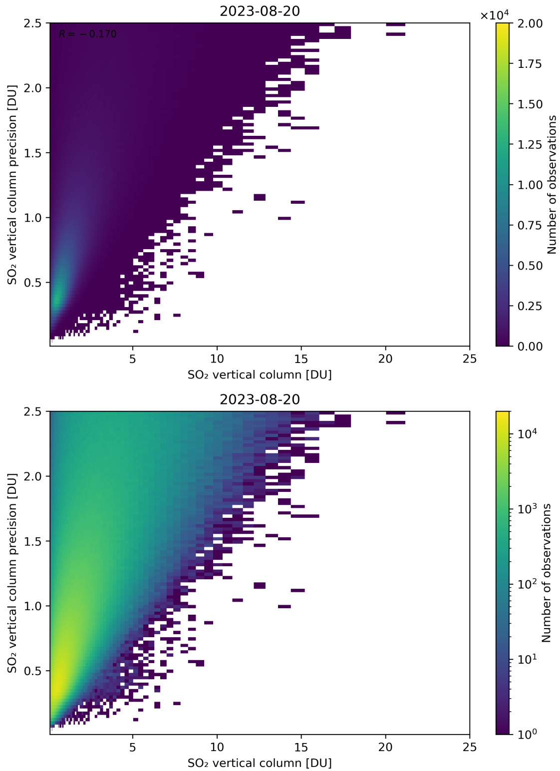
Figure 307: Scatter density plot of “SO 2 vertical column” against “SO 2 vertical column precision” for 2023-08-20 to 2023-08-21.
