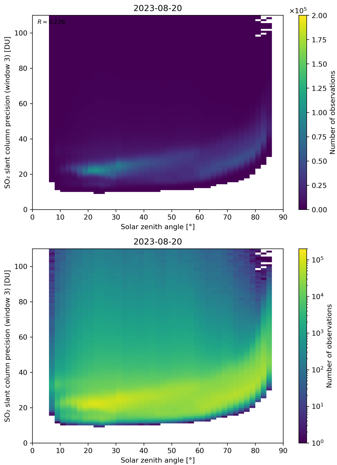
Figure 173: Scatter density plot of “Solar zenith angle” against “SO 2 slant column precision (window 3)” for 2023-08-20 to 2023-08-21.
