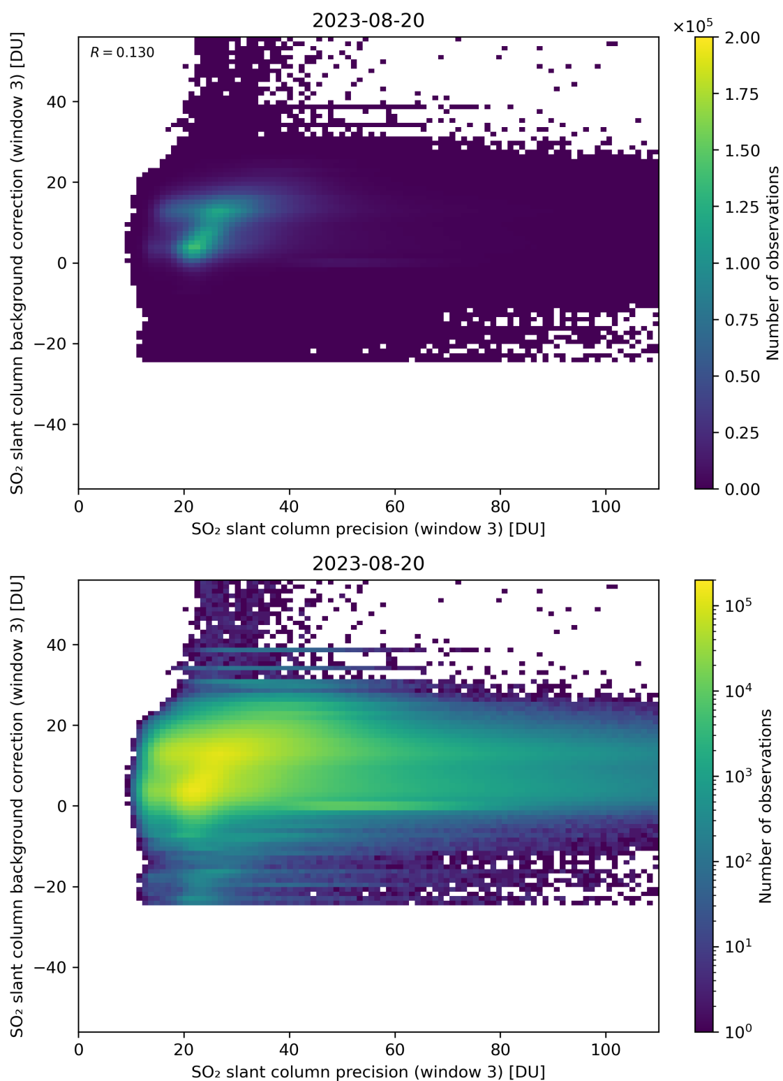
Figure 257: Scatter density plot of “SO 2 slant column precision (window 3)” against “SO 2 slant column background correction (window 3)” for 2023-08-20 to 2023-08-21.
