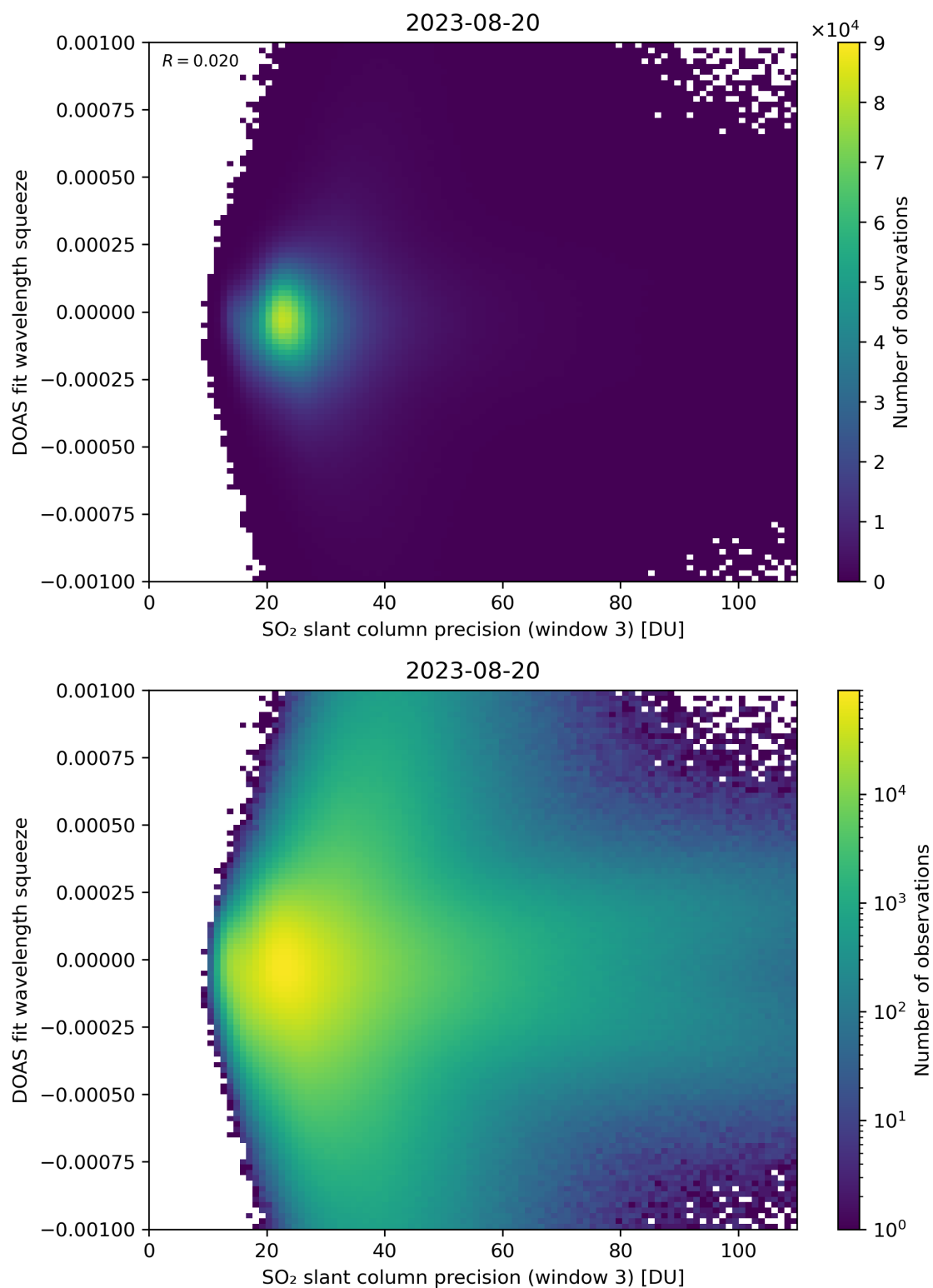
Figure 259: Scatter density plot of “SO 2 slant column precision (window 3)” against “DOAS fit wavelength squeeze” for 2023-08-20 to 2023-08-21.
