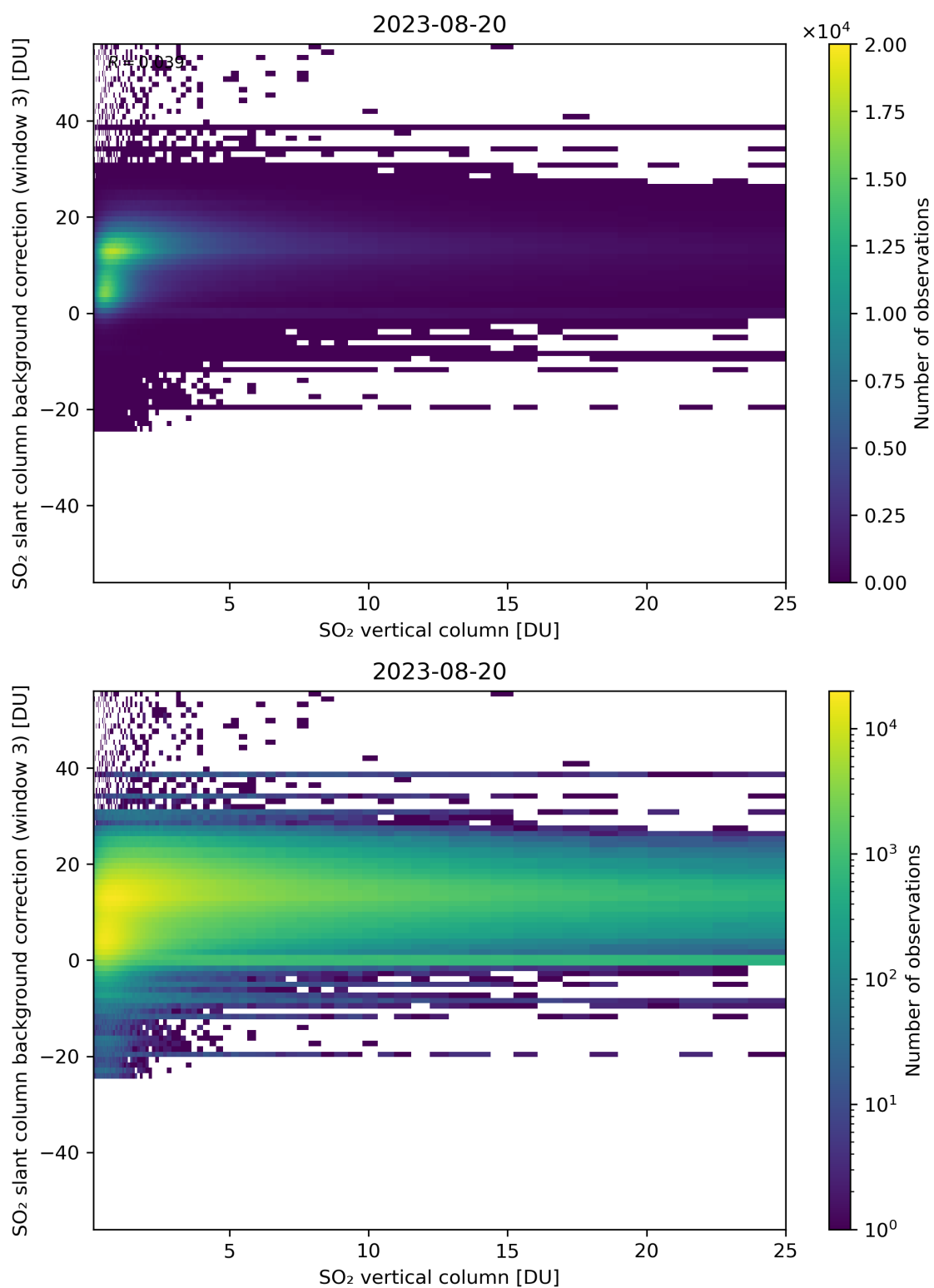
Figure 275: Scatter density plot of “SO 2 vertical column” against “SO 2 slant column background correction (window 3)” for 2023-08-20 to 2023-08-21.
