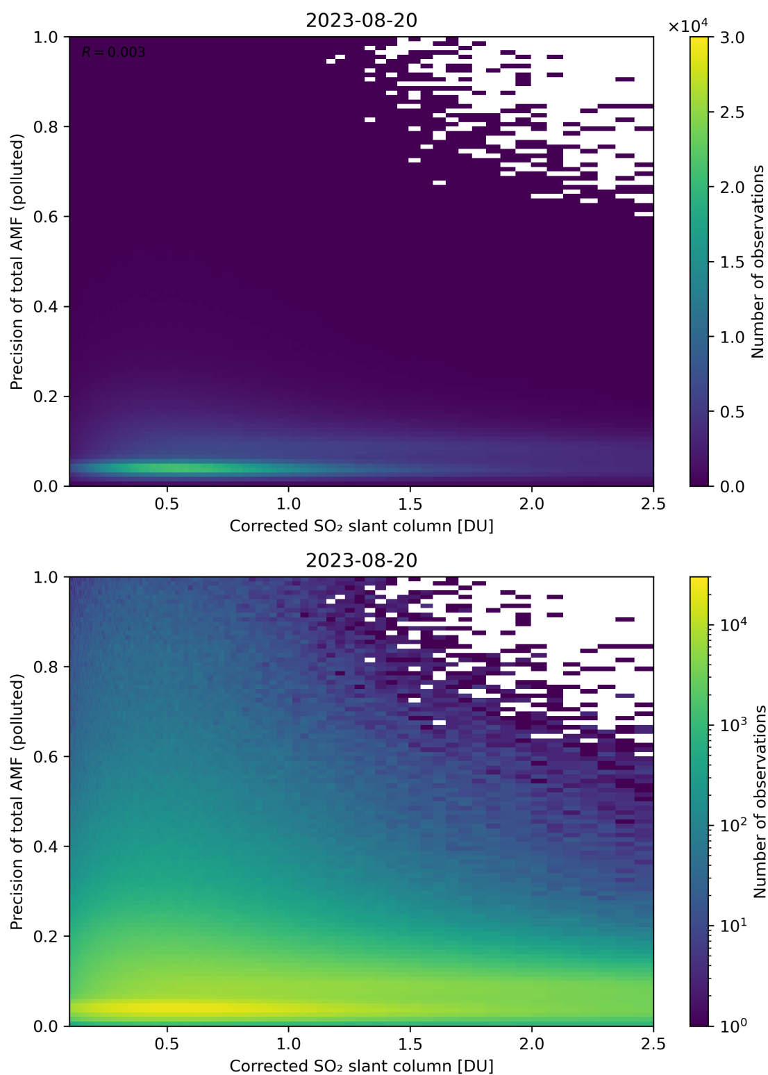
Figure 193: Scatter density plot of “Corrected SO 2 slant column” against “Precision of total AMF (polluted)” for 2023-08-20 to 2023-08-21.
