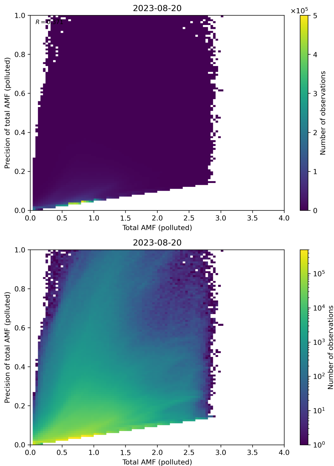
Figure 272: Scatter density plot of “Total AMF (polluted)” against “Precision of total AMF (polluted)” for 2023-08-20 to 2023-08-21.
