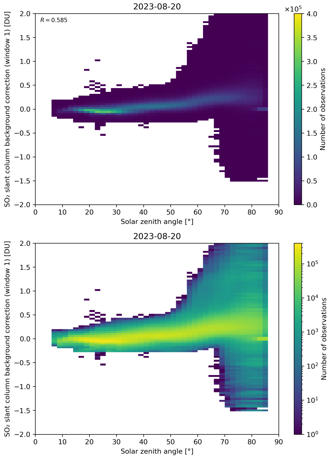
Figure 158: Scatter density plot of “Solar zenith angle” against “SO 2 slant column background correction (window 1)” for 2023-08-20 to 2023-08-21.
