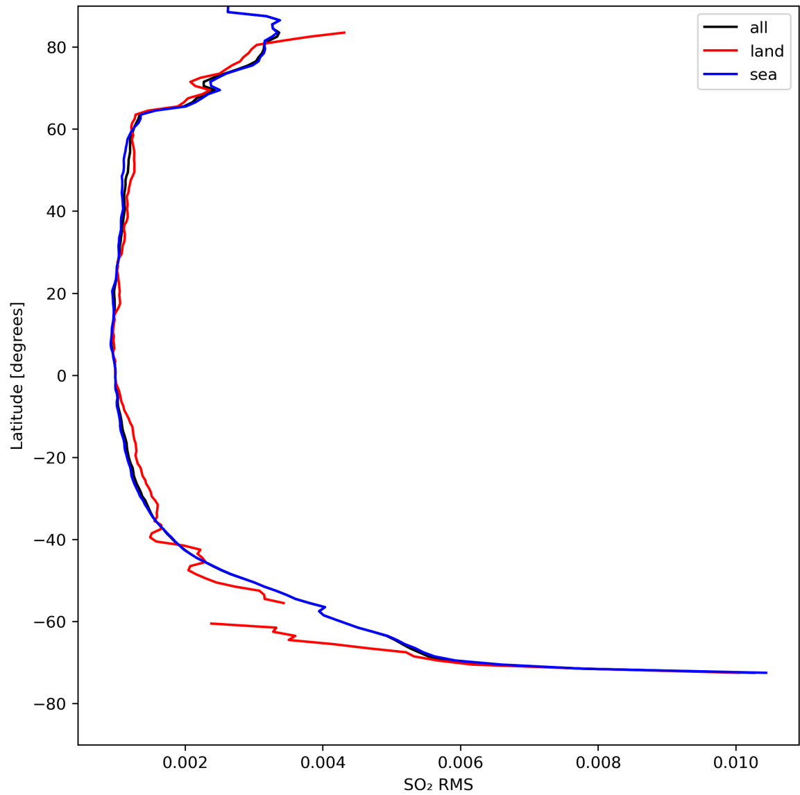
Figure 47: Zonal average of “SO 2 RMS” for 2023-08-20 to 2023-08-21.
