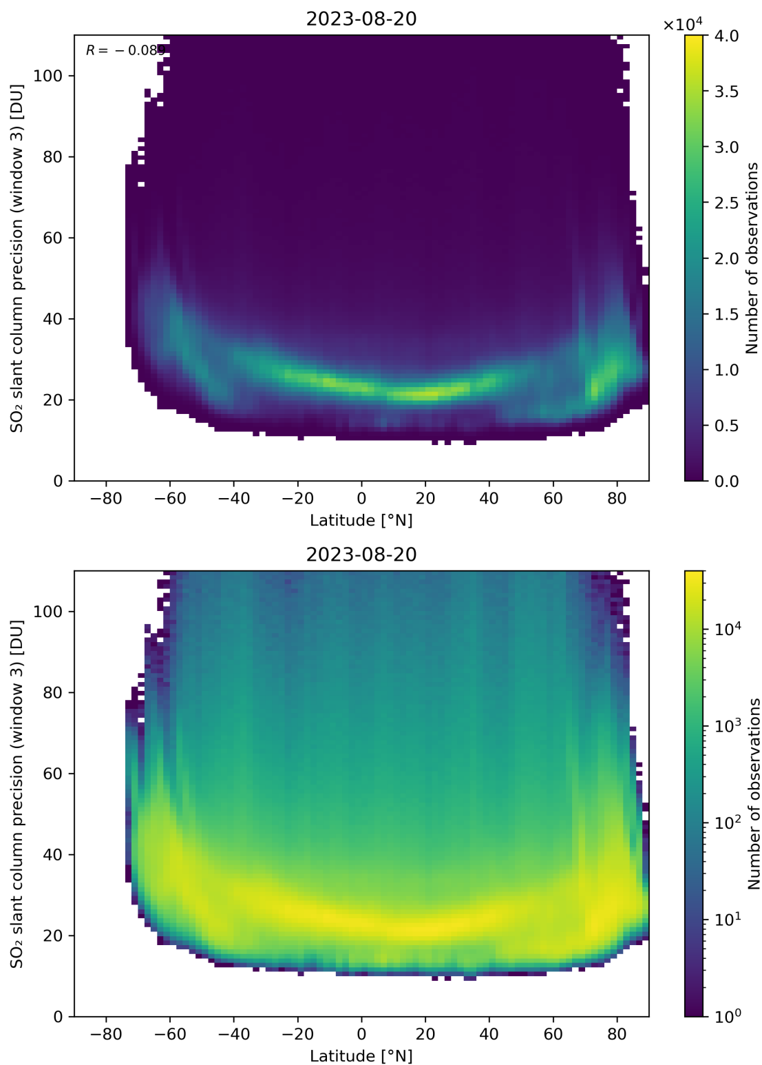
Figure 153: Scatter density plot of “Latitude” against “SO 2 slant column precision (window 3)” for 2023-08-20 to 2023-08-21.
