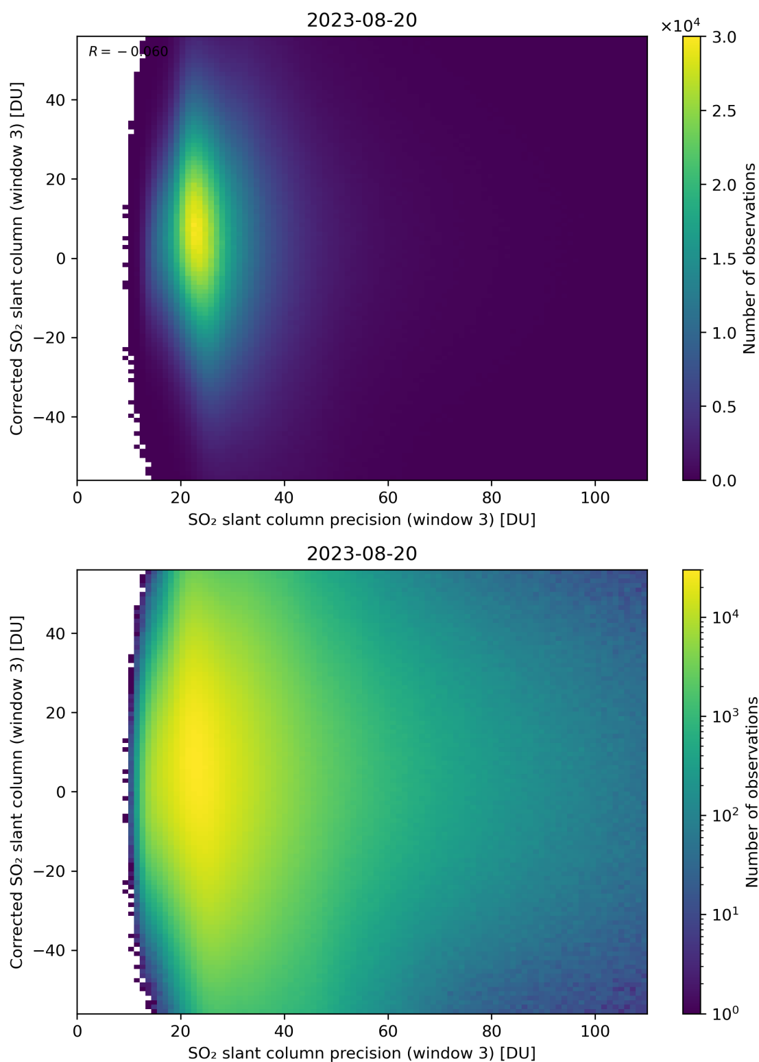
Figure 262: Scatter density plot of “SO 2 slant column precision (window 3)” against “Corrected SO 2 slant column (window 3)” for 2023-08-20 to 2023-08-21.
