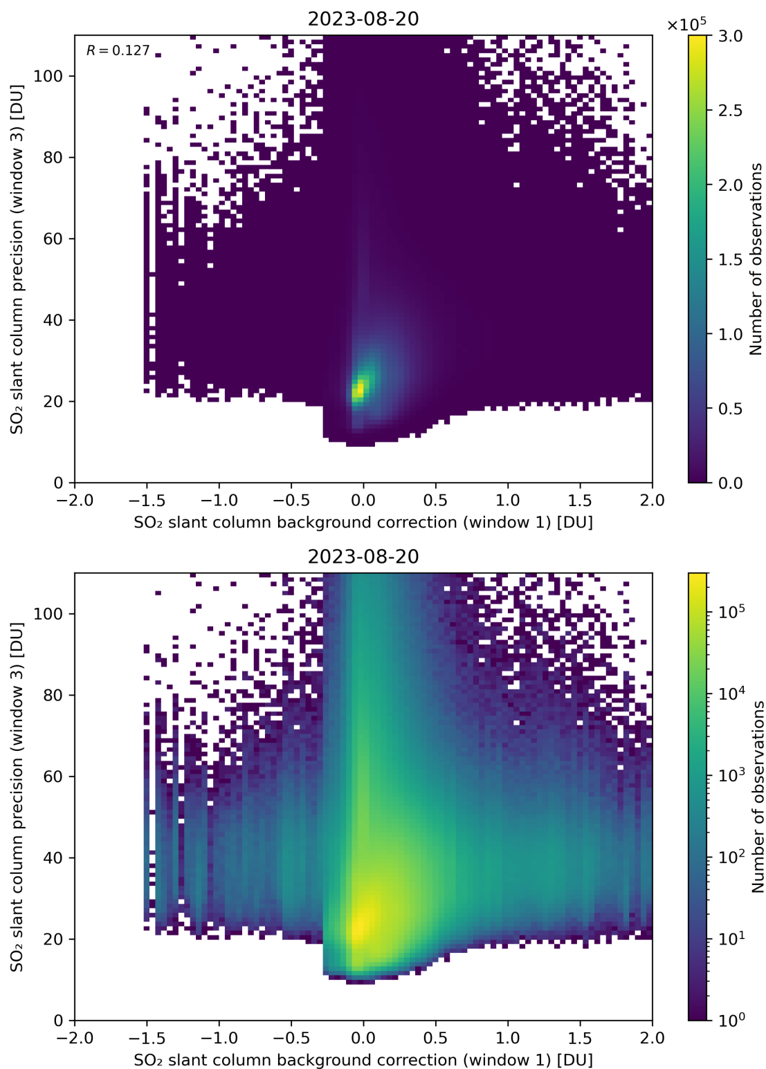
Figure 108: Scatter density plot of “SO 2 slant column background correction (window 1)” against “SO 2 slant column precision (window 3)” for 2023-08-20 to 2023-08-21.
