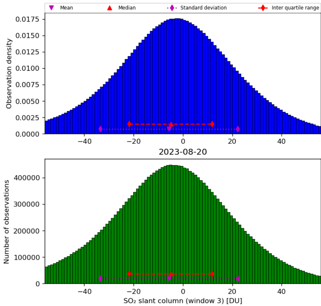
Figure 64: Histogram of “SO 2 slant column (window 3)” for 2023-08-20 to 2023-08-21
