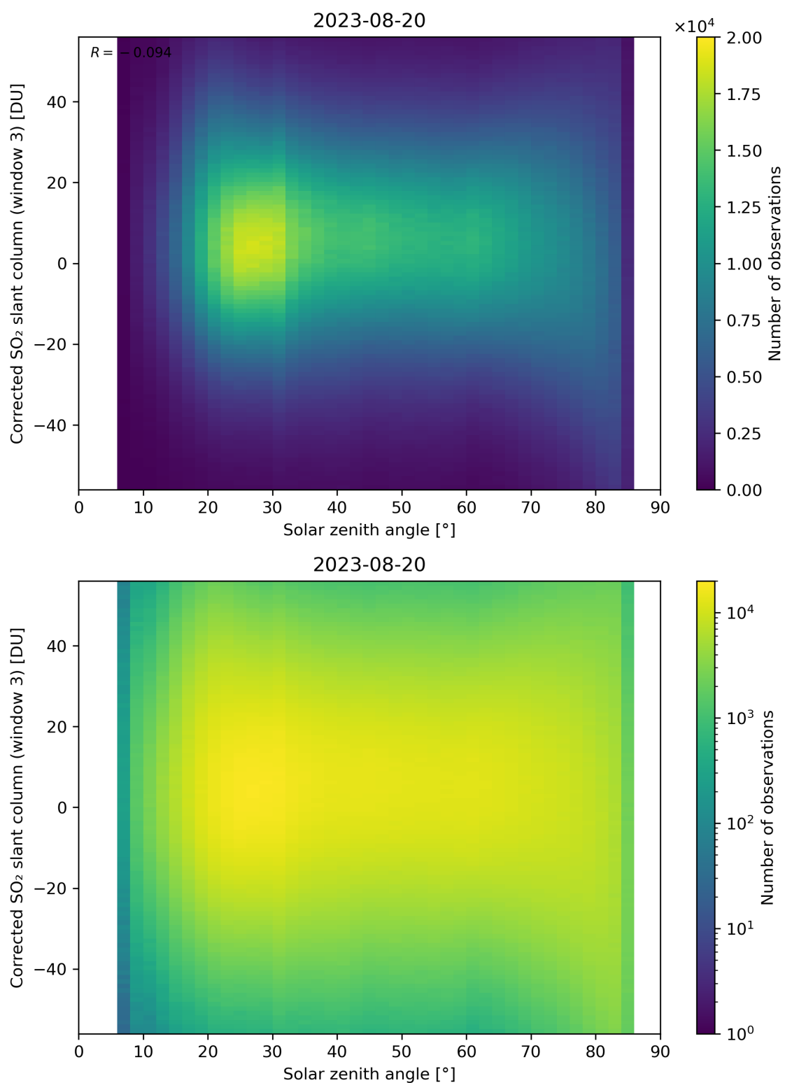
Figure 168: Scatter density plot of “Solar zenith angle” against “Corrected SO 2 slant column (window 3)” for 2023-08-20 to 2023-08-21.
