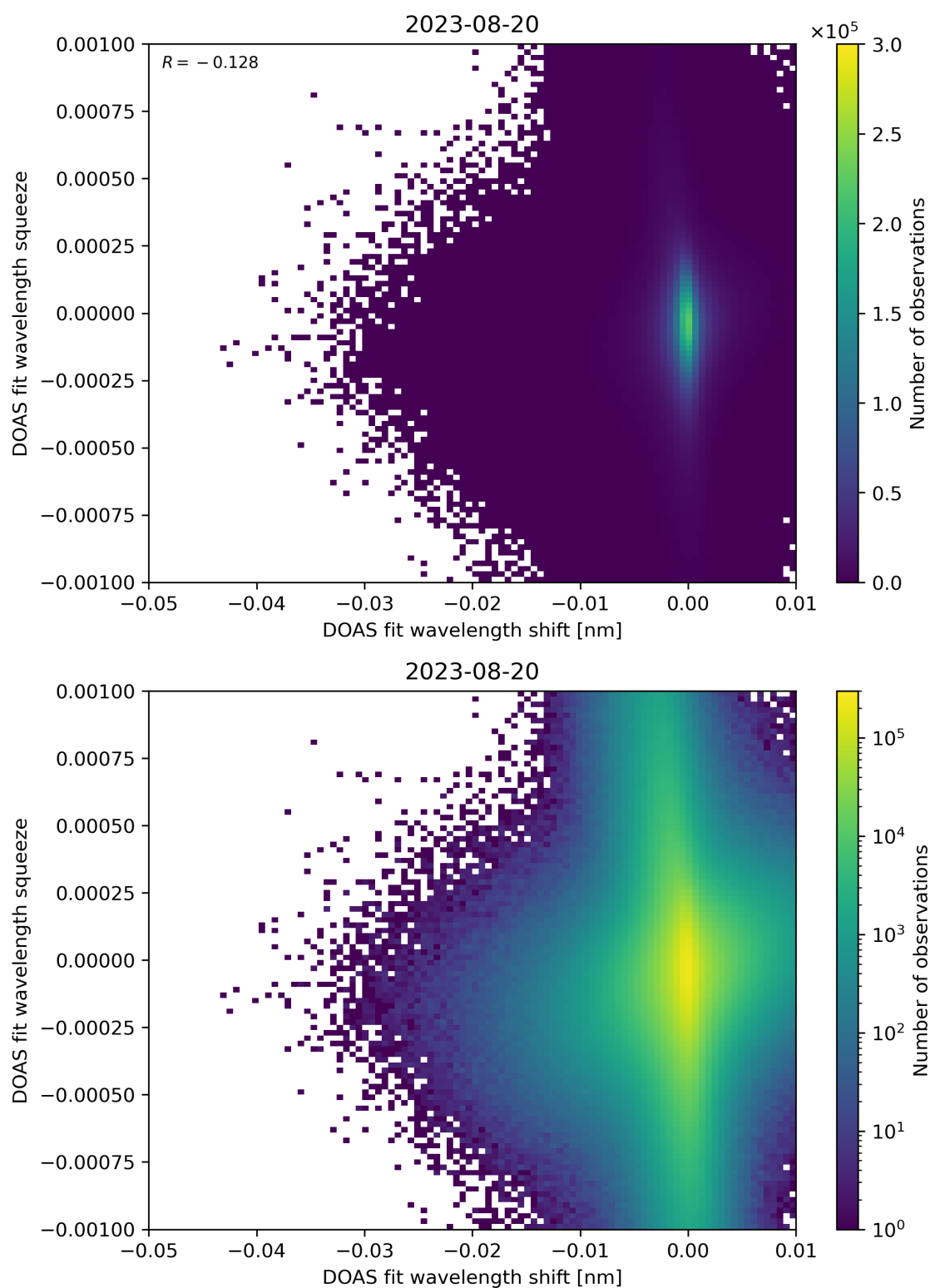
Figure 127: Scatter density plot of “DOAS fit wavelength shift” against “DOAS fit wavelength squeeze” for 2023-08-20 to 2023-08-21.
