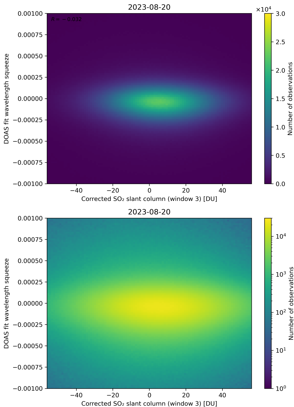
Figure 207: Scatter density plot of “Corrected SO 2 slant column (window 3)” against “DOAS fit wavelength squeeze” for 2023-08-20 to 2023-08-21.
