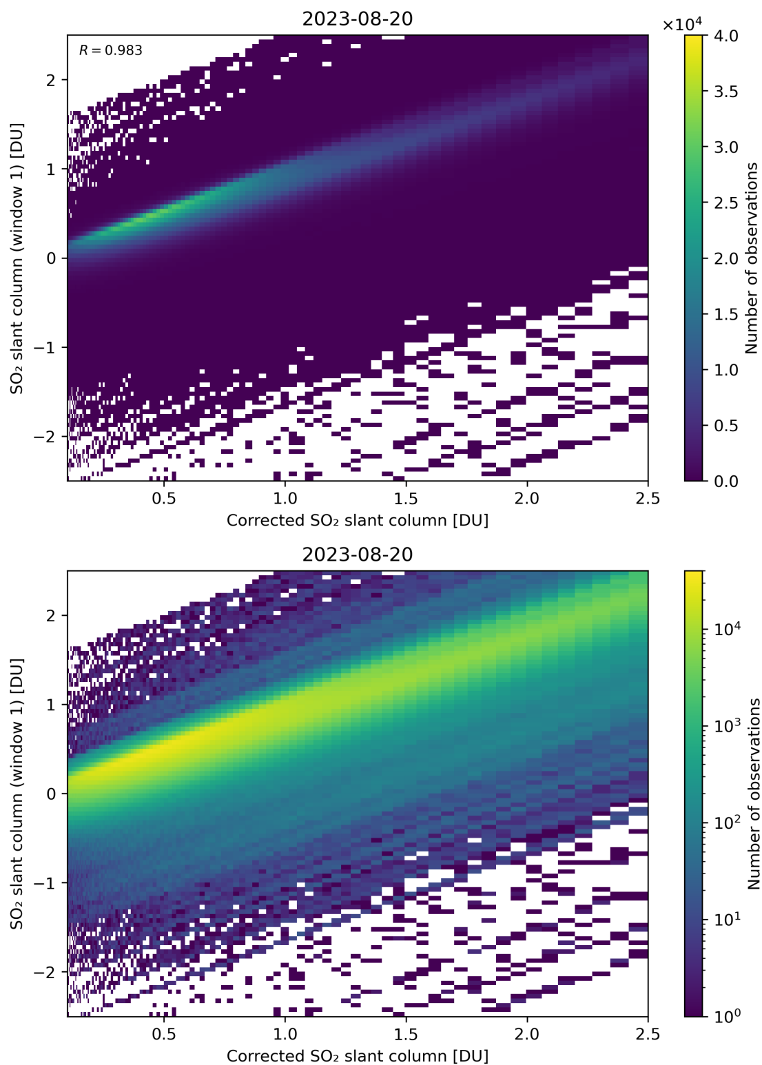
Figure 187: Scatter density plot of “Corrected SO 2 slant column” against “SO 2 slant column (window 1)” for 2023-08-20 to 2023-08-21.
