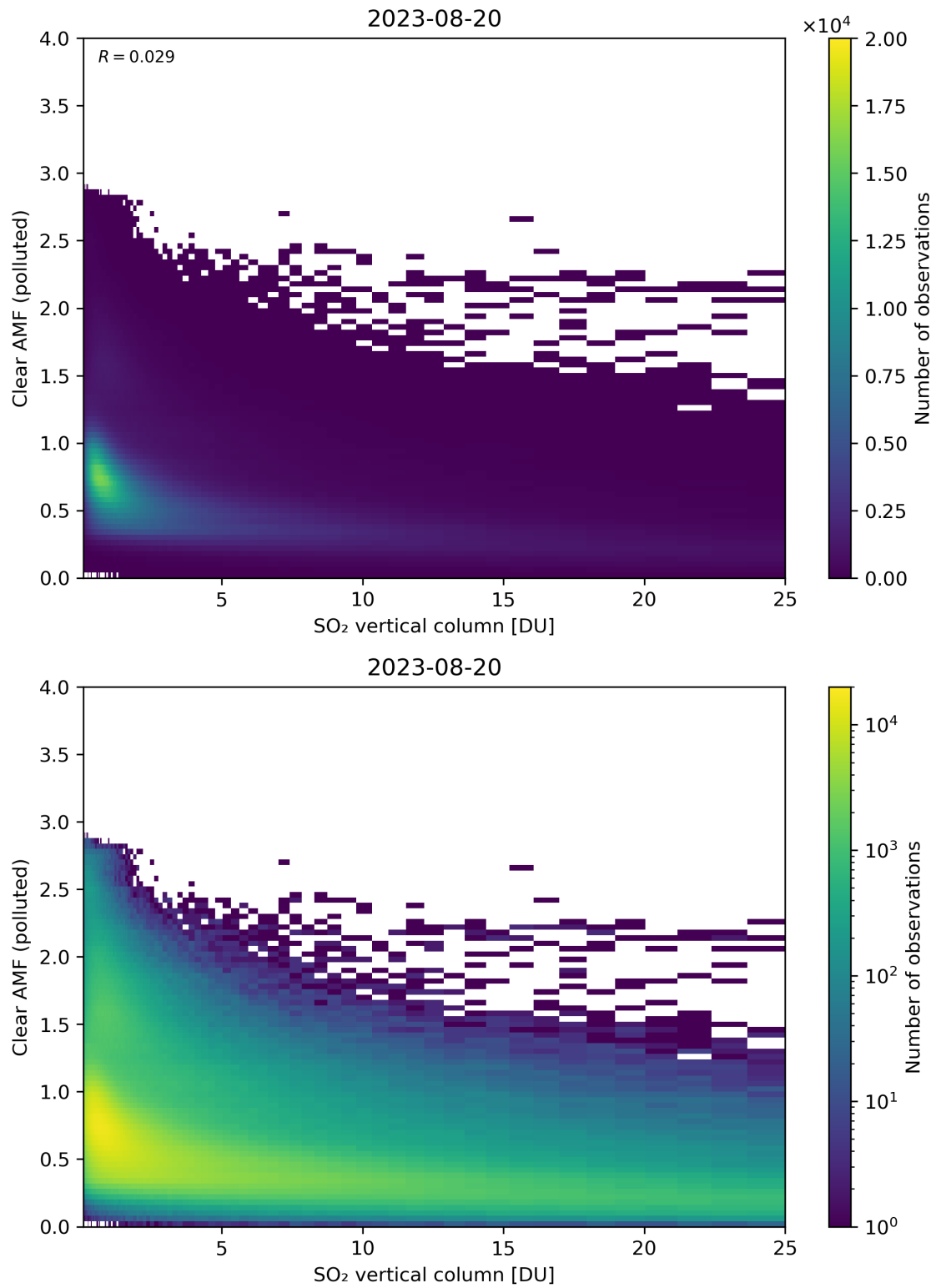
Figure 296: Scatter density plot of “SO 2 vertical column” against “Clear AMF (polluted)” for 2023-08-20 to 2023-08-21.
