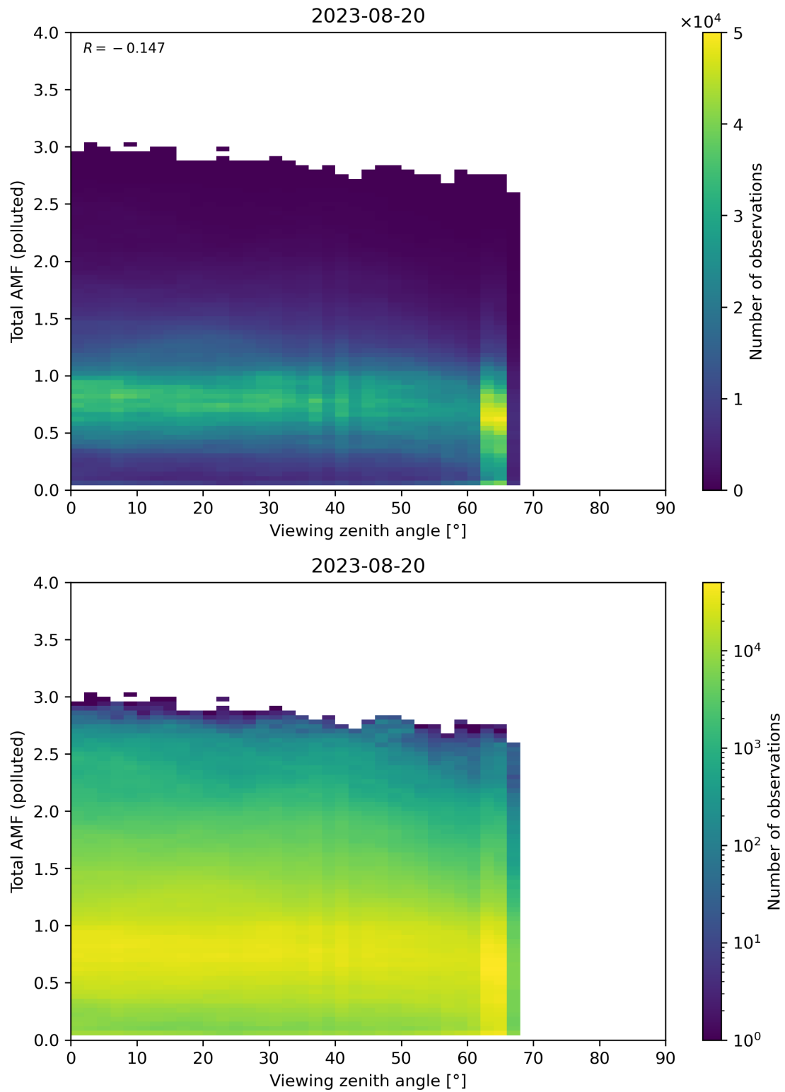
Figure 325: Scatter density plot of “Viewing zenith angle” against “Total AMF (polluted)” for 2023-08-20 to 2023-08-21.
