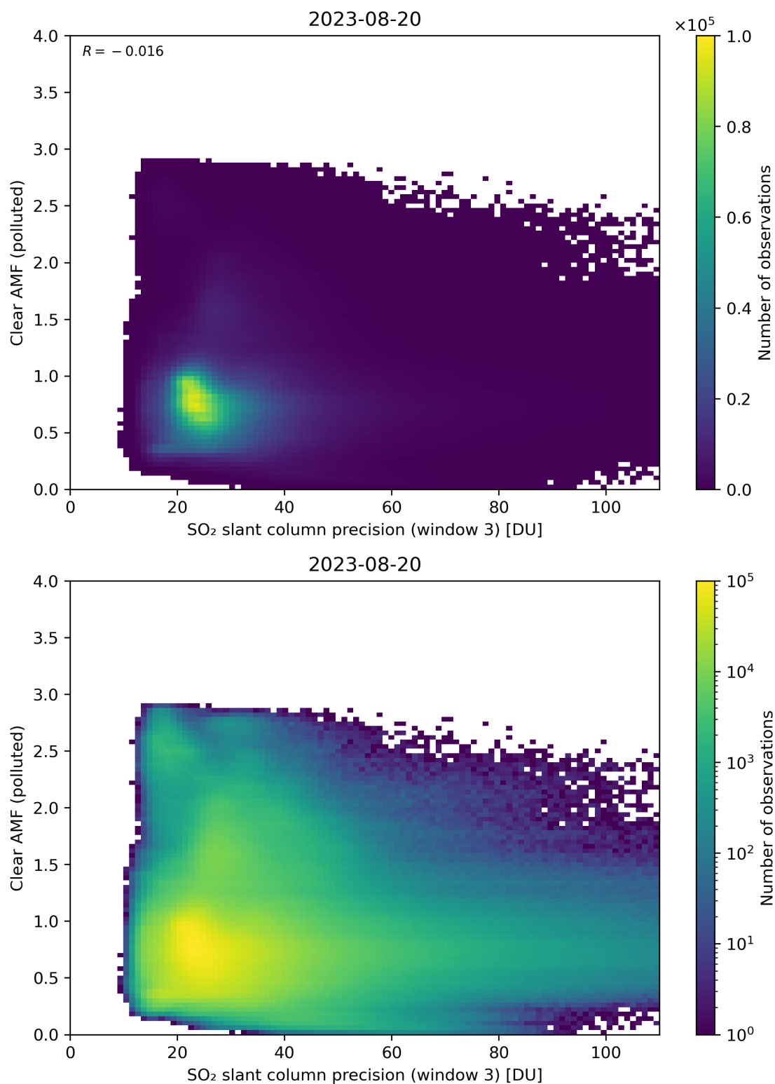
Figure 261: Scatter density plot of “SO 2 slant column precision (window 3)” against “Clear AMF (polluted)” for 2023-08-20 to 2023-08-21.
