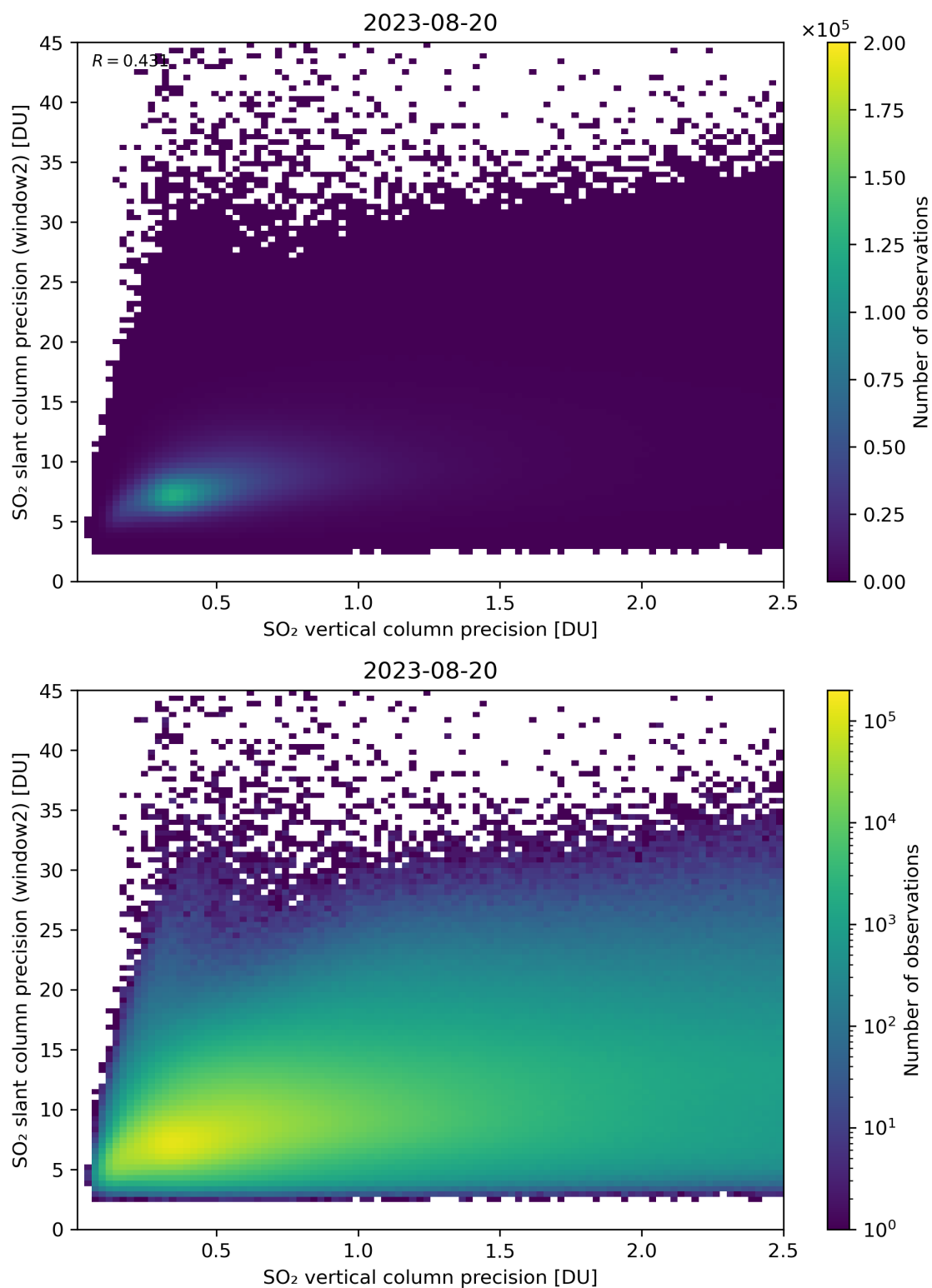
Figure 291: Scatter density plot of “SO 2 vertical column precision” against “SO 2 slant column precision (window2)” for 2023-08-20 to 2023-08-21.
