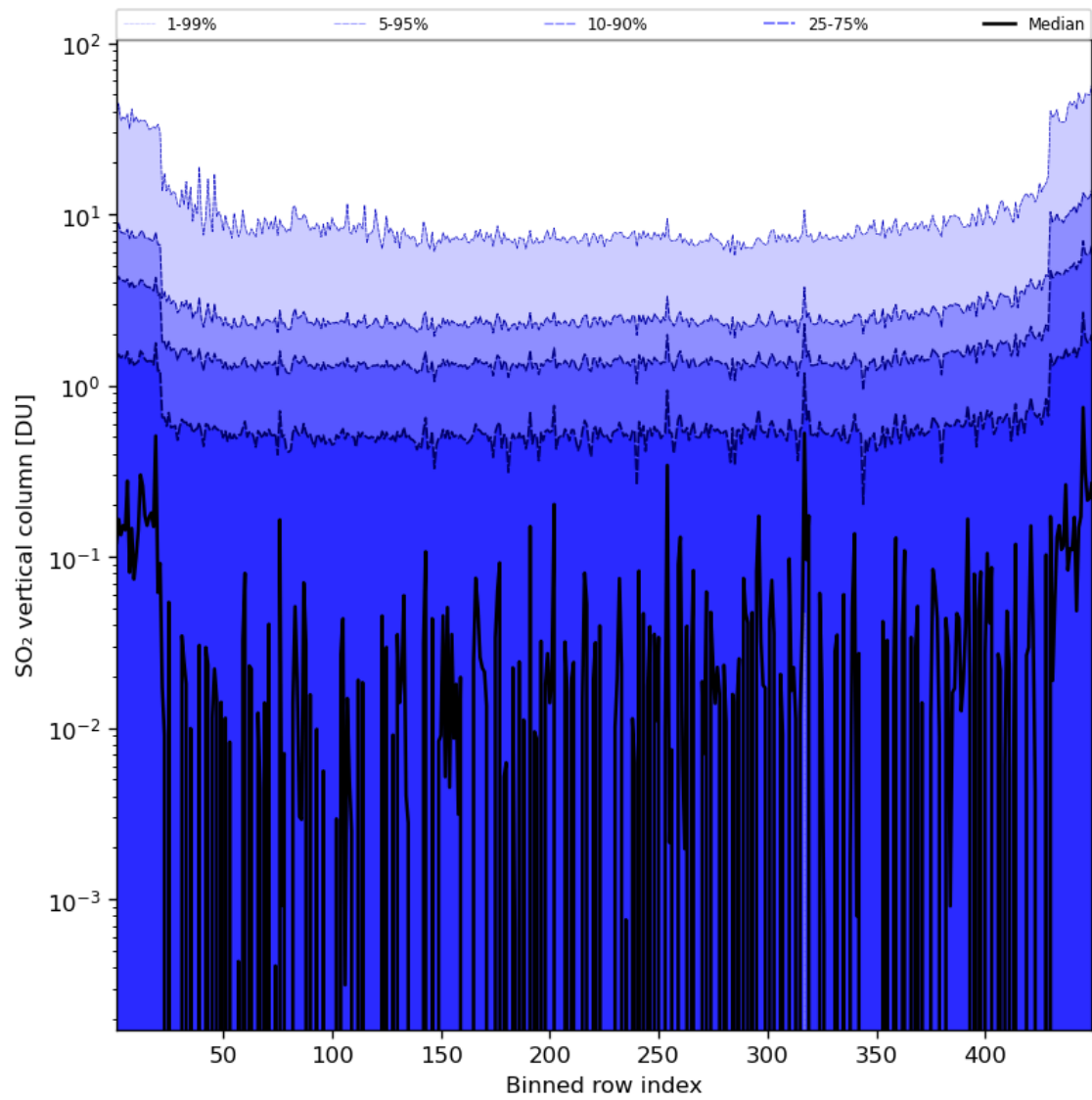
Figure 76: Along track statistics of “SO 2 vertical column” for 2023-08-20 to 2023-08-21
