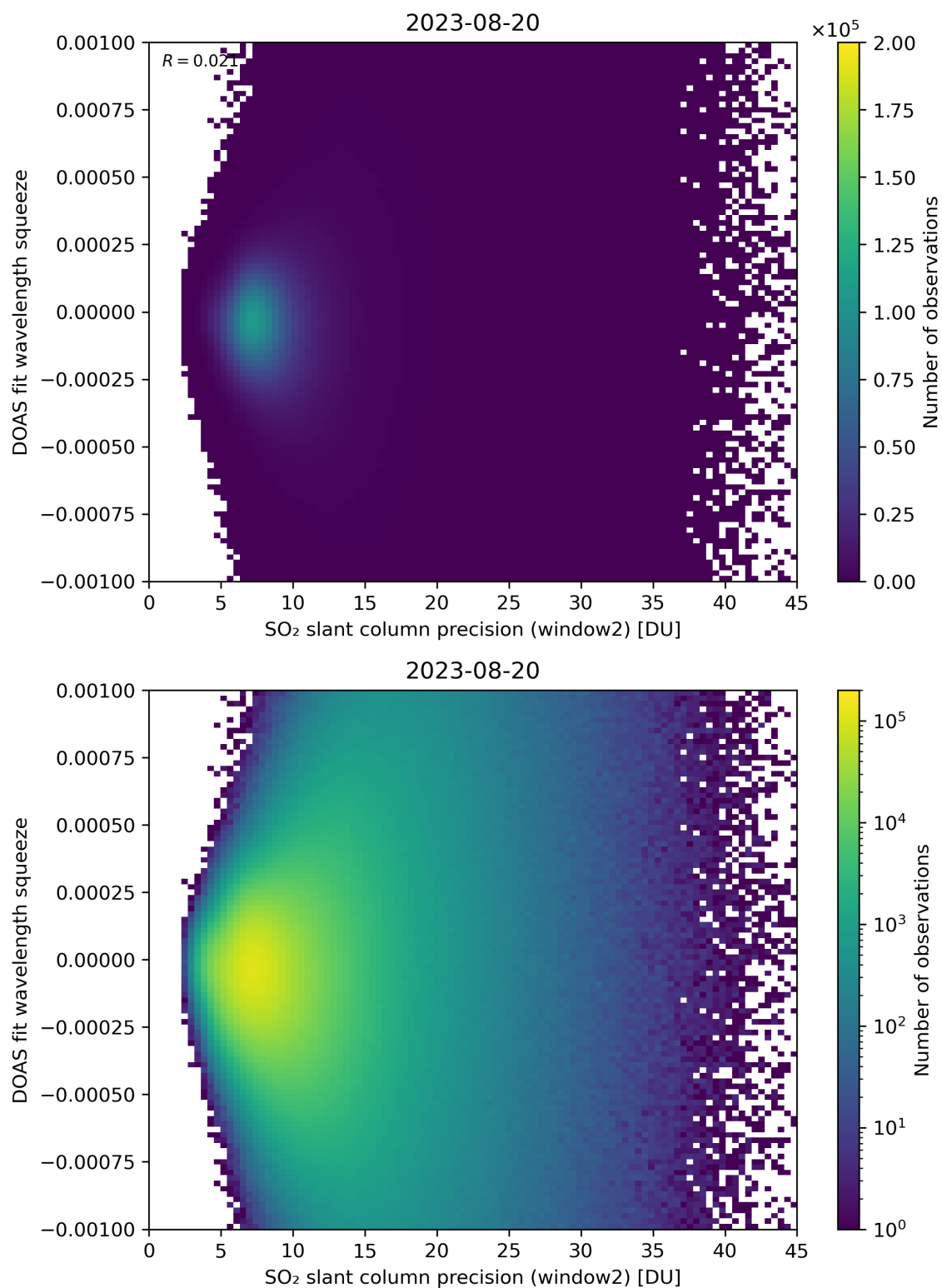
Figure 244: Scatter density plot of “SO 2 slant column precision (window2)” against “DOAS fit wavelength squeeze” for 2023-08-20 to 2023-08-21.
