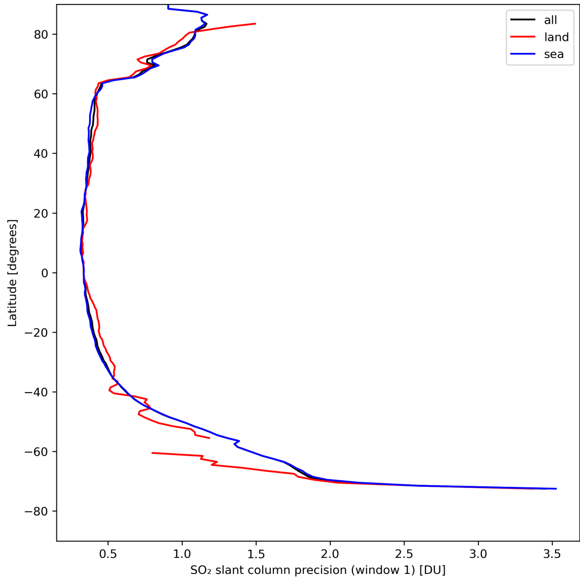
Figure 34: Zonal average of “SO 2 slant column precision (window 1)” for 2023-08-20 to 2023-08-21.
