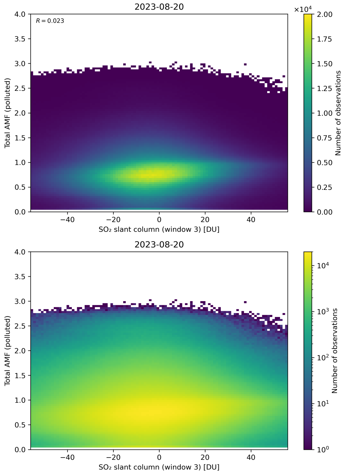
Figure 268: Scatter density plot of “SO 2 slant column (window 3)” against “Total AMF (polluted)” for 2023-08-20 to 2023-08-21.
