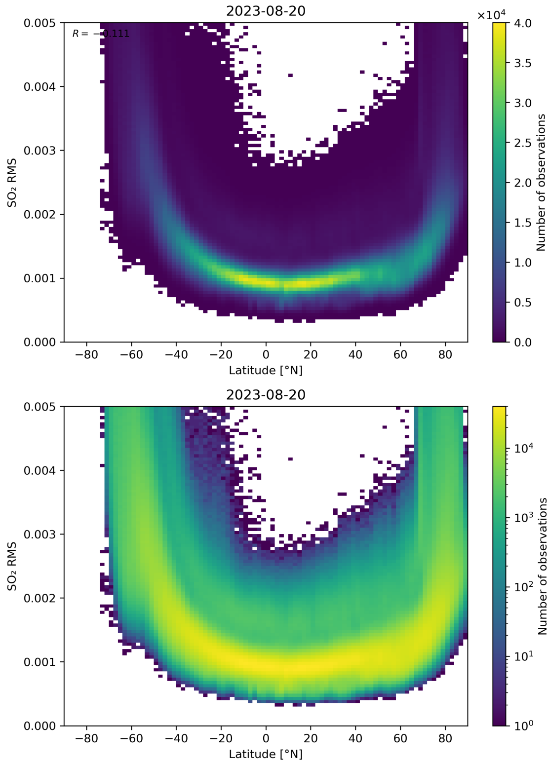
Figure 144: Scatter density plot of “Latitude” against “SO 2 RMS” for 2023-08-20 to 2023-08-21.
