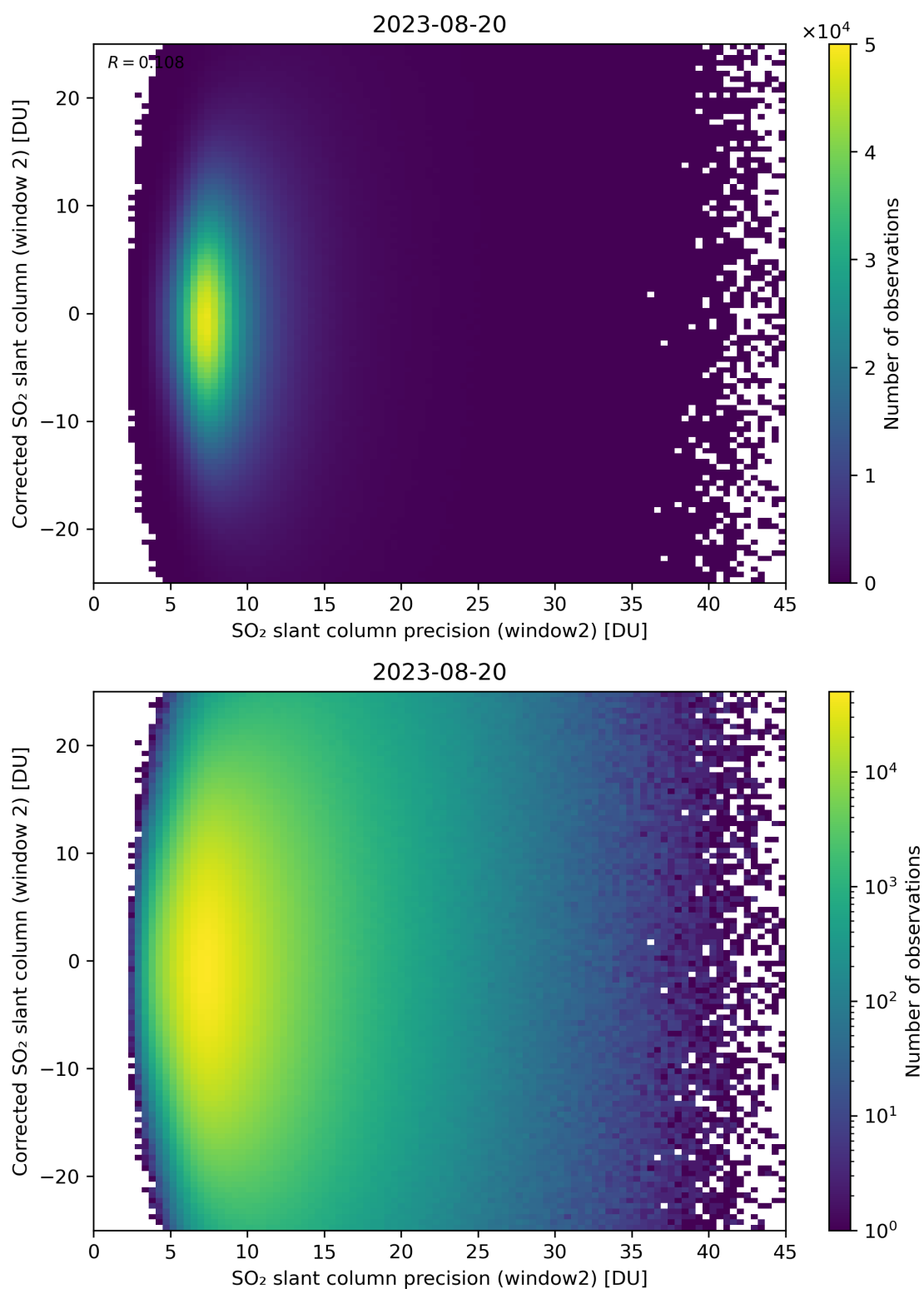
Figure 247: Scatter density plot of “SO 2 slant column precision (window2)” against “Corrected SO 2 slant column (window 2)” for 2023-08-20 to 2023-08-21.
