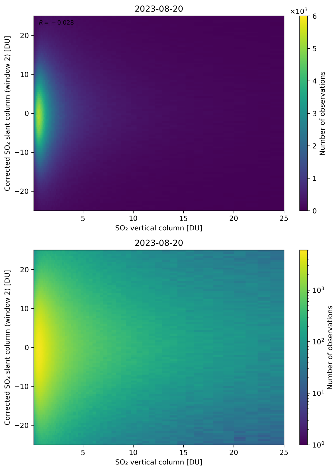
Figure 298: Scatter density plot of “SO 2 vertical column” against “Corrected SO 2 slant column (window 2)” for 2023-08-20 to 2023-08-21.
