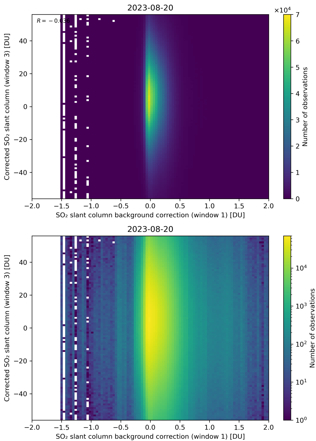
Figure 105: Scatter density plot of “SO 2 slant column background correction (window 1)” against “Corrected SO 2 slant column (window 3)” for 2023-08-20 to 2023-08-21.
