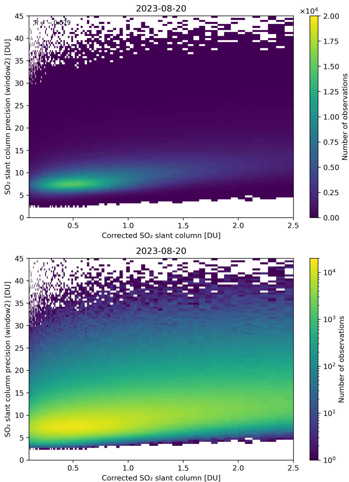
Figure 189: Scatter density plot of “Corrected SO 2 slant column” against “SO 2 slant column precision (window2)” for 2023-08-20 to 2023-08-21.
