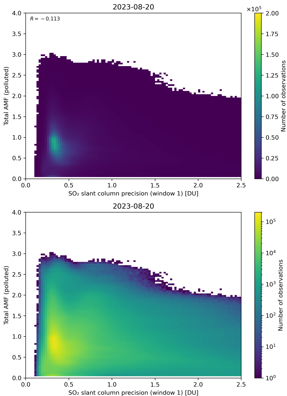
Figure 230: Scatter density plot of “SO 2 slant column precision (window 1)” against “Total AMF (polluted)” for 2023-08-20 to 2023-08-21.
