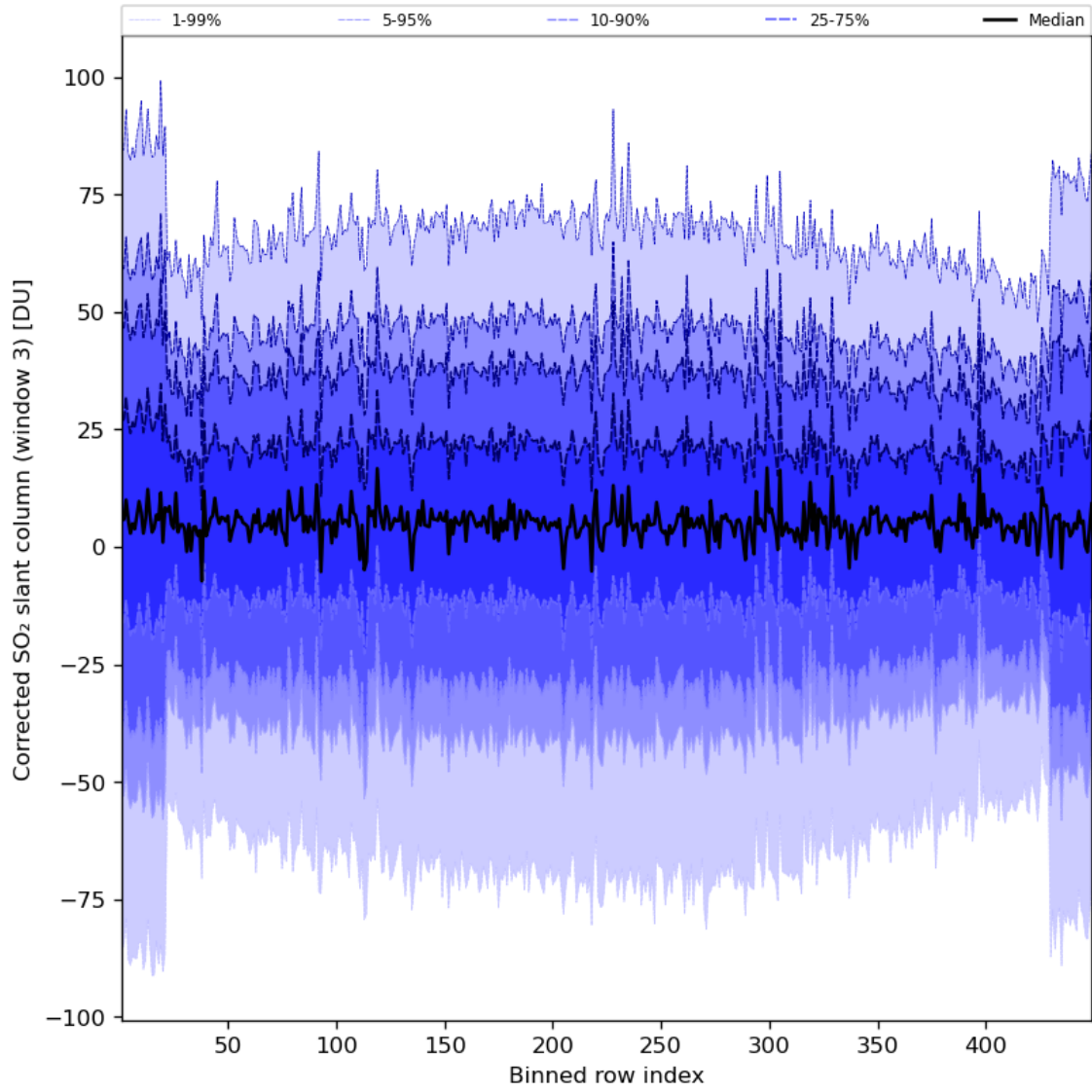
Figure 89: Along track statistics of “Corrected SO 2 slant column (window 3)” for 2023-08-20 to 2023-08-21
