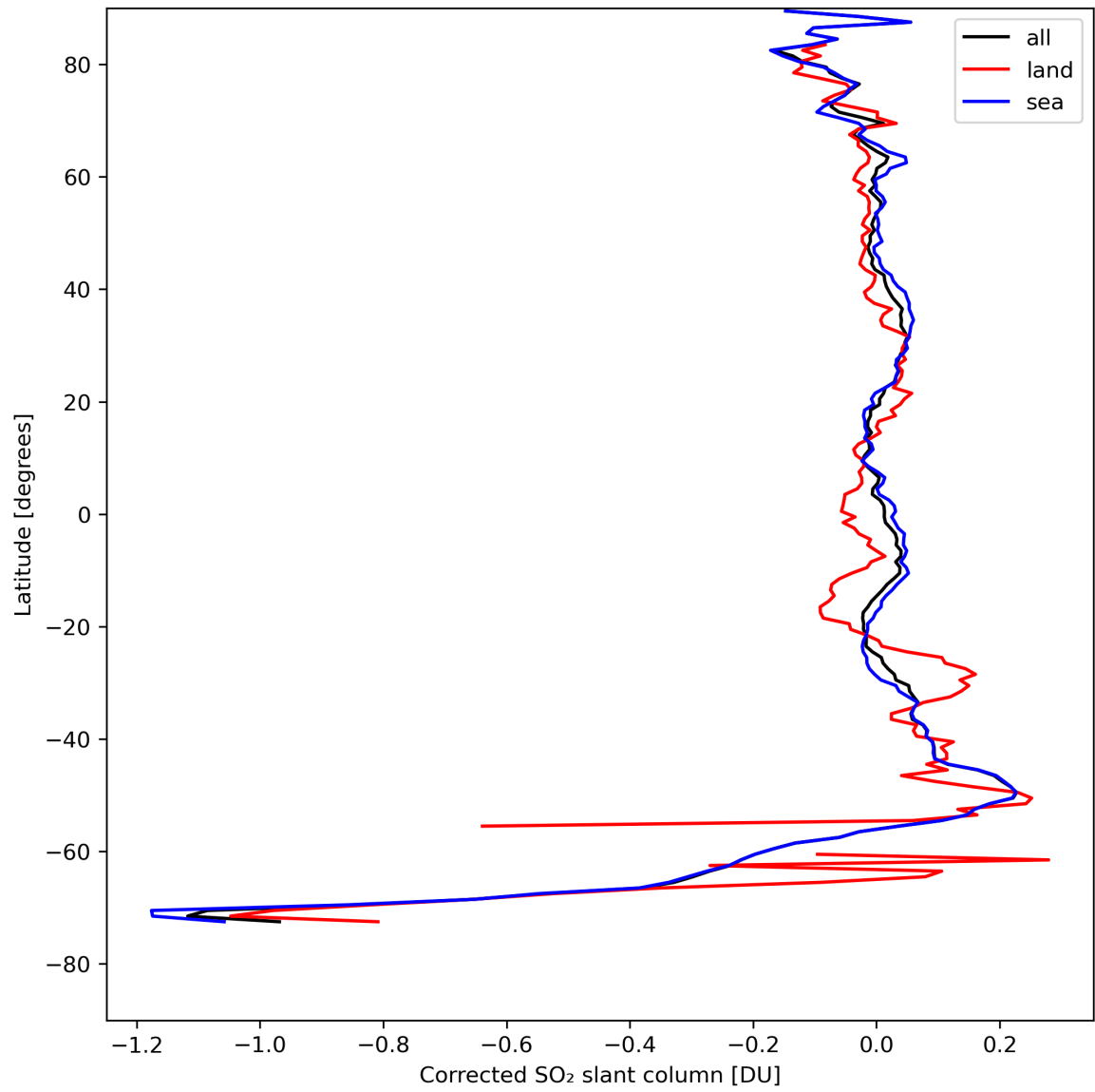
Figure 32: Zonal average of “Corrected SO 2 slant column” for 2023-08-20 to 2023-08-21.
