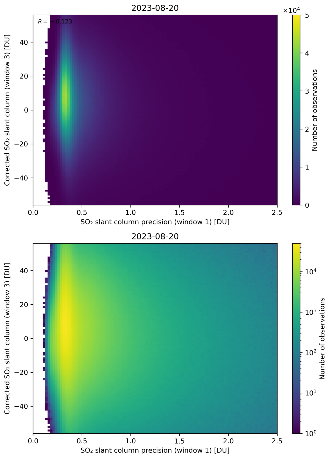
Figure 226: Scatter density plot of “SO 2 slant column precision (window 1)” against “Corrected SO 2 slant column (window 3)” for 2023-08-20 to 2023-08-21.
