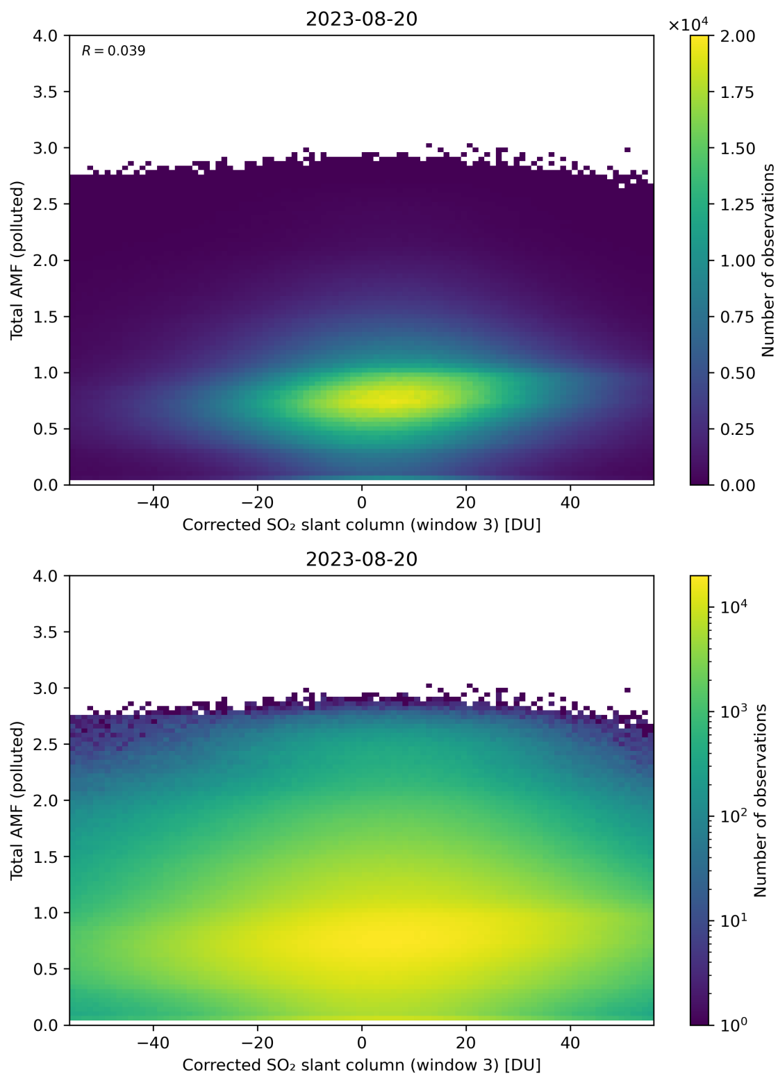
Figure 210: Scatter density plot of “Corrected SO 2 slant column (window 3)” against “Total AMF (polluted)” for 2023-08-20 to 2023-08-21.
