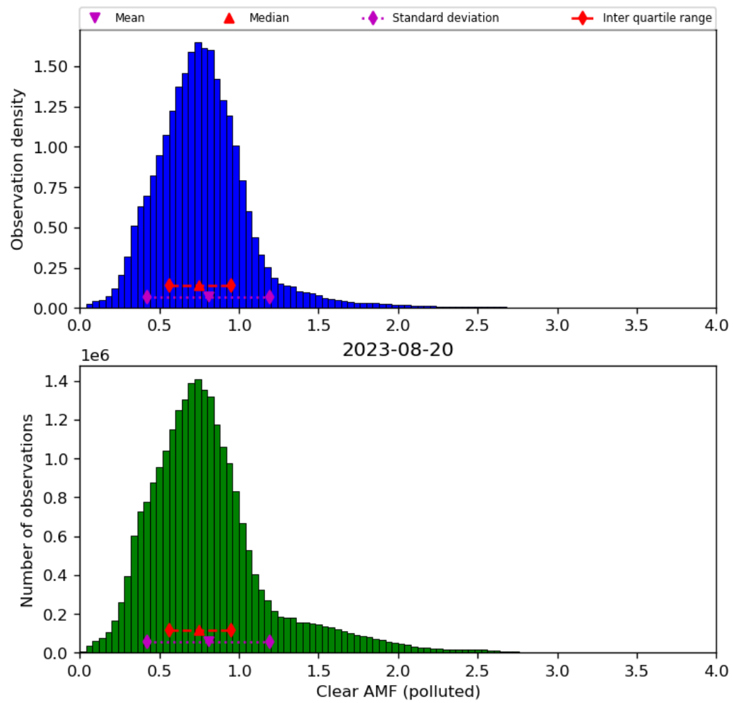
Figure 73: Histogram of “Clear AMF (polluted)” for 2023-08-20 to 2023-08-21
