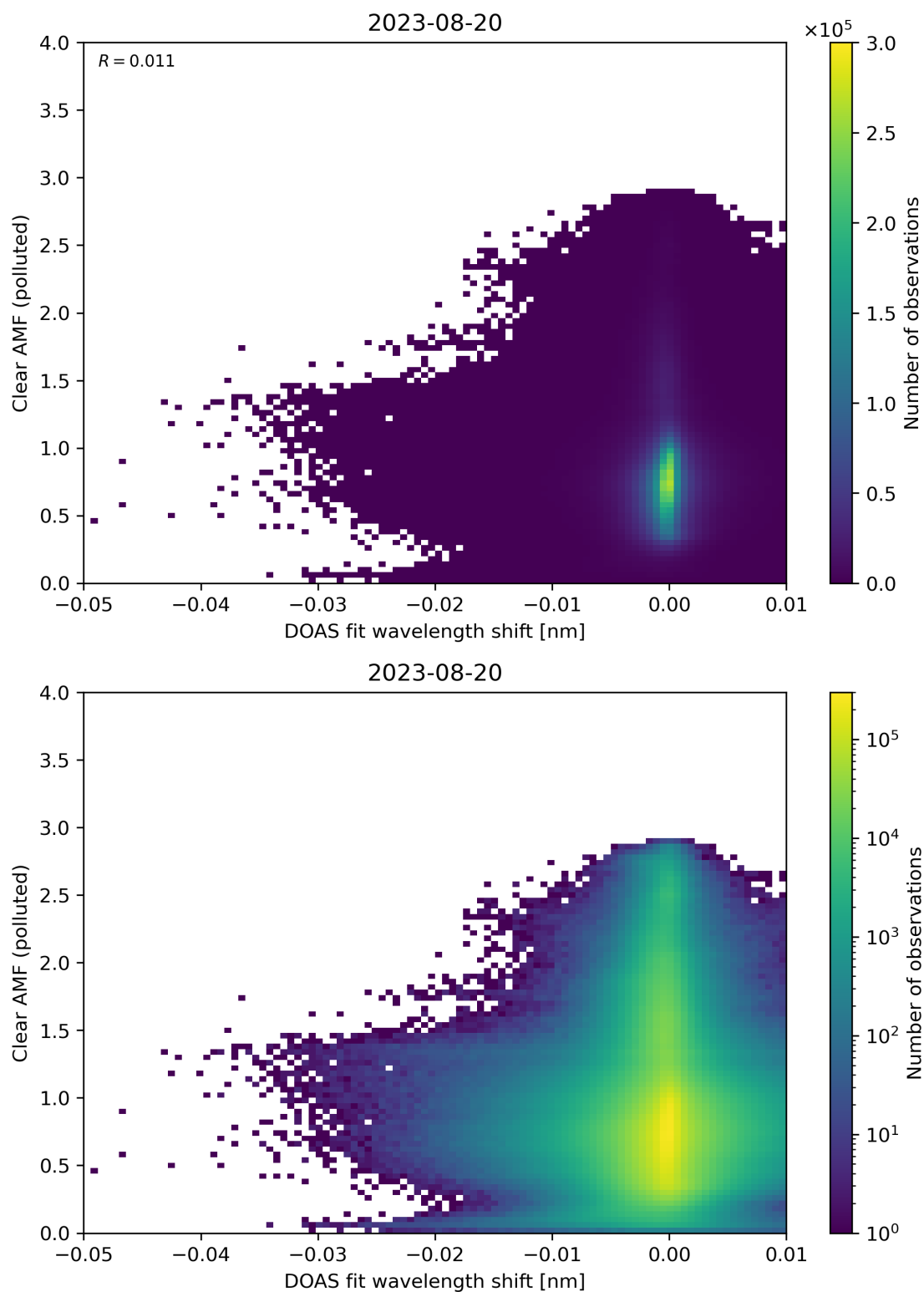
Figure 129: Scatter density plot of “DOAS fit wavelength shift” against “Clear AMF (polluted)” for 2023-08-20 to 2023-08-21.
