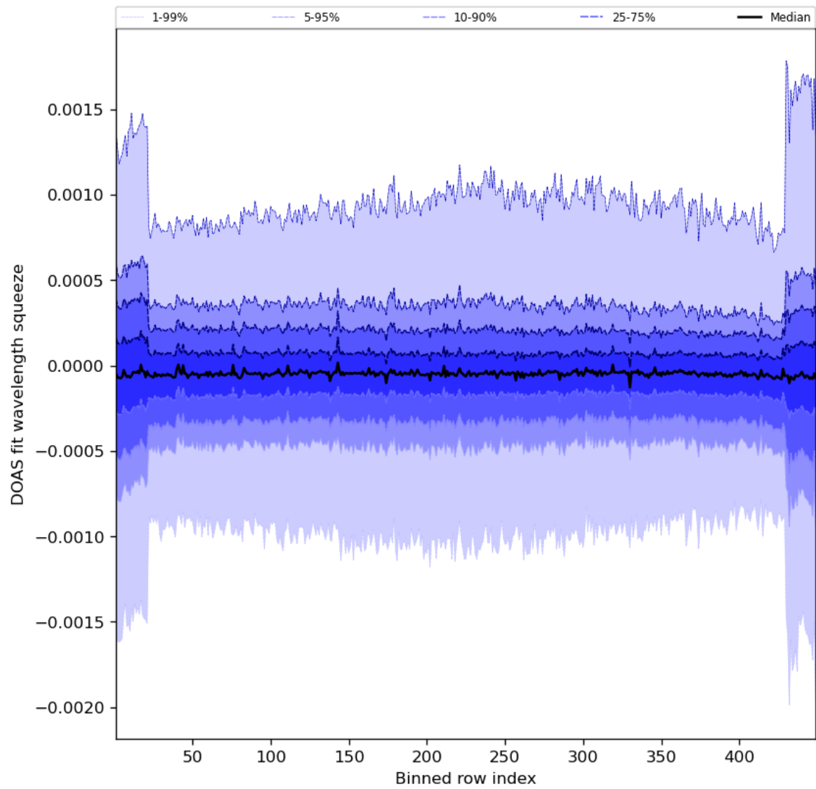
Figure 92: Along track statistics of “DOAS fit wavelength squeeze” for 2023-08-20 to 2023-08-21
