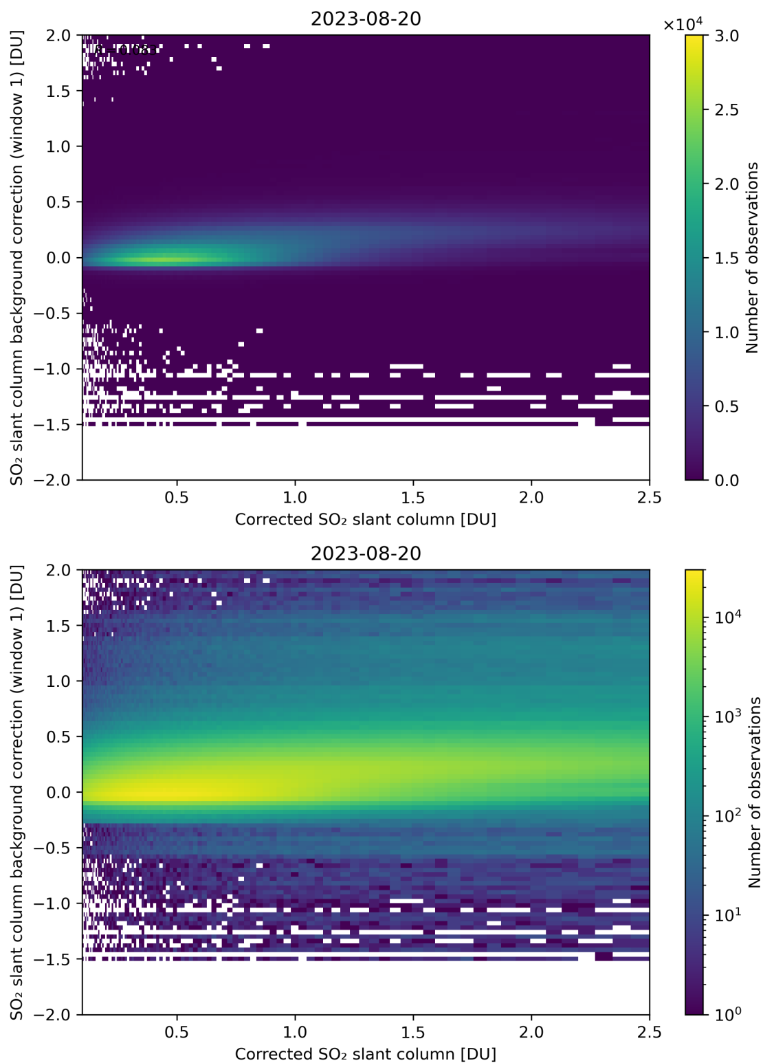
Figure 178: Scatter density plot of “Corrected SO 2 slant column” against “SO 2 slant column background correction (window 1)” for 2023-08-20 to 2023-08-21.
