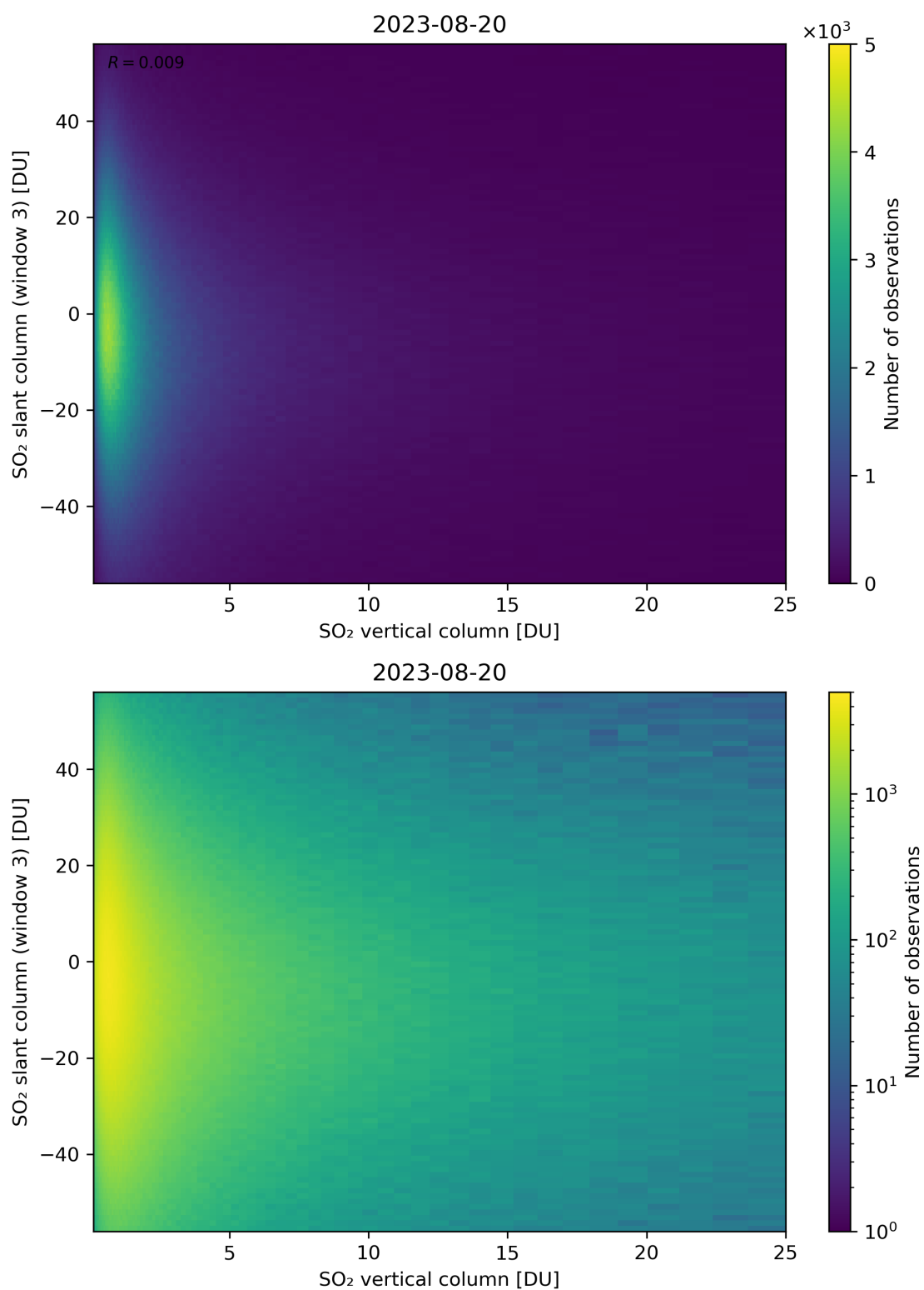
Figure 303: Scatter density plot of “SO 2 vertical column” against “SO 2 slant column (window 3)” for 2023-08-20 to 2023-08-21.
