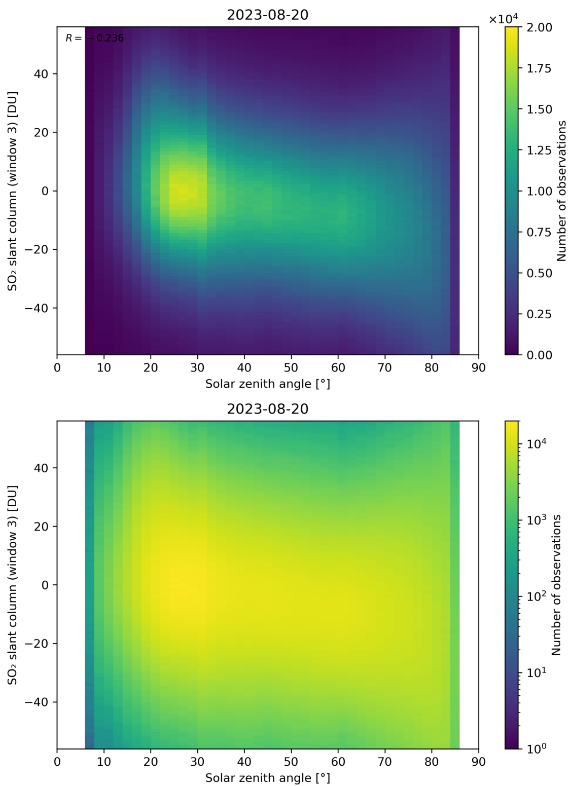
Figure 172: Scatter density plot of “Solar zenith angle” against “SO 2 slant column (window 3)” for 2023-08-20 to 2023-08-21.
