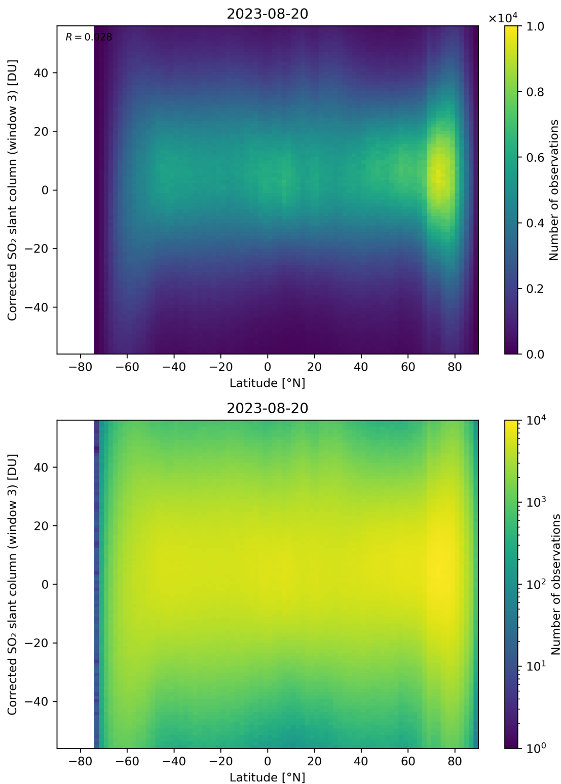
Figure 148: Scatter density plot of “Latitude” against “Corrected SO 2 slant column (window 3)” for 2023-08-20 to 2023-08-21.
