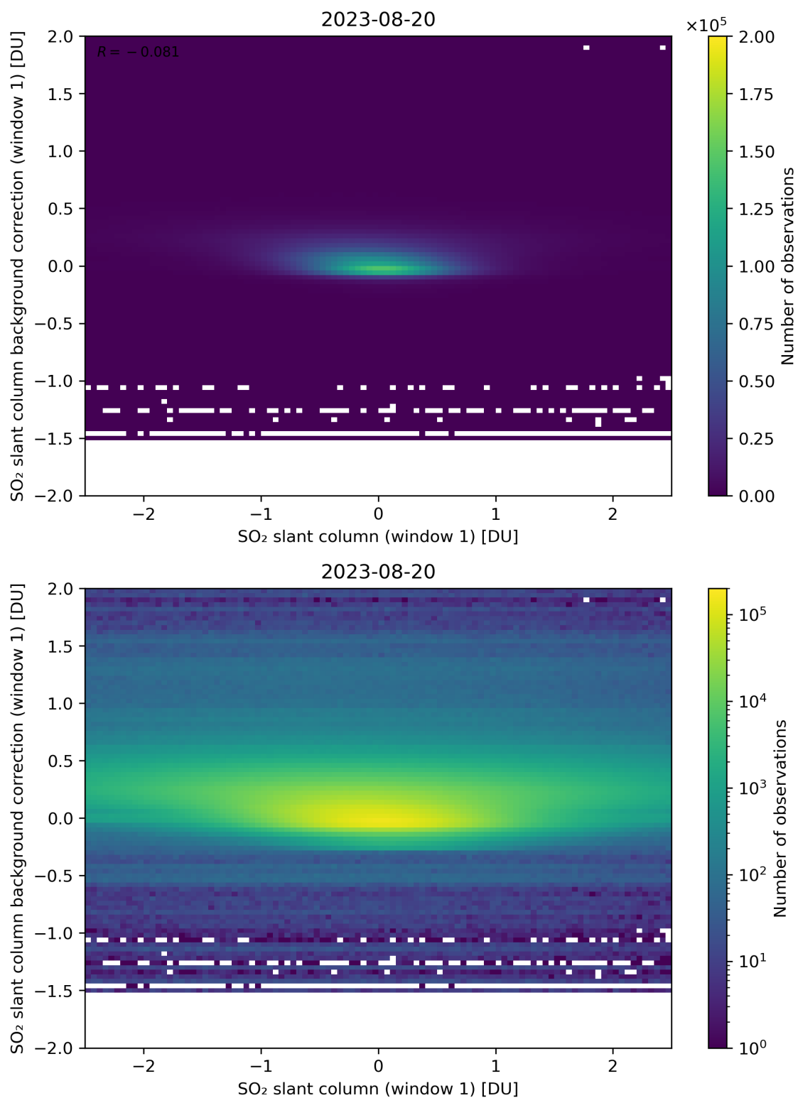
Figure 212: Scatter density plot of “SO 2 slant column (window 1)” against “SO 2 slant column background correction (window 1)” for 2023-08-20 to 2023-08-21.
