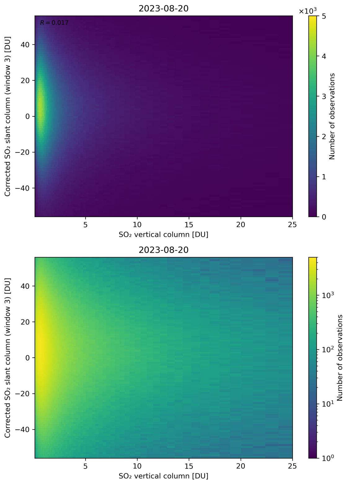
Figure 299: Scatter density plot of “SO 2 vertical column” against “Corrected SO 2 slant column (window 3)” for 2023-08-20 to 2023-08-21.
