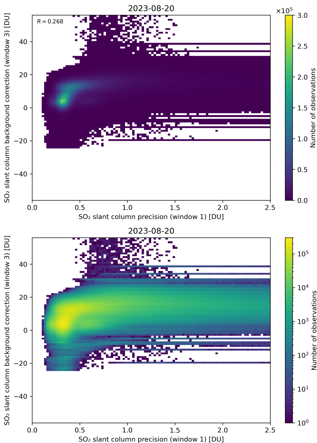
Figure 220: Scatter density plot of “SO 2 slant column precision (window 1)” against “SO 2 slant column background correction (window 3)” for 2023-08-20 to 2023-08-21.
