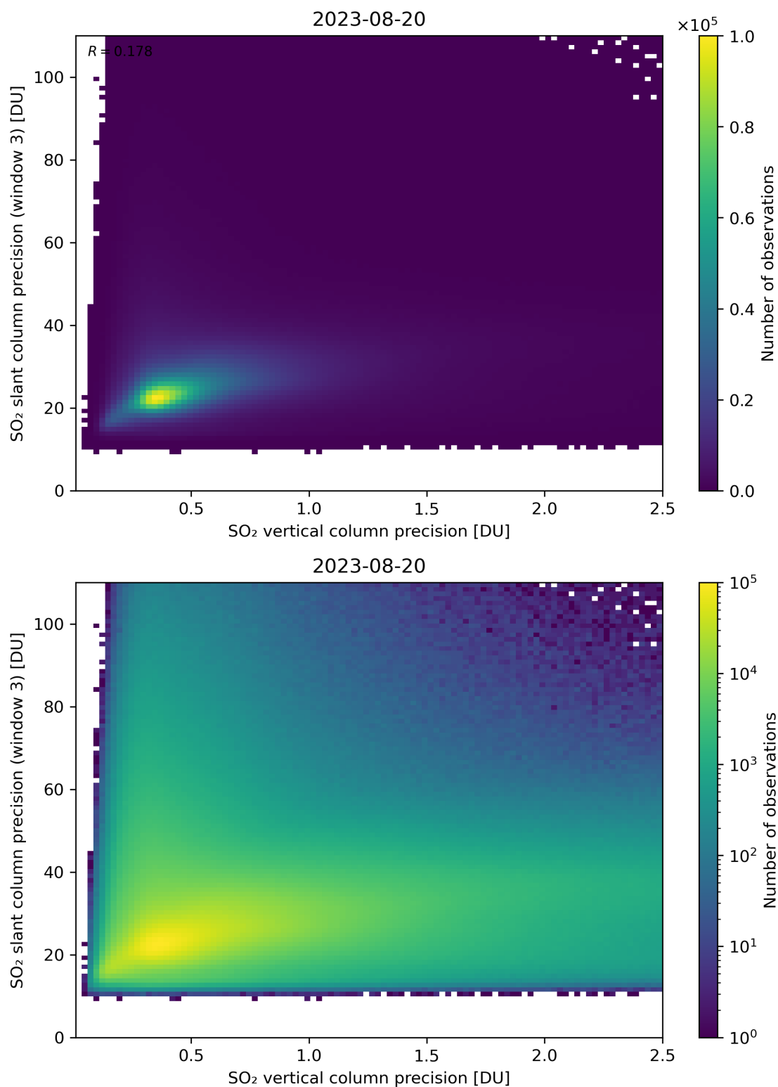
Figure 293: Scatter density plot of “SO 2 vertical column precision” against “SO 2 slant column precision (window 3)” for 2023-08-20 to 2023-08-21.
