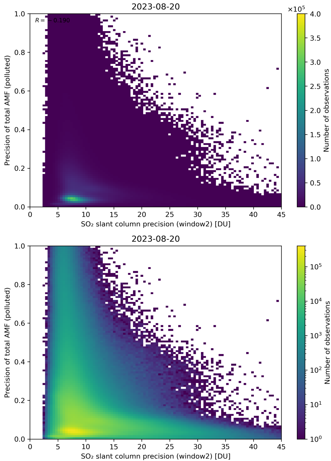
Figure 252: Scatter density plot of “SO 2 slant column precision (window2)” against “Precision of total AMF (polluted)” for 2023-08-20 to 2023-08-21.
