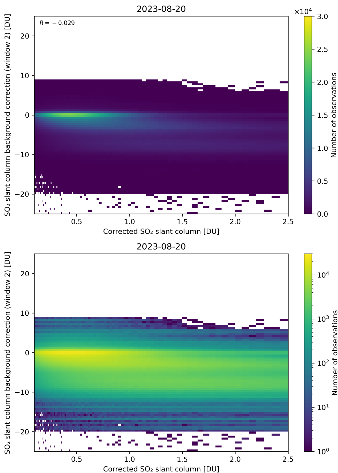
Figure 179: Scatter density plot of “Corrected SO 2 slant column” against “SO 2 slant column background correction (window 2)” for 2023-08-20 to 2023-08-21.
