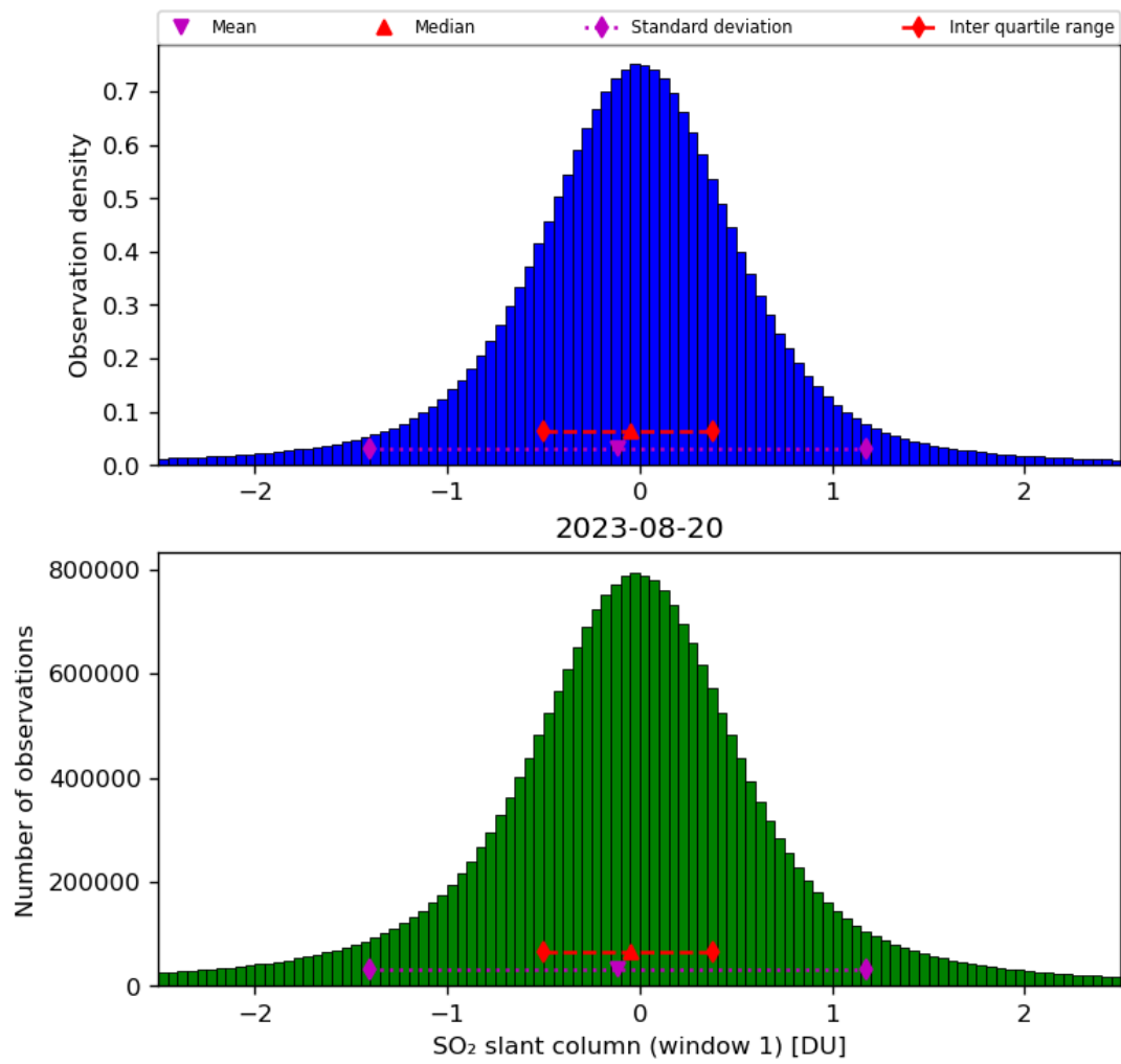
Figure 56: Histogram of “SO 2 slant column (window 1)” for 2023-08-20 to 2023-08-21
