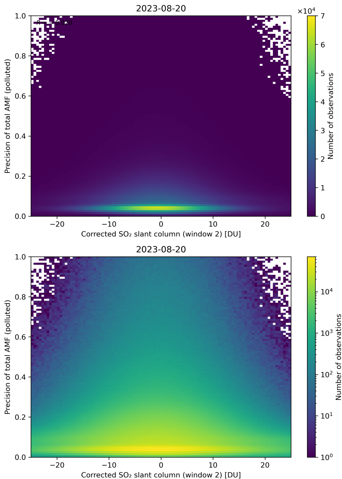
Figure 204: Scatter density plot of “Corrected SO 2 slant column (window 2)” against “Precision of total AMF (polluted)” for 2023-08-20 to 2023-08-21.
