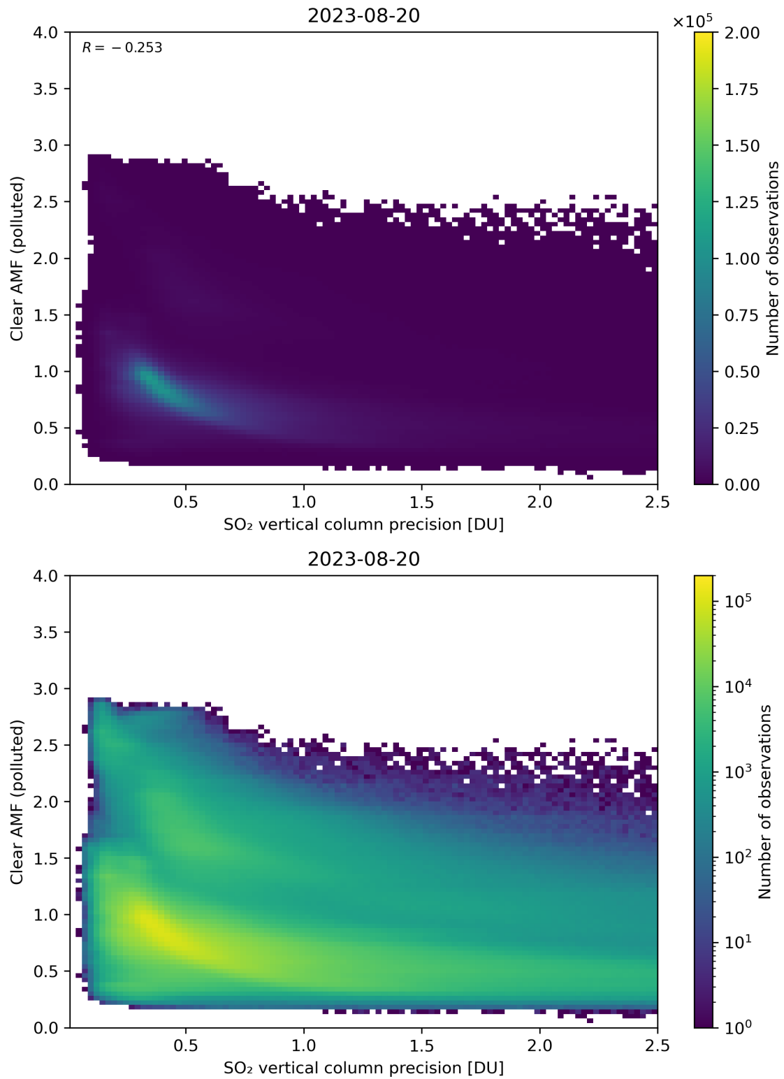
Figure 285: Scatter density plot of “SO 2 vertical column precision” against “Clear AMF (polluted)” for 2023-08-20 to 2023-08-21.
