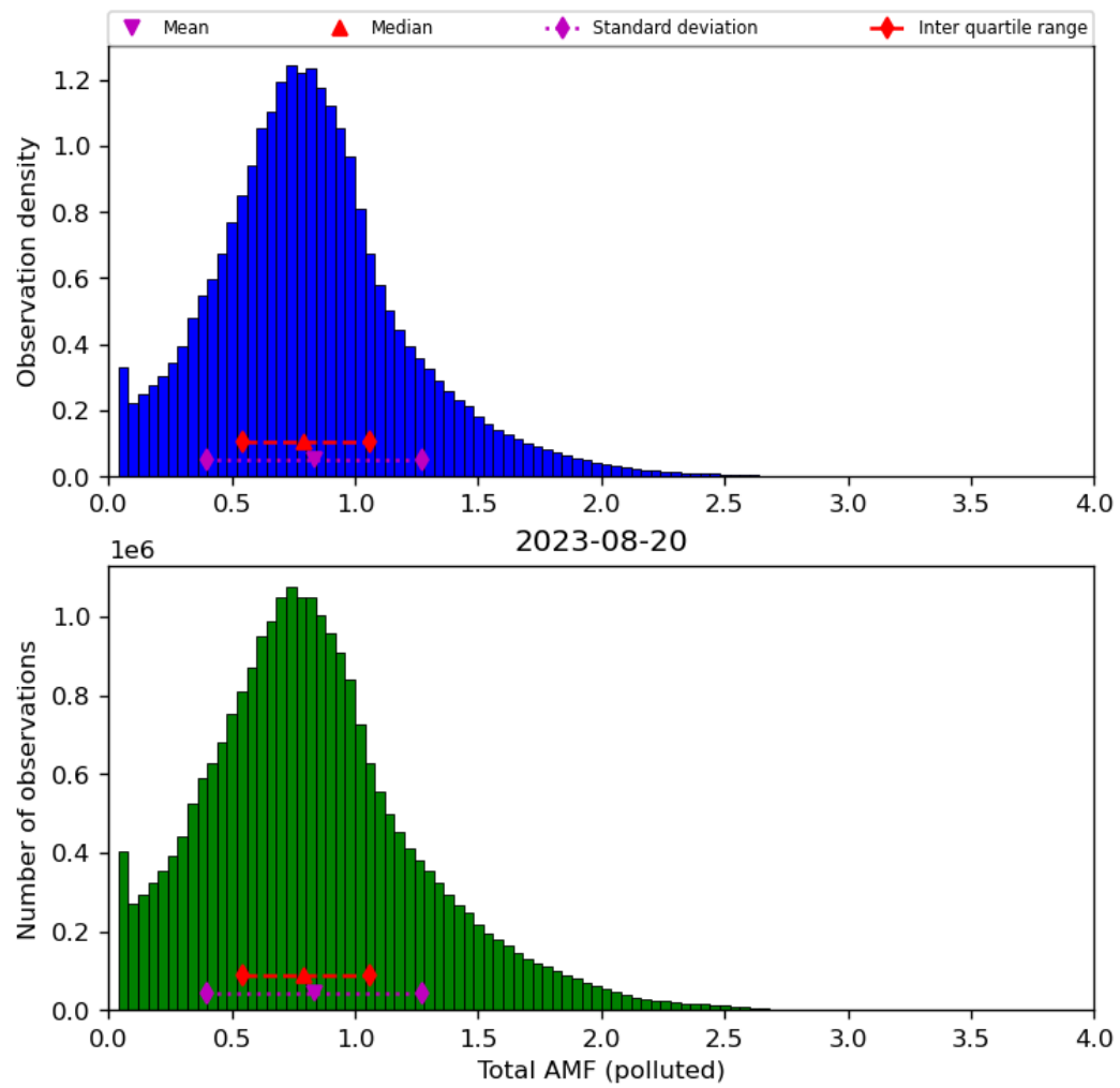
Figure 71: Histogram of “Total AMF (polluted)” for 2023-08-20 to 2023-08-21
