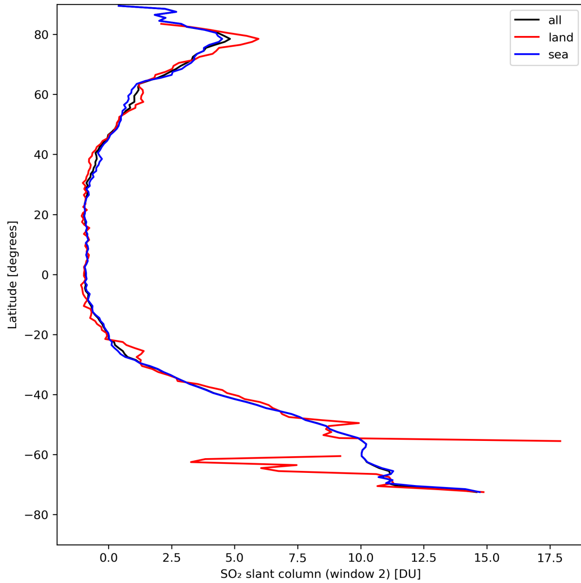
Figure 37: Zonal average of “SO 2 slant column (window 2)” for 2023-08-20 to 2023-08-21.
