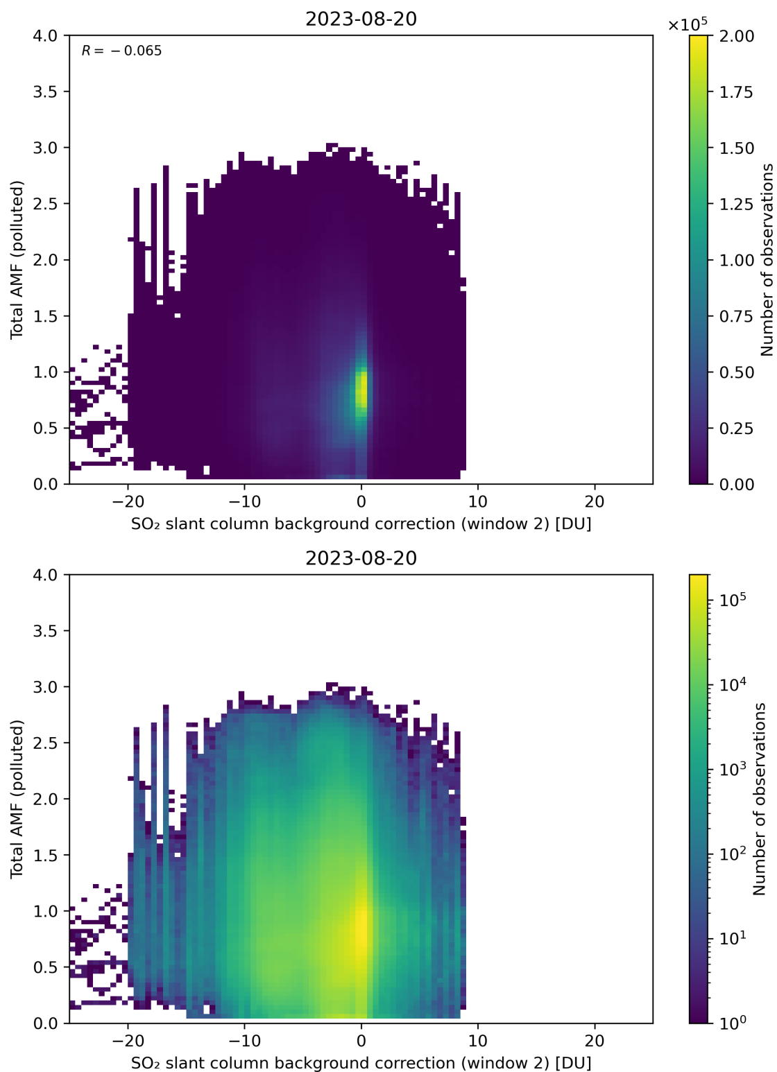
Figure 119: Scatter density plot of “SO 2 slant column background correction (window 2)” against “Total AMF (polluted)” for 2023-08-20 to 2023-08-21.
