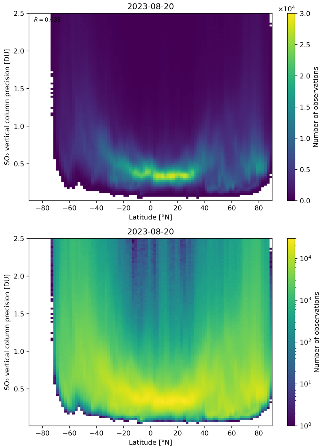
Figure 157: Scatter density plot of “Latitude” against “SO 2 vertical column precision” for 2023-08-20 to 2023-08-21.
