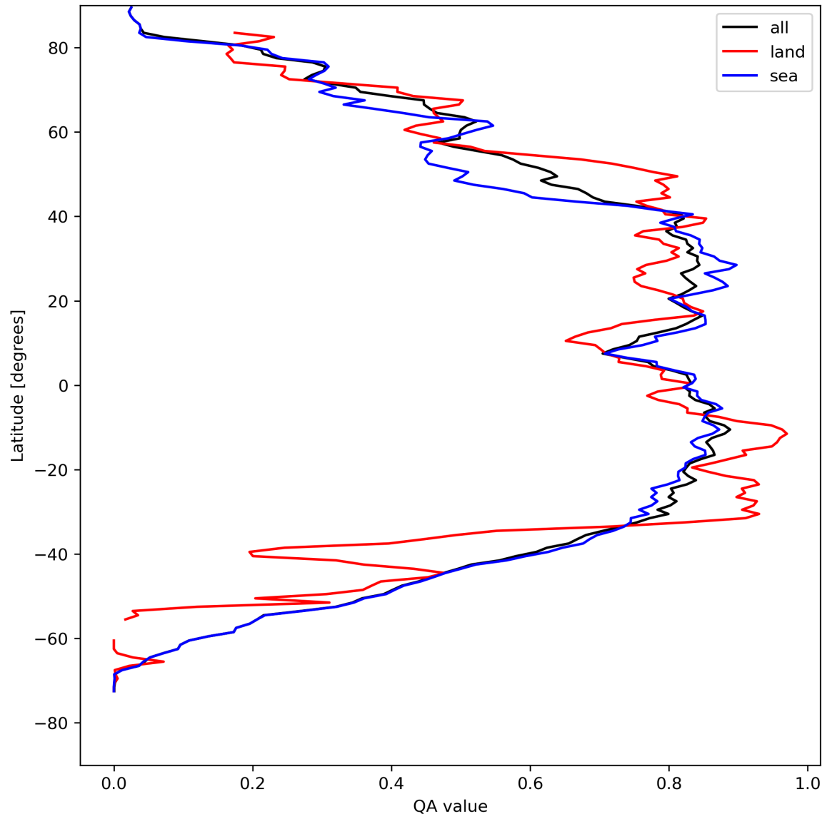
Figure 29: Zonal average of “QA value” for 2023-08-20 to 2023-08-21.
