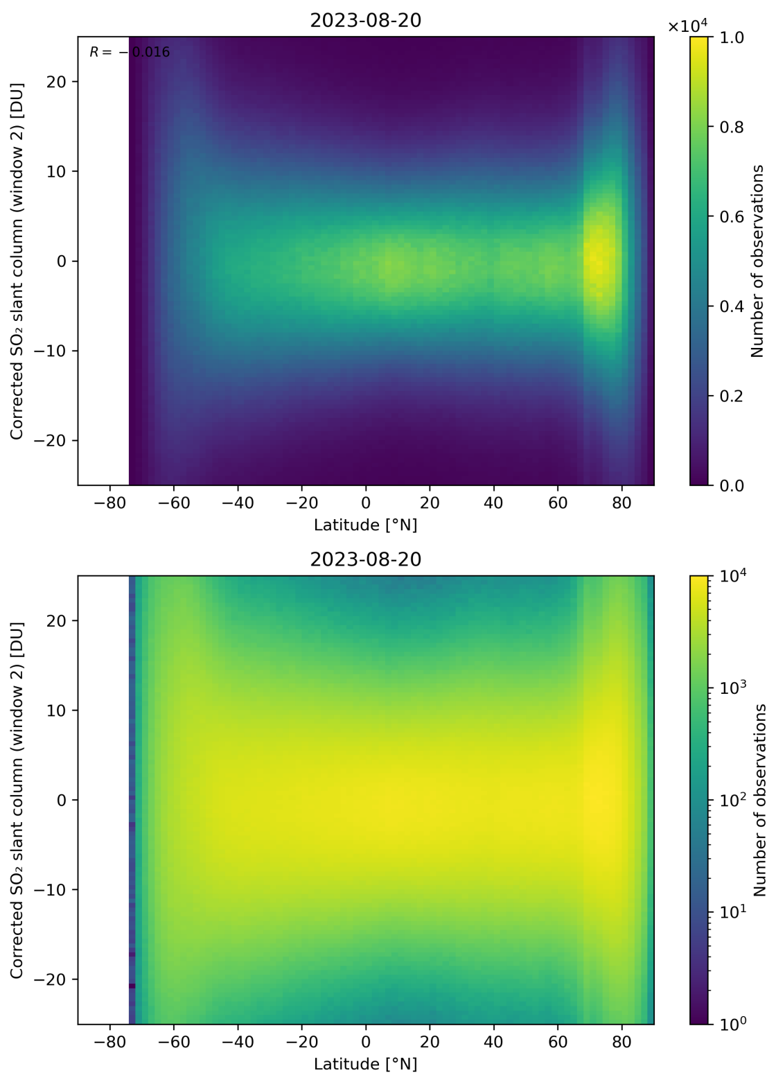
Figure 147: Scatter density plot of “Latitude” against “Corrected SO 2 slant column (window 2)” for 2023-08-20 to 2023-08-21.
