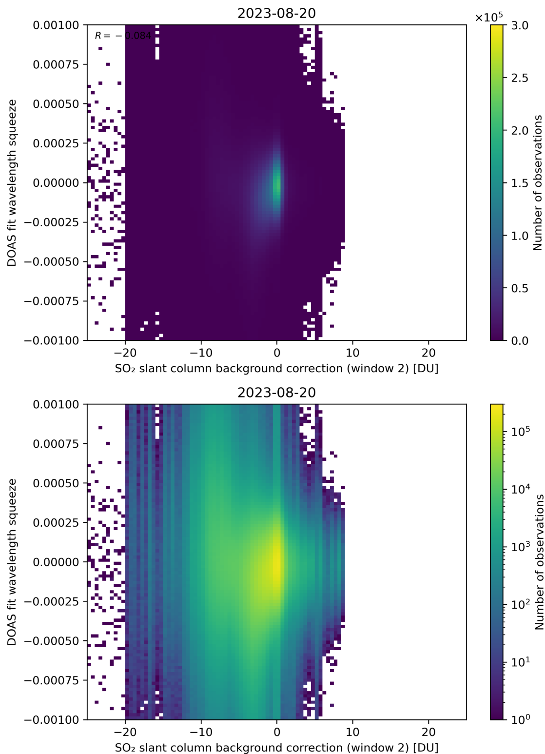
Figure 113: Scatter density plot of “SO 2 slant column background correction (window 2)” against “DOAS fit wavelength squeeze” for 2023-08-20 to 2023-08-21.
