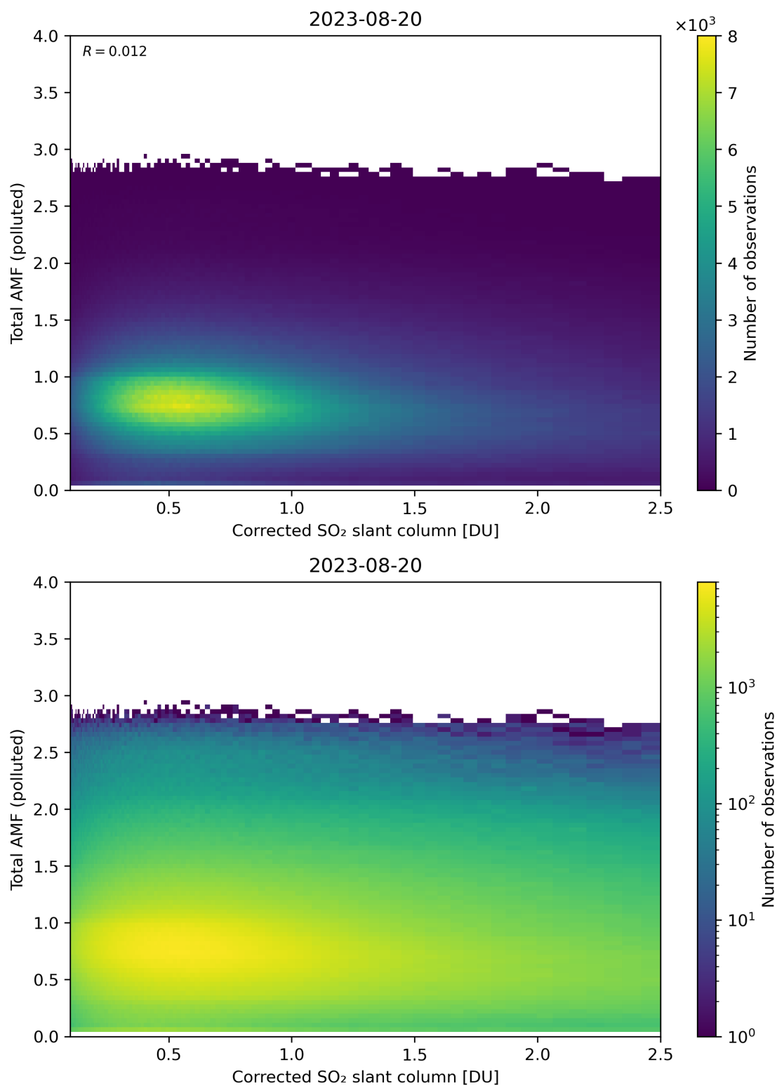
Figure 192: Scatter density plot of “Corrected SO 2 slant column” against “Total AMF (polluted)” for 2023-08-20 to 2023-08-21.
