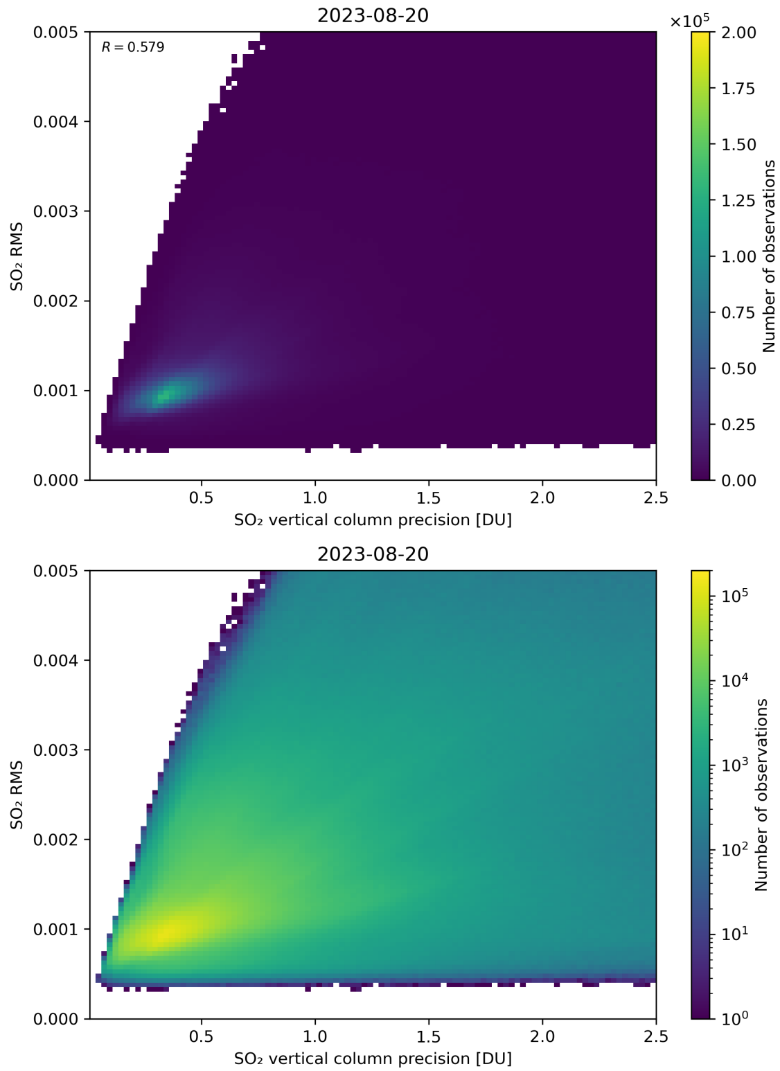
Figure 284: Scatter density plot of “SO 2 vertical column precision” against “SO 2 RMS” for 2023-08-20 to 2023-08-21.
