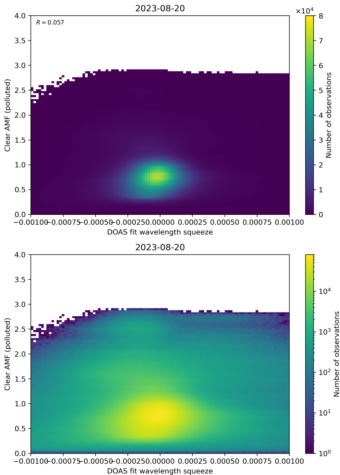
Figure 133: Scatter density plot of “DOAS fit wavelength squeeze” against “Clear AMF (polluted)” for 2023-08-20 to 2023-08-21.
