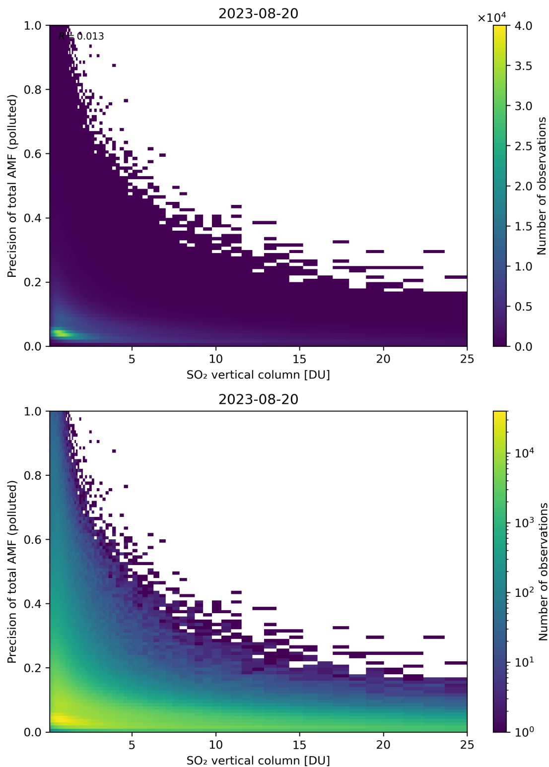
Figure 306: Scatter density plot of “SO 2 vertical column” against “Precision of total AMF (polluted)” for 2023-08-20 to 2023-08-21.
