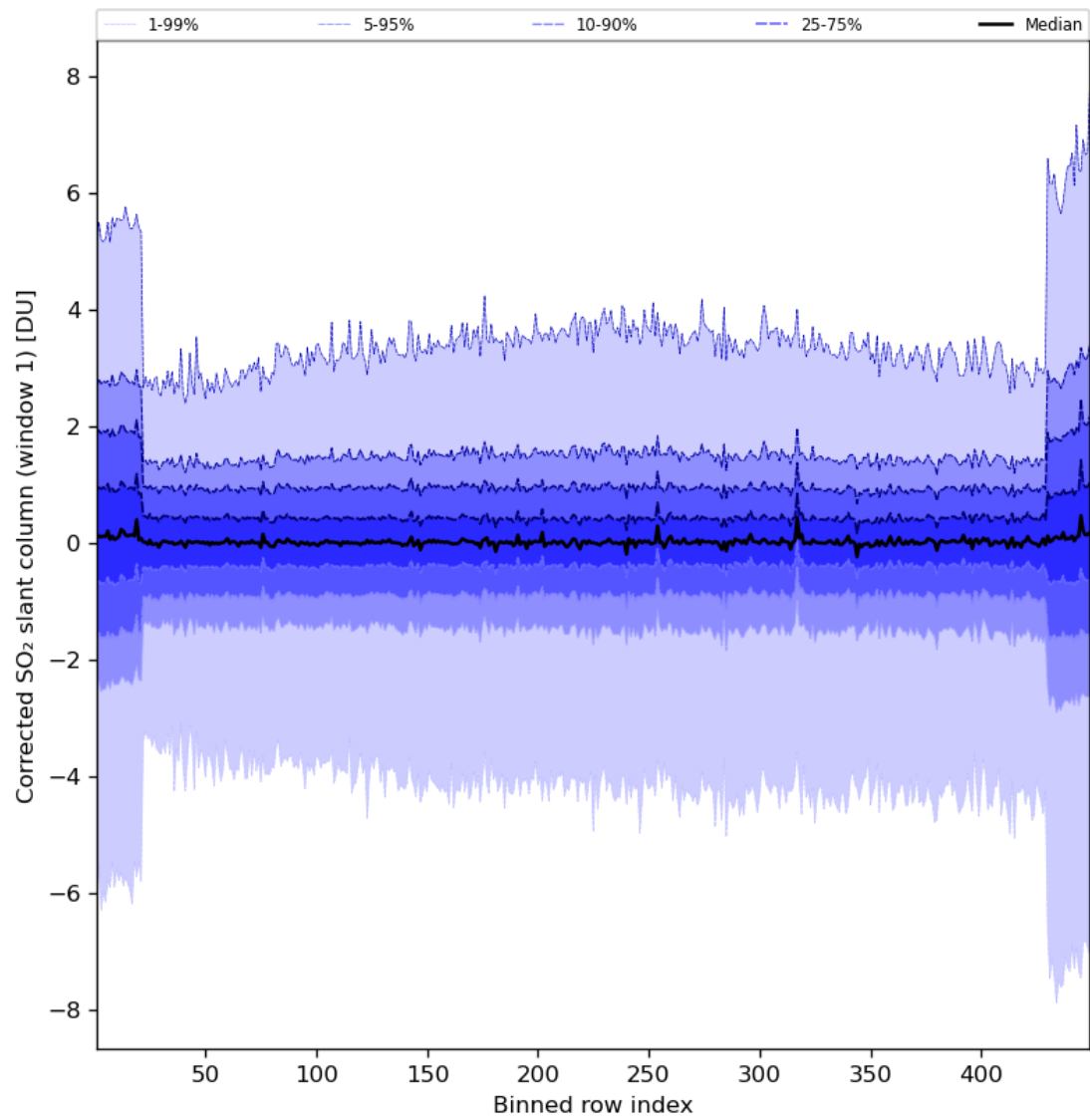
Figure 81: Along track statistics of “Corrected SO 2 slant column (window 1)” for 2023-08-20 to 2023-08-21
