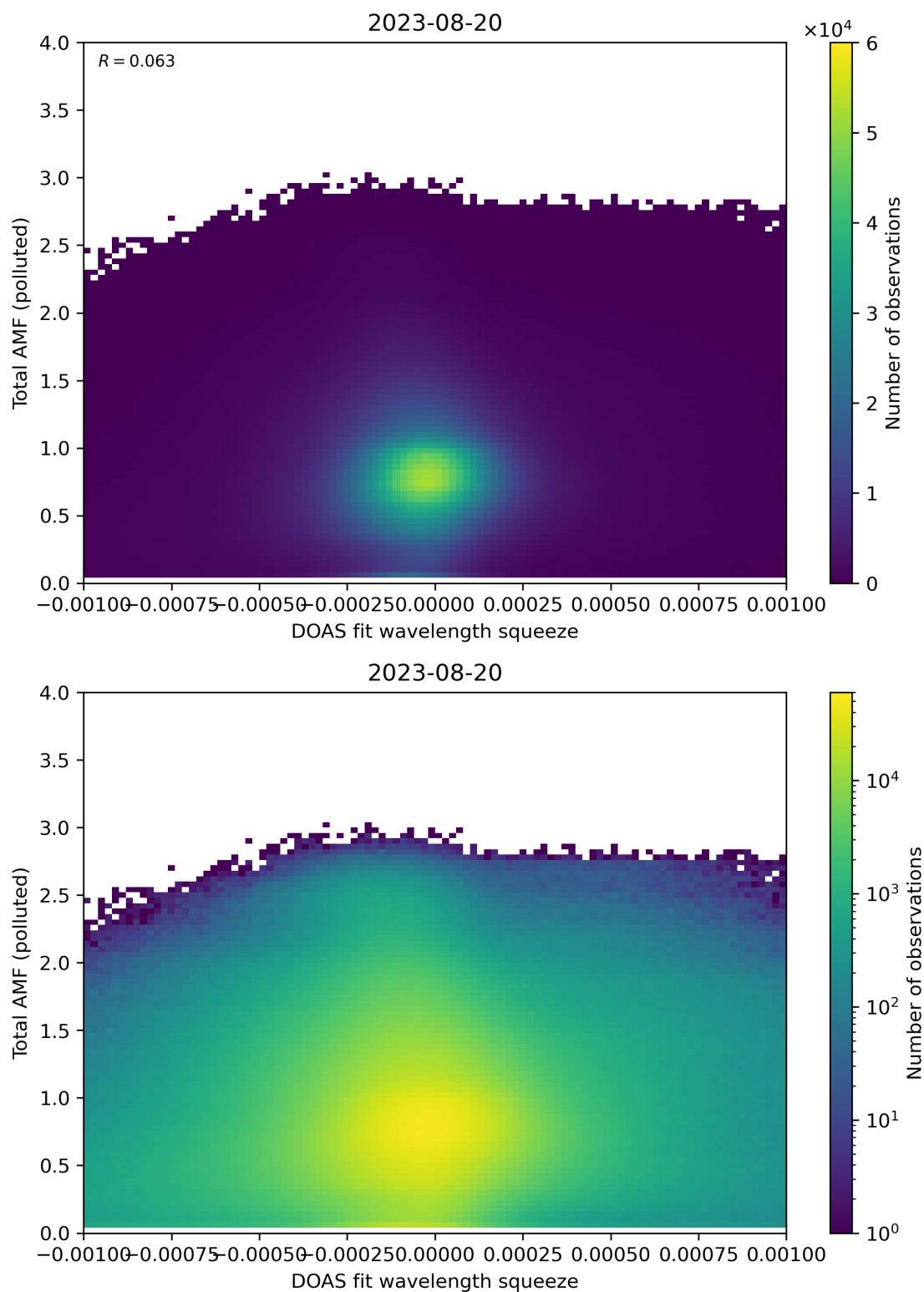
Figure 134: Scatter density plot of “DOAS fit wavelength squeeze” against “Total AMF (polluted)” for 2023-08-20 to 2023-08-21.
