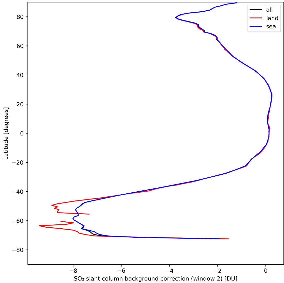
Figure 40: Zonal average of “SO 2 slant column background correction (window 2)” for 2023-08-20 to 2023-08-21.
