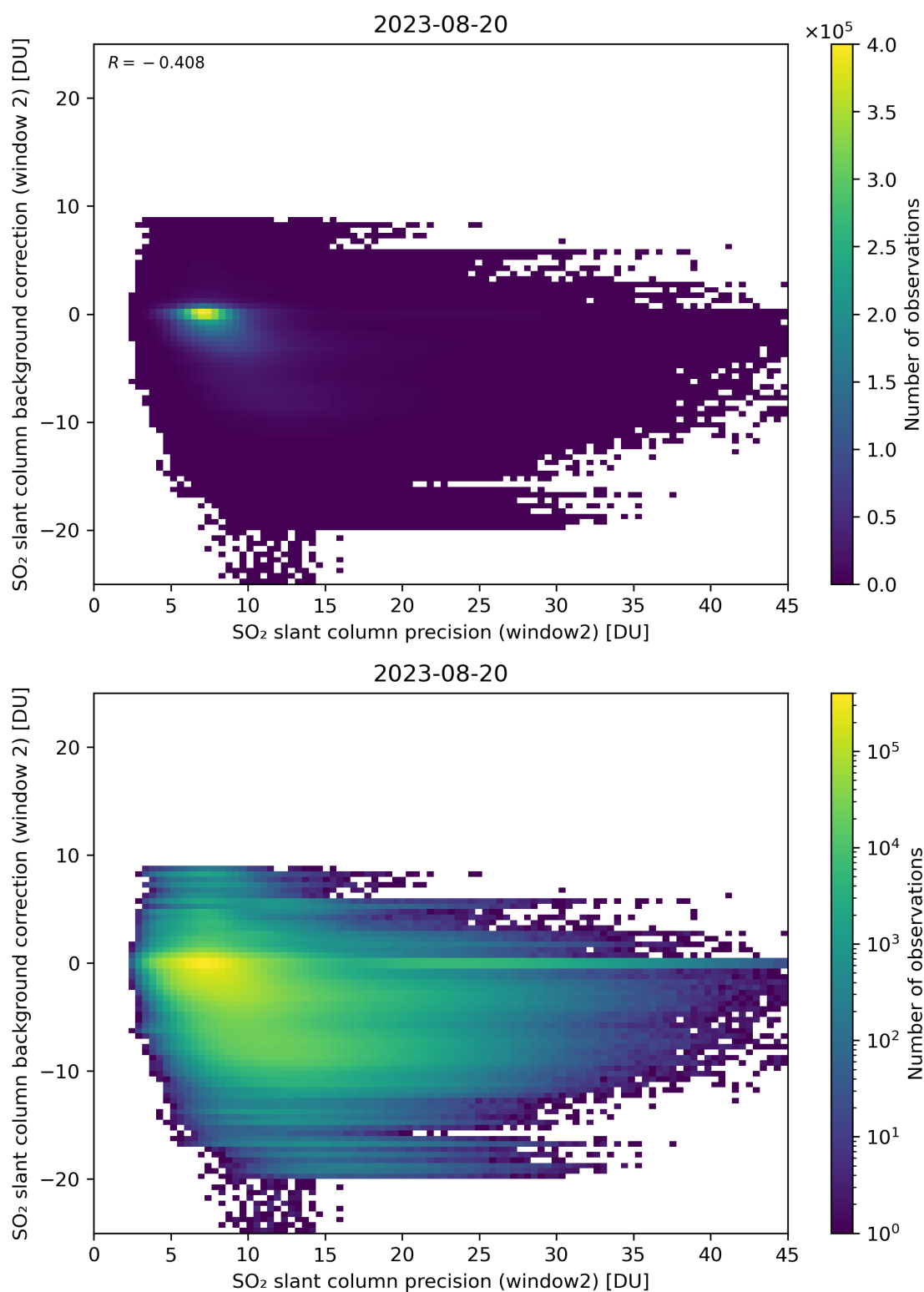
Figure 241: Scatter density plot of “SO 2 slant column precision (window2)” against “SO 2 slant column background correction (window 2)” for 2023-08-20 to 2023-08-21.
