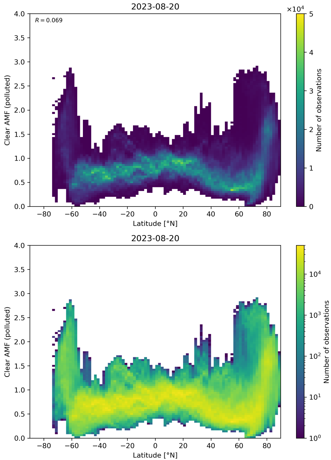
Figure 145: Scatter density plot of “Latitude” against “Clear AMF (polluted)” for 2023-08-20 to 2023-08-21.
