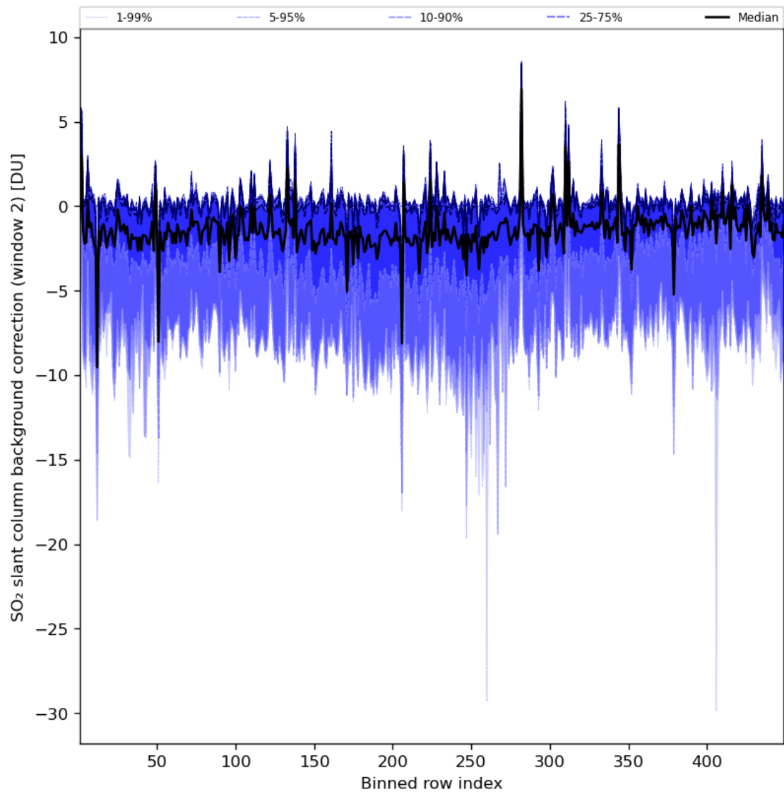
Figure 86: Along track statistics of “SO 2 slant column background correction (window 2)” for 2023-08-20 to 2023-08-21
