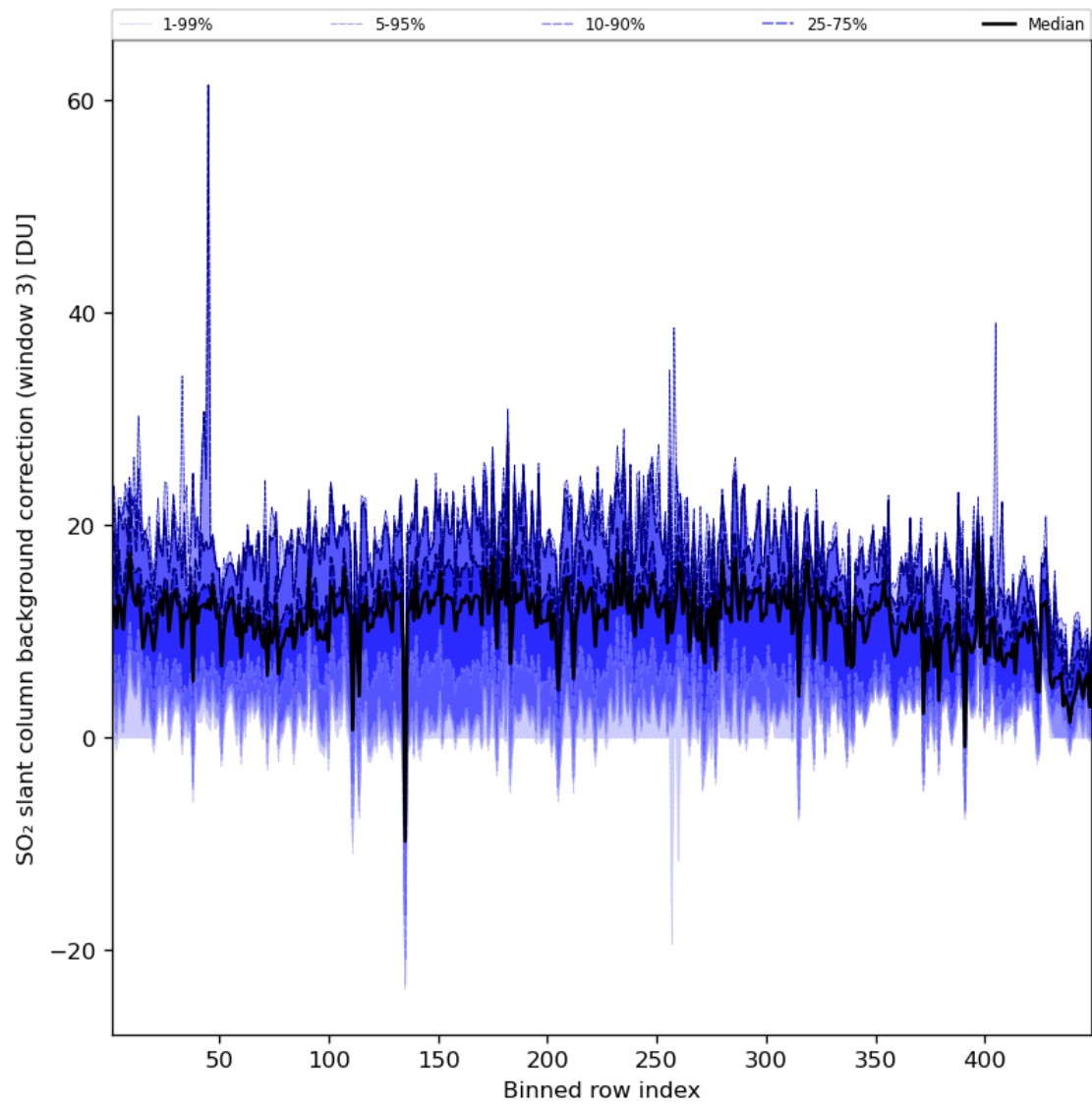
Figure 90: Along track statistics of “SO 2 slant column background correction (window 3)” for 2023-08-20 to 2023-08-21
