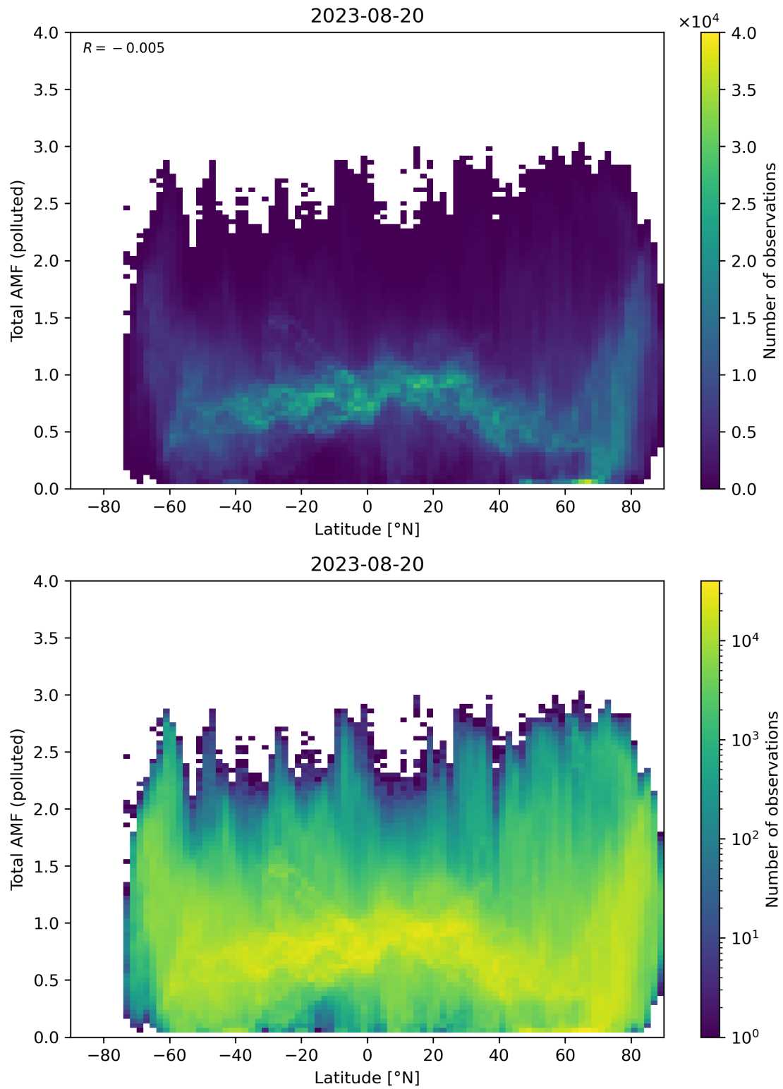
Figure 154: Scatter density plot of “Latitude” against “Total AMF (polluted)” for 2023-08-20 to 2023-08-21.
