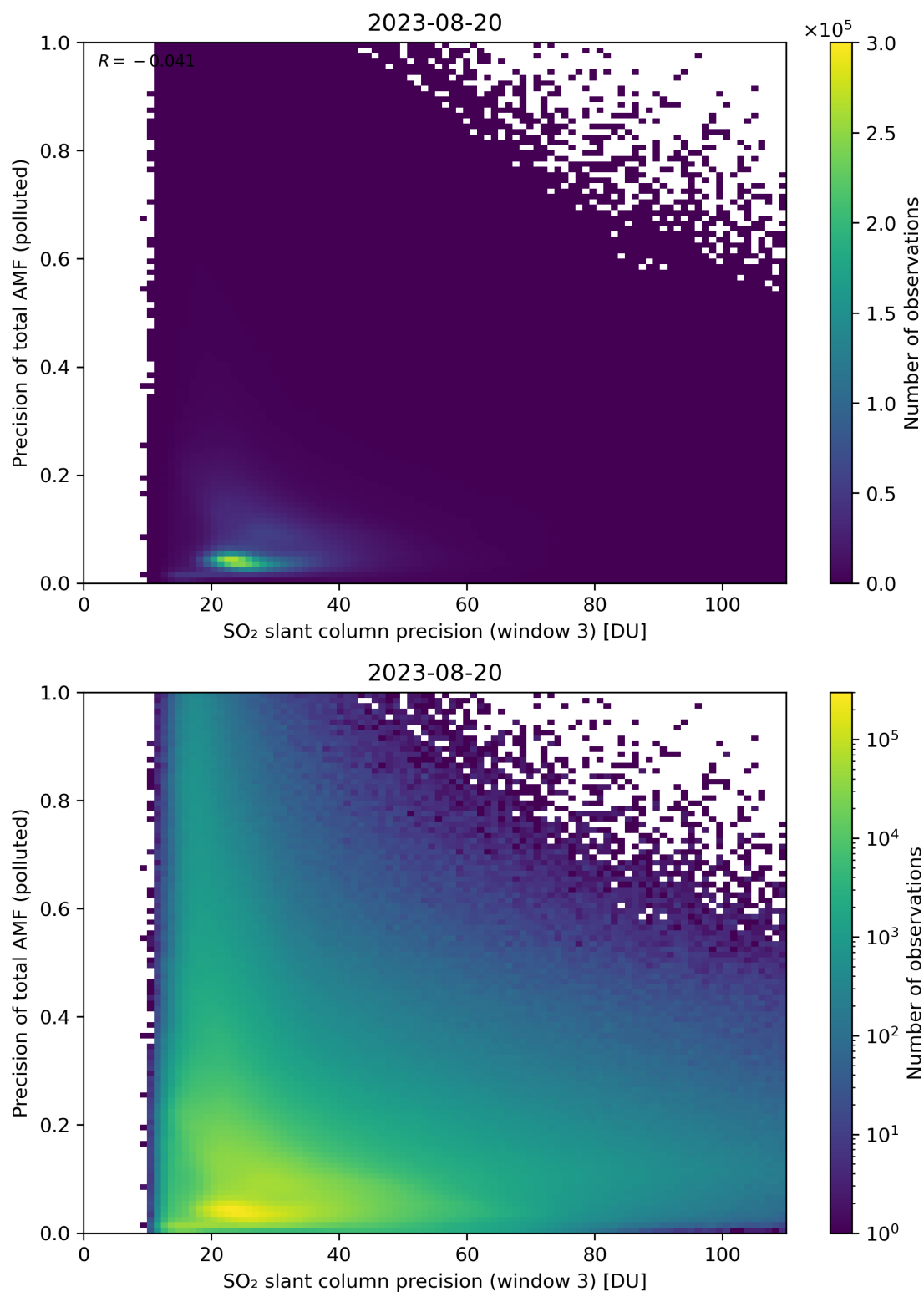
Figure 264: Scatter density plot of “SO 2 slant column precision (window 3)” against “Precision of total AMF (polluted)” for 2023-08-20 to 2023-08-21.
