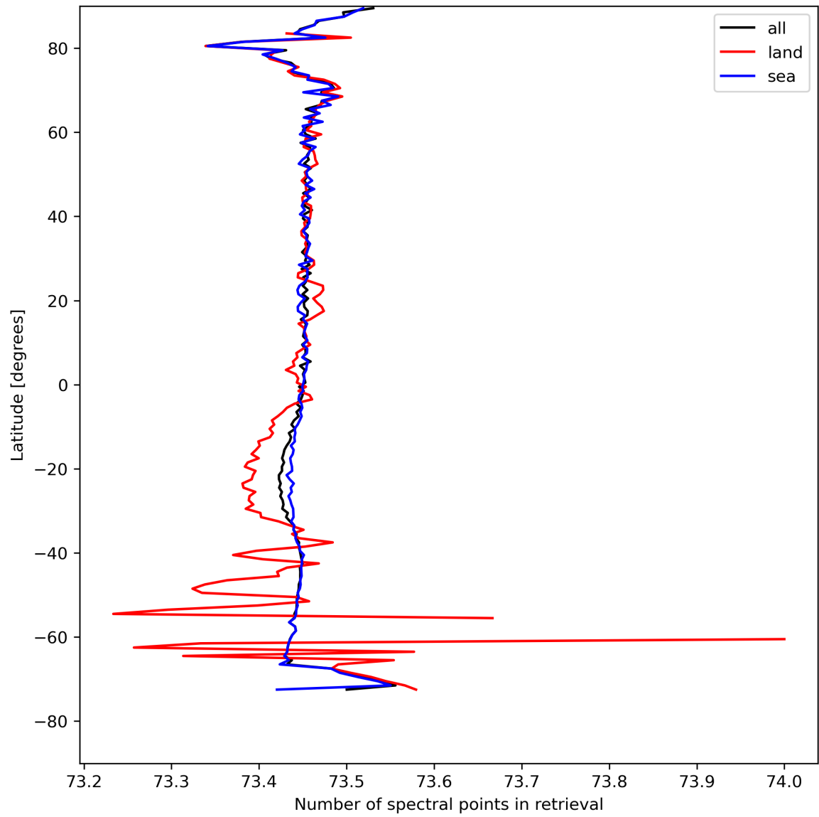
Figure 51: Zonal average of “Number of spectral points in retrieval” for 2023-08-20 to 2023-08-21.
