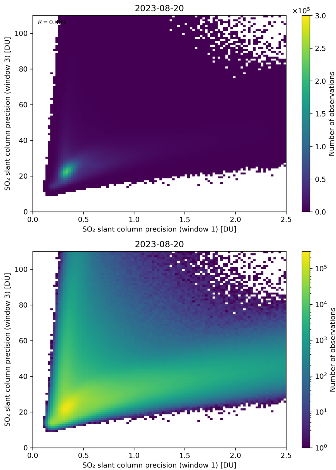
Figure 229: Scatter density plot of “SO 2 slant column precision (window 1)” against “SO 2 slant column precision (window 3)” for 2023-08-20 to 2023-08-21.
