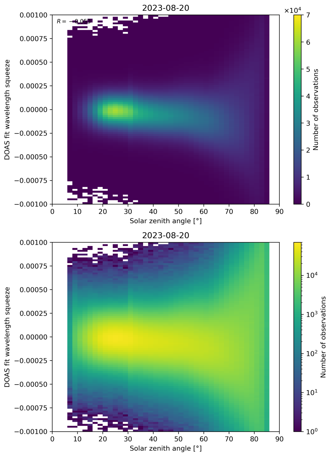
Figure 162: Scatter density plot of “Solar zenith angle” against “DOAS fit wavelength squeeze” for 2023-08-20 to 2023-08-21.
