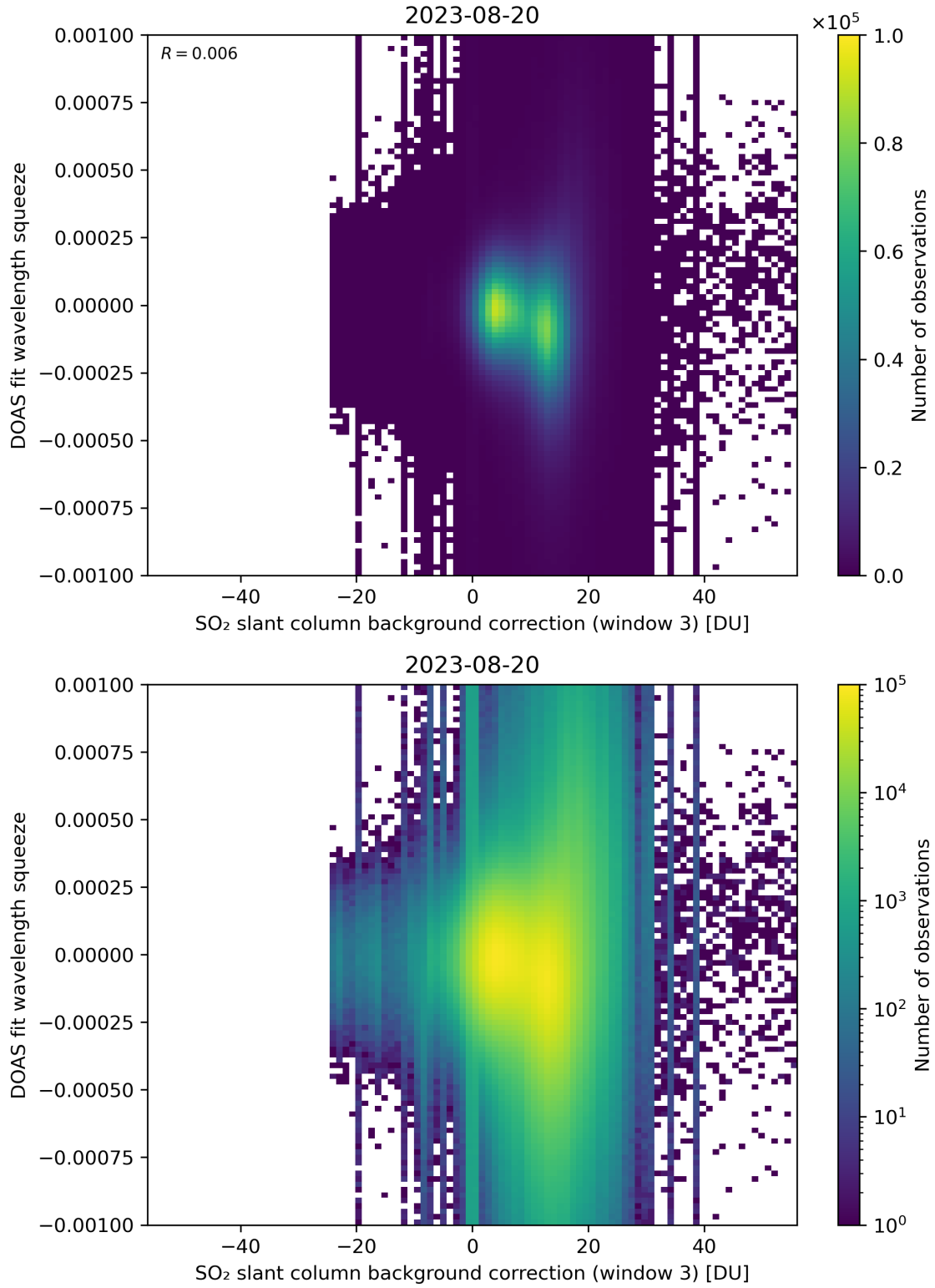
Figure 122: Scatter density plot of “SO 2 slant column background correction (window 3)” against “DOAS fit wavelength squeeze” for 2023-08-20 to 2023-08-21.
