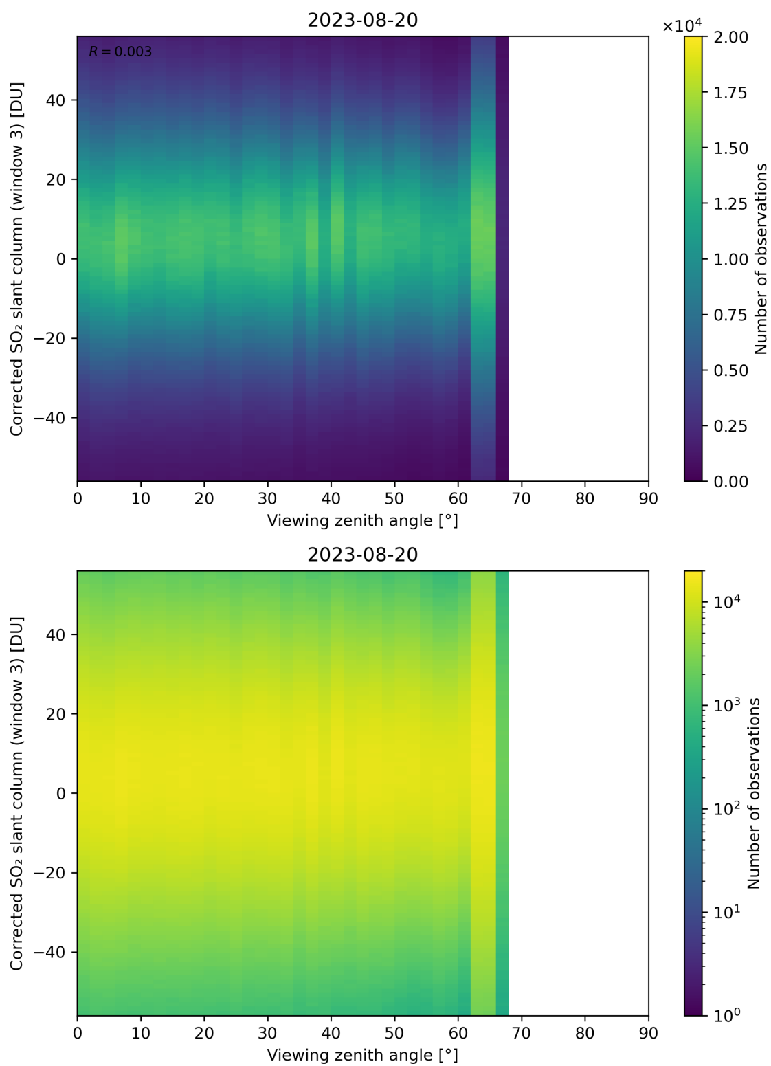
Figure 319: Scatter density plot of “Viewing zenith angle” against “Corrected SO 2 slant column (window 3)” for 2023-08-20 to 2023-08-21.
