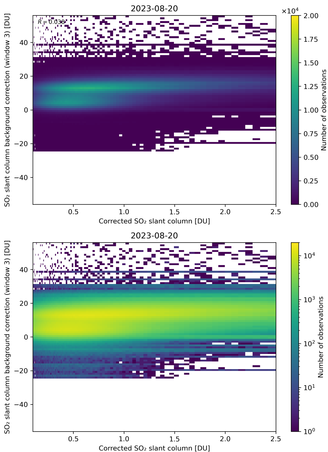
Figure 180: Scatter density plot of “Corrected SO 2 slant column” against “SO 2 slant column background correction (window 3)” for 2023-08-20 to 2023-08-21.
