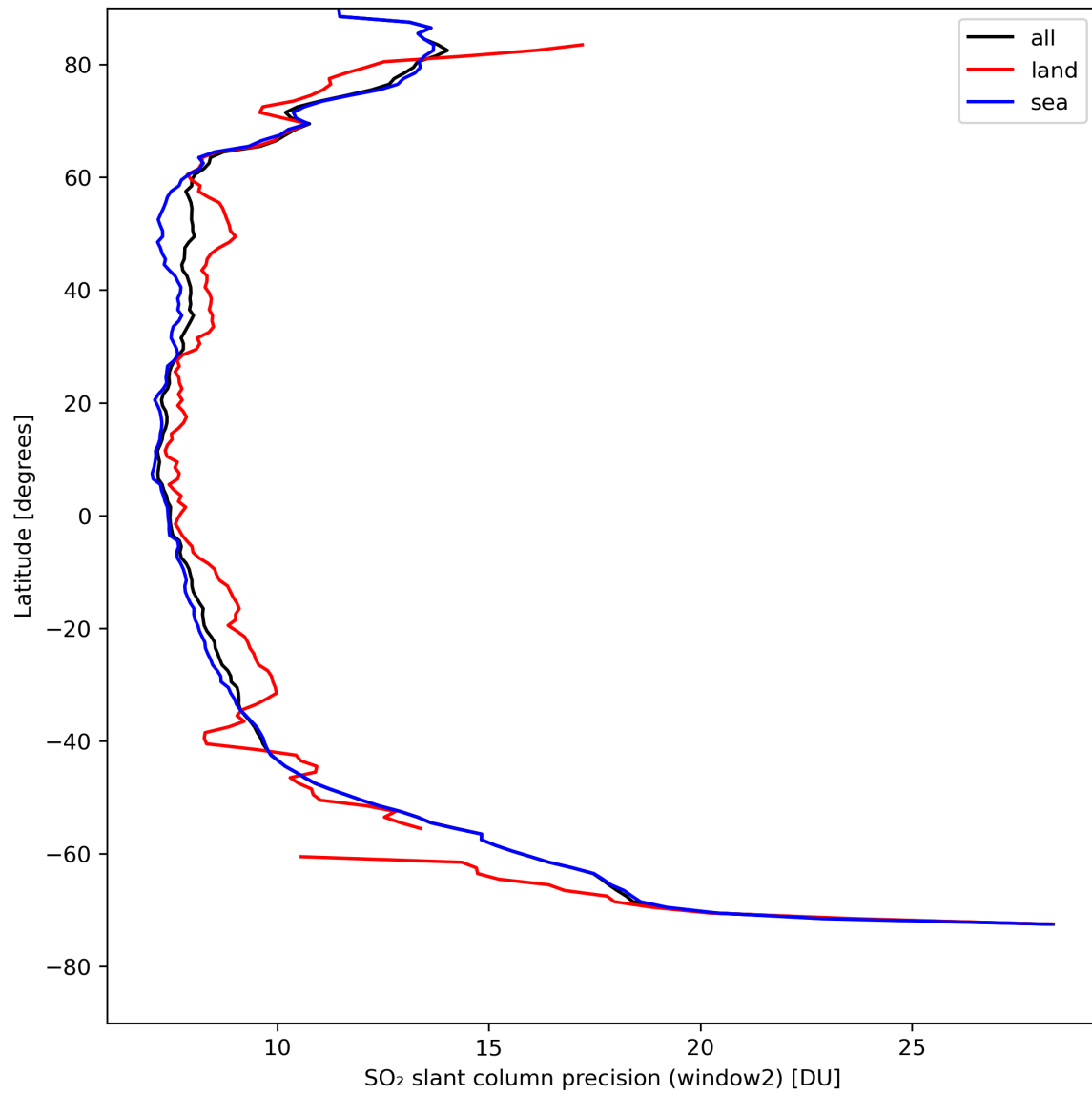
Figure 38: Zonal average of “SO 2 slant column precision (window2)” for 2023-08-20 to 2023-08-21.
