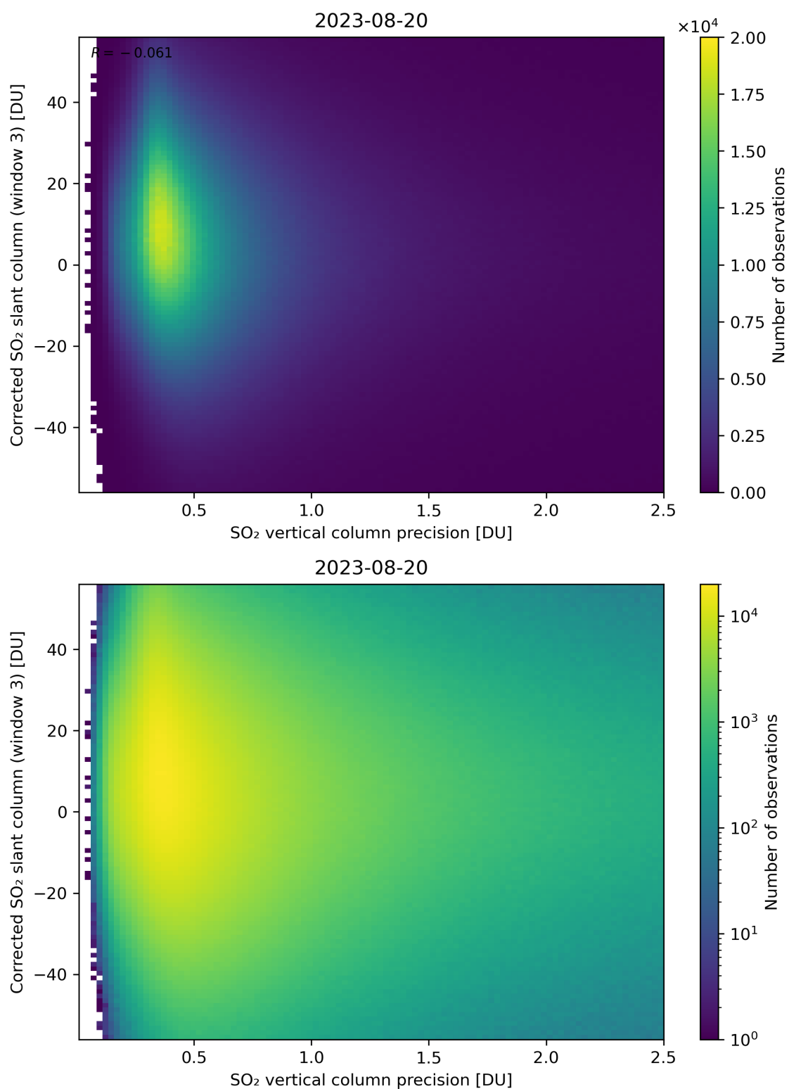
Figure 288: Scatter density plot of “SO 2 vertical column precision” against “Corrected SO 2 slant column (window 3)” for 2023-08-20 to 2023-08-21.
