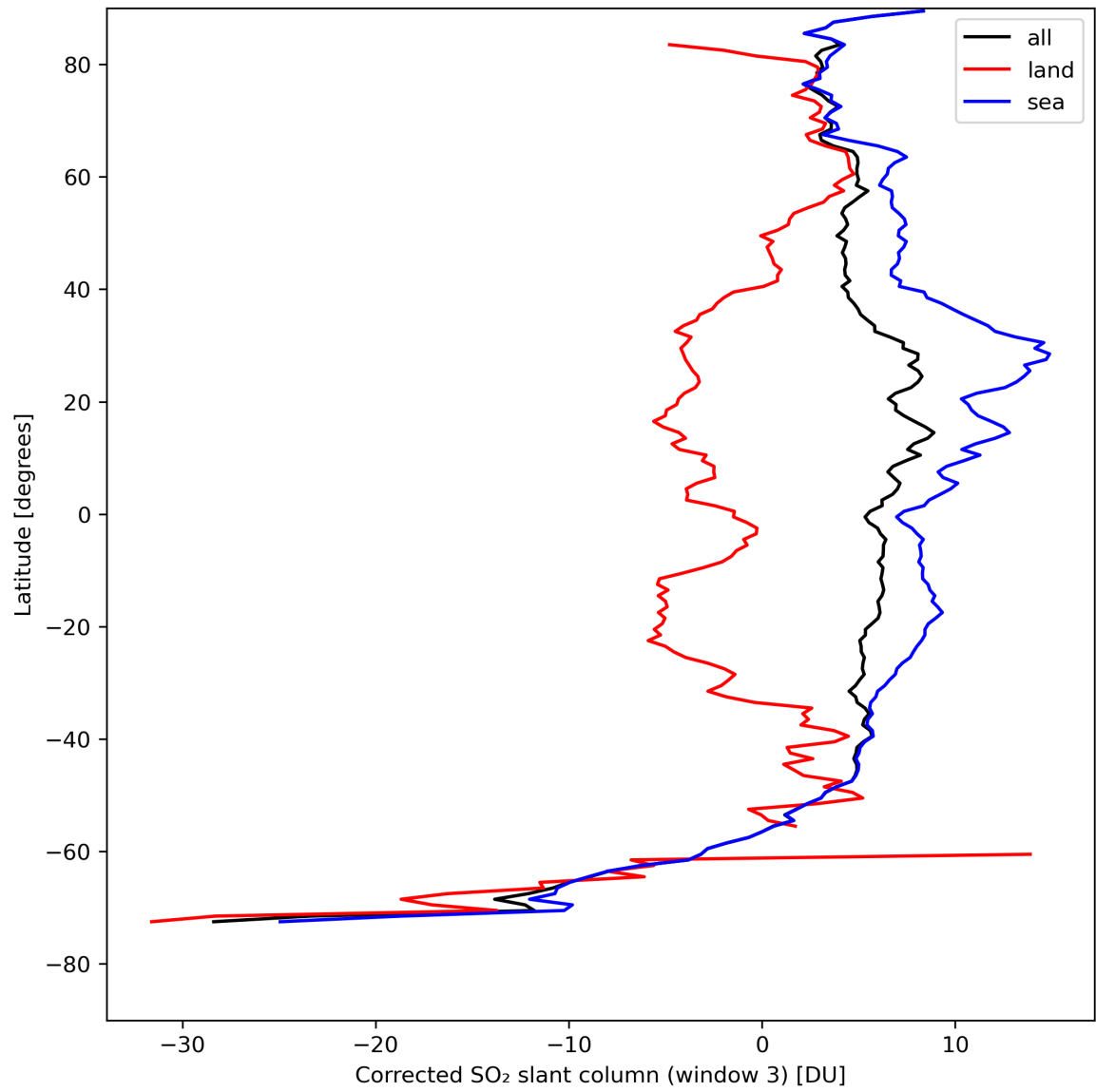
Figure 43: Zonal average of “Corrected SO 2 slant column (window 3)” for 2023-08-20 to 2023-08-21.
