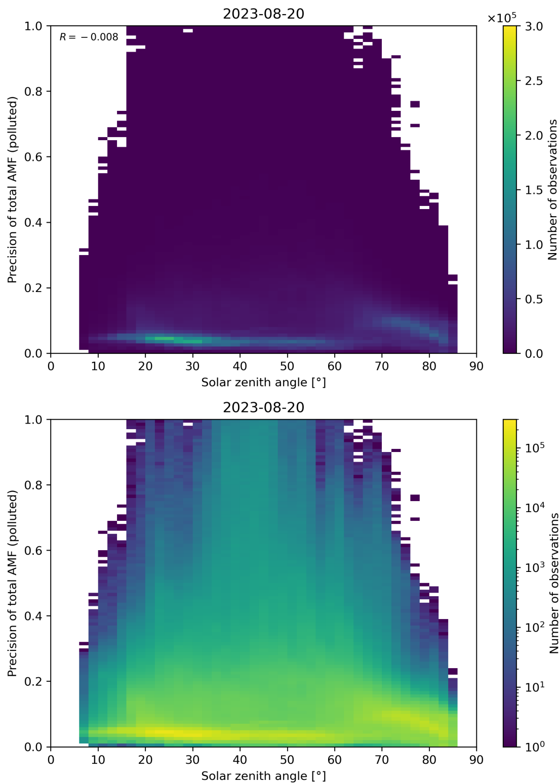
Figure 175: Scatter density plot of “Solar zenith angle” against “Precision of total AMF (polluted)” for 2023-08-20 to 2023-08-21.
