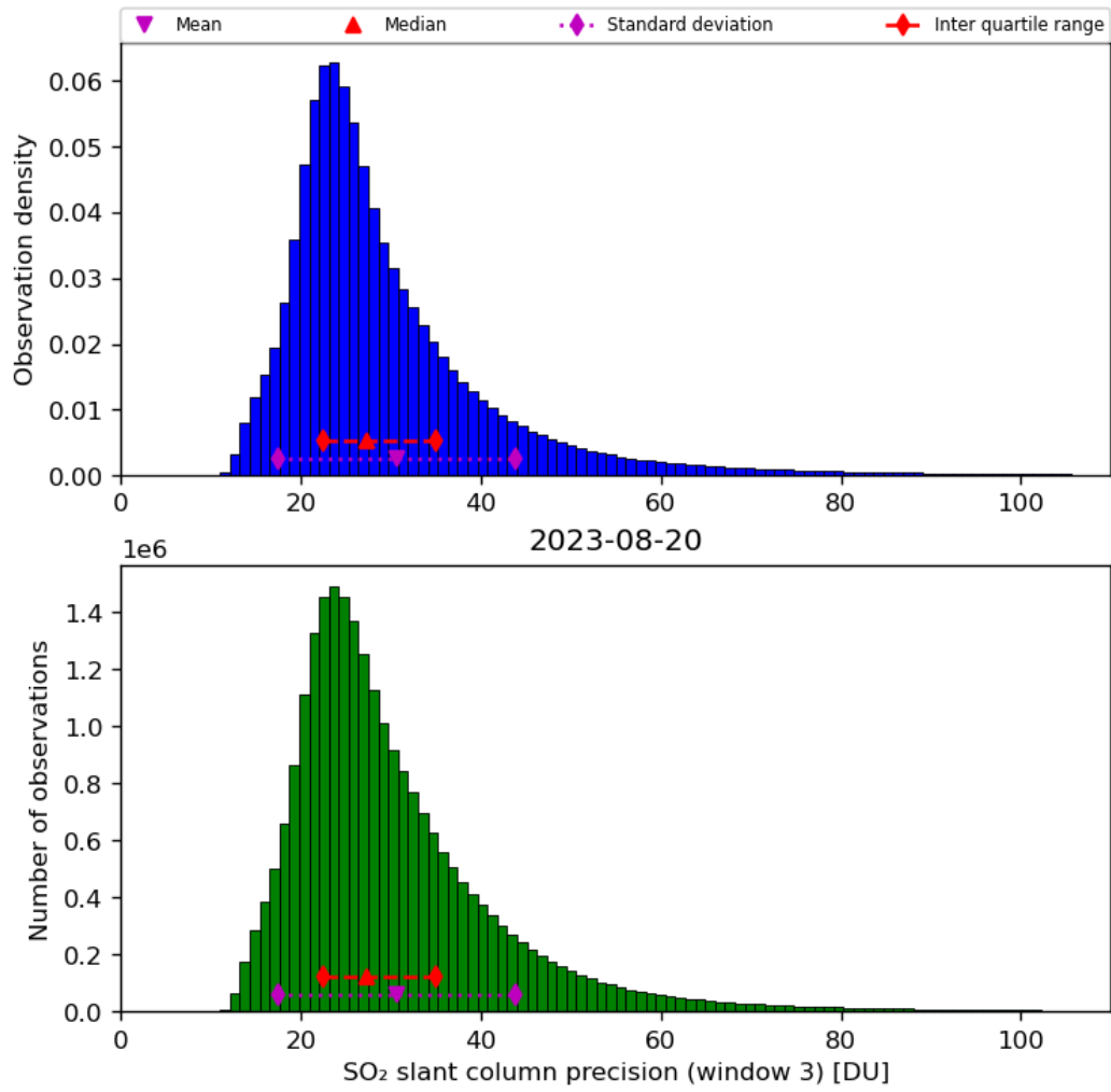
Figure 65: Histogram of “SO 2 slant column precision (window 3)” for 2023-08-20 to 2023-08-21
