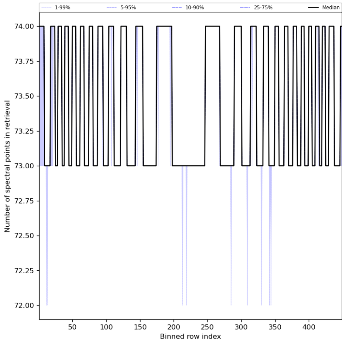
Figure 97: Along track statistics of “Number of spectral points in retrieval” for 2023-08-20 to 2023-08-21
