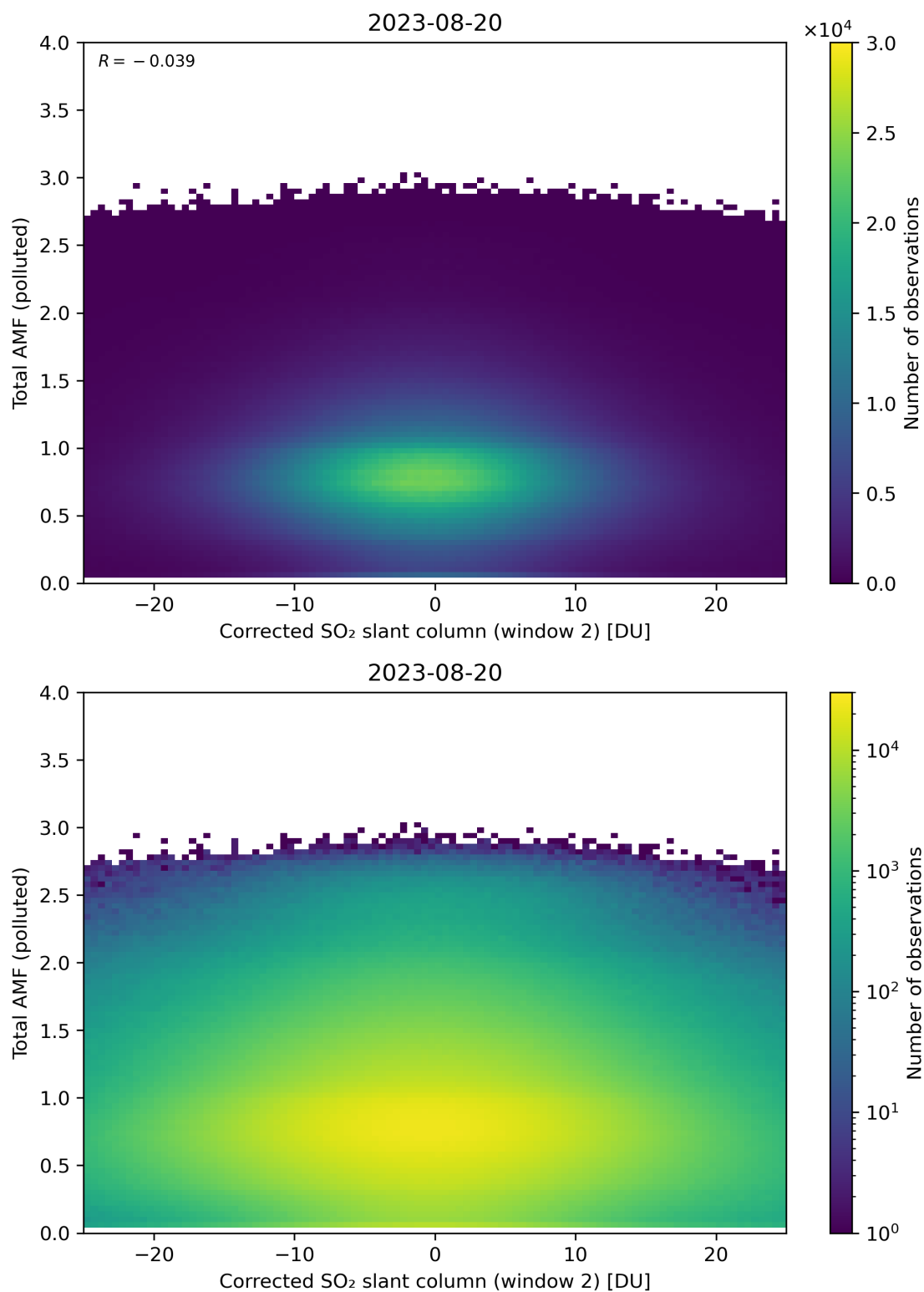
Figure 203: Scatter density plot of “Corrected SO 2 slant column (window 2)” against “Total AMF (polluted)” for 2023-08-20 to 2023-08-21.
