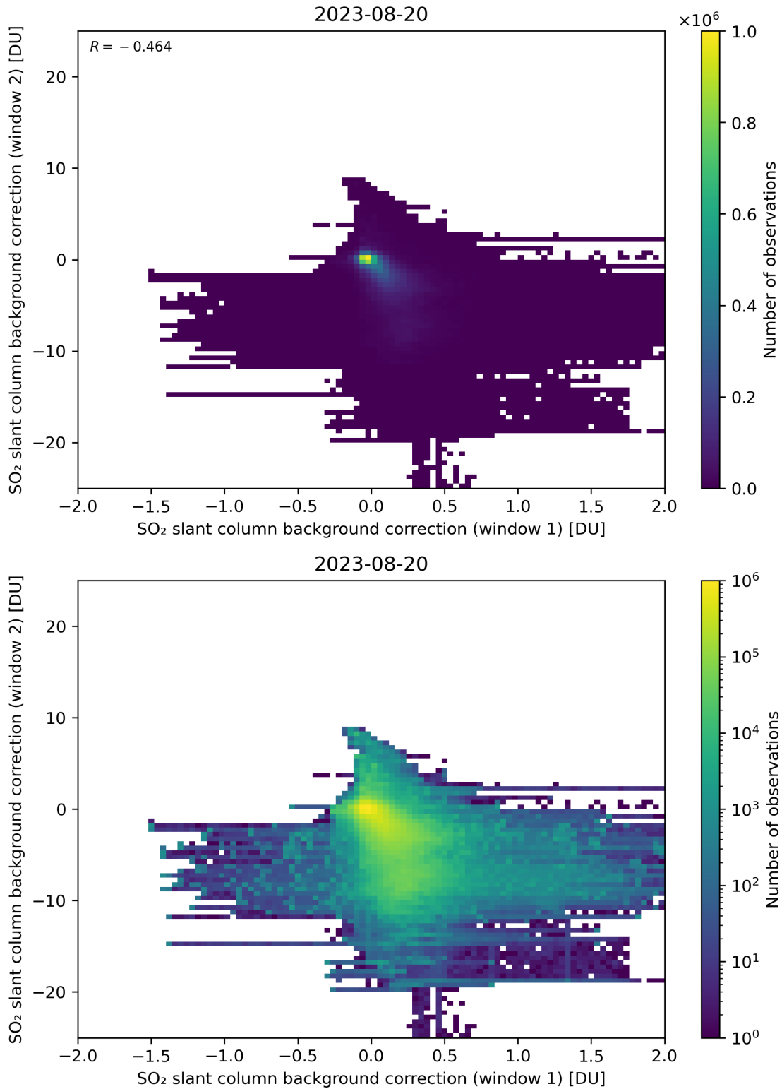
Figure 98: Scatter density plot of “SO 2 slant column background correction (window 1)” against “SO 2 slant column background correction (window 2)” for 2023-08-20 to 2023-08-21.
