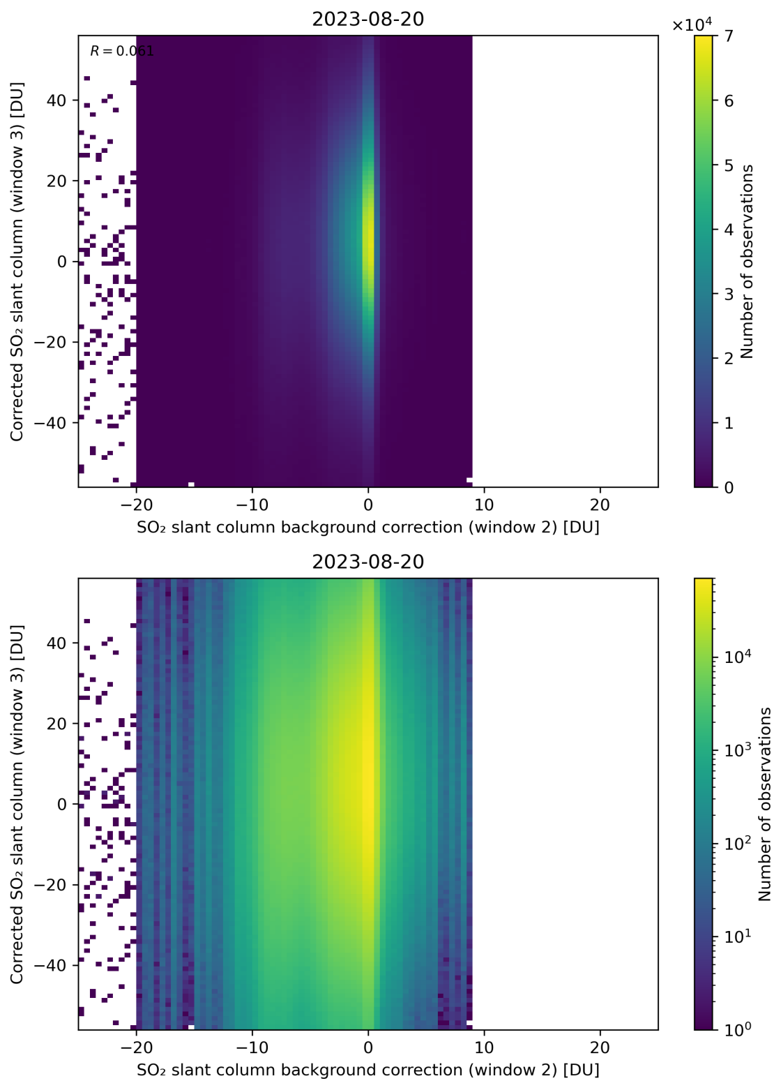
Figure 116: Scatter density plot of “SO 2 slant column background correction (window 2)” against “Corrected SO 2 slant column (window 3)” for 2023-08-20 to 2023-08-21.
