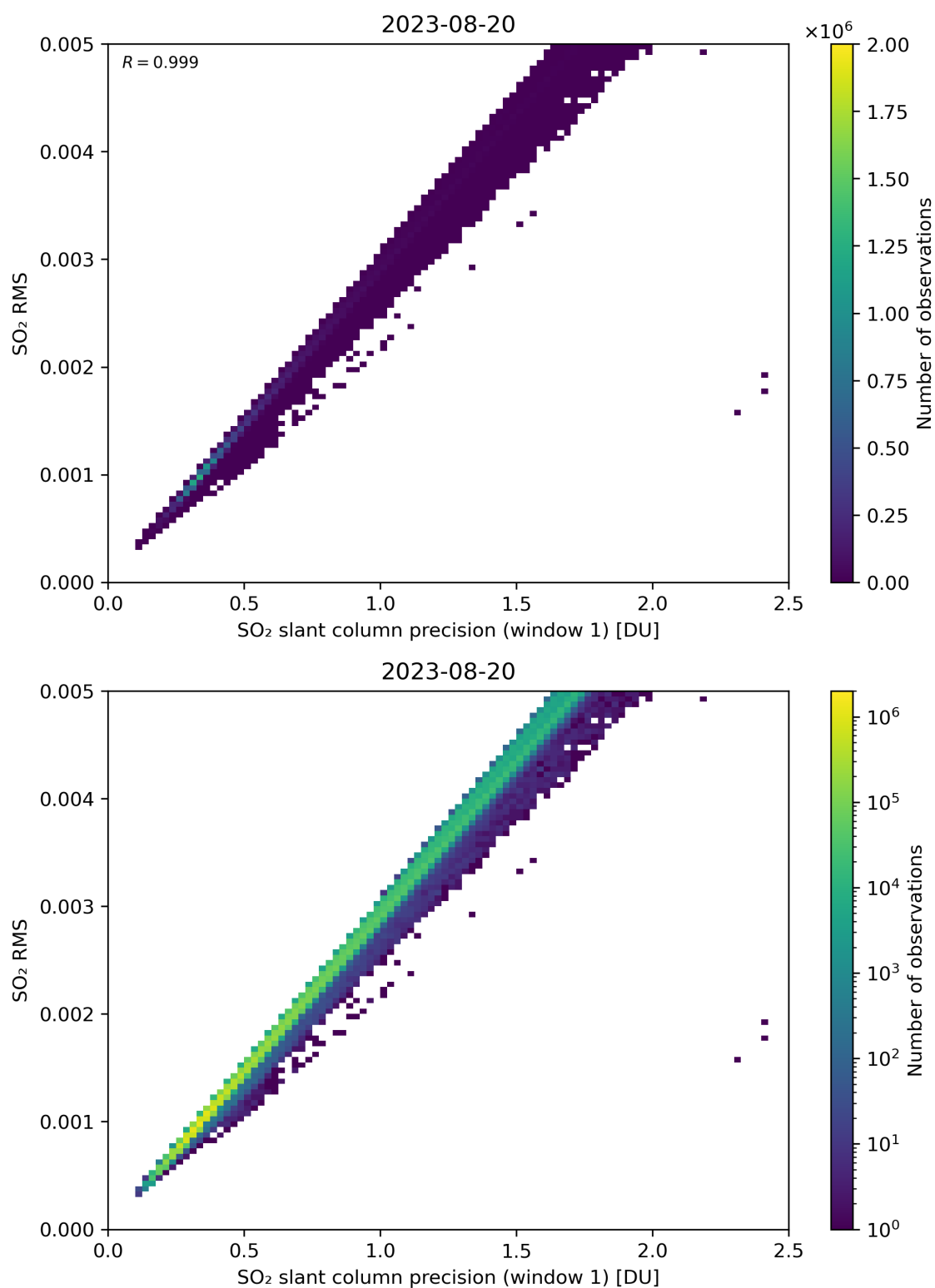
Figure 223: Scatter density plot of “SO 2 slant column precision (window 1)” against “SO 2 RMS” for 2023-08-20 to 2023-08-21.
