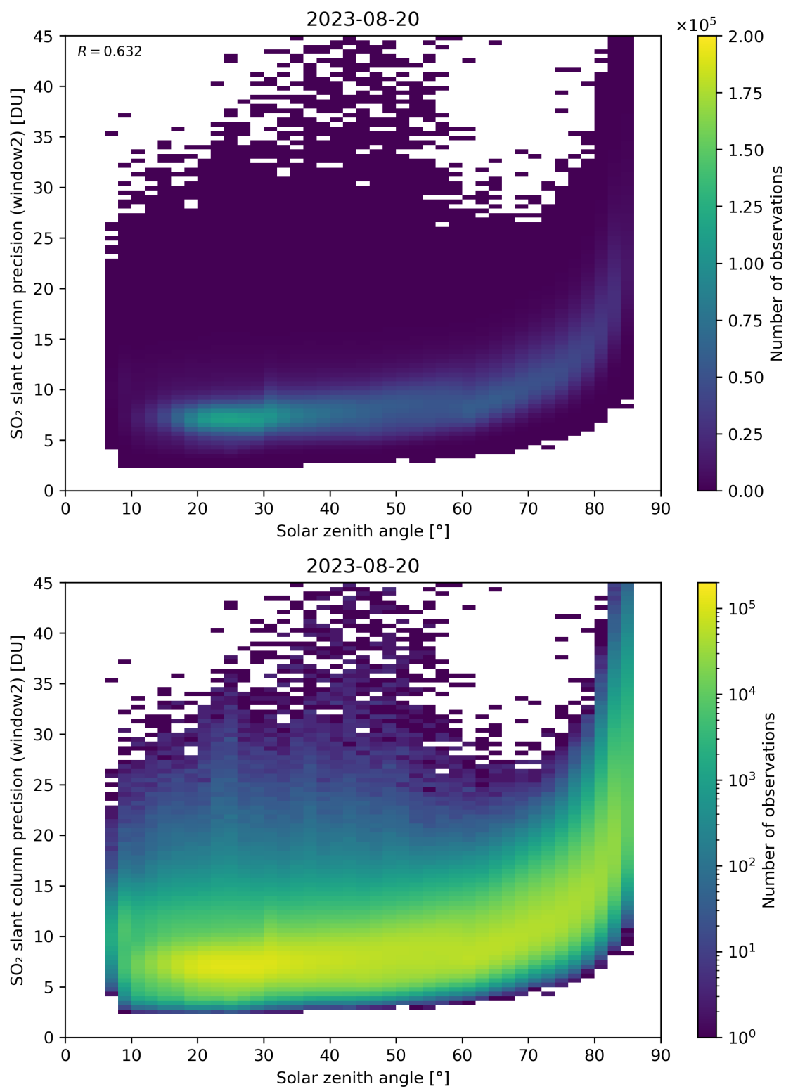
Figure 171: Scatter density plot of “Solar zenith angle” against “SO 2 slant column precision (window2)” for 2023-08-20 to 2023-08-21.
