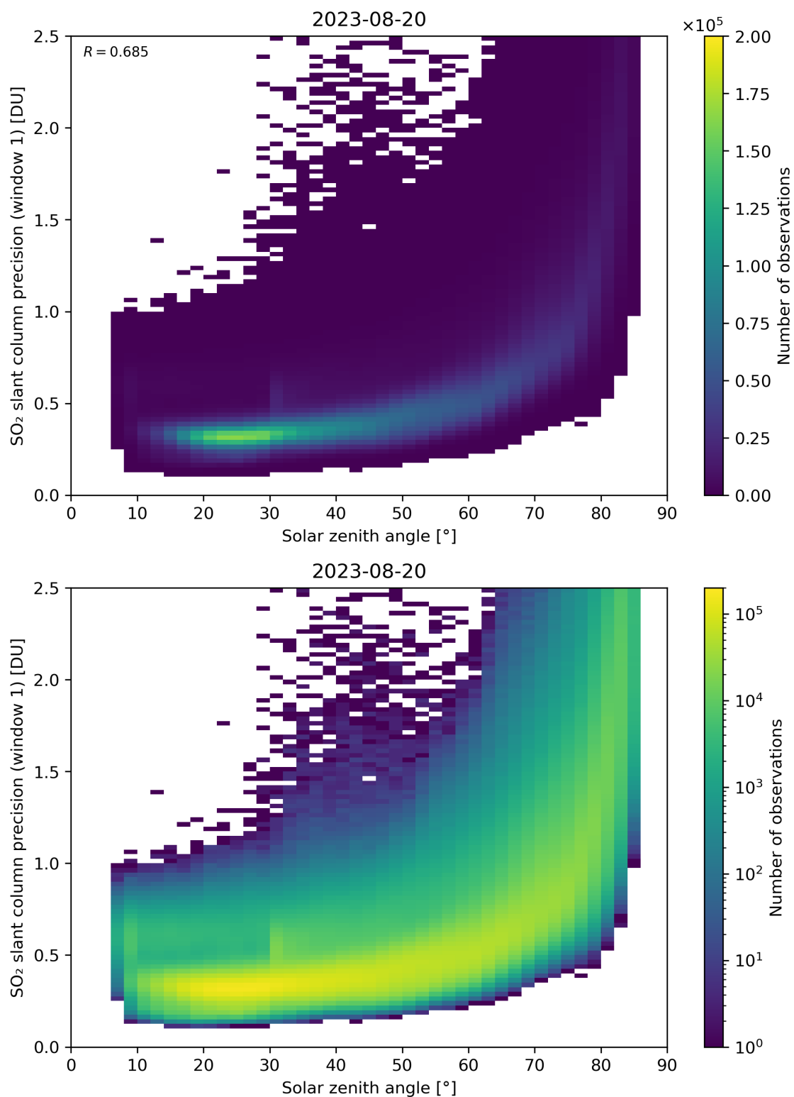
Figure 170: Scatter density plot of “Solar zenith angle” against “SO 2 slant column precision (window 1)” for 2023-08-20 to 2023-08-21.
