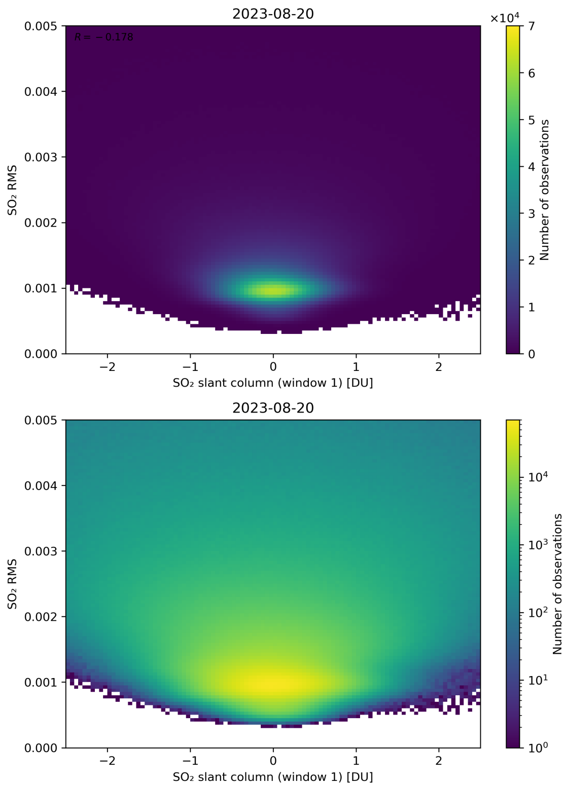
Figure 217: Scatter density plot of “SO 2 slant column (window 1)” against “SO 2 RMS” for 2023-08-20 to 2023-08-21.
