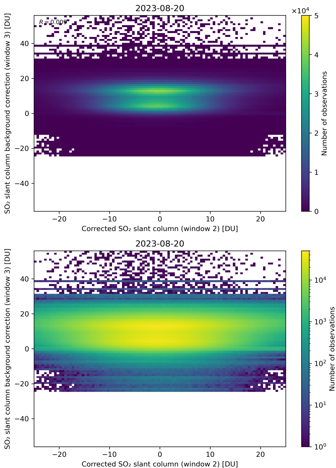
Figure 195: Scatter density plot of “Corrected SO 2 slant column (window 2)” against “SO 2 slant column background correction (window 3)” for 2023-08-20 to 2023-08-21.
