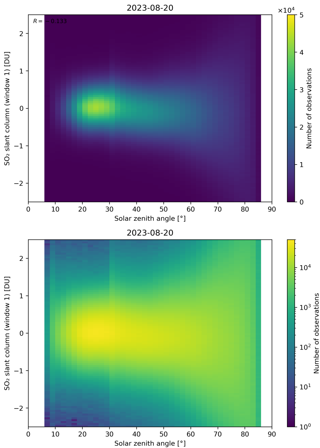
Figure 169: Scatter density plot of “Solar zenith angle” against “SO 2 slant column (window 1)” for 2023-08-20 to 2023-08-21.
