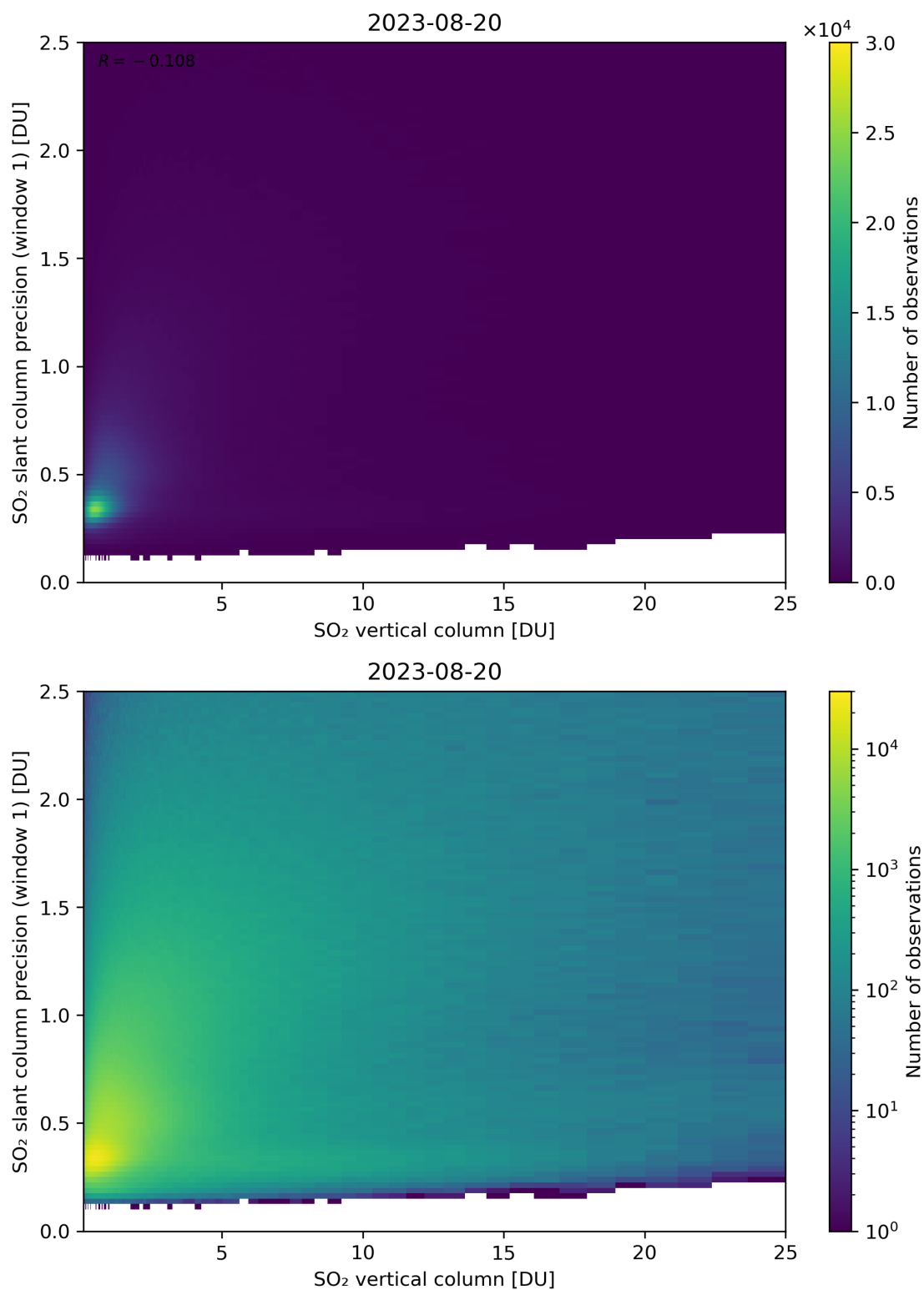
Figure 301: Scatter density plot of “SO 2 vertical column” against “SO 2 slant column precision (window 1)” for 2023-08-20 to 2023-08-21.
