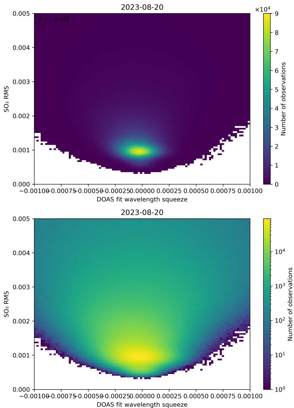
Figure 132: Scatter density plot of “DOAS fit wavelength squeeze” against “SO 2 RMS” for 2023-08-20 to 2023-08-21.
