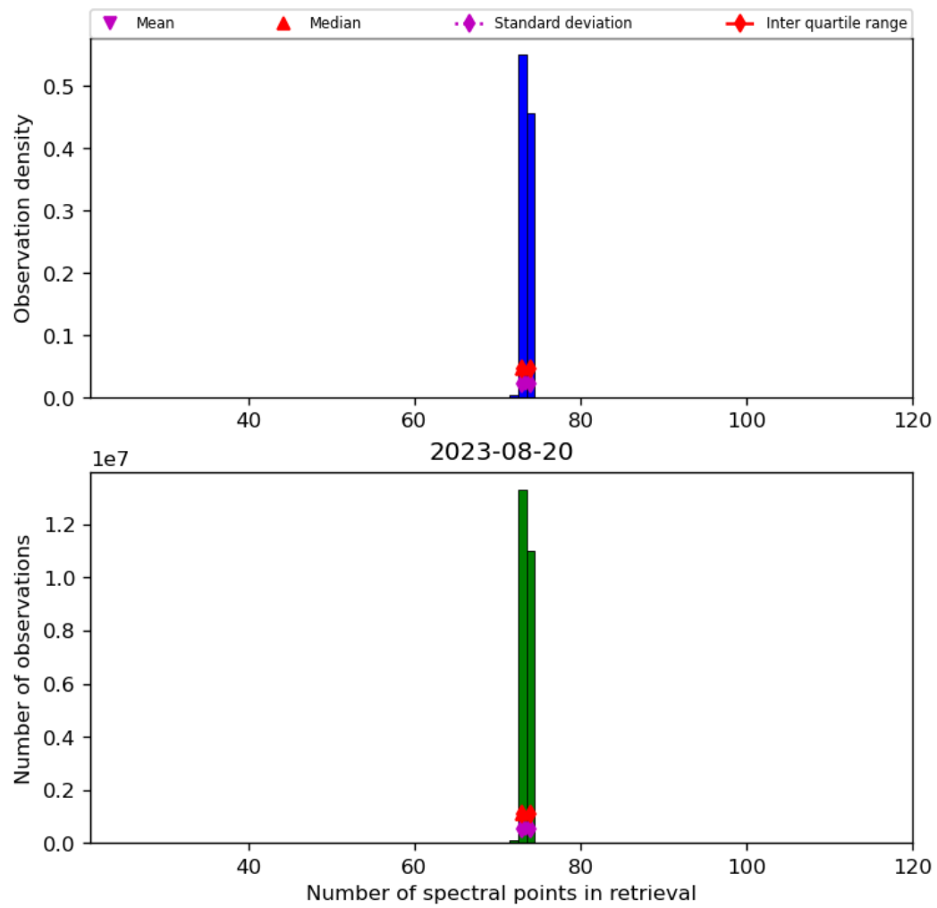
Figure 74: Histogram of “Number of spectral points in retrieval” for 2023-08-20 to 2023-08-21
