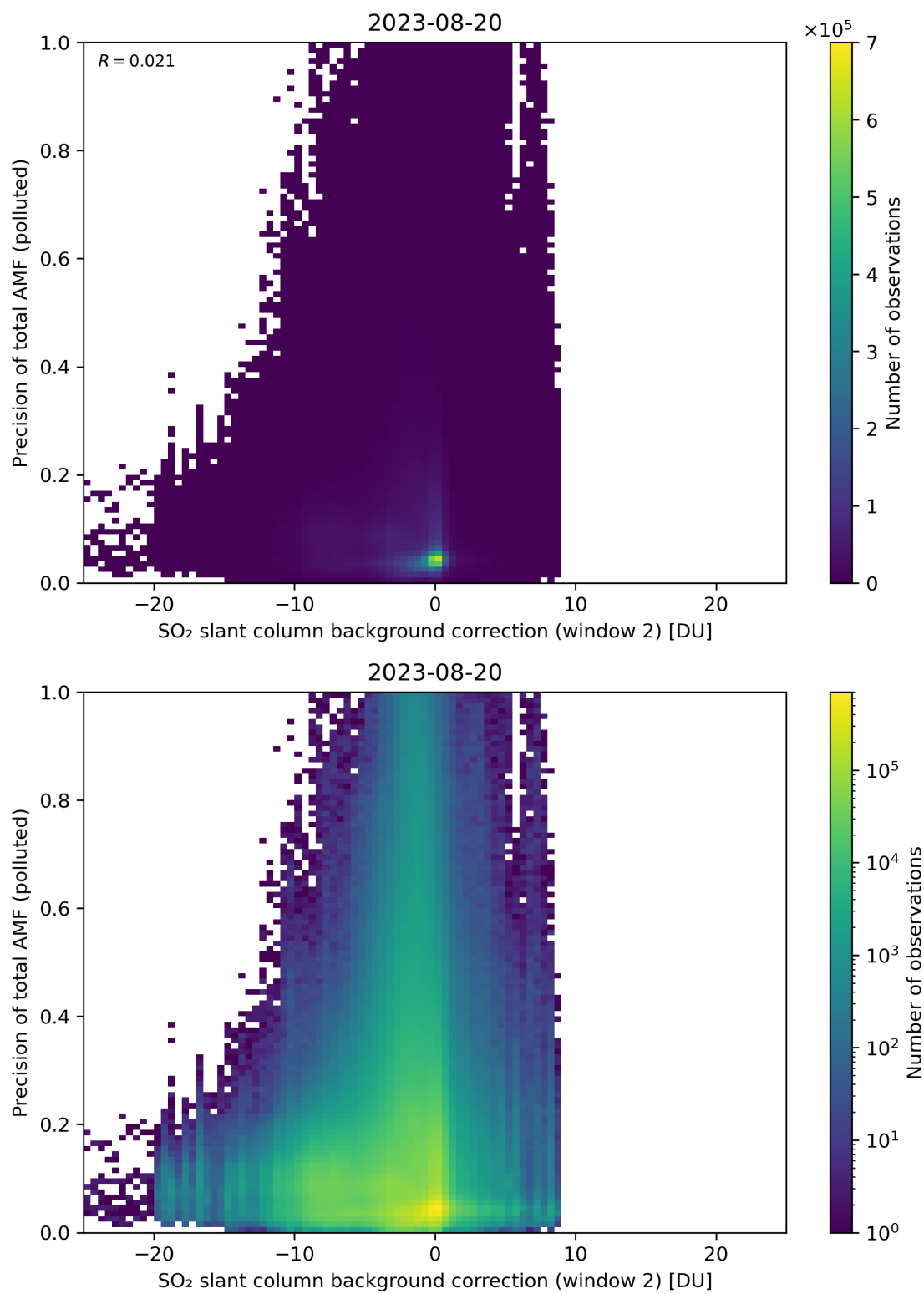
Figure 120: Scatter density plot of “SO 2 slant column background correction (window 2)” against “Precision of total AMF (polluted)” for 2023-08-20 to 2023-08-21.
