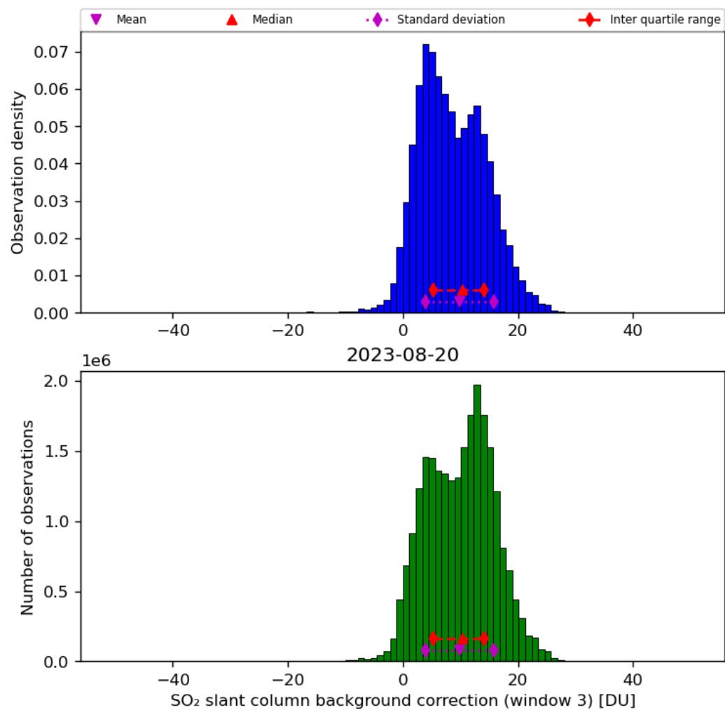
Figure 67: Histogram of “SO 2 slant column background correction (window 3)” for 2023-08-20 to 2023-08-21
