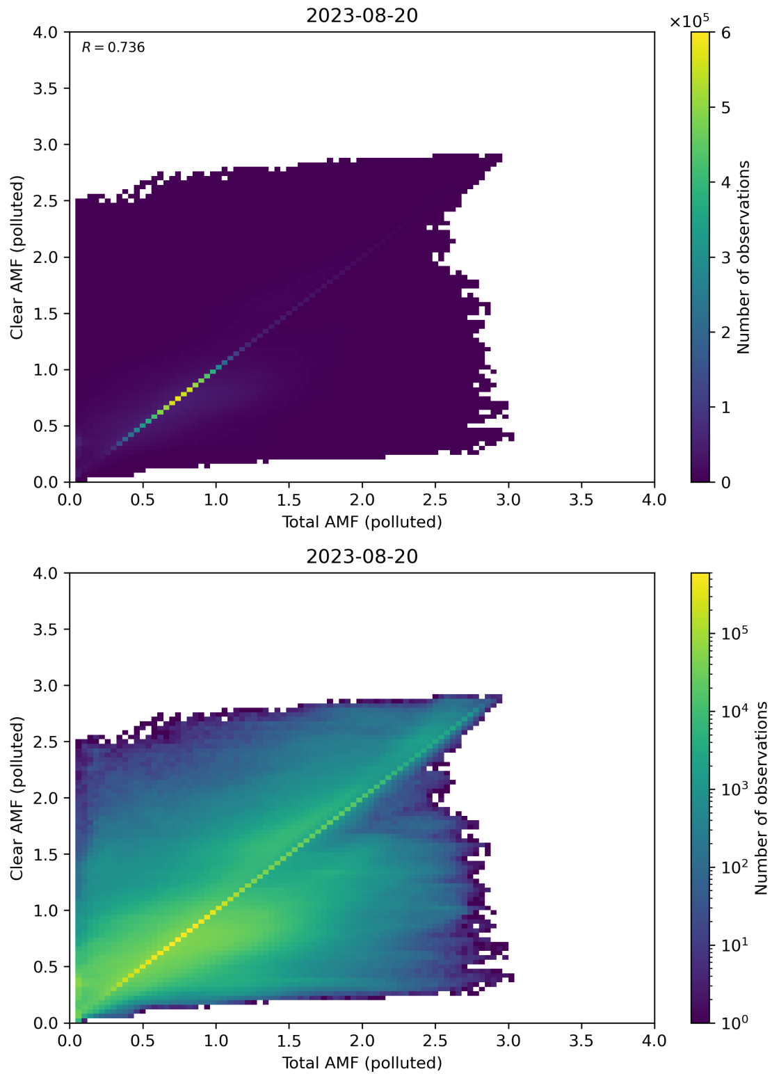
Figure 271: Scatter density plot of “Total AMF (polluted)” against “Clear AMF (polluted)” for 2023-08-20 to 2023-08-21.
