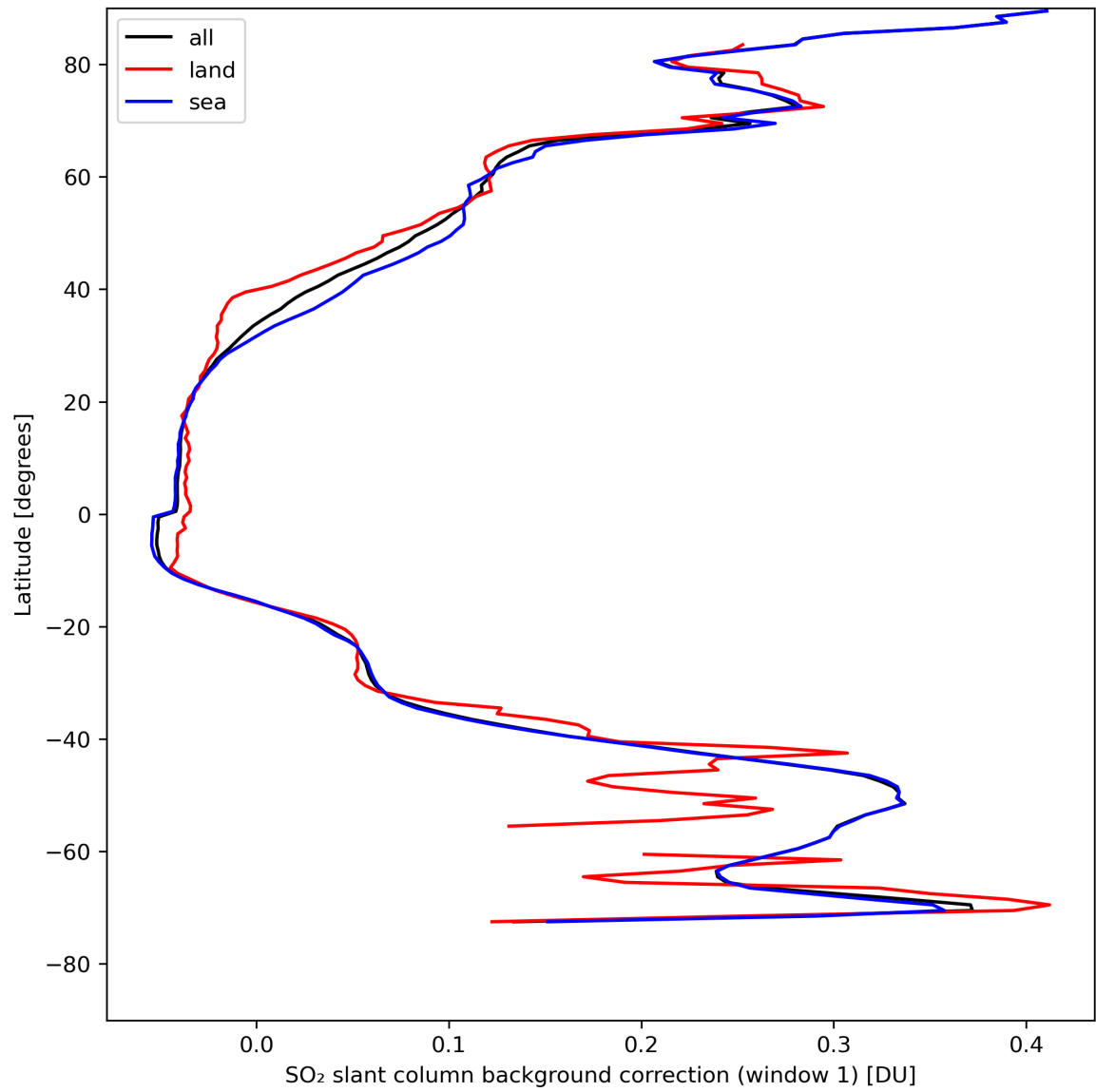
Figure 36: Zonal average of “SO 2 slant column background correction (window 1)” for 2023-08-20 to 2023-08-21.
