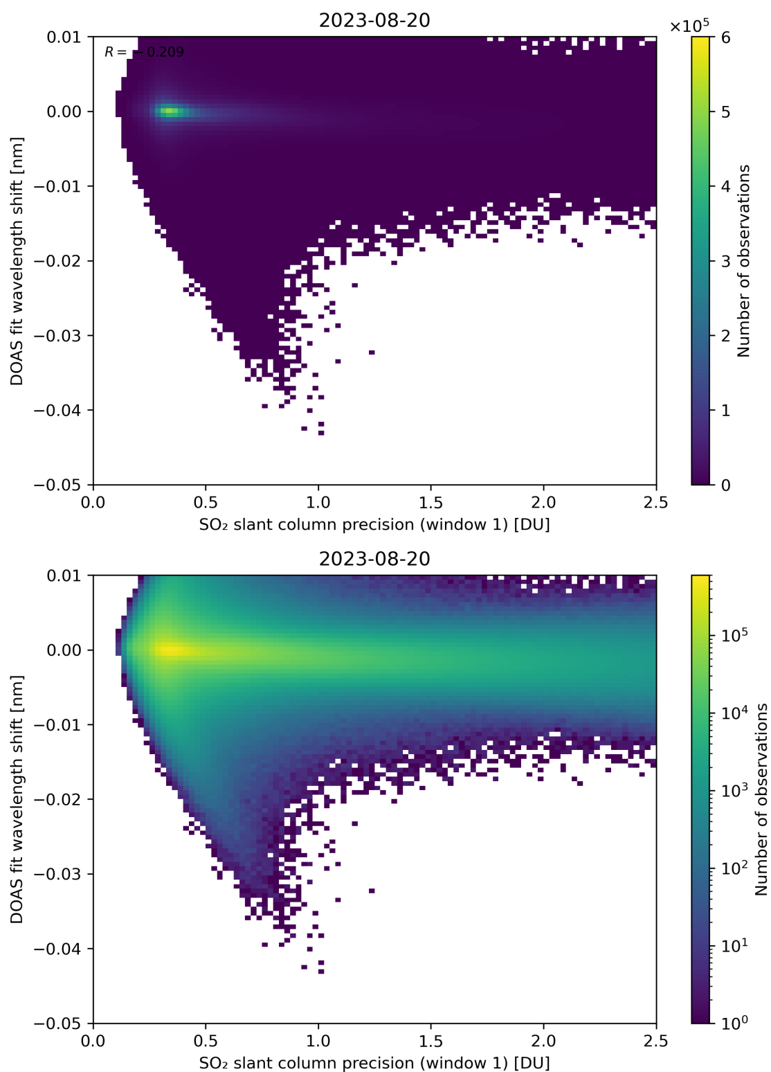
Figure 221: Scatter density plot of “SO 2 slant column precision (window 1)” against “DOAS fit wavelength shift” for 2023-08-20 to 2023-08-21.
