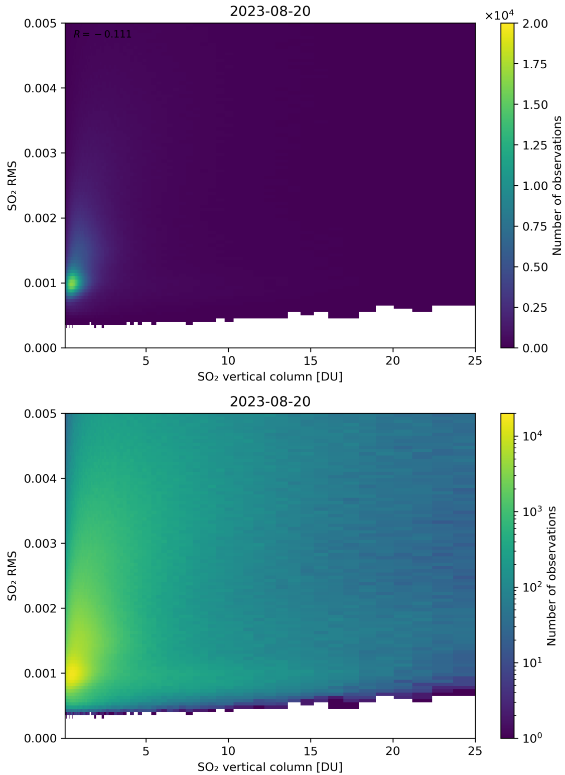
Figure 278: Scatter density plot of “SO 2 vertical column” against “SO 2 RMS” for 2023-08-20 to 2023-08-21.
