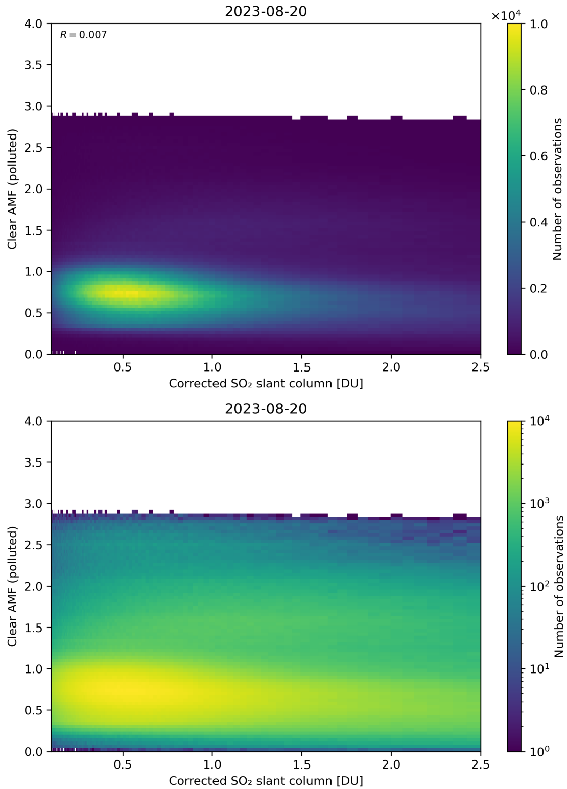
Figure 184: Scatter density plot of “Corrected SO 2 slant column” against “Clear AMF (polluted)” for 2023-08-20 to 2023-08-21.
