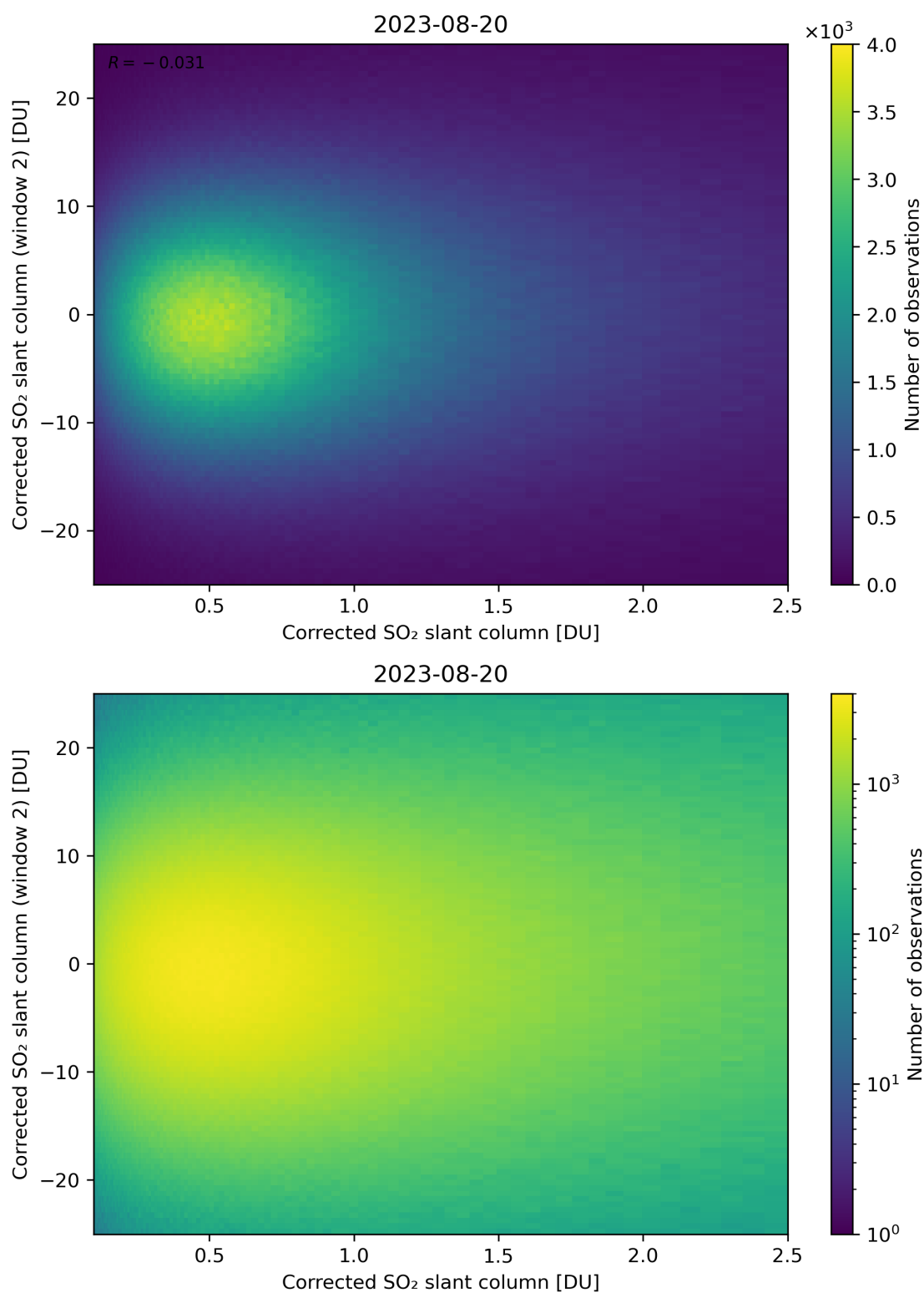
Figure 185: Scatter density plot of “Corrected SO 2 slant column” against “Corrected SO 2 slant column (window 2)” for 2023-08-20 to 2023-08-21.
