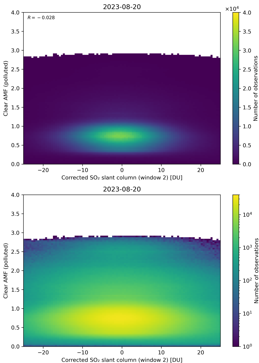
Figure 199: Scatter density plot of “Corrected SO 2 slant column (window 2)” against “Clear AMF (polluted)” for 2023-08-20 to 2023-08-21.
