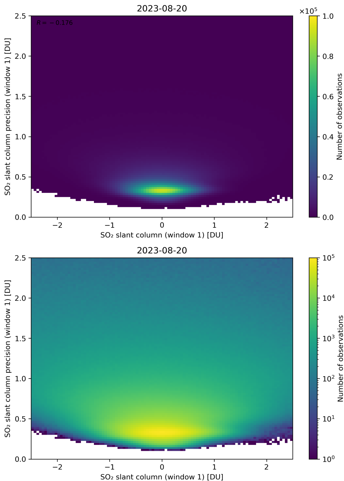
Figure 235: Scatter density plot of “SO 2 slant column (window 1)” against “SO 2 slant column precision (window 1)” for 2023-08-20 to 2023-08-21.
