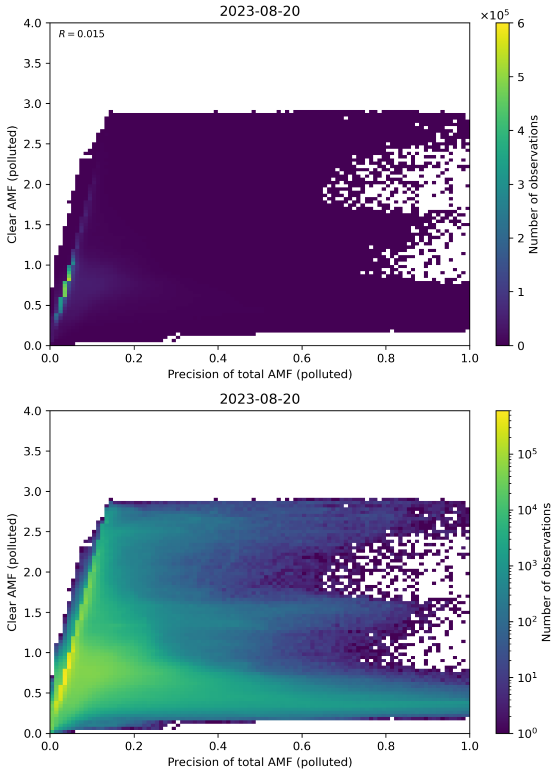
Figure 270: Scatter density plot of “Precision of total AMF (polluted)” against “Clear AMF (polluted)” for 2023-08-20 to 2023-08-21.
