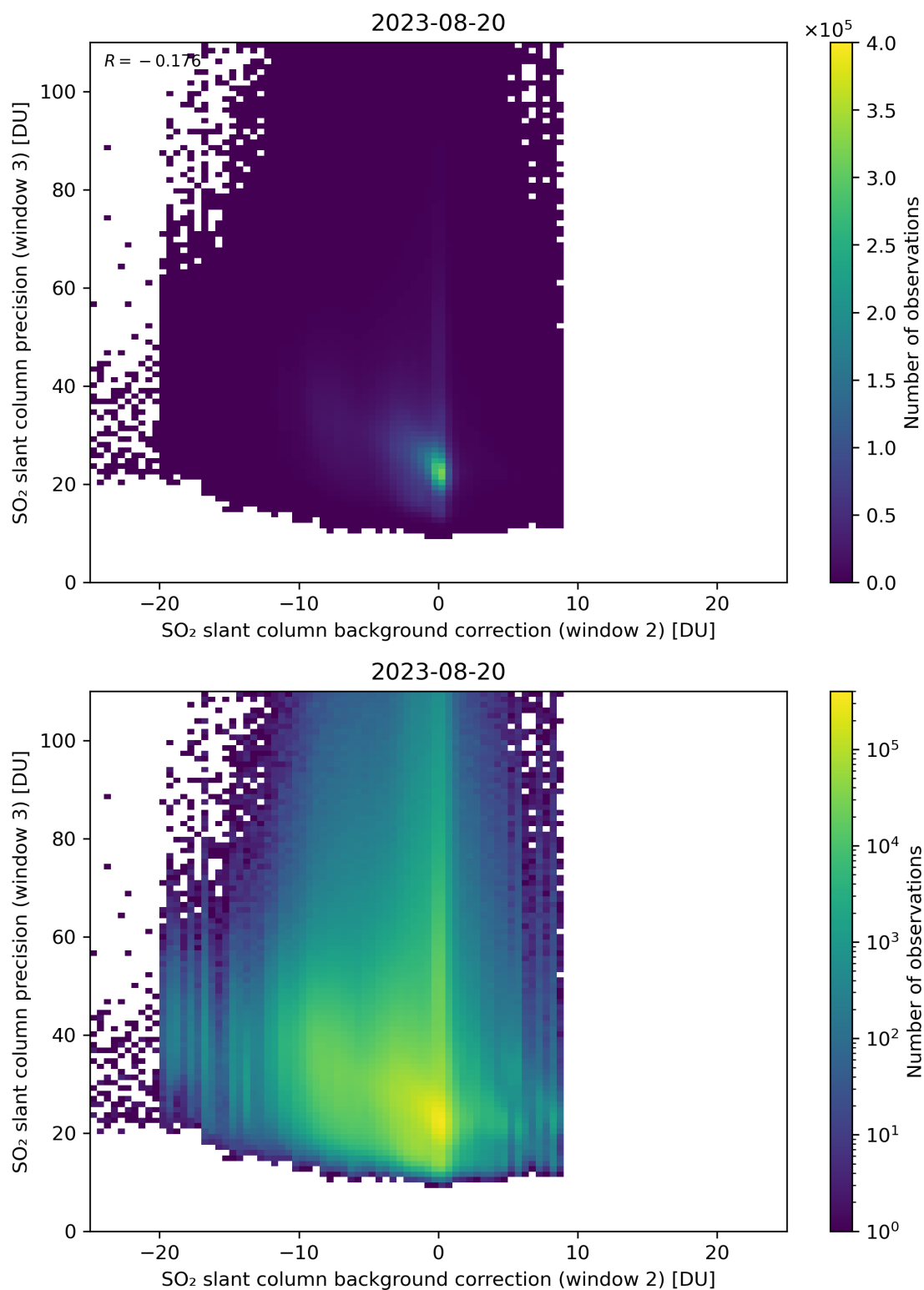
Figure 118: Scatter density plot of “SO 2 slant column background correction (window 2)” against “SO 2 slant column precision (window 3)” for 2023-08-20 to 2023-08-21.
