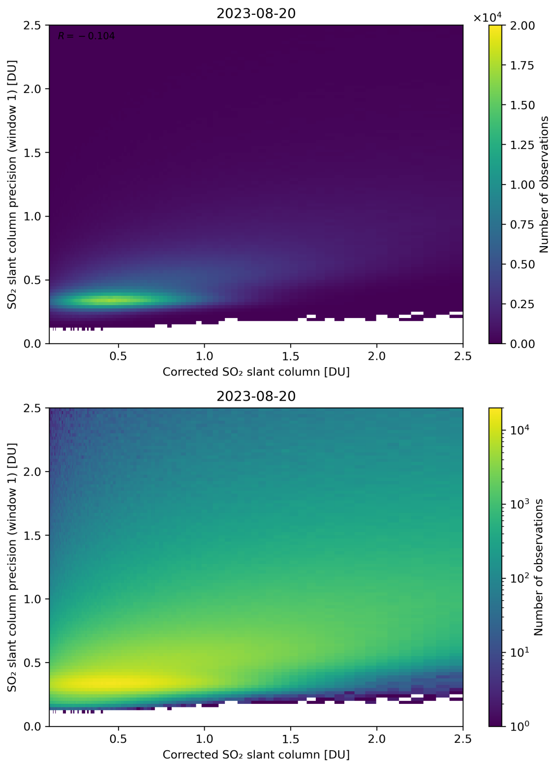
Figure 188: Scatter density plot of “Corrected SO 2 slant column” against “SO 2 slant column precision (window 1)” for 2023-08-20 to 2023-08-21.
