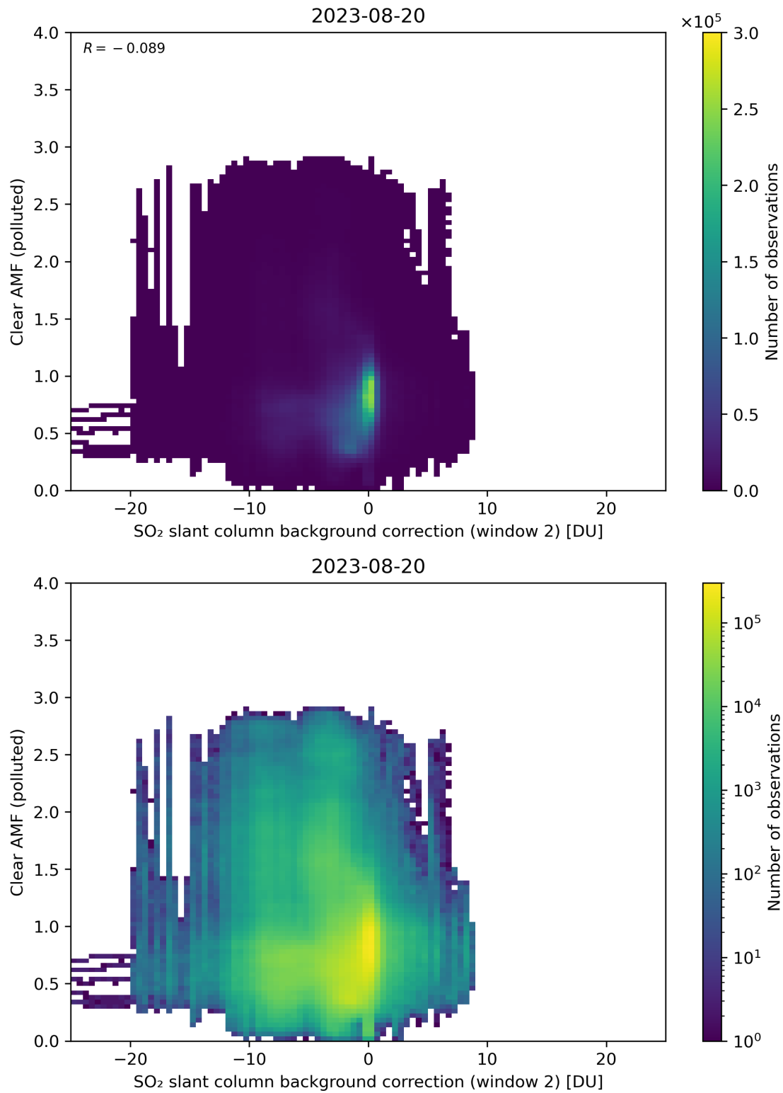
Figure 115: Scatter density plot of “SO 2 slant column background correction (window 2)” against “Clear AMF (polluted)” for 2023-08-20 to 2023-08-21.
