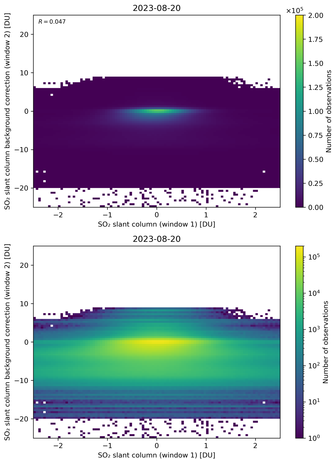
Figure 213: Scatter density plot of “SO 2 slant column (window 1)” against “SO 2 slant column background correction (window 2)” for 2023-08-20 to 2023-08-21.
