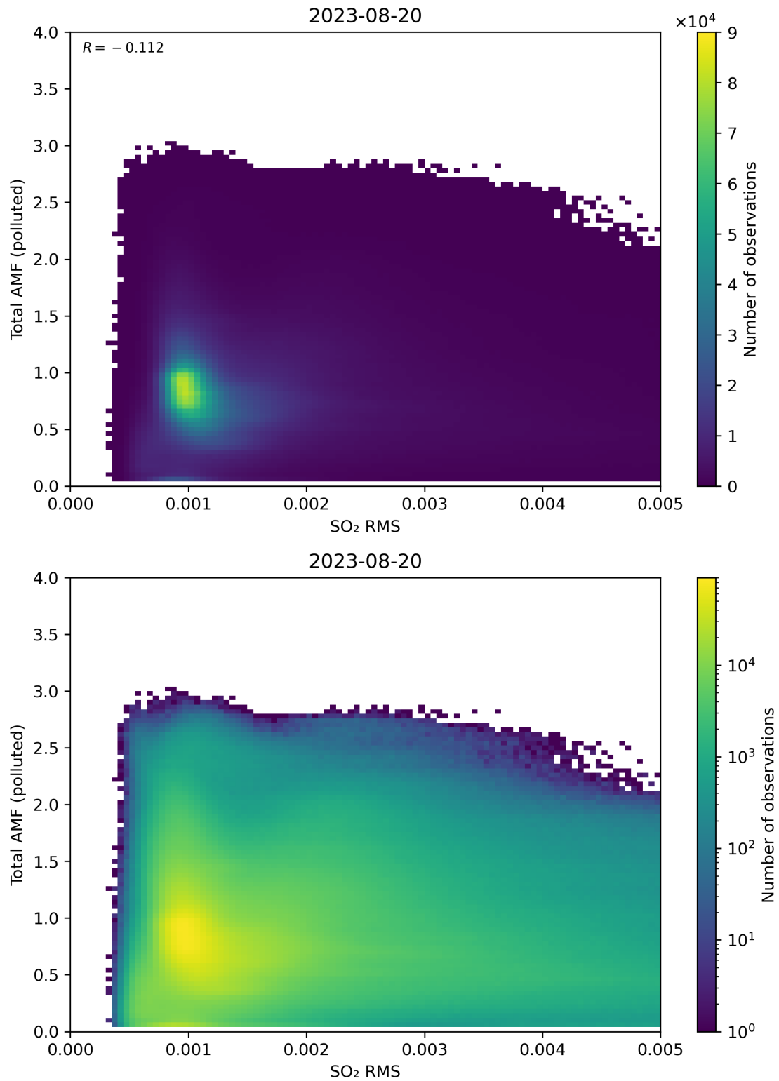
Figure 137: Scatter density plot of “SO 2 RMS” against “Total AMF (polluted)” for 2023-08-20 to 2023-08-21.
