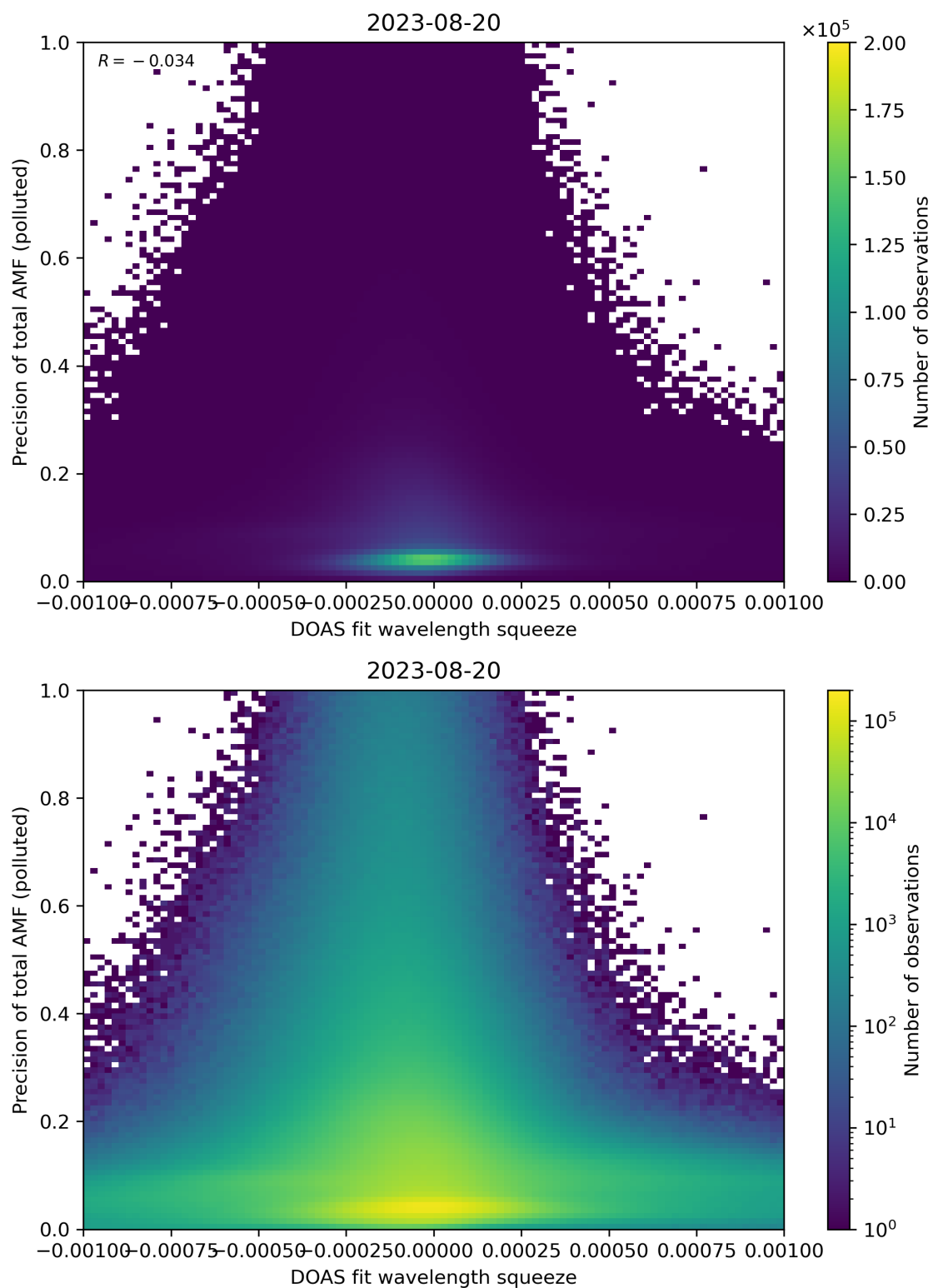
Figure 135: Scatter density plot of “DOAS fit wavelength squeeze” against “Precision of total AMF (polluted)” for 2023-08-20 to 2023-08-21.
