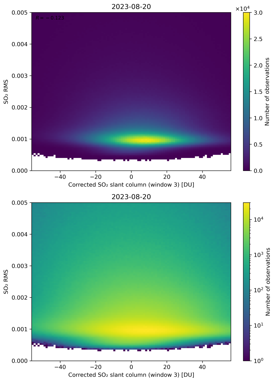
Figure 208: Scatter density plot of “Corrected SO 2 slant column (window 3)” against “SO 2 RMS” for 2023-08-20 to 2023-08-21.
