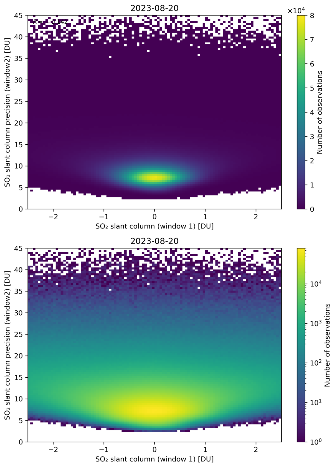
Figure 236: Scatter density plot of “SO 2 slant column (window 1)” against “SO 2 slant column precision (window2)” for 2023-08-20 to 2023-08-21.
