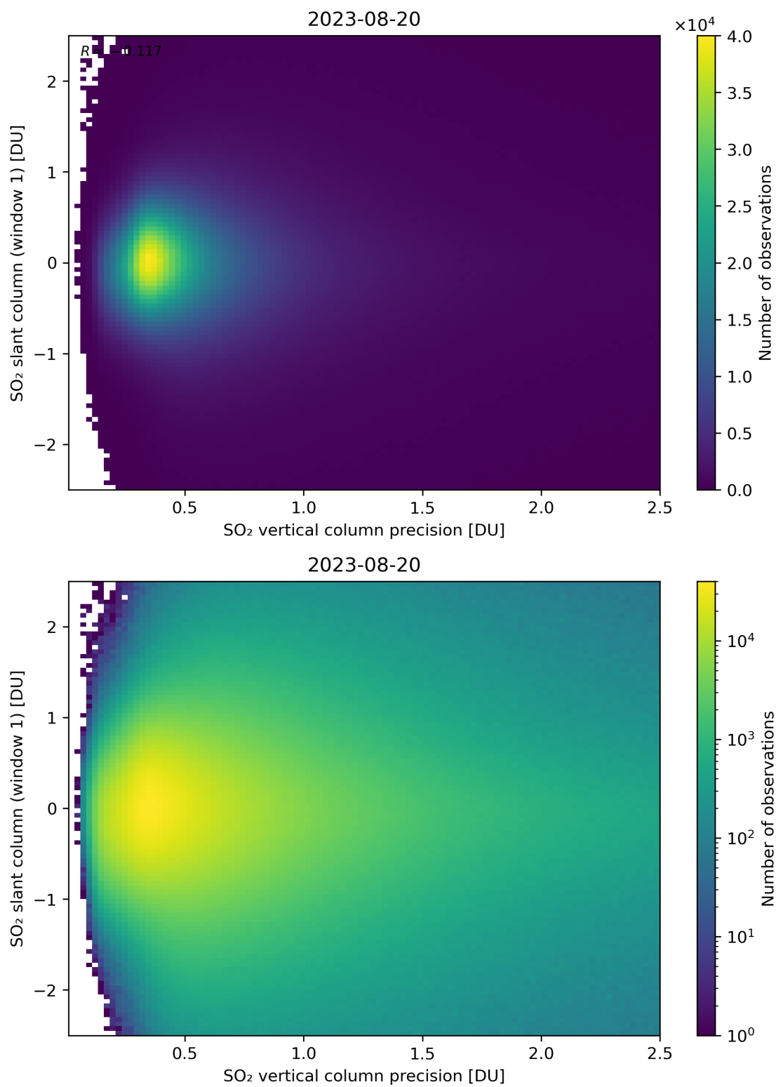
Figure 289: Scatter density plot of “SO 2 vertical column precision” against “SO 2 slant column (window 1)” for 2023-08-20 to 2023-08-21.
