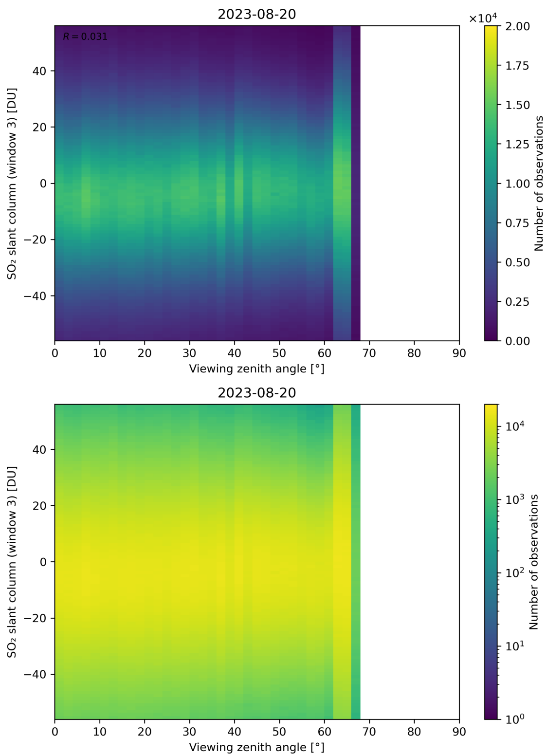
Figure 323: Scatter density plot of “Viewing zenith angle” against “SO 2 slant column (window 3)” for 2023-08-20 to 2023-08-21.
