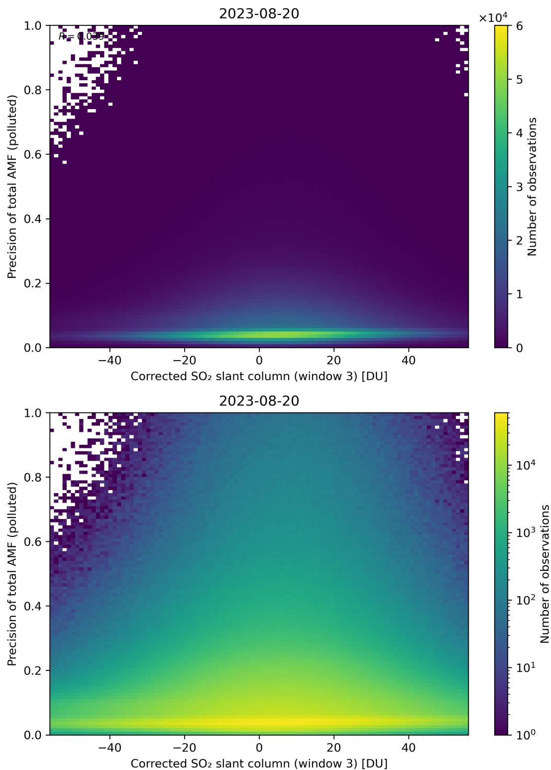
Figure 211: Scatter density plot of “Corrected SO 2 slant column (window 3)” against “Precision of total AMF (polluted)” for 2023-08-20 to 2023-08-21.
