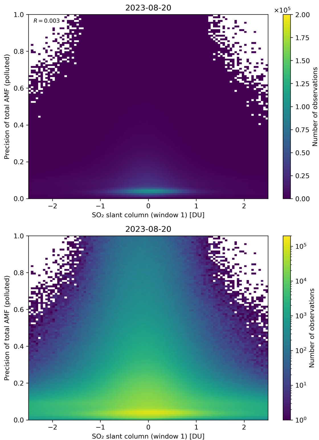
Figure 240: Scatter density plot of “SO 2 slant column (window 1)” against “Precision of total AMF (polluted)” for 2023-08-20 to 2023-08-21.
