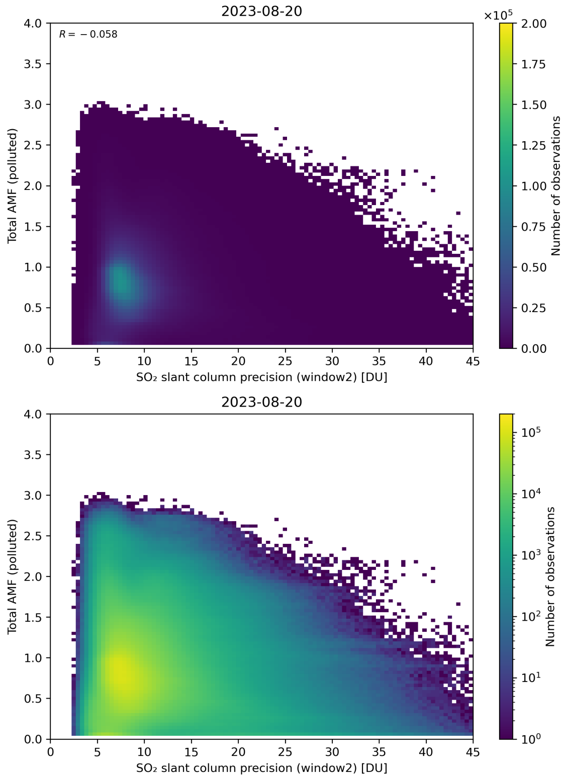
Figure 251: Scatter density plot of “SO 2 slant column precision (window2)” against “Total AMF (polluted)” for 2023-08-20 to 2023-08-21.
