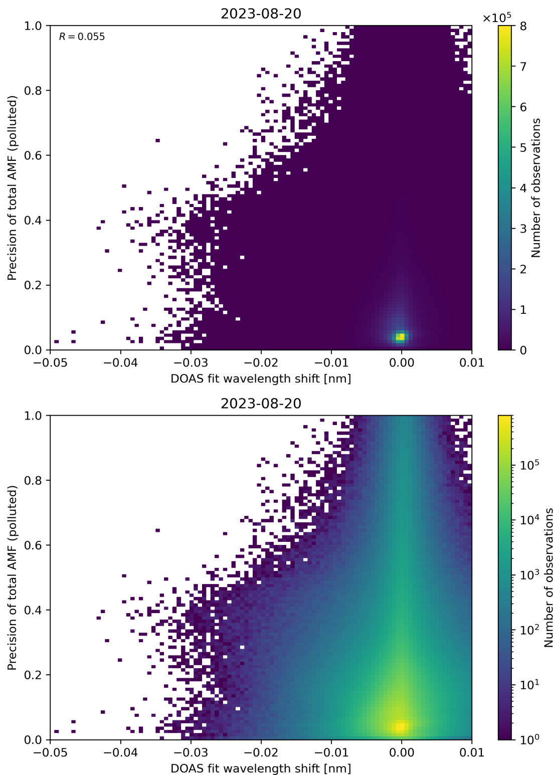
Figure 131: Scatter density plot of “DOAS fit wavelength shift” against “Precision of total AMF (polluted)” for 2023-08-20 to 2023-08-21.
