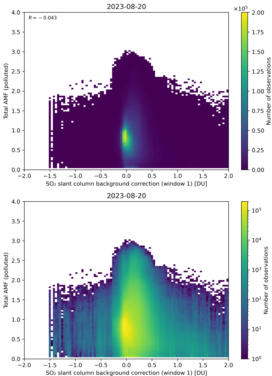
Figure 109: Scatter density plot of “SO 2 slant column background correction (window 1)” against “Total AMF (polluted)” for 2023-08-20 to 2023-08-21.
