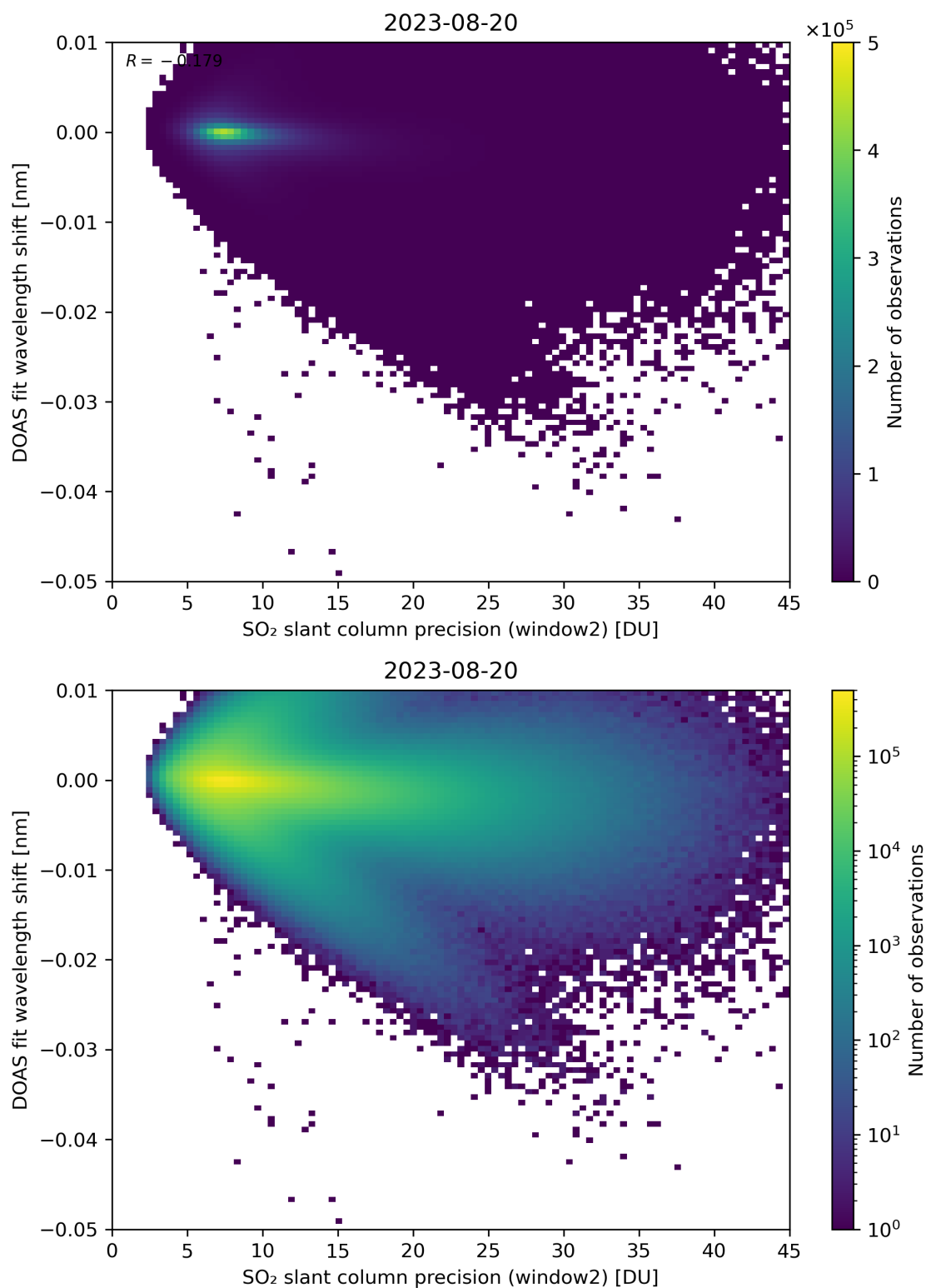
Figure 243: Scatter density plot of “SO 2 slant column precision (window2)” against “DOAS fit wavelength shift” for 2023-08-20 to 2023-08-21.
