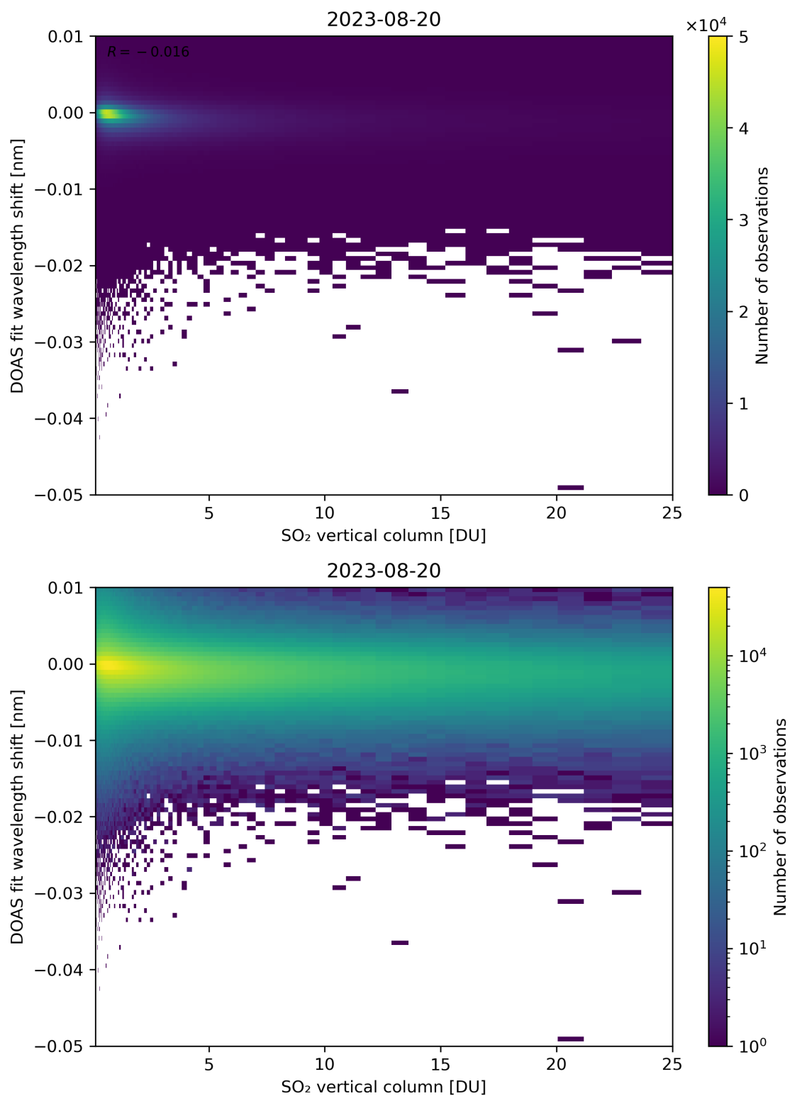
Figure 276: Scatter density plot of “SO 2 vertical column” against “DOAS fit wavelength shift” for 2023-08-20 to 2023-08-21.
