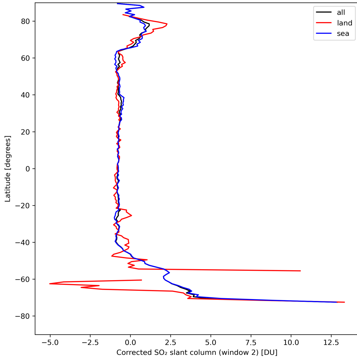
Figure 39: Zonal average of “Corrected SO 2 slant column (window 2)” for 2023-08-20 to 2023-08-21.
