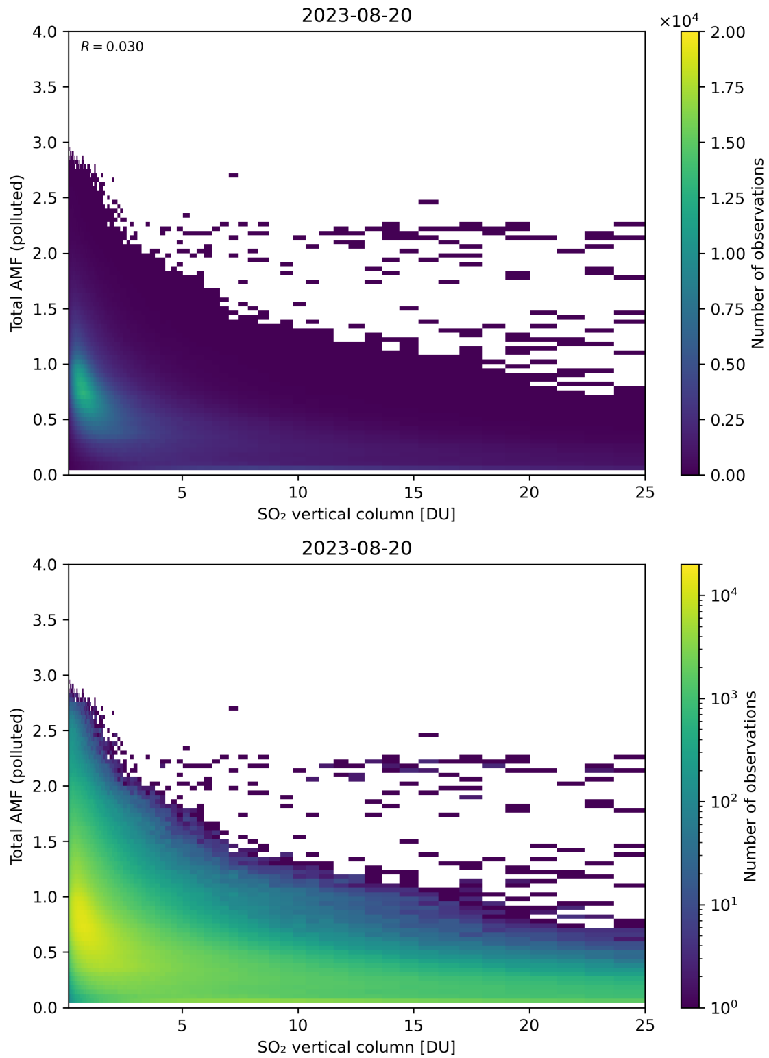
Figure 305: Scatter density plot of “SO 2 vertical column” against “Total AMF (polluted)” for 2023-08-20 to 2023-08-21.
