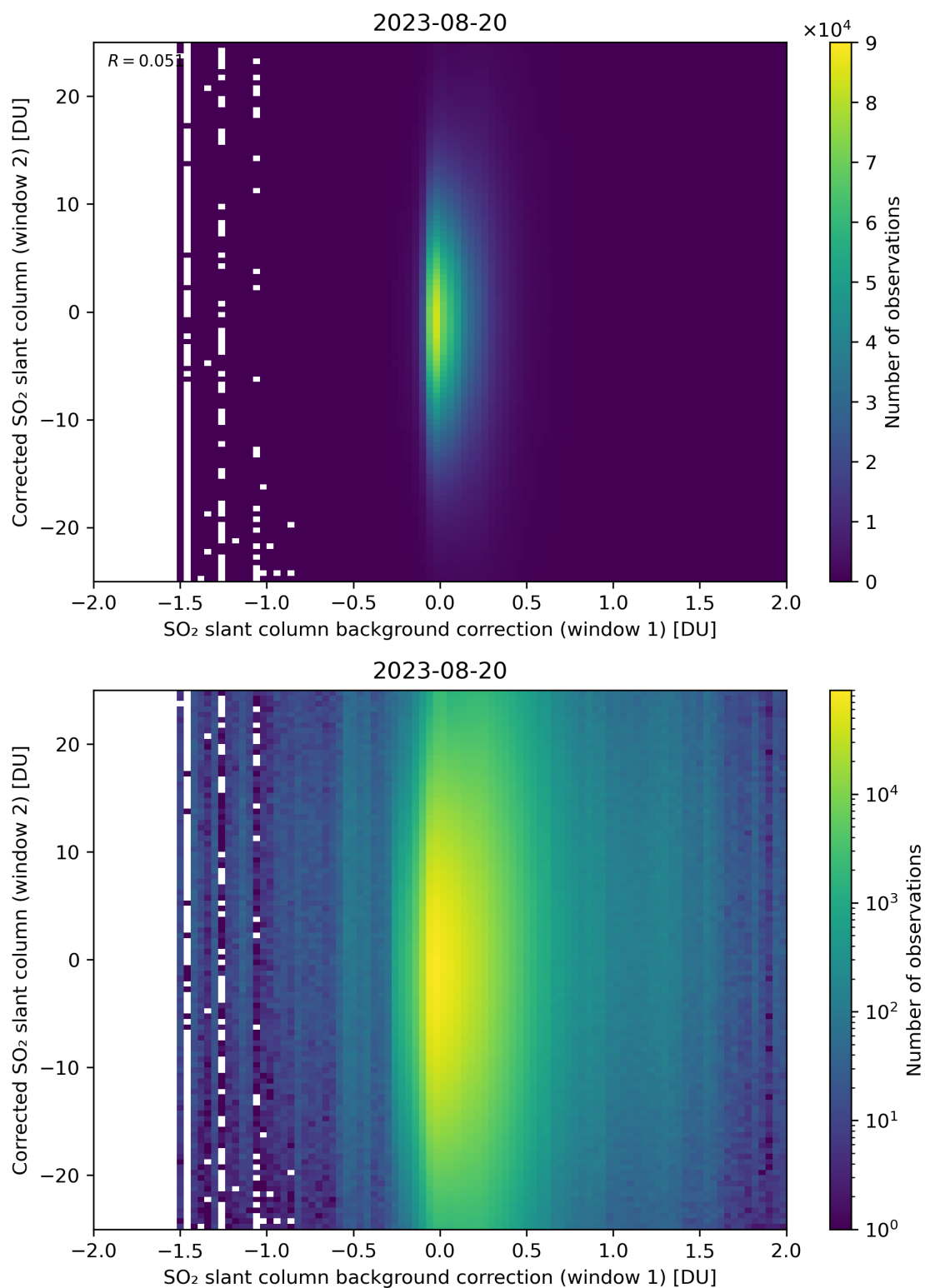
Figure 104: Scatter density plot of “SO 2 slant column background correction (window 1)” against “Corrected SO 2 slant column (window 2)” for 2023-08-20 to 2023-08-21.
