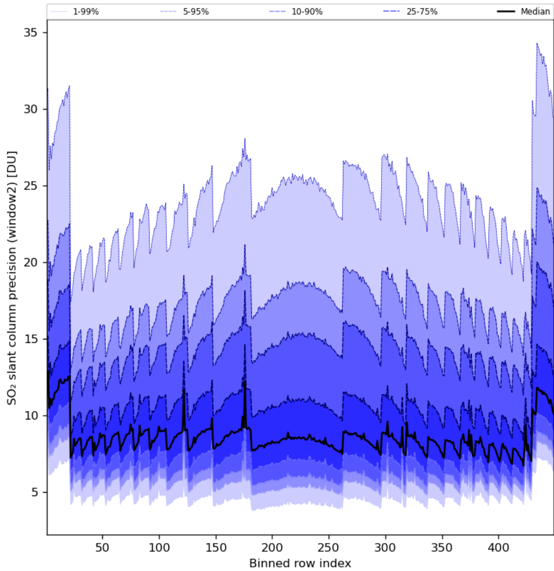
Figure 84: Along track statistics of “SO 2 slant column precision (window2)” for 2023-08-20 to 2023-08-21
