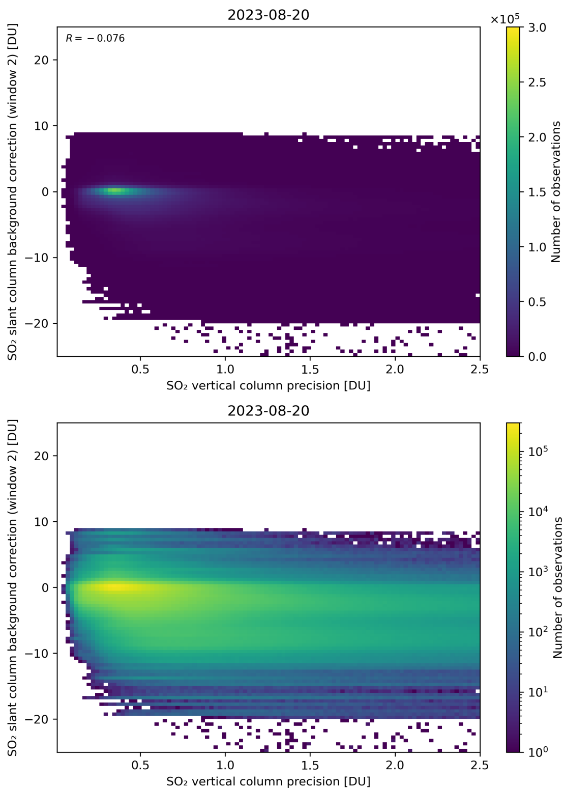
Figure 280: Scatter density plot of “SO 2 vertical column precision” against “SO 2 slant column background correction (window 2)” for 2023-08-20 to 2023-08-21.
