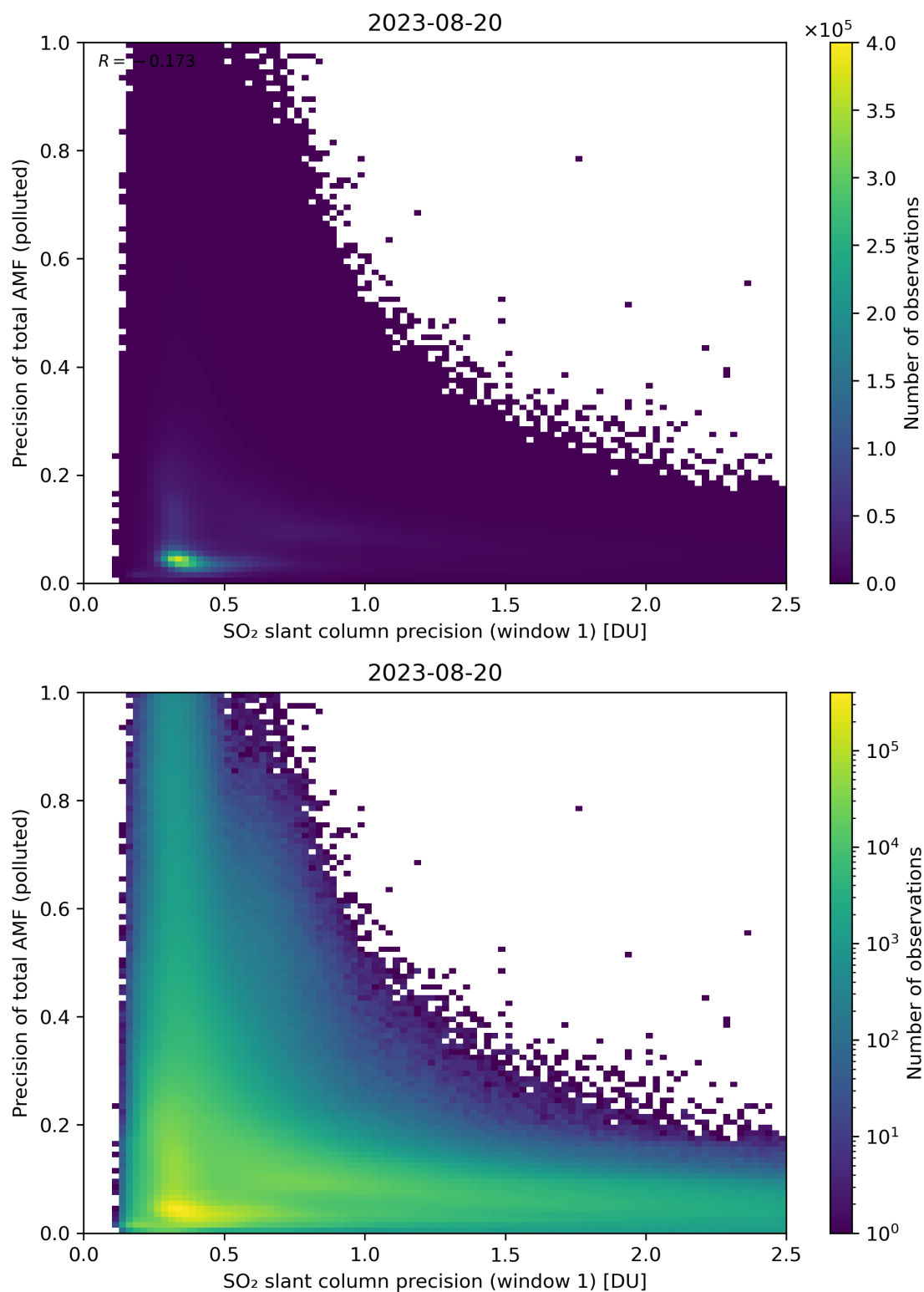
Figure 231: Scatter density plot of “SO 2 slant column precision (window 1)” against “Precision of total AMF (polluted)” for 2023-08-20 to 2023-08-21.
