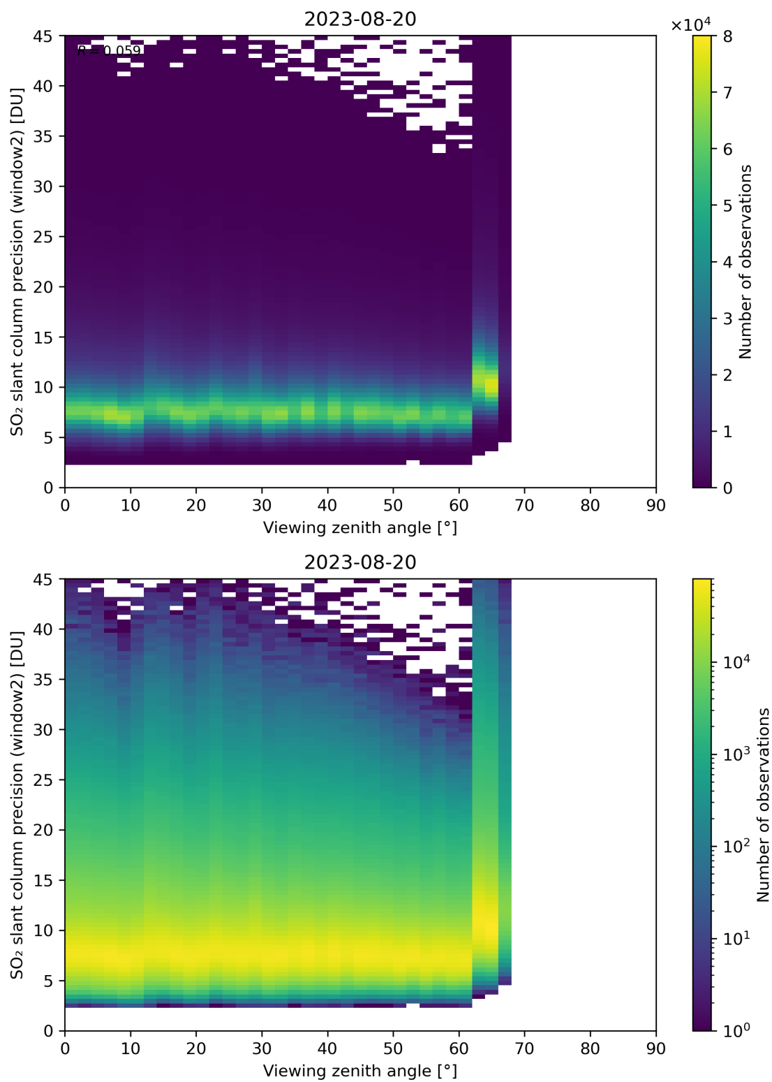
Figure 322: Scatter density plot of “Viewing zenith angle” against “SO 2 slant column precision (window2)” for 2023-08-20 to 2023-08-21.
