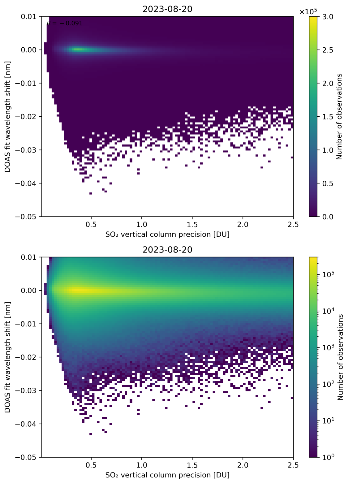
Figure 282: Scatter density plot of “SO 2 vertical column precision” against “DOAS fit wavelength shift” for 2023-08-20 to 2023-08-21.
