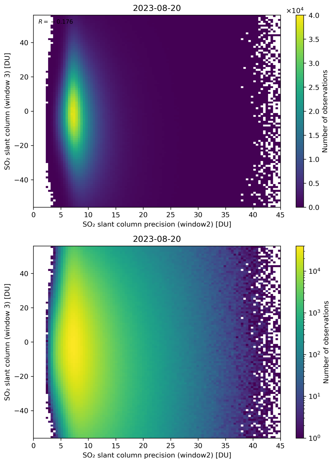
Figure 249: Scatter density plot of “SO 2 slant column precision (window2)” against “SO 2 slant column (window 3)” for 2023-08-20 to 2023-08-21.
