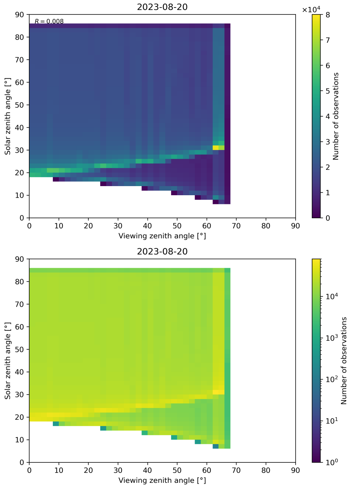
Figure 315: Scatter density plot of “Viewing zenith angle” against “Solar zenith angle” for 2023-08-20 to 2023-08-21.
