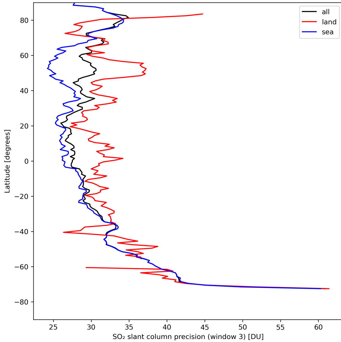
Figure 42: Zonal average of “SO 2 slant column precision (window 3)” for 2023-08-20 to 2023-08-21.
