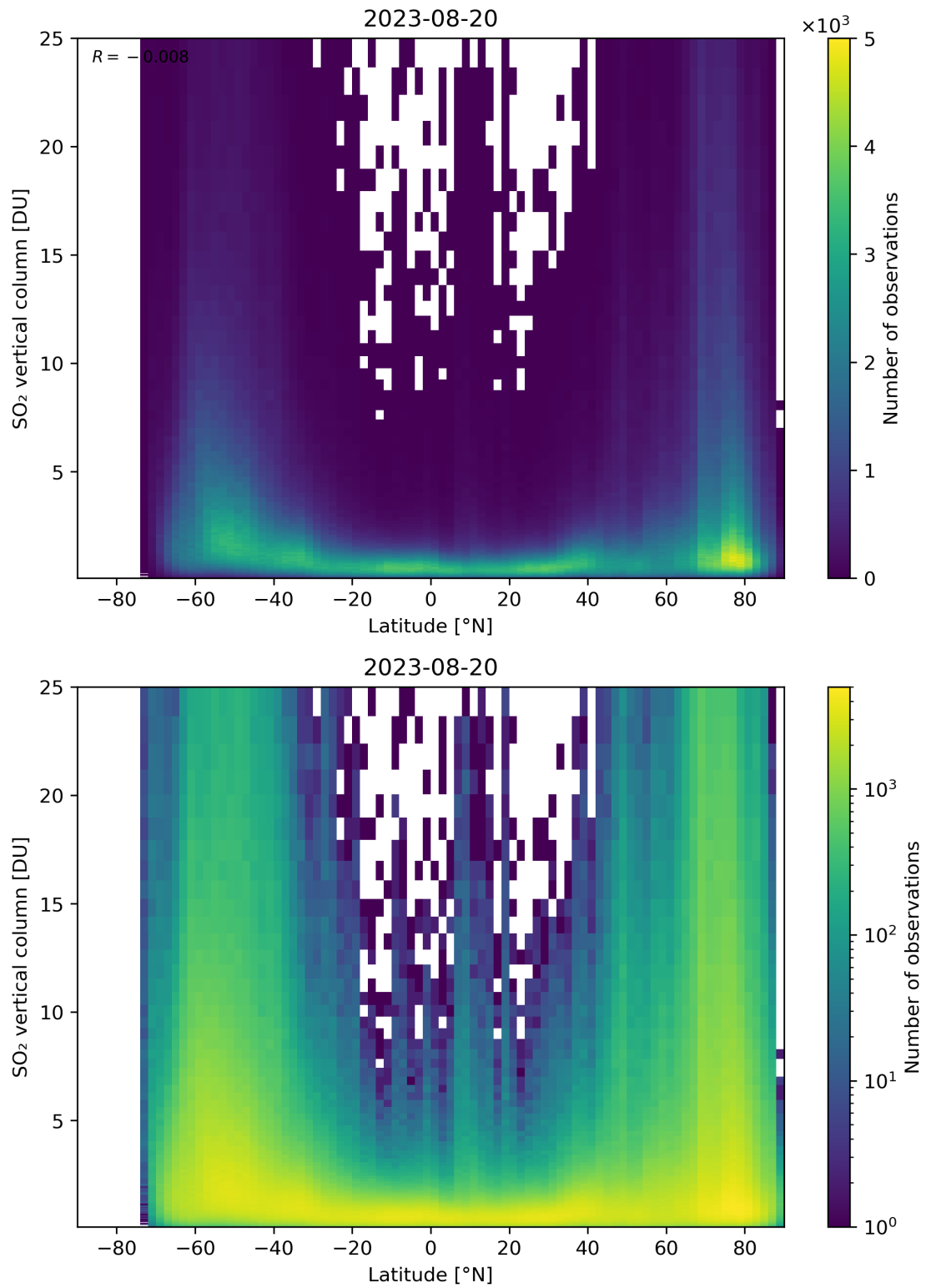
Figure 156: Scatter density plot of “Latitude” against “SO 2 vertical column” for 2023-08-20 to 2023-08-21.
