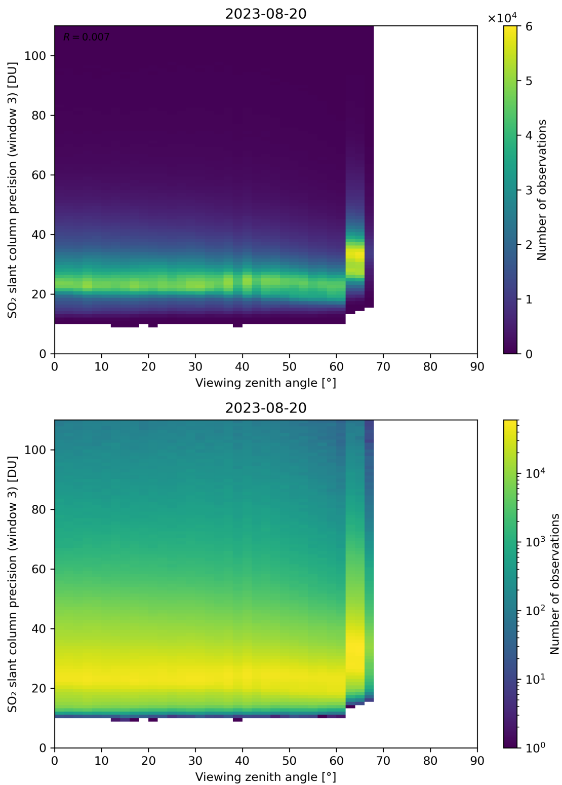
Figure 324: Scatter density plot of “Viewing zenith angle” against “SO 2 slant column precision (window 3)” for 2023-08-20 to 2023-08-21.
