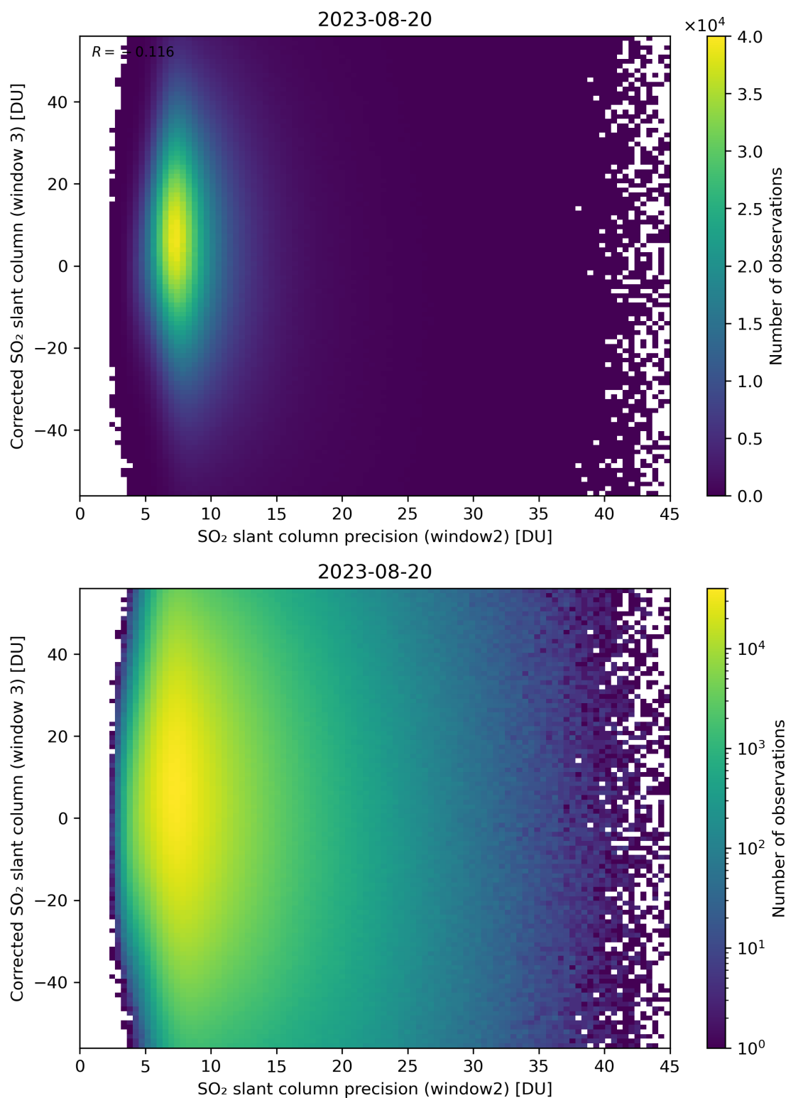
Figure 248: Scatter density plot of “SO 2 slant column precision (window2)” against “Corrected SO 2 slant column (window 3)” for 2023-08-20 to 2023-08-21.
