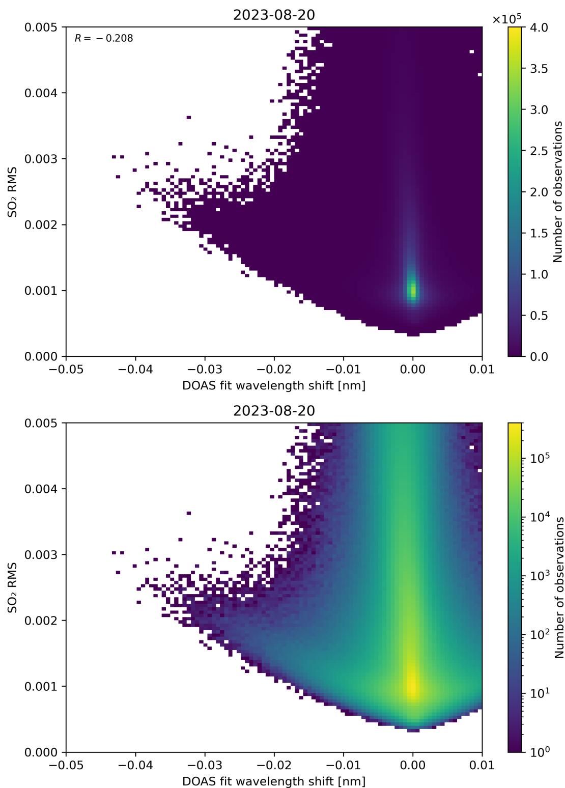
Figure 128: Scatter density plot of “DOAS fit wavelength shift” against “SO 2 RMS” for 2023-08-20 to 2023-08-21.
