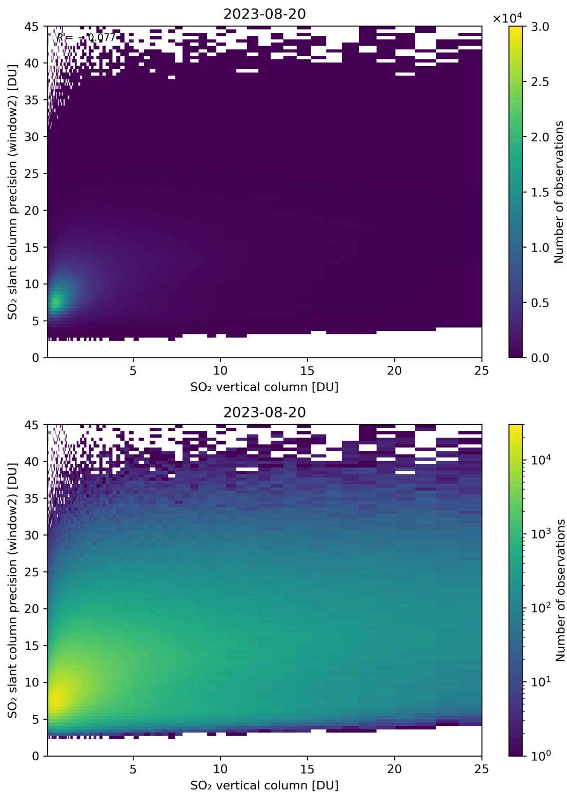
Figure 302: Scatter density plot of “SO 2 vertical column” against “SO 2 slant column precision (window2)” for 2023-08-20 to 2023-08-21.
