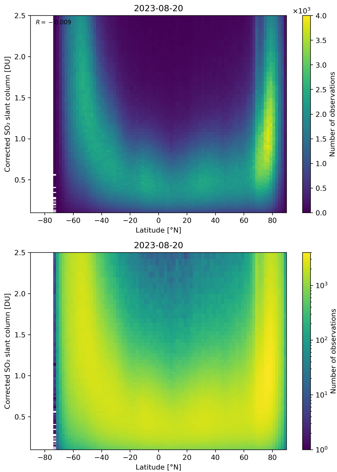
Figure 146: Scatter density plot of “Latitude” against “Corrected SO 2 slant column” for 2023-08-20 to 2023-08-21.
