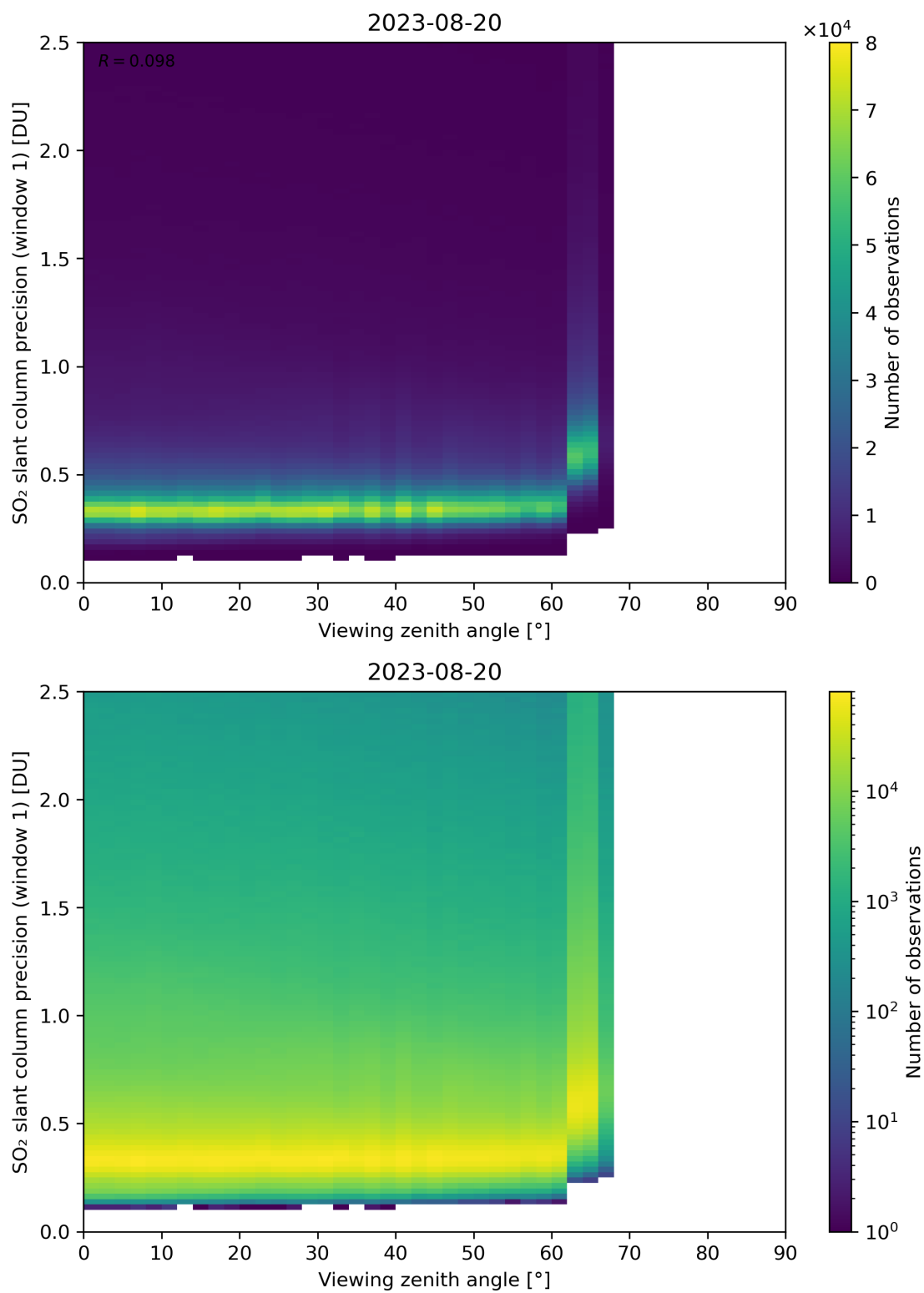
Figure 321: Scatter density plot of “Viewing zenith angle” against “SO 2 slant column precision (window 1)” for 2023-08-20 to 2023-08-21.
