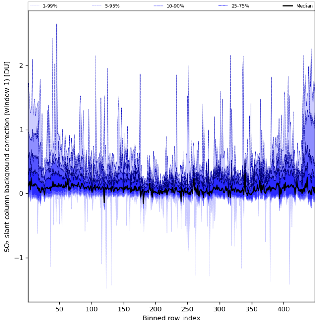
Figure 82: Along track statistics of “SO 2 slant column background correction (window 1)” for 2023-08-20 to 2023-08-21
