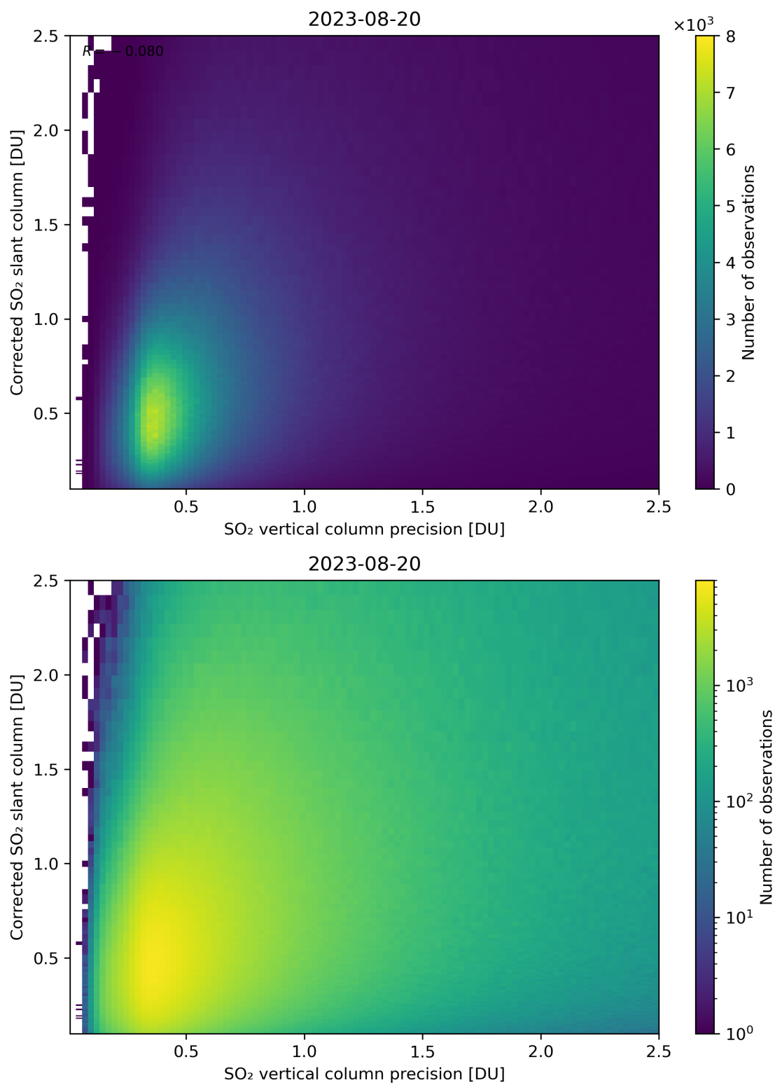
Figure 286: Scatter density plot of “SO 2 vertical column precision” against “Corrected SO 2 slant column” for 2023-08-20 to 2023-08-21.
