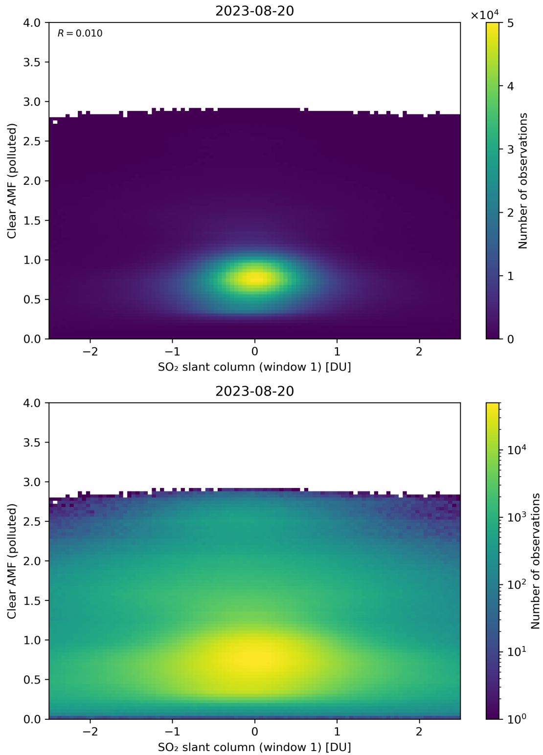
Figure 232: Scatter density plot of “SO 2 slant column (window 1)” against “Clear AMF (polluted)” for 2023-08-20 to 2023-08-21.
