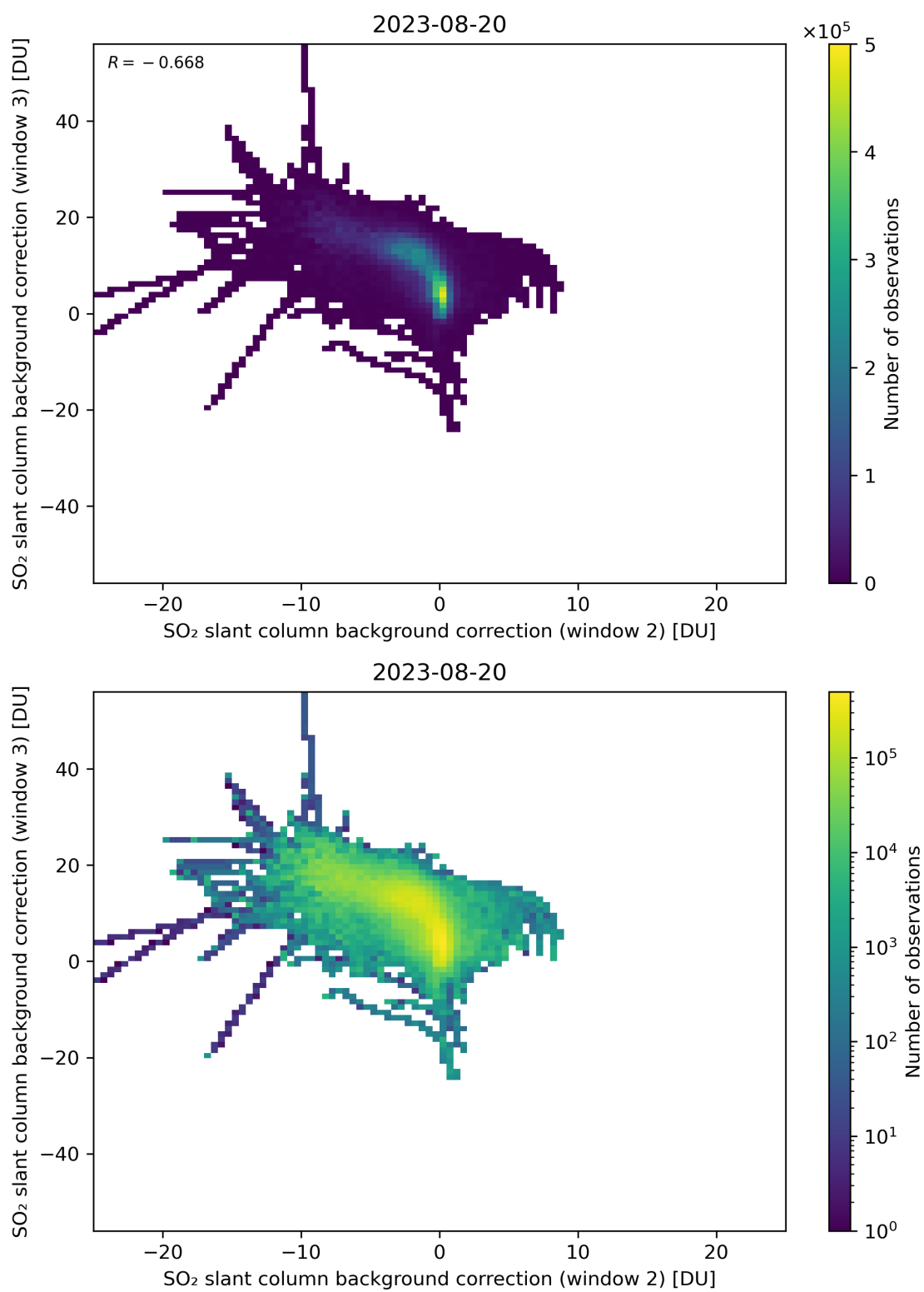
Figure 111: Scatter density plot of “SO 2 slant column background correction (window 2)” against “SO 2 slant column background correction (window 3)” for 2023-08-20 to 2023-08-21.
