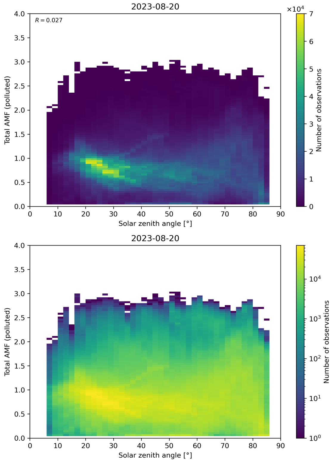
Figure 174: Scatter density plot of “Solar zenith angle” against “Total AMF (polluted)” for 2023-08-20 to 2023-08-21.
