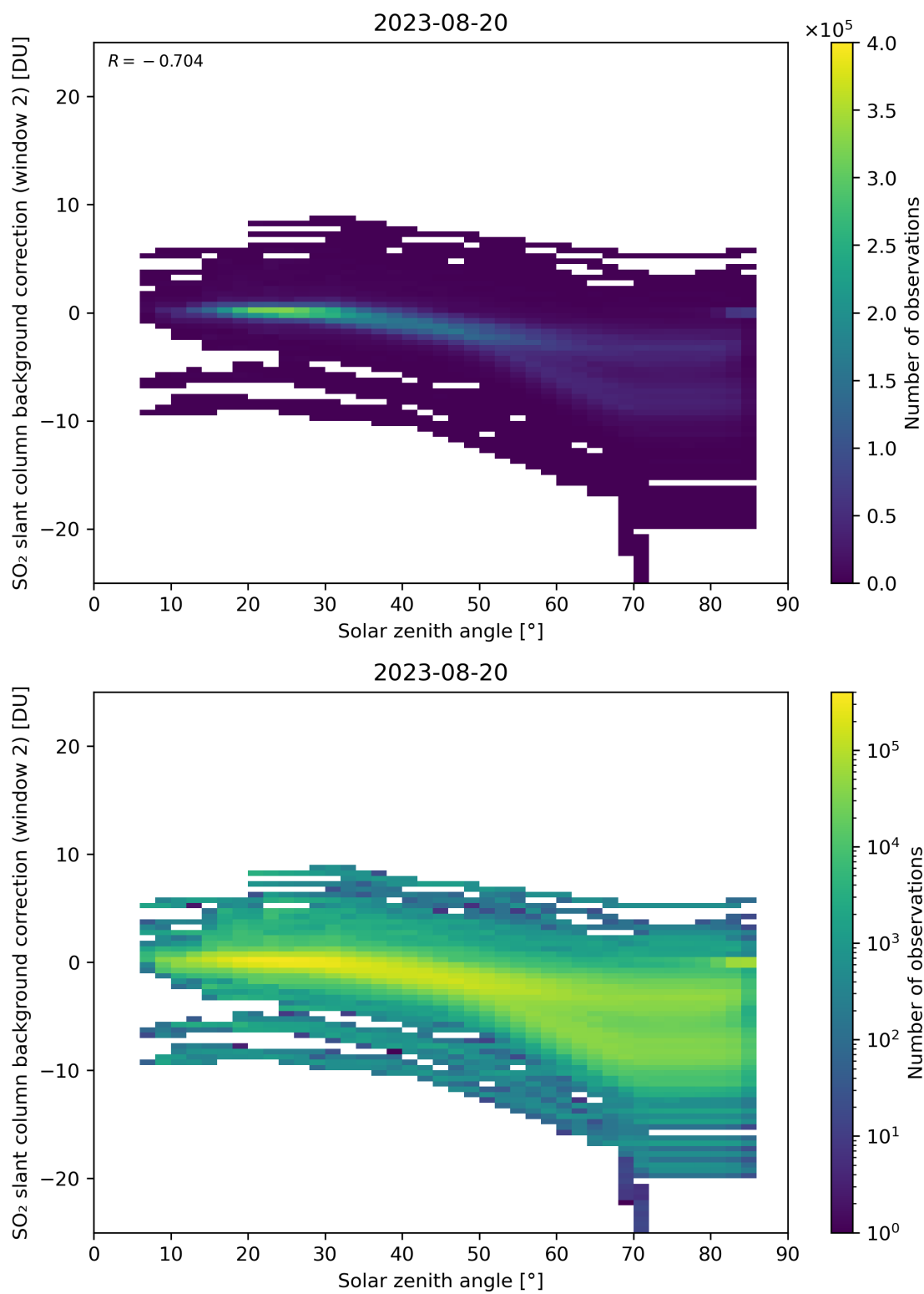
Figure 159: Scatter density plot of “Solar zenith angle” against “SO 2 slant column background correction (window 2)” for 2023-08-20 to 2023-08-21.
