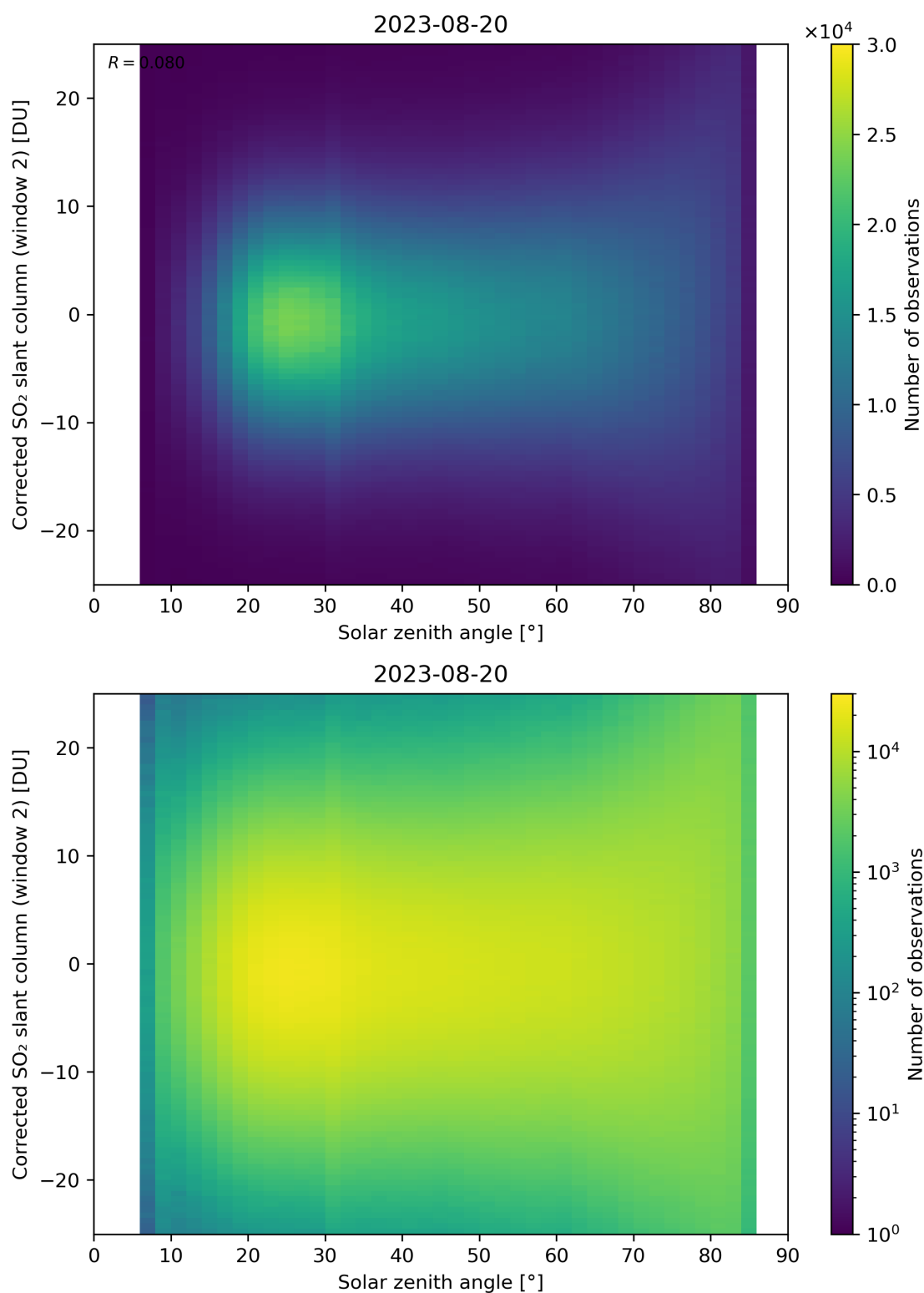
Figure 167: Scatter density plot of “Solar zenith angle” against “Corrected SO 2 slant column (window 2)” for 2023-08-20 to 2023-08-21.
