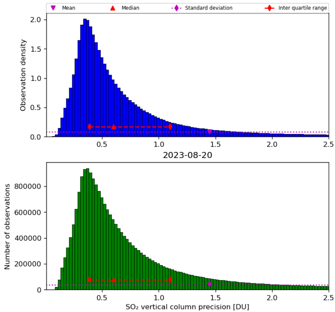
Figure 54: Histogram of “SO 2 vertical column precision” for 2023-08-20 to 2023-08-21
