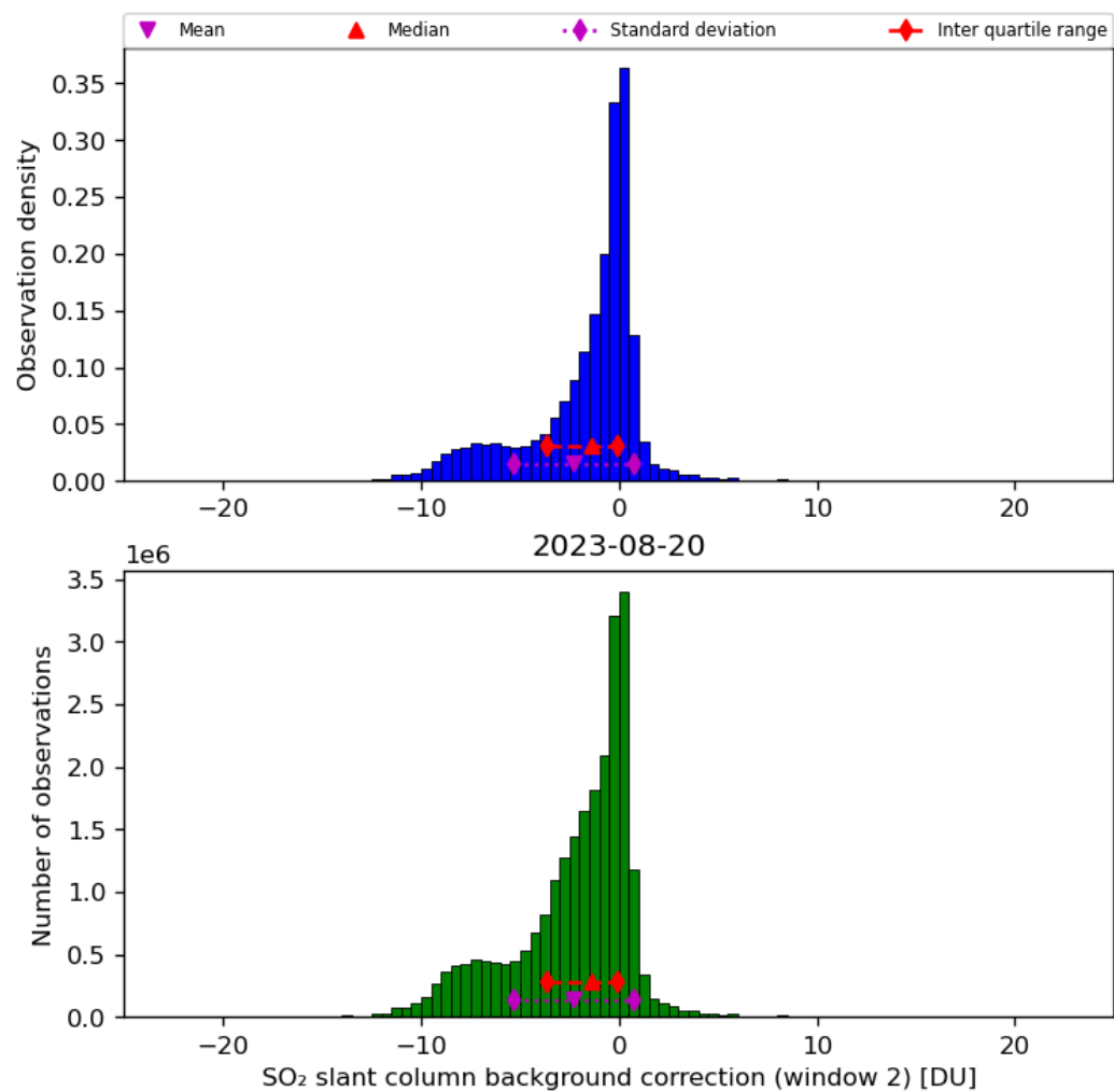
Figure 63: Histogram of “SO 2 slant column background correction (window 2)” for 2023-08-20 to 2023-08-21
