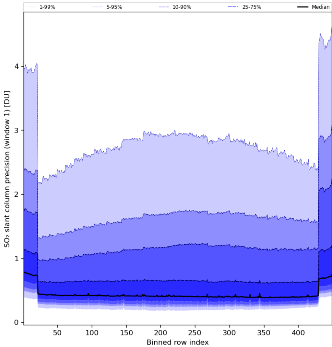
Figure 80: Along track statistics of “SO 2 slant column precision (window 1)” for 2023-08-20 to 2023-08-21
