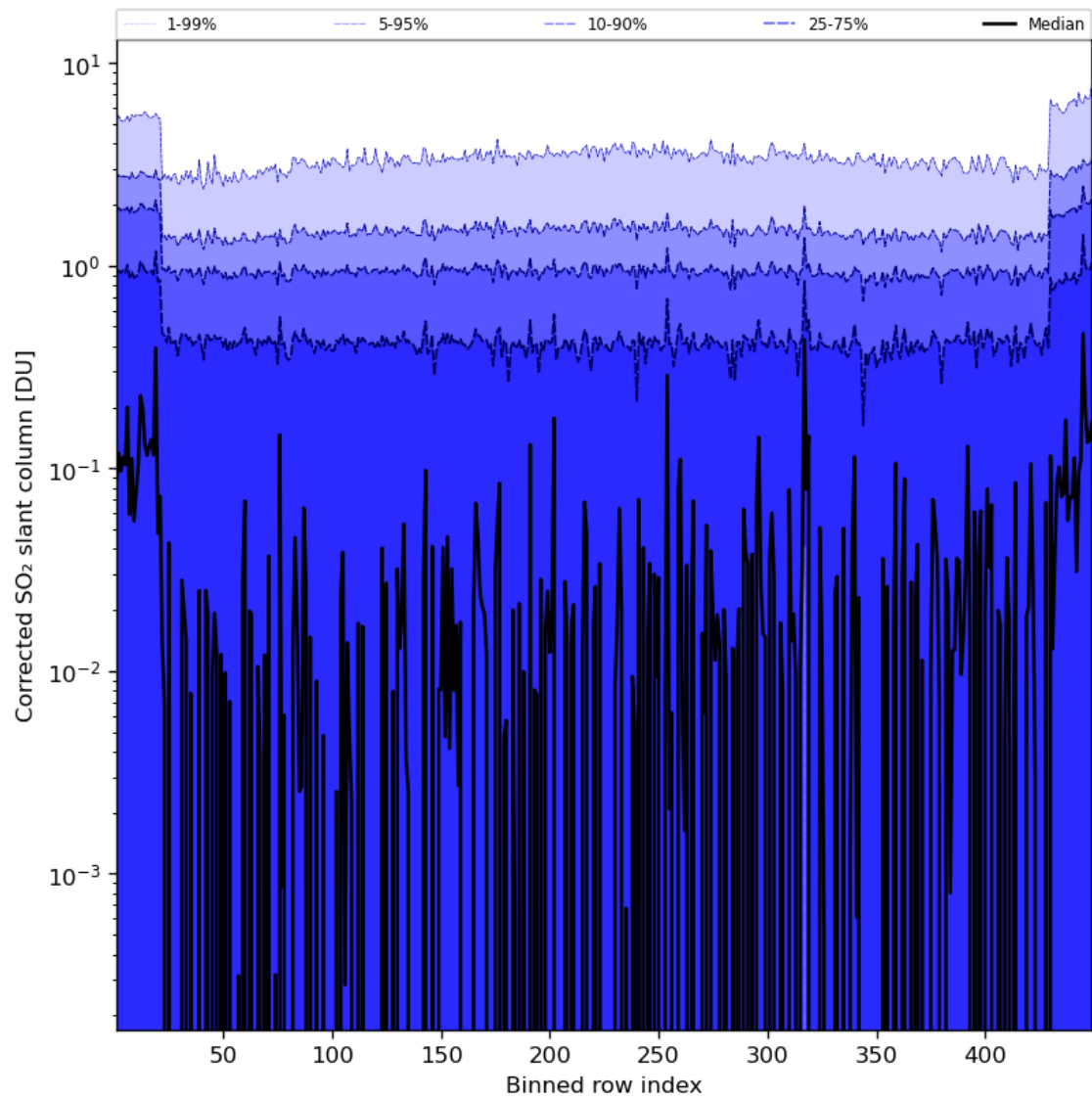
Figure 78: Along track statistics of “Corrected SO 2 slant column” for 2023-08-20 to 2023-08-21
