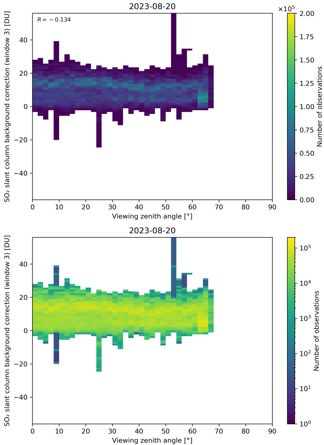
Figure 310: Scatter density plot of “Viewing zenith angle” against “SO 2 slant column background correction (window 3)” for 2023-08-20 to 2023-08-21.
