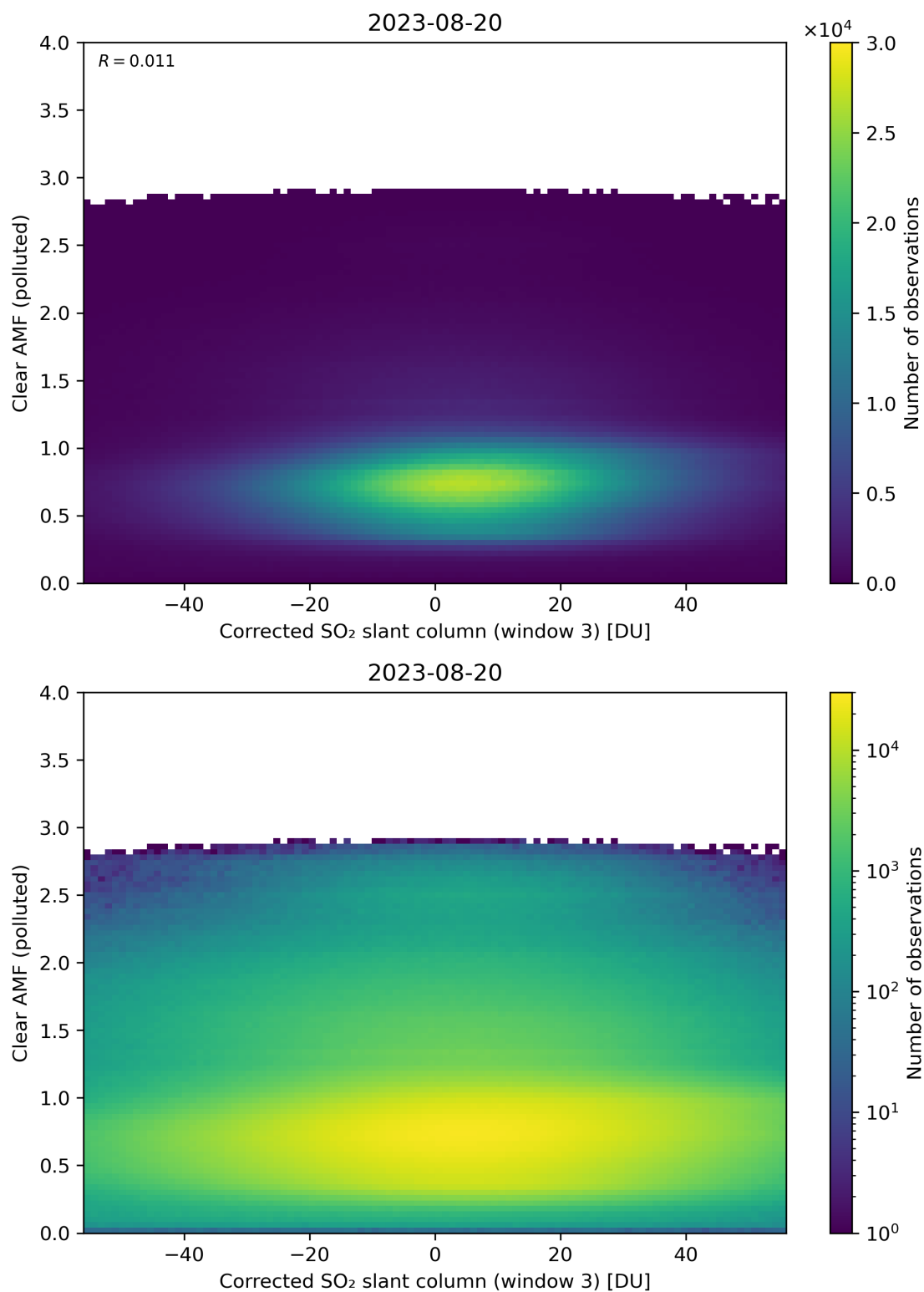
Figure 209: Scatter density plot of “Corrected SO 2 slant column (window 3)” against “Clear AMF (polluted)” for 2023-08-20 to 2023-08-21.
