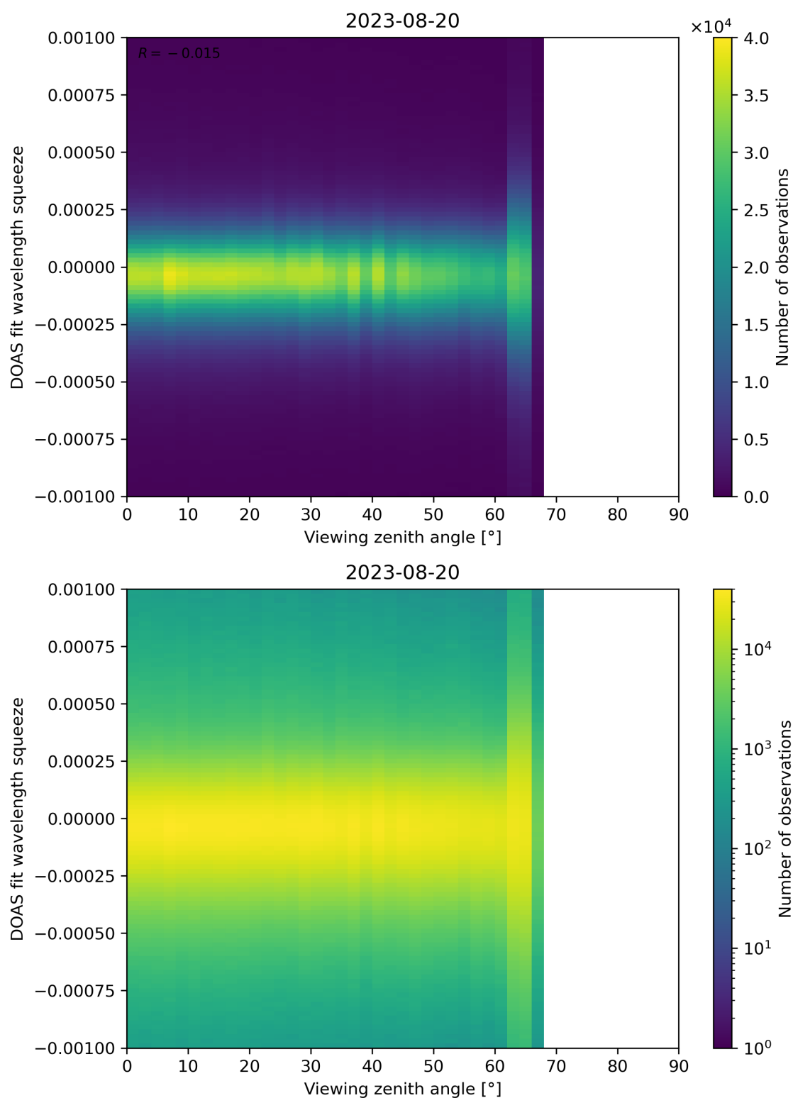
Figure 312: Scatter density plot of “Viewing zenith angle” against “DOAS fit wavelength squeeze” for 2023-08-20 to 2023-08-21.
