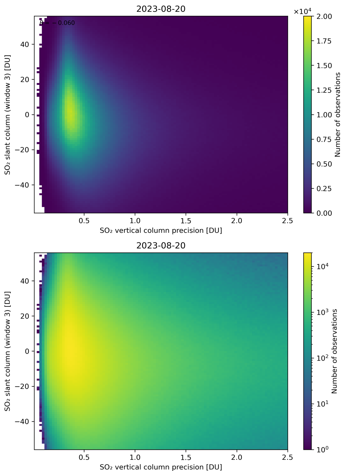
Figure 292: Scatter density plot of “SO 2 vertical column precision” against “SO 2 slant column (window 3)” for 2023-08-20 to 2023-08-21.
