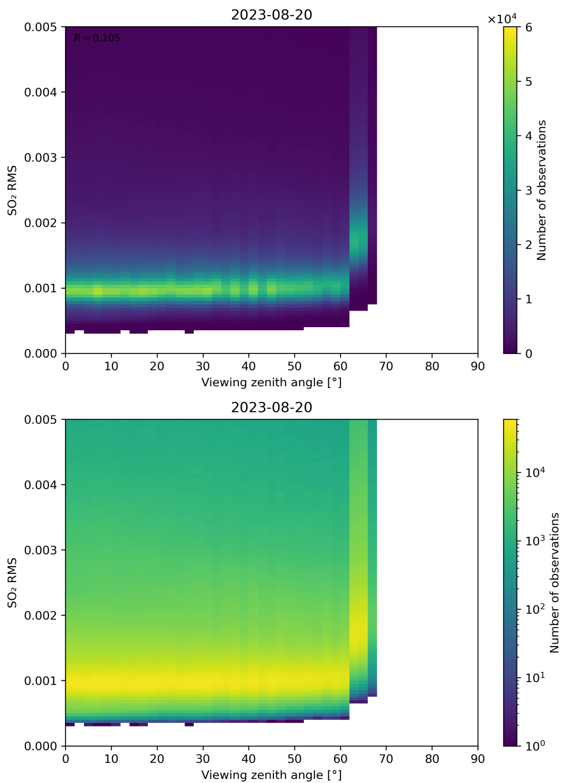
Figure 313: Scatter density plot of “Viewing zenith angle” against “SO 2 RMS” for 2023-08-20 to 2023-08-21.
