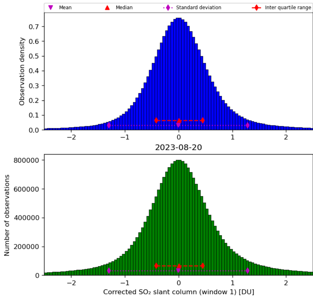
Figure 58: Histogram of “Corrected SO 2 slant column (window 1)” for 2023-08-20 to 2023-08-21
