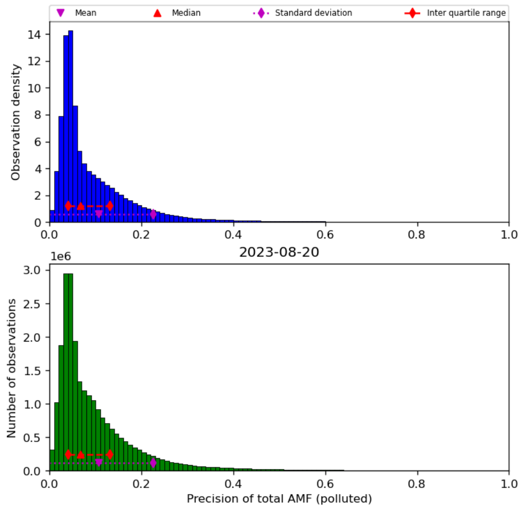
Figure 72: Histogram of “Precision of total AMF (polluted)” for 2023-08-20 to 2023-08-21
