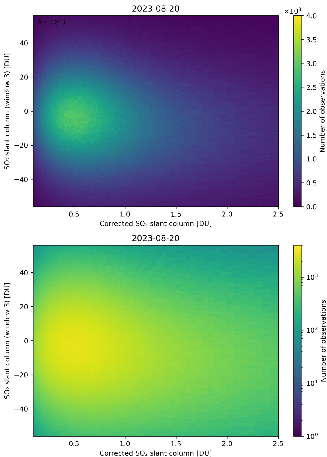
Figure 190: Scatter density plot of “Corrected SO 2 slant column” against “SO 2 slant column (window 3)” for 2023-08-20 to 2023-08-21.
