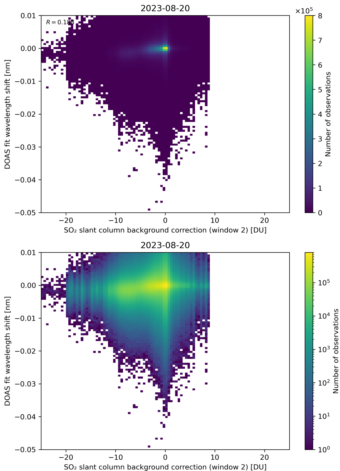
Figure 112: Scatter density plot of “SO 2 slant column background correction (window 2)” against “DOAS fit wavelength shift” for 2023-08-20 to 2023-08-21.
