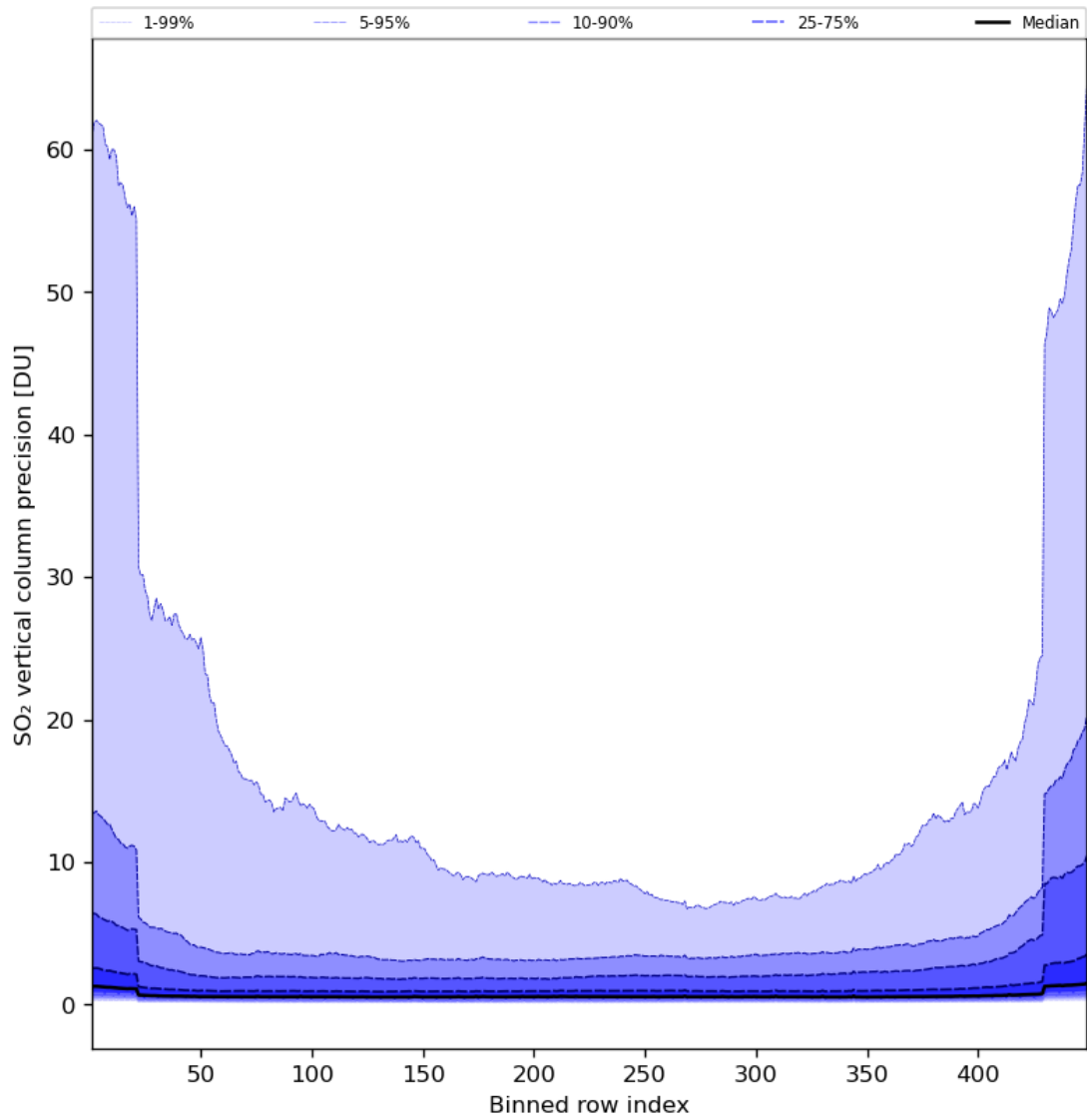
Figure 77: Along track statistics of “SO 2 vertical column precision” for 2023-08-20 to 2023-08-21
