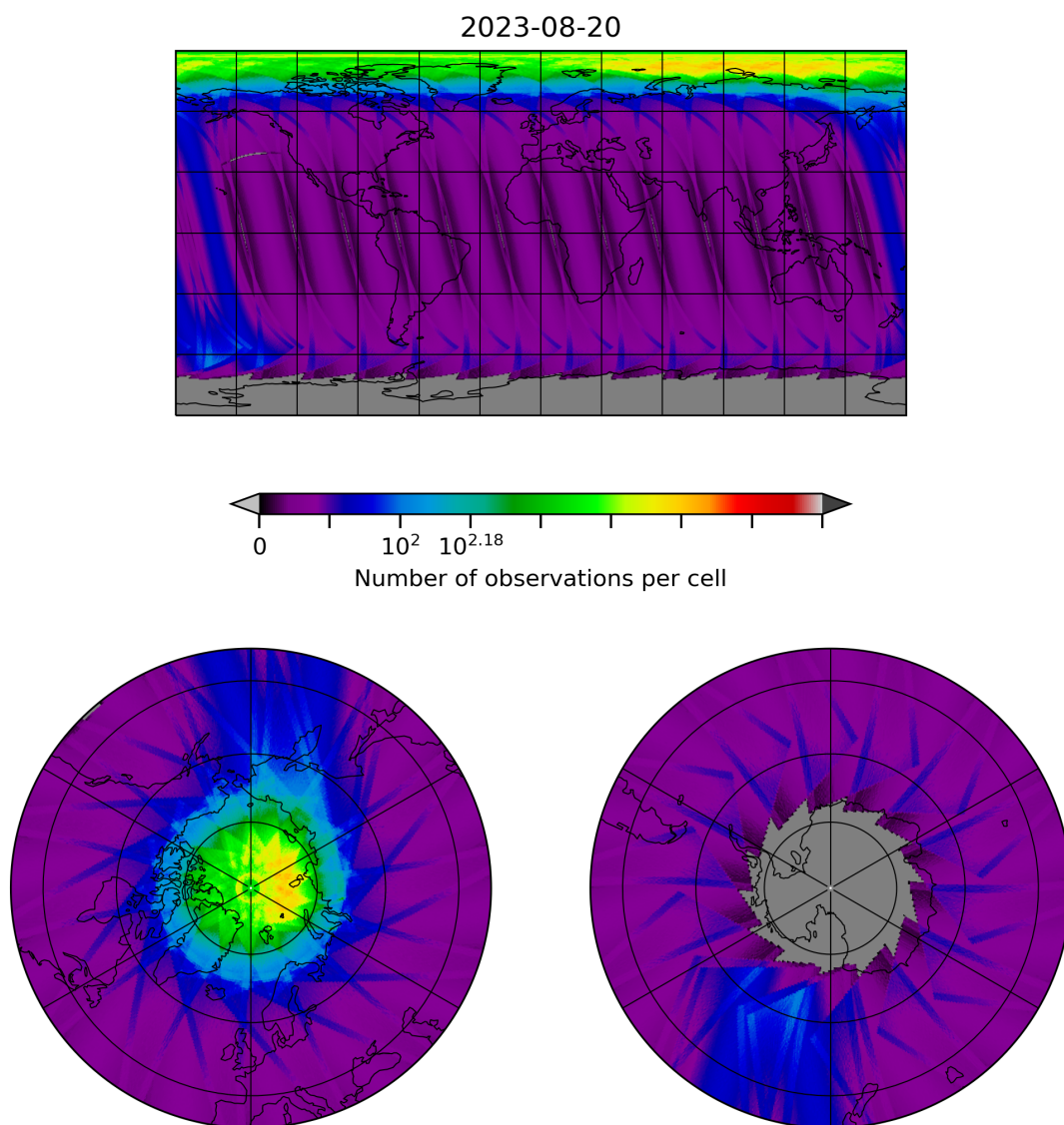
Figure 28: Map of the number of observations for 2023-08-20 to 2023-08-21
