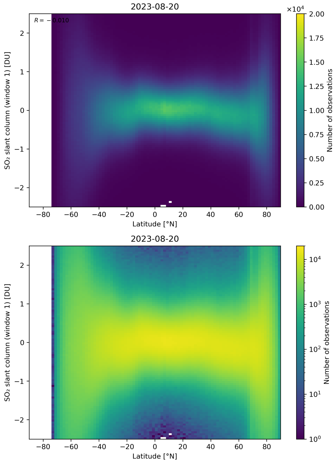
Figure 149: Scatter density plot of “Latitude” against “SO 2 slant column (window 1)” for 2023-08-20 to 2023-08-21.
