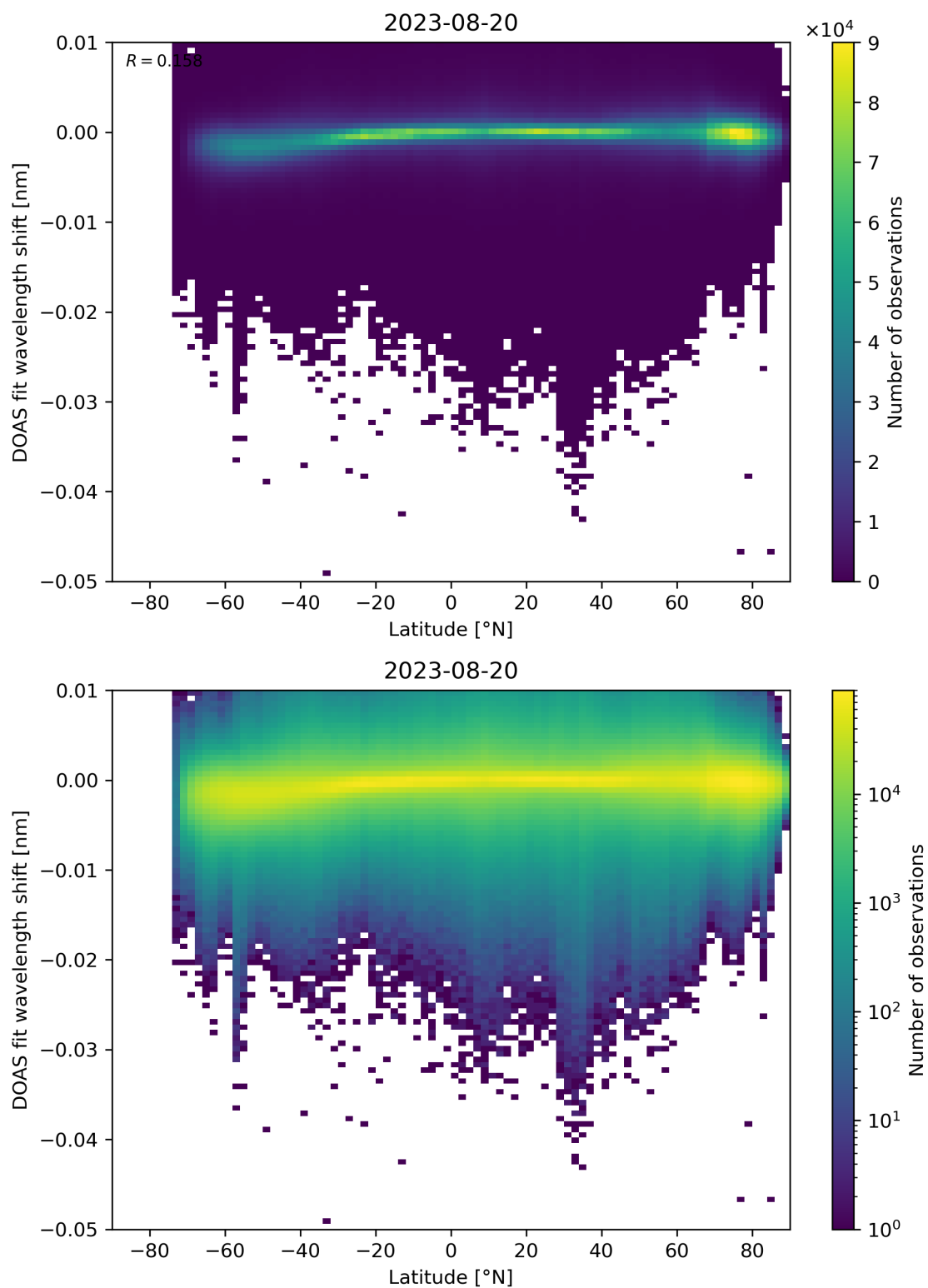
Figure 142: Scatter density plot of “Latitude” against “DOAS fit wavelength shift” for 2023-08-20 to 2023-08-21.
