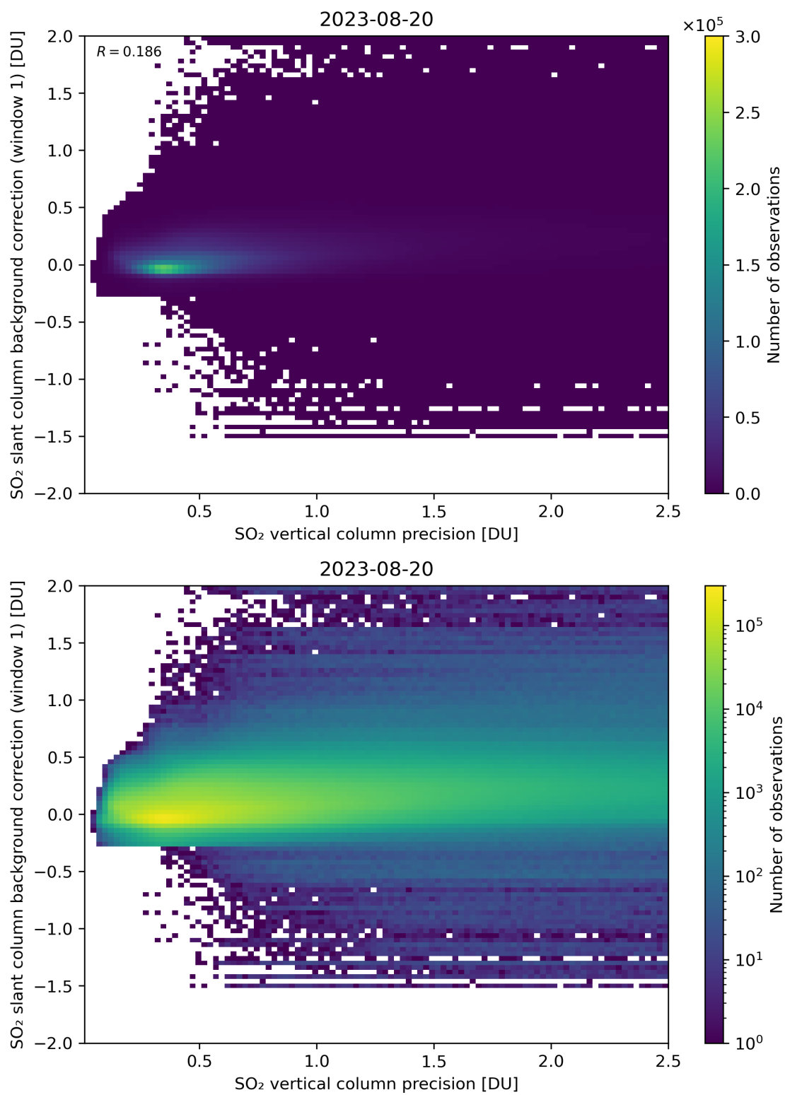
Figure 279: Scatter density plot of “SO 2 vertical column precision” against “SO 2 slant column background correction (window 1)” for 2023-08-20 to 2023-08-21.
