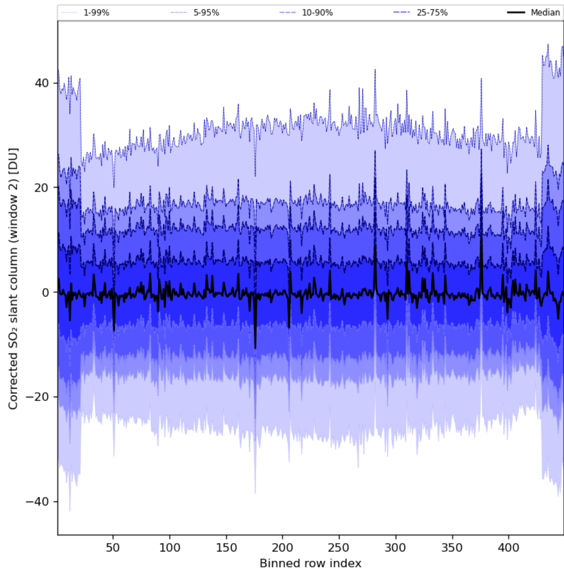
Figure 85: Along track statistics of “Corrected SO 2 slant column (window 2)” for 2023-08-20 to 2023-08-21
