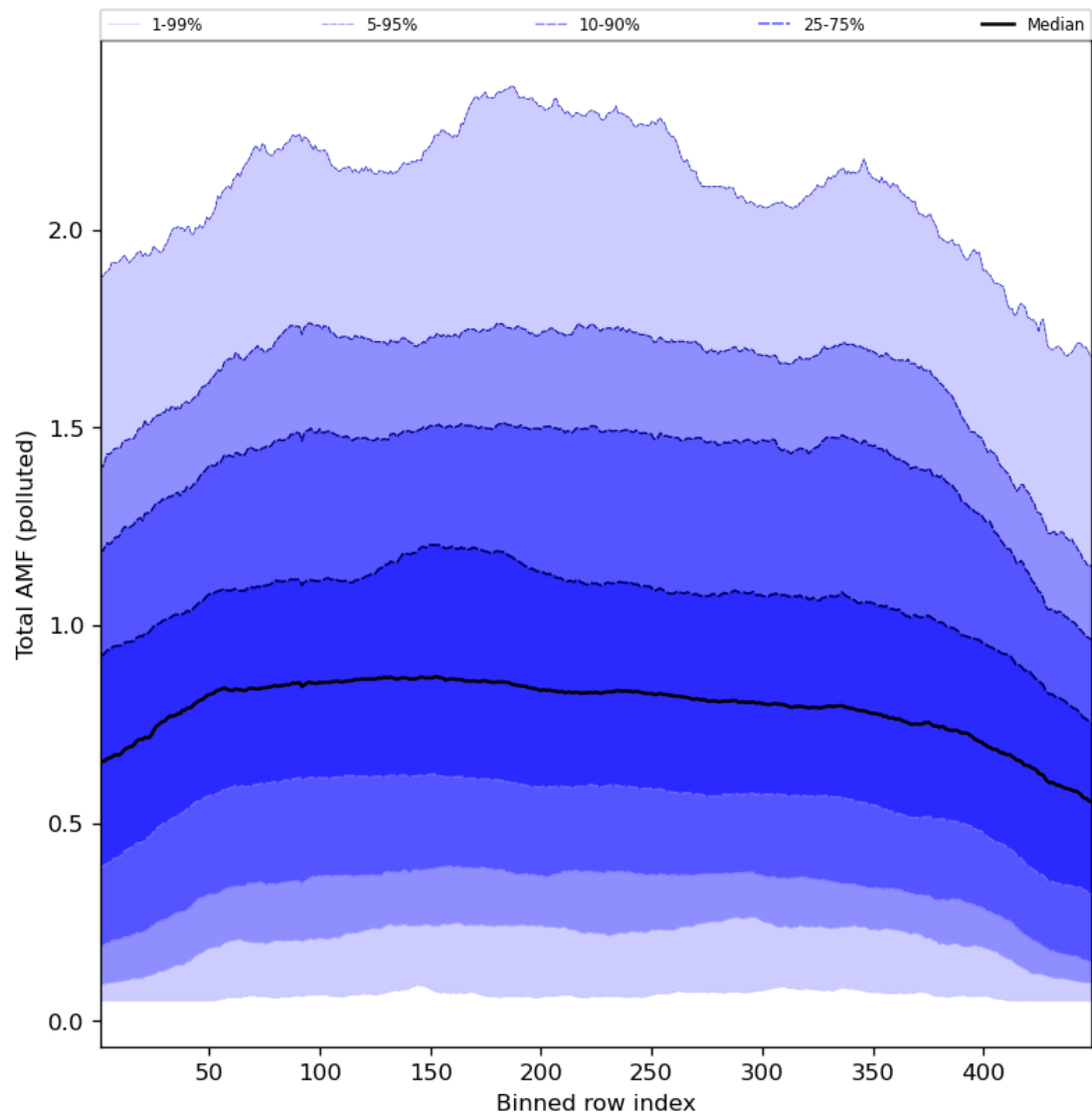
Figure 94: Along track statistics of “Total AMF (polluted)” for 2023-08-20 to 2023-08-21
