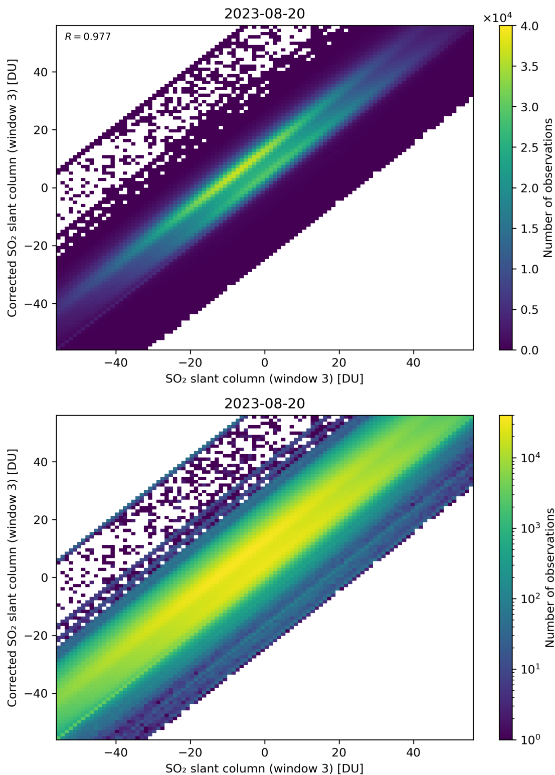
Figure 266: Scatter density plot of “SO 2 slant column (window 3)” against “Corrected SO 2 slant column (window 3)” for 2023-08-20 to 2023-08-21.
