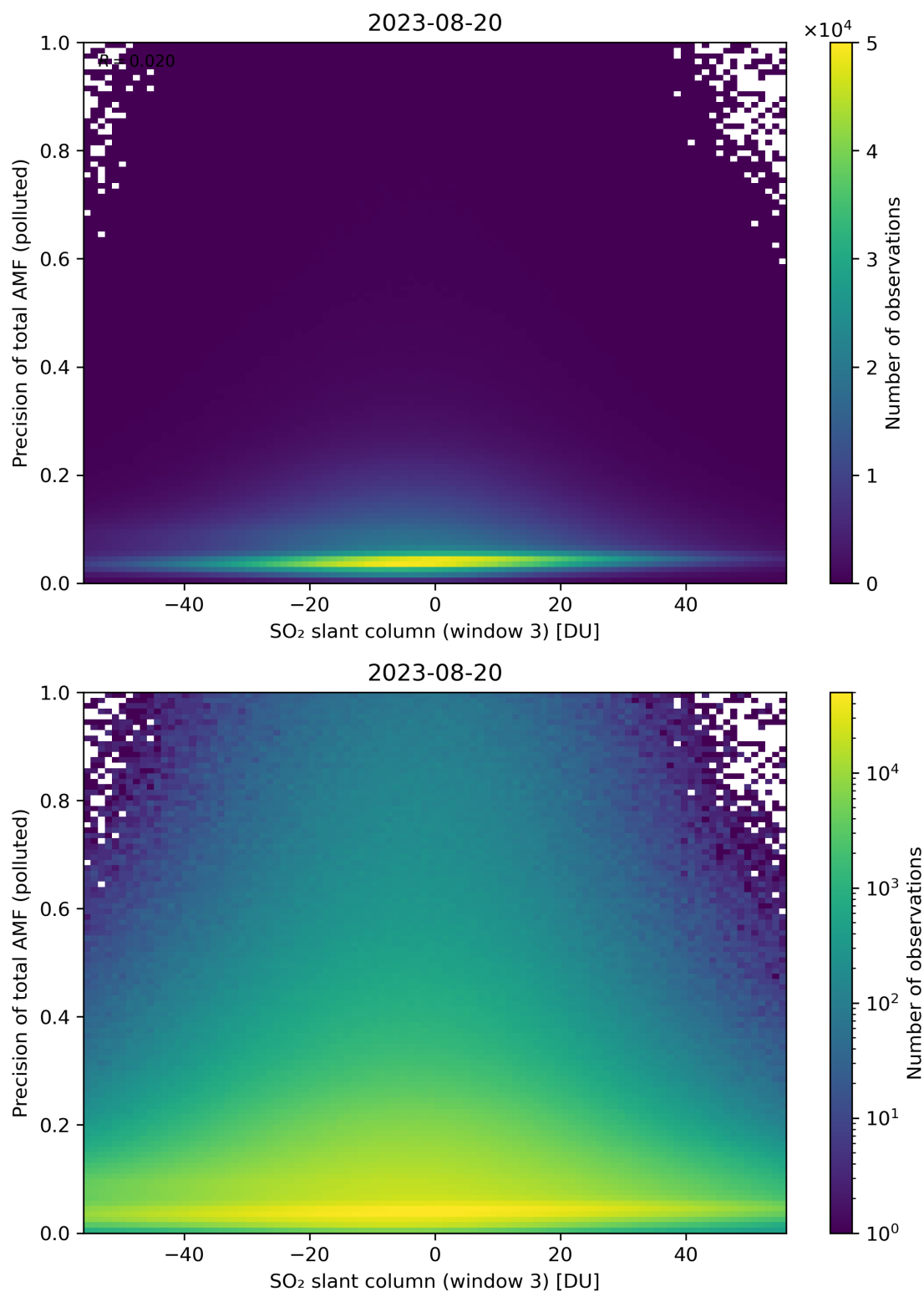
Figure 269: Scatter density plot of “SO 2 slant column (window 3)” against “Precision of total AMF (polluted)” for 2023-08-20 to 2023-08-21.
