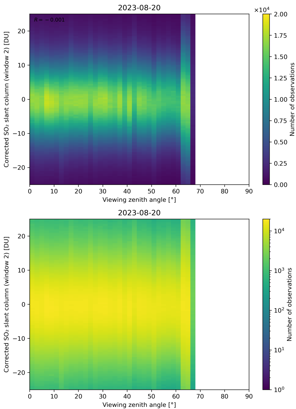
Figure 318: Scatter density plot of “Viewing zenith angle” against “Corrected SO 2 slant column (window 2)” for 2023-08-20 to 2023-08-21.
