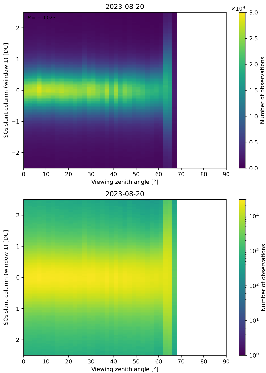
Figure 320: Scatter density plot of “Viewing zenith angle” against “SO 2 slant column (window 1)” for 2023-08-20 to 2023-08-21.
