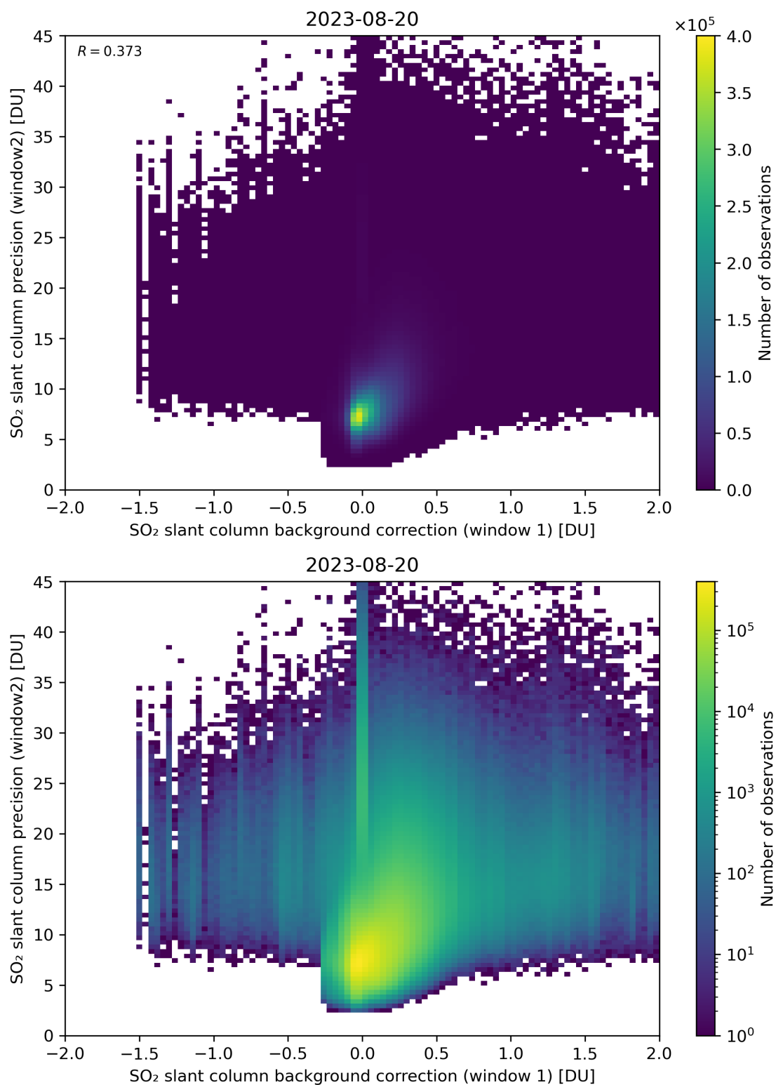
Figure 106: Scatter density plot of “SO 2 slant column background correction (window 1)” against “SO 2 slant column precision (window2)” for 2023-08-20 to 2023-08-21.
