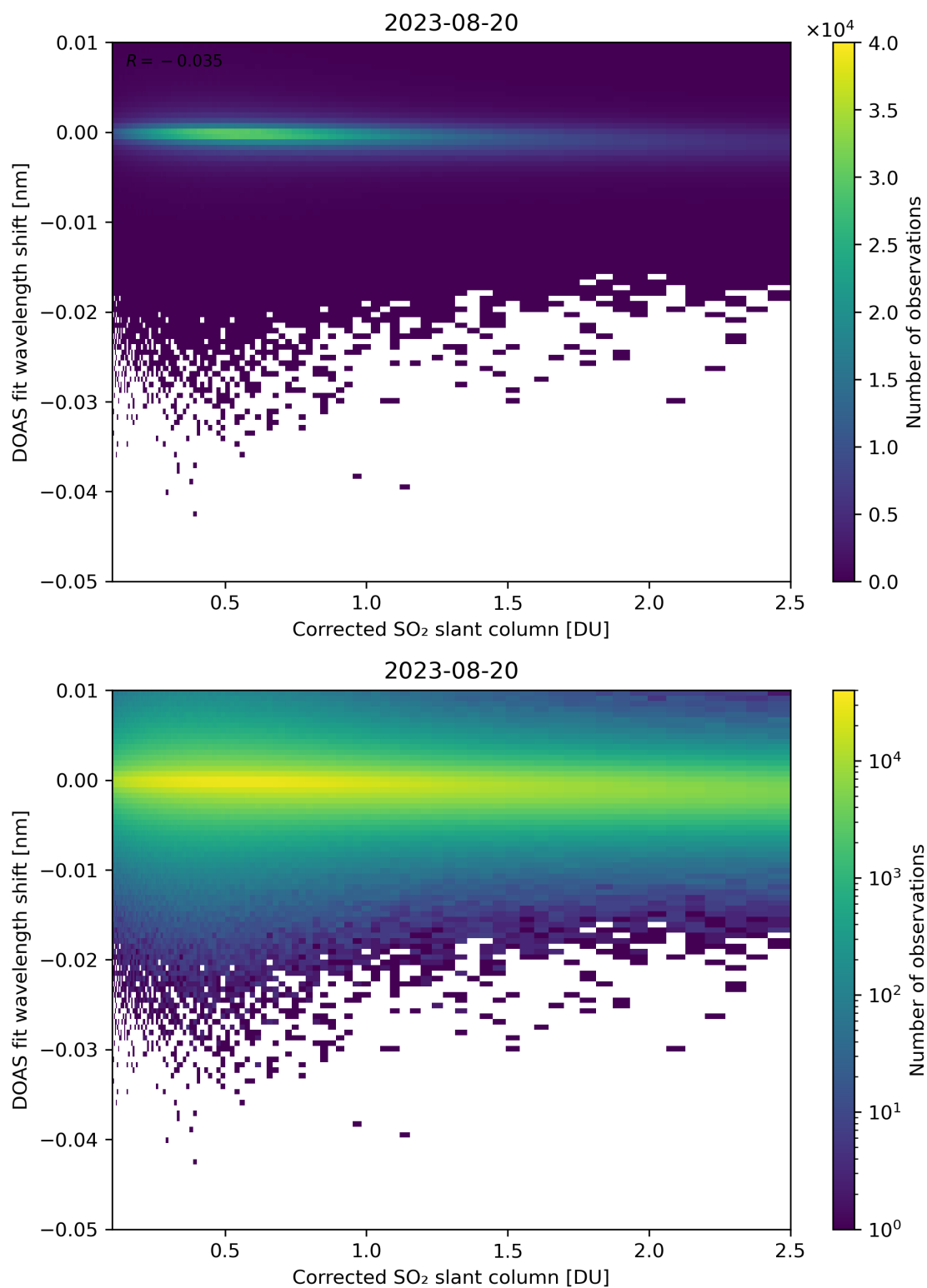
Figure 181: Scatter density plot of “Corrected SO 2 slant column” against “DOAS fit wavelength shift” for 2023-08-20 to 2023-08-21.
