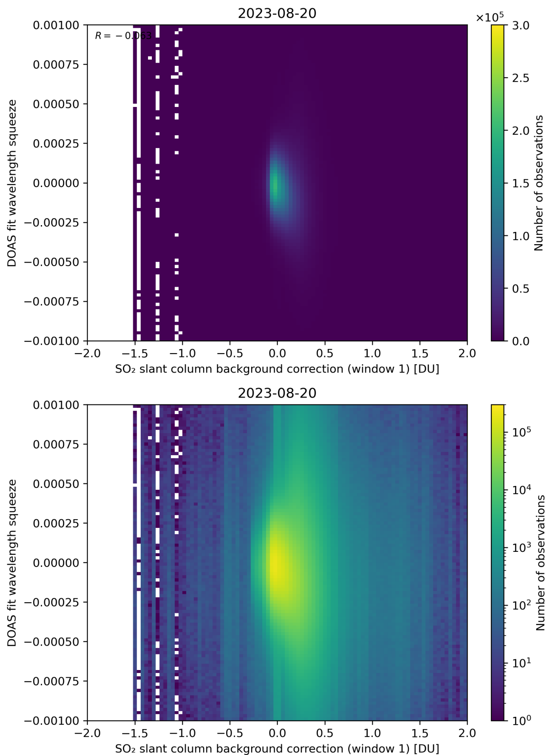
Figure 101: Scatter density plot of “SO 2 slant column background correction (window 1)” against “DOAS fit wavelength squeeze” for 2023-08-20 to 2023-08-21.
