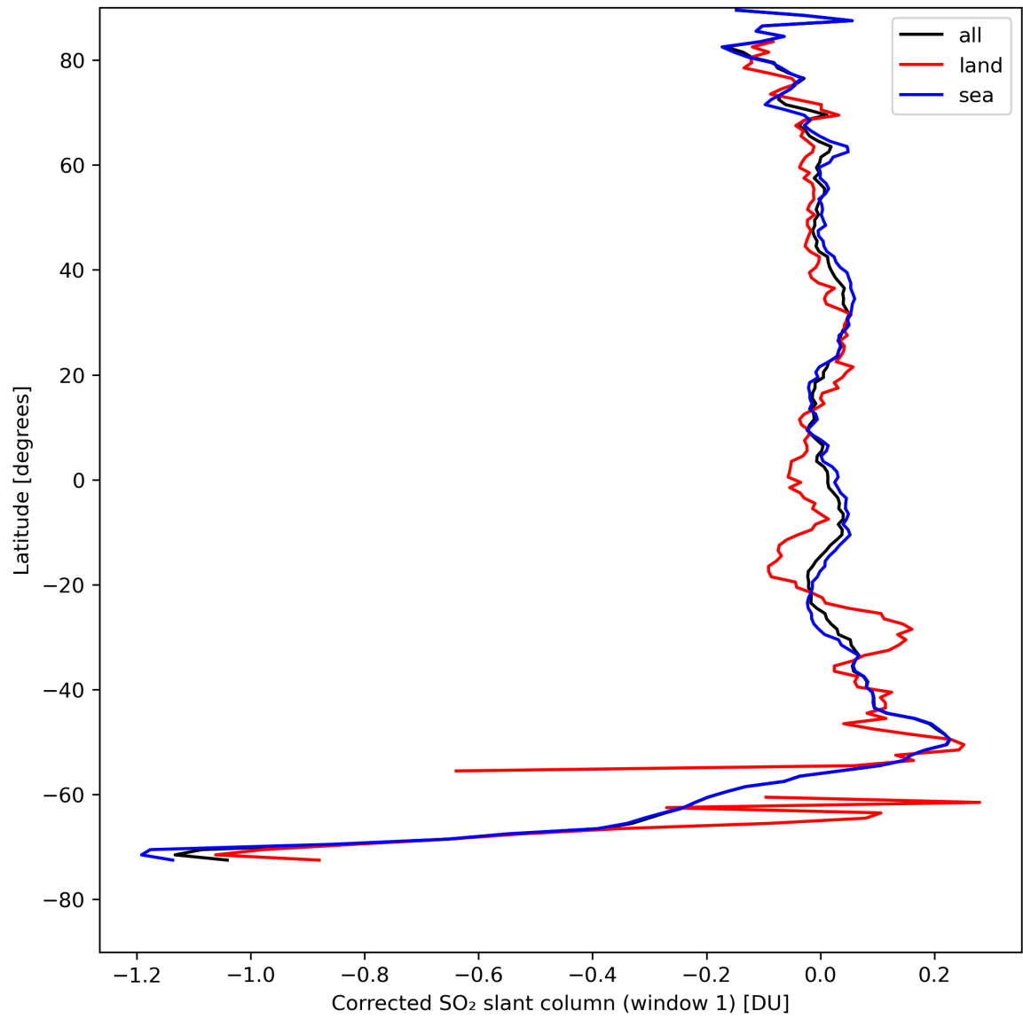
Figure 35: Zonal average of “Corrected SO 2 slant column (window 1)” for 2023-08-20 to 2023-08-21.
