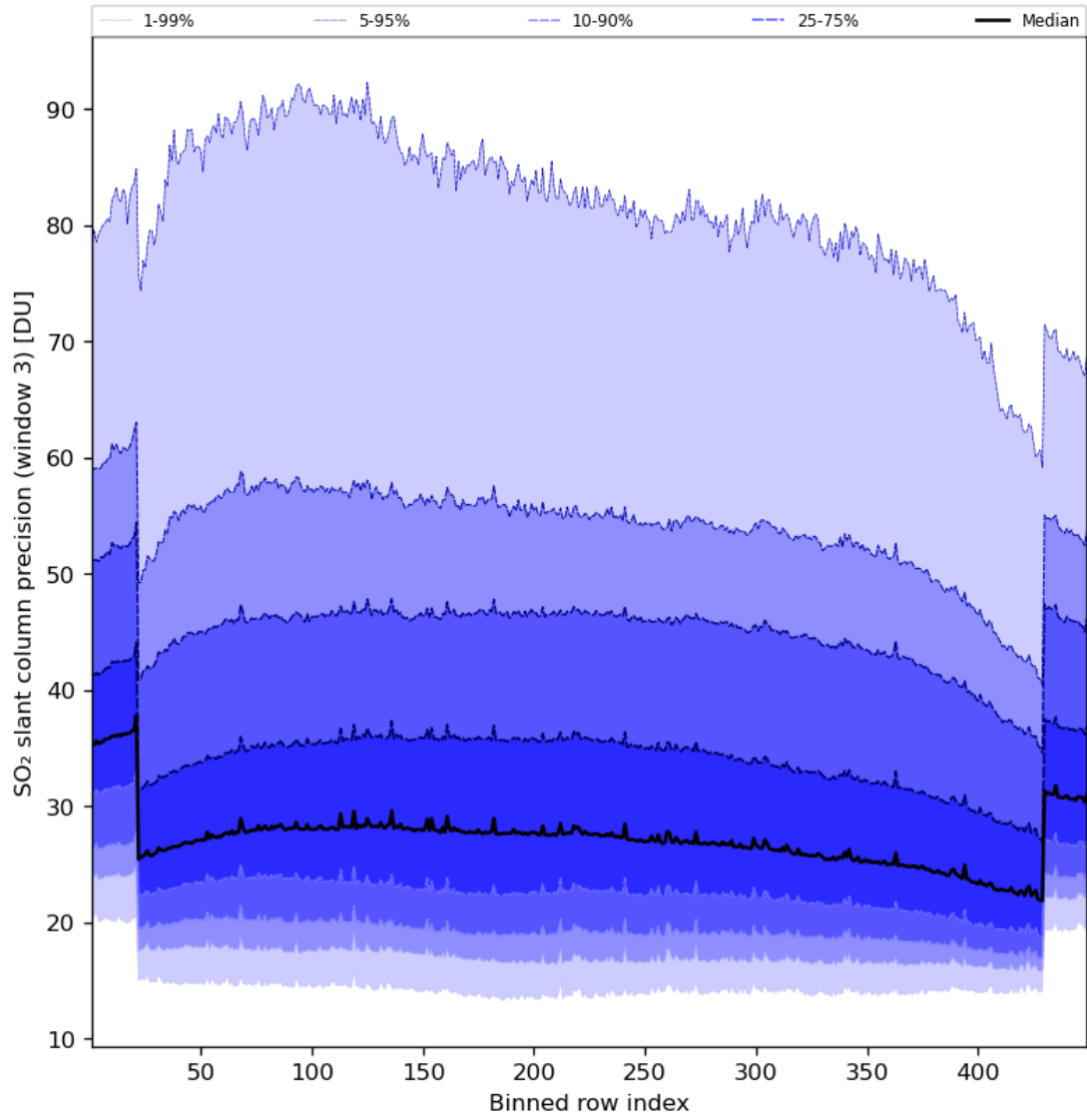
Figure 88: Along track statistics of “SO 2 slant column precision (window 3)” for 2023-08-20 to 2023-08-21
