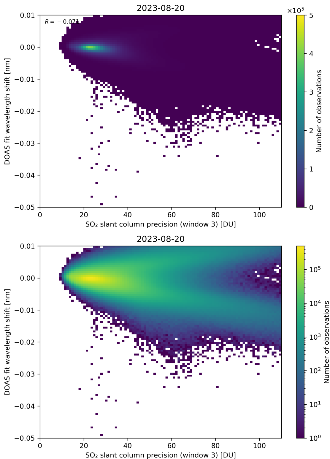
Figure 258: Scatter density plot of “SO 2 slant column precision (window 3)” against “DOAS fit wavelength shift” for 2023-08-20 to 2023-08-21.
