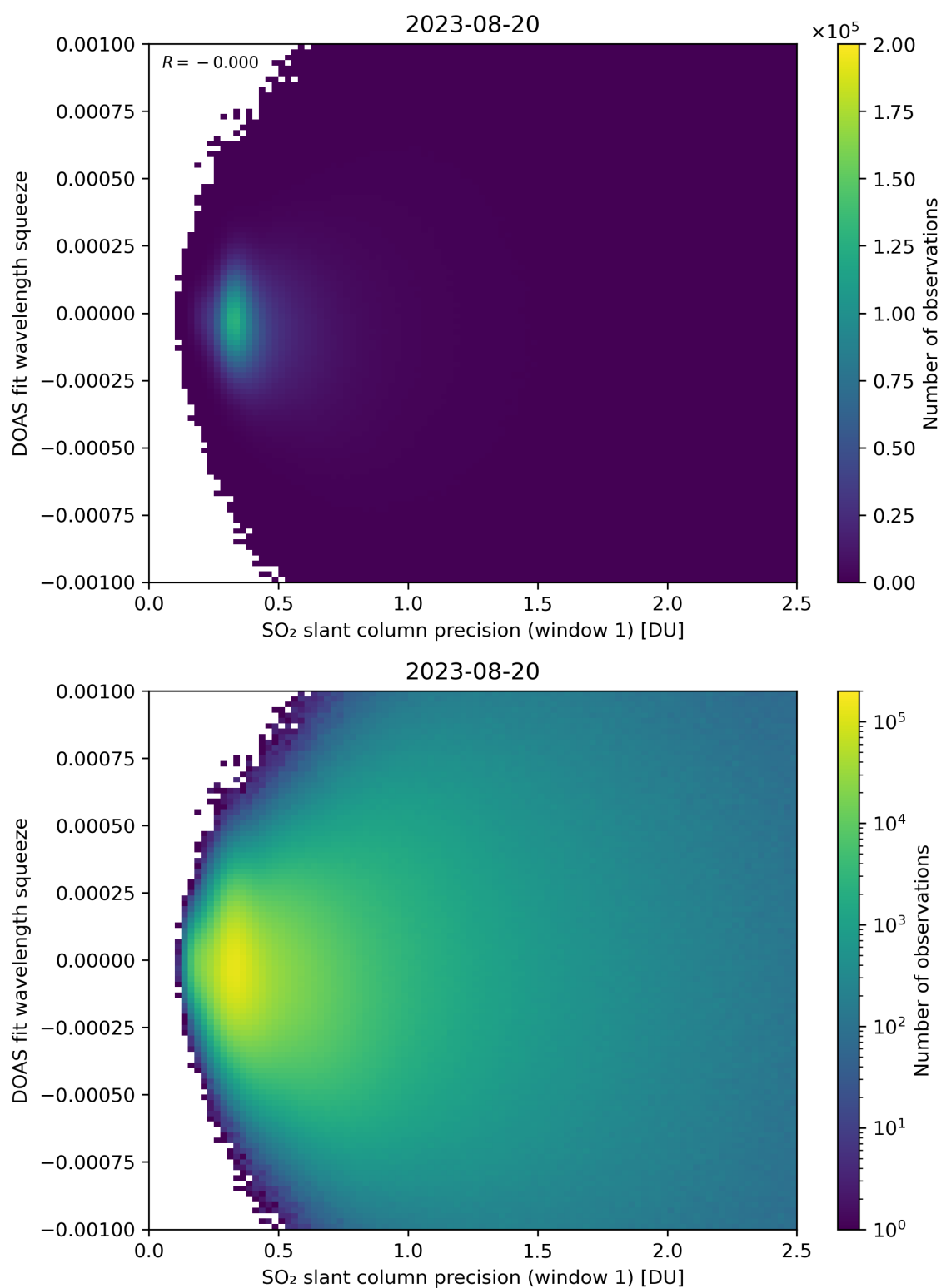
Figure 222: Scatter density plot of “SO 2 slant column precision (window 1)” against “DOAS fit wavelength squeeze” for 2023-08-20 to 2023-08-21.
