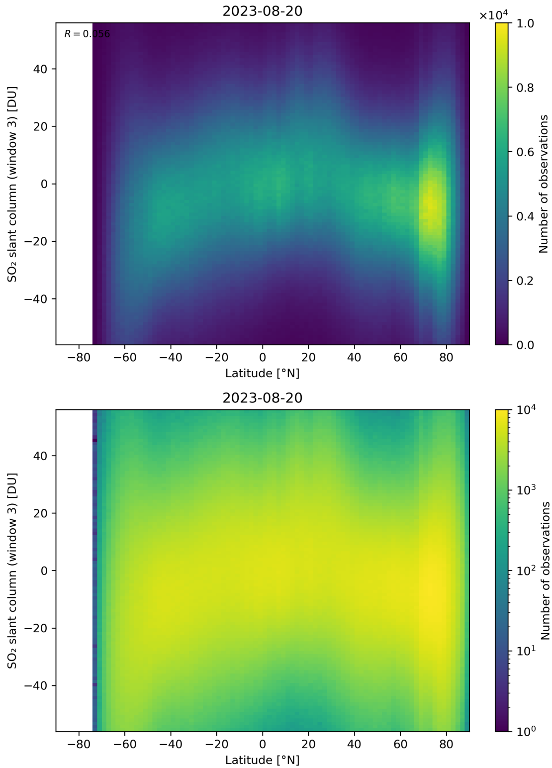
Figure 152: Scatter density plot of “Latitude” against “SO 2 slant column (window 3)” for 2023-08-20 to 2023-08-21.
