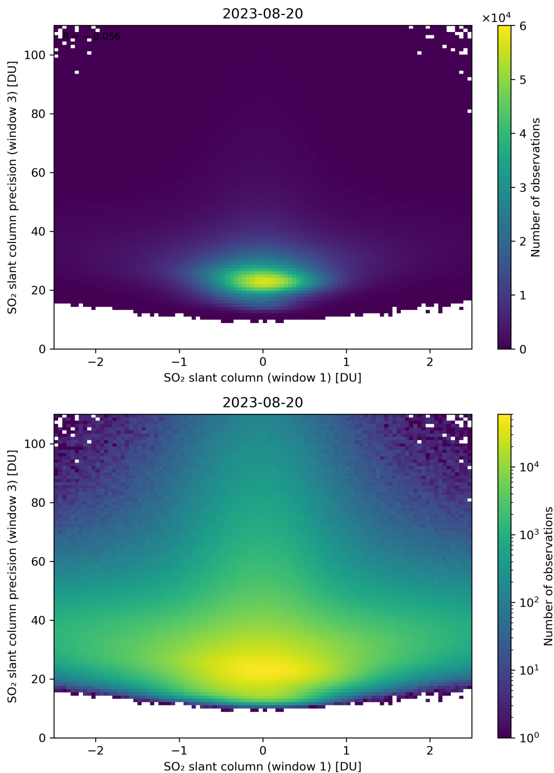
Figure 238: Scatter density plot of “SO 2 slant column (window 1)” against “SO 2 slant column precision (window 3)” for 2023-08-20 to 2023-08-21.
