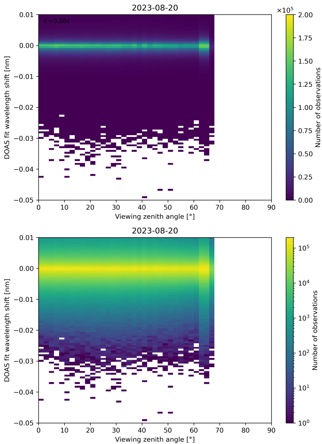
Figure 311: Scatter density plot of “Viewing zenith angle” against “DOAS fit wavelength shift” for 2023-08-20 to 2023-08-21.
