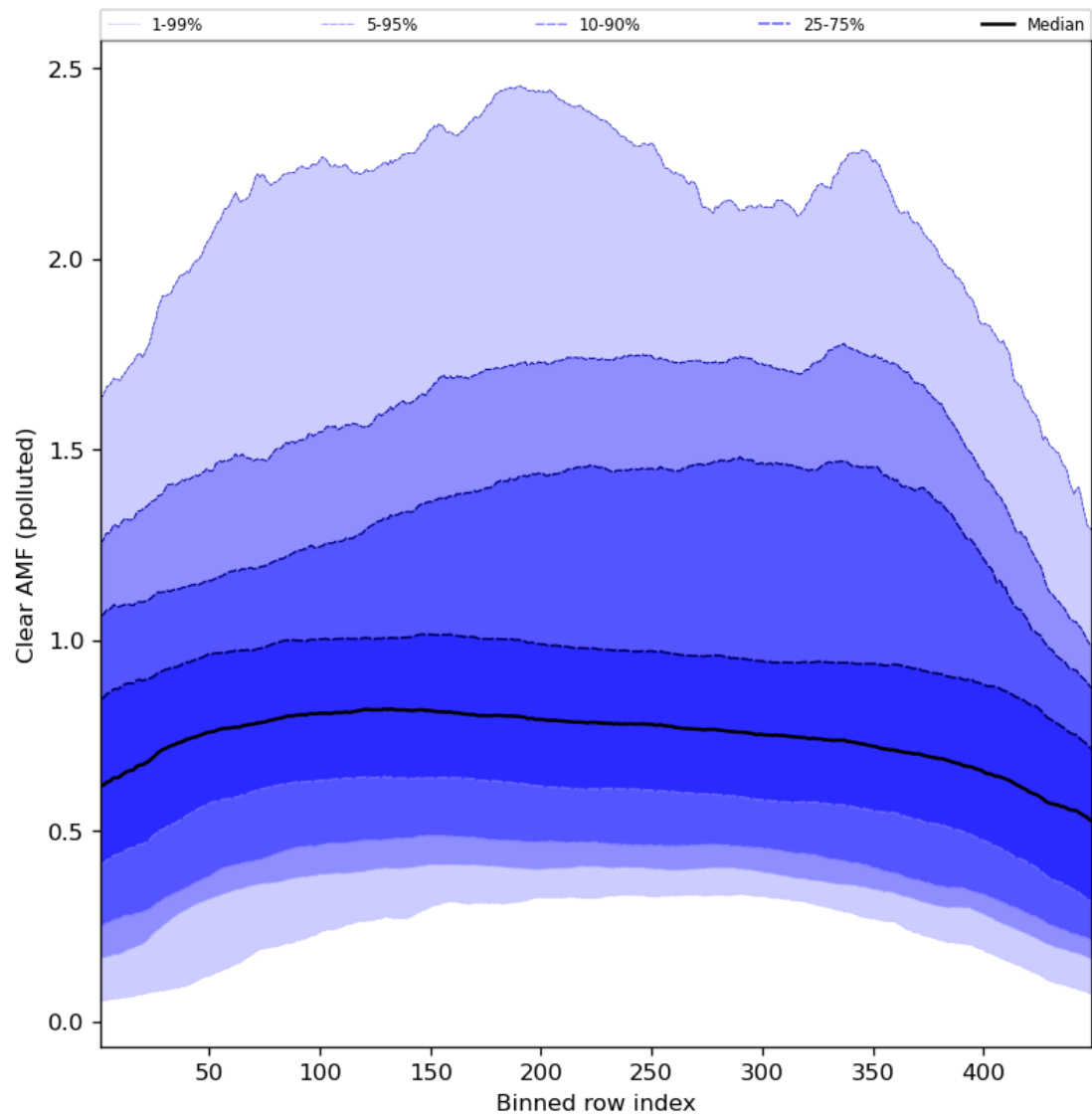
Figure 96: Along track statistics of “Clear AMF (polluted)” for 2023-08-20 to 2023-08-21
