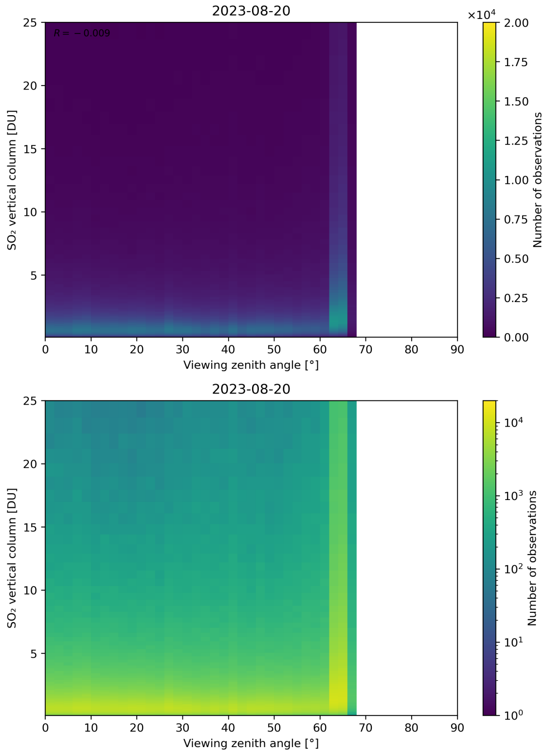
Figure 327: Scatter density plot of “Viewing zenith angle” against “SO 2 vertical column” for 2023-08-20 to 2023-08-21.
