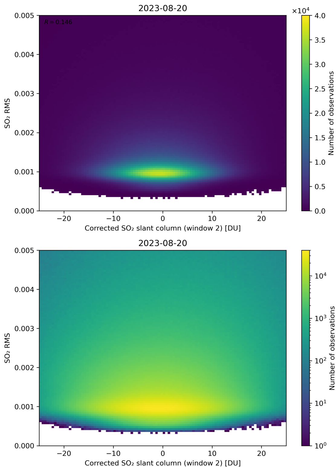
Figure 198: Scatter density plot of “Corrected SO 2 slant column (window 2)” against “SO 2 RMS” for 2023-08-20 to 2023-08-21.
