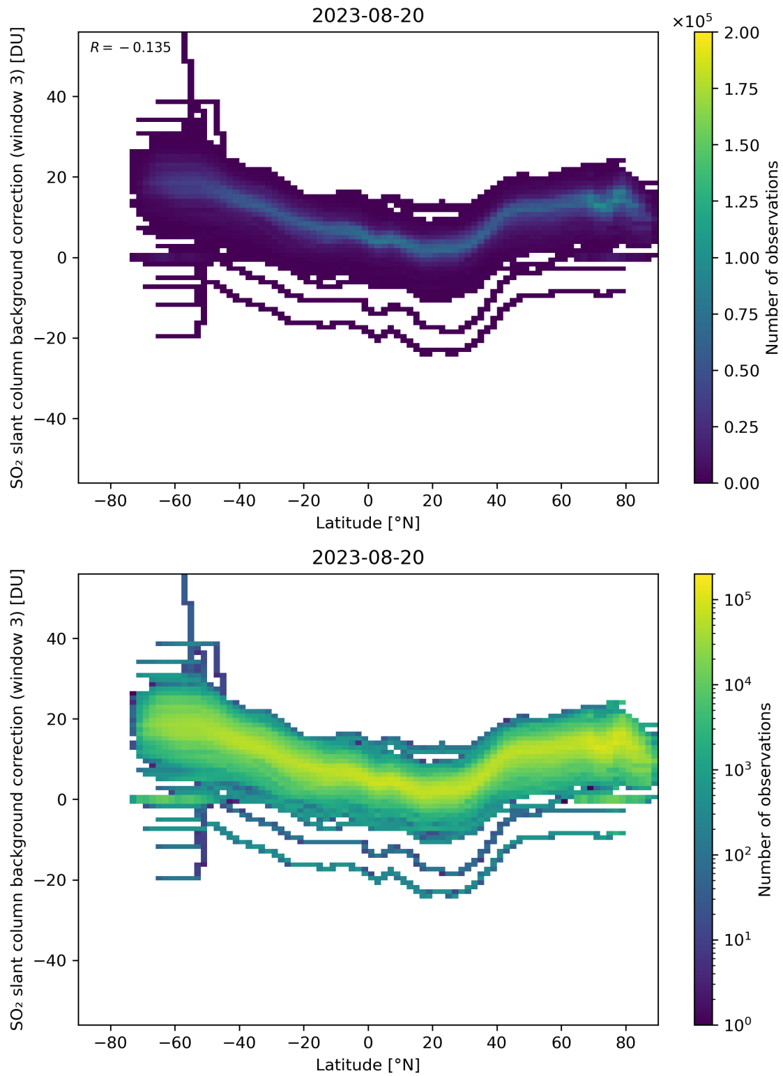
Figure 141: Scatter density plot of “Latitude” against “SO 2 slant column background correction (window 3)” for 2023-08-20 to 2023-08-21.
