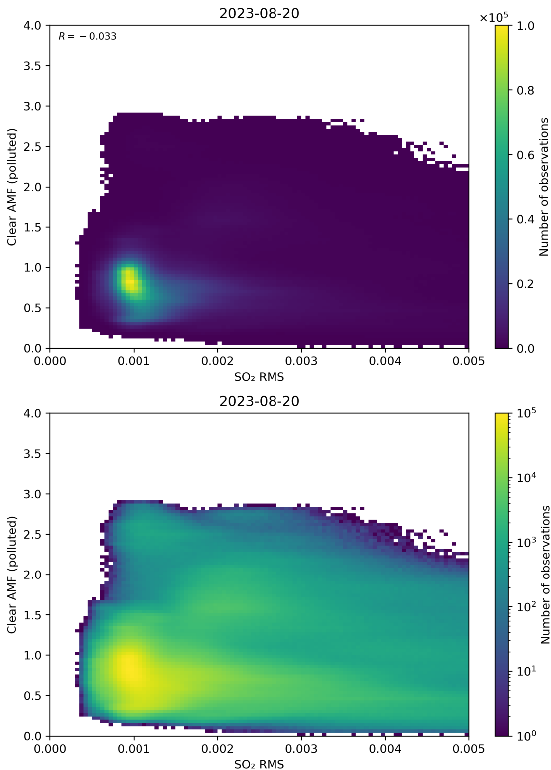
Figure 136: Scatter density plot of “SO 2 RMS” against “Clear AMF (polluted)” for 2023-08-20 to 2023-08-21.
