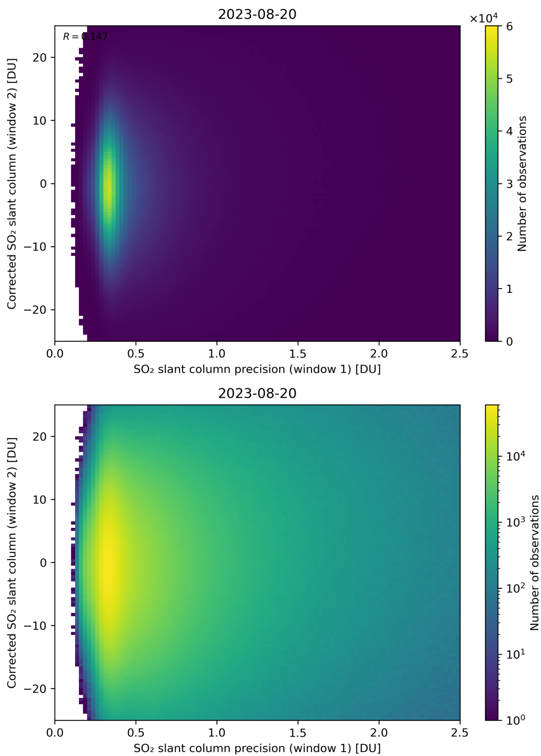
Figure 225: Scatter density plot of “SO 2 slant column precision (window 1)” against “Corrected SO 2 slant column (window 2)” for 2023-08-20 to 2023-08-21.
