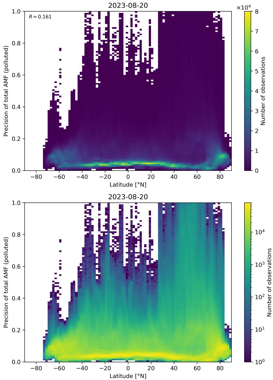
Figure 155: Scatter density plot of “Latitude” against “Precision of total AMF (polluted)” for 2023-08-20 to 2023-08-21.
