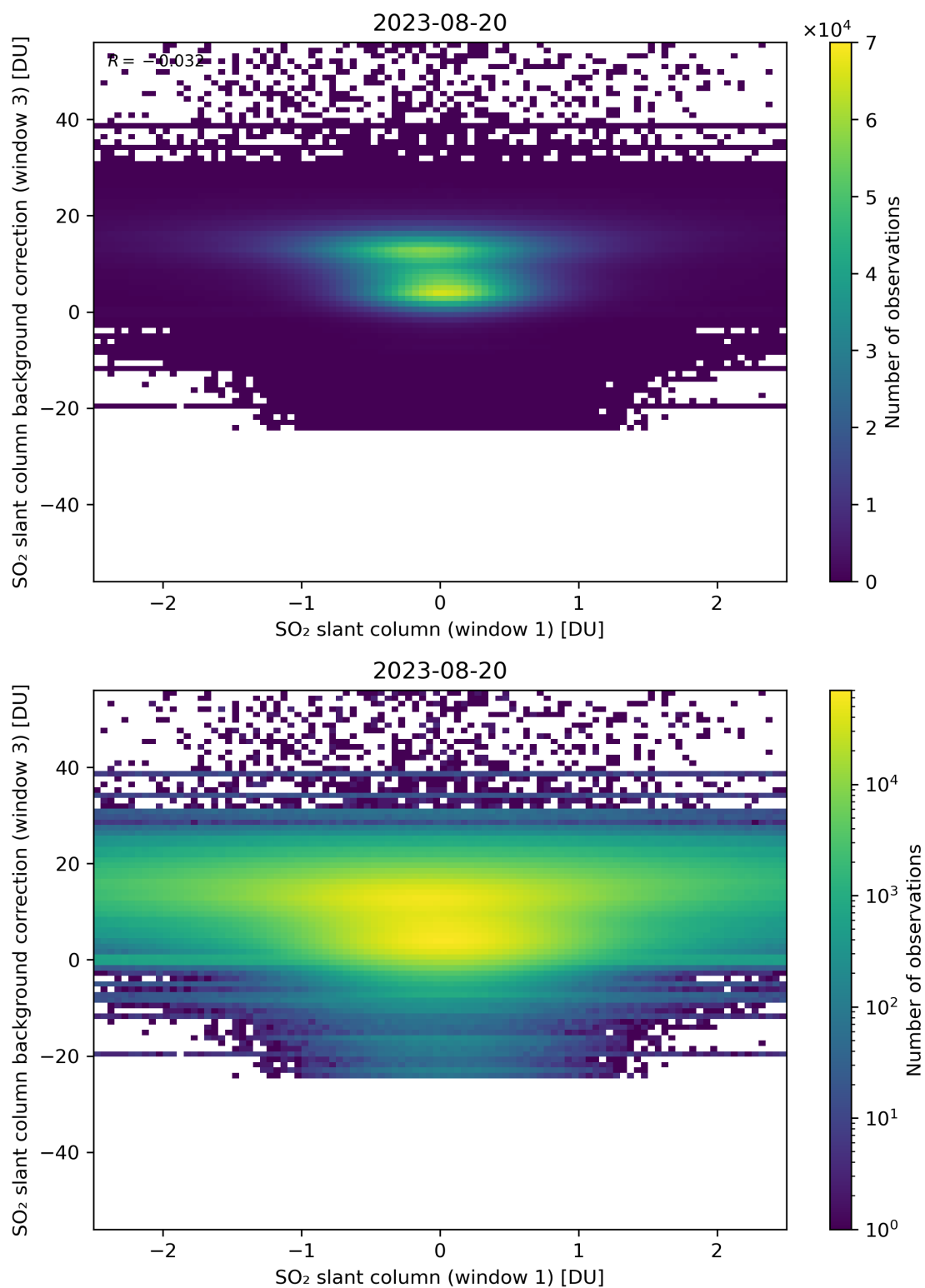
Figure 214: Scatter density plot of “SO 2 slant column (window 1)” against “SO 2 slant column background correction (window 3)” for 2023-08-20 to 2023-08-21.
