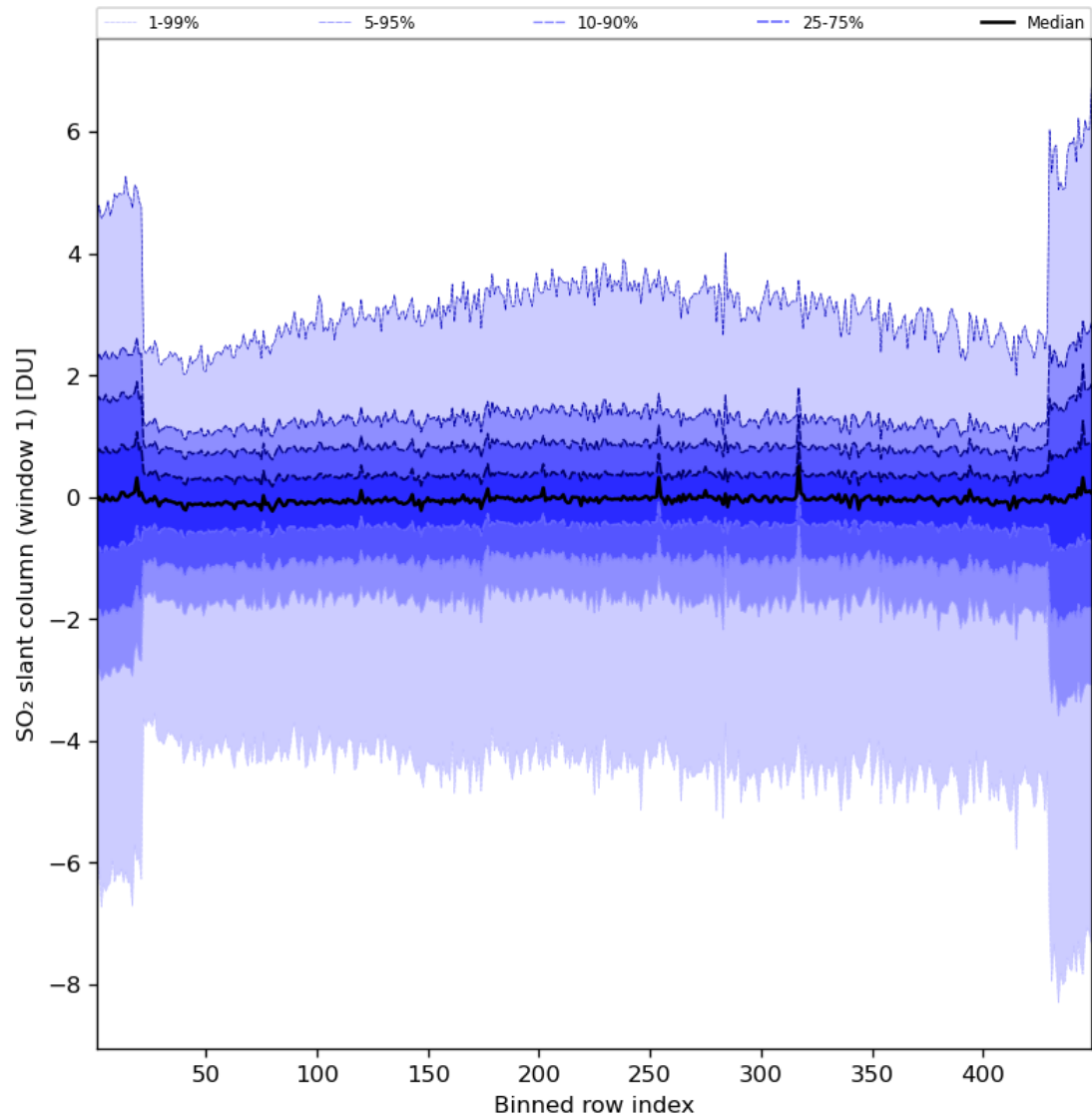
Figure 79: Along track statistics of “SO 2 slant column (window 1)” for 2023-08-20 to 2023-08-21
