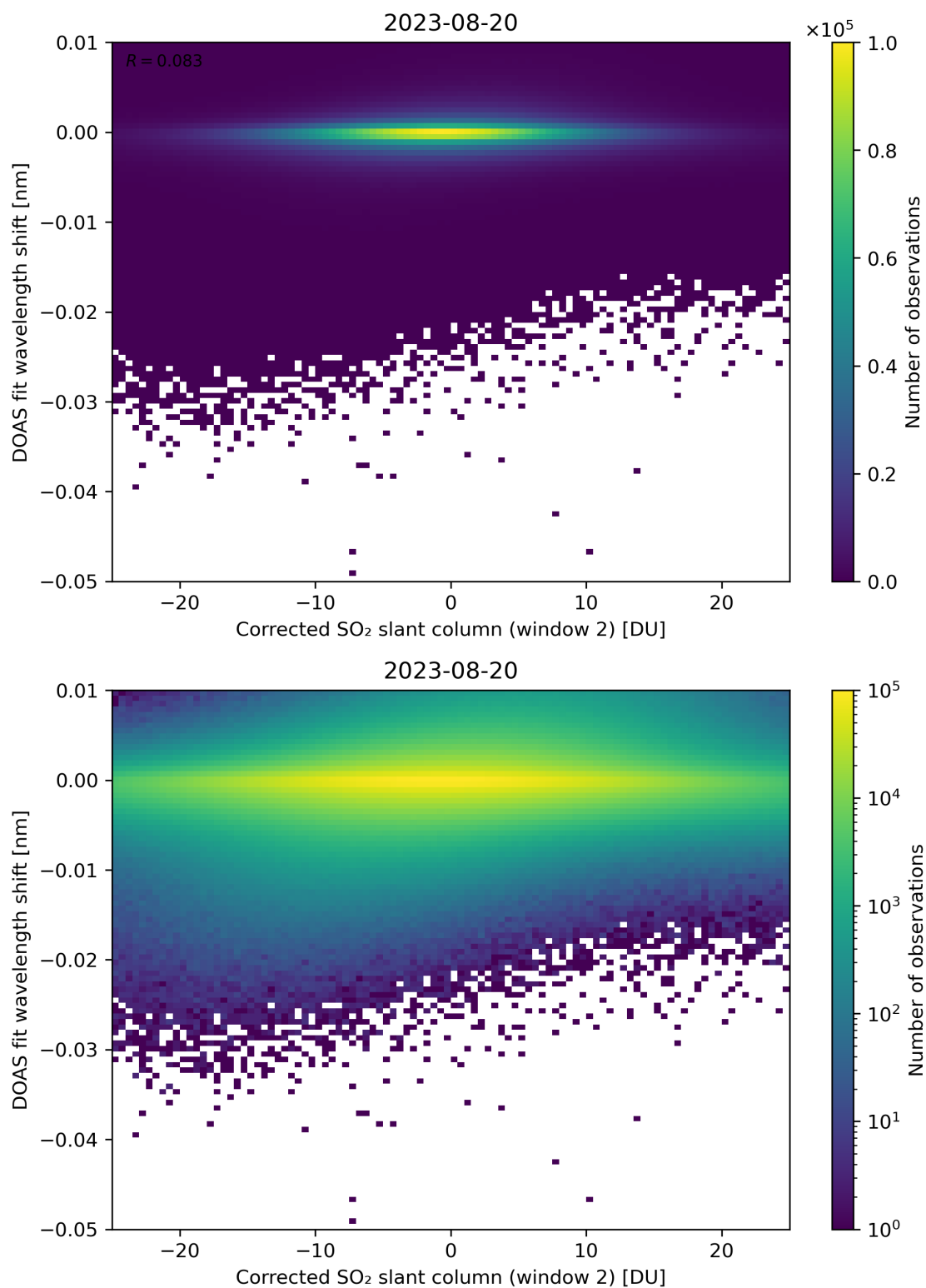
Figure 196: Scatter density plot of “Corrected SO 2 slant column (window 2)” against “DOAS fit wavelength shift” for 2023-08-20 to 2023-08-21.
