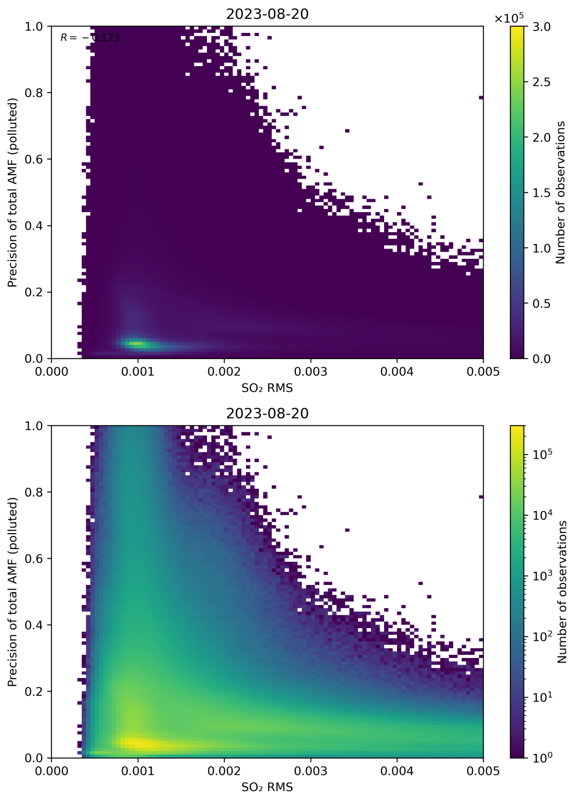
Figure 138: Scatter density plot of “SO 2 RMS” against “Precision of total AMF (polluted)” for 2023-08-20 to 2023-08-21.
