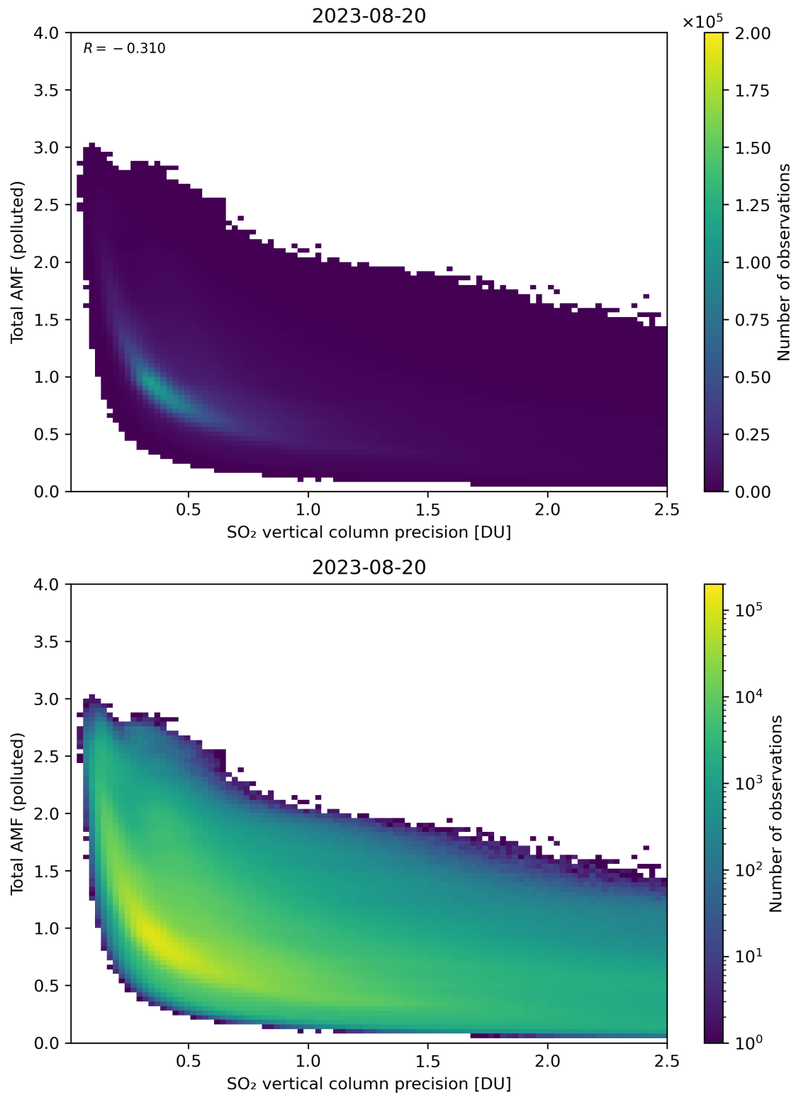
Figure 294: Scatter density plot of “SO 2 vertical column precision” against “Total AMF (polluted)” for 2023-08-20 to 2023-08-21.
