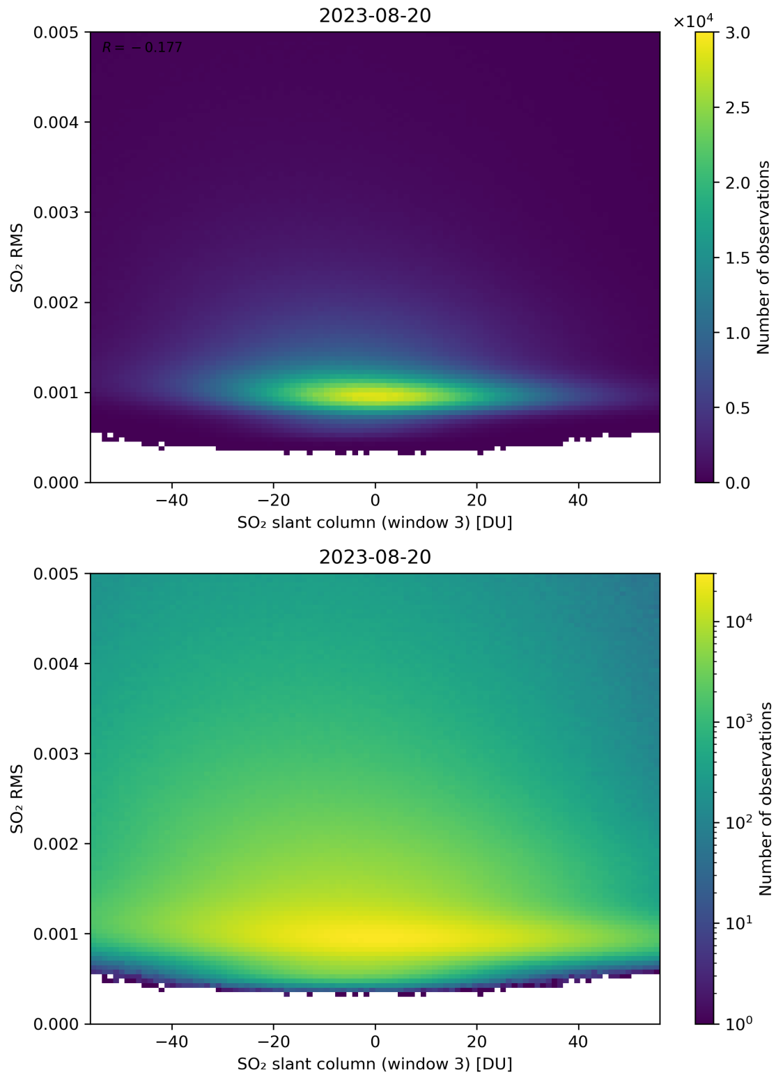
Figure 256: Scatter density plot of “SO 2 slant column (window 3)” against “SO 2 RMS” for 2023-08-20 to 2023-08-21.
