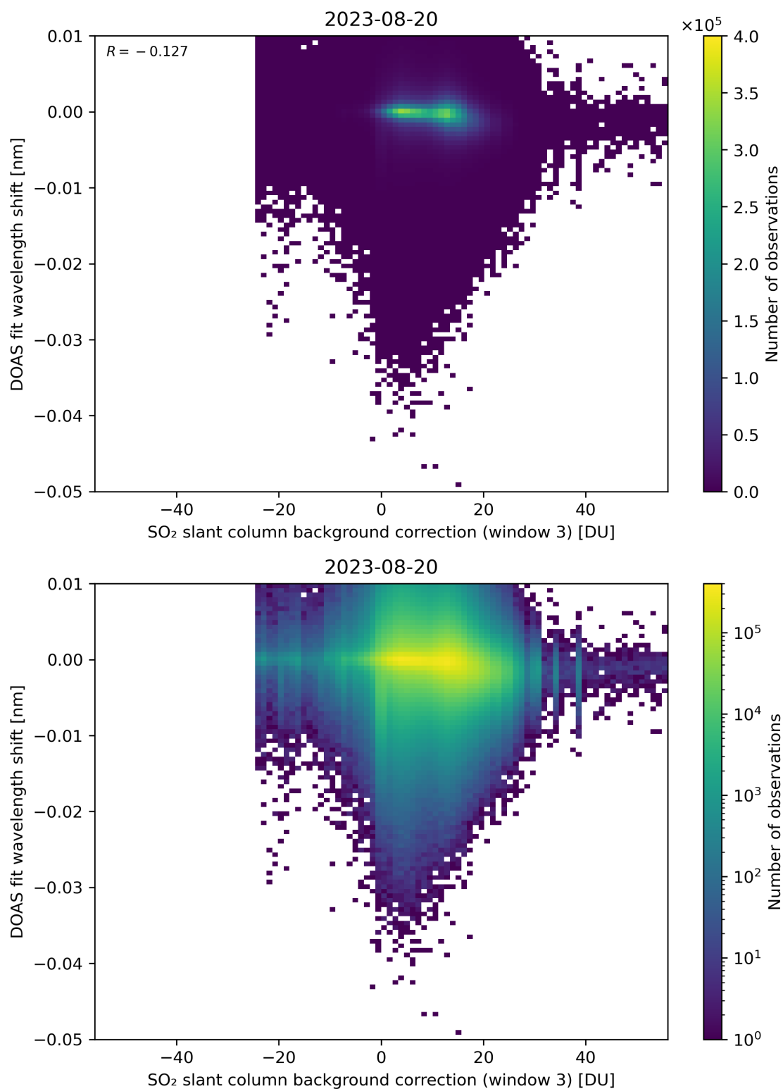
Figure 121: Scatter density plot of “SO 2 slant column background correction (window 3)” against “DOAS fit wavelength shift” for 2023-08-20 to 2023-08-21.
