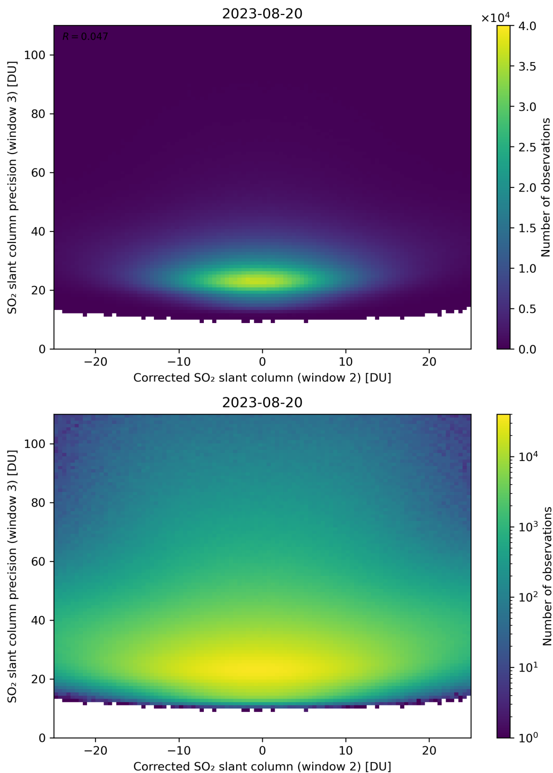
Figure 202: Scatter density plot of “Corrected SO 2 slant column (window 2)” against “SO 2 slant column precision (window 3)” for 2023-08-20 to 2023-08-21.
