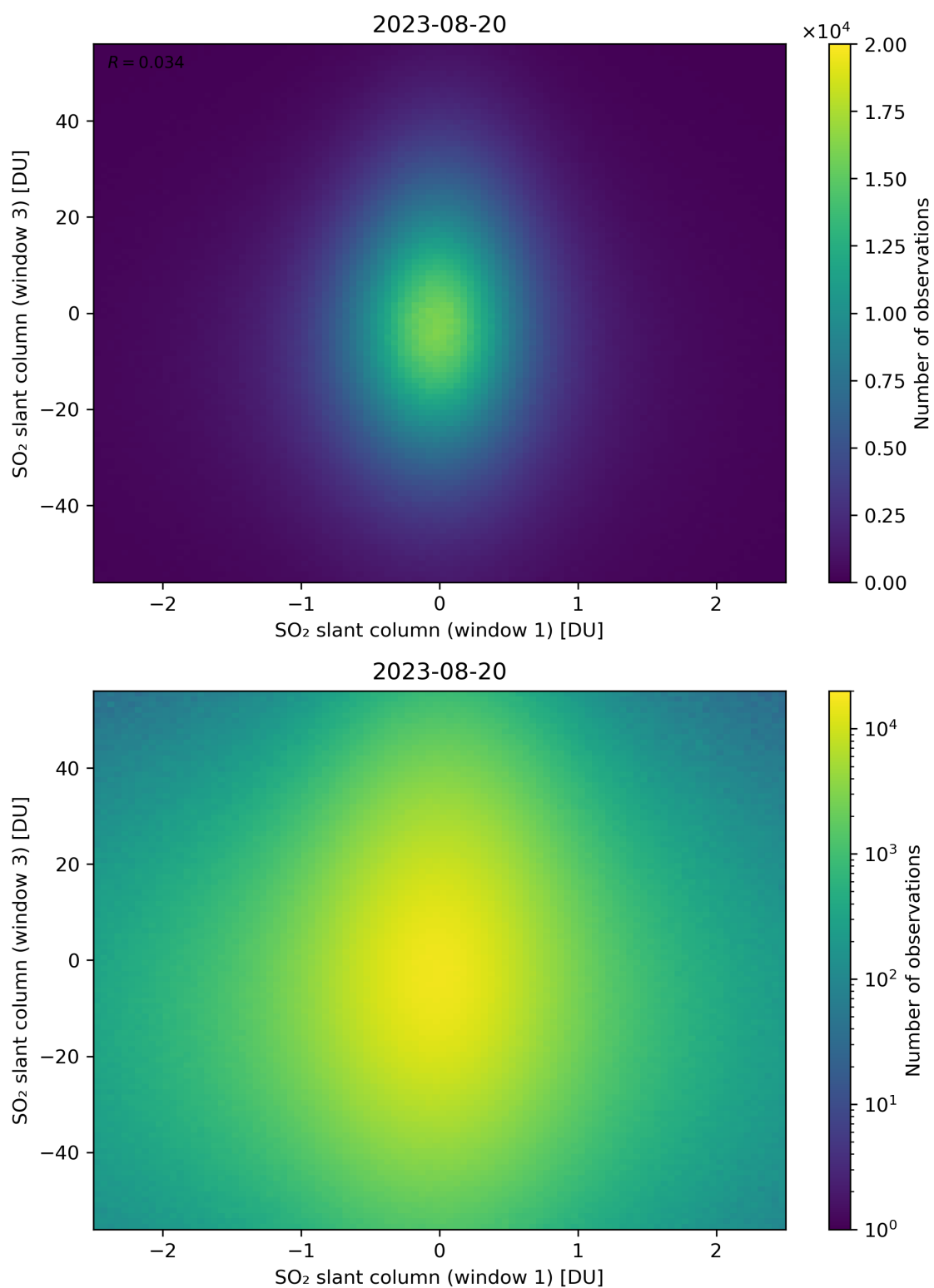
Figure 237: Scatter density plot of “SO 2 slant column (window 1)” against “SO 2 slant column (window 3)” for 2023-08-20 to 2023-08-21.
