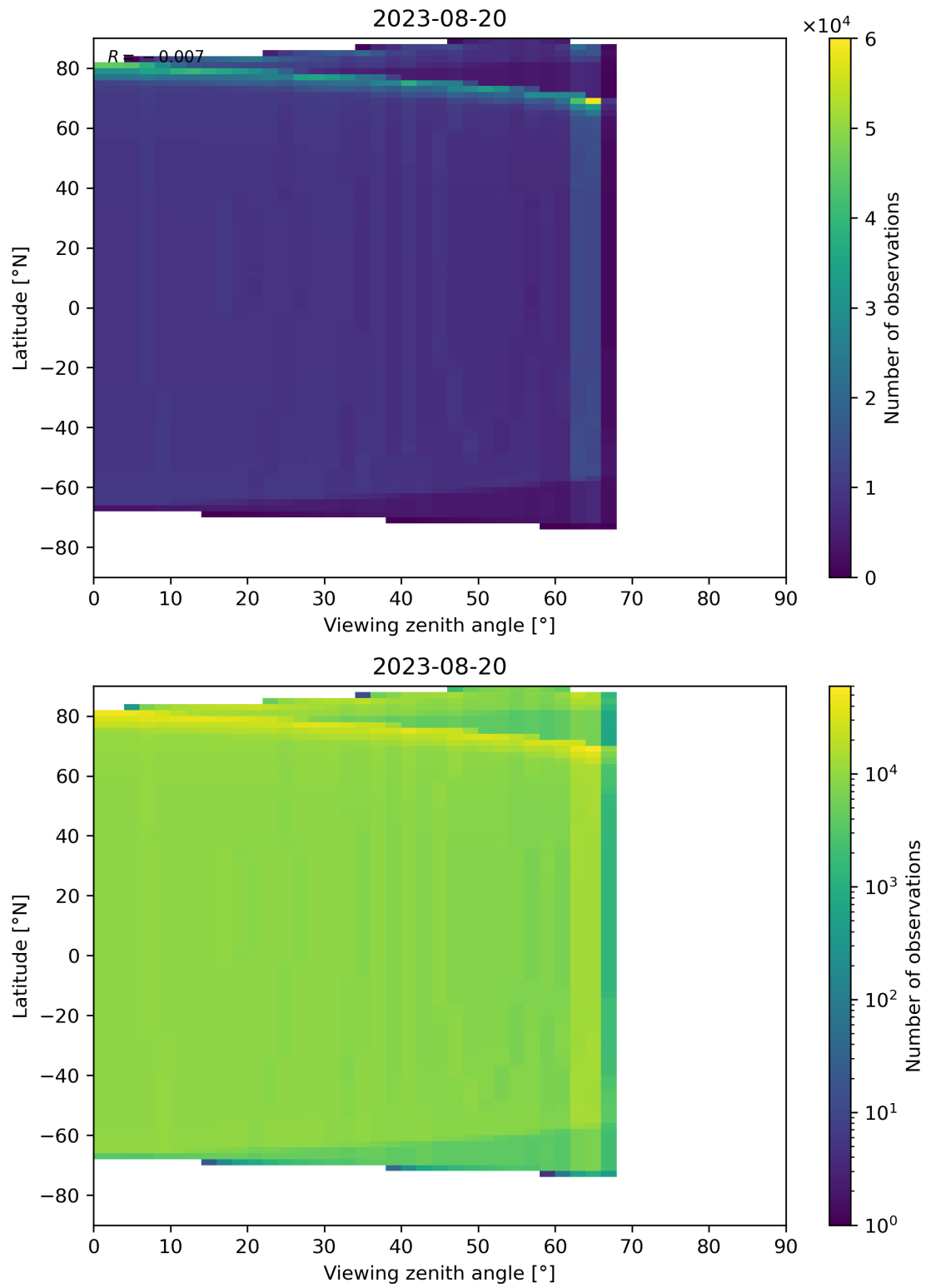
Figure 314: Scatter density plot of “Viewing zenith angle” against “Latitude” for 2023-08-20 to 2023-08-21.
