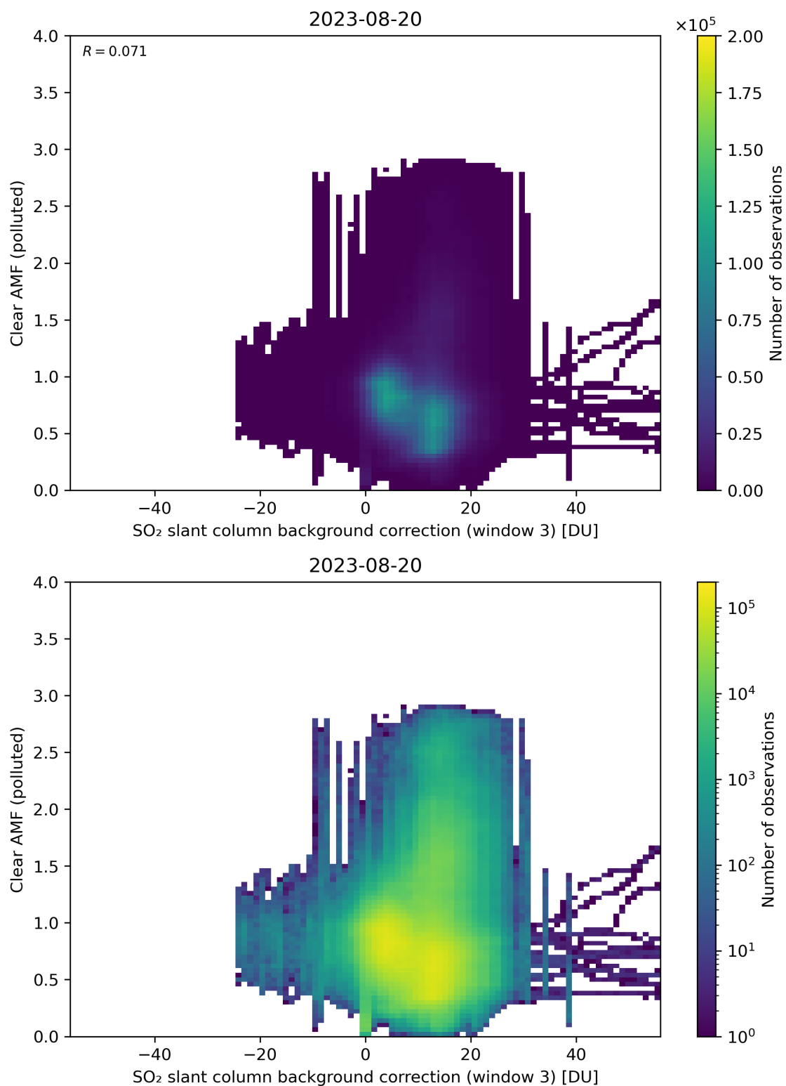
Figure 124: Scatter density plot of “SO 2 slant column background correction (window 3)” against “Clear AMF (polluted)” for 2023-08-20 to 2023-08-21.
