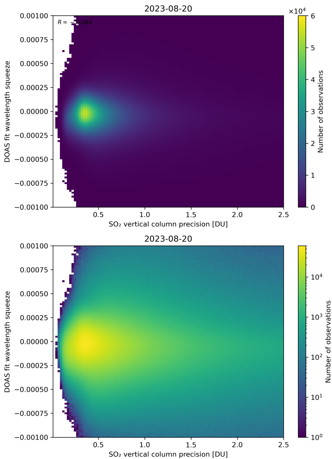
Figure 283: Scatter density plot of “SO 2 vertical column precision” against “DOAS fit wavelength squeeze” for 2023-08-20 to 2023-08-21.
