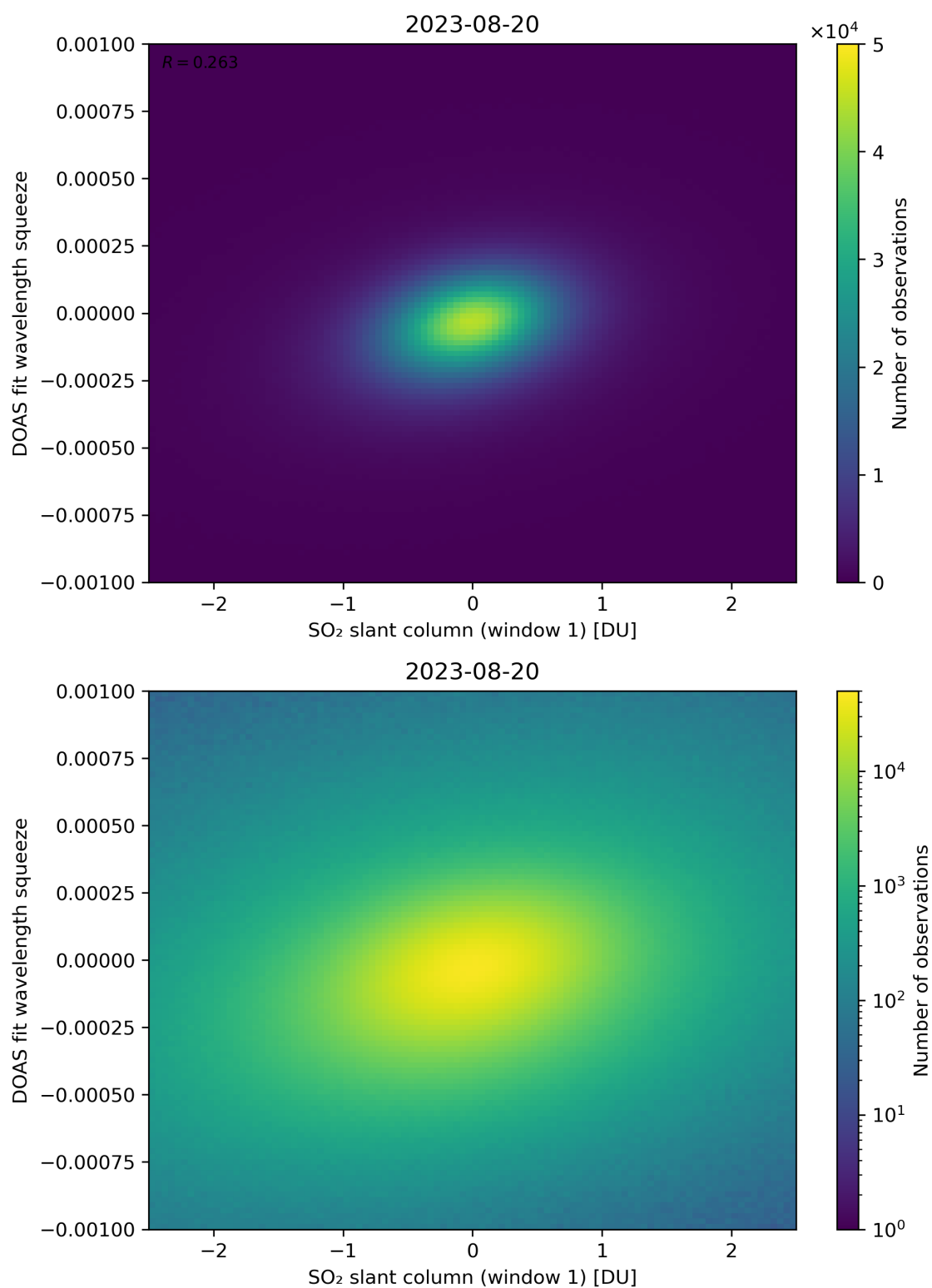
Figure 216: Scatter density plot of “SO 2 slant column (window 1)” against “DOAS fit wavelength squeeze” for 2023-08-20 to 2023-08-21.
