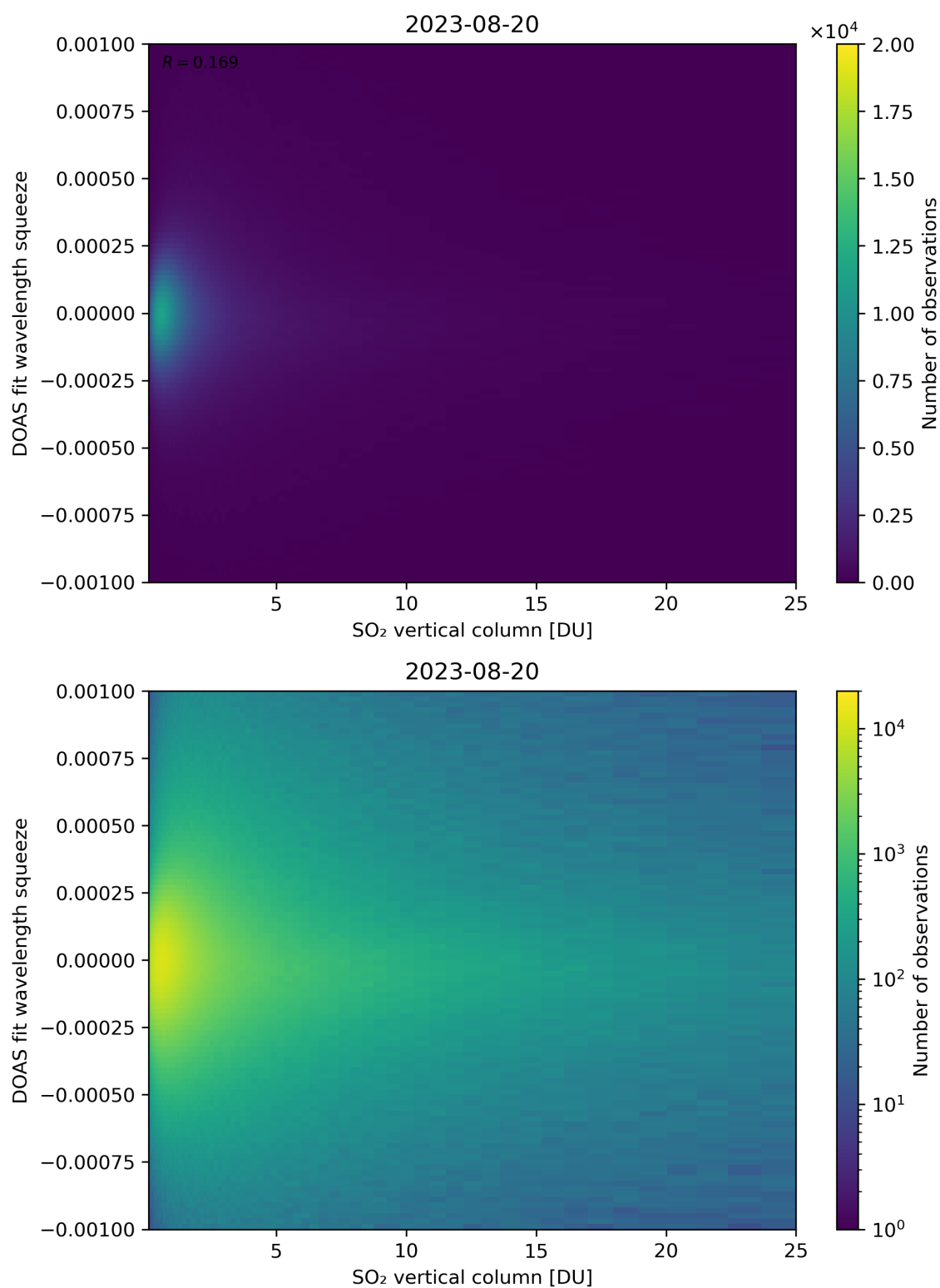
Figure 277: Scatter density plot of “SO 2 vertical column” against “DOAS fit wavelength squeeze” for 2023-08-20 to 2023-08-21.
