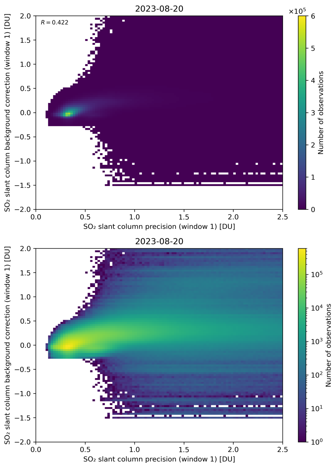
Figure 218: Scatter density plot of “SO 2 slant column precision (window 1)” against “SO 2 slant column background correction (window 1)” for 2023-08-20 to 2023-08-21.
