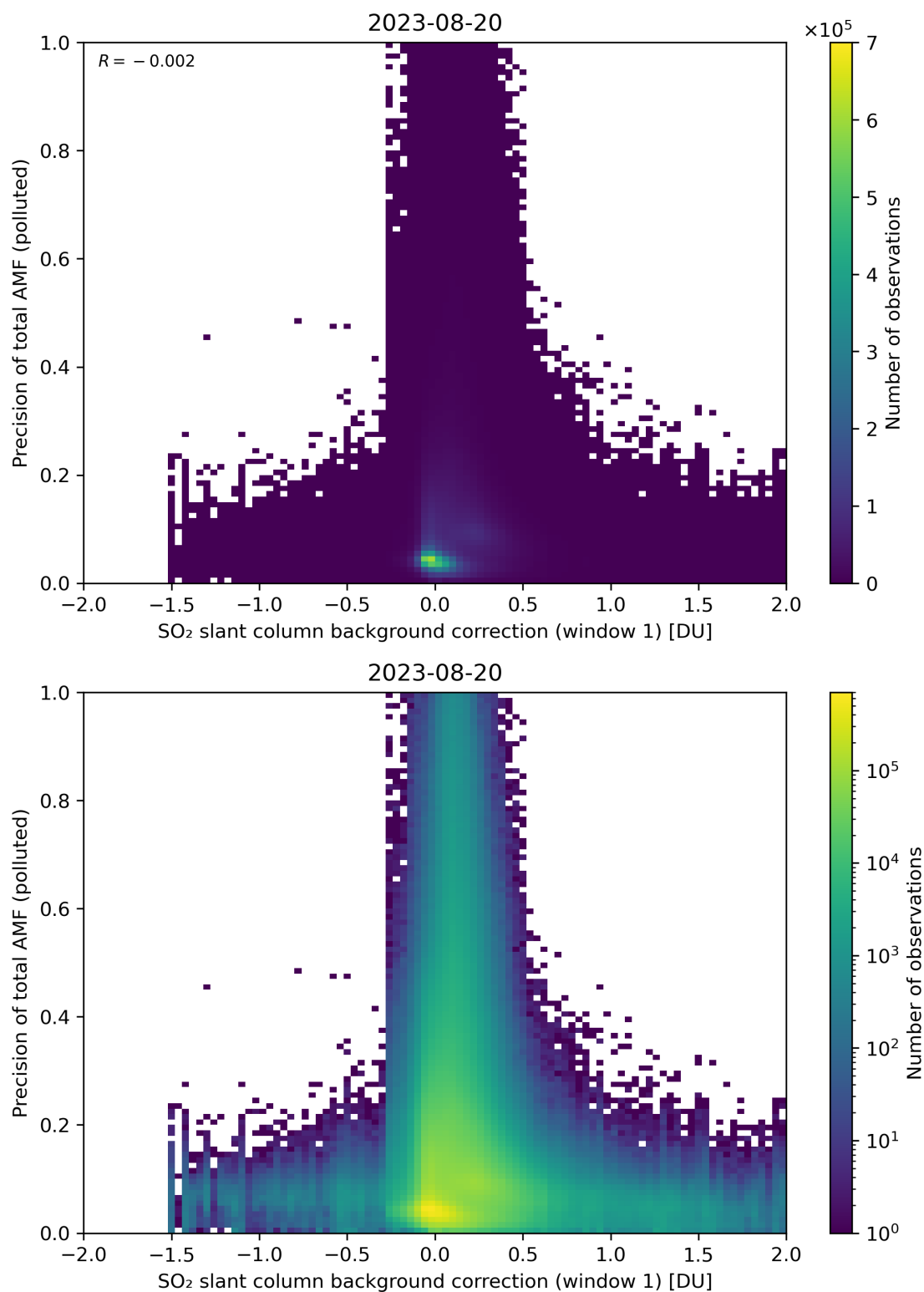
Figure 110: Scatter density plot of “SO 2 slant column background correction (window 1)” against “Precision of total AMF (polluted)” for 2023-08-20 to 2023-08-21.
