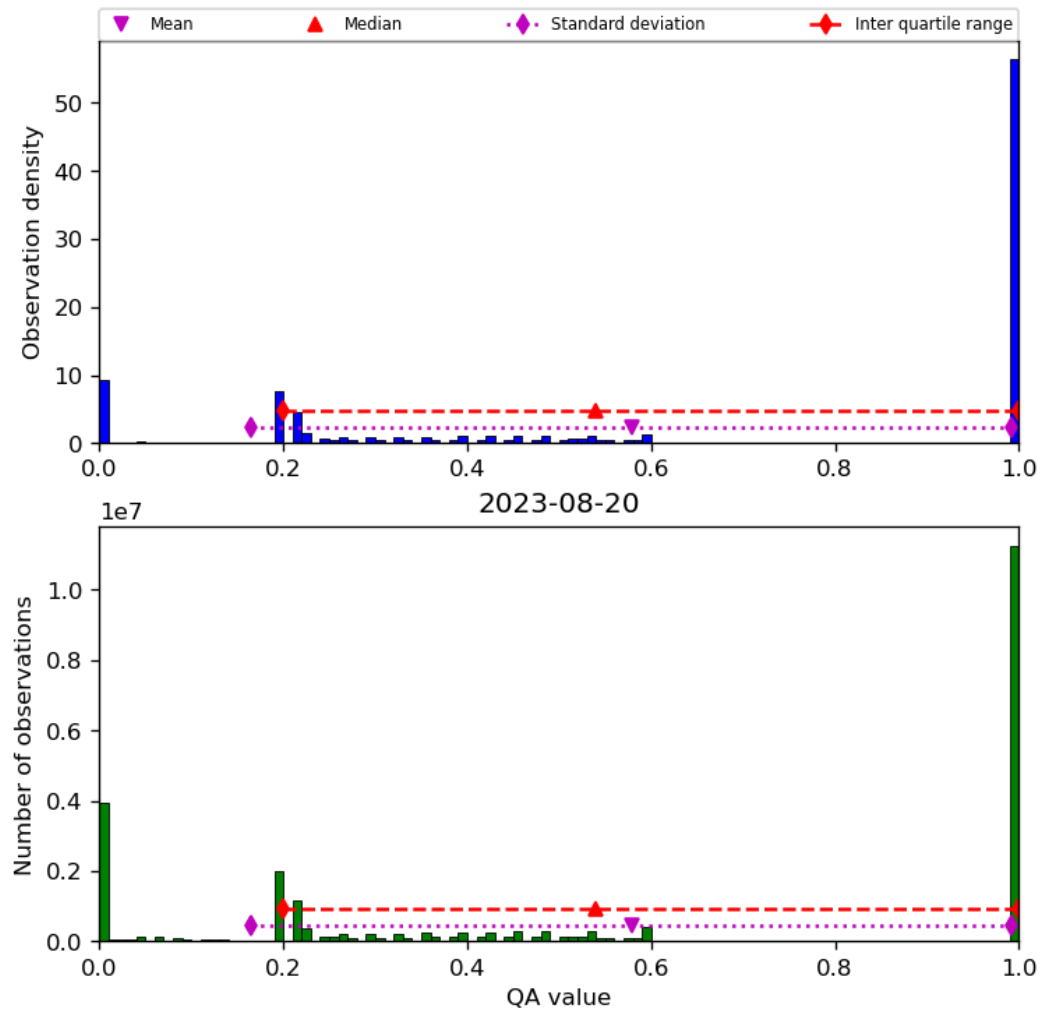
Figure 52: Histogram of “QA value” for 2023-08-20 to 2023-08-21
