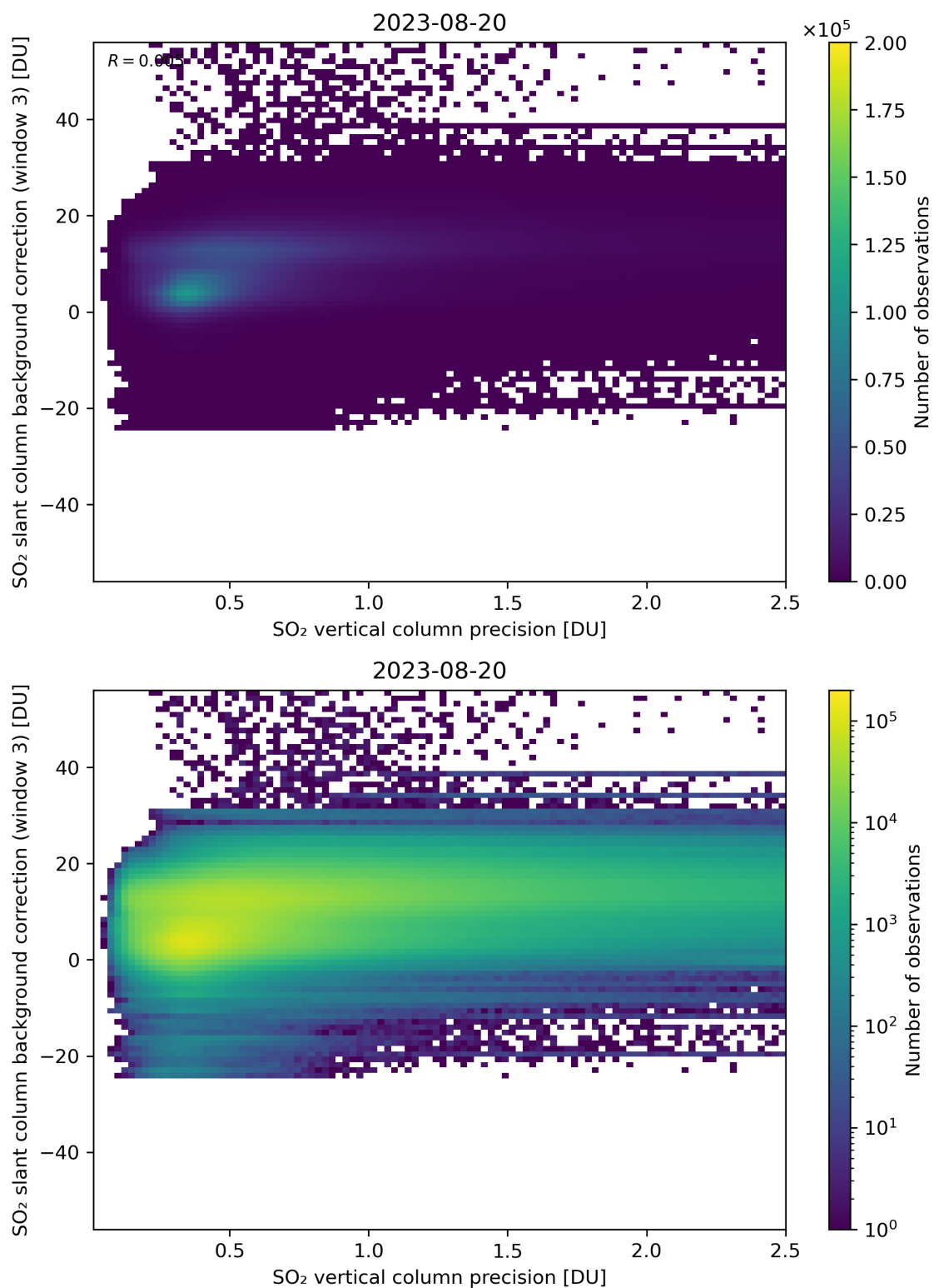
Figure 281: Scatter density plot of “SO 2 vertical column precision” against “SO 2 slant column background correction (window 3)” for 2023-08-20 to 2023-08-21.
