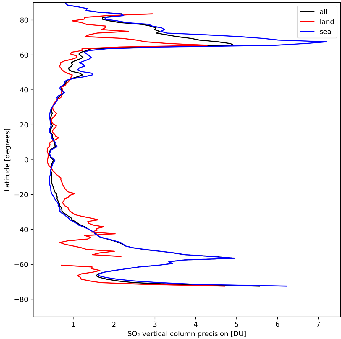
Figure 31: Zonal average of “SO 2 vertical column precision” for 2023-08-20 to 2023-08-21.
