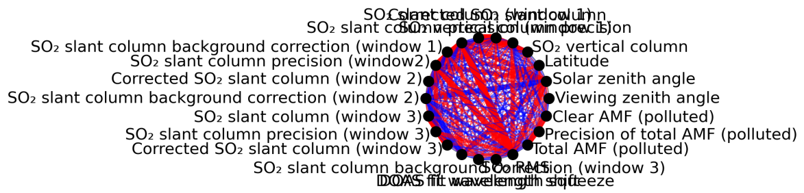
Figure 1: Map of correlation graph for 2023-08-20 to 2023-08-21.
