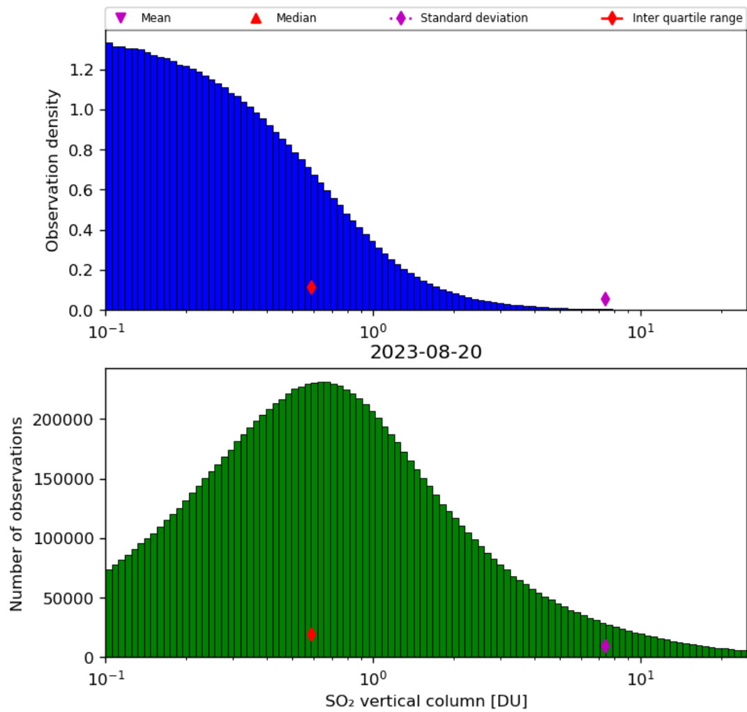
Figure 53: Histogram of “SO 2 vertical column” for 2023-08-20 to 2023-08-21
