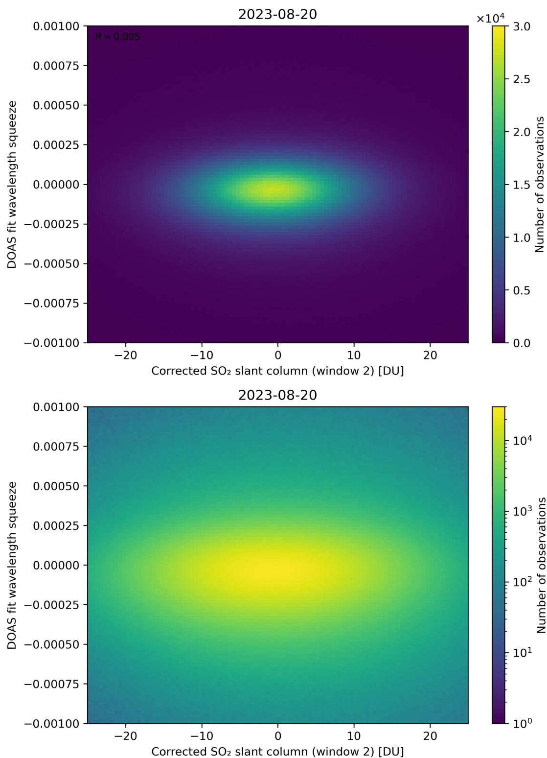
Figure 197: Scatter density plot of “Corrected SO 2 slant column (window 2)” against “DOAS fit wavelength squeeze” for 2023-08-20 to 2023-08-21.
