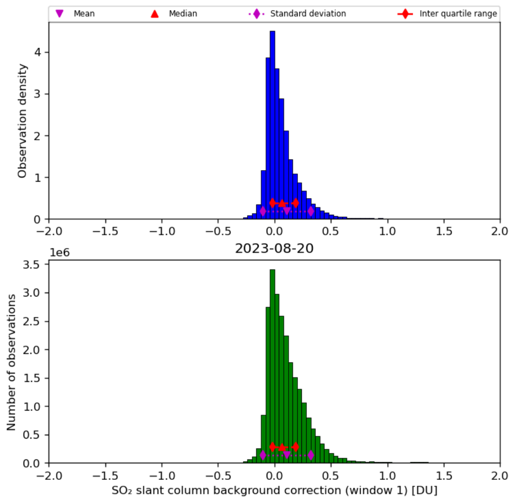
Figure 59: Histogram of “SO 2 slant column background correction (window 1)” for 2023-08-20 to 2023-08-21
