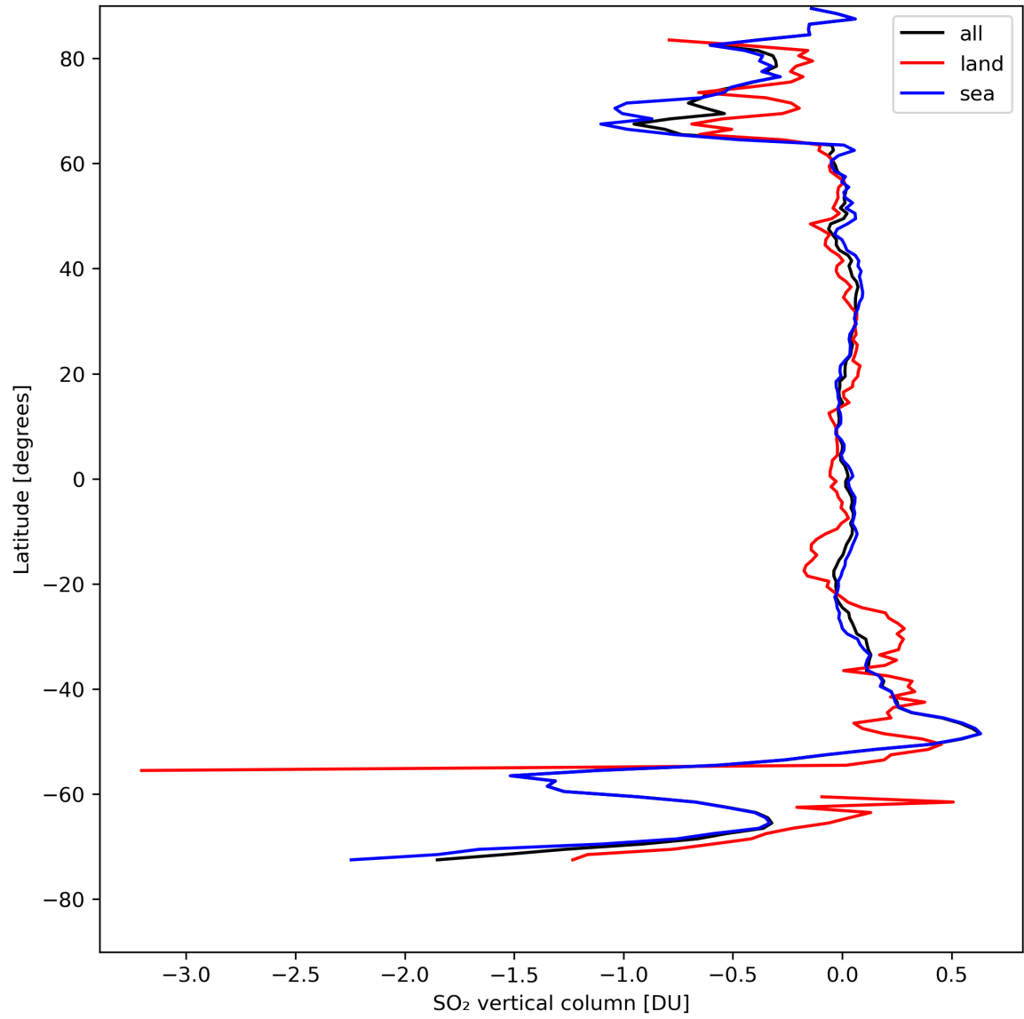
Figure 30: Zonal average of “SO 2 vertical column” for 2023-08-20 to 2023-08-21.
