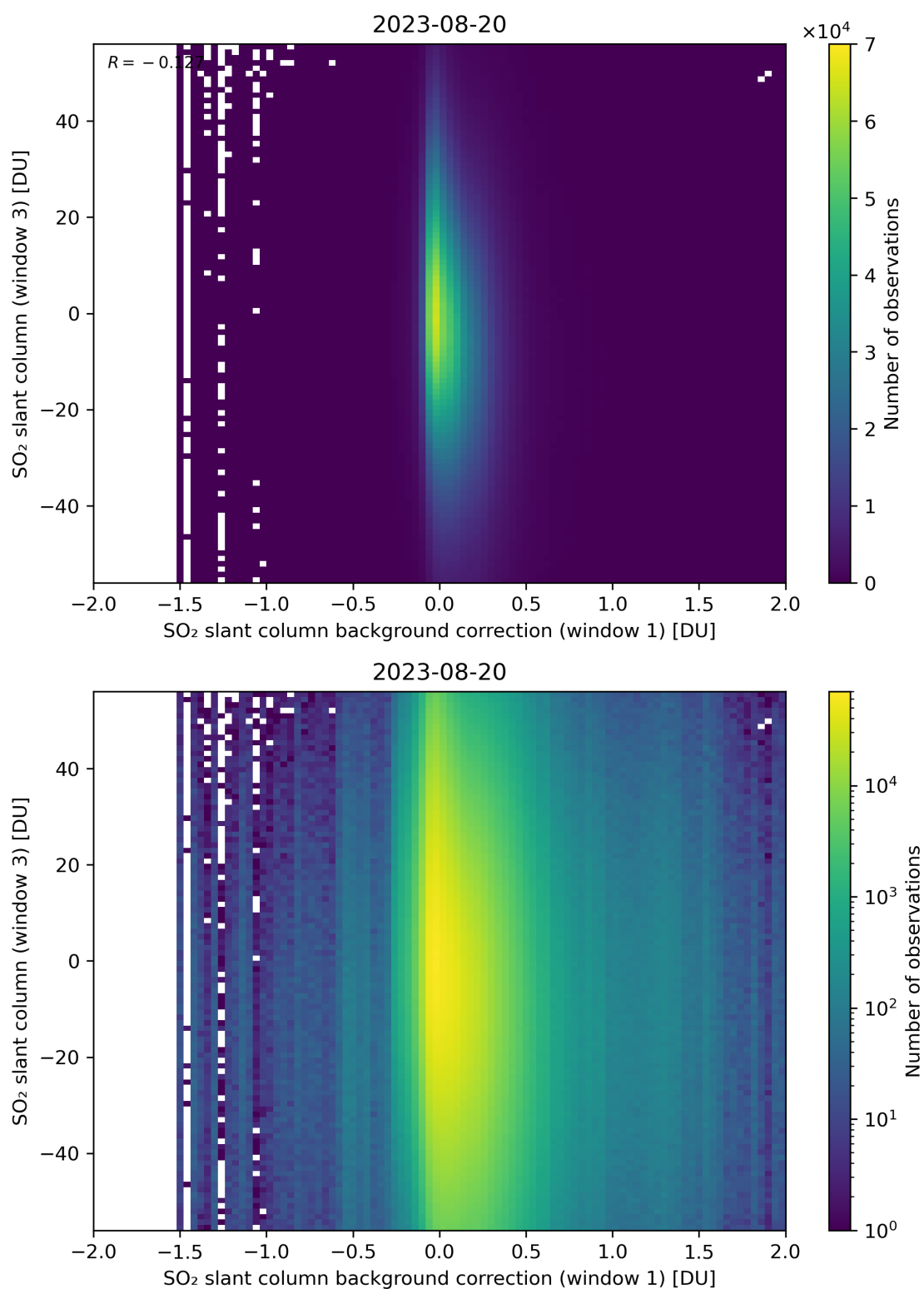
Figure 107: Scatter density plot of “SO 2 slant column background correction (window 1)” against “SO 2 slant column (window 3)” for 2023-08-20 to 2023-08-21.
