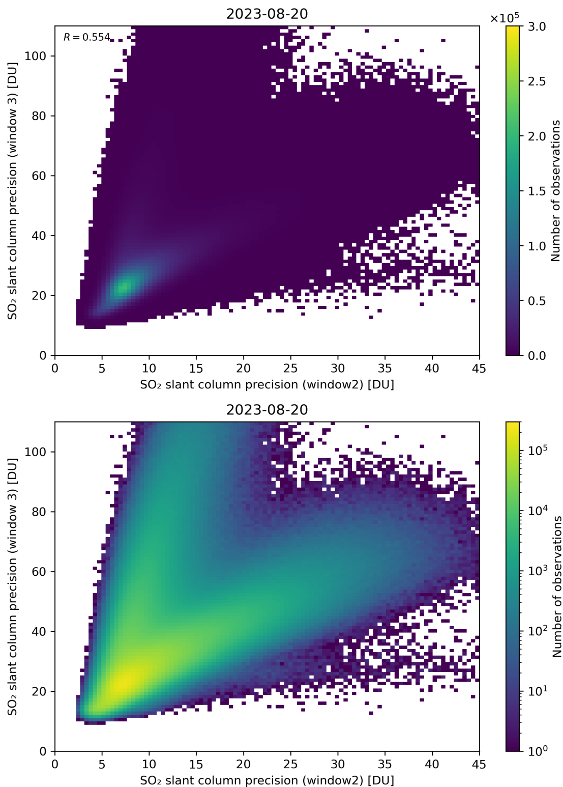
Figure 250: Scatter density plot of “SO 2 slant column precision (window2)” against “SO 2 slant column precision (window 3)” for 2023-08-20 to 2023-08-21.
