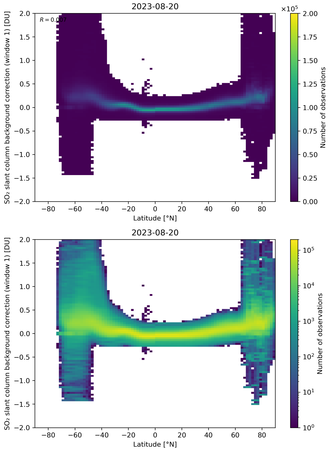
Figure 139: Scatter density plot of “Latitude” against “SO 2 slant column background correction (window 1)” for 2023-08-20 to 2023-08-21.
