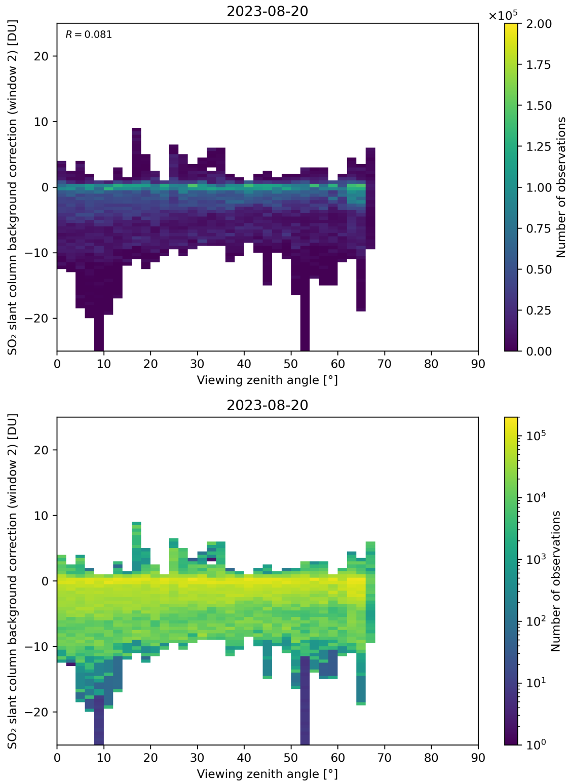
Figure 309: Scatter density plot of “Viewing zenith angle” against “SO 2 slant column background correction (window 2)” for 2023-08-20 to 2023-08-21.
