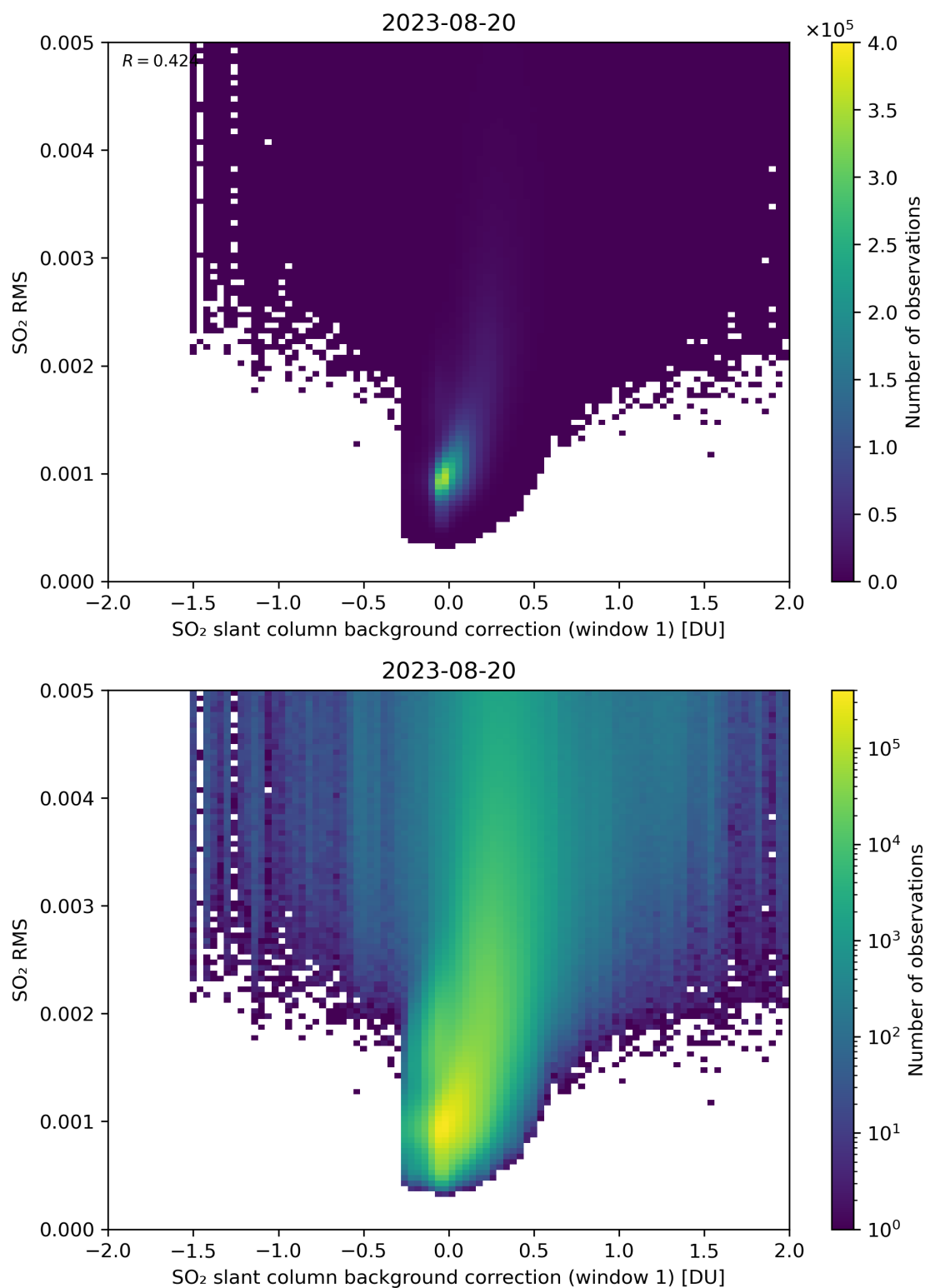
Figure 102: Scatter density plot of “SO 2 slant column background correction (window 1)” against “SO 2 RMS” for 2023-08-20 to 2023-08-21.
