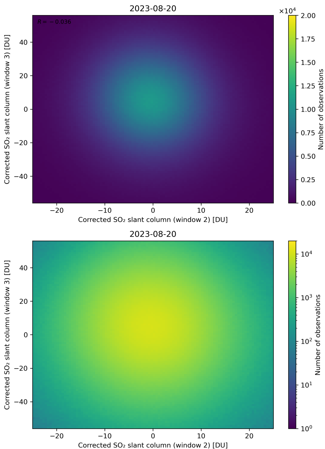
Figure 200: Scatter density plot of “Corrected SO 2 slant column (window 2)” against “Corrected SO 2 slant column (window 3)” for 2023-08-20 to 2023-08-21.
