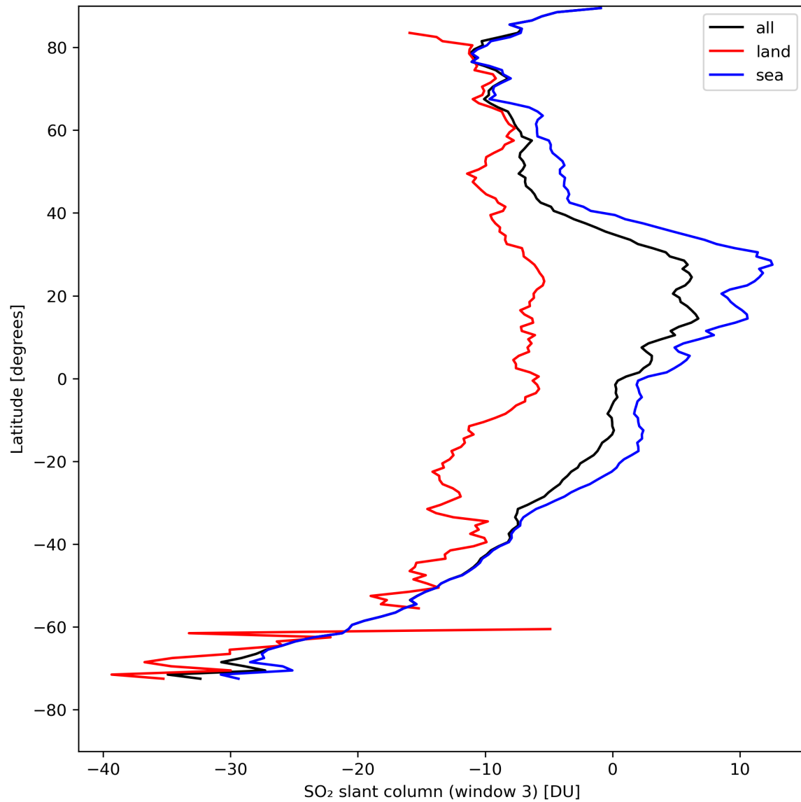
Figure 41: Zonal average of “SO 2 slant column (window 3)” for 2023-08-20 to 2023-08-21.
