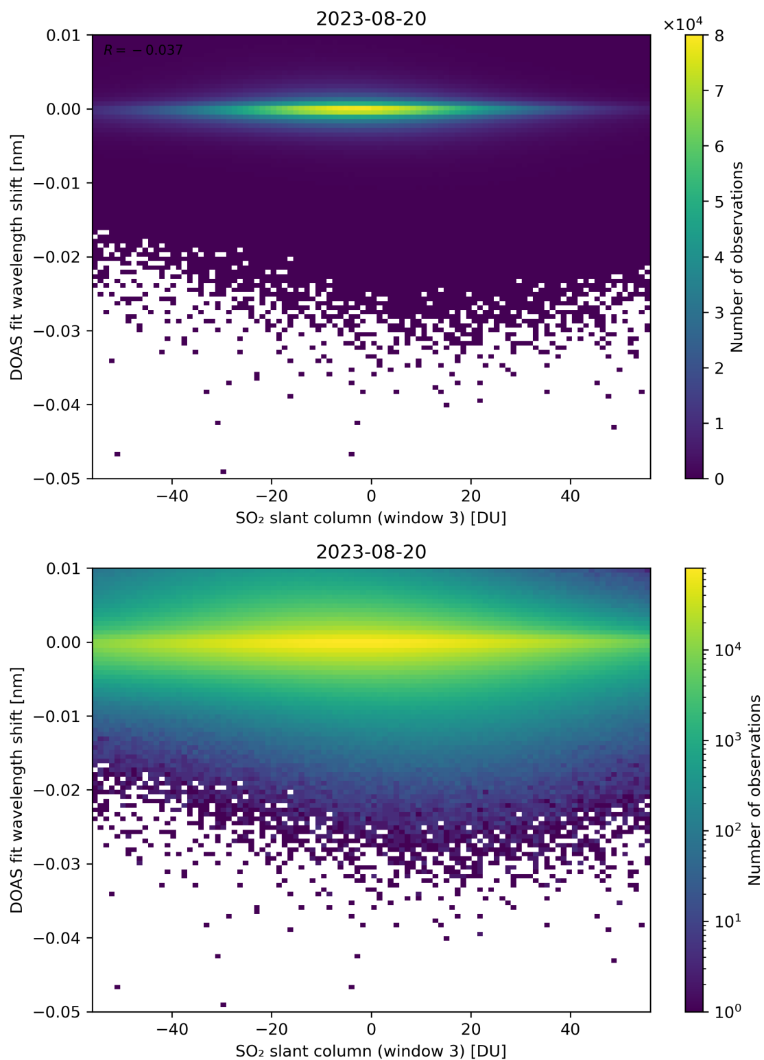
Figure 254: Scatter density plot of “SO 2 slant column (window 3)” against “DOAS fit wavelength shift” for 2023-08-20 to 2023-08-21.
