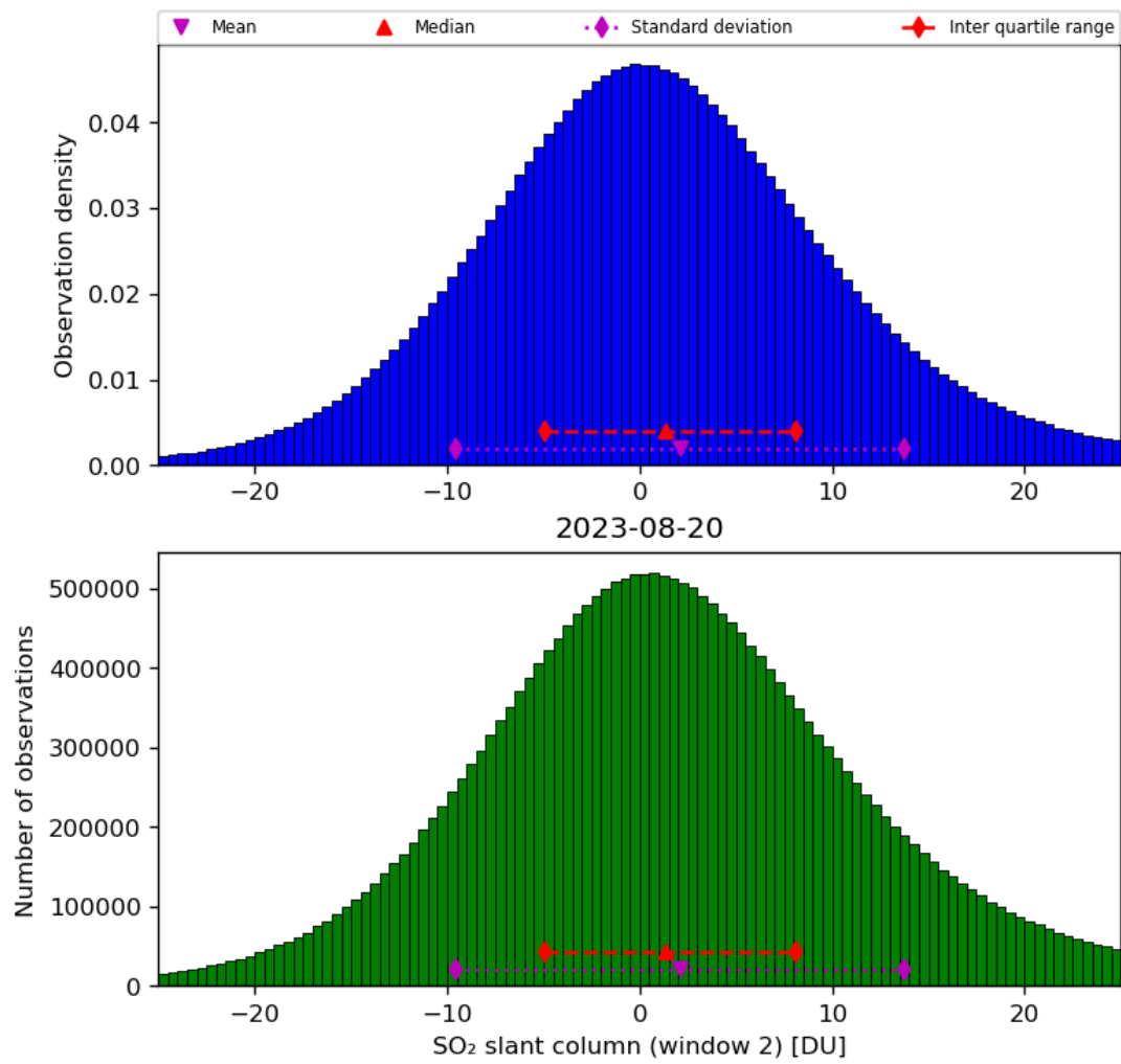
Figure 60: Histogram of “SO 2 slant column (window 2)” for 2023-08-20 to 2023-08-21
