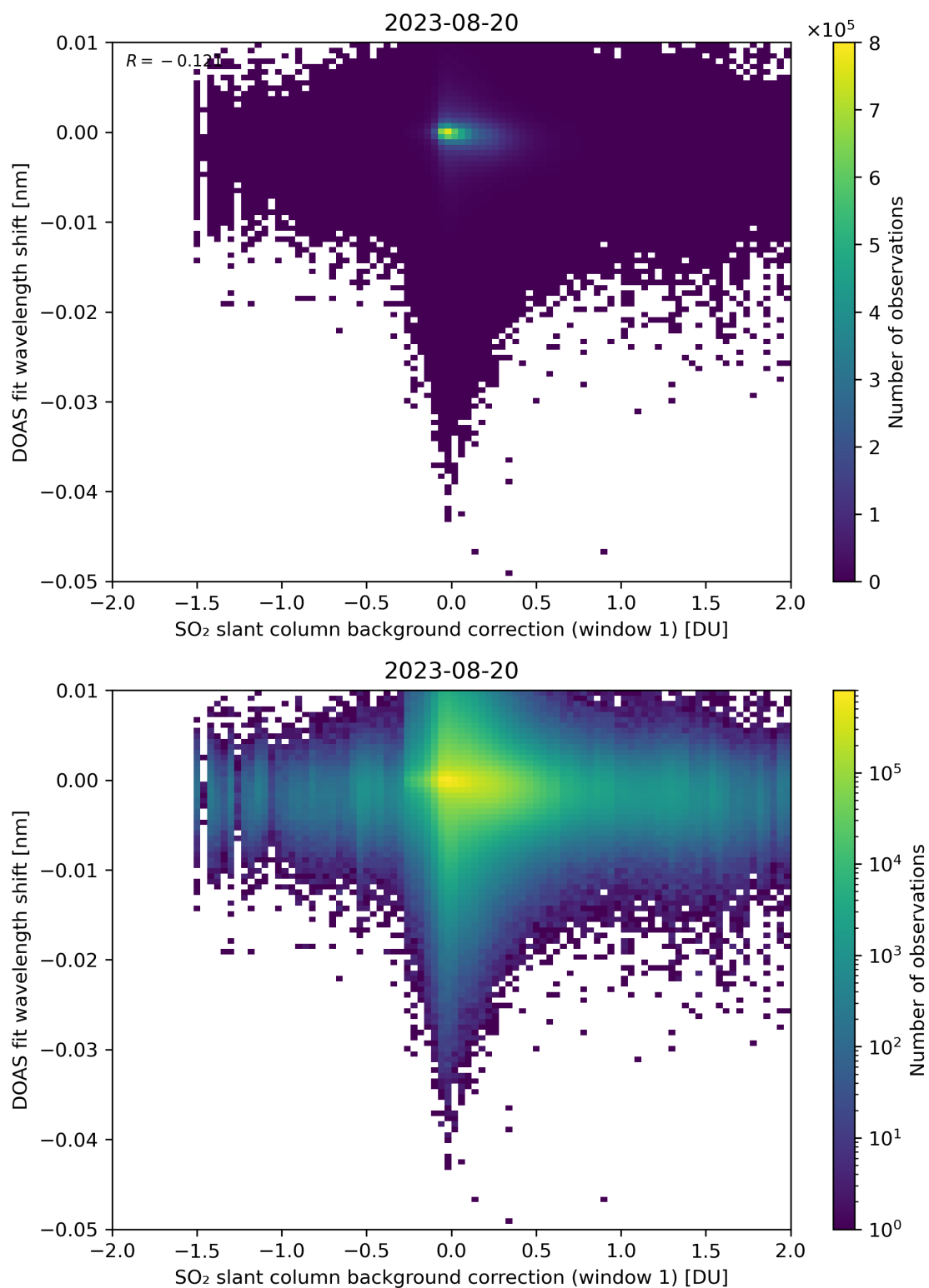
Figure 100: Scatter density plot of “SO 2 slant column background correction (window 1)” against “DOAS fit wavelength shift” for 2023-08-20 to 2023-08-21.
