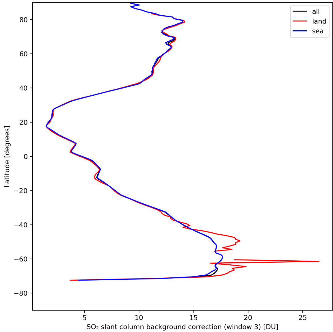
Figure 44: Zonal average of “SO 2 slant column background correction (window 3)” for 2023-08-20 to 2023-08-21.
