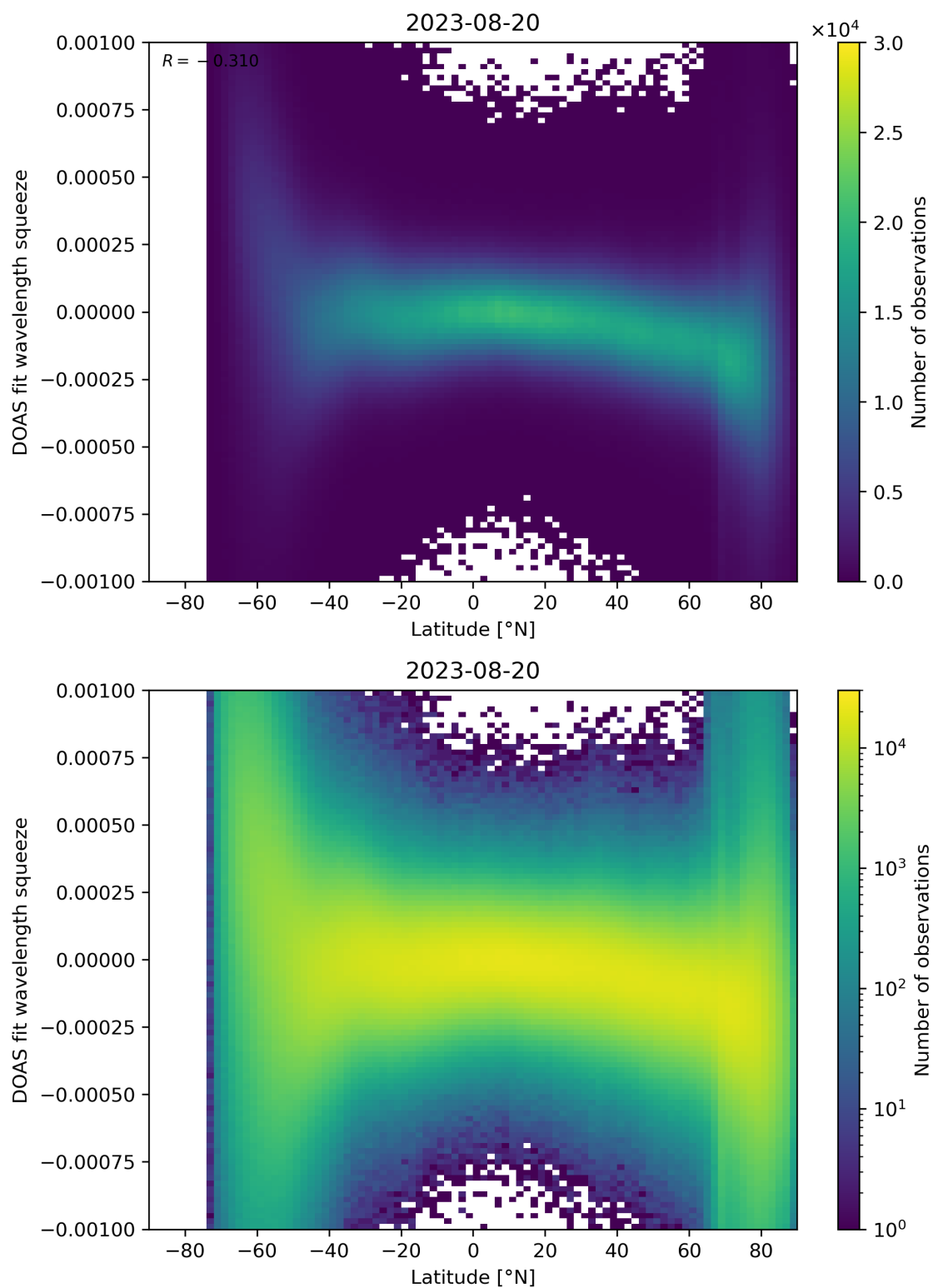
Figure 143: Scatter density plot of “Latitude” against “DOAS fit wavelength squeeze” for 2023-08-20 to 2023-08-21.
