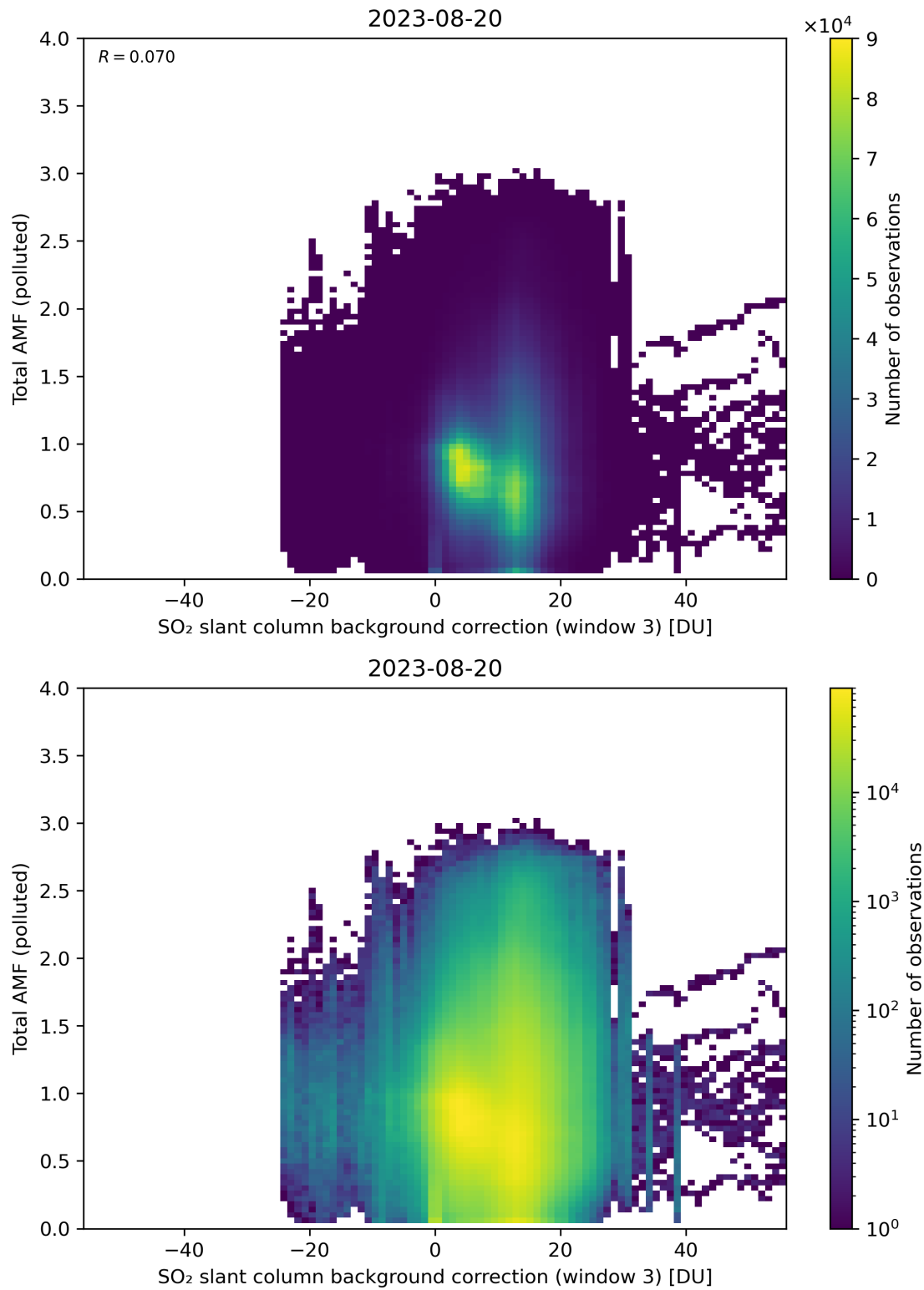
Figure 125: Scatter density plot of “SO 2 slant column background correction (window 3)” against “Total AMF (polluted)” for 2023-08-20 to 2023-08-21.
