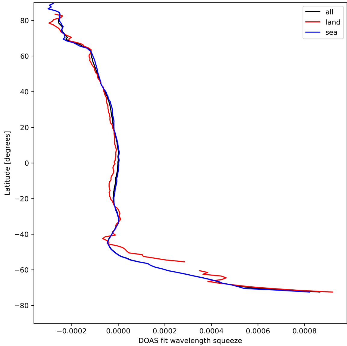
Figure 46: Zonal average of “DOAS fit wavelength squeeze” for 2023-08-20 to 2023-08-21.
