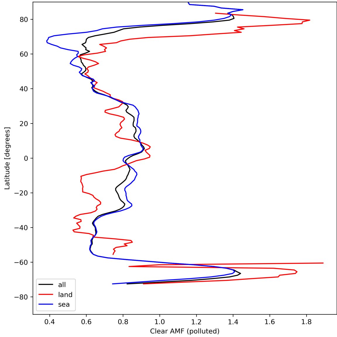
Figure 50: Zonal average of “Clear AMF (polluted)” for 2023-08-20 to 2023-08-21.
