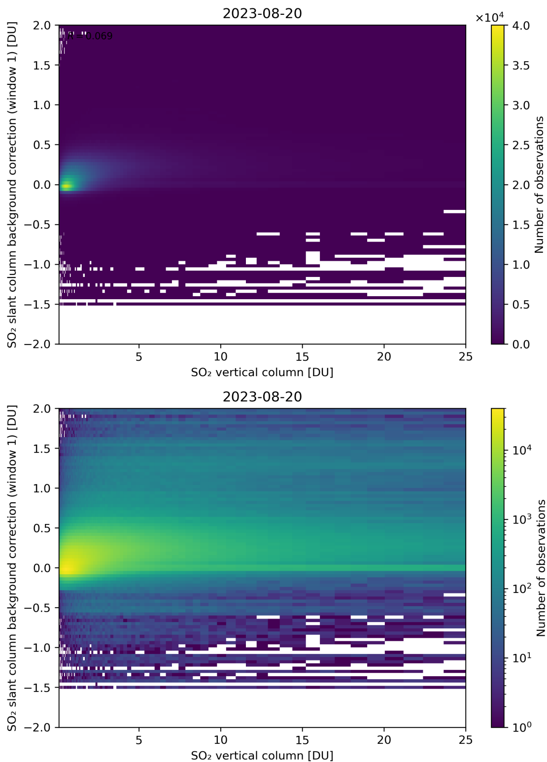
Figure 273: Scatter density plot of “SO 2 vertical column” against “SO 2 slant column background correction (window 1)” for 2023-08-20 to 2023-08-21.
