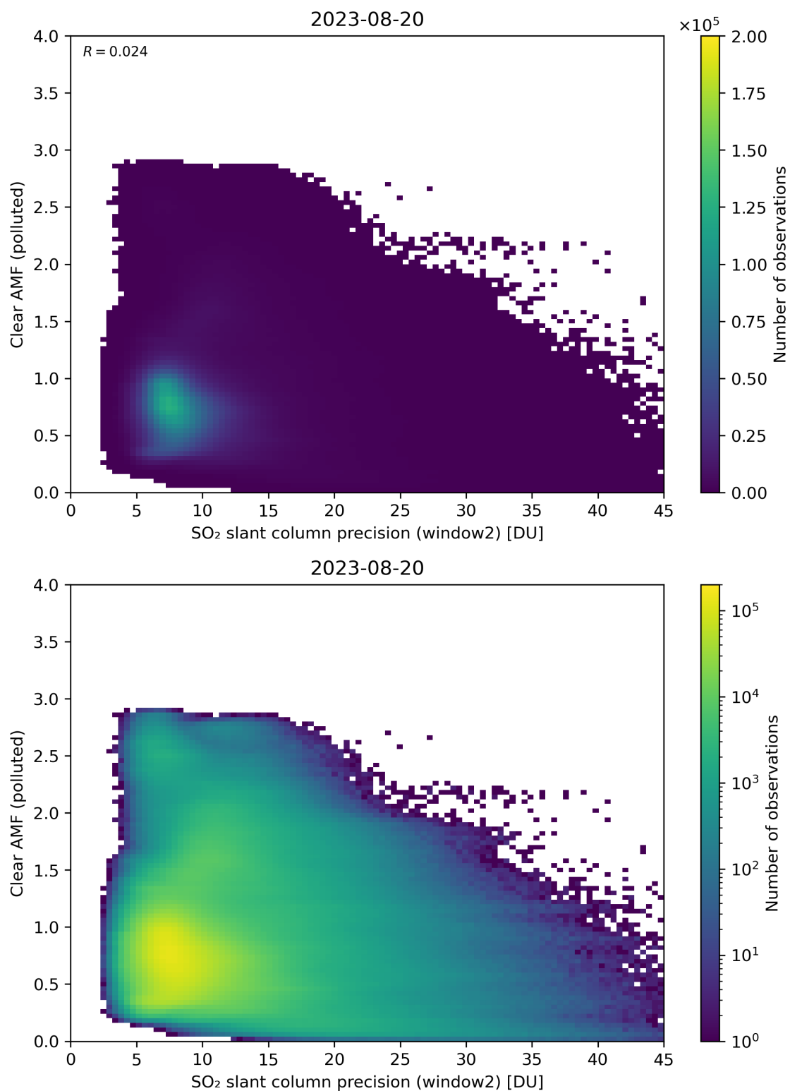
Figure 246: Scatter density plot of “SO 2 slant column precision (window2)” against “Clear AMF (polluted)” for 2023-08-20 to 2023-08-21.
