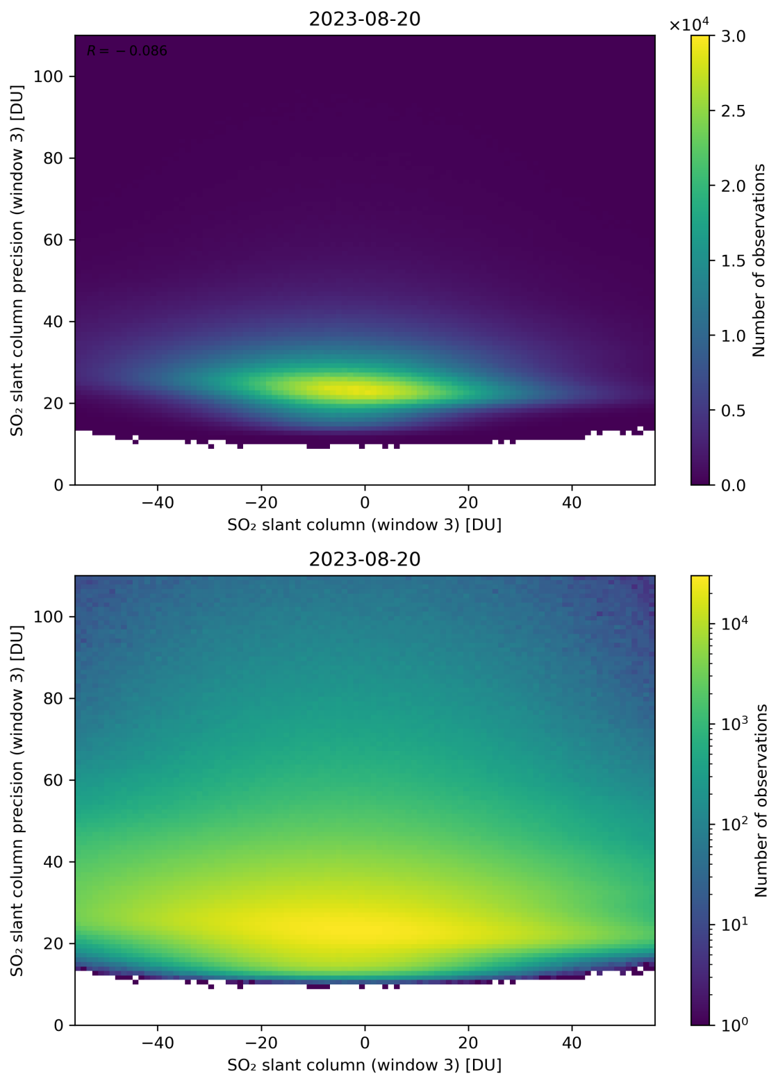
Figure 267: Scatter density plot of “SO 2 slant column (window 3)” against “SO 2 slant column precision (window 3)” for 2023-08-20 to 2023-08-21.
