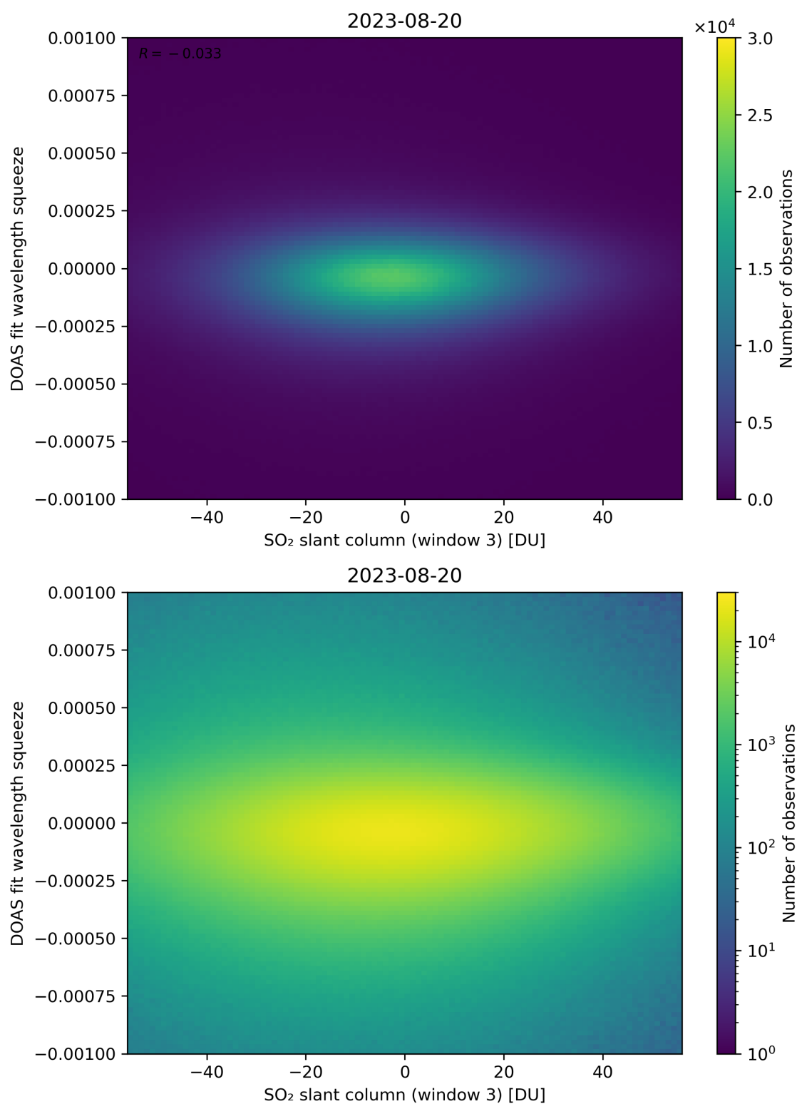
Figure 255: Scatter density plot of “SO 2 slant column (window 3)” against “DOAS fit wavelength squeeze” for 2023-08-20 to 2023-08-21.
