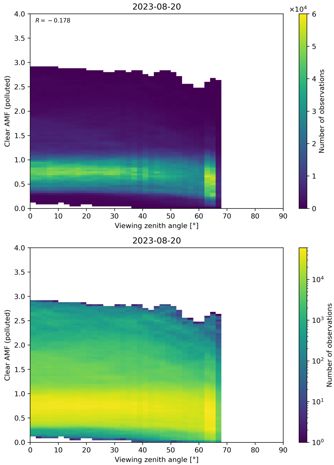
Figure 316: Scatter density plot of “Viewing zenith angle” against “Clear AMF (polluted)” for 2023-08-20 to 2023-08-21.
