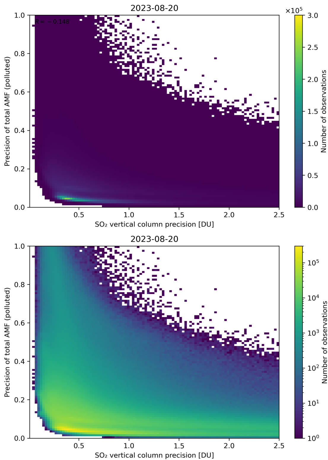
Figure 295: Scatter density plot of “SO 2 vertical column precision” against “Precision of total AMF (polluted)” for 2023-08-20 to 2023-08-21.
