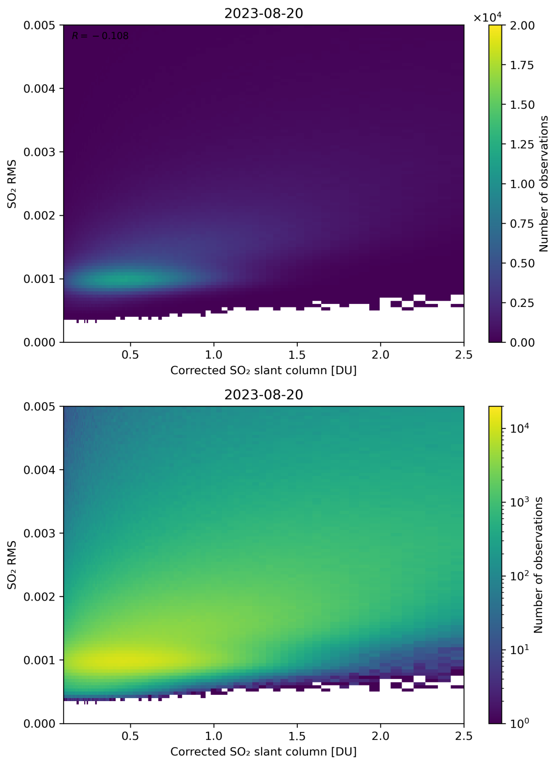
Figure 183: Scatter density plot of “Corrected SO 2 slant column” against “SO 2 RMS” for 2023-08-20 to 2023-08-21.
