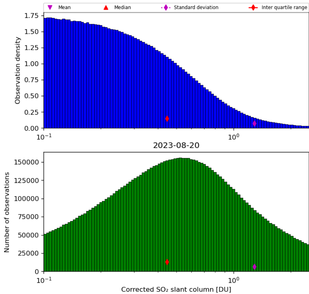
Figure 55: Histogram of “Corrected SO 2 slant column” for 2023-08-20 to 2023-08-21
