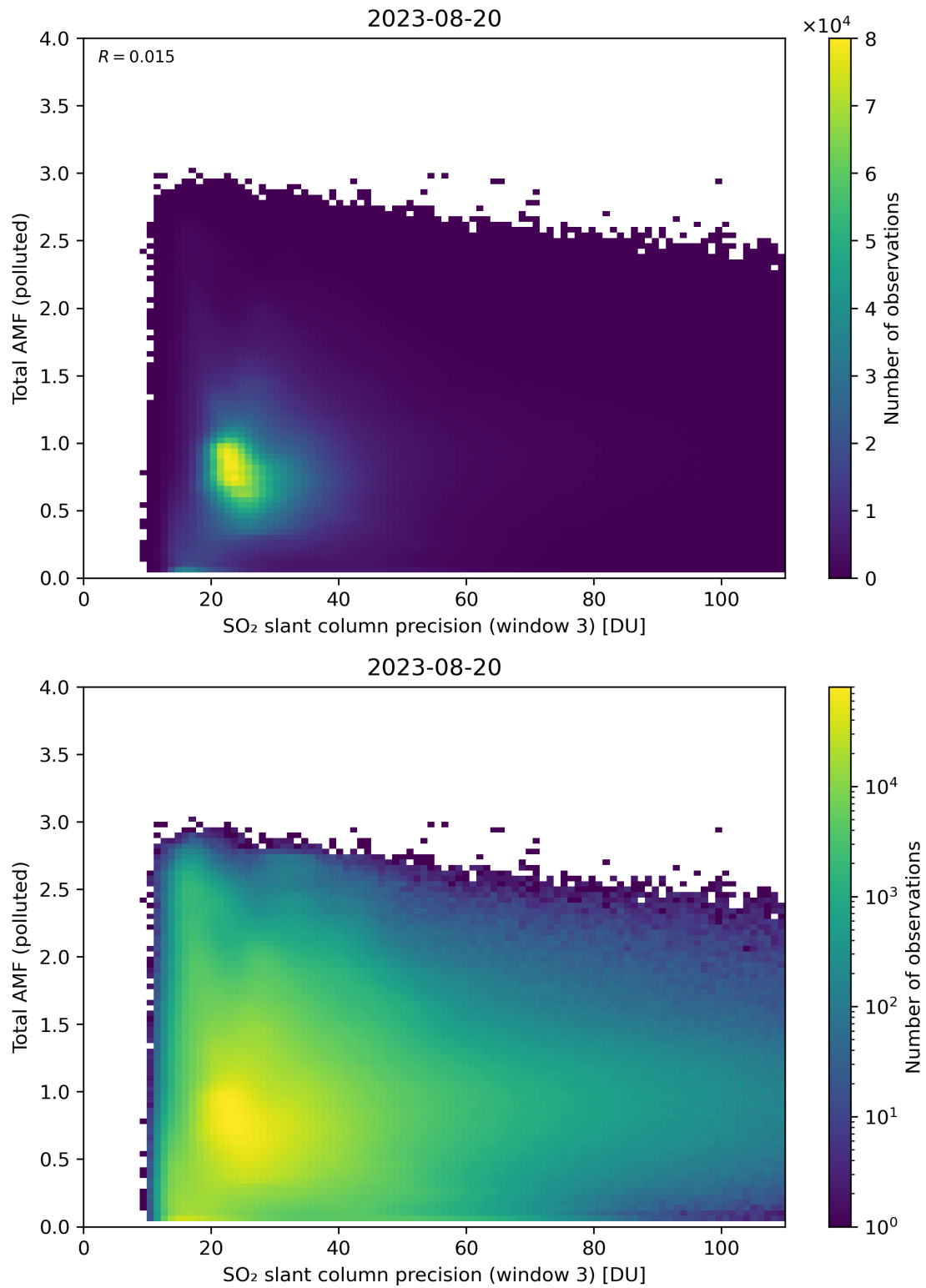
Figure 263: Scatter density plot of “SO 2 slant column precision (window 3)” against “Total AMF (polluted)” for 2023-08-20 to 2023-08-21.
