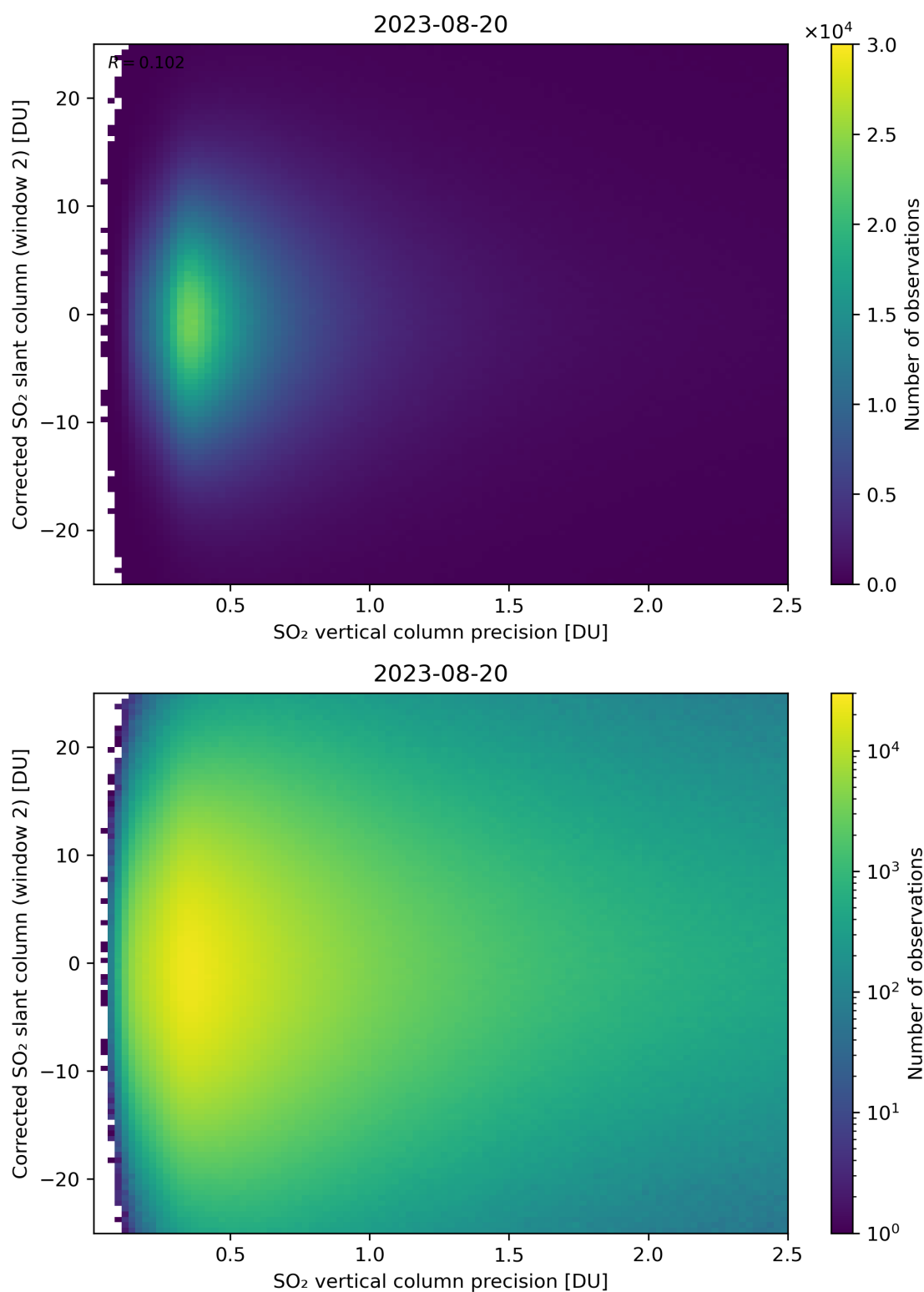
Figure 287: Scatter density plot of “SO 2 vertical column precision” against “Corrected SO 2 slant column (window 2)” for 2023-08-20 to 2023-08-21.
