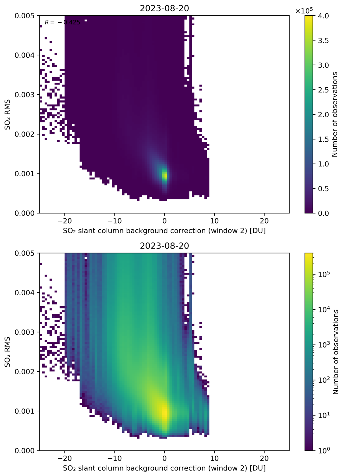
Figure 114: Scatter density plot of “SO 2 slant column background correction (window 2)” against “SO 2 RMS” for 2023-08-20 to 2023-08-21.
