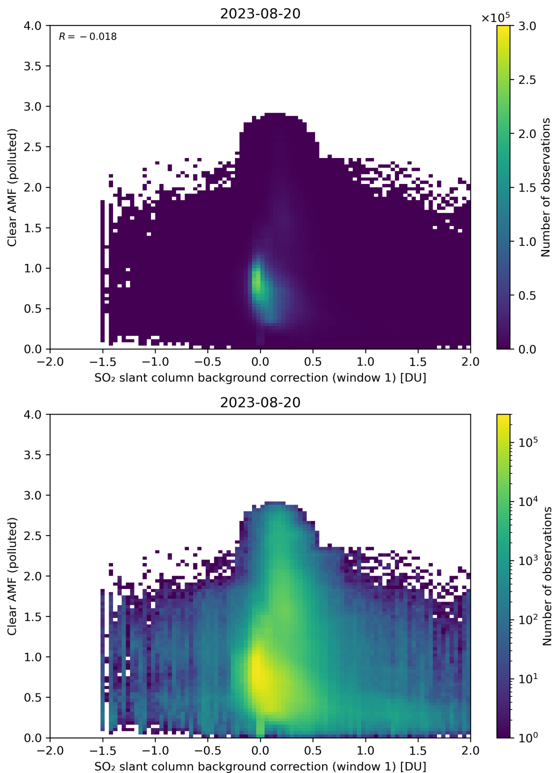
Figure 103: Scatter density plot of “SO 2 slant column background correction (window 1)” against “Clear AMF (polluted)” for 2023-08-20 to 2023-08-21.
