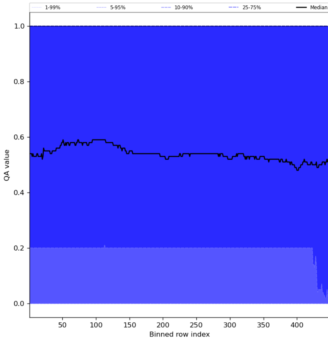
Figure 75: Along track statistics of “QA value” for 2023-08-20 to 2023-08-21
