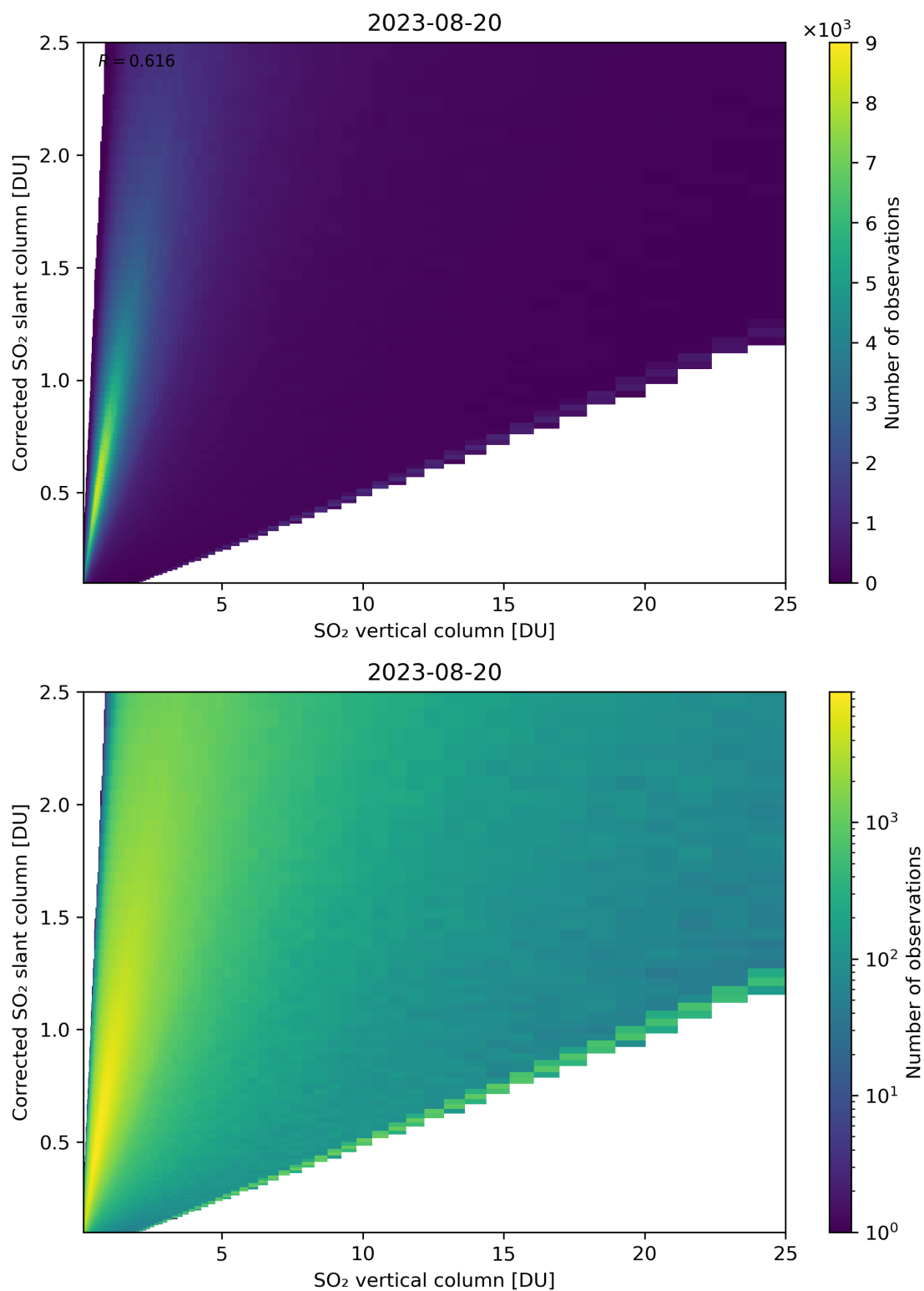
Figure 297: Scatter density plot of “SO 2 vertical column” against “Corrected SO 2 slant column” for 2023-08-20 to 2023-08-21.
