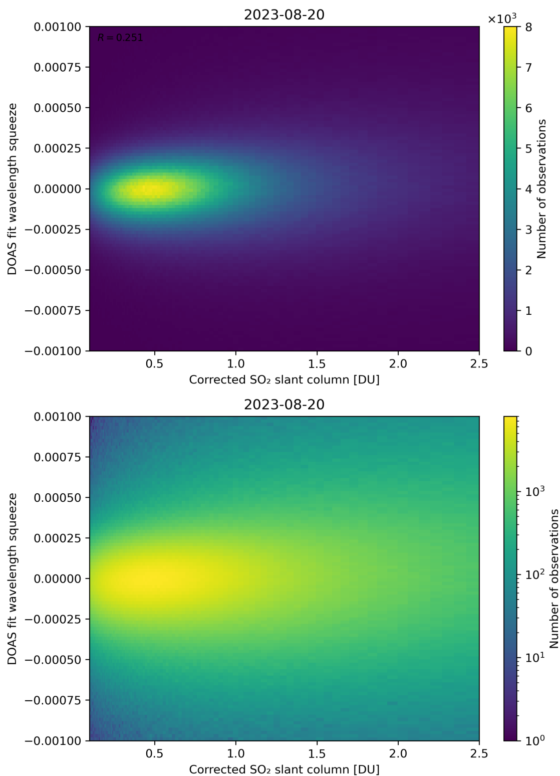
Figure 182: Scatter density plot of “Corrected SO 2 slant column” against “DOAS fit wavelength squeeze” for 2023-08-20 to 2023-08-21.
