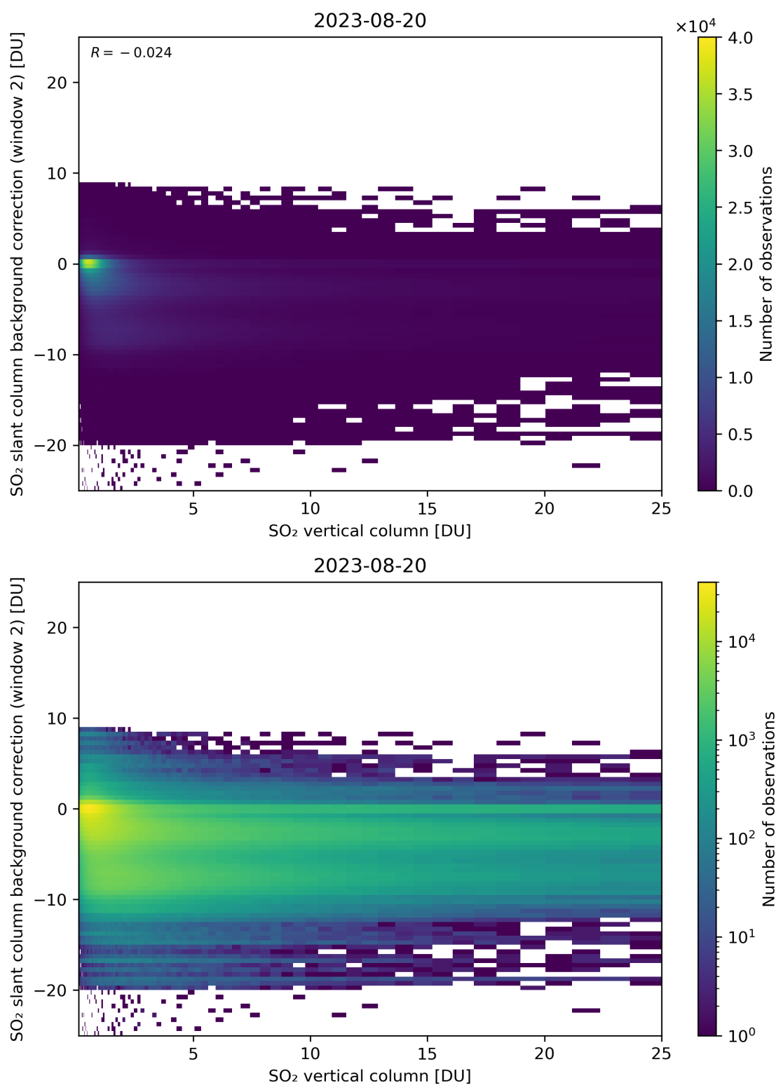
Figure 274: Scatter density plot of “SO 2 vertical column” against “SO 2 slant column background correction (window 2)” for 2023-08-20 to 2023-08-21.
