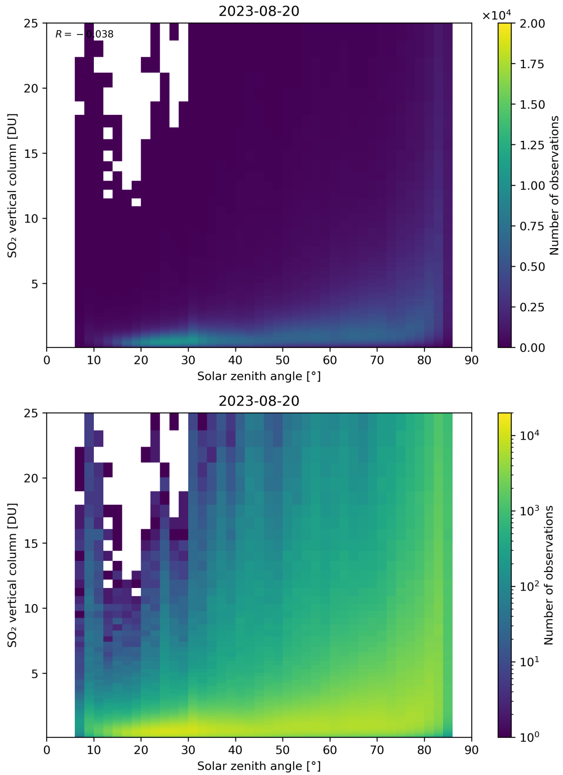
Figure 176: Scatter density plot of “Solar zenith angle” against “SO 2 vertical column” for 2023-08-20 to 2023-08-21.
