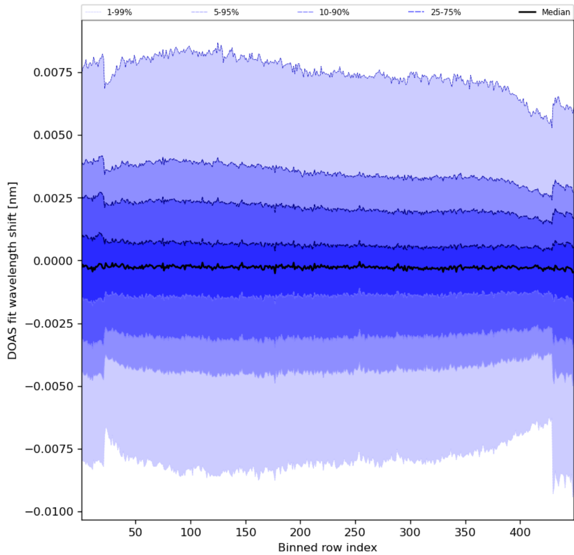
Figure 91: Along track statistics of “DOAS fit wavelength shift” for 2023-08-20 to 2023-08-21
