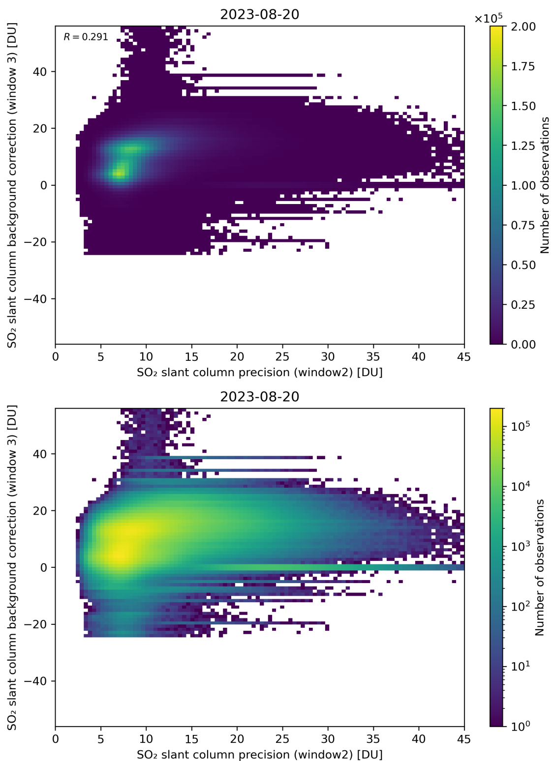
Figure 242: Scatter density plot of “SO 2 slant column precision (window2)” against “SO 2 slant column background correction (window 3)” for 2023-08-20 to 2023-08-21.
