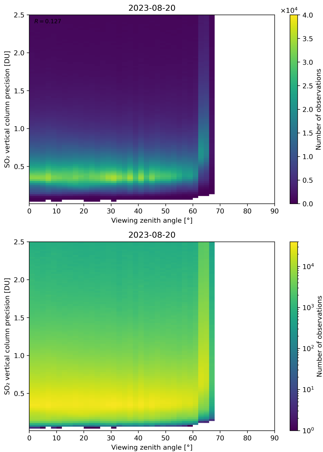
Figure 328: Scatter density plot of “Viewing zenith angle” against “SO 2 vertical column precision” for 2023-08-20 to 2023-08-21.
