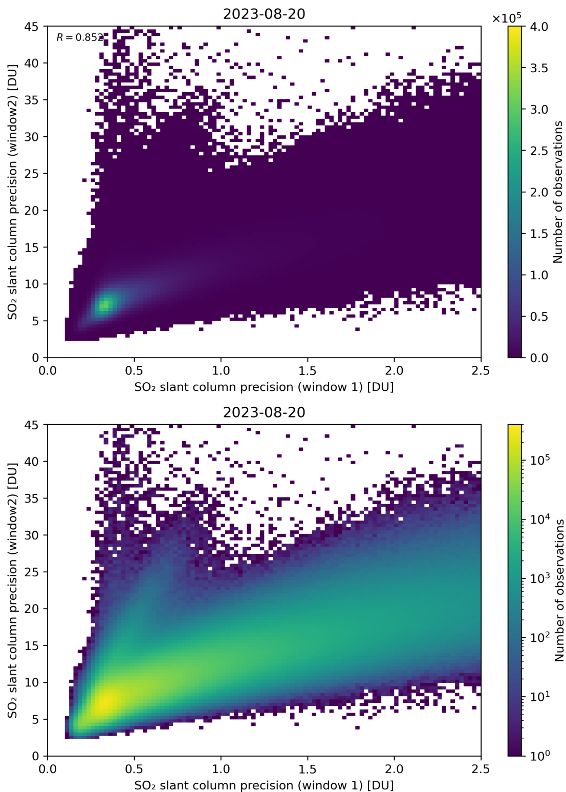
Figure 227: Scatter density plot of “SO 2 slant column precision (window 1)” against “SO 2 slant column precision (window 2)” for 2023-08-20 to 2023-08-21.
