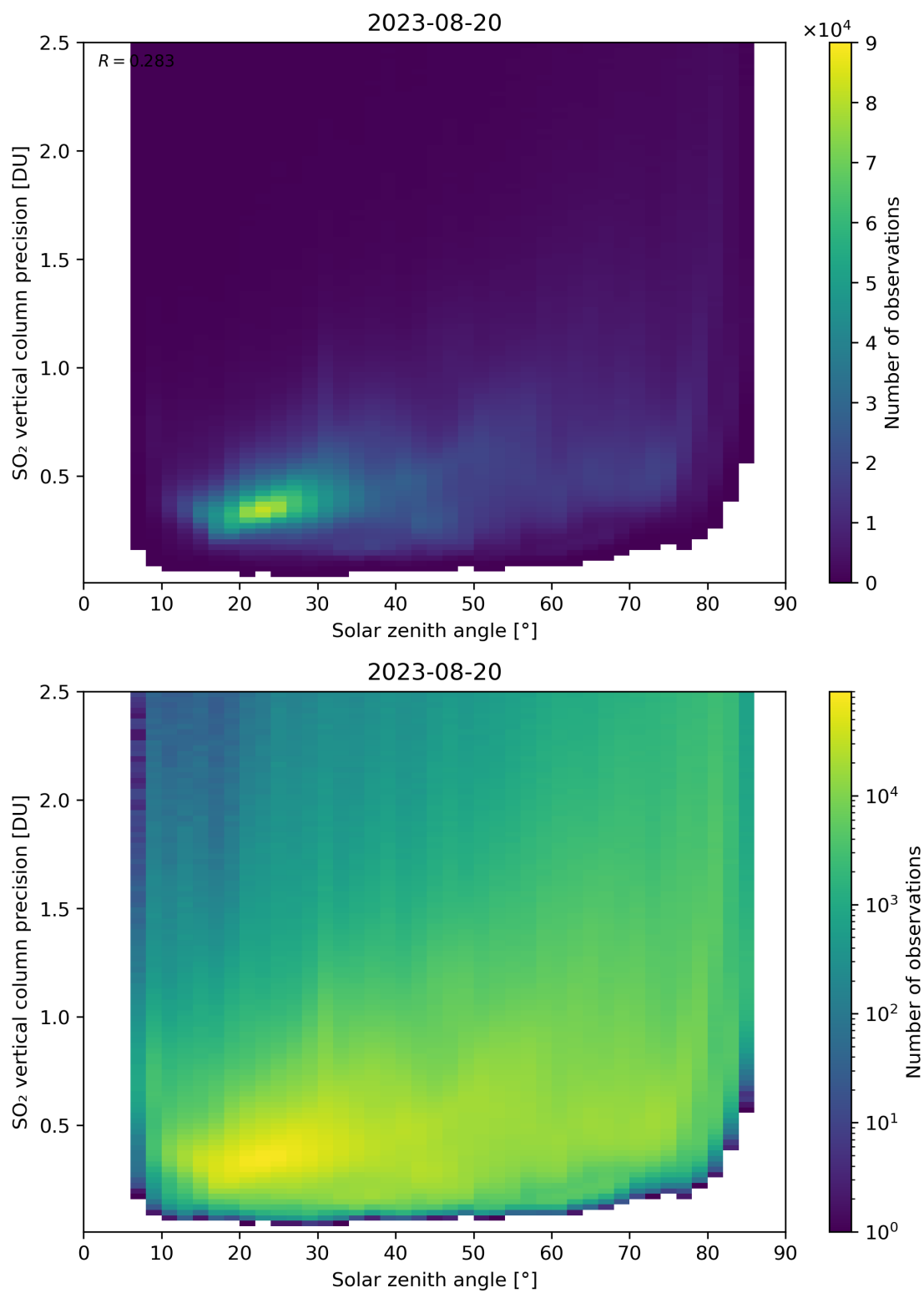
Figure 177: Scatter density plot of “Solar zenith angle” against “SO 2 vertical column precision” for 2023-08-20 to 2023-08-21.
