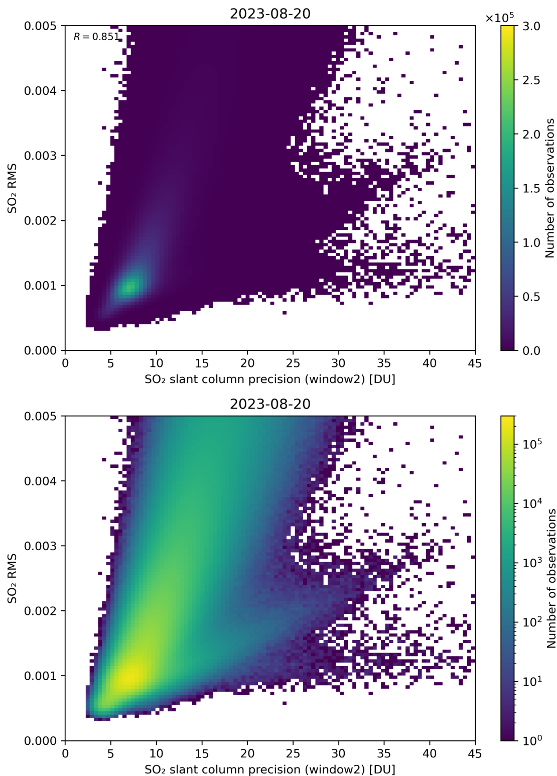
Figure 245: Scatter density plot of “SO 2 slant column precision (window2)” against “SO 2 RMS” for 2023-08-20 to 2023-08-21.
