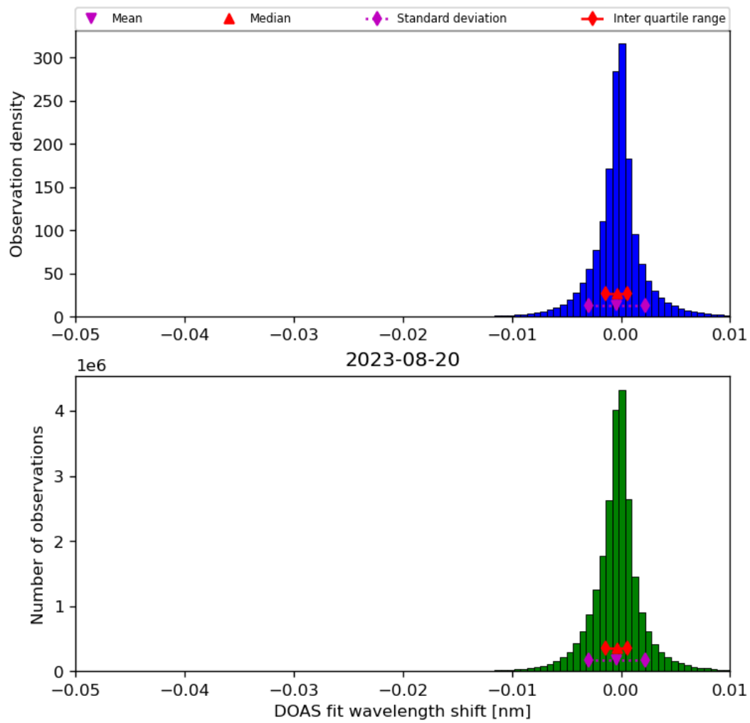
Figure 68: Histogram of “DOAS fit wavelength shift” for 2023-08-20 to 2023-08-21
