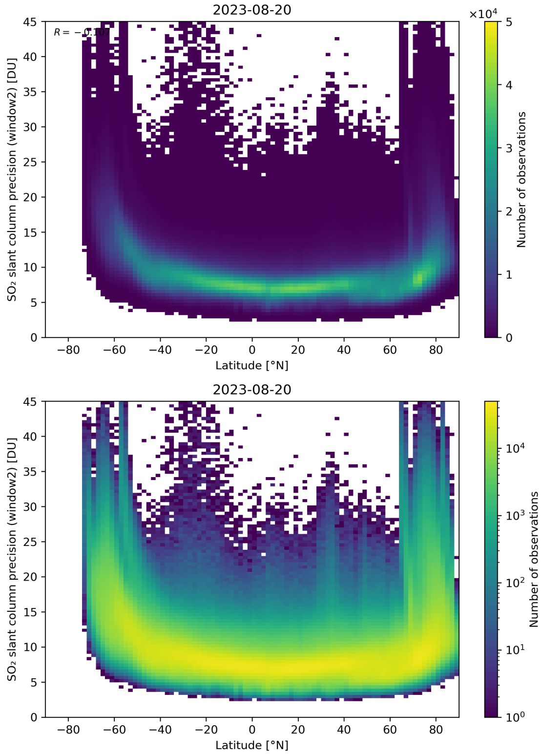
Figure 151: Scatter density plot of “Latitude” against “SO 2 slant column precision (window2)” for 2023-08-20 to 2023-08-21.
