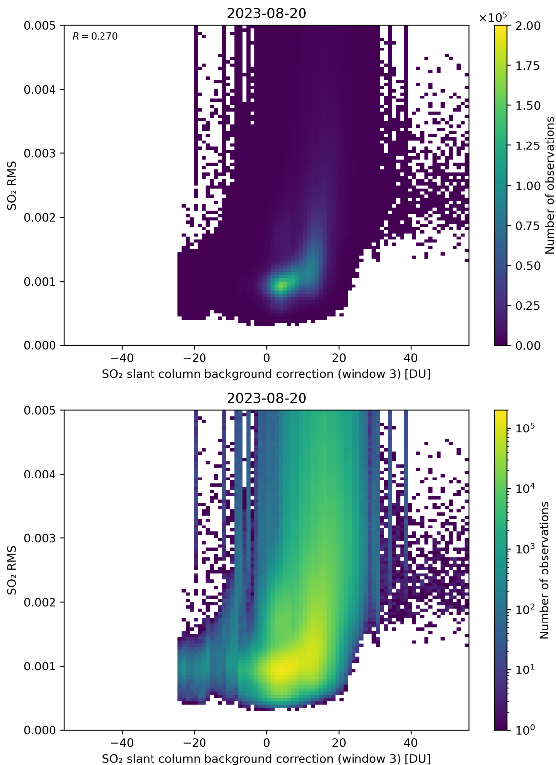
Figure 123: Scatter density plot of “SO 2 slant column background correction (window 3)” against “SO 2 RMS” for 2023-08-20 to 2023-08-21.
