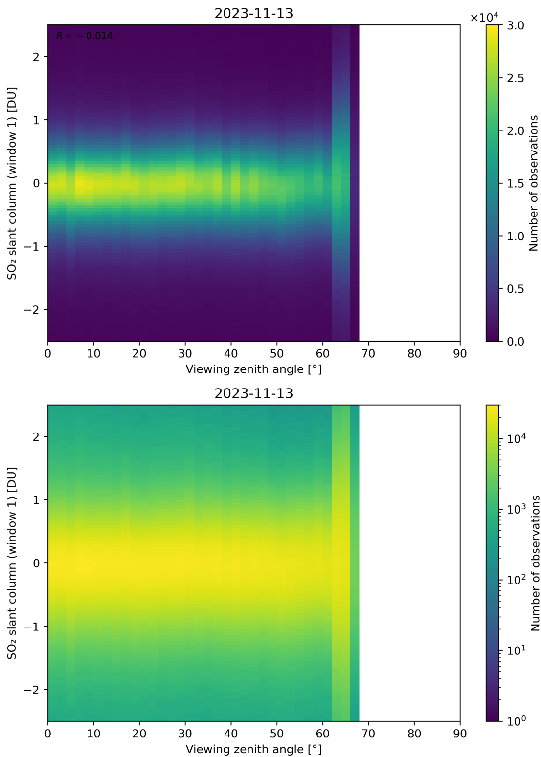
Figure 320: Scatter density plot of “Viewing zenith angle” against “SO 2 slant column (window 1)” for 2023-11-13 to 2023-11-14.
