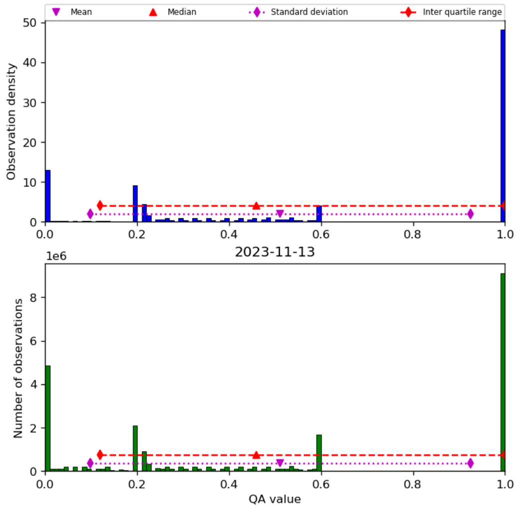
Figure 52: Histogram of “QA value” for 2023-11-13 to 2023-11-14
