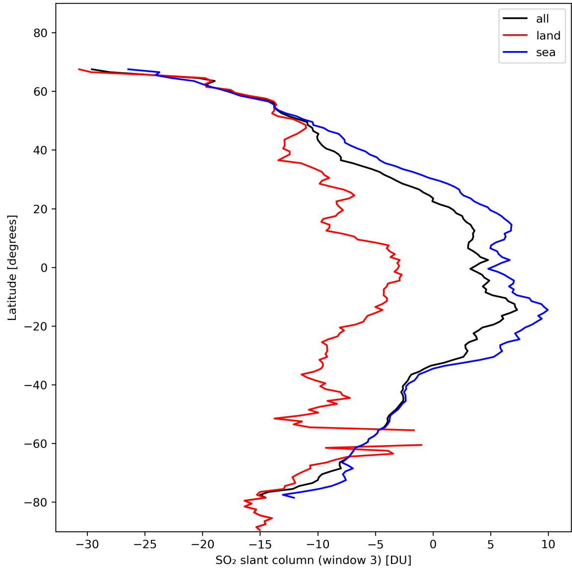
Figure 41: Zonal average of “SO 2 slant column (window 3)” for 2023-11-13 to 2023-11-14.
