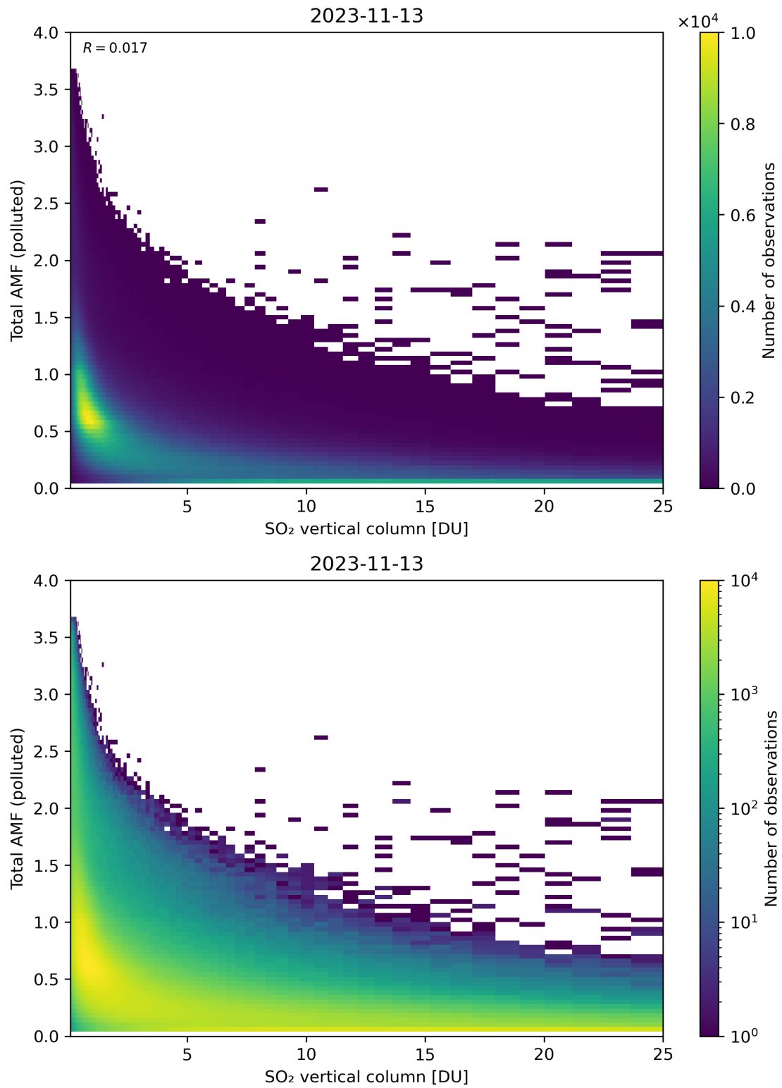
Figure 305: Scatter density plot of “SO 2 vertical column” against “Total AMF (polluted)” for 2023-11-13 to 2023-11-14.
