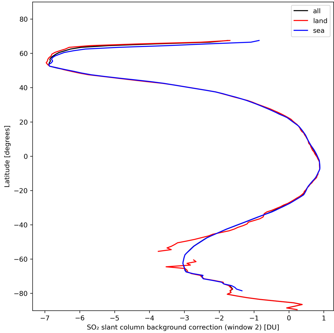
Figure 40: Zonal average of “SO 2 slant column background correction (window 2)” for 2023-11-13 to 2023-11-14.
