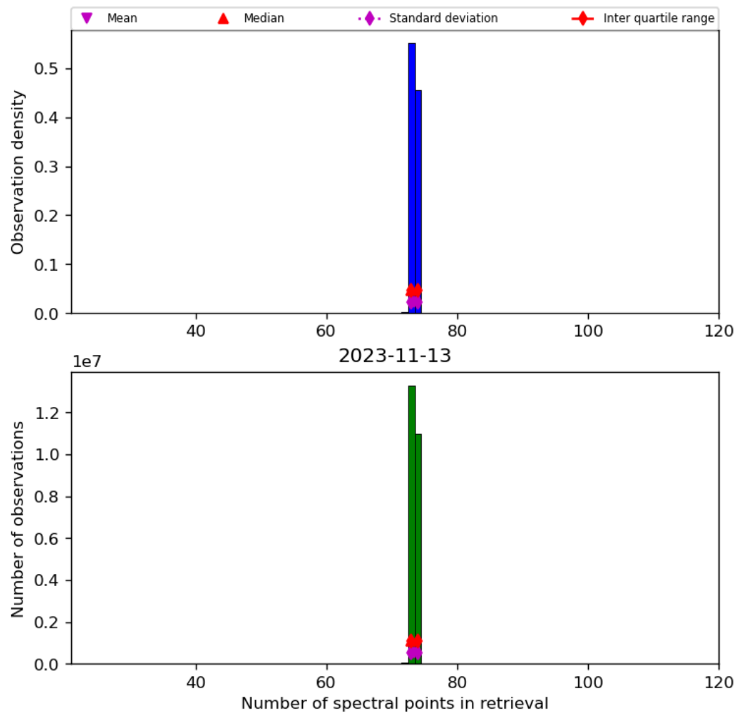
Figure 74: Histogram of “Number of spectral points in retrieval” for 2023-11-13 to 2023-11-14
