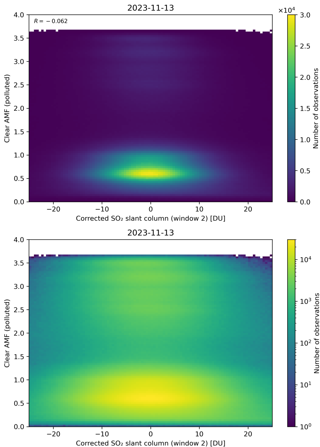
Figure 199: Scatter density plot of “Corrected SO 2 slant column (window 2)” against “Clear AMF (polluted)” for 2023-11-13 to 2023-11-14.
