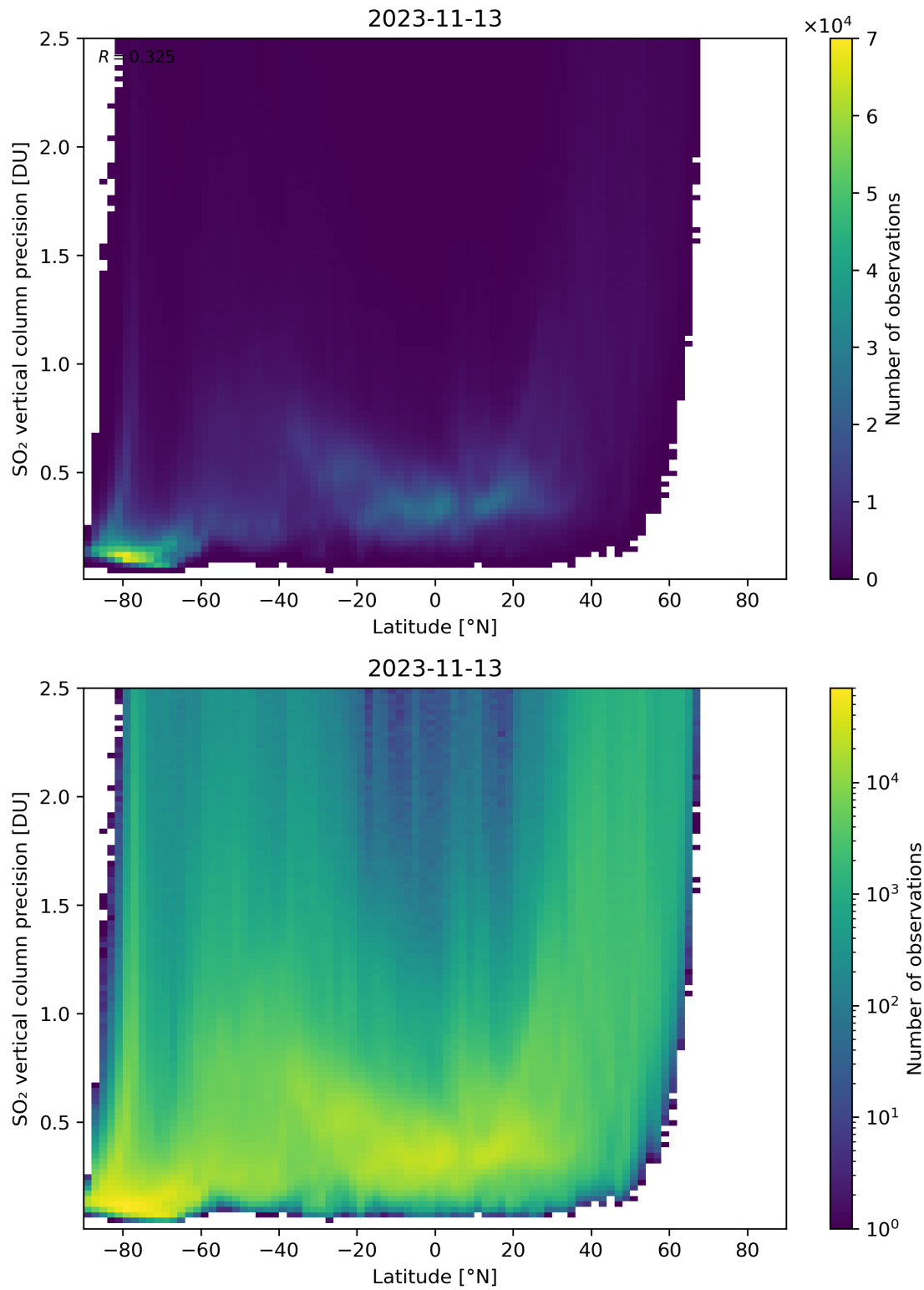
Figure 157: Scatter density plot of “Latitude” against “SO 2 vertical column precision” for 2023-11-13 to 2023-11-14.
