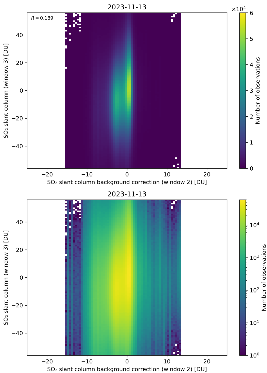
Figure 117: Scatter density plot of “SO 2 slant column background correction (window 2)” against “SO 2 slant column (window 3)” for 2023-11-13 to 2023-11-14.
