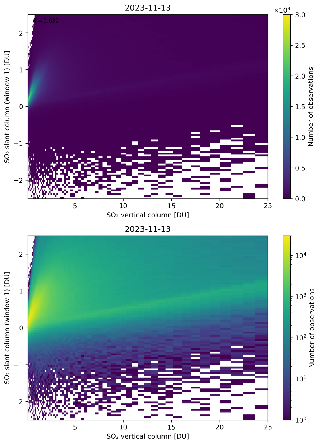
Figure 300: Scatter density plot of “SO 2 vertical column” against “SO 2 slant column (window 1)” for 2023-11-13 to 2023-11-14.
