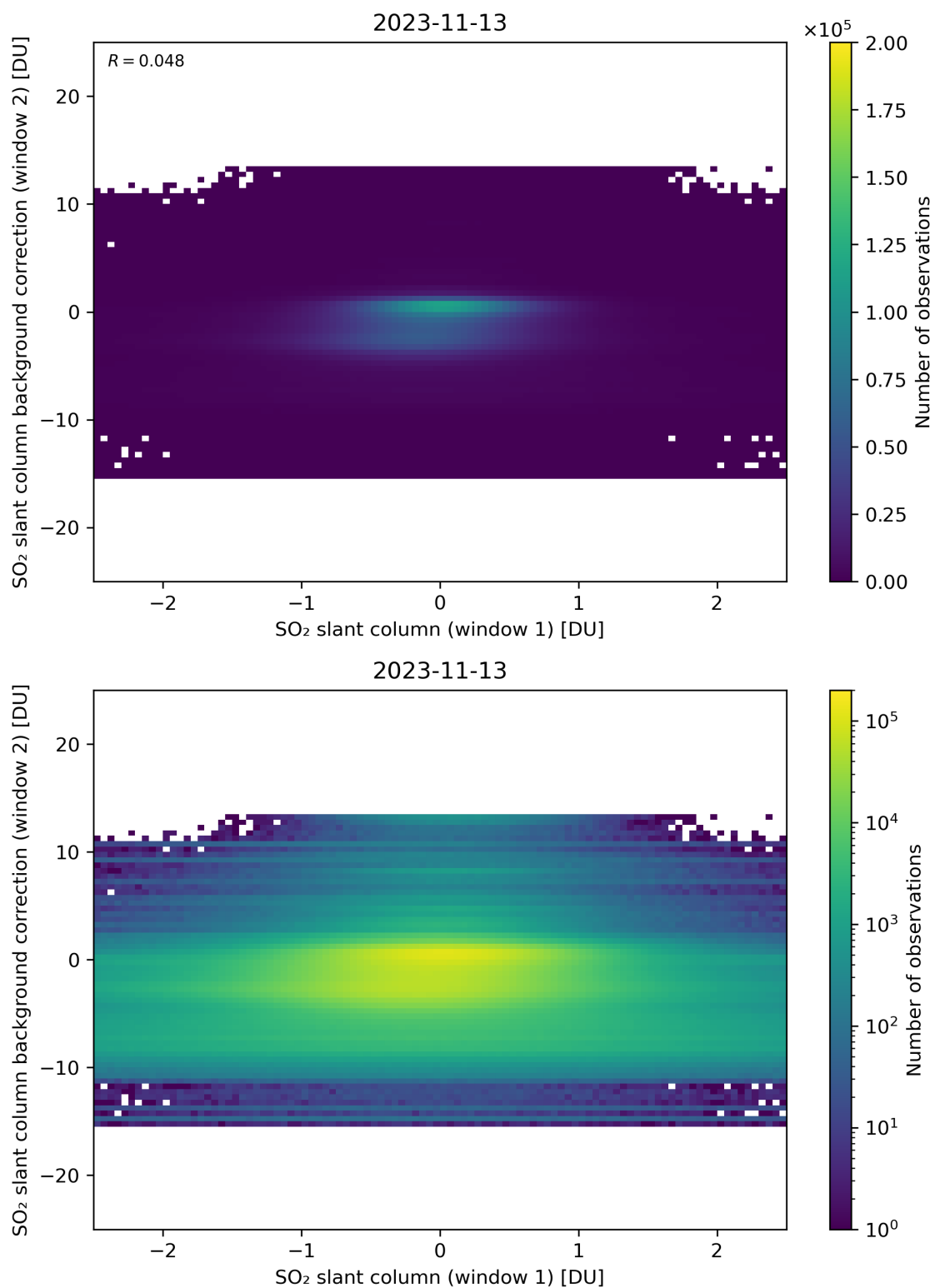
Figure 213: Scatter density plot of “SO 2 slant column (window 1)” against “SO 2 slant column background correction (window 2)” for 2023-11-13 to 2023-11-14.
