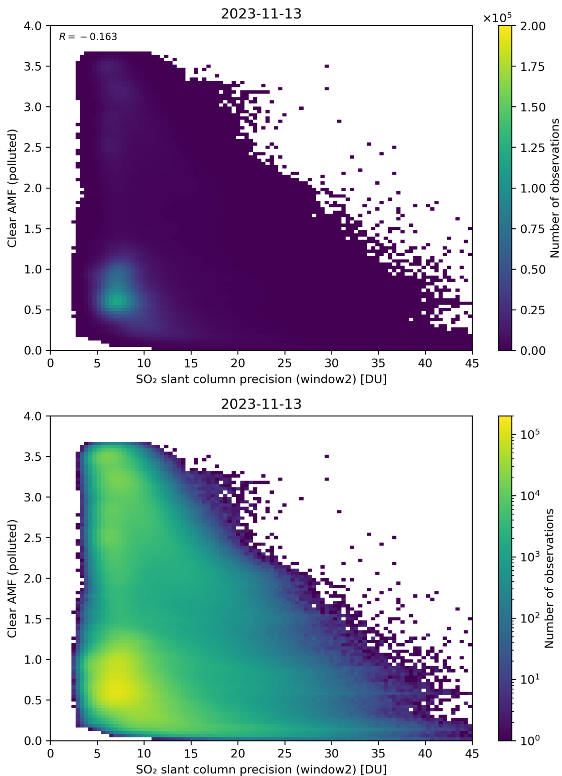
Figure 246: Scatter density plot of “SO 2 slant column precision (window2)” against “Clear AMF (polluted)” for 2023-11-13 to 2023-11-14.
