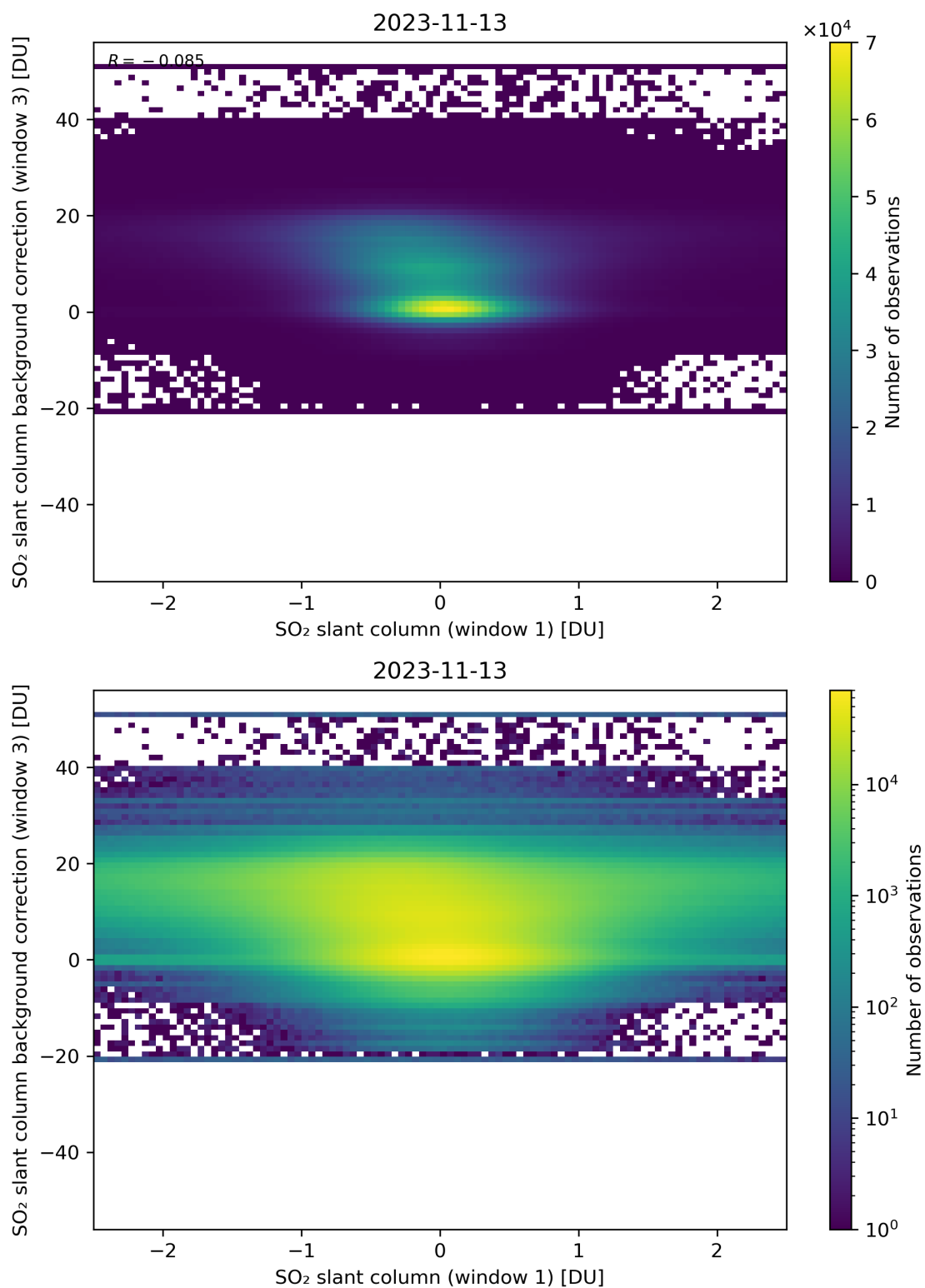
Figure 214: Scatter density plot of “SO 2 slant column (window 1)” against “SO 2 slant column background correction (window 3)” for 2023-11-13 to 2023-11-14.
