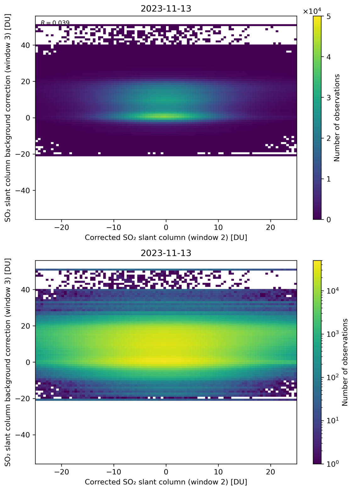
Figure 195: Scatter density plot of “Corrected SO 2 slant column (window 2)” against “SO 2 slant column background correction (window 3)” for 2023-11-13 to 2023-11-14.
