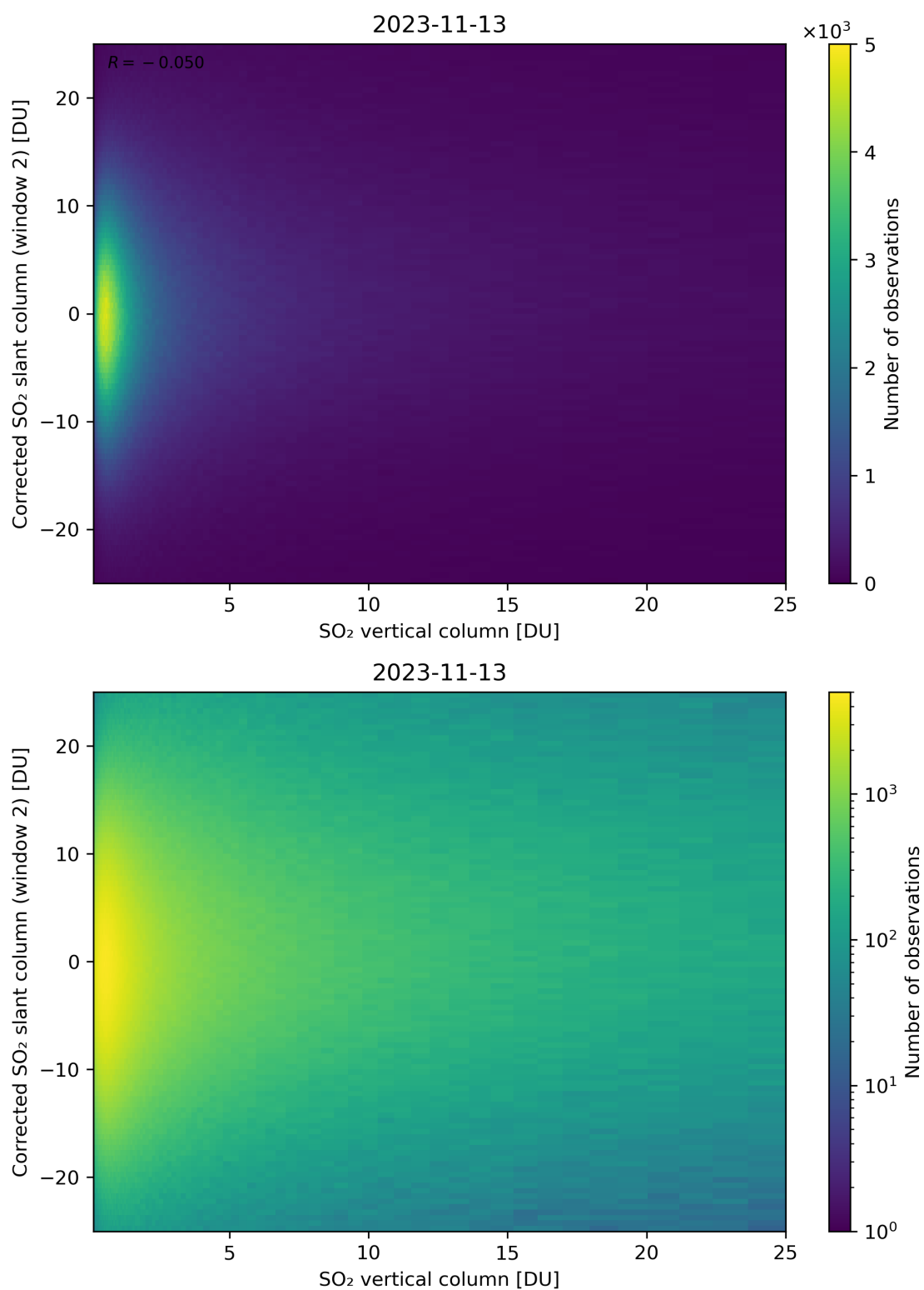
Figure 298: Scatter density plot of “SO 2 vertical column” against “Corrected SO 2 slant column (window 2)” for 2023-11-13 to 2023-11-14.
