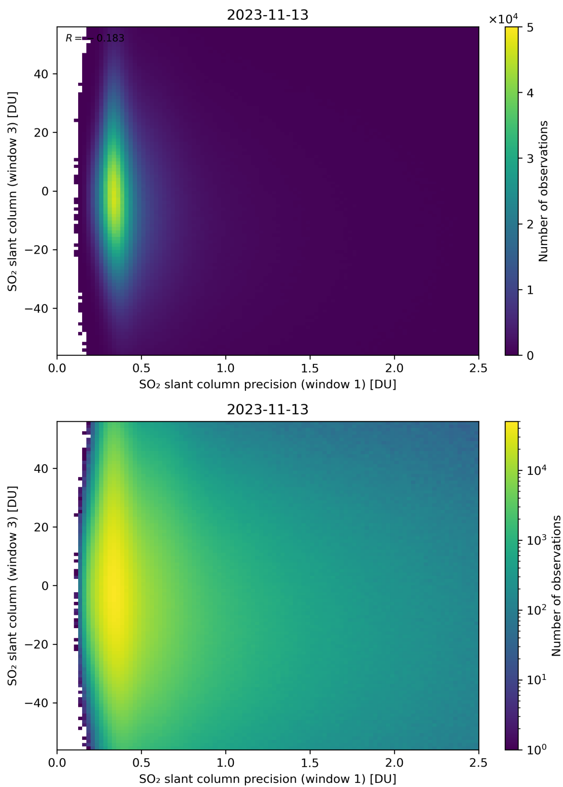
Figure 228: Scatter density plot of “SO 2 slant column precision (window 1)” against “SO 2 slant column (window 3)” for 2023-11-13 to 2023-11-14.
