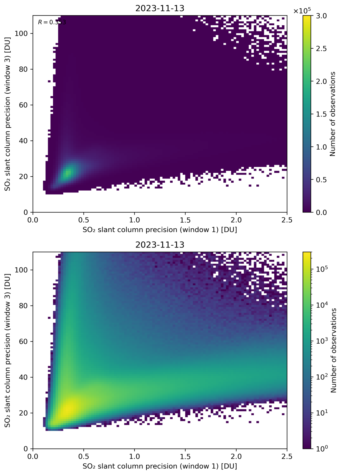
Figure 229: Scatter density plot of “SO 2 slant column precision (window 1)” against “SO 2 slant column precision (window 3)” for 2023-11-13 to 2023-11-14.
