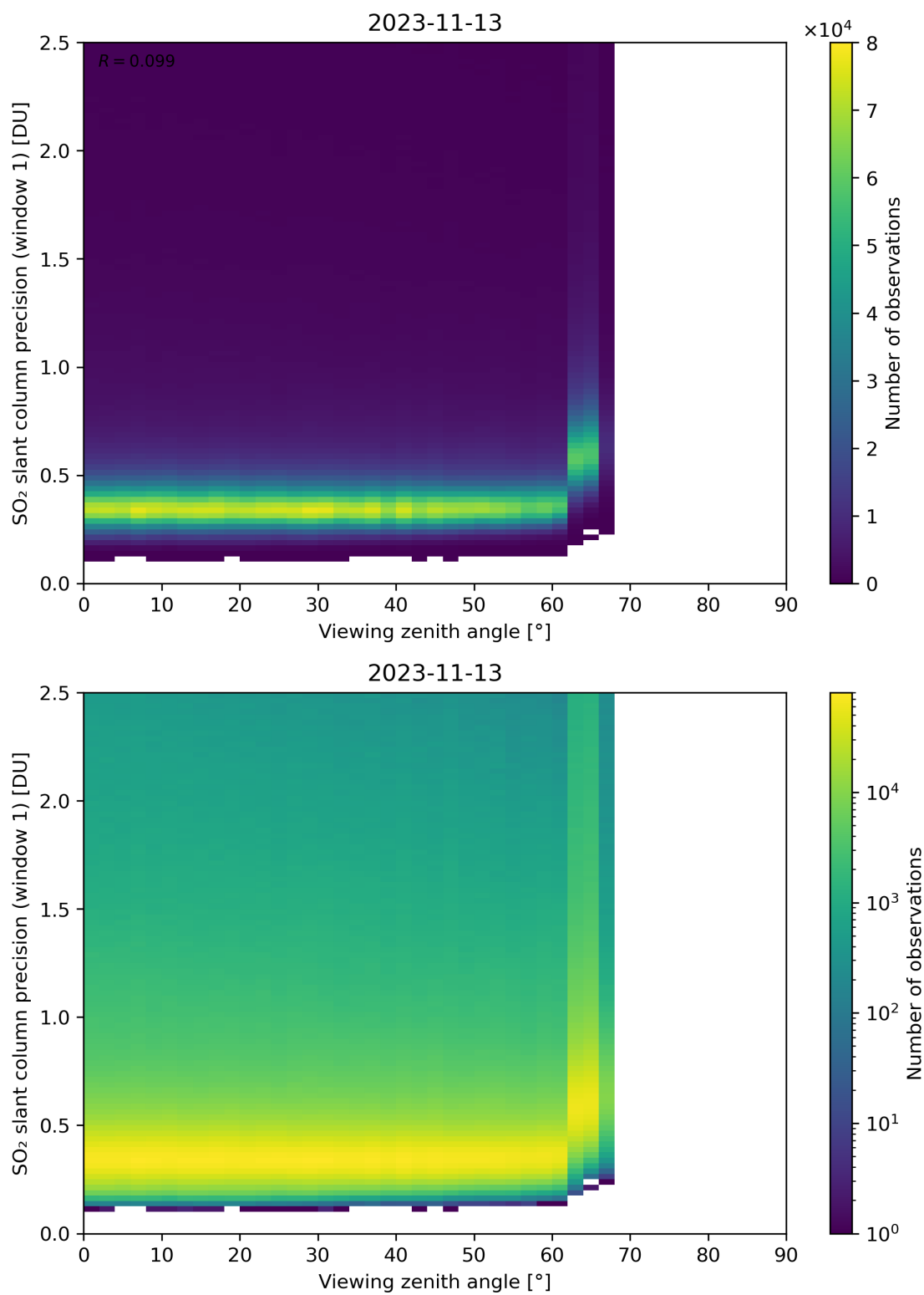
Figure 321: Scatter density plot of “Viewing zenith angle” against “SO 2 slant column precision (window 1)” for 2023-11-13 to 2023-11-14.
