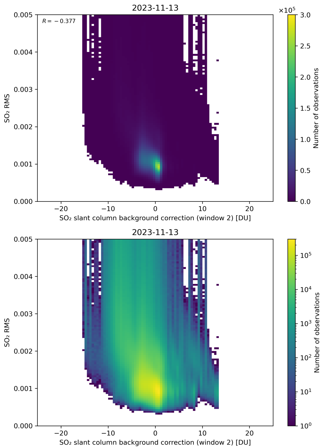
Figure 114: Scatter density plot of “SO 2 slant column background correction (window 2)” against “SO 2 RMS” for 2023-11-13 to 2023-11-14.
