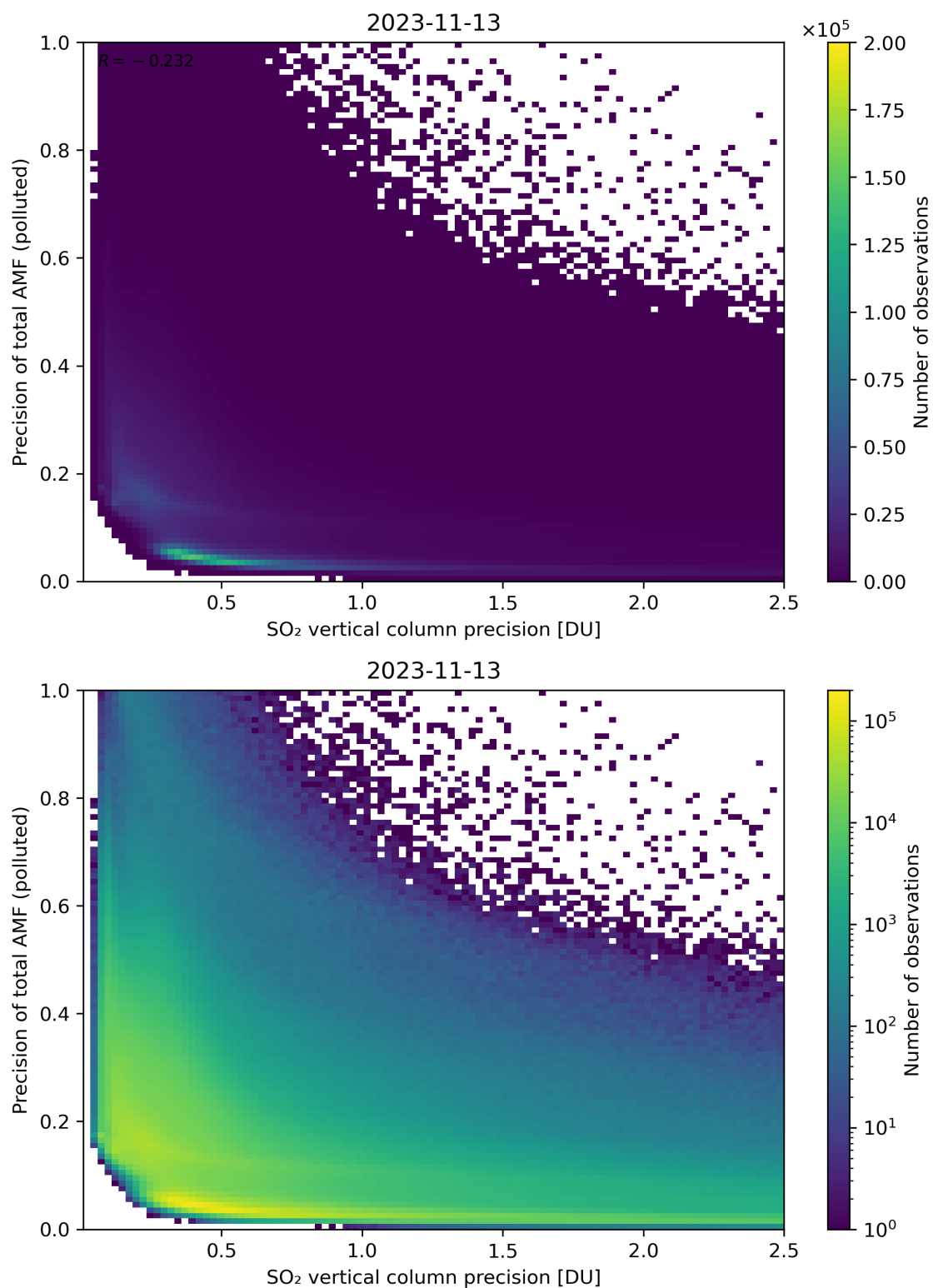
Figure 295: Scatter density plot of “SO 2 vertical column precision” against “Precision of total AMF (polluted)” for 2023-11-13 to 2023-11-14.
