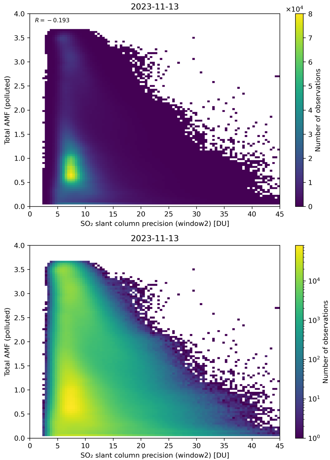
Figure 251: Scatter density plot of “SO 2 slant column precision (window2)” against “Total AMF (polluted)” for 2023-11-13 to 2023-11-14.
