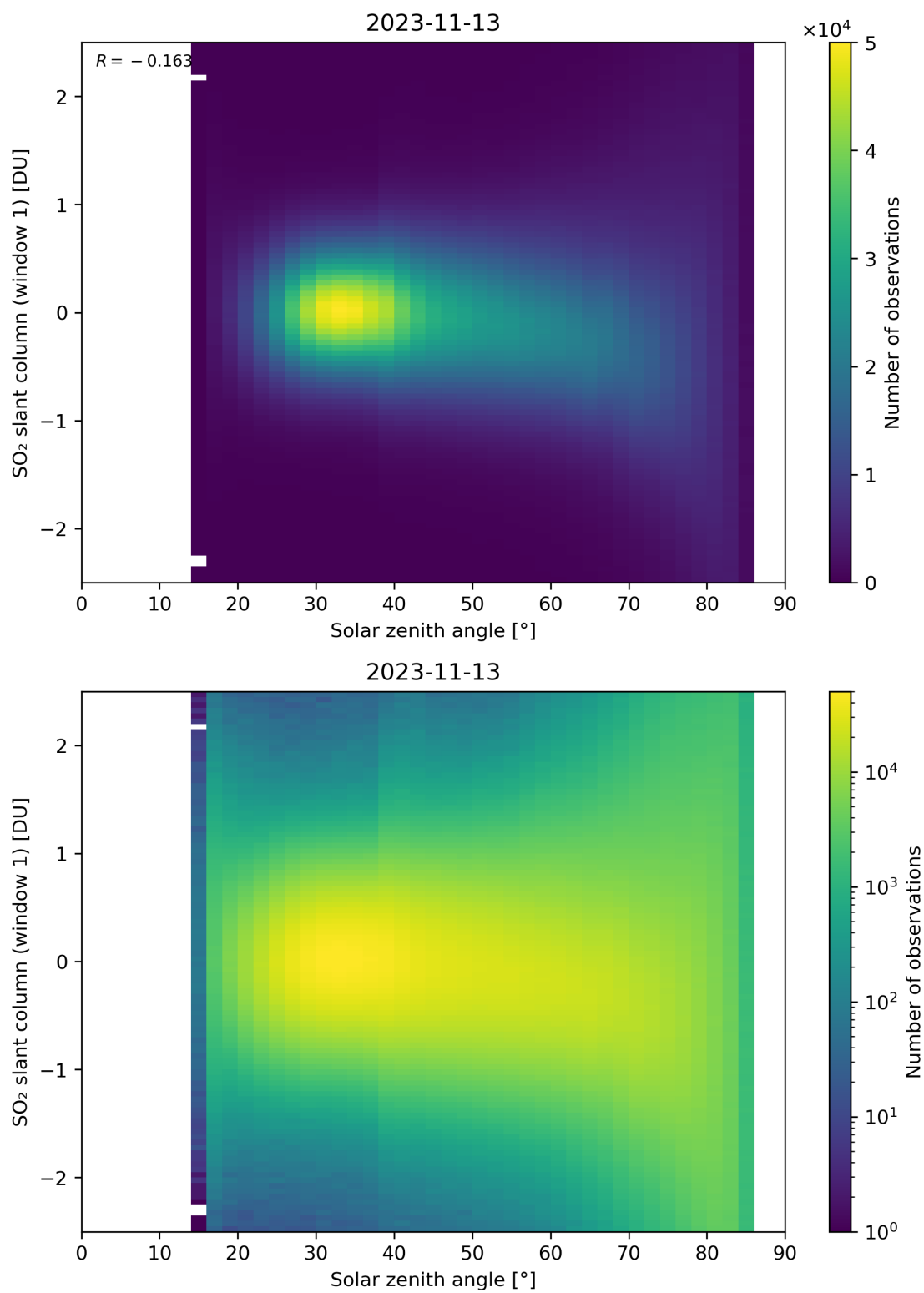
Figure 169: Scatter density plot of “Solar zenith angle” against “SO 2 slant column (window 1)” for 2023-11-13 to 2023-11-14.
