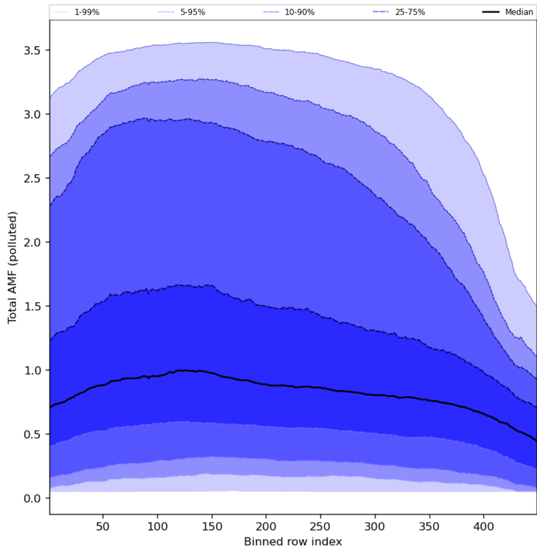
Figure 94: Along track statistics of “Total AMF (polluted)” for 2023-11-13 to 2023-11-14
