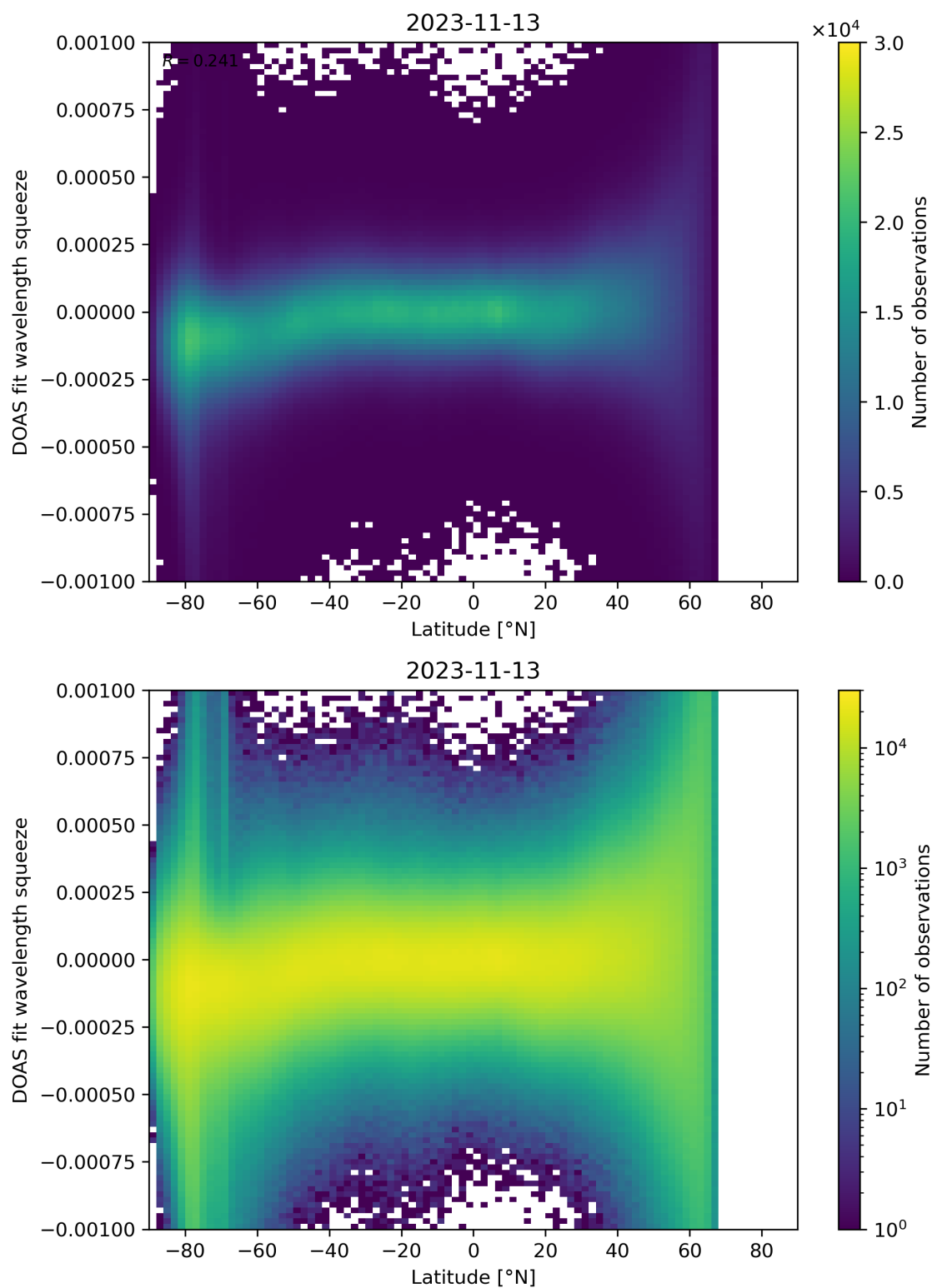
Figure 143: Scatter density plot of “Latitude” against “DOAS fit wavelength squeeze” for 2023-11-13 to 2023-11-14.
