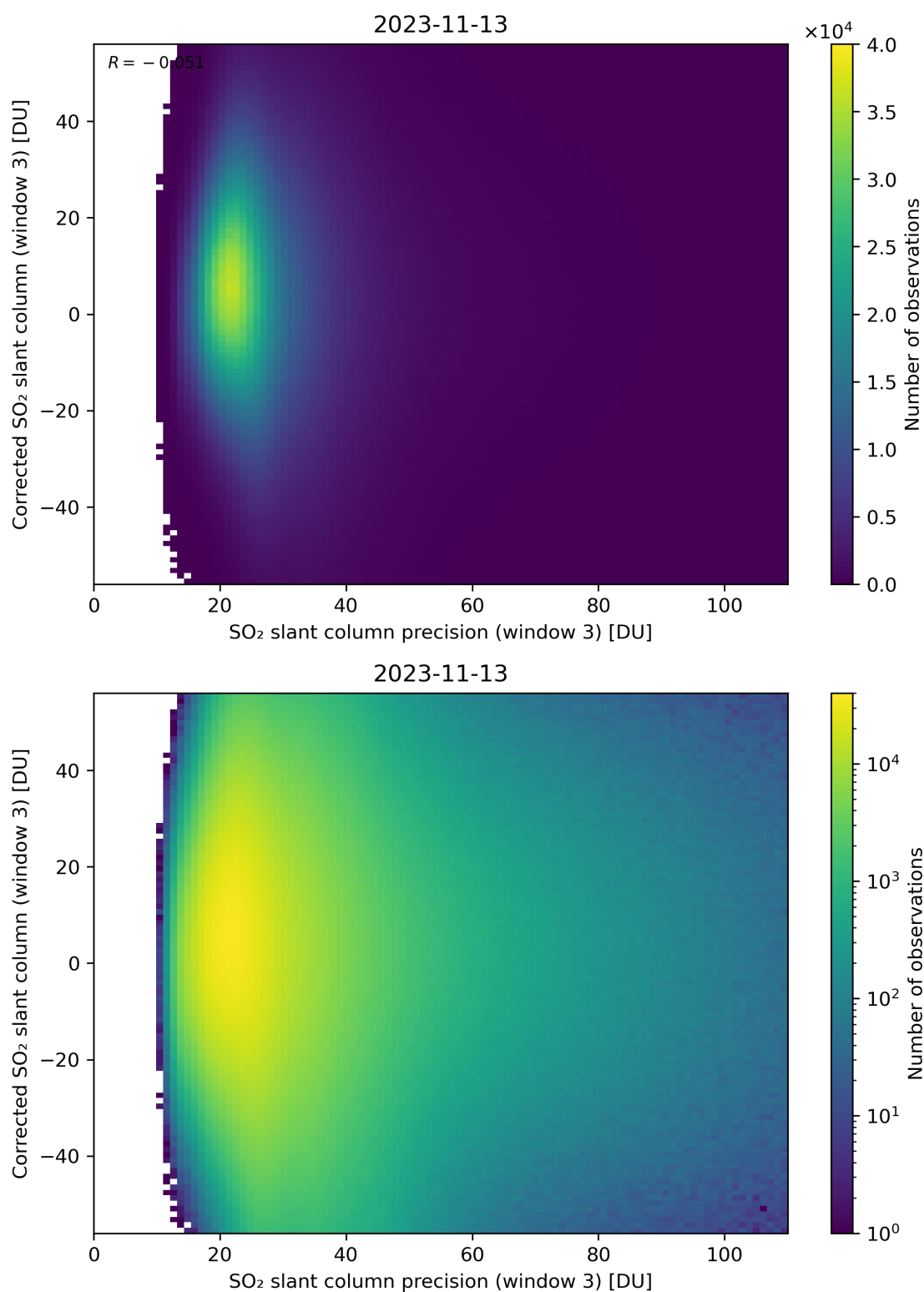
Figure 262: Scatter density plot of “SO 2 slant column precision (window 3)” against “Corrected SO 2 slant column (window 3)” for 2023-11-13 to 2023-11-14.
