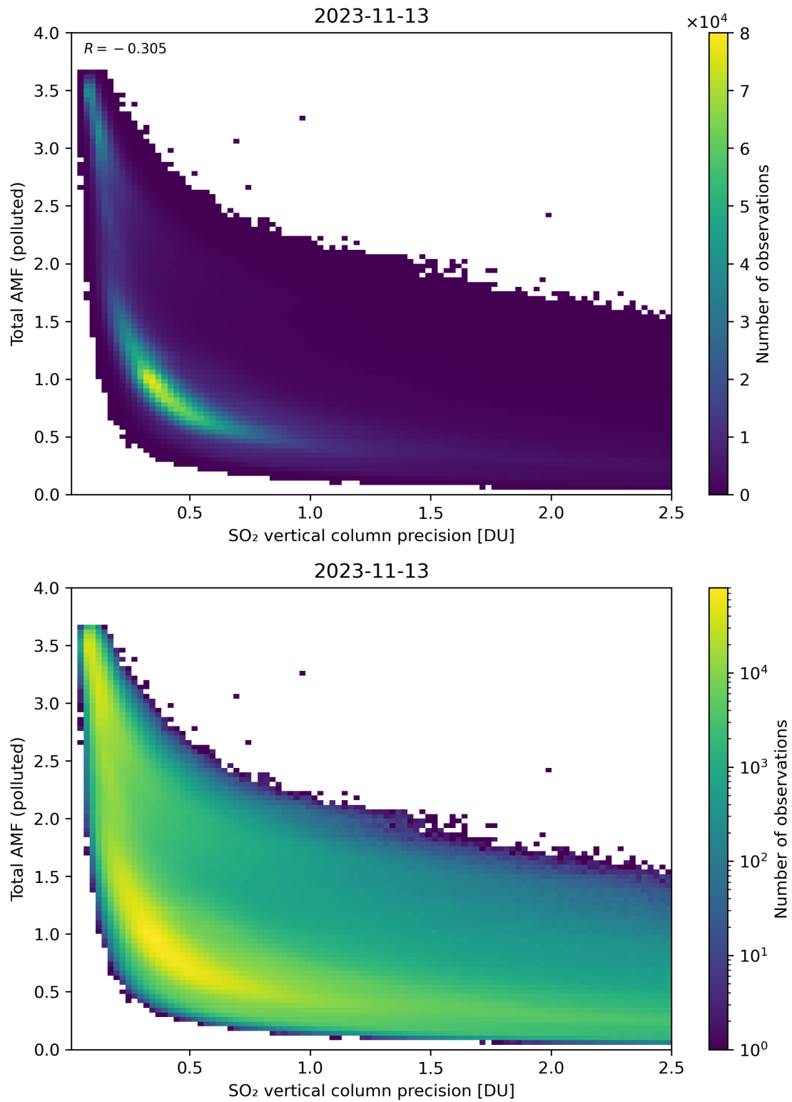
Figure 294: Scatter density plot of “SO 2 vertical column precision” against “Total AMF (polluted)” for 2023-11-13 to 2023-11-14.
