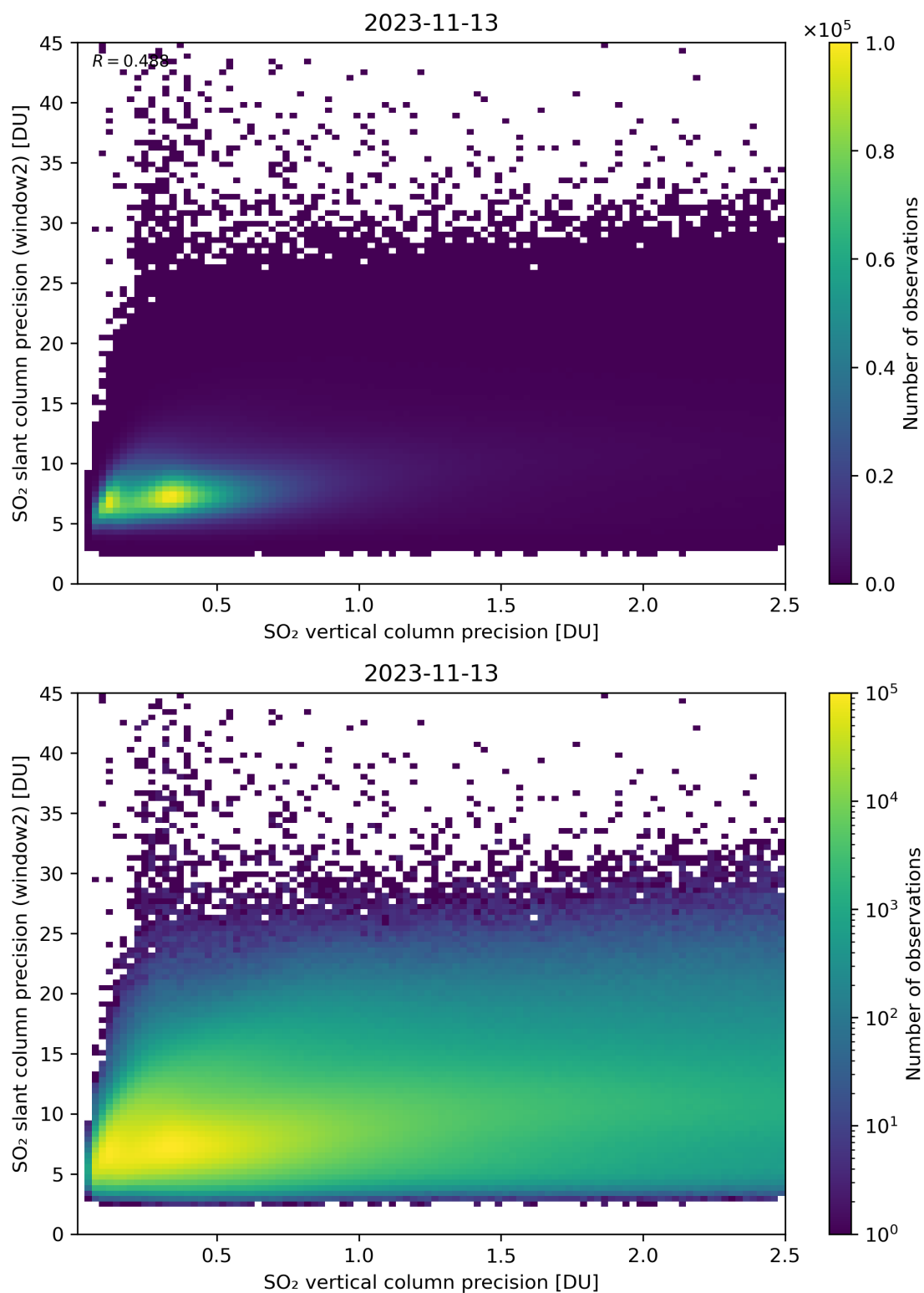
Figure 291: Scatter density plot of “SO 2 vertical column precision” against “SO 2 slant column precision (window2)” for 2023-11-13 to 2023-11-14.
