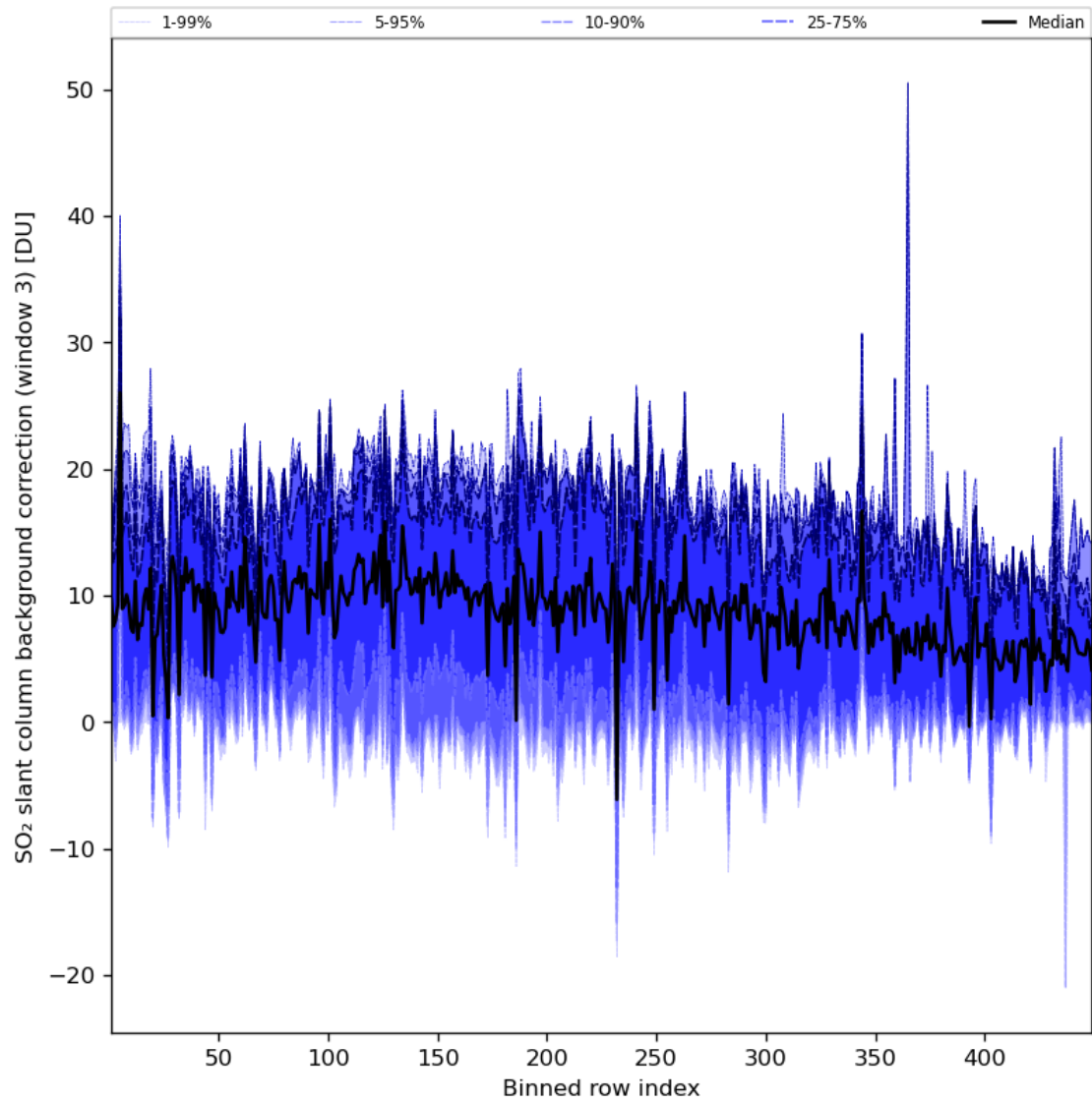
Figure 90: Along track statistics of “SO 2 slant column background correction (window 3)” for 2023-11-13 to 2023-11-14
