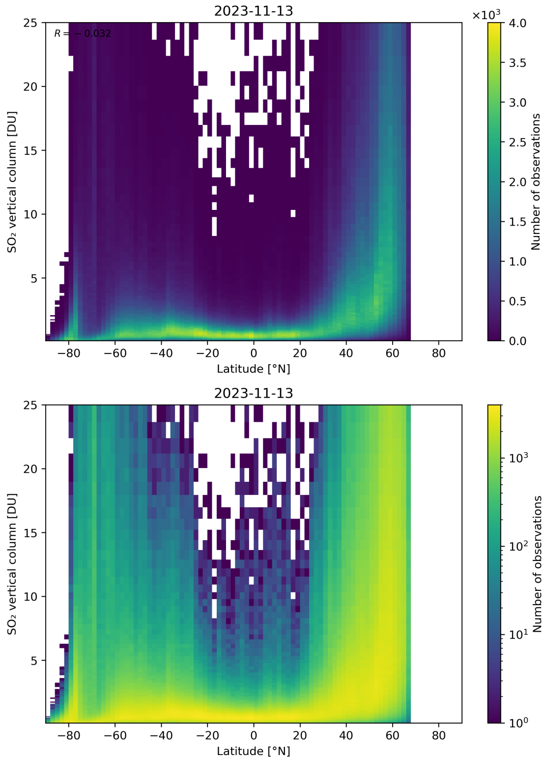
Figure 156: Scatter density plot of “Latitude” against “SO 2 vertical column” for 2023-11-13 to 2023-11-14.
