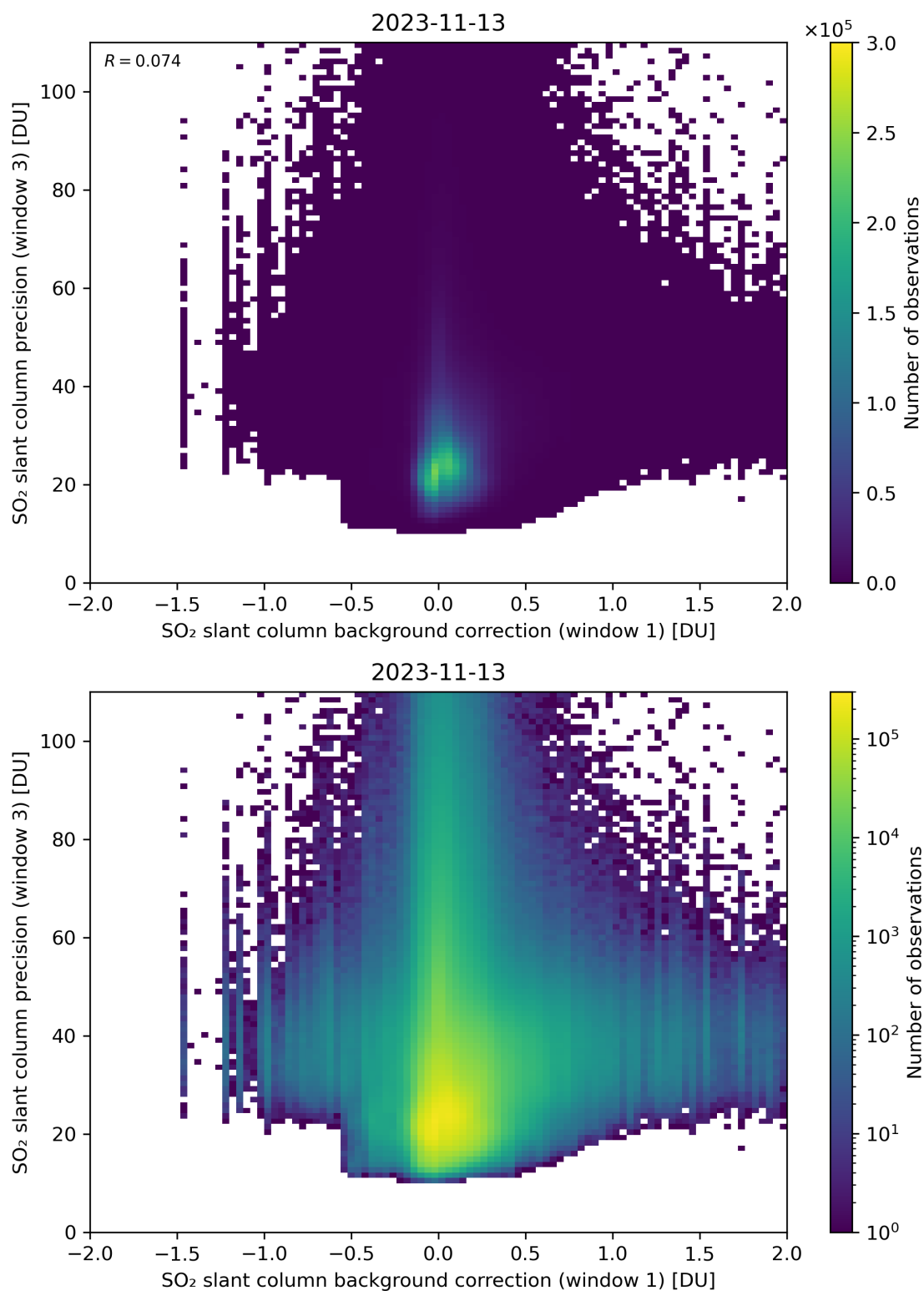
Figure 108: Scatter density plot of “SO 2 slant column background correction (window 1)” against “SO 2 slant column precision (window 3)” for 2023-11-13 to 2023-11-14.
