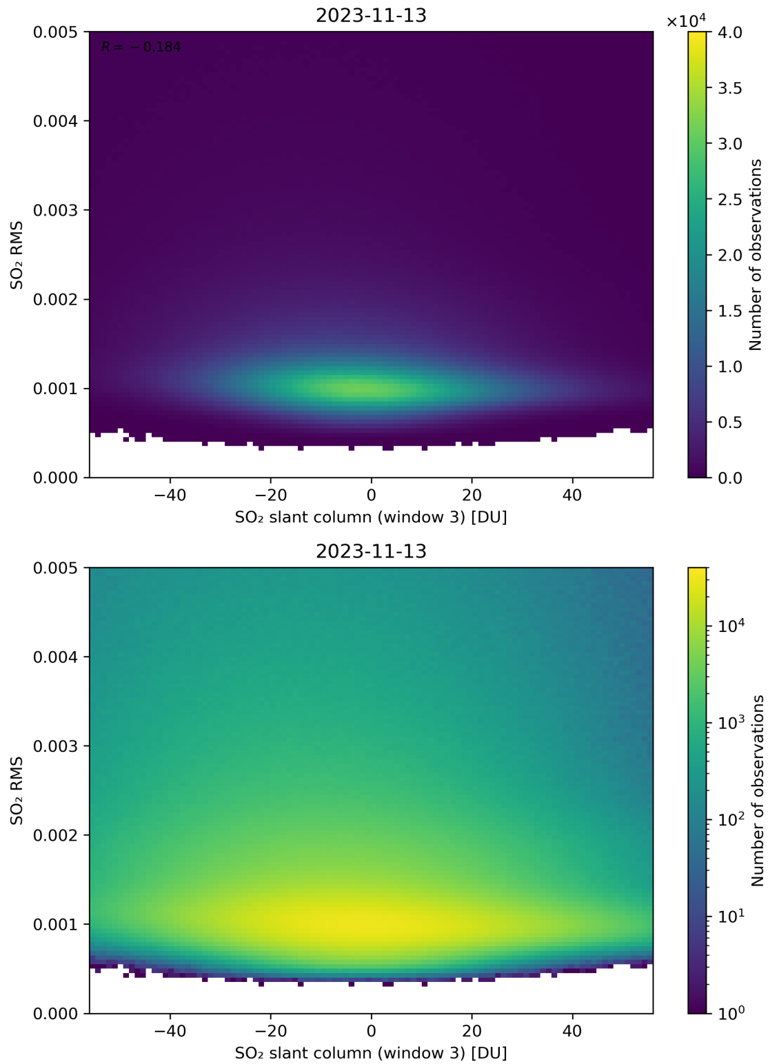
Figure 256: Scatter density plot of “SO 2 slant column (window 3)” against “SO 2 RMS” for 2023-11-13 to 2023-11-14.
