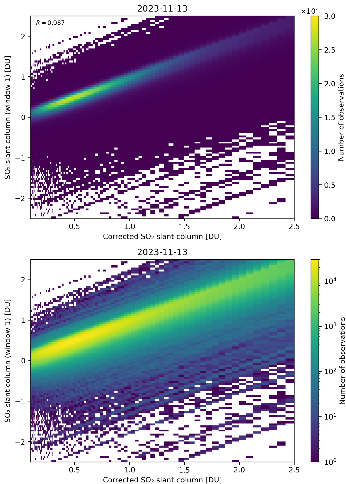
Figure 187: Scatter density plot of “Corrected SO 2 slant column” against “SO 2 slant column (window 1)” for 2023-11-13 to 2023-11-14.
