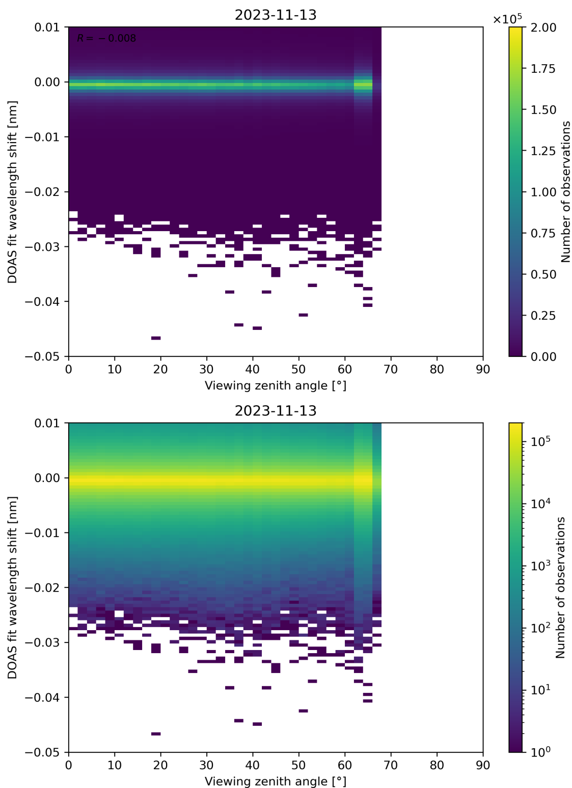
Figure 311: Scatter density plot of “Viewing zenith angle” against “DOAS fit wavelength shift” for 2023-11-13 to 2023-11-14.
