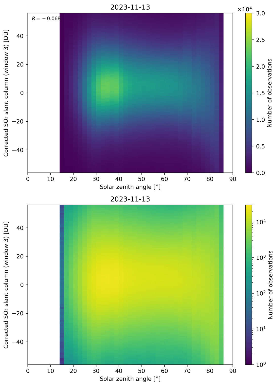
Figure 168: Scatter density plot of “Solar zenith angle” against “Corrected SO 2 slant column (window 3)” for 2023-11-13 to 2023-11-14.
