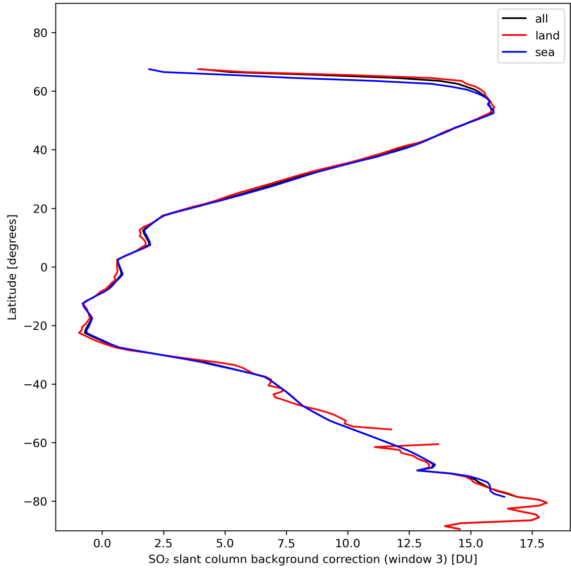
Figure 44: Zonal average of “SO 2 slant column background correction (window 3)” for 2023-11-13 to 2023-11-14.
