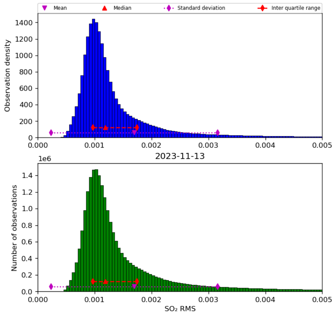
Figure 70: Histogram of “SO 2 RMS” for 2023-11-13 to 2023-11-14
