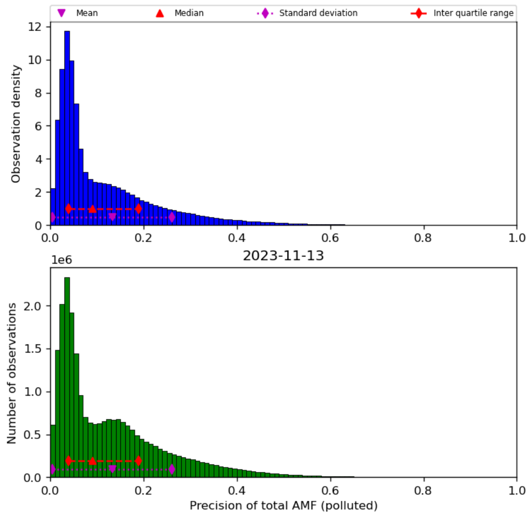
Figure 72: Histogram of “Precision of total AMF (polluted)” for 2023-11-13 to 2023-11-14
