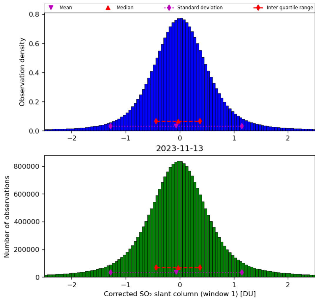
Figure 58: Histogram of “Corrected SO 2 slant column (window 1)” for 2023-11-13 to 2023-11-14
