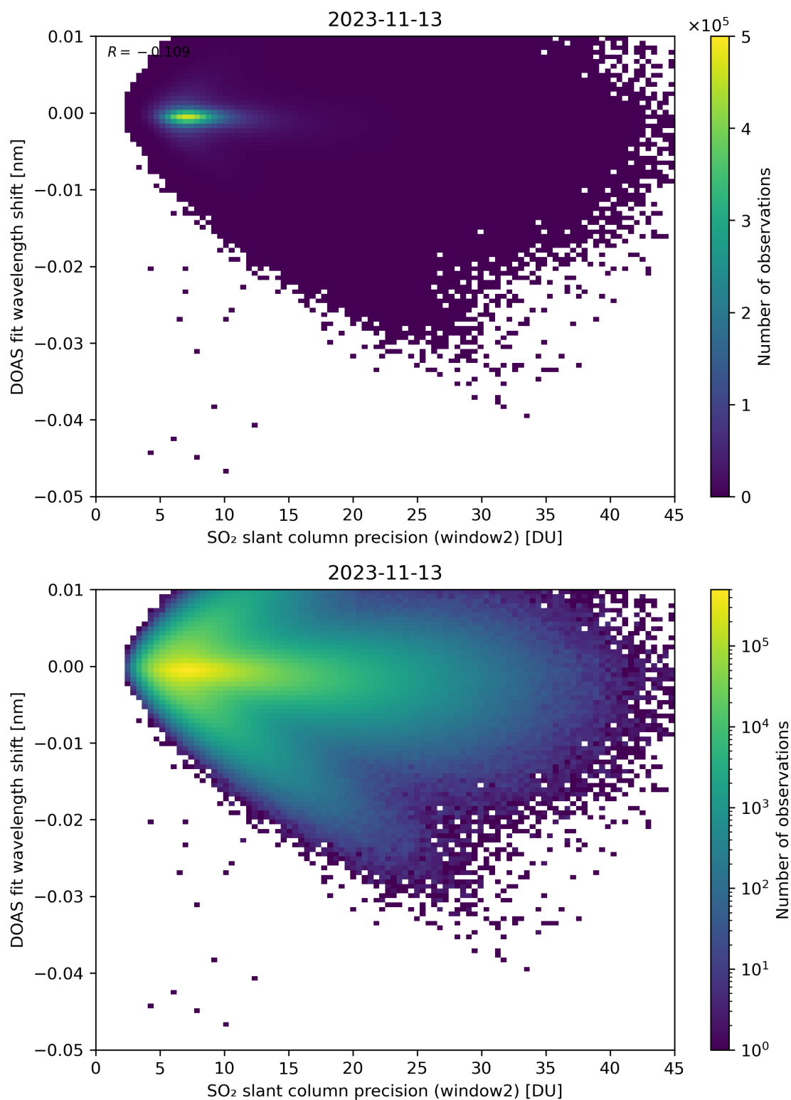
Figure 243: Scatter density plot of “SO 2 slant column precision (window2)” against “DOAS fit wavelength shift” for 2023-11-13 to 2023-11-14.
