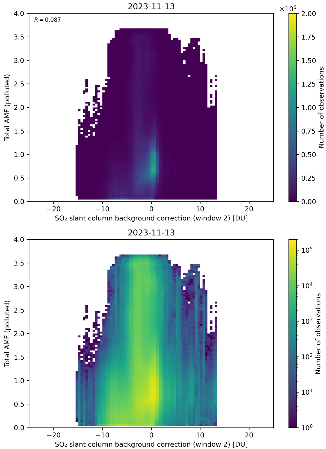
Figure 119: Scatter density plot of “SO 2 slant column background correction (window 2)” against “Total AMF (polluted)” for 2023-11-13 to 2023-11-14.
