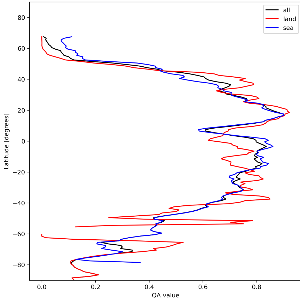
Figure 29: Zonal average of “QA value” for 2023-11-13 to 2023-11-14.
