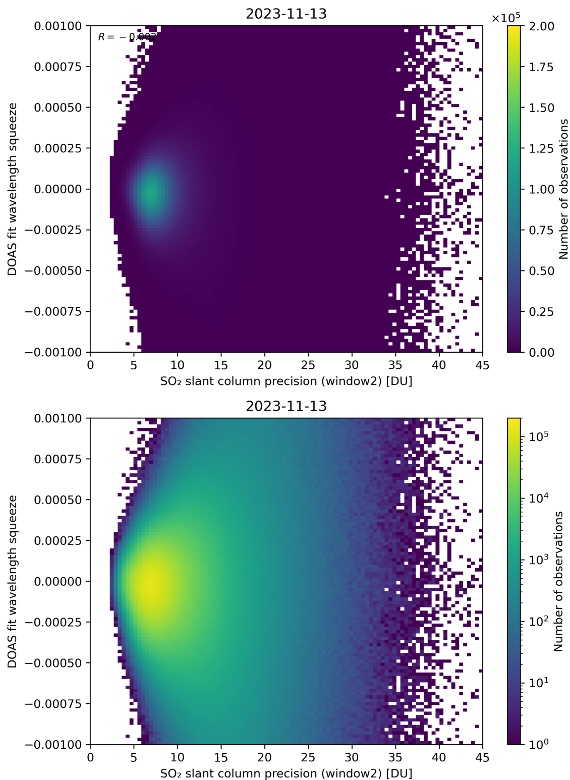
Figure 244: Scatter density plot of “SO 2 slant column precision (window2)” against “DOAS fit wavelength squeeze” for 2023-11-13 to 2023-11-14.
