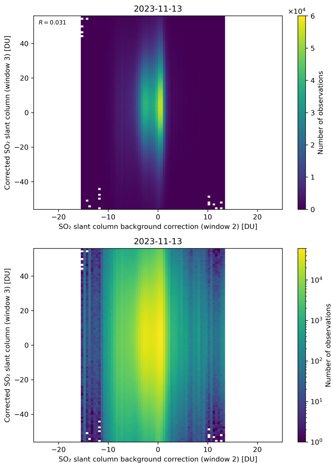
Figure 116: Scatter density plot of “SO 2 slant column background correction (window 2)” against “Corrected SO 2 slant column (window 3)” for 2023-11-13 to 2023-11-14.
