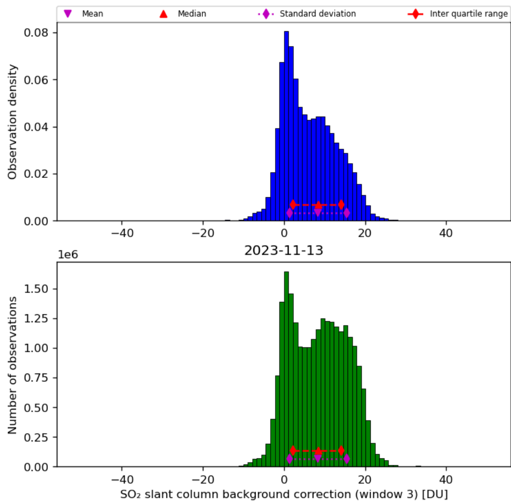
Figure 67: Histogram of “SO 2 slant column background correction (window 3)” for 2023-11-13 to 2023-11-14
