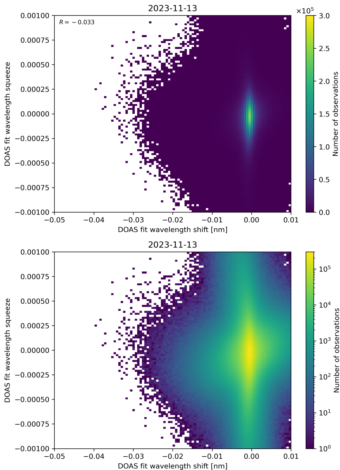
Figure 127: Scatter density plot of “DOAS fit wavelength shift” against “DOAS fit wavelength squeeze” for 2023-11-13 to 2023-11-14.
