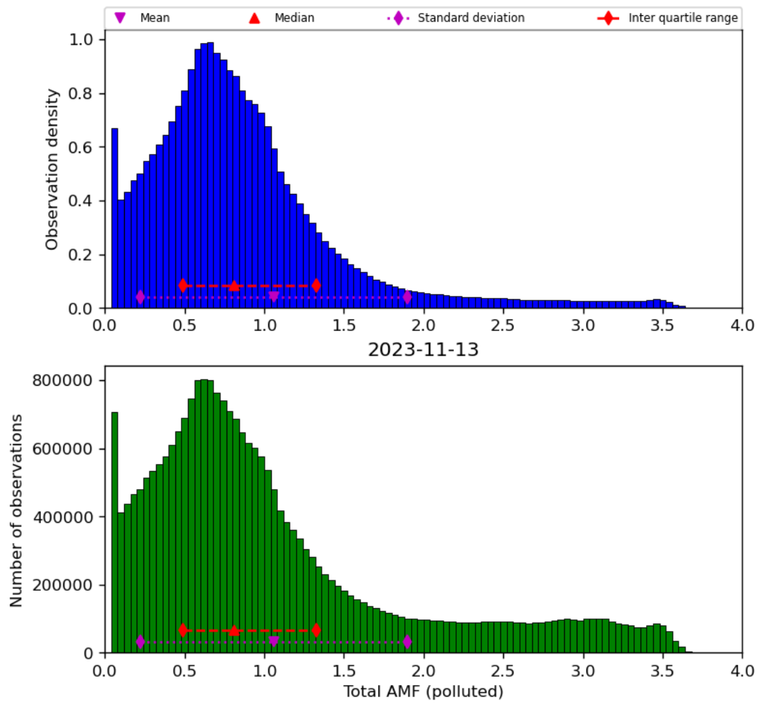
Figure 71: Histogram of “Total AMF (polluted)” for 2023-11-13 to 2023-11-14
