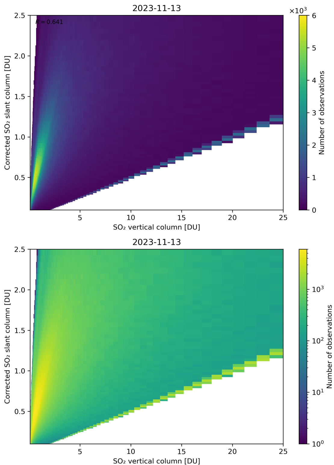
Figure 297: Scatter density plot of “SO 2 vertical column” against “Corrected SO 2 slant column” for 2023-11-13 to 2023-11-14.
