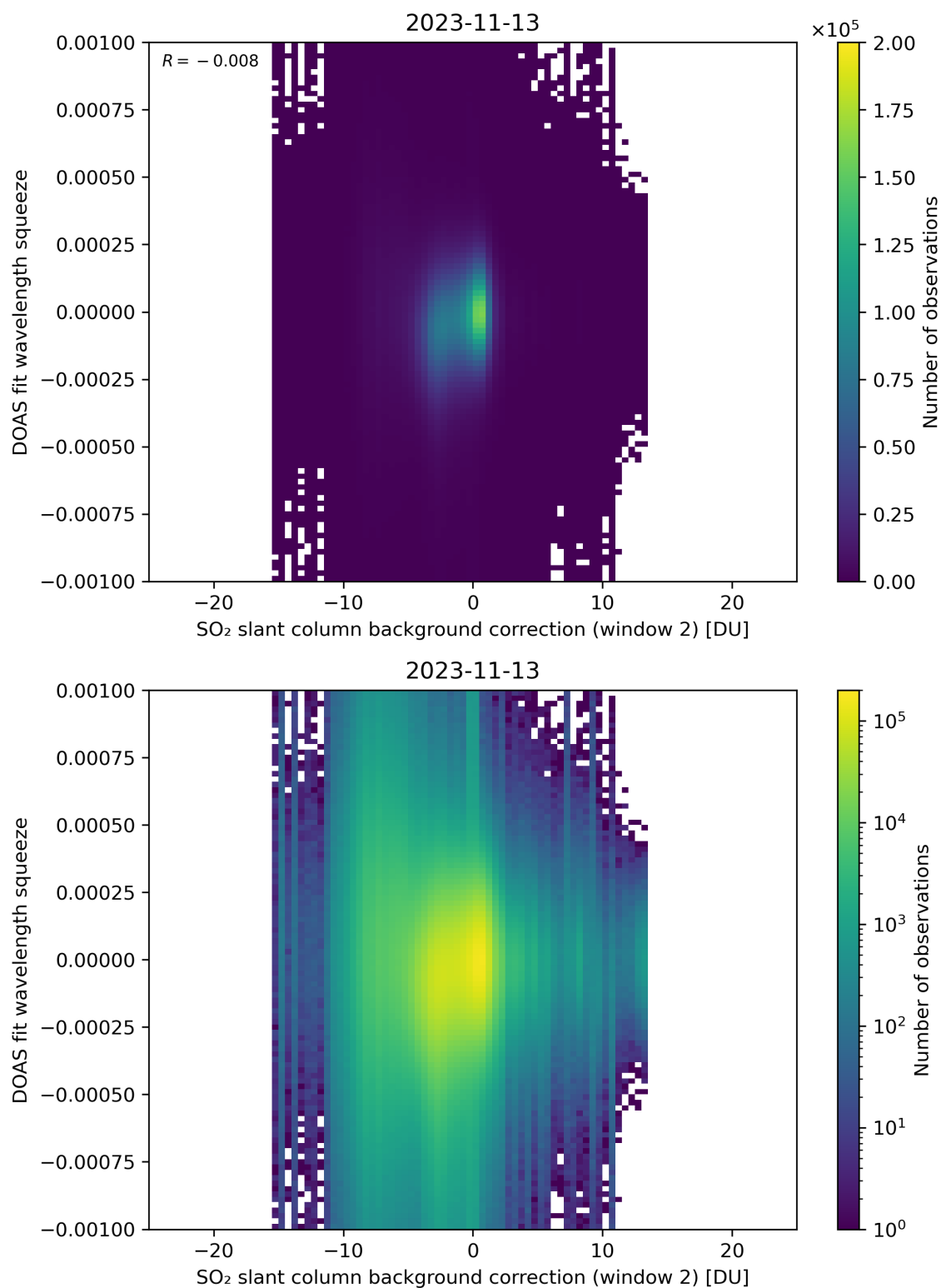
Figure 113: Scatter density plot of “SO 2 slant column background correction (window 2)” against “DOAS fit wavelength squeeze” for 2023-11-13 to 2023-11-14.
