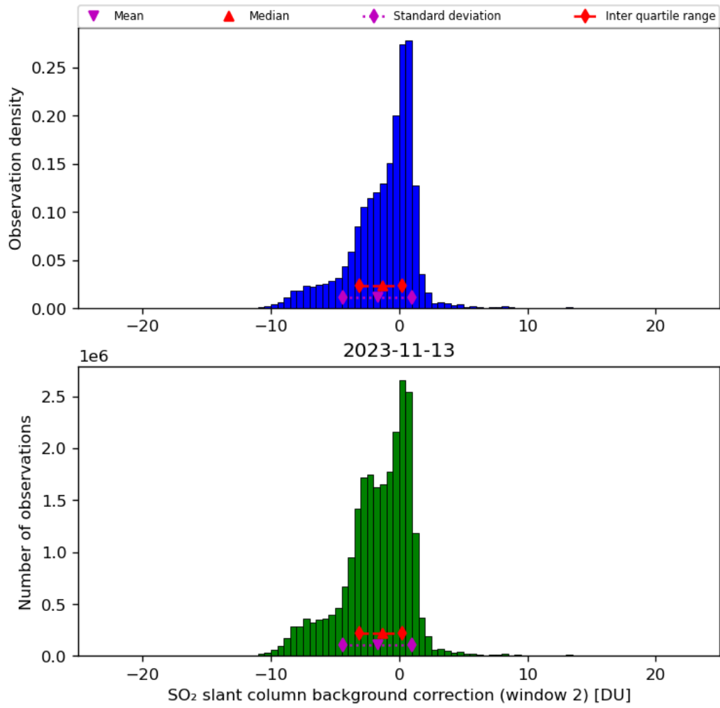
Figure 63: Histogram of “SO 2 slant column background correction (window 2)” for 2023-11-13 to 2023-11-14
