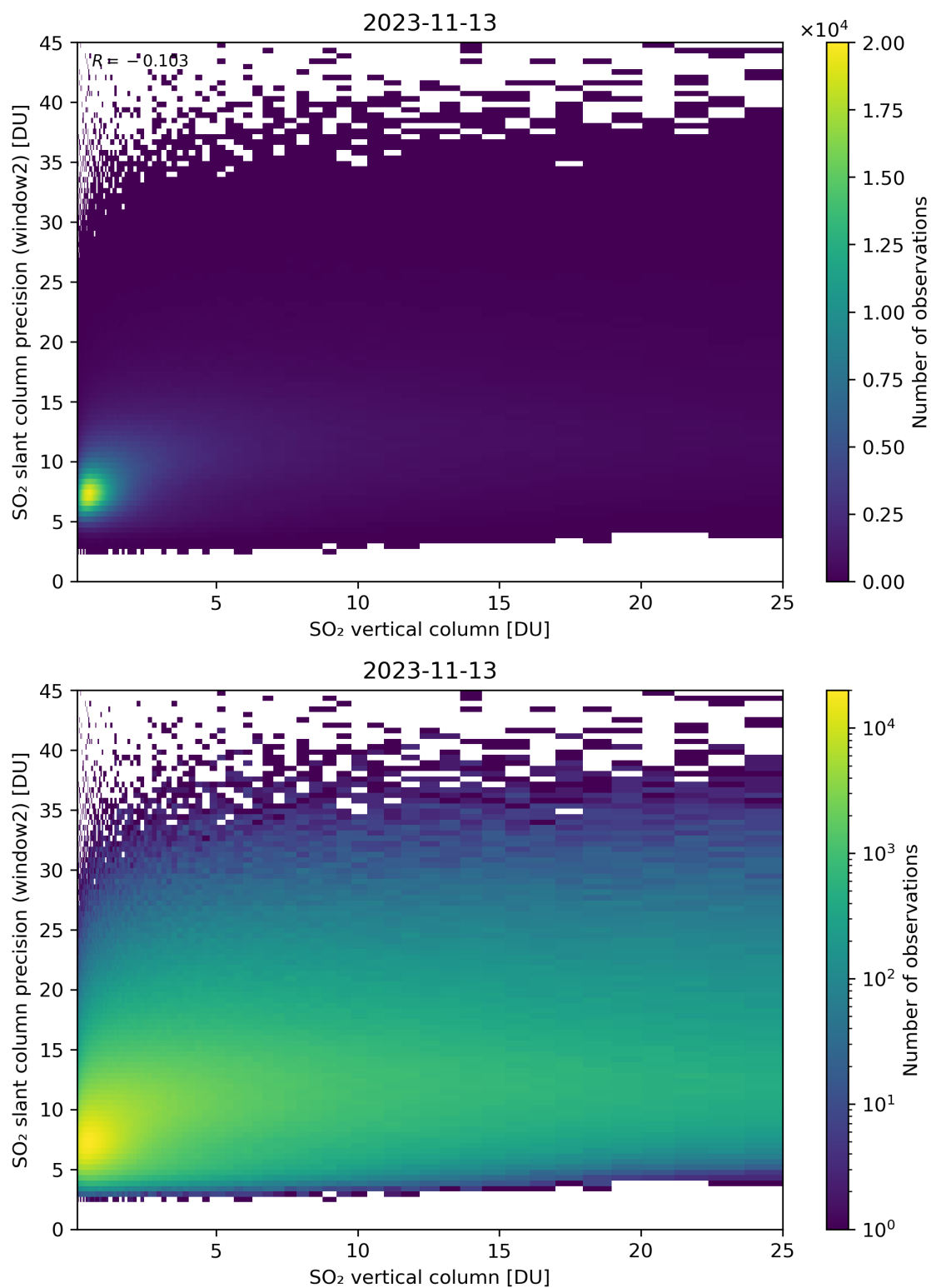
Figure 302: Scatter density plot of “SO 2 vertical column” against “SO 2 slant column precision (window2)” for 2023-11-13 to 2023-11-14.
