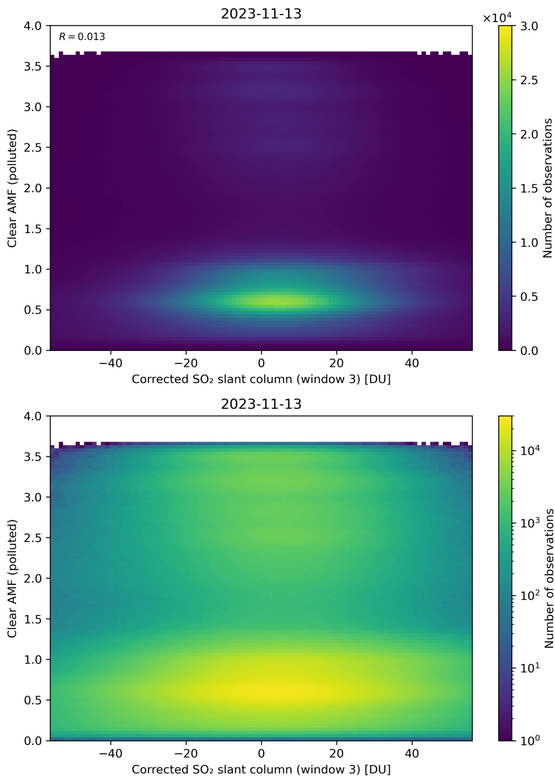
Figure 209: Scatter density plot of “Corrected SO 2 slant column (window 3)” against “Clear AMF (polluted)” for 2023-11-13 to 2023-11-14.
