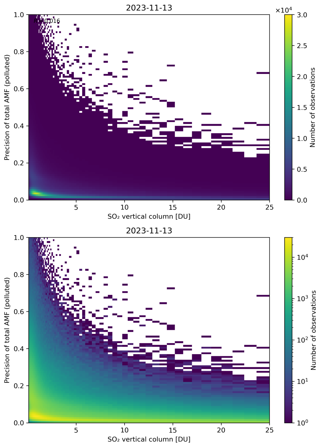
Figure 306: Scatter density plot of “SO 2 vertical column” against “Precision of total AMF (polluted)” for 2023-11-13 to 2023-11-14.
