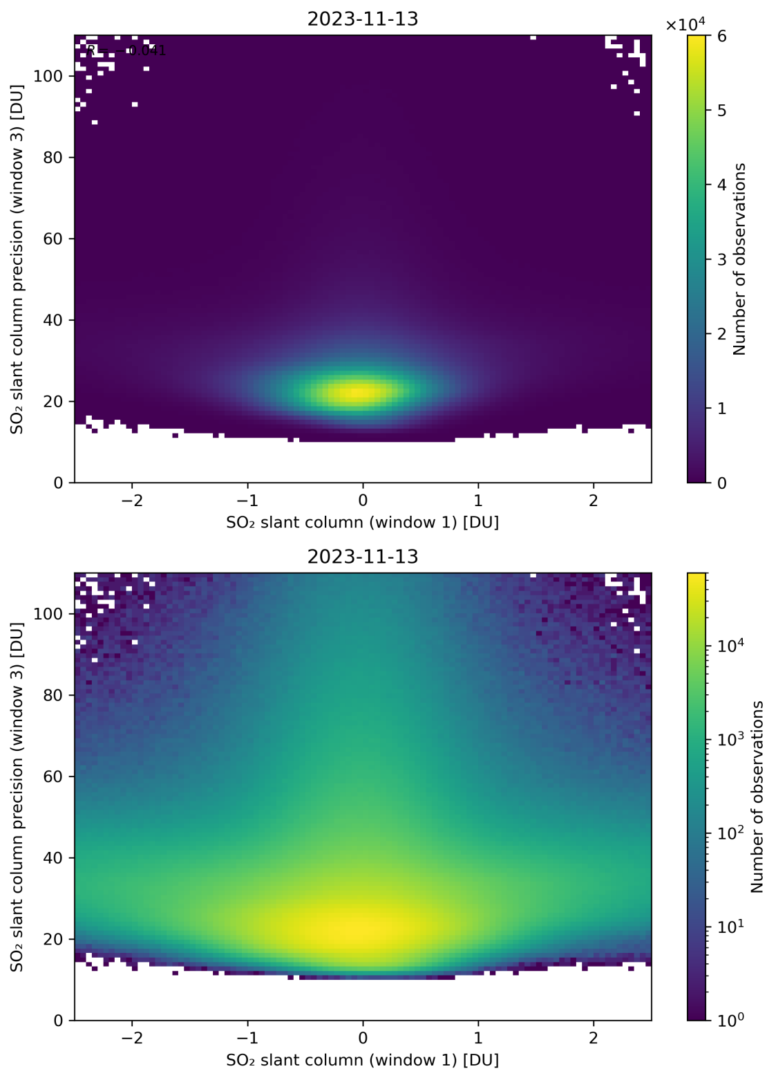
Figure 238: Scatter density plot of “SO 2 slant column (window 1)” against “SO 2 slant column precision (window 3)” for 2023-11-13 to 2023-11-14.
