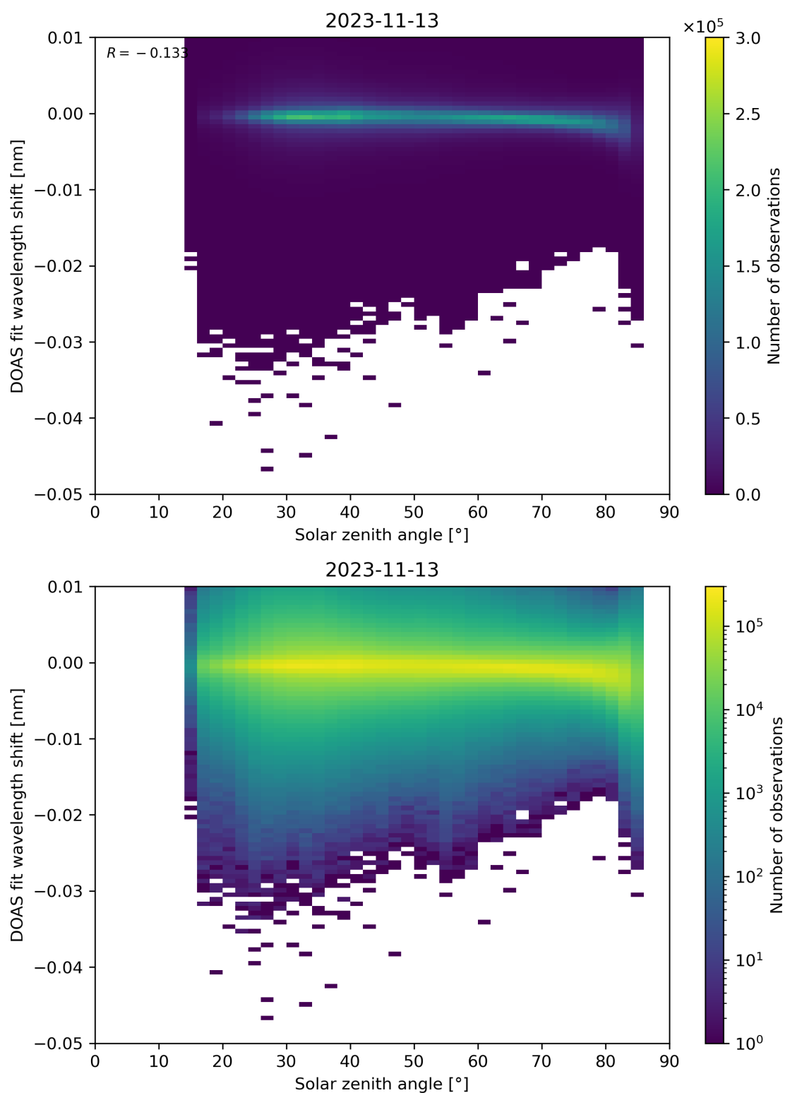
Figure 161: Scatter density plot of “Solar zenith angle” against “DOAS fit wavelength shift” for 2023-11-13 to 2023-11-14.
