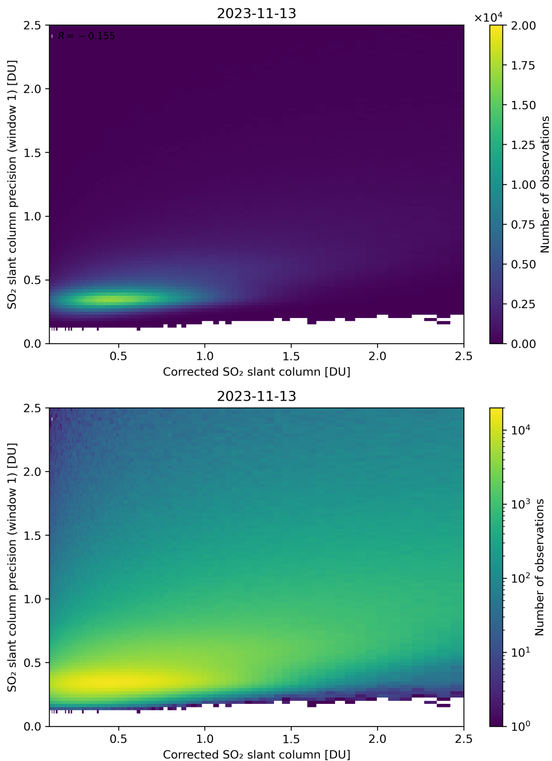
Figure 188: Scatter density plot of “Corrected SO 2 slant column” against “SO 2 slant column precision (window 1)” for 2023-11-13 to 2023-11-14.
