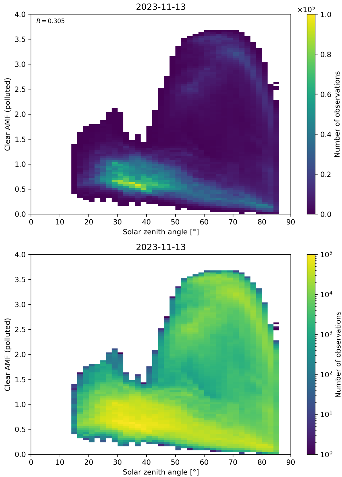
Figure 165: Scatter density plot of “Solar zenith angle” against “Clear AMF (polluted)” for 2023-11-13 to 2023-11-14.
