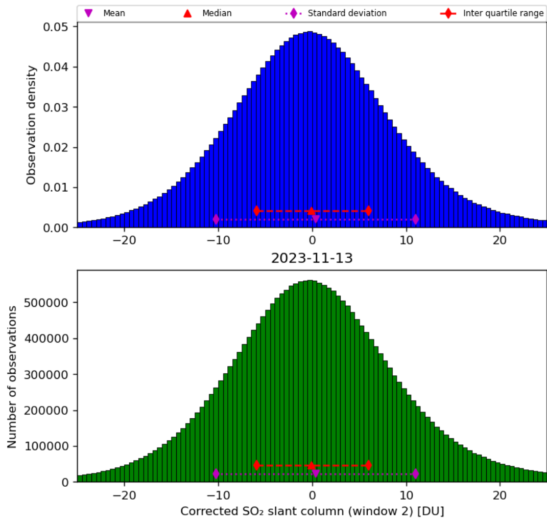
Figure 62: Histogram of “Corrected SO 2 slant column (window 2)” for 2023-11-13 to 2023-11-14
