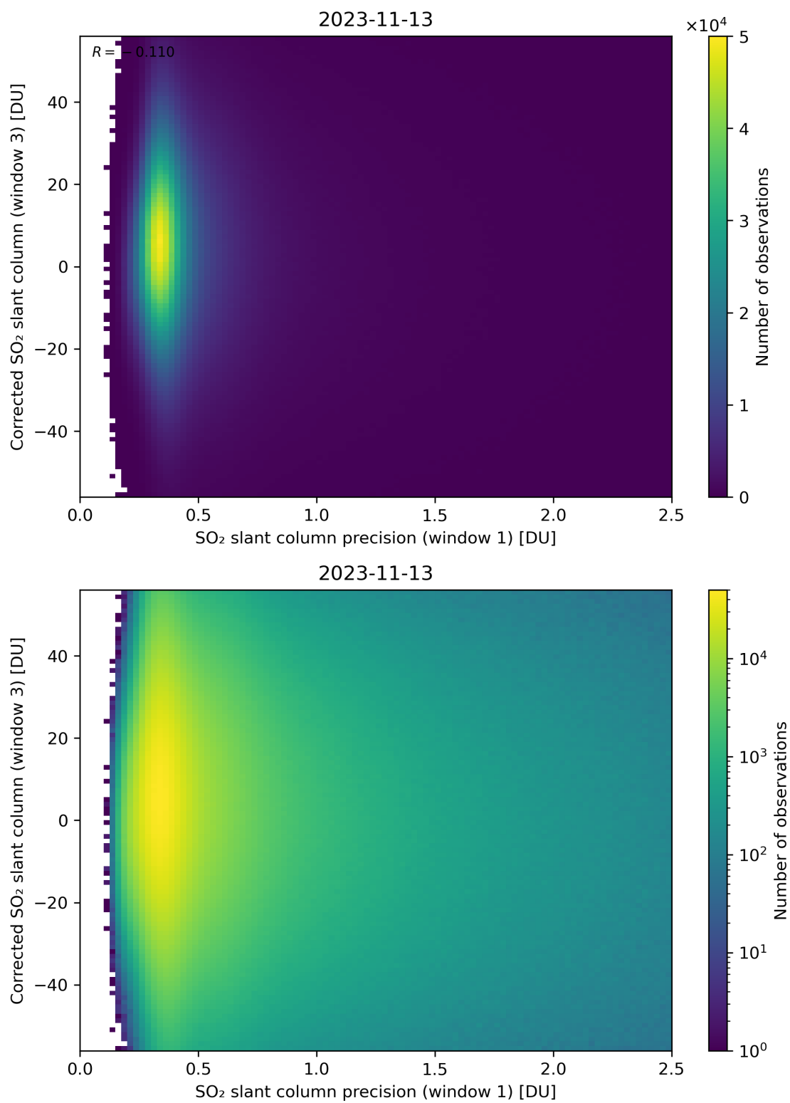
Figure 226: Scatter density plot of “SO 2 slant column precision (window 1)” against “Corrected SO 2 slant column (window 3)” for 2023-11-13 to 2023-11-14.
