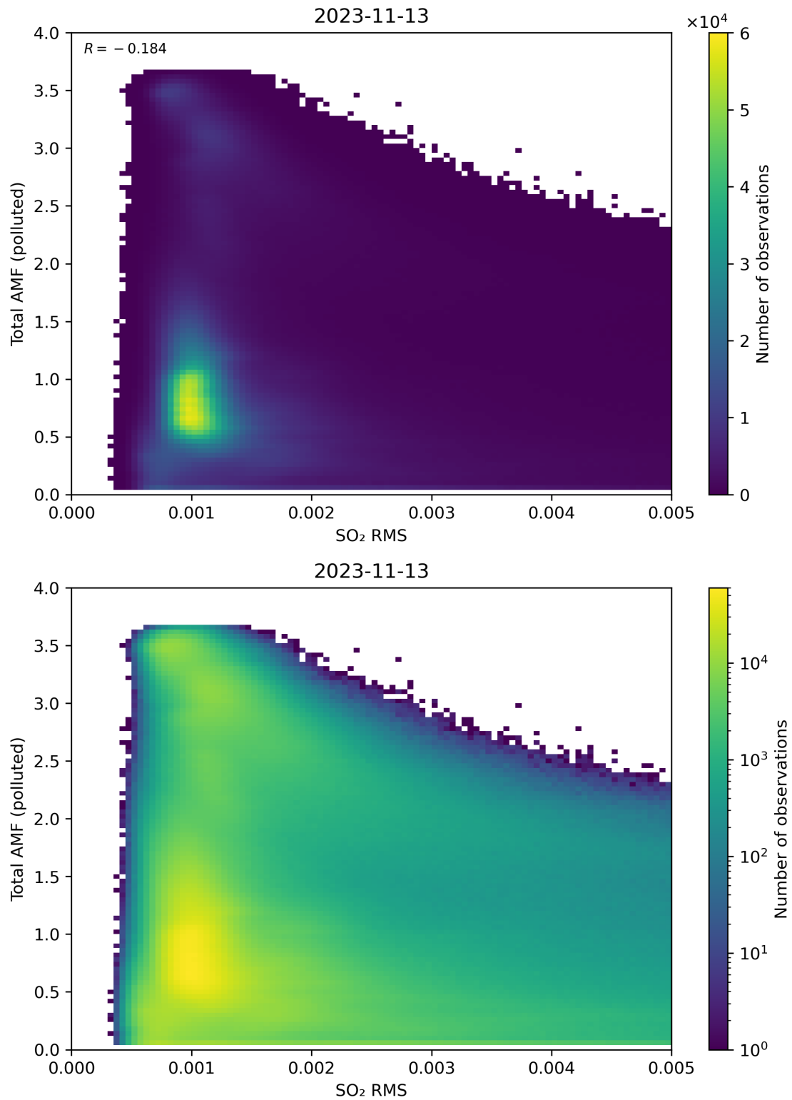
Figure 137: Scatter density plot of “SO 2 RMS” against “Total AMF (polluted)” for 2023-11-13 to 2023-11-14.
