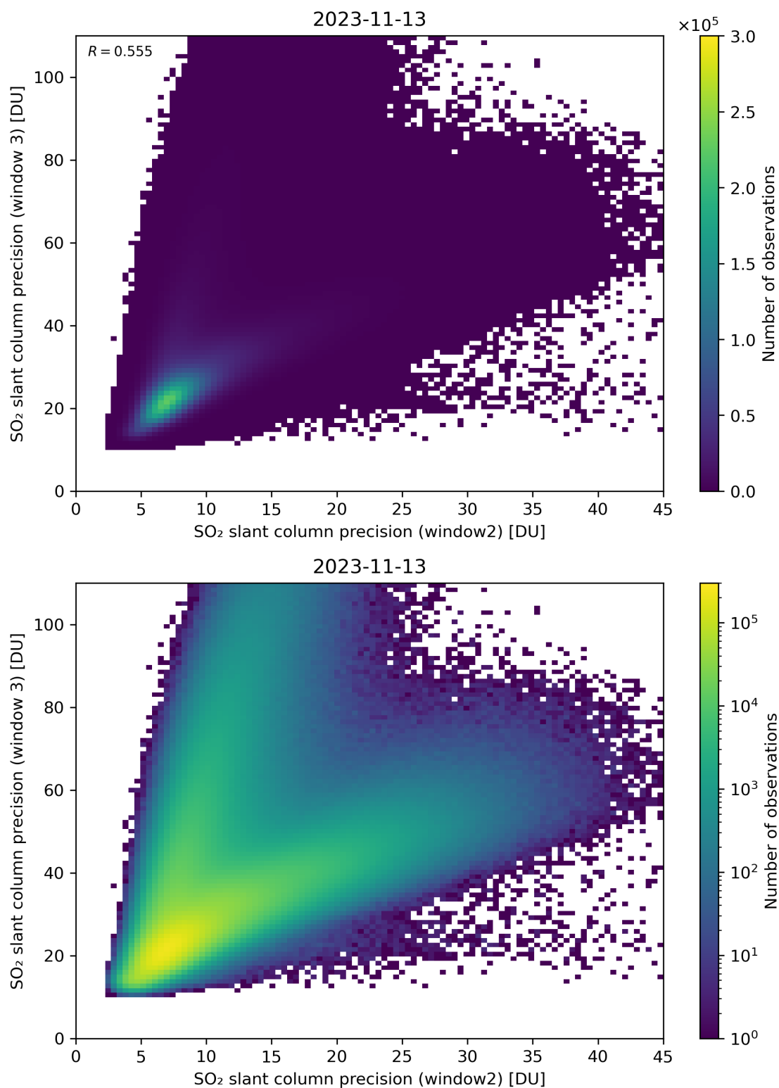
Figure 250: Scatter density plot of “SO 2 slant column precision (window2)” against “SO 2 slant column precision (window 3)” for 2023-11-13 to 2023-11-14.
