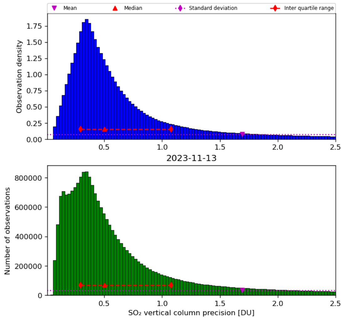
Figure 54: Histogram of “SO 2 vertical column precision” for 2023-11-13 to 2023-11-14
