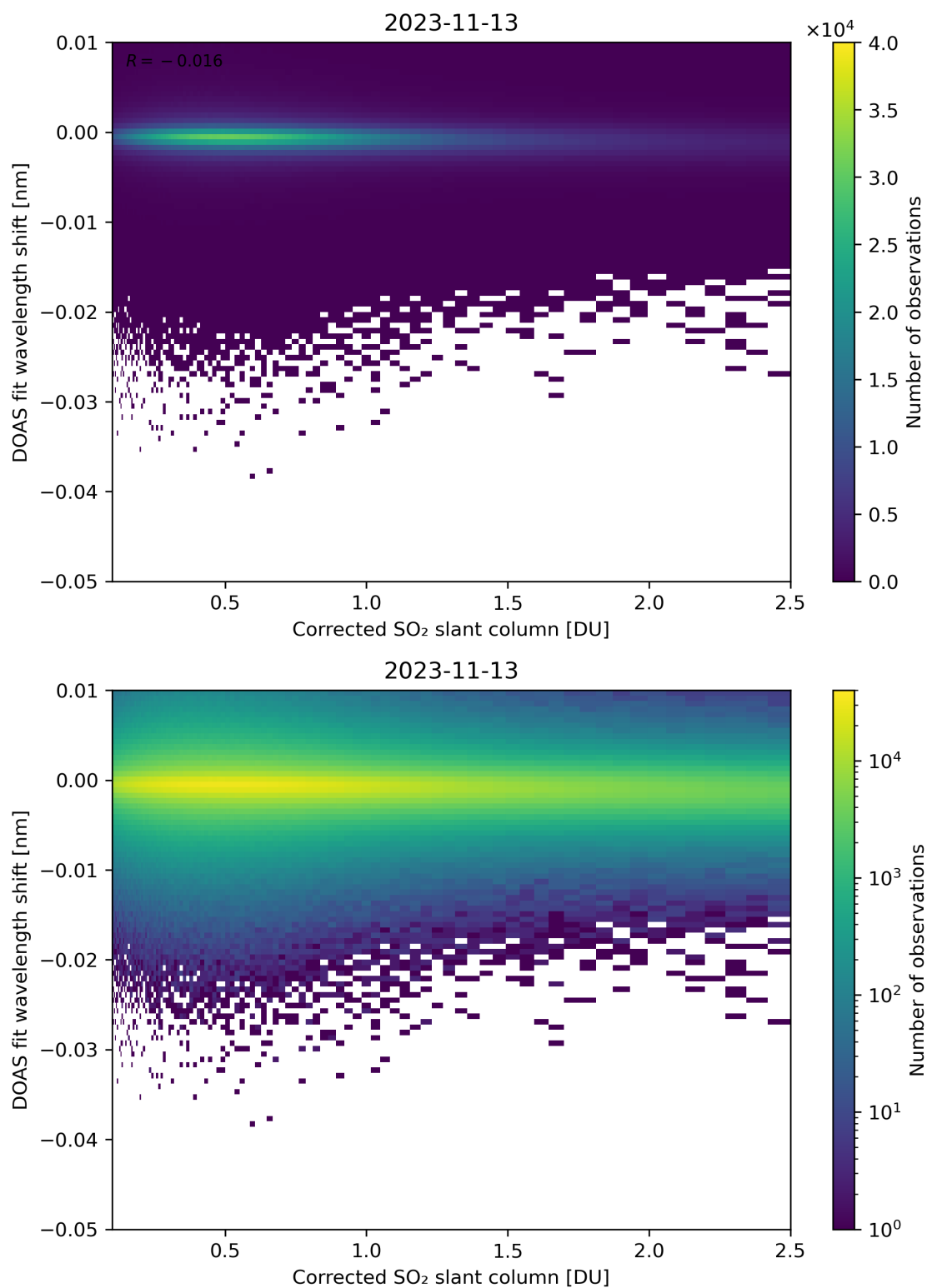
Figure 181: Scatter density plot of “Corrected SO 2 slant column” against “DOAS fit wavelength shift” for 2023-11-13 to 2023-11-14.
