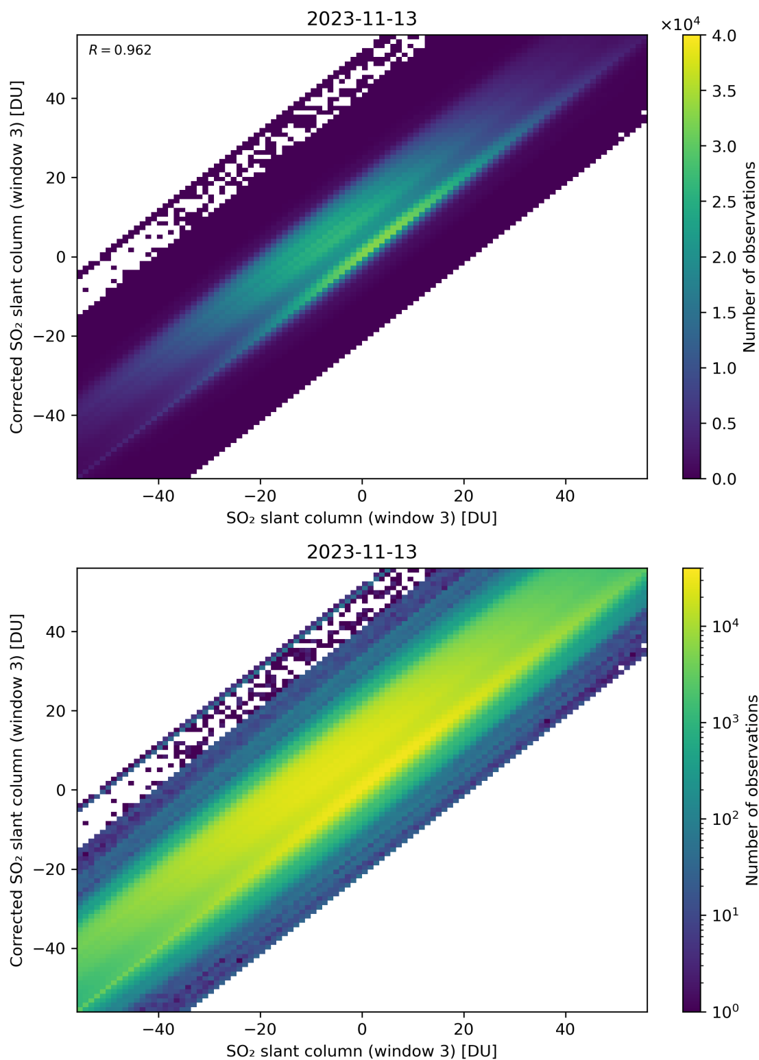
Figure 266: Scatter density plot of “SO 2 slant column (window 3)” against “Corrected SO 2 slant column (window 3)” for 2023-11-13 to 2023-11-14.
