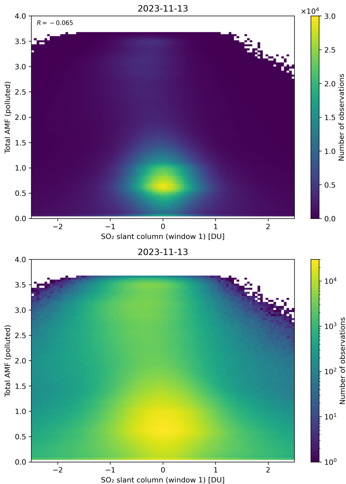
Figure 239: Scatter density plot of “SO 2 slant column (window 1)” against “Total AMF (polluted)” for 2023-11-13 to 2023-11-14.
