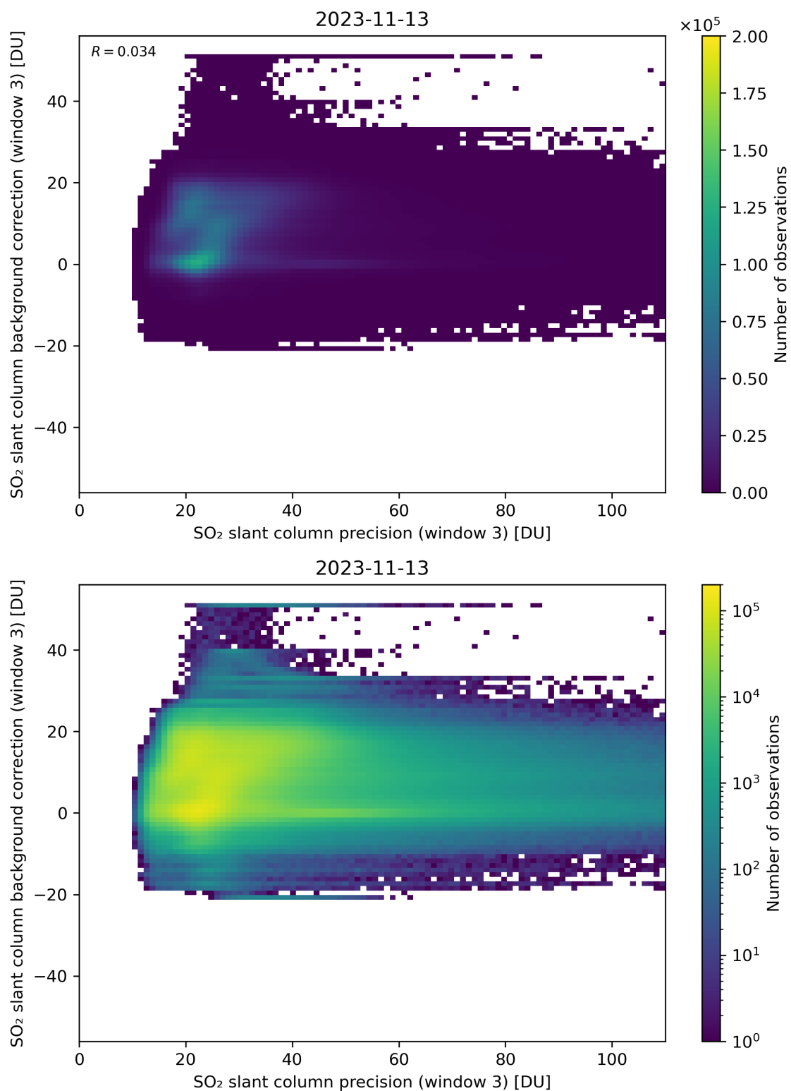
Figure 257: Scatter density plot of “SO 2 slant column precision (window 3)” against “SO 2 slant column background correction (window 3)” for 2023-11-13 to 2023-11-14.
