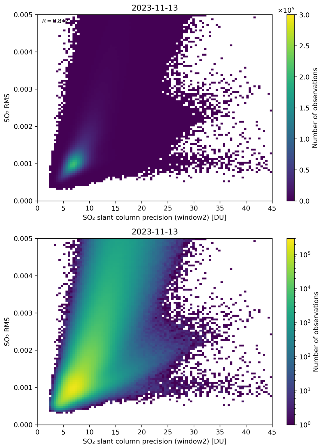
Figure 245: Scatter density plot of “SO 2 slant column precision (window2)” against “SO 2 RMS” for 2023-11-13 to 2023-11-14.
