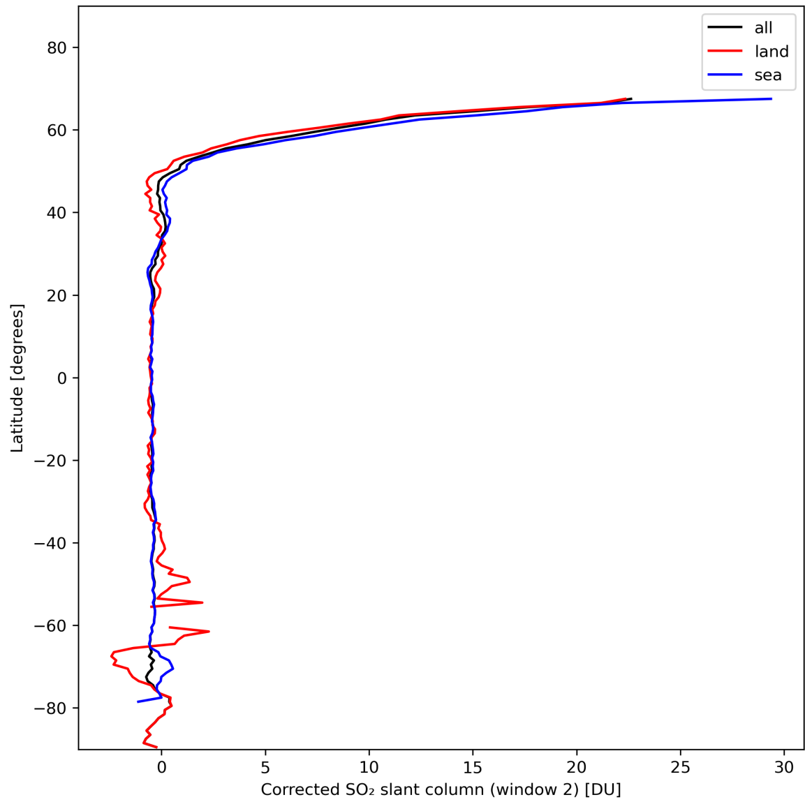
Figure 39: Zonal average of “Corrected SO 2 slant column (window 2)” for 2023-11-13 to 2023-11-14.
