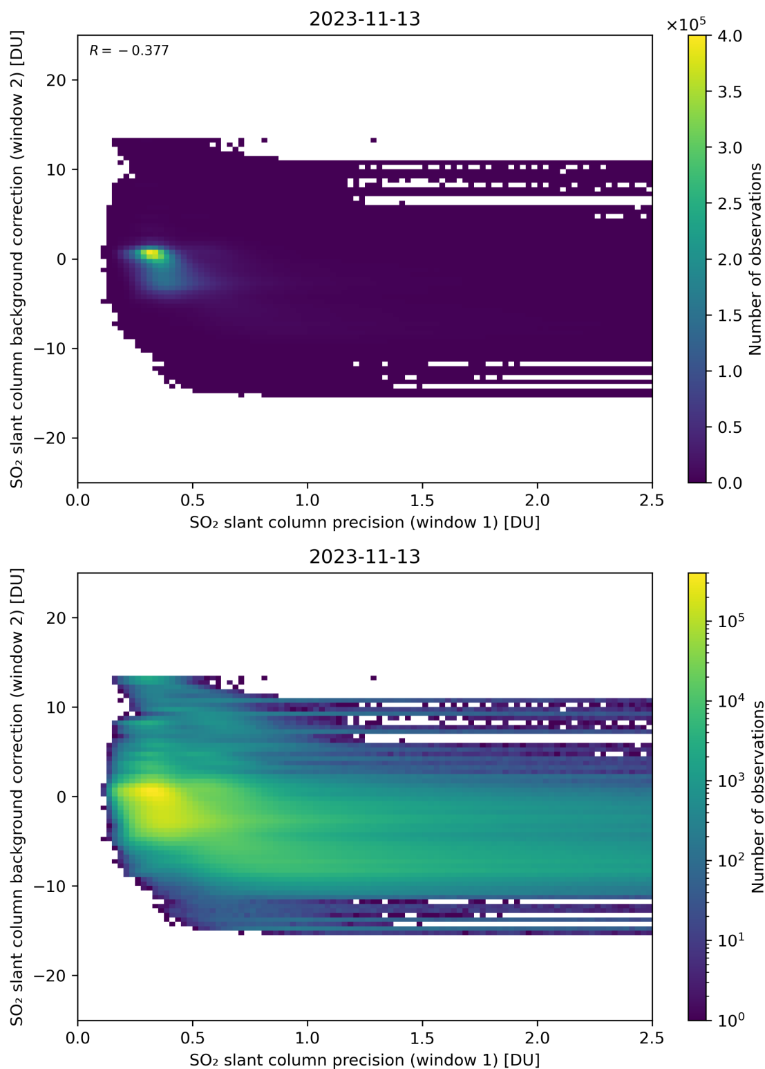
Figure 219: Scatter density plot of “SO 2 slant column precision (window 1)” against “SO 2 slant column background correction (window 2)” for 2023-11-13 to 2023-11-14.
