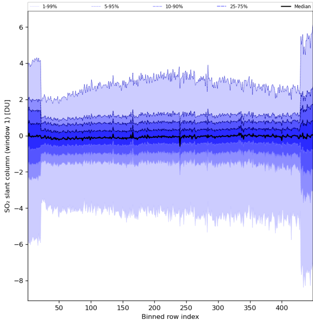
Figure 79: Along track statistics of “SO 2 slant column (window 1)” for 2023-11-13 to 2023-11-14
