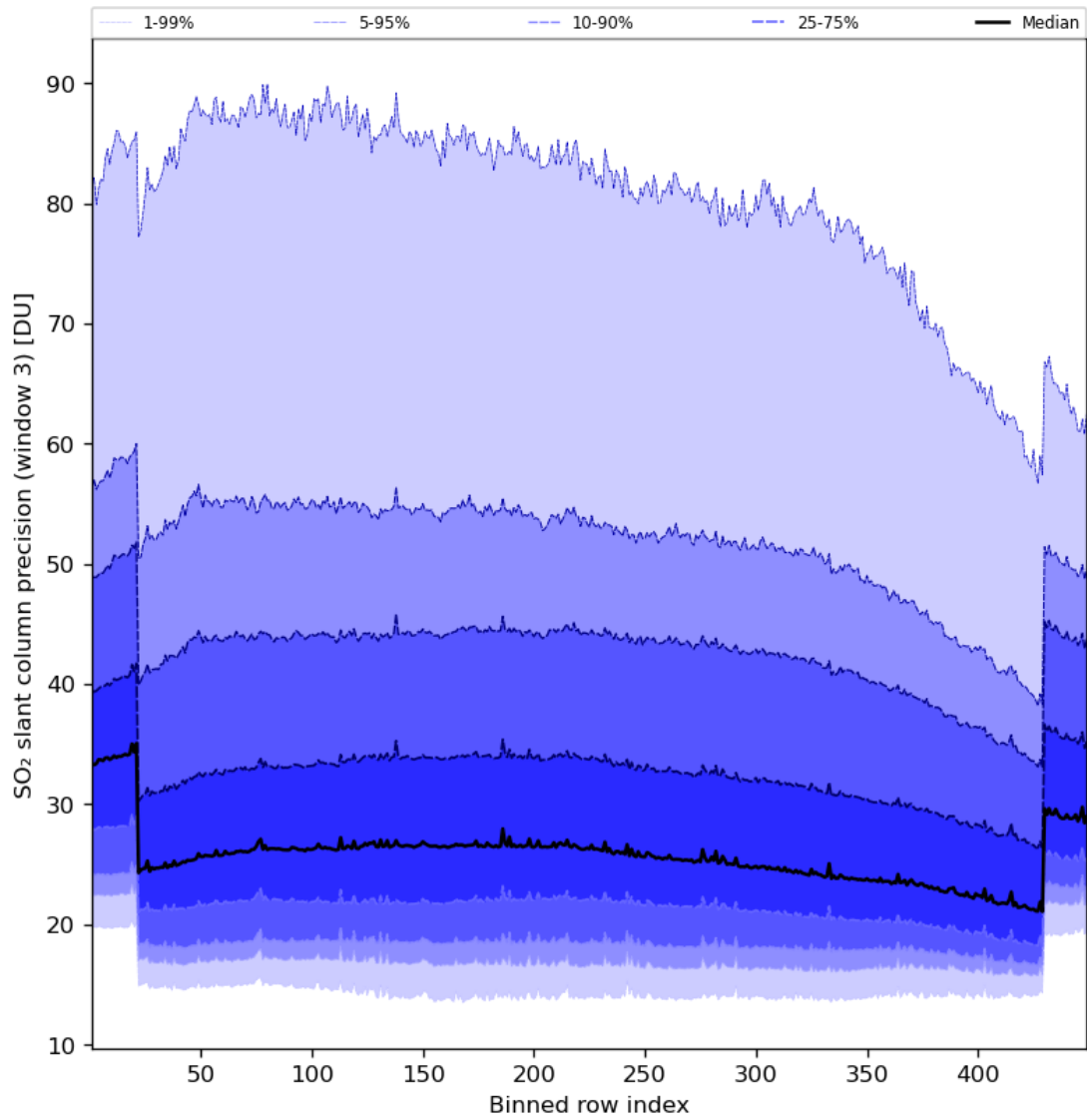
Figure 88: Along track statistics of “SO 2 slant column precision (window 3)” for 2023-11-13 to 2023-11-14
