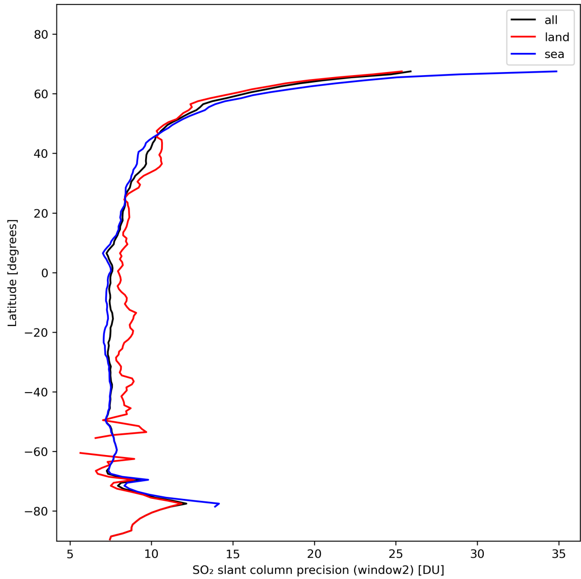
Figure 38: Zonal average of “SO 2 slant column precision (window2)” for 2023-11-13 to 2023-11-14.
