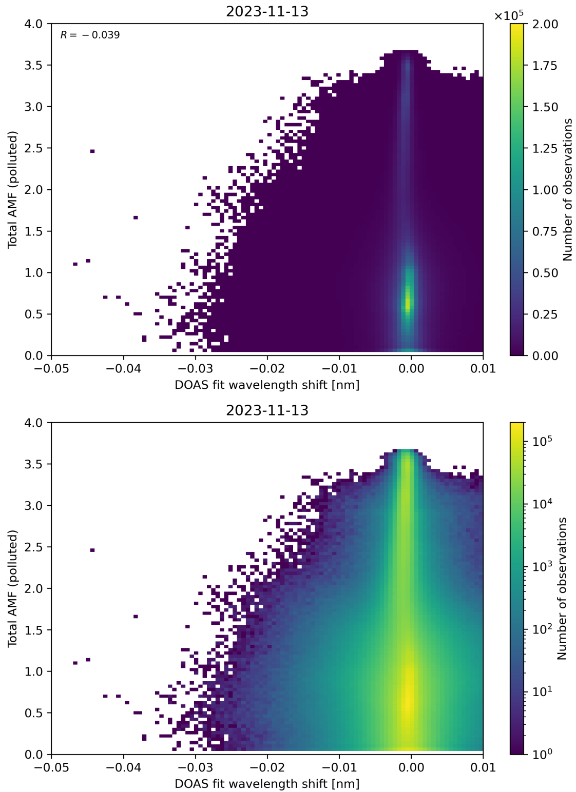
Figure 130: Scatter density plot of “DOAS fit wavelength shift” against “Total AMF (polluted)” for 2023-11-13 to 2023-11-14.
