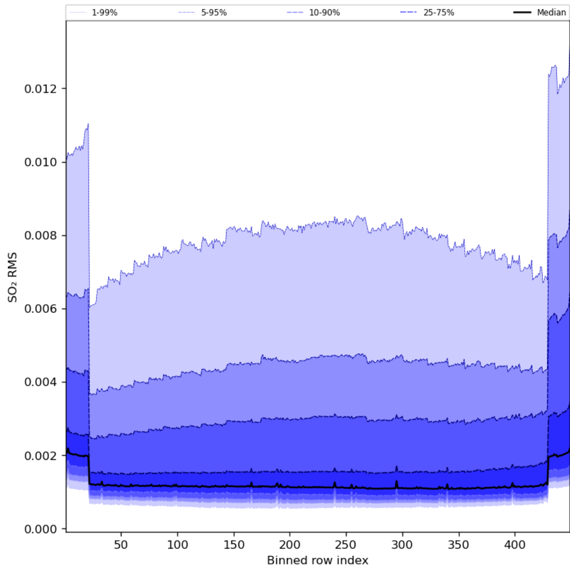
Figure 93: Along track statistics of “SO 2 RMS” for 2023-11-13 to 2023-11-14
