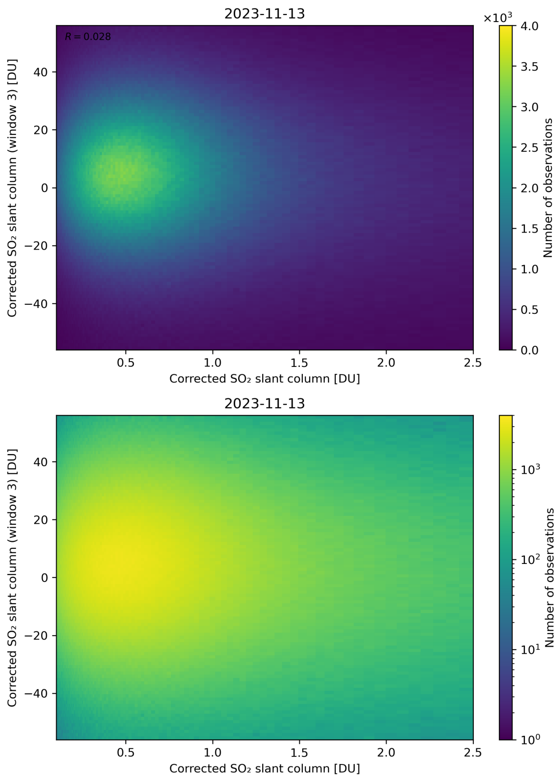
Figure 186: Scatter density plot of “Corrected SO 2 slant column” against “Corrected SO 2 slant column (window 3)” for 2023-11-13 to 2023-11-14.
