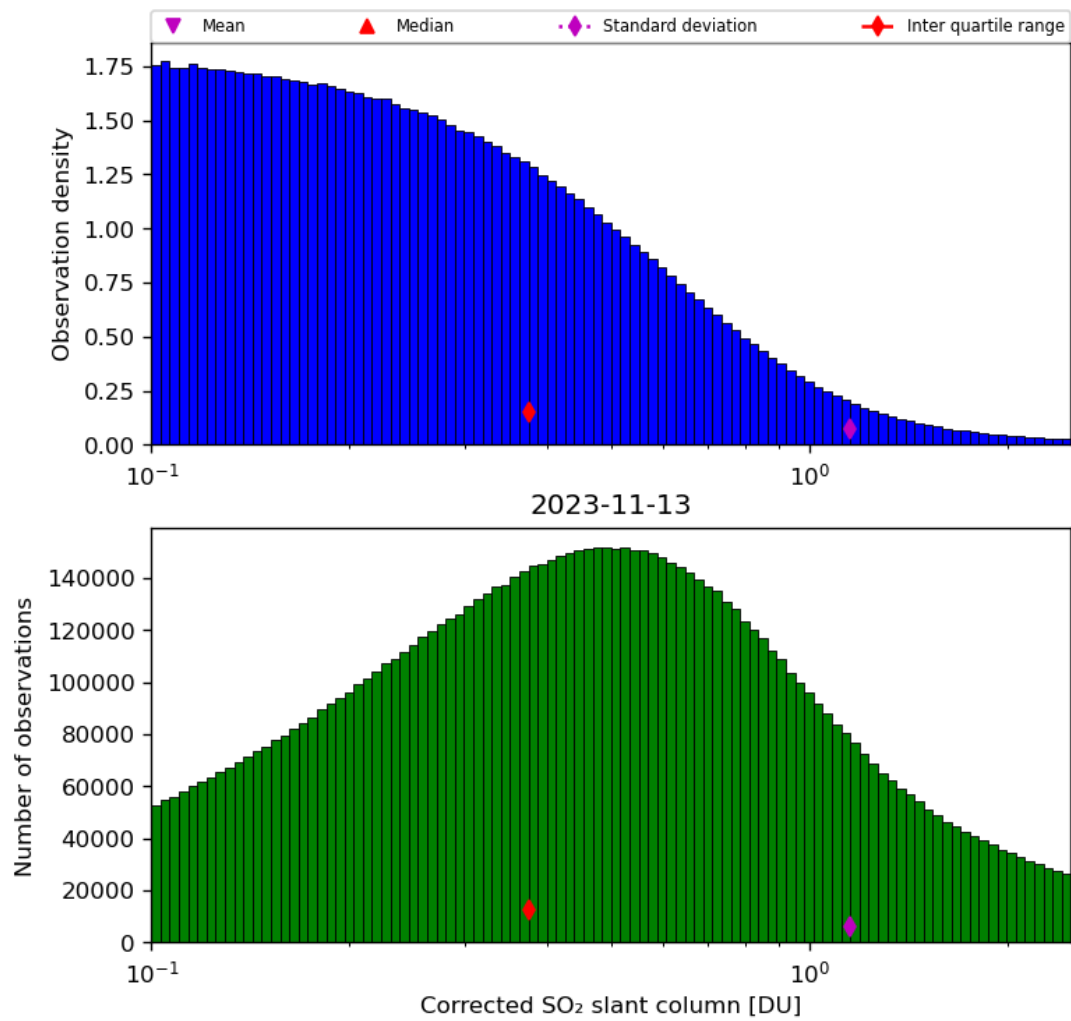
Figure 55: Histogram of “Corrected SO 2 slant column” for 2023-11-13 to 2023-11-14
