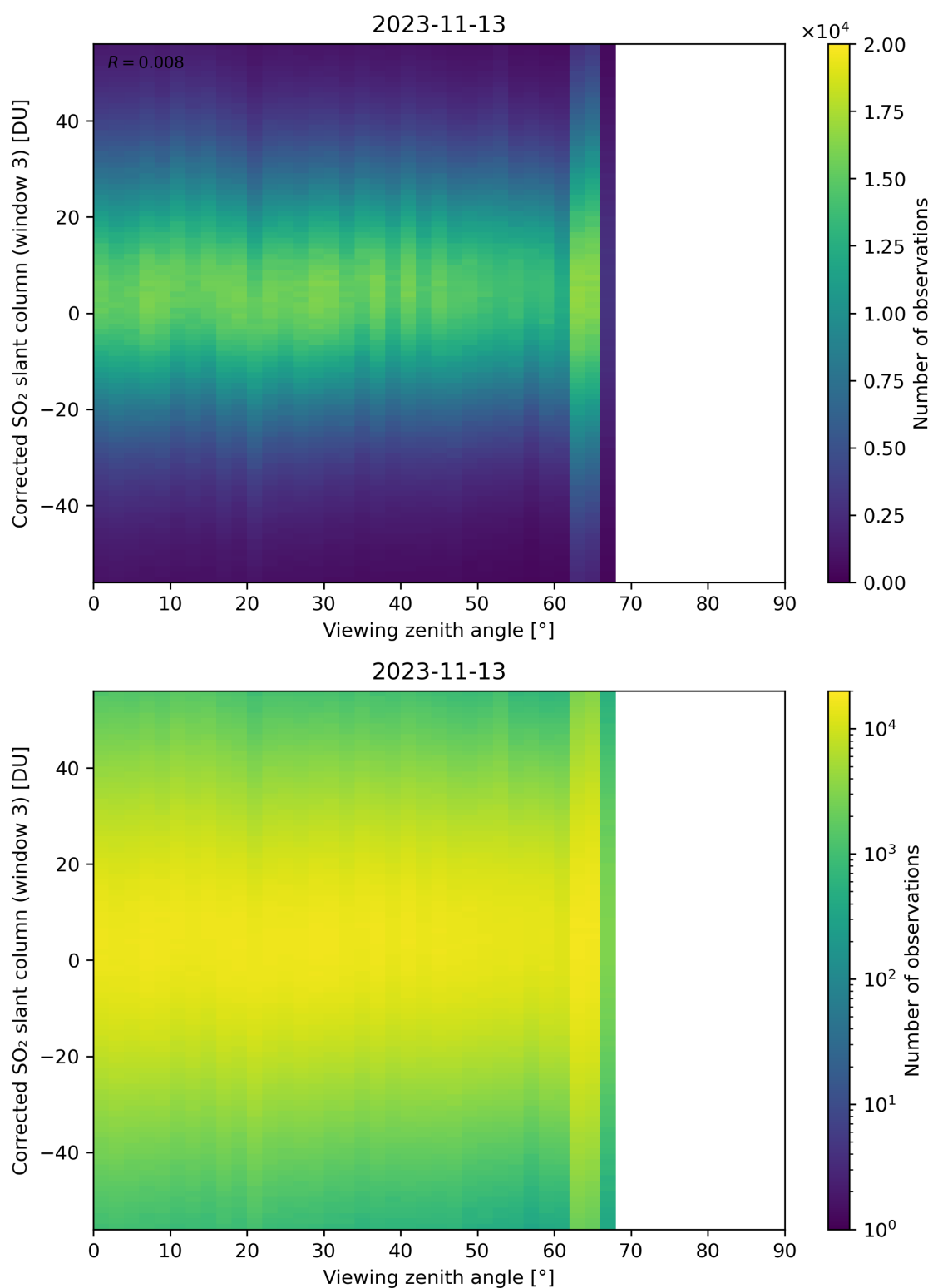
Figure 319: Scatter density plot of “Viewing zenith angle” against “Corrected SO 2 slant column (window 3)” for 2023-11-13 to 2023-11-14.
