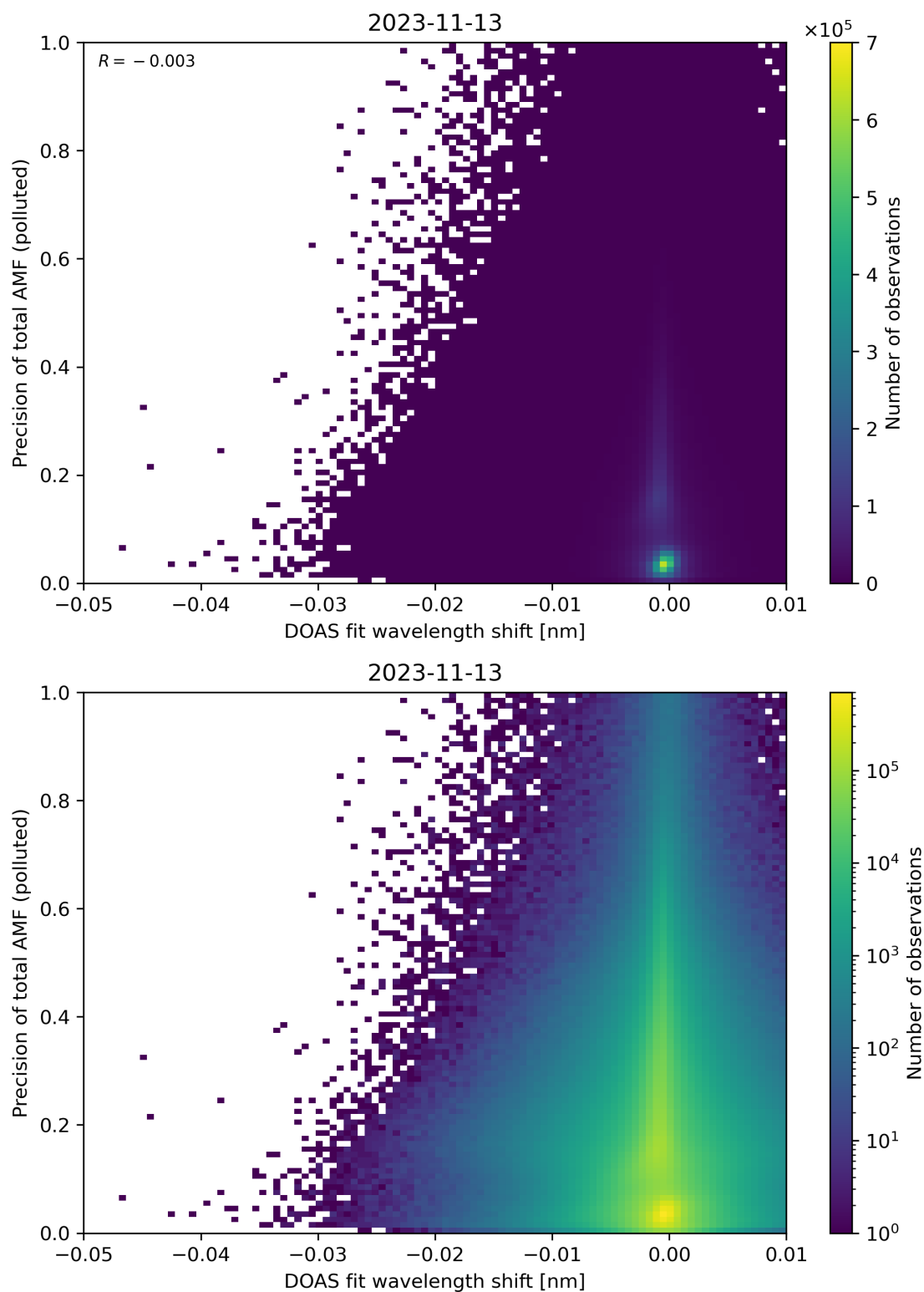
Figure 131: Scatter density plot of “DOAS fit wavelength shift” against “Precision of total AMF (polluted)” for 2023-11-13 to 2023-11-14.
