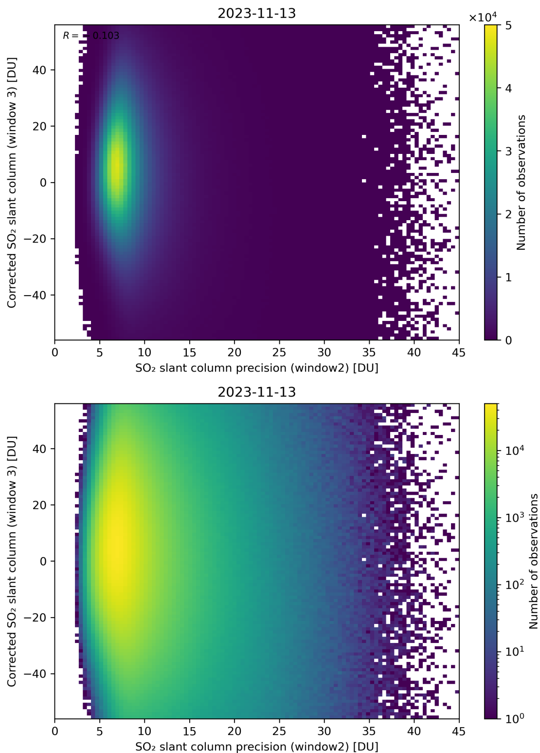
Figure 248: Scatter density plot of “SO 2 slant column precision (window2)” against “Corrected SO 2 slant column (window 3)” for 2023-11-13 to 2023-11-14.
