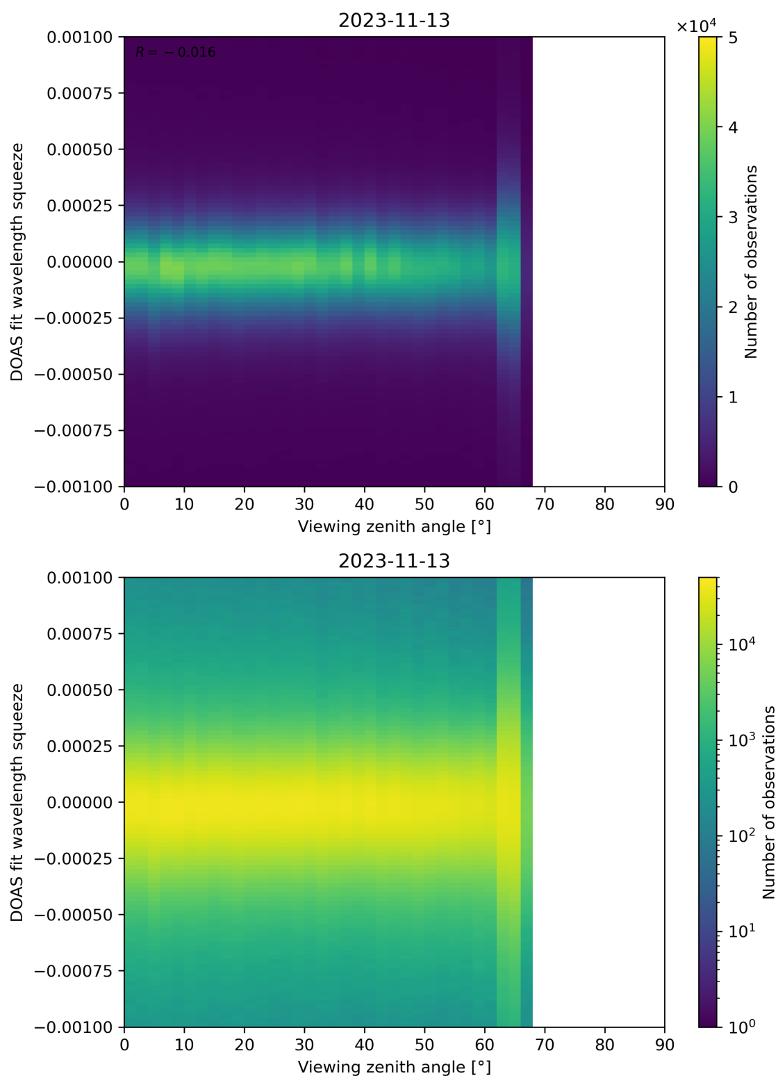
Figure 312: Scatter density plot of “Viewing zenith angle” against “DOAS fit wavelength squeeze” for 2023-11-13 to 2023-11-14.
