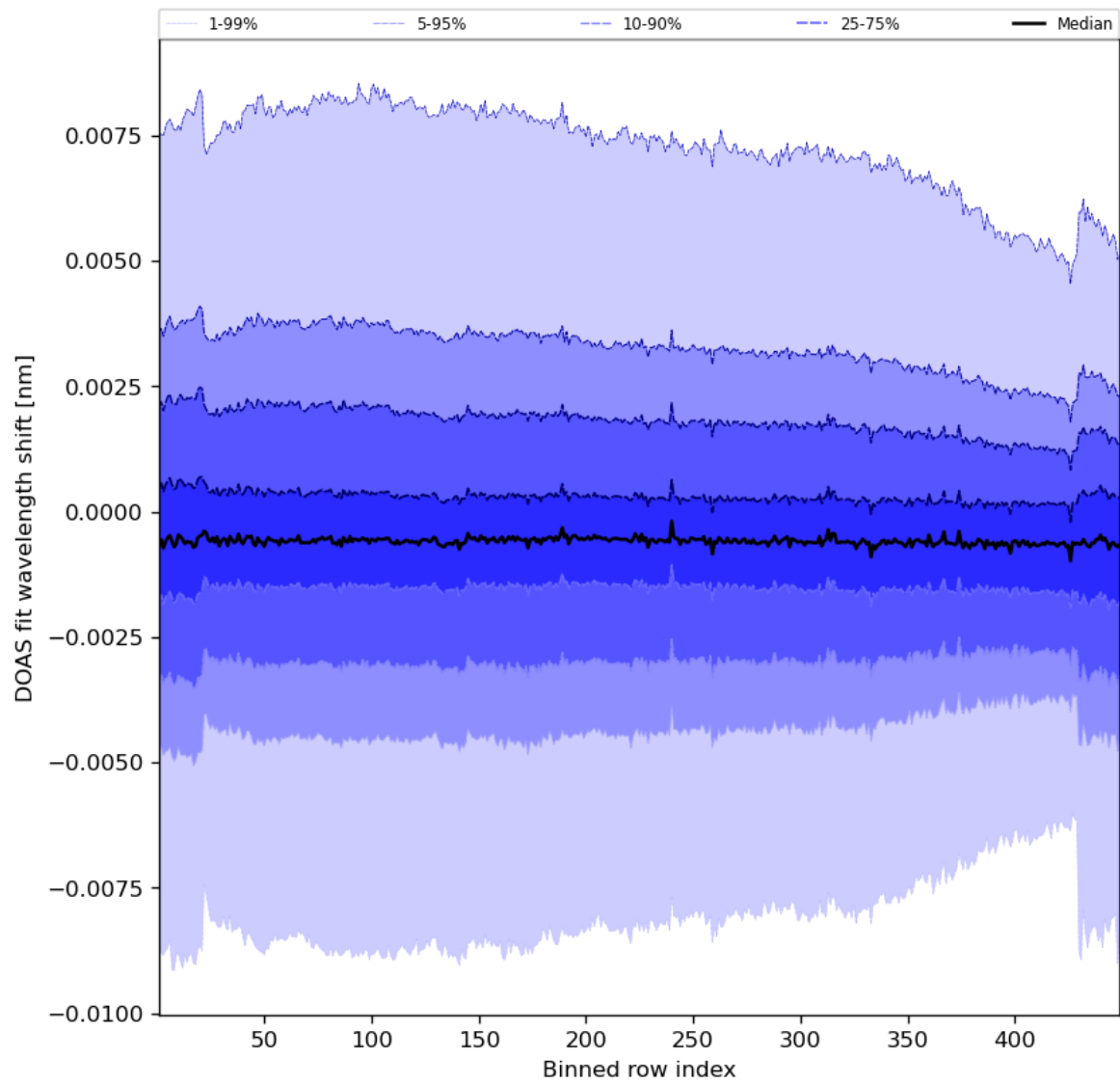
Figure 91: Along track statistics of “DOAS fit wavelength shift” for 2023-11-13 to 2023-11-14
