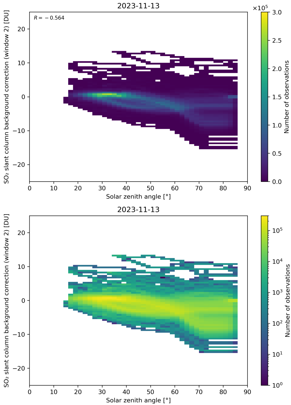
Figure 159: Scatter density plot of “Solar zenith angle” against “SO 2 slant column background correction (window 2)” for 2023-11-13 to 2023-11-14.
