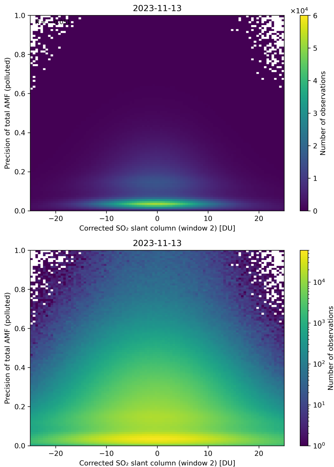
Figure 204: Scatter density plot of “Corrected SO 2 slant column (window 2)” against “Precision of total AMF (polluted)” for 2023-11-13 to 2023-11-14.
