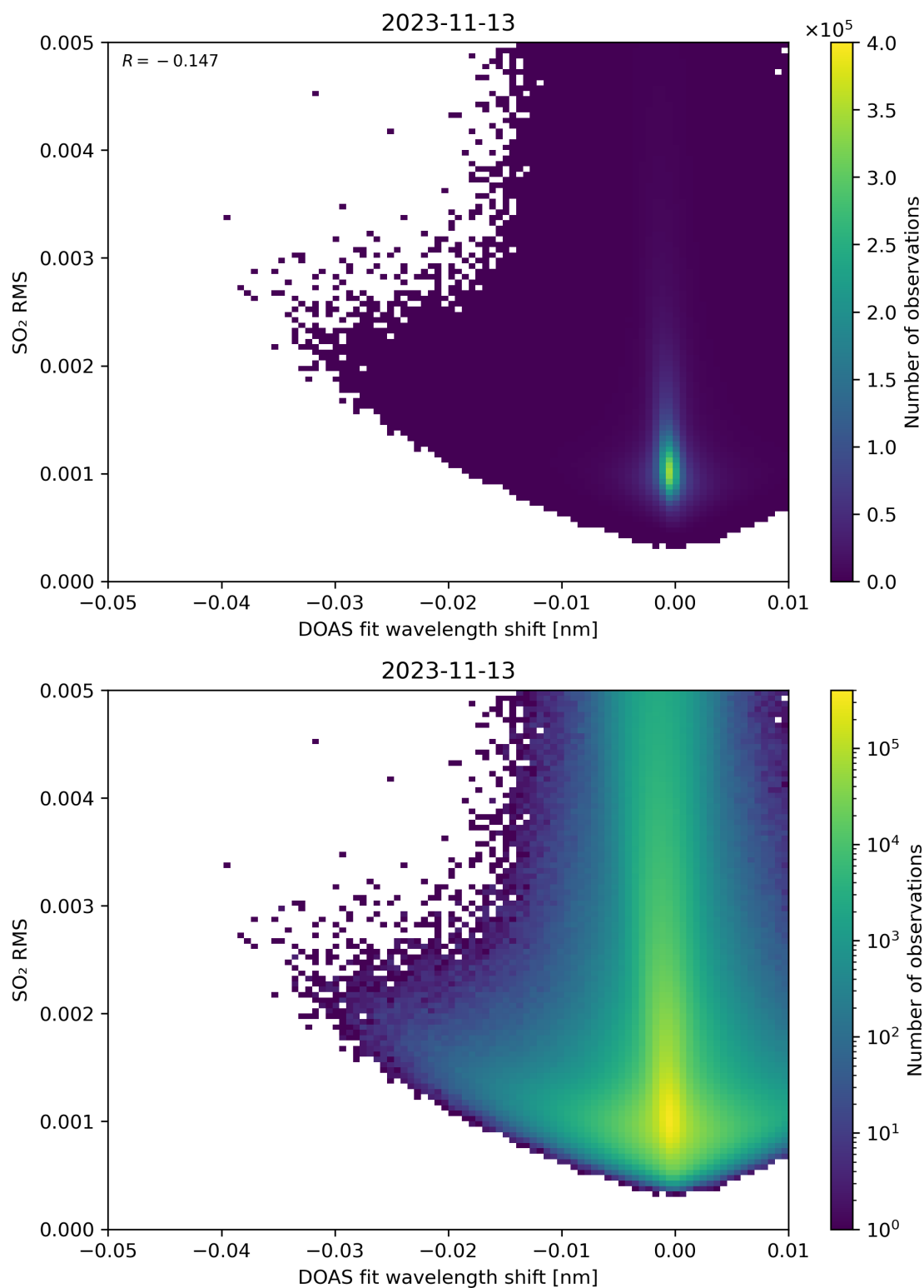
Figure 128: Scatter density plot of “DOAS fit wavelength shift” against “SO 2 RMS” for 2023-11-13 to 2023-11-14.
