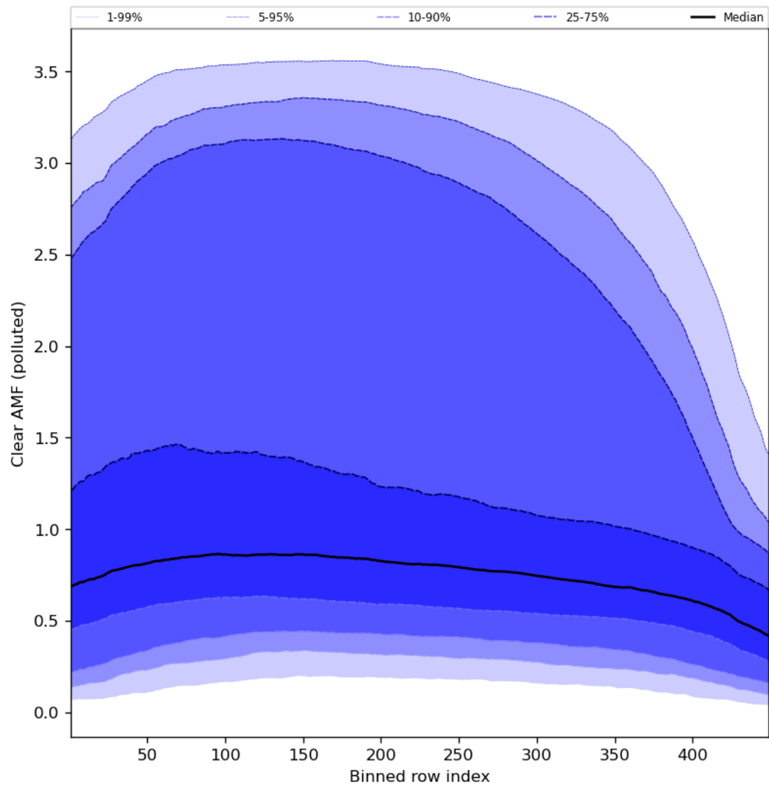
Figure 96: Along track statistics of “Clear AMF (polluted)” for 2023-11-13 to 2023-11-14
