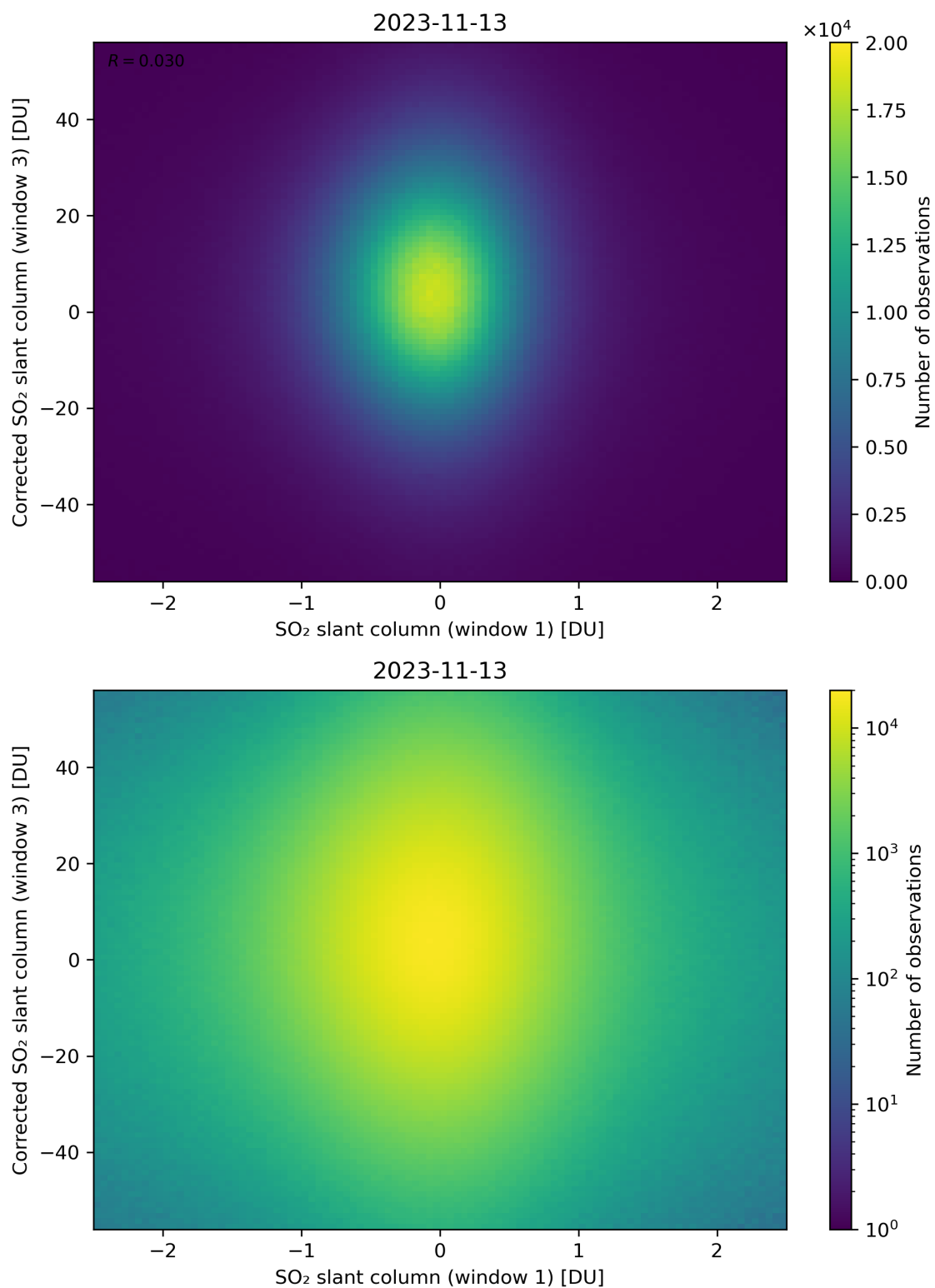
Figure 234: Scatter density plot of “SO 2 slant column (window 1)” against “Corrected SO 2 slant column (window 3)” for 2023-11-13 to 2023-11-14.
