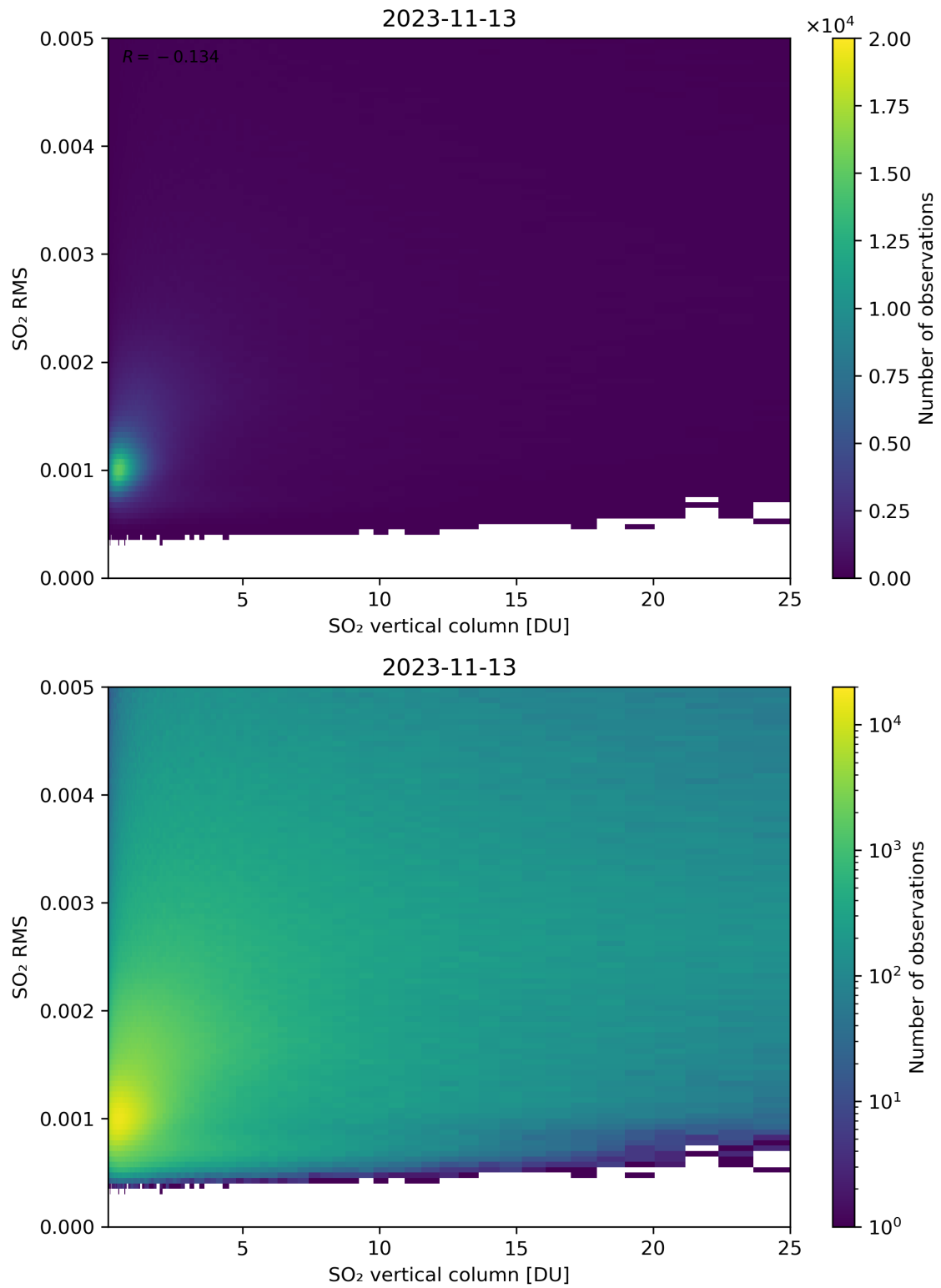
Figure 278: Scatter density plot of “SO 2 vertical column” against “SO 2 RMS” for 2023-11-13 to 2023-11-14.
