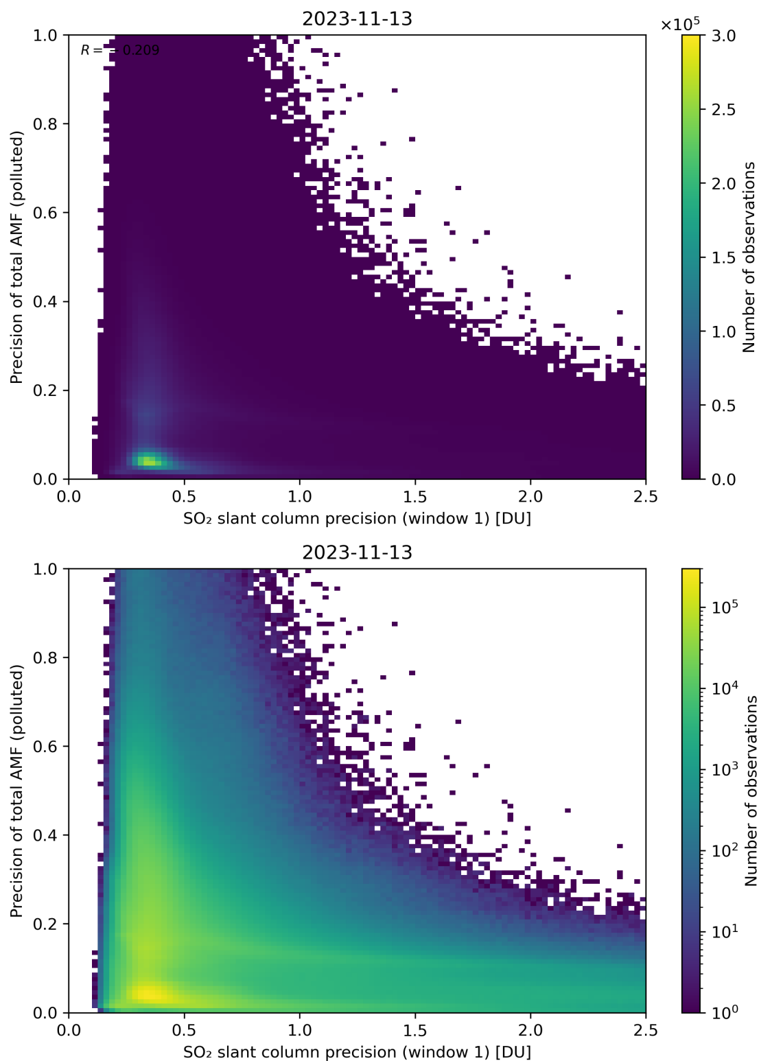
Figure 231: Scatter density plot of “SO 2 slant column precision (window 1)” against “Precision of total AMF (polluted)” for 2023-11-13 to 2023-11-14.
