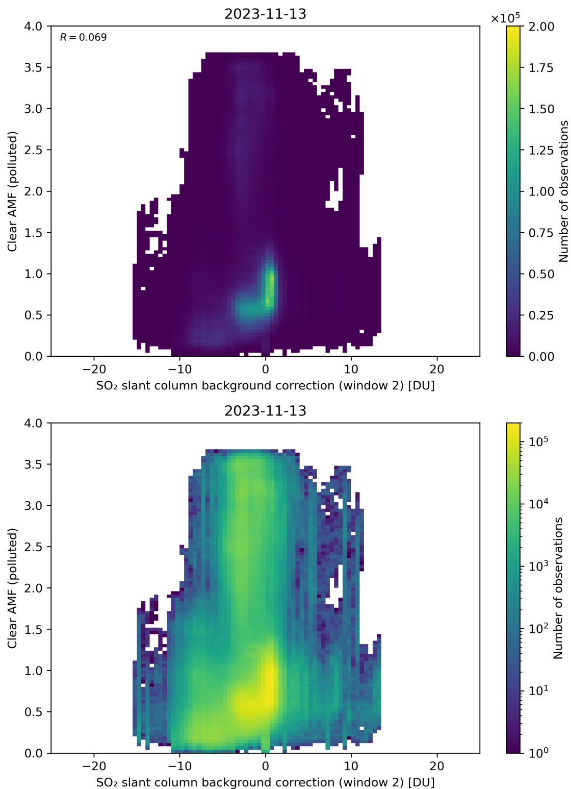
Figure 115: Scatter density plot of “SO 2 slant column background correction (window 2)” against “Clear AMF (polluted)” for 2023-11-13 to 2023-11-14.
