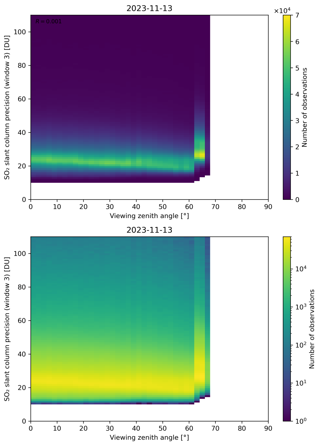
Figure 324: Scatter density plot of “Viewing zenith angle” against “SO 2 slant column precision (window 3)” for 2023-11-13 to 2023-11-14.
