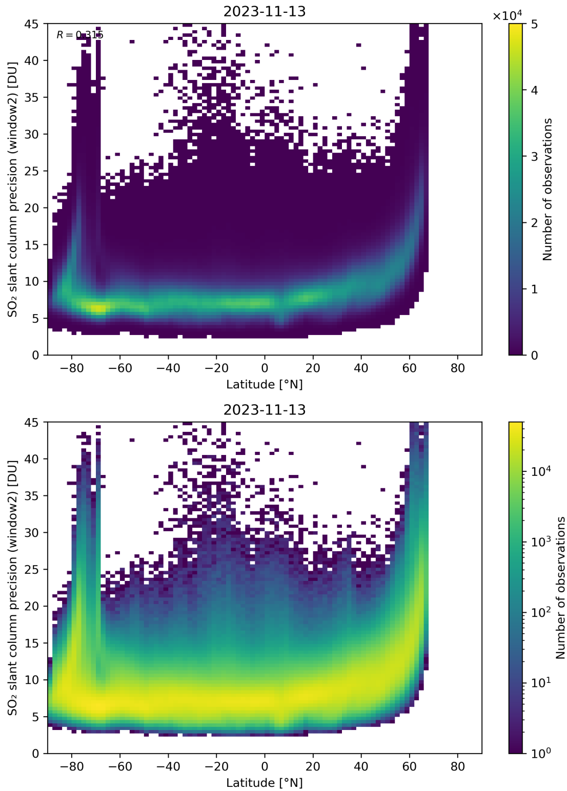
Figure 151: Scatter density plot of “Latitude” against “SO 2 slant column precision (window2)” for 2023-11-13 to 2023-11-14.
