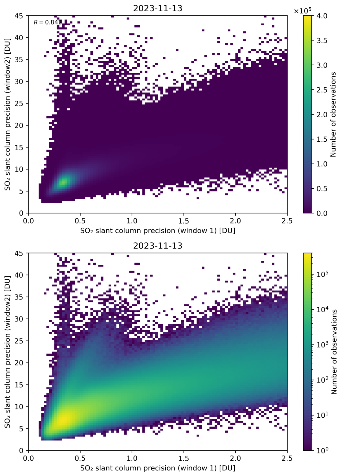
Figure 227: Scatter density plot of “SO 2 slant column precision (window 1)” against “SO 2 slant column precision (window2)” for 2023-11-13 to 2023-11-14.
