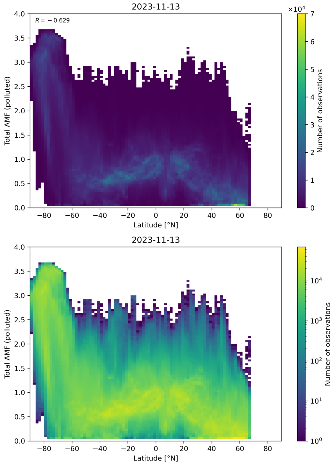
Figure 154: Scatter density plot of “Latitude” against “Total AMF (polluted)” for 2023-11-13 to 2023-11-14.
