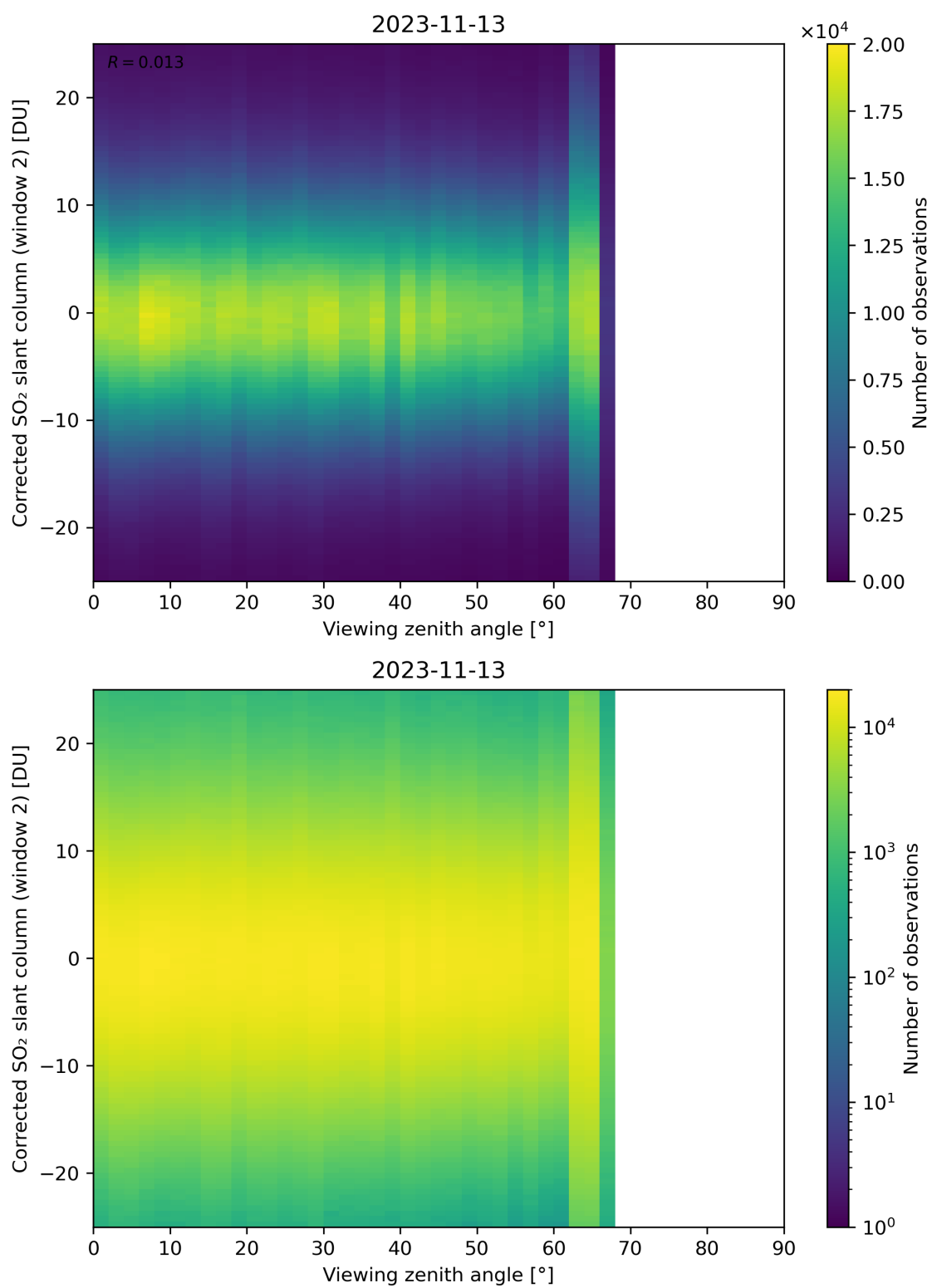
Figure 318: Scatter density plot of “Viewing zenith angle” against “Corrected SO 2 slant column (window 2)” for 2023-11-13 to 2023-11-14.
