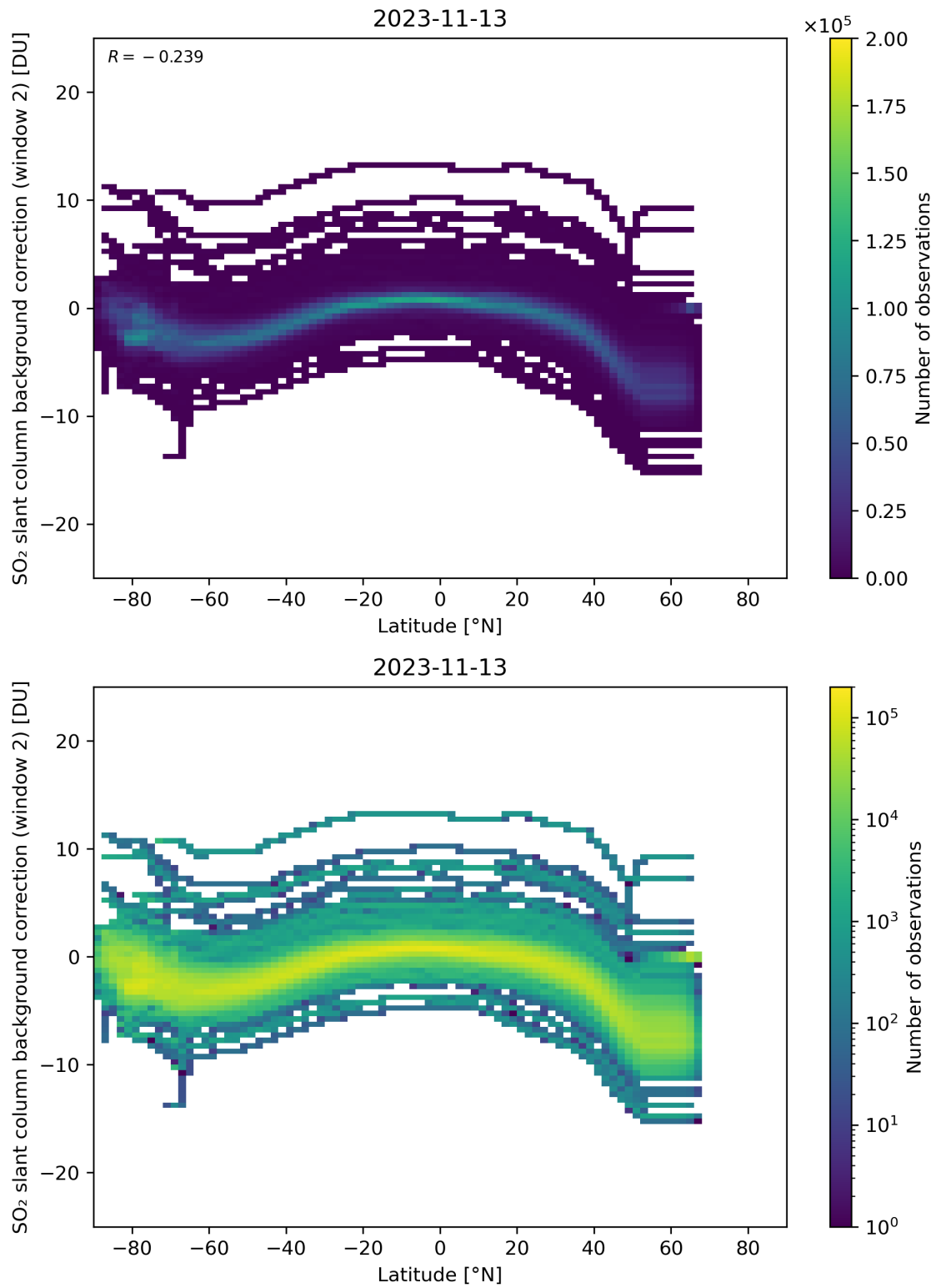
Figure 140: Scatter density plot of “Latitude” against “SO 2 slant column background correction (window 2)” for 2023-11-13 to 2023-11-14.
