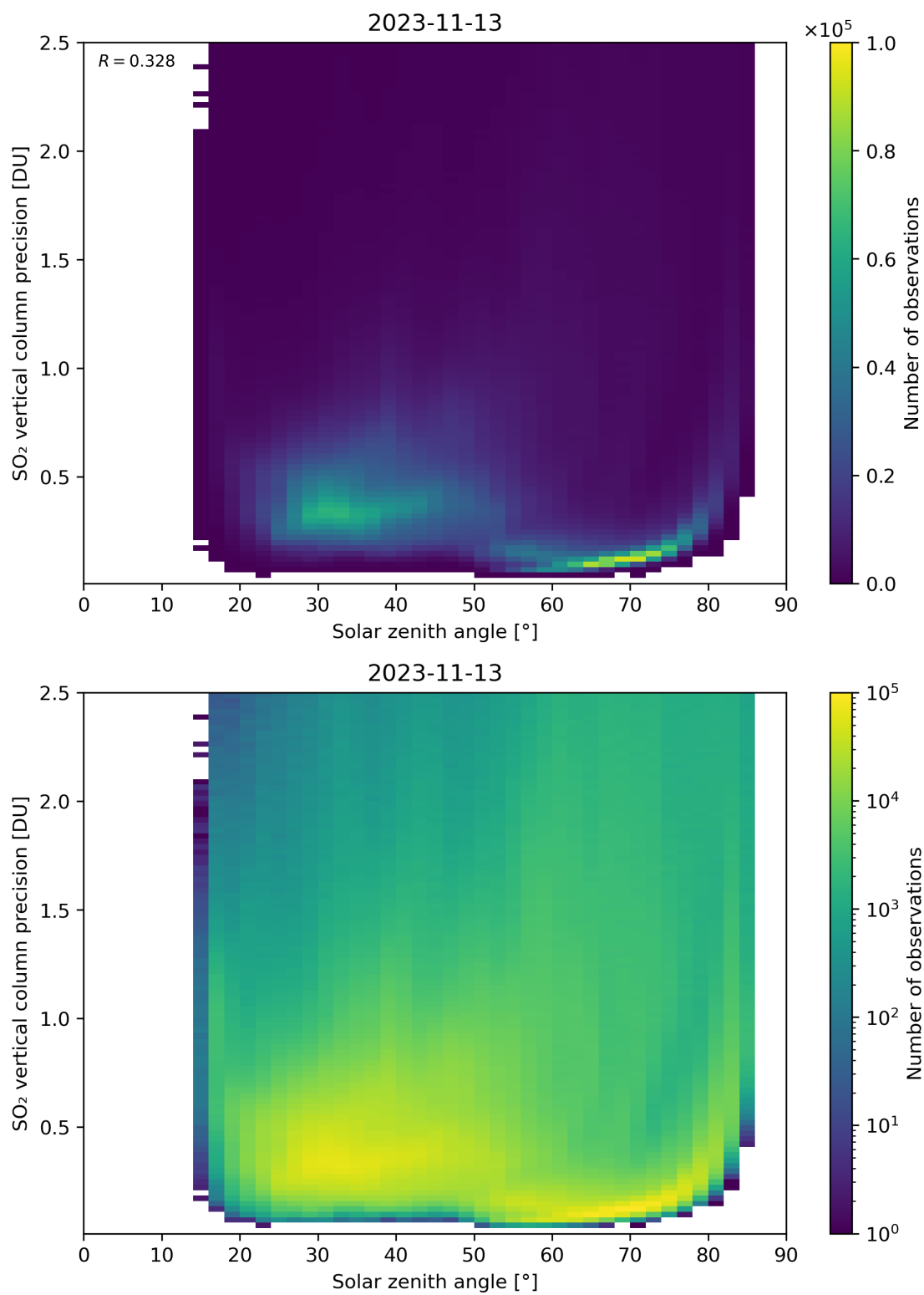
Figure 177: Scatter density plot of “Solar zenith angle” against “SO 2 vertical column precision” for 2023-11-13 to 2023-11-14.
