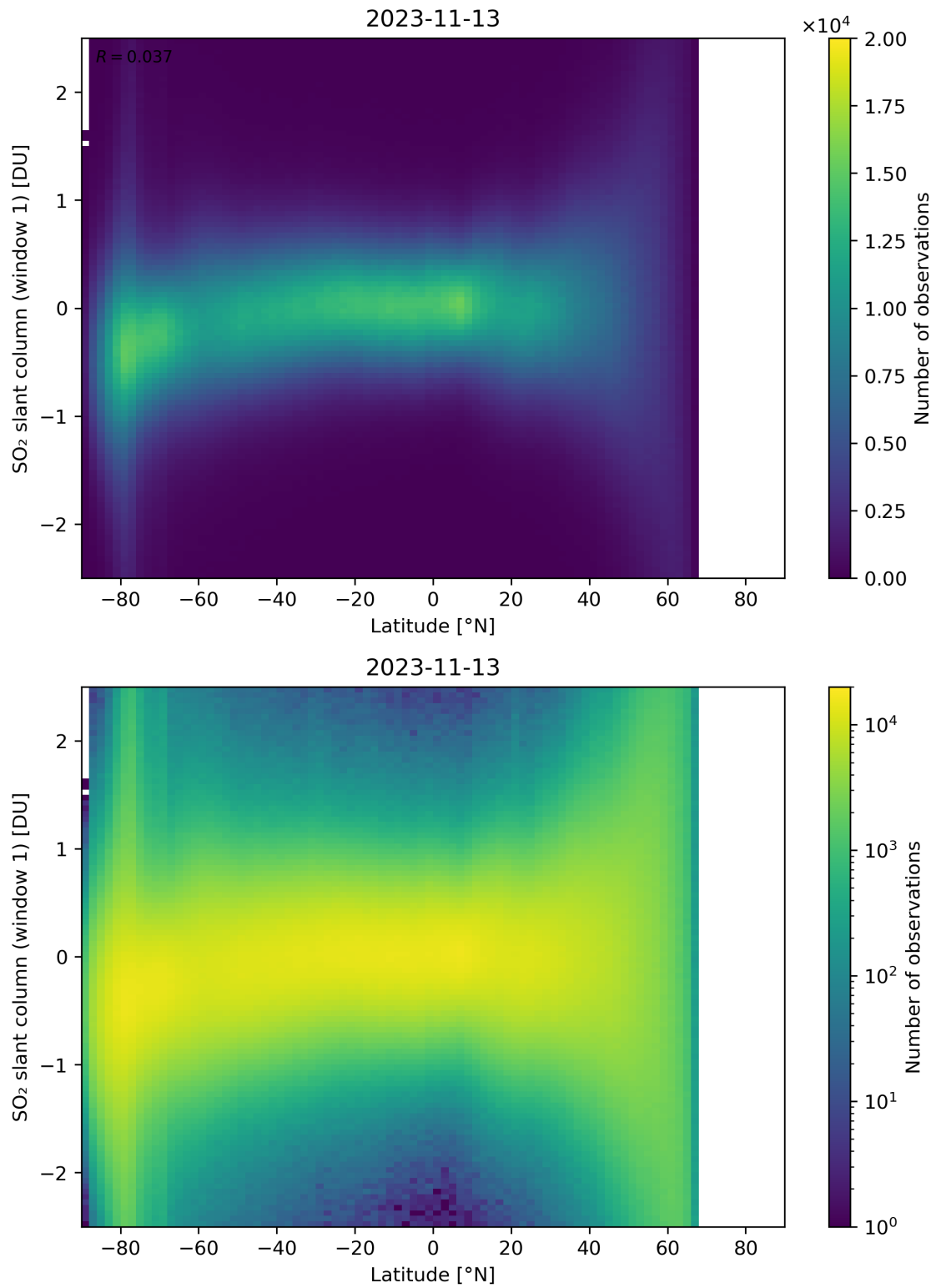
Figure 149: Scatter density plot of “Latitude” against “SO 2 slant column (window 1)” for 2023-11-13 to 2023-11-14.
