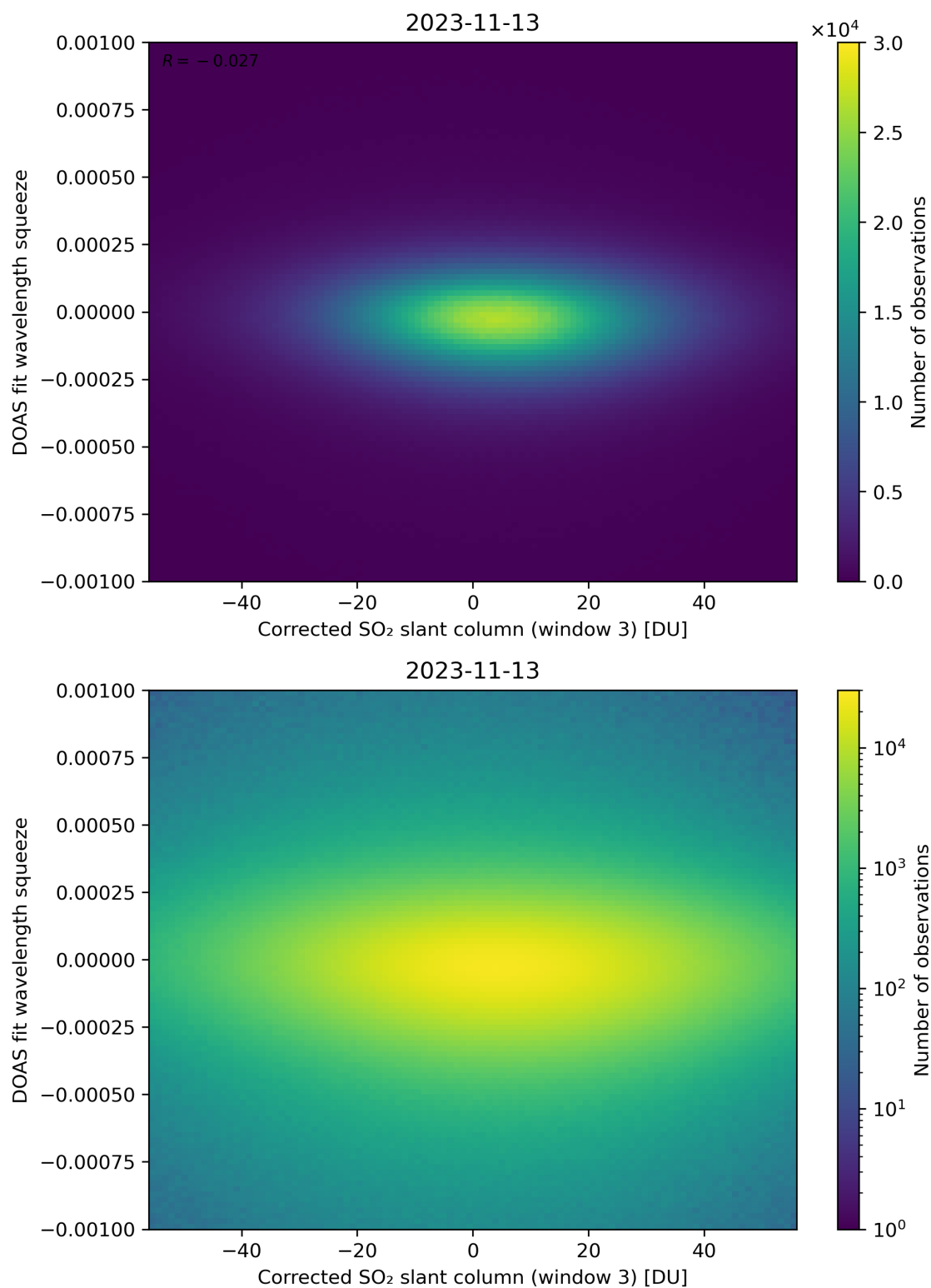
Figure 207: Scatter density plot of “Corrected SO 2 slant column (window 3)” against “DOAS fit wavelength squeeze” for 2023-11-13 to 2023-11-14.
