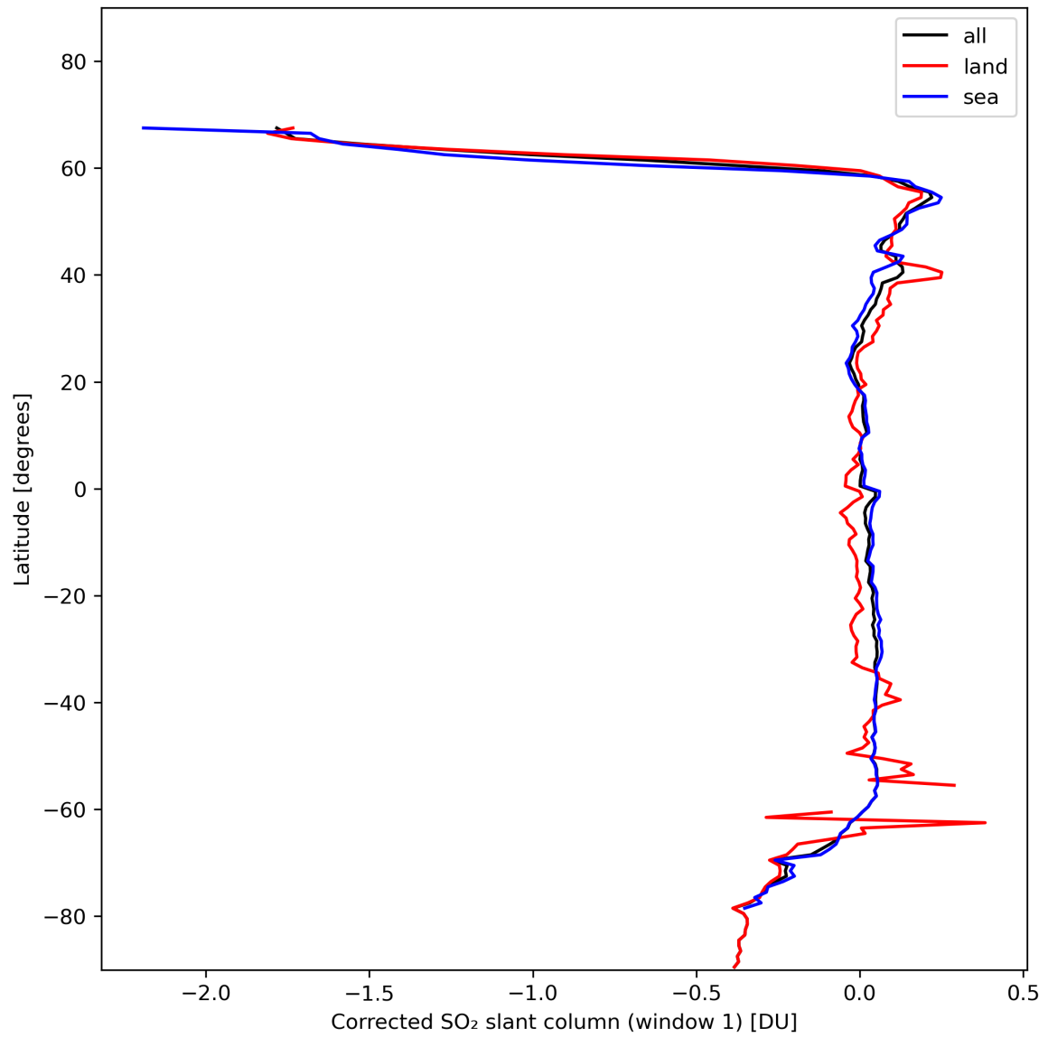
Figure 35: Zonal average of “Corrected SO 2 slant column (window 1)” for 2023-11-13 to 2023-11-14.
