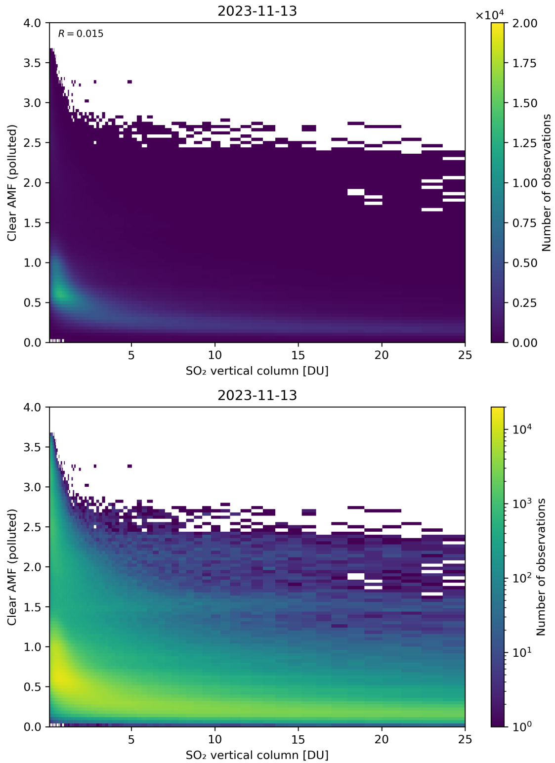
Figure 296: Scatter density plot of “SO 2 vertical column” against “Clear AMF (polluted)” for 2023-11-13 to 2023-11-14.
