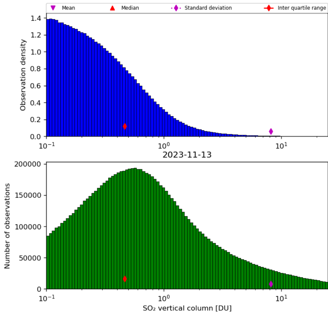
Figure 53: Histogram of “SO 2 vertical column” for 2023-11-13 to 2023-11-14
