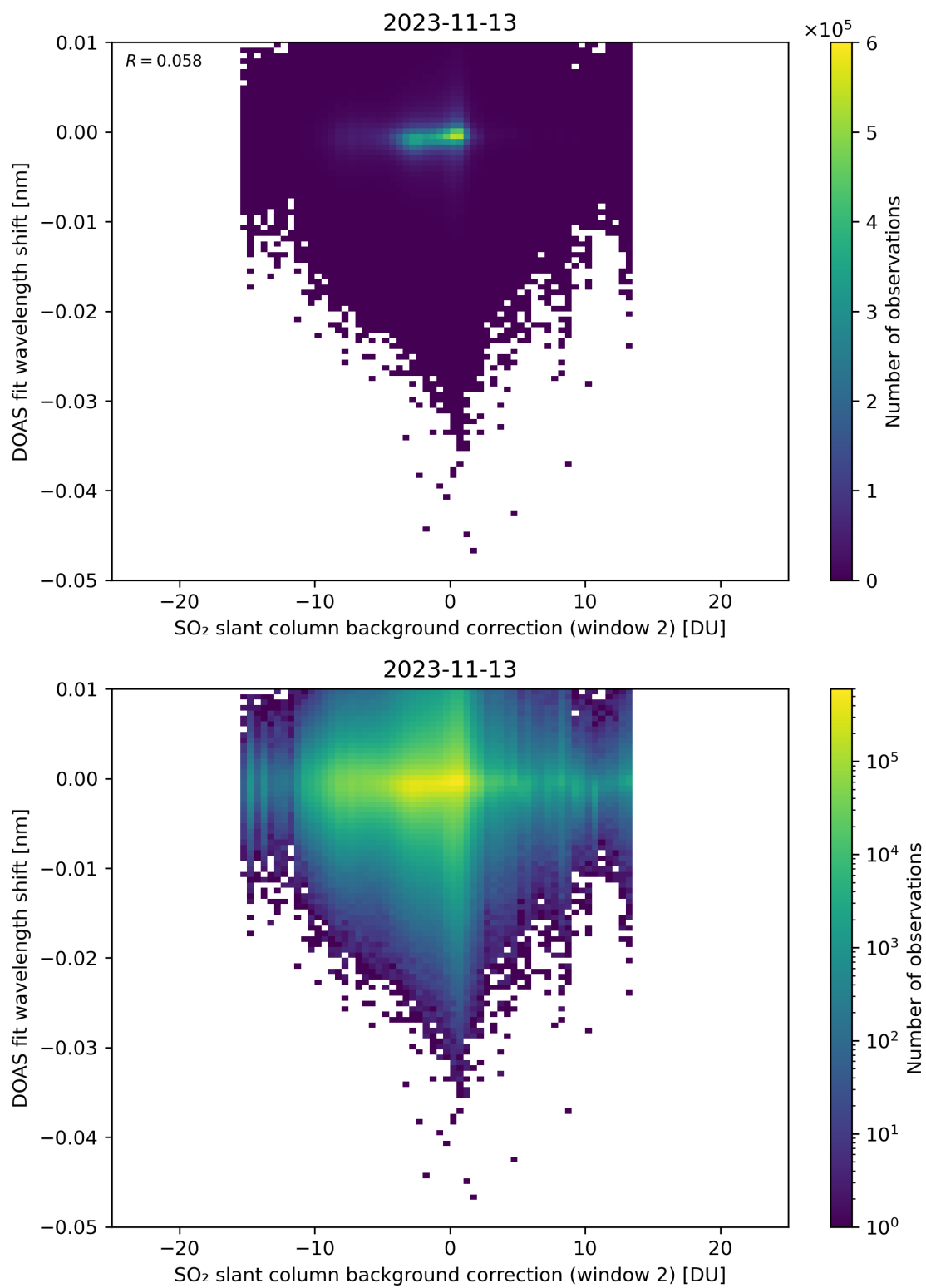
Figure 112: Scatter density plot of “SO 2 slant column background correction (window 2)” against “DOAS fit wavelength shift” for 2023-11-13 to 2023-11-14.
