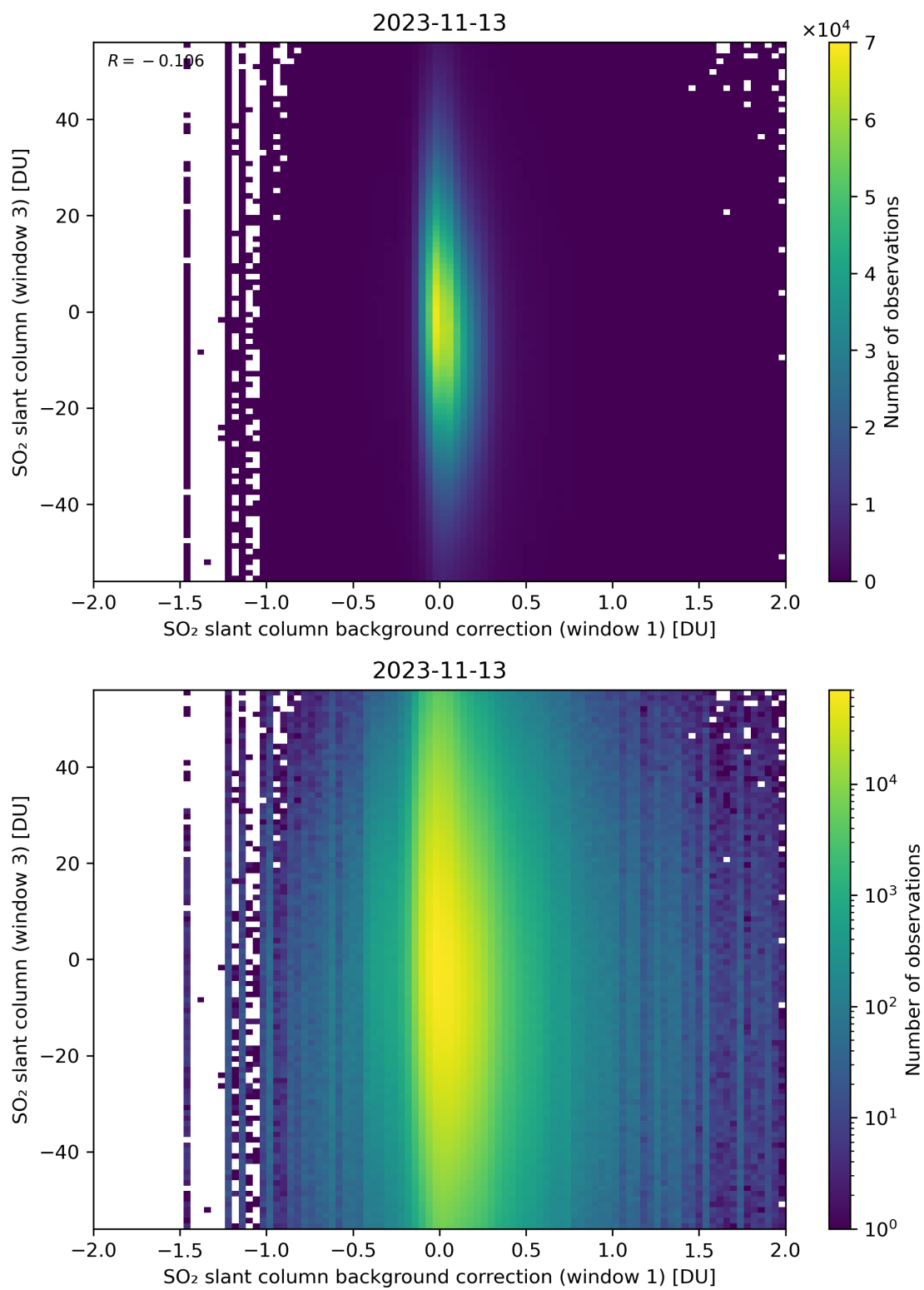
Figure 107: Scatter density plot of “SO 2 slant column background correction (window 1)” against “SO 2 slant column (window 3)” for 2023-11-13 to 2023-11-14.
