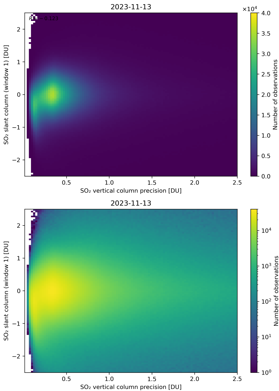
Figure 289: Scatter density plot of “SO 2 vertical column precision” against “SO 2 slant column (window 1)” for 2023-11-13 to 2023-11-14.
