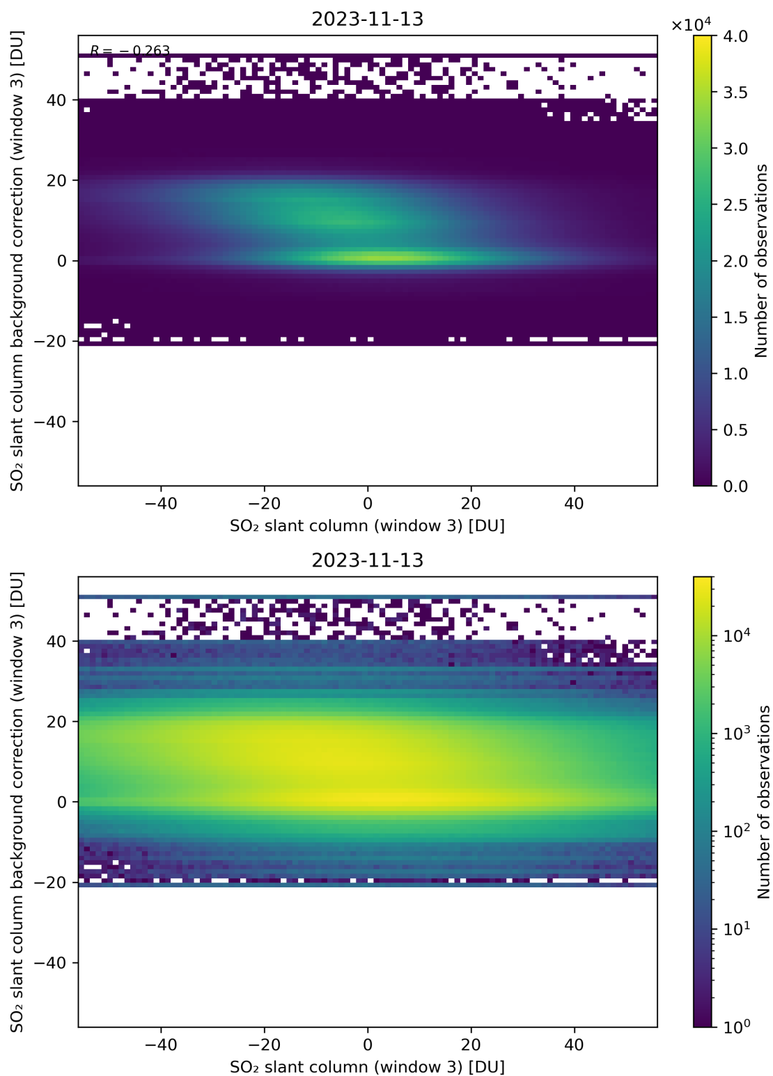
Figure 253: Scatter density plot of “SO 2 slant column (window 3)” against “SO 2 slant column background correction (window 3)” for 2023-11-13 to 2023-11-14.
