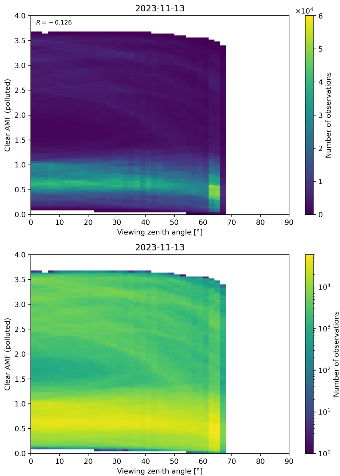
Figure 316: Scatter density plot of “Viewing zenith angle” against “Clear AMF (polluted)” for 2023-11-13 to 2023-11-14.
