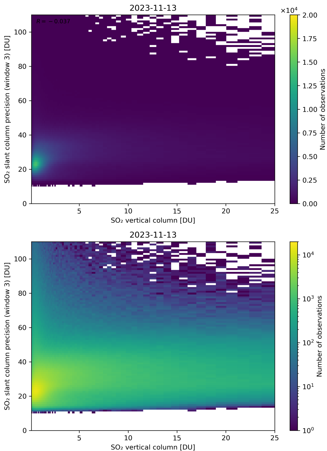
Figure 304: Scatter density plot of “SO 2 vertical column” against “SO 2 slant column precision (window 3)” for 2023-11-13 to 2023-11-14.
