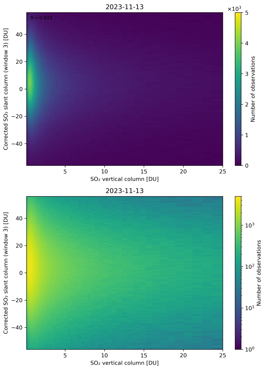
Figure 299: Scatter density plot of “SO 2 vertical column” against “Corrected SO 2 slant column (window 3)” for 2023-11-13 to 2023-11-14.
