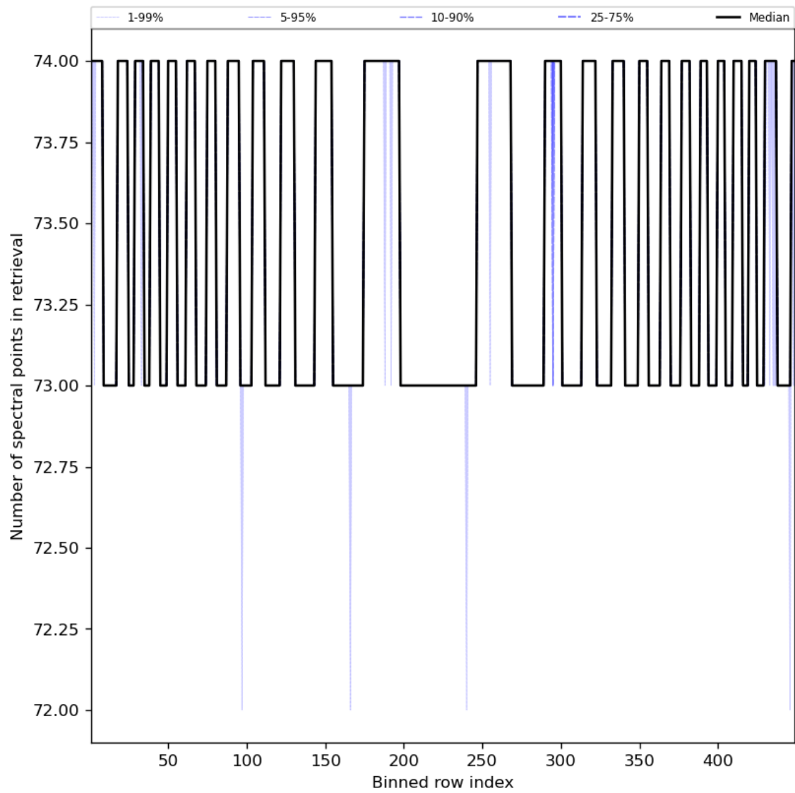
Figure 97: Along track statistics of “Number of spectral points in retrieval” for 2023-11-13 to 2023-11-14
