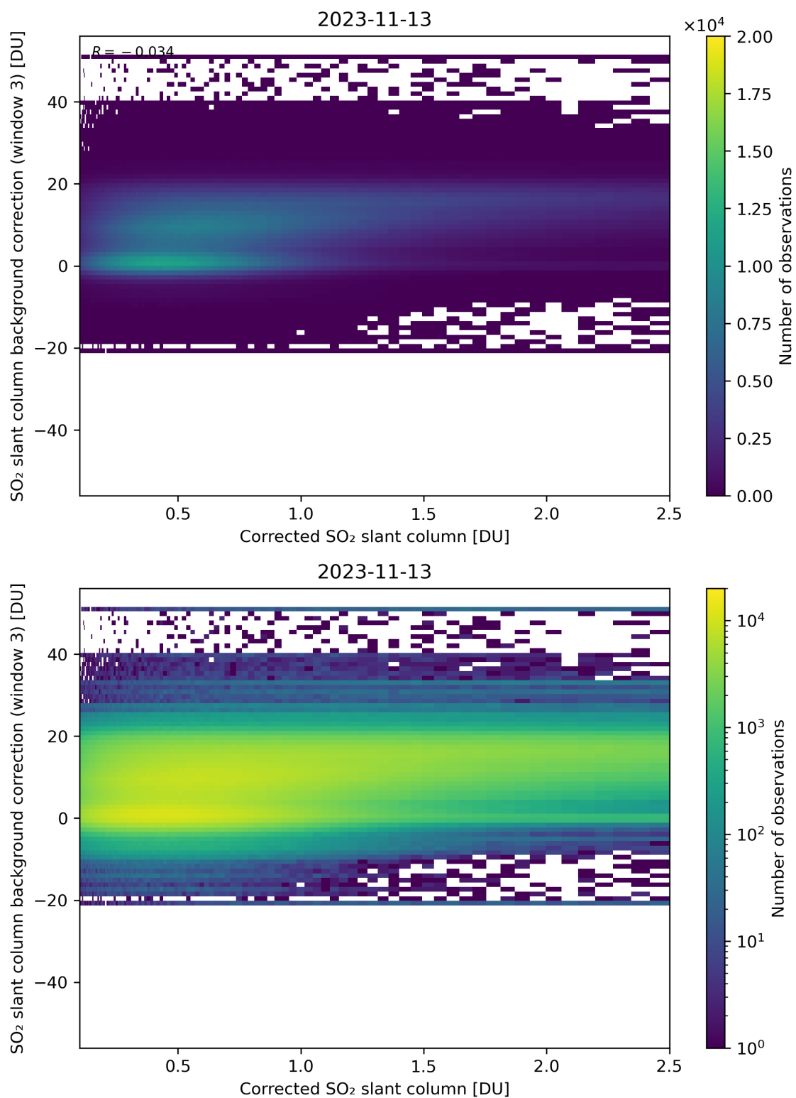
Figure 180: Scatter density plot of “Corrected SO 2 slant column” against “SO 2 slant column background correction (window 3)” for 2023-11-13 to 2023-11-14.
