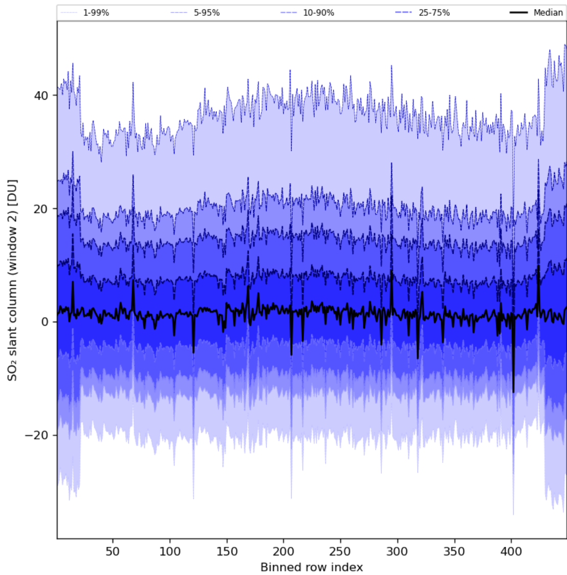
Figure 83: Along track statistics of “SO 2 slant column (window 2)” for 2023-11-13 to 2023-11-14
