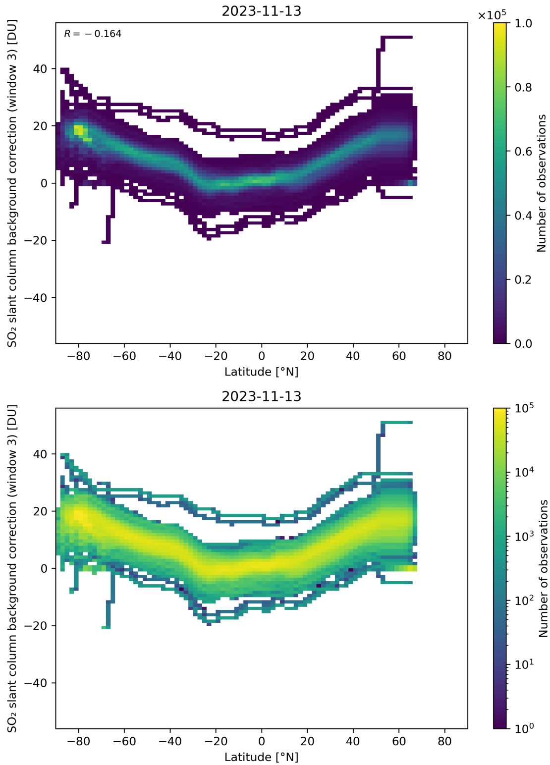
Figure 141: Scatter density plot of “Latitude” against “SO 2 slant column background correction (window 3)” for 2023-11-13 to 2023-11-14.
