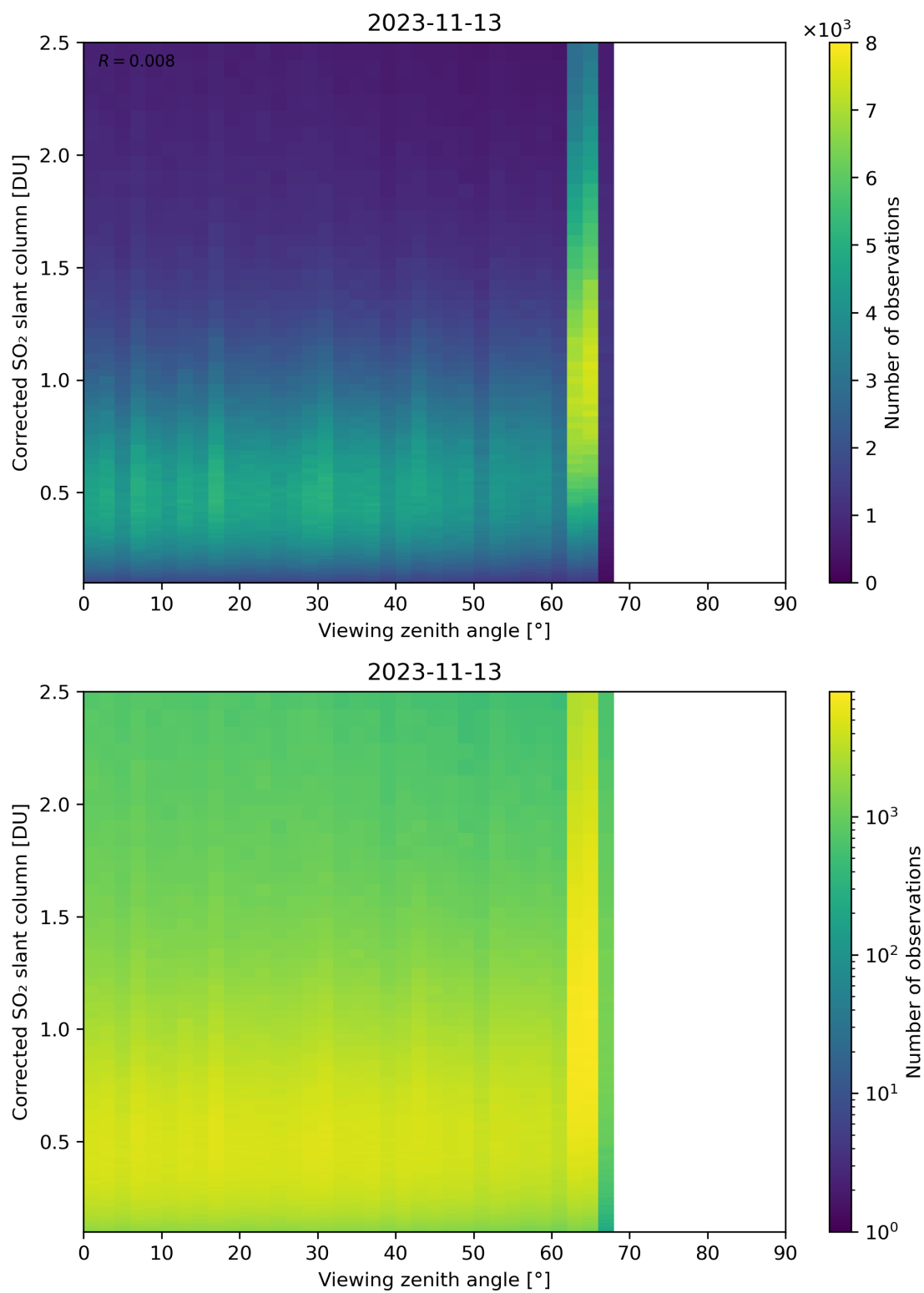
Figure 317: Scatter density plot of “Viewing zenith angle” against “Corrected SO 2 slant column” for 2023-11-13 to 2023-11-14.
