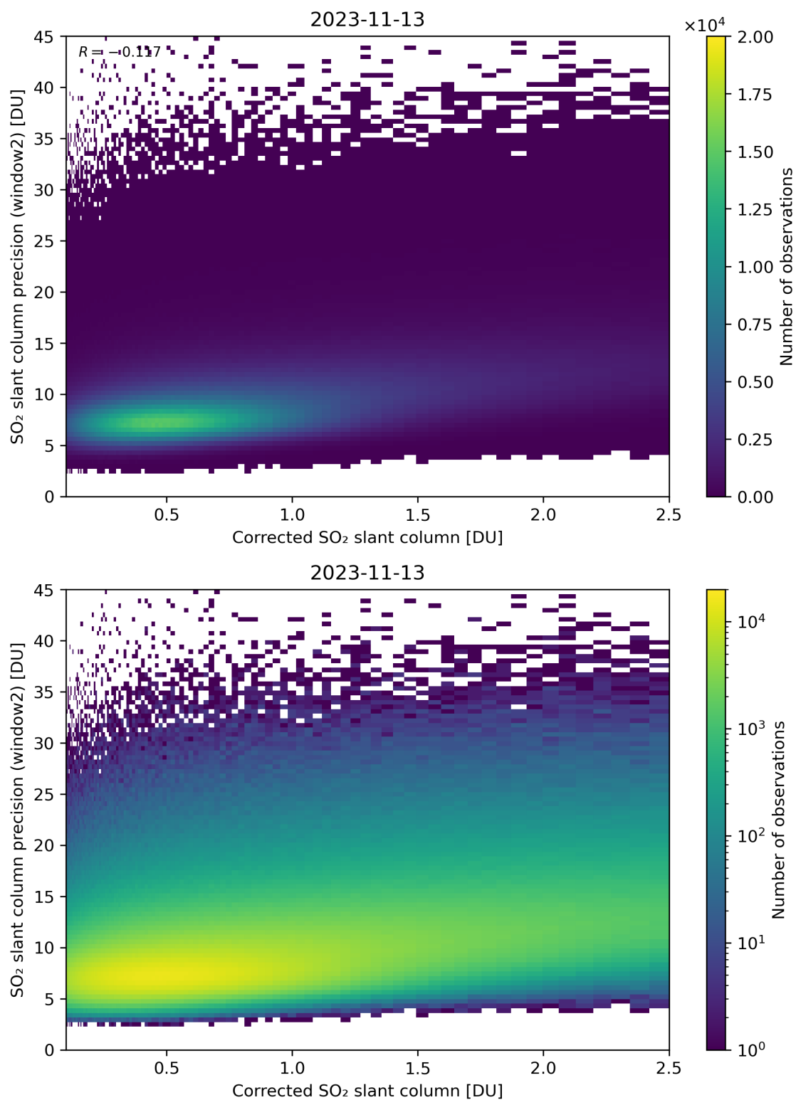
Figure 189: Scatter density plot of “Corrected SO 2 slant column” against “SO 2 slant column precision (window2)” for 2023-11-13 to 2023-11-14.
