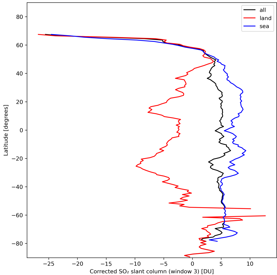
Figure 43: Zonal average of “Corrected SO 2 slant column (window 3)” for 2023-11-13 to 2023-11-14.
