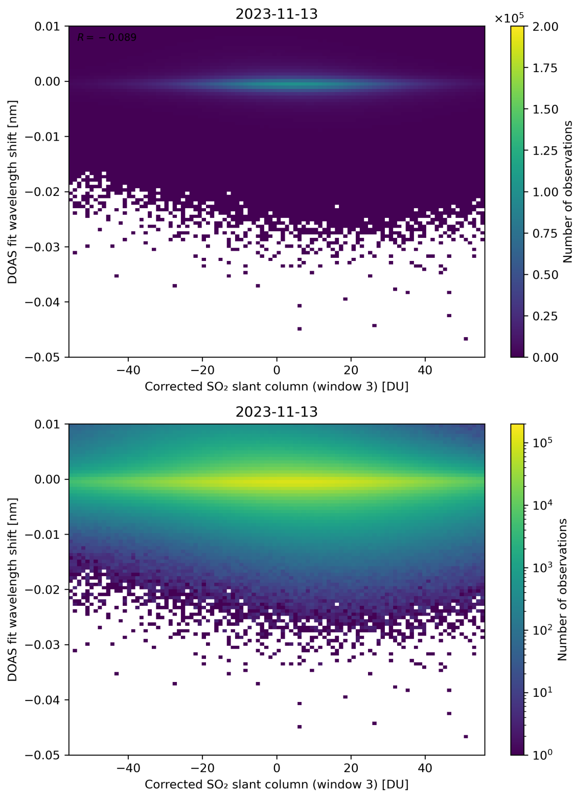
Figure 206: Scatter density plot of “Corrected SO 2 slant column (window 3)” against “DOAS fit wavelength shift” for 2023-11-13 to 2023-11-14.
