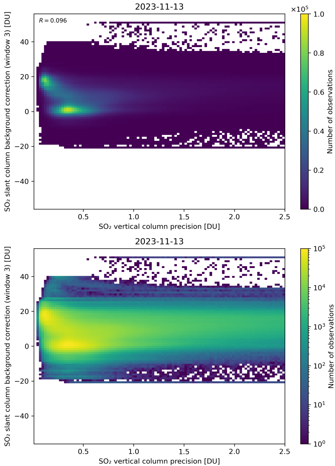
Figure 281: Scatter density plot of “SO 2 vertical column precision” against “SO 2 slant column background correction (window 3)” for 2023-11-13 to 2023-11-14.
