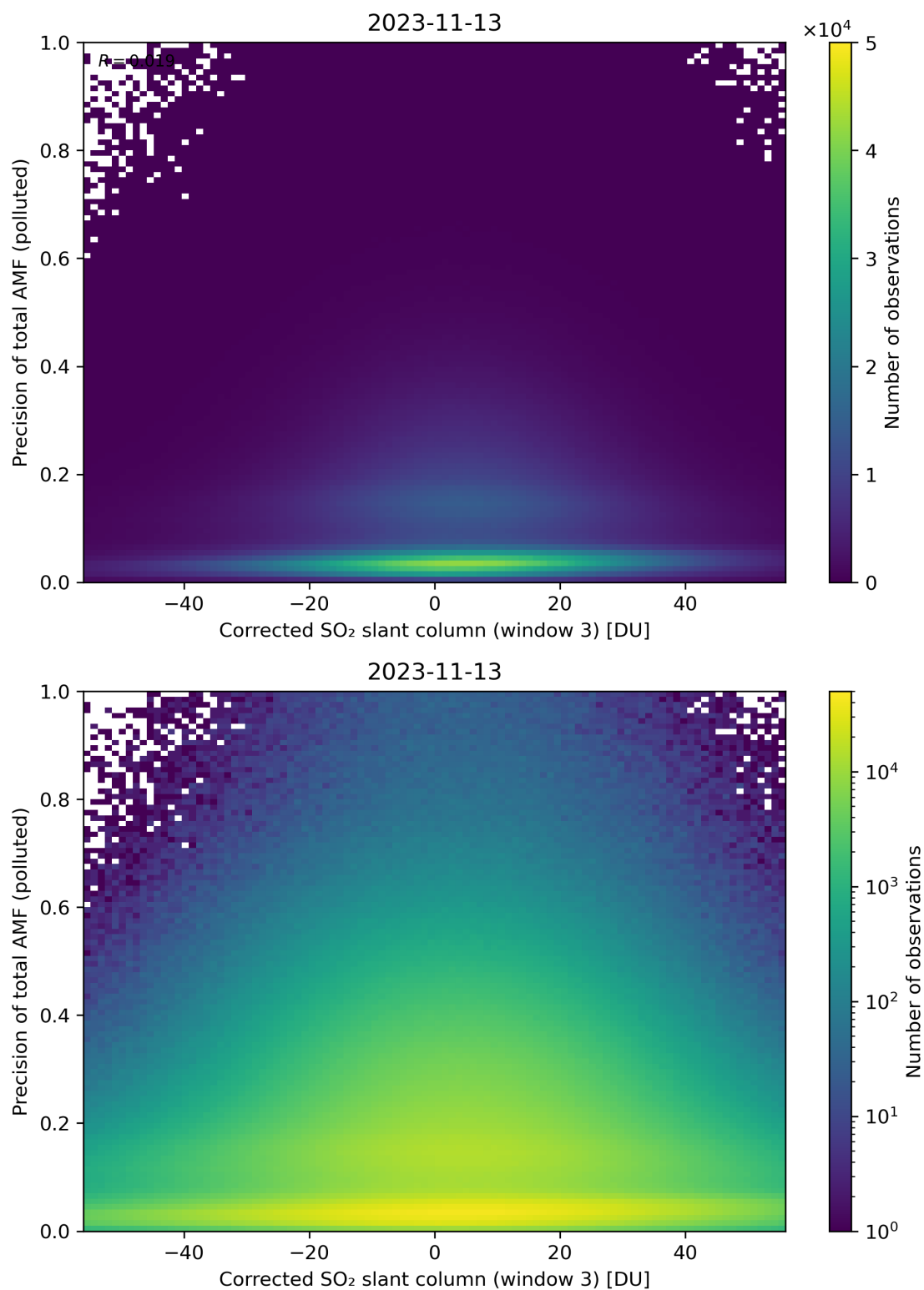
Figure 211: Scatter density plot of “Corrected SO 2 slant column (window 3)” against “Precision of total AMF (polluted)” for 2023-11-13 to 2023-11-14.
