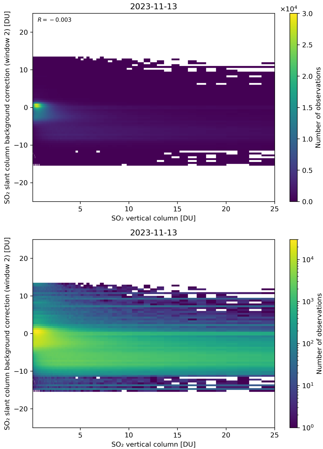
Figure 274: Scatter density plot of “SO 2 vertical column” against “SO 2 slant column background correction (window 2)” for 2023-11-13 to 2023-11-14.
