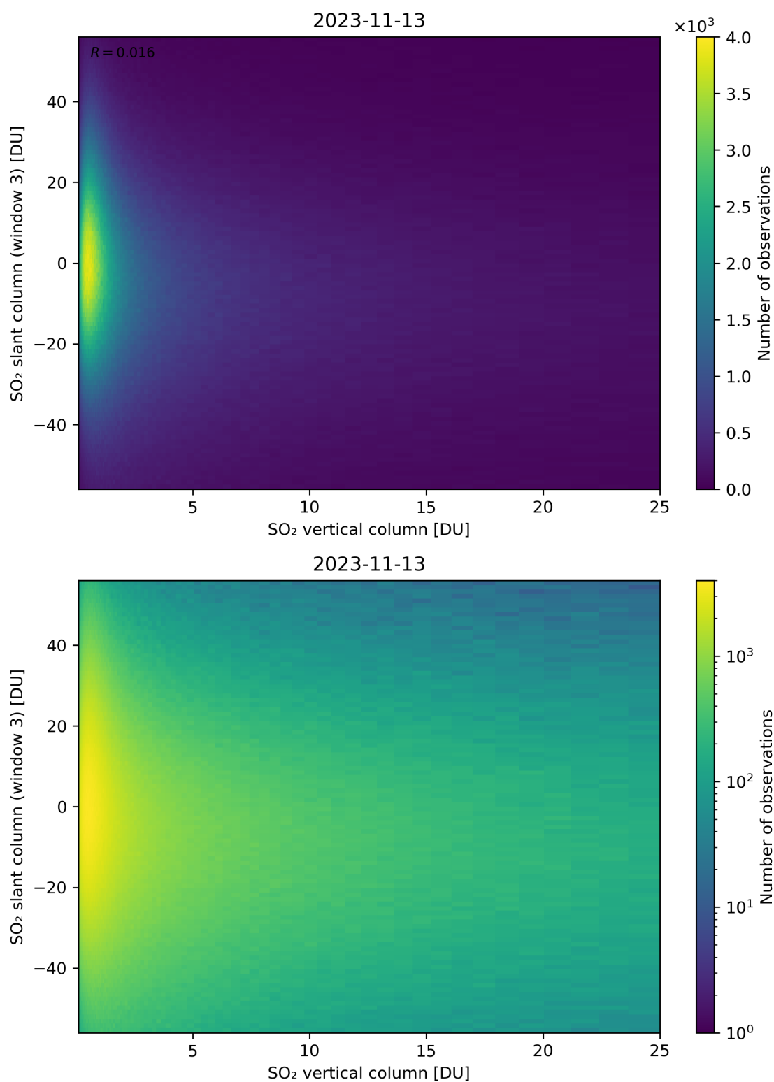
Figure 303: Scatter density plot of “SO 2 vertical column” against “SO 2 slant column (window 3)” for 2023-11-13 to 2023-11-14.
