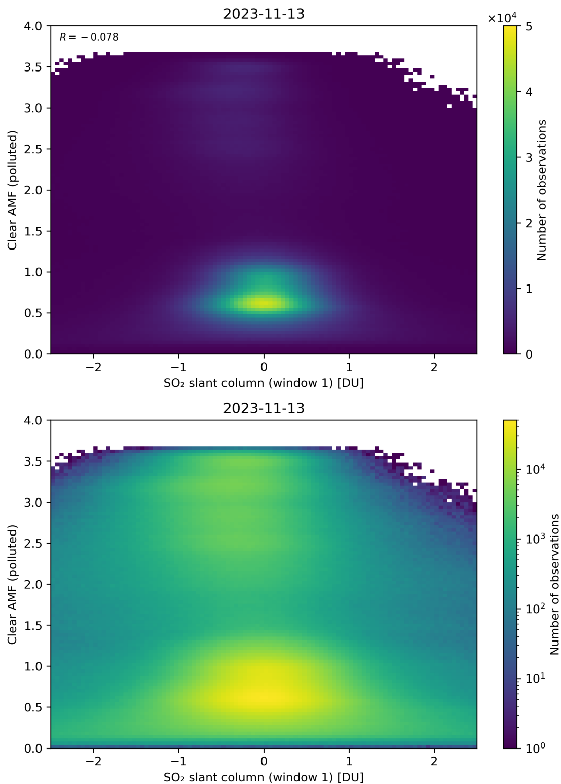
Figure 232: Scatter density plot of “SO 2 slant column (window 1)” against “Clear AMF (polluted)” for 2023-11-13 to 2023-11-14.
