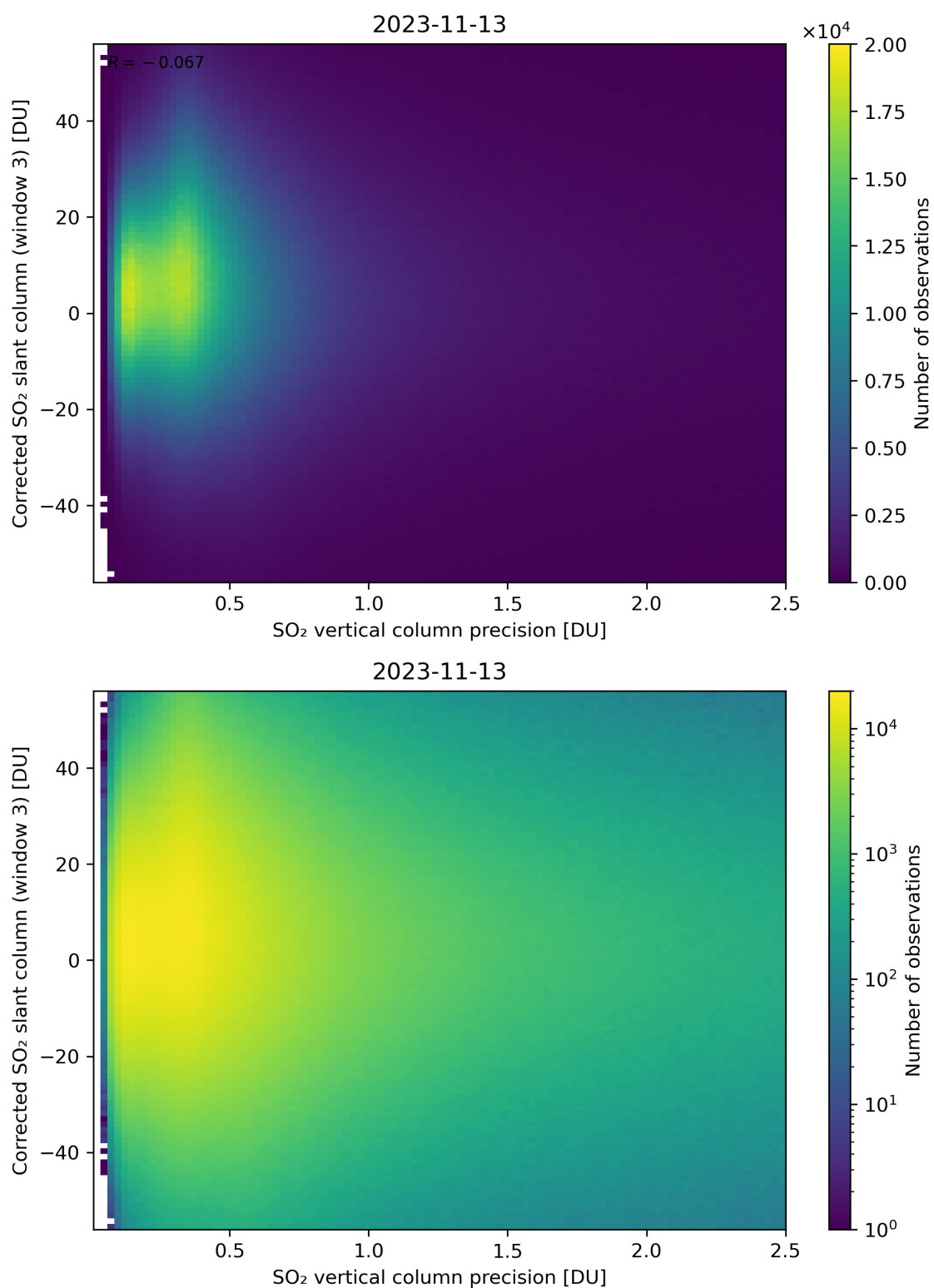
Figure 288: Scatter density plot of “SO 2 vertical column precision” against “Corrected SO 2 slant column (window 3)” for 2023-11-13 to 2023-11-14.
