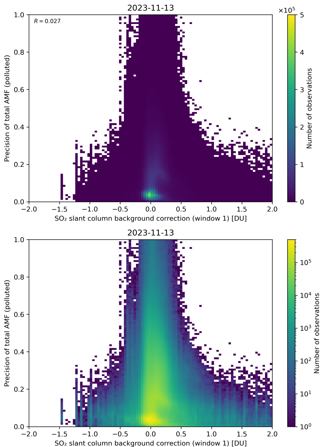
Figure 110: Scatter density plot of “SO 2 slant column background correction (window 1)” against “Precision of total AMF (polluted)” for 2023-11-13 to 2023-11-14.
