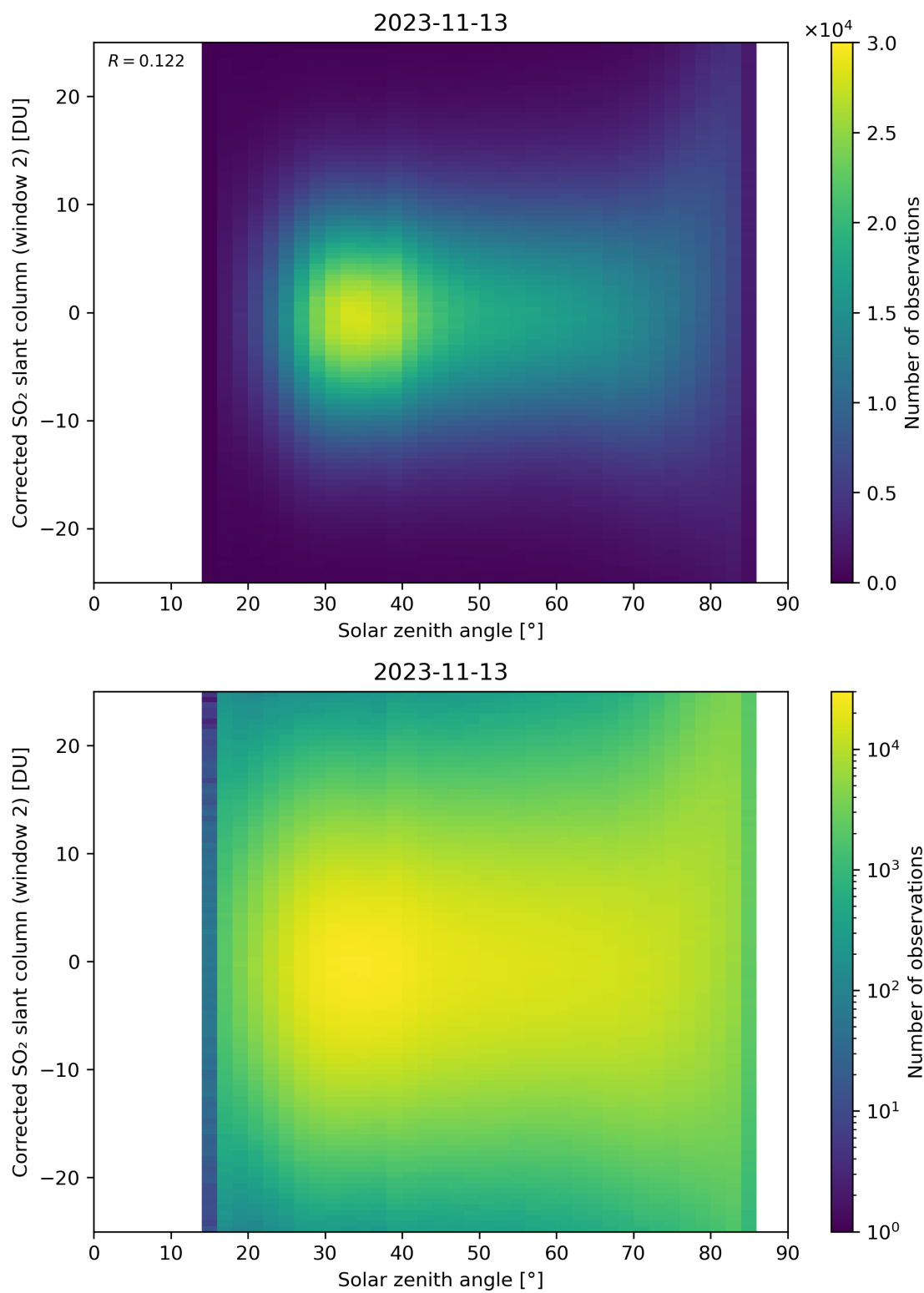
Figure 167: Scatter density plot of “Solar zenith angle” against “Corrected SO 2 slant column (window 2)” for 2023-11-13 to 2023-11-14.
