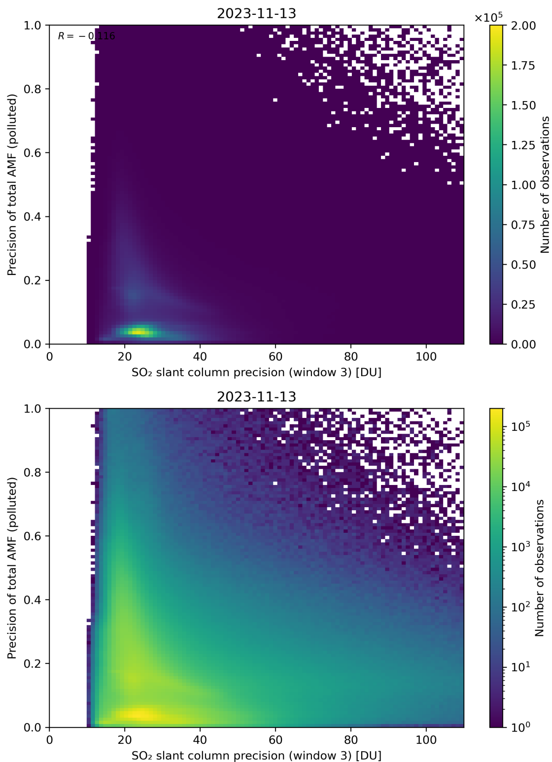
Figure 264: Scatter density plot of “SO 2 slant column precision (window 3)” against “Precision of total AMF (polluted)” for 2023-11-13 to 2023-11-14.
