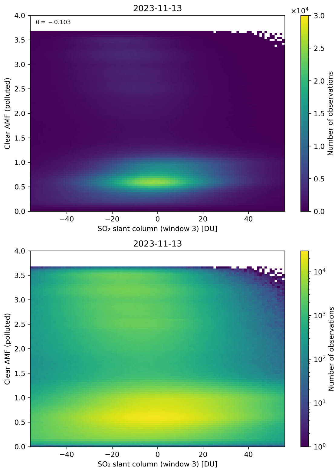
Figure 265: Scatter density plot of “SO 2 slant column (window 3)” against “Clear AMF (polluted)” for 2023-11-13 to 2023-11-14.
