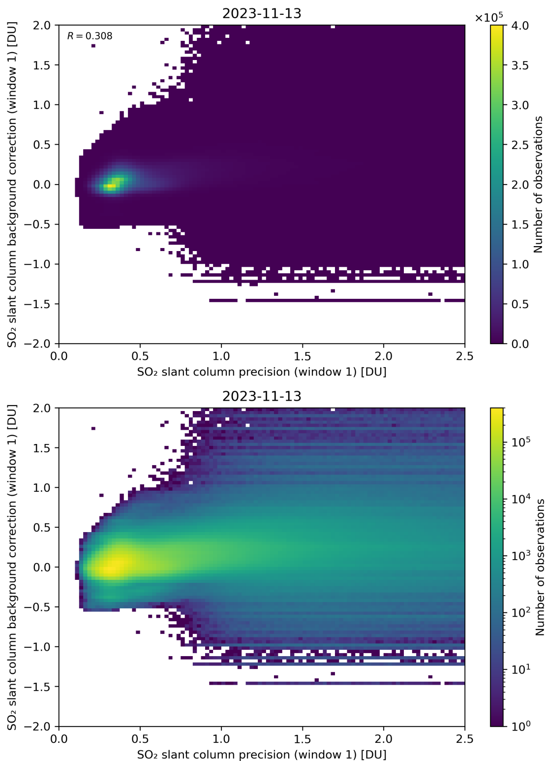
Figure 218: Scatter density plot of “SO 2 slant column precision (window 1)” against “SO 2 slant column background correction (window 1)” for 2023-11-13 to 2023-11-14.
