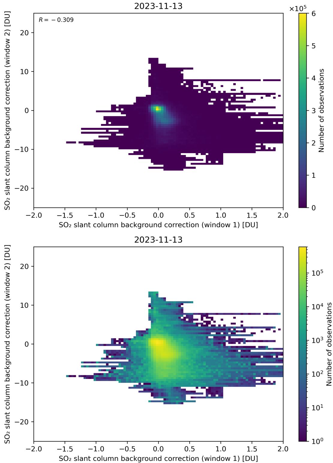
Figure 98: Scatter density plot of “SO 2 slant column background correction (window 1)” against “SO 2 slant column background correction (window 2)” for 2023-11-13 to 2023-11-14.
