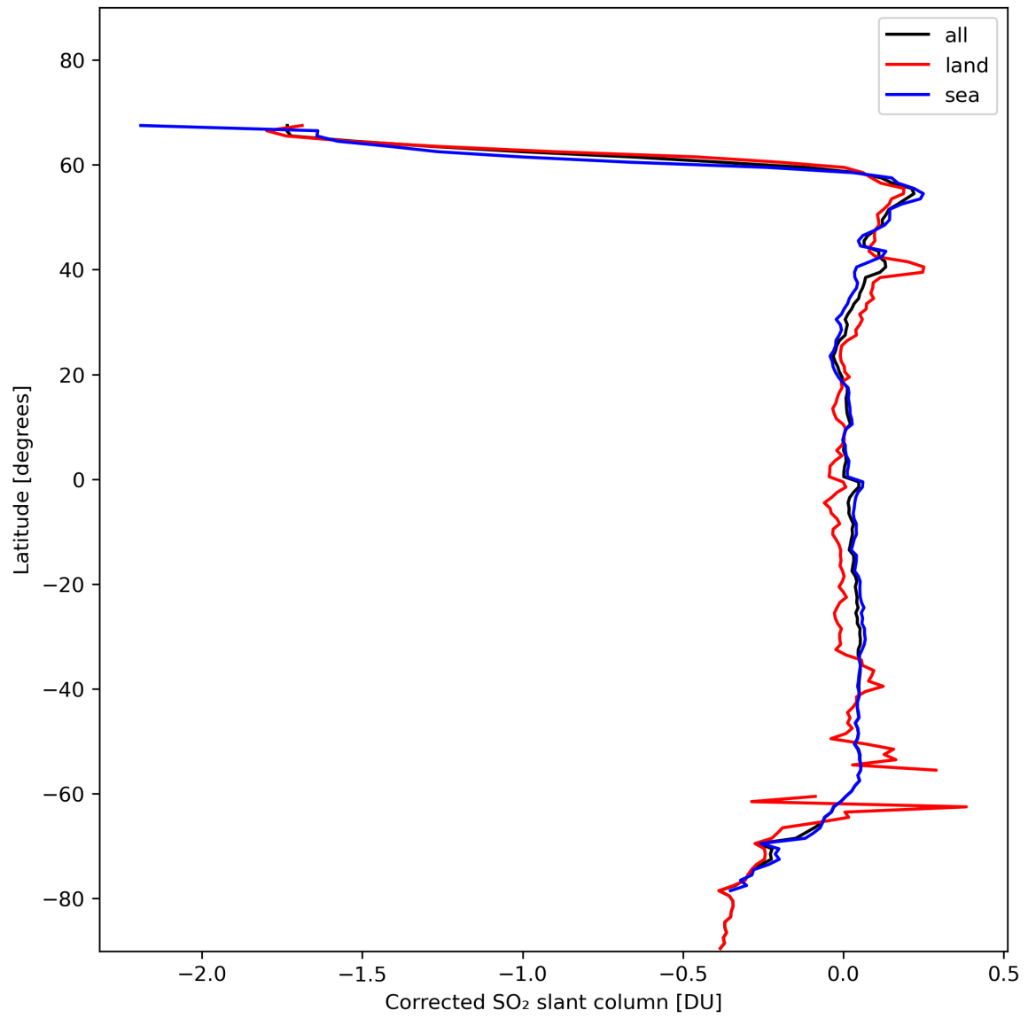
Figure 32: Zonal average of “Corrected SO 2 slant column” for 2023-11-13 to 2023-11-14.
