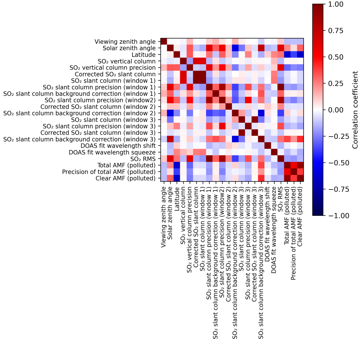
Figure 2: Map of correlation matrix for 2023-11-13 to 2023-11-14.
