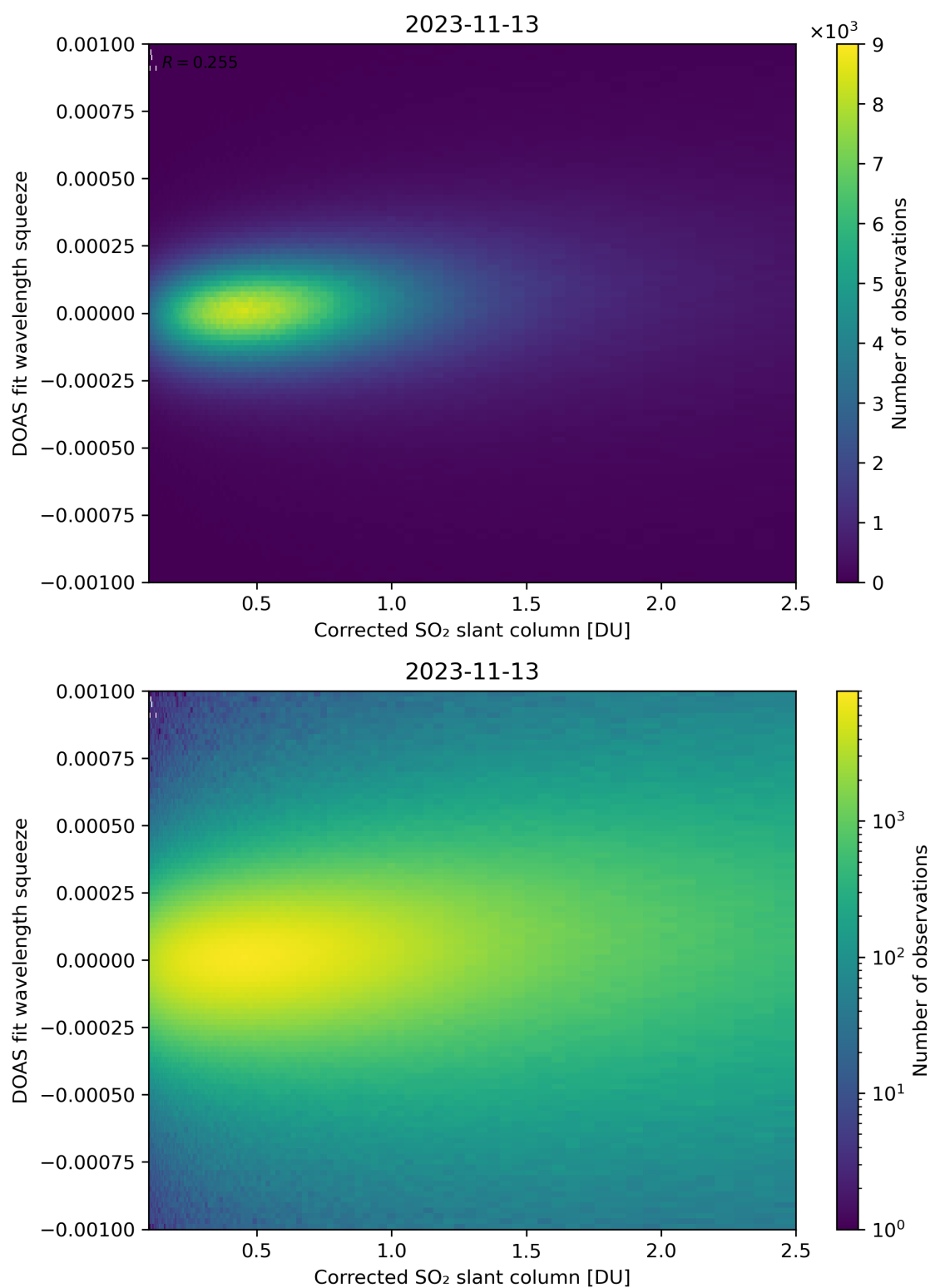
Figure 182: Scatter density plot of “Corrected SO 2 slant column” against “DOAS fit wavelength squeeze” for 2023-11-13 to 2023-11-14.
