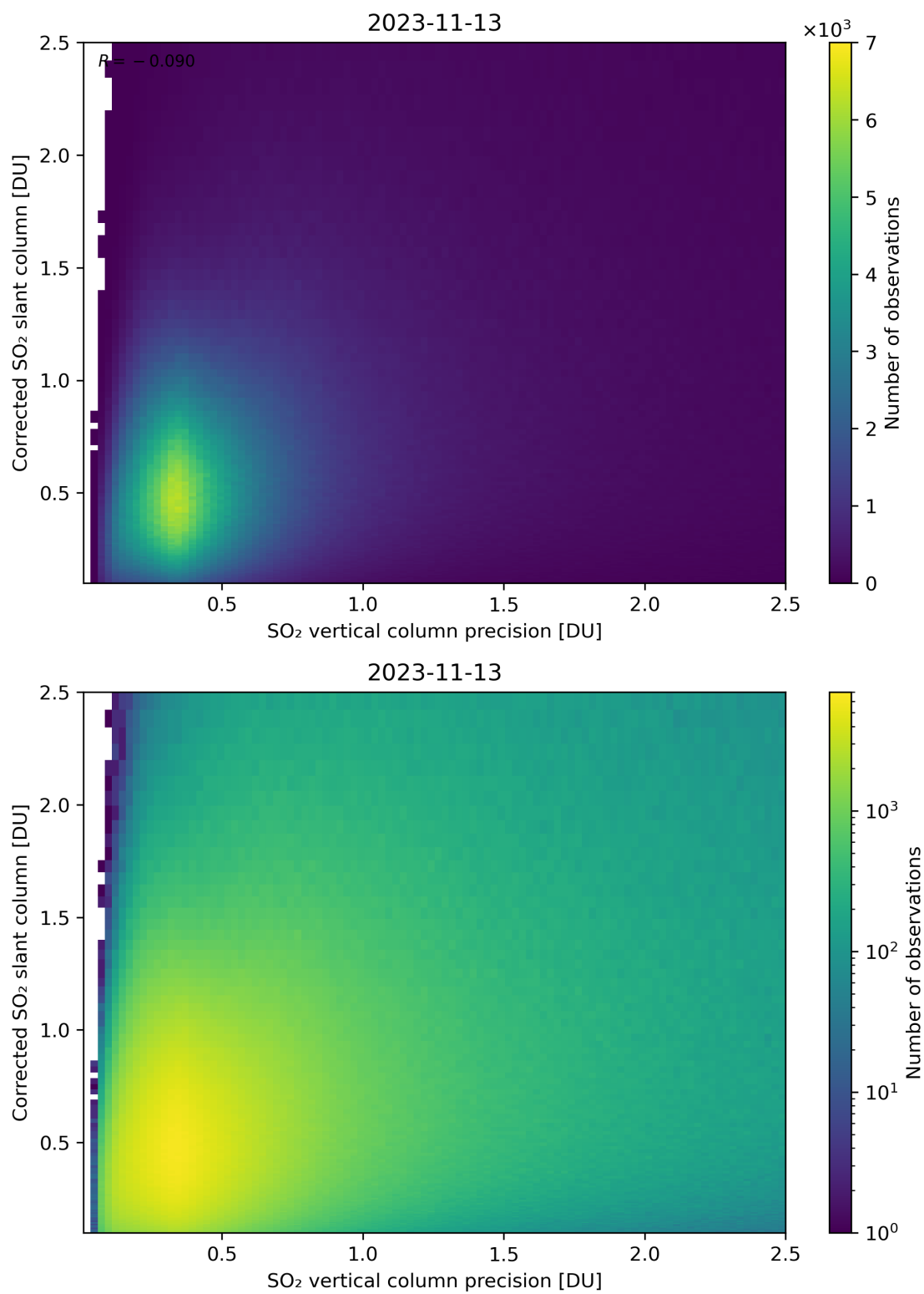
Figure 286: Scatter density plot of “SO 2 vertical column precision” against “Corrected SO 2 slant column” for 2023-11-13 to 2023-11-14.
