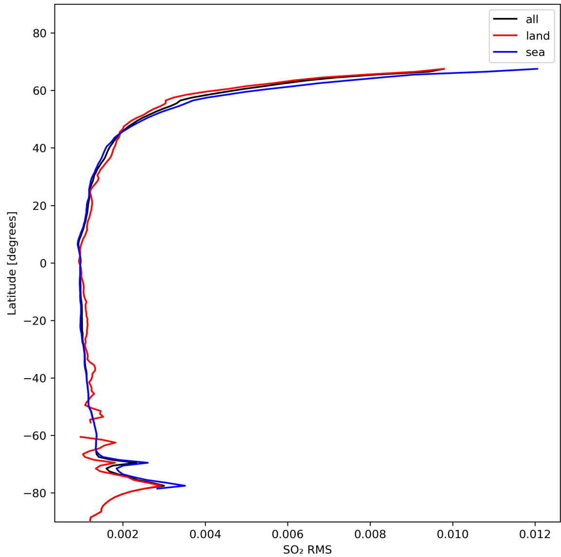
Figure 47: Zonal average of “SO 2 RMS” for 2023-11-13 to 2023-11-14.
