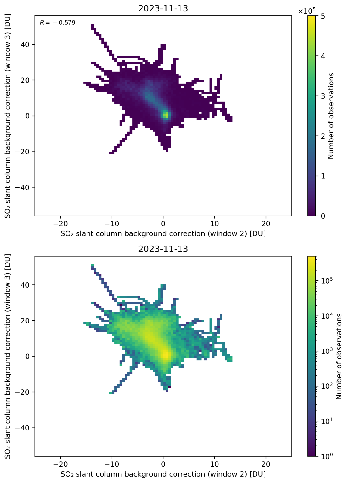
Figure 111: Scatter density plot of “SO 2 slant column background correction (window 2)” against “SO 2 slant column background correction (window 3)” for 2023-11-13 to 2023-11-14.
