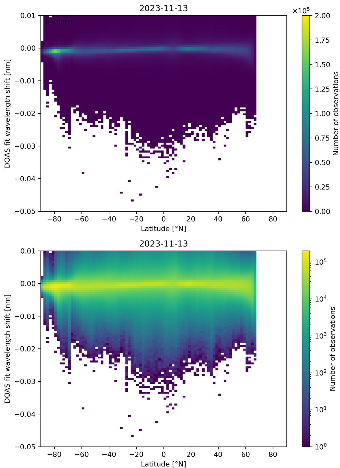
Figure 142: Scatter density plot of “Latitude” against “DOAS fit wavelength shift” for 2023-11-13 to 2023-11-14.
