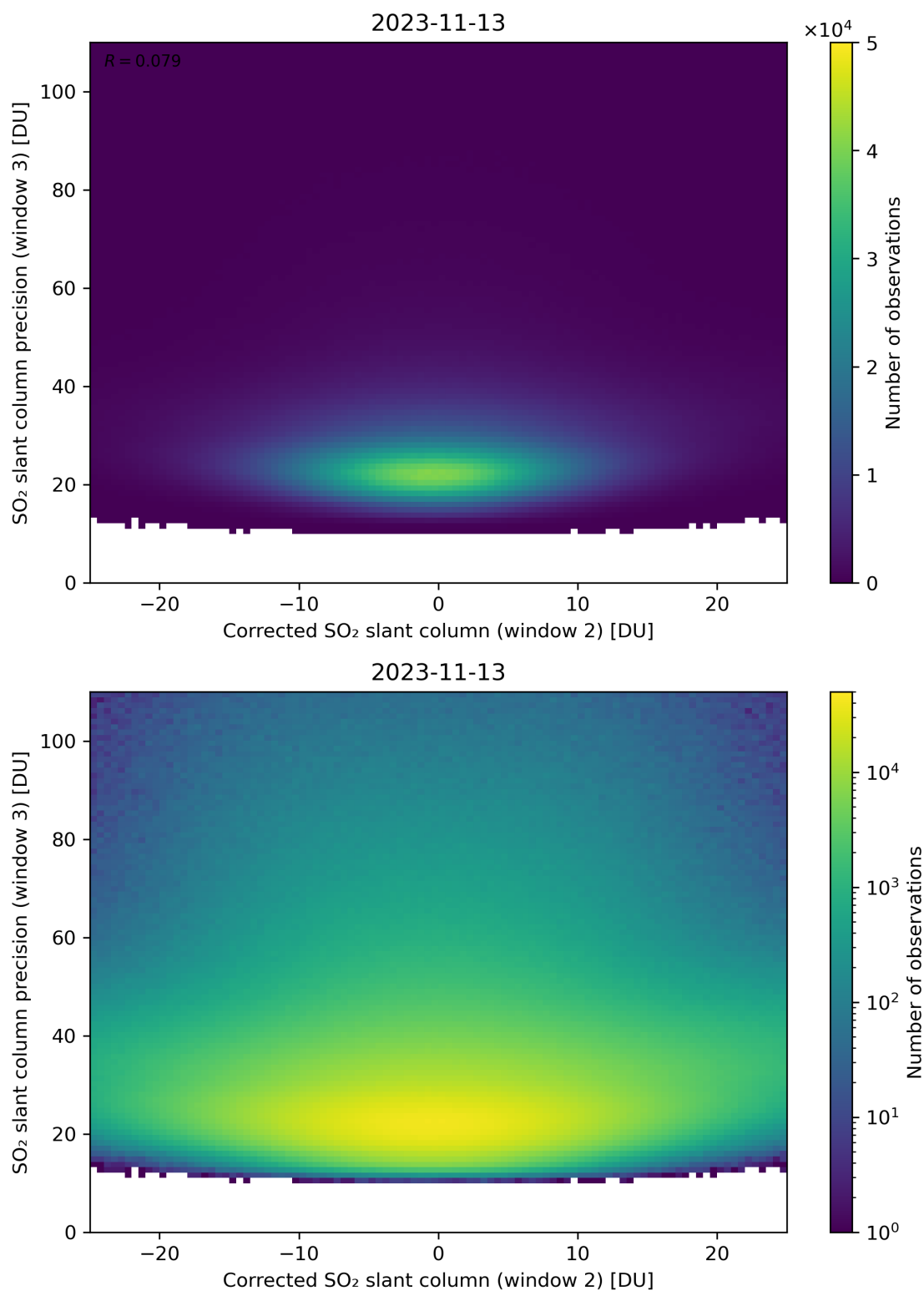
Figure 202: Scatter density plot of “Corrected SO 2 slant column (window 2)” against “SO 2 slant column precision (window 3)” for 2023-11-13 to 2023-11-14.
