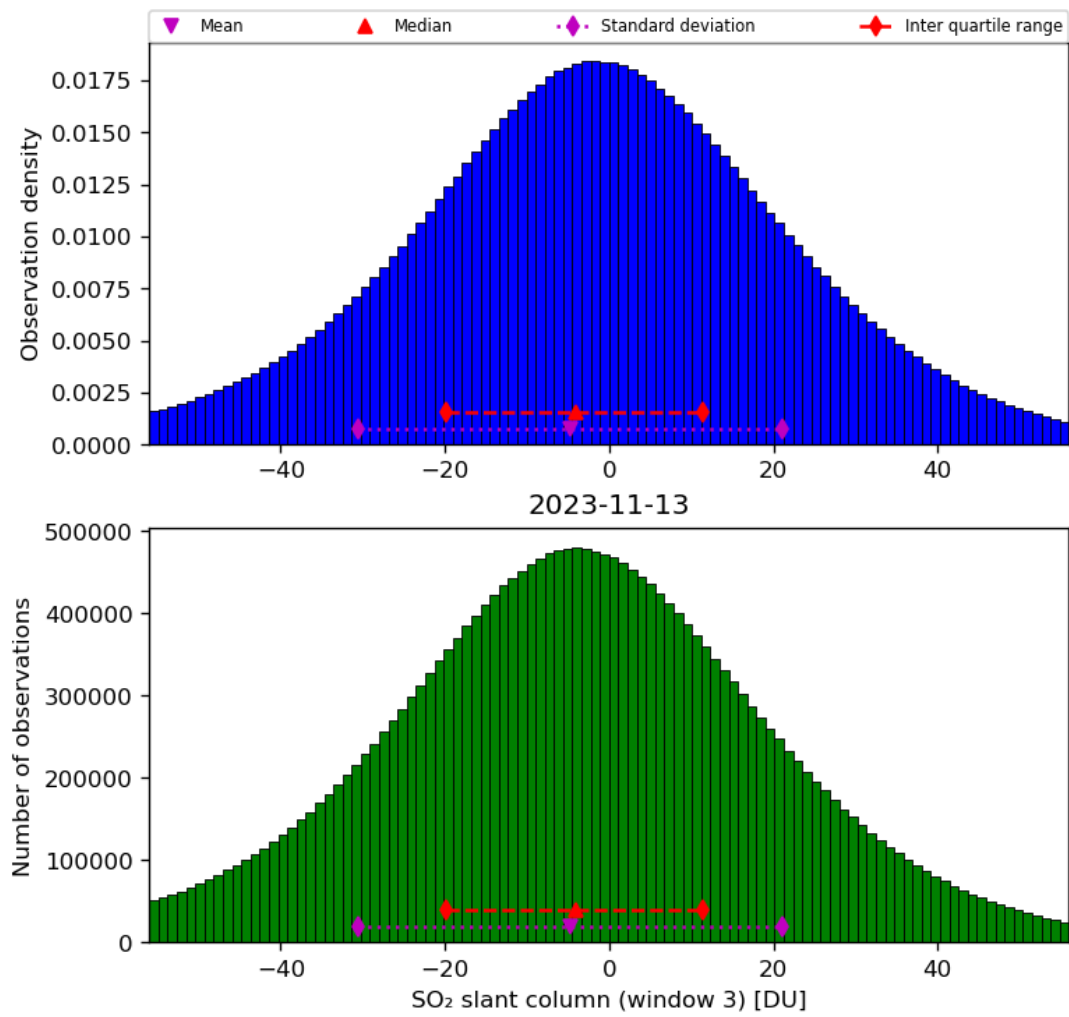
Figure 64: Histogram of “SO 2 slant column (window 3)” for 2023-11-13 to 2023-11-14
