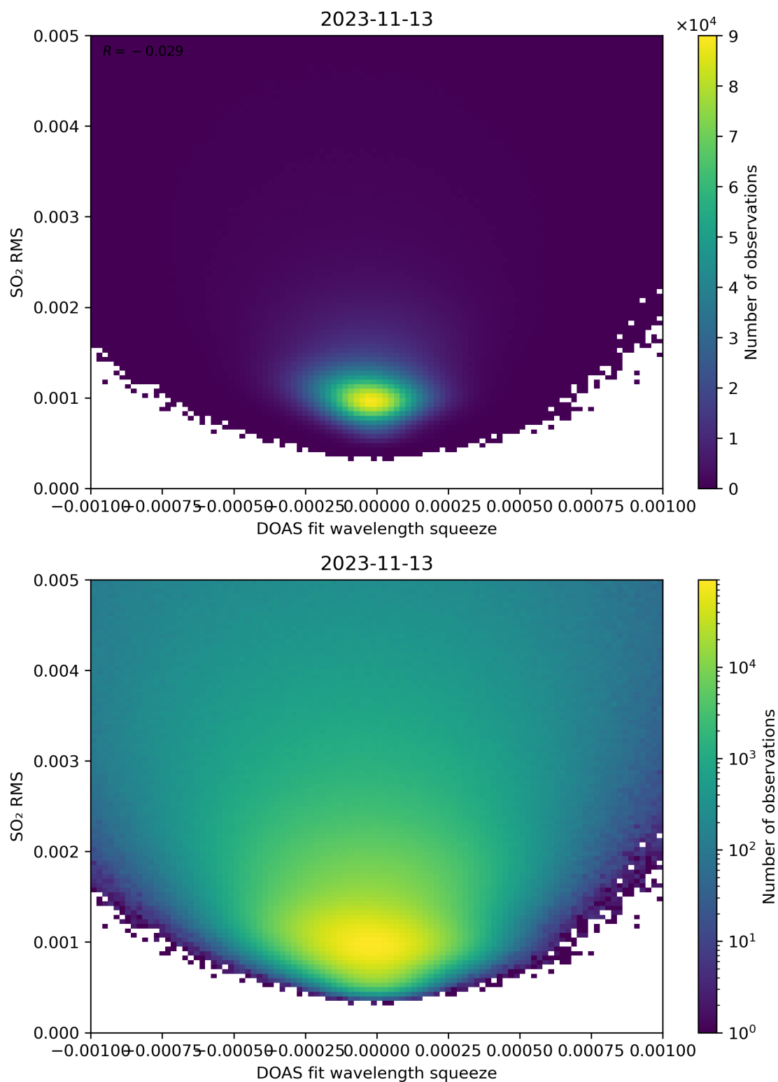
Figure 132: Scatter density plot of “DOAS fit wavelength squeeze” against “SO 2 RMS” for 2023-11-13 to 2023-11-14.
