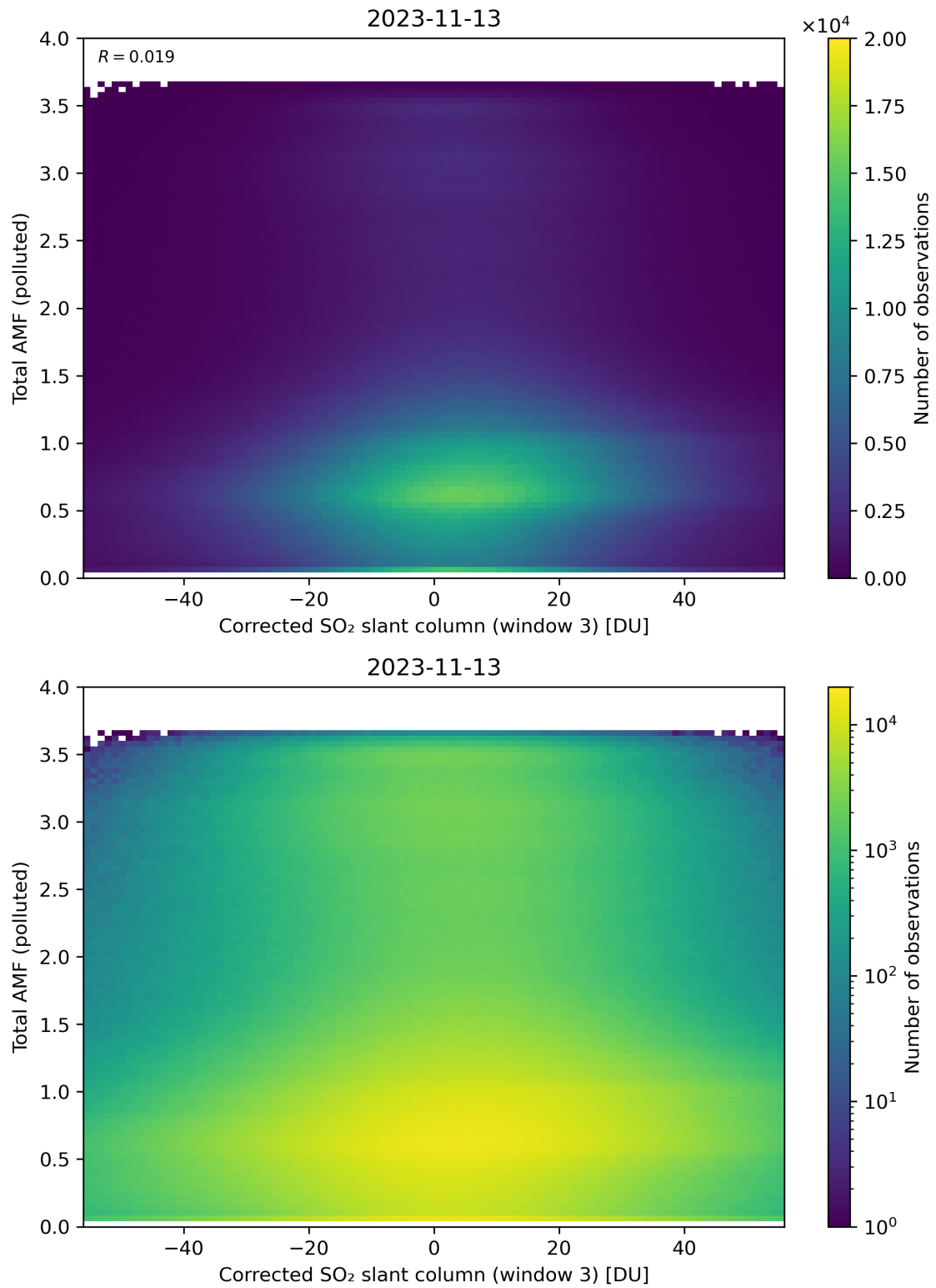
Figure 210: Scatter density plot of “Corrected SO 2 slant column (window 3)” against “Total AMF (polluted)” for 2023-11-13 to 2023-11-14.
