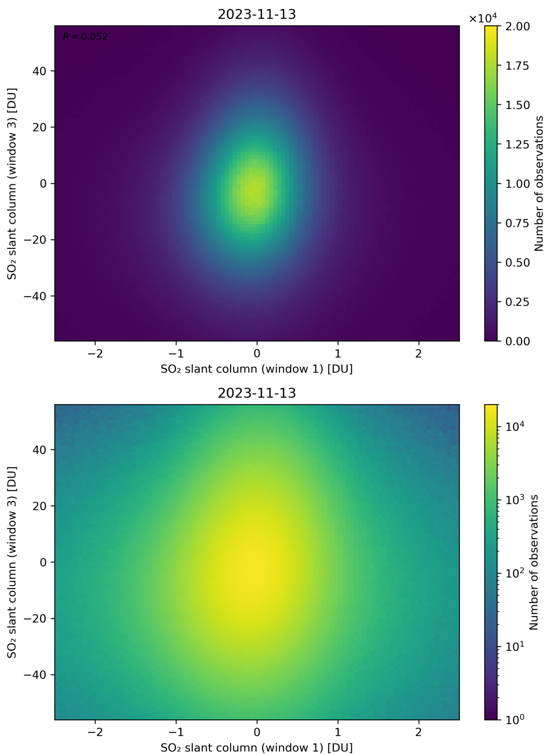
Figure 237: Scatter density plot of “SO 2 slant column (window 1)” against “SO 2 slant column (window 3)” for 2023-11-13 to 2023-11-14.
