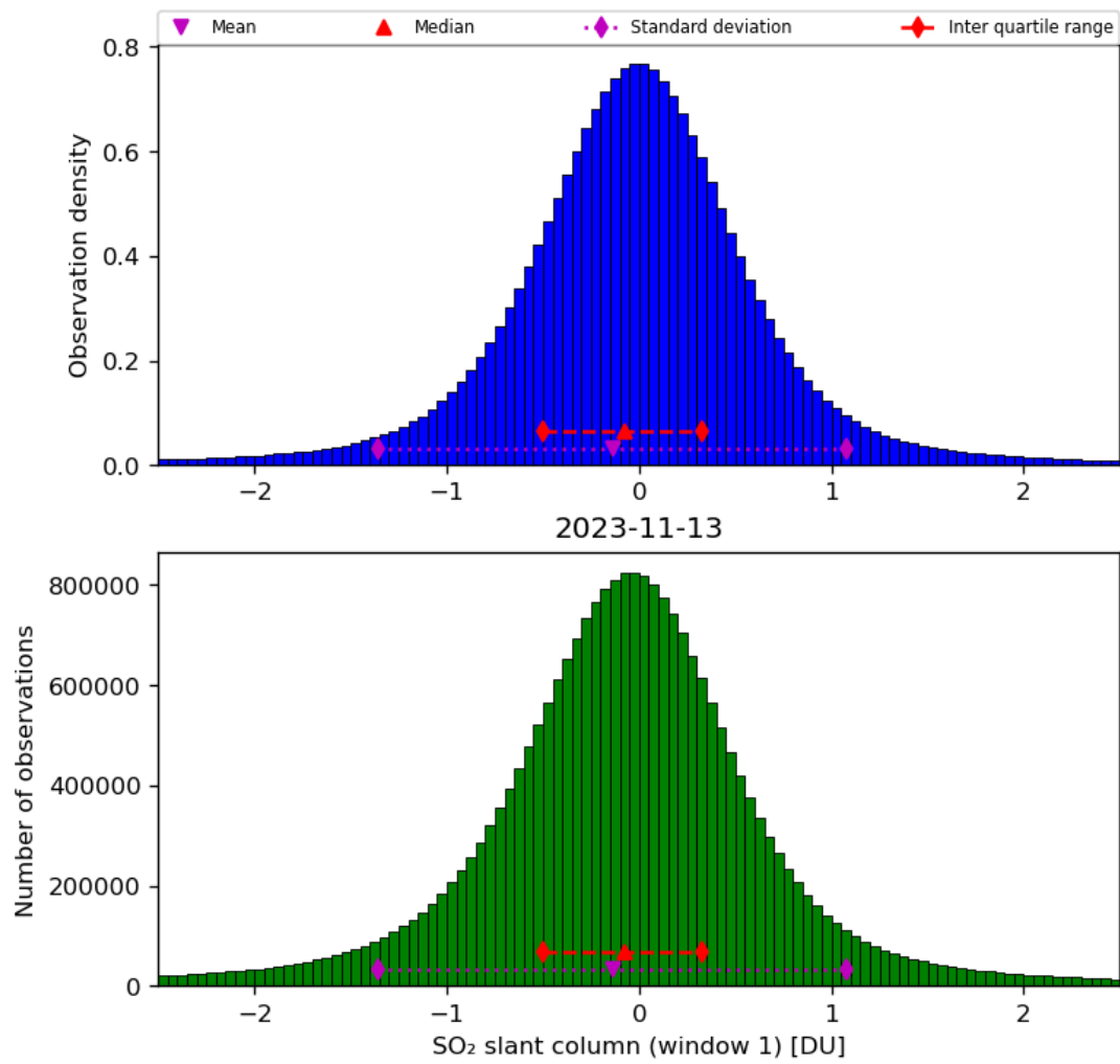
Figure 56: Histogram of “SO 2 slant column (window 1)” for 2023-11-13 to 2023-11-14
