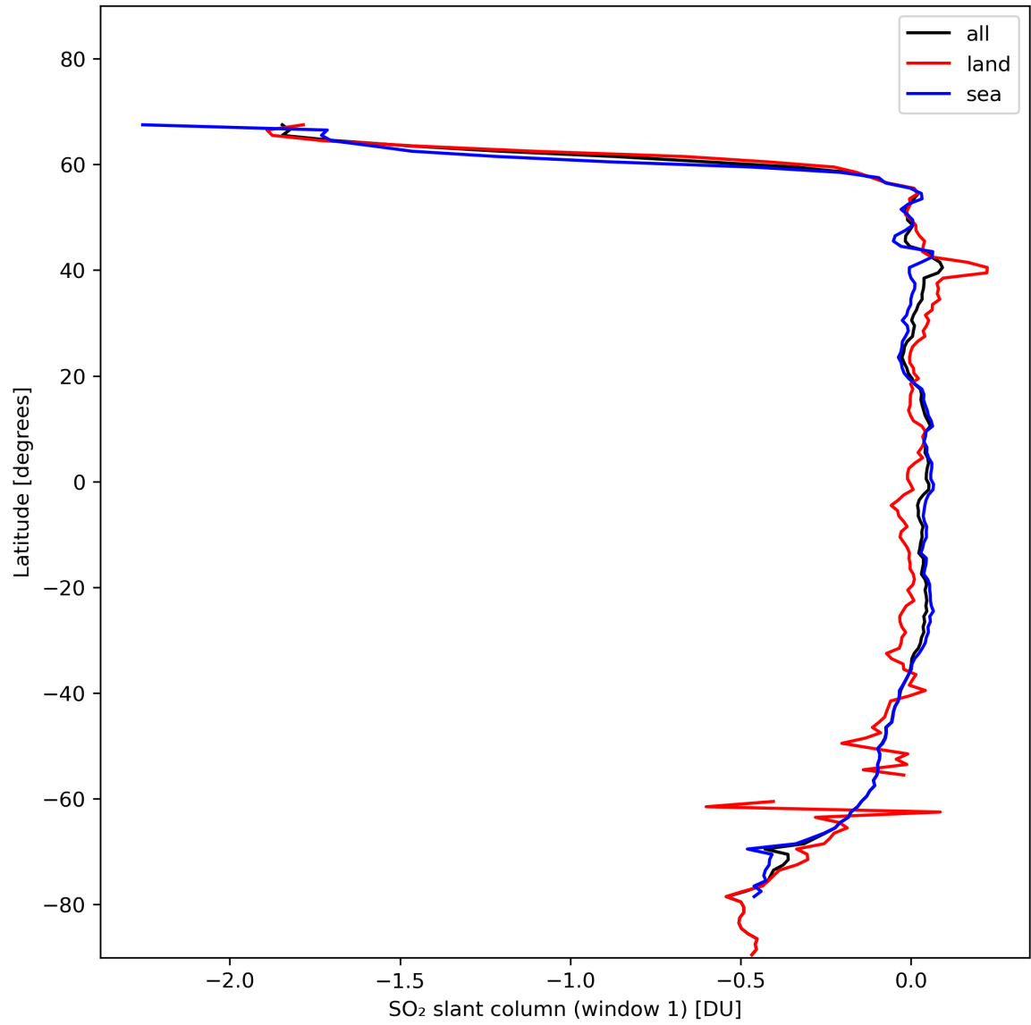
Figure 33: Zonal average of “SO 2 slant column (window 1)” for 2023-11-13 to 2023-11-14.
