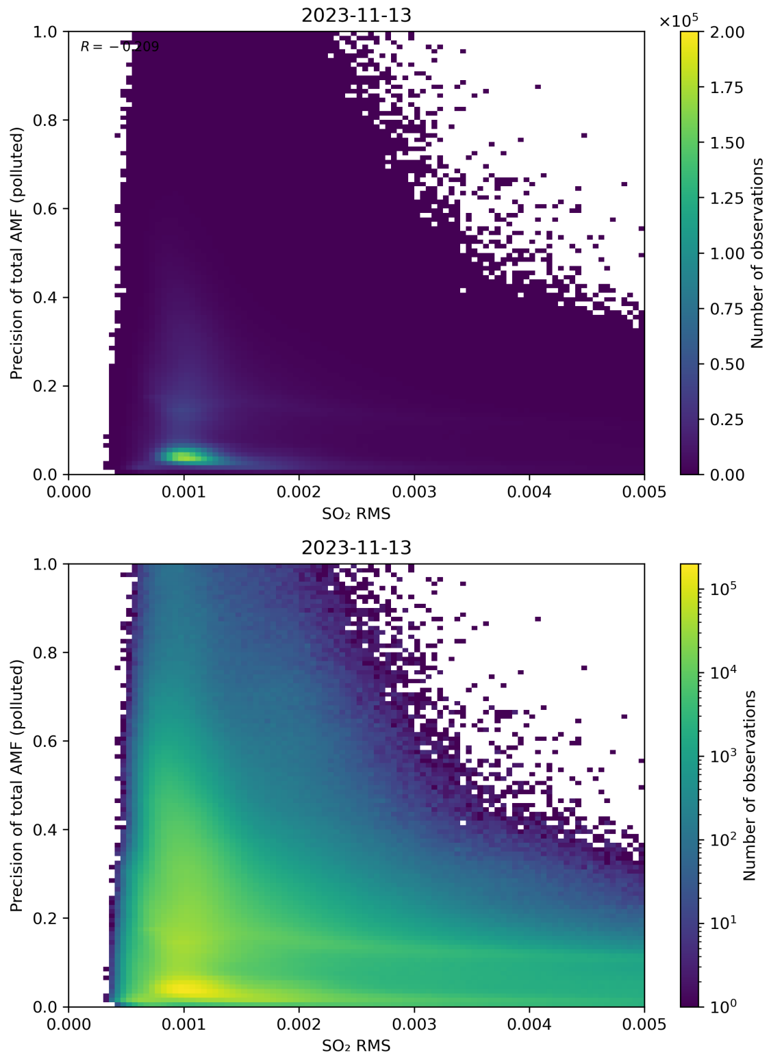
Figure 138: Scatter density plot of “SO 2 RMS” against “Precision of total AMF (polluted)” for 2023-11-13 to 2023-11-14.
