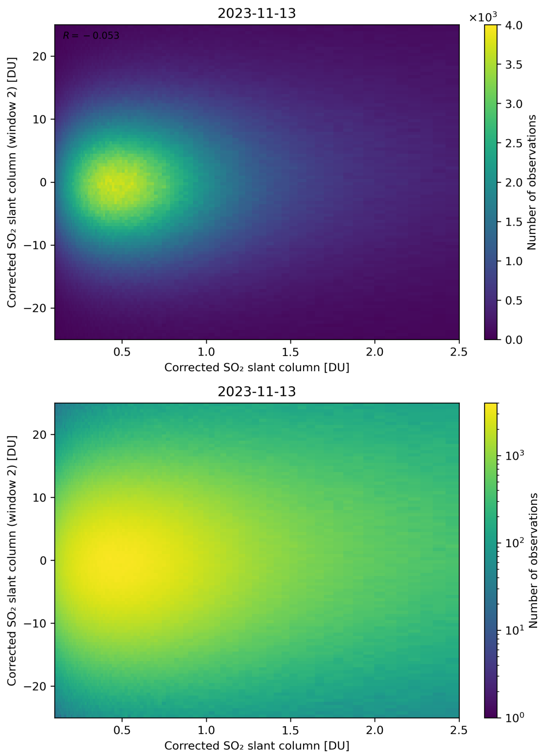
Figure 185: Scatter density plot of “Corrected SO 2 slant column” against “Corrected SO 2 slant column (window 2)” for 2023-11-13 to 2023-11-14.
