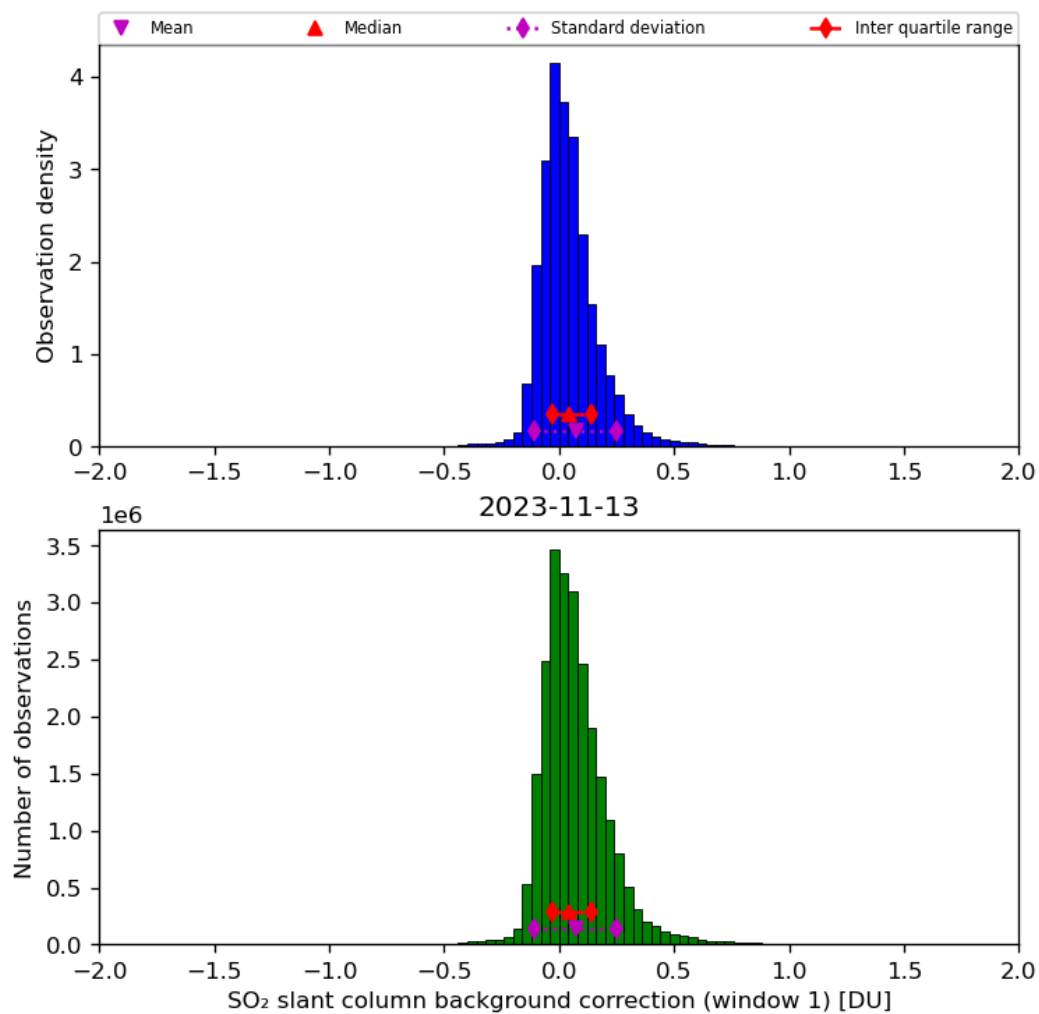
Figure 59: Histogram of “SO 2 slant column background correction (window 1)” for 2023-11-13 to 2023-11-14
