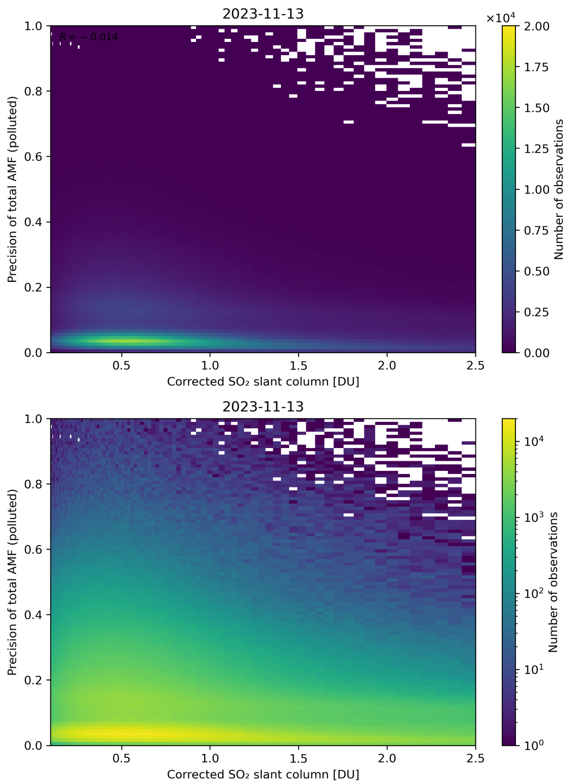
Figure 193: Scatter density plot of “Corrected SO 2 slant column” against “Precision of total AMF (polluted)” for 2023-11-13 to 2023-11-14.
