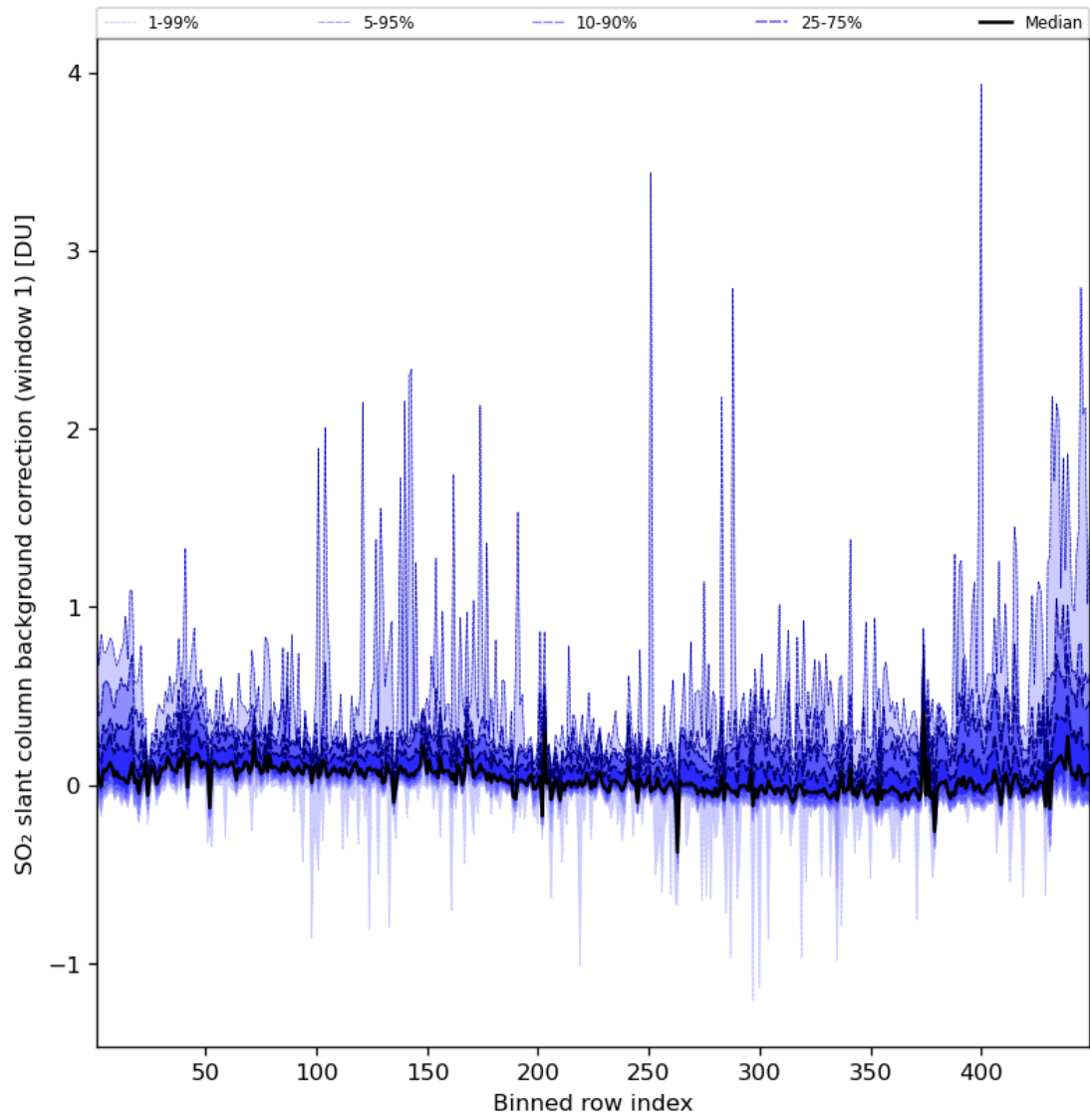
Figure 82: Along track statistics of “SO 2 slant column background correction (window 1)” for 2023-11-13 to 2023-11-14
