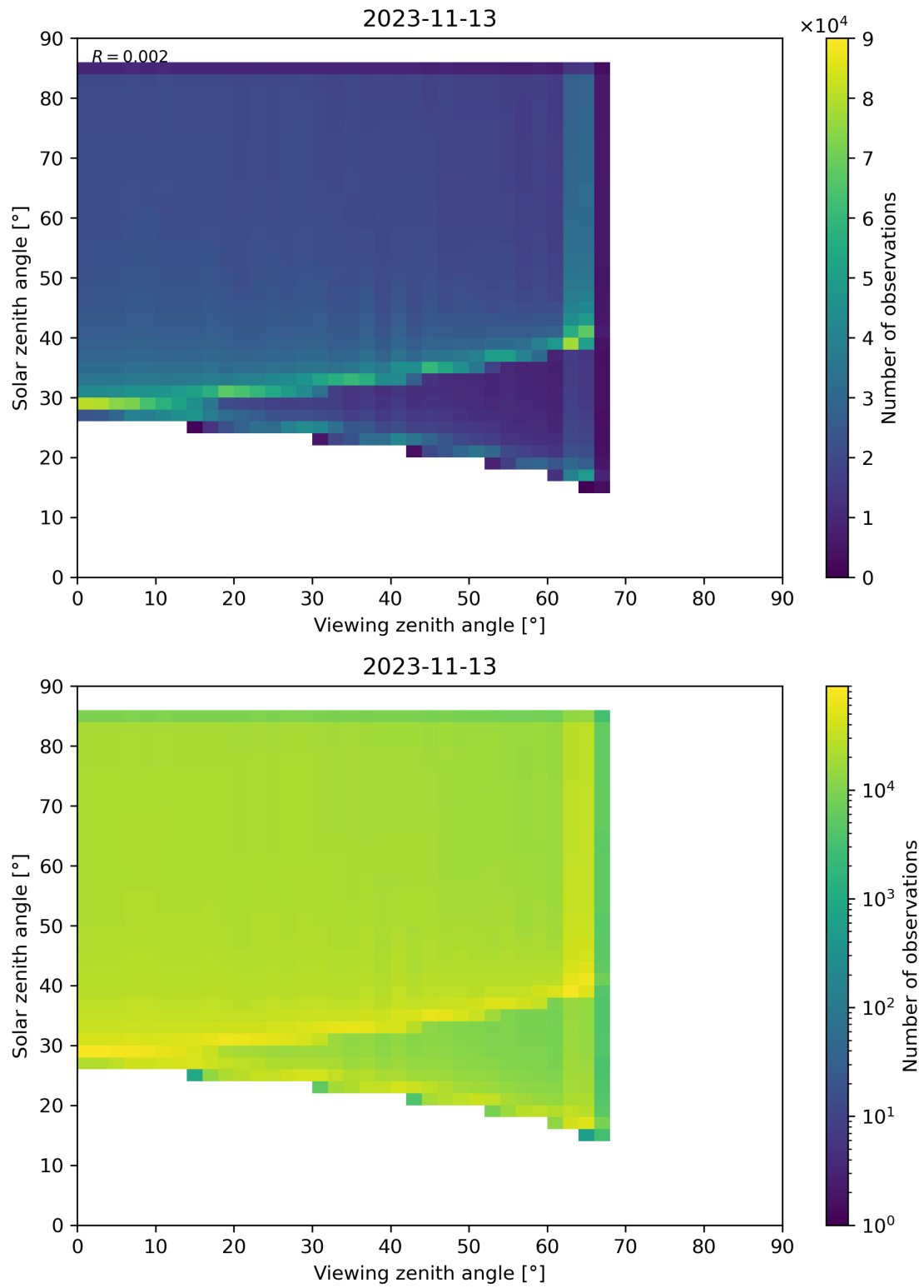
Figure 315: Scatter density plot of “Viewing zenith angle” against “Solar zenith angle” for 2023-11-13 to 2023-11-14.
