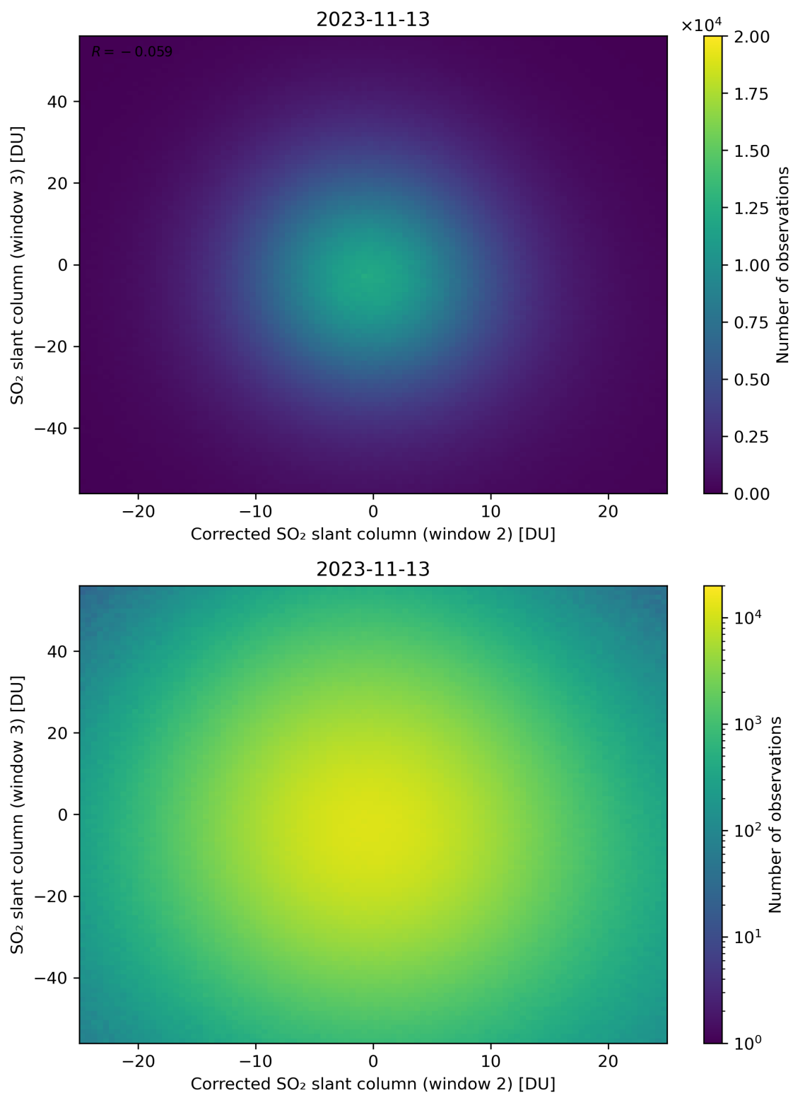
Figure 201: Scatter density plot of “Corrected SO 2 slant column (window 2)” against “SO 2 slant column (window 3)” for 2023-11-13 to 2023-11-14.
