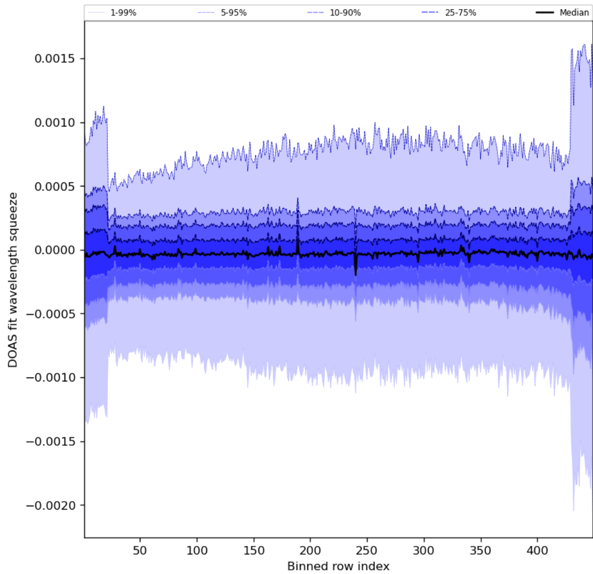
Figure 92: Along track statistics of “DOAS fit wavelength squeeze” for 2023-11-13 to 2023-11-14
