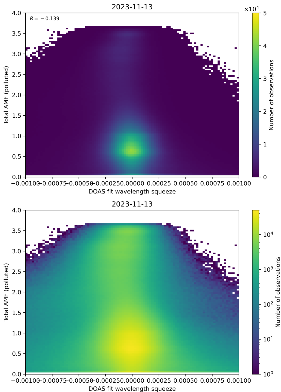
Figure 134: Scatter density plot of “DOAS fit wavelength squeeze” against “Total AMF (polluted)” for 2023-11-13 to 2023-11-14.
