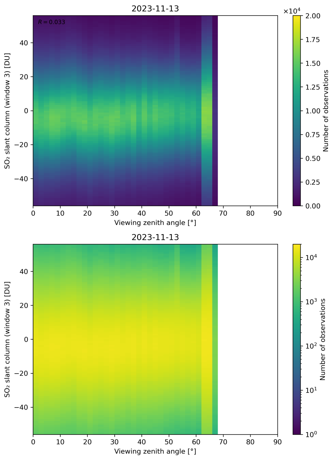
Figure 323: Scatter density plot of “Viewing zenith angle” against “SO 2 slant column (window 3)” for 2023-11-13 to 2023-11-14.
