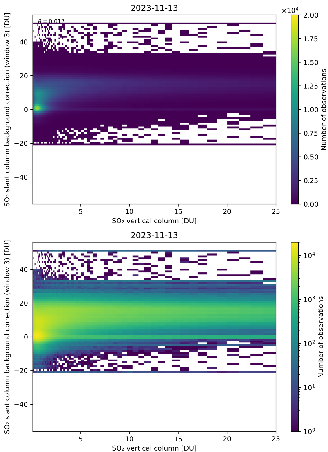
Figure 275: Scatter density plot of “SO 2 vertical column” against “SO 2 slant column background correction (window 3)” for 2023-11-13 to 2023-11-14.
