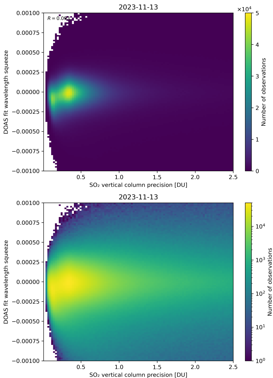
Figure 283: Scatter density plot of “SO 2 vertical column precision” against “DOAS fit wavelength squeeze” for 2023-11-13 to 2023-11-14.
