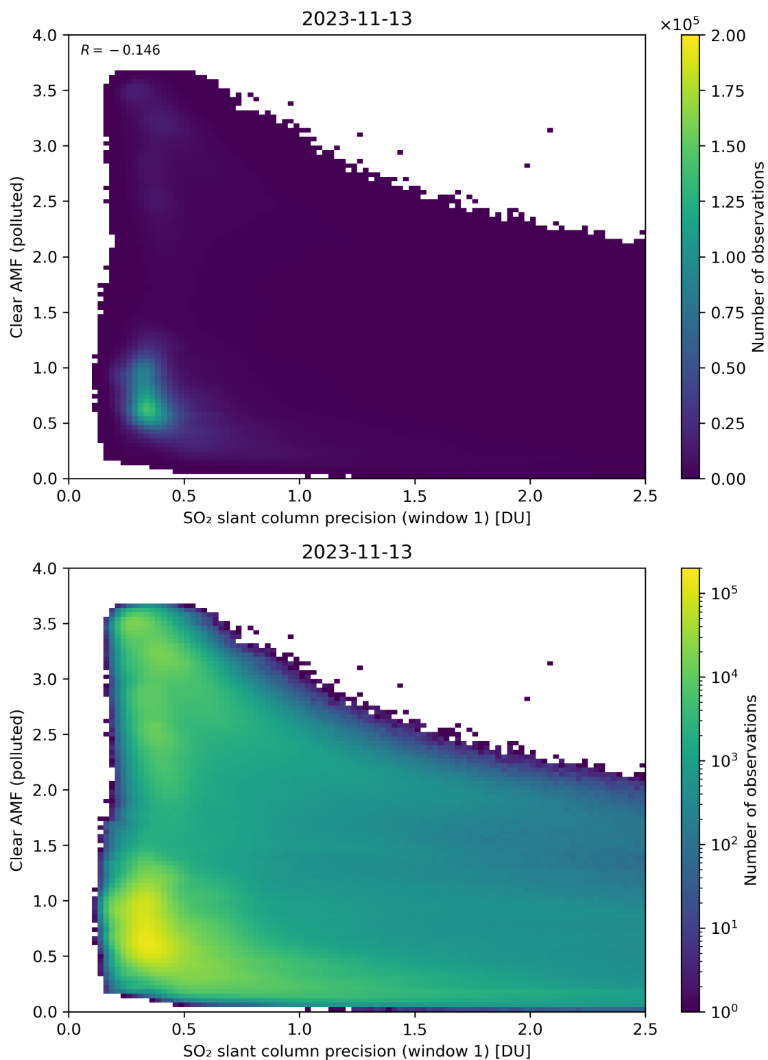
Figure 224: Scatter density plot of “SO 2 slant column precision (window 1)” against “Clear AMF (polluted)” for 2023-11-13 to 2023-11-14.
