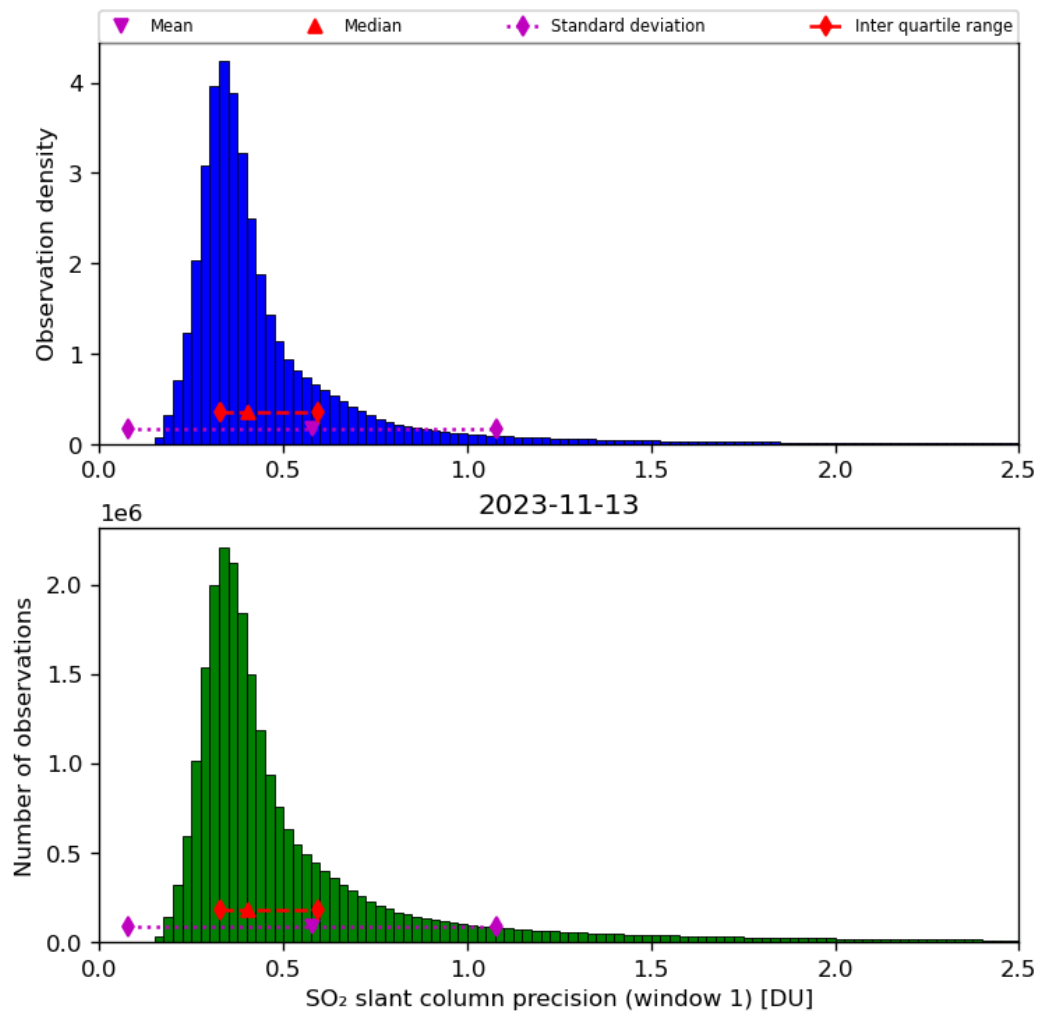
Figure 57: Histogram of “SO 2 slant column precision (window 1)” for 2023-11-13 to 2023-11-14
