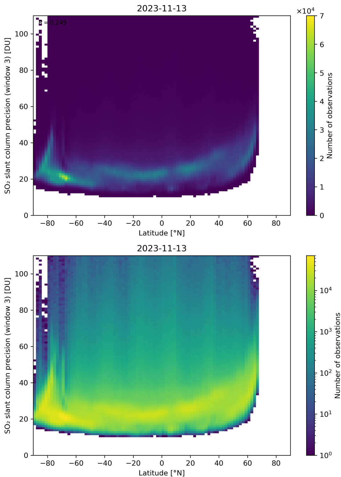
Figure 153: Scatter density plot of “Latitude” against “SO 2 slant column precision (window 3)” for 2023-11-13 to 2023-11-14.
