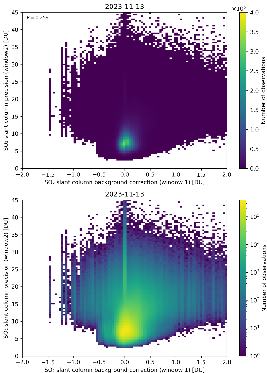
Figure 106: Scatter density plot of “SO 2 slant column background correction (window 1)” against “SO 2 slant column precision (window2)” for 2023-11-13 to 2023-11-14.
