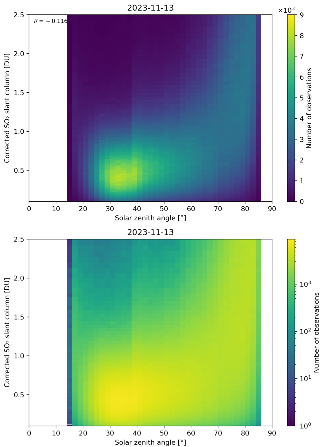
Figure 166: Scatter density plot of “Solar zenith angle” against “Corrected SO 2 slant column” for 2023-11-13 to 2023-11-14.
