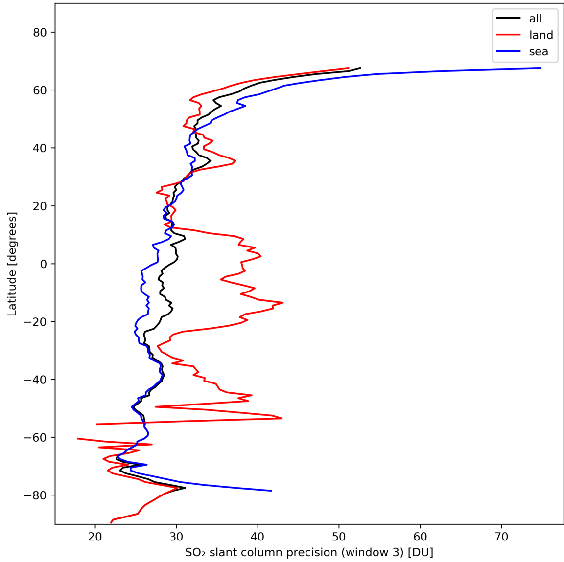
Figure 42: Zonal average of “SO 2 slant column precision (window 3)” for 2023-11-13 to 2023-11-14.
