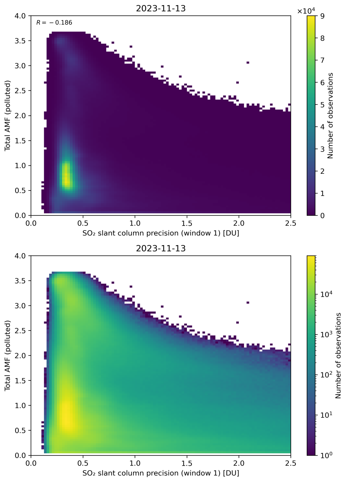
Figure 230: Scatter density plot of “SO 2 slant column precision (window 1)” against “Total AMF (polluted)” for 2023-11-13 to 2023-11-14.
