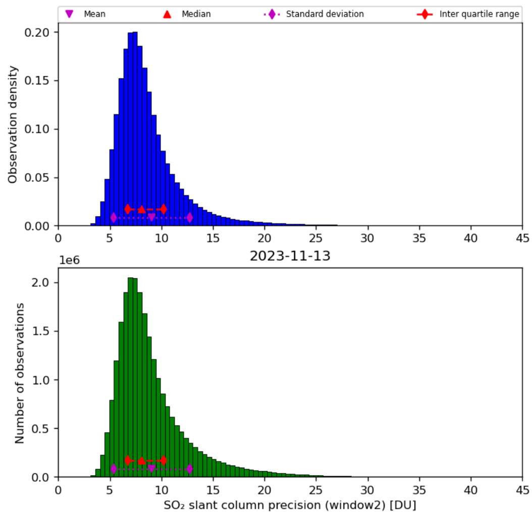
Figure 61: Histogram of “SO 2 slant column precision (window2)” for 2023-11-13 to 2023-11-14
