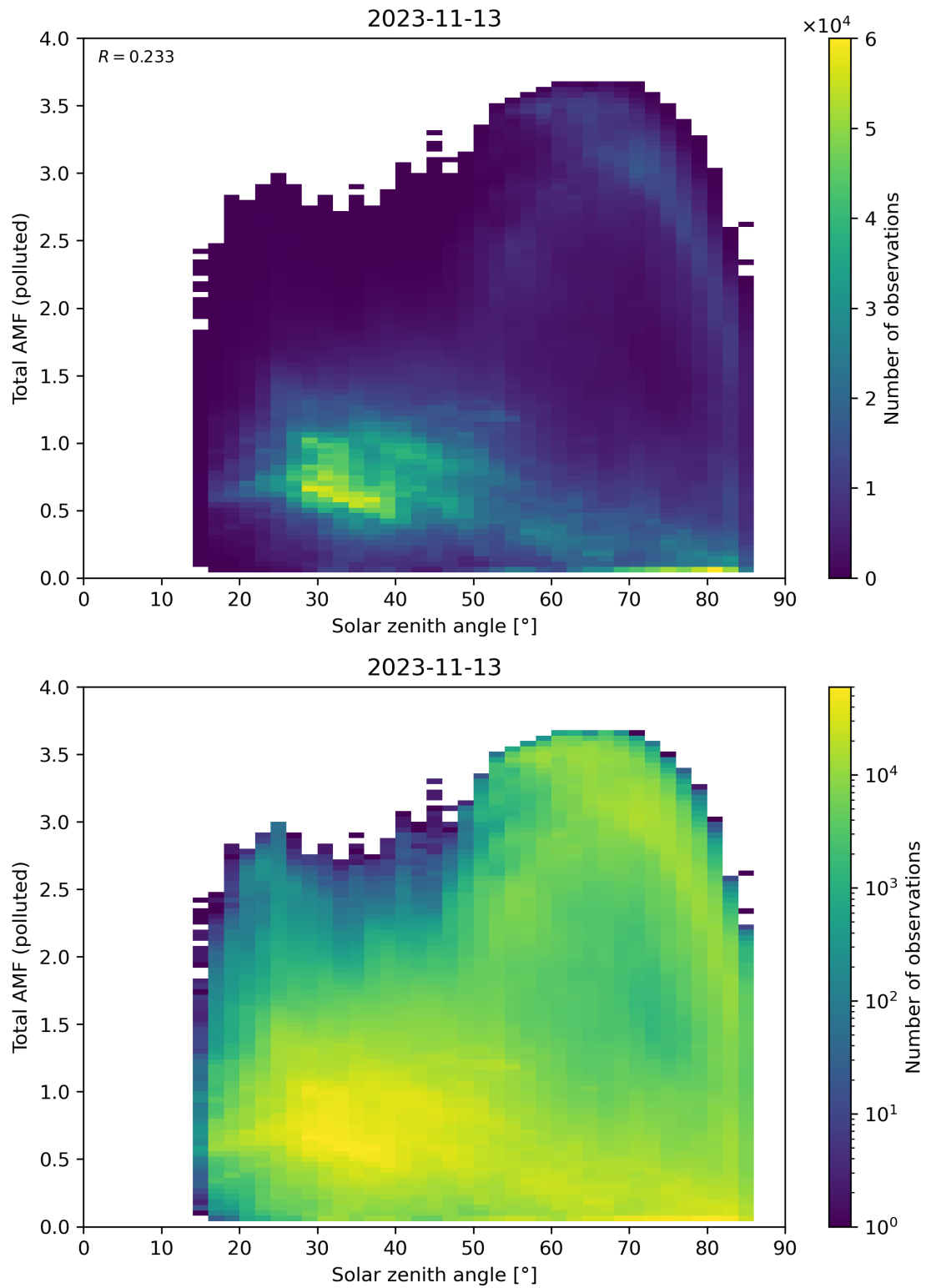
Figure 174: Scatter density plot of “Solar zenith angle” against “Total AMF (polluted)” for 2023-11-13 to 2023-11-14.
