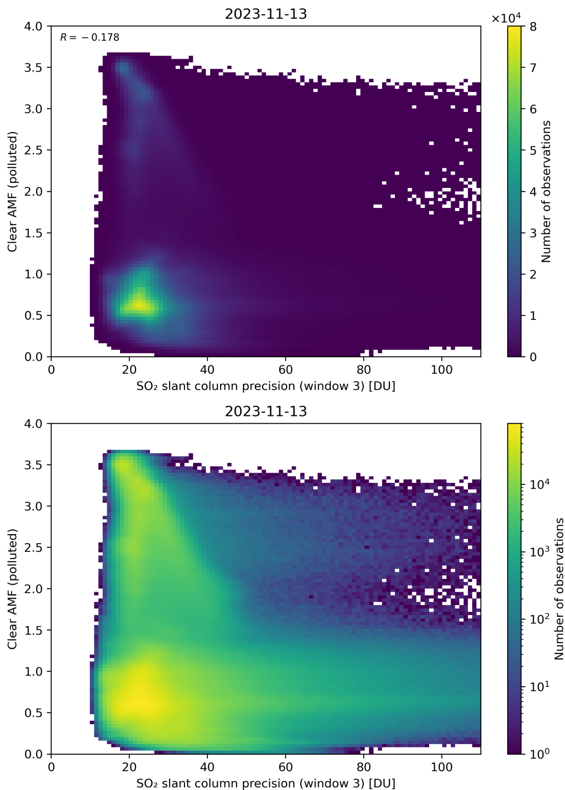
Figure 261: Scatter density plot of “SO 2 slant column precision (window 3)” against “Clear AMF (polluted)” for 2023-11-13 to 2023-11-14.
