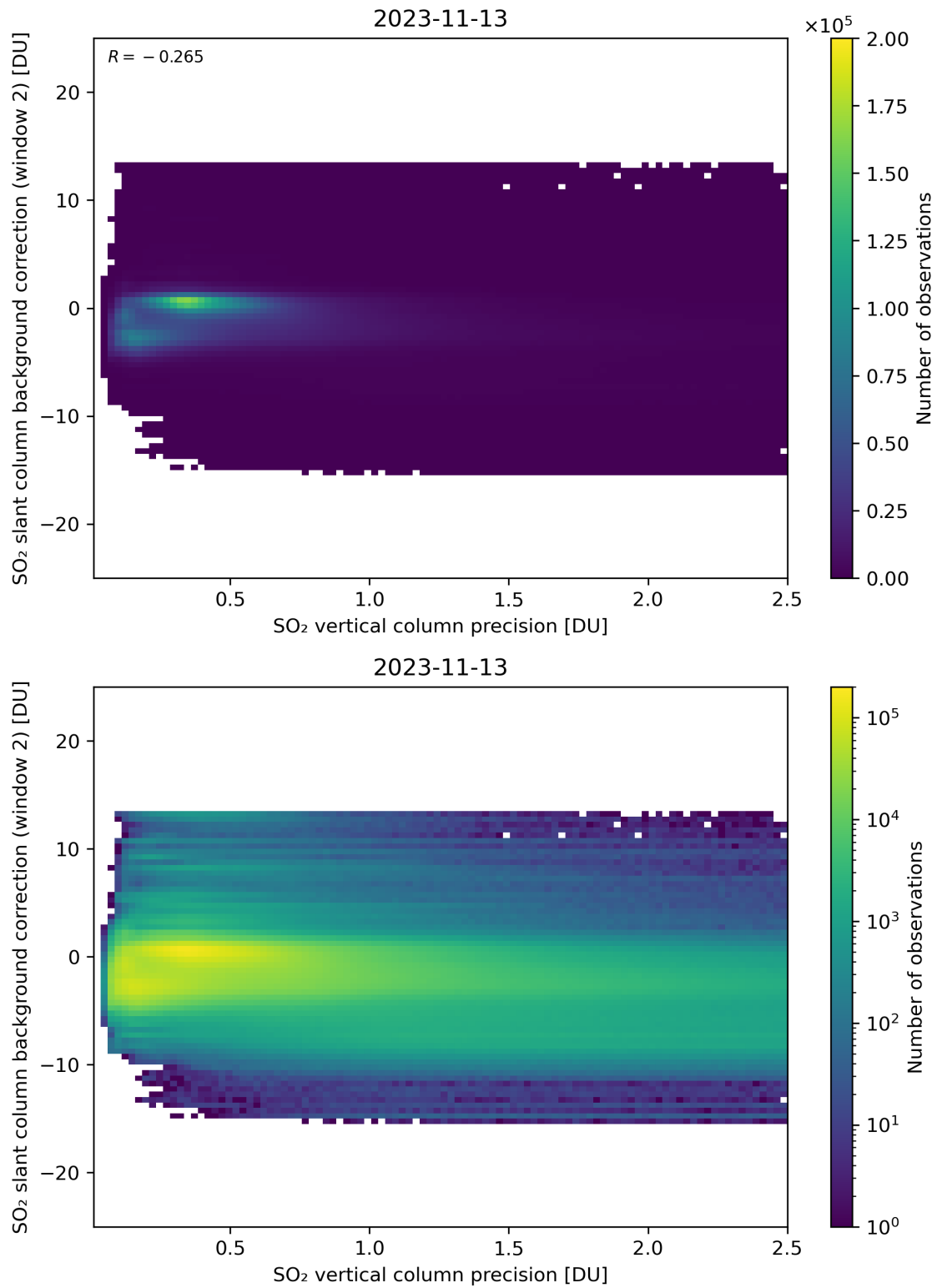
Figure 280: Scatter density plot of “SO 2 vertical column precision” against “SO 2 slant column background correction (window 2)” for 2023-11-13 to 2023-11-14.
