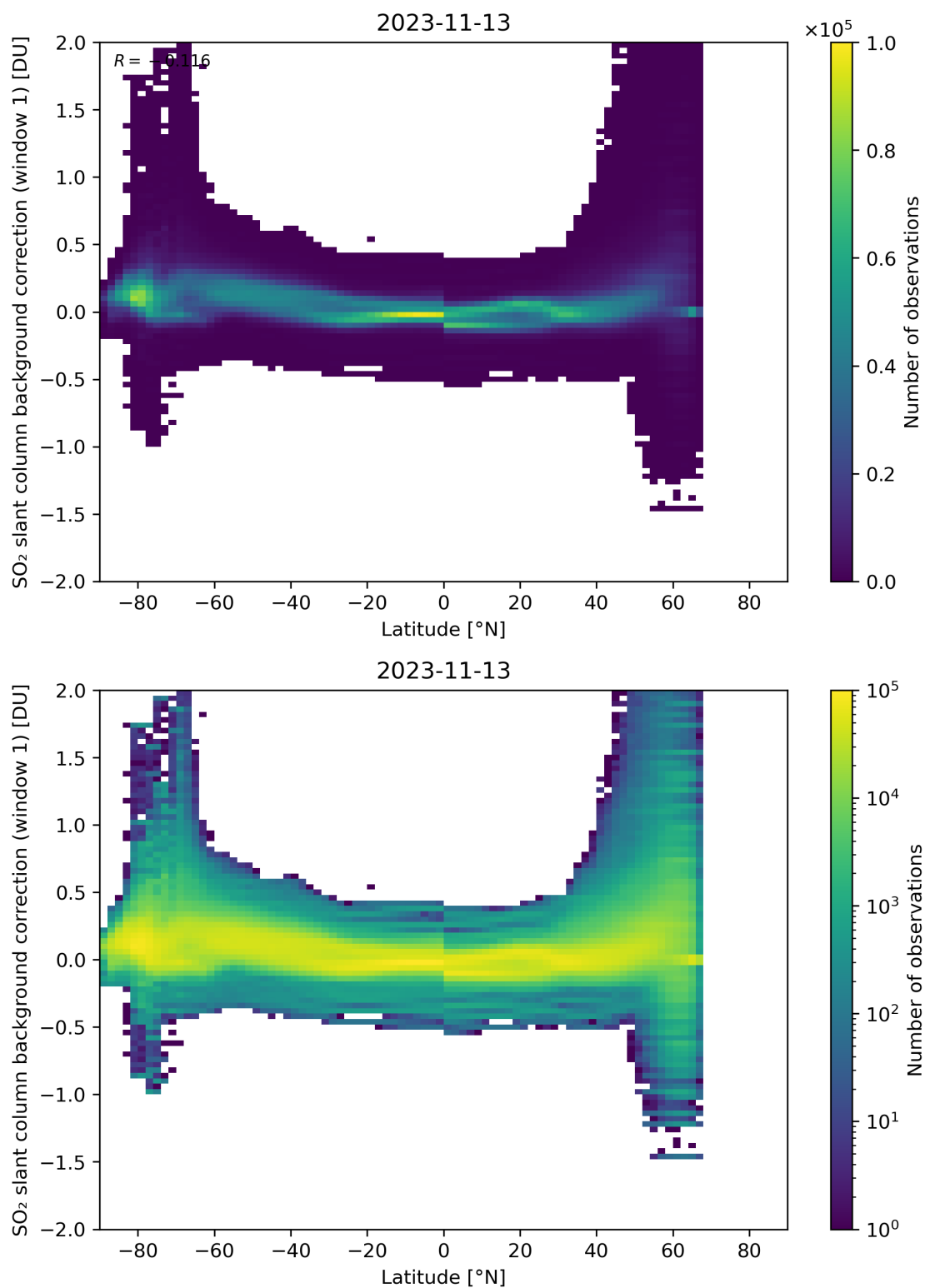
Figure 139: Scatter density plot of “Latitude” against “SO 2 slant column background correction (window 1)” for 2023-11-13 to 2023-11-14.
