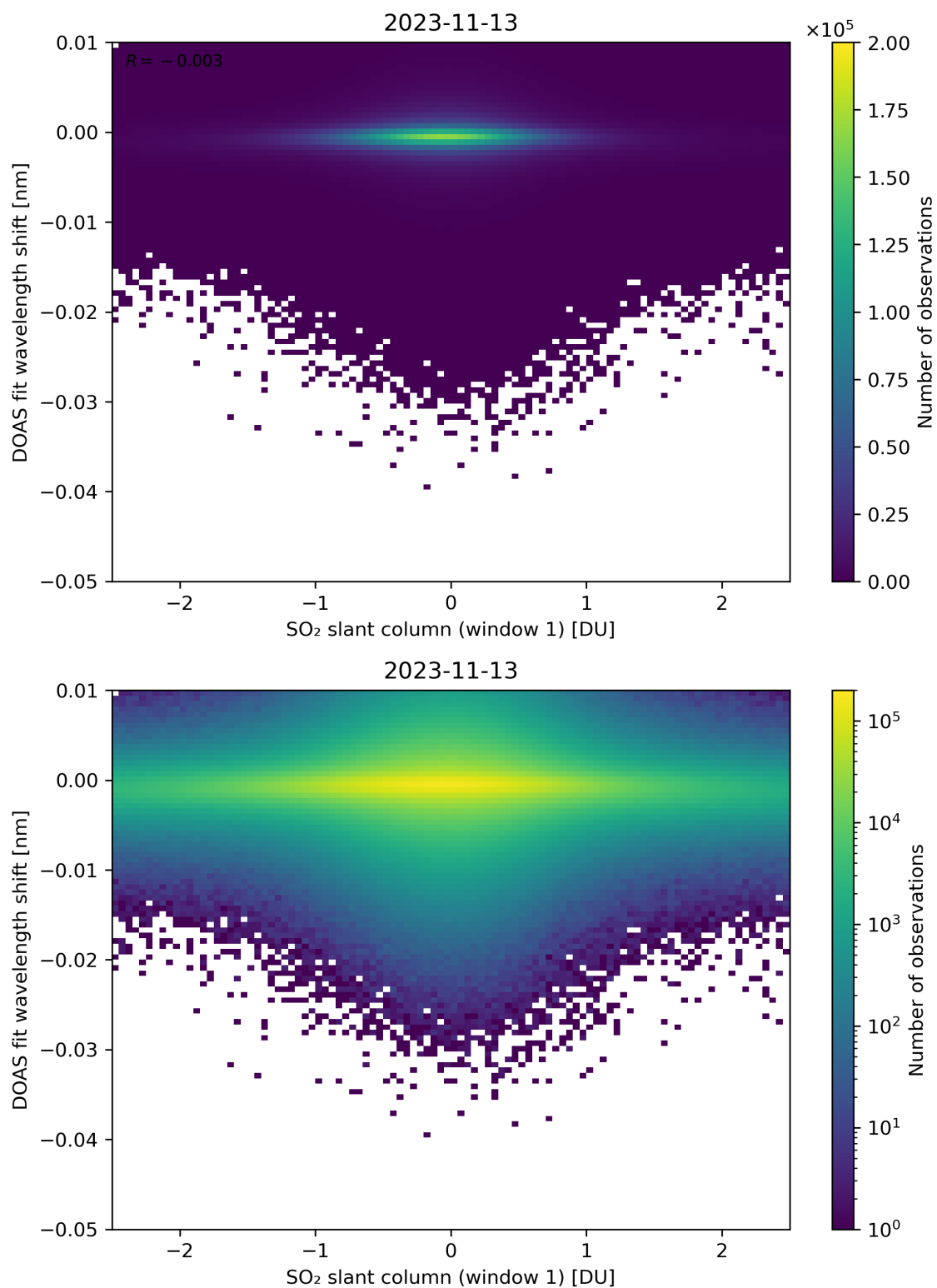
Figure 215: Scatter density plot of “SO 2 slant column (window 1)” against “DOAS fit wavelength shift” for 2023-11-13 to 2023-11-14.
