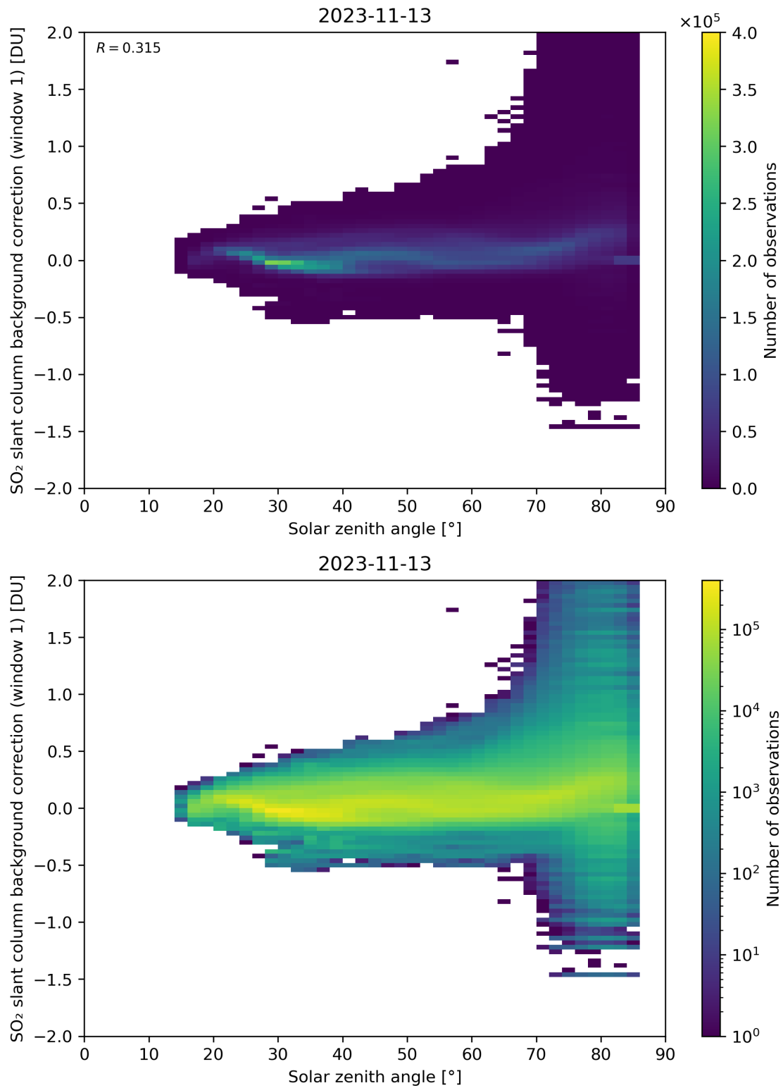
Figure 158: Scatter density plot of “Solar zenith angle” against “SO 2 slant column background correction (window 1)” for 2023-11-13 to 2023-11-14.
