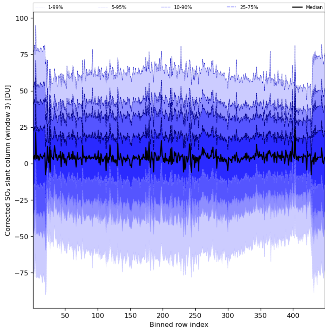
Figure 89: Along track statistics of “Corrected SO 2 slant column (window 3)” for 2023-11-13 to 2023-11-14
