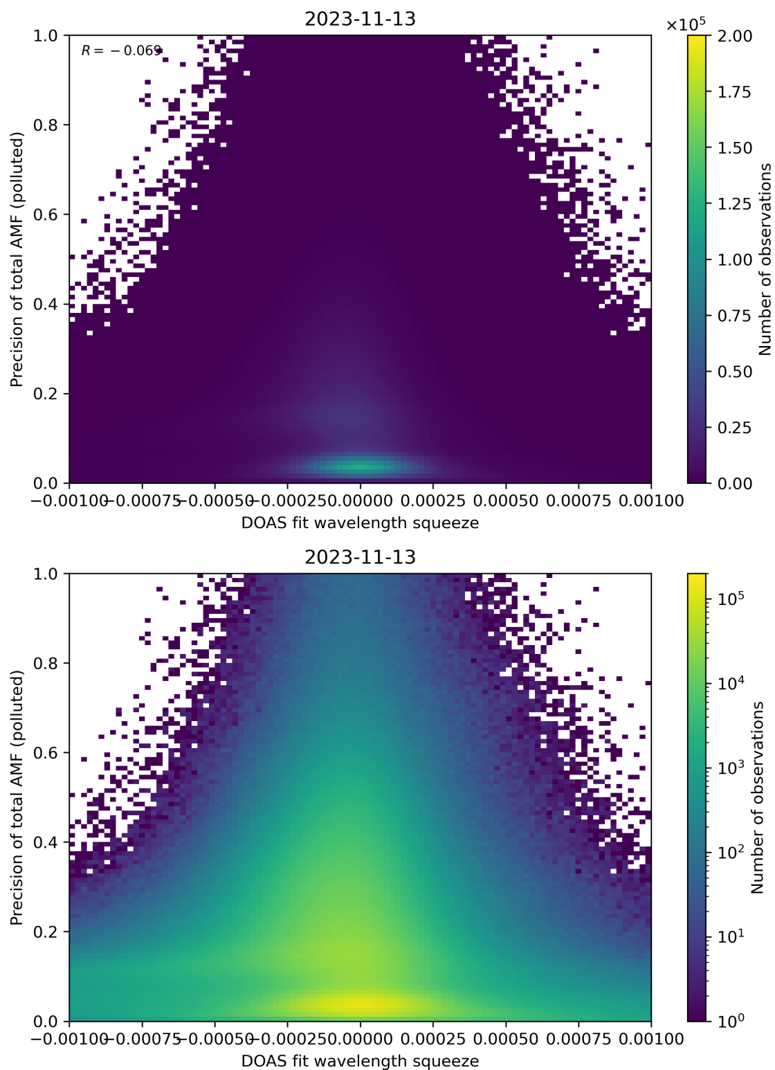
Figure 135: Scatter density plot of “DOAS fit wavelength squeeze” against “Precision of total AMF (polluted)” for 2023-11-13 to 2023-11-14.
