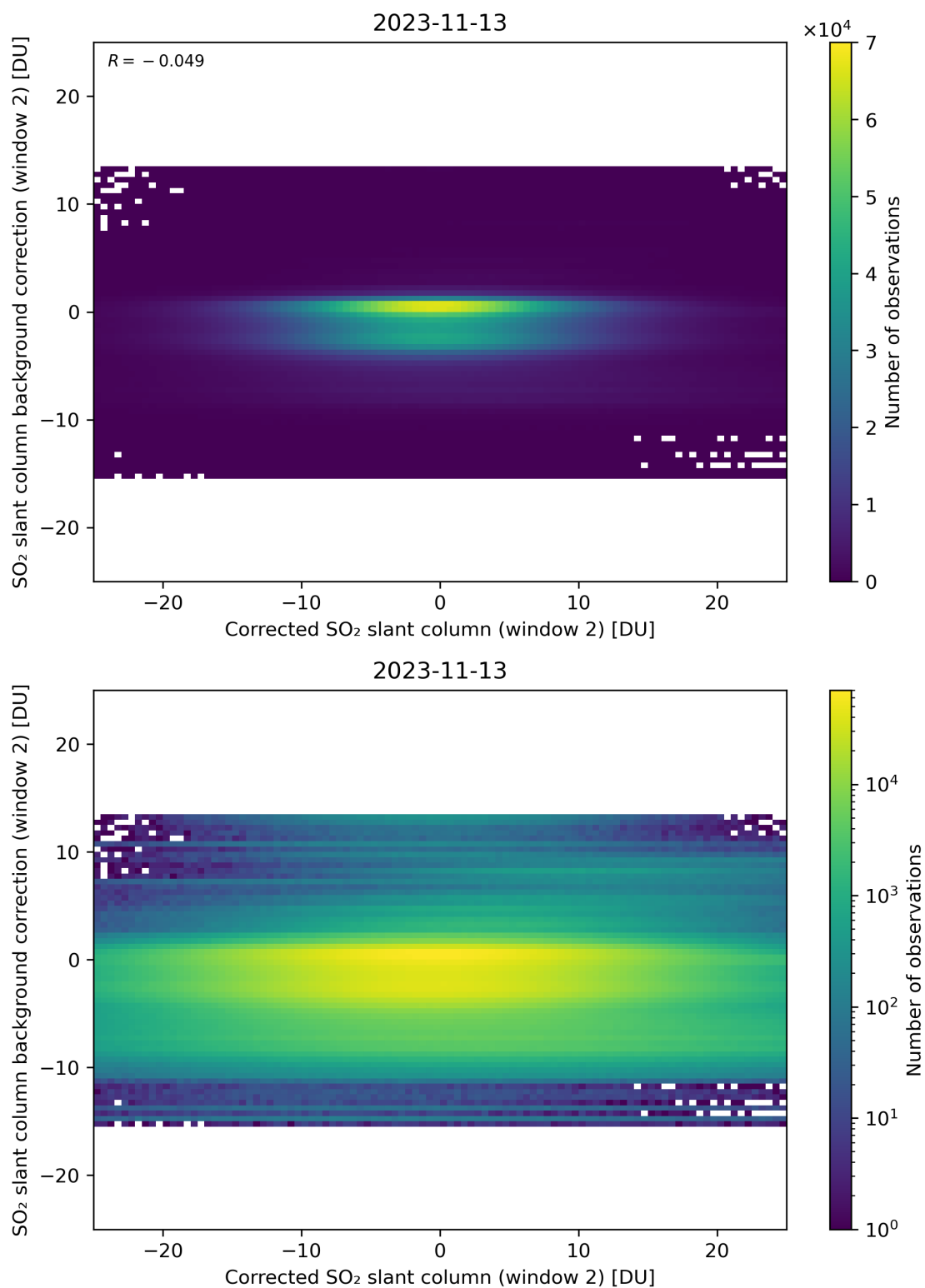
Figure 194: Scatter density plot of “Corrected SO 2 slant column (window 2)” against “SO 2 slant column background correction (window 2)” for 2023-11-13 to 2023-11-14.
