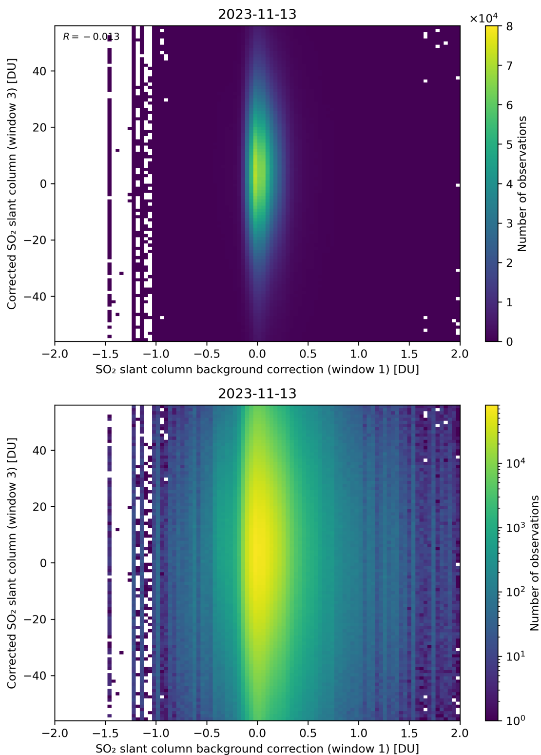
Figure 105: Scatter density plot of “SO 2 slant column background correction (window 1)” against “Corrected SO 2 slant column (window 3)” for 2023-11-13 to 2023-11-14.
