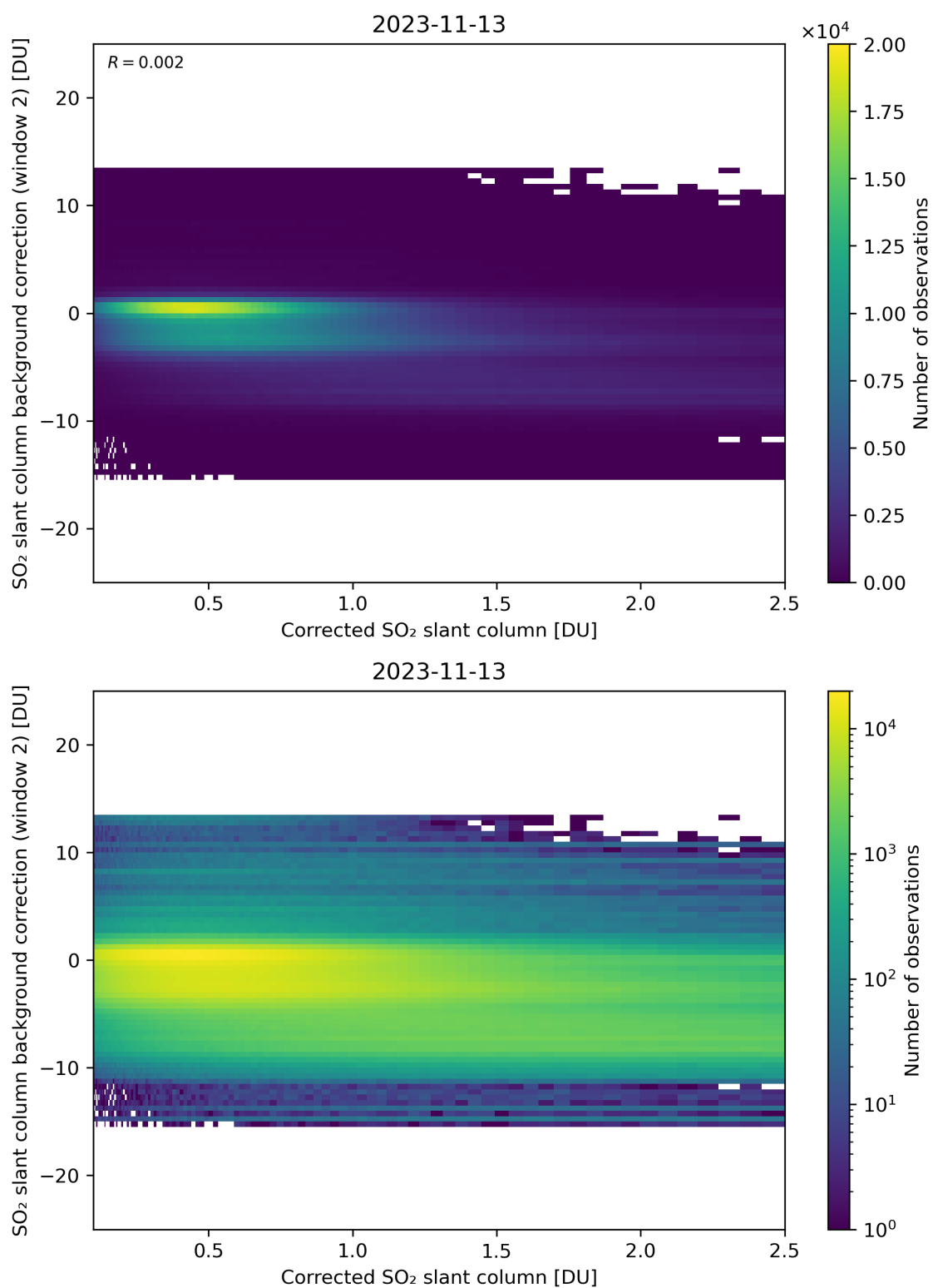
Figure 179: Scatter density plot of “Corrected SO 2 slant column” against “SO 2 slant column background correction (window 2)” for 2023-11-13 to 2023-11-14.
