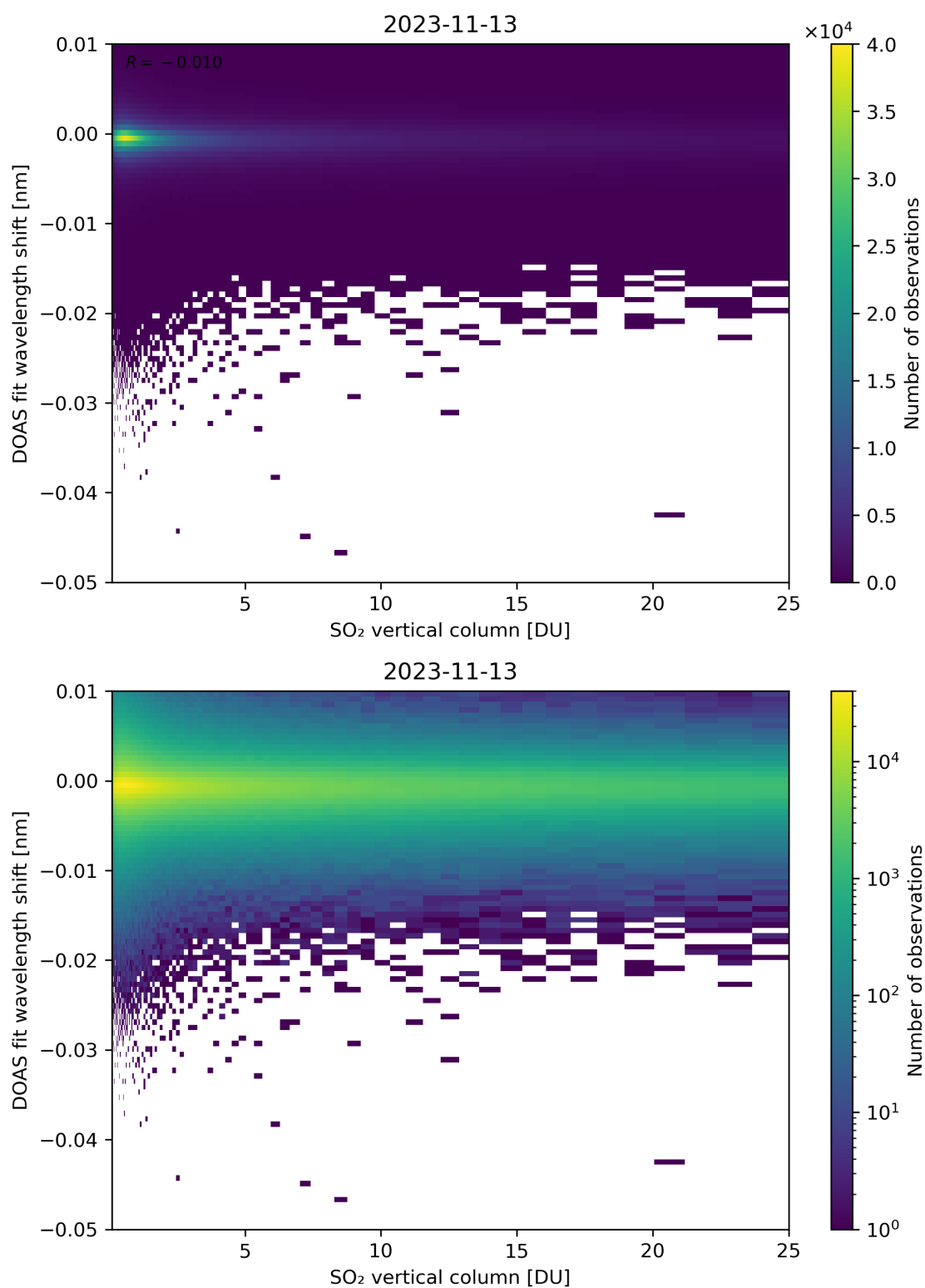
Figure 276: Scatter density plot of “SO 2 vertical column” against “DOAS fit wavelength shift” for 2023-11-13 to 2023-11-14.
