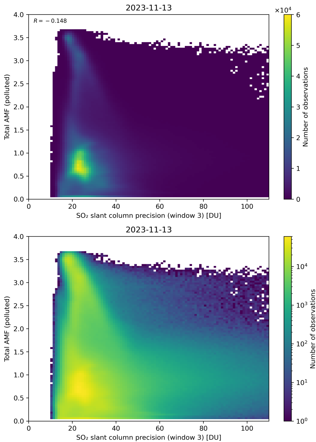
Figure 263: Scatter density plot of “SO 2 slant column precision (window 3)” against “Total AMF (polluted)” for 2023-11-13 to 2023-11-14.
