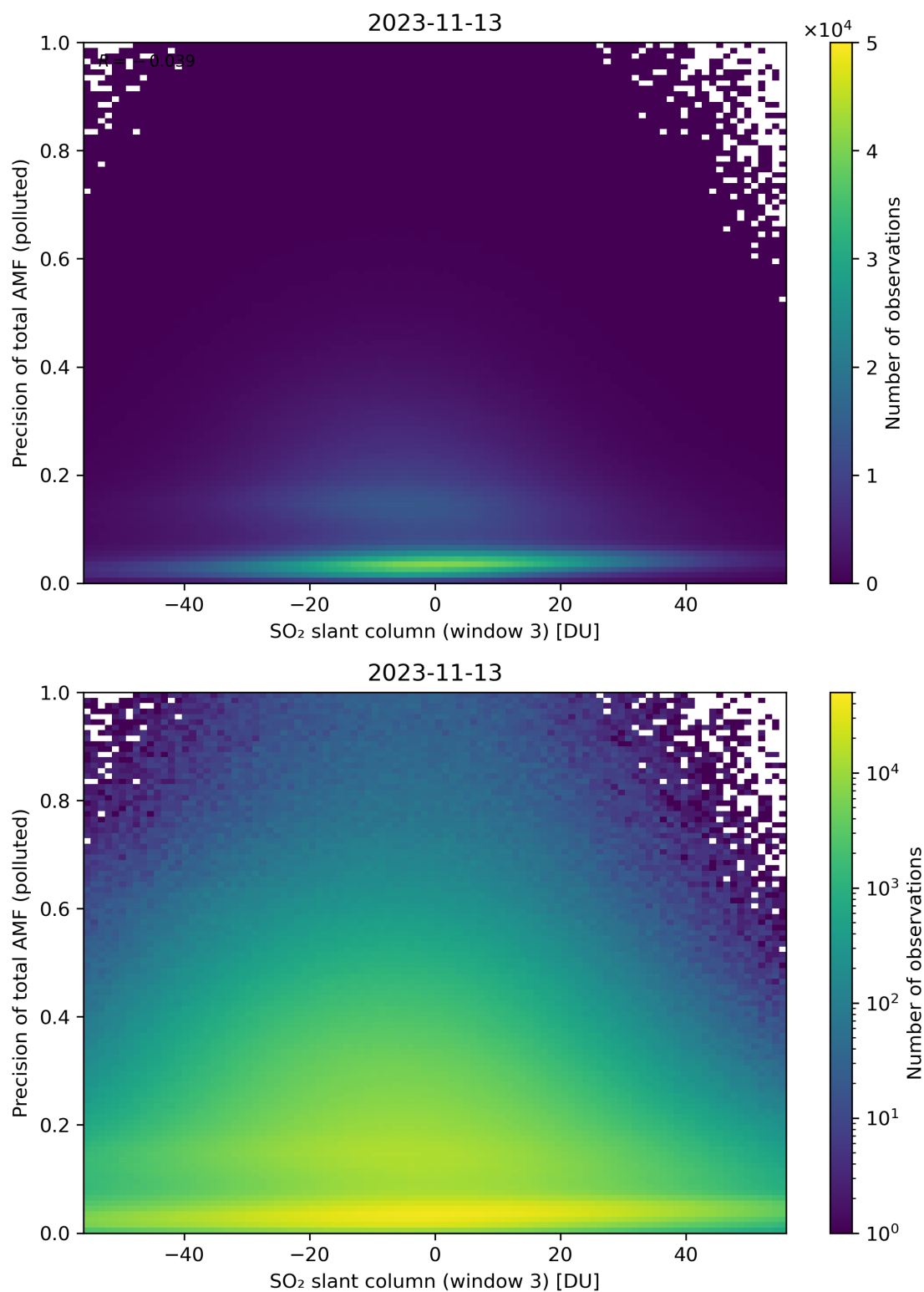
Figure 269: Scatter density plot of “SO 2 slant column (window 3)” against “Precision of total AMF (polluted)” for 2023-11-13 to 2023-11-14.
