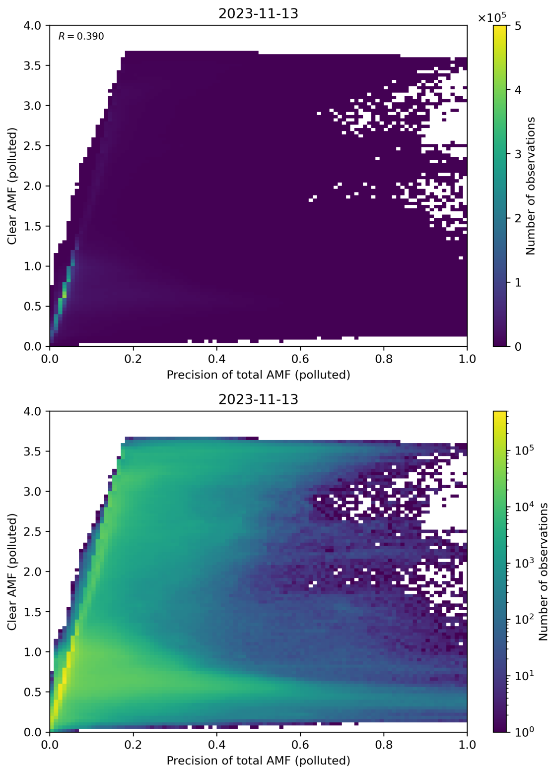
Figure 270: Scatter density plot of “Precision of total AMF (polluted)” against “Clear AMF (polluted)” for 2023-11-13 to 2023-11-14.
