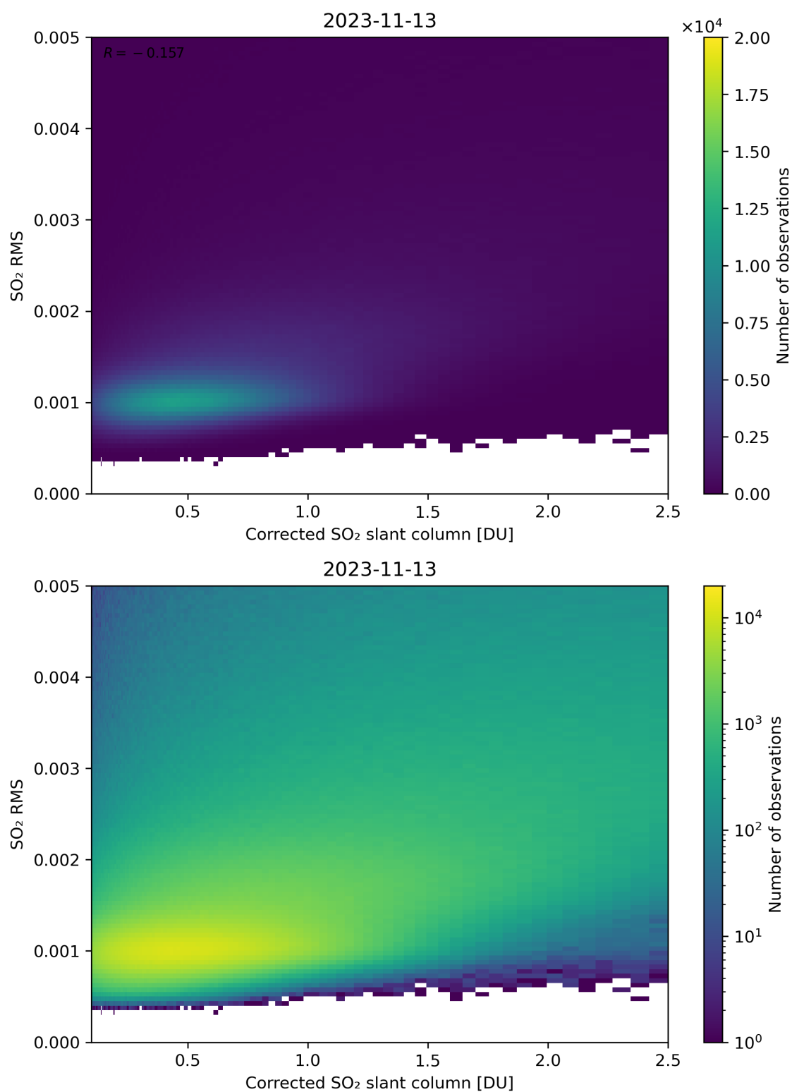
Figure 183: Scatter density plot of “Corrected SO 2 slant column” against “SO 2 RMS” for 2023-11-13 to 2023-11-14.
