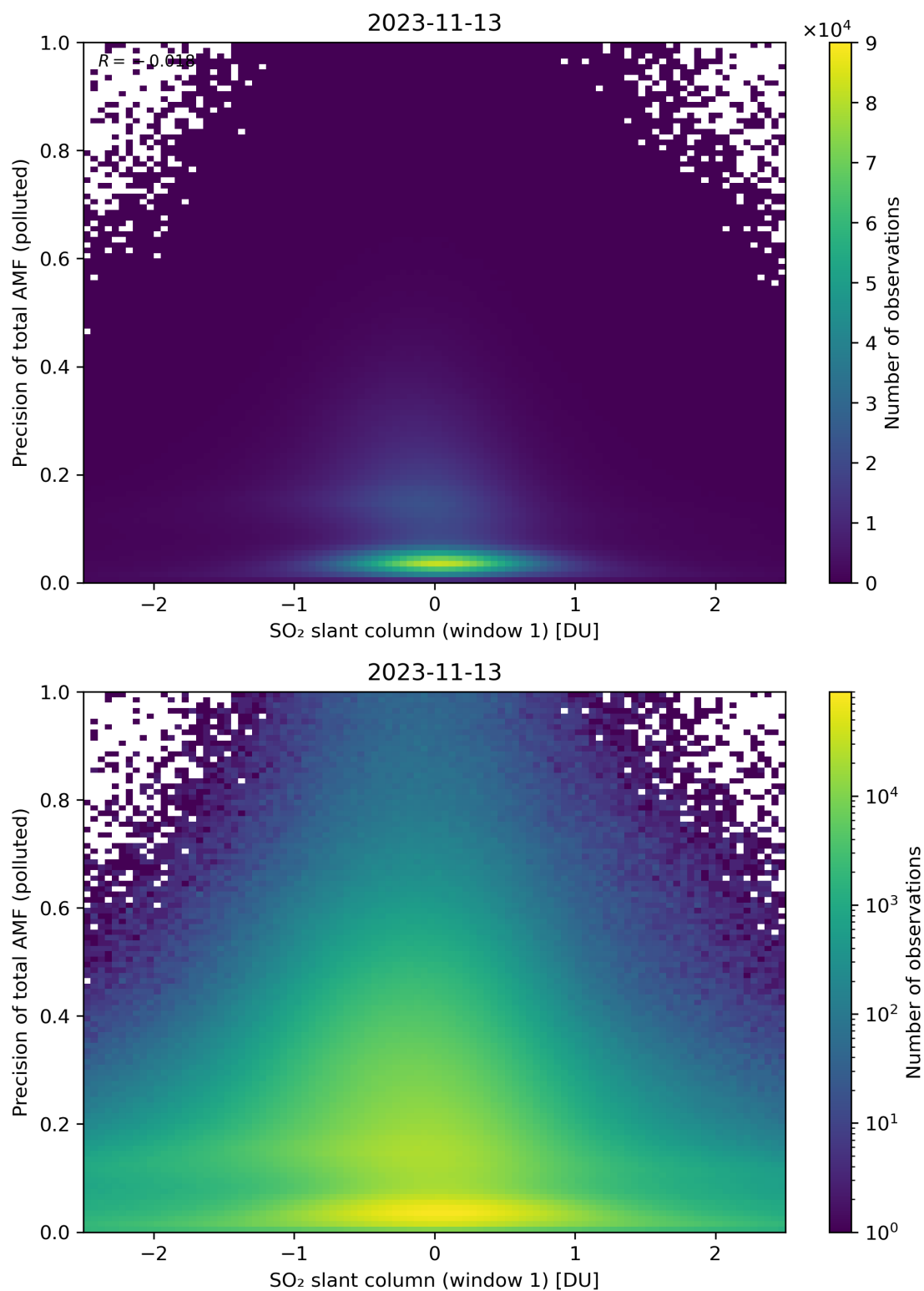
Figure 240: Scatter density plot of “SO 2 slant column (window 1)” against “Precision of total AMF (polluted)” for 2023-11-13 to 2023-11-14.
