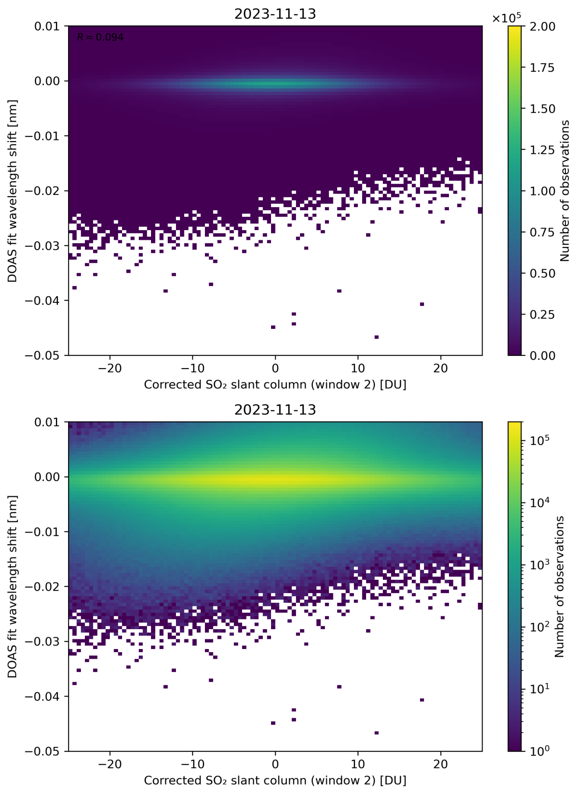
Figure 196: Scatter density plot of “Corrected SO 2 slant column (window 2)” against “DOAS fit wavelength shift” for 2023-11-13 to 2023-11-14.
