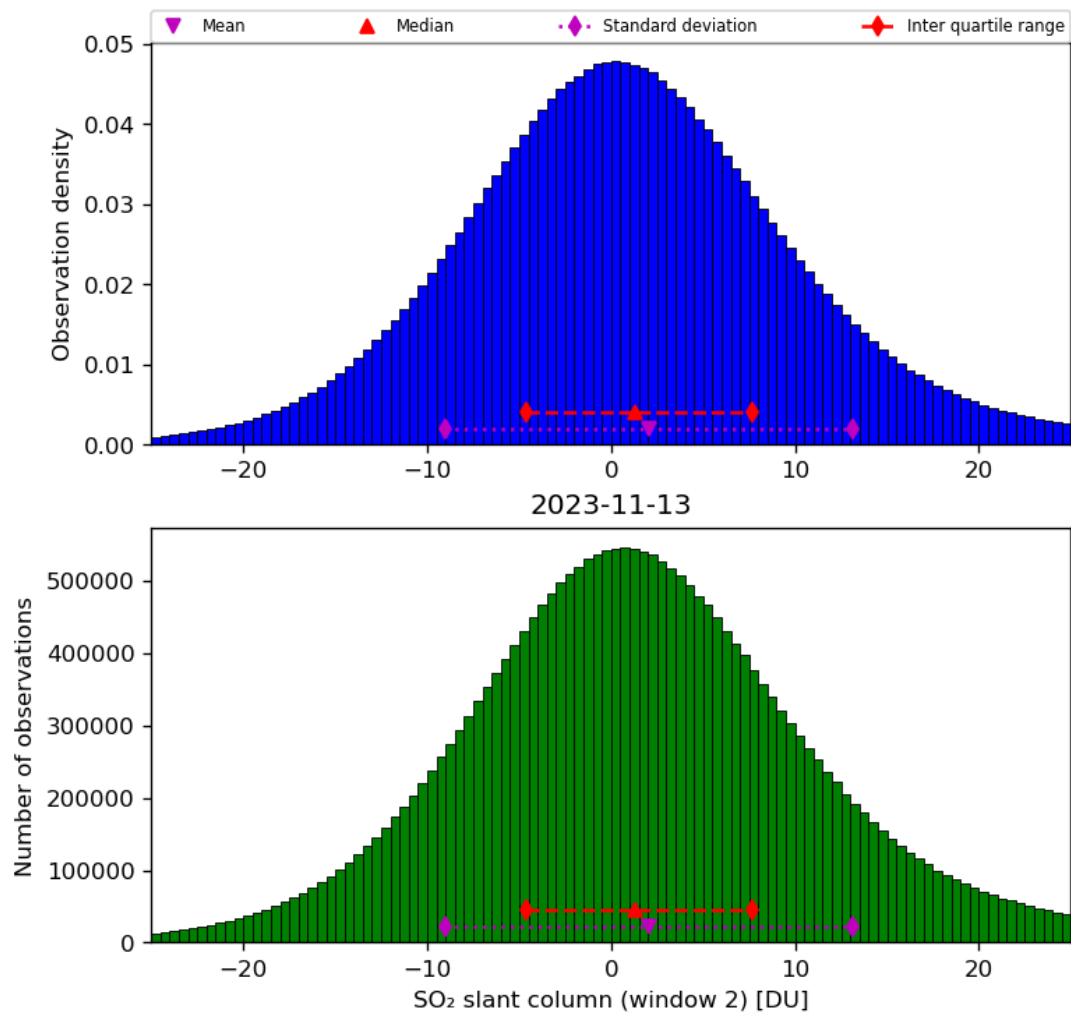
Figure 60: Histogram of “SO 2 slant column (window 2)” for 2023-11-13 to 2023-11-14
