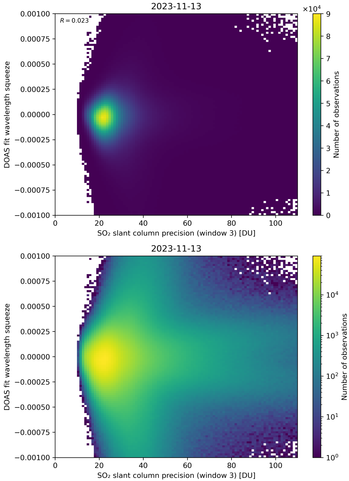
Figure 259: Scatter density plot of “SO 2 slant column precision (window 3)” against “DOAS fit wavelength squeeze” for 2023-11-13 to 2023-11-14.
