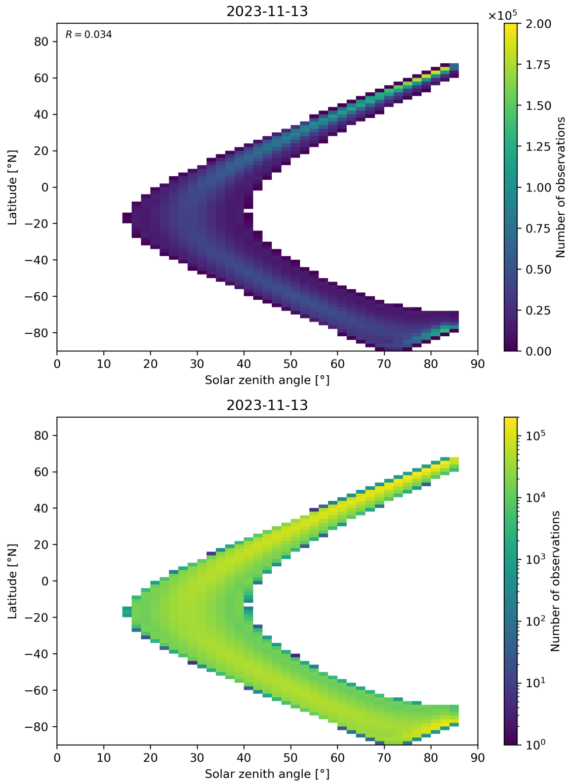
Figure 164: Scatter density plot of “Solar zenith angle” against “Latitude” for 2023-11-13 to 2023-11-14.
