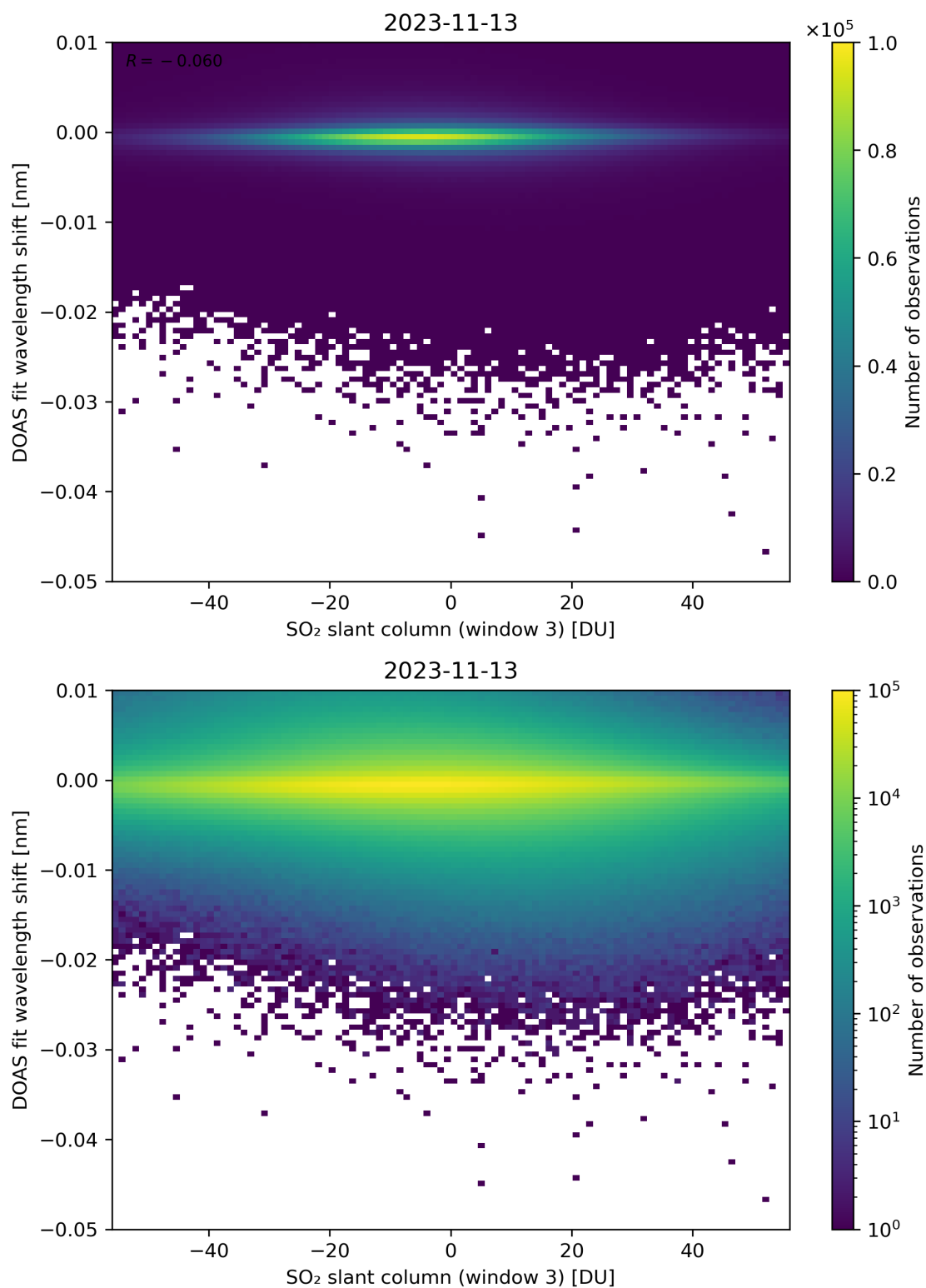
Figure 254: Scatter density plot of “SO 2 slant column (window 3)” against “DOAS fit wavelength shift” for 2023-11-13 to 2023-11-14.
