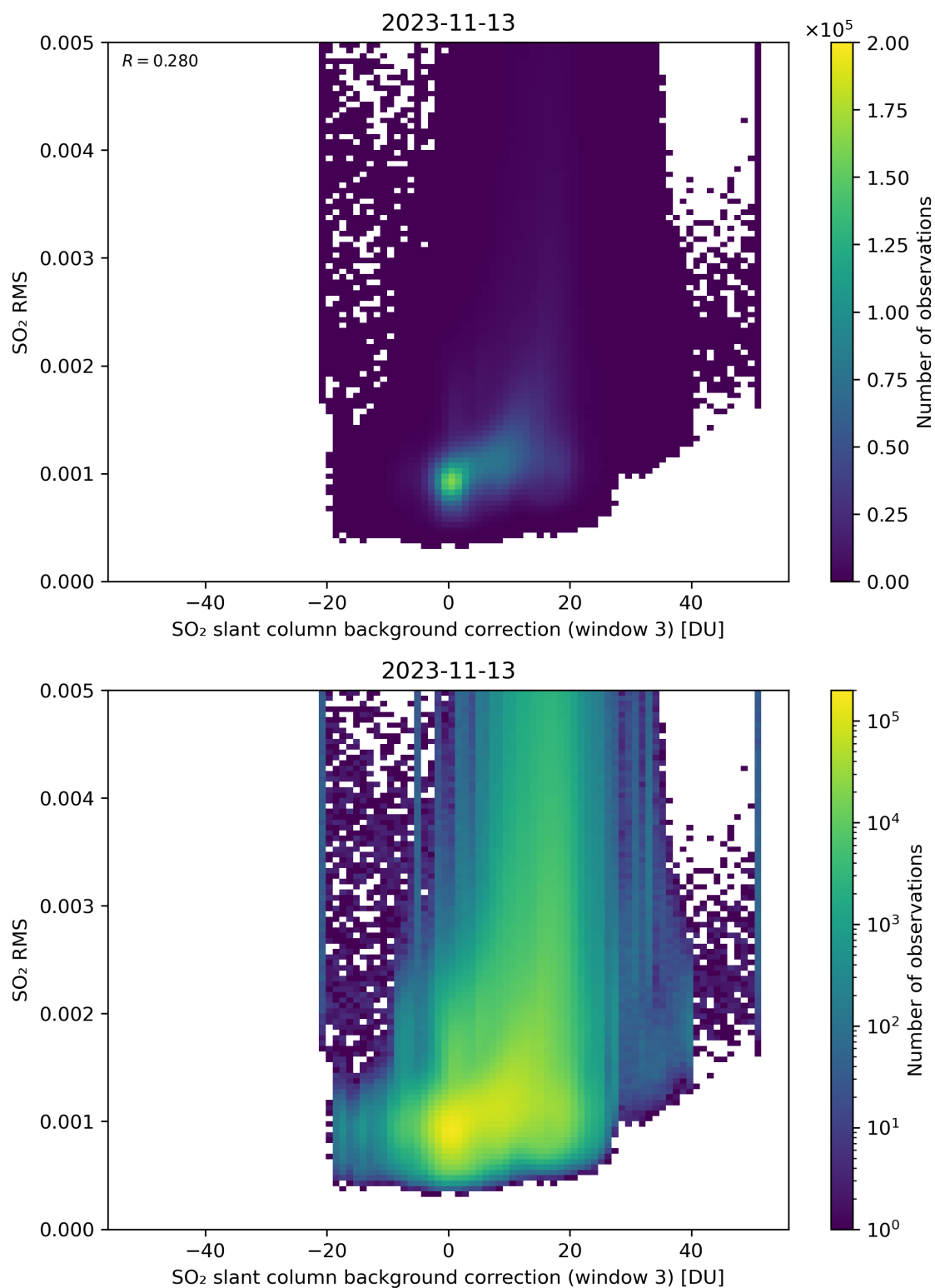
Figure 123: Scatter density plot of “SO 2 slant column background correction (window 3)” against “SO 2 RMS” for 2023-11-13 to 2023-11-14.
