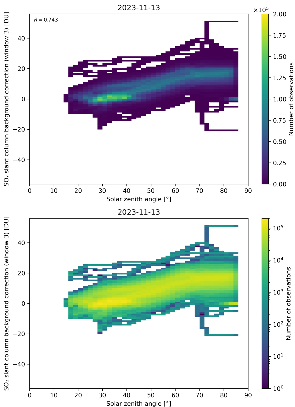
Figure 160: Scatter density plot of “Solar zenith angle” against “SO 2 slant column background correction (window 3)” for 2023-11-13 to 2023-11-14.
