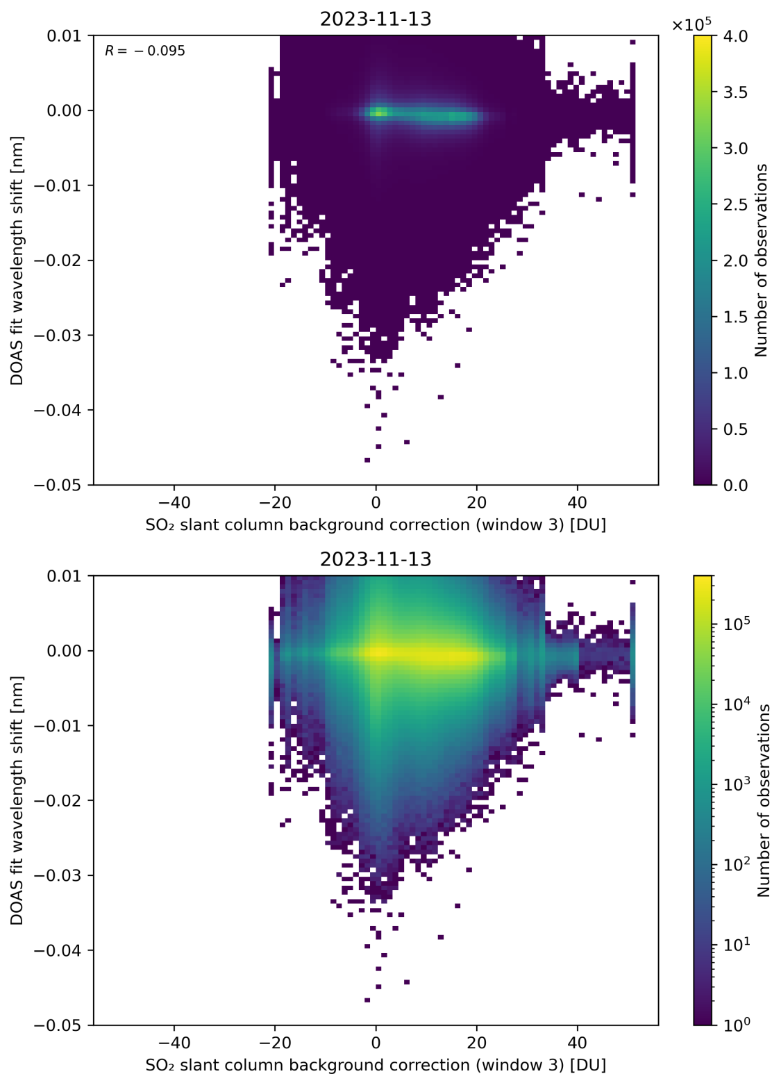
Figure 121: Scatter density plot of “SO 2 slant column background correction (window 3)” against “DOAS fit wavelength shift” for 2023-11-13 to 2023-11-14.
