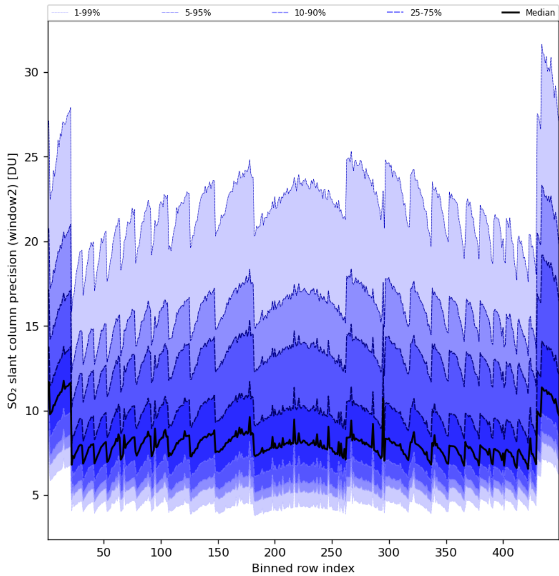
Figure 84: Along track statistics of “SO 2 slant column precision (window2)” for 2023-11-13 to 2023-11-14
