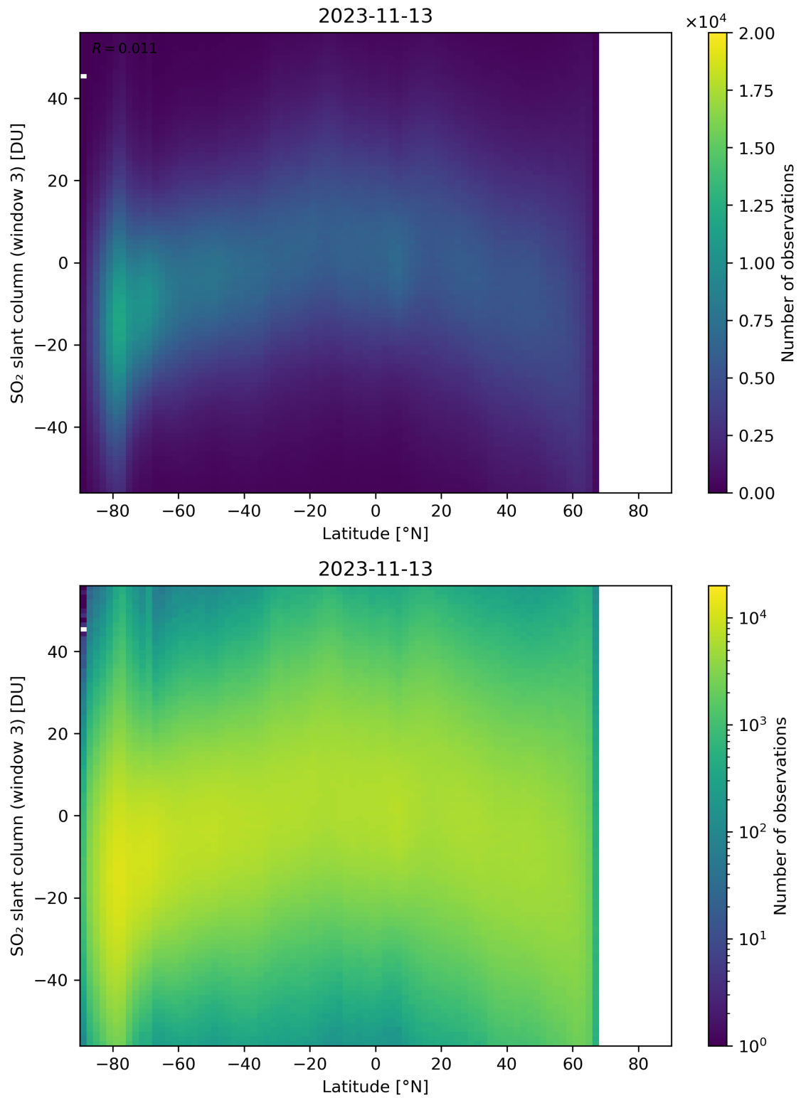
Figure 152: Scatter density plot of “Latitude” against “SO 2 slant column (window 3)” for 2023-11-13 to 2023-11-14.
