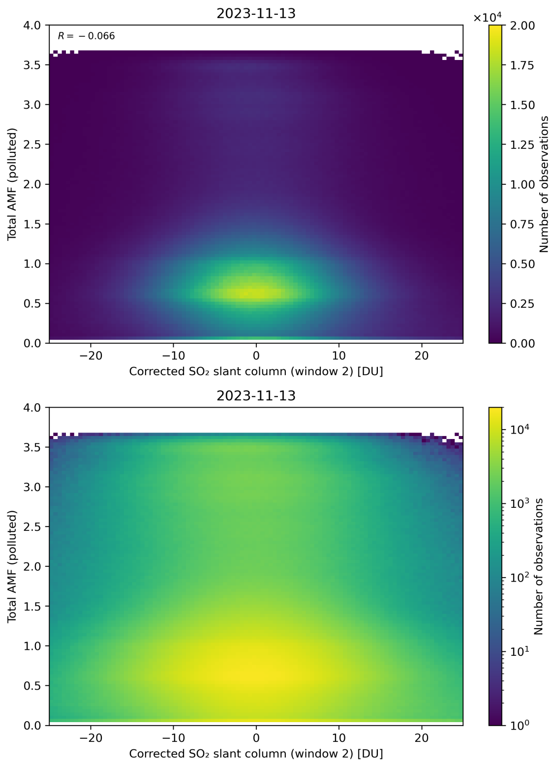
Figure 203: Scatter density plot of “Corrected SO 2 slant column (window 2)” against “Total AMF (polluted)” for 2023-11-13 to 2023-11-14.
