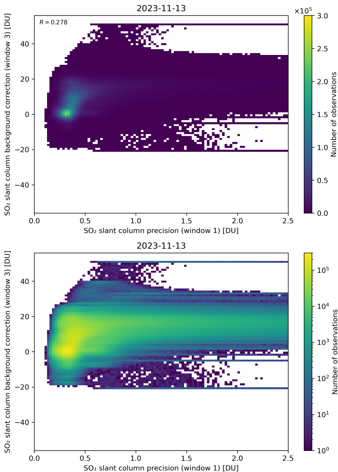
Figure 220: Scatter density plot of “SO 2 slant column precision (window 1)” against “SO 2 slant column background correction (window 3)” for 2023-11-13 to 2023-11-14.
