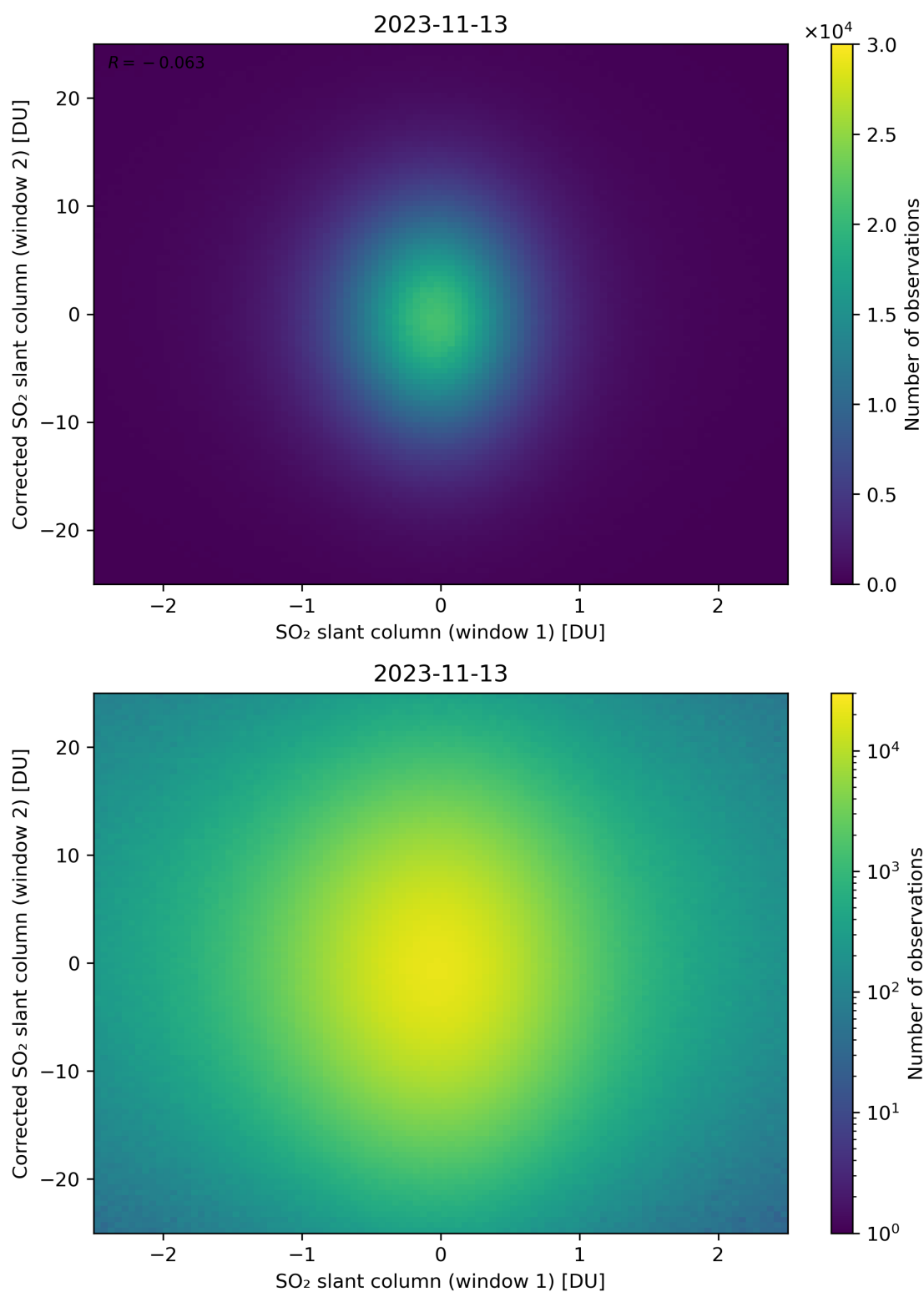
Figure 233: Scatter density plot of “SO 2 slant column (window 1)” against “Corrected SO 2 slant column (window 2)” for 2023-11-13 to 2023-11-14.
