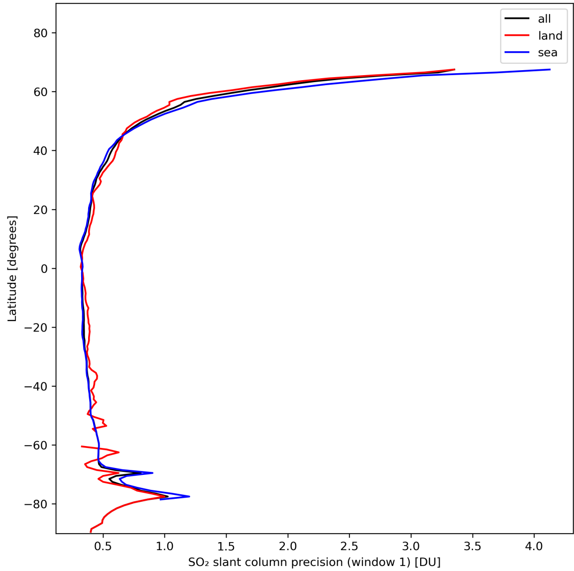
Figure 34: Zonal average of “SO 2 slant column precision (window 1)” for 2023-11-13 to 2023-11-14.
