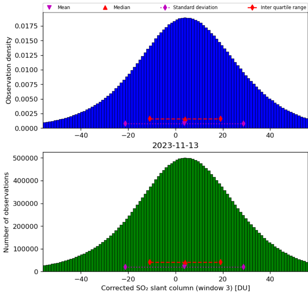
Figure 66: Histogram of “Corrected SO 2 slant column (window 3)” for 2023-11-13 to 2023-11-14
