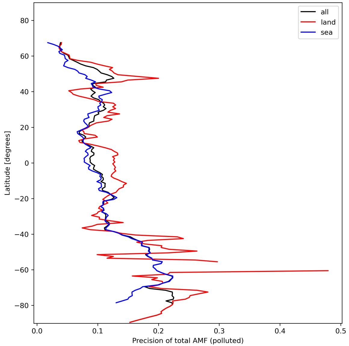
Figure 49: Zonal average of “Precision of total AMF (polluted)” for 2023-11-13 to 2023-11-14.
