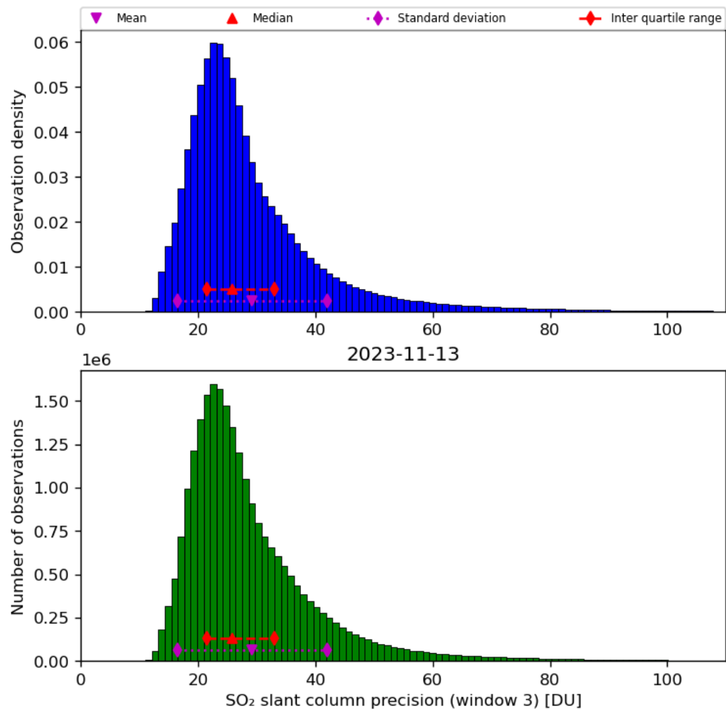
Figure 65: Histogram of “SO 2 slant column precision (window 3)” for 2023-11-13 to 2023-11-14
