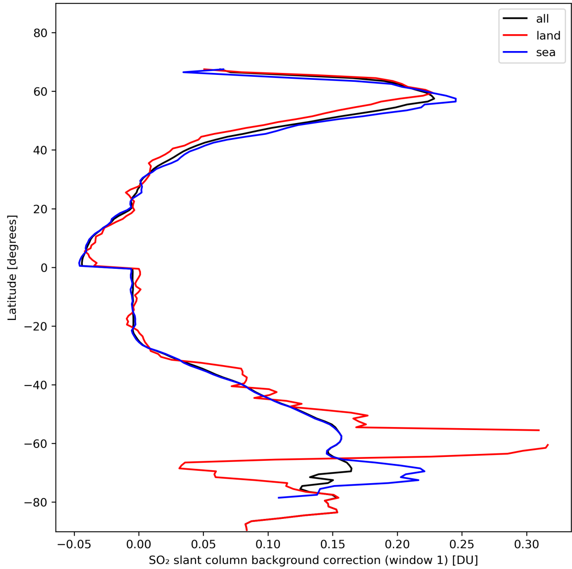
Figure 36: Zonal average of “SO 2 slant column background correction (window 1)” for 2023-11-13 to 2023-11-14.
