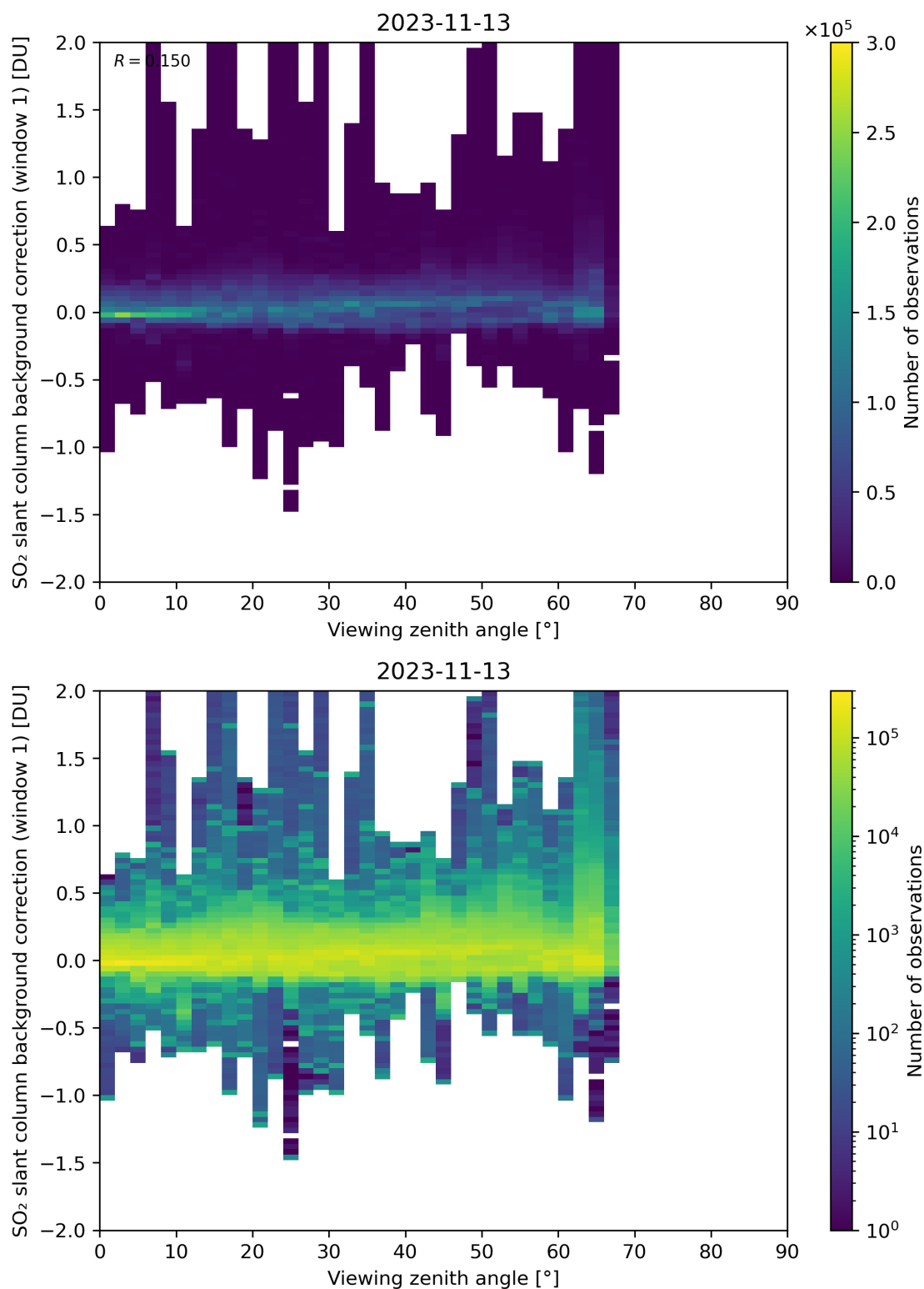
Figure 308: Scatter density plot of “Viewing zenith angle” against “SO 2 slant column background correction (window 1)” for 2023-11-13 to 2023-11-14.
