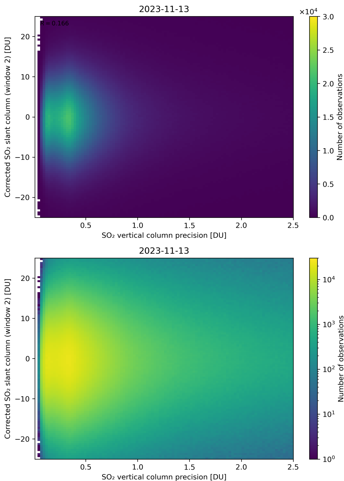
Figure 287: Scatter density plot of “SO 2 vertical column precision” against “Corrected SO 2 slant column (window 2)” for 2023-11-13 to 2023-11-14.
