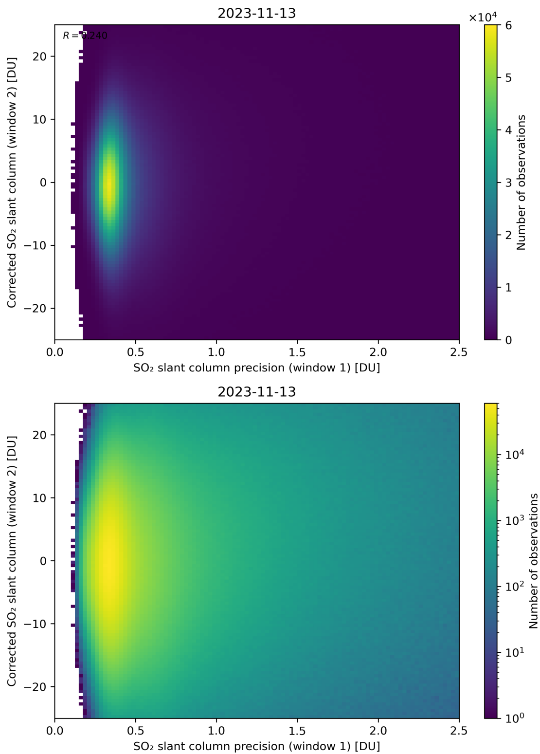
Figure 225: Scatter density plot of “SO 2 slant column precision (window 1)” against “Corrected SO 2 slant column (window 2)” for 2023-11-13 to 2023-11-14.
