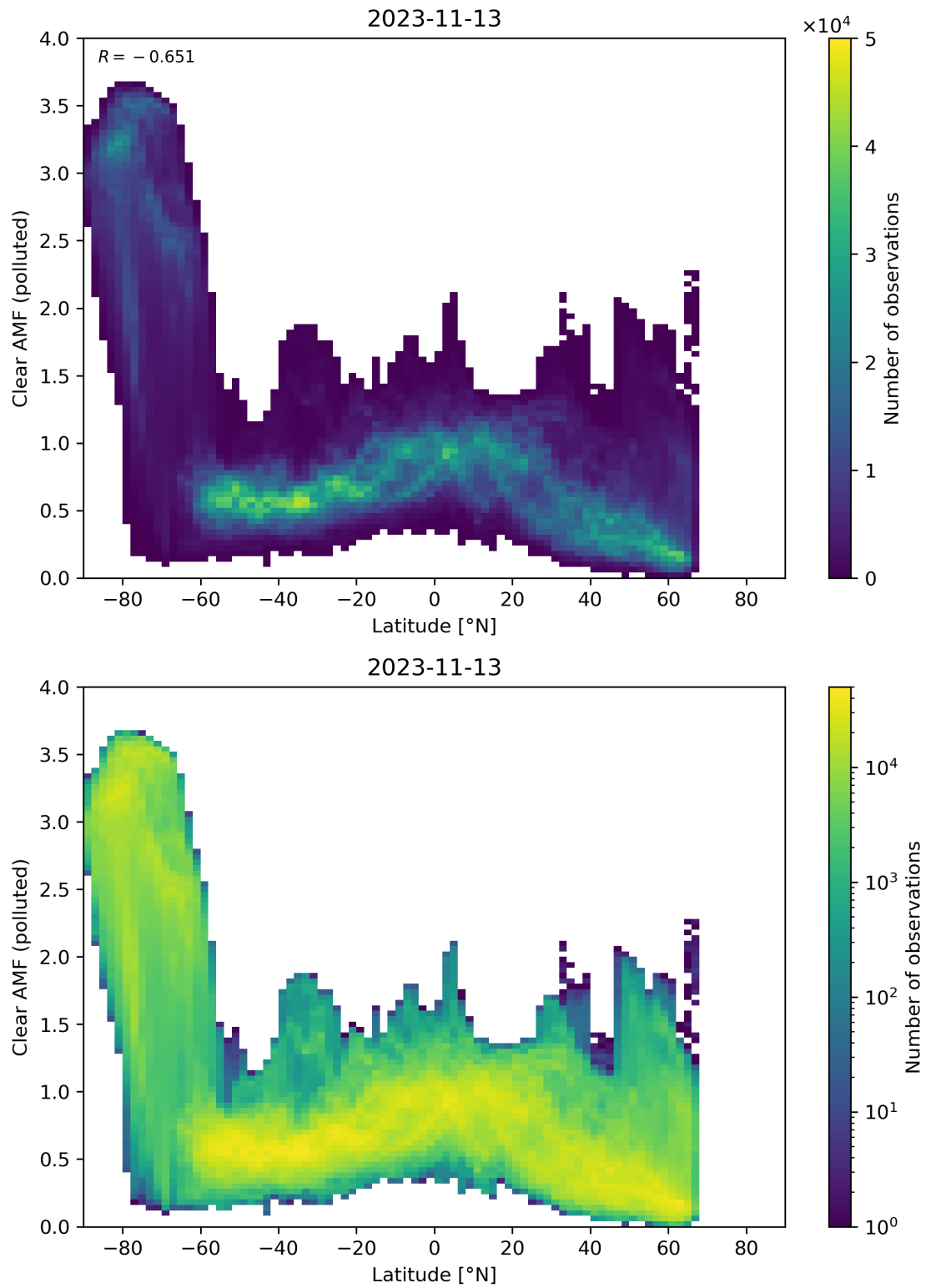
Figure 145: Scatter density plot of “Latitude” against “Clear AMF (polluted)” for 2023-11-13 to 2023-11-14.
