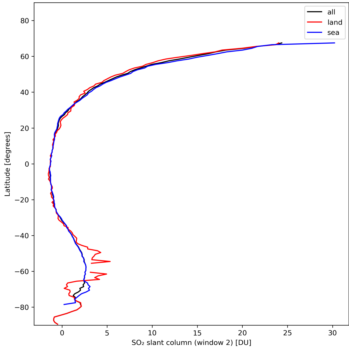
Figure 37: Zonal average of “SO 2 slant column (window 2)” for 2023-11-13 to 2023-11-14.
