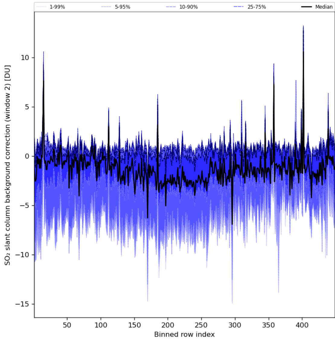
Figure 86: Along track statistics of “SO 2 slant column background correction (window 2)” for 2023-11-13 to 2023-11-14
