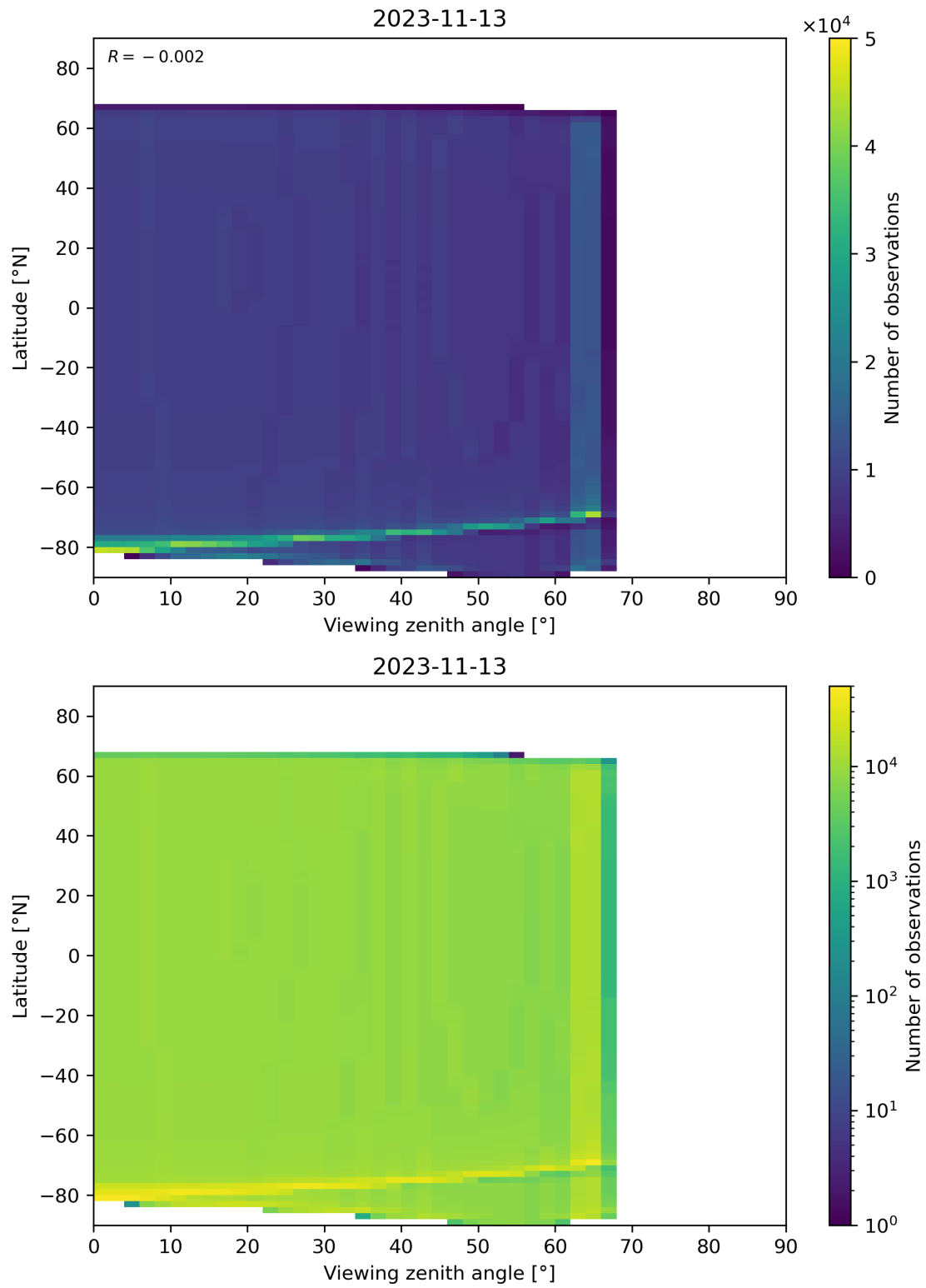
Figure 314: Scatter density plot of “Viewing zenith angle” against “Latitude” for 2023-11-13 to 2023-11-14.
