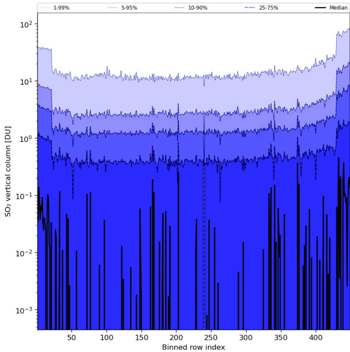
Figure 76: Along track statistics of “SO 2 vertical column” for 2023-11-13 to 2023-11-14
