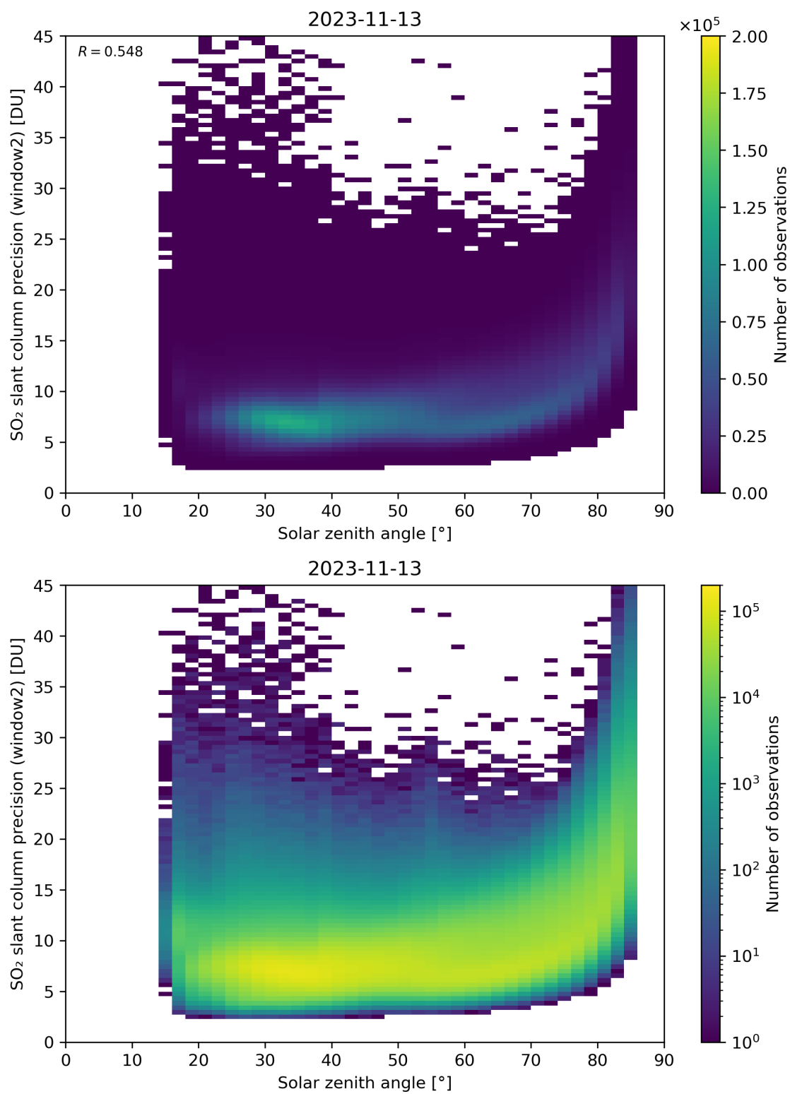
Figure 171: Scatter density plot of “Solar zenith angle” against “SO 2 slant column precision (window2)” for 2023-11-13 to 2023-11-14.
