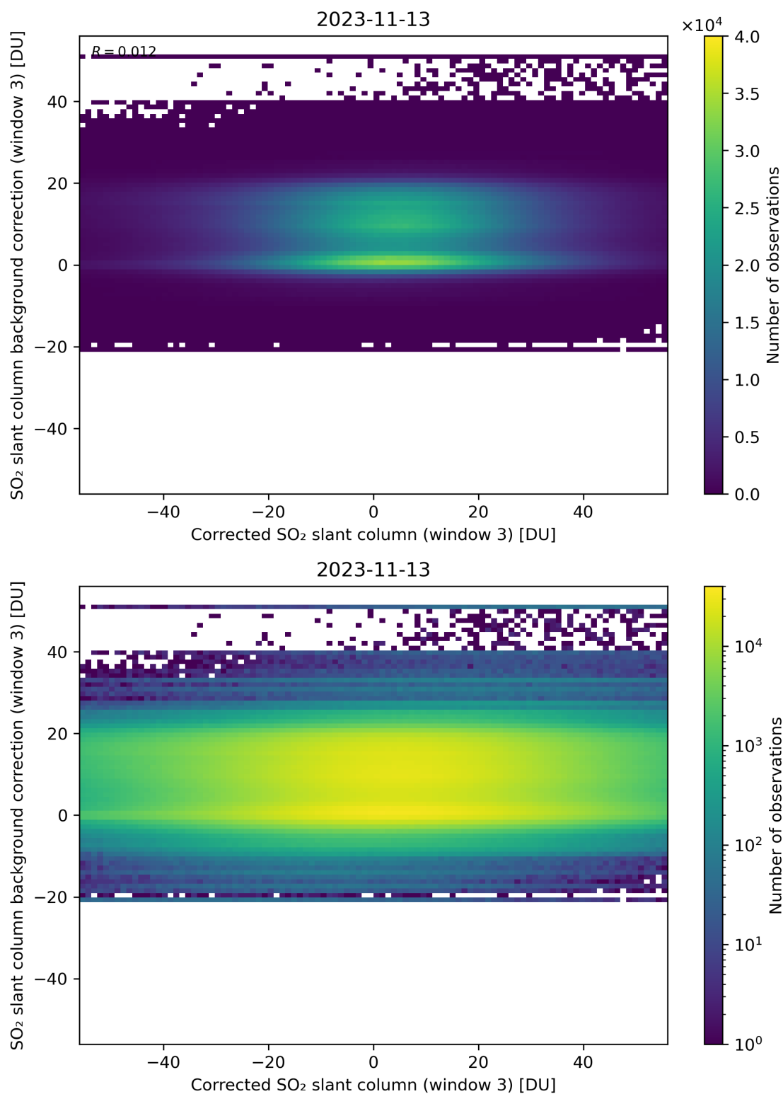
Figure 205: Scatter density plot of “Corrected SO 2 slant column (window 3)” against “SO 2 slant column background correction (window 3)” for 2023-11-13 to 2023-11-14.
