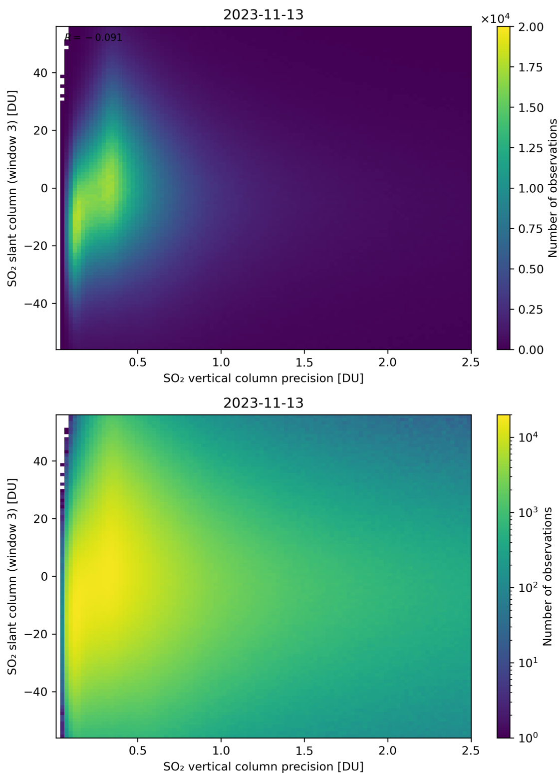
Figure 292: Scatter density plot of “SO 2 vertical column precision” against “SO 2 slant column (window 3)” for 2023-11-13 to 2023-11-14.
