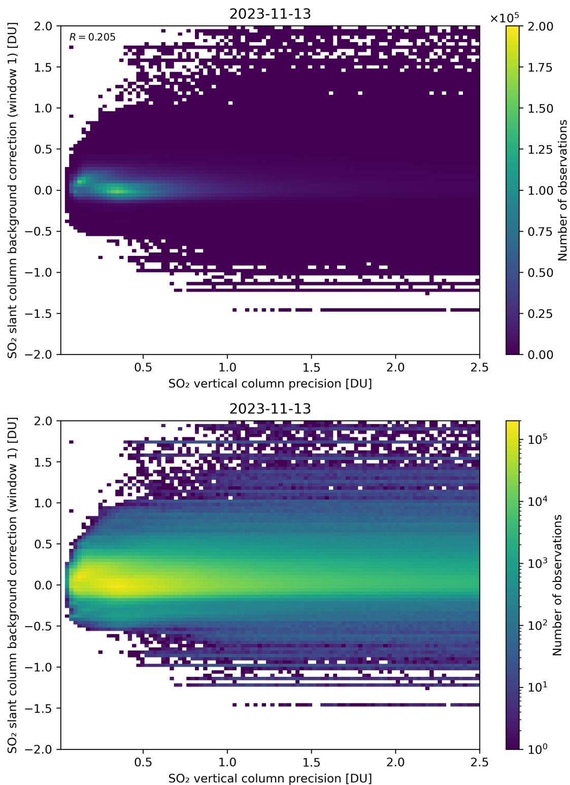
Figure 279: Scatter density plot of “SO 2 vertical column precision” against “SO 2 slant column background correction (window 1)” for 2023-11-13 to 2023-11-14.
