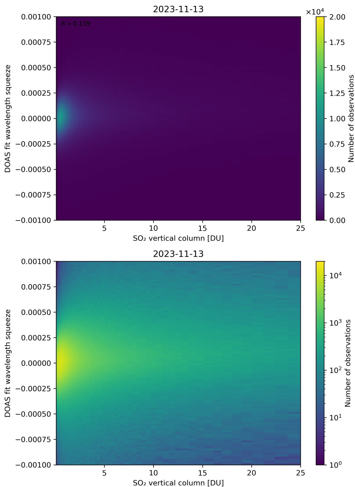
Figure 277: Scatter density plot of “SO 2 vertical column” against “DOAS fit wavelength squeeze” for 2023-11-13 to 2023-11-14.
