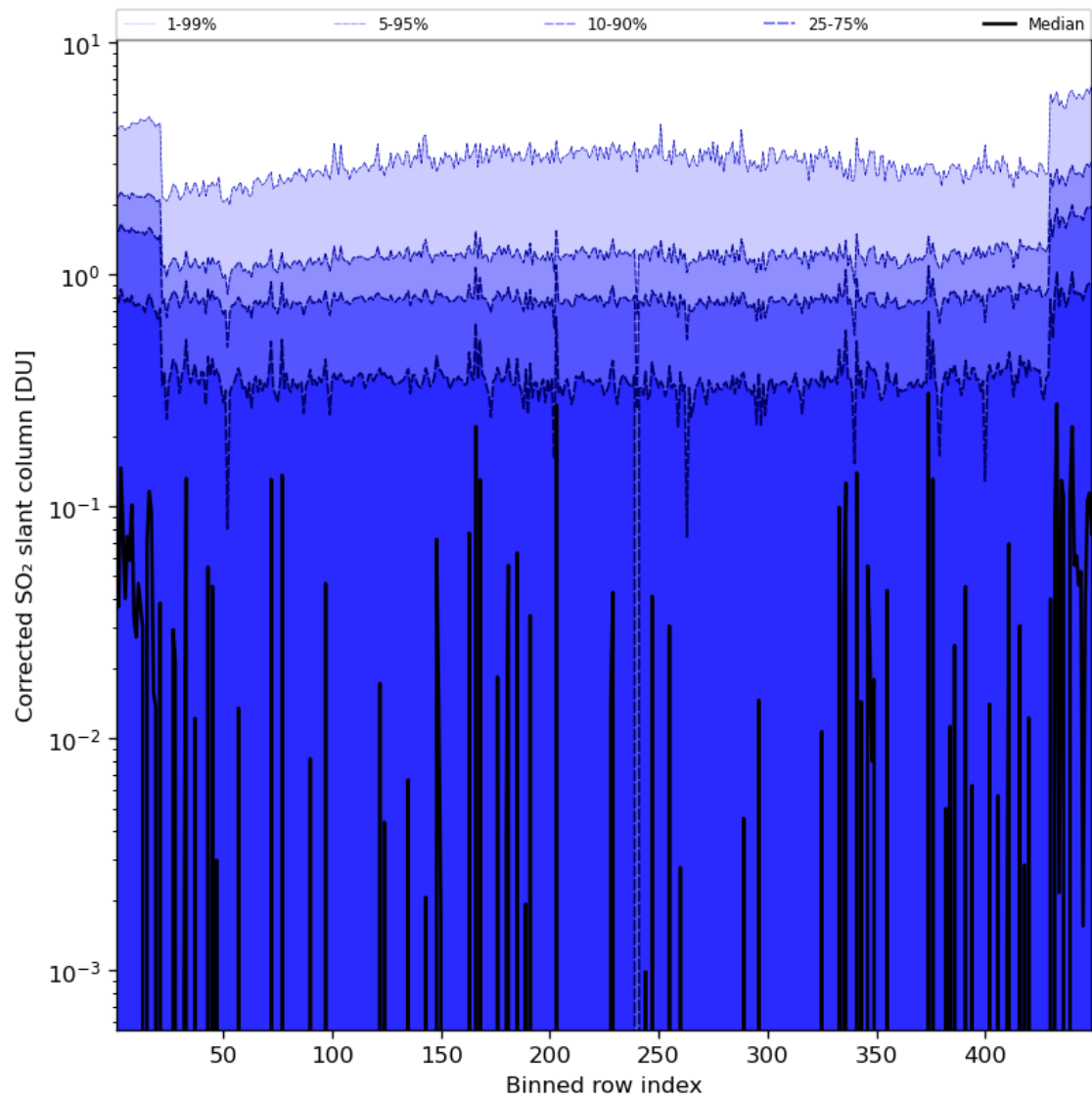
Figure 78: Along track statistics of “Corrected SO 2 slant column” for 2023-11-13 to 2023-11-14
