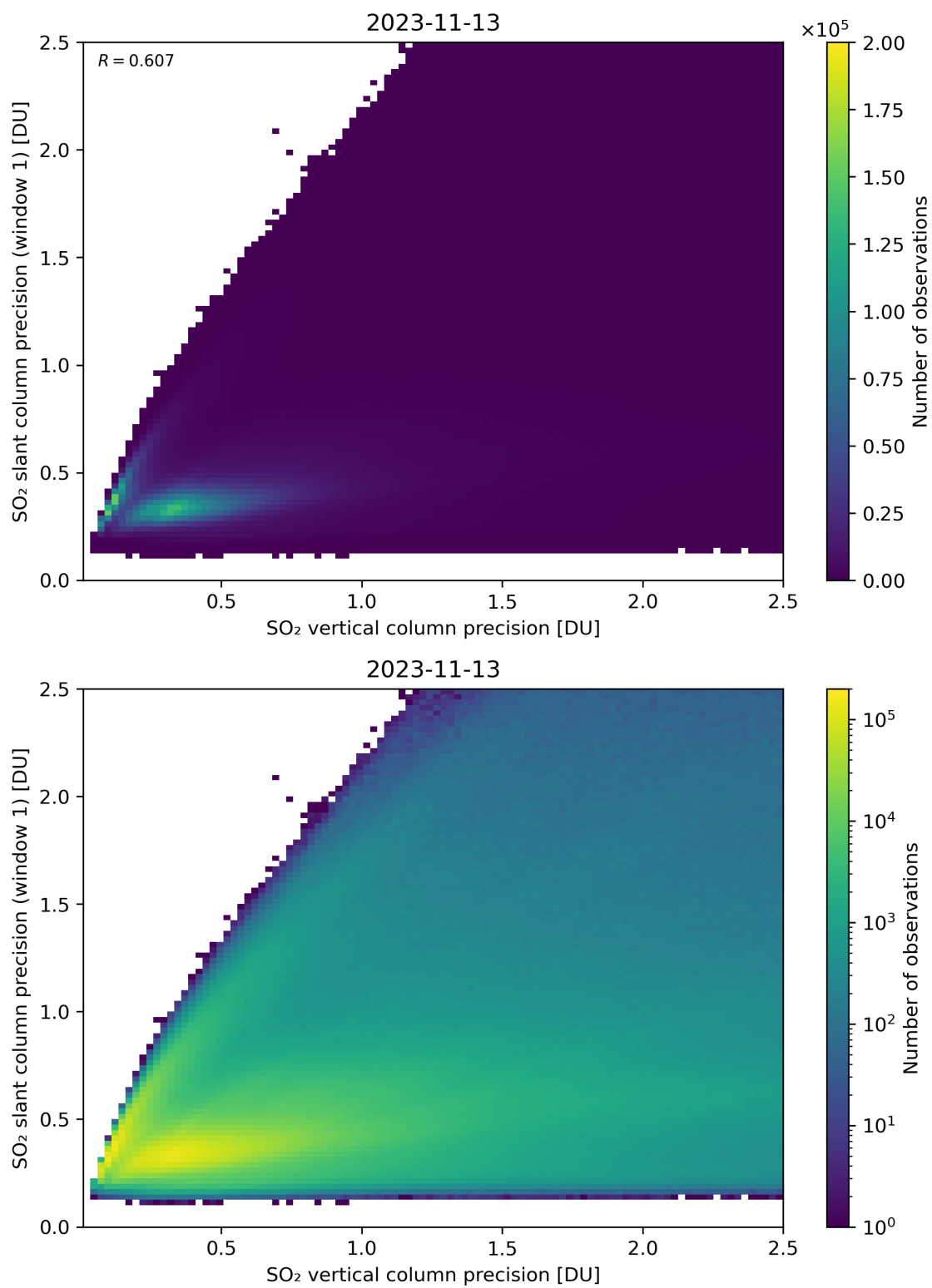
Figure 290: Scatter density plot of “SO 2 vertical column precision” against “SO 2 slant column precision (window 1)” for 2023-11-13 to 2023-11-14.
