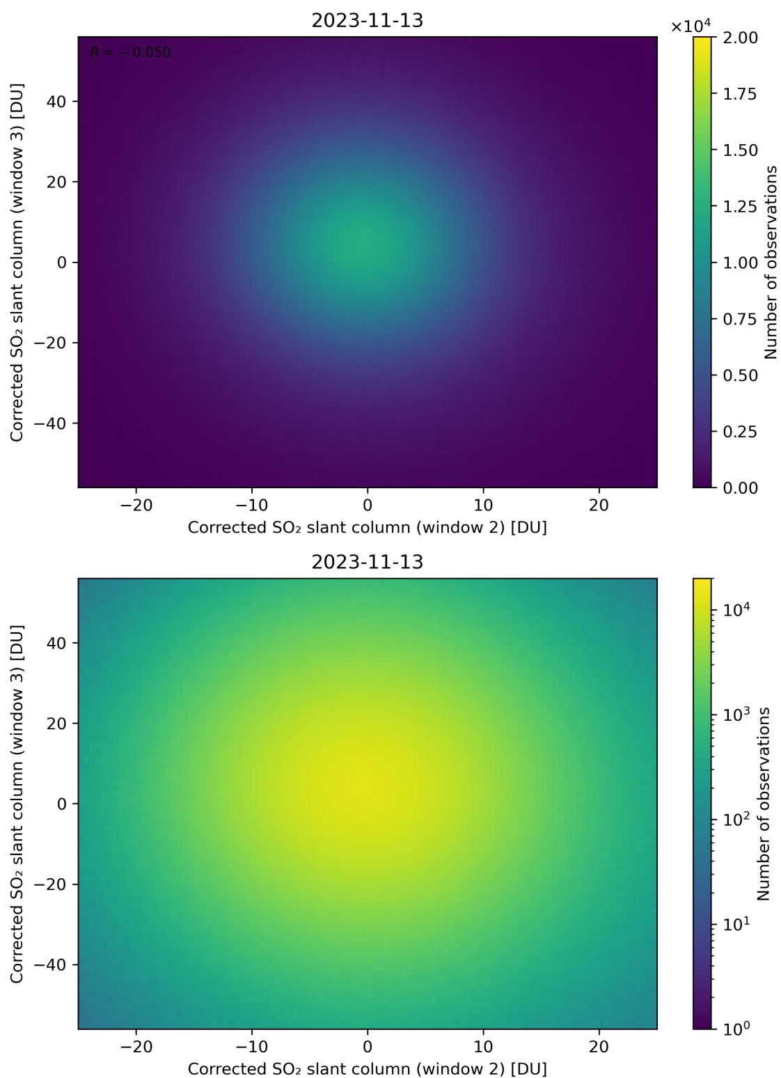
Figure 200: Scatter density plot of “Corrected SO 2 slant column (window 2)” against “Corrected SO 2 slant column (window 3)” for 2023-11-13 to 2023-11-14.
