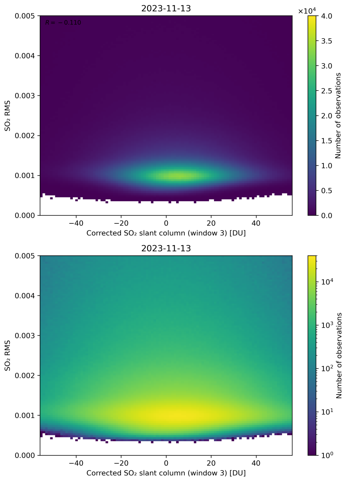
Figure 208: Scatter density plot of “Corrected SO 2 slant column (window 3)” against “SO 2 RMS” for 2023-11-13 to 2023-11-14.
