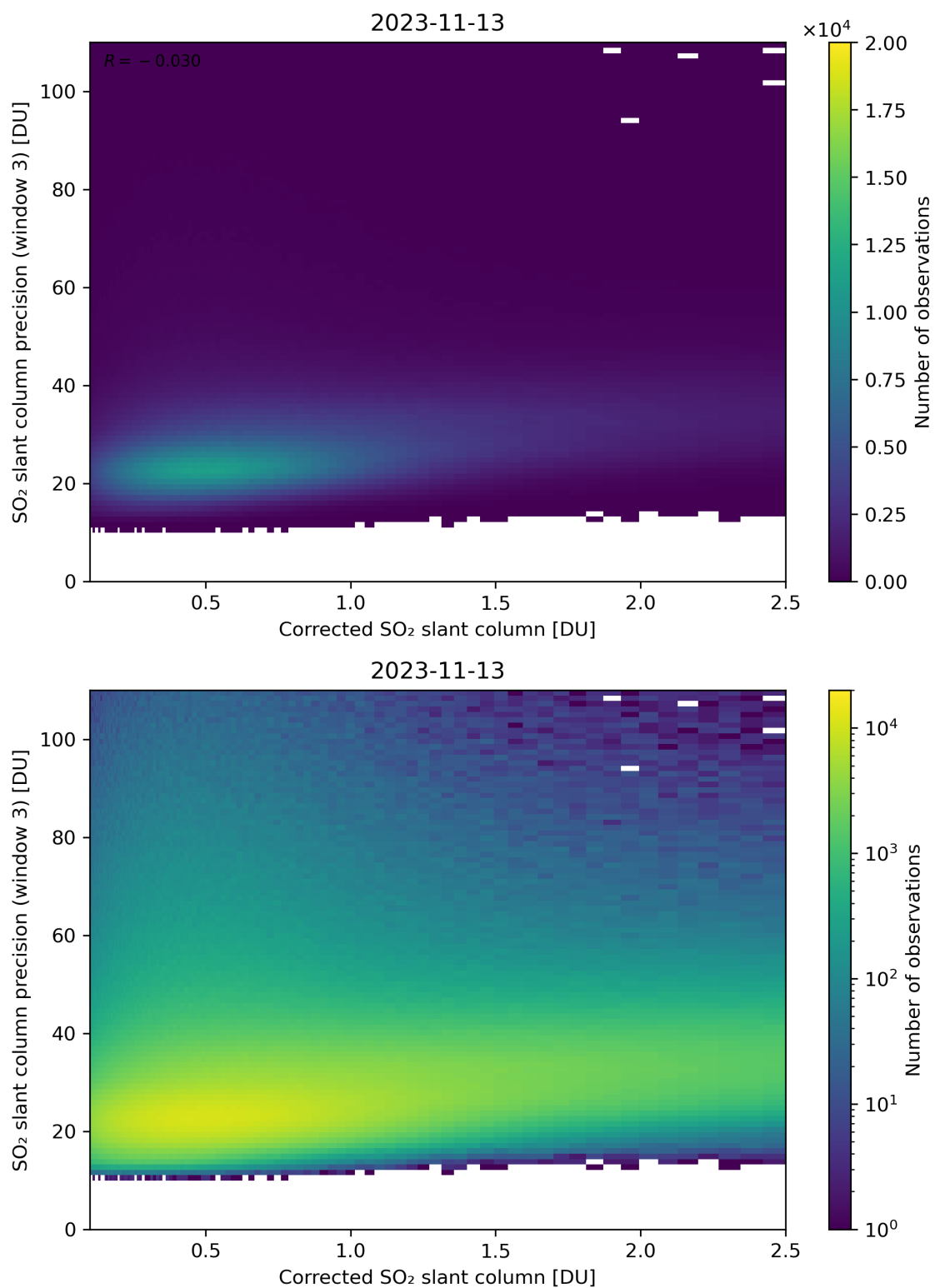
Figure 191: Scatter density plot of “Corrected SO 2 slant column” against “SO 2 slant column precision (window 3)” for 2023-11-13 to 2023-11-14.
