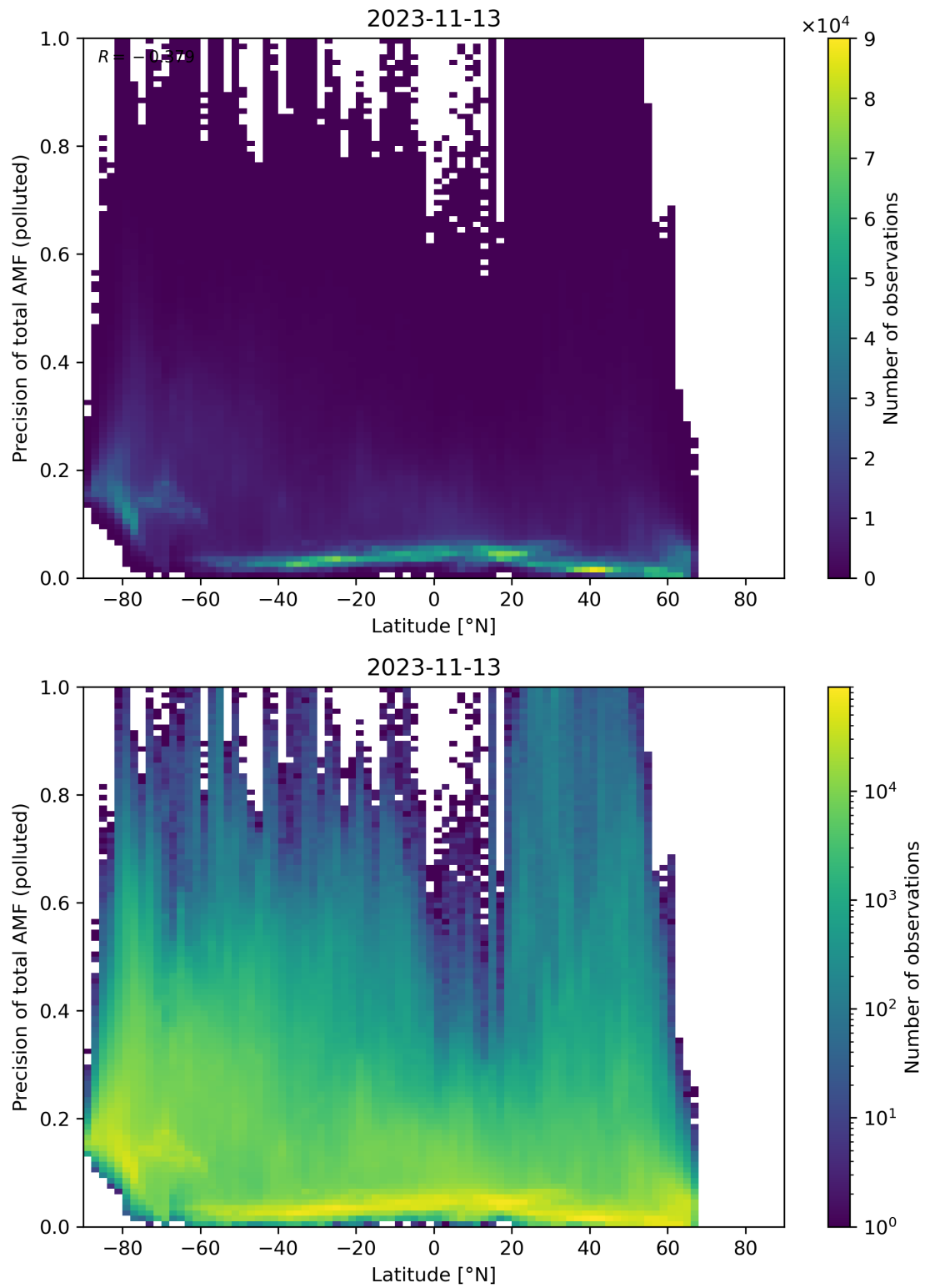
Figure 155: Scatter density plot of “Latitude” against “Precision of total AMF (polluted)” for 2023-11-13 to 2023-11-14.
