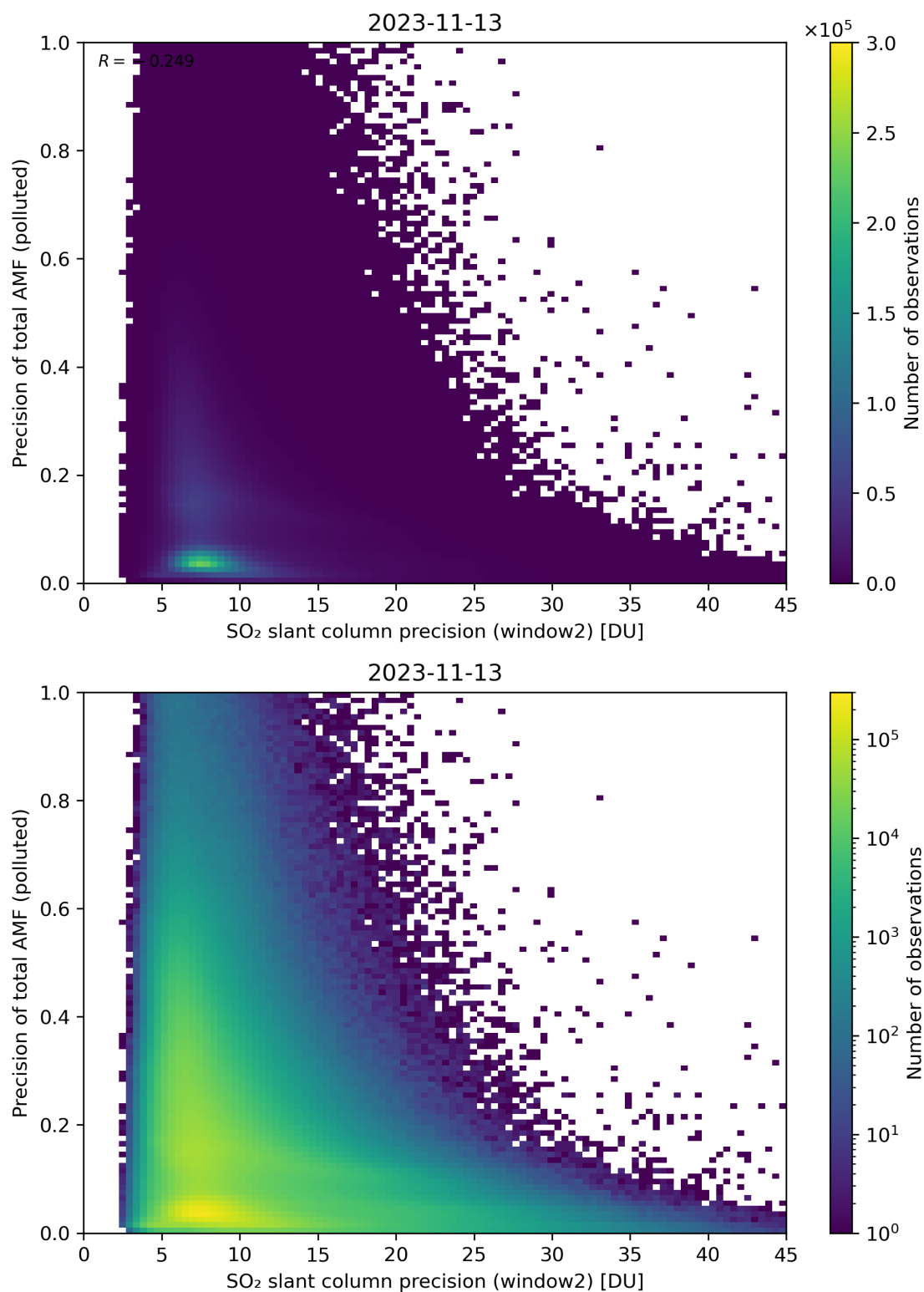
Figure 252: Scatter density plot of “SO 2 slant column precision (window2)” against “Precision of total AMF (polluted)” for 2023-11-13 to 2023-11-14.
