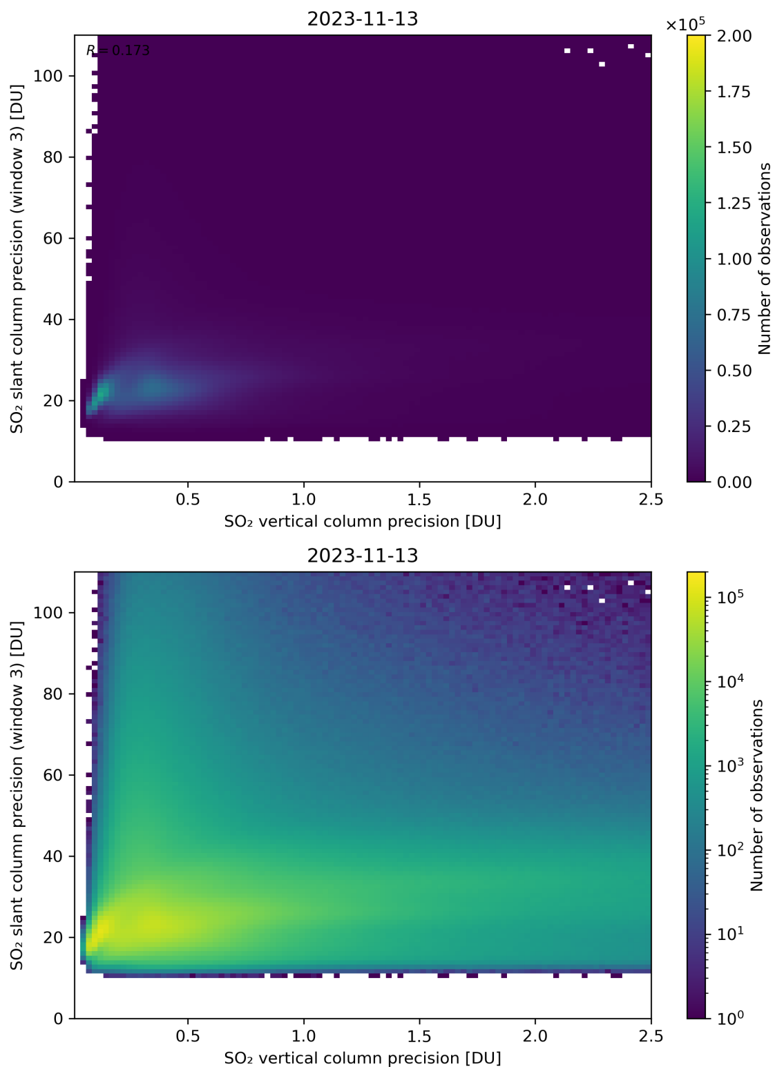
Figure 293: Scatter density plot of “SO 2 vertical column precision” against “SO 2 slant column precision (window 3)” for 2023-11-13 to 2023-11-14.
