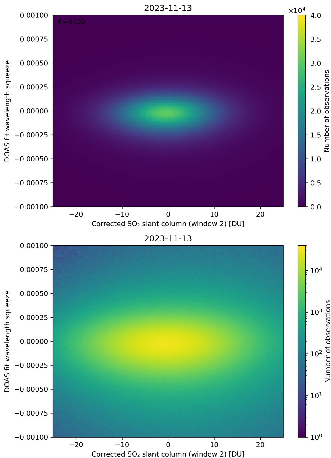
Figure 197: Scatter density plot of “Corrected SO 2 slant column (window 2)” against “DOAS fit wavelength squeeze” for 2023-11-13 to 2023-11-14.
