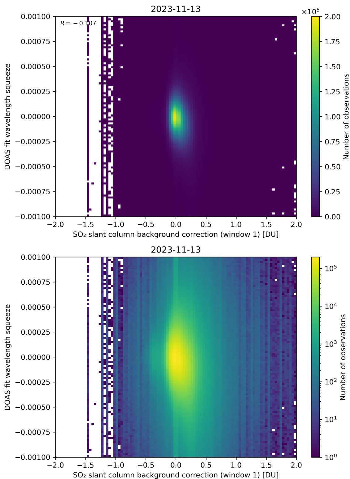
Figure 101: Scatter density plot of “SO 2 slant column background correction (window 1)” against “DOAS fit wavelength squeeze” for 2023-11-13 to 2023-11-14.
