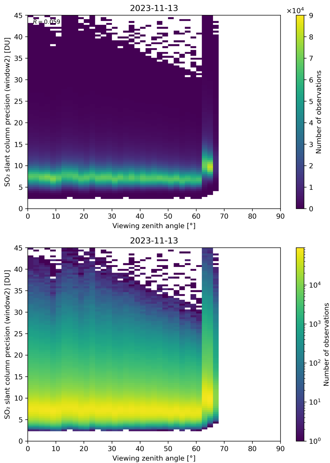
Figure 322: Scatter density plot of “Viewing zenith angle” against “SO 2 slant column precision (window2)” for 2023-11-13 to 2023-11-14.
