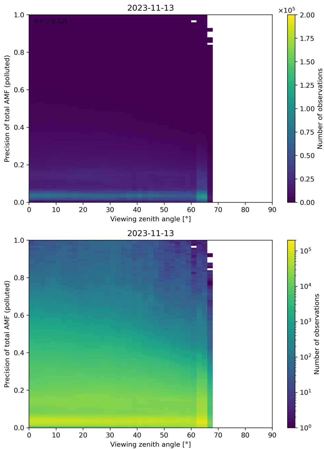
Figure 326: Scatter density plot of “Viewing zenith angle” against “Precision of total AMF (polluted)” for 2023-11-13 to 2023-11-14.
