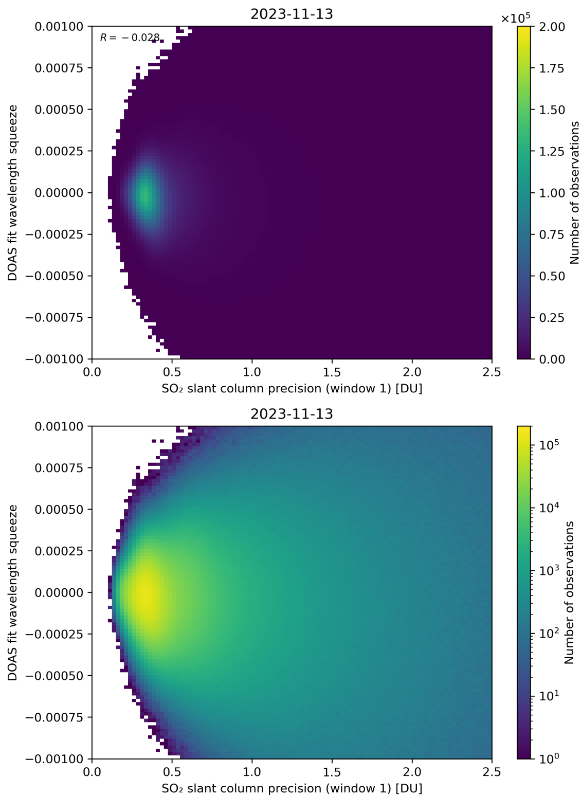
Figure 222: Scatter density plot of “SO 2 slant column precision (window 1)” against “DOAS fit wavelength squeeze” for 2023-11-13 to 2023-11-14.
