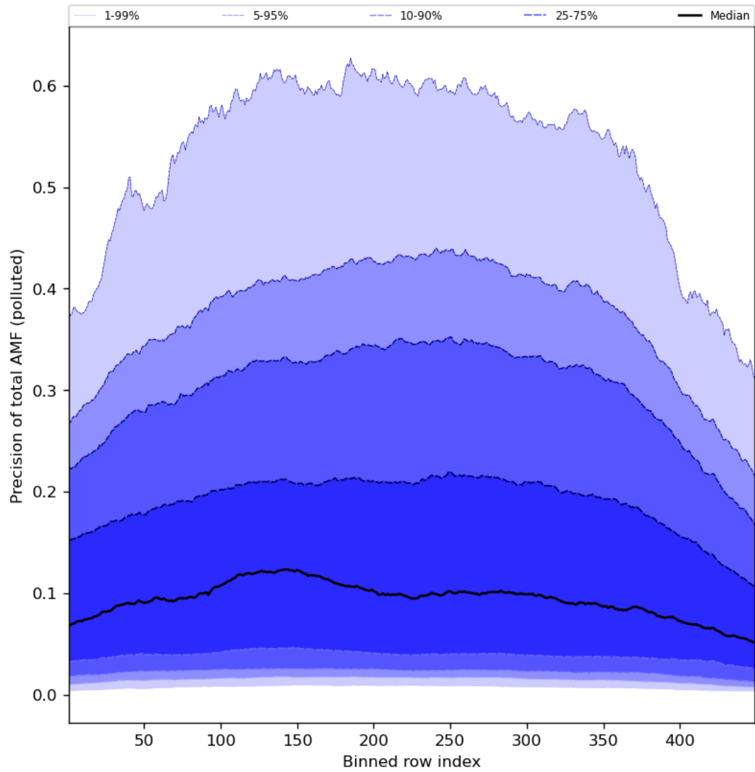
Figure 95: Along track statistics of “Precision of total AMF (polluted)” for 2023-11-13 to 2023-11-14
