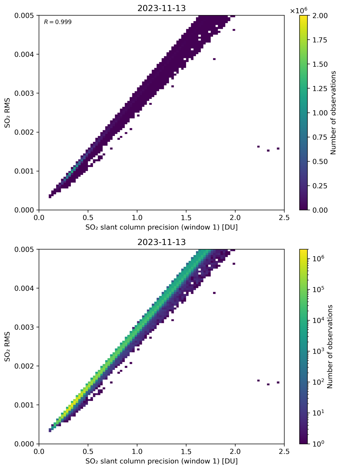
Figure 223: Scatter density plot of “SO 2 slant column precision (window 1)” against “SO 2 RMS” for 2023-11-13 to 2023-11-14.
