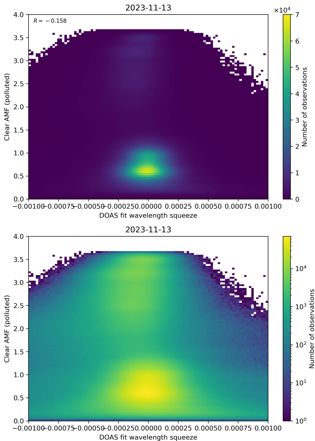
Figure 133: Scatter density plot of “DOAS fit wavelength squeeze” against “Clear AMF (polluted)” for 2023-11-13 to 2023-11-14.
