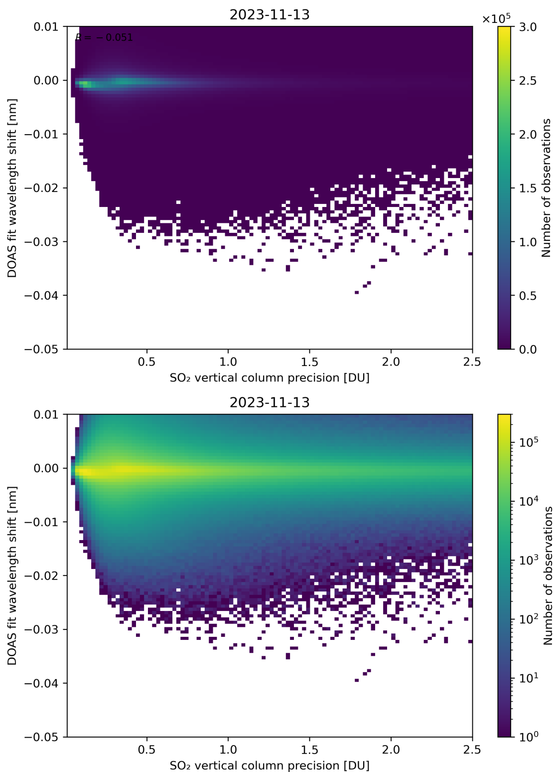
Figure 282: Scatter density plot of “SO 2 vertical column precision” against “DOAS fit wavelength shift” for 2023-11-13 to 2023-11-14.
