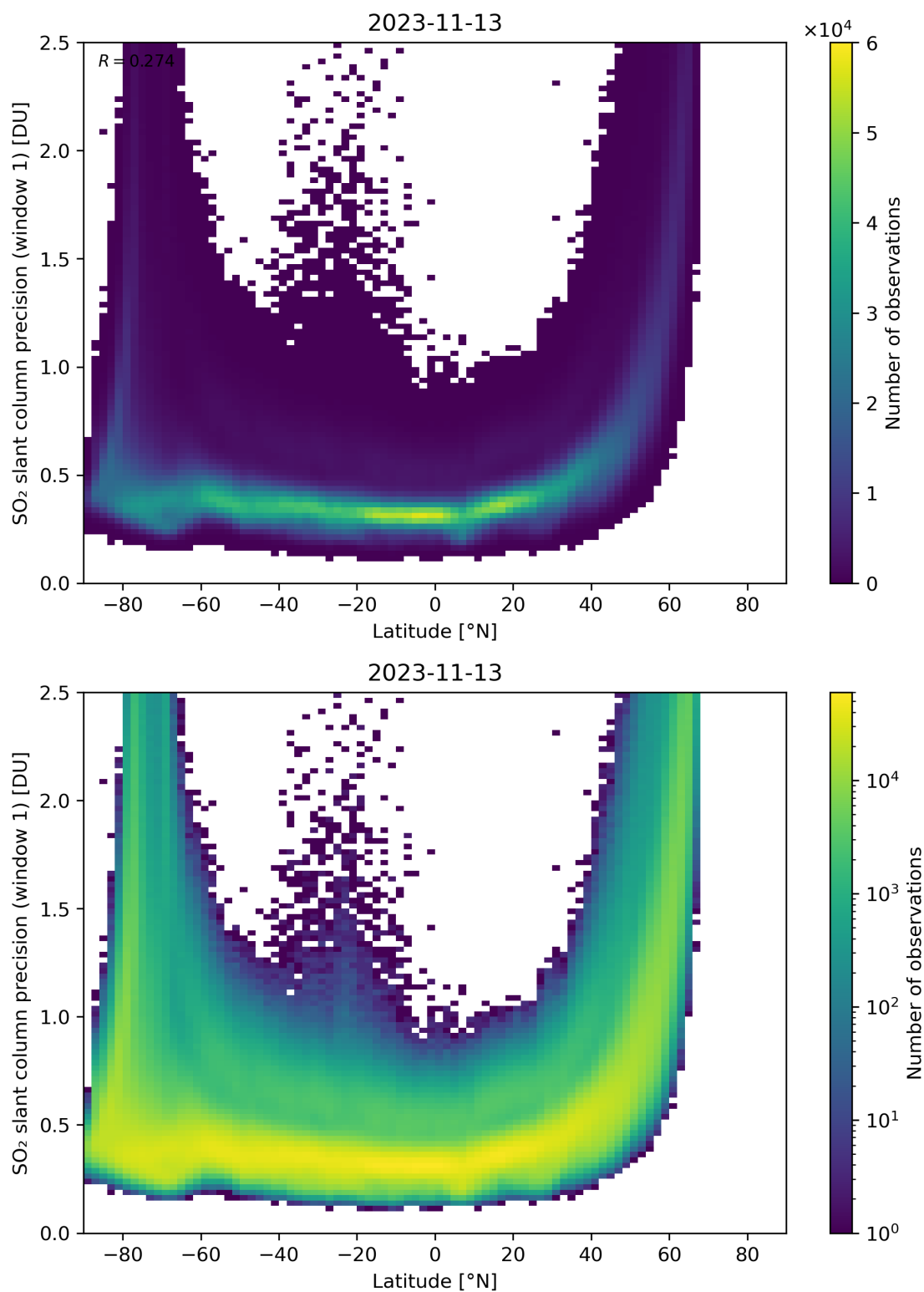
Figure 150: Scatter density plot of “Latitude” against “SO 2 slant column precision (window 1)” for 2023-11-13 to 2023-11-14.
