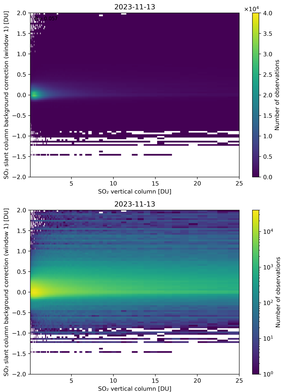
Figure 273: Scatter density plot of “SO 2 vertical column” against “SO 2 slant column background correction (window 1)” for 2023-11-13 to 2023-11-14.
