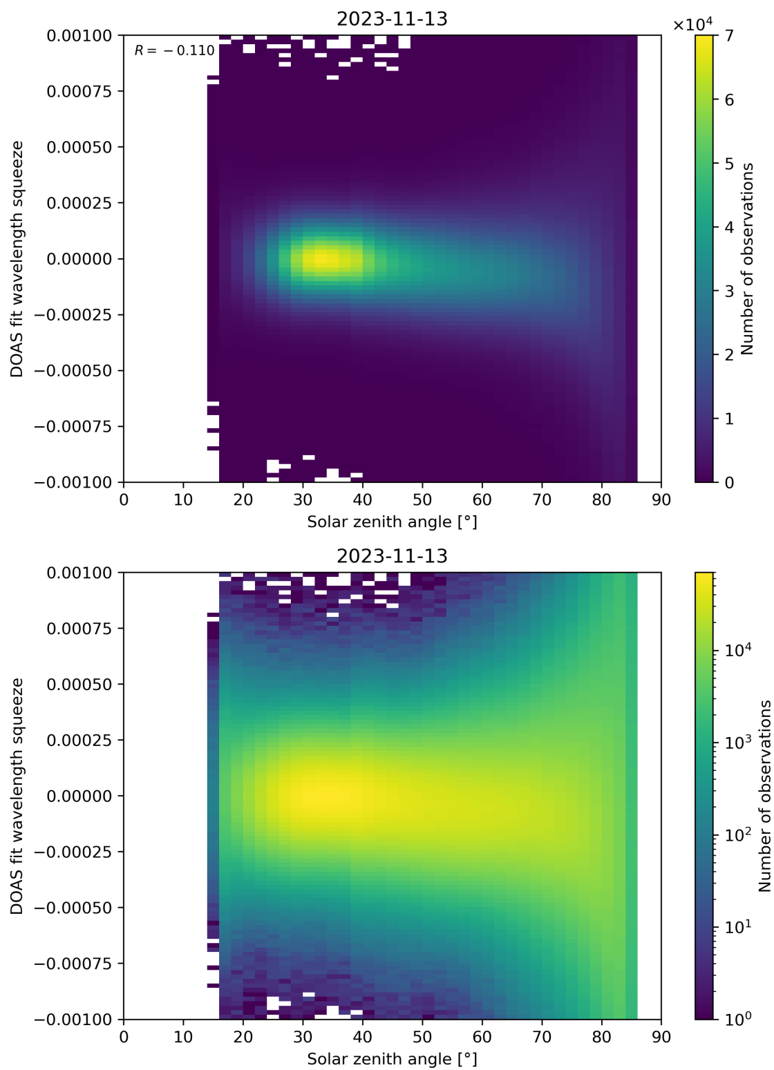
Figure 162: Scatter density plot of “Solar zenith angle” against “DOAS fit wavelength squeeze” for 2023-11-13 to 2023-11-14.
