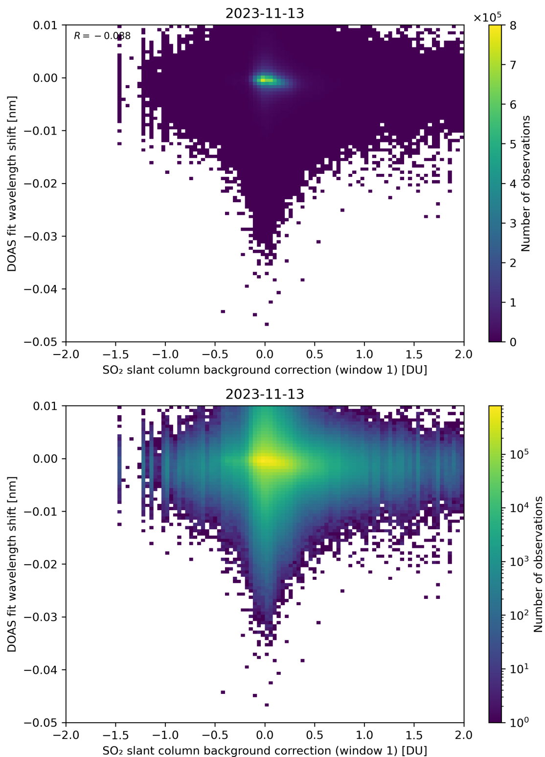
Figure 100: Scatter density plot of “SO 2 slant column background correction (window 1)” against “DOAS fit wavelength shift” for 2023-11-13 to 2023-11-14.
