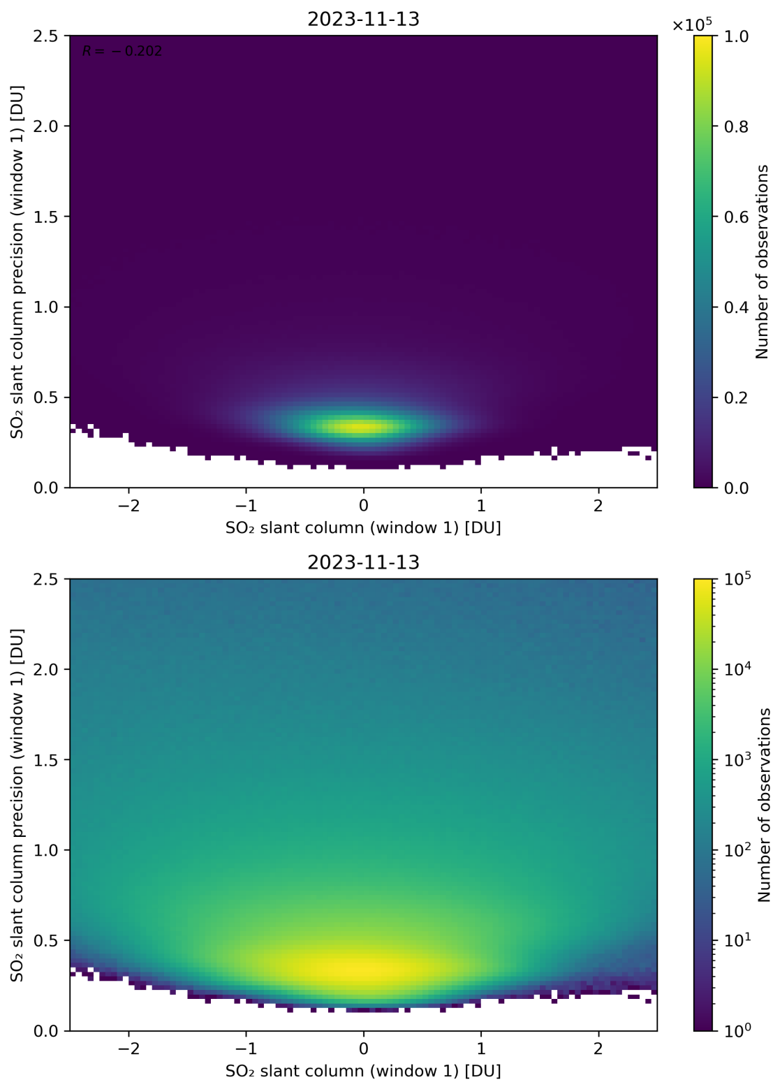
Figure 235: Scatter density plot of “SO 2 slant column (window 1)” against “SO 2 slant column precision (window 1)” for 2023-11-13 to 2023-11-14.
