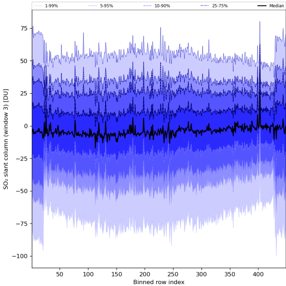
Figure 87: Along track statistics of “SO 2 slant column (window 3)” for 2023-11-13 to 2023-11-14
