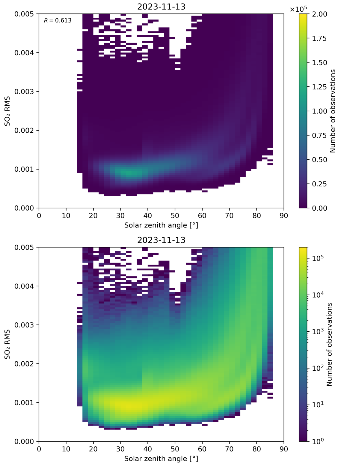
Figure 163: Scatter density plot of “Solar zenith angle” against “SO 2 RMS” for 2023-11-13 to 2023-11-14.
