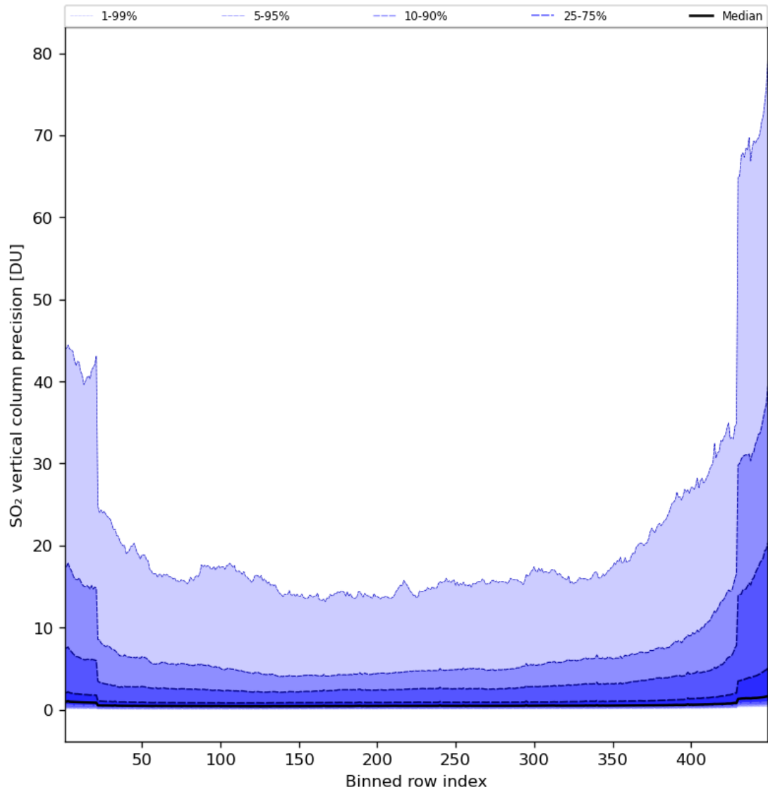
Figure 77: Along track statistics of “SO 2 vertical column precision” for 2023-11-13 to 2023-11-14
