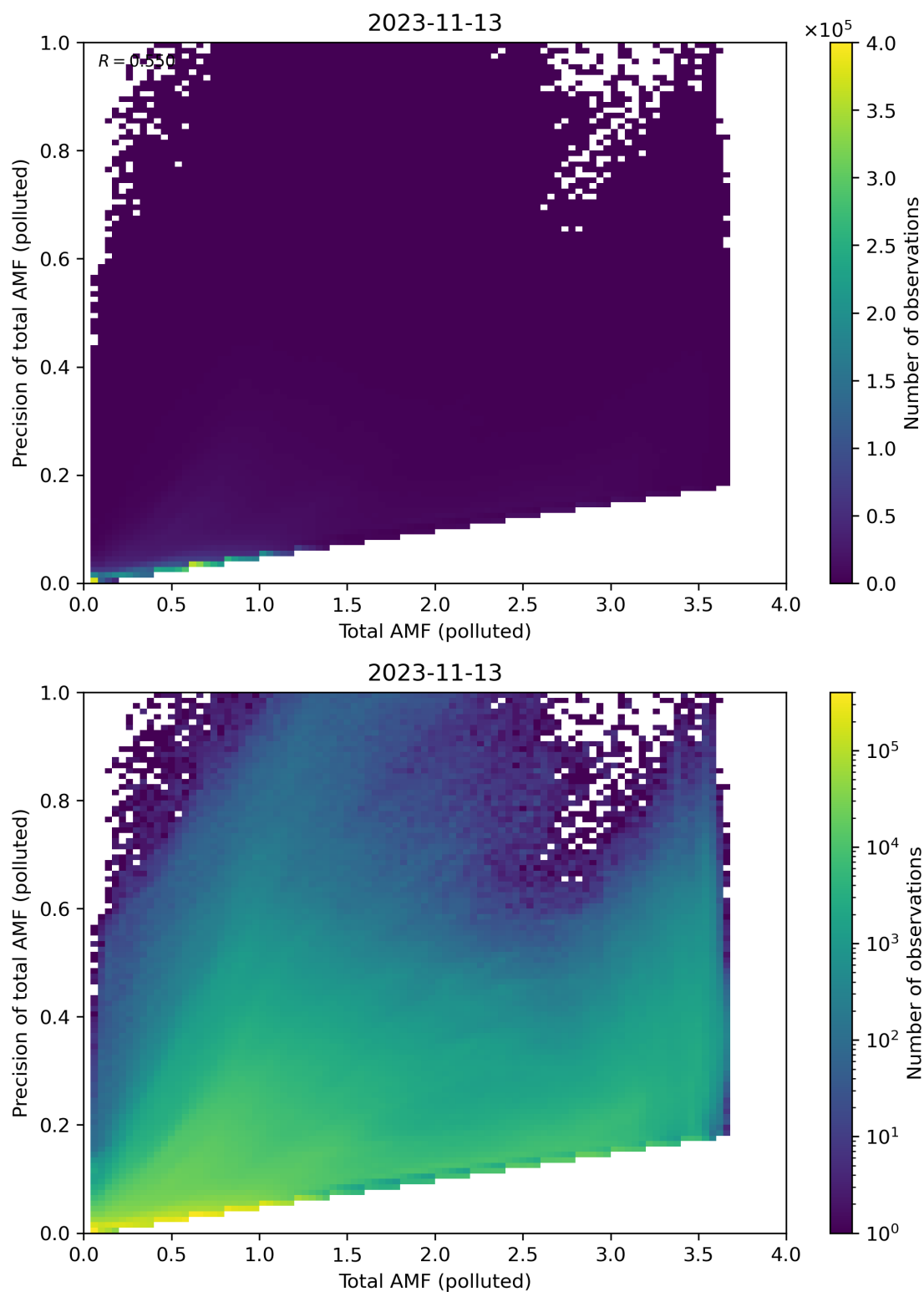
Figure 272: Scatter density plot of “Total AMF (polluted)” against “Precision of total AMF (polluted)” for 2023-11-13 to 2023-11-14.
