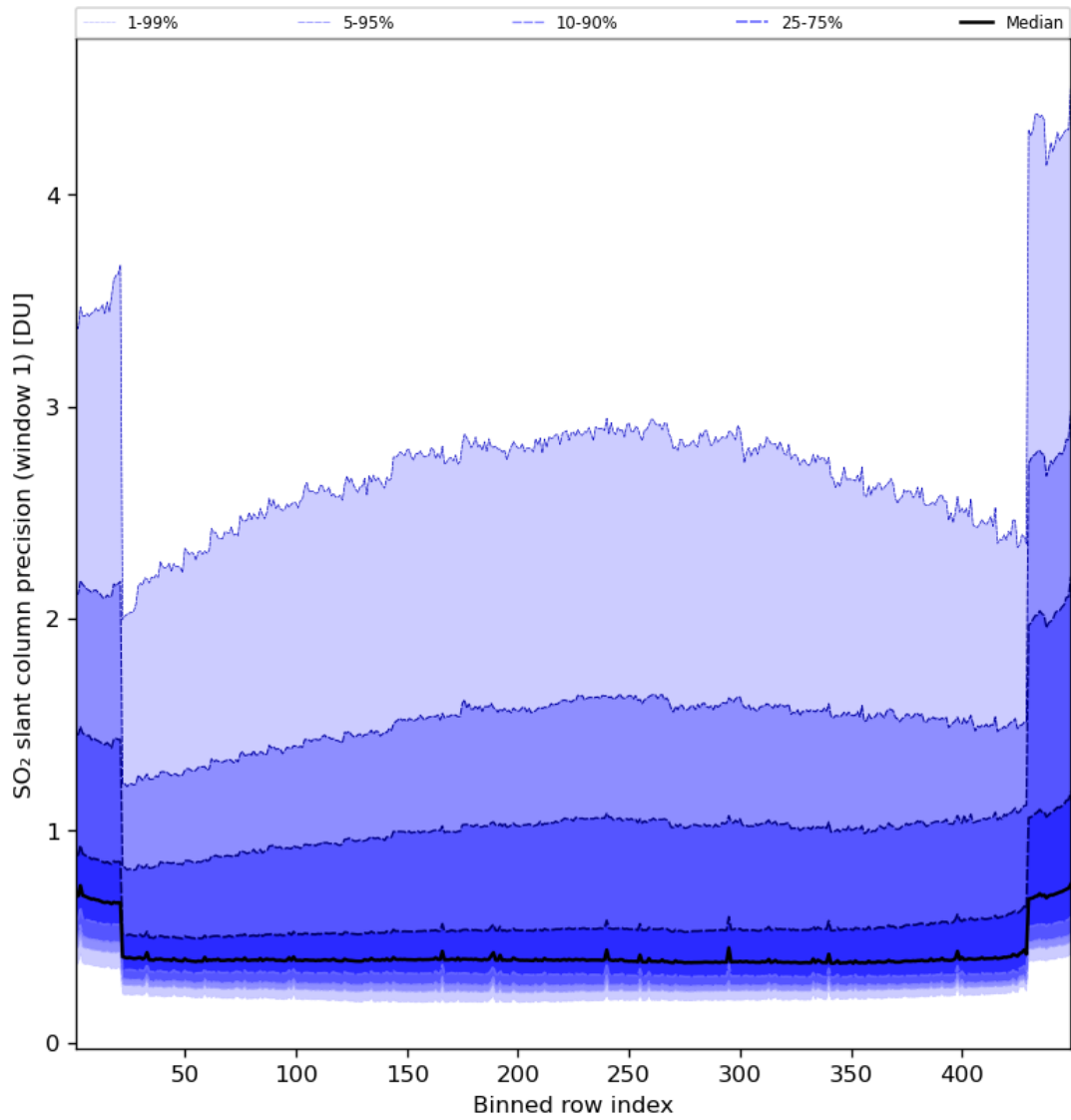
Figure 80: Along track statistics of “SO 2 slant column precision (window 1)” for 2023-11-13 to 2023-11-14
