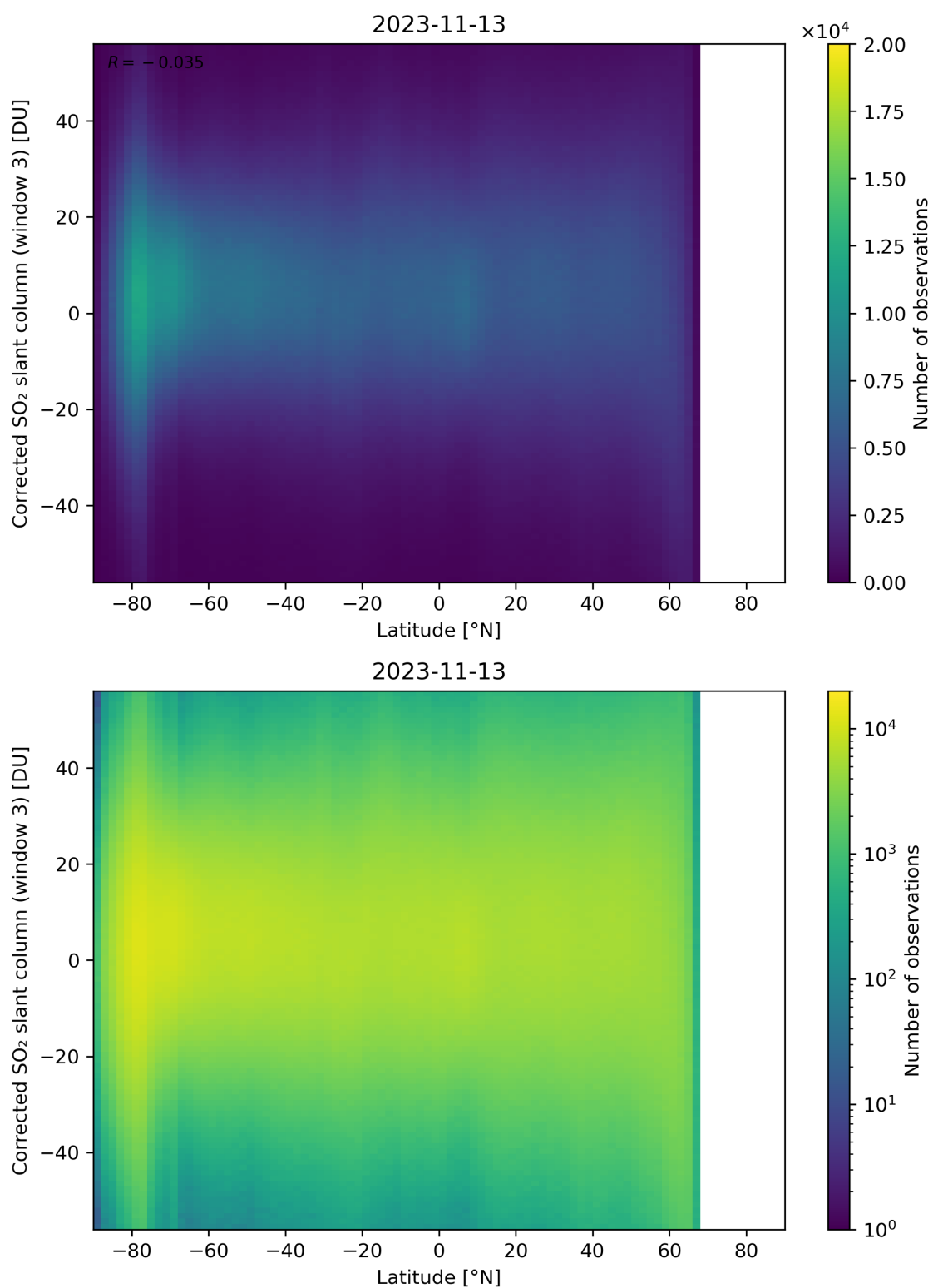
Figure 148: Scatter density plot of “Latitude” against “Corrected SO 2 slant column (window 3)” for 2023-11-13 to 2023-11-14.
