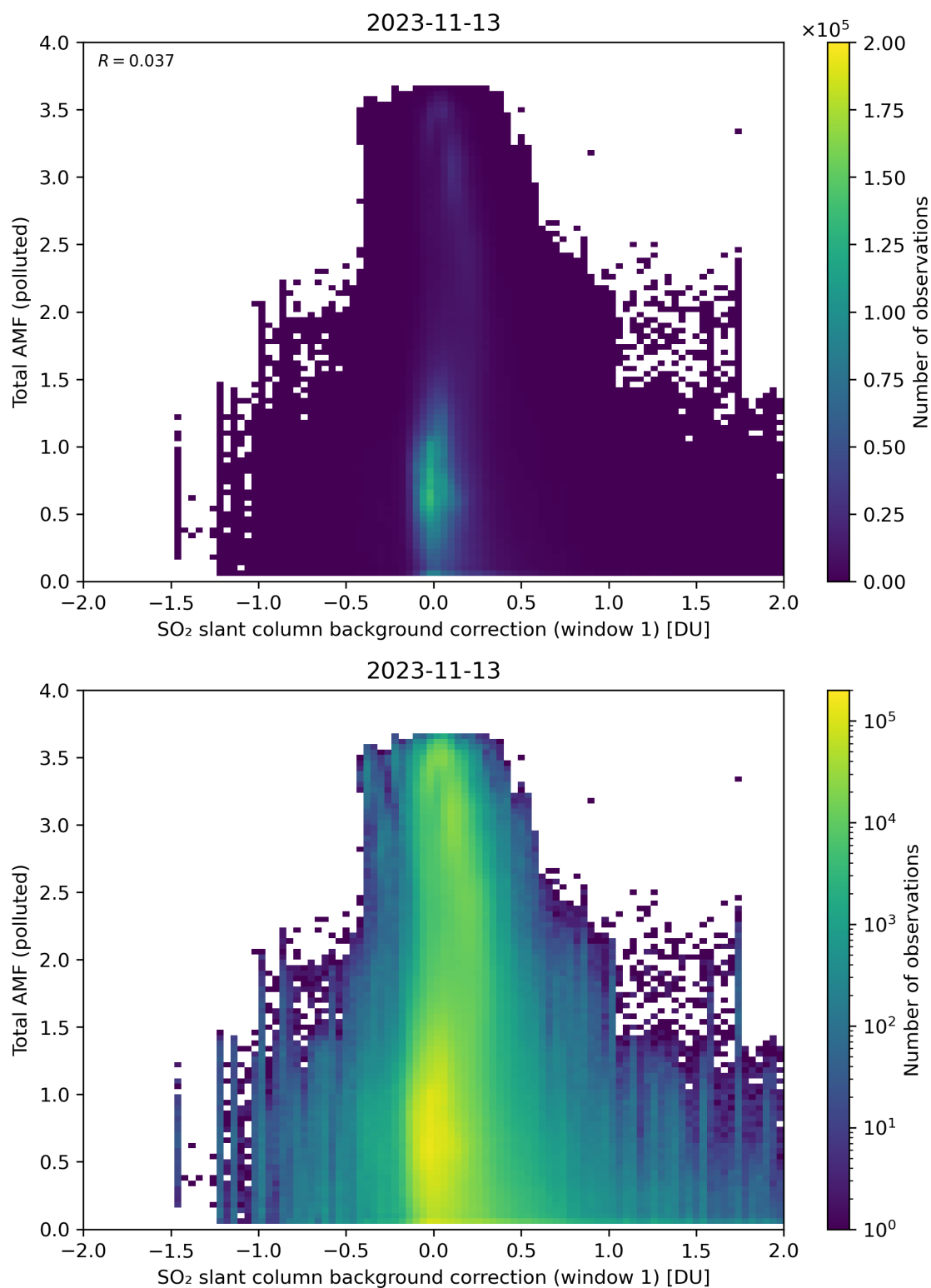
Figure 109: Scatter density plot of “SO 2 slant column background correction (window 1)” against “Total AMF (polluted)” for 2023-11-13 to 2023-11-14.
