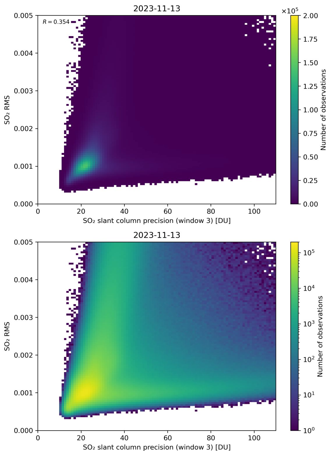
Figure 260: Scatter density plot of “SO 2 slant column precision (window 3)” against “SO 2 RMS” for 2023-11-13 to 2023-11-14.
