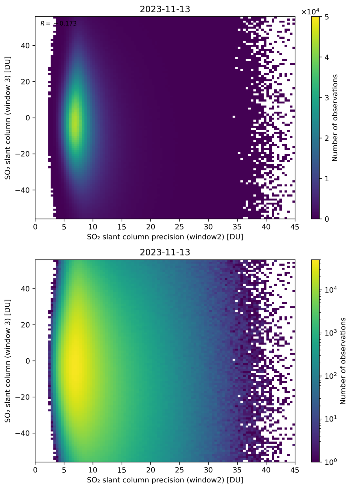
Figure 249: Scatter density plot of “SO 2 slant column precision (window2)” against “SO 2 slant column (window 3)” for 2023-11-13 to 2023-11-14.
