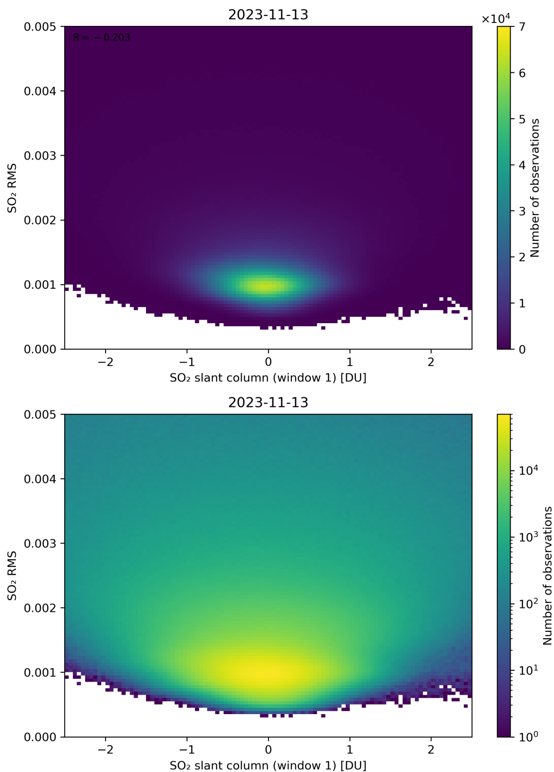
Figure 217: Scatter density plot of “SO 2 slant column (window 1)” against “SO 2 RMS” for 2023-11-13 to 2023-11-14.
