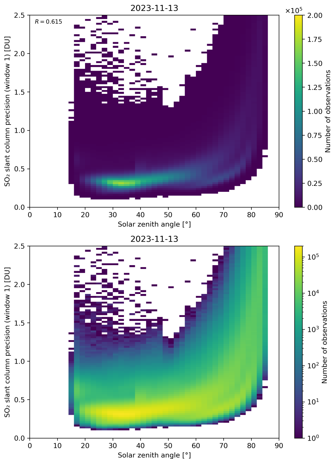
Figure 170: Scatter density plot of “Solar zenith angle” against “SO 2 slant column precision (window 1)” for 2023-11-13 to 2023-11-14.
