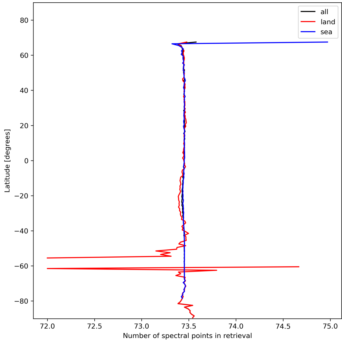
Figure 51: Zonal average of “Number of spectral points in retrieval” for 2023-11-13 to 2023-11-14.
