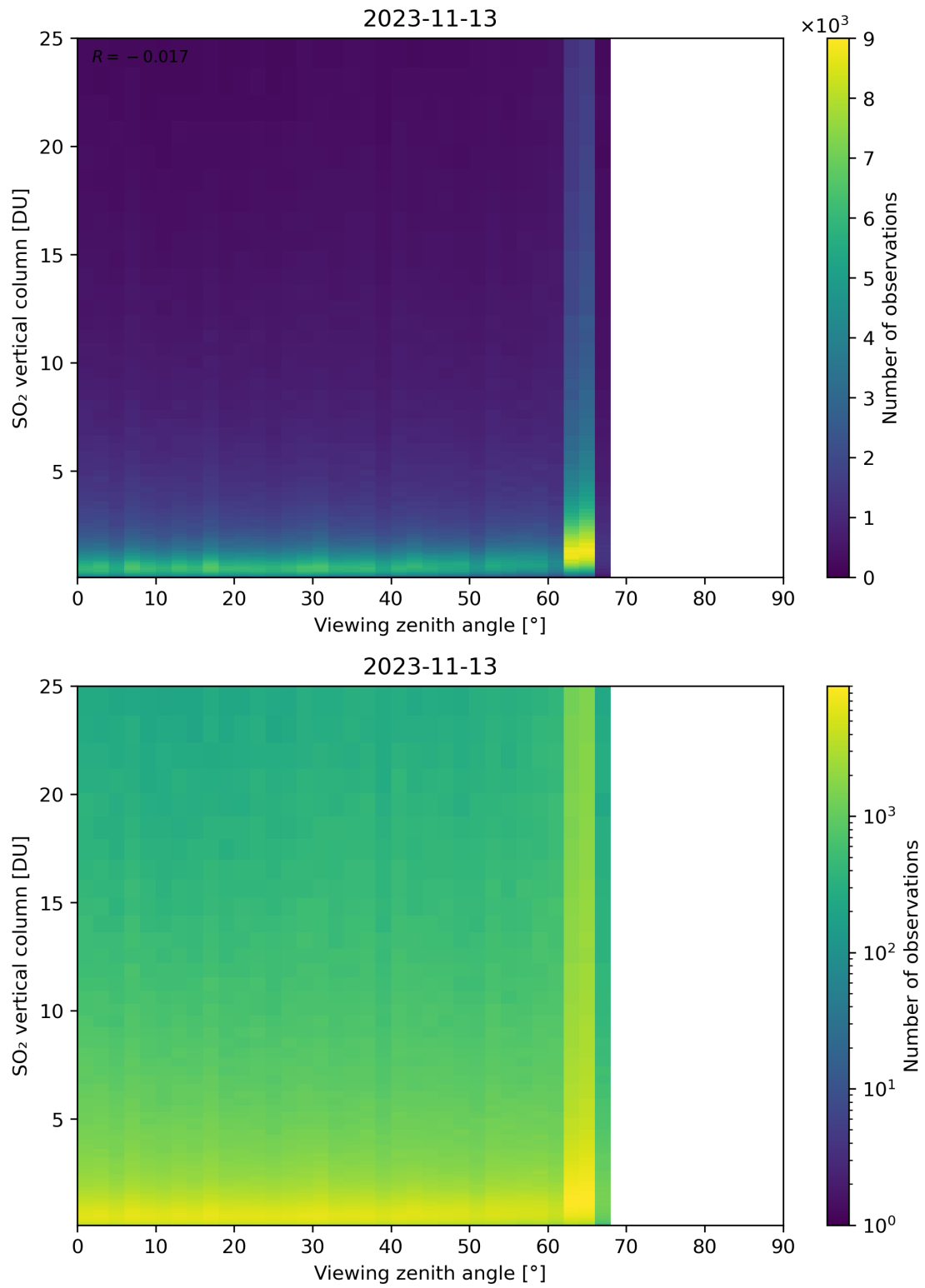
Figure 327: Scatter density plot of “Viewing zenith angle” against “SO 2 vertical column” for 2023-11-13 to 2023-11-14.
