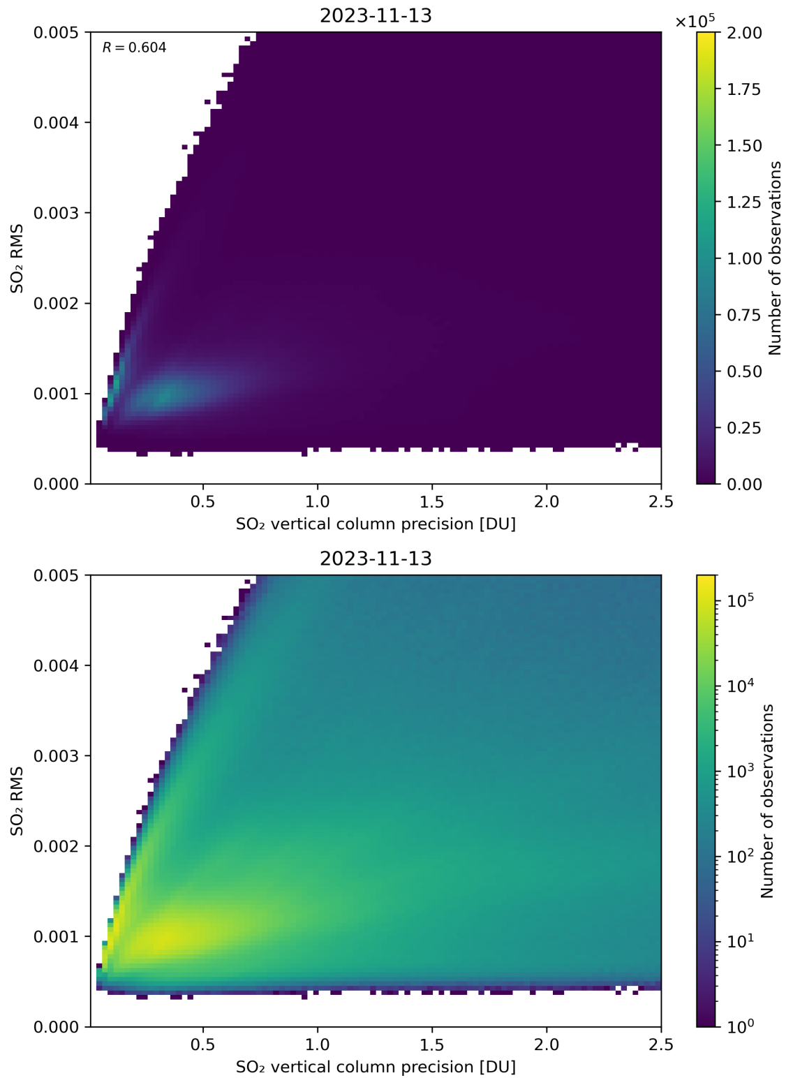
Figure 284: Scatter density plot of “SO 2 vertical column precision” against “SO 2 RMS” for 2023-11-13 to 2023-11-14.
