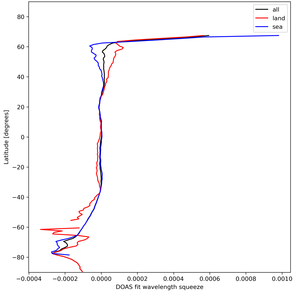
Figure 46: Zonal average of “DOAS fit wavelength squeeze” for 2023-11-13 to 2023-11-14.
