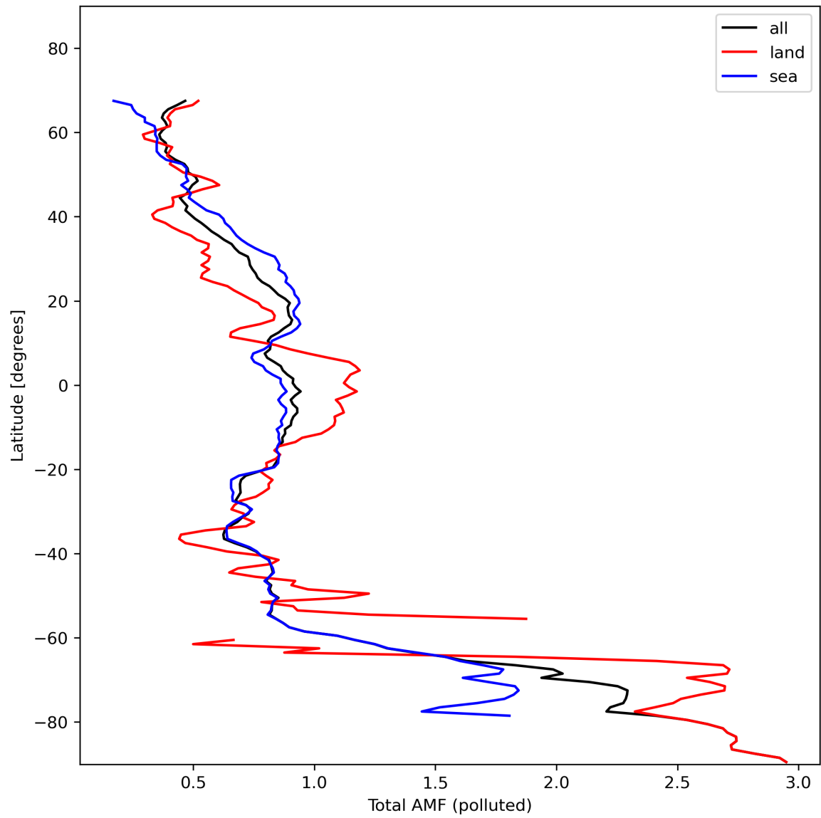
Figure 48: Zonal average of “Total AMF (polluted)” for 2023-11-13 to 2023-11-14.
