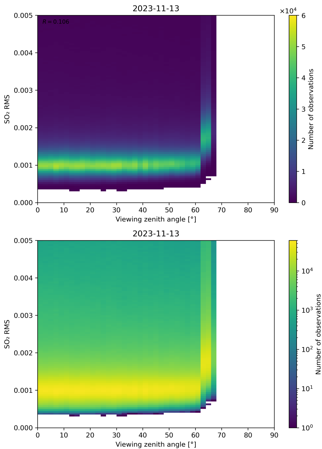
Figure 313: Scatter density plot of “Viewing zenith angle” against “SO 2 RMS” for 2023-11-13 to 2023-11-14.
