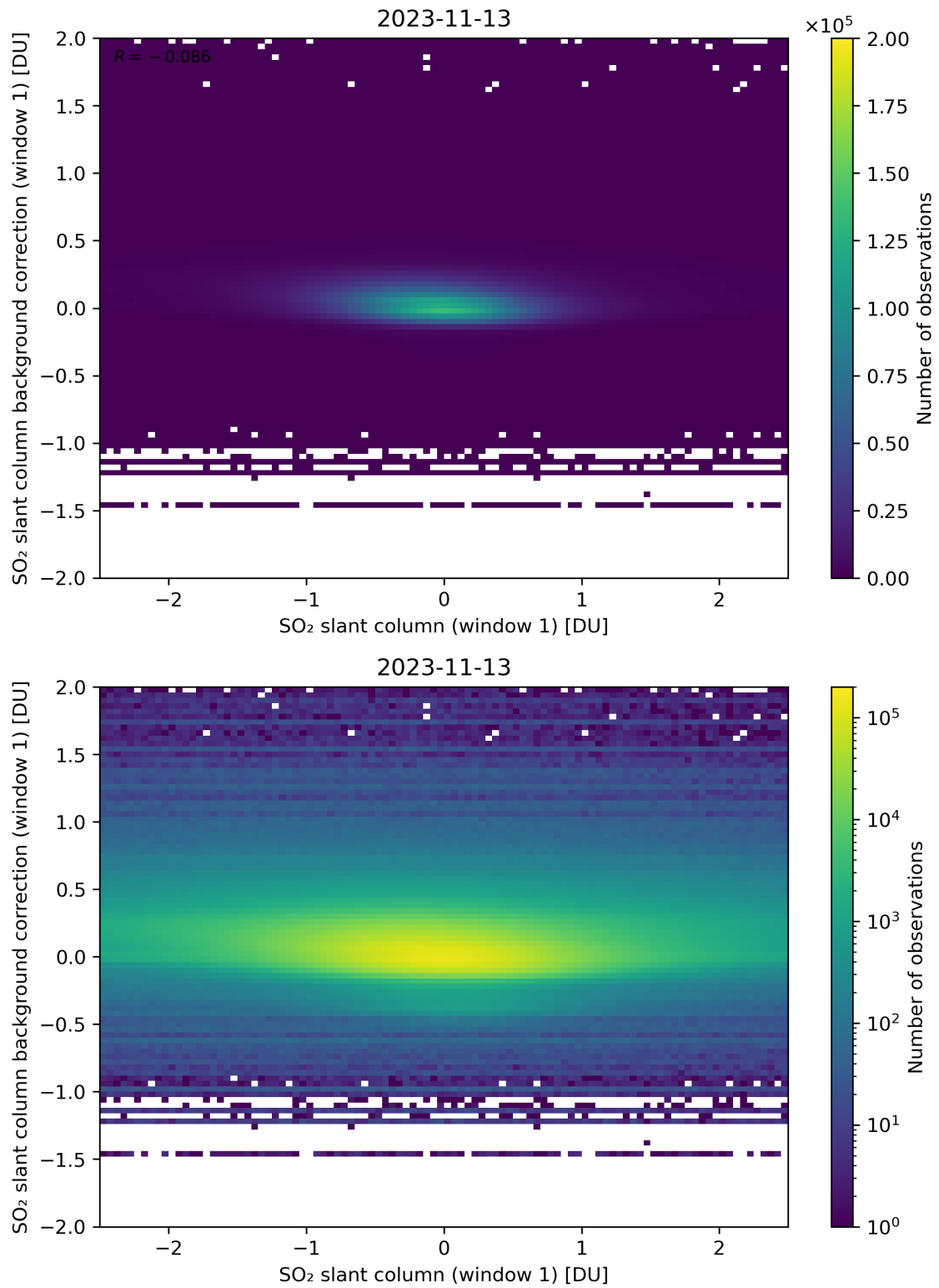
Figure 212: Scatter density plot of “SO 2 slant column (window 1)” against “SO 2 slant column background correction (window 1)” for 2023-11-13 to 2023-11-14.
