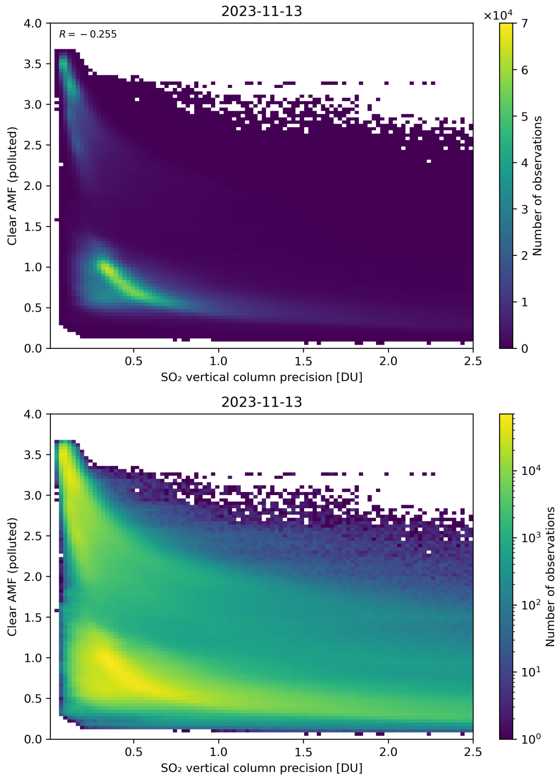
Figure 285: Scatter density plot of “SO 2 vertical column precision” against “Clear AMF (polluted)” for 2023-11-13 to 2023-11-14.
