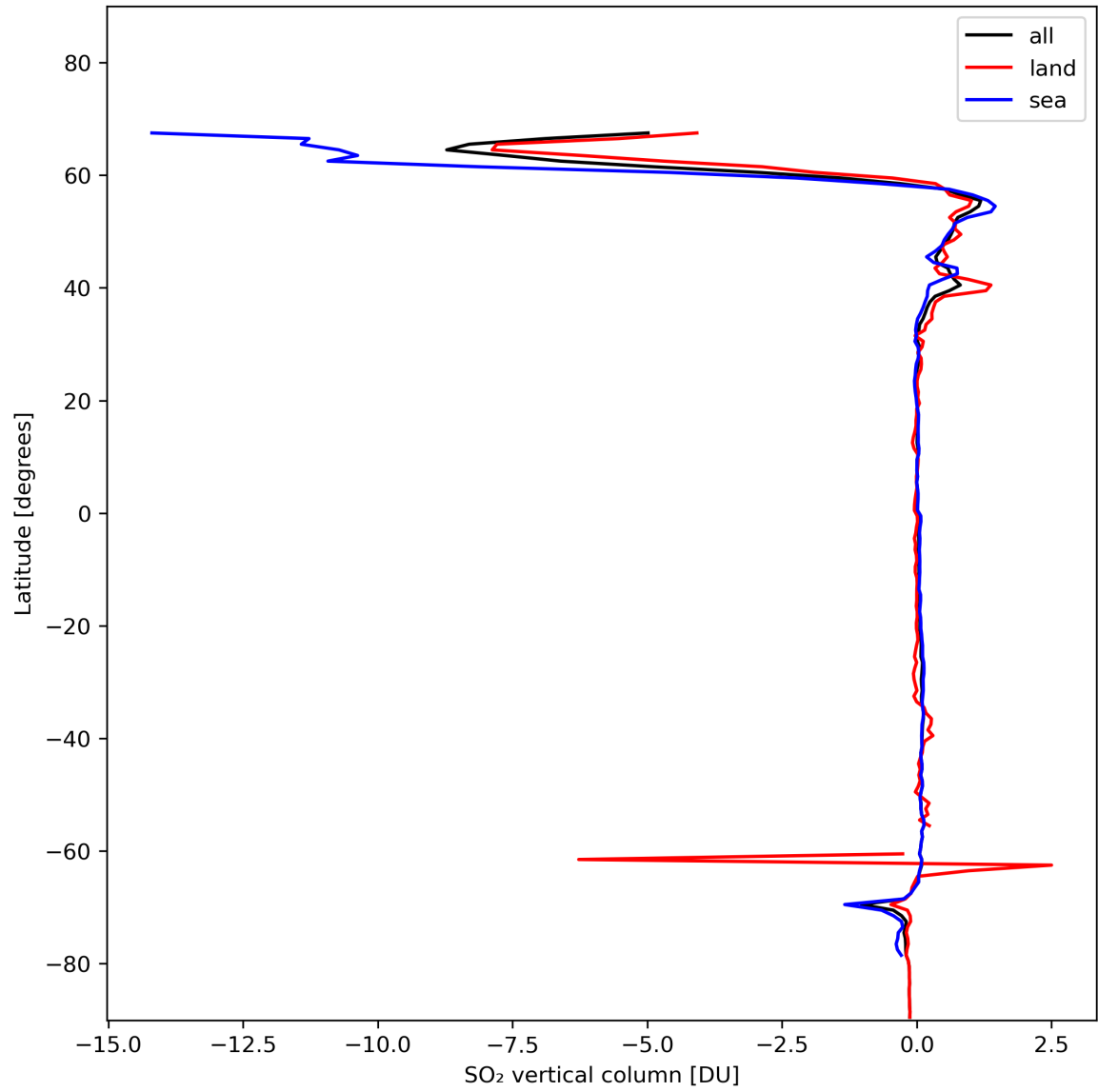
Figure 30: Zonal average of “SO 2 vertical column” for 2023-11-13 to 2023-11-14.
