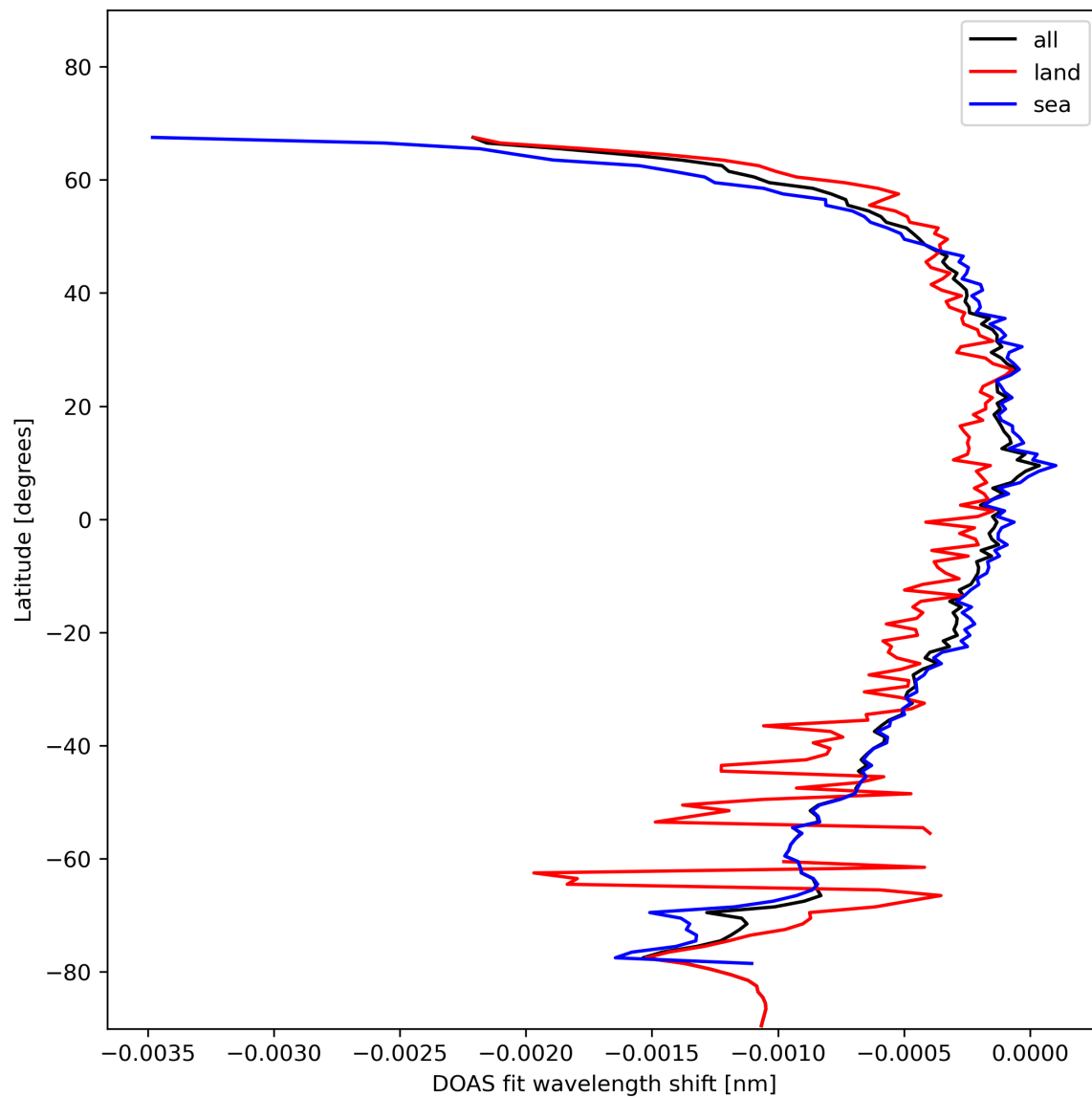
Figure 45: Zonal average of “DOAS fit wavelength shift” for 2023-11-13 to 2023-11-14.
