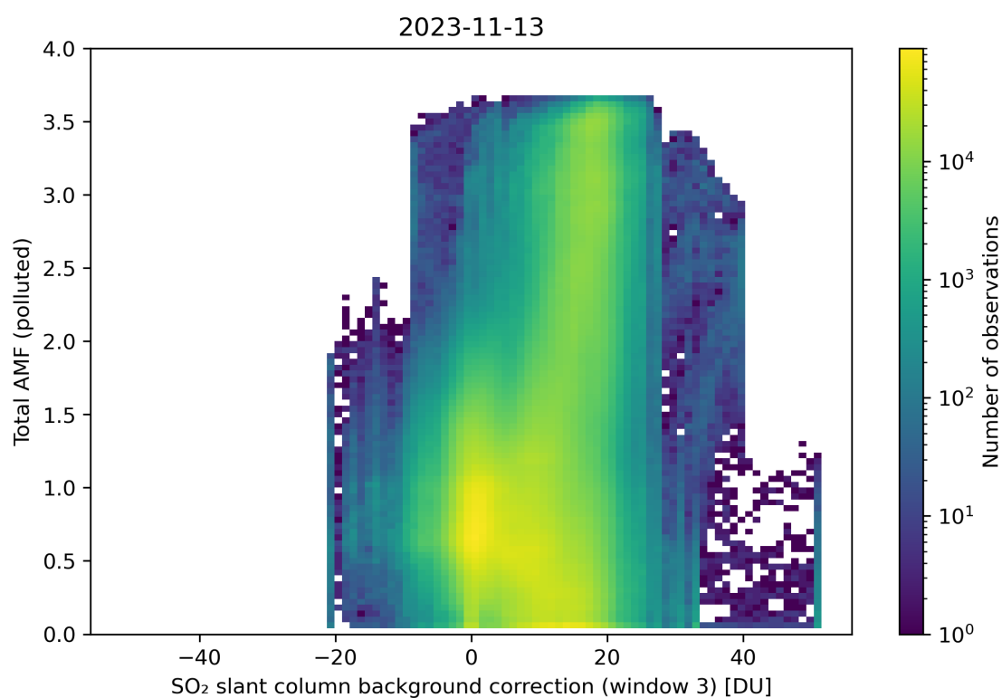
Figure 125: Scatter density plot of “SO 2 slant column background correction (window 3)” against “Total AMF (polluted)” for 2023-11-13 to 2023-11-14.
