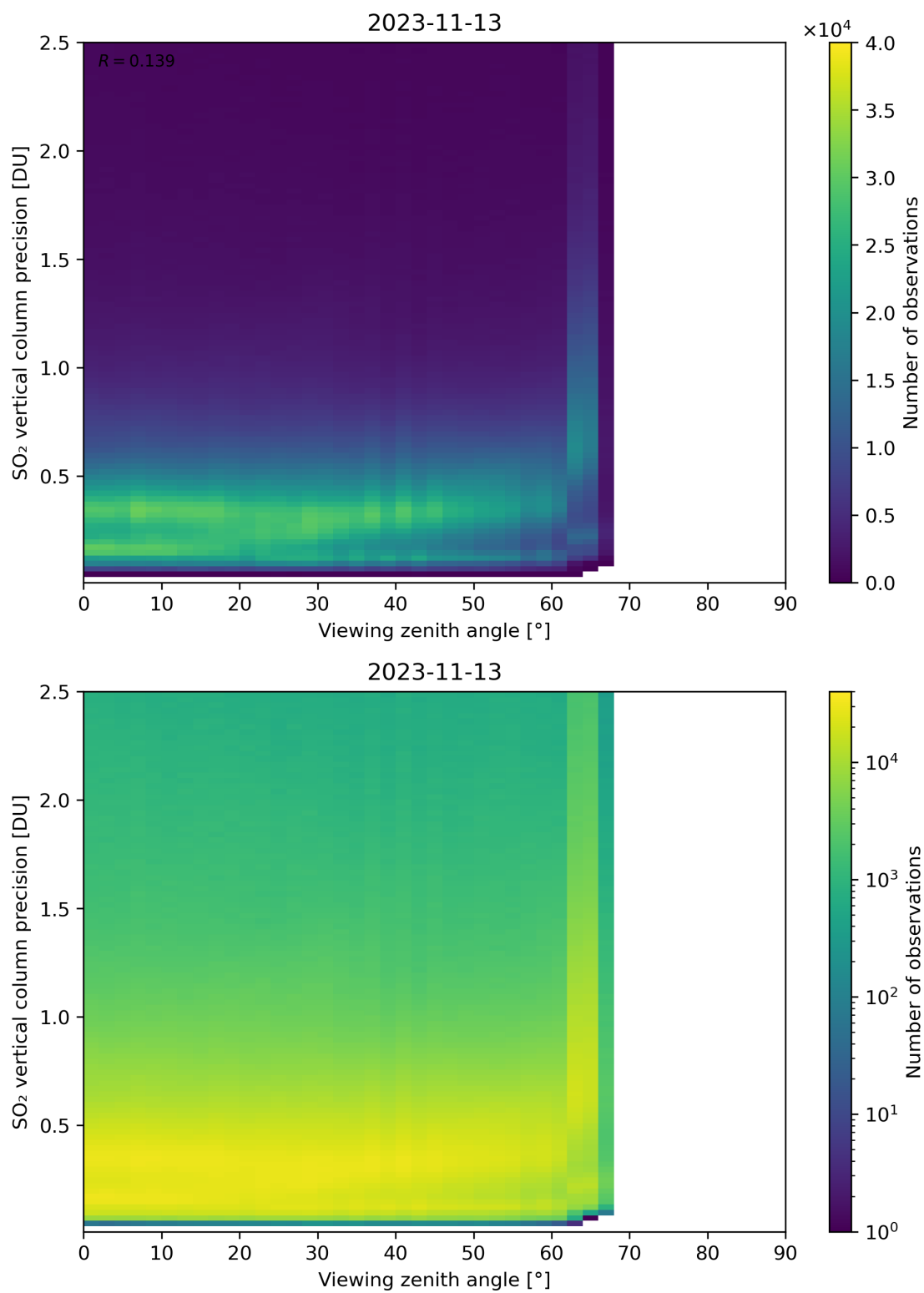
Figure 328: Scatter density plot of “Viewing zenith angle” against “SO 2 vertical column precision” for 2023-11-13 to 2023-11-14.
