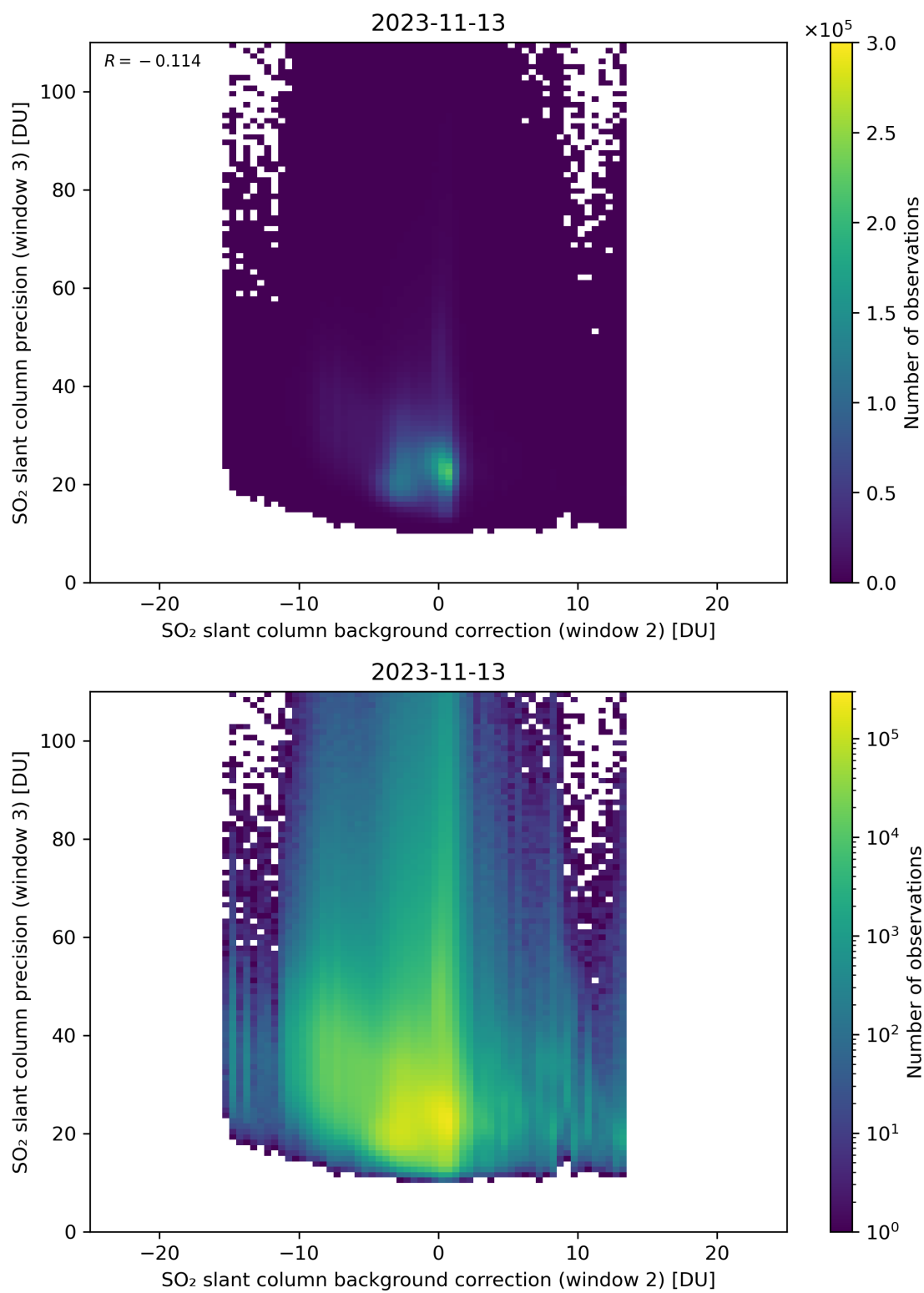
Figure 118: Scatter density plot of “SO 2 slant column background correction (window 2)” against “SO 2 slant column precision (window 3)” for 2023-11-13 to 2023-11-14.
