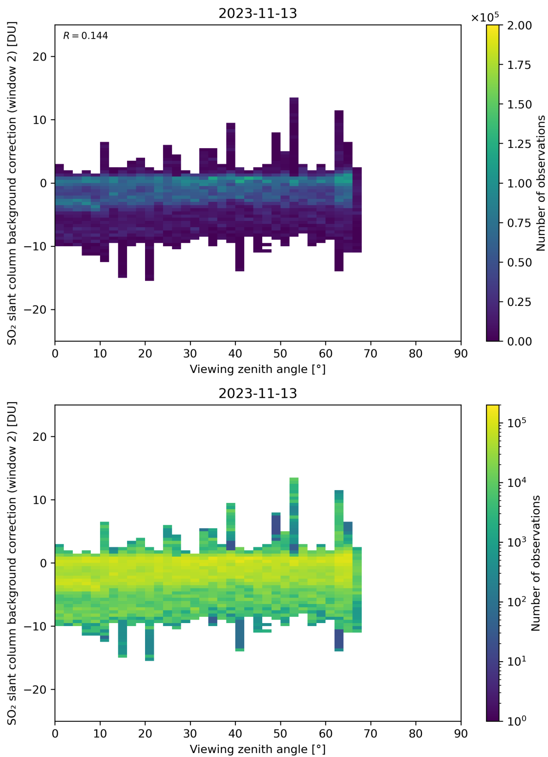
Figure 309: Scatter density plot of “Viewing zenith angle” against “SO 2 slant column background correction (window 2)” for 2023-11-13 to 2023-11-14.
