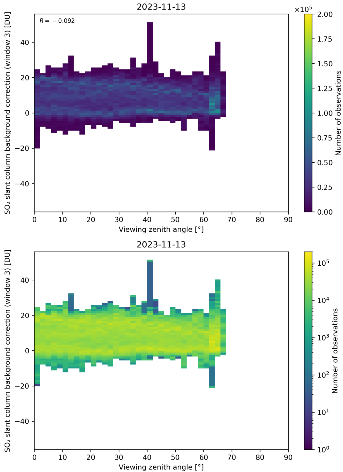
Figure 310: Scatter density plot of “Viewing zenith angle” against “SO 2 slant column background correction (window 3)” for 2023-11-13 to 2023-11-14.
