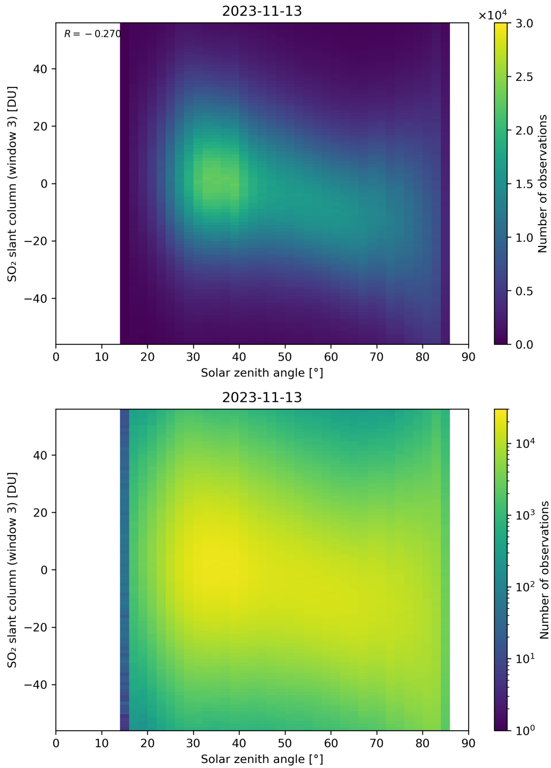
Figure 172: Scatter density plot of “Solar zenith angle” against “SO 2 slant column (window 3)” for 2023-11-13 to 2023-11-14.
