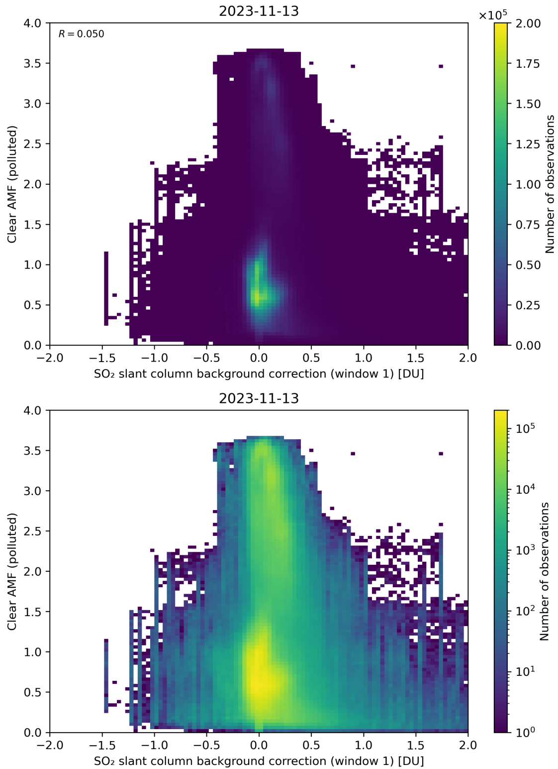
Figure 103: Scatter density plot of “SO 2 slant column background correction (window 1)” against “Clear AMF (polluted)” for 2023-11-13 to 2023-11-14.
