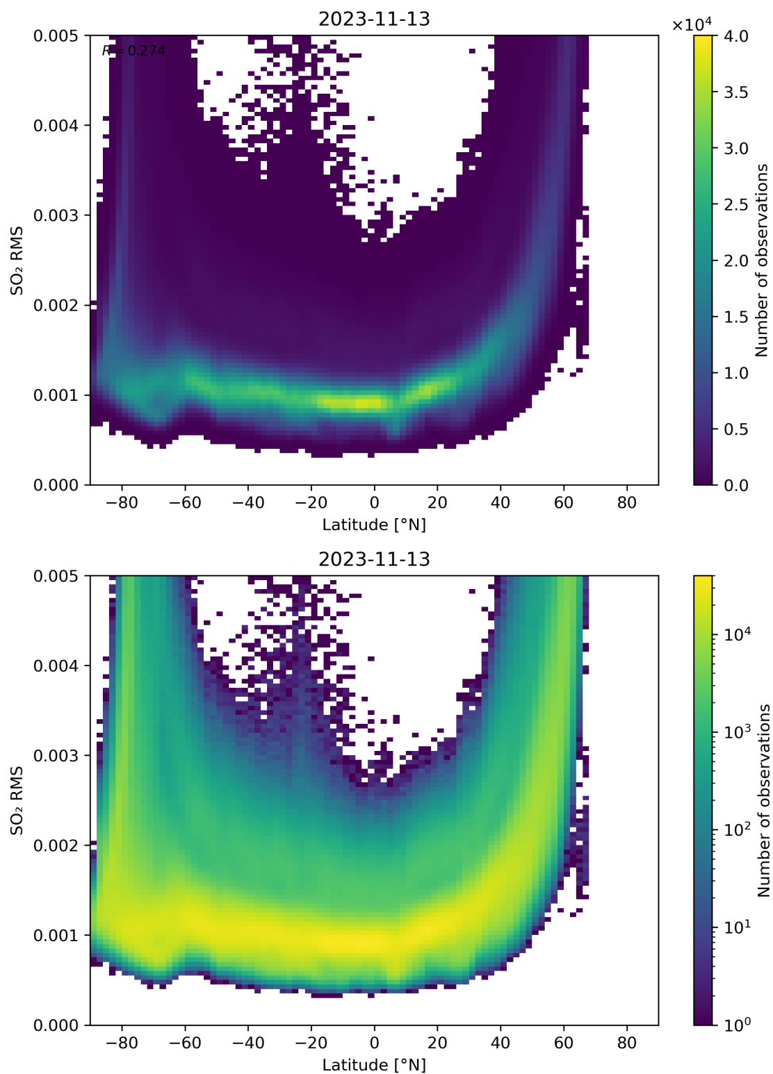
Figure 144: Scatter density plot of “Latitude” against “SO 2 RMS” for 2023-11-13 to 2023-11-14.
