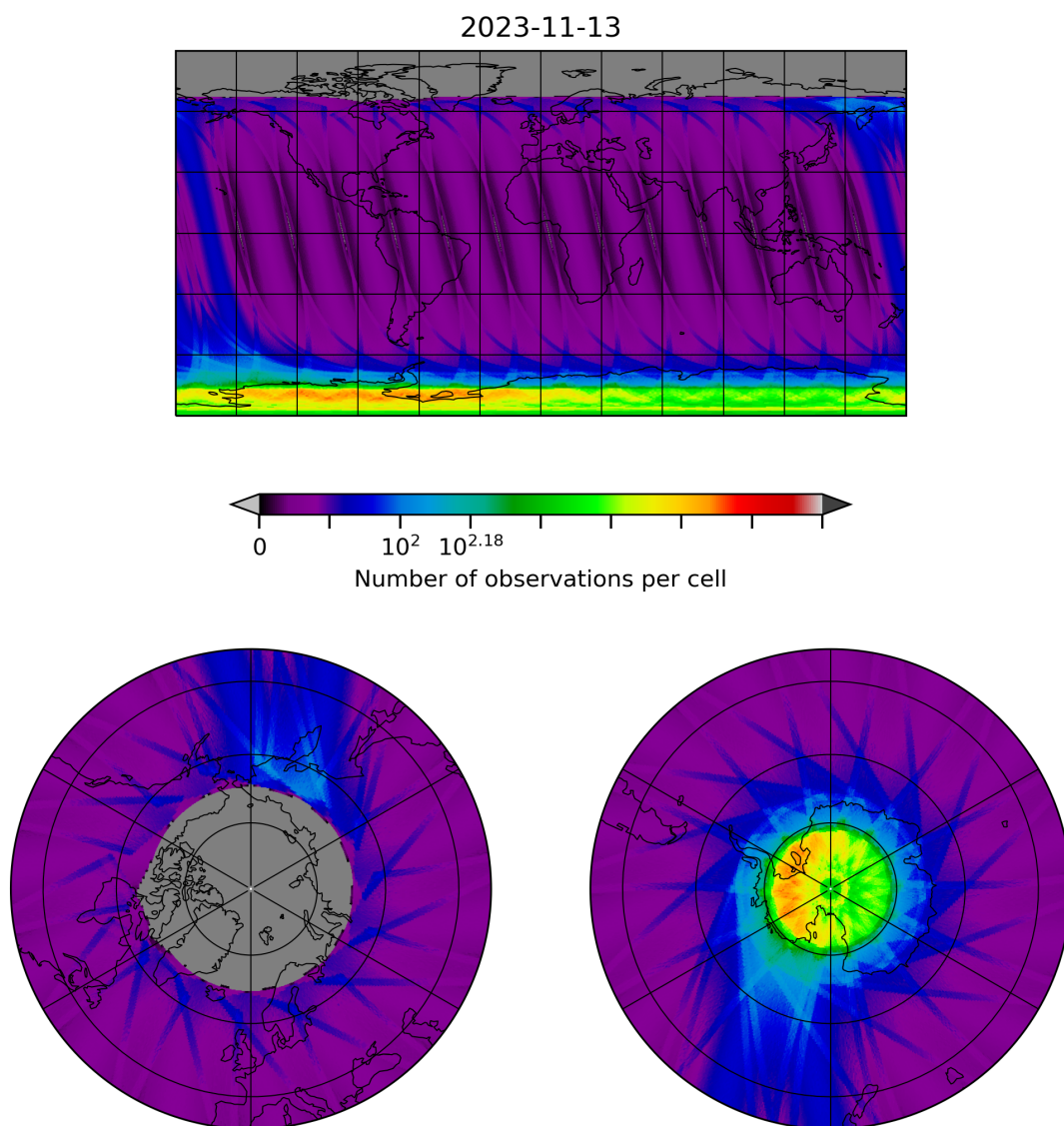
Figure 28: Map of the number of observations for 2023-11-13 to 2023-11-14
