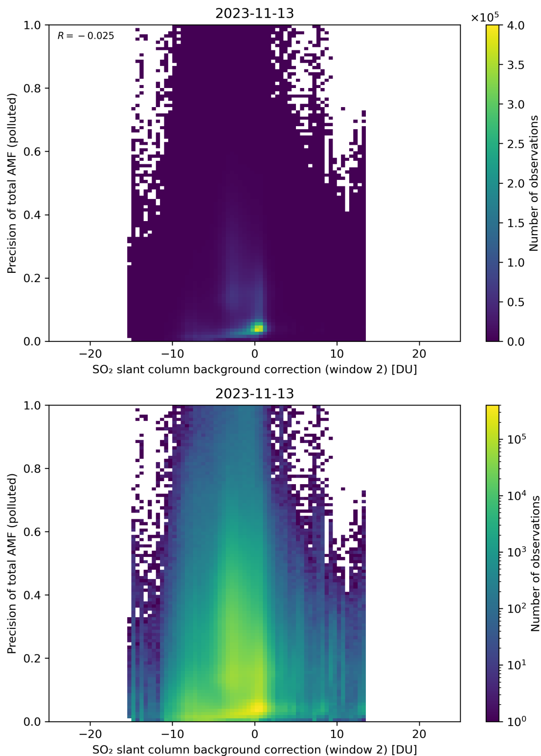
Figure 120: Scatter density plot of “SO 2 slant column background correction (window 2)” against “Precision of total AMF (polluted)” for 2023-11-13 to 2023-11-14.
