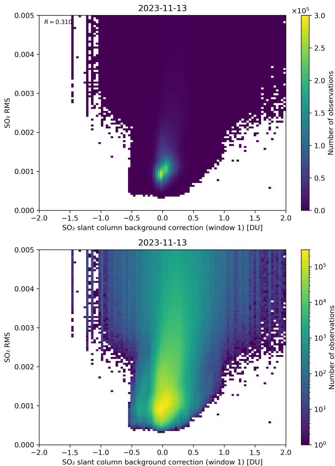
Figure 102: Scatter density plot of “SO 2 slant column background correction (window 1)” against “SO 2 RMS” for 2023-11-13 to 2023-11-14.
