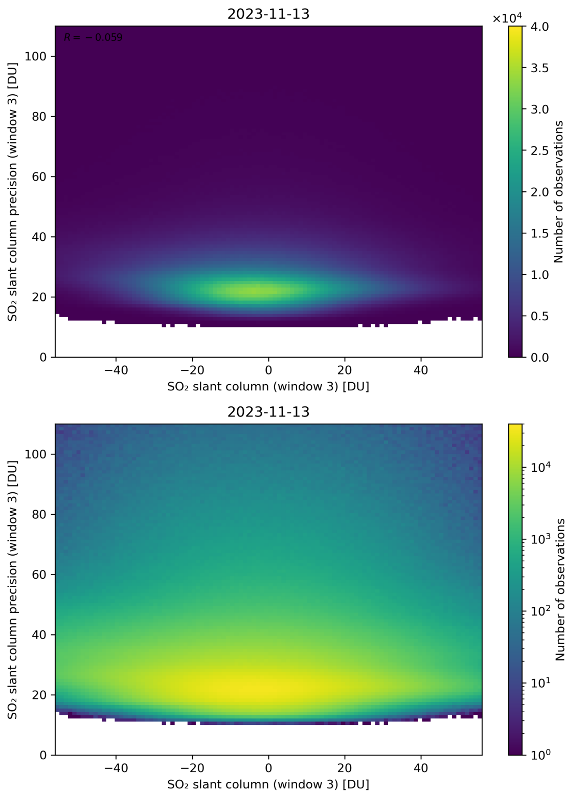
Figure 267: Scatter density plot of “SO 2 slant column (window 3)” against “SO 2 slant column precision (window 3)” for 2023-11-13 to 2023-11-14.
