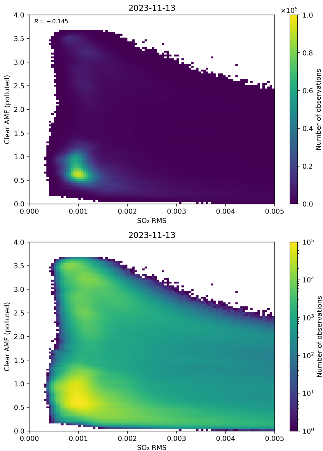
Figure 136: Scatter density plot of “SO 2 RMS” against “Clear AMF (polluted)” for 2023-11-13 to 2023-11-14.
