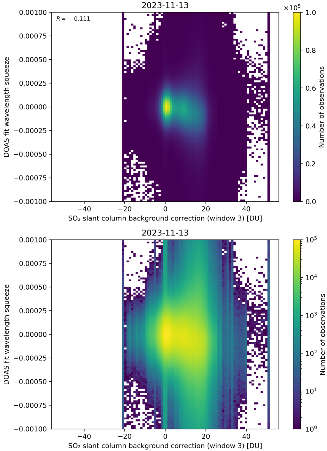
Figure 122: Scatter density plot of “SO 2 slant column background correction (window 3)” against “DOAS fit wavelength squeeze” for 2023-11-13 to 2023-11-14.
