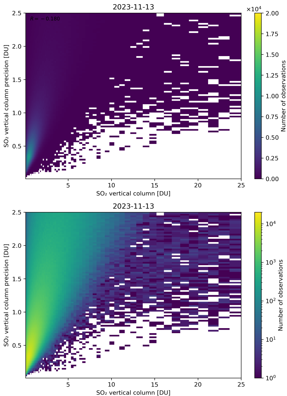
Figure 307: Scatter density plot of “SO 2 vertical column” against “SO 2 vertical column precision” for 2023-11-13 to 2023-11-14.
