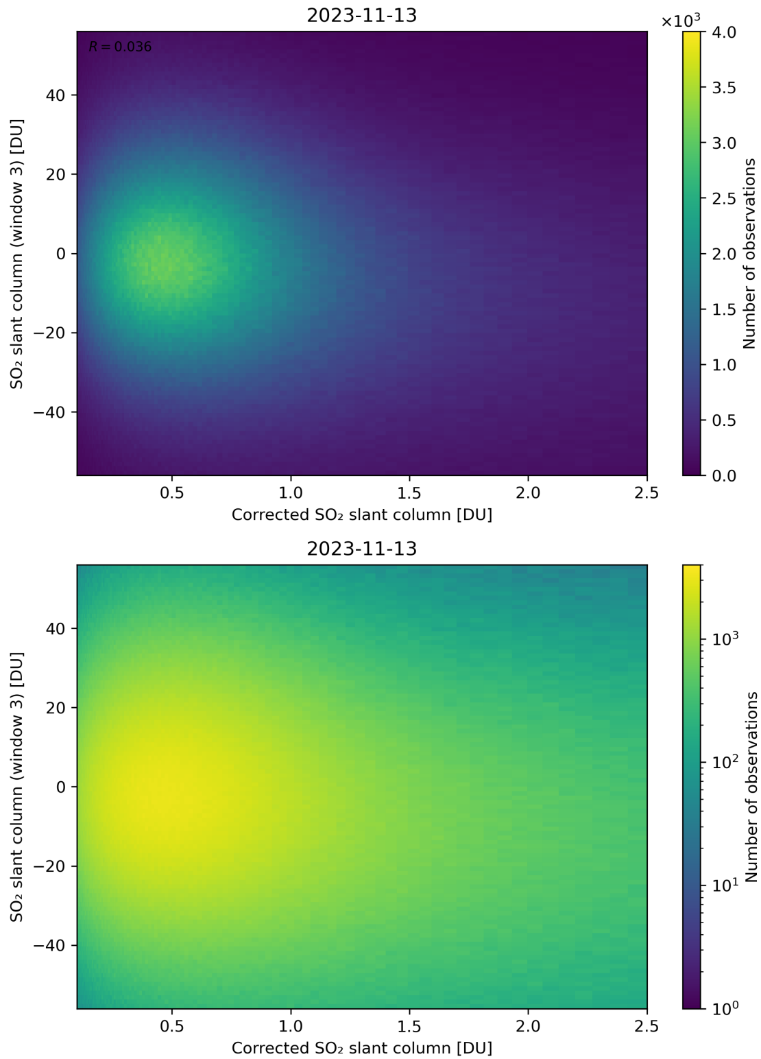
Figure 190: Scatter density plot of “Corrected SO 2 slant column” against “SO 2 slant column (window 3)” for 2023-11-13 to 2023-11-14.
