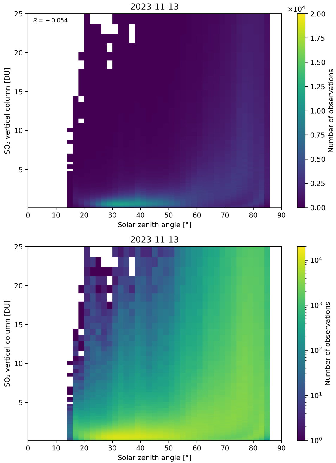
Figure 176: Scatter density plot of “Solar zenith angle” against “SO 2 vertical column” for 2023-11-13 to 2023-11-14.
