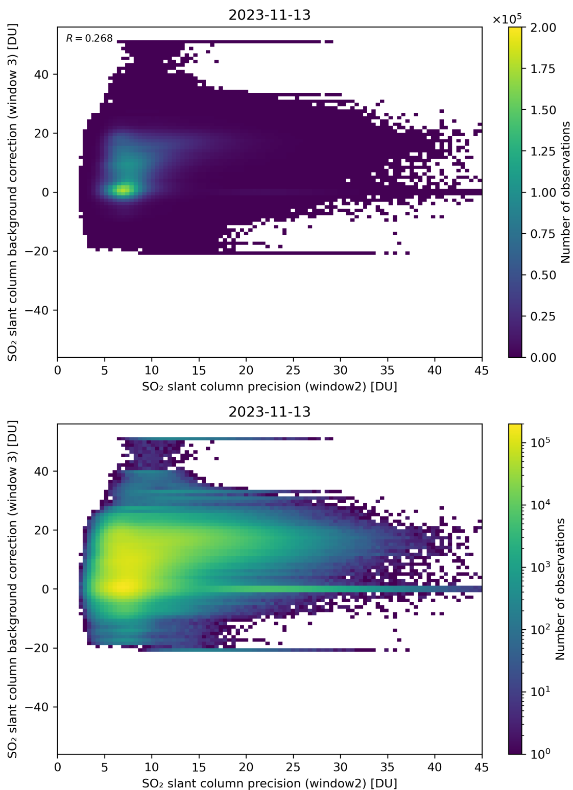
Figure 242: Scatter density plot of “SO 2 slant column precision (window2)” against “SO 2 slant column background correction (window 3)” for 2023-11-13 to 2023-11-14.
