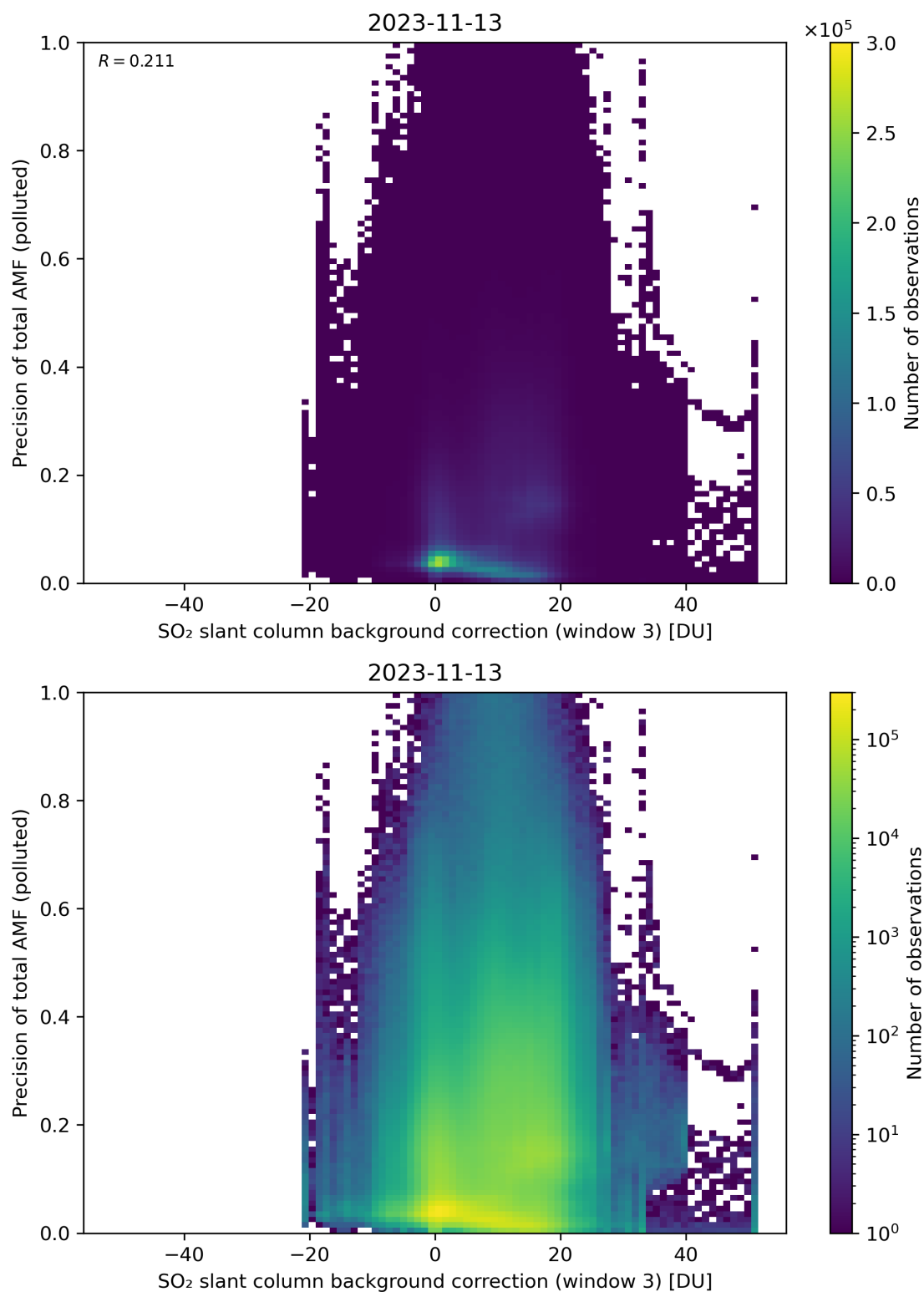
Figure 126: Scatter density plot of “SO 2 slant column background correction (window 3)” against “Precision of total AMF (polluted)” for 2023-11-13 to 2023-11-14.
