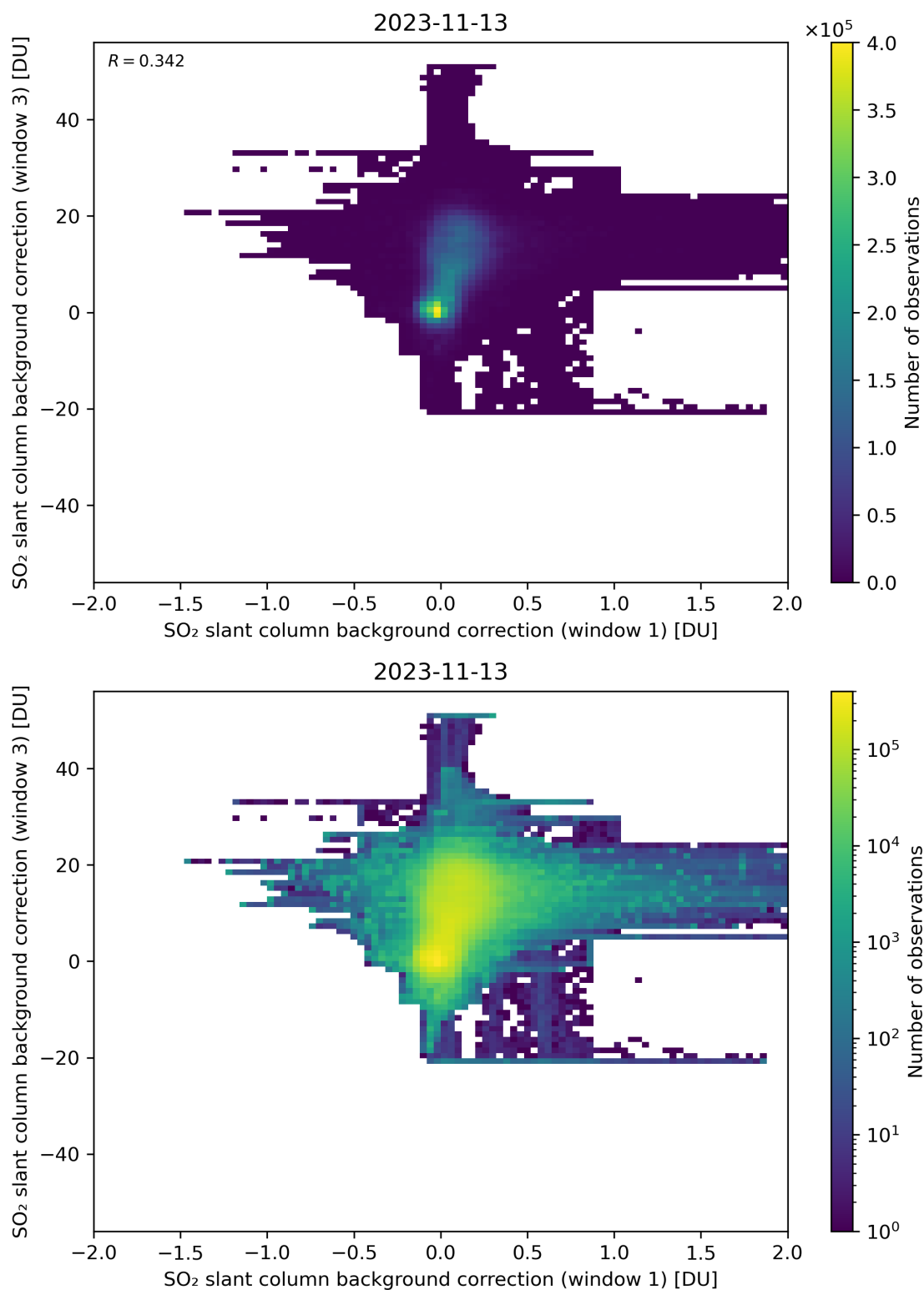
Figure 99: Scatter density plot of “SO 2 slant column background correction (window 1)” against “SO 2 slant column background correction (window 3)” for 2023-11-13 to 2023-11-14.
