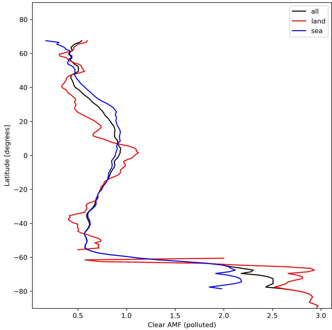
Figure 50: Zonal average of “Clear AMF (polluted)” for 2023-11-13 to 2023-11-14.
