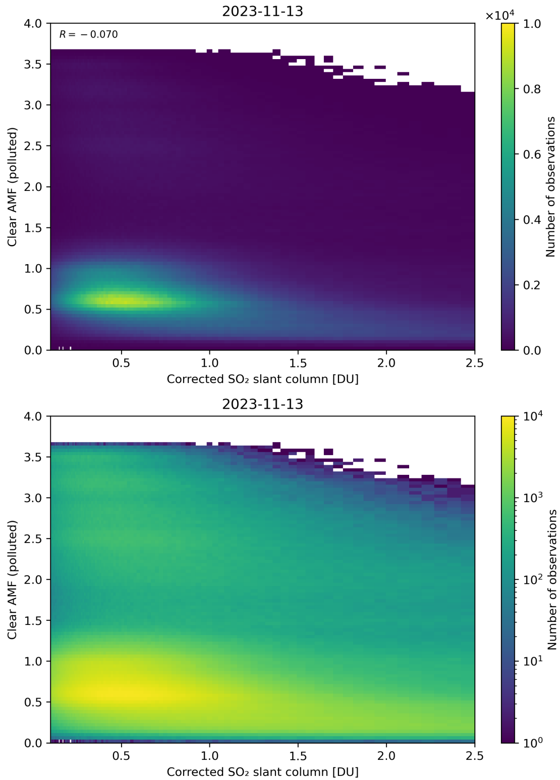
Figure 184: Scatter density plot of “Corrected SO 2 slant column” against “Clear AMF (polluted)” for 2023-11-13 to 2023-11-14.
