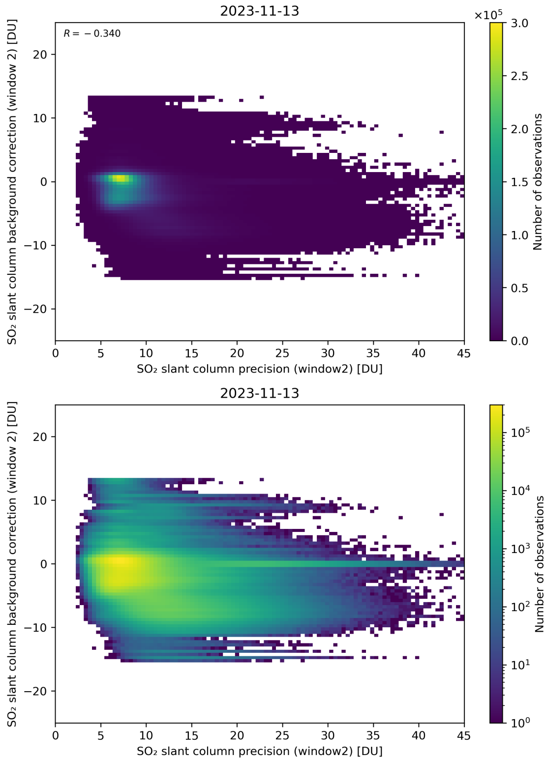
Figure 241: Scatter density plot of “SO 2 slant column precision (window2)” against “SO 2 slant column background correction (window 2)” for 2023-11-13 to 2023-11-14.
