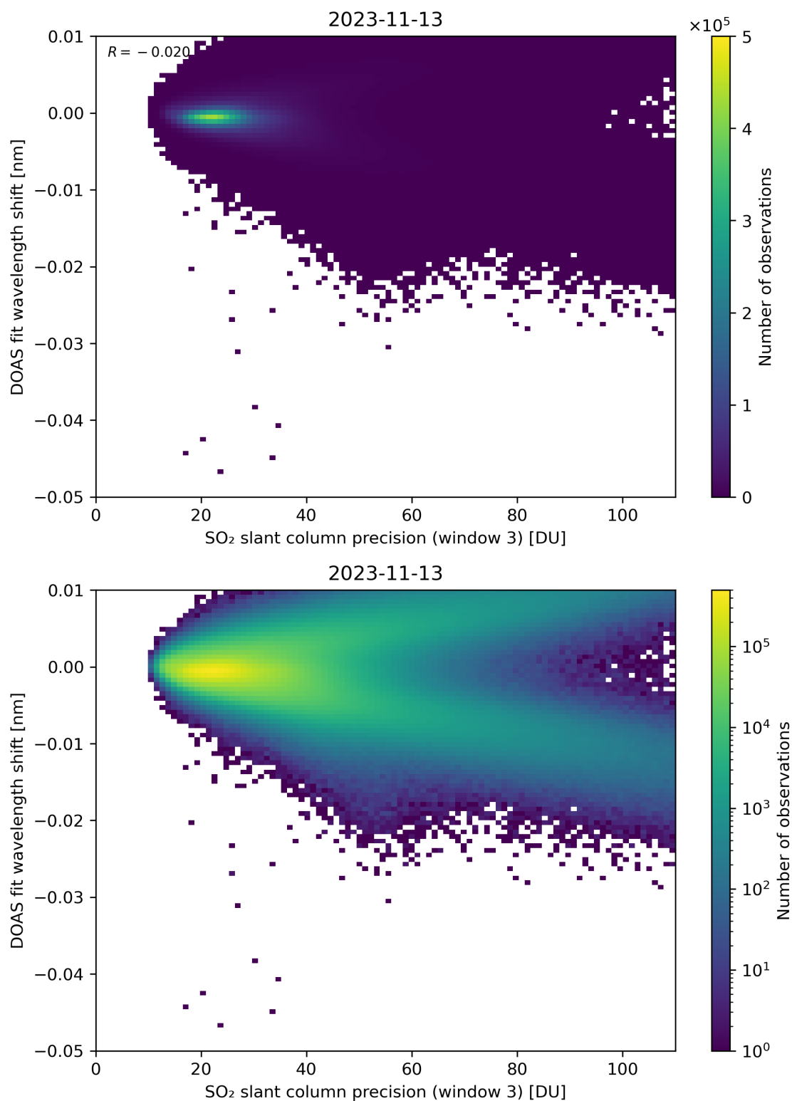
Figure 258: Scatter density plot of “SO 2 slant column precision (window 3)” against “DOAS fit wavelength shift” for 2023-11-13 to 2023-11-14.
