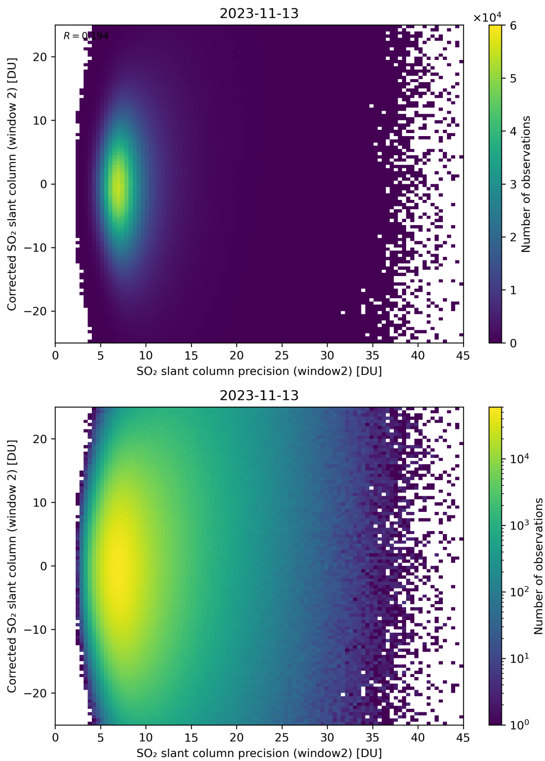
Figure 247: Scatter density plot of “SO 2 slant column precision (window2)” against “Corrected SO 2 slant column (window 2)” for 2023-11-13 to 2023-11-14.
