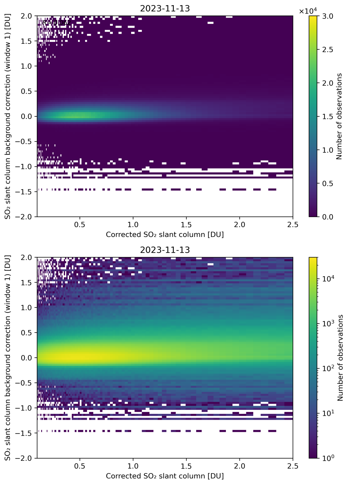
Figure 178: Scatter density plot of “Corrected SO 2 slant column” against “SO 2 slant column background correction (window 1)” for 2023-11-13 to 2023-11-14.
