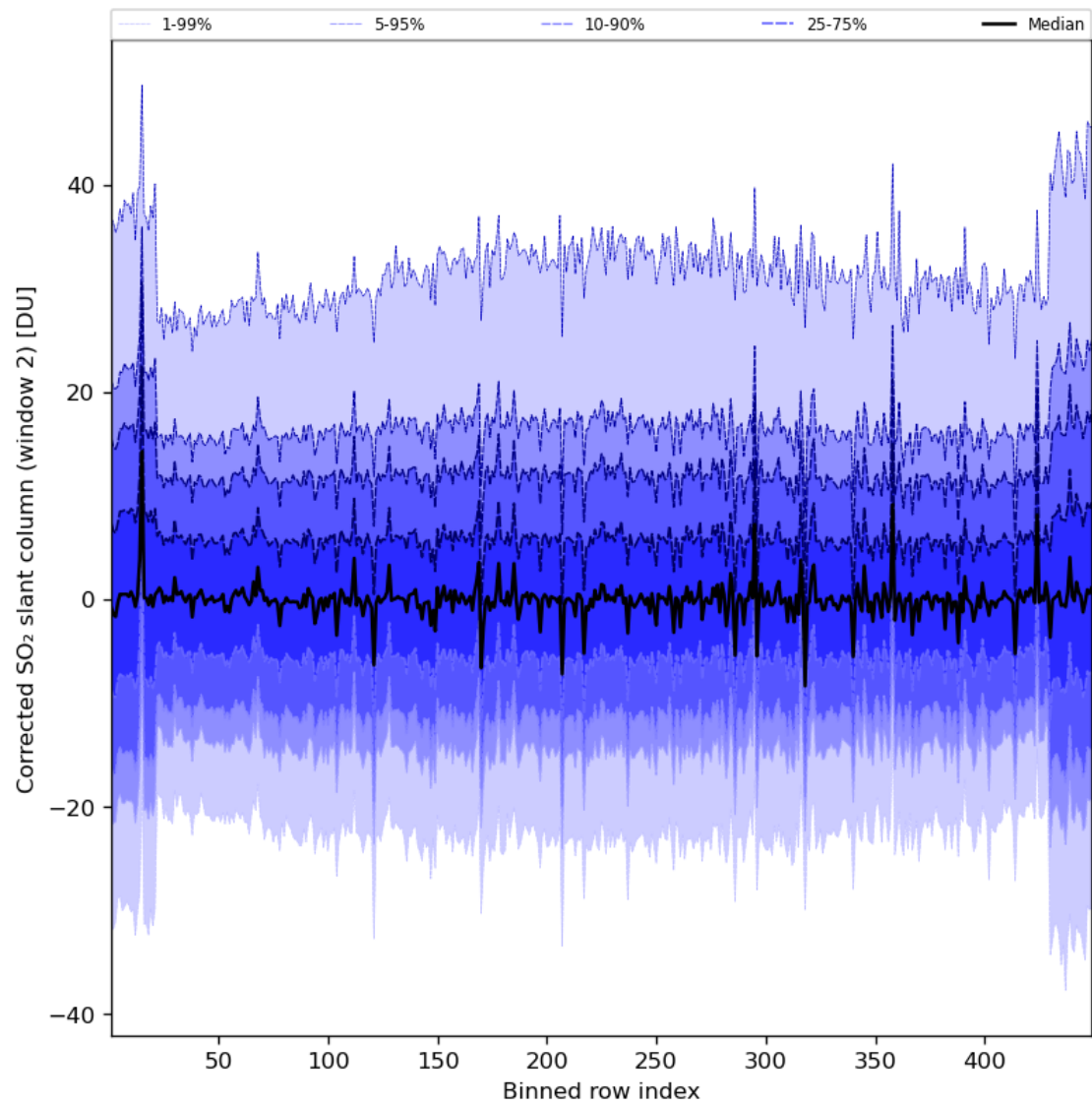
Figure 85: Along track statistics of “Corrected SO 2 slant column (window 2)” for 2023-11-13 to 2023-11-14
