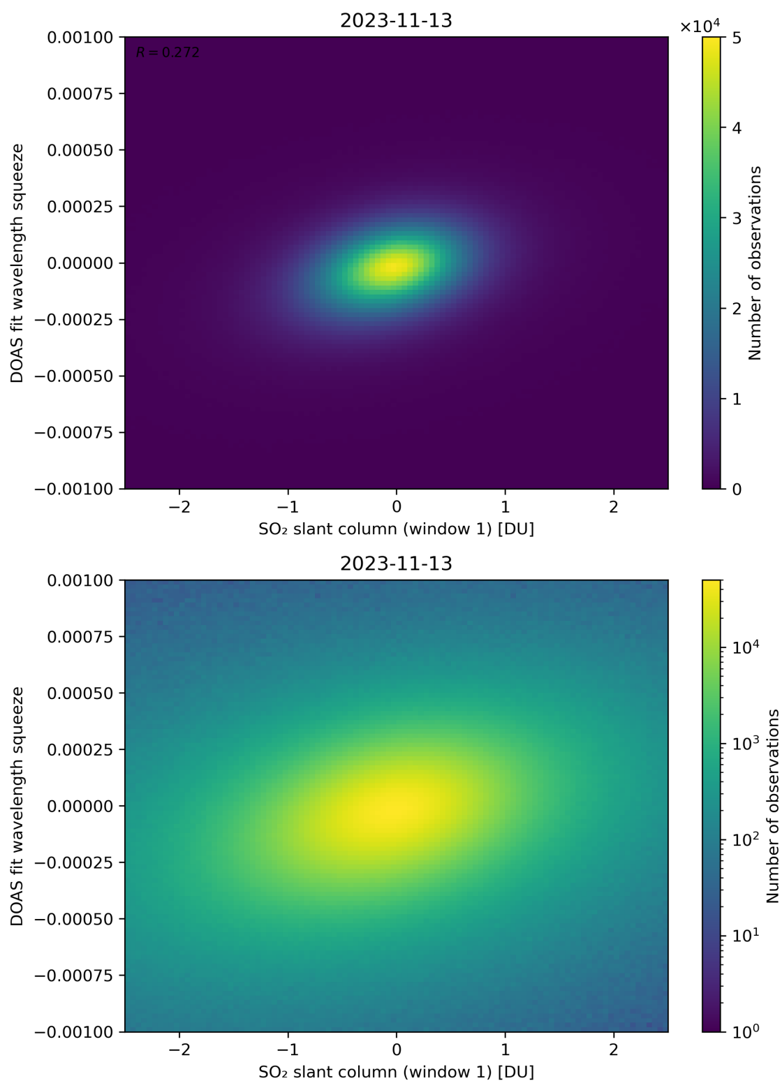
Figure 216: Scatter density plot of “SO 2 slant column (window 1)” against “DOAS fit wavelength squeeze” for 2023-11-13 to 2023-11-14.
