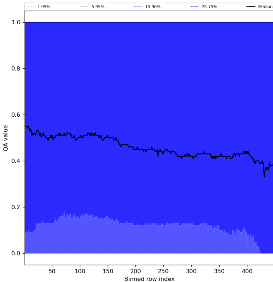
Figure 75: Along track statistics of “QA value” for 2023-11-13 to 2023-11-14
