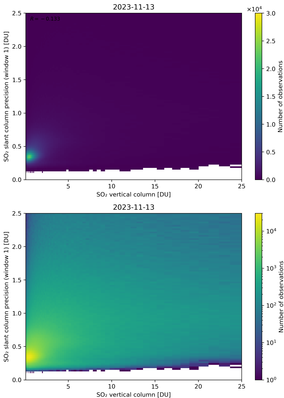
Figure 301: Scatter density plot of “SO 2 vertical column” against “SO 2 slant column precision (window 1)” for 2023-11-13 to 2023-11-14.
