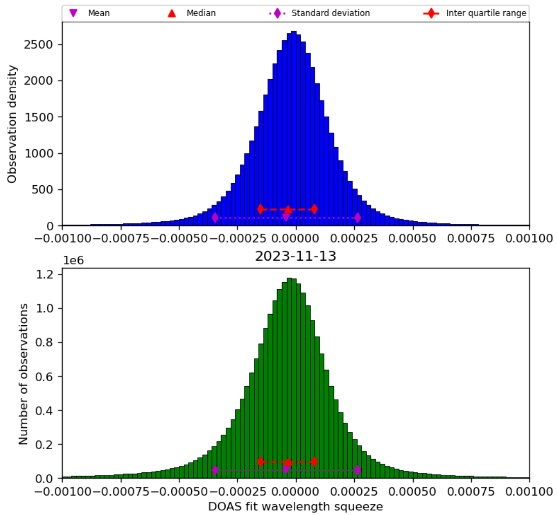
Figure 69: Histogram of “DOAS fit wavelength squeeze” for 2023-11-13 to 2023-11-14
