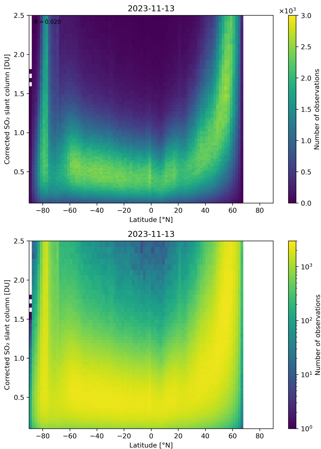
Figure 146: Scatter density plot of “Latitude” against “Corrected SO 2 slant column” for 2023-11-13 to 2023-11-14.
