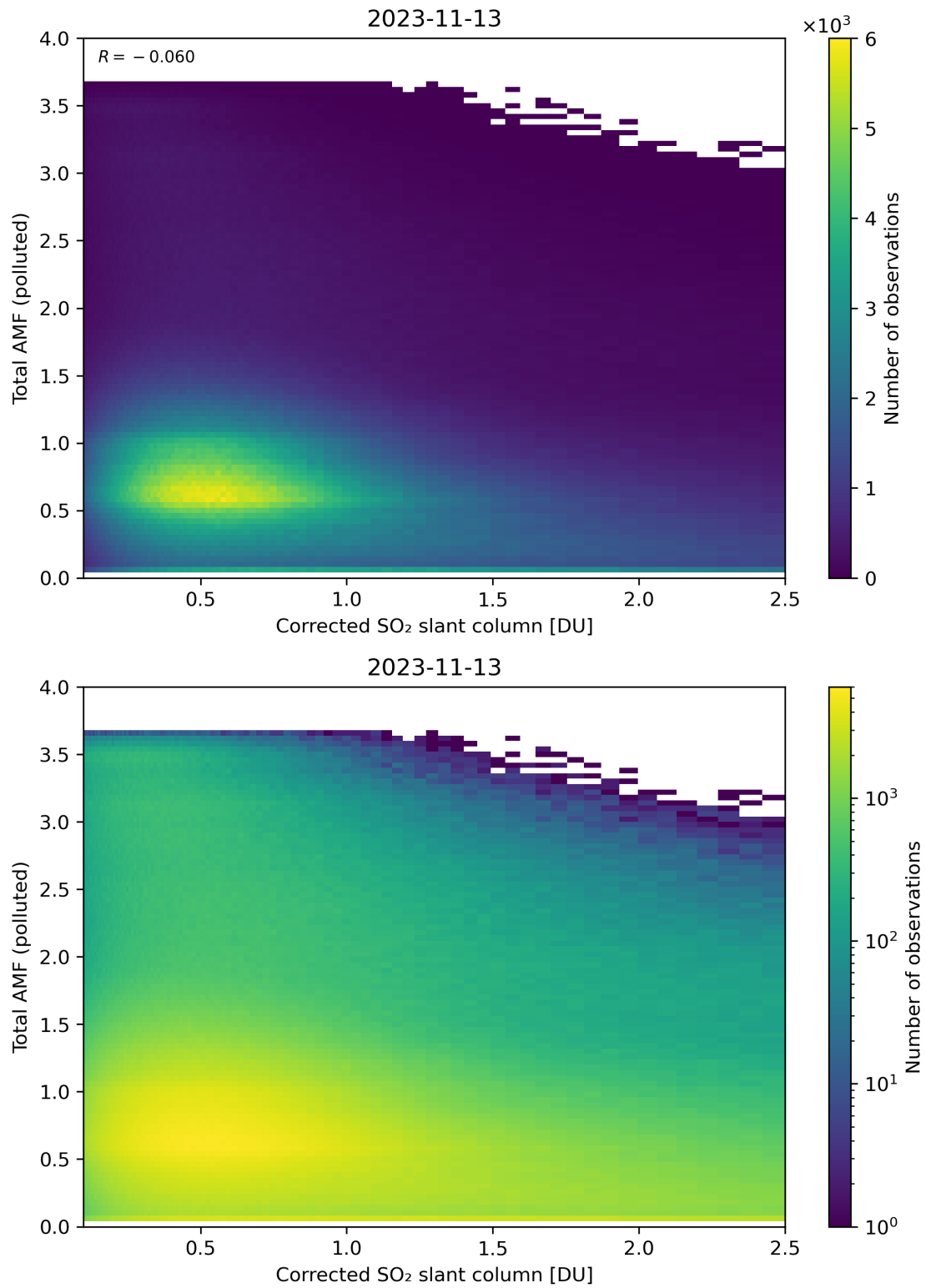
Figure 192: Scatter density plot of “Corrected SO 2 slant column” against “Total AMF (polluted)” for 2023-11-13 to 2023-11-14.
