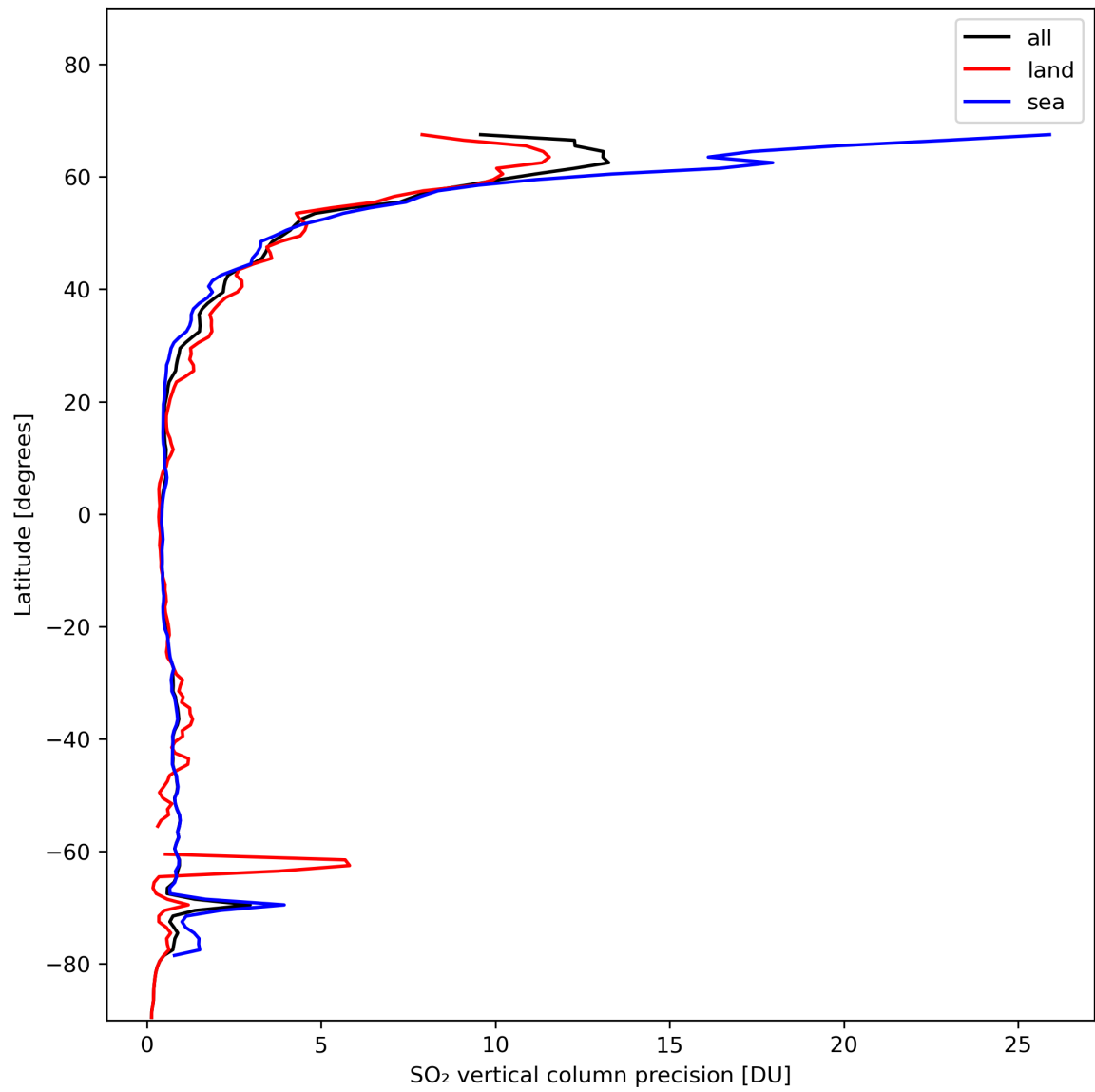
Figure 31: Zonal average of “SO 2 vertical column precision” for 2023-11-13 to 2023-11-14.
