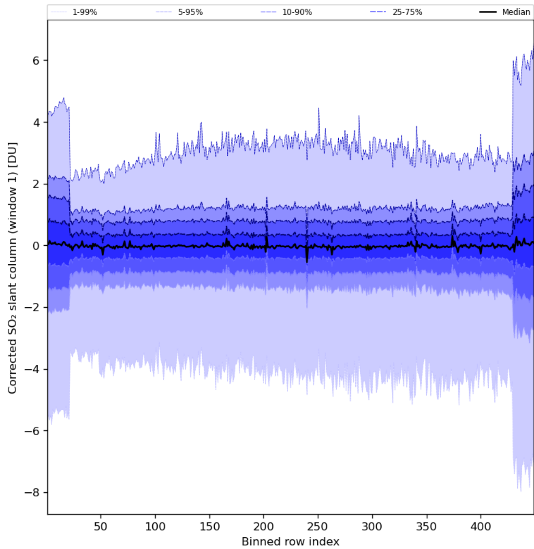
Figure 81: Along track statistics of “Corrected SO 2 slant column (window 1)” for 2023-11-13 to 2023-11-14
