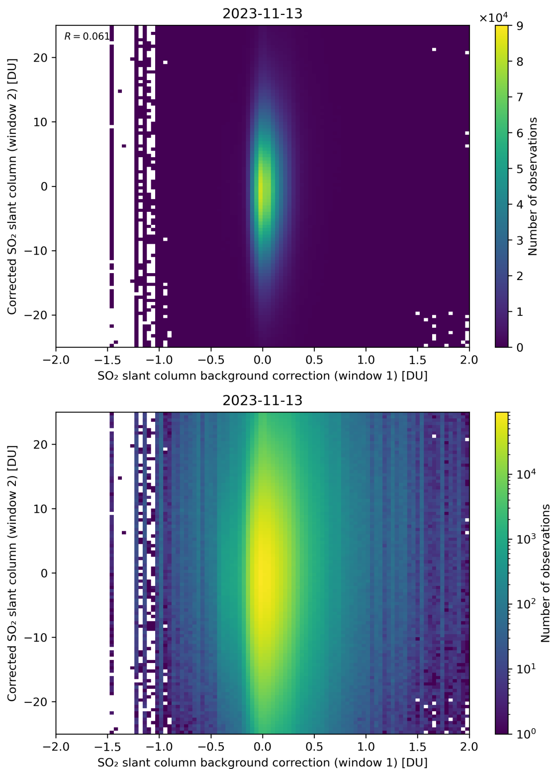
Figure 104: Scatter density plot of “SO 2 slant column background correction (window 1)” against “Corrected SO 2 slant column (window 2)” for 2023-11-13 to 2023-11-14.
