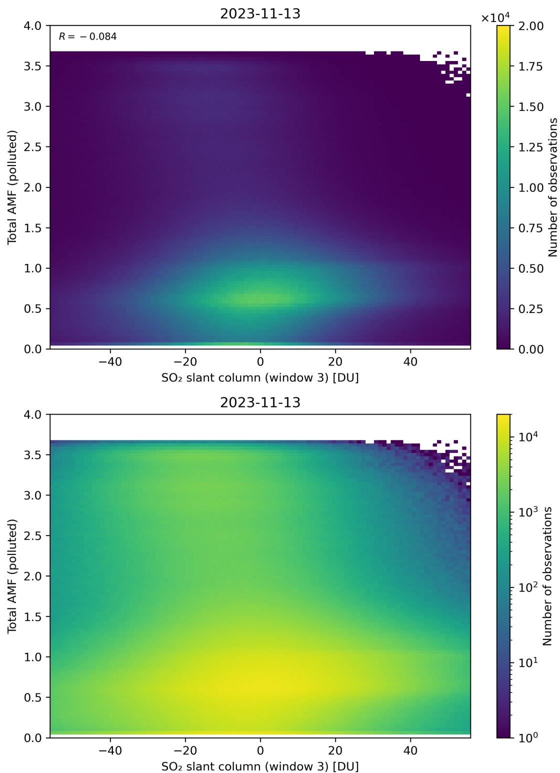
Figure 268: Scatter density plot of “SO 2 slant column (window 3)” against “Total AMF (polluted)” for 2023-11-13 to 2023-11-14.
