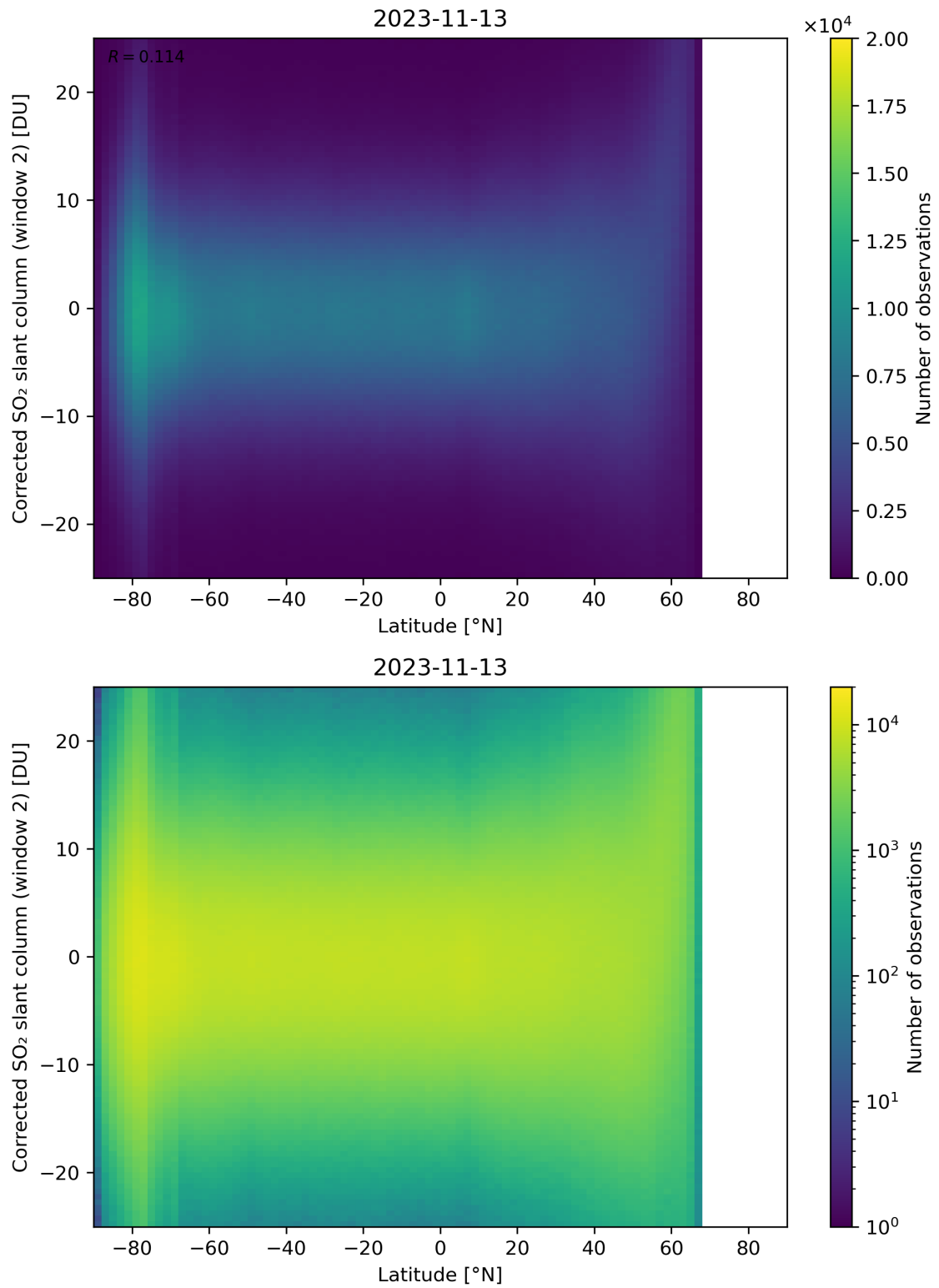
Figure 147: Scatter density plot of “Latitude” against “Corrected SO 2 slant column (window 2)” for 2023-11-13 to 2023-11-14.
