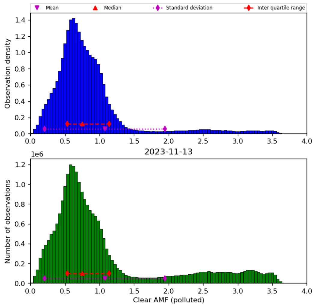
Figure 73: Histogram of “Clear AMF (polluted)” for 2023-11-13 to 2023-11-14
