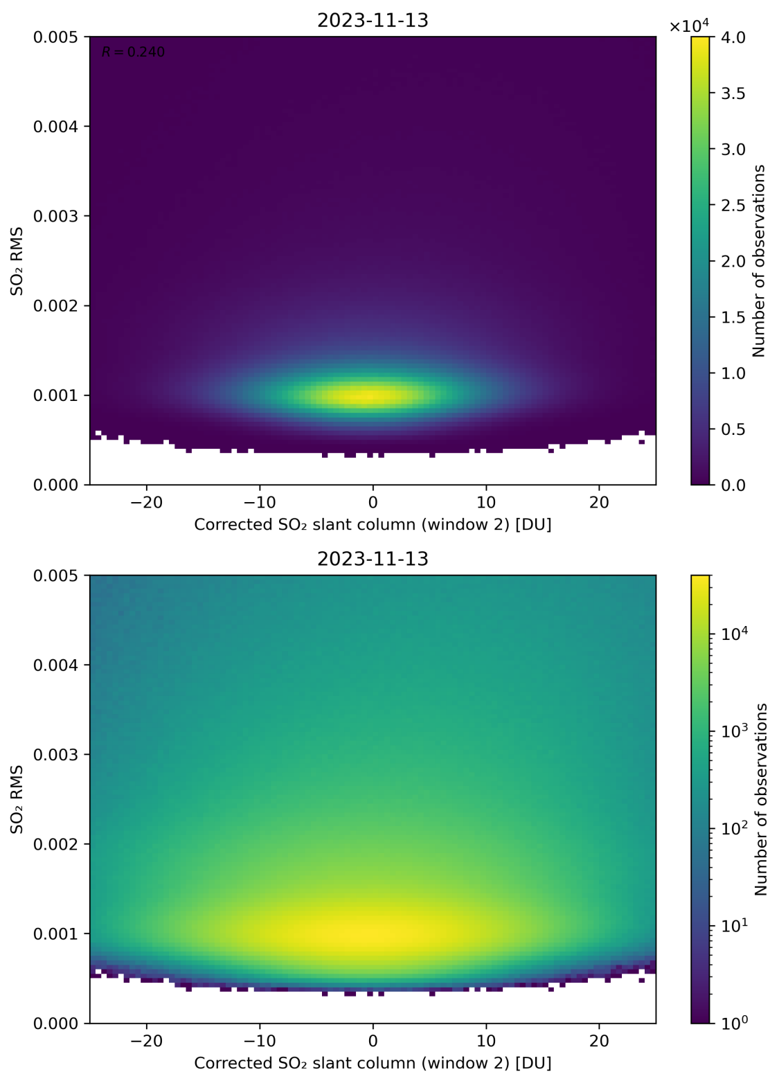
Figure 198: Scatter density plot of “Corrected SO 2 slant column (window 2)” against “SO 2 RMS” for 2023-11-13 to 2023-11-14.
