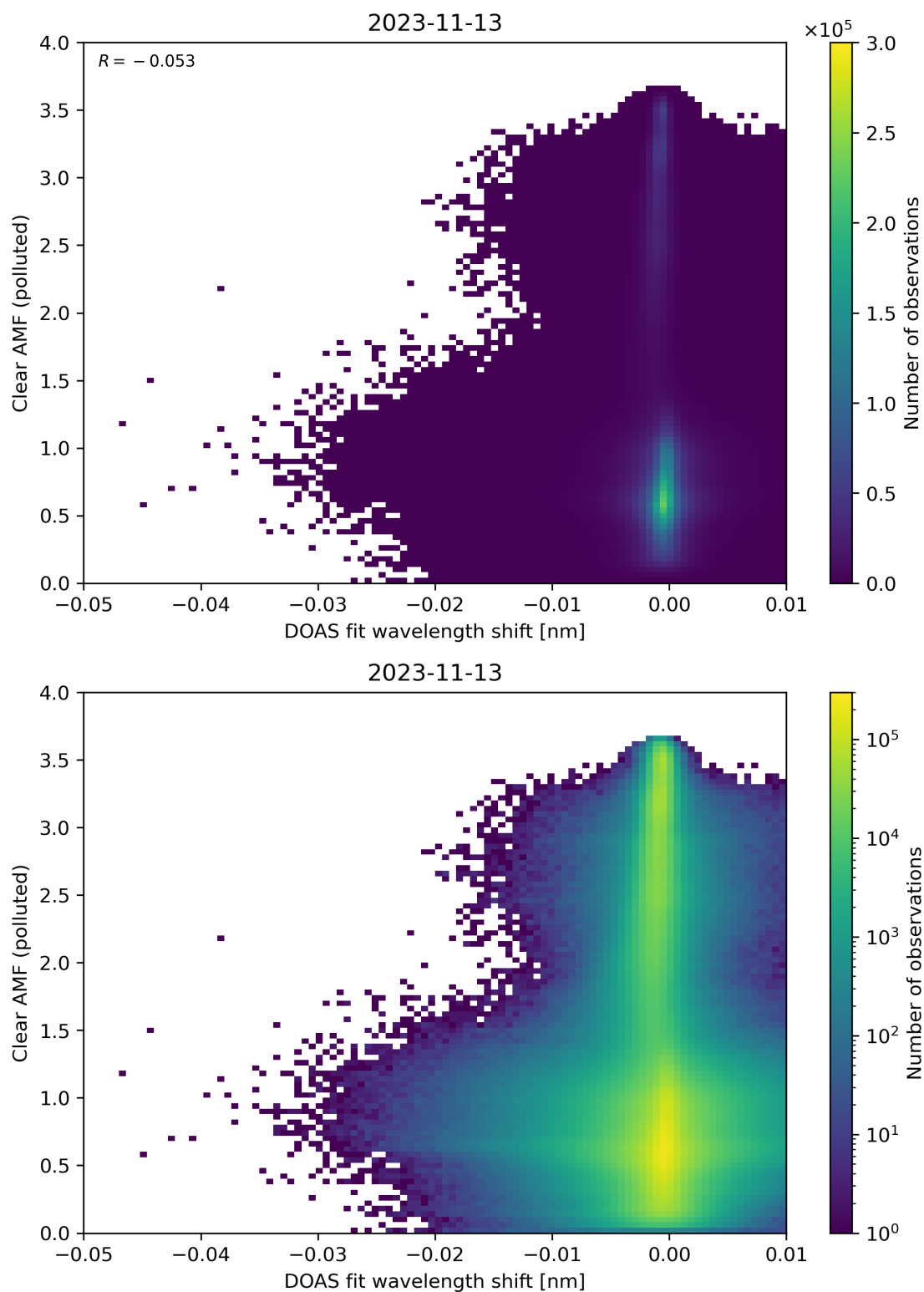
Figure 129: Scatter density plot of “DOAS fit wavelength shift” against “Clear AMF (polluted)” for 2023-11-13 to 2023-11-14.
