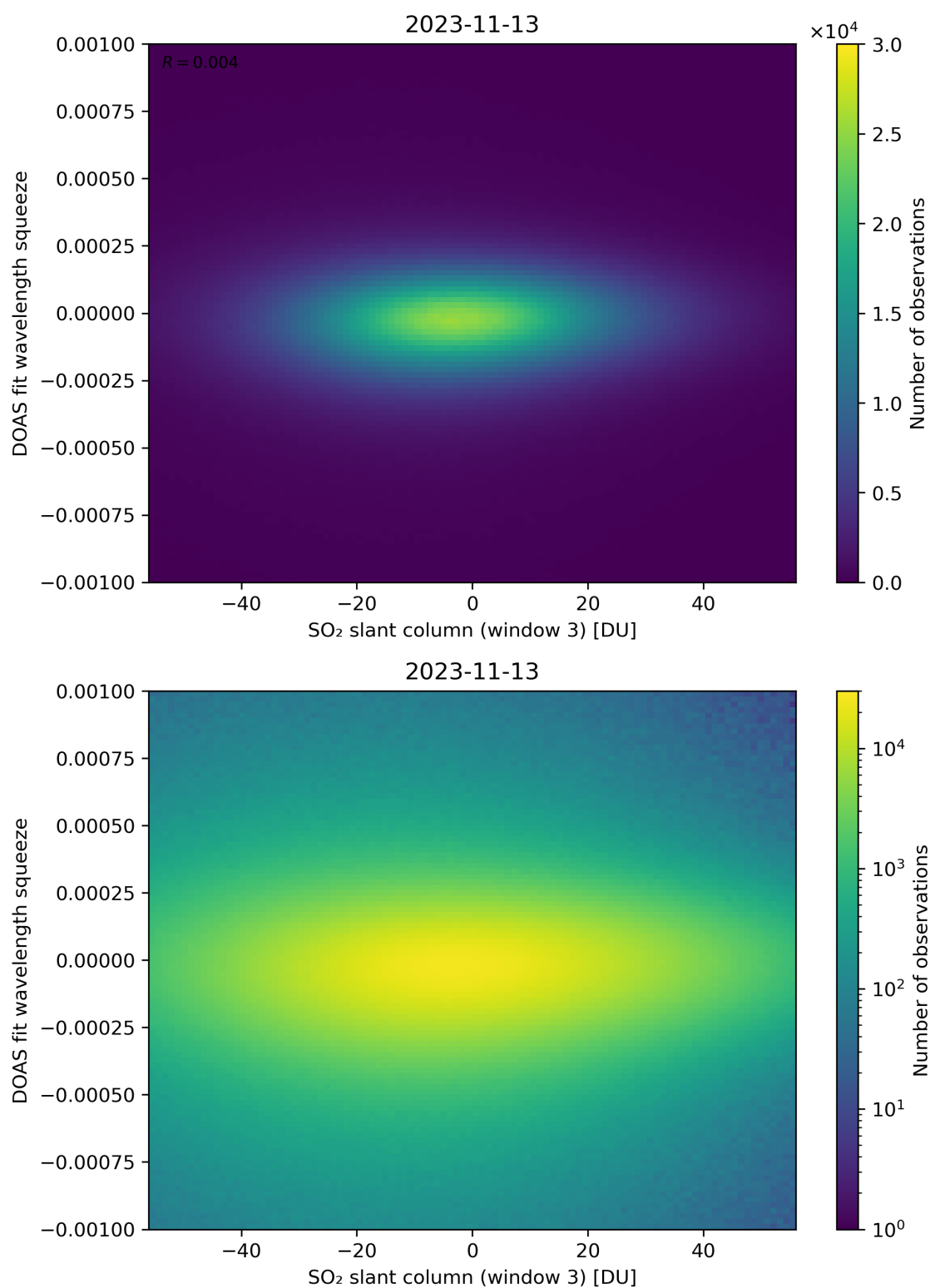
Figure 255: Scatter density plot of “SO 2 slant column (window 3)” against “DOAS fit wavelength squeeze” for 2023-11-13 to 2023-11-14.
