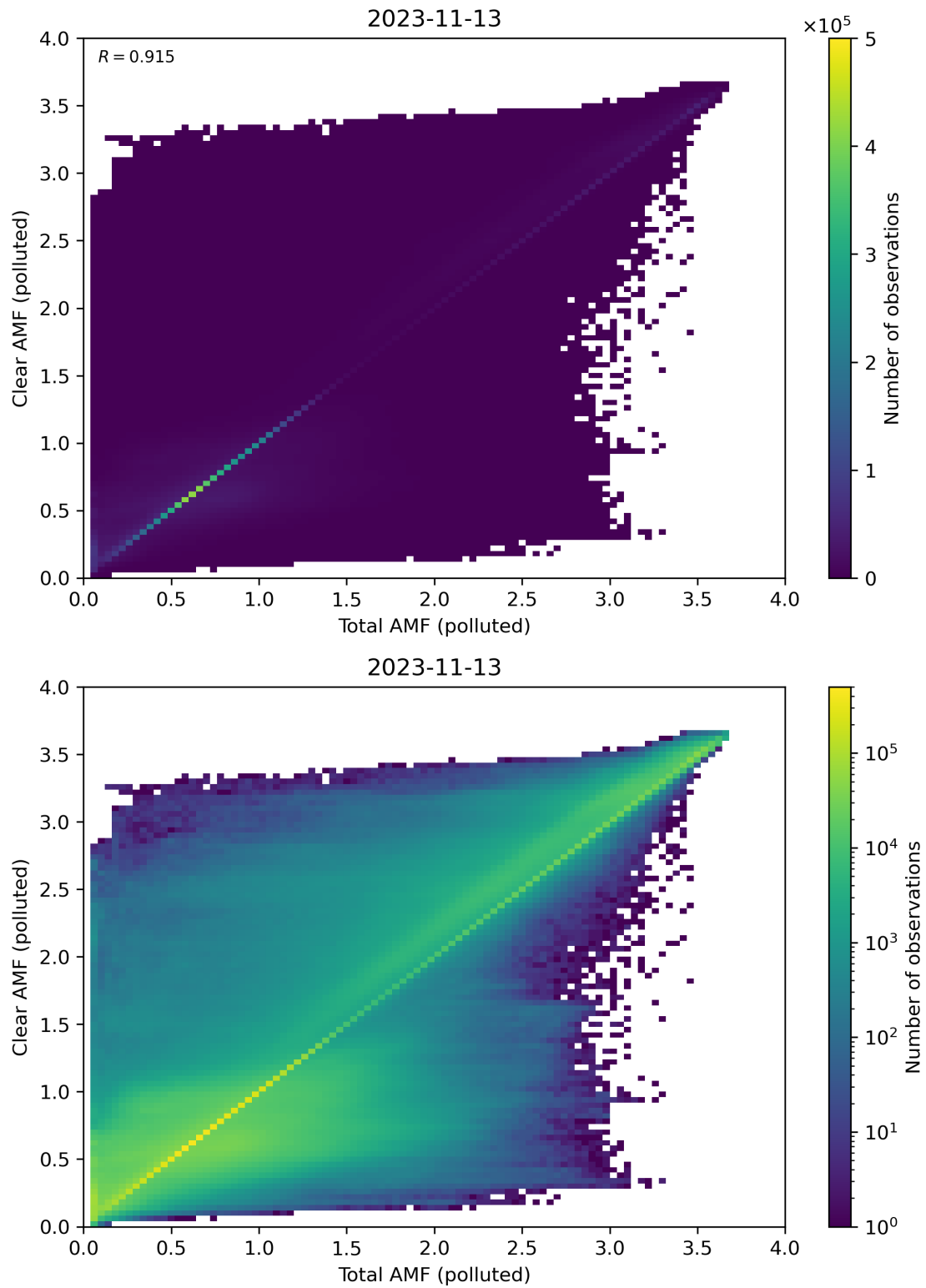
Figure 271: Scatter density plot of “Total AMF (polluted)” against “Clear AMF (polluted)” for 2023-11-13 to 2023-11-14.
