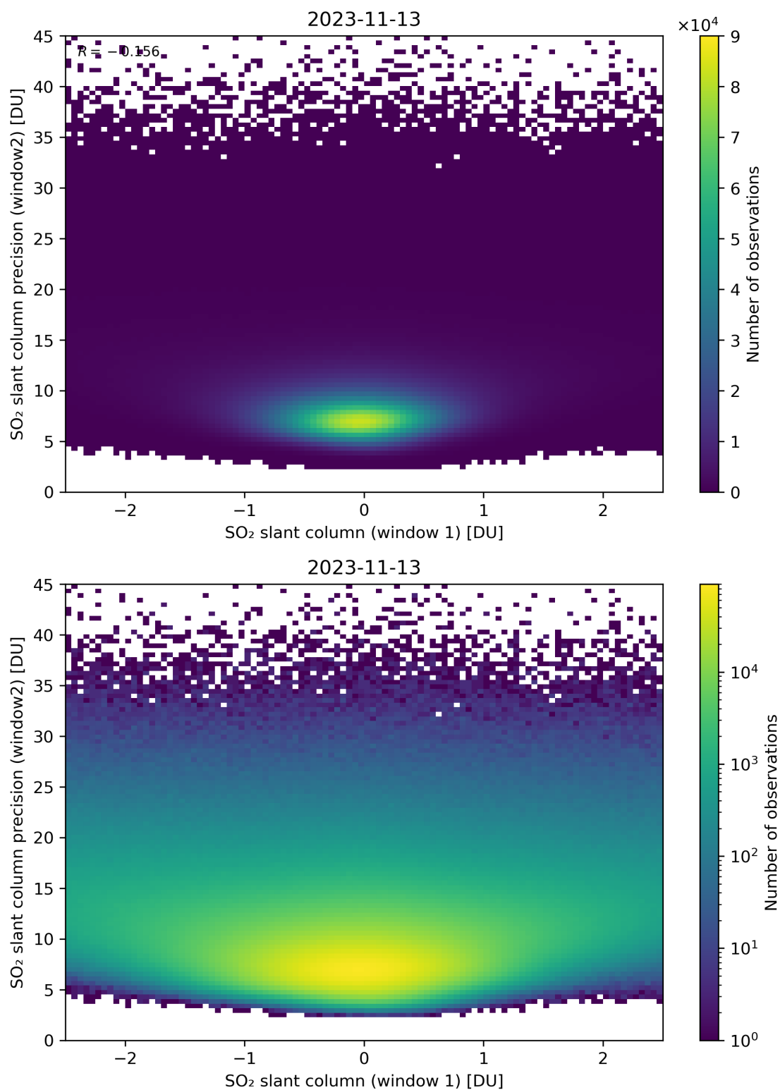
Figure 236: Scatter density plot of “SO 2 slant column (window 1)” against “SO 2 slant column precision (window2)” for 2023-11-13 to 2023-11-14.
