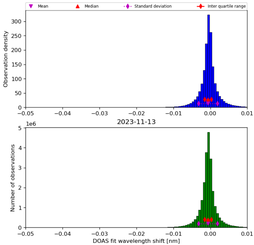
Figure 68: Histogram of “DOAS fit wavelength shift” for 2023-11-13 to 2023-11-14
