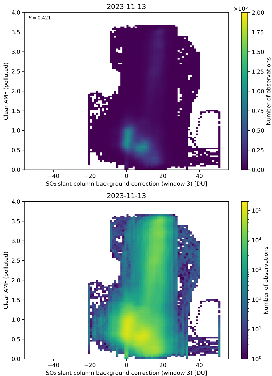
Figure 124: Scatter density plot of “SO 2 slant column background correction (window 3)” against “Clear AMF (polluted)” for 2023-11-13 to 2023-11-14.
