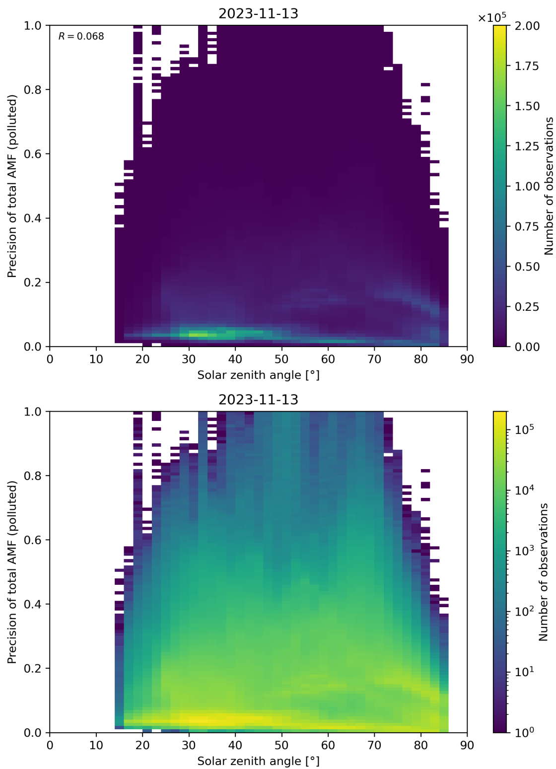
Figure 175: Scatter density plot of “Solar zenith angle” against “Precision of total AMF (polluted)” for 2023-11-13 to 2023-11-14.
