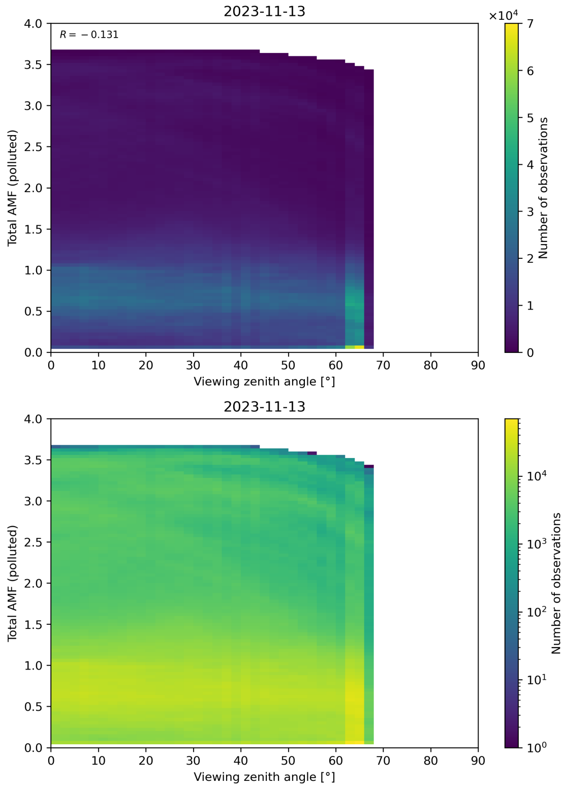
Figure 325: Scatter density plot of “Viewing zenith angle” against “Total AMF (polluted)” for 2023-11-13 to 2023-11-14.
