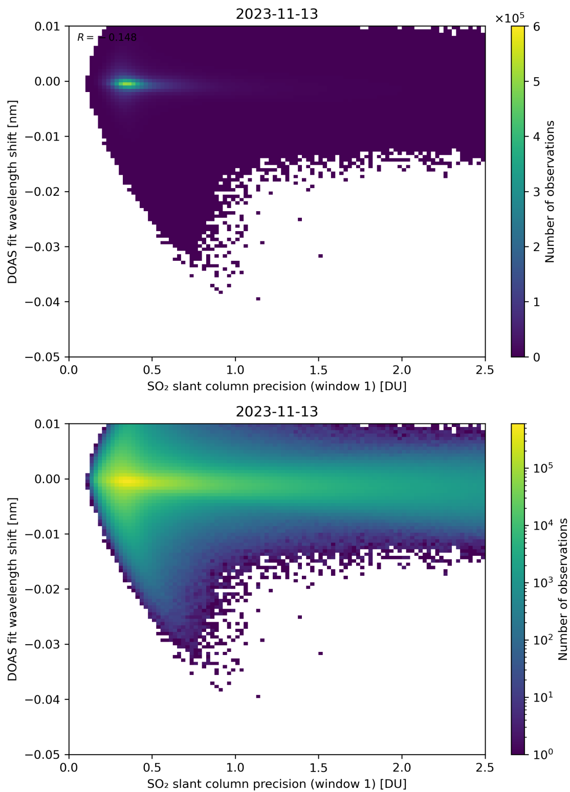
Figure 221: Scatter density plot of “SO 2 slant column precision (window 1)” against “DOAS fit wavelength shift” for 2023-11-13 to 2023-11-14.
