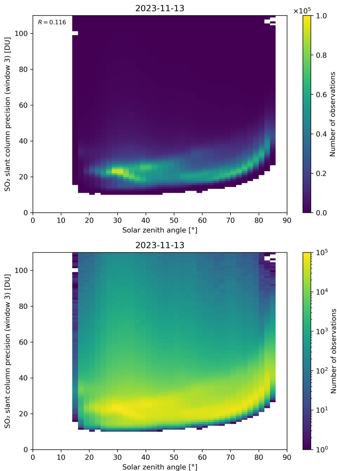
Figure 173: Scatter density plot of “Solar zenith angle” against “SO 2 slant column precision (window 3)” for 2023-11-13 to 2023-11-14.
