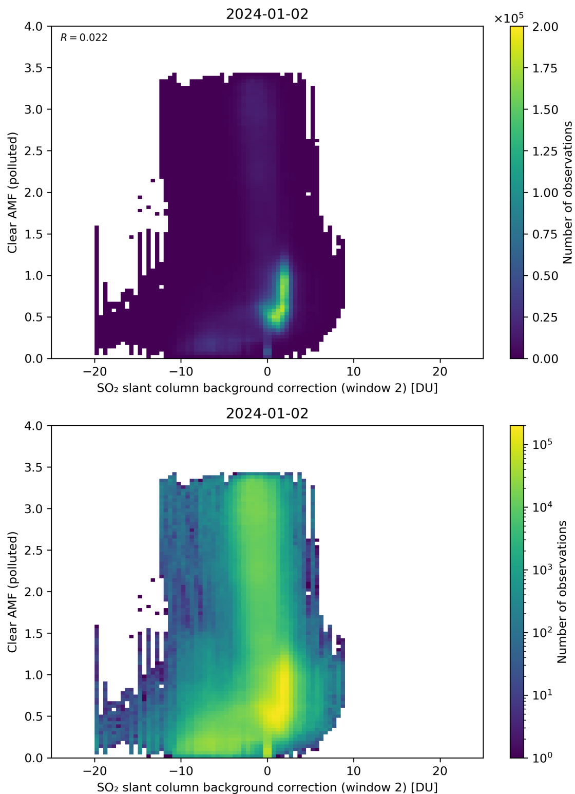
Figure 115: Scatter density plot of “SO 2 slant column background correction (window 2)” against “Clear AMF (polluted)” for 2024-01-01 to 2024-01-03.
