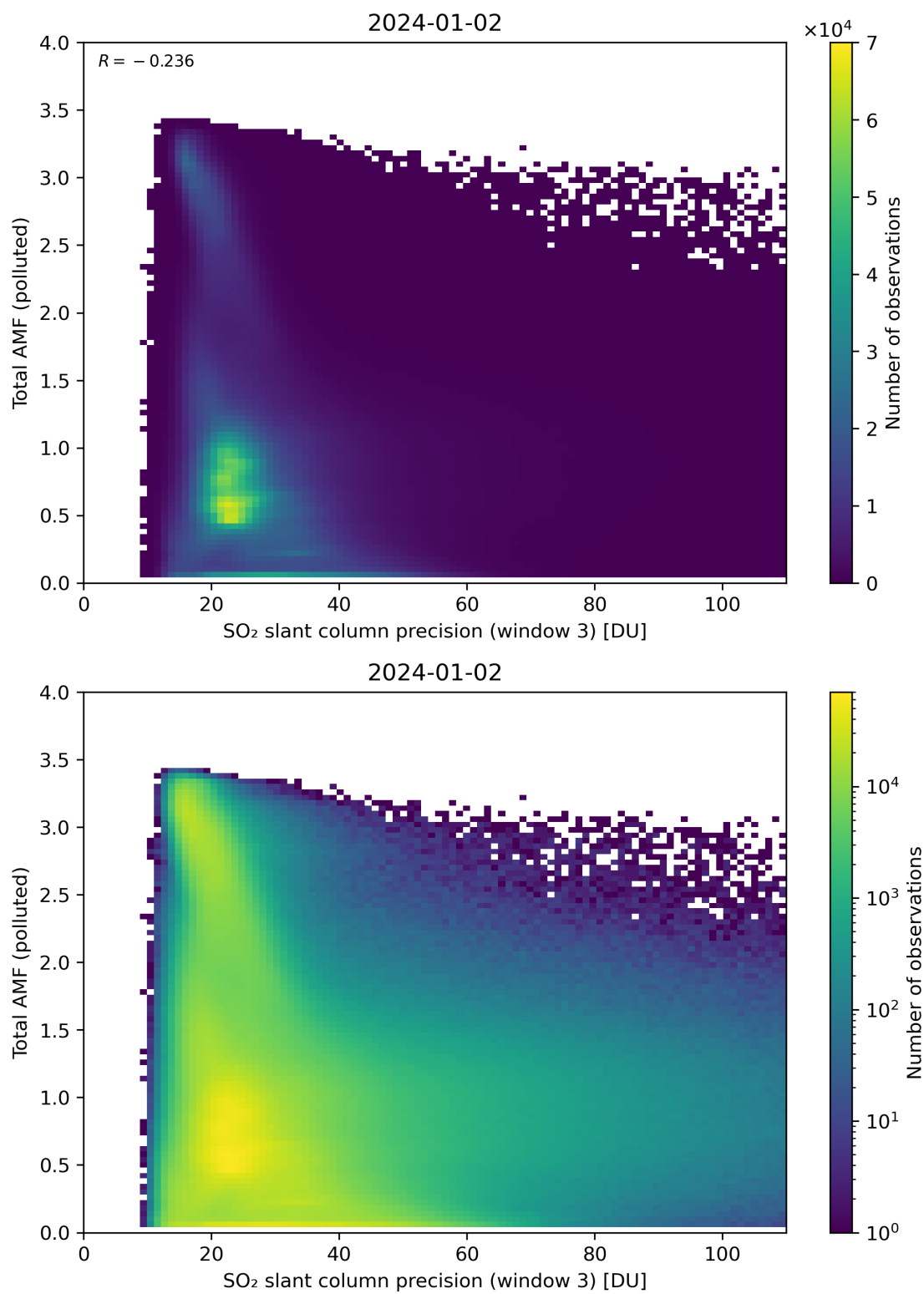
Figure 263: Scatter density plot of “SO 2 slant column precision (window 3)” against “Total AMF (polluted)” for 2024-01-01 to 2024-01-03.
