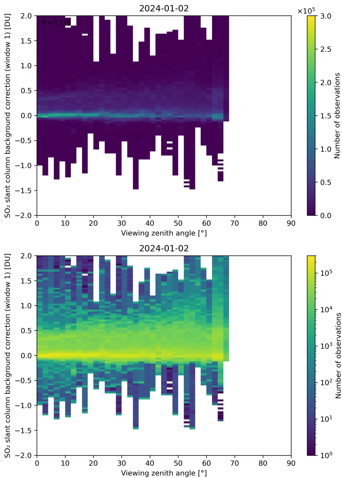
Figure 308: Scatter density plot of “Viewing zenith angle” against “SO 2 slant column background correction (window 1)” for 2024-01-01 to 2024-01-03.
