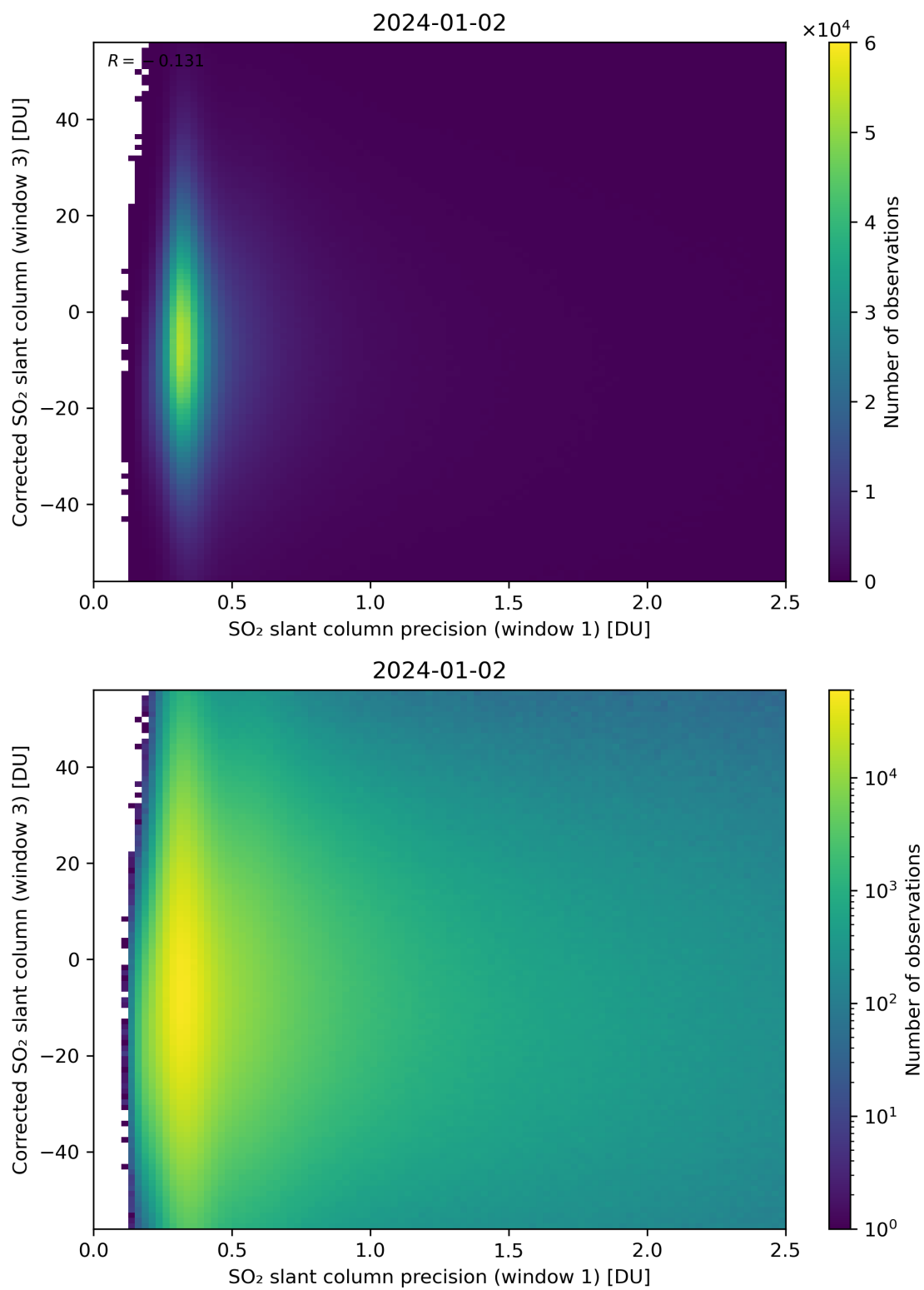
Figure 226: Scatter density plot of “SO 2 slant column precision (window 1)” against “Corrected SO 2 slant column (window 3)” for 2024-01-01 to 2024-01-03.
