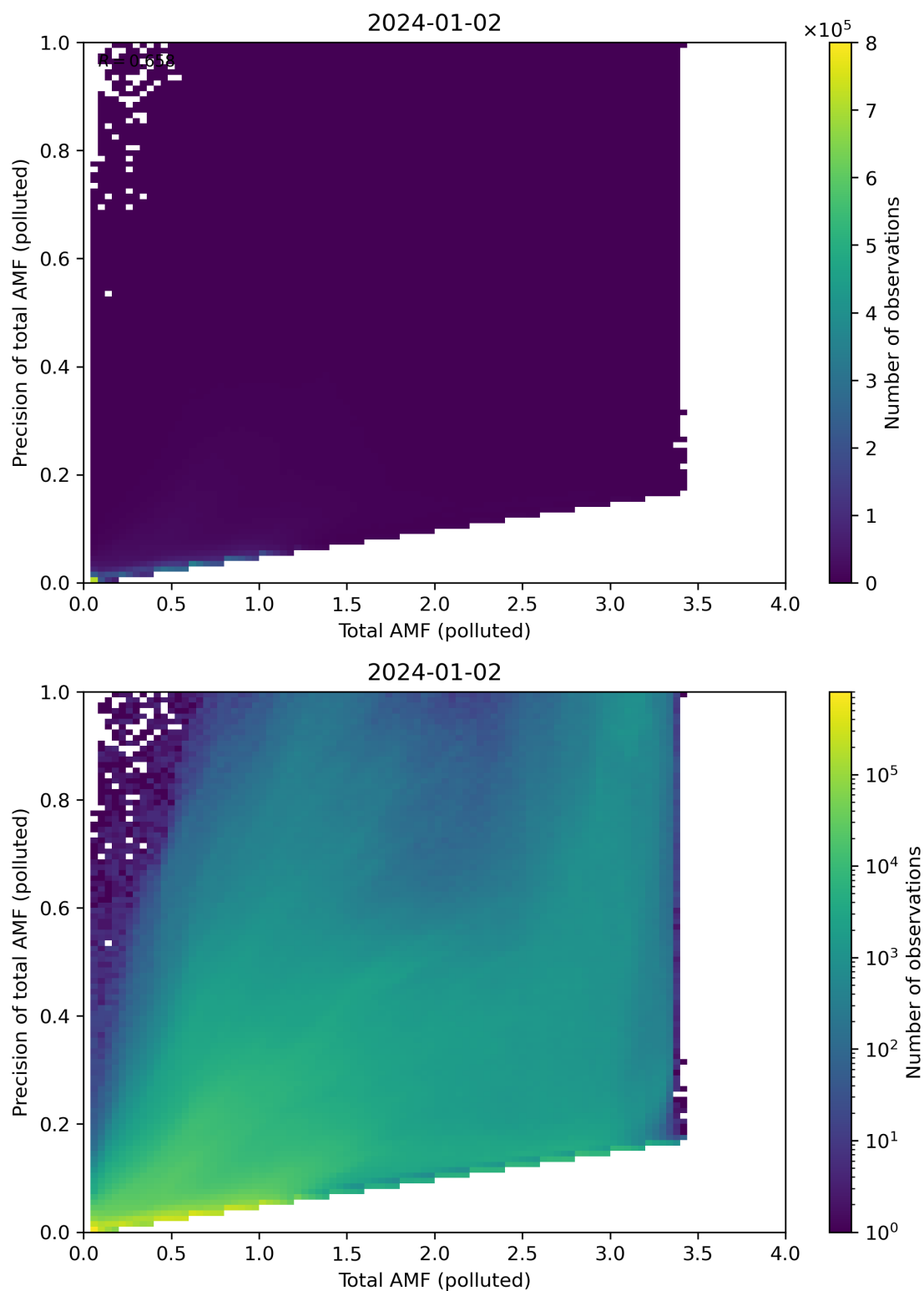
Figure 272: Scatter density plot of “Total AMF (polluted)” against “Precision of total AMF (polluted)” for 2024-01-01 to 2024-01-03.
