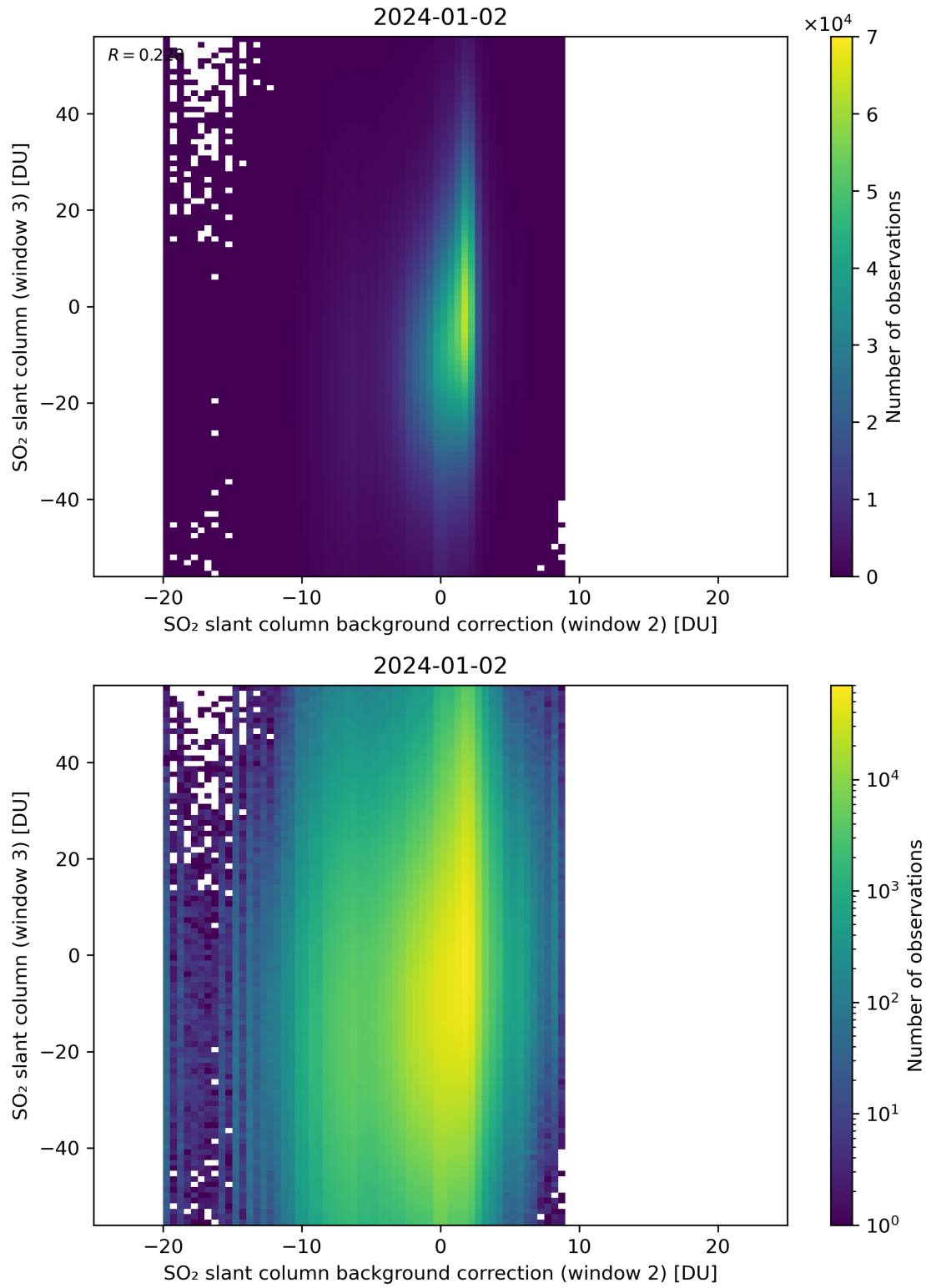
Figure 117: Scatter density plot of “SO 2 slant column background correction (window 2)” against “SO 2 slant column (window 3)” for 2024-01-01 to 2024-01-03.
