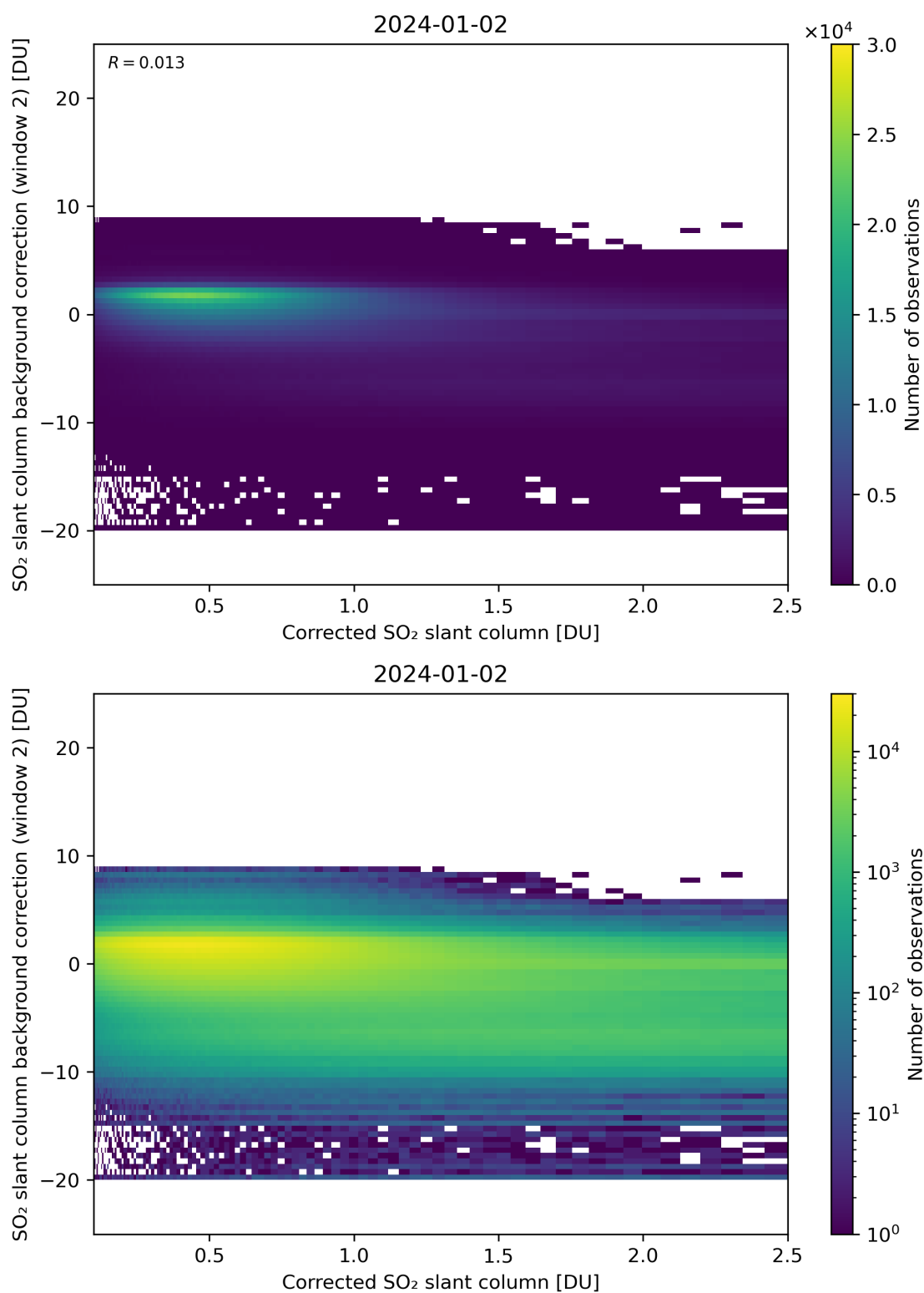
Figure 179: Scatter density plot of “Corrected SO 2 slant column” against “SO 2 slant column background correction (window 2)” for 2024-01-01 to 2024-01-03.
