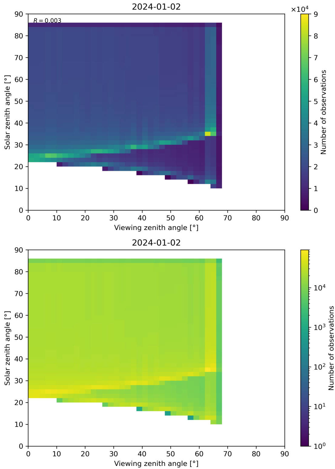
Figure 315: Scatter density plot of “Viewing zenith angle” against “Solar zenith angle” for 2024-01-01 to 2024-01-03.
