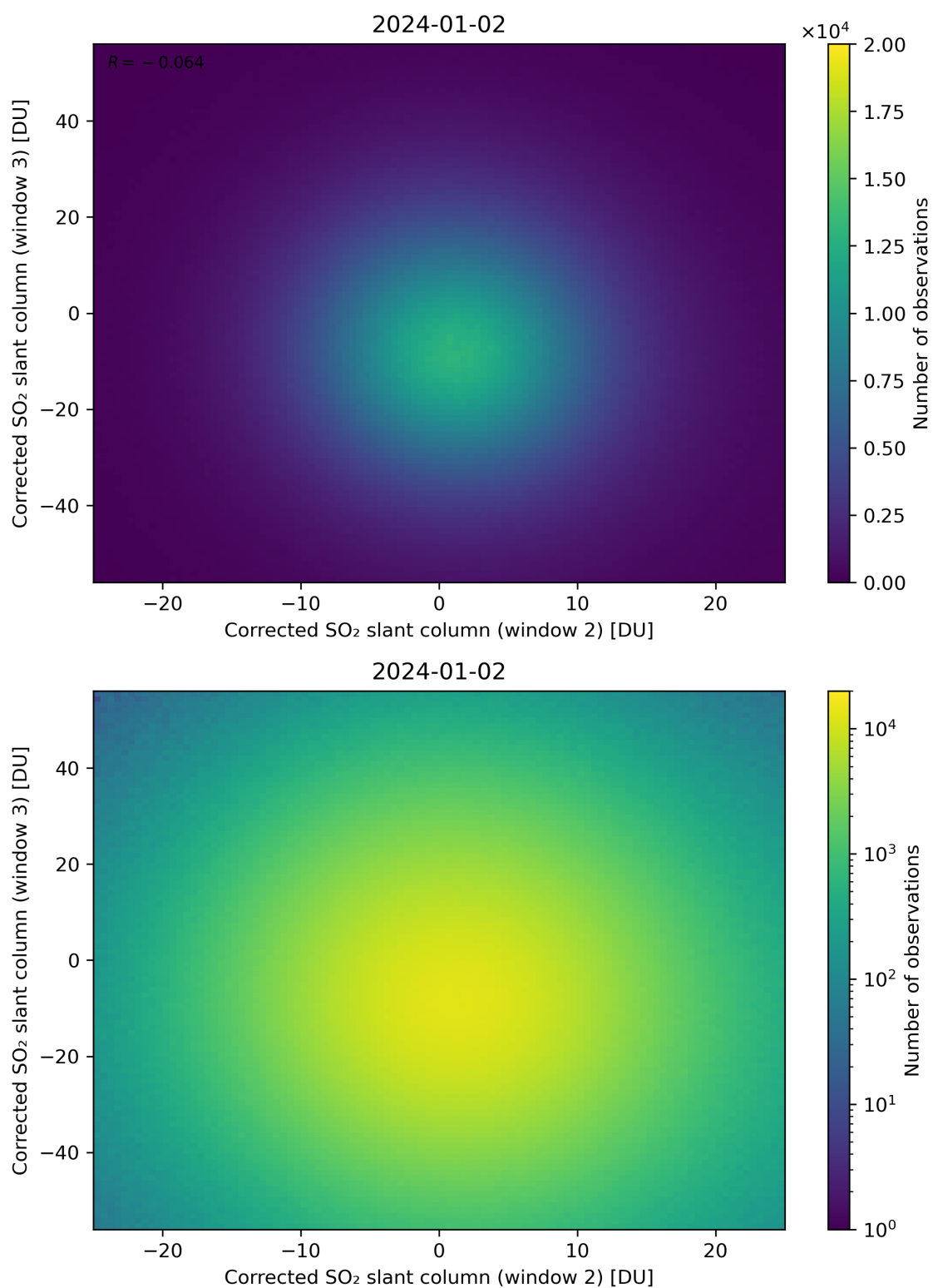
Figure 200: Scatter density plot of “Corrected SO 2 slant column (window 2)” against “Corrected SO 2 slant column (window 3)” for 2024-01-01 to 2024-01-03.
