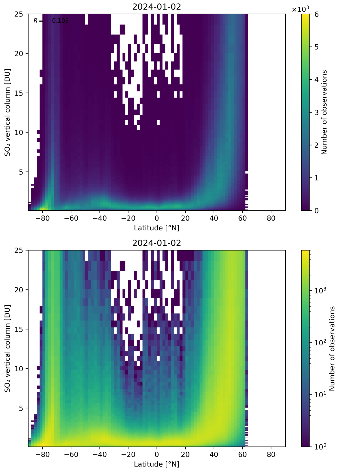
Figure 156: Scatter density plot of “Latitude” against “SO 2 vertical column” for 2024-01-01 to 2024-01-03.
