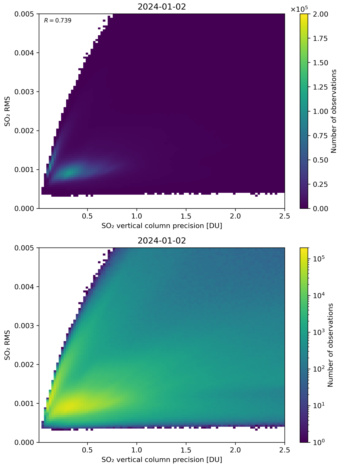
Figure 284: Scatter density plot of “SO 2 vertical column precision” against “SO 2 RMS” for 2024-01-01 to 2024-01-03.
