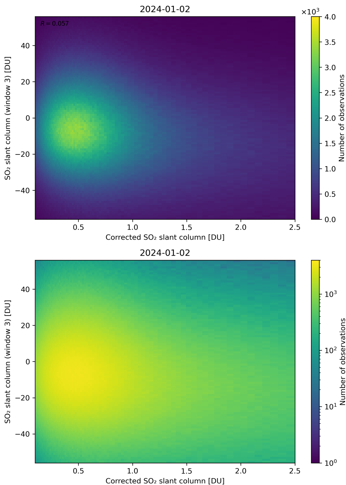
Figure 190: Scatter density plot of “Corrected SO 2 slant column” against “SO 2 slant column (window 3)” for 2024-01-01 to 2024-01-03.
