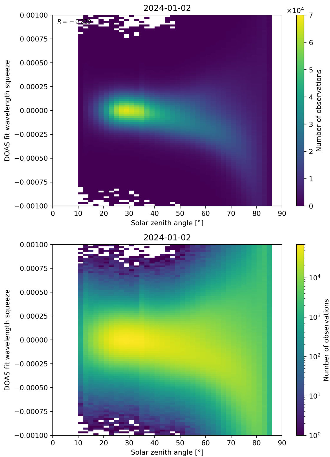
Figure 162: Scatter density plot of “Solar zenith angle” against “DOAS fit wavelength squeeze” for 2024-01-01 to 2024-01-03.
