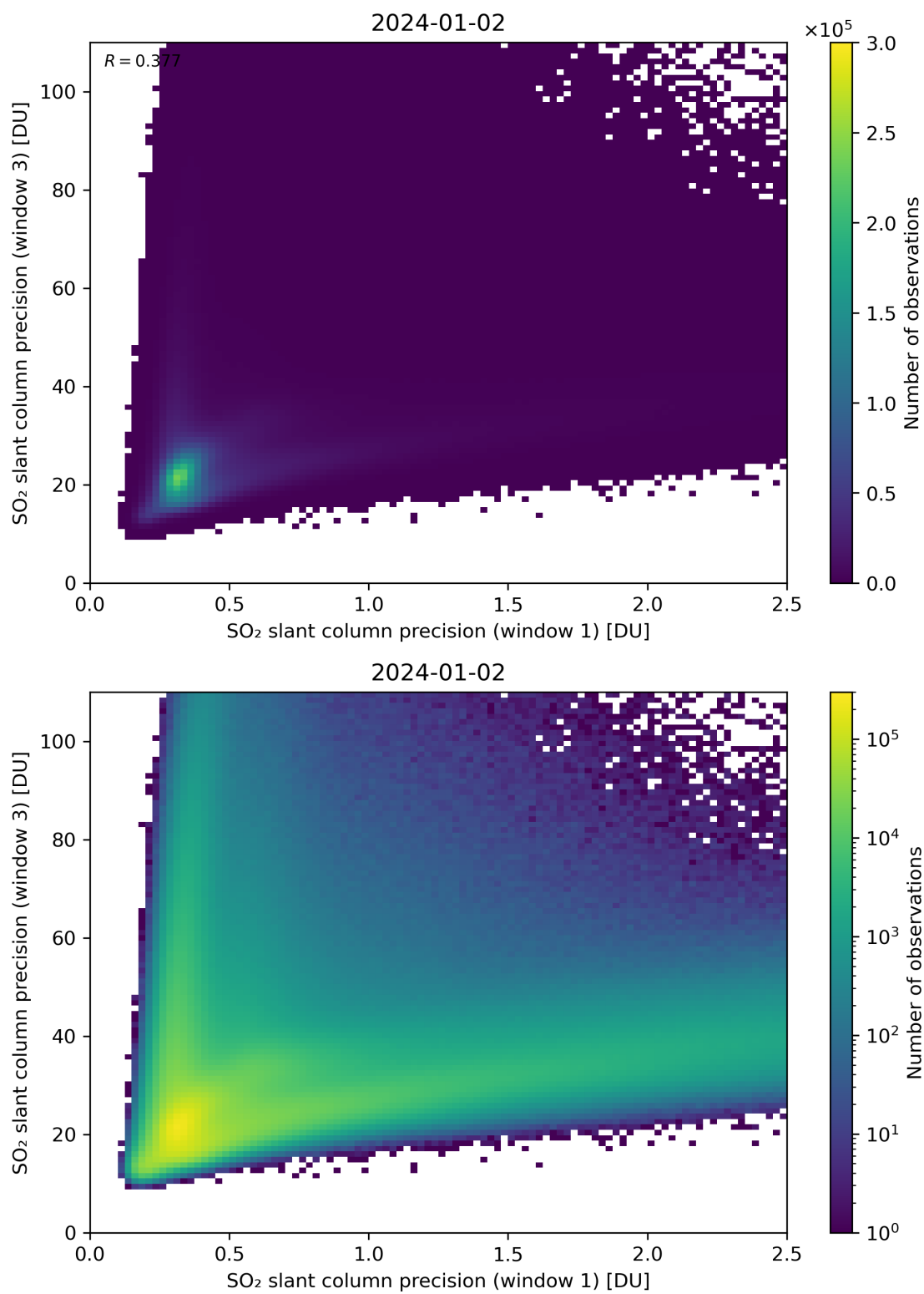
Figure 229: Scatter density plot of “SO 2 slant column precision (window 1)” against “SO 2 slant column precision (window 3)” for 2024-01-01 to 2024-01-03.
