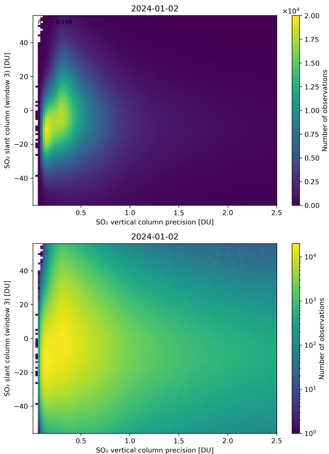
Figure 292: Scatter density plot of “SO 2 vertical column precision” against “SO 2 slant column (window 3)” for 2024-01-01 to 2024-01-03.
