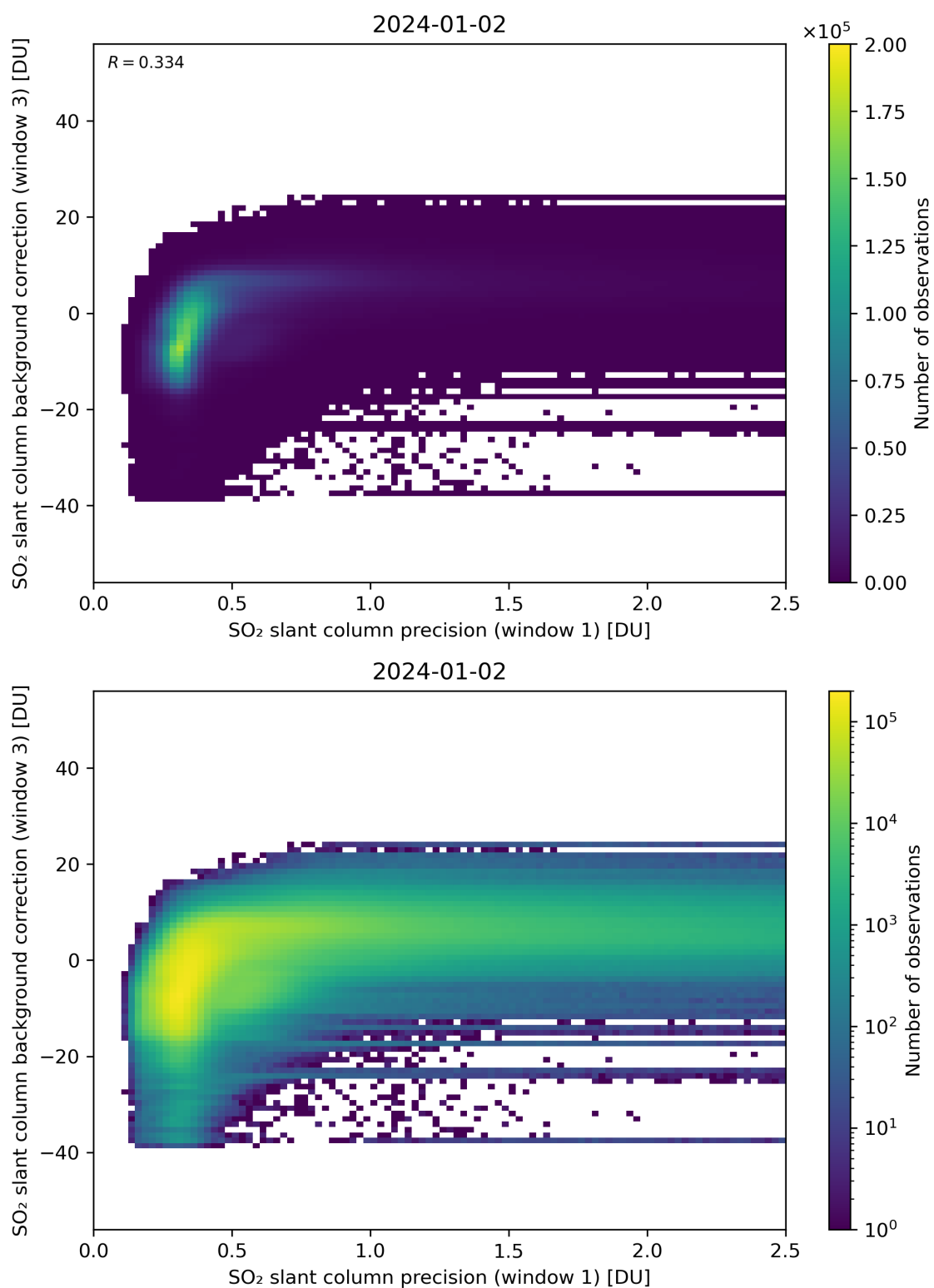
Figure 220: Scatter density plot of “SO 2 slant column precision (window 1)” against “SO 2 slant column background correction (window 3)” for 2024-01-01 to 2024-01-03.
