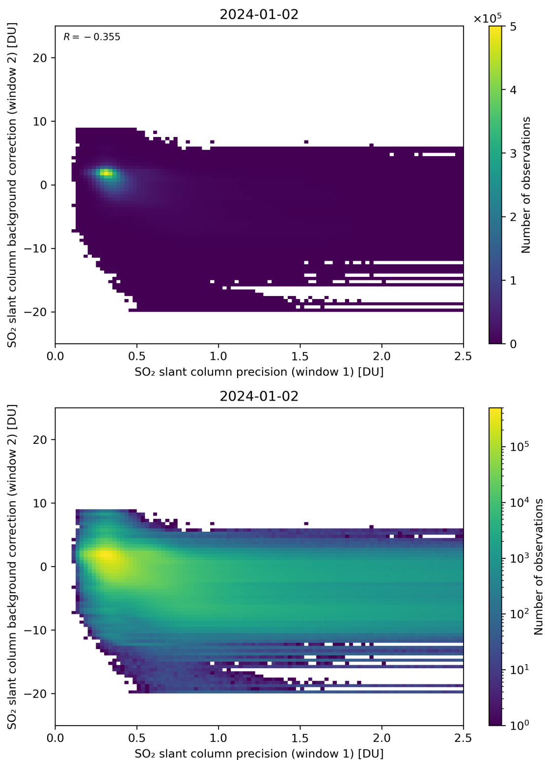
Figure 219: Scatter density plot of “SO 2 slant column precision (window 1)” against “SO 2 slant column background correction (window 2)” for 2024-01-01 to 2024-01-03.
