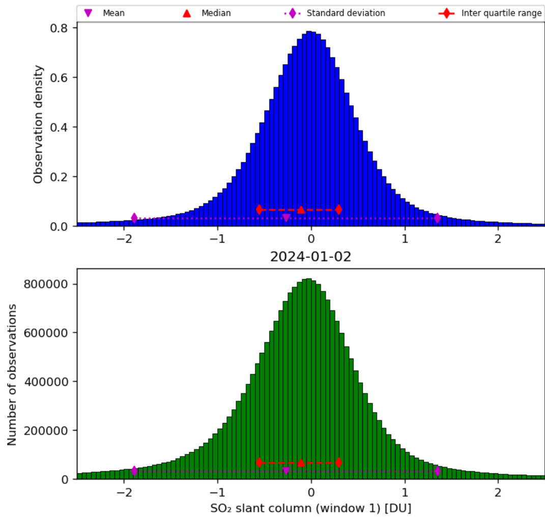
Figure 56: Histogram of “SO 2 slant column (window 1)” for 2024-01-01 to 2024-01-03
