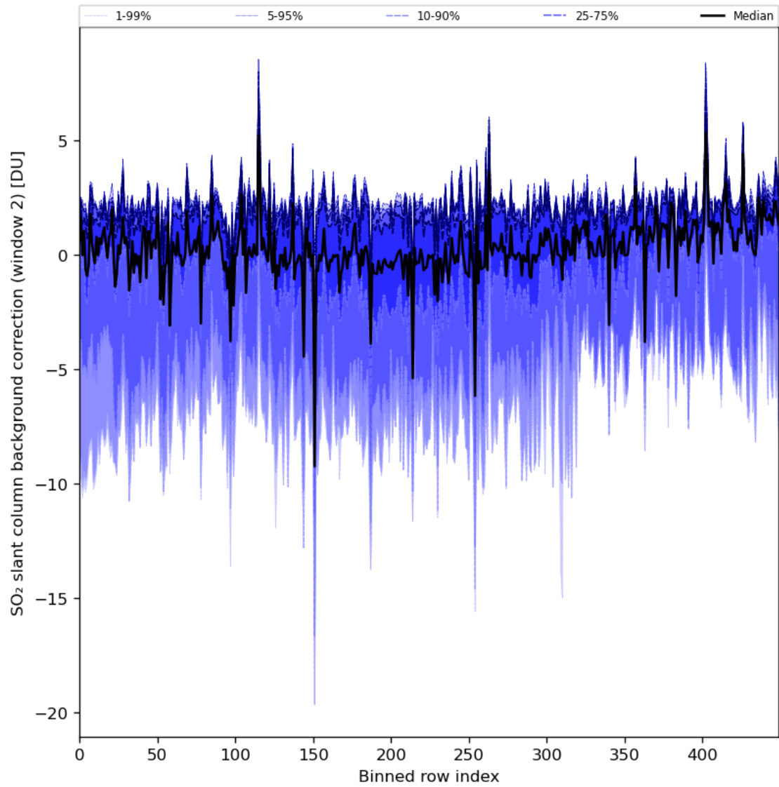
Figure 86: Along track statistics of “SO 2 slant column background correction (window 2)” for 2024-01-01 to 2024-01-03
