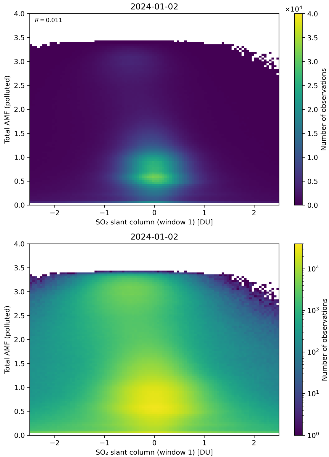
Figure 239: Scatter density plot of “SO 2 slant column (window 1)” against “Total AMF (polluted)” for 2024-01-01 to 2024-01-03.
