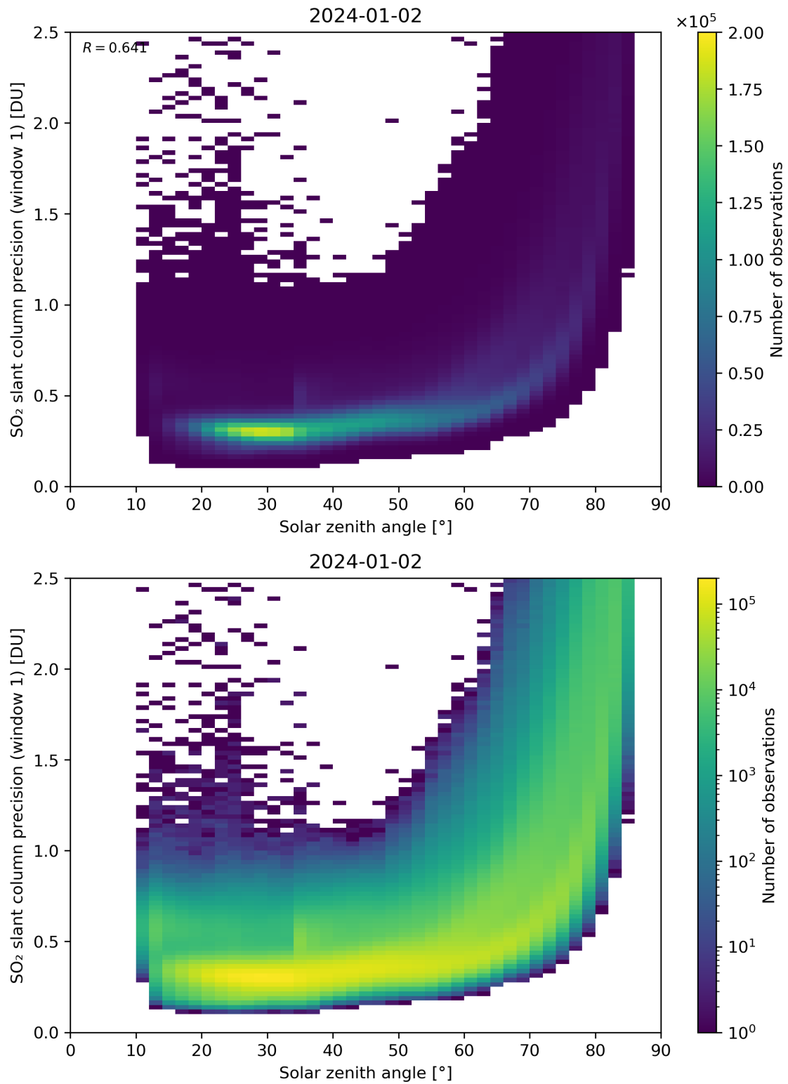
Figure 170: Scatter density plot of “Solar zenith angle” against “SO 2 slant column precision (window 1)” for 2024-01-01 to 2024-01-03.
