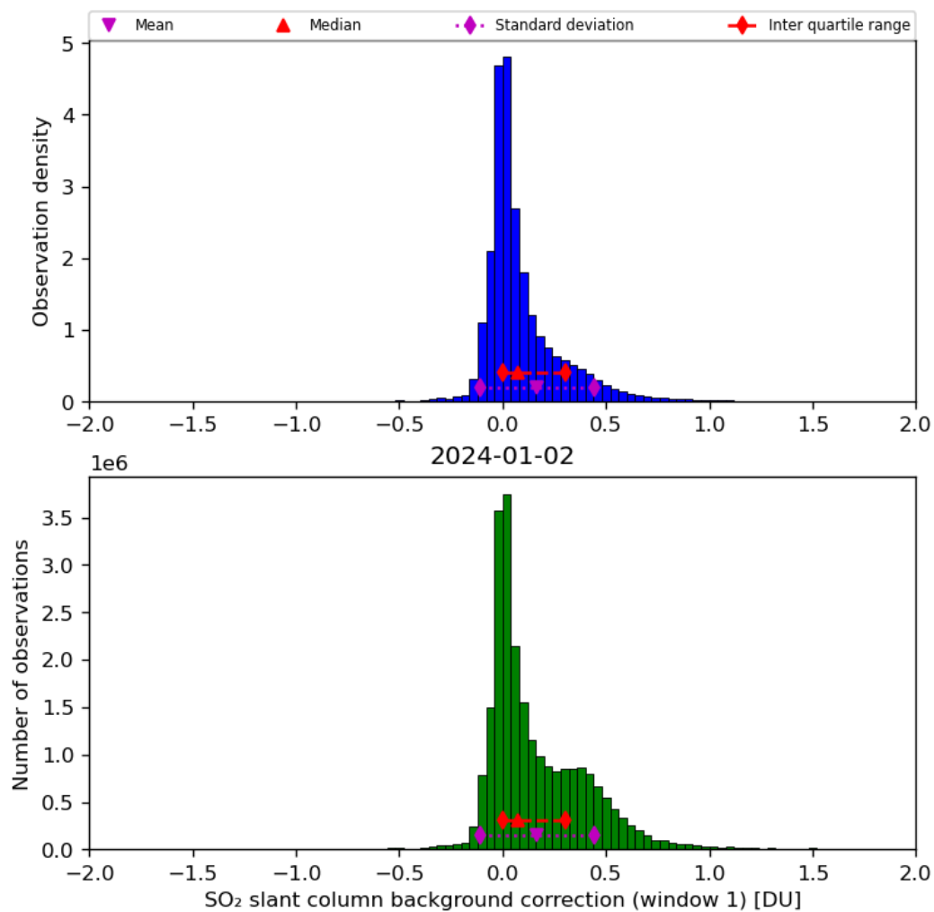
Figure 59: Histogram of “SO 2 slant column background correction (window 1)” for 2024-01-01 to 2024-01-03
