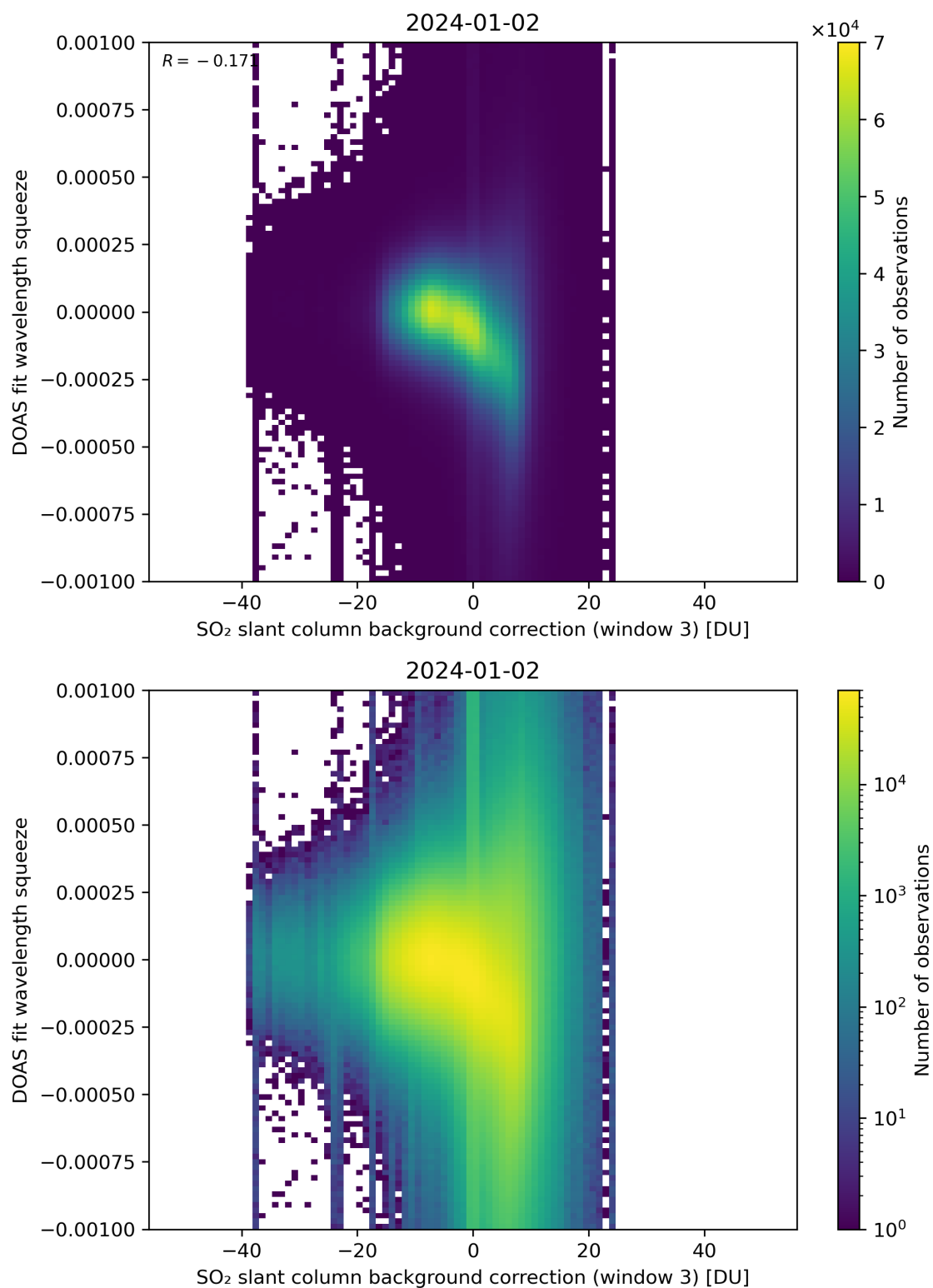
Figure 122: Scatter density plot of “SO 2 slant column background correction (window 3)” against “DOAS fit wavelength squeeze” for 2024-01-01 to 2024-01-03.
