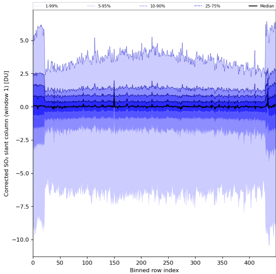
Figure 81: Along track statistics of “Corrected SO 2 slant column (window 1)” for 2024-01-01 to 2024-01-03
