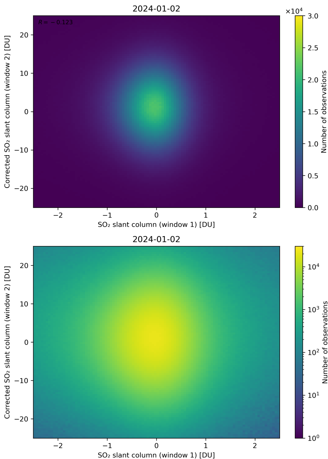
Figure 233: Scatter density plot of “SO 2 slant column (window 1)” against “Corrected SO 2 slant column (window 2)” for 2024-01-01 to 2024-01-03.
