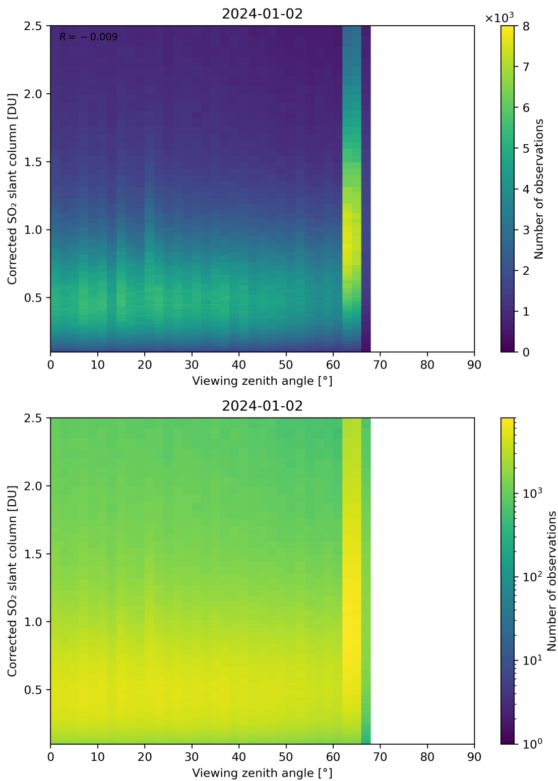
Figure 317: Scatter density plot of “Viewing zenith angle” against “Corrected SO 2 slant column” for 2024-01-01 to 2024-01-03.
