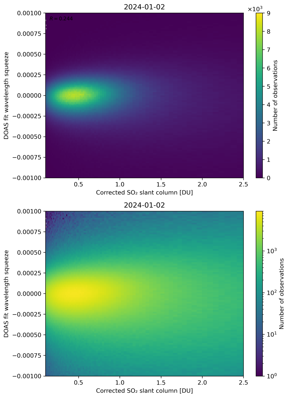
Figure 182: Scatter density plot of “Corrected SO 2 slant column” against “DOAS fit wavelength squeeze” for 2024-01-01 to 2024-01-03.
