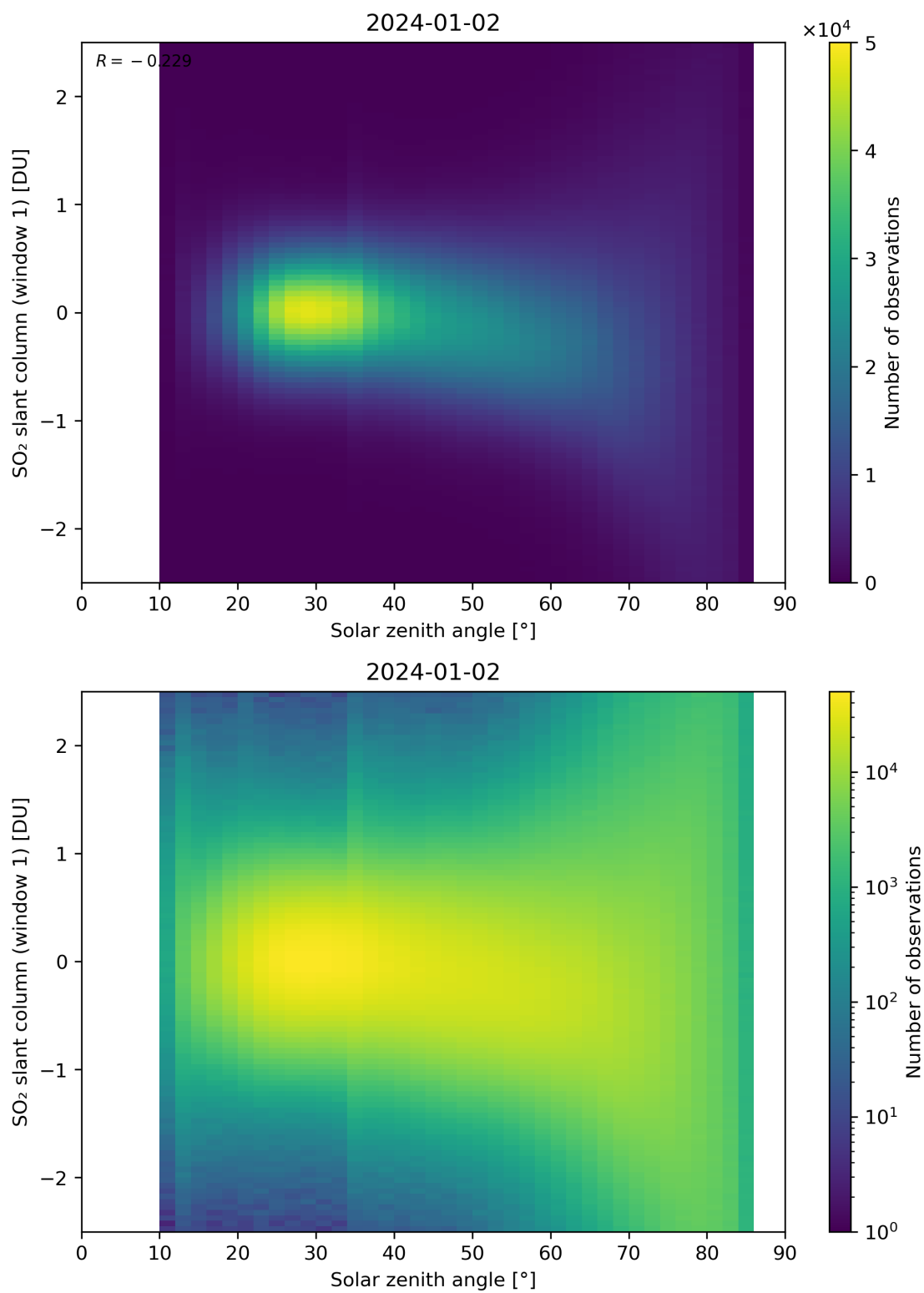
Figure 169: Scatter density plot of “Solar zenith angle” against “SO 2 slant column (window 1)” for 2024-01-01 to 2024-01-03.
