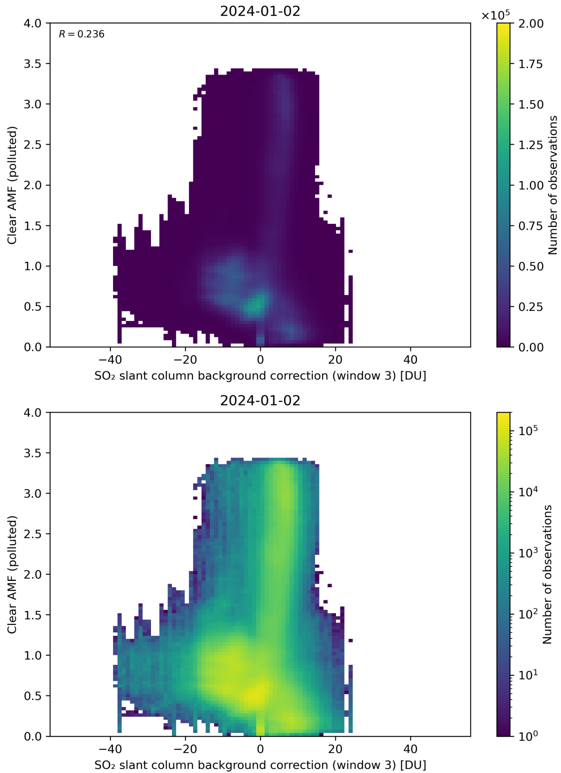
Figure 124: Scatter density plot of “SO 2 slant column background correction (window 3)” against “Clear AMF (polluted)” for 2024-01-01 to 2024-01-03.
