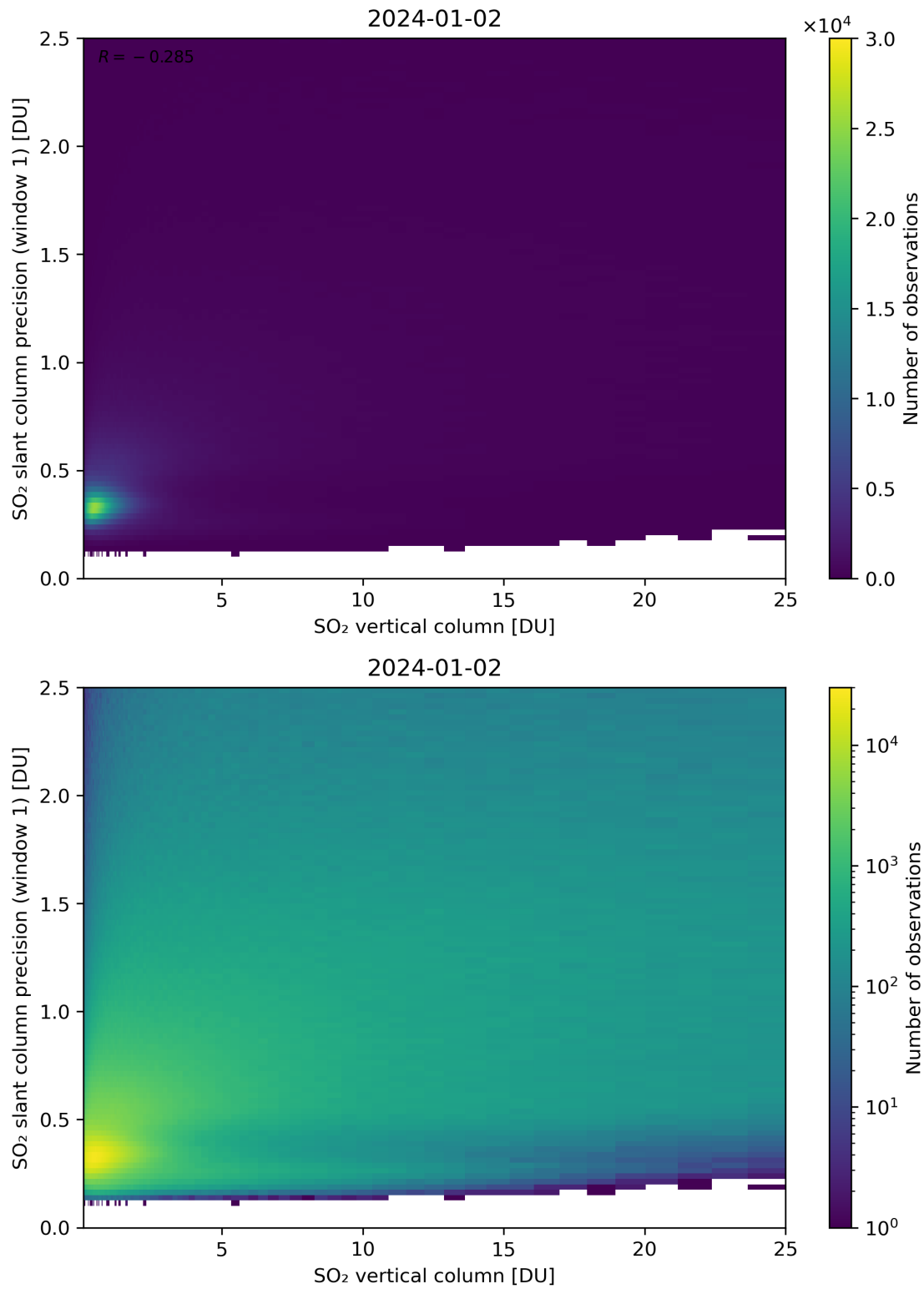
Figure 301: Scatter density plot of “SO 2 vertical column” against “SO 2 slant column precision (window 1)” for 2024-01-01 to 2024-01-03.
