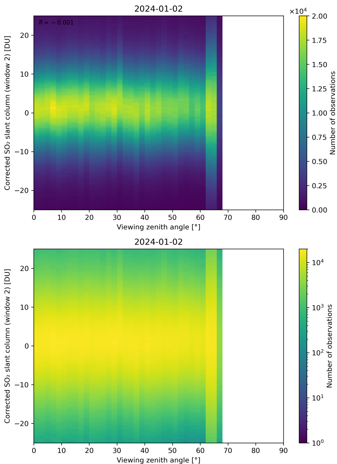
Figure 318: Scatter density plot of “Viewing zenith angle” against “Corrected SO 2 slant column (window 2)” for 2024-01-01 to 2024-01-03.
