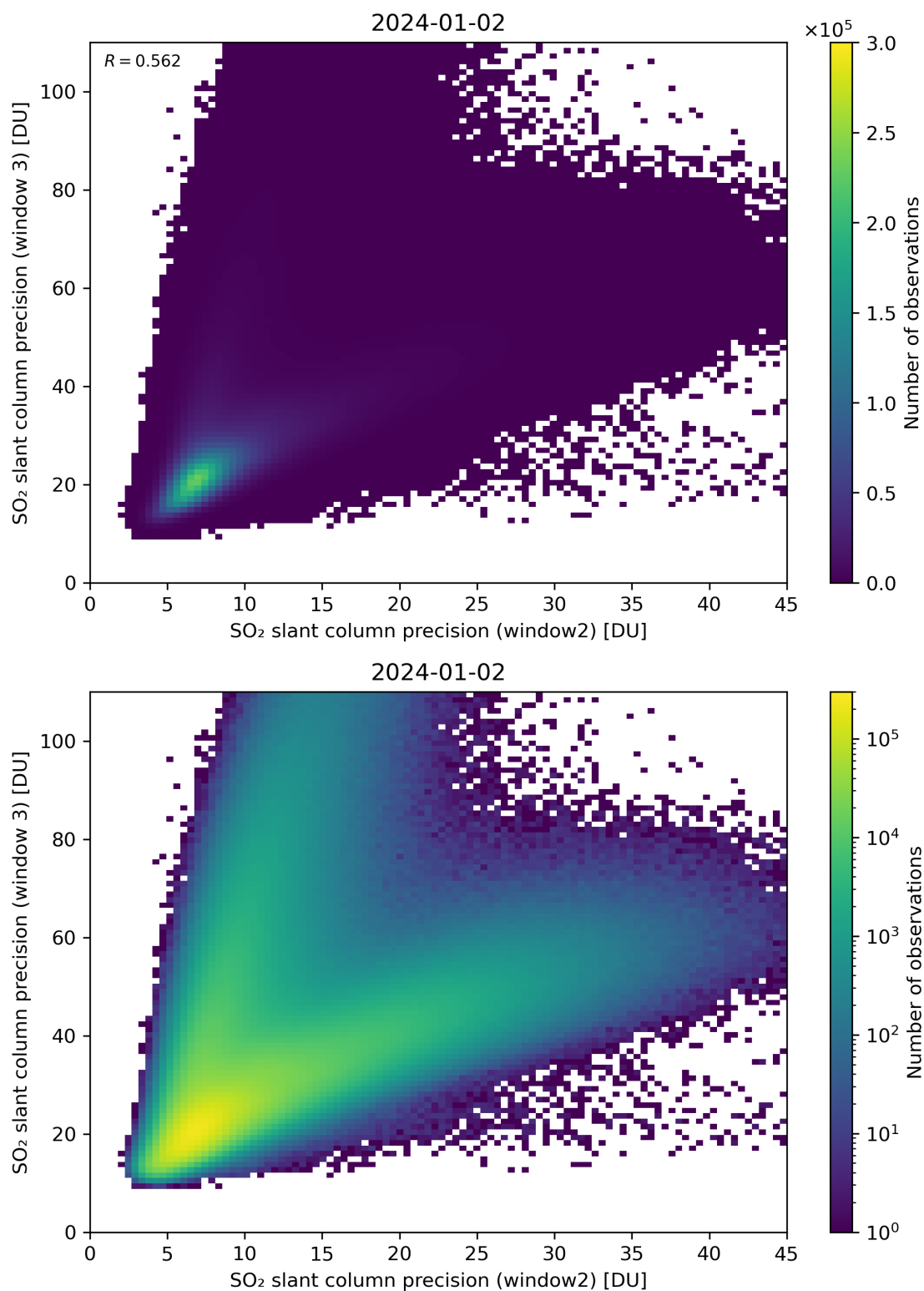
Figure 250: Scatter density plot of “SO 2 slant column precision (window2)” against “SO 2 slant column precision (window 3)” for 2024-01-01 to 2024-01-03.
