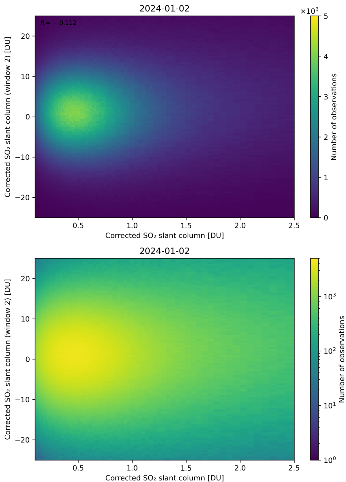
Figure 185: Scatter density plot of “Corrected SO 2 slant column” against “Corrected SO 2 slant column (window 2)” for 2024-01-01 to 2024-01-03.
