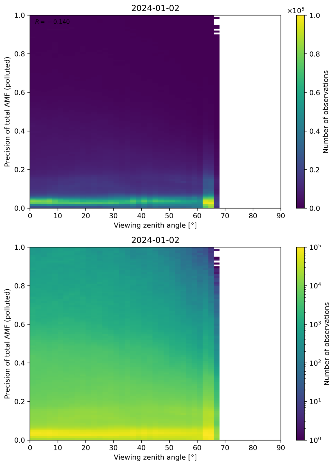
Figure 326: Scatter density plot of “Viewing zenith angle” against “Precision of total AMF (polluted)” for 2024-01-01 to 2024-01-03.
