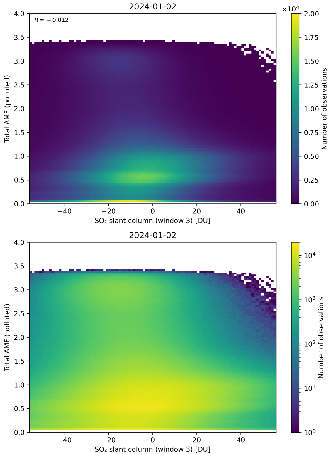
Figure 268: Scatter density plot of “SO 2 slant column (window 3)” against “Total AMF (polluted)” for 2024-01-01 to 2024-01-03.
