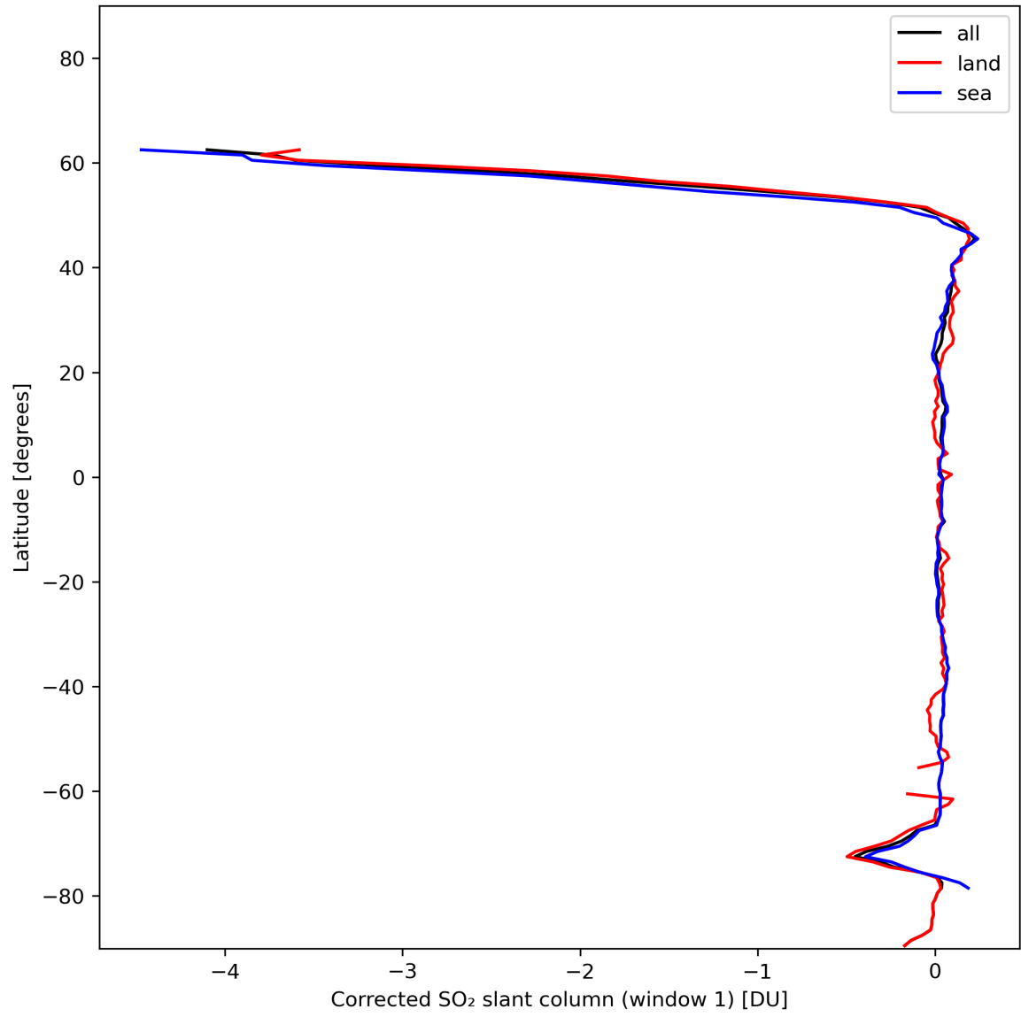
Figure 35: Zonal average of “Corrected SO 2 slant column (window 1)” for 2024-01-01 to 2024-01-03.
