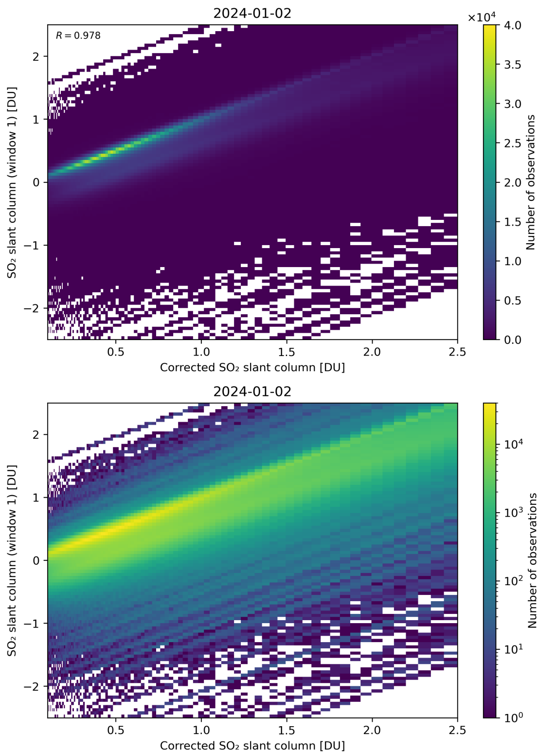
Figure 187: Scatter density plot of “Corrected SO 2 slant column” against “SO 2 slant column (window 1)” for 2024-01-01 to 2024-01-03.
