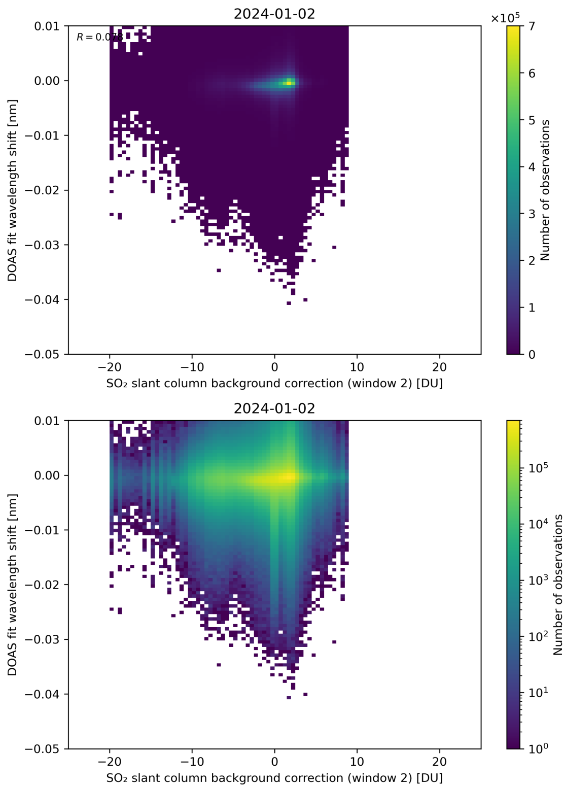
Figure 112: Scatter density plot of “SO 2 slant column background correction (window 2)” against “DOAS fit wavelength shift” for 2024-01-01 to 2024-01-03.
