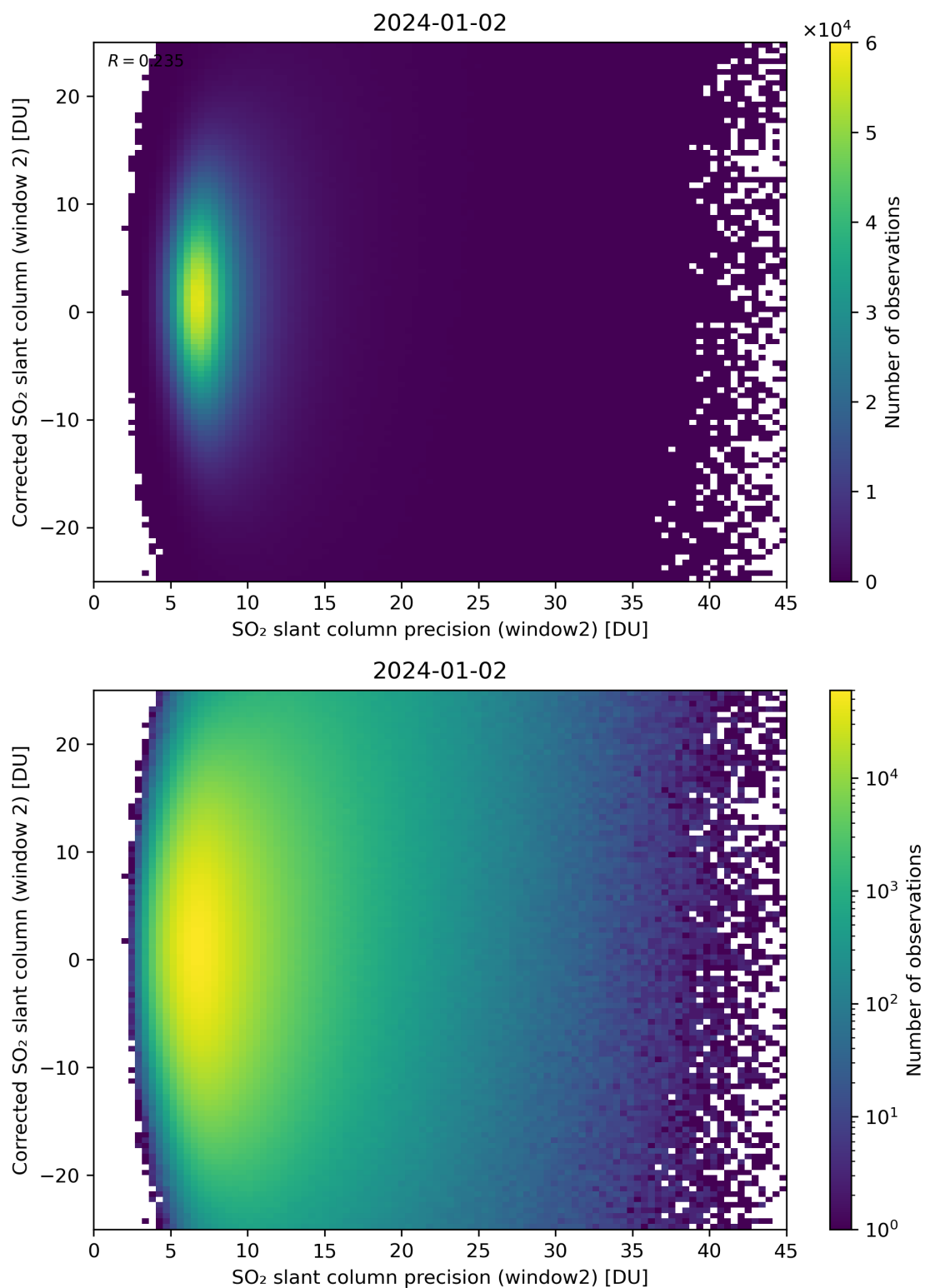
Figure 247: Scatter density plot of “SO 2 slant column precision (window2)” against “Corrected SO 2 slant column (window 2)” for 2024-01-01 to 2024-01-03.
