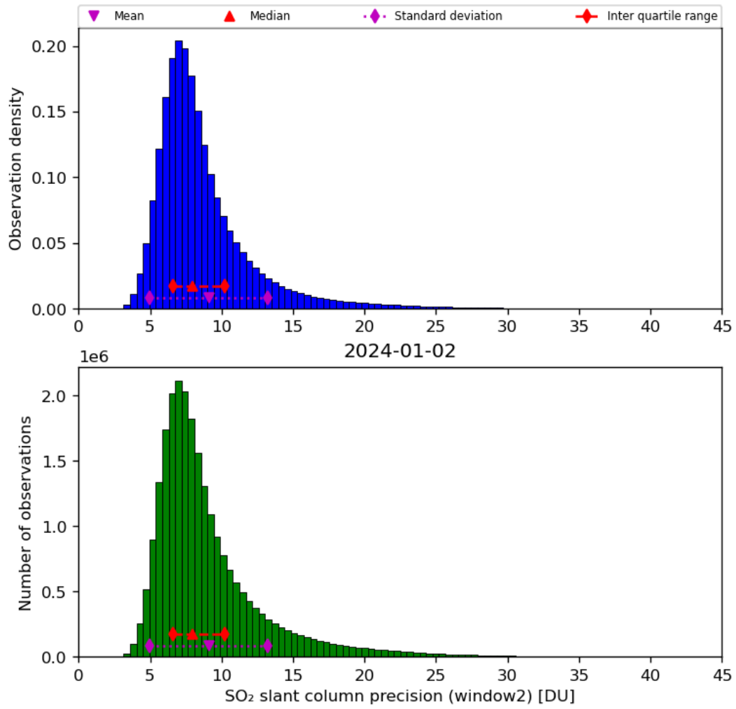
Figure 61: Histogram of “SO 2 slant column precision (window2)” for 2024-01-01 to 2024-01-03
