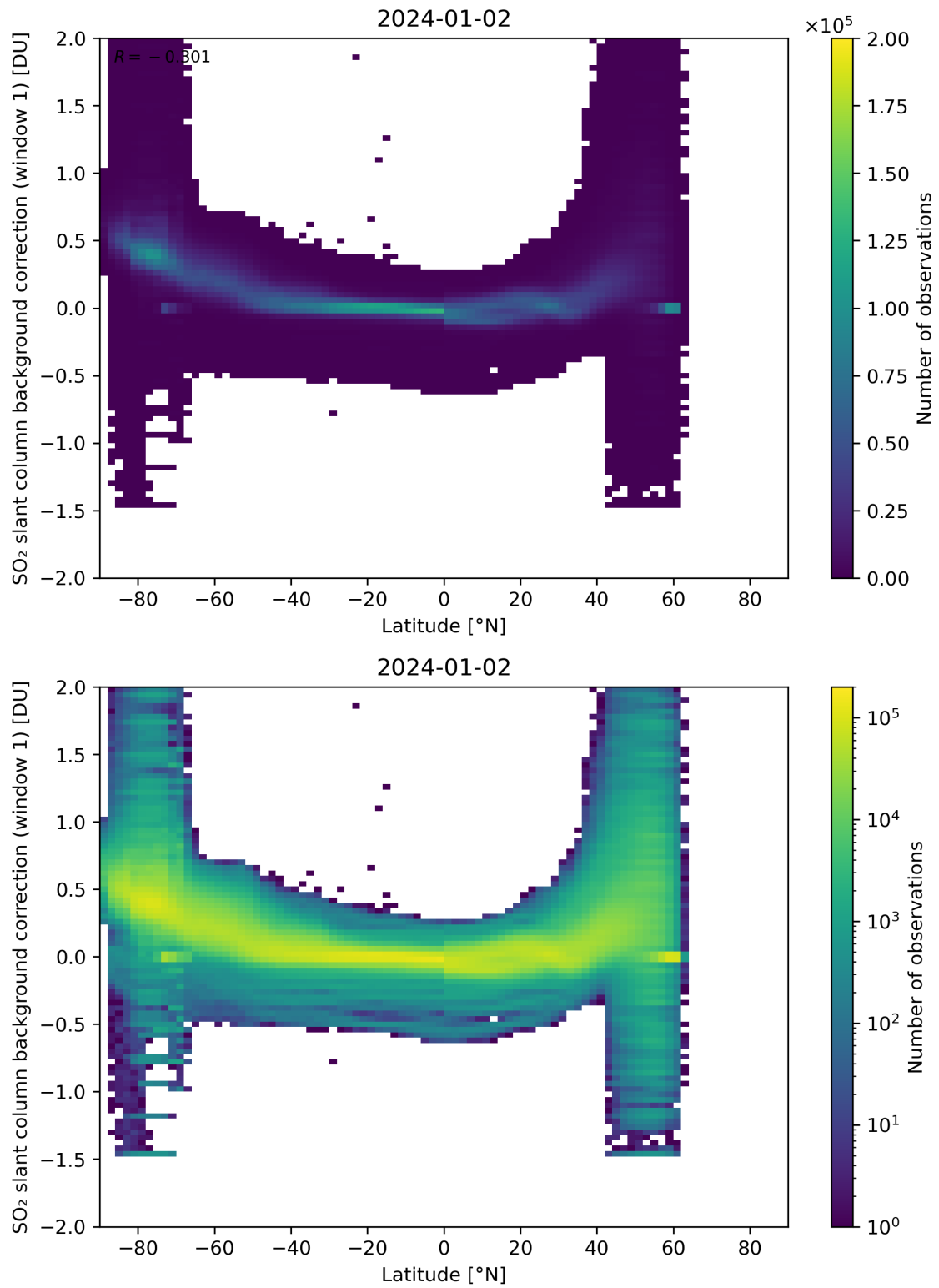
Figure 139: Scatter density plot of “Latitude” against “SO 2 slant column background correction (window 1)” for 2024-01-01 to 2024-01-03.
