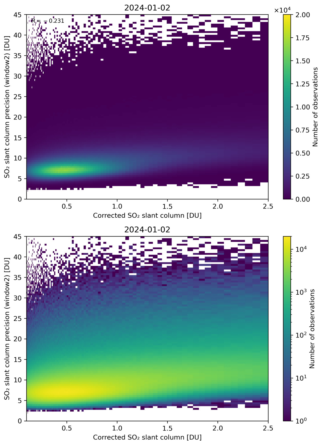
Figure 189: Scatter density plot of “Corrected SO 2 slant column” against “SO 2 slant column precision (window2)” for 2024-01-01 to 2024-01-03.
