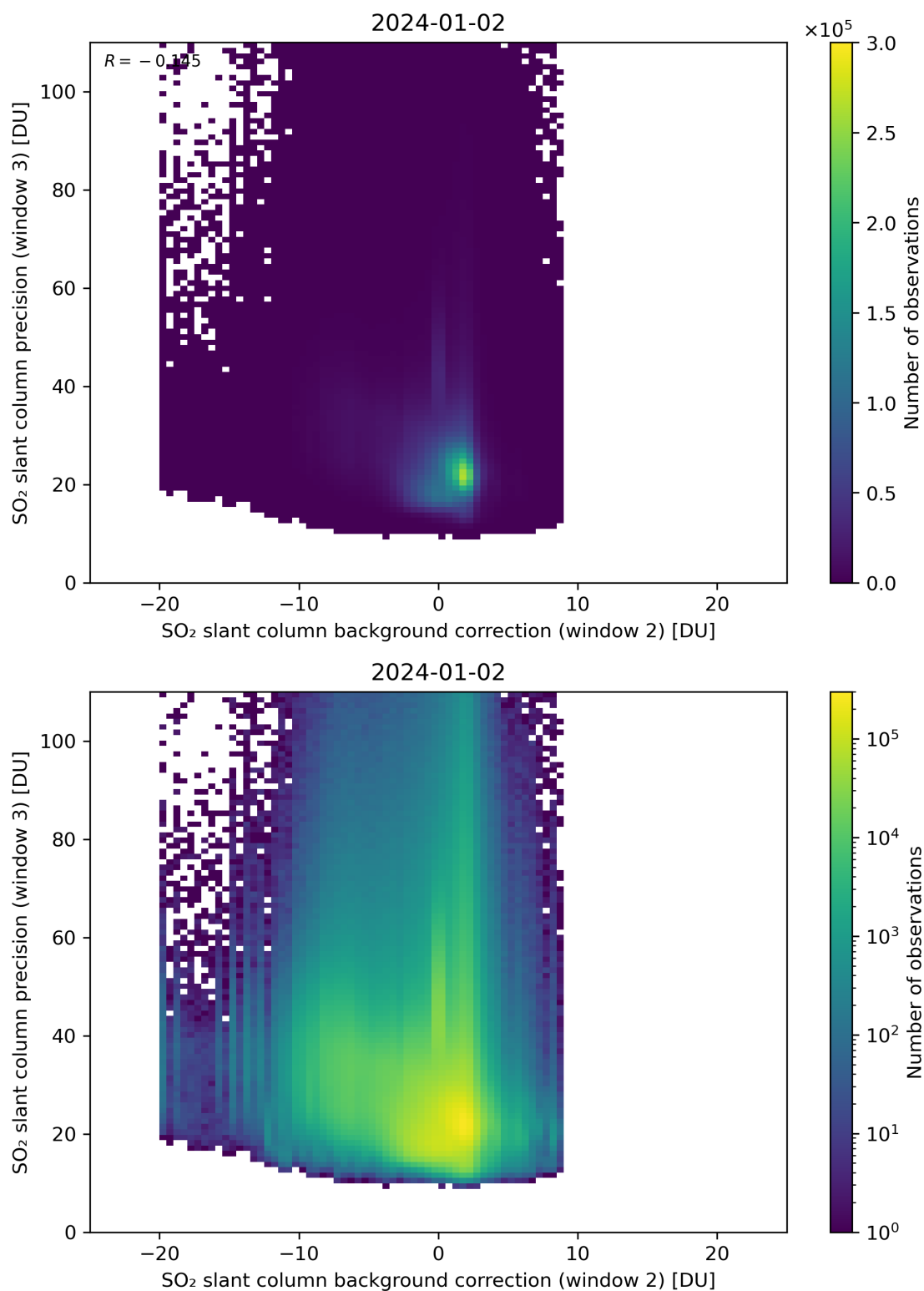
Figure 118: Scatter density plot of “SO 2 slant column background correction (window 2)” against “SO 2 slant column precision (window 3)” for 2024-01-01 to 2024-01-03.
