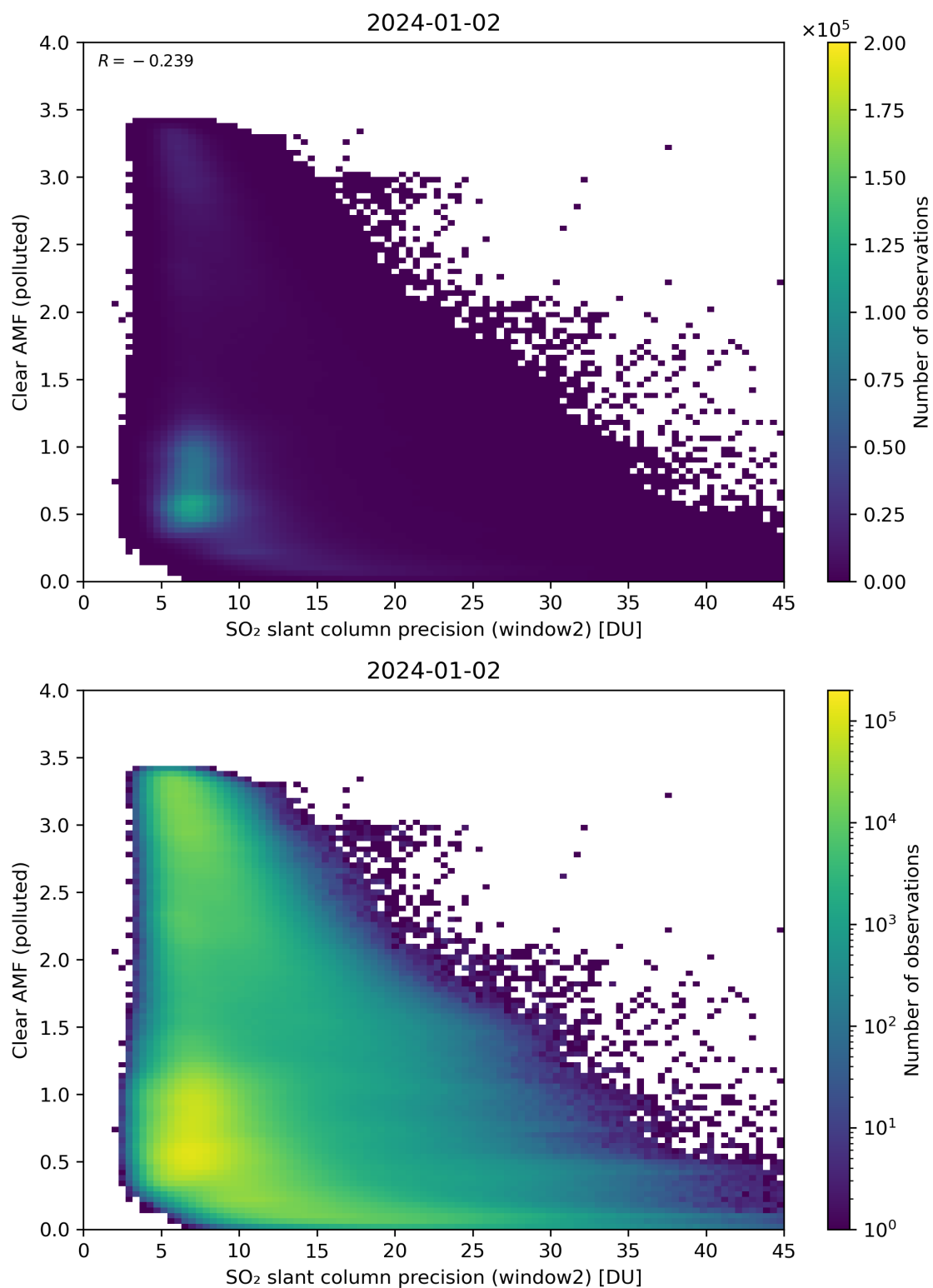
Figure 246: Scatter density plot of “SO 2 slant column precision (window2)” against “Clear AMF (polluted)” for 2024-01-01 to 2024-01-03.
