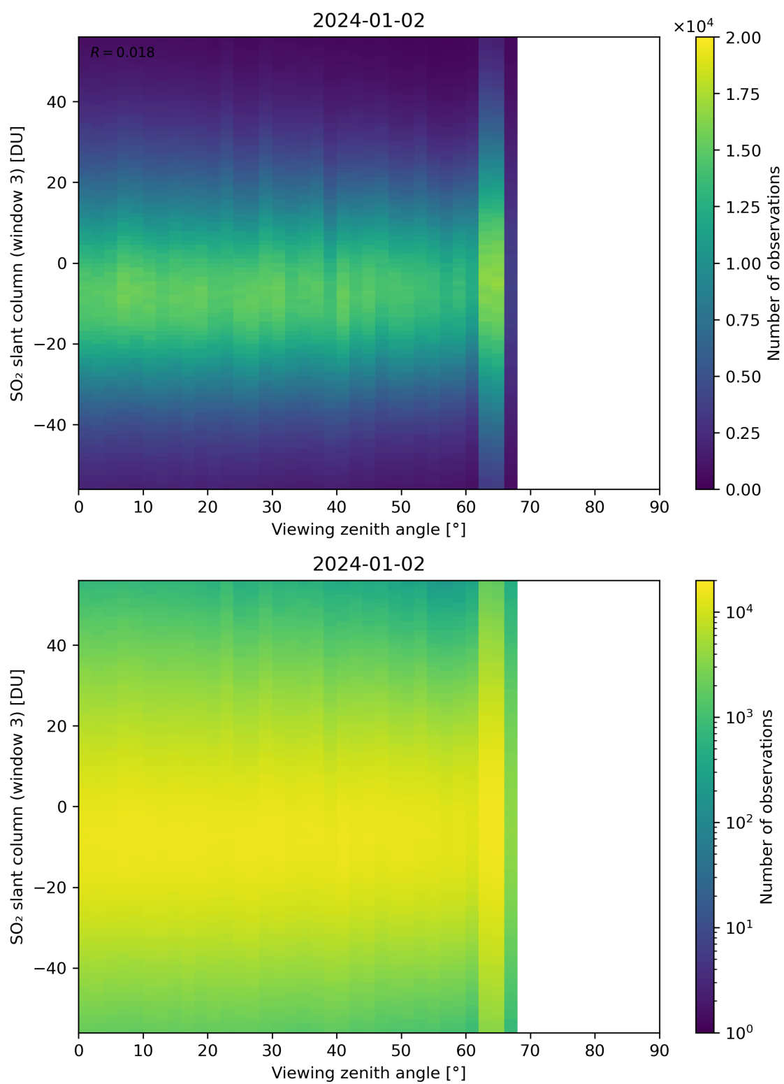
Figure 323: Scatter density plot of “Viewing zenith angle” against “SO 2 slant column (window 3)” for 2024-01-01 to 2024-01-03.
