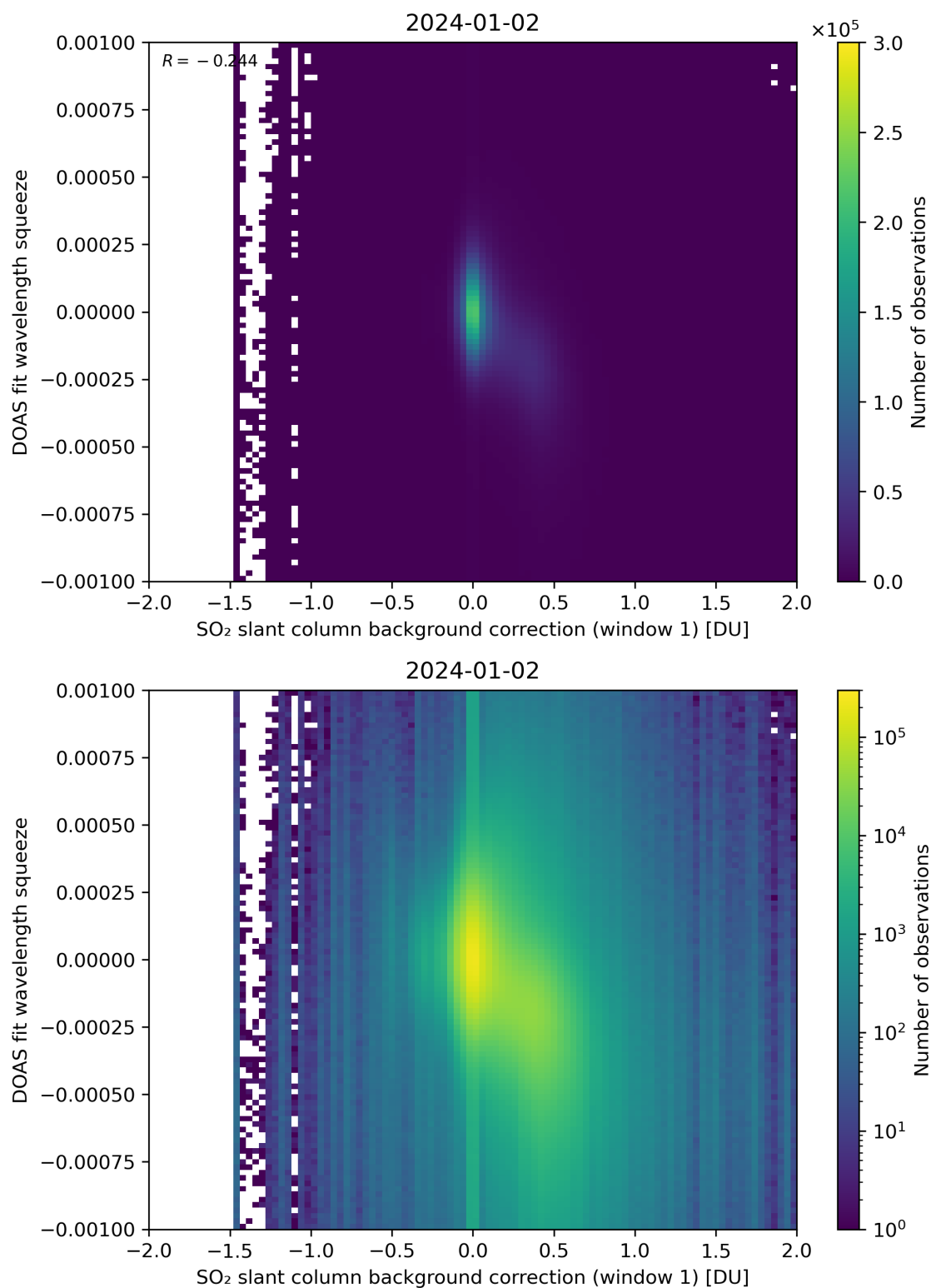
Figure 101: Scatter density plot of “SO 2 slant column background correction (window 1)” against “DOAS fit wavelength squeeze” for 2024-01-01 to 2024-01-03.
