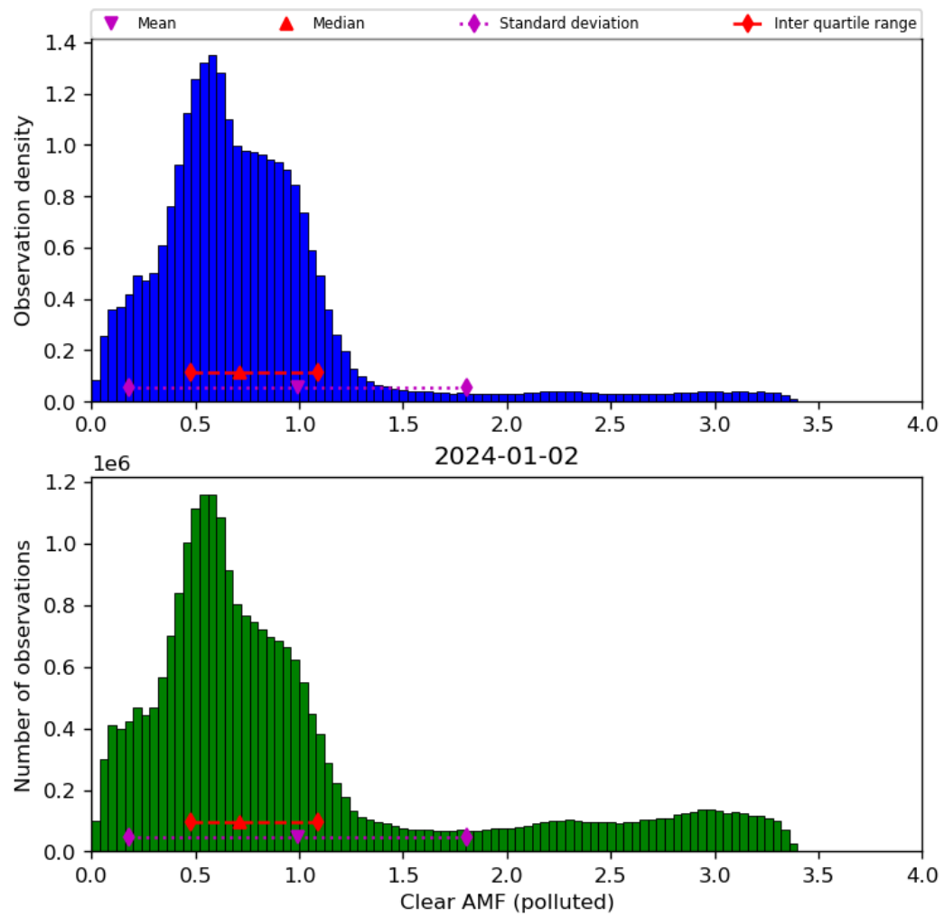
Figure 73: Histogram of “Clear AMF (polluted)” for 2024-01-01 to 2024-01-03
