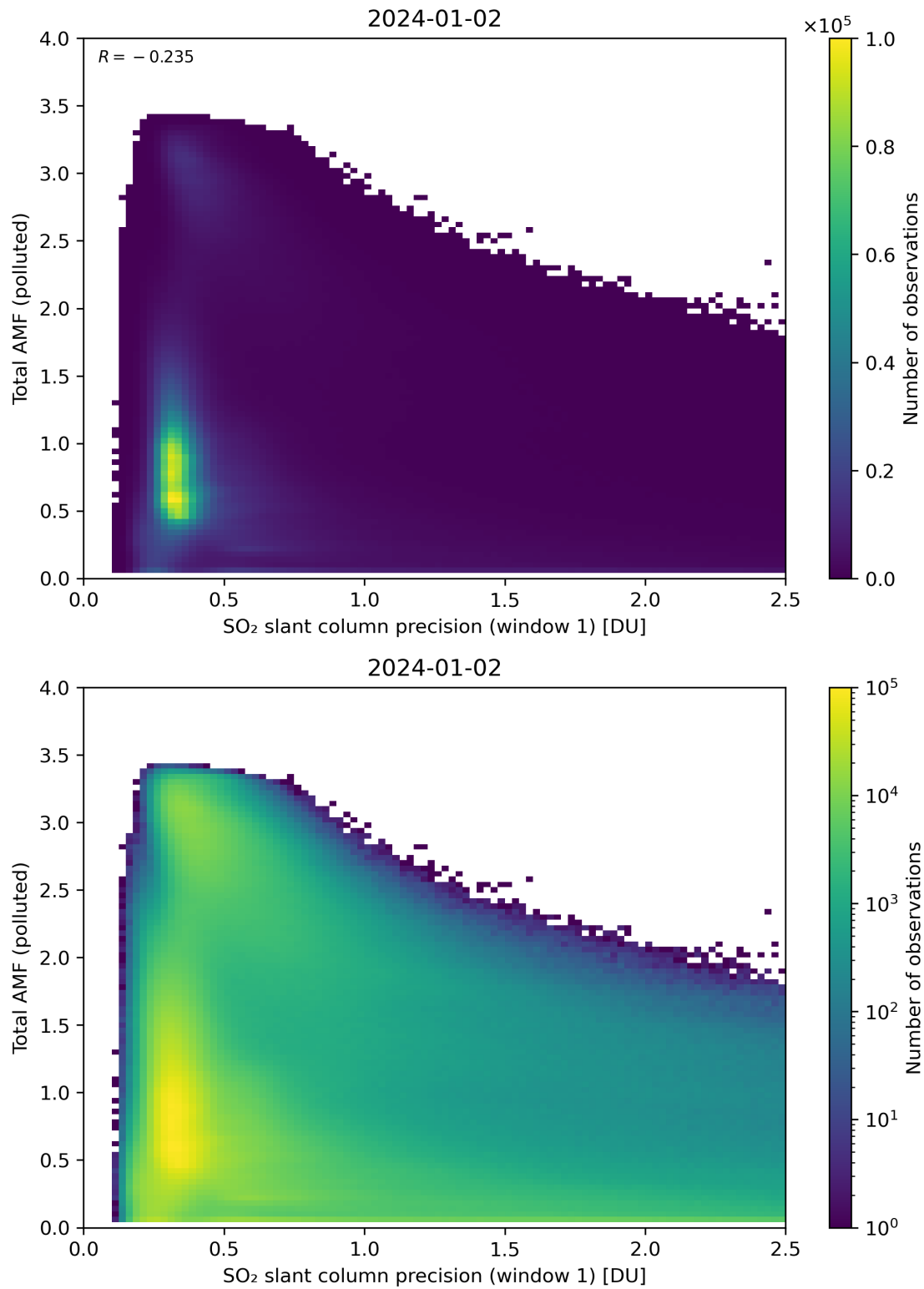
Figure 230: Scatter density plot of “SO 2 slant column precision (window 1)” against “Total AMF (polluted)” for 2024-01-01 to 2024-01-03.
