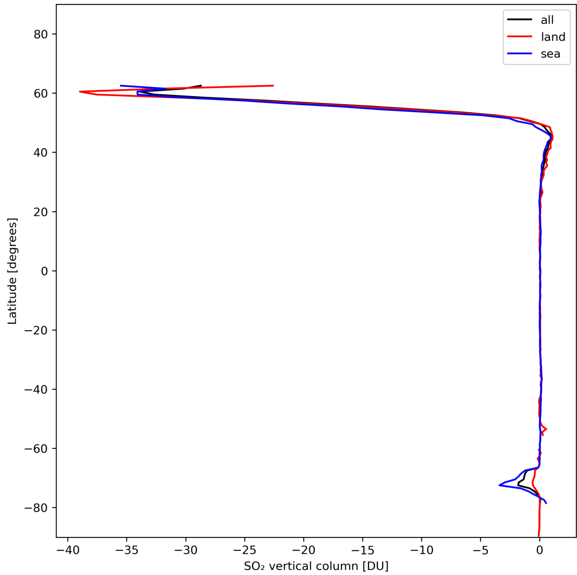
Figure 30: Zonal average of “SO 2 vertical column” for 2024-01-01 to 2024-01-03.
