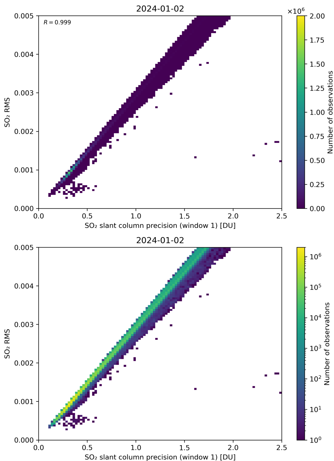
Figure 223: Scatter density plot of “SO 2 slant column precision (window 1)” against “SO 2 RMS” for 2024-01-01 to 2024-01-03.
