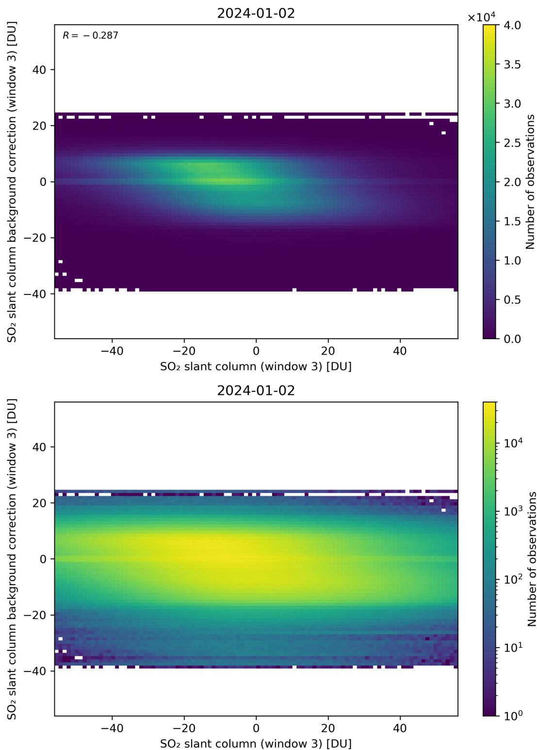
Figure 253: Scatter density plot of “SO 2 slant column (window 3)” against “SO 2 slant column background correction (window 3)” for 2024-01-01 to 2024-01-03.
