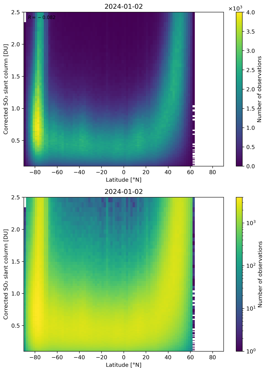
Figure 146: Scatter density plot of “Latitude” against “Corrected SO 2 slant column” for 2024-01-01 to 2024-01-03.
