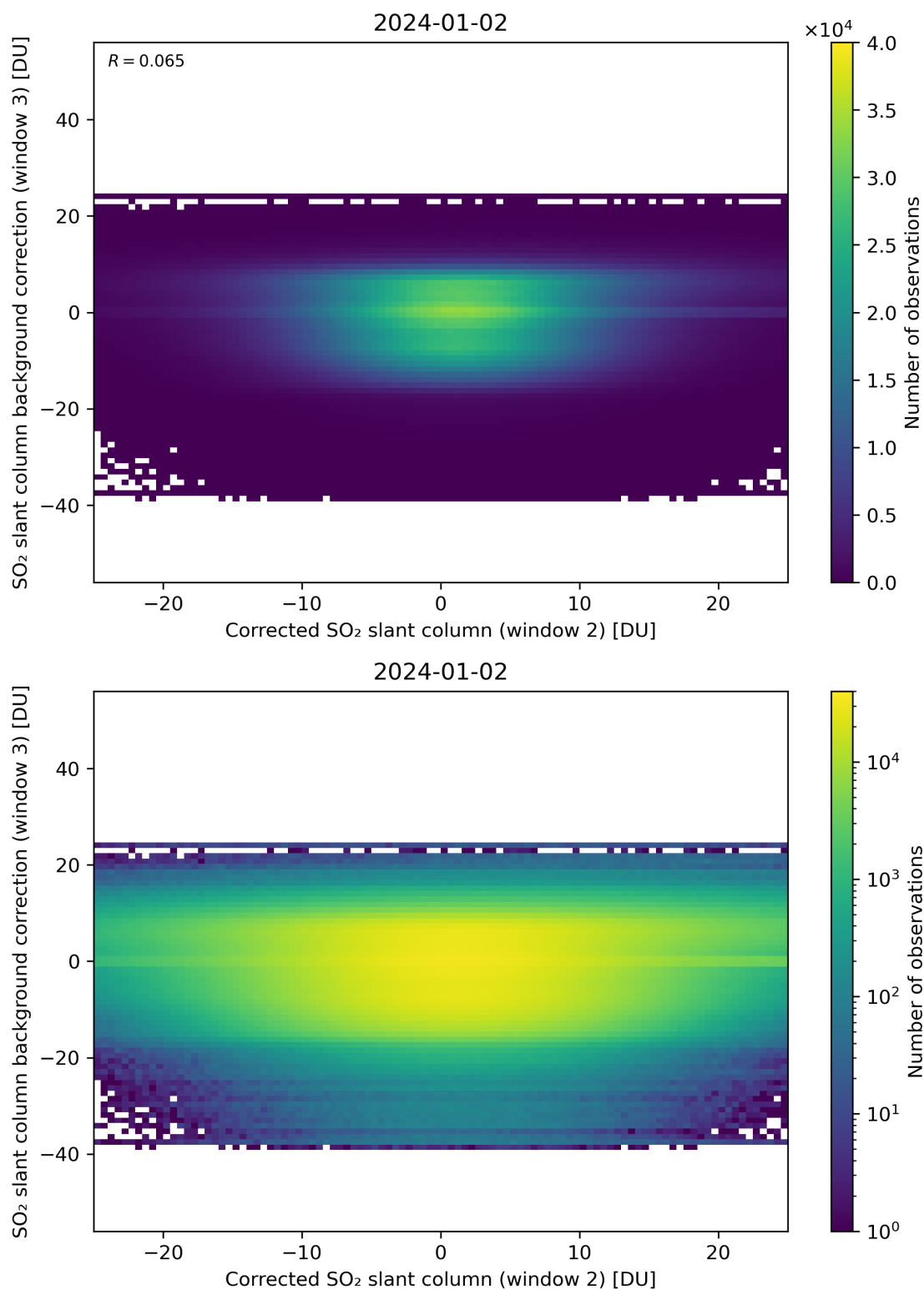
Figure 195: Scatter density plot of “Corrected SO 2 slant column (window 2)” against “SO 2 slant column background correction (window 3)” for 2024-01-01 to 2024-01-03.
