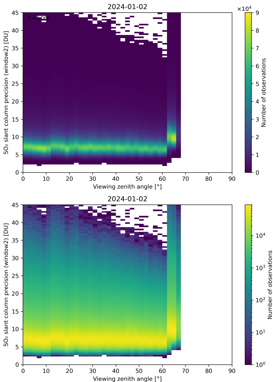
Figure 322: Scatter density plot of “Viewing zenith angle” against “SO 2 slant column precision (window2)” for 2024-01-01 to 2024-01-03.
