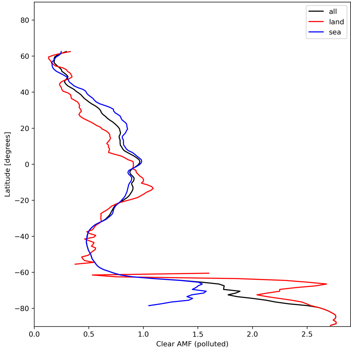
Figure 50: Zonal average of “Clear AMF (polluted)” for 2024-01-01 to 2024-01-03.
