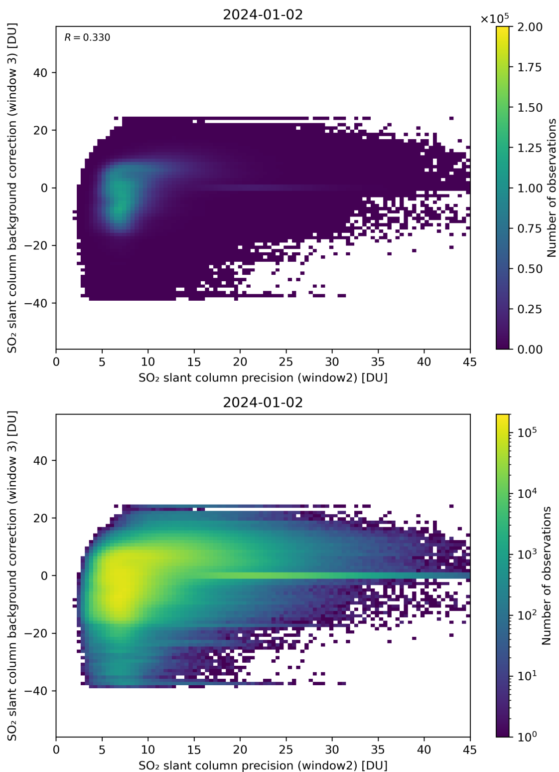
Figure 242: Scatter density plot of “SO 2 slant column precision (window2)” against “SO 2 slant column background correction (window 3)” for 2024-01-01 to 2024-01-03.
