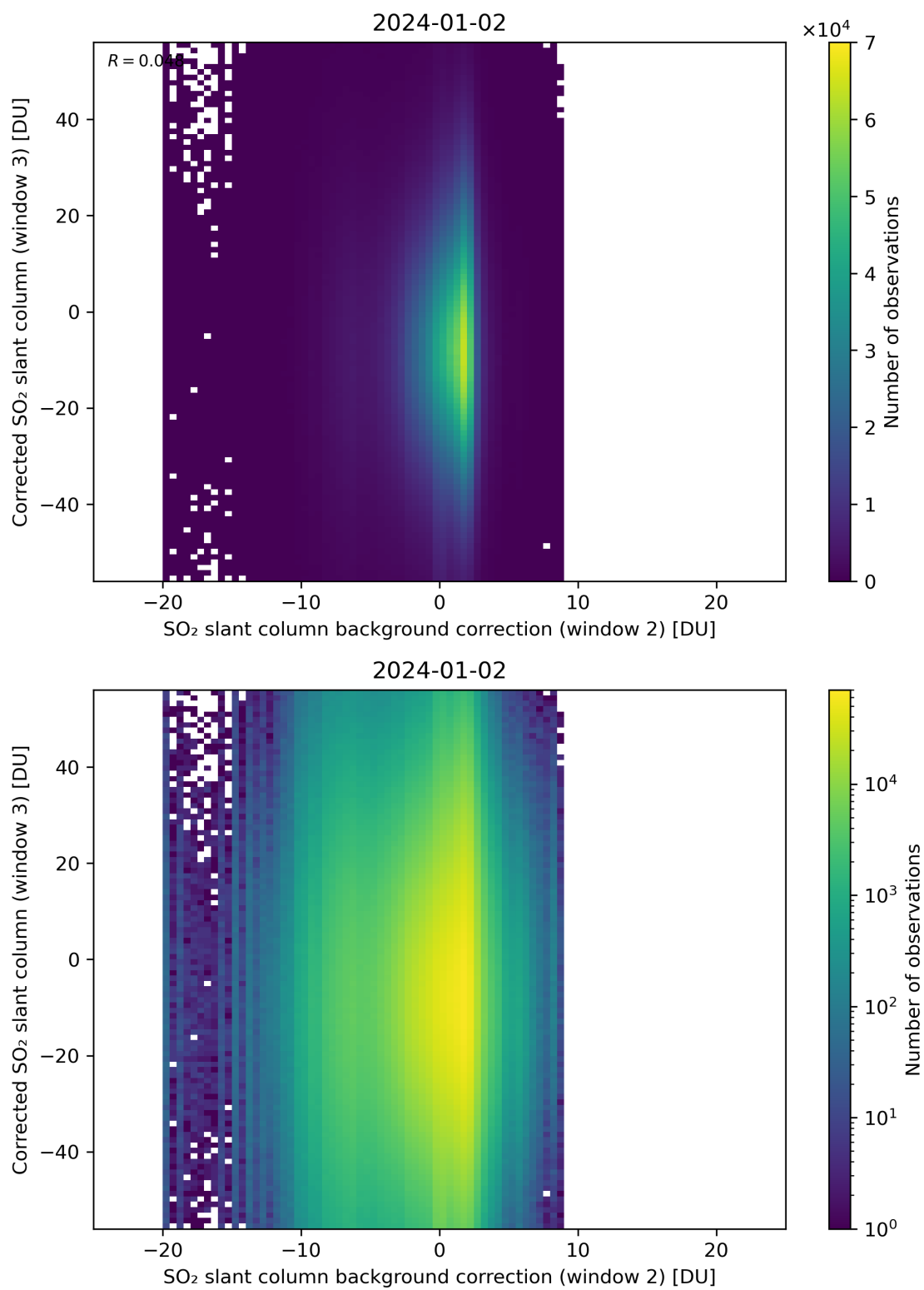
Figure 116: Scatter density plot of “SO 2 slant column background correction (window 2)” against “Corrected SO 2 slant column (window 3)” for 2024-01-01 to 2024-01-03.
