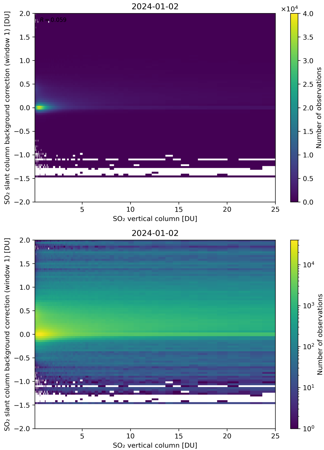
Figure 273: Scatter density plot of “SO 2 vertical column” against “SO 2 slant column background correction (window 1)” for 2024-01-01 to 2024-01-03.
