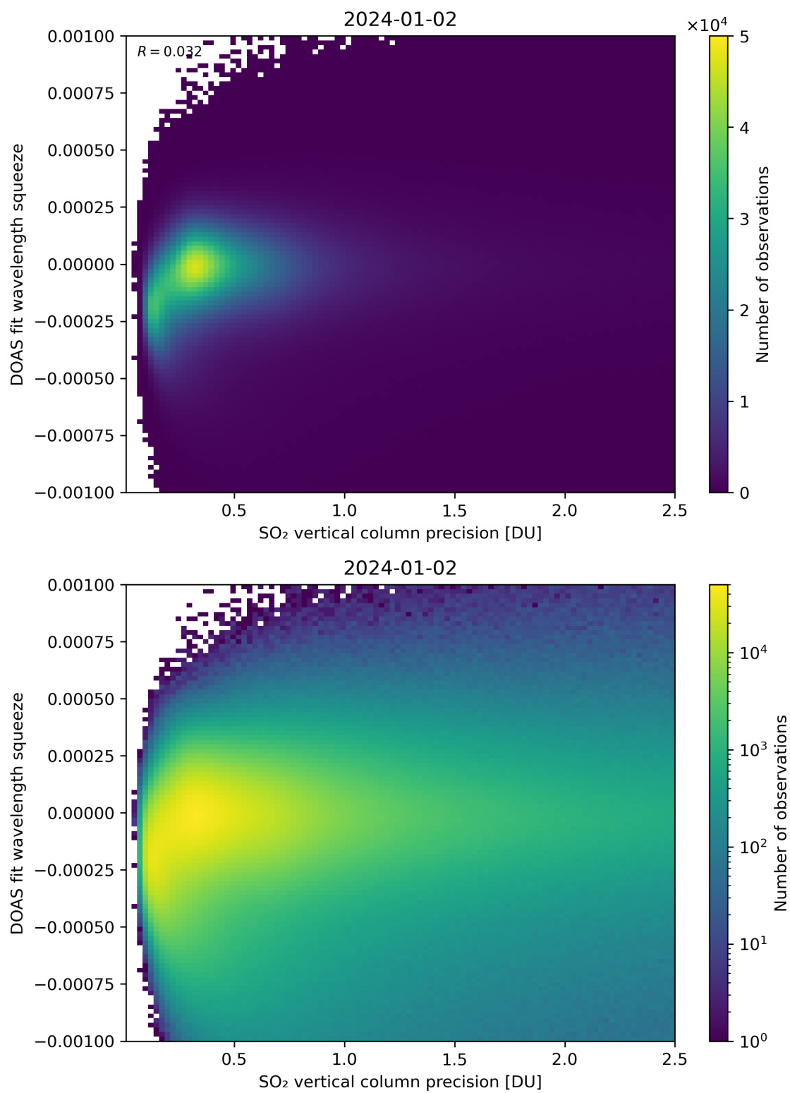
Figure 283: Scatter density plot of “SO 2 vertical column precision” against “DOAS fit wavelength squeeze” for 2024-01-01 to 2024-01-03.
