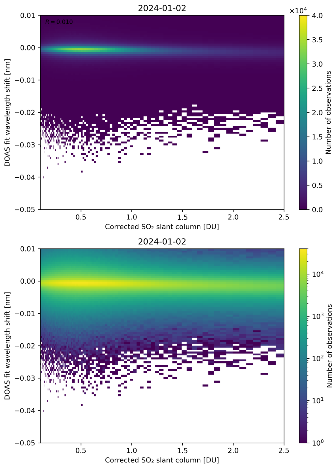
Figure 181: Scatter density plot of “Corrected SO 2 slant column” against “DOAS fit wavelength shift” for 2024-01-01 to 2024-01-03.
