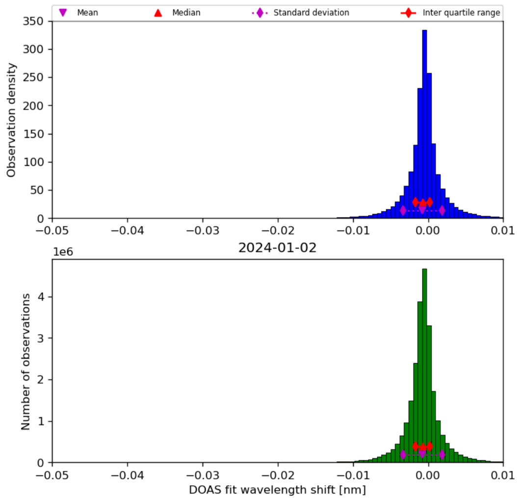
Figure 68: Histogram of “DOAS fit wavelength shift” for 2024-01-01 to 2024-01-03
