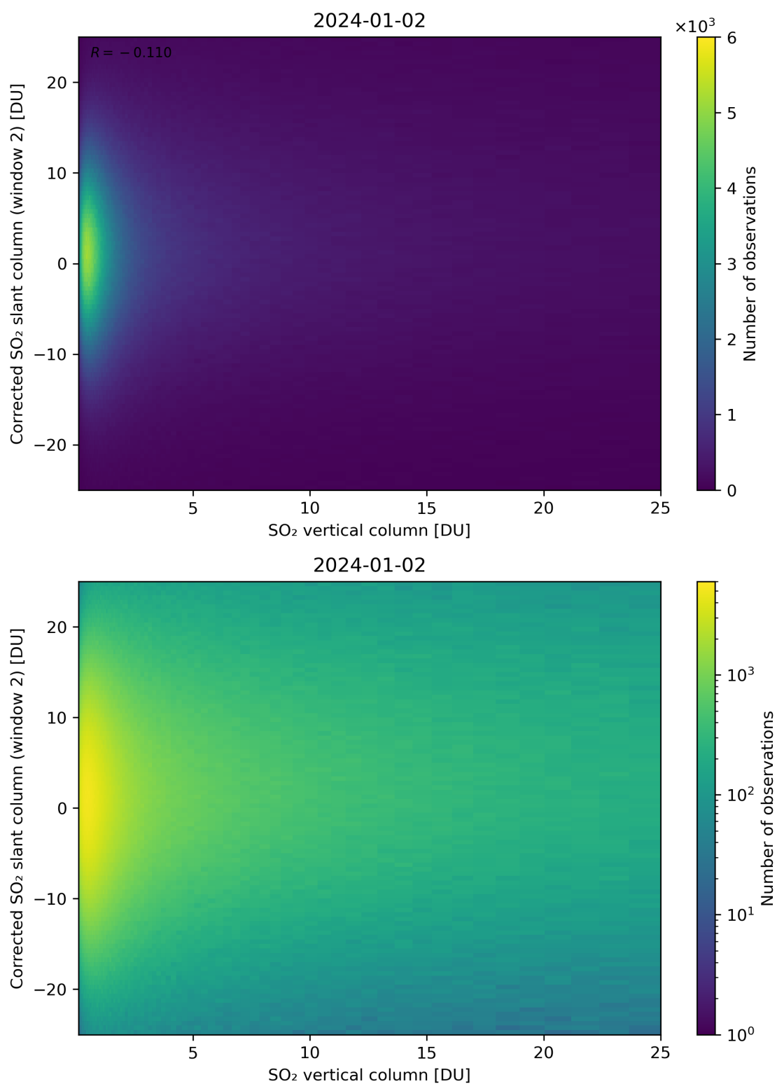
Figure 298: Scatter density plot of “SO 2 vertical column” against “Corrected SO 2 slant column (window 2)” for 2024-01-01 to 2024-01-03.
