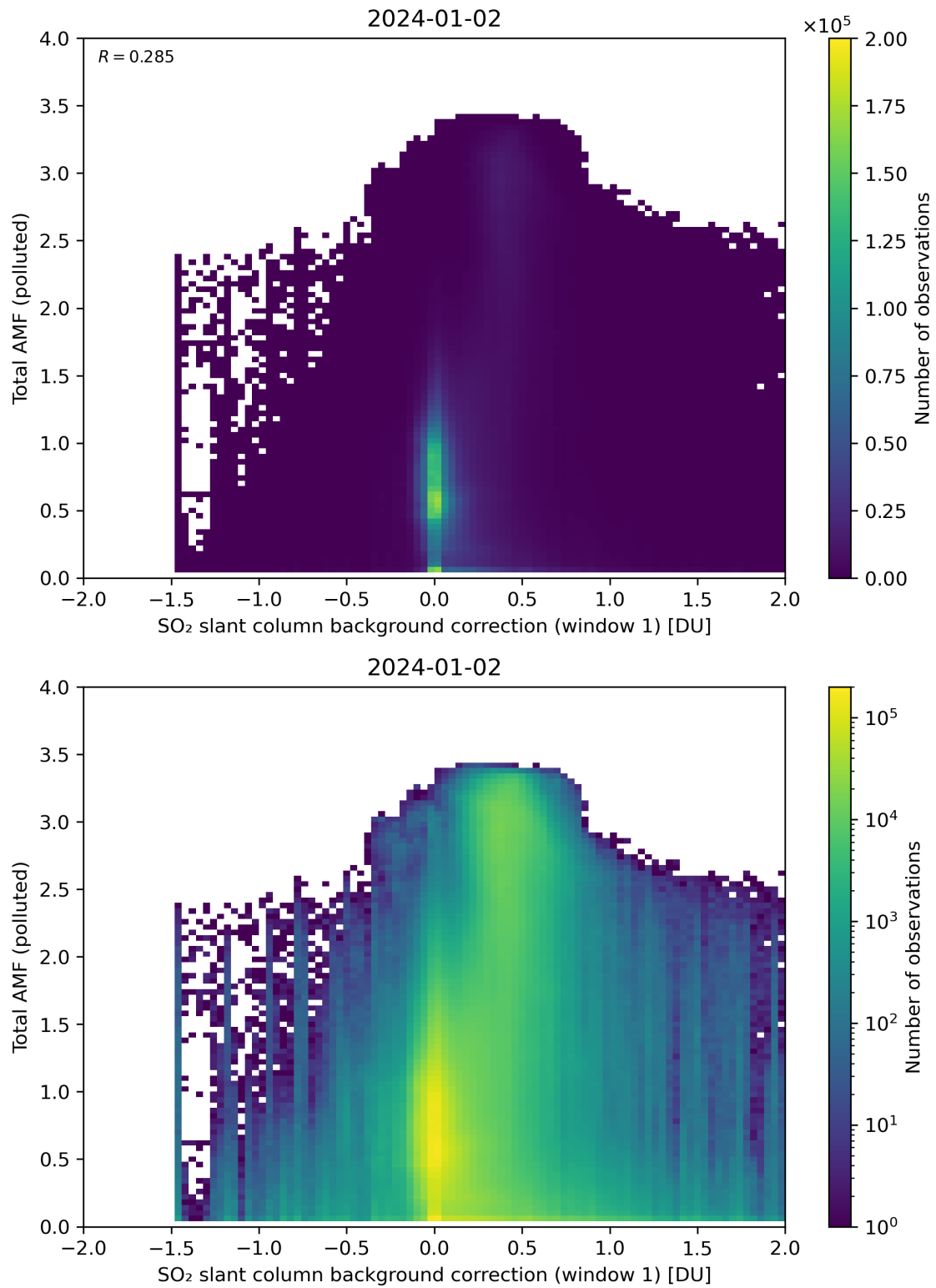
Figure 109: Scatter density plot of “SO 2 slant column background correction (window 1)” against “Total AMF (polluted)” for 2024-01-01 to 2024-01-03.
