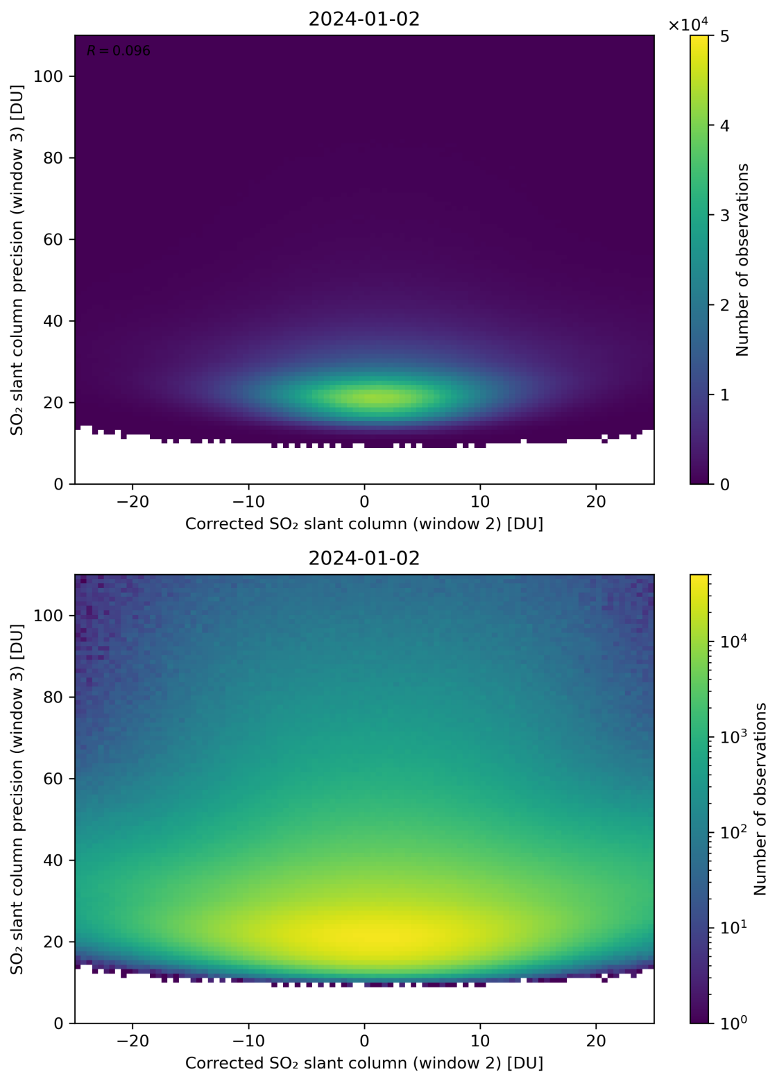
Figure 202: Scatter density plot of “Corrected SO 2 slant column (window 2)” against “SO 2 slant column precision (window 3)” for 2024-01-01 to 2024-01-03.
