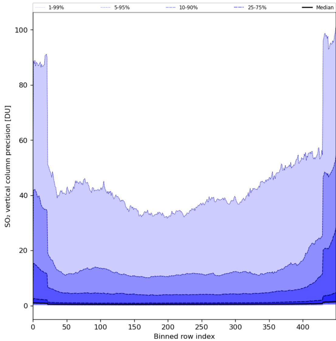
Figure 77: Along track statistics of “SO 2 vertical column precision” for 2024-01-01 to 2024-01-03
