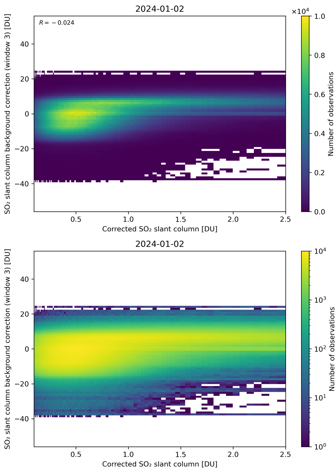
Figure 180: Scatter density plot of “Corrected SO 2 slant column” against “SO 2 slant column background correction (window 3)” for 2024-01-01 to 2024-01-03.
