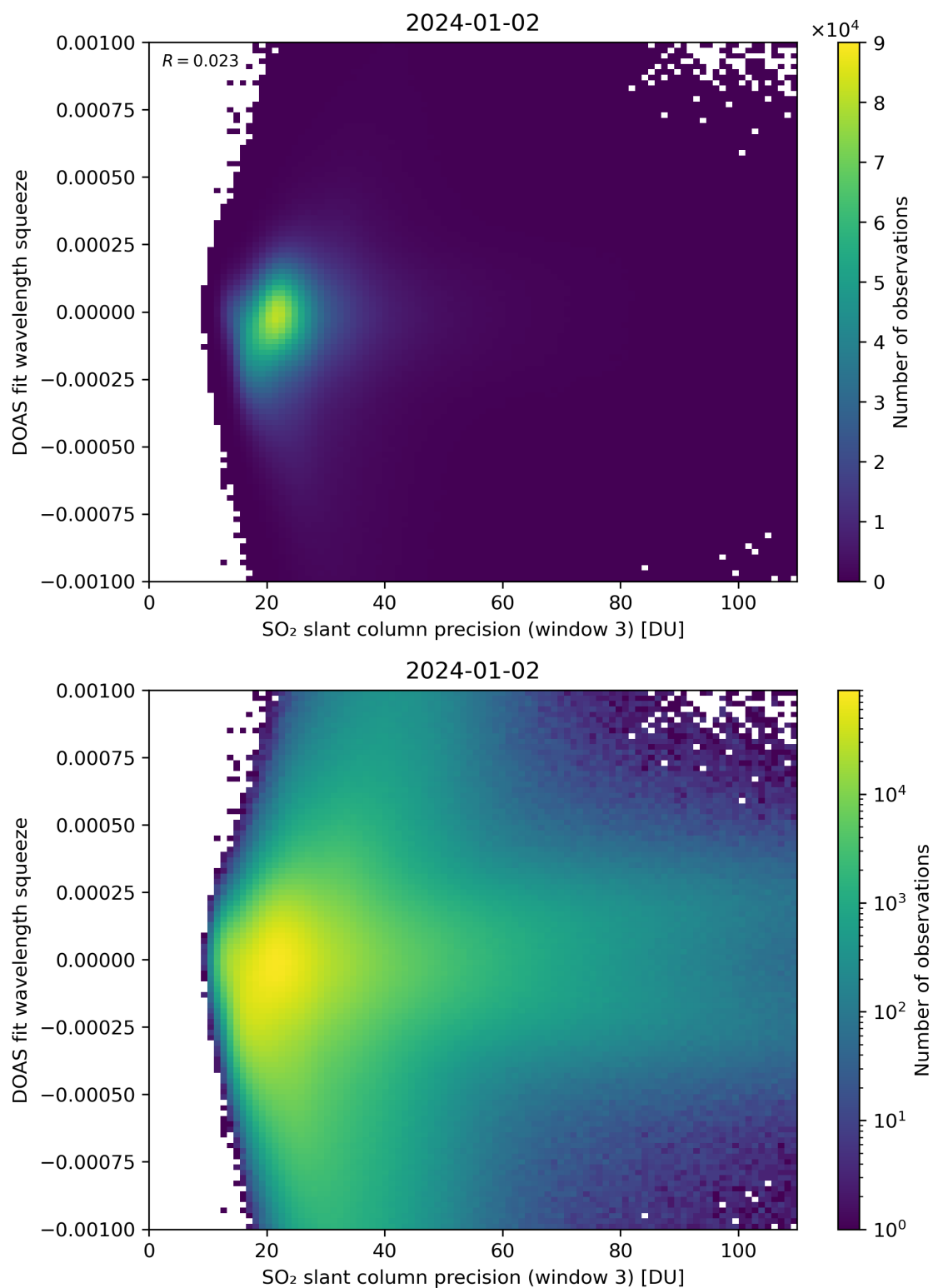
Figure 259: Scatter density plot of “SO 2 slant column precision (window 3)” against “DOAS fit wavelength squeeze” for 2024-01-01 to 2024-01-03.
