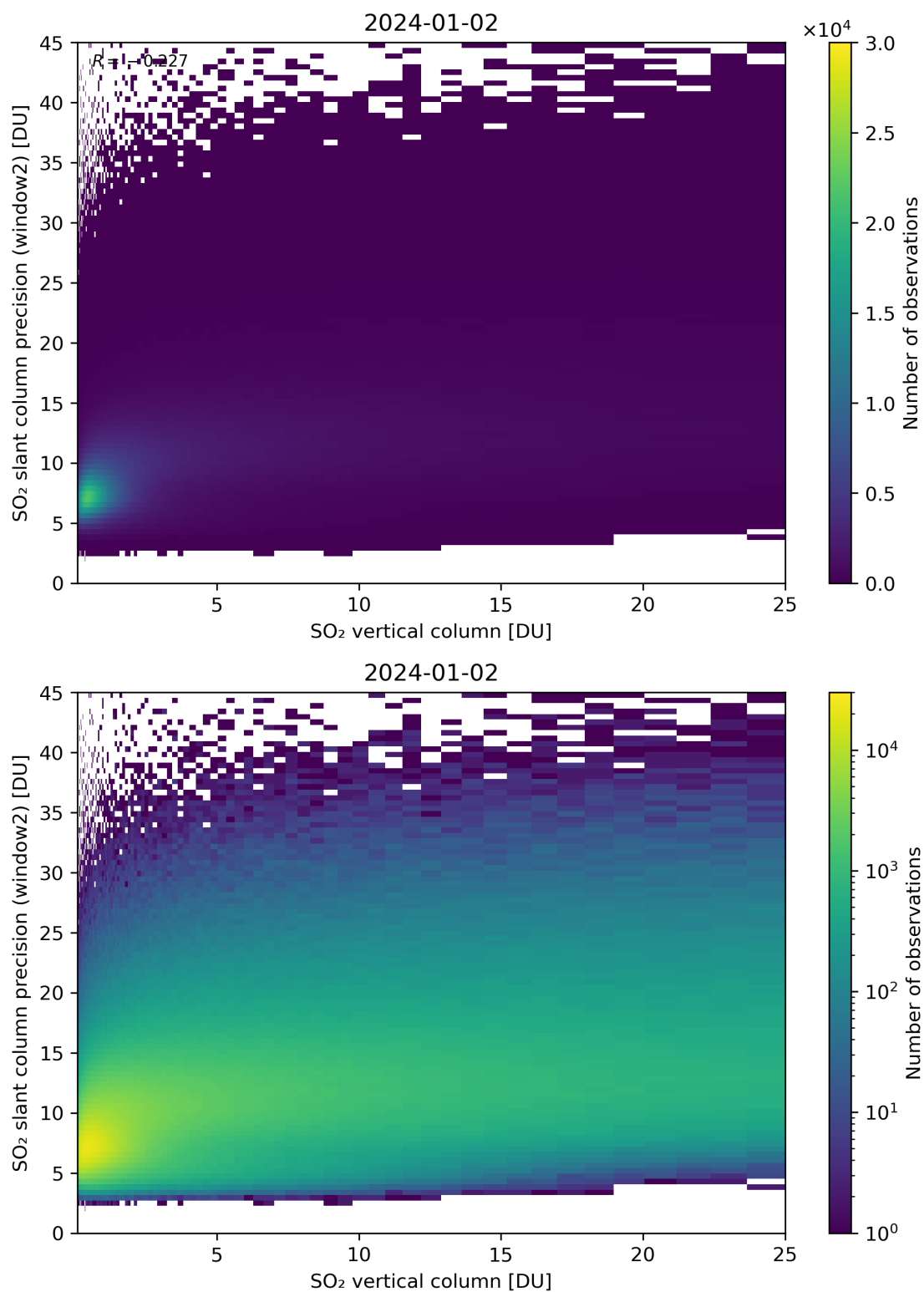
Figure 302: Scatter density plot of “SO 2 vertical column” against “SO 2 slant column precision (window2)” for 2024-01-01 to 2024-01-03.
