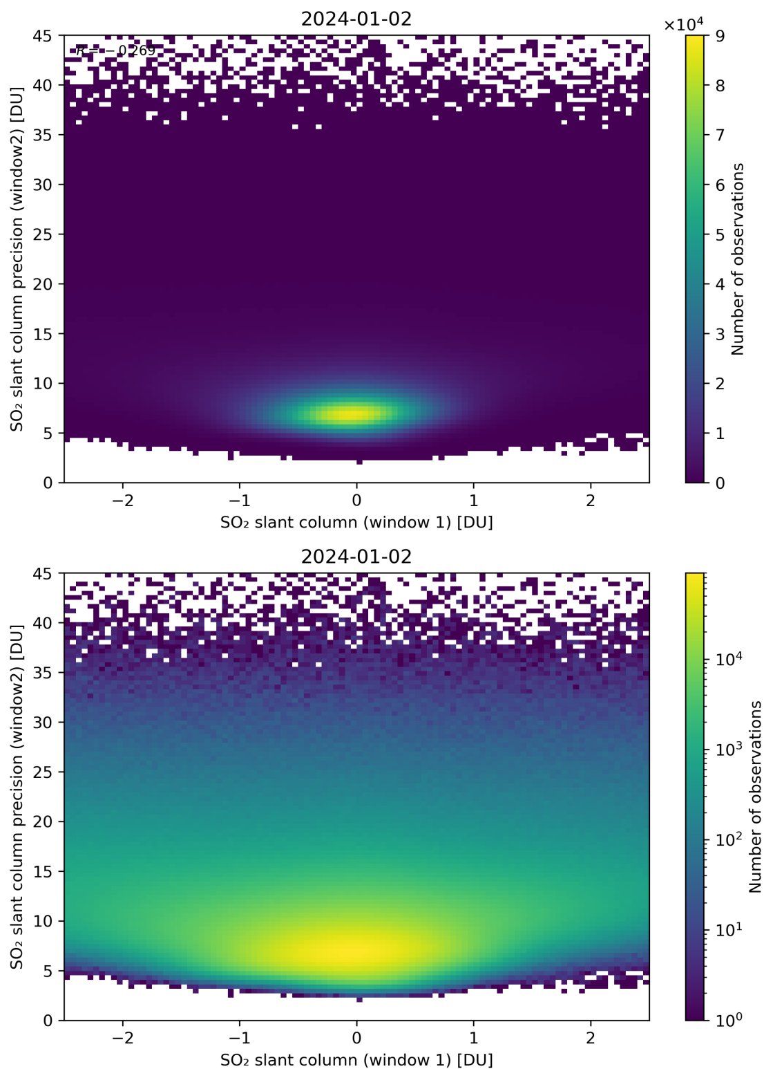
Figure 236: Scatter density plot of “SO 2 slant column (window 1)” against “SO 2 slant column precision (window2)” for 2024-01-01 to 2024-01-03.
