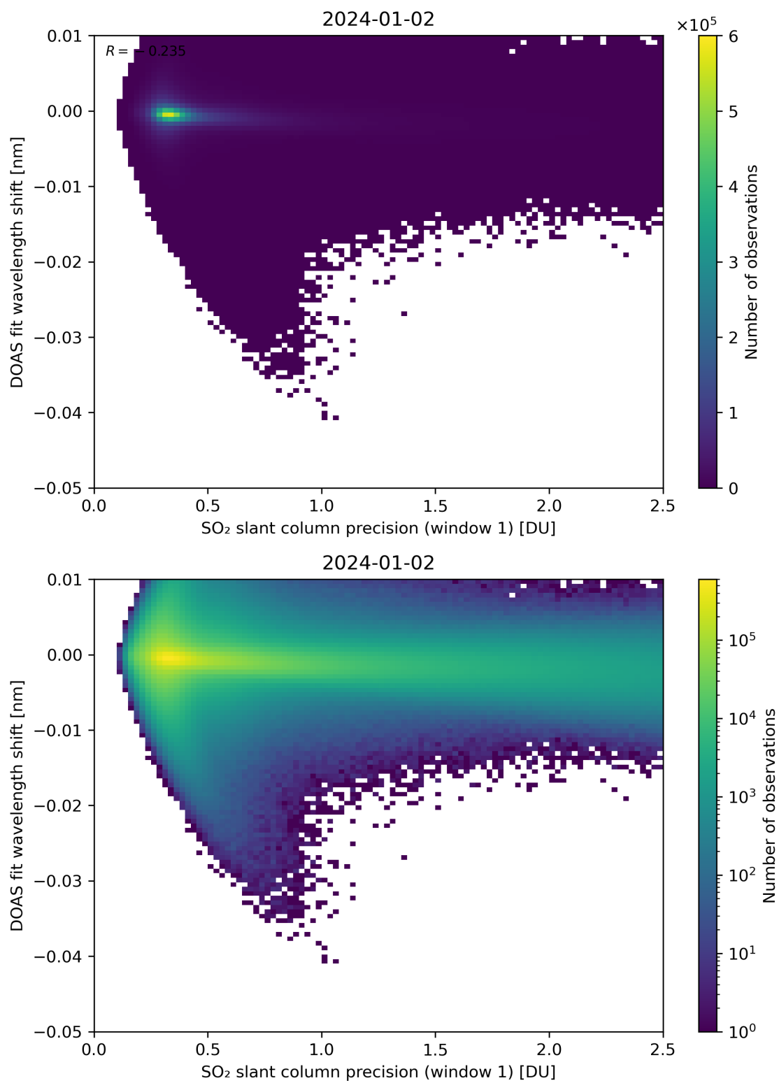
Figure 221: Scatter density plot of “SO 2 slant column precision (window 1)” against “DOAS fit wavelength shift” for 2024-01-01 to 2024-01-03.
