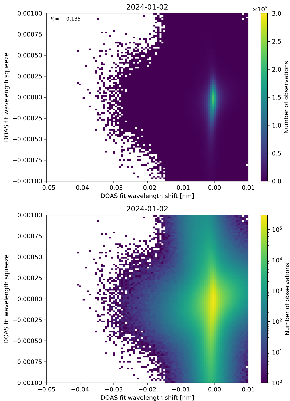
Figure 127: Scatter density plot of “DOAS fit wavelength shift” against “DOAS fit wavelength squeeze” for 2024-01-01 to 2024-01-03.
