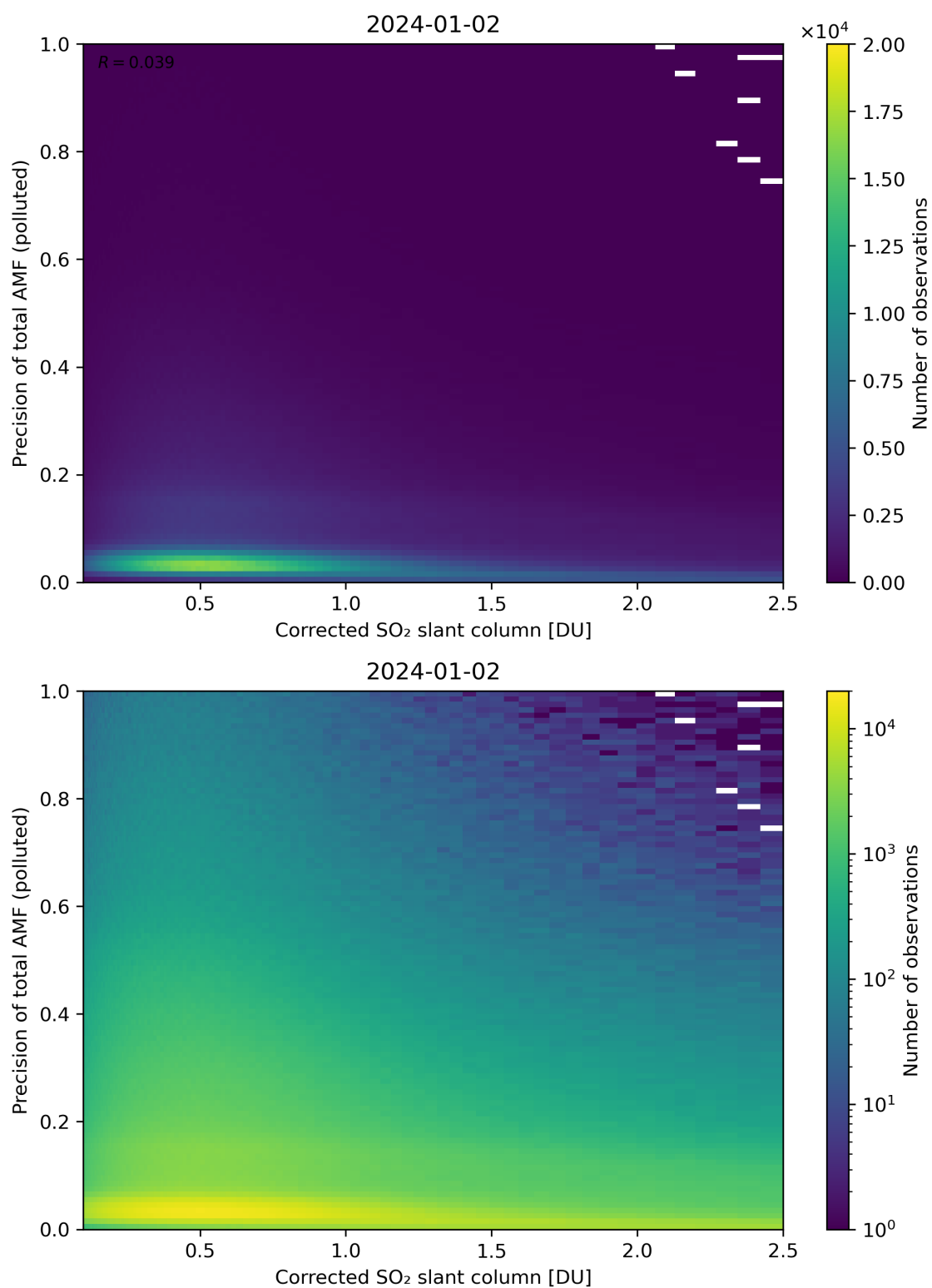
Figure 193: Scatter density plot of “Corrected SO 2 slant column” against “Precision of total AMF (polluted)” for 2024-01-01 to 2024-01-03.
