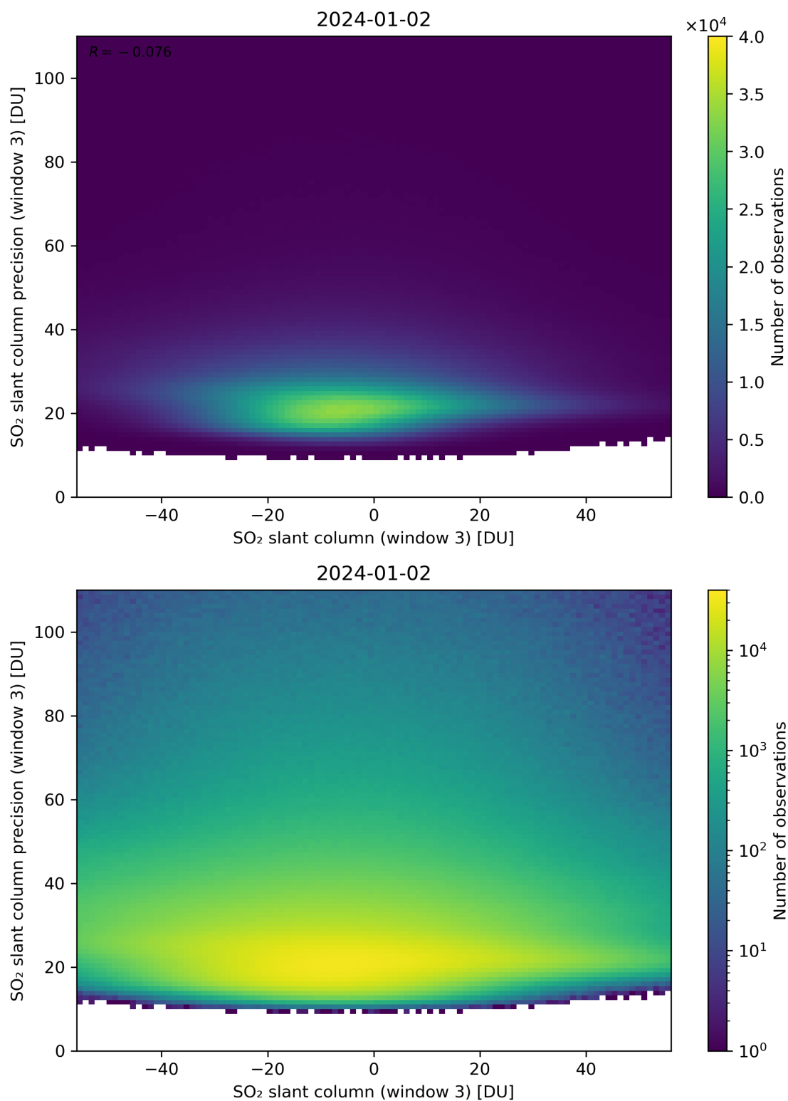
Figure 267: Scatter density plot of “SO 2 slant column (window 3)” against “SO 2 slant column precision (window 3)” for 2024-01-01 to 2024-01-03.
