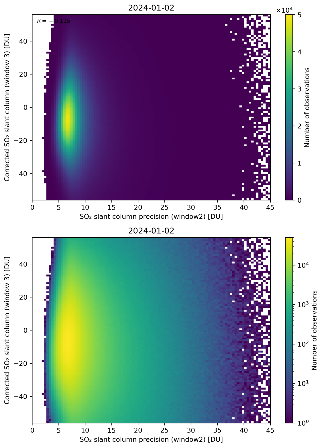
Figure 248: Scatter density plot of “SO 2 slant column precision (window2)” against “Corrected SO 2 slant column (window 3)” for 2024-01-01 to 2024-01-03.
