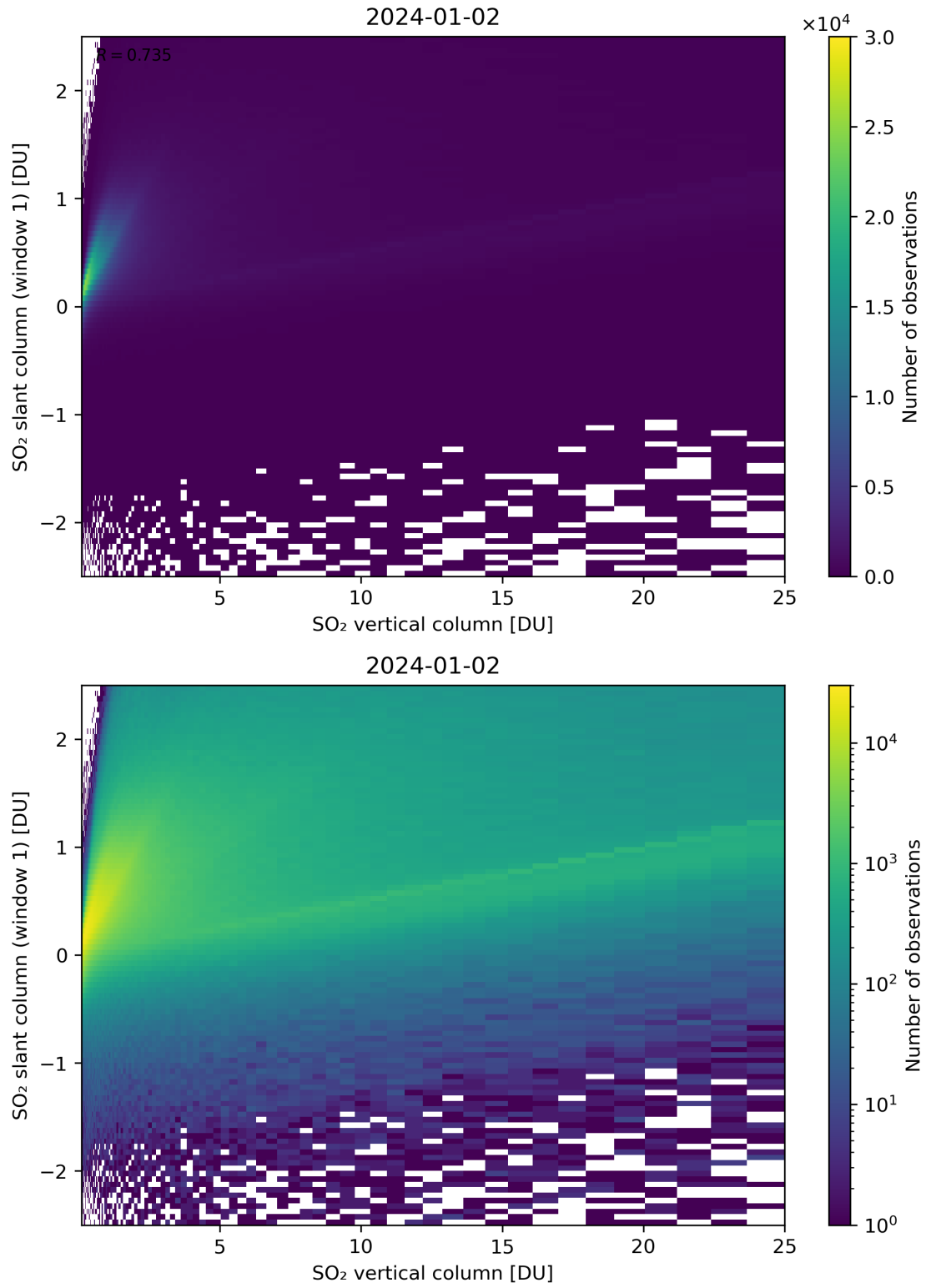
Figure 300: Scatter density plot of “SO 2 vertical column” against “SO 2 slant column (window 1)” for 2024-01-01 to 2024-01-03.
