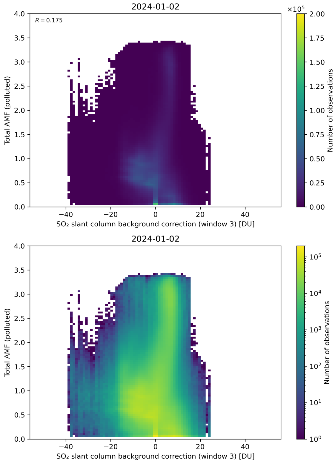
Figure 125: Scatter density plot of “SO 2 slant column background correction (window 3)” against “Total AMF (polluted)” for 2024-01-01 to 2024-01-03.
