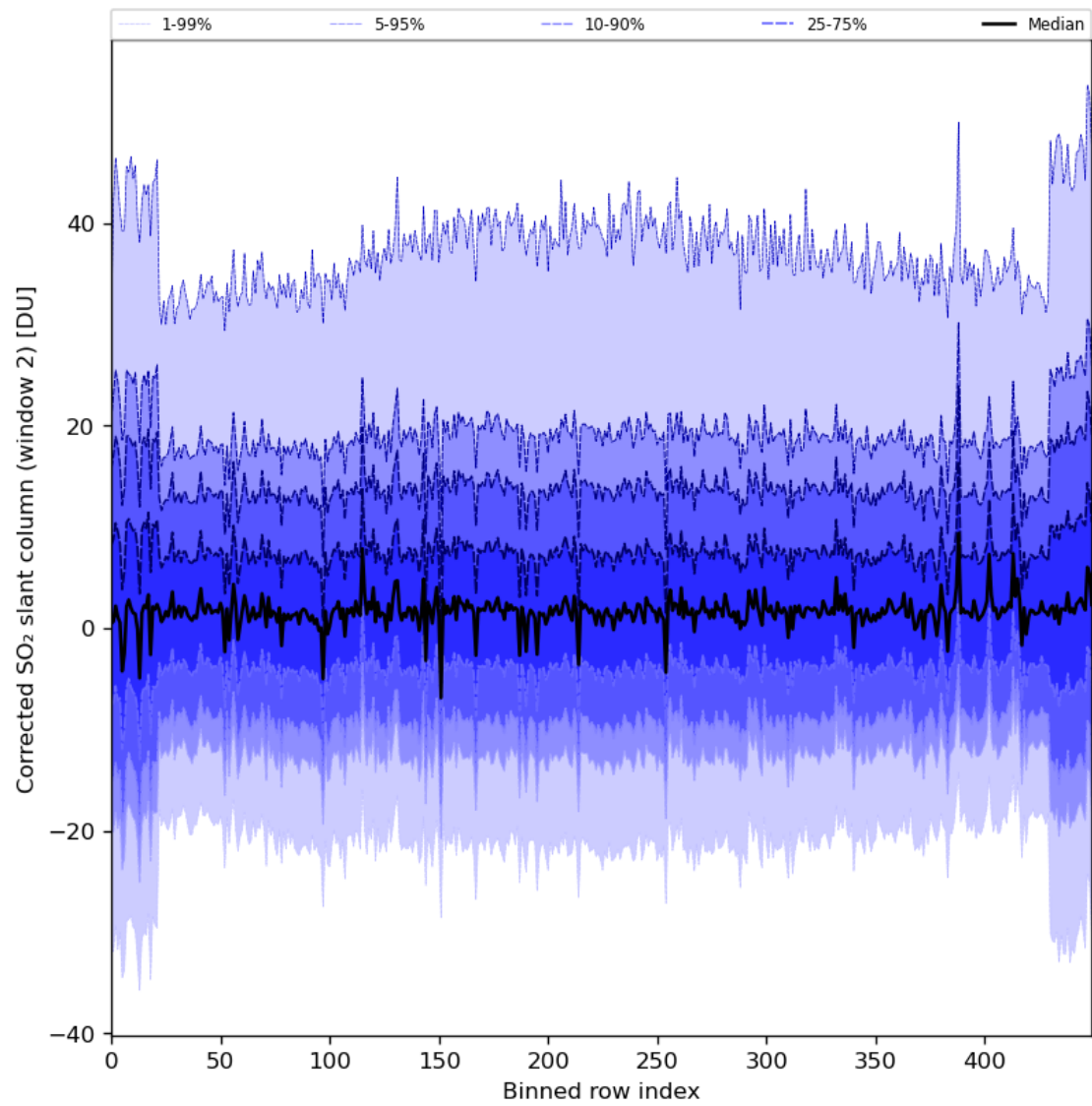
Figure 85: Along track statistics of “Corrected SO 2 slant column (window 2)” for 2024-01-01 to 2024-01-03
