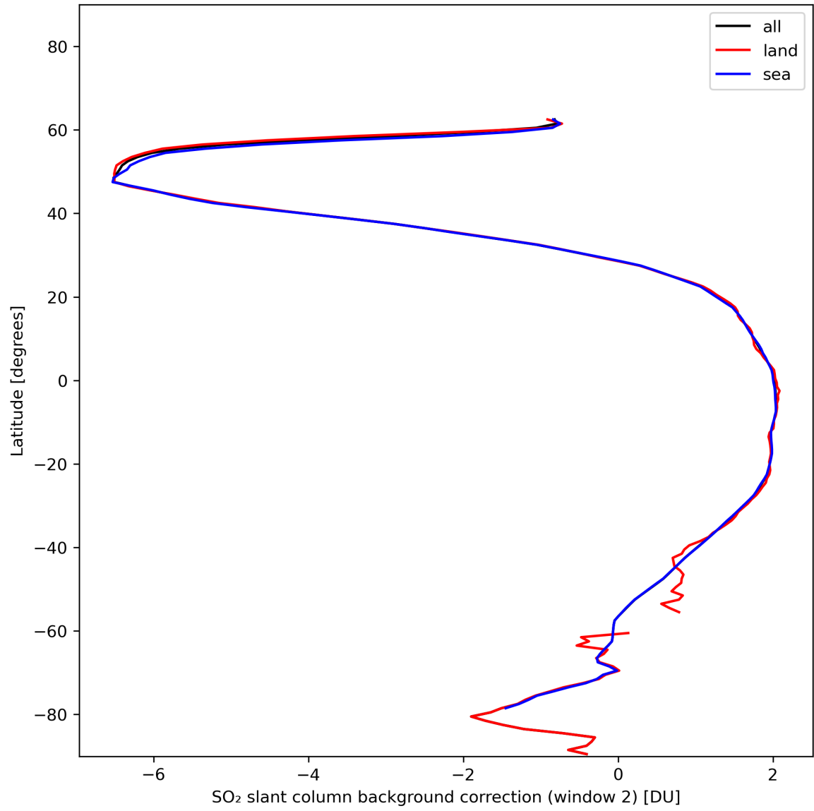
Figure 40: Zonal average of “SO 2 slant column background correction (window 2)” for 2024-01-01 to 2024-01-03.
