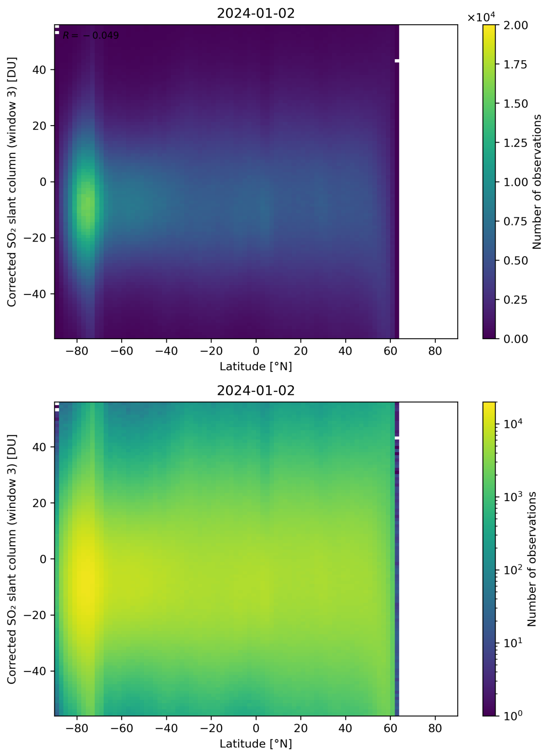
Figure 148: Scatter density plot of “Latitude” against “Corrected SO 2 slant column (window 3)” for 2024-01-01 to 2024-01-03.
