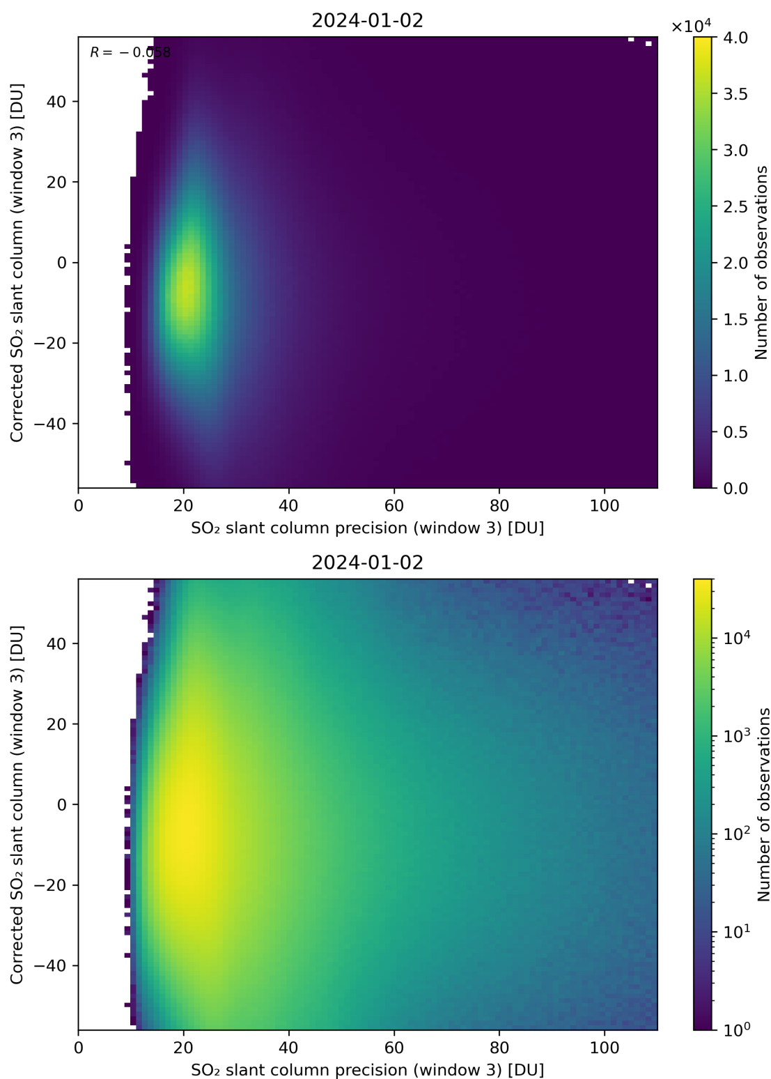
Figure 262: Scatter density plot of “SO 2 slant column precision (window 3)” against “Corrected SO 2 slant column (window 3)” for 2024-01-01 to 2024-01-03.
