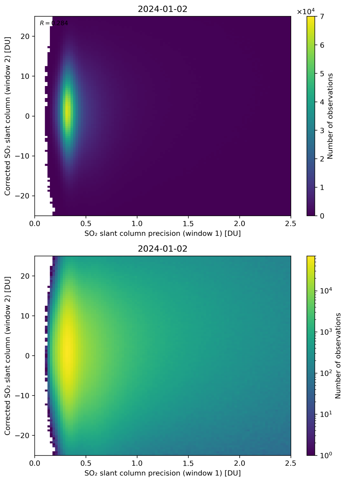
Figure 225: Scatter density plot of “SO 2 slant column precision (window 1)” against “Corrected SO 2 slant column (window 2)” for 2024-01-01 to 2024-01-03.
