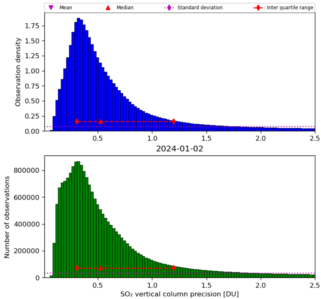
Figure 54: Histogram of “SO 2 vertical column precision” for 2024-01-01 to 2024-01-03
