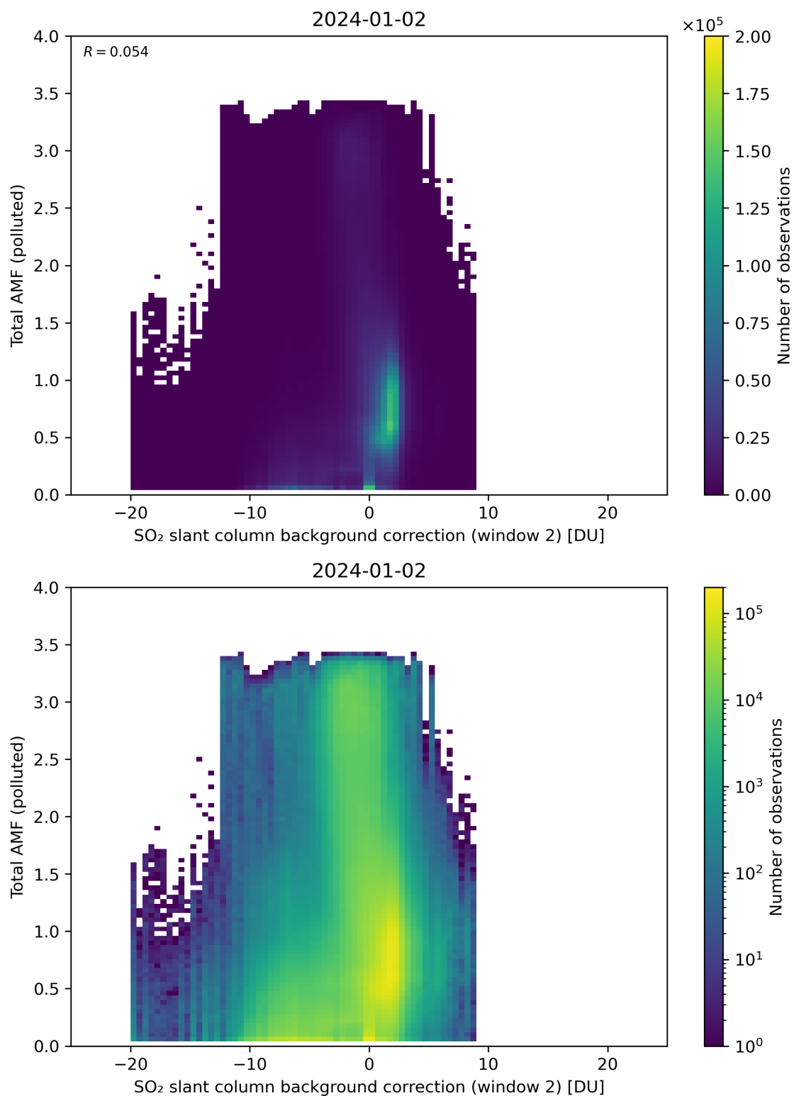
Figure 119: Scatter density plot of “SO 2 slant column background correction (window 2)” against “Total AMF (polluted)” for 2024-01-01 to 2024-01-03.
