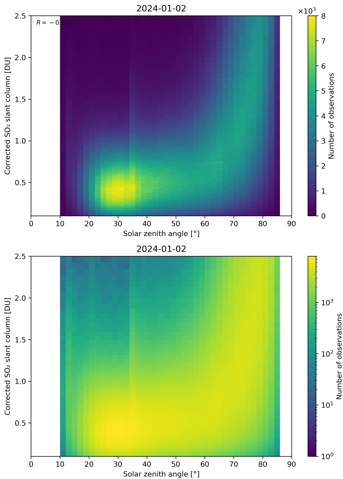
Figure 166: Scatter density plot of “Solar zenith angle” against “Corrected SO 2 slant column” for 2024-01-01 to 2024-01-03.
