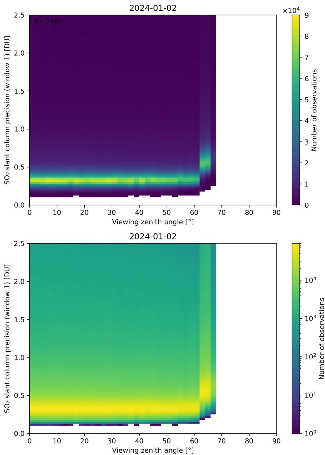
Figure 321: Scatter density plot of “Viewing zenith angle” against “SO 2 slant column precision (window 1)” for 2024-01-01 to 2024-01-03.
