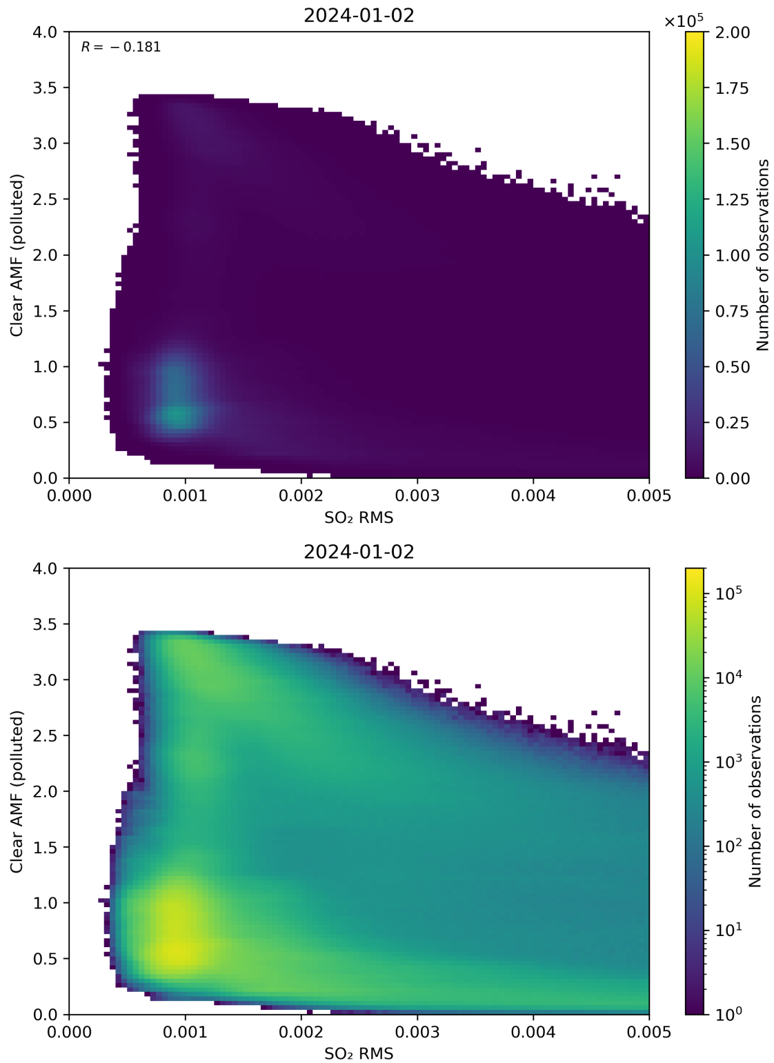
Figure 136: Scatter density plot of “SO 2 RMS” against “Clear AMF (polluted)” for 2024-01-01 to 2024-01-03.
