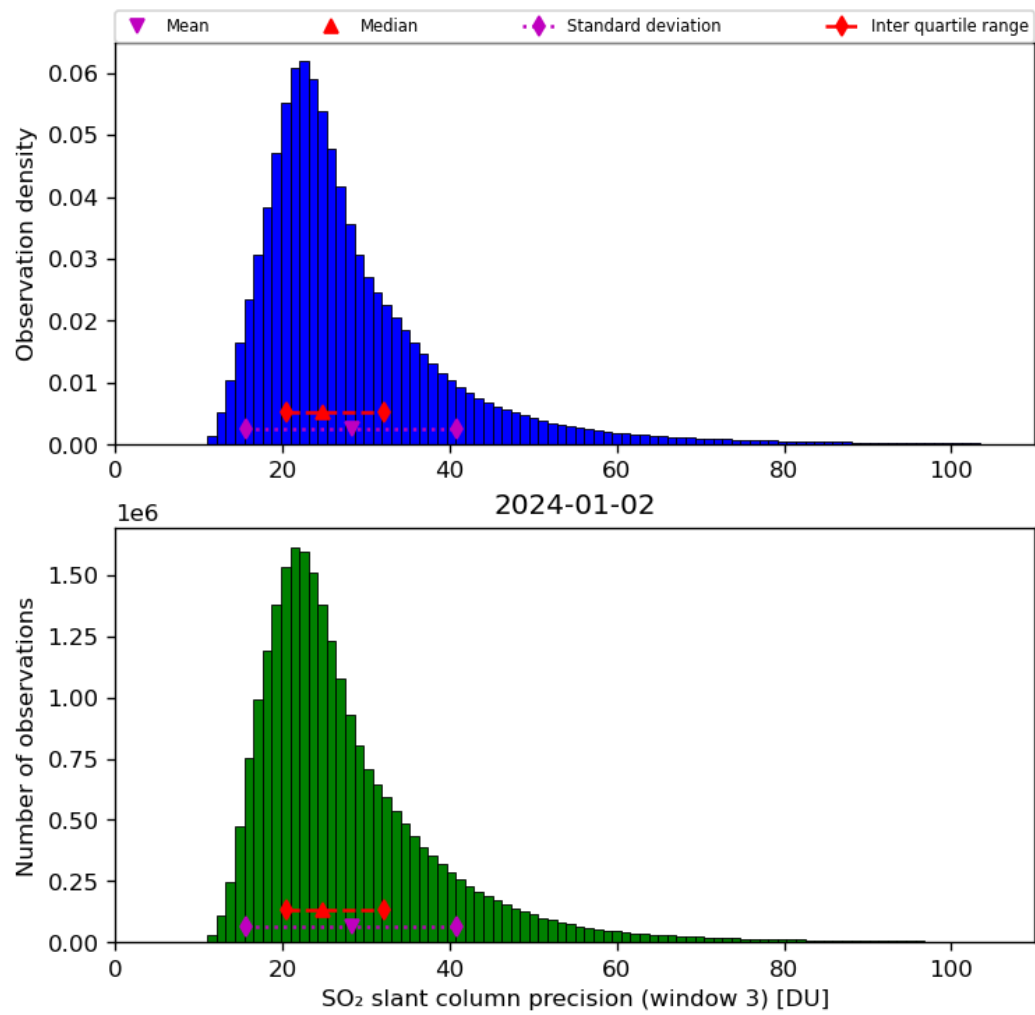
Figure 65: Histogram of “SO 2 slant column precision (window 3)” for 2024-01-01 to 2024-01-03
