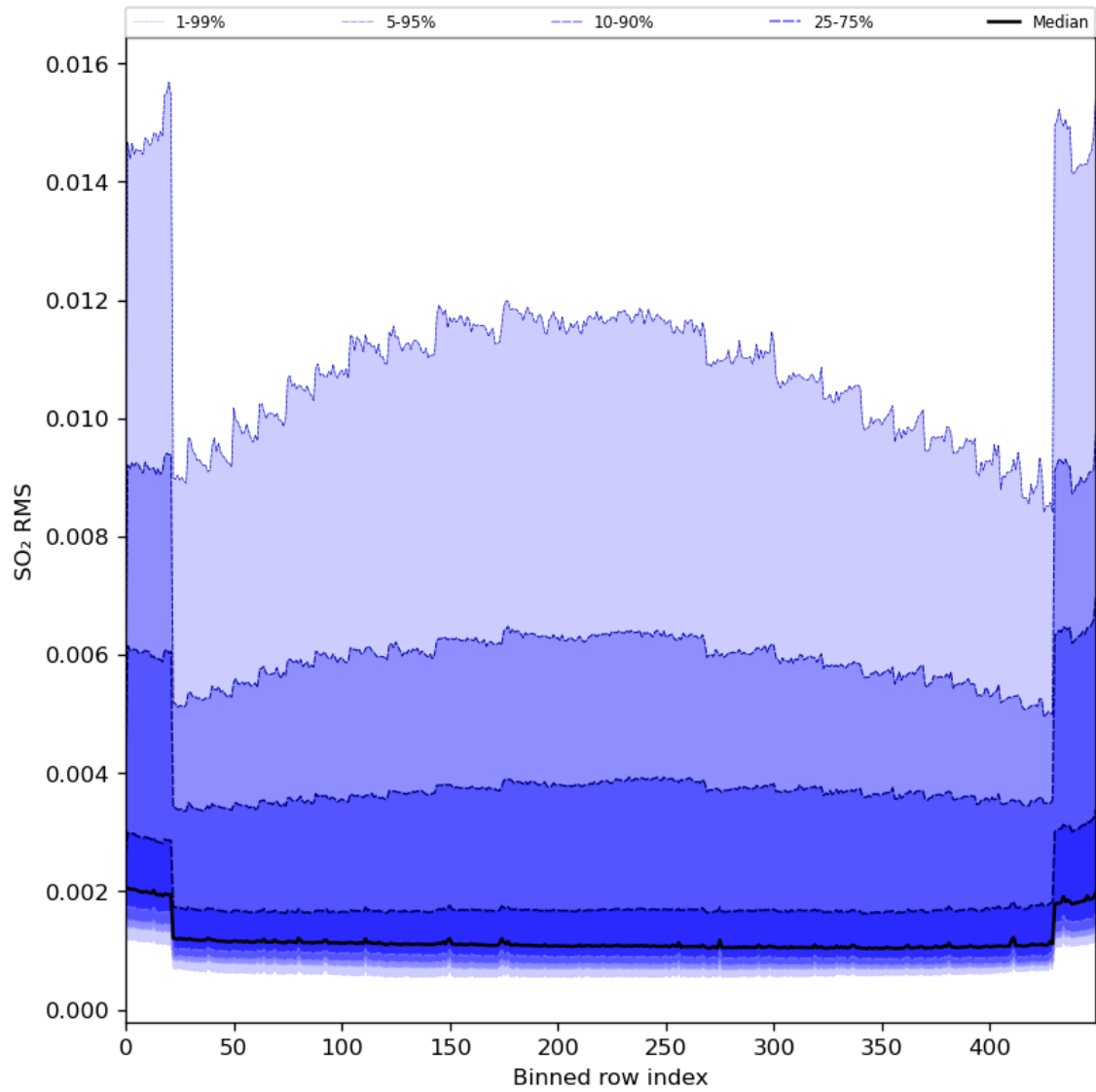
Figure 93: Along track statistics of “SO 2 RMS” for 2024-01-01 to 2024-01-03
