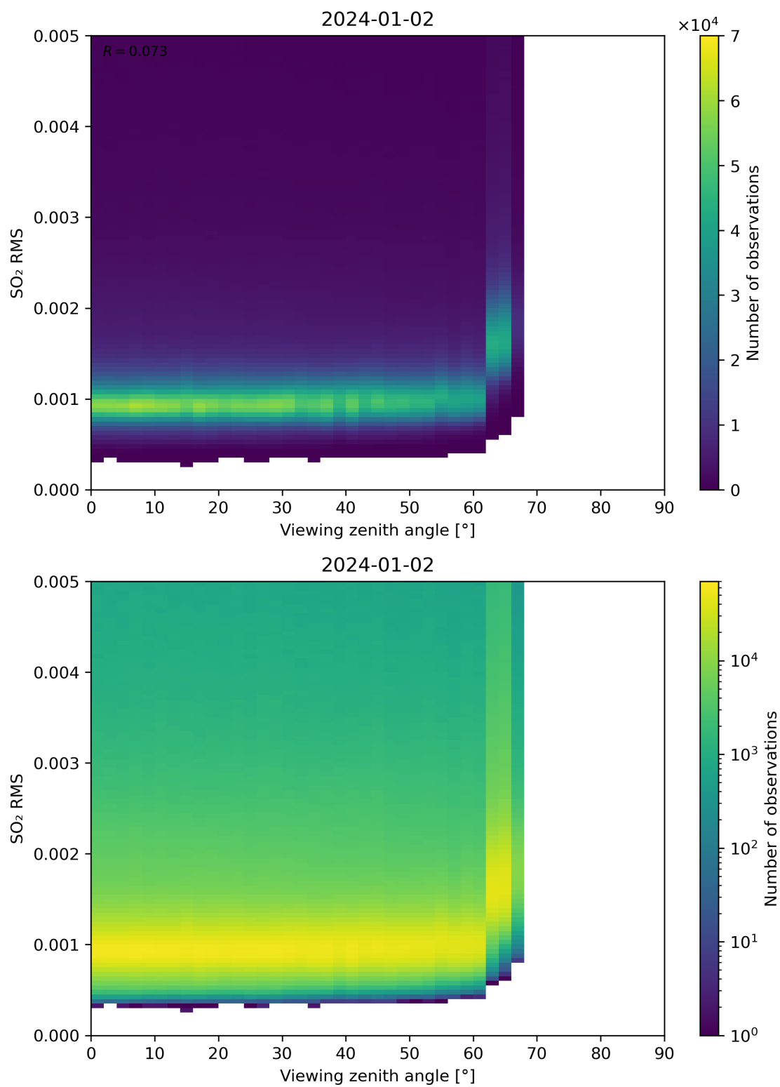
Figure 313: Scatter density plot of “Viewing zenith angle” against “SO 2 RMS” for 2024-01-01 to 2024-01-03.
