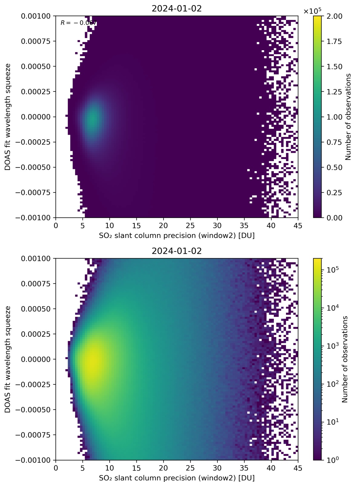
Figure 244: Scatter density plot of “SO 2 slant column precision (window2)” against “DOAS fit wavelength squeeze” for 2024-01-01 to 2024-01-03.
