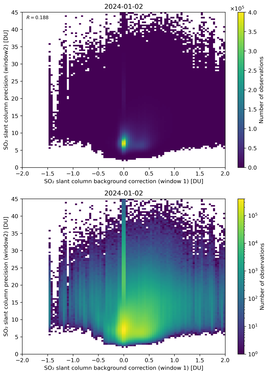
Figure 106: Scatter density plot of “SO 2 slant column background correction (window 1)” against “SO 2 slant column precision (window2)” for 2024-01-01 to 2024-01-03.
