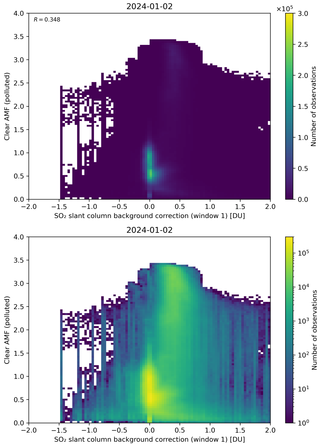
Figure 103: Scatter density plot of “SO 2 slant column background correction (window 1)” against “Clear AMF (polluted)” for 2024-01-01 to 2024-01-03.
