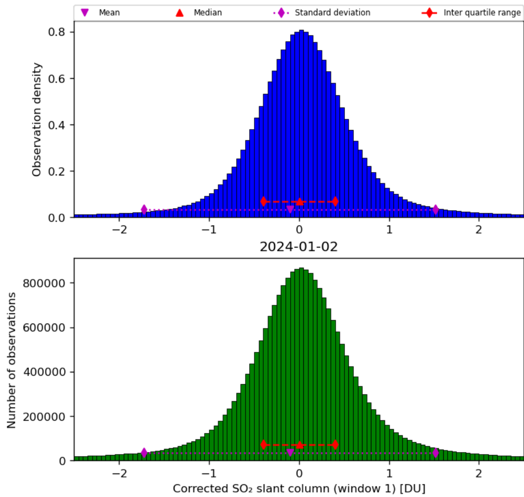
Figure 58: Histogram of “Corrected SO 2 slant column (window 1)” for 2024-01-01 to 2024-01-03
