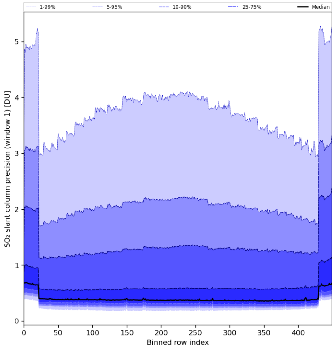
Figure 80: Along track statistics of “SO 2 slant column precision (window 1)” for 2024-01-01 to 2024-01-03
