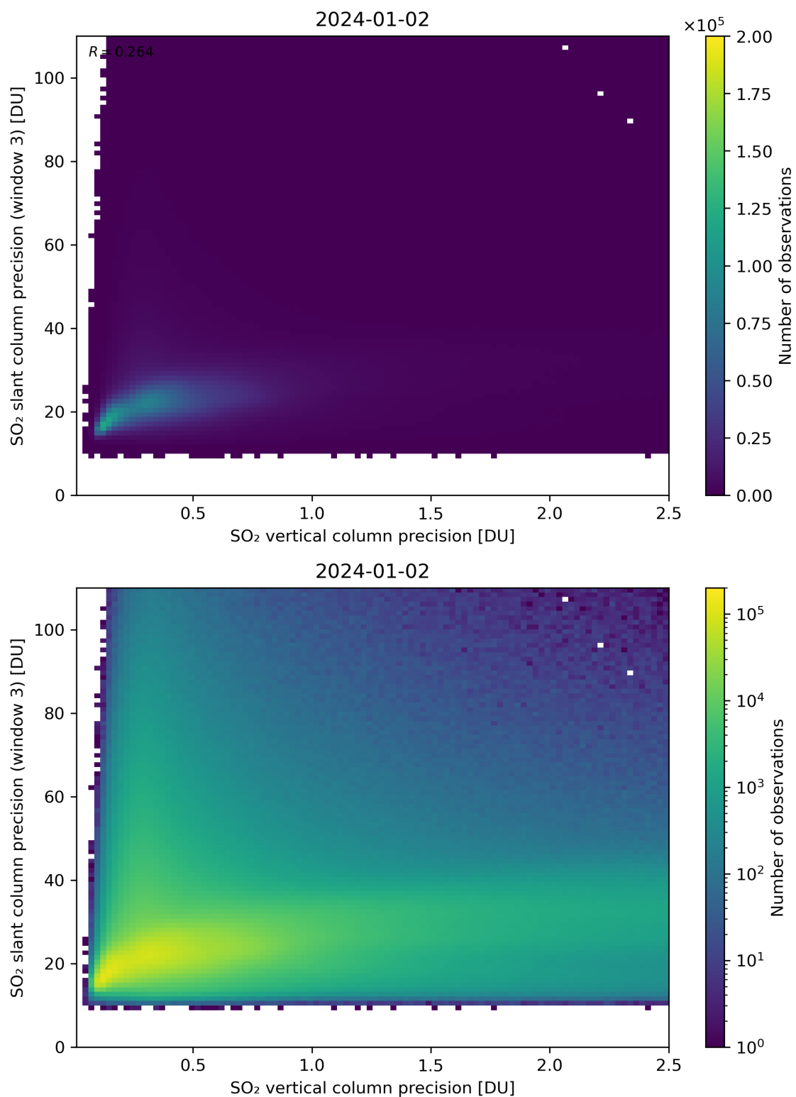
Figure 293: Scatter density plot of “SO 2 vertical column precision” against “SO 2 slant column precision (window 3)” for 2024-01-01 to 2024-01-03.
