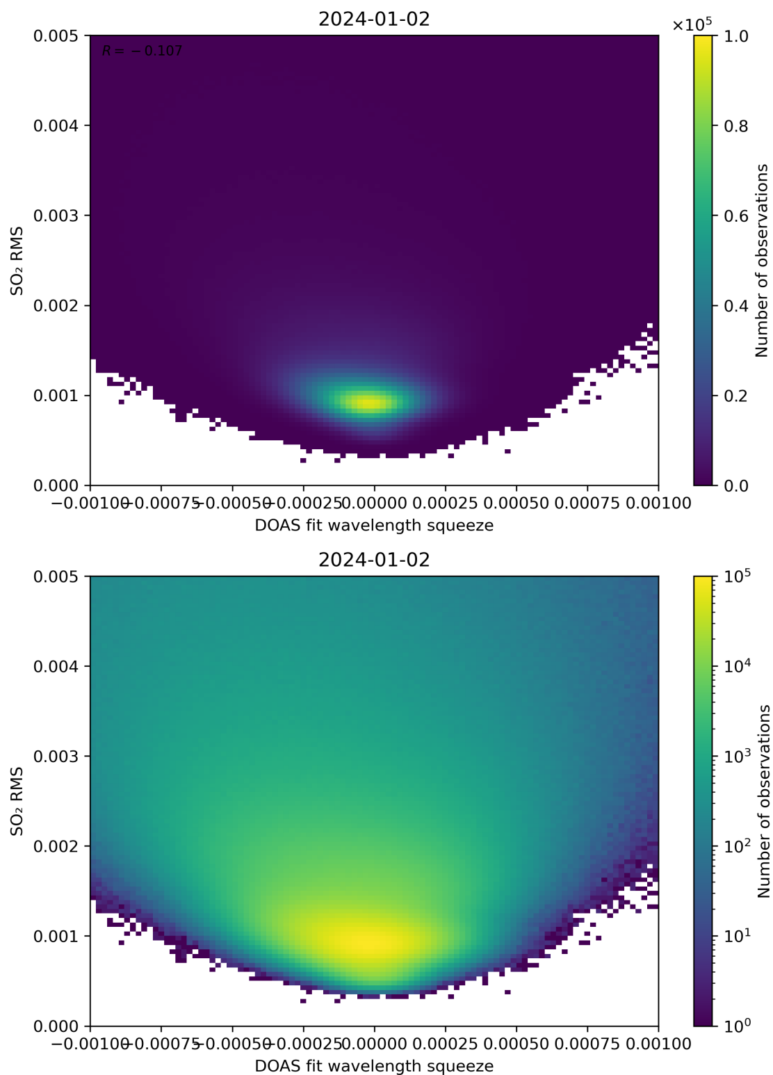
Figure 132: Scatter density plot of “DOAS fit wavelength squeeze” against “SO 2 RMS” for 2024-01-01 to 2024-01-03.
