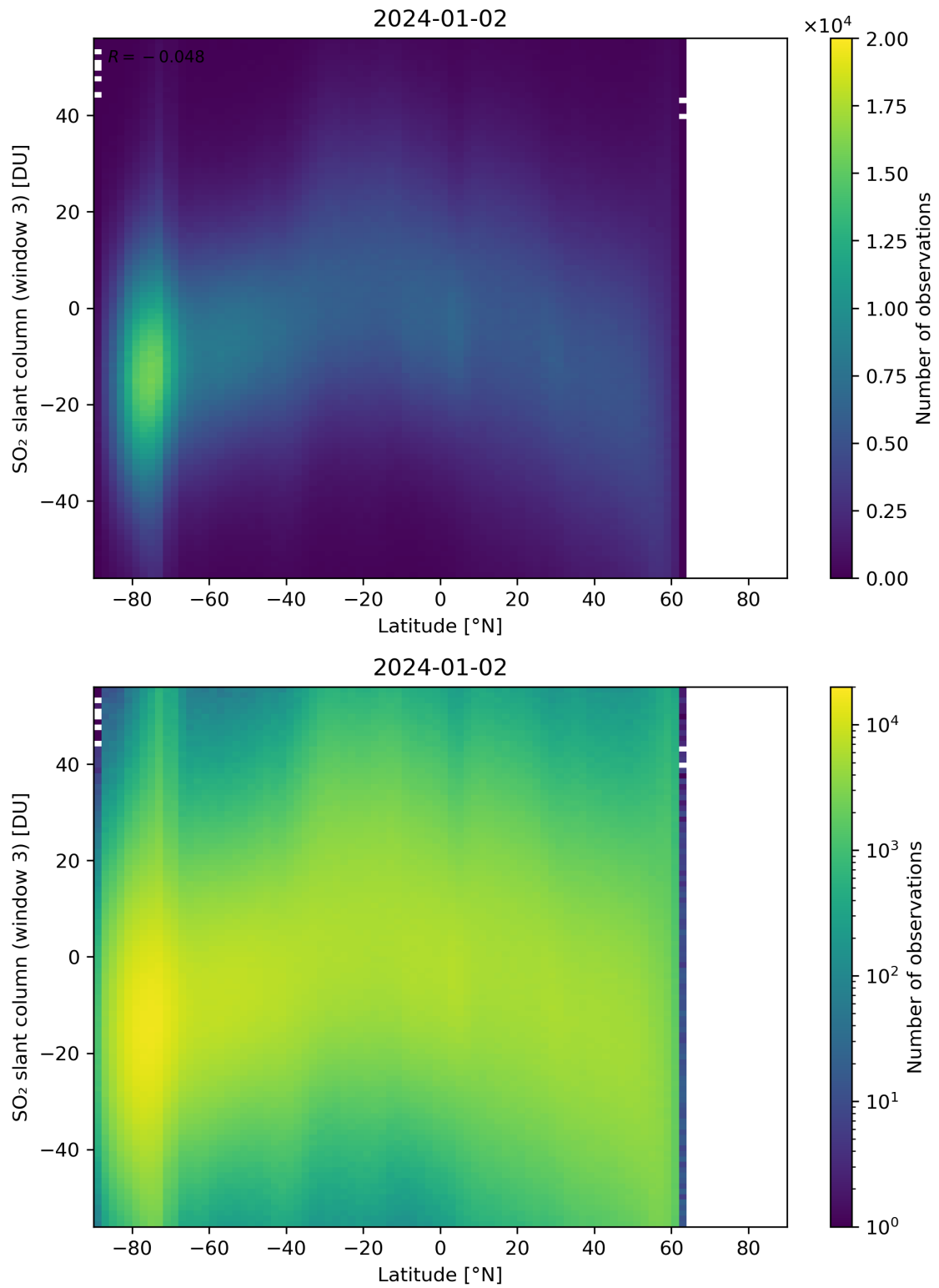
Figure 152: Scatter density plot of “Latitude” against “SO 2 slant column (window 3)” for 2024-01-01 to 2024-01-03.
