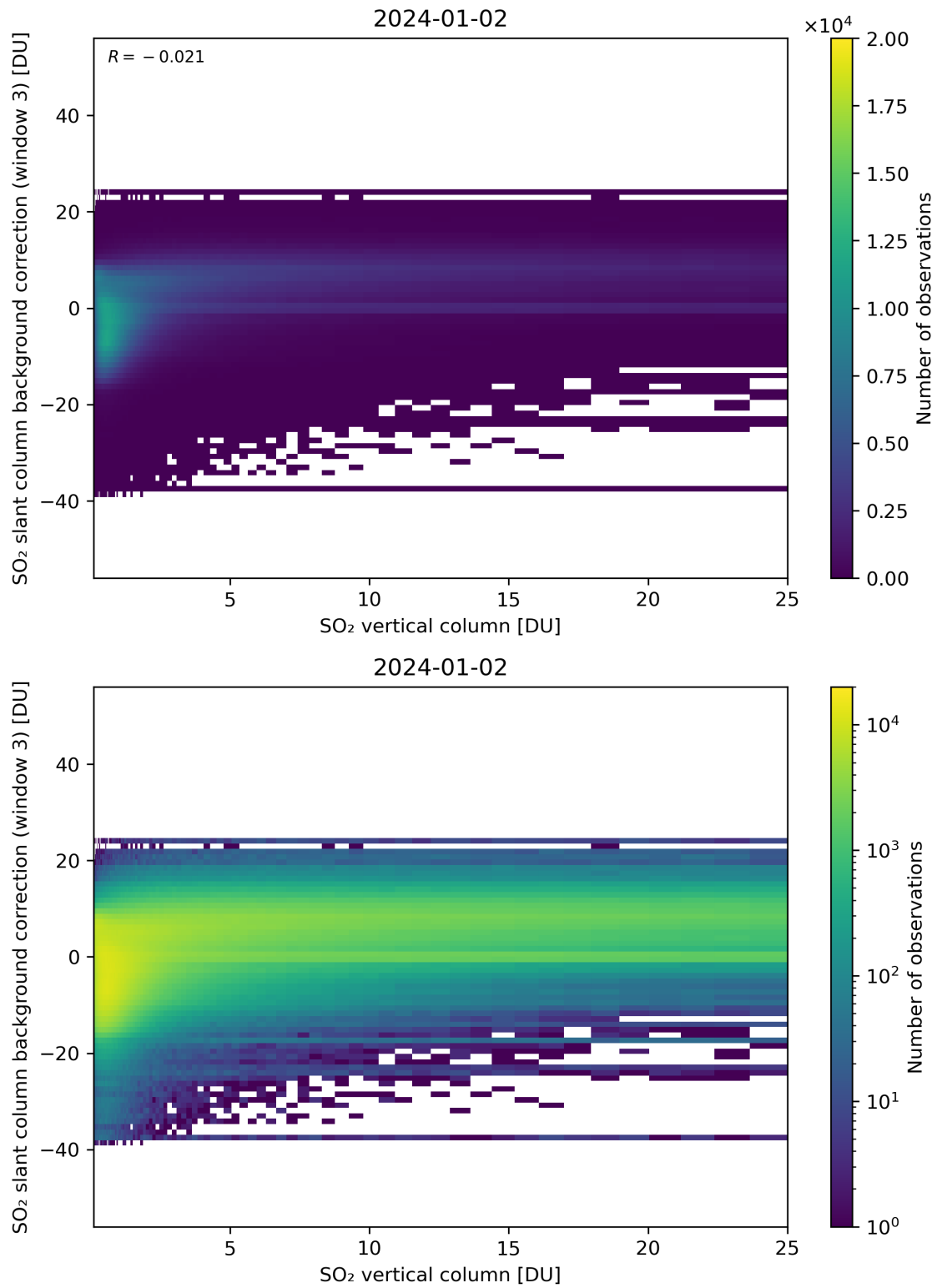
Figure 275: Scatter density plot of “SO 2 vertical column” against “SO 2 slant column background correction (window 3)” for 2024-01-01 to 2024-01-03.
