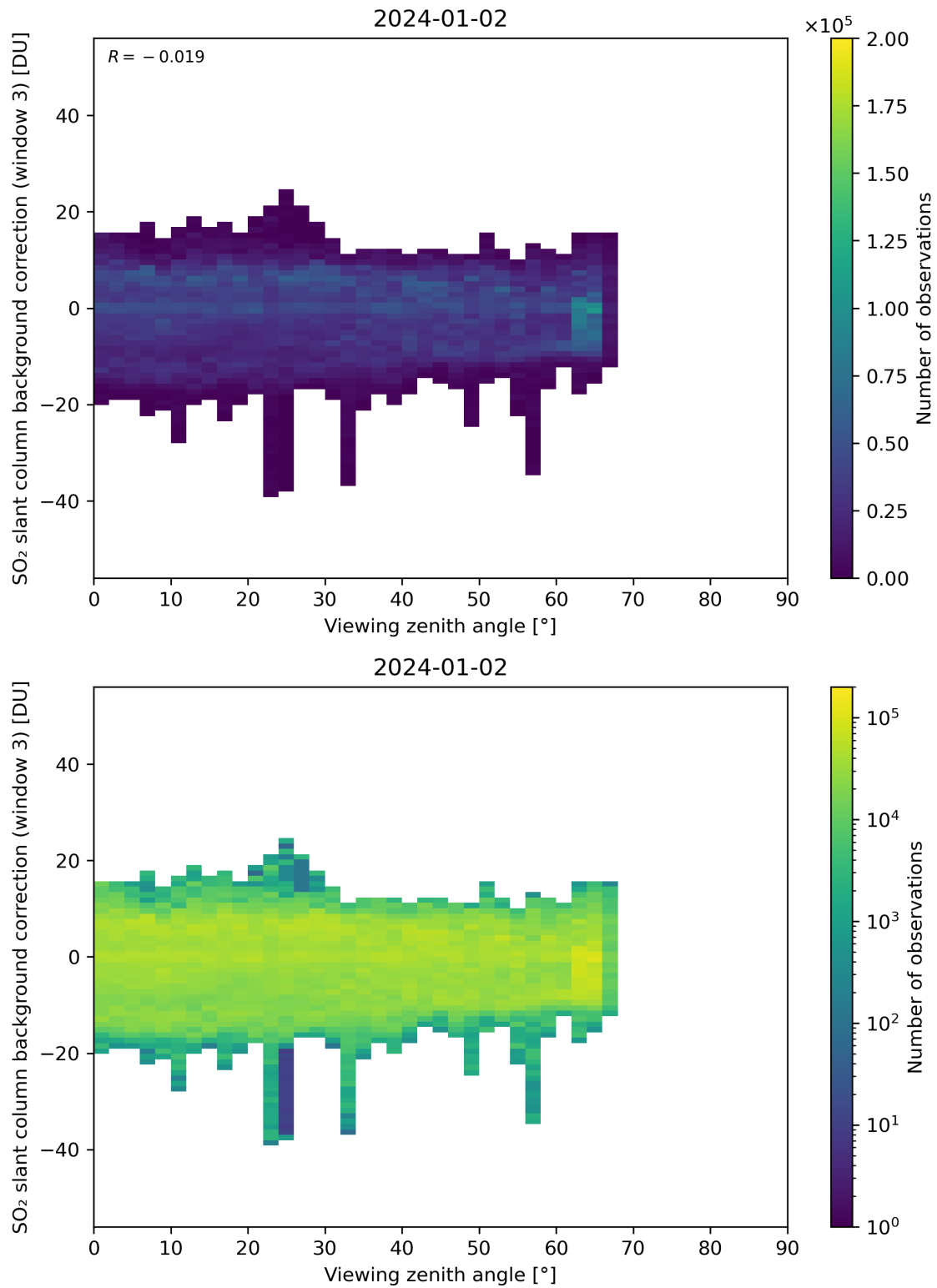
Figure 310: Scatter density plot of “Viewing zenith angle” against “SO 2 slant column background correction (window 3)” for 2024-01-01 to 2024-01-03.
