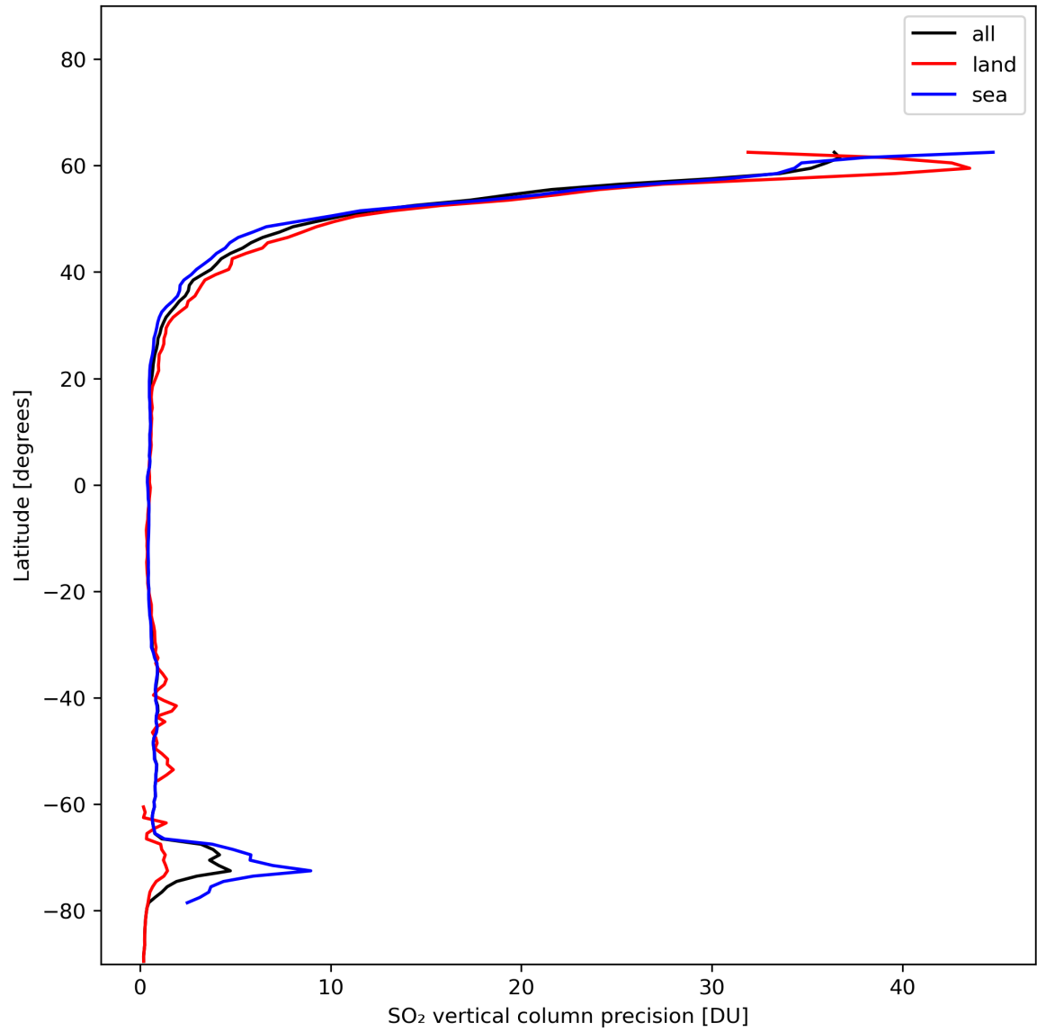
Figure 31: Zonal average of “SO 2 vertical column precision” for 2024-01-01 to 2024-01-03.
