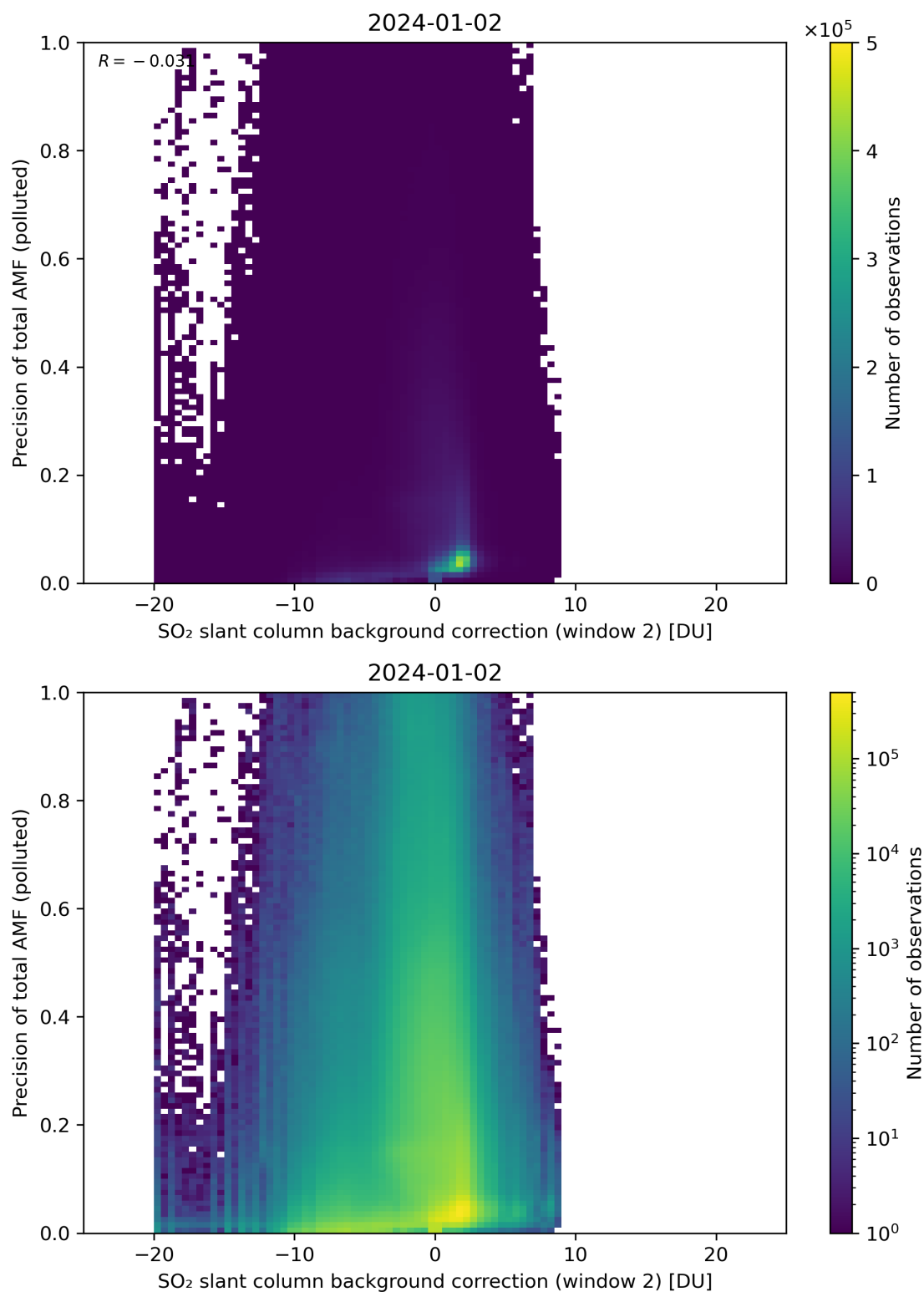
Figure 120: Scatter density plot of “SO 2 slant column background correction (window 2)” against “Precision of total AMF (polluted)” for 2024-01-01 to 2024-01-03.
