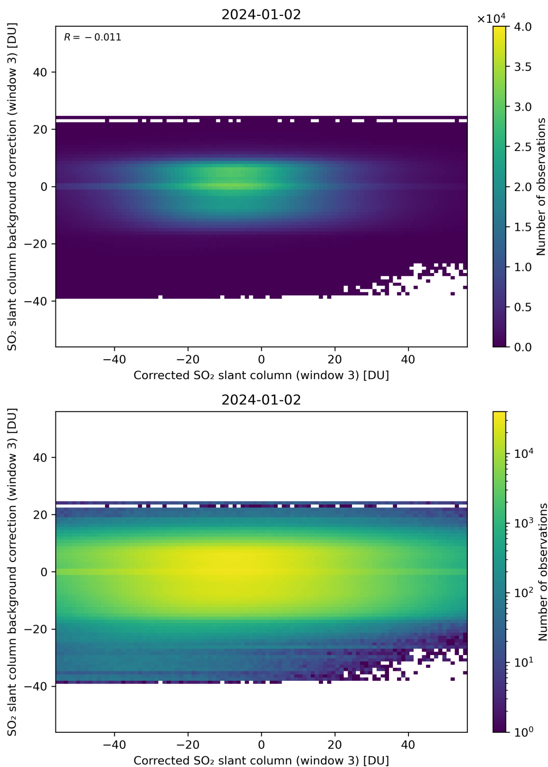
Figure 205: Scatter density plot of “Corrected SO 2 slant column (window 3)” against “SO 2 slant column background correction (window 3)” for 2024-01-01 to 2024-01-03.
