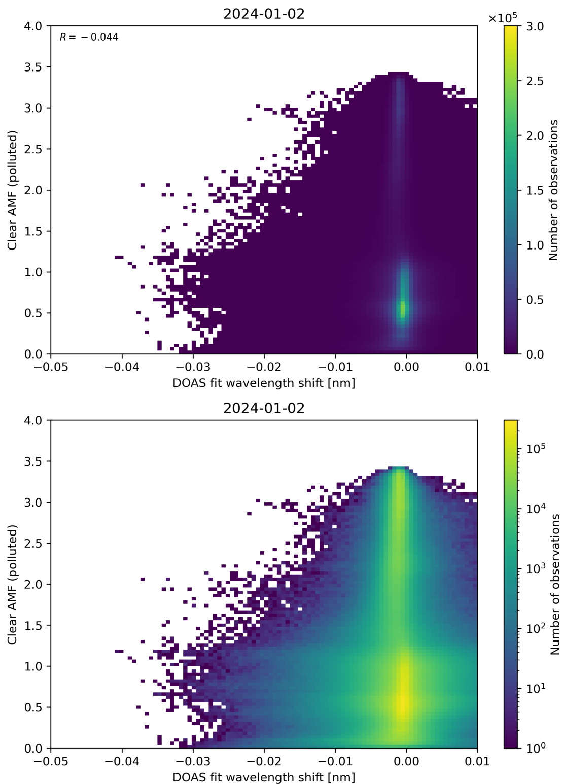
Figure 129: Scatter density plot of “DOAS fit wavelength shift” against “Clear AMF (polluted)” for 2024-01-01 to 2024-01-03.
