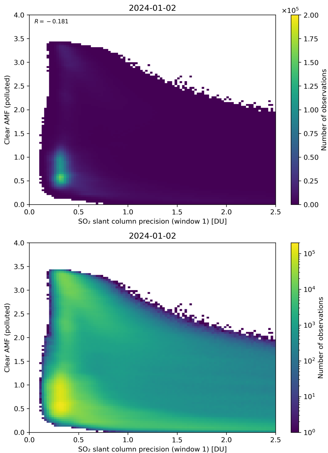
Figure 224: Scatter density plot of “SO 2 slant column precision (window 1)” against “Clear AMF (polluted)” for 2024-01-01 to 2024-01-03.
