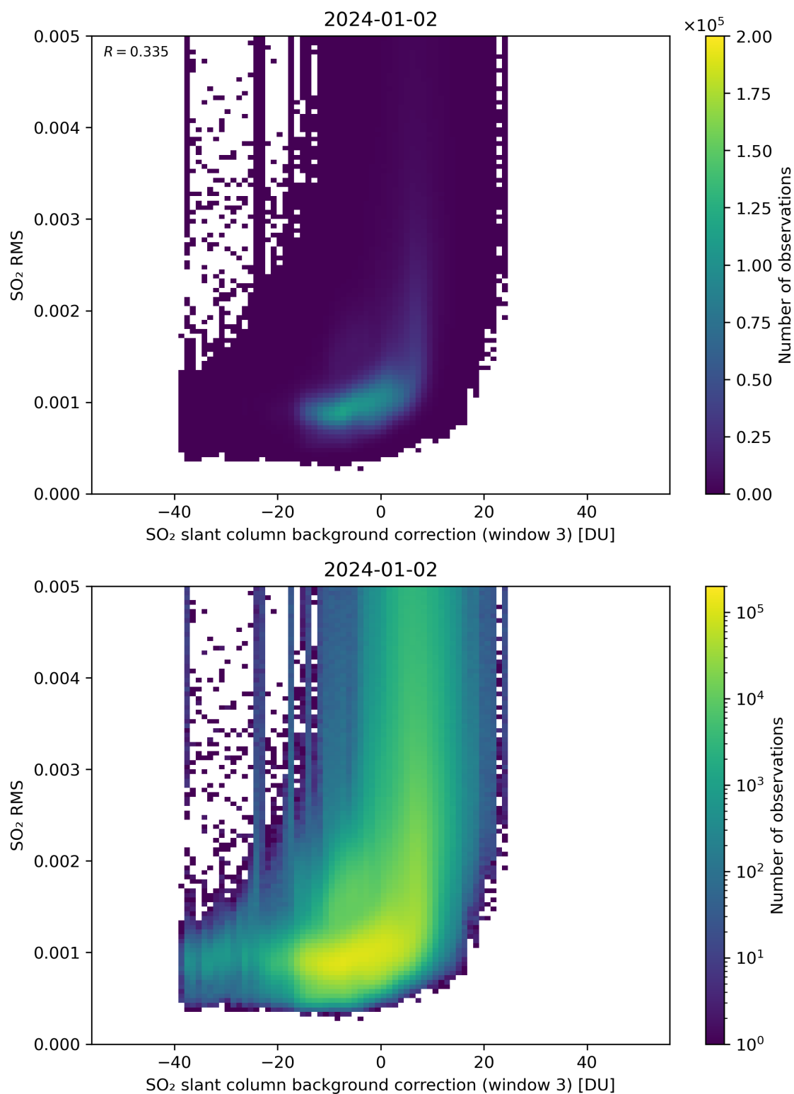
Figure 123: Scatter density plot of “SO 2 slant column background correction (window 3)” against “SO 2 RMS” for 2024-01-01 to 2024-01-03.
