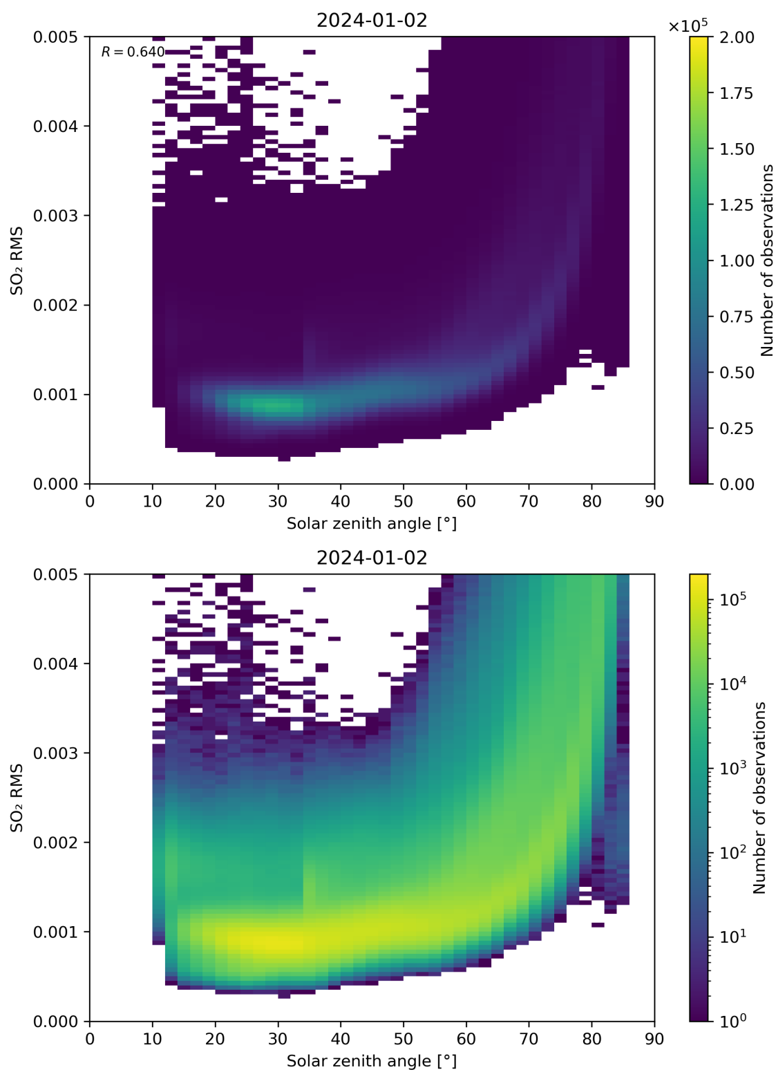
Figure 163: Scatter density plot of “Solar zenith angle” against “SO 2 RMS” for 2024-01-01 to 2024-01-03.
