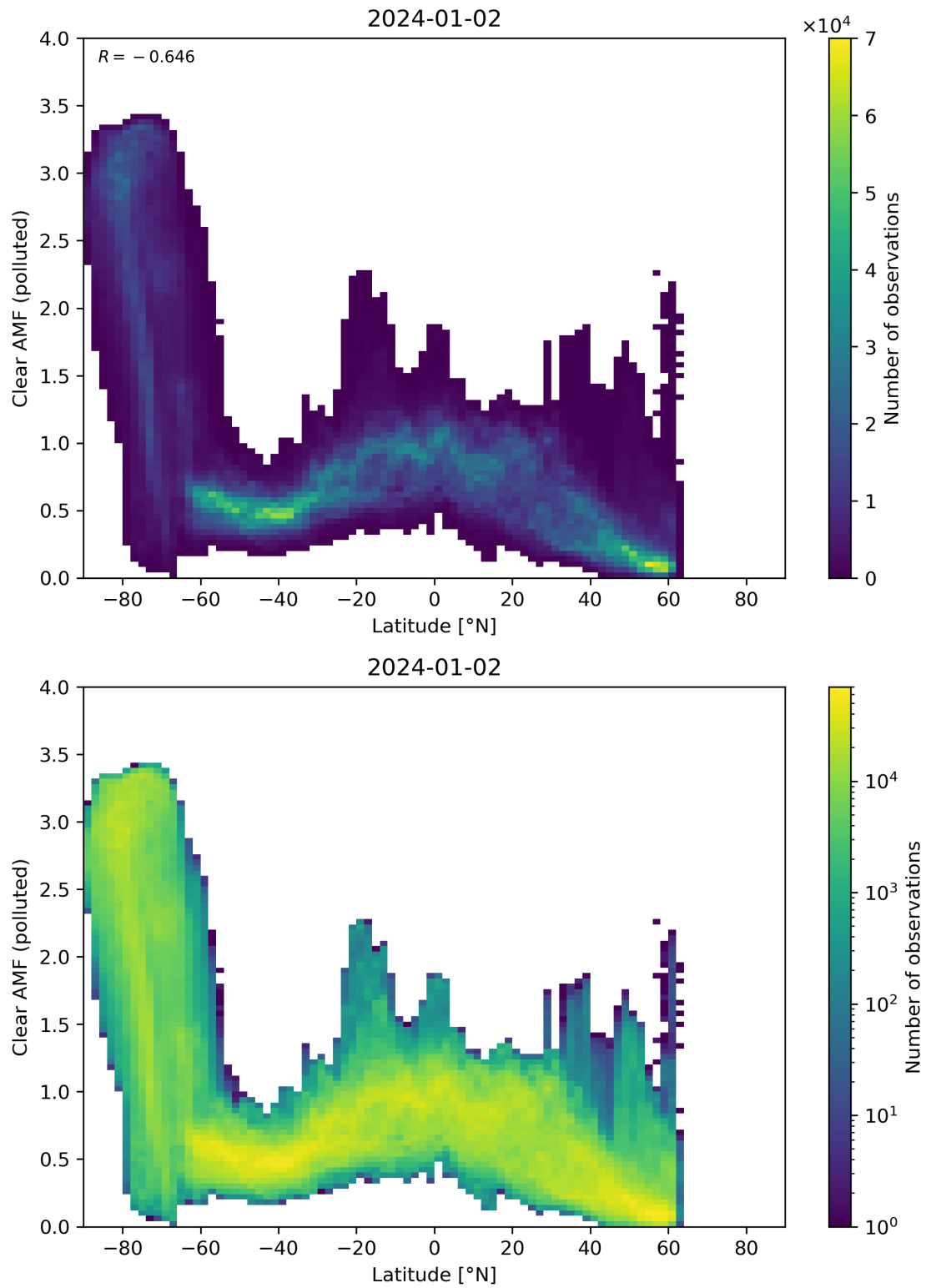
Figure 145: Scatter density plot of “Latitude” against “Clear AMF (polluted)” for 2024-01-01 to 2024-01-03.
