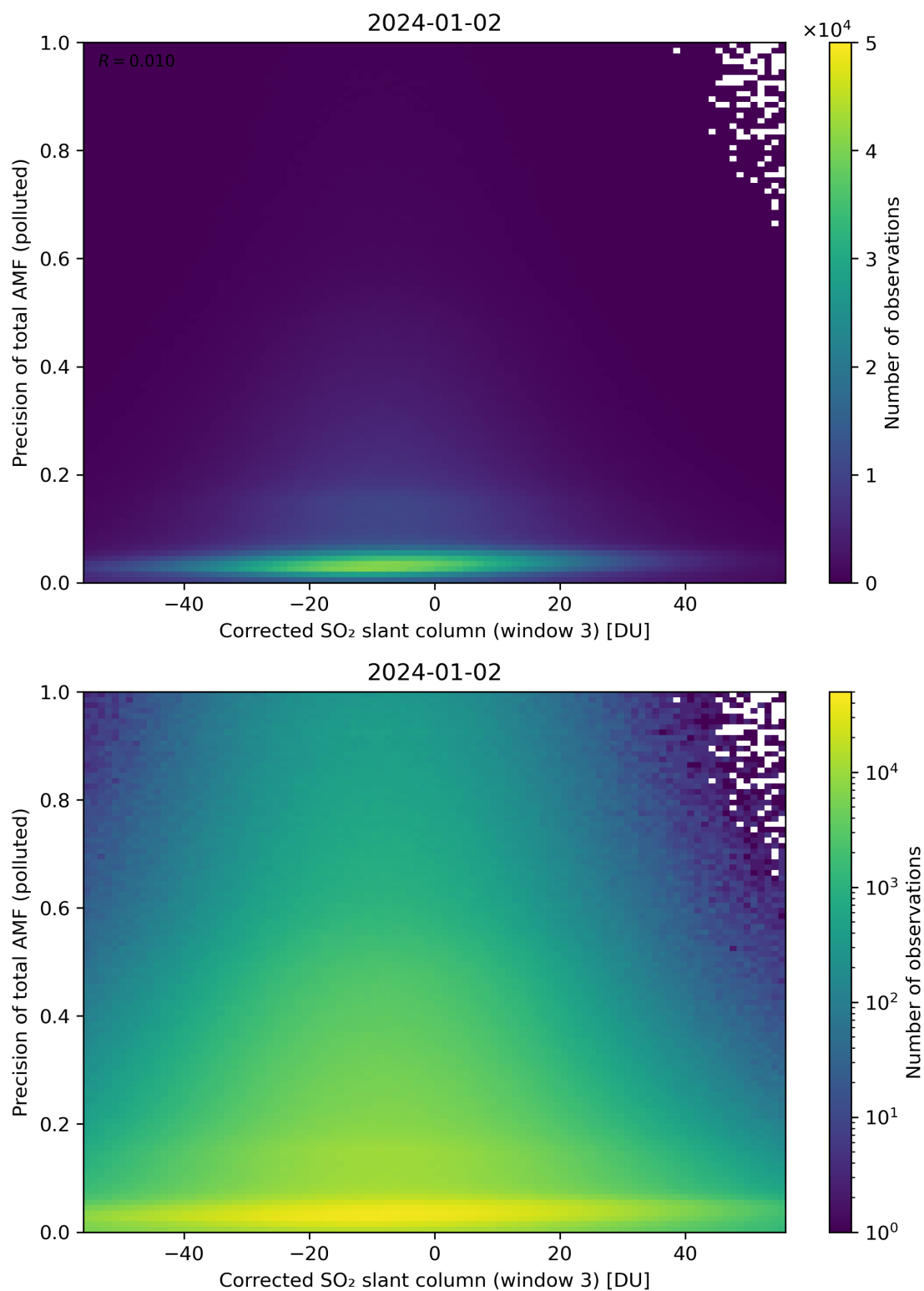
Figure 211: Scatter density plot of “Corrected SO 2 slant column (window 3)” against “Precision of total AMF (polluted)” for 2024-01-01 to 2024-01-03.
