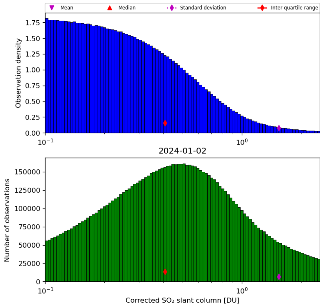
Figure 55: Histogram of “Corrected SO 2 slant column” for 2024-01-01 to 2024-01-03
