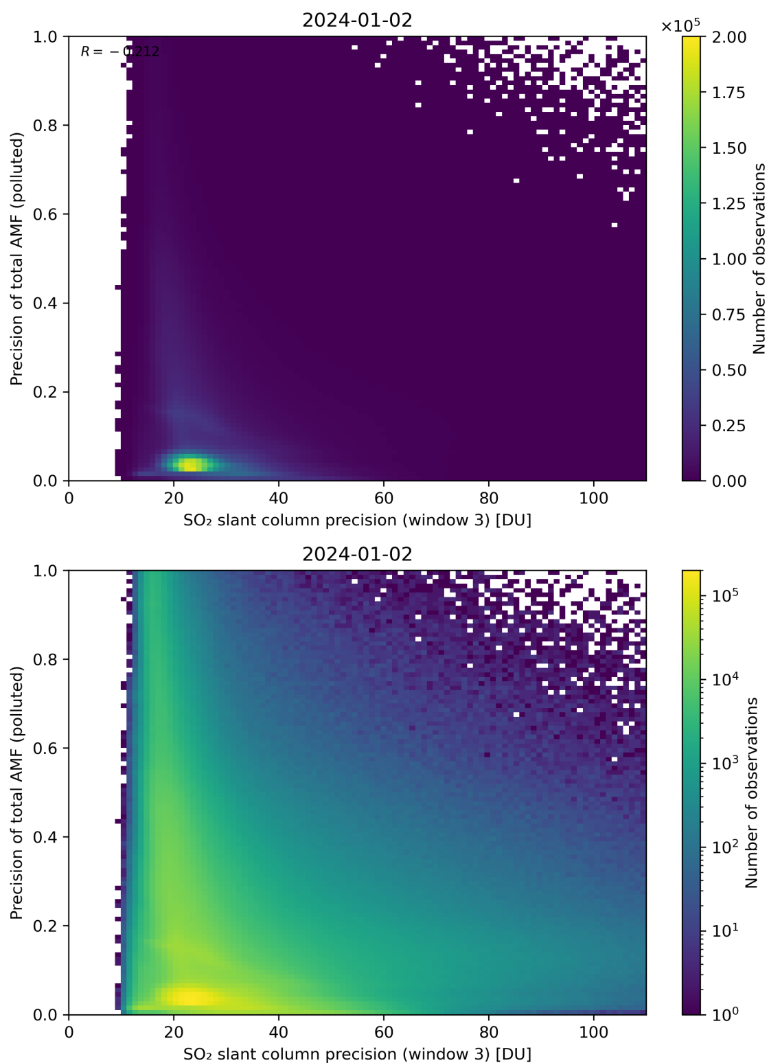
Figure 264: Scatter density plot of “SO 2 slant column precision (window 3)” against “Precision of total AMF (polluted)” for 2024-01-01 to 2024-01-03.
