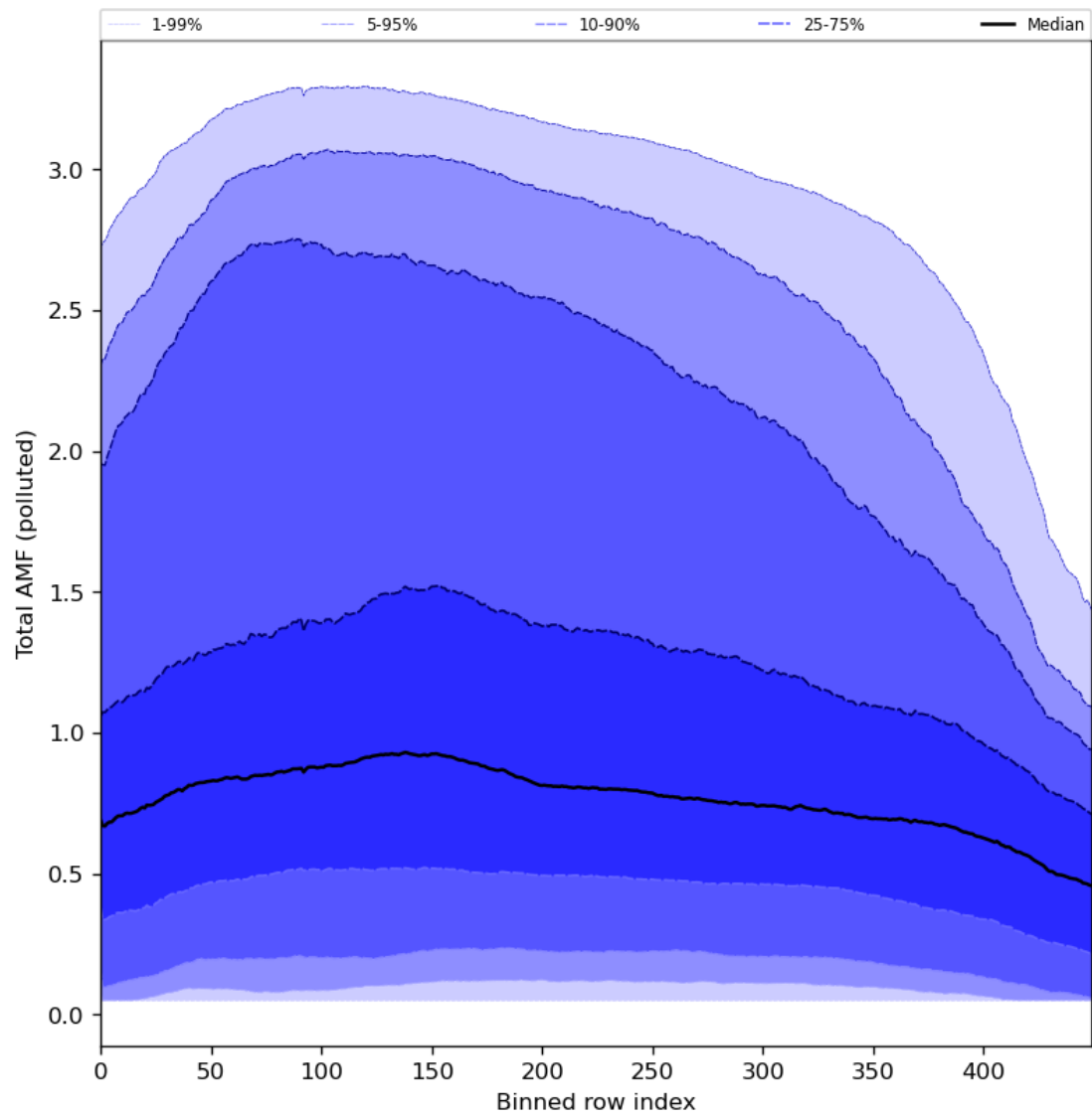
Figure 94: Along track statistics of “Total AMF (polluted)” for 2024-01-01 to 2024-01-03
