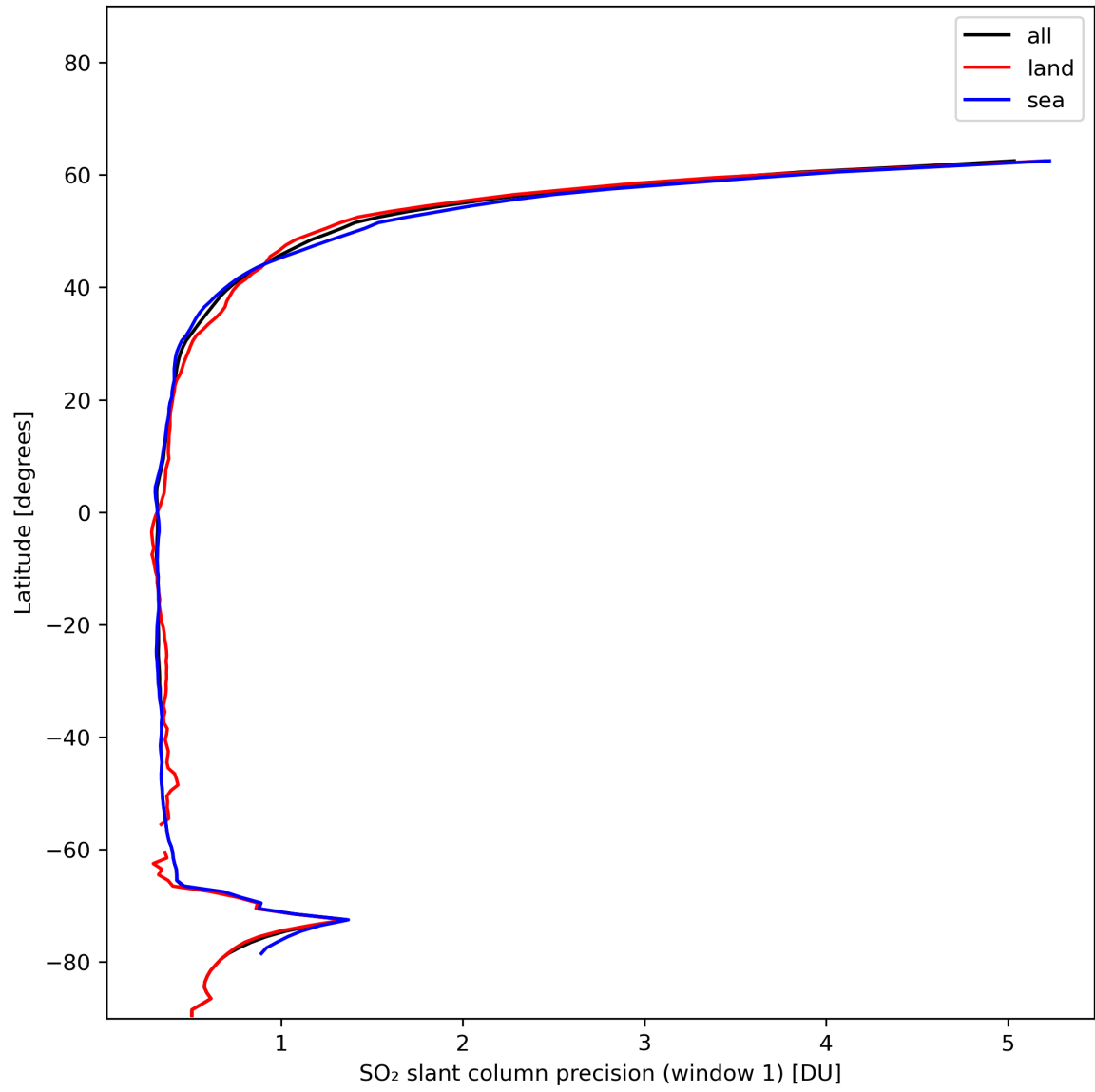
Figure 34: Zonal average of “SO 2 slant column precision (window 1)” for 2024-01-01 to 2024-01-03.
