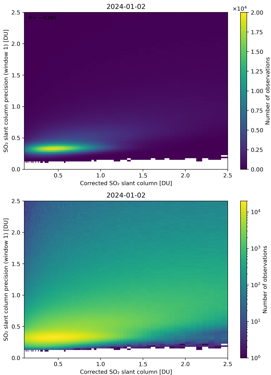
Figure 188: Scatter density plot of “Corrected SO 2 slant column” against “SO 2 slant column precision (window 1)” for 2024-01-01 to 2024-01-03.
