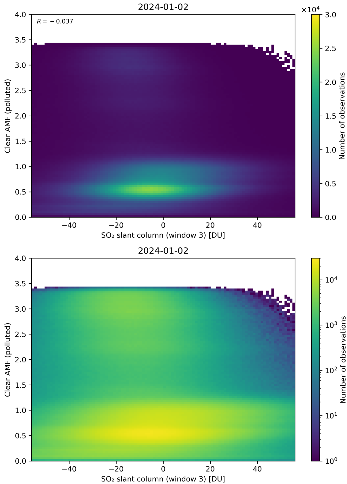
Figure 265: Scatter density plot of “SO 2 slant column (window 3)” against “Clear AMF (polluted)” for 2024-01-01 to 2024-01-03.
