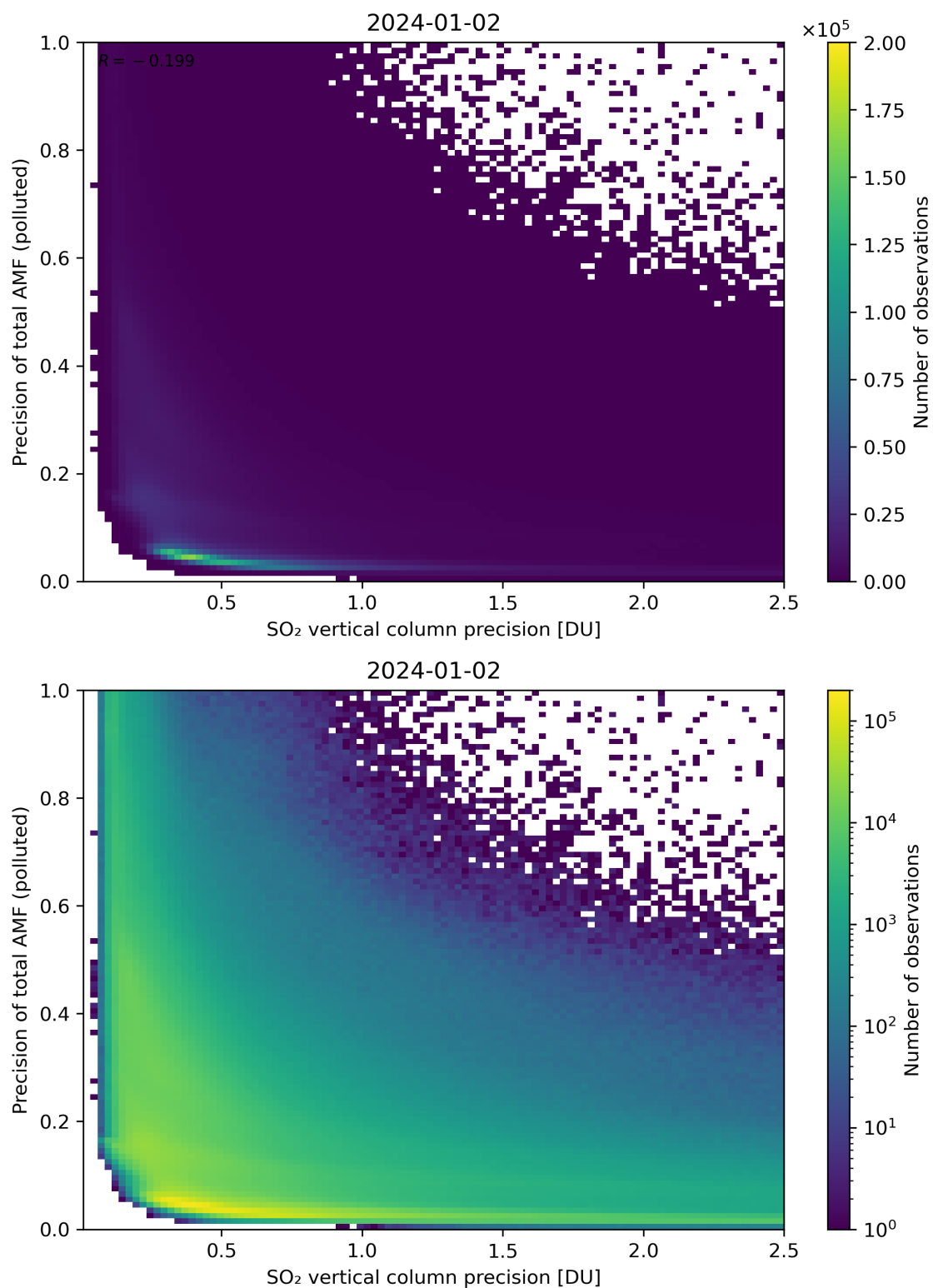
Figure 295: Scatter density plot of “SO 2 vertical column precision” against “Precision of total AMF (polluted)” for 2024-01-01 to 2024-01-03.
