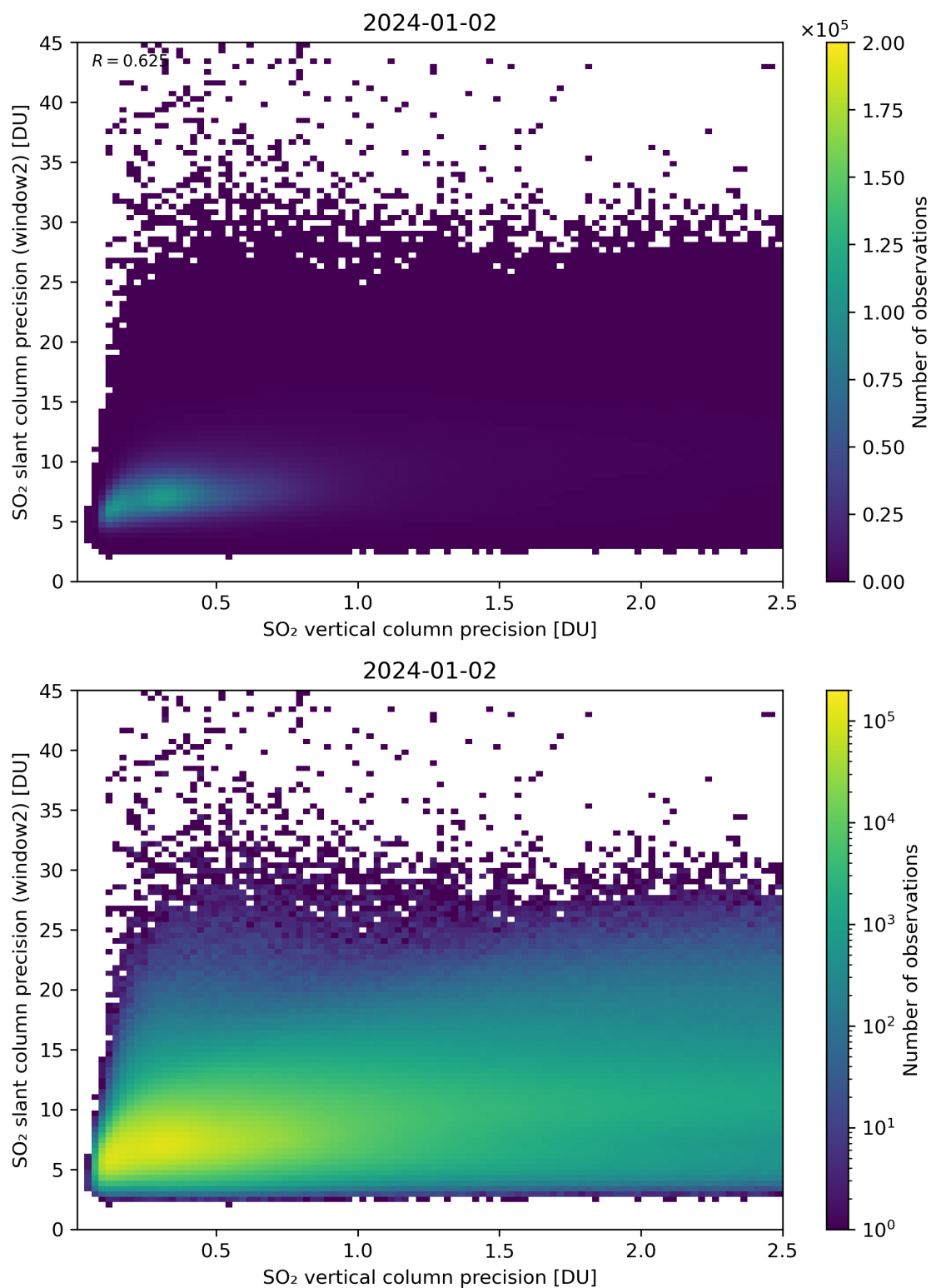
Figure 291: Scatter density plot of “SO 2 vertical column precision” against “SO 2 slant column precision (window2)” for 2024-01-01 to 2024-01-03.
