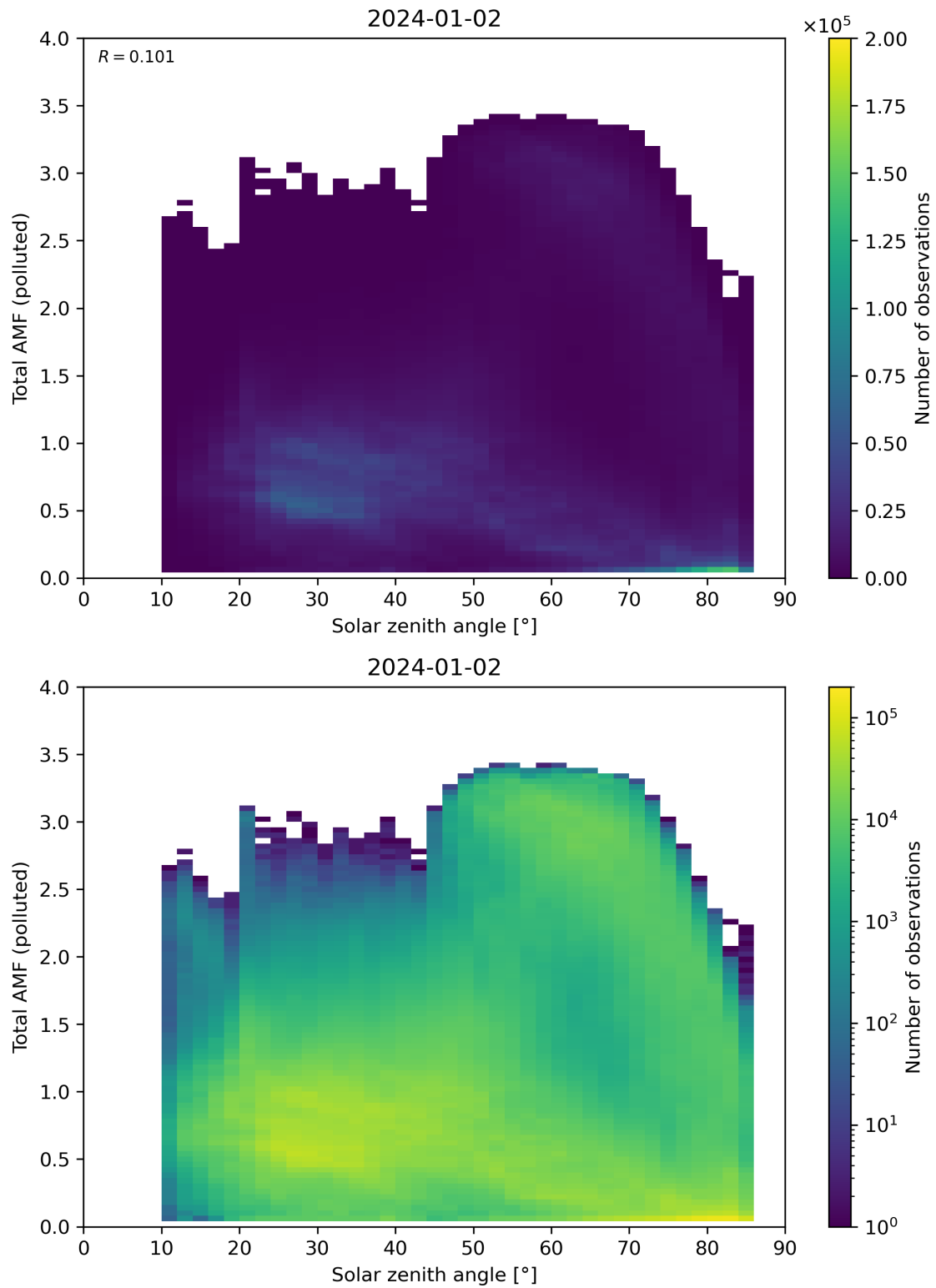
Figure 174: Scatter density plot of “Solar zenith angle” against “Total AMF (polluted)” for 2024-01-01 to 2024-01-03.
