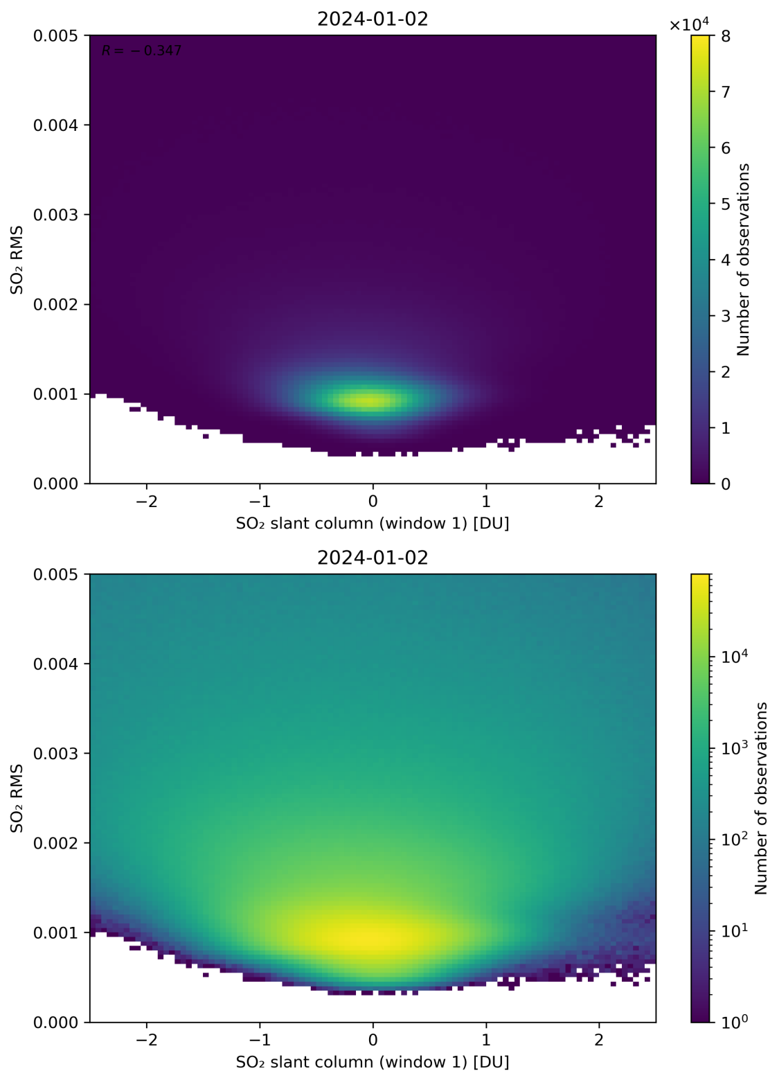
Figure 217: Scatter density plot of “SO 2 slant column (window 1)” against “SO 2 RMS” for 2024-01-01 to 2024-01-03.
