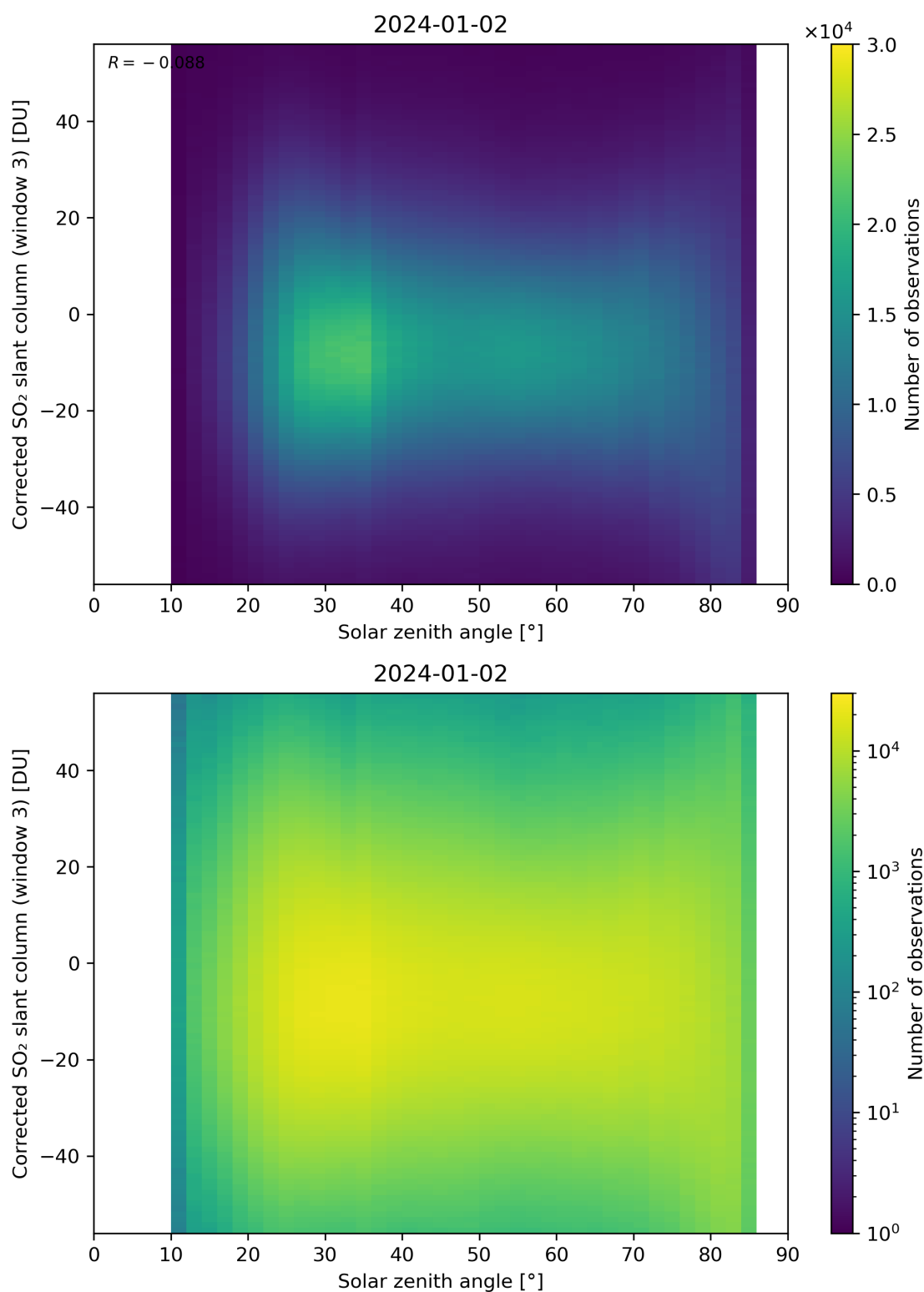
Figure 168: Scatter density plot of “Solar zenith angle” against “Corrected SO 2 slant column (window 3)” for 2024-01-01 to 2024-01-03.
