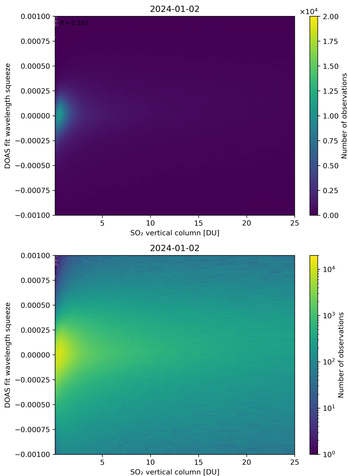
Figure 277: Scatter density plot of “SO 2 vertical column” against “DOAS fit wavelength squeeze” for 2024-01-01 to 2024-01-03.
