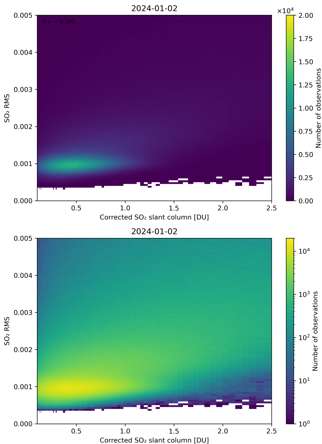
Figure 183: Scatter density plot of “Corrected SO 2 slant column” against “SO 2 RMS” for 2024-01-01 to 2024-01-03.
