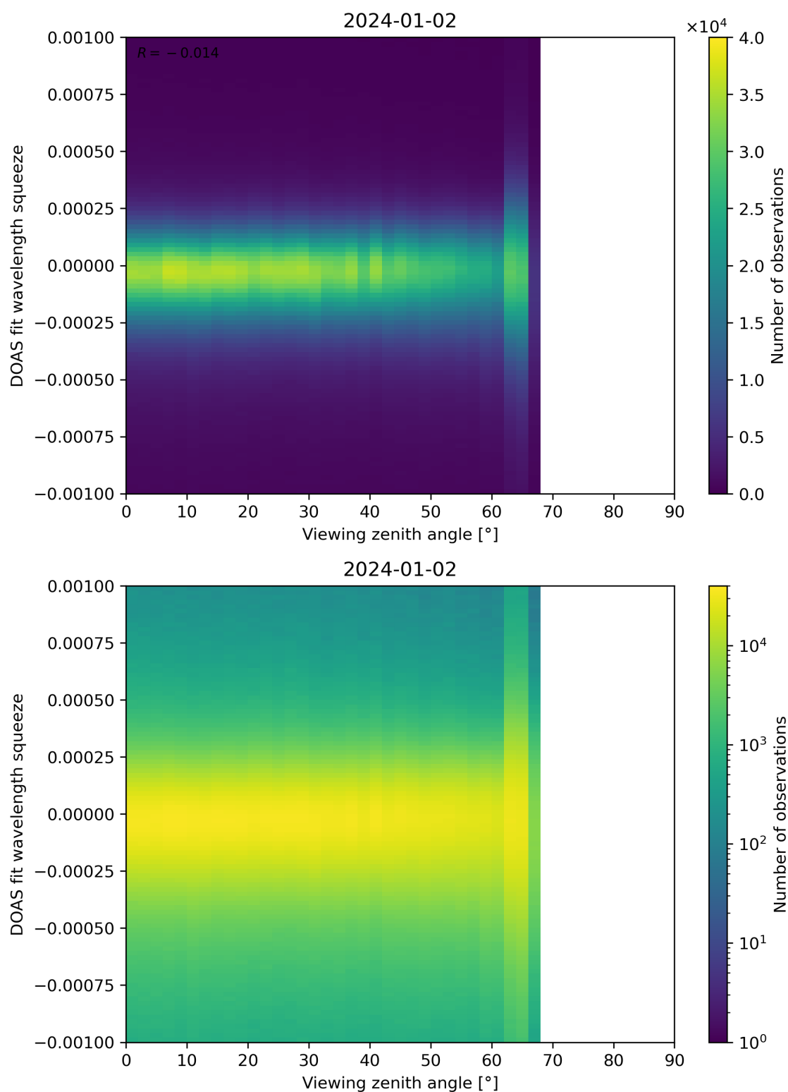
Figure 312: Scatter density plot of “Viewing zenith angle” against “DOAS fit wavelength squeeze” for 2024-01-01 to 2024-01-03.
