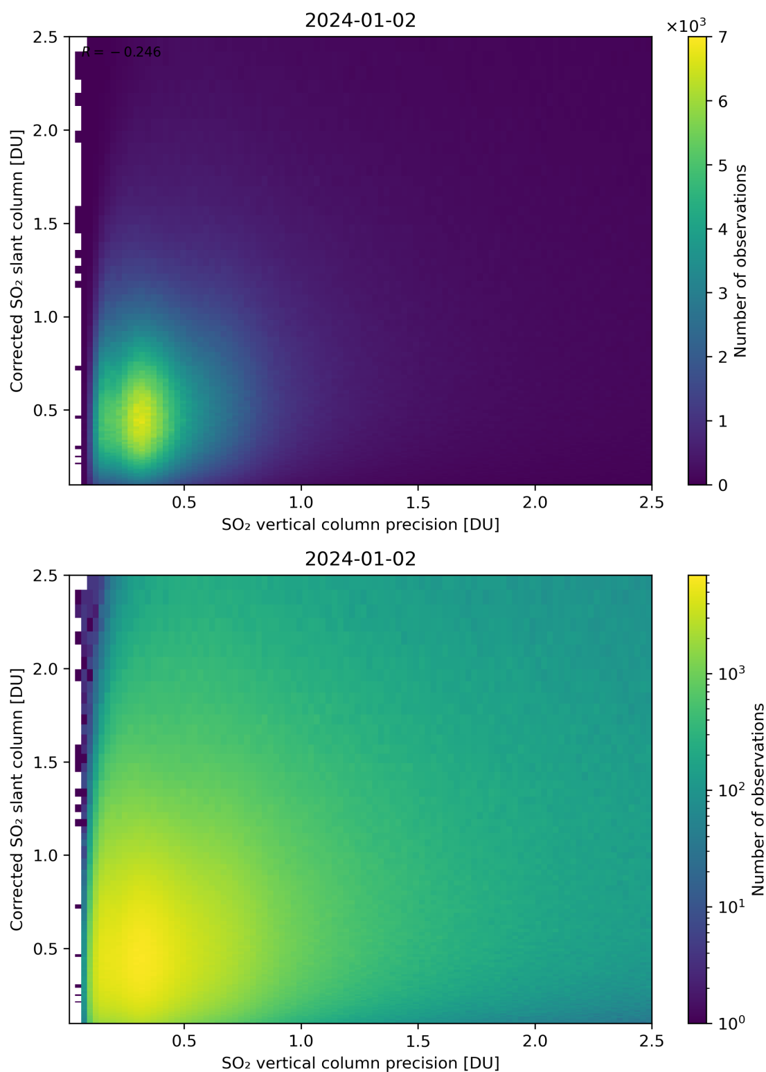
Figure 286: Scatter density plot of “SO 2 vertical column precision” against “Corrected SO 2 slant column” for 2024-01-01 to 2024-01-03.
