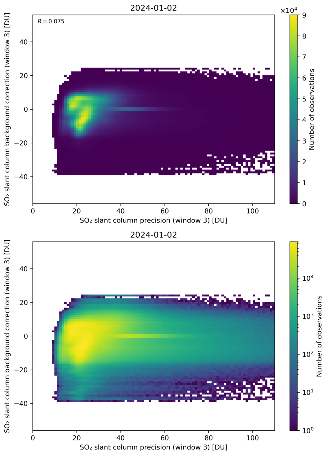
Figure 257: Scatter density plot of “SO 2 slant column precision (window 3)” against “SO 2 slant column background correction (window 3)” for 2024-01-01 to 2024-01-03.
