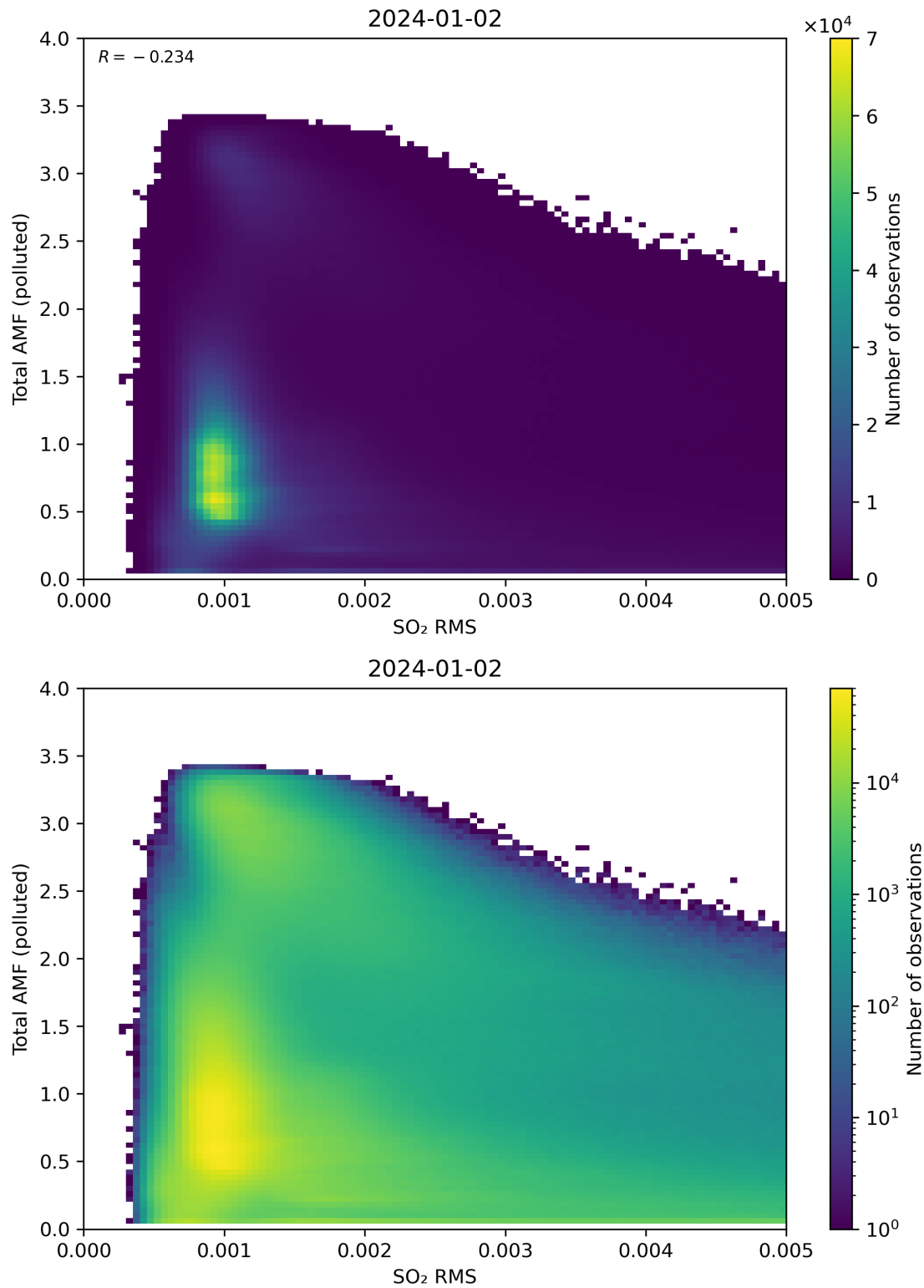
Figure 137: Scatter density plot of “SO 2 RMS” against “Total AMF (polluted)” for 2024-01-01 to 2024-01-03.
