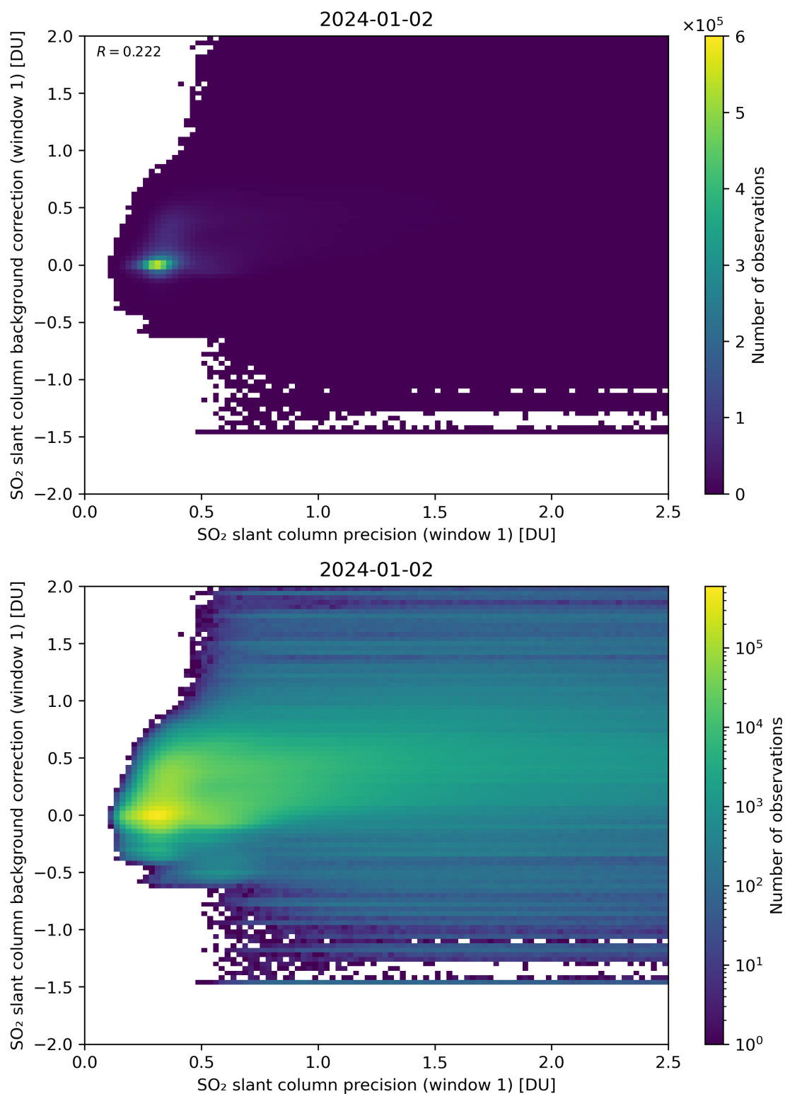
Figure 218: Scatter density plot of “SO 2 slant column precision (window 1)” against “SO 2 slant column background correction (window 1)” for 2024-01-01 to 2024-01-03.
