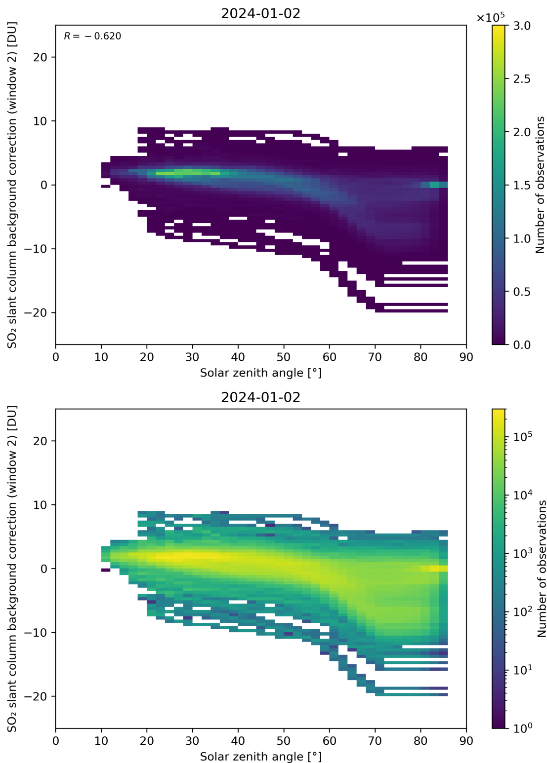
Figure 159: Scatter density plot of “Solar zenith angle” against “SO 2 slant column background correction (window 2)” for 2024-01-01 to 2024-01-03.
