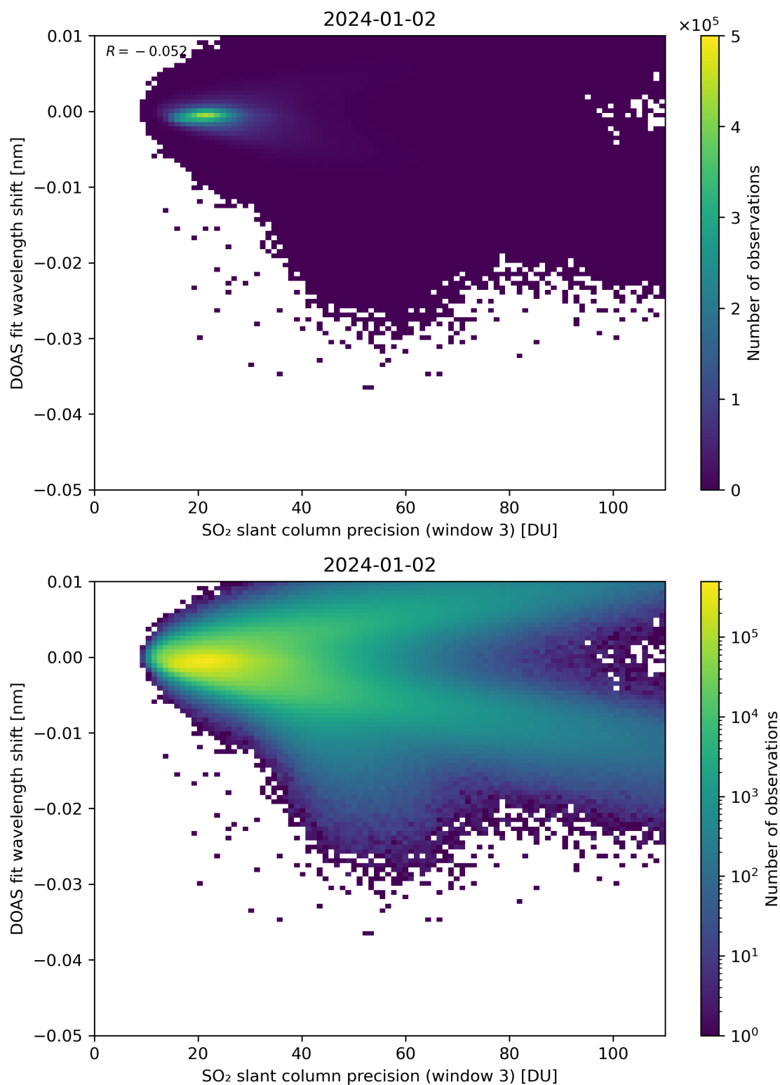
Figure 258: Scatter density plot of “SO 2 slant column precision (window 3)” against “DOAS fit wavelength shift” for 2024-01-01 to 2024-01-03.
