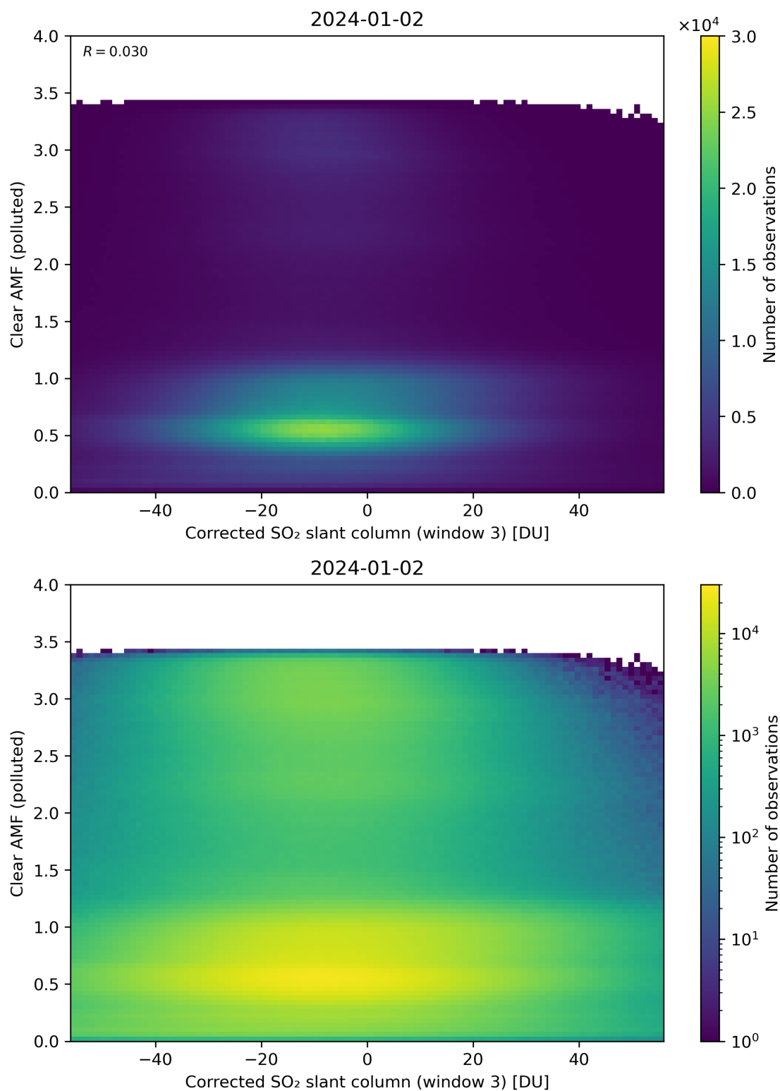
Figure 209: Scatter density plot of “Corrected SO 2 slant column (window 3)” against “Clear AMF (polluted)” for 2024-01-01 to 2024-01-03.
