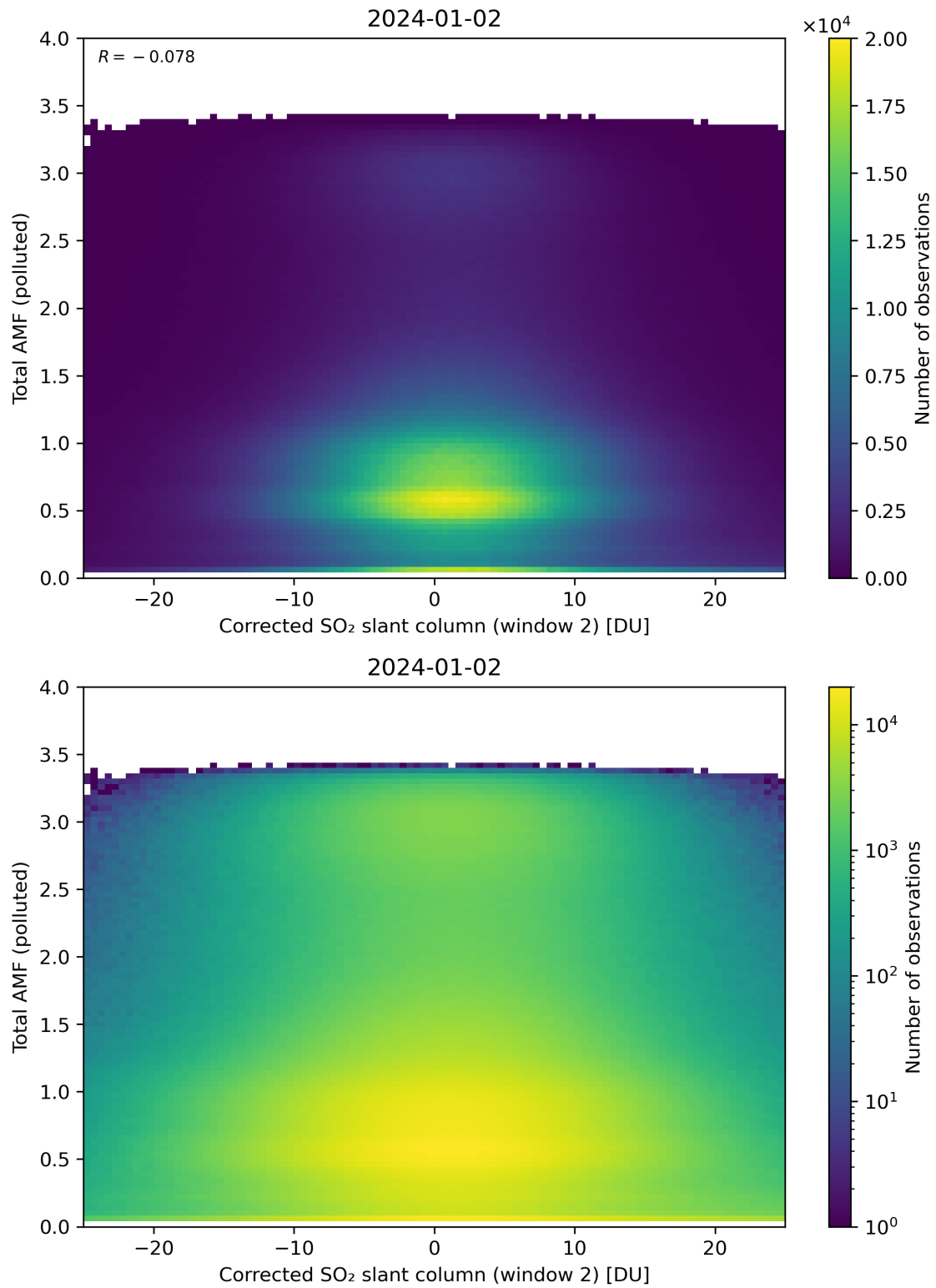
Figure 203: Scatter density plot of “Corrected SO 2 slant column (window 2)” against “Total AMF (polluted)” for 2024-01-01 to 2024-01-03.
