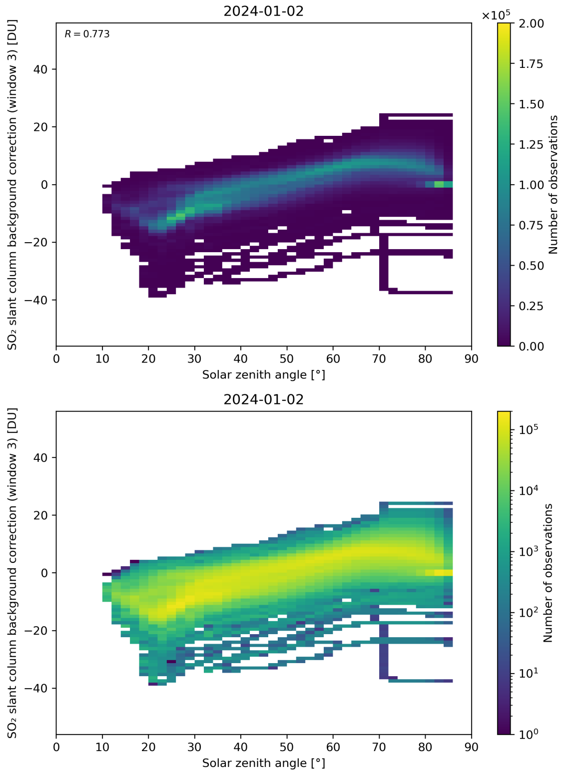
Figure 160: Scatter density plot of “Solar zenith angle” against “SO 2 slant column background correction (window 3)” for 2024-01-01 to 2024-01-03.
