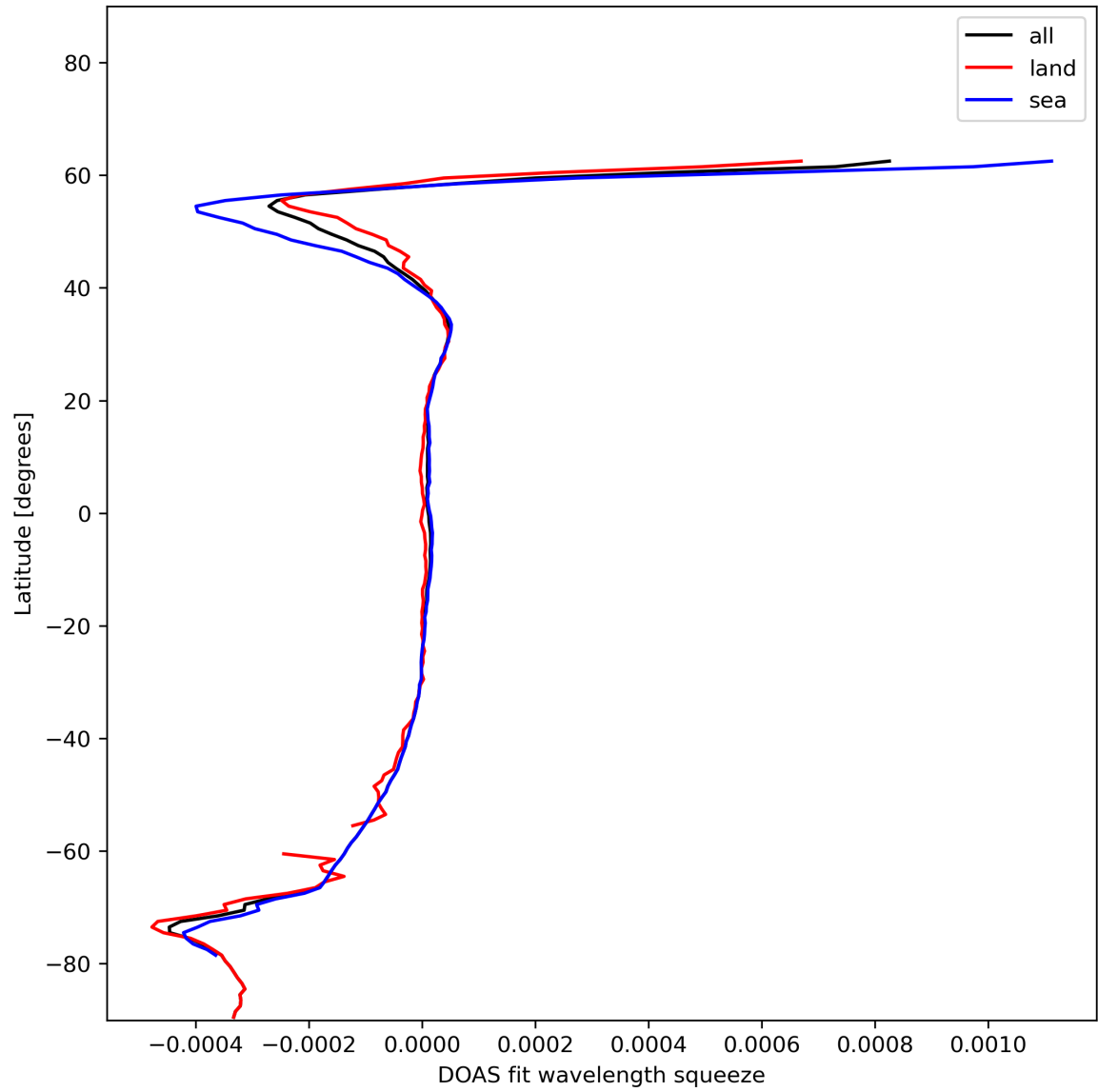
Figure 46: Zonal average of "DOAS fit wavelength squeeze" for 2024-01-01 to 2024-01-03.
