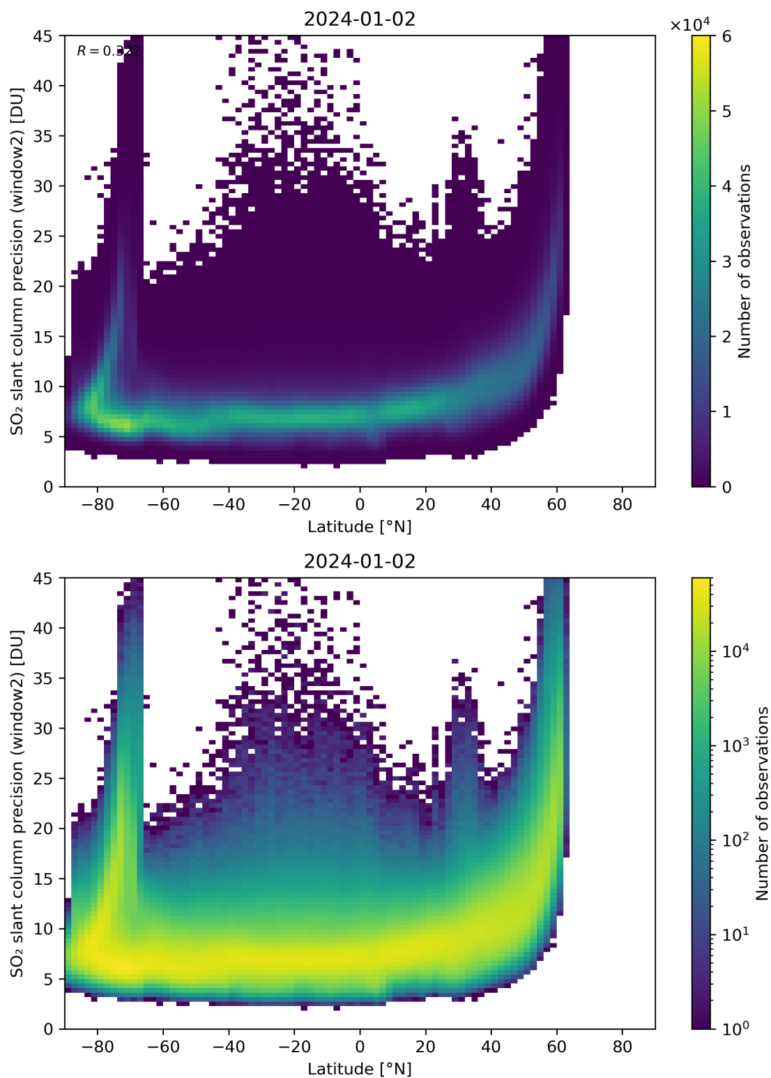
Figure 151: Scatter density plot of “Latitude” against “SO 2 slant column precision (window2)” for 2024-01-01 to 2024-01-03.
