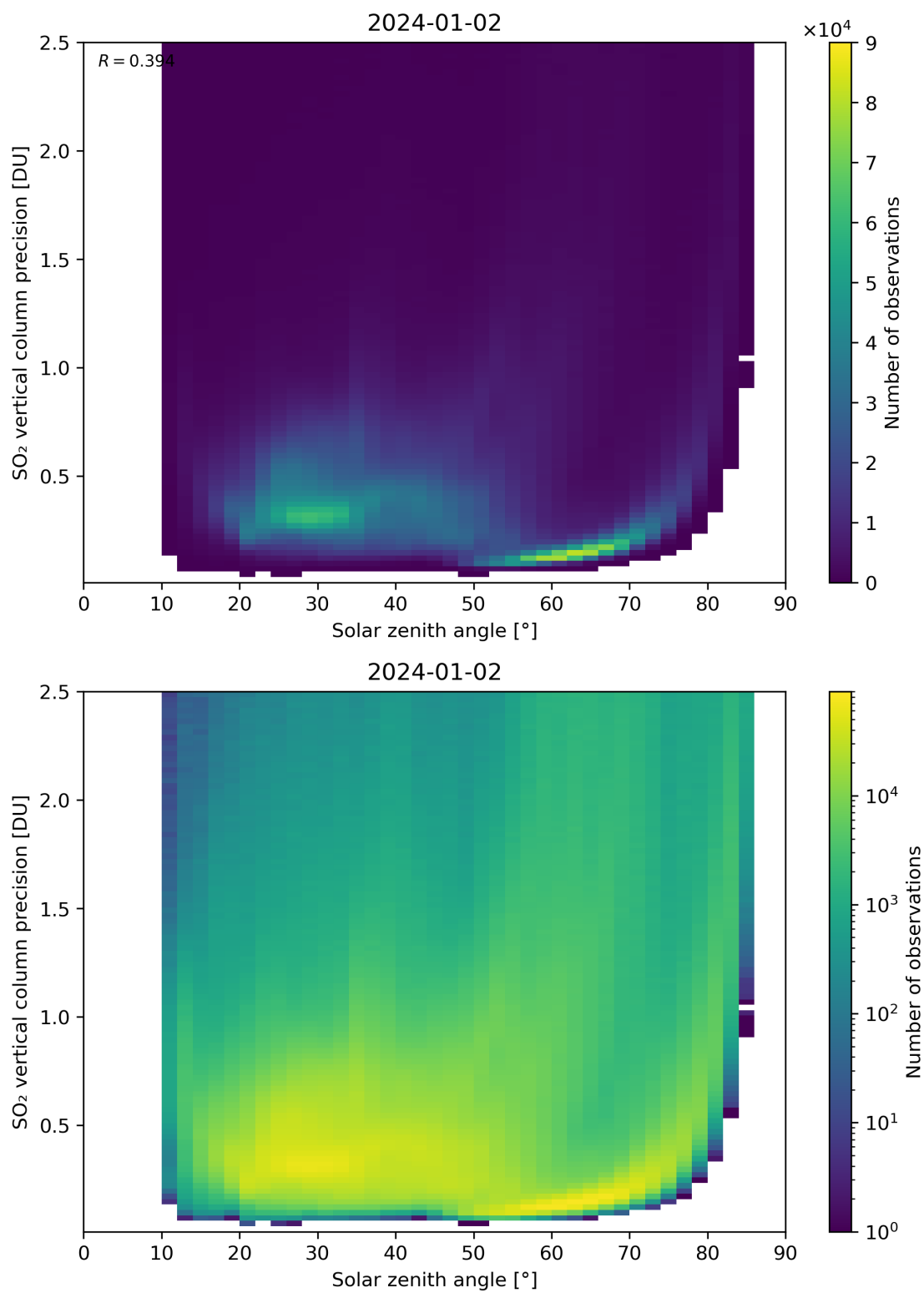
Figure 177: Scatter density plot of “Solar zenith angle” against “SO 2 vertical column precision” for 2024-01-01 to 2024-01-03.
