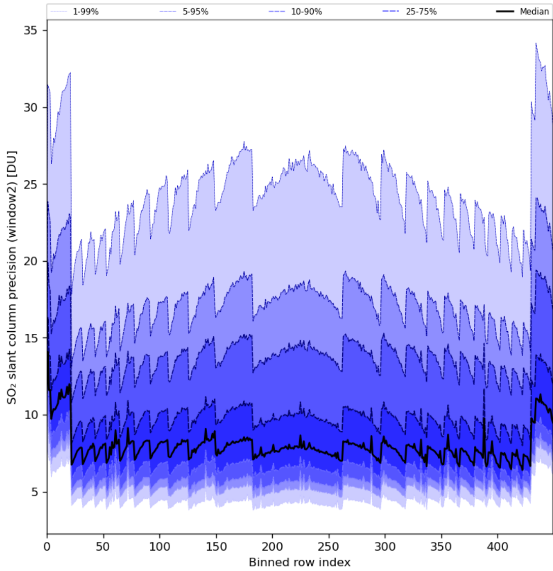
Figure 84: Along track statistics of “SO 2 slant column precision (window2)” for 2024-01-01 to 2024-01-03
