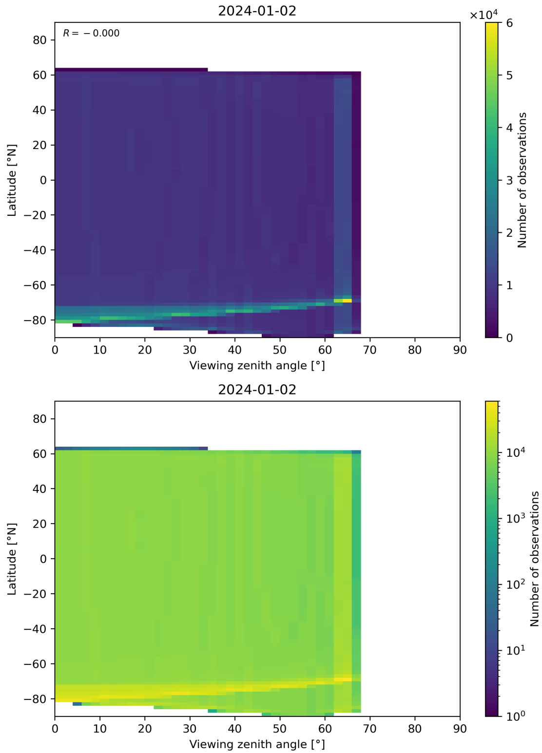
Figure 314: Scatter density plot of “Viewing zenith angle” against “Latitude” for 2024-01-01 to 2024-01-03.
