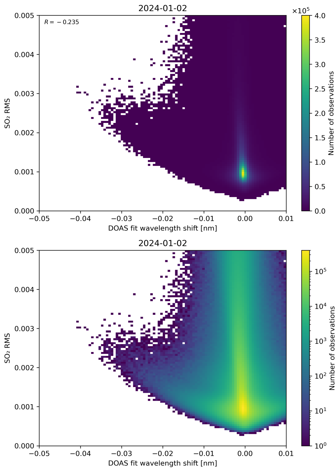
Figure 128: Scatter density plot of “DOAS fit wavelength shift” against “SO 2 RMS” for 2024-01-01 to 2024-01-03.
