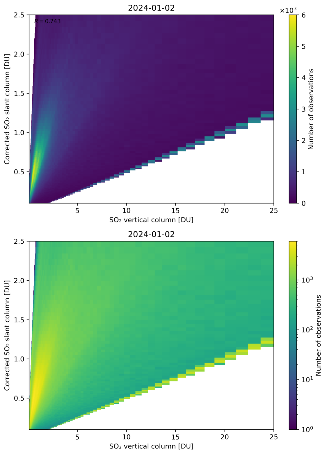
Figure 297: Scatter density plot of “SO 2 vertical column” against “Corrected SO 2 slant column” for 2024-01-01 to 2024-01-03.
