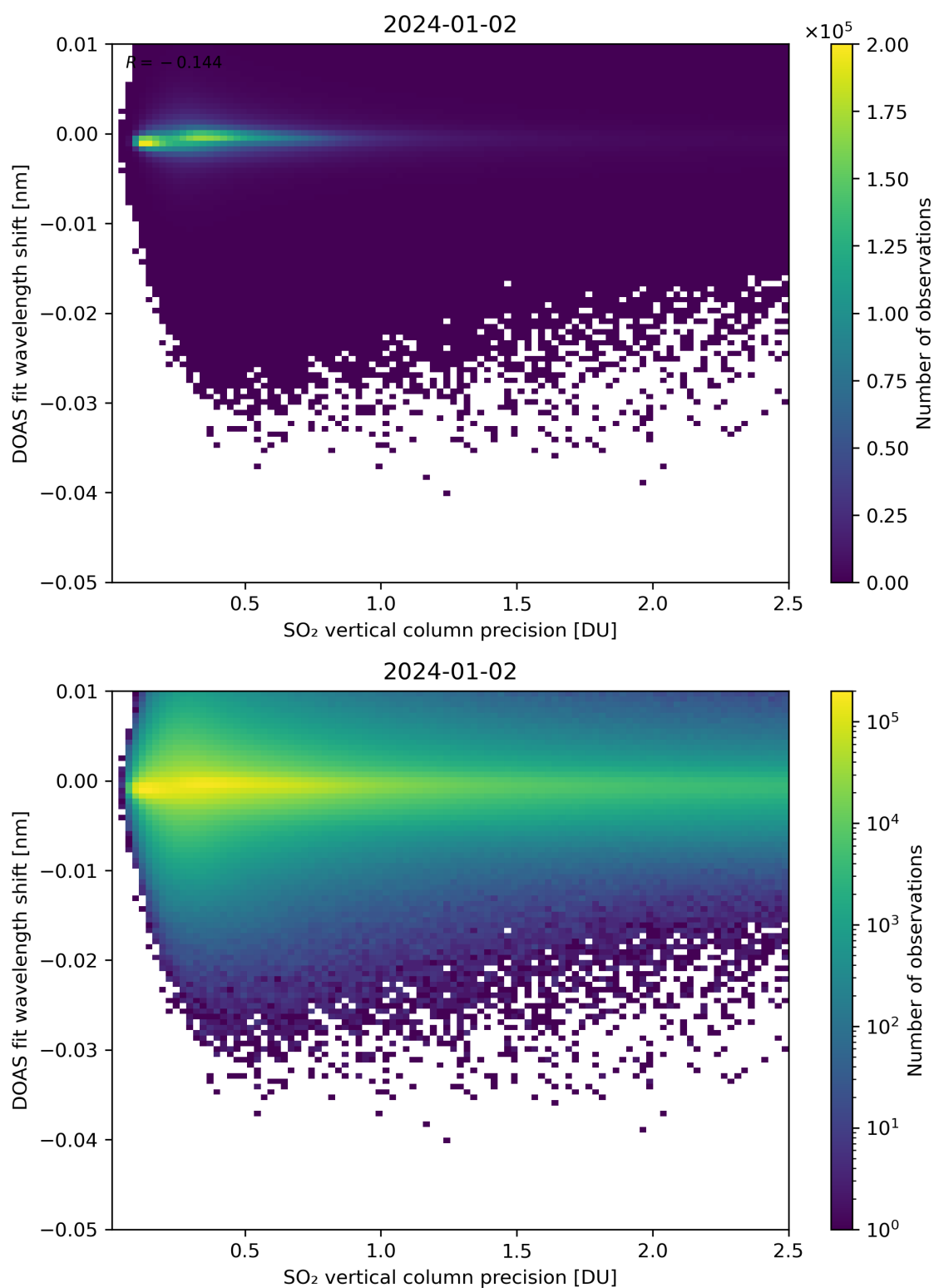
Figure 282: Scatter density plot of “SO 2 vertical column precision” against “DOAS fit wavelength shift” for 2024-01-01 to 2024-01-03.
