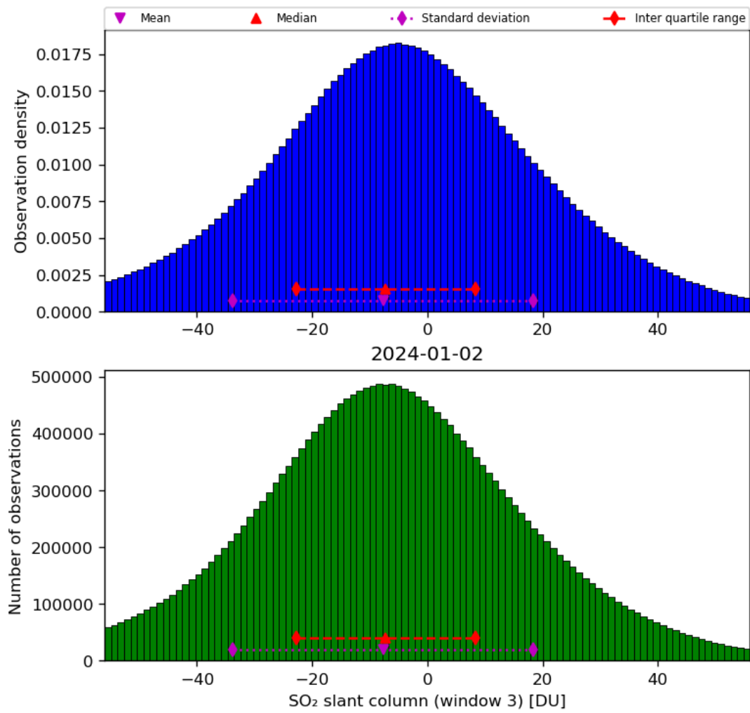
Figure 64: Histogram of “SO 2 slant column (window 3)” for 2024-01-01 to 2024-01-03
