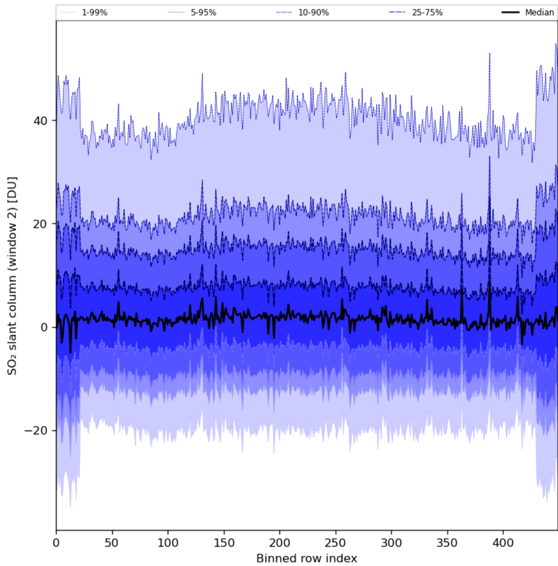
Figure 83: Along track statistics of “SO 2 slant column (window 2)” for 2024-01-01 to 2024-01-03
