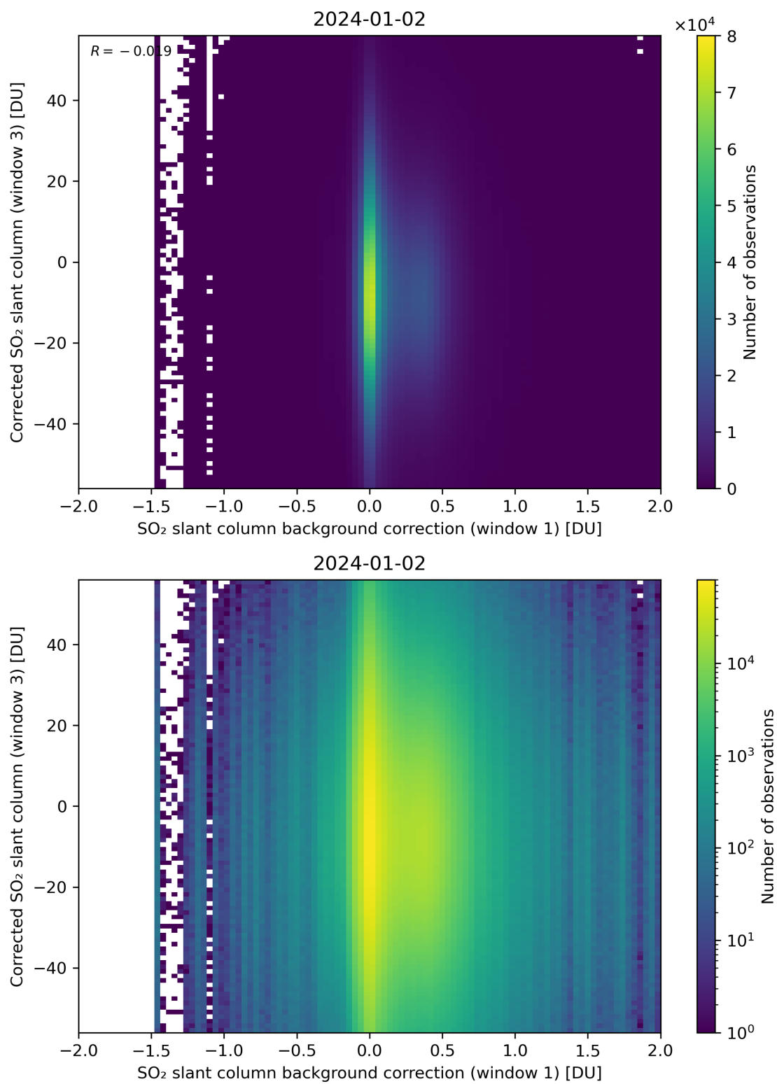
Figure 105: Scatter density plot of “SO 2 slant column background correction (window 1)” against “Corrected SO 2 slant column (window 3)” for 2024-01-01 to 2024-01-03.
