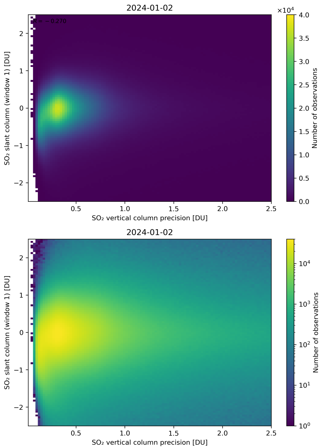
Figure 289: Scatter density plot of “SO 2 vertical column precision” against “SO 2 slant column (window 1)” for 2024-01-01 to 2024-01-03.
