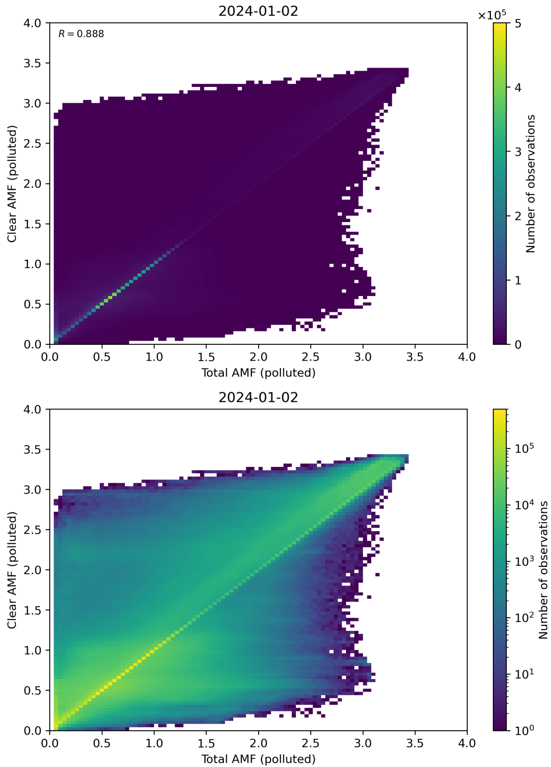
Figure 271: Scatter density plot of “Total AMF (polluted)” against “Clear AMF (polluted)” for 2024-01-01 to 2024-01-03.
