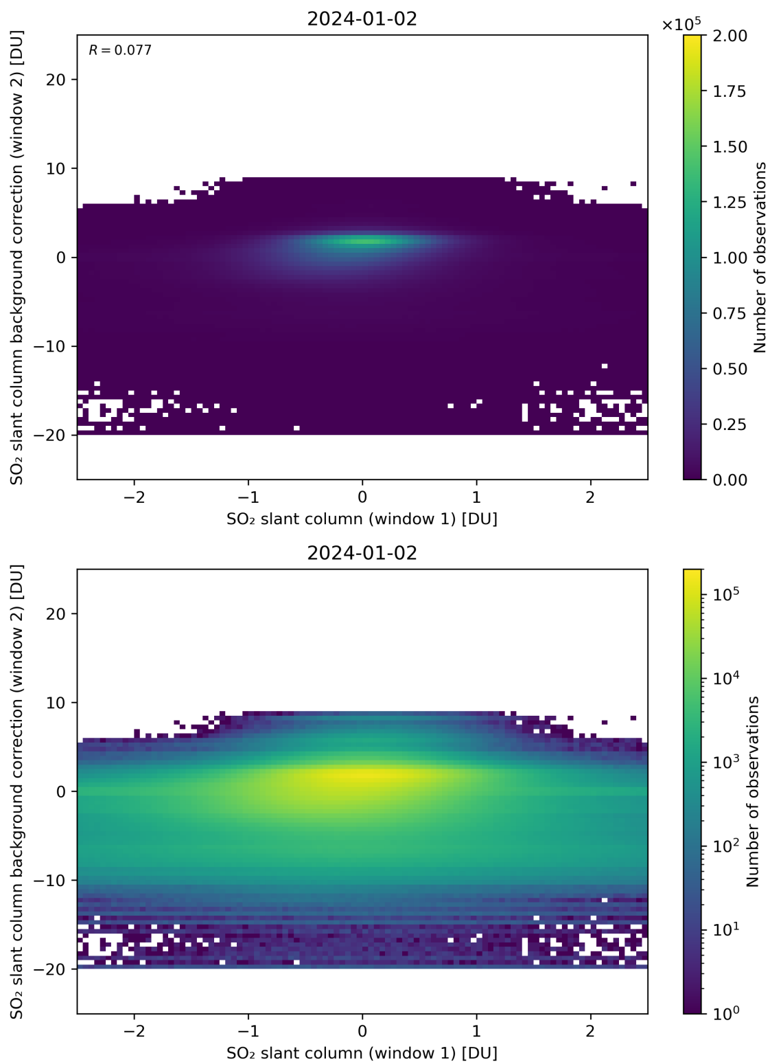
Figure 213: Scatter density plot of “SO 2 slant column (window 1)” against “SO 2 slant column background correction (window 2)” for 2024-01-01 to 2024-01-03.
