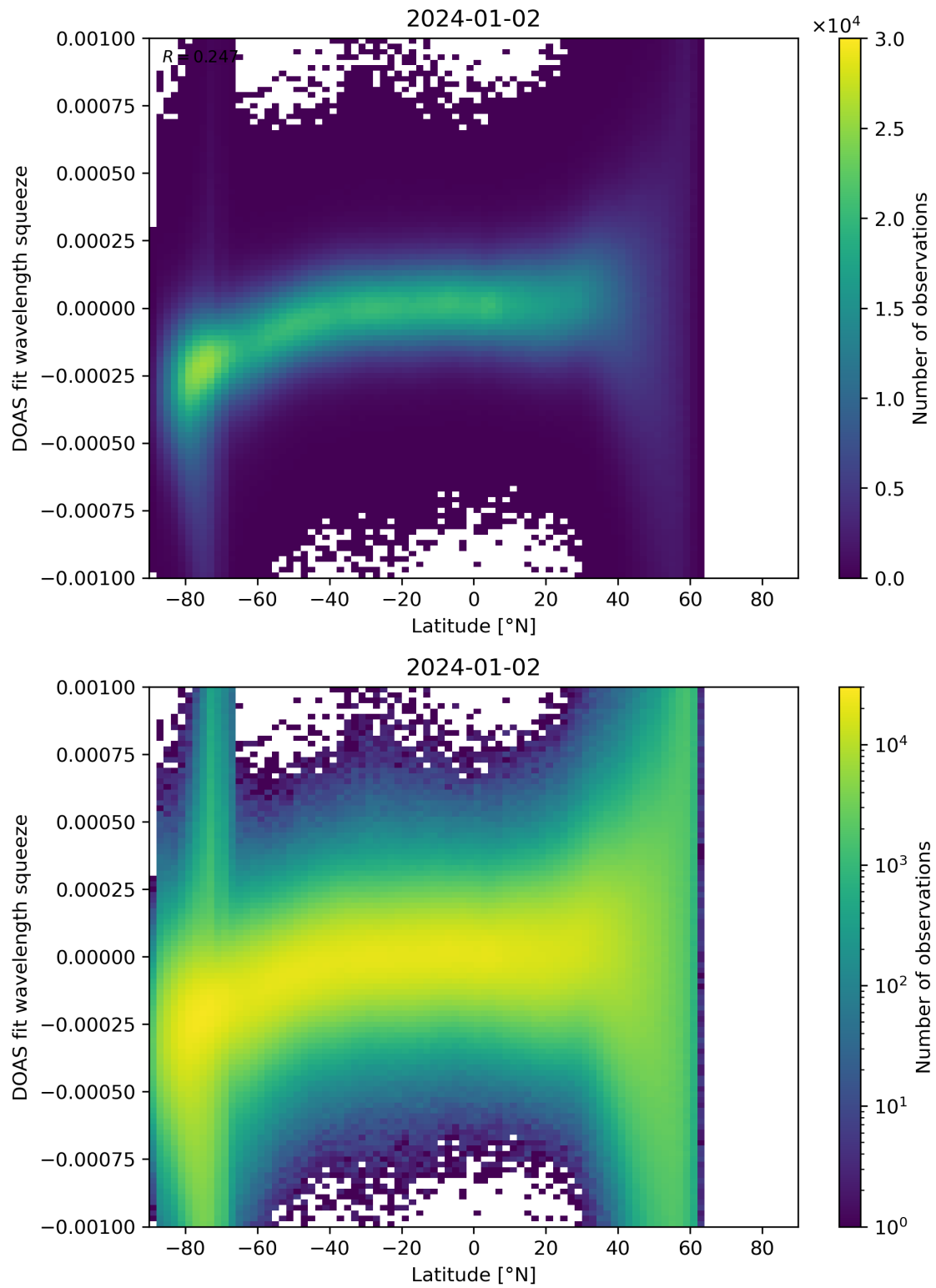
Figure 143: Scatter density plot of “Latitude” against “DOAS fit wavelength squeeze” for 2024-01-01 to 2024-01-03.
