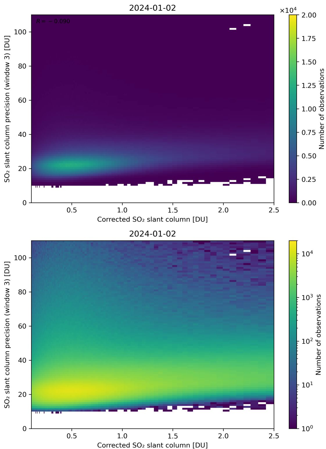
Figure 191: Scatter density plot of “Corrected SO 2 slant column” against “SO 2 slant column precision (window 3)” for 2024-01-01 to 2024-01-03.
