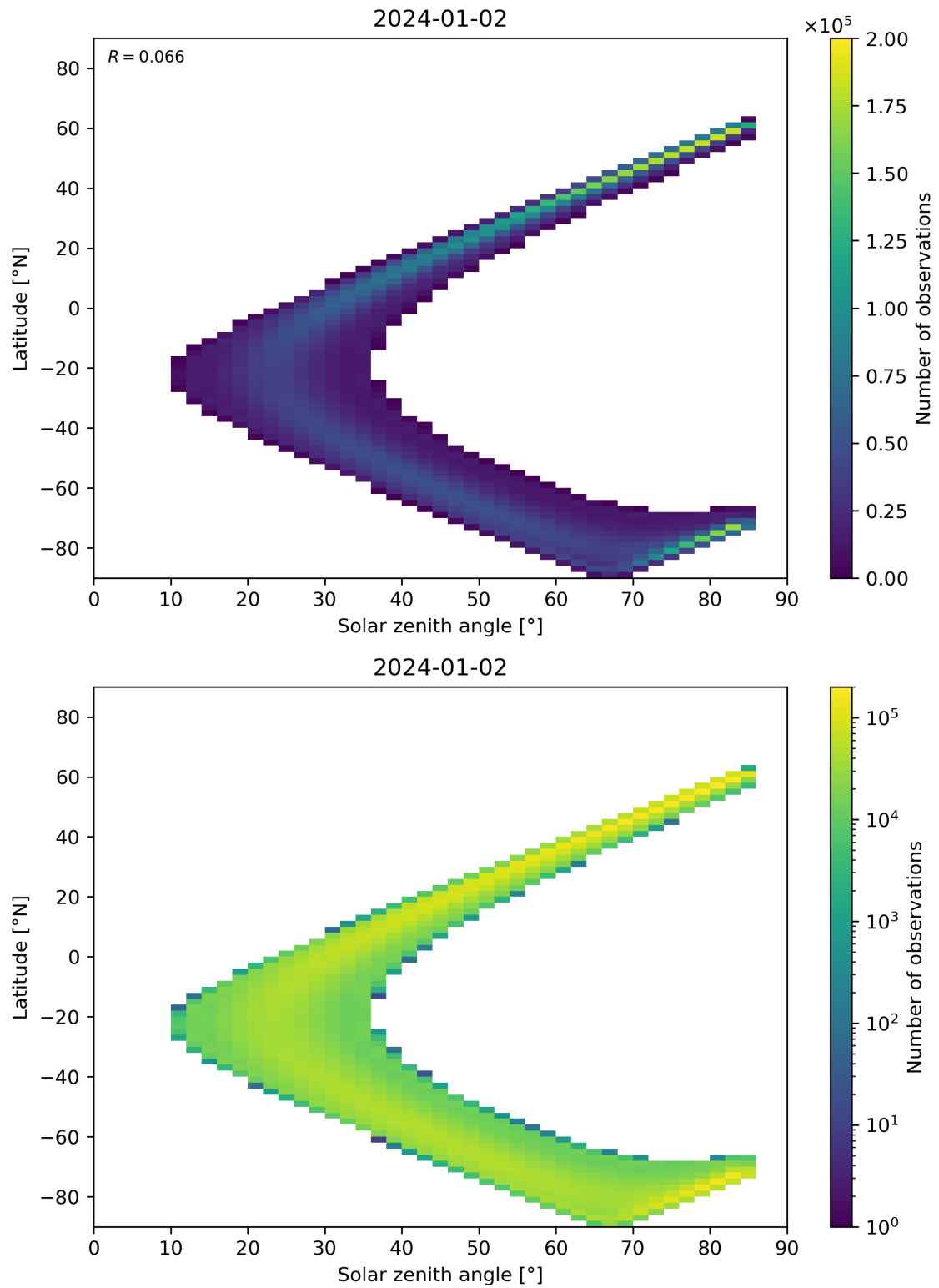
Figure 164: Scatter density plot of “Solar zenith angle” against “Latitude” for 2024-01-01 to 2024-01-03.
