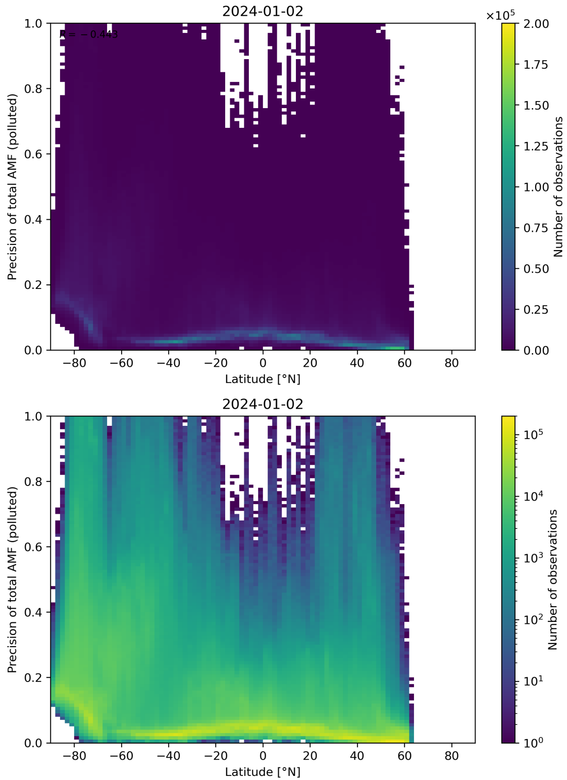
Figure 155: Scatter density plot of “Latitude” against “Precision of total AMF (polluted)” for 2024-01-01 to 2024-01-03.
