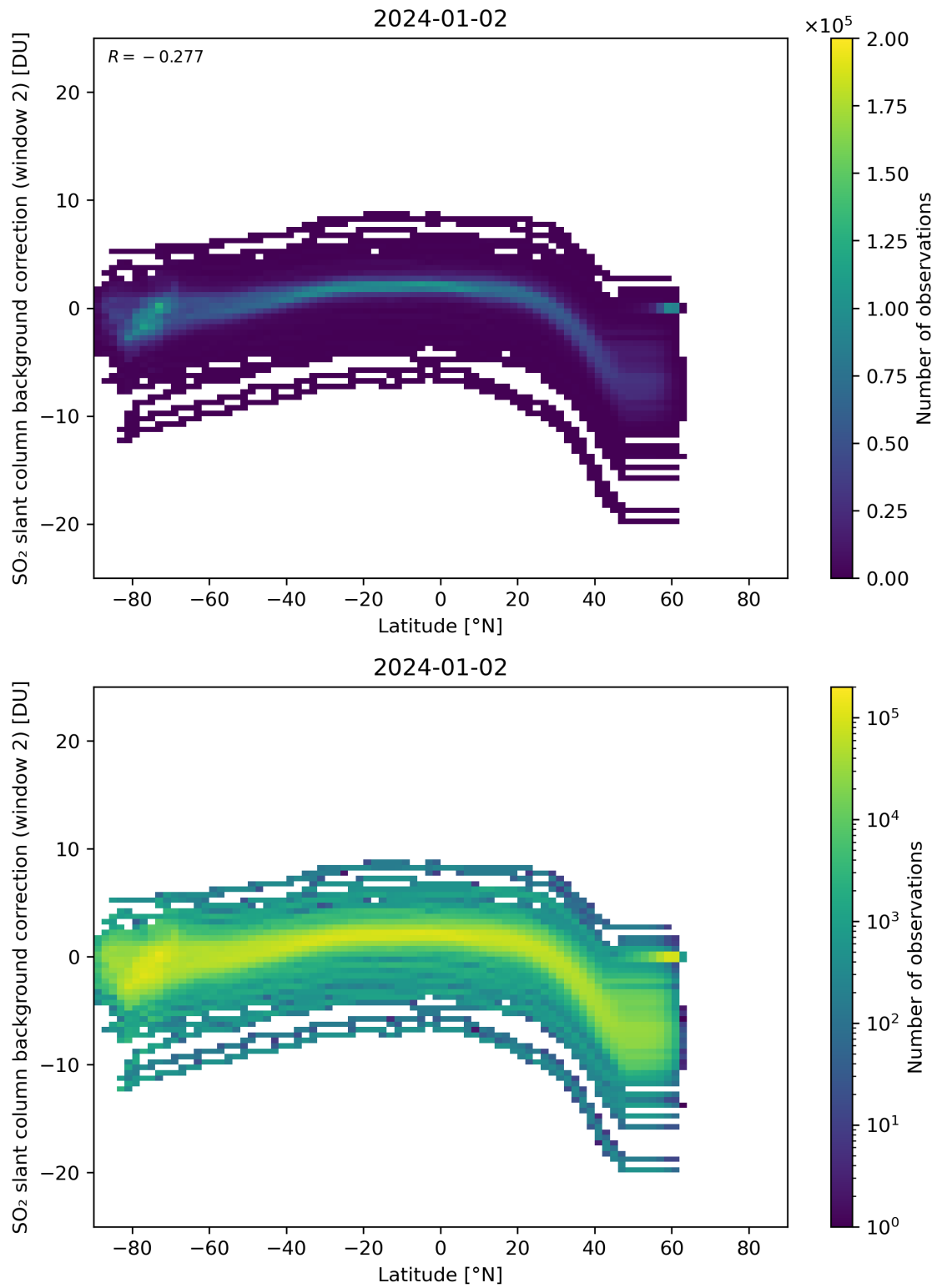
Figure 140: Scatter density plot of “Latitude” against “SO 2 slant column background correction (window 2)” for 2024-01-01 to 2024-01-03.
