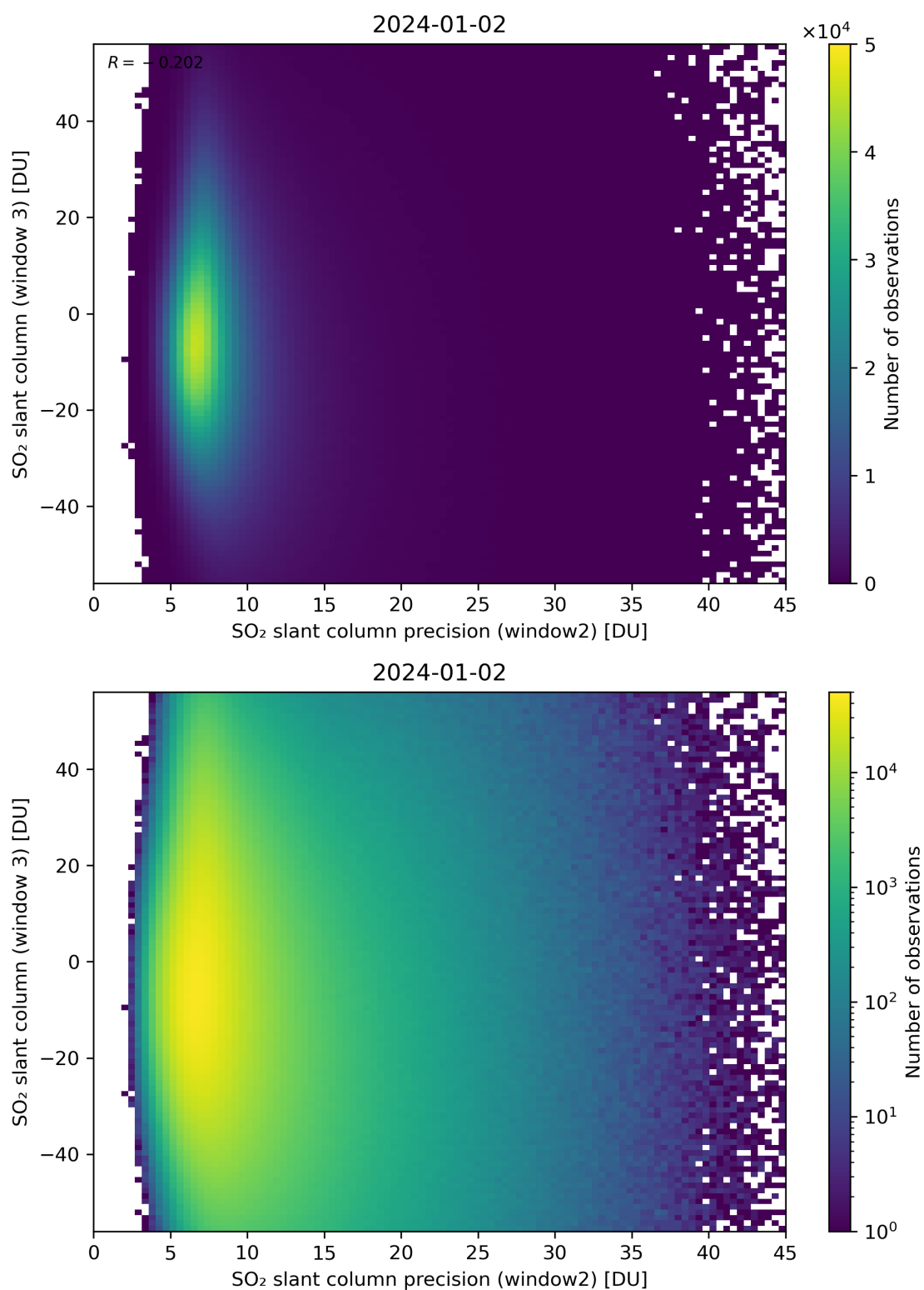
Figure 249: Scatter density plot of “SO 2 slant column precision (window2)” against “SO 2 slant column (window 3)” for 2024-01-01 to 2024-01-03.
