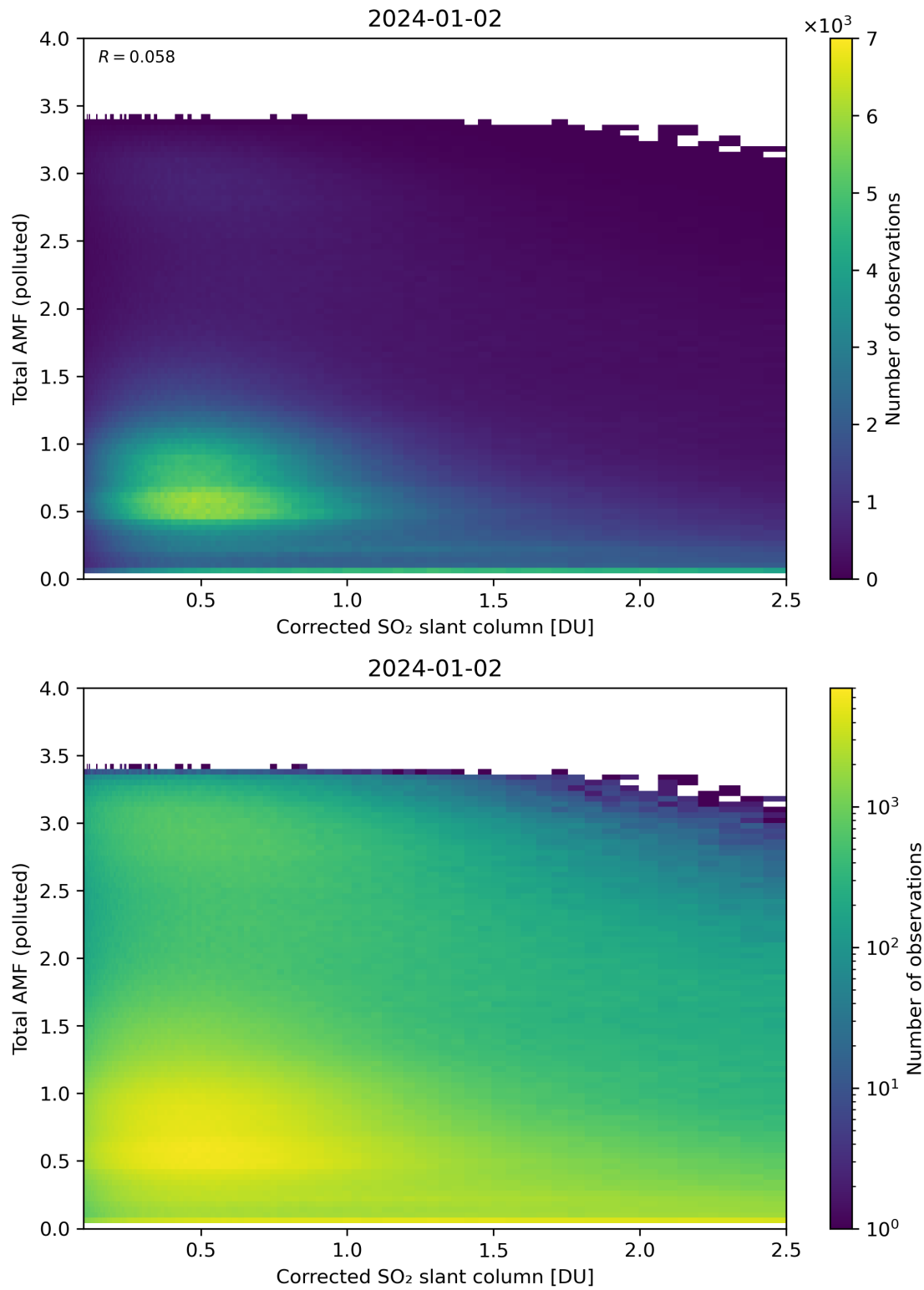
Figure 192: Scatter density plot of “Corrected SO 2 slant column” against “Total AMF (polluted)” for 2024-01-01 to 2024-01-03.
