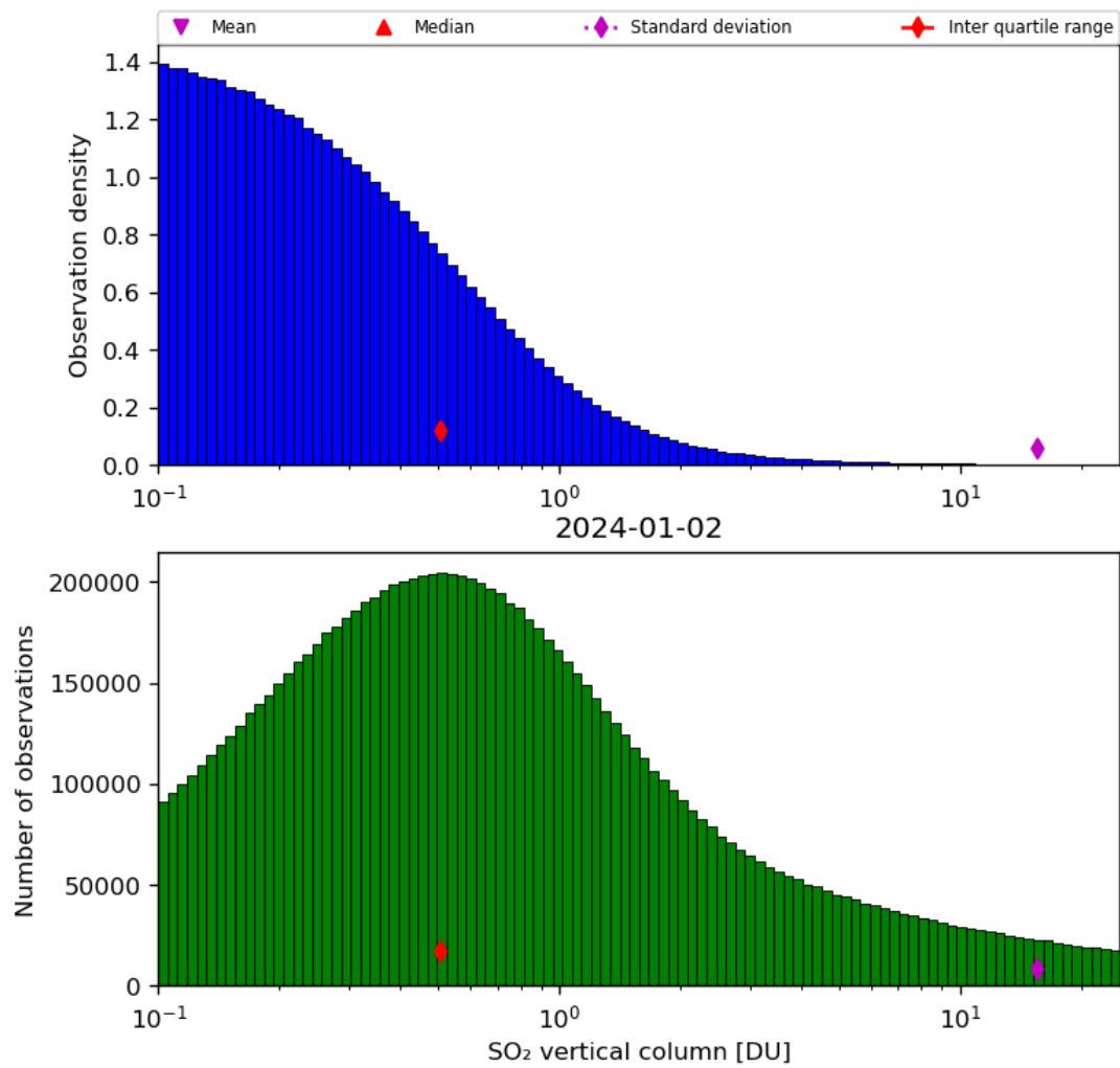
Figure 53: Histogram of “SO 2 vertical column” for 2024-01-01 to 2024-01-03
