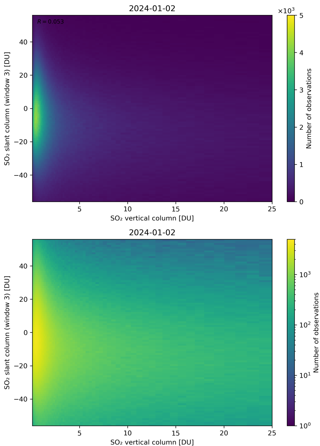
Figure 303: Scatter density plot of “SO 2 vertical column” against “SO 2 slant column (window 3)” for 2024-01-01 to 2024-01-03.
