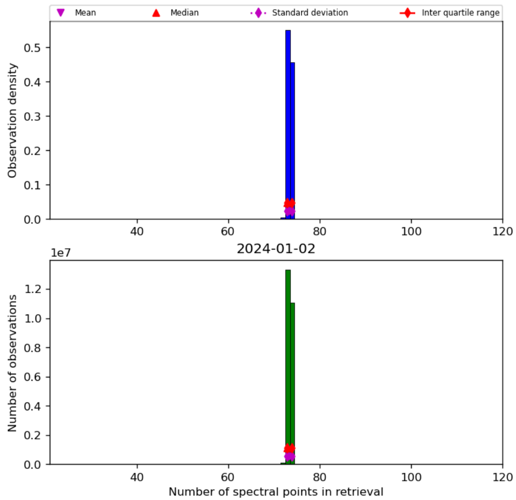
Figure 74: Histogram of “Number of spectral points in retrieval” for 2024-01-01 to 2024-01-03
