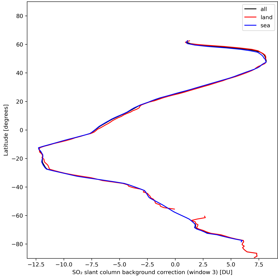
Figure 44: Zonal average of “SO 2 slant column background correction (window 3)” for 2024-01-01 to 2024-01-03.
