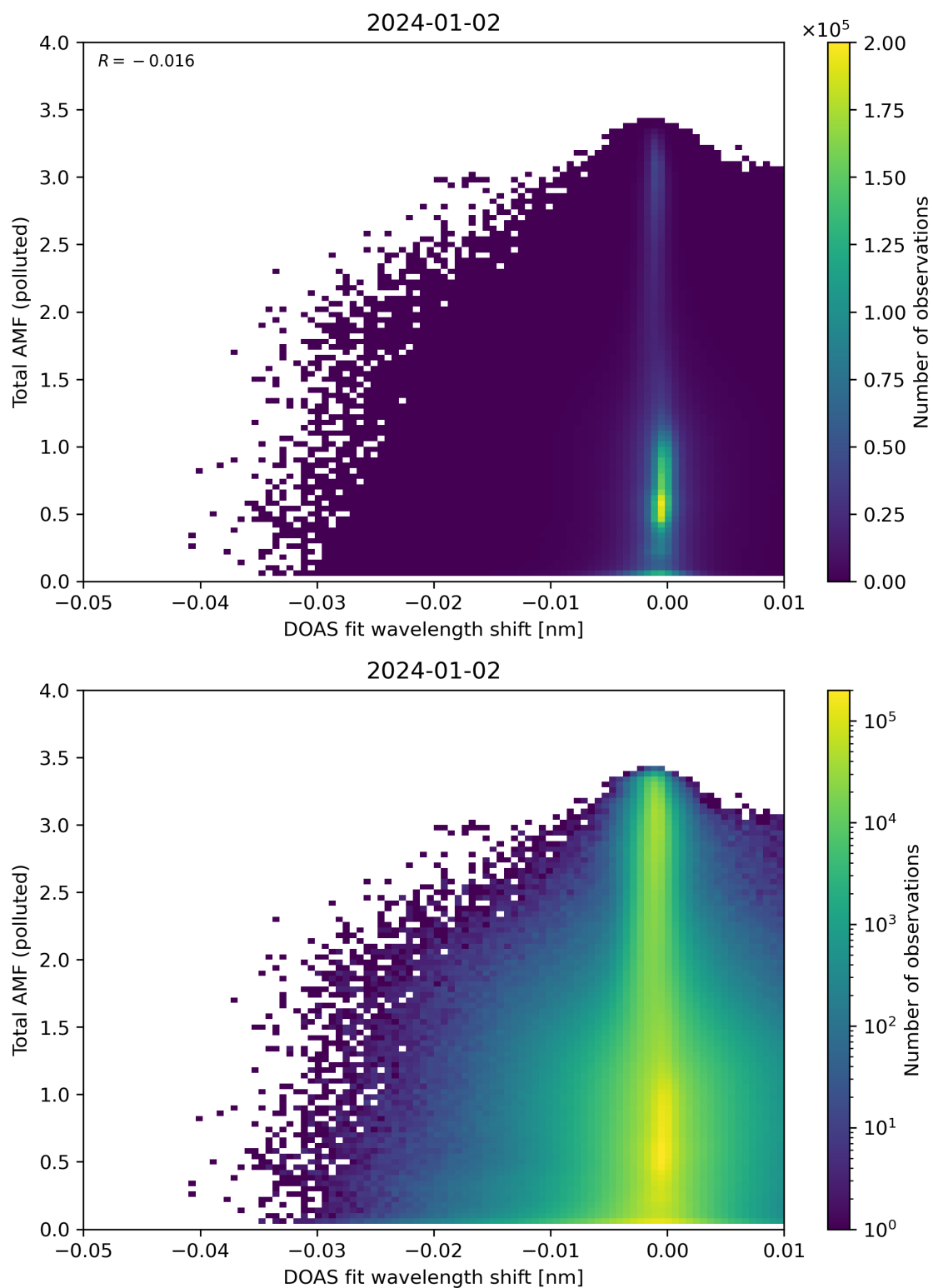
Figure 130: Scatter density plot of “DOAS fit wavelength shift” against “Total AMF (polluted)” for 2024-01-01 to 2024-01-03.
