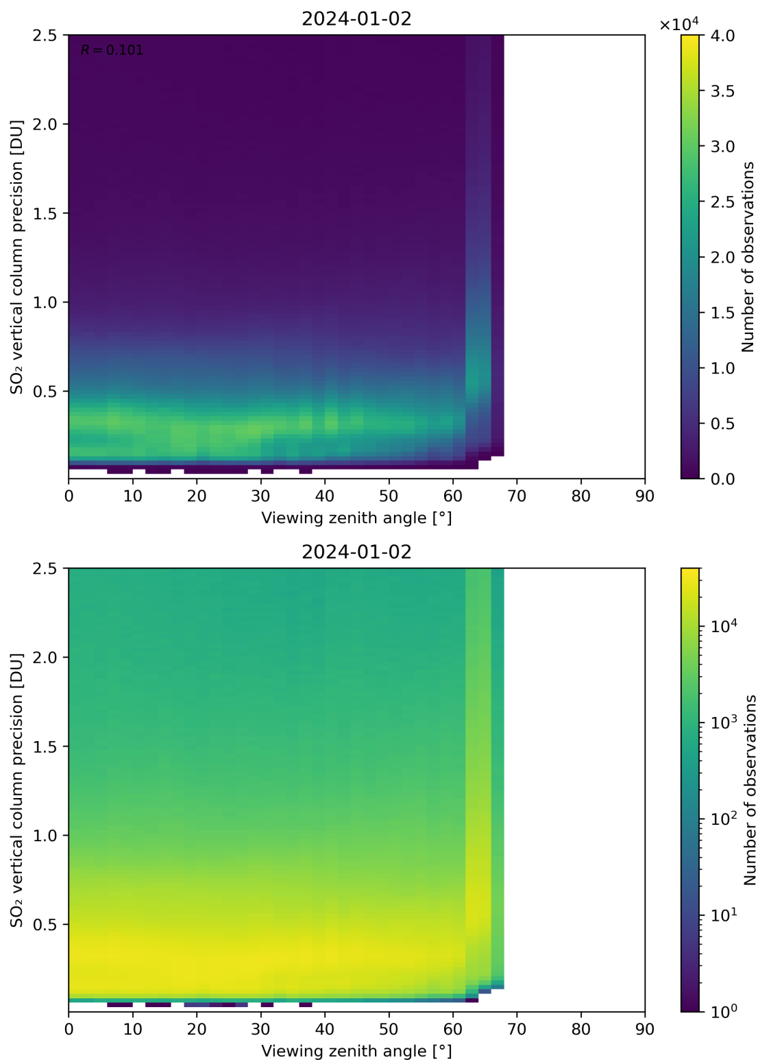
Figure 328: Scatter density plot of “Viewing zenith angle” against “SO 2 vertical column precision” for 2024-01-01 to 2024-01-03.
