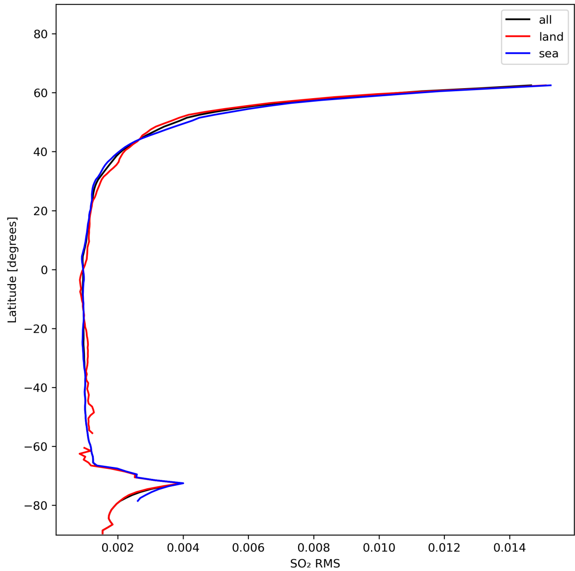
Figure 47: Zonal average of “SO 2 RMS” for 2024-01-01 to 2024-01-03.
