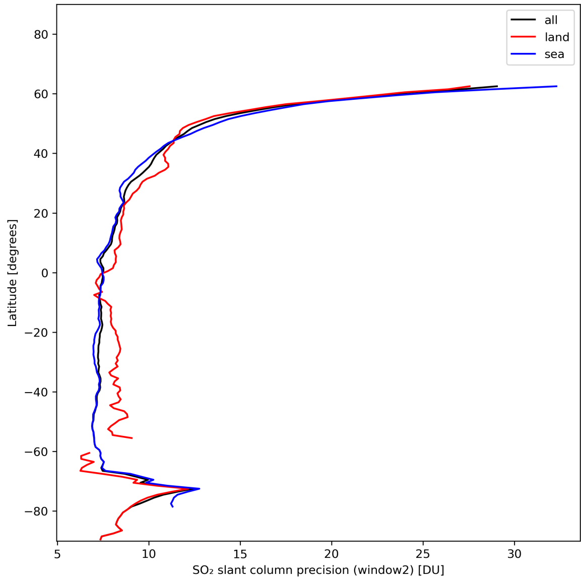
Figure 38: Zonal average of “SO 2 slant column precision (window2)” for 2024-01-01 to 2024-01-03.
