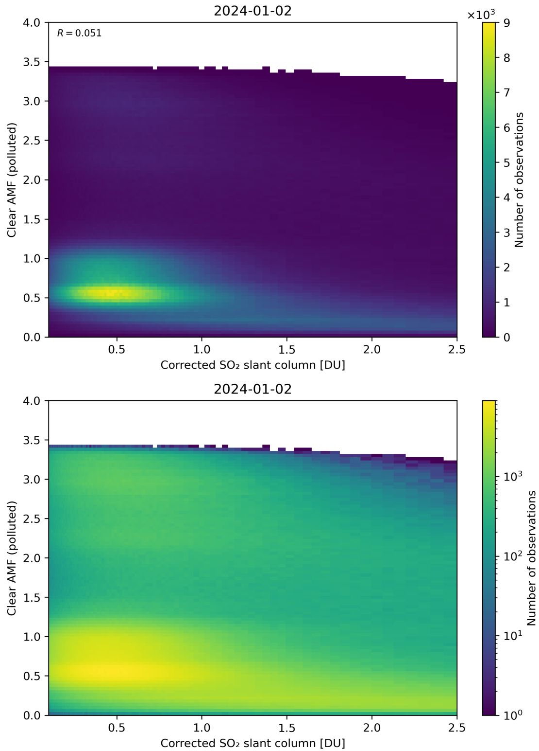
Figure 184: Scatter density plot of “Corrected SO 2 slant column” against “Clear AMF (polluted)” for 2024-01-01 to 2024-01-03.
