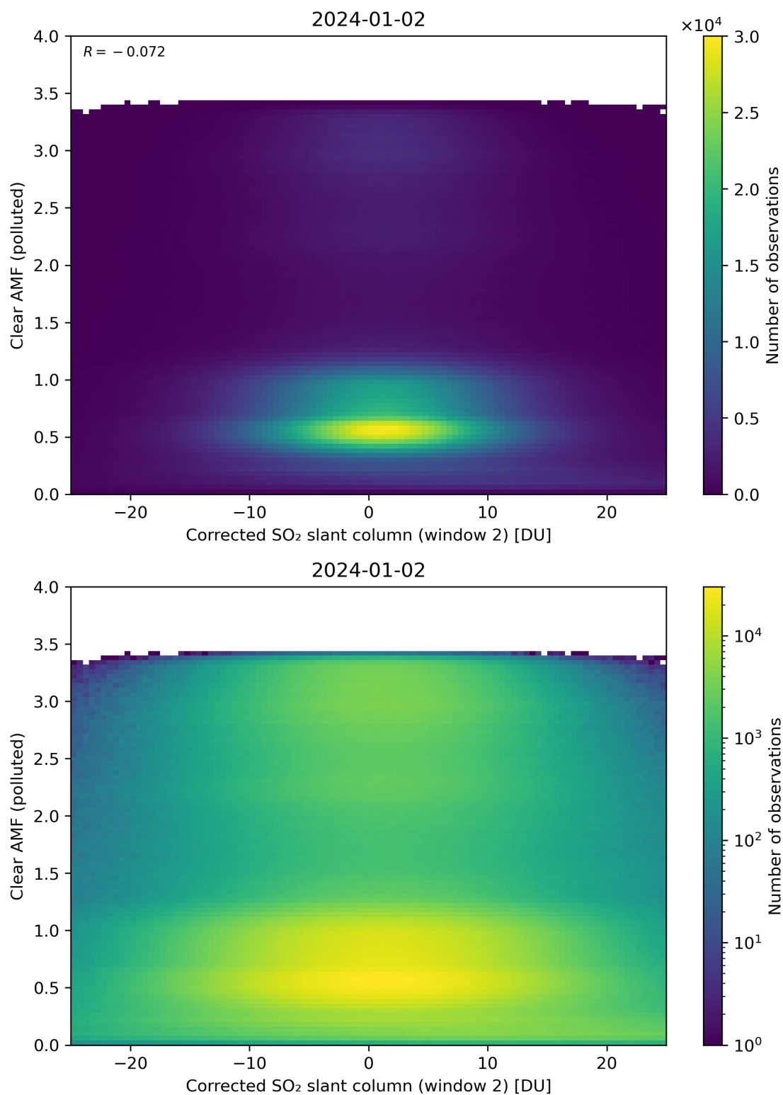
Figure 199: Scatter density plot of “Corrected SO 2 slant column (window 2)” against “Clear AMF (polluted)” for 2024-01-01 to 2024-01-03.
