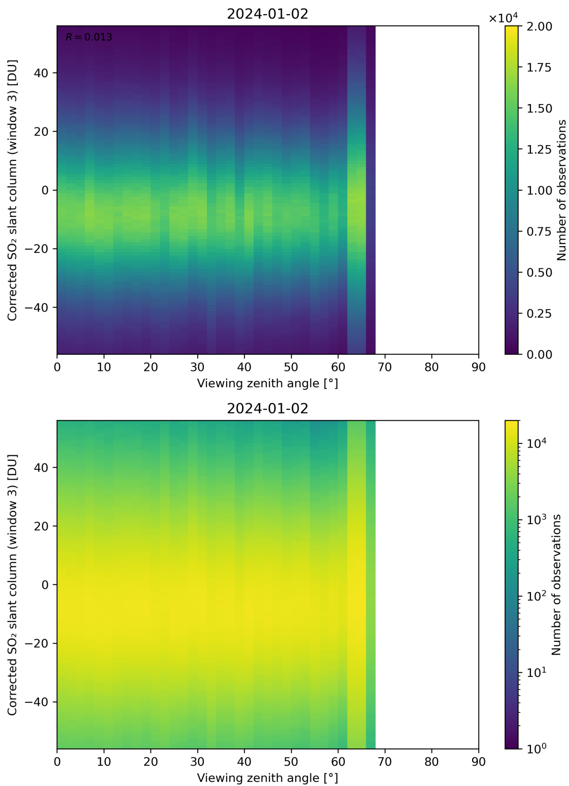
Figure 319: Scatter density plot of “Viewing zenith angle” against “Corrected SO 2 slant column (window 3)” for 2024-01-01 to 2024-01-03.
