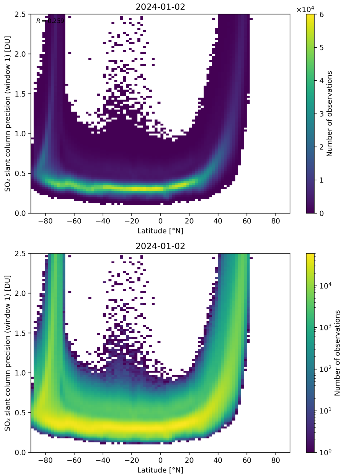
Figure 150: Scatter density plot of “Latitude” against “SO 2 slant column precision (window 1)” for 2024-01-01 to 2024-01-03.
