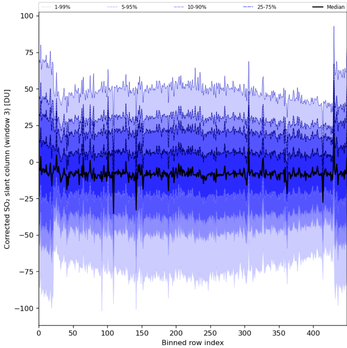
Figure 89: Along track statistics of “Corrected SO 2 slant column (window 3)” for 2024-01-01 to 2024-01-03
