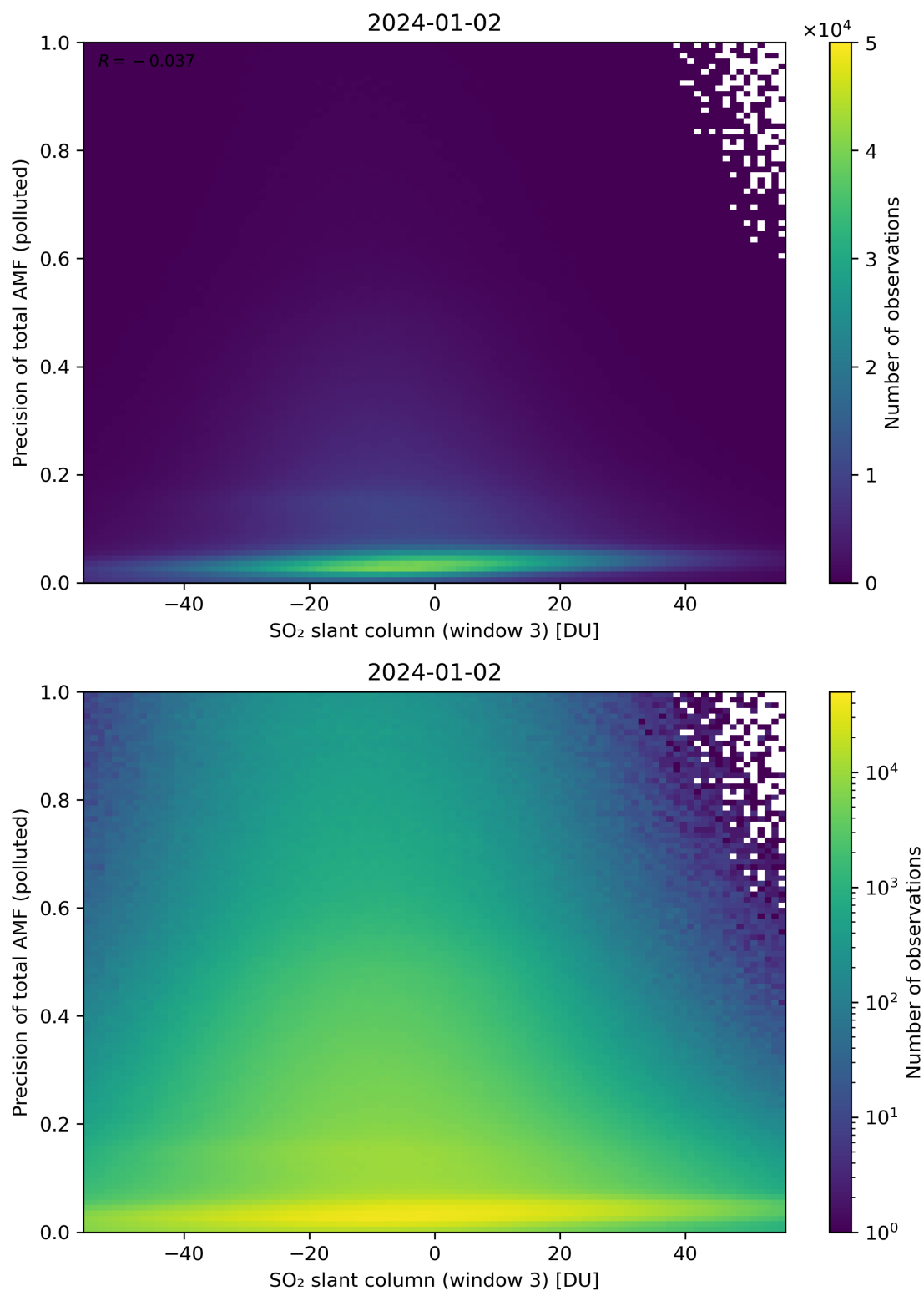
Figure 269: Scatter density plot of “SO 2 slant column (window 3)” against “Precision of total AMF (polluted)” for 2024-01-01 to 2024-01-03.
