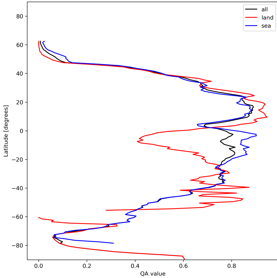
Figure 29: Zonal average of “QA value” for 2024-01-01 to 2024-01-03.
