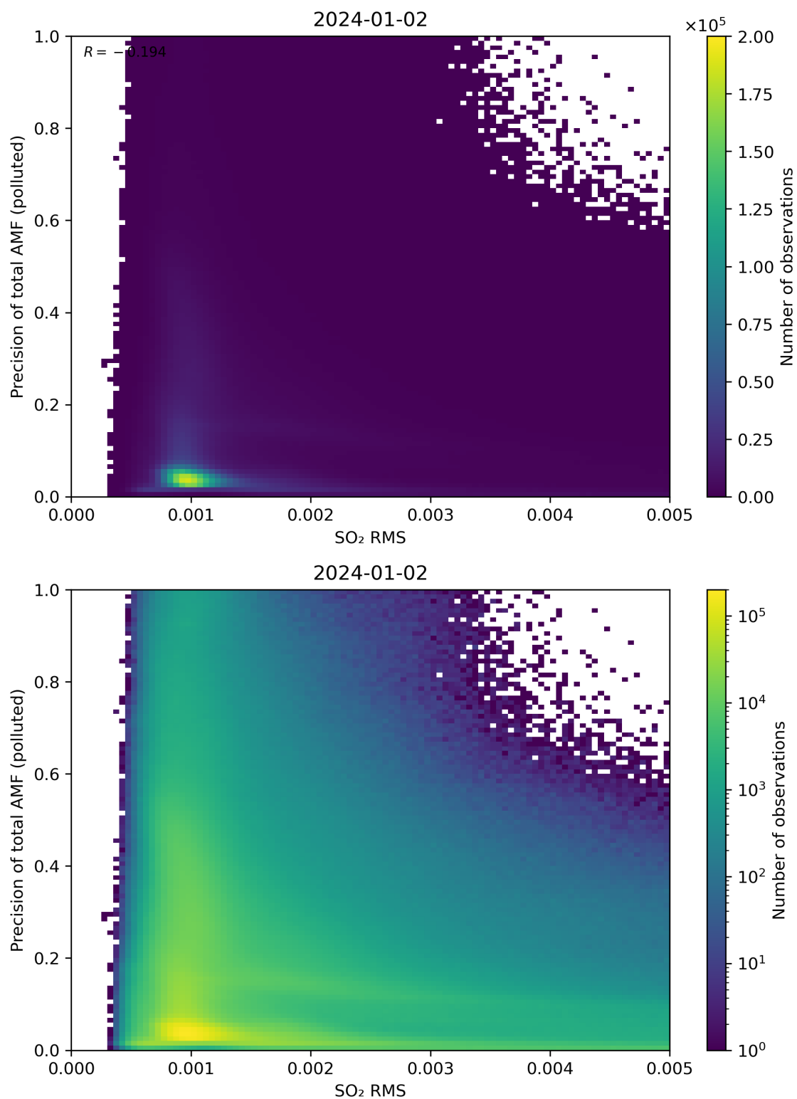
Figure 138: Scatter density plot of “SO 2 RMS” against “Precision of total AMF (polluted)” for 2024-01-01 to 2024-01-03.
