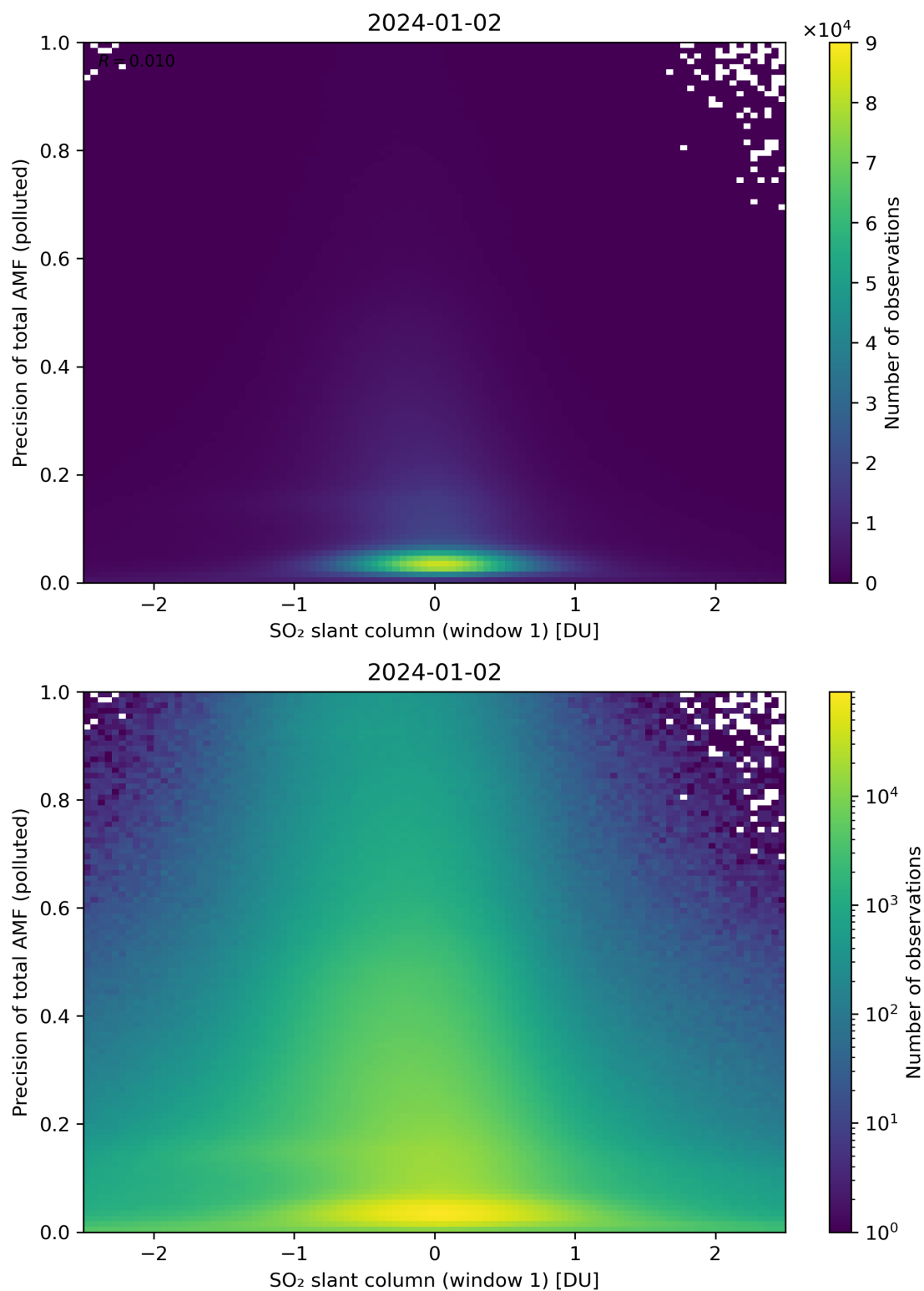
Figure 240: Scatter density plot of “SO 2 slant column (window 1)” against “Precision of total AMF (polluted)” for 2024-01-01 to 2024-01-03.
