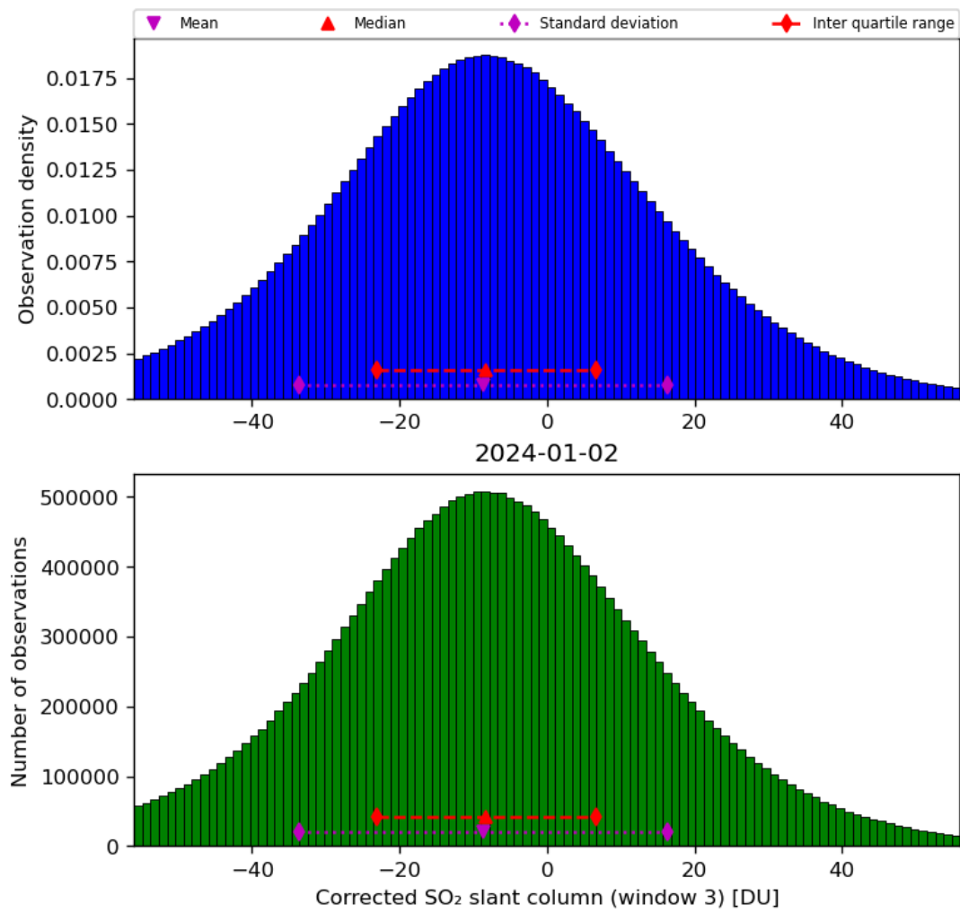
Figure 66: Histogram of “Corrected SO 2 slant column (window 3)” for 2024-01-01 to 2024-01-03
