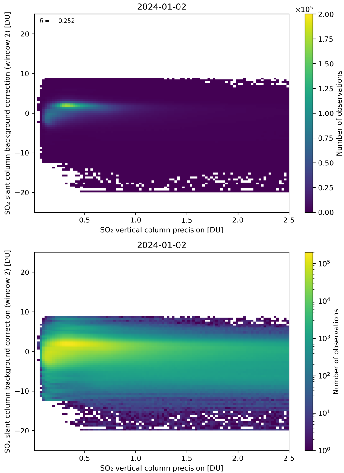
Figure 280: Scatter density plot of “SO 2 vertical column precision” against “SO 2 slant column background correction (window 2)” for 2024-01-01 to 2024-01-03.
