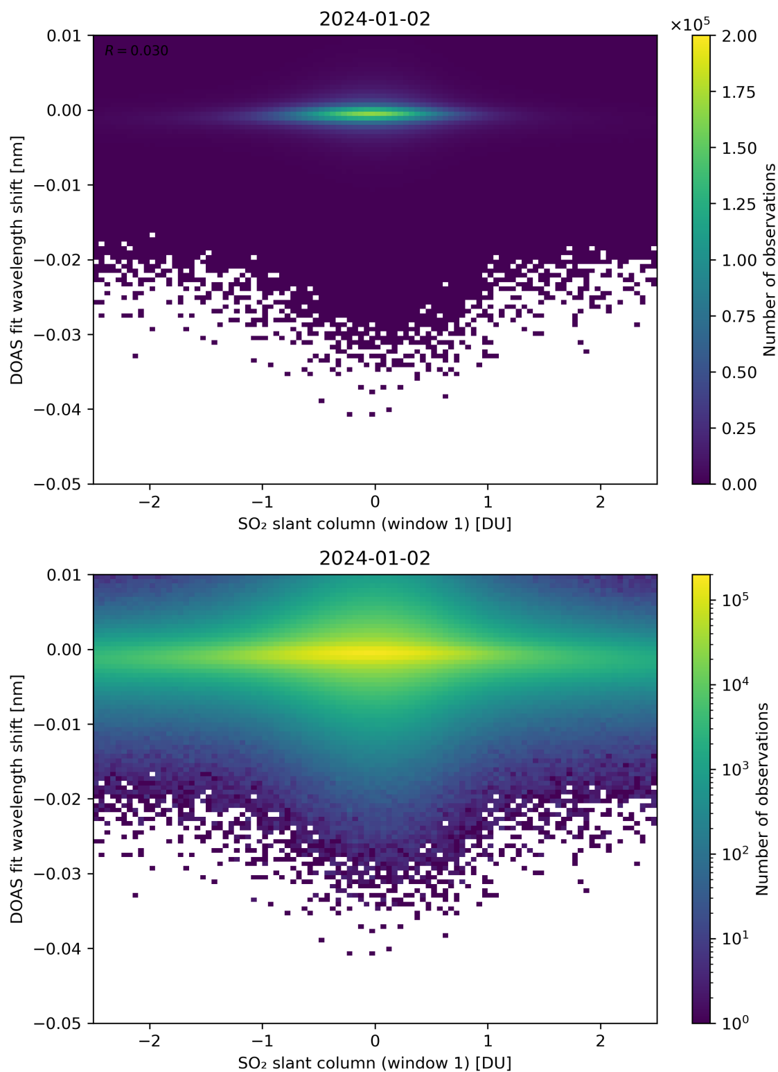
Figure 215: Scatter density plot of “SO 2 slant column (window 1)” against “DOAS fit wavelength shift” for 2024-01-01 to 2024-01-03.
