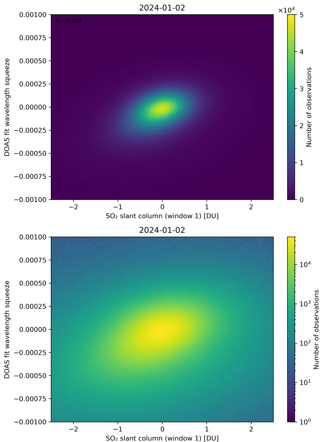
Figure 216: Scatter density plot of “SO 2 slant column (window 1)” against “DOAS fit wavelength squeeze” for 2024-01-01 to 2024-01-03.
