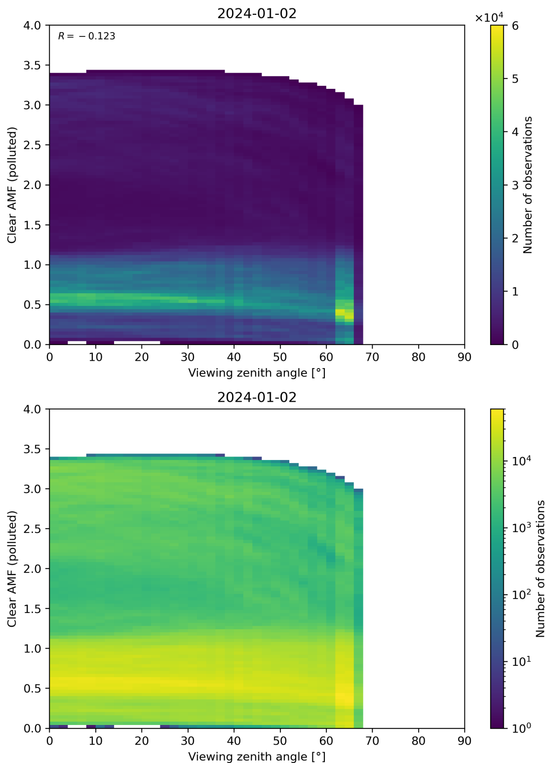
Figure 316: Scatter density plot of “Viewing zenith angle” against “Clear AMF (polluted)” for 2024-01-01 to 2024-01-03.
