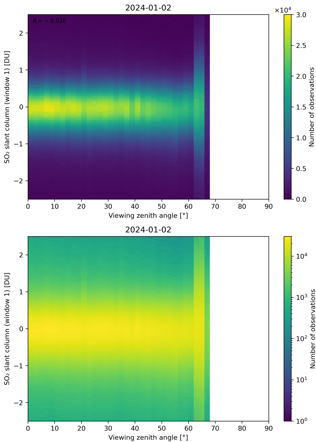
Figure 320: Scatter density plot of “Viewing zenith angle” against “SO 2 slant column (window 1)” for 2024-01-01 to 2024-01-03.
