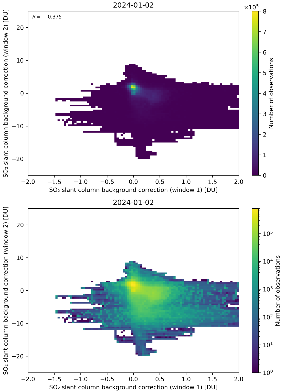
Figure 98: Scatter density plot of “SO 2 slant column background correction (window 1)” against “SO 2 slant column background correction (window 2)” for 2024-01-01 to 2024-01-03.
