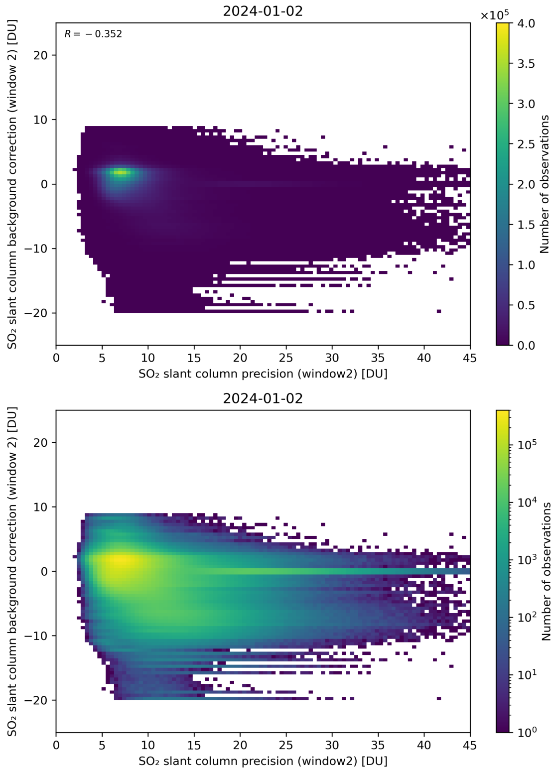
Figure 241: Scatter density plot of “SO 2 slant column precision (window2)” against “SO 2 slant column background correction (window 2)” for 2024-01-01 to 2024-01-03.
