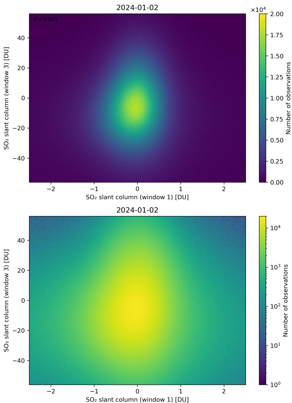
Figure 237: Scatter density plot of “SO 2 slant column (window 1)” against “SO 2 slant column (window 3)” for 2024-01-01 to 2024-01-03.
