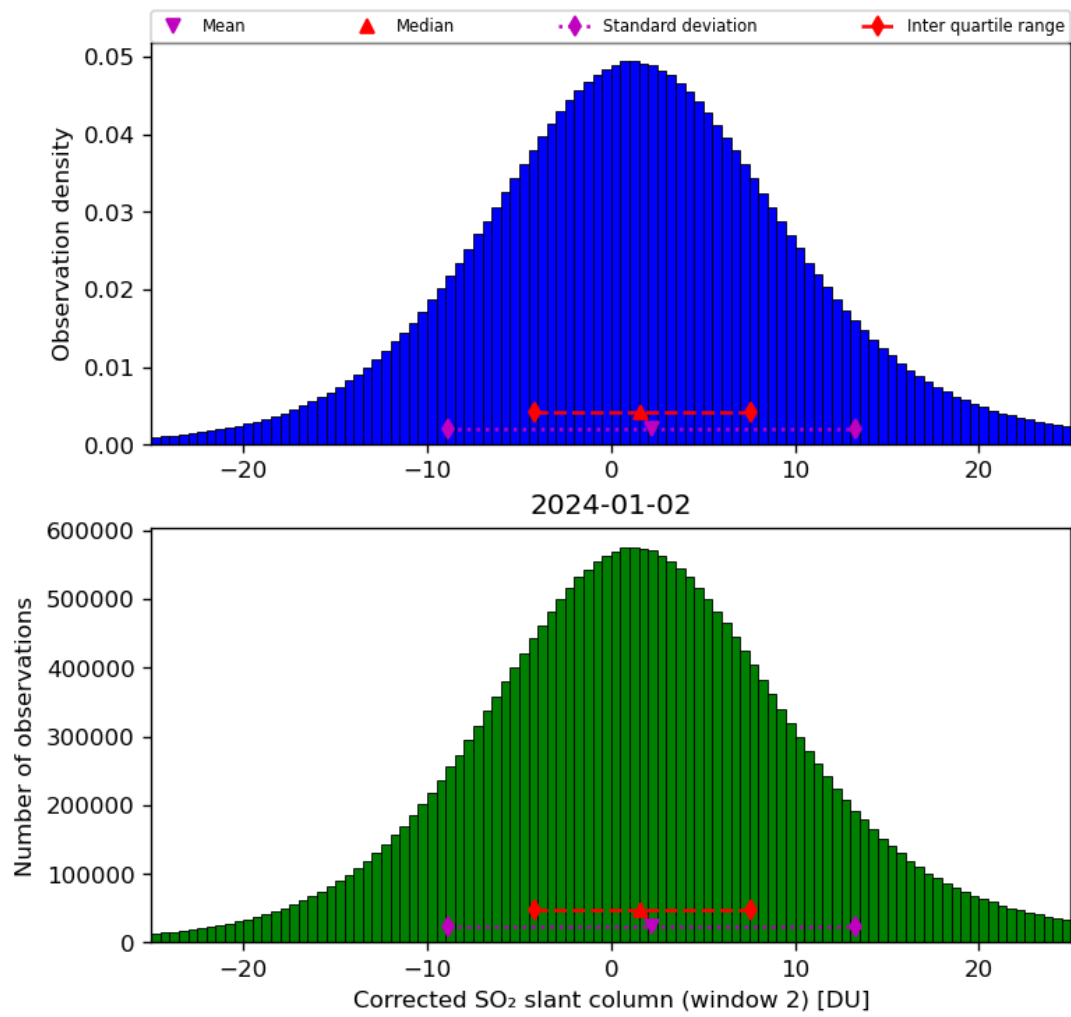
Figure 62: Histogram of “Corrected SO 2 slant column (window 2)” for 2024-01-01 to 2024-01-03
