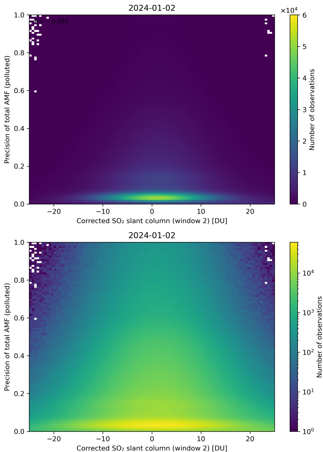
Figure 204: Scatter density plot of “Corrected SO 2 slant column (window 2)” against “Precision of total AMF (polluted)” for 2024-01-01 to 2024-01-03.
