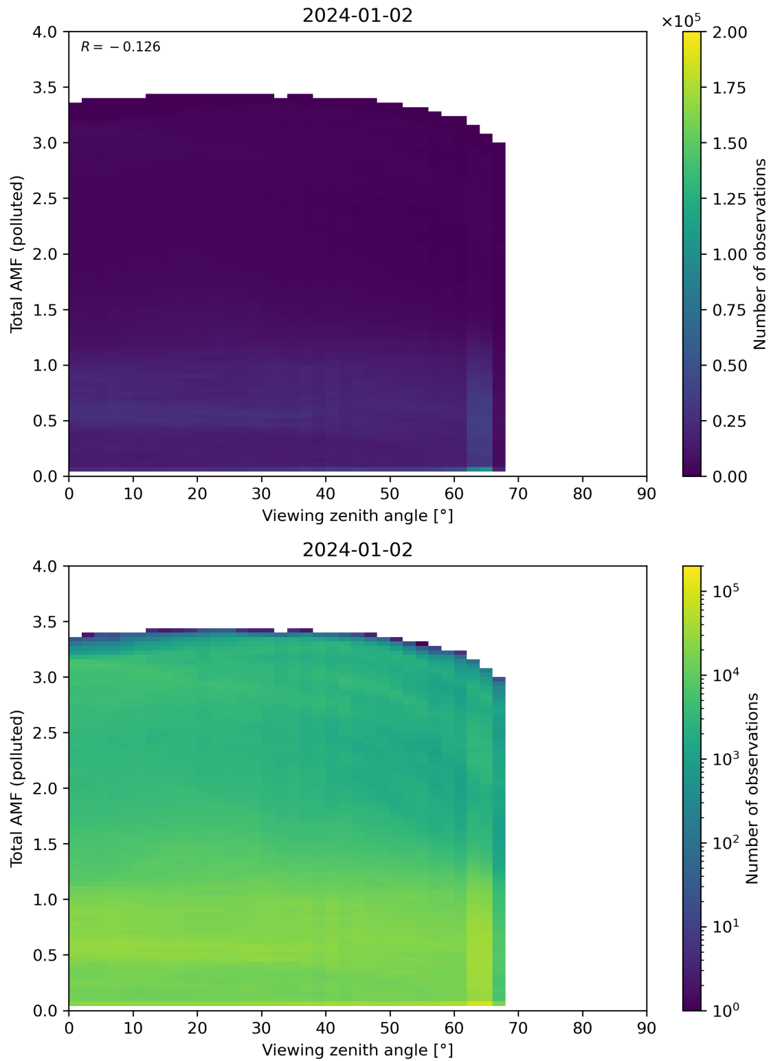
Figure 325: Scatter density plot of “Viewing zenith angle” against “Total AMF (polluted)” for 2024-01-01 to 2024-01-03.
