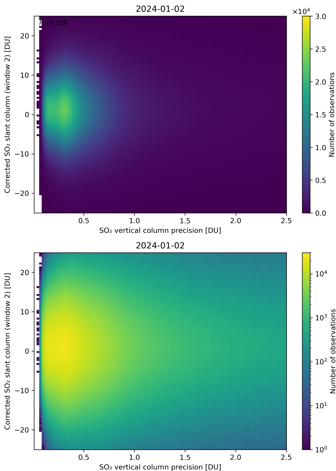
Figure 287: Scatter density plot of “SO 2 vertical column precision” against “Corrected SO 2 slant column (window 2)” for 2024-01-01 to 2024-01-03.
