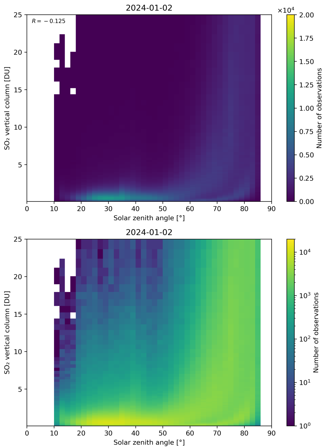
Figure 176: Scatter density plot of “Solar zenith angle” against “SO 2 vertical column” for 2024-01-01 to 2024-01-03.
