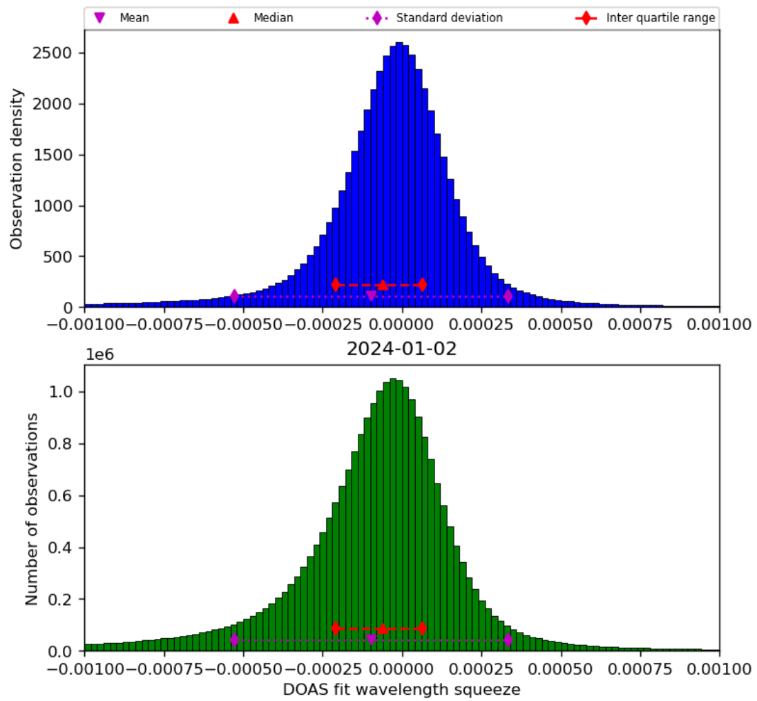
Figure 69: Histogram of “DOAS fit wavelength squeeze” for 2024-01-01 to 2024-01-03
