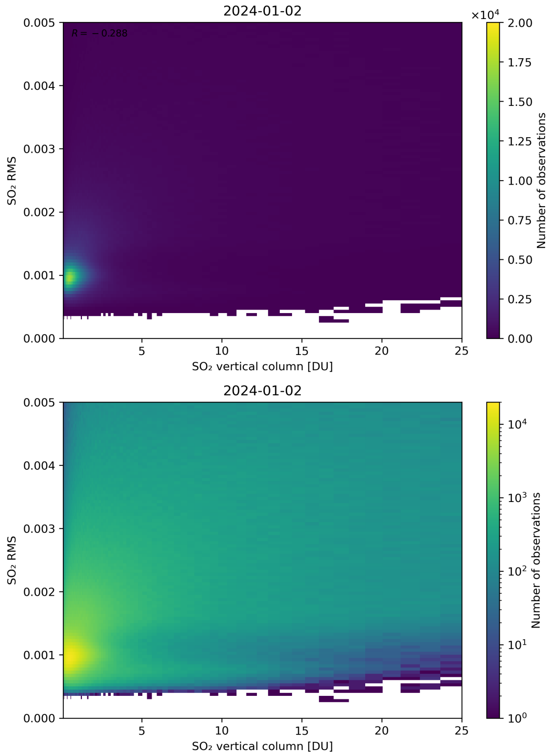
Figure 278: Scatter density plot of “SO 2 vertical column” against “SO 2 RMS” for 2024-01-01 to 2024-01-03.
