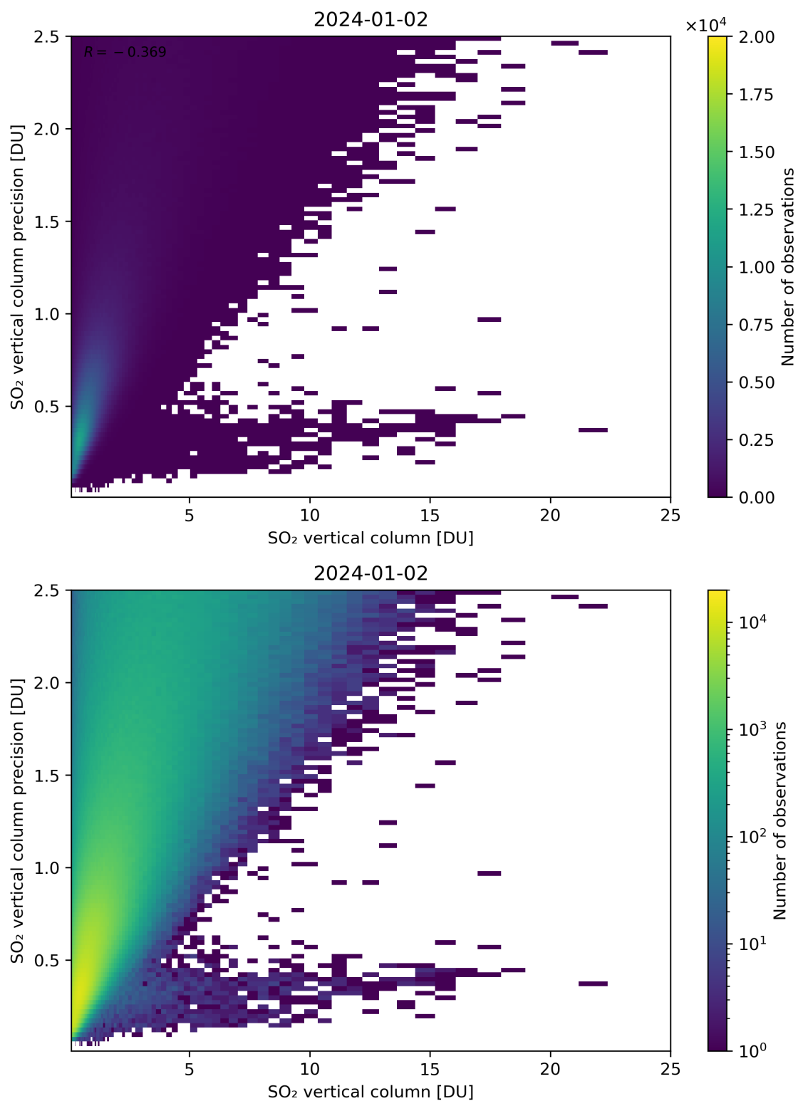
Figure 307: Scatter density plot of “SO 2 vertical column” against “SO 2 vertical column precision” for 2024-01-01 to 2024-01-03.
