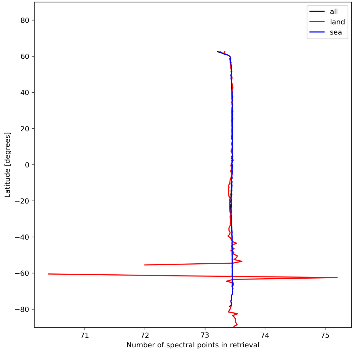
Figure 51: Zonal average of “Number of spectral points in retrieval” for 2024-01-01 to 2024-01-03.
