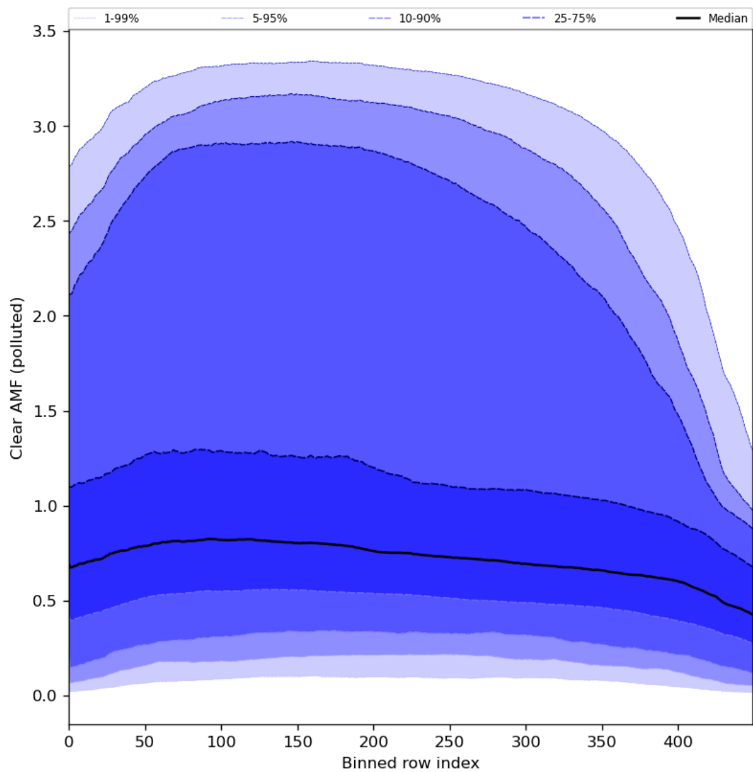
Figure 96: Along track statistics of “Clear AMF (polluted)” for 2024-01-01 to 2024-01-03
