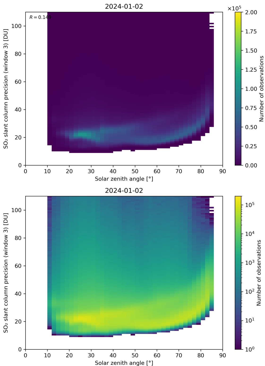
Figure 173: Scatter density plot of “Solar zenith angle” against “SO 2 slant column precision (window 3)” for 2024-01-01 to 2024-01-03.
