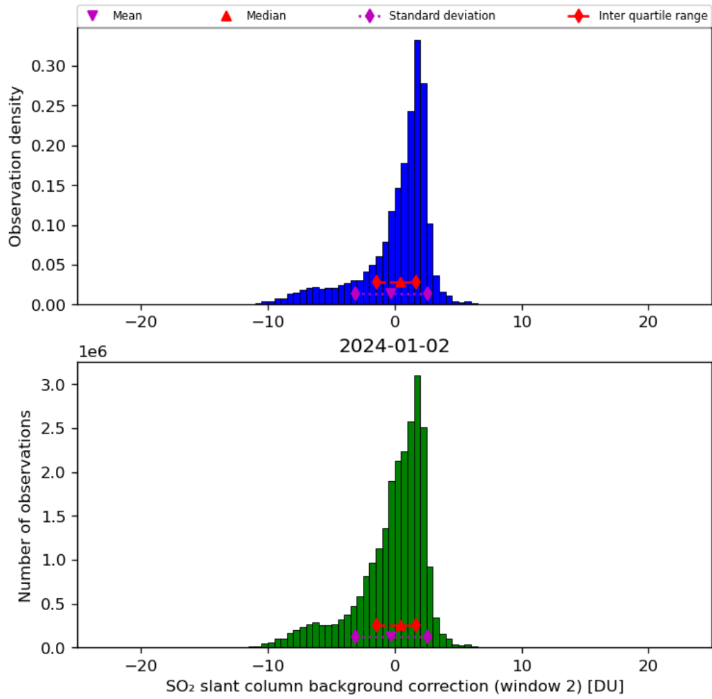
Figure 63: Histogram of “SO 2 slant column background correction (window 2)” for 2024-01-01 to 2024-01-03
