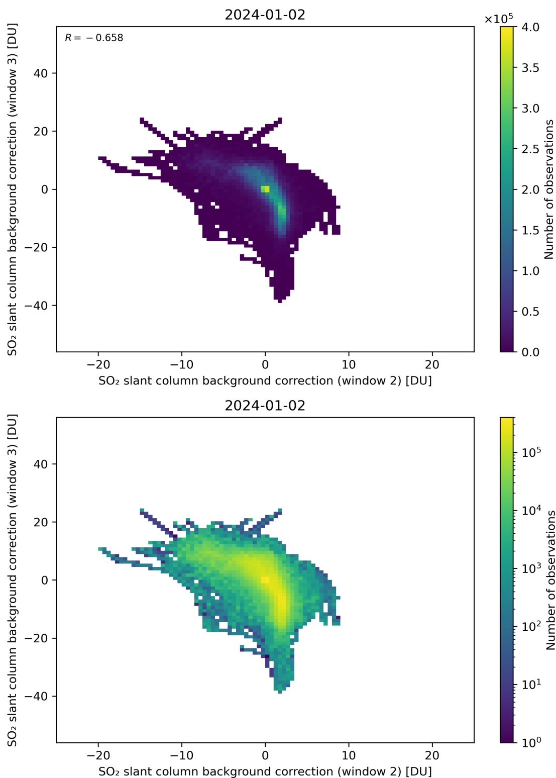
Figure 111: Scatter density plot of “SO 2 slant column background correction (window 2)” against “SO 2 slant column background correction (window 3)” for 2024-01-01 to 2024-01-03.
