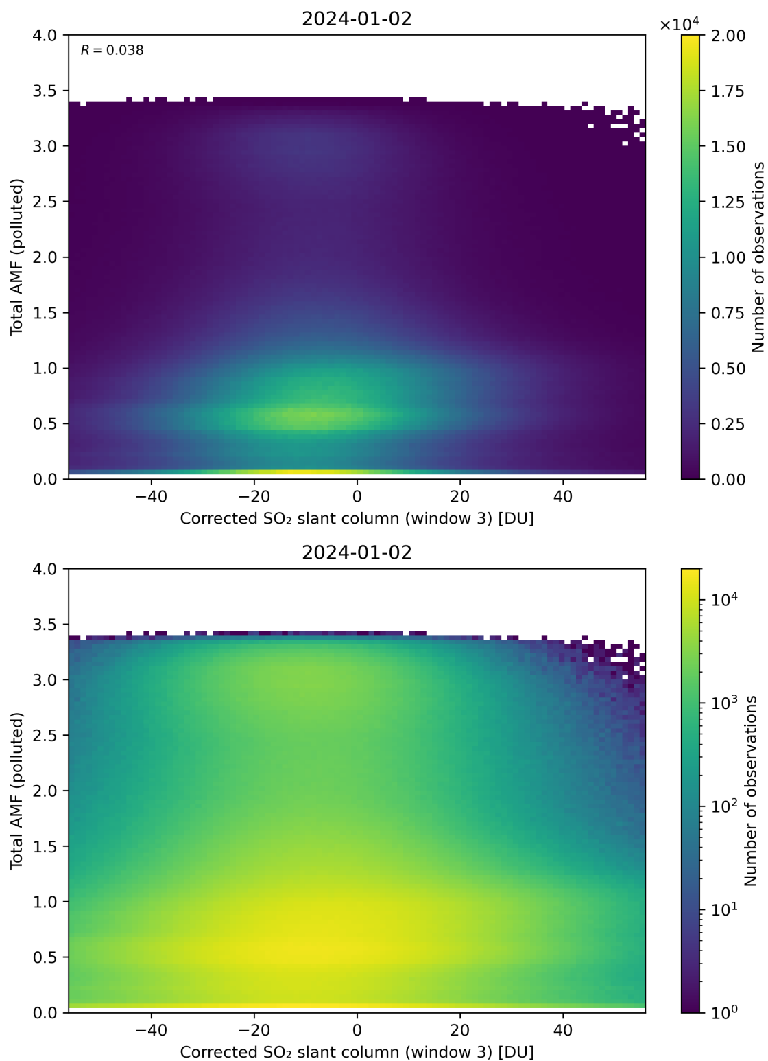
Figure 210: Scatter density plot of “Corrected SO 2 slant column (window 3)” against “Total AMF (polluted)” for 2024-01-01 to 2024-01-03.
