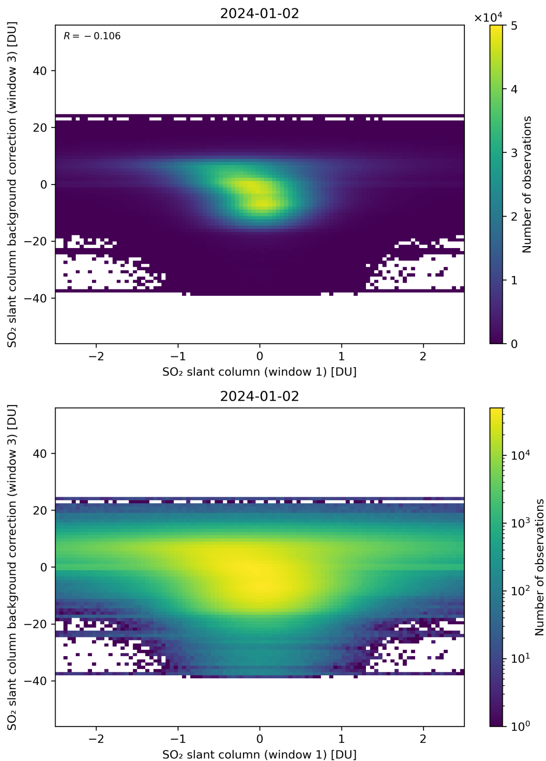
Figure 214: Scatter density plot of “SO 2 slant column (window 1)” against “SO 2 slant column background correction (window 3)” for 2024-01-01 to 2024-01-03.
