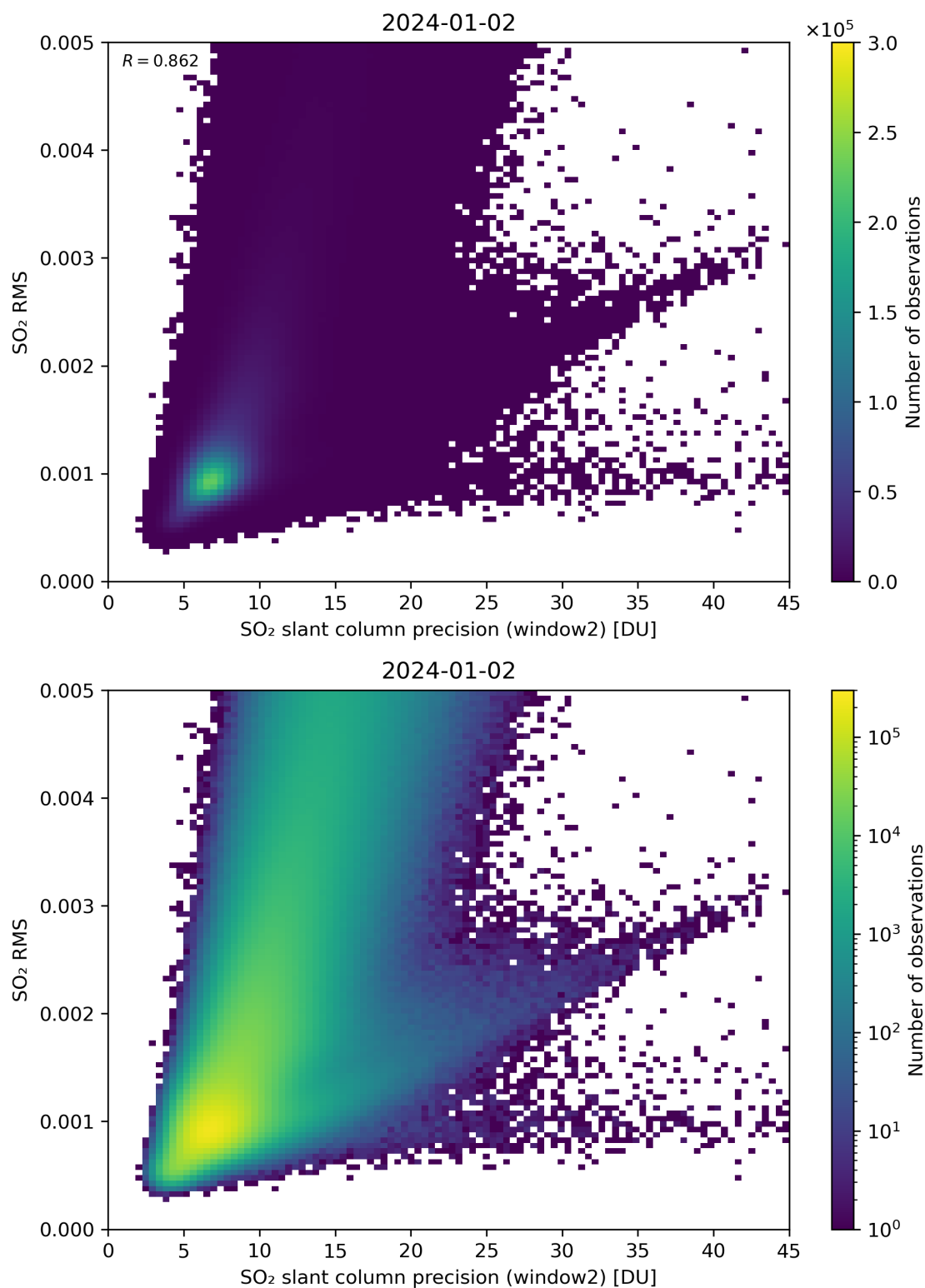
Figure 245: Scatter density plot of “SO 2 slant column precision (window2)” against “SO 2 RMS” for 2024-01-01 to 2024-01-03.
