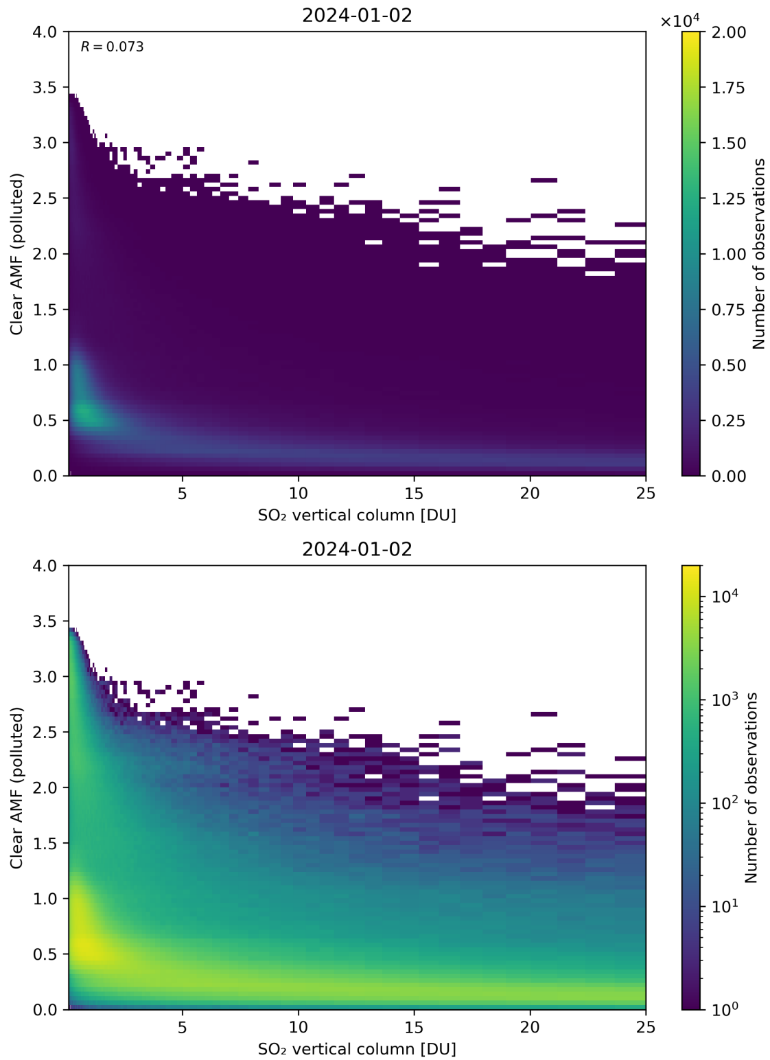
Figure 296: Scatter density plot of “SO 2 vertical column” against “Clear AMF (polluted)” for 2024-01-01 to 2024-01-03.
