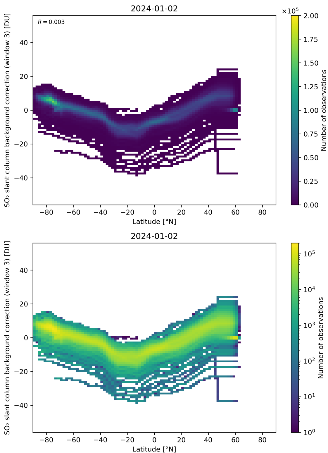
Figure 141: Scatter density plot of “Latitude” against “SO 2 slant column background correction (window 3)” for 2024-01-01 to 2024-01-03.
