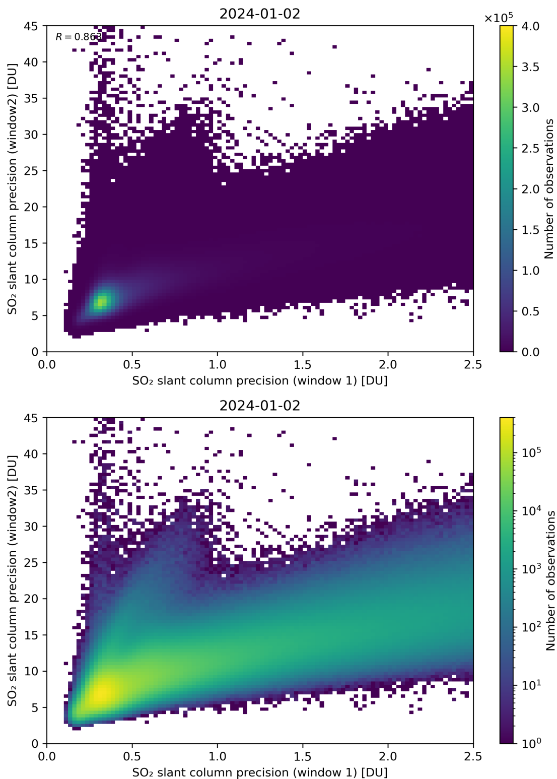
Figure 227: Scatter density plot of “SO 2 slant column precision (window 1)” against “SO 2 slant column precision (window2)” for 2024-01-01 to 2024-01-03.
