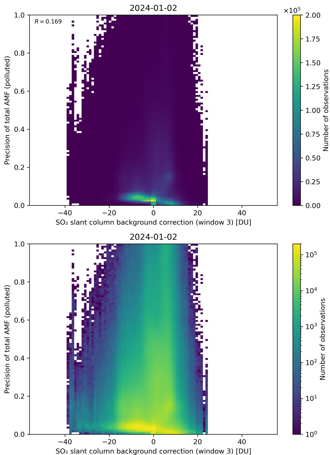
Figure 126: Scatter density plot of “SO 2 slant column background correction (window 3)” against “Precision of total AMF (polluted)” for 2024-01-01 to 2024-01-03.
