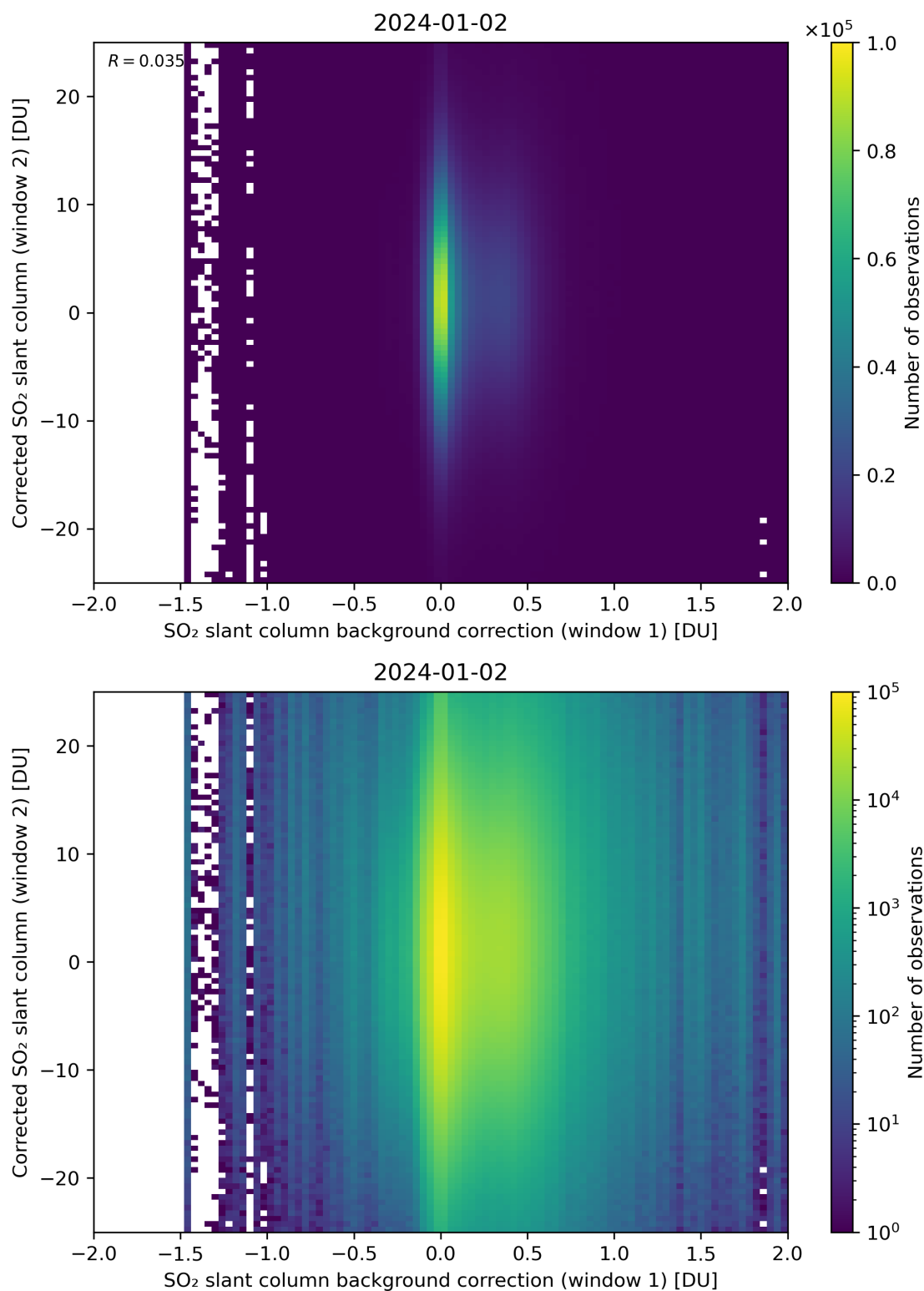
Figure 104: Scatter density plot of “SO 2 slant column background correction (window 1)” against “Corrected SO 2 slant column (window 2)” for 2024-01-01 to 2024-01-03.
