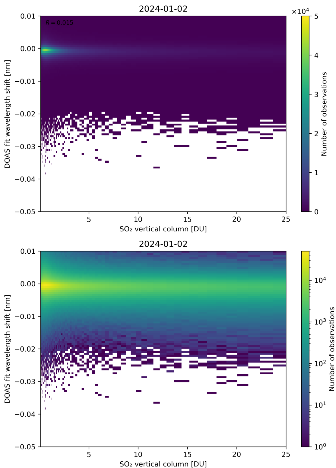
Figure 276: Scatter density plot of “SO 2 vertical column” against “DOAS fit wavelength shift” for 2024-01-01 to 2024-01-03.
