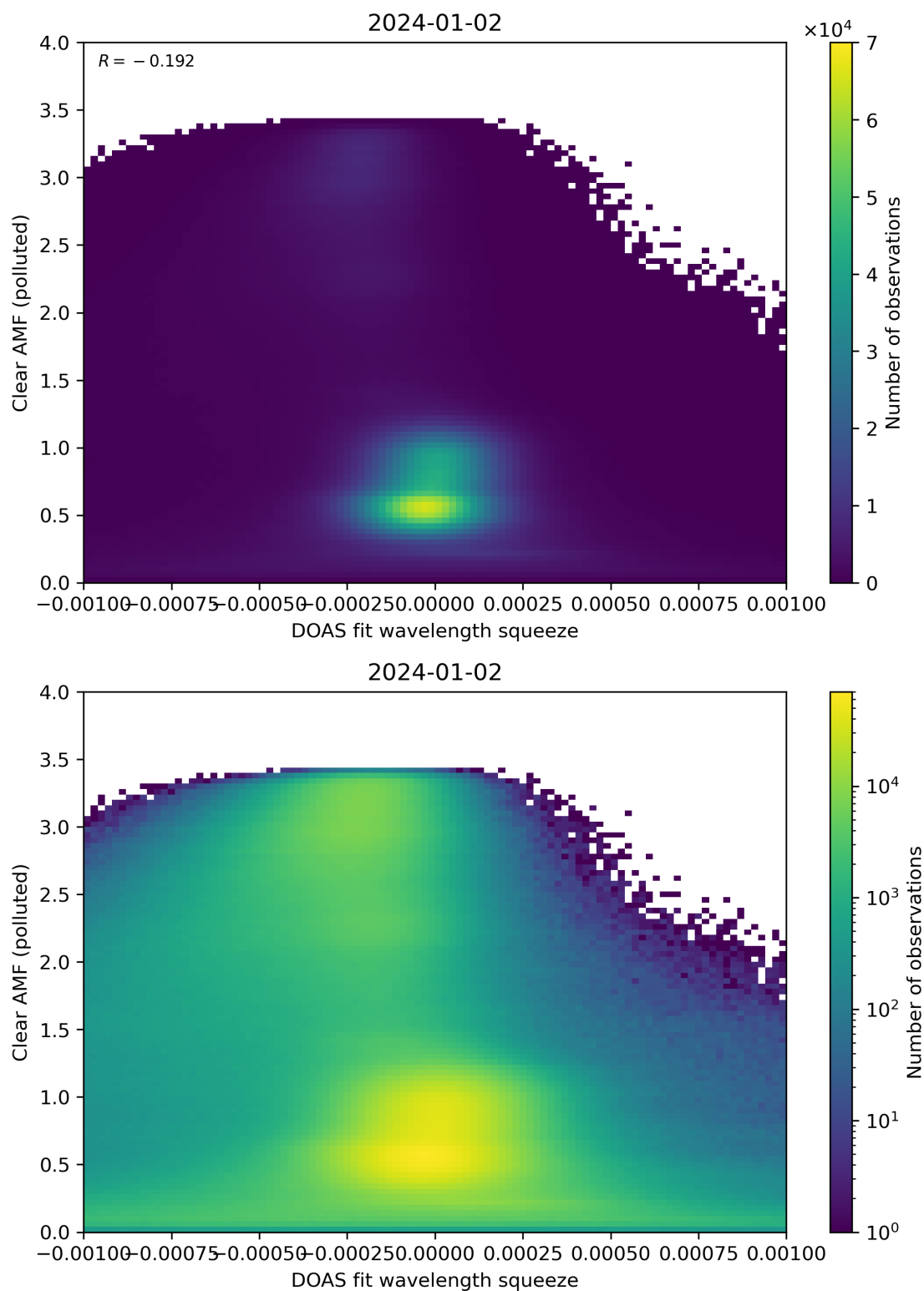
Figure 133: Scatter density plot of “DOAS fit wavelength squeeze” against “Clear AMF (polluted)” for 2024-01-01 to 2024-01-03.
