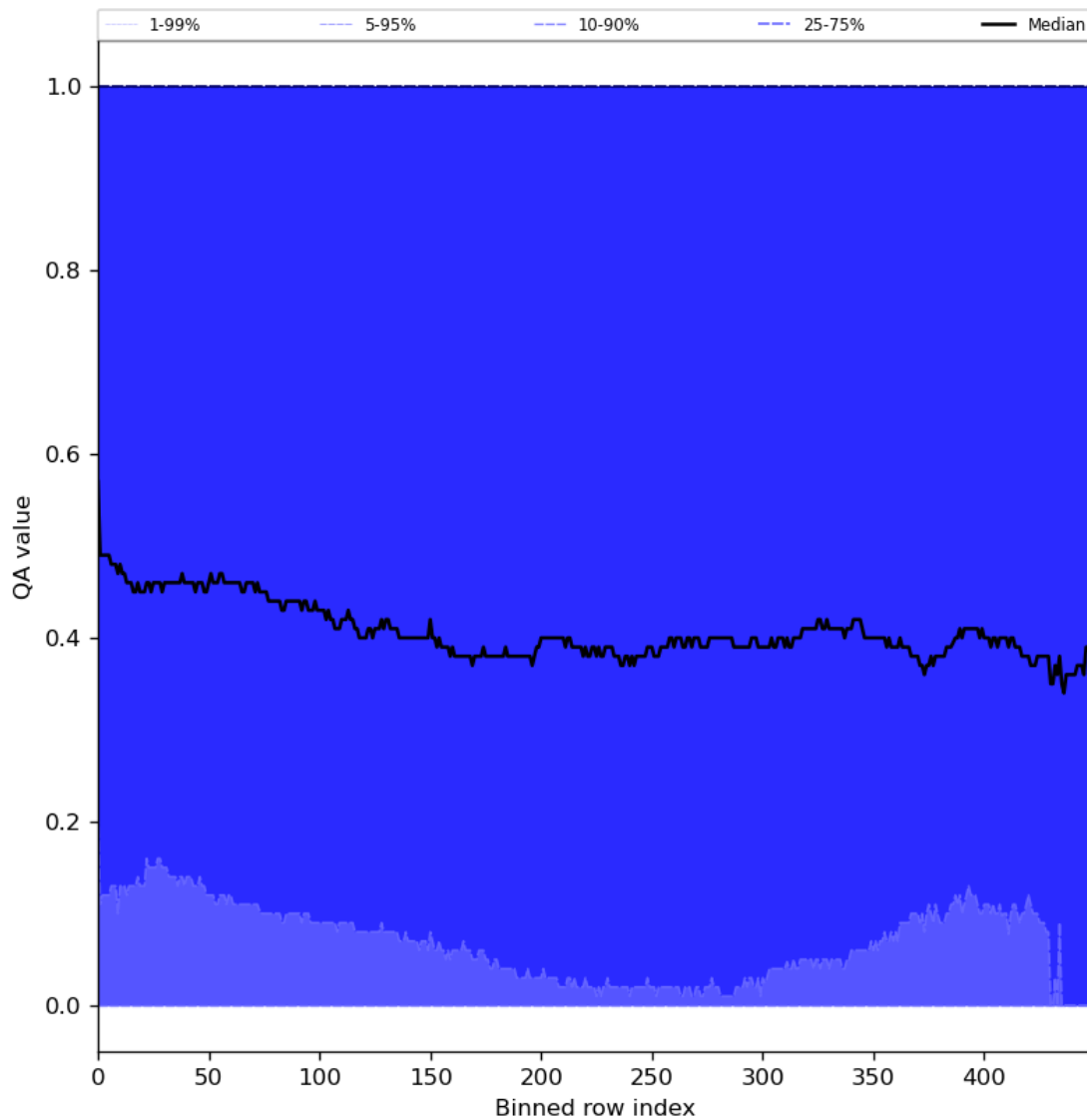
Figure 75: Along track statistics of “QA value” for 2024-01-01 to 2024-01-03
