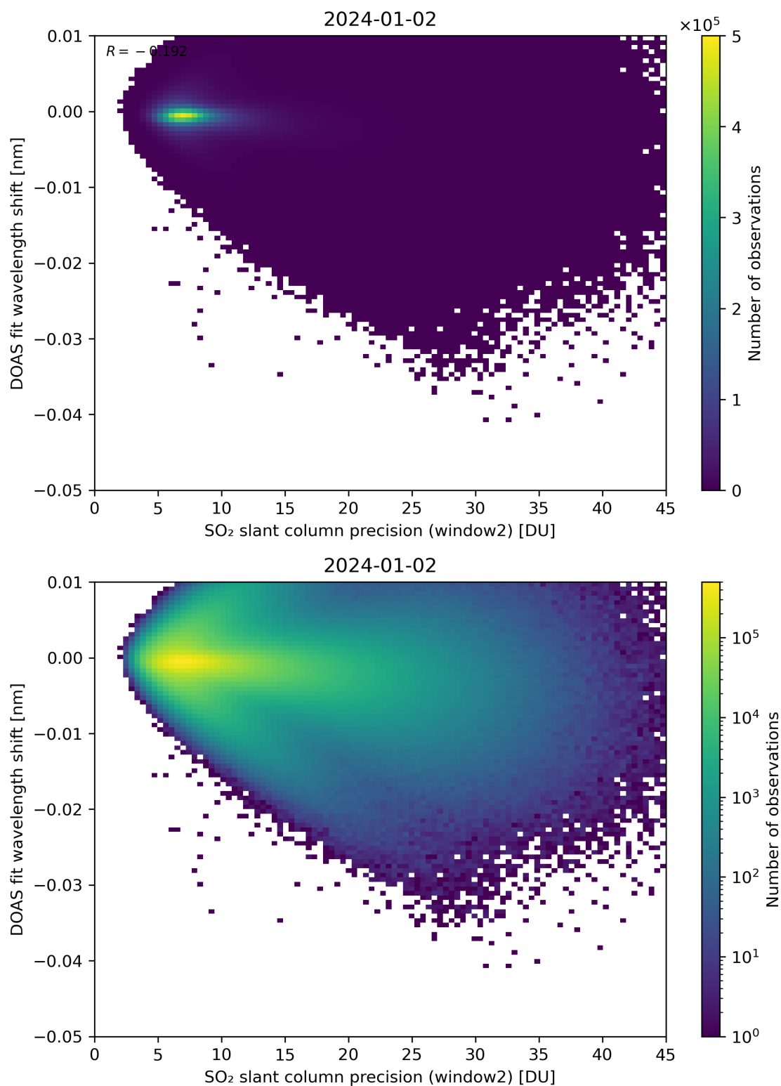
Figure 243: Scatter density plot of “SO 2 slant column precision (window2)” against “DOAS fit wavelength shift” for 2024-01-01 to 2024-01-03.
