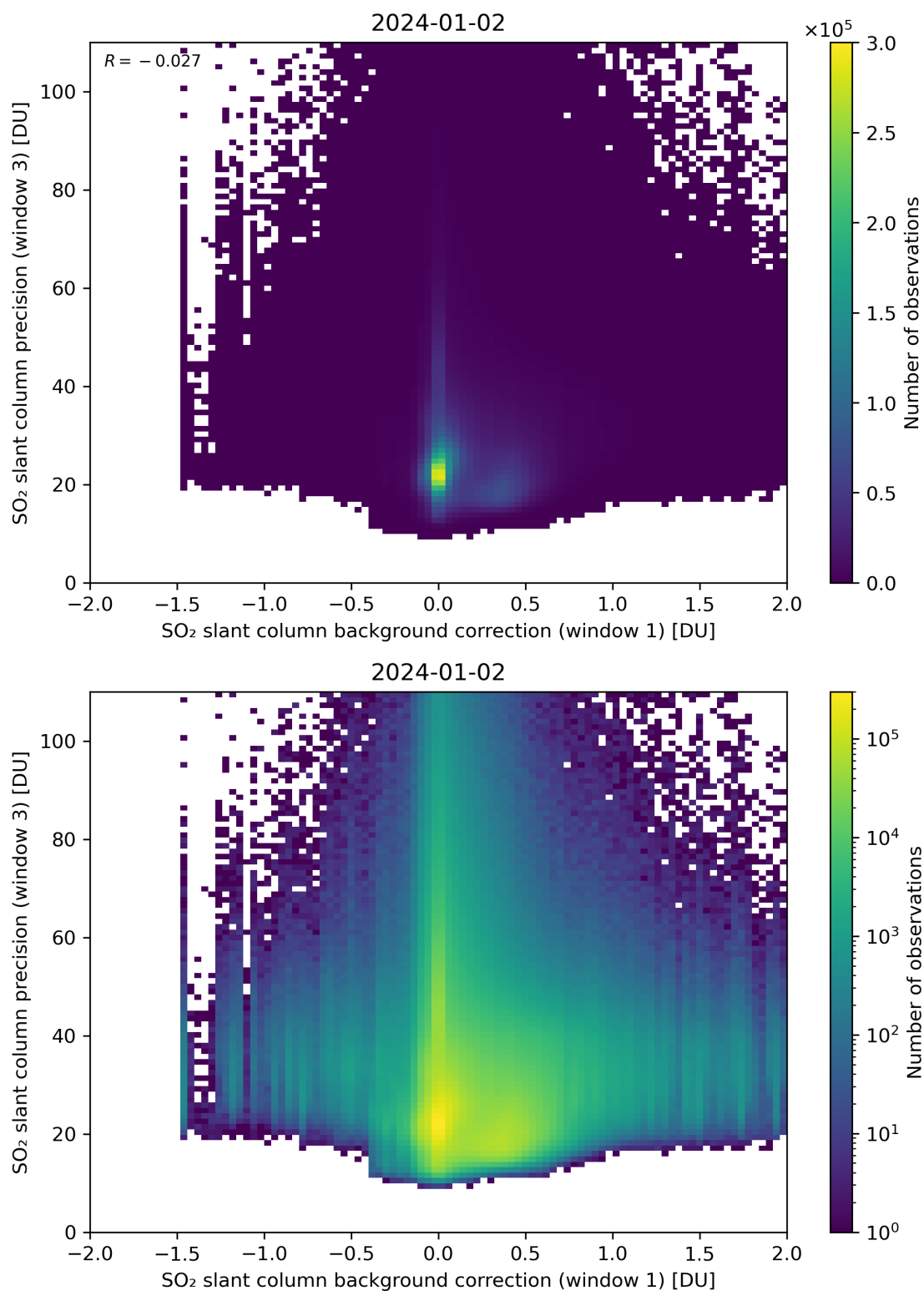
Figure 108: Scatter density plot of “SO 2 slant column background correction (window 1)” against “SO 2 slant column precision (window 3)” for 2024-01-01 to 2024-01-03.
