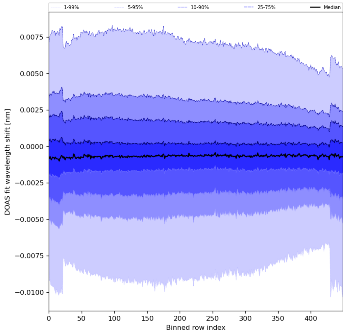
Figure 91: Along track statistics of “DOAS fit wavelength shift” for 2024-01-01 to 2024-01-03
