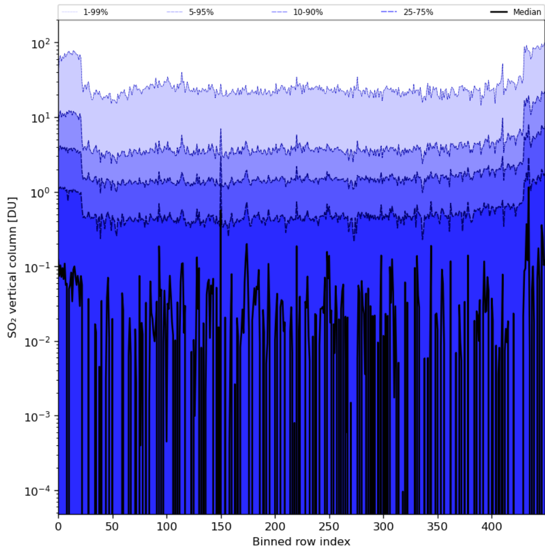
Figure 76: Along track statistics of “SO 2 vertical column” for 2024-01-01 to 2024-01-03
