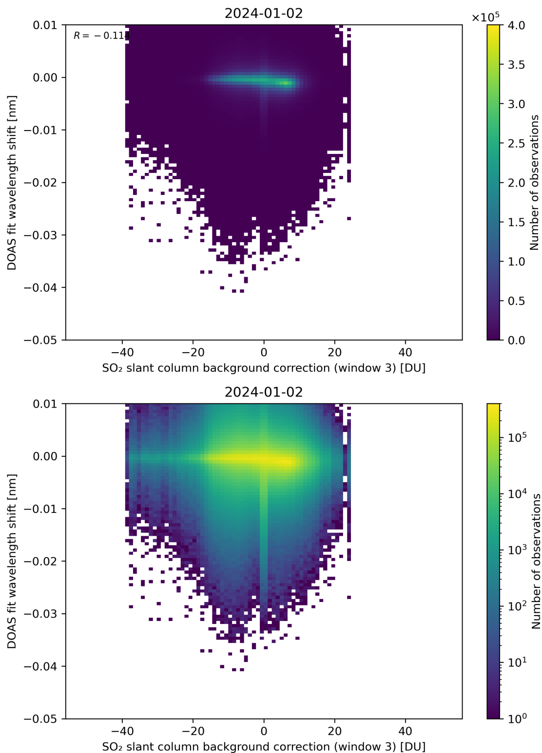
Figure 121: Scatter density plot of “SO 2 slant column background correction (window 3)” against “DOAS fit wavelength shift” for 2024-01-01 to 2024-01-03.
