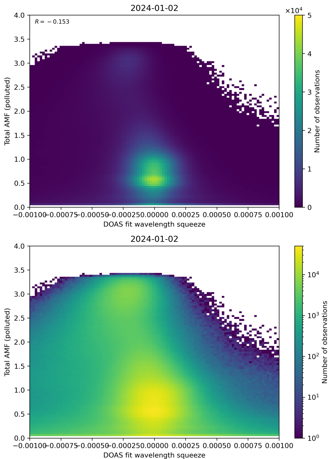
Figure 134: Scatter density plot of “DOAS fit wavelength squeeze” against “Total AMF (polluted)” for 2024-01-01 to 2024-01-03.
