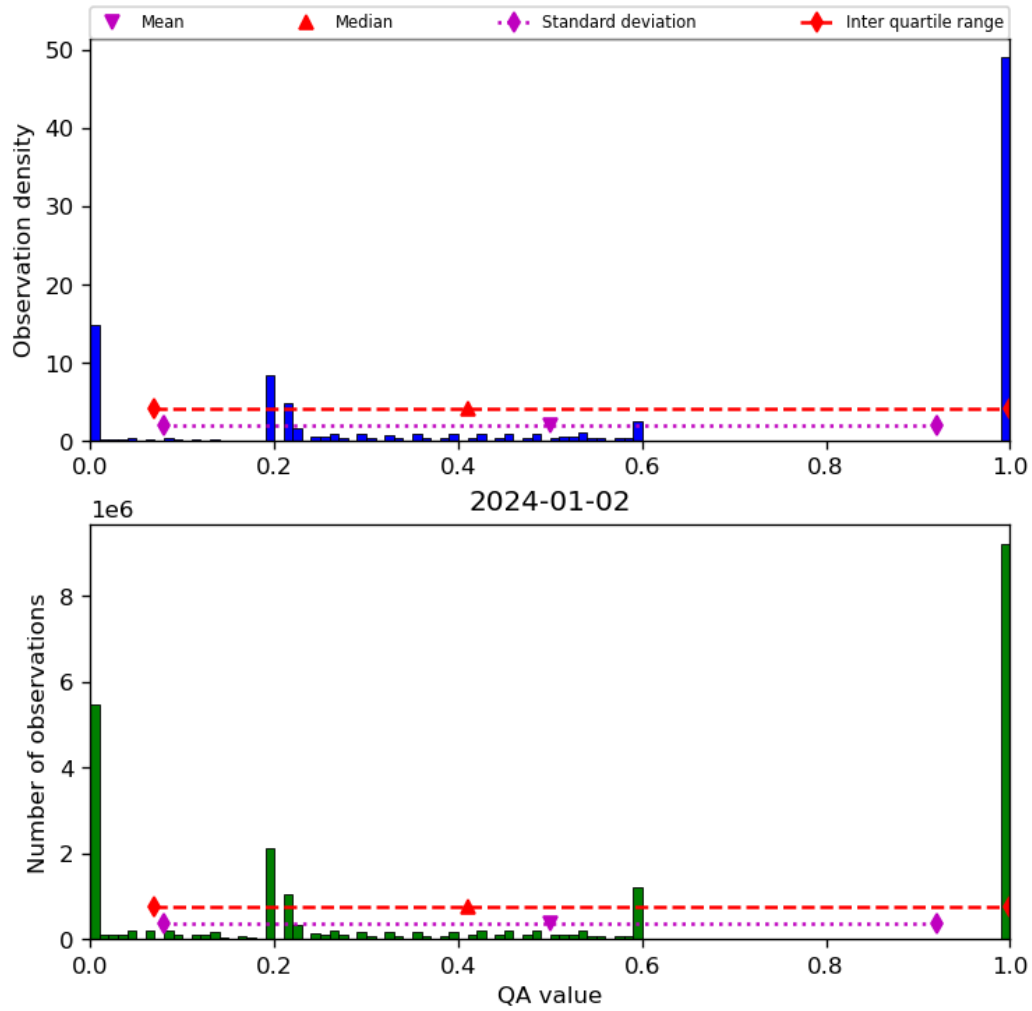
Figure 52: Histogram of “QA value” for 2024-01-01 to 2024-01-03
