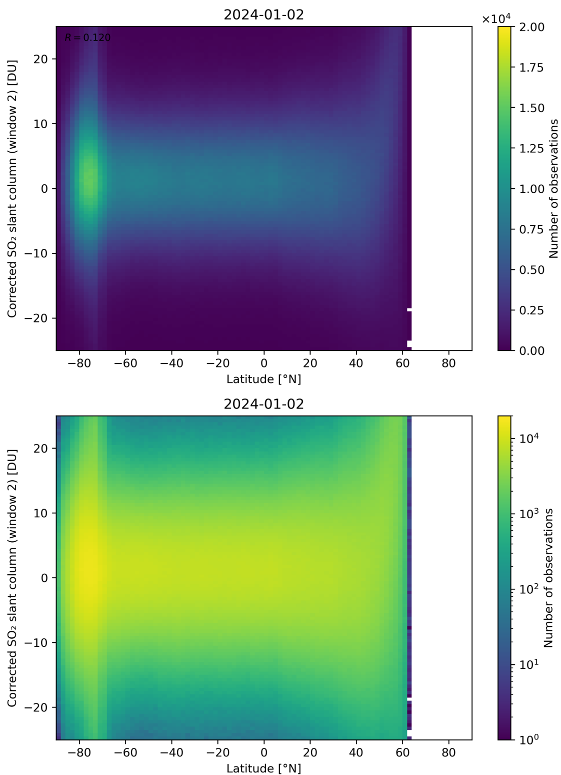
Figure 147: Scatter density plot of “Latitude” against “Corrected SO 2 slant column (window 2)” for 2024-01-01 to 2024-01-03.
