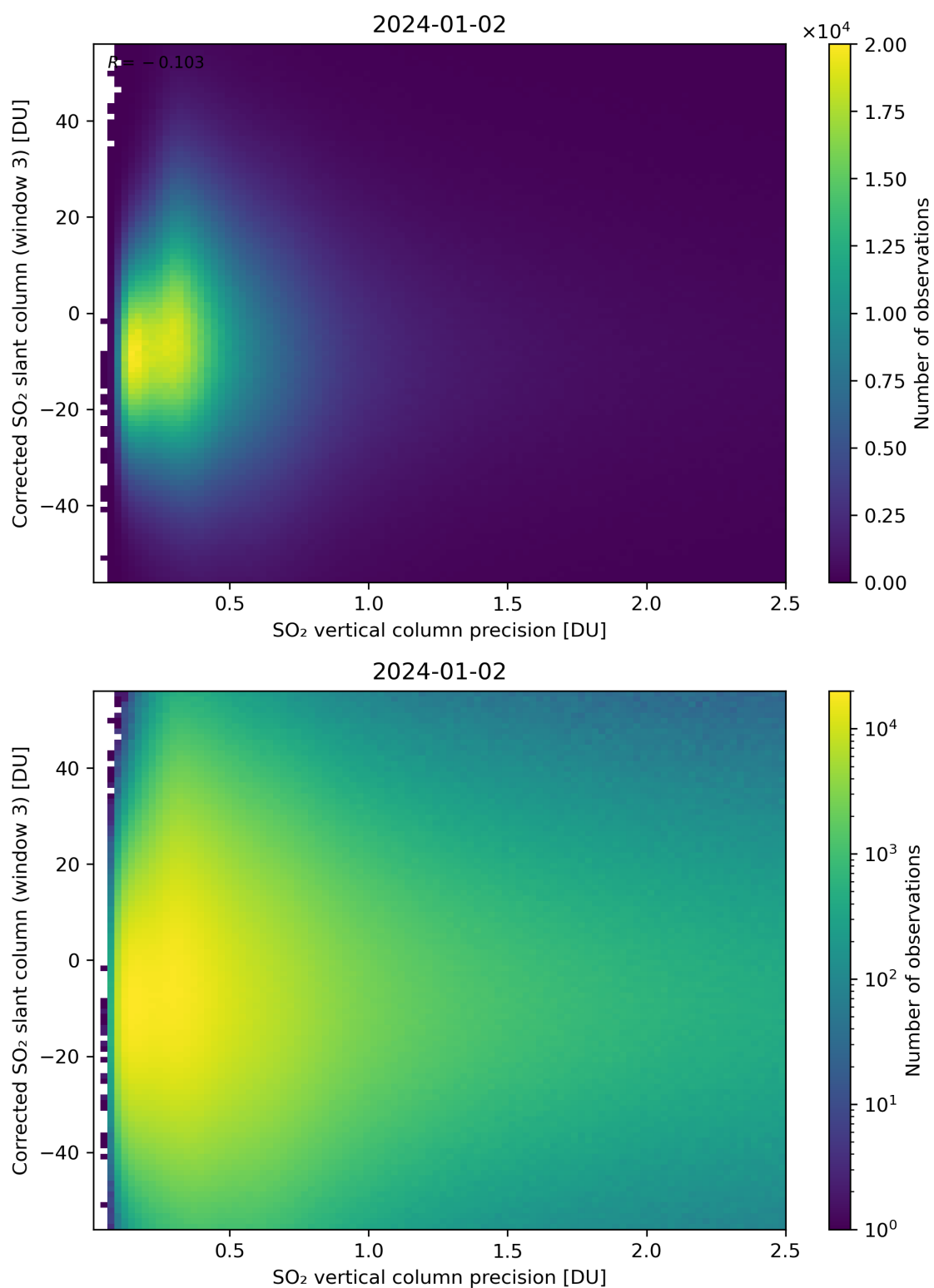
Figure 288: Scatter density plot of “SO 2 vertical column precision” against “Corrected SO 2 slant column (window 3)” for 2024-01-01 to 2024-01-03.
