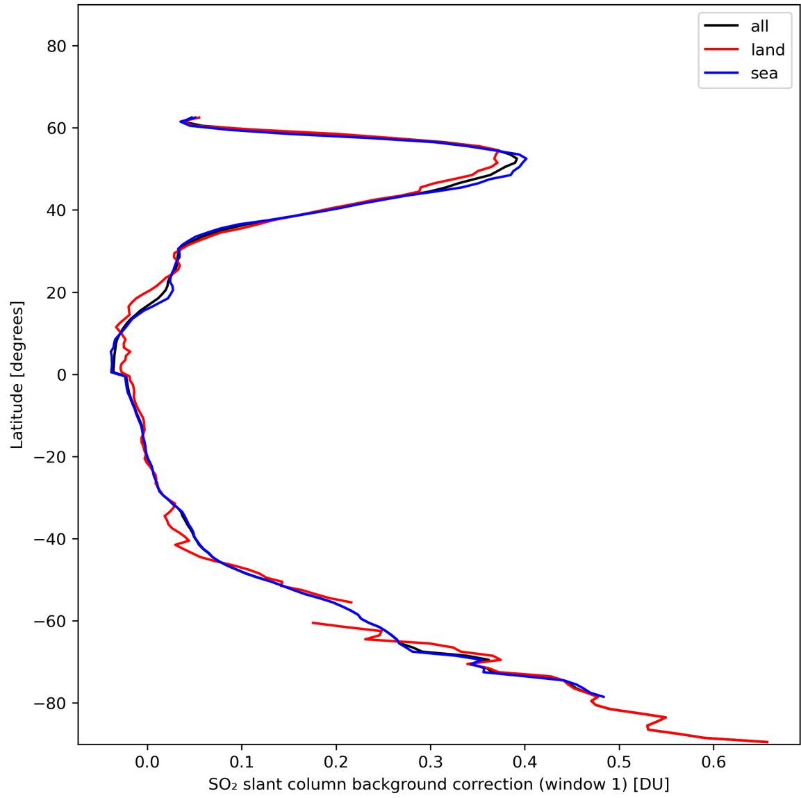
Figure 36: Zonal average of “SO 2 slant column background correction (window 1)” for 2024-01-01 to 2024-01-03.
