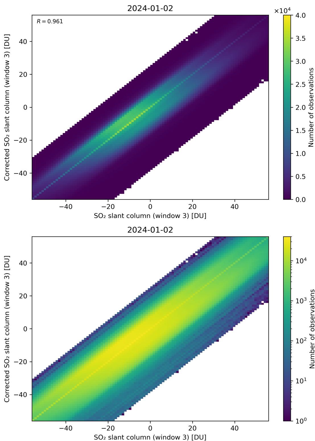
Figure 266: Scatter density plot of “SO 2 slant column (window 3)” against “Corrected SO 2 slant column (window 3)” for 2024-01-01 to 2024-01-03.
