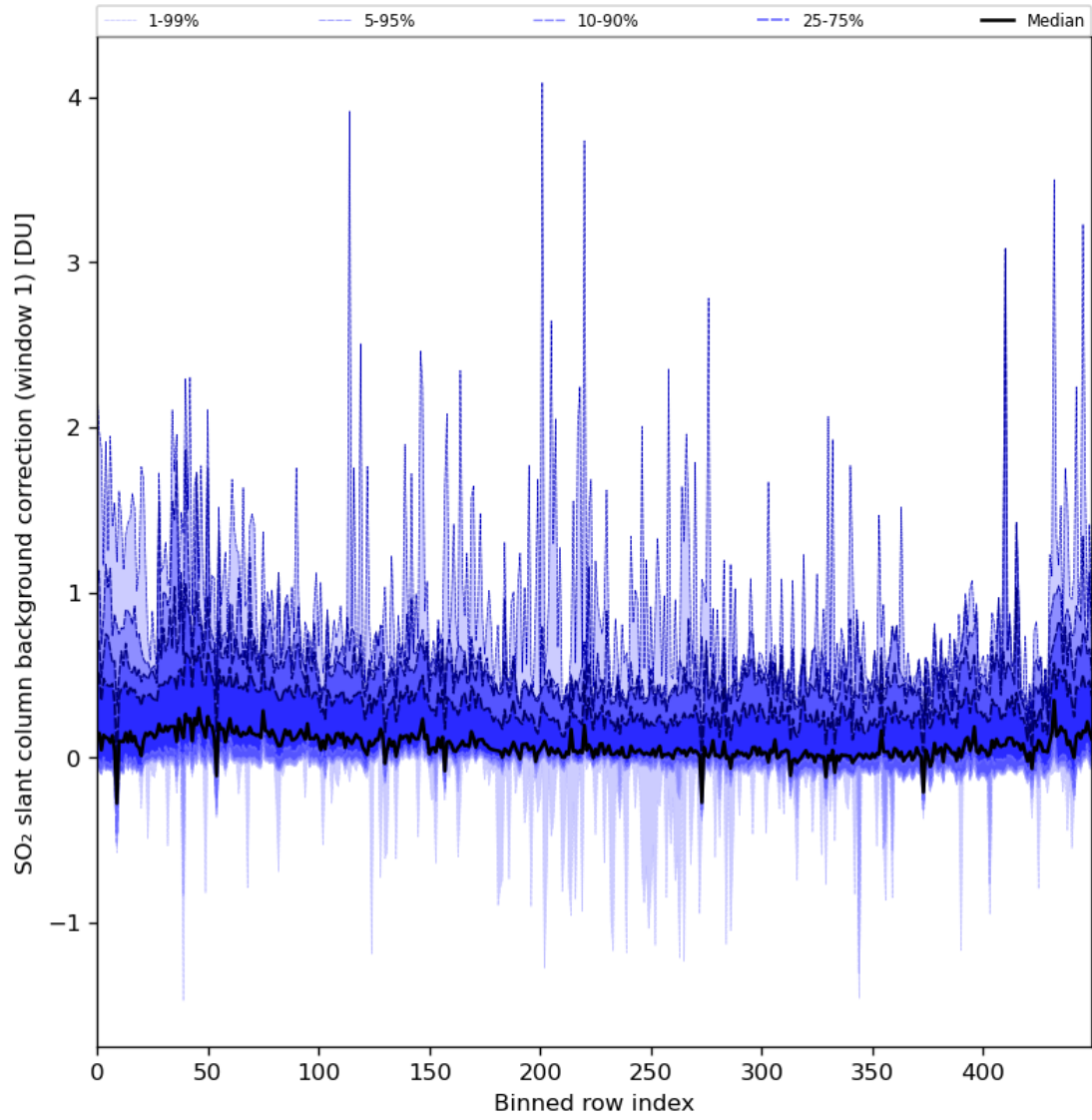
Figure 82: Along track statistics of “SO 2 slant column background correction (window 1)” for 2024-01-01 to 2024-01-03
