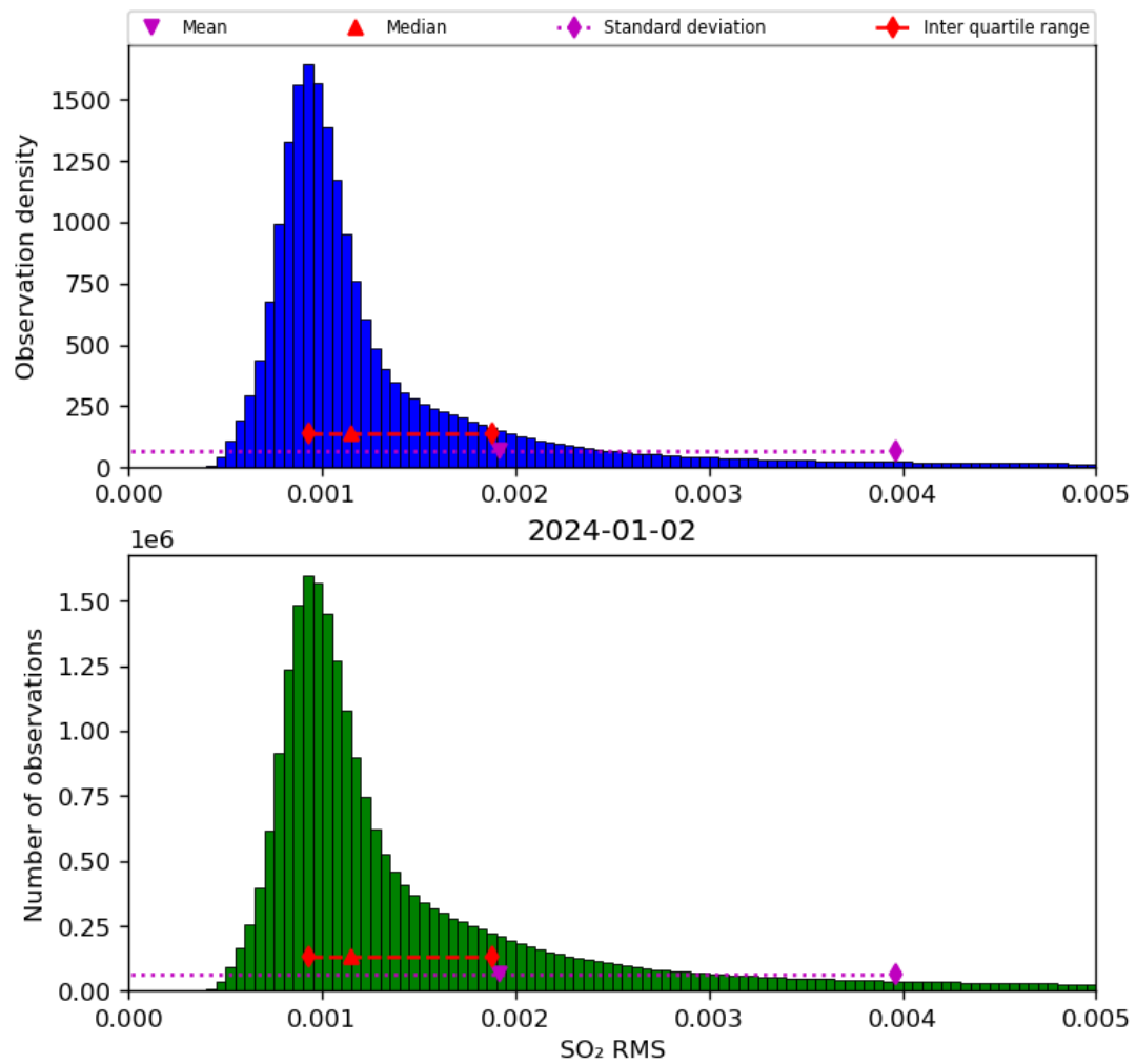
Figure 70: Histogram of “SO 2 RMS” for 2024-01-01 to 2024-01-03
