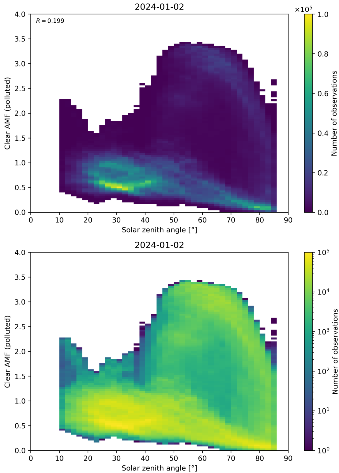
Figure 165: Scatter density plot of “Solar zenith angle” against “Clear AMF (polluted)” for 2024-01-01 to 2024-01-03.
