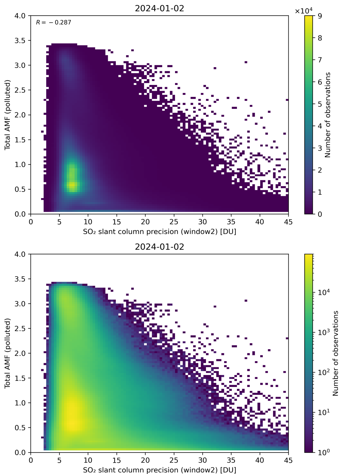
Figure 251: Scatter density plot of “SO 2 slant column precision (window2)” against “Total AMF (polluted)” for 2024-01-01 to 2024-01-03.
