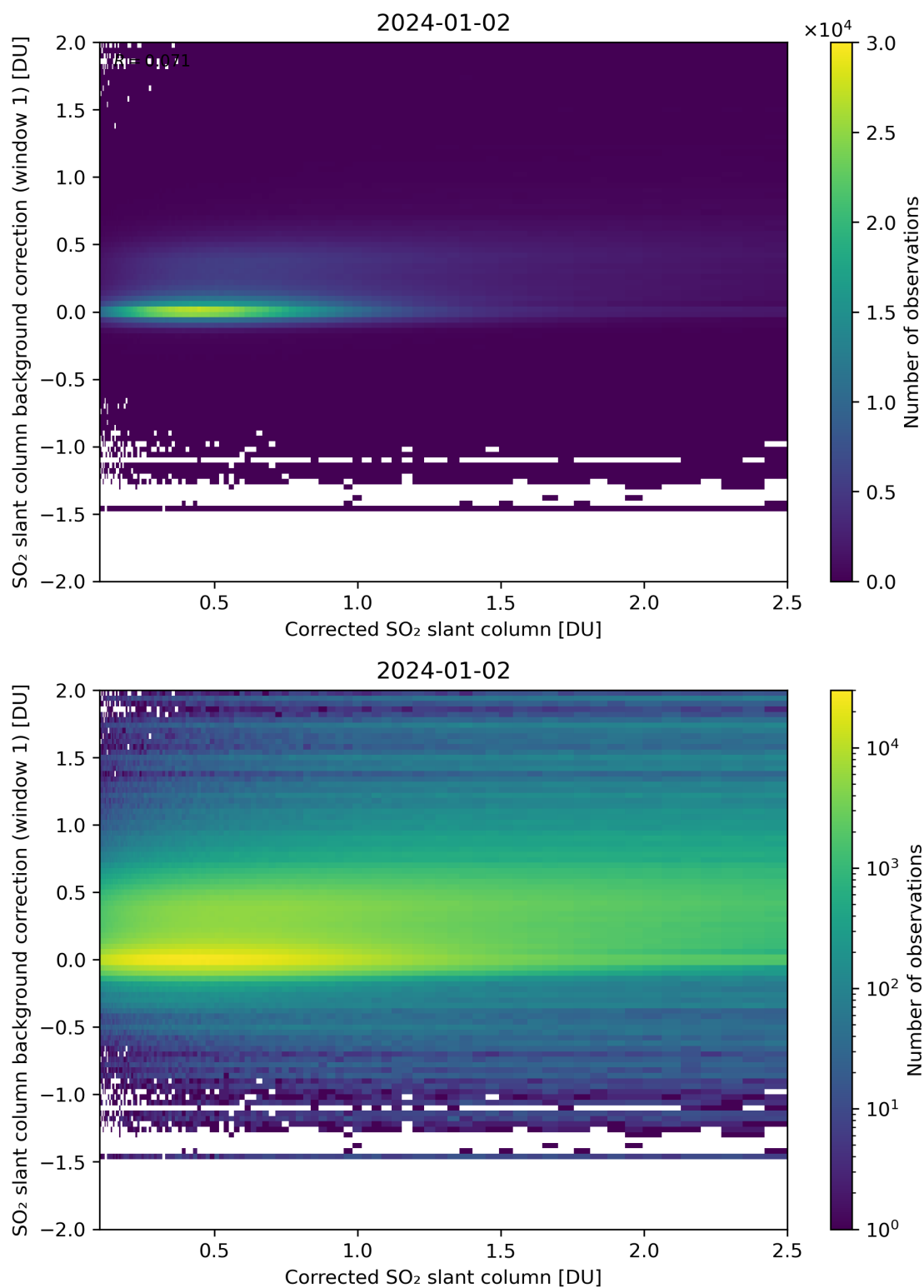
Figure 178: Scatter density plot of “Corrected SO 2 slant column” against “SO 2 slant column background correction (window 1)” for 2024-01-01 to 2024-01-03.
