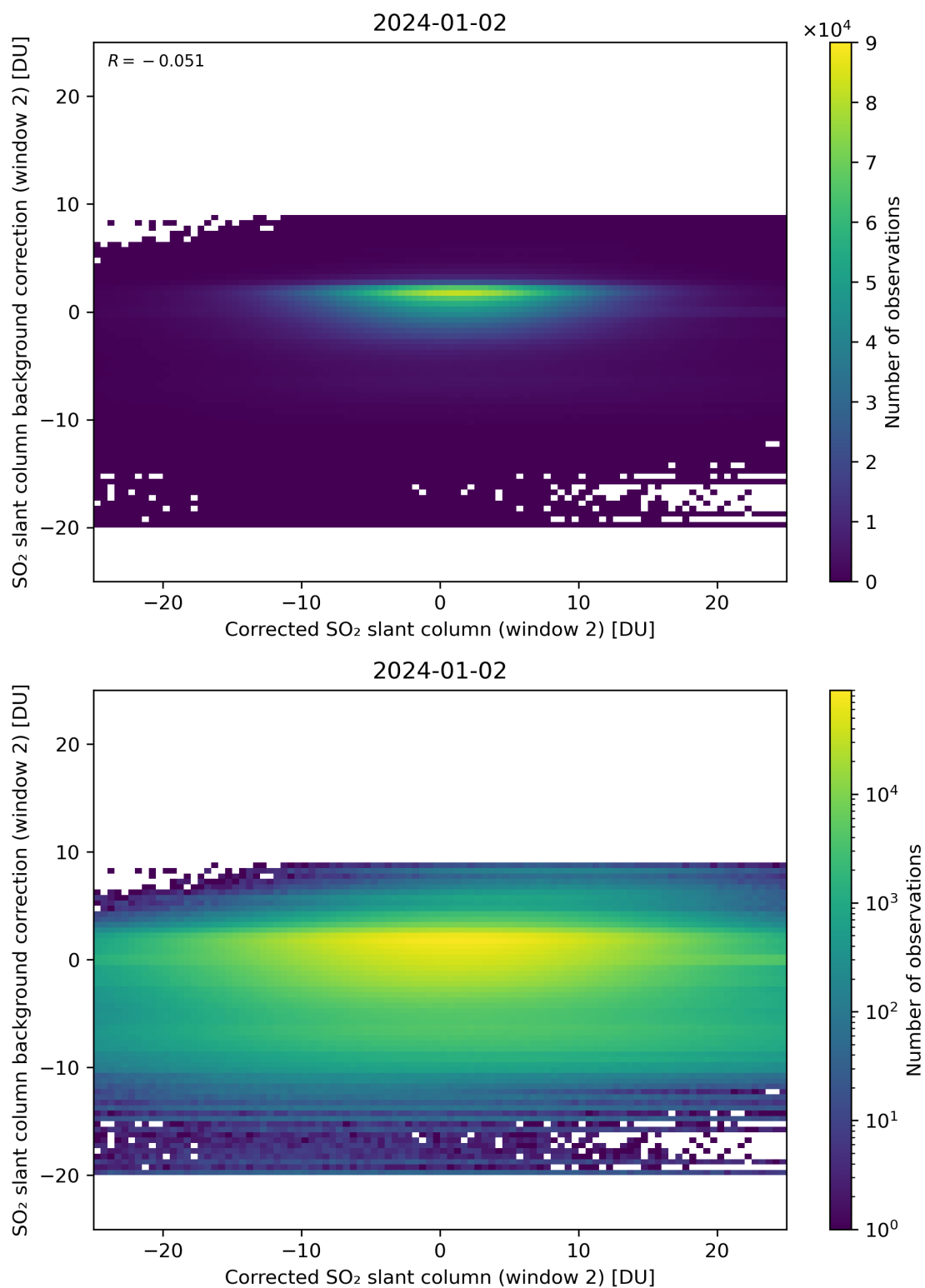
Figure 194: Scatter density plot of “Corrected SO 2 slant column (window 2)” against “SO 2 slant column background correction (window 2)” for 2024-01-01 to 2024-01-03.
