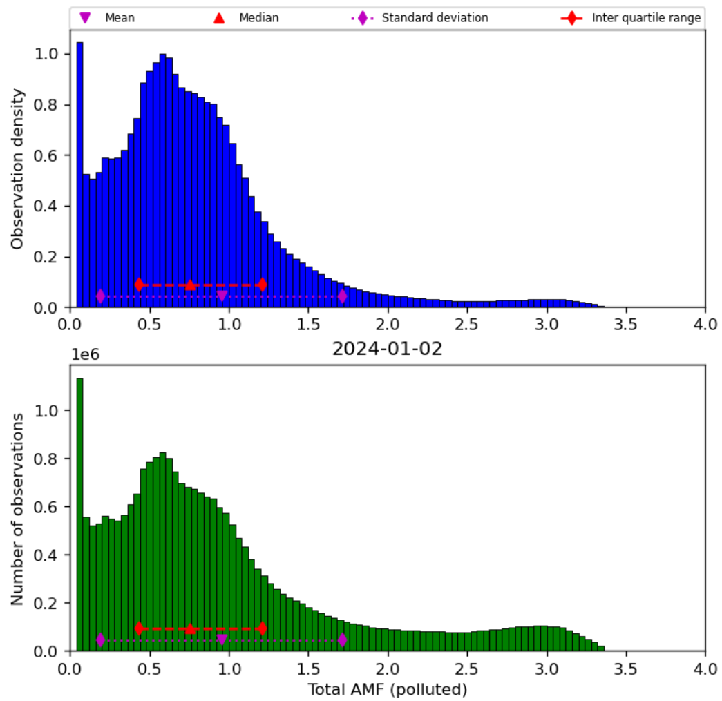
Figure 71: Histogram of “Total AMF (polluted)” for 2024-01-01 to 2024-01-03
