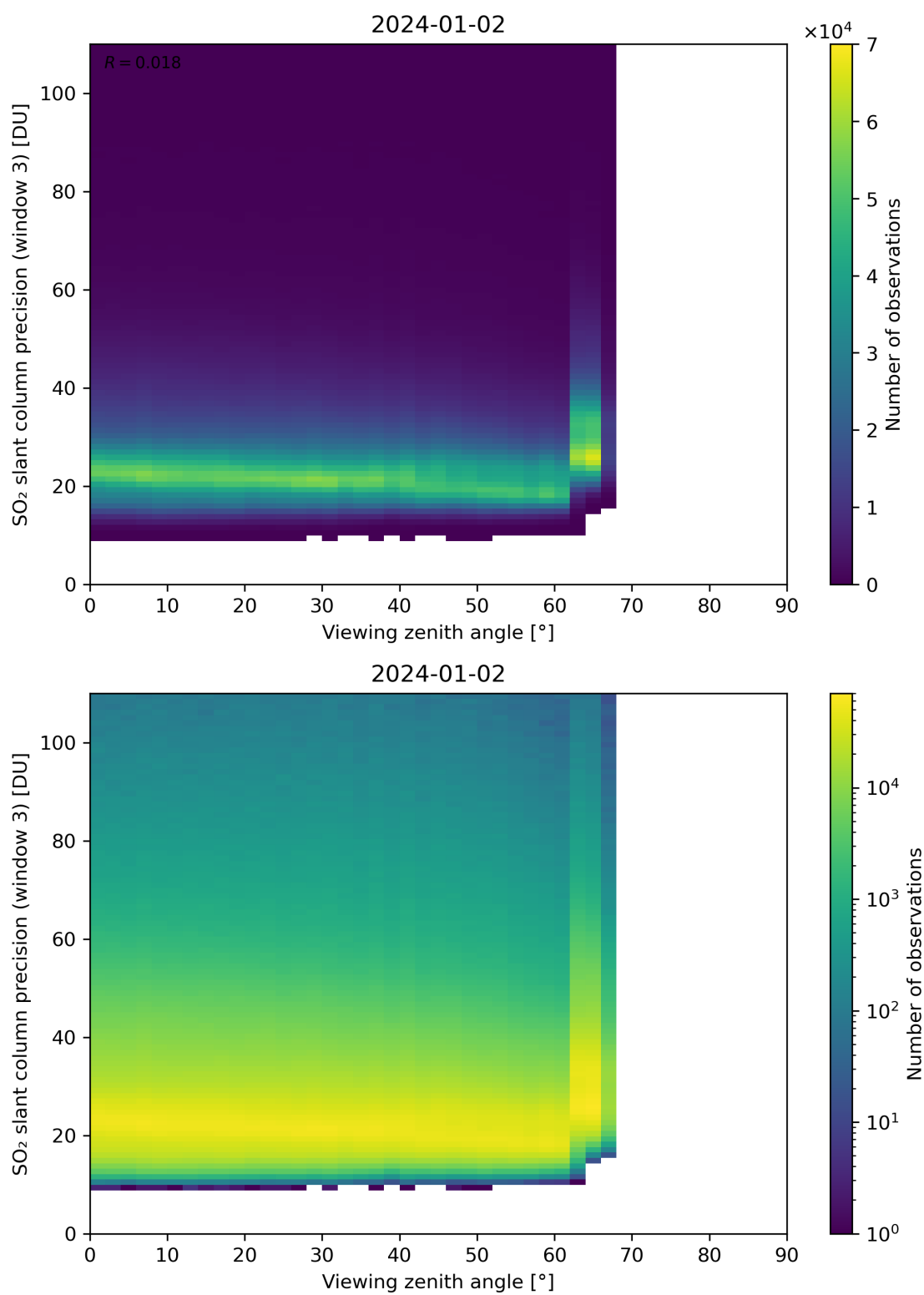
Figure 324: Scatter density plot of “Viewing zenith angle” against “SO 2 slant column precision (window 3)” for 2024-01-01 to 2024-01-03.
