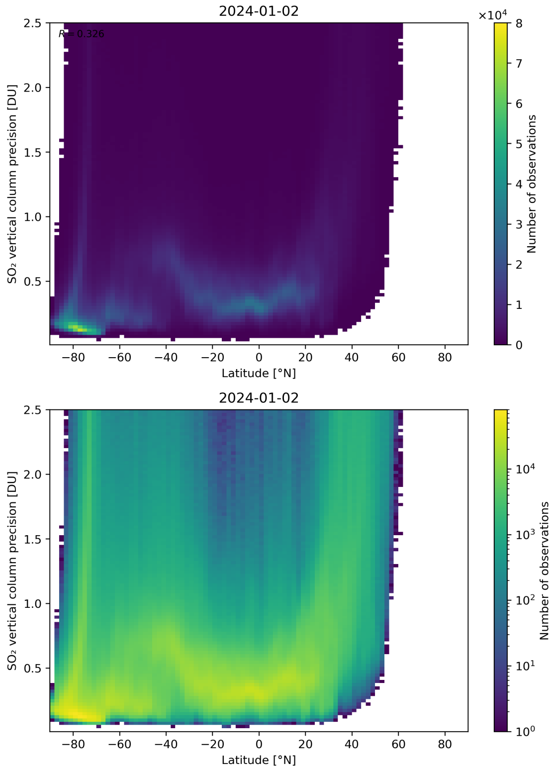
Figure 157: Scatter density plot of “Latitude” against “SO 2 vertical column precision” for 2024-01-01 to 2024-01-03.
