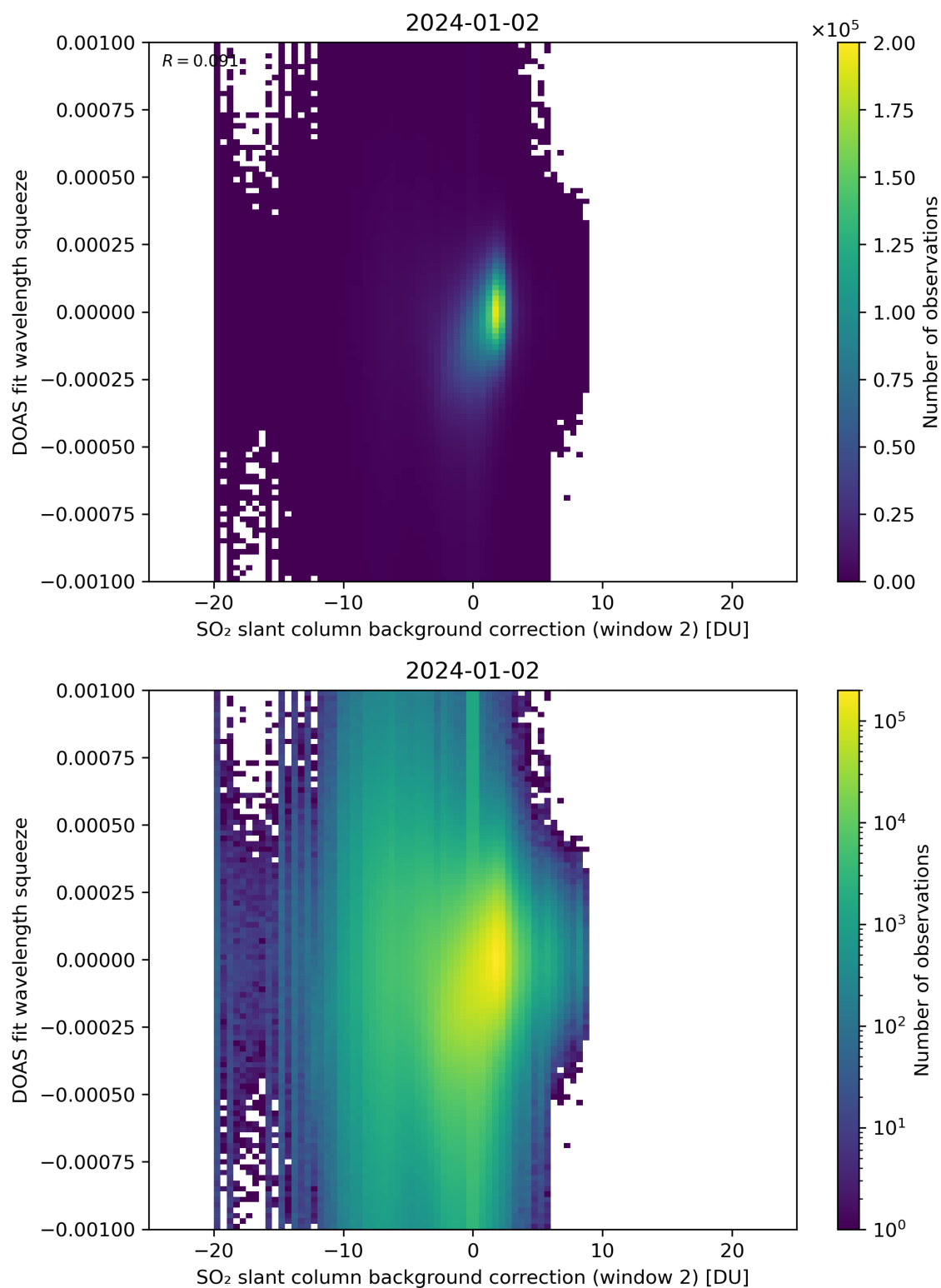
Figure 113: Scatter density plot of “SO 2 slant column background correction (window 2)” against “DOAS fit wavelength squeeze” for 2024-01-01 to 2024-01-03.
