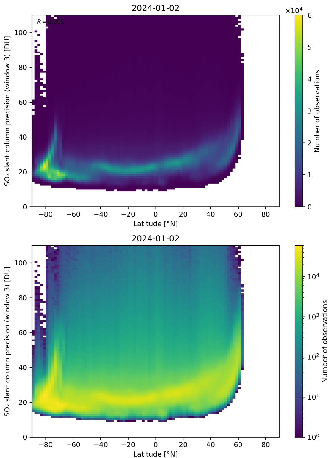
Figure 153: Scatter density plot of “Latitude” against “SO 2 slant column precision (window 3)” for 2024-01-01 to 2024-01-03.
