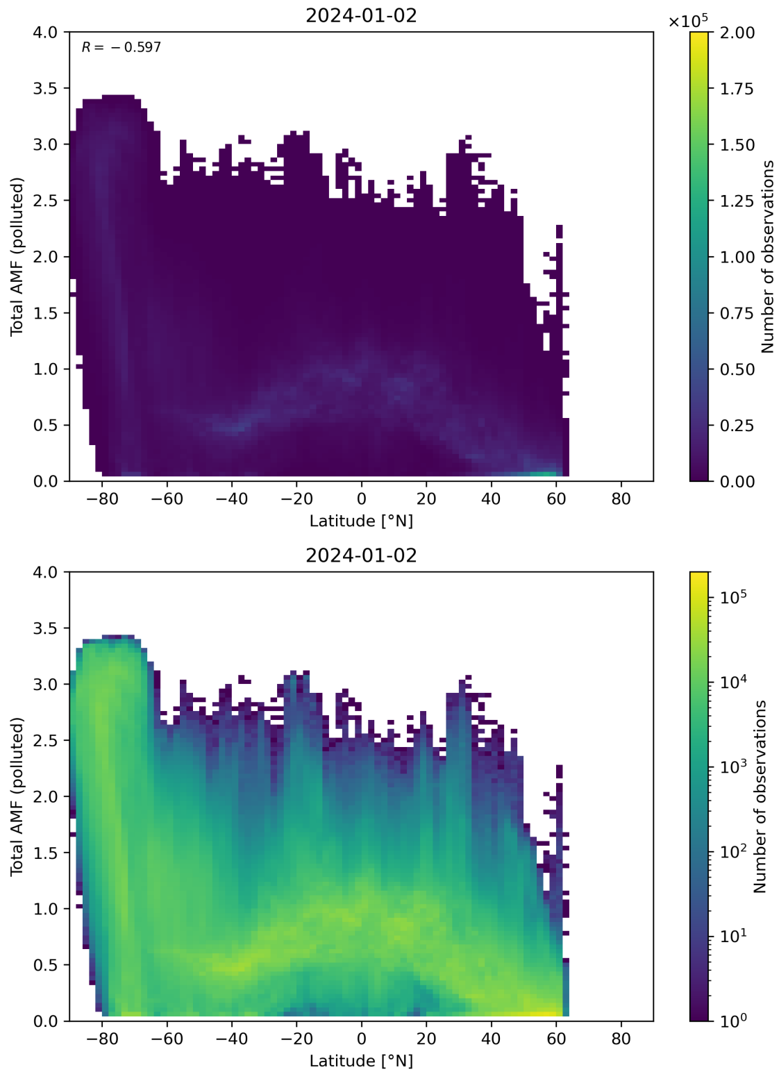
Figure 154: Scatter density plot of “Latitude” against “Total AMF (polluted)” for 2024-01-01 to 2024-01-03.
