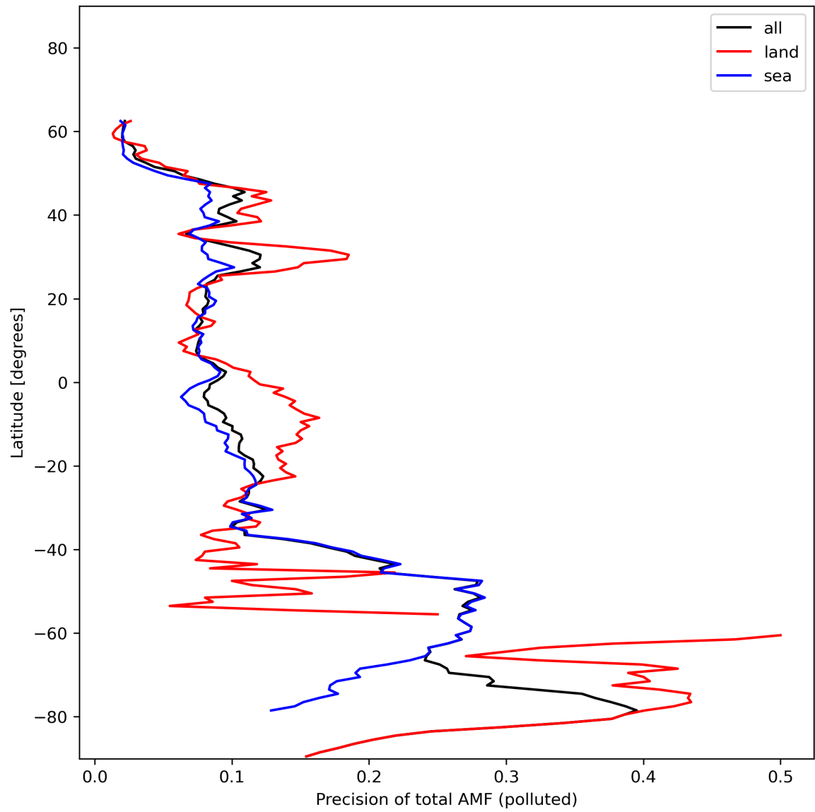
Figure 49: Zonal average of “Precision of total AMF (polluted)” for 2024-01-01 to 2024-01-03.
