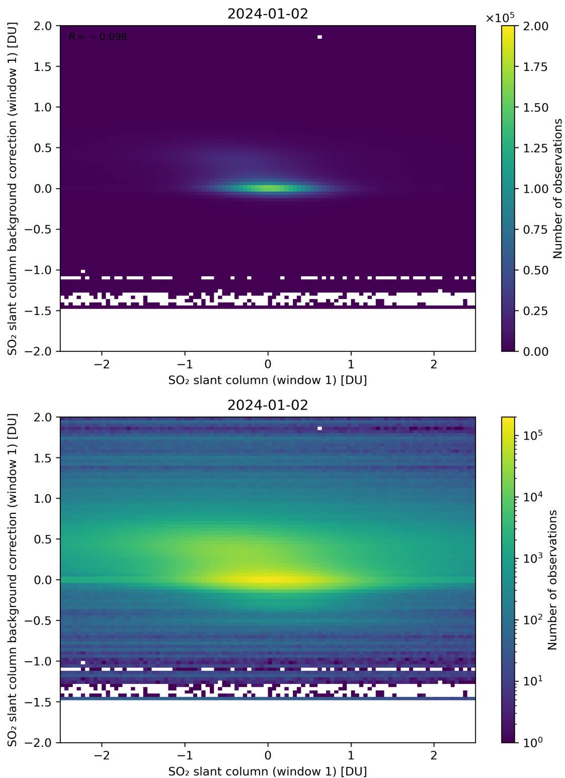
Figure 212: Scatter density plot of “SO 2 slant column (window 1)” against “SO 2 slant column background correction (window 1)” for 2024-01-01 to 2024-01-03.
