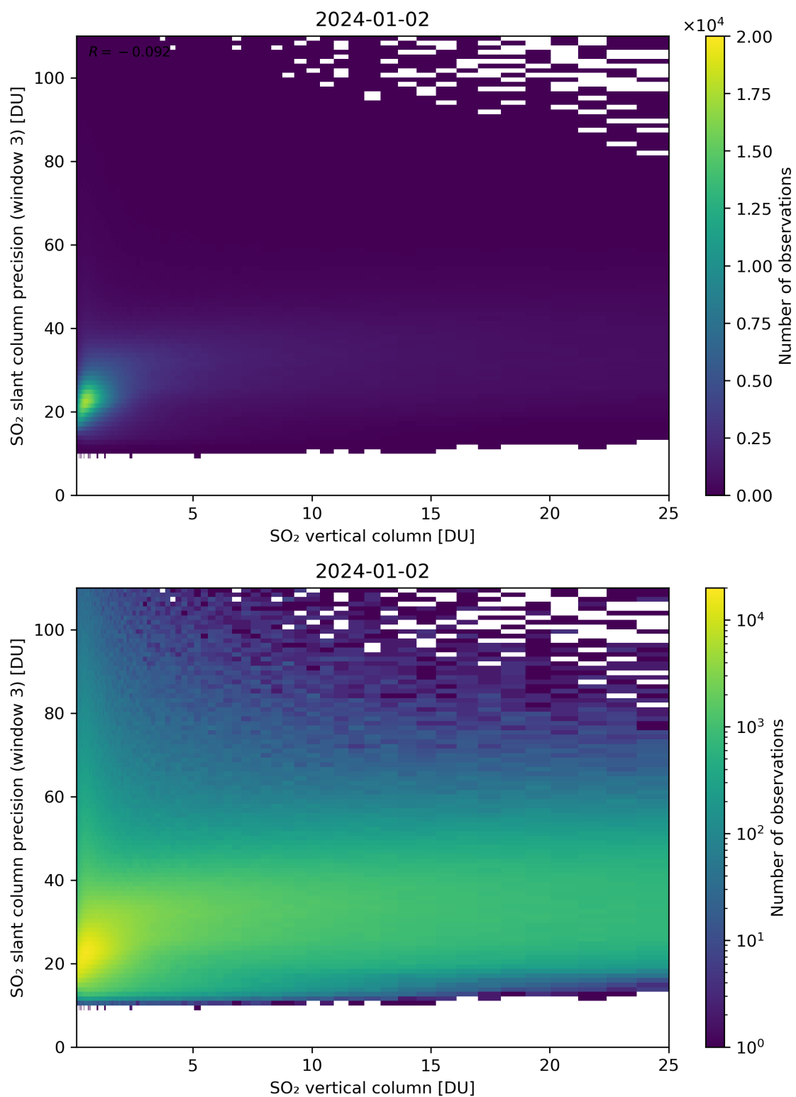
Figure 304: Scatter density plot of “SO 2 vertical column” against “SO 2 slant column precision (window 3)” for 2024-01-01 to 2024-01-03.
