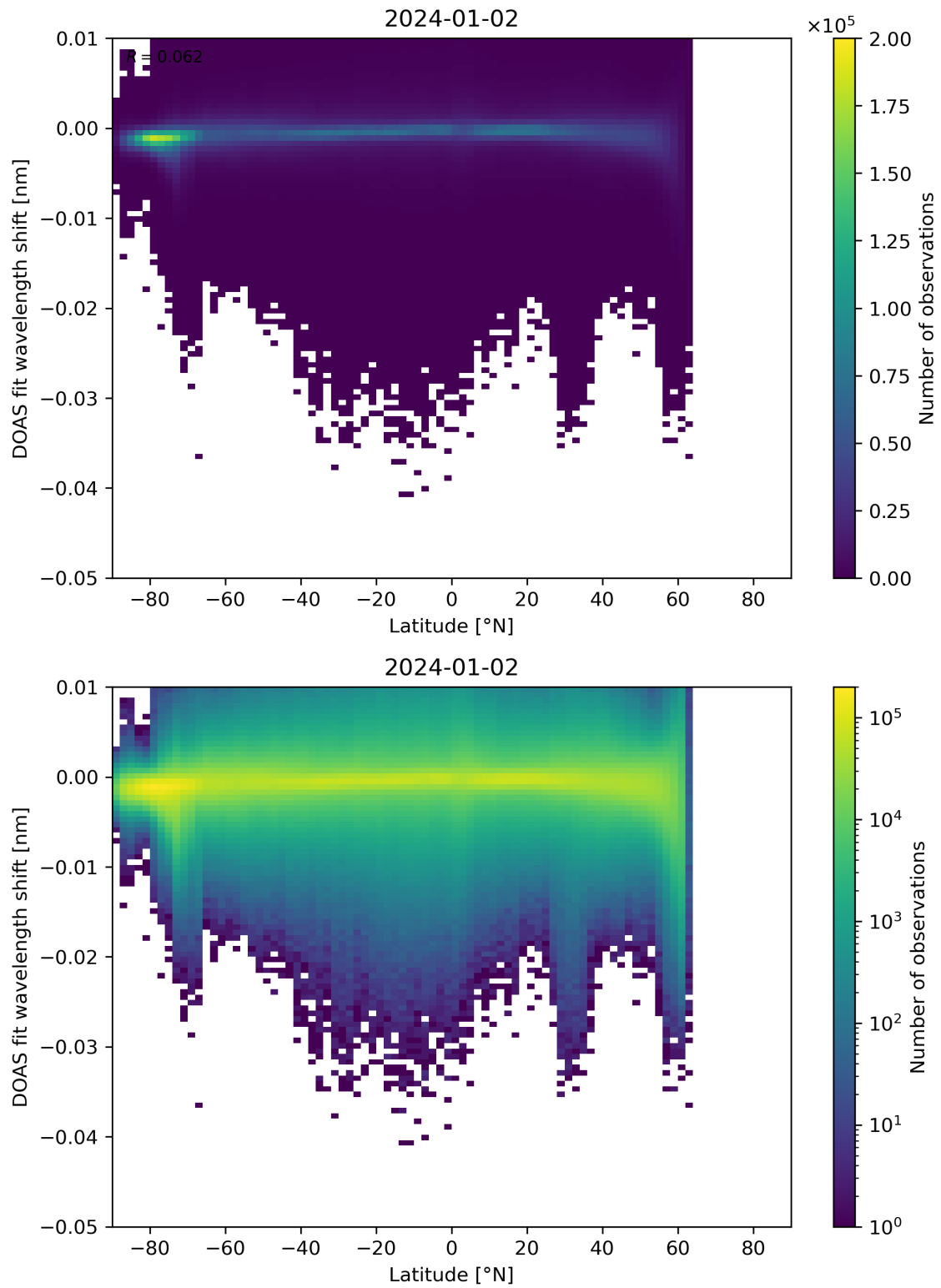
Figure 142: Scatter density plot of “Latitude” against “DOAS fit wavelength shift” for 2024-01-01 to 2024-01-03.
