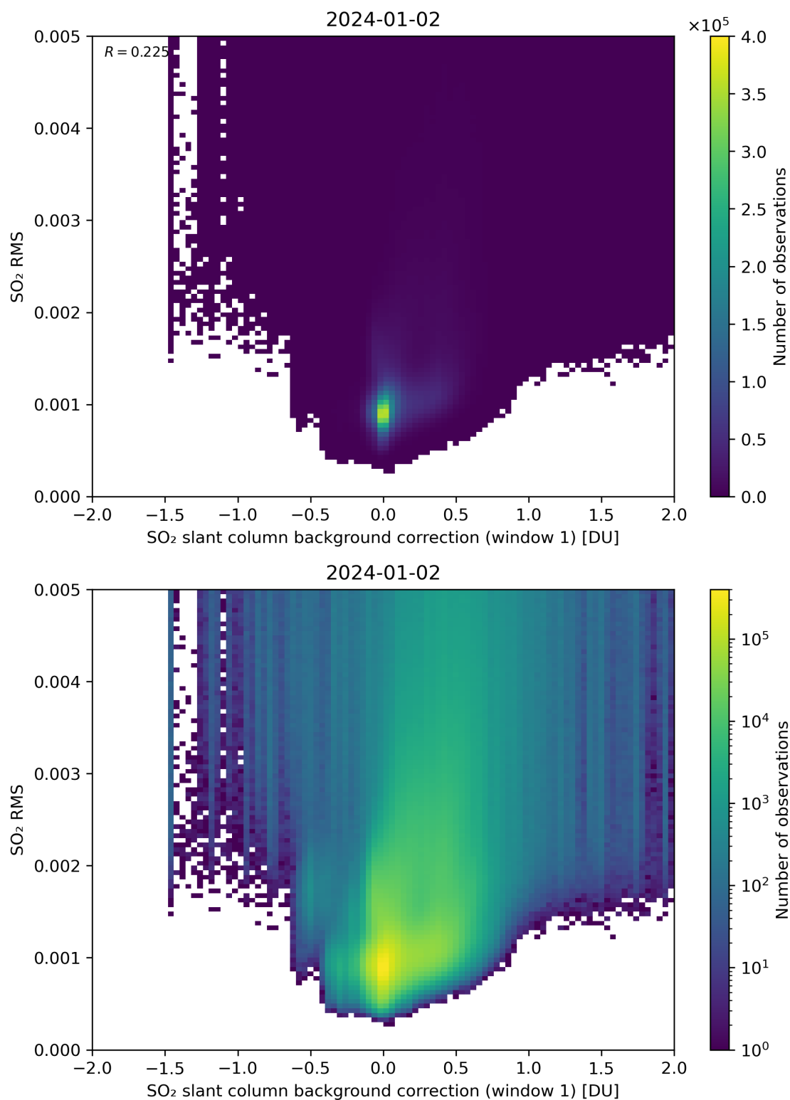
Figure 102: Scatter density plot of “SO 2 slant column background correction (window 1)” against “SO 2 RMS” for 2024-01-01 to 2024-01-03.
