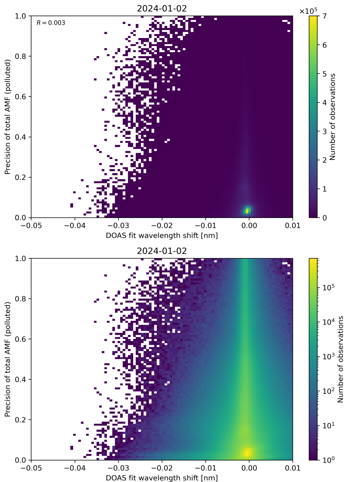
Figure 131: Scatter density plot of “DOAS fit wavelength shift” against “Precision of total AMF (polluted)” for 2024-01-01 to 2024-01-03.
