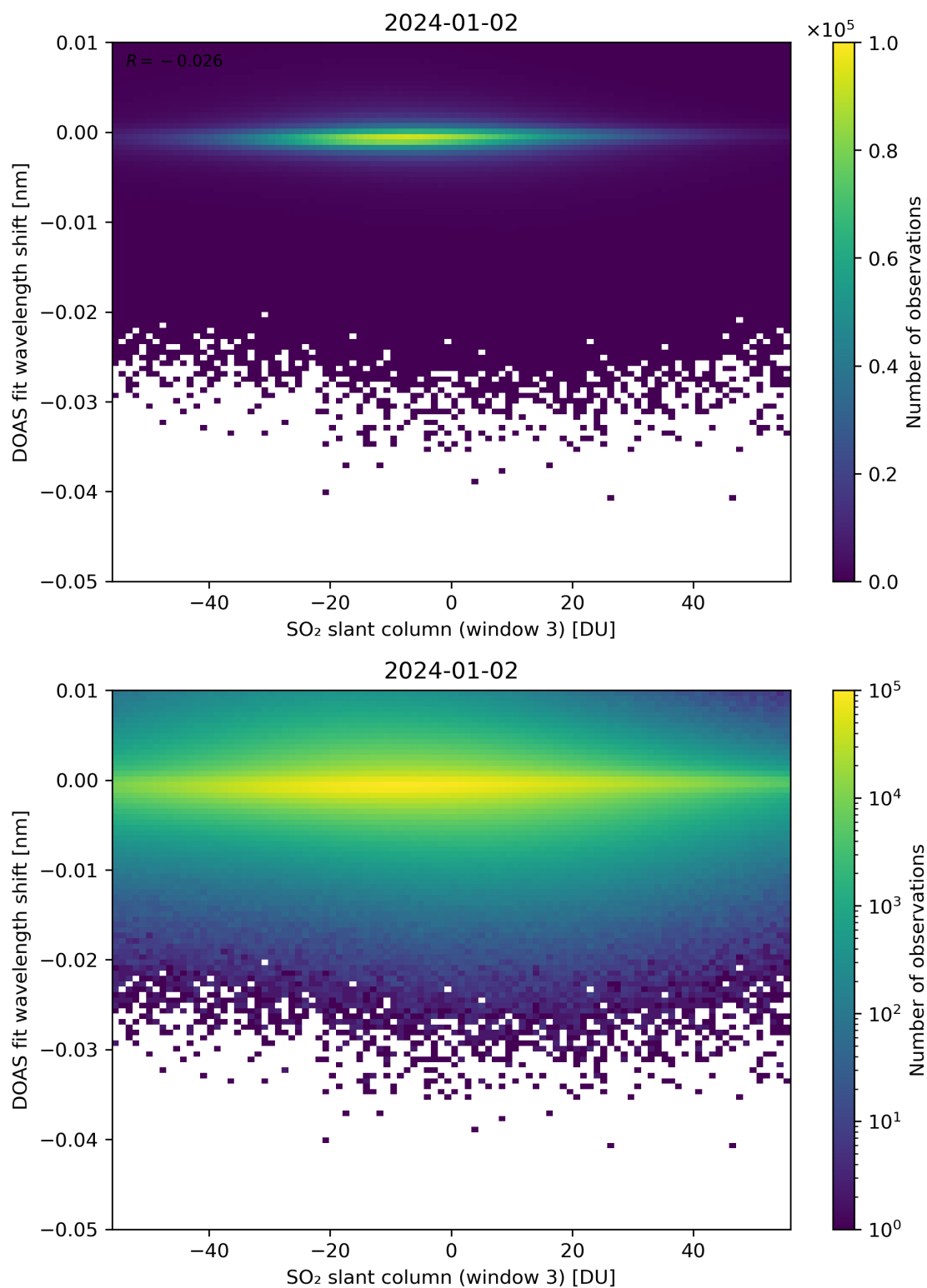
Figure 254: Scatter density plot of “SO 2 slant column (window 3)” against “DOAS fit wavelength shift” for 2024-01-01 to 2024-01-03.
