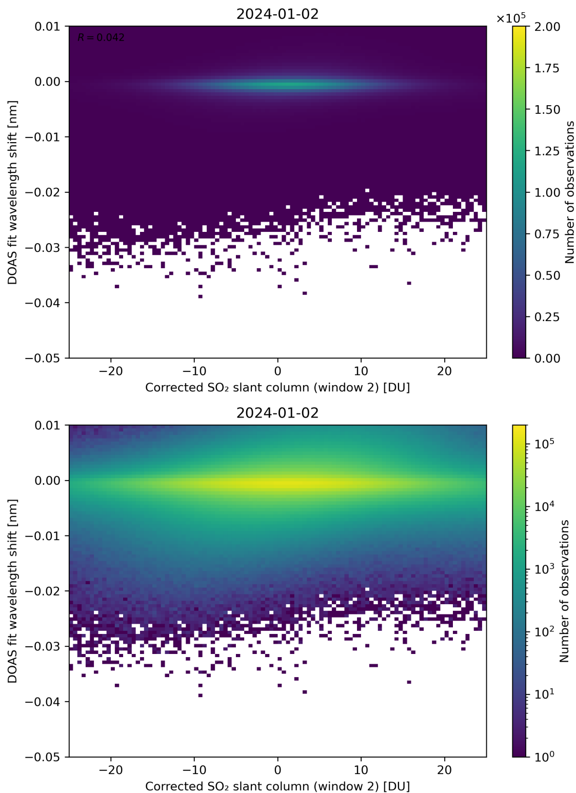
Figure 196: Scatter density plot of “Corrected SO 2 slant column (window 2)” against “DOAS fit wavelength shift” for 2024-01-01 to 2024-01-03.
