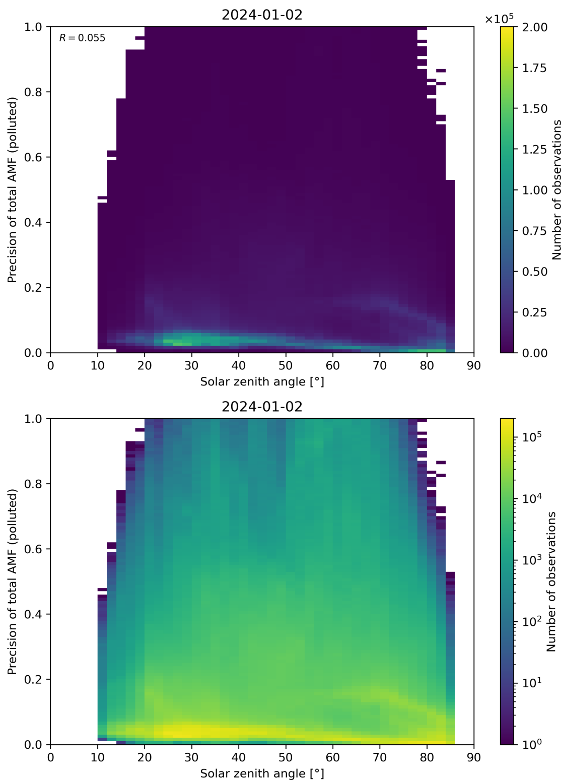
Figure 175: Scatter density plot of “Solar zenith angle” against “Precision of total AMF (polluted)” for 2024-01-01 to 2024-01-03.
