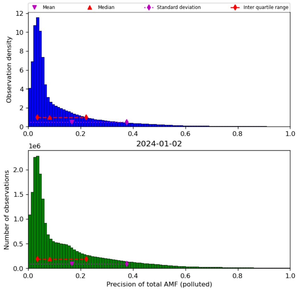
Figure 72: Histogram of “Precision of total AMF (polluted)” for 2024-01-01 to 2024-01-03
