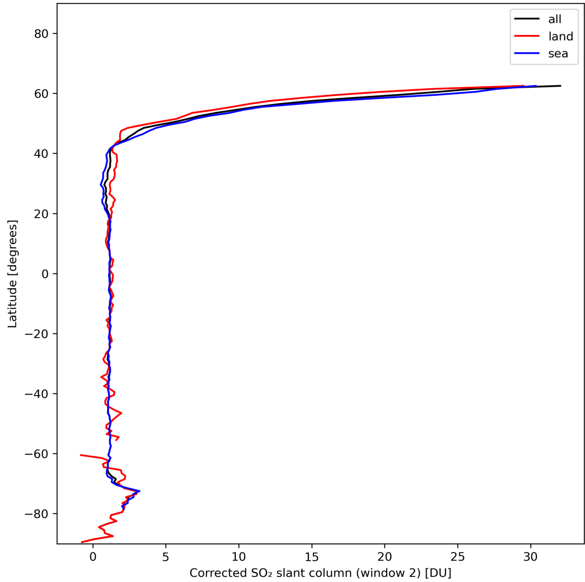
Figure 39: Zonal average of “Corrected SO 2 slant column (window 2)” for 2024-01-01 to 2024-01-03.
