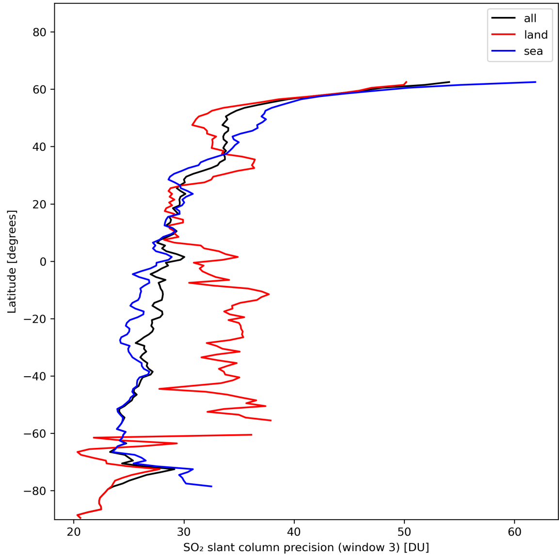
Figure 42: Zonal average of “SO 2 slant column precision (window 3)” for 2024-01-01 to 2024-01-03.
