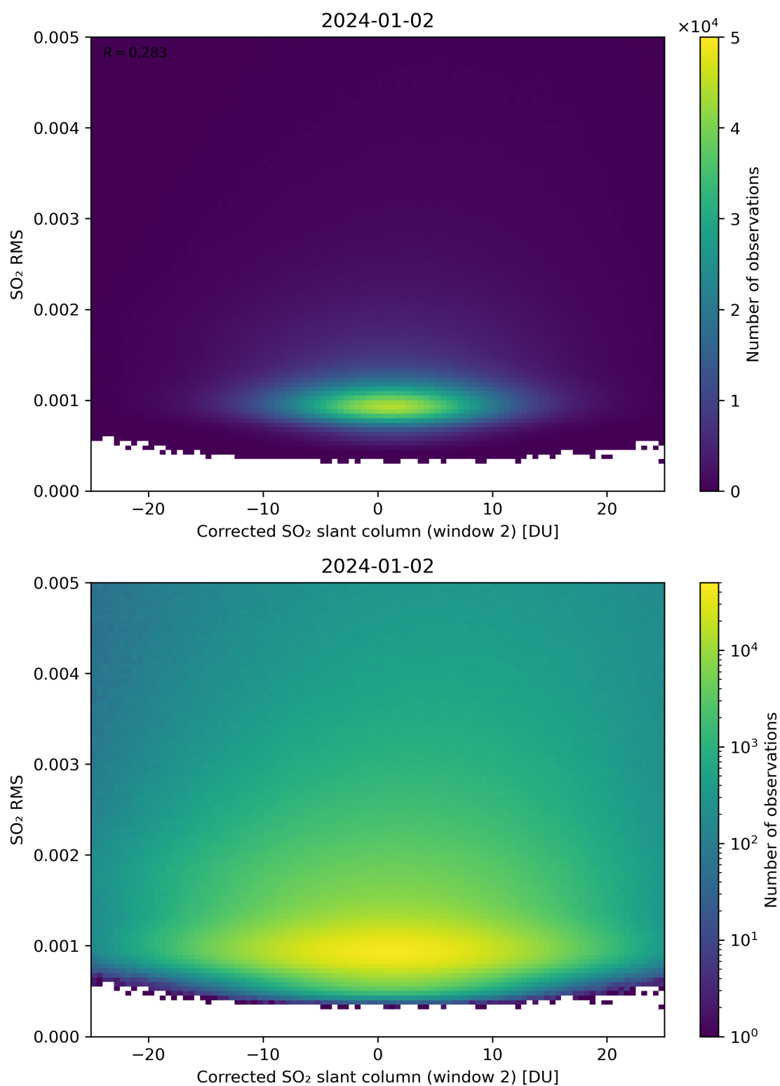
Figure 198: Scatter density plot of “Corrected SO 2 slant column (window 2)” against “SO 2 RMS” for 2024-01-01 to 2024-01-03.
