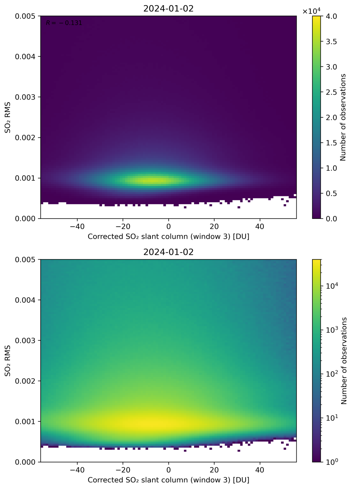
Figure 208: Scatter density plot of “Corrected SO 2 slant column (window 3)” against “SO 2 RMS” for 2024-01-01 to 2024-01-03.
