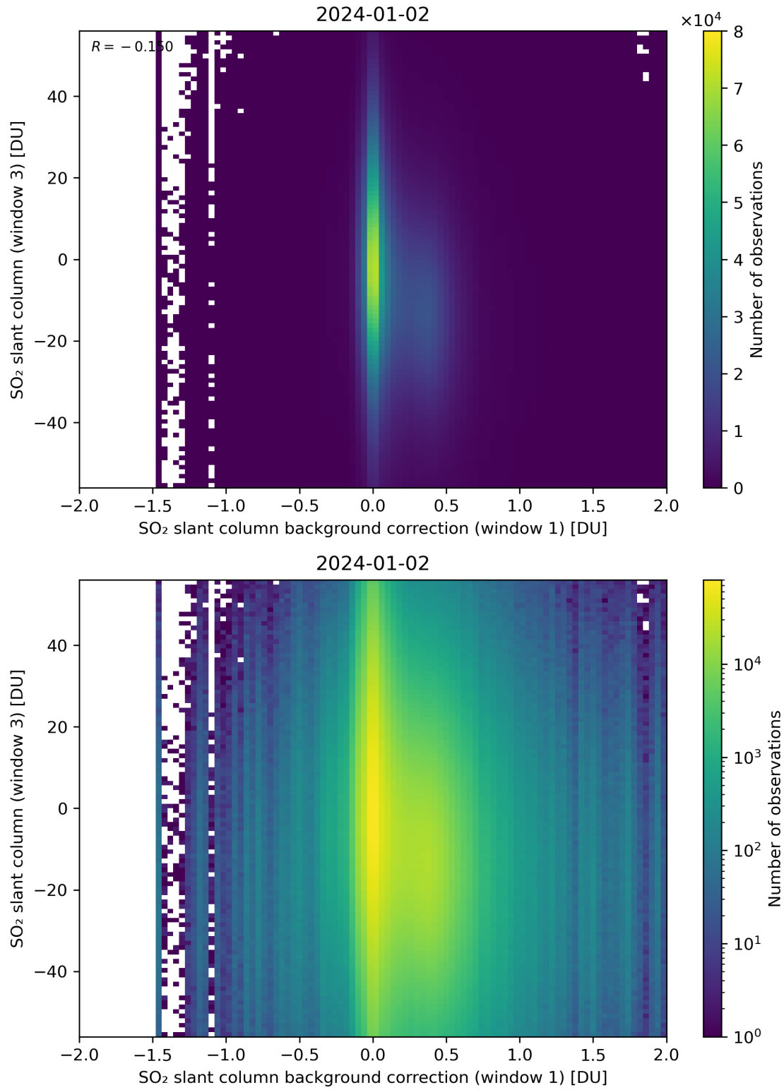
Figure 107: Scatter density plot of “SO 2 slant column background correction (window 1)” against “SO 2 slant column (window 3)” for 2024-01-01 to 2024-01-03.
