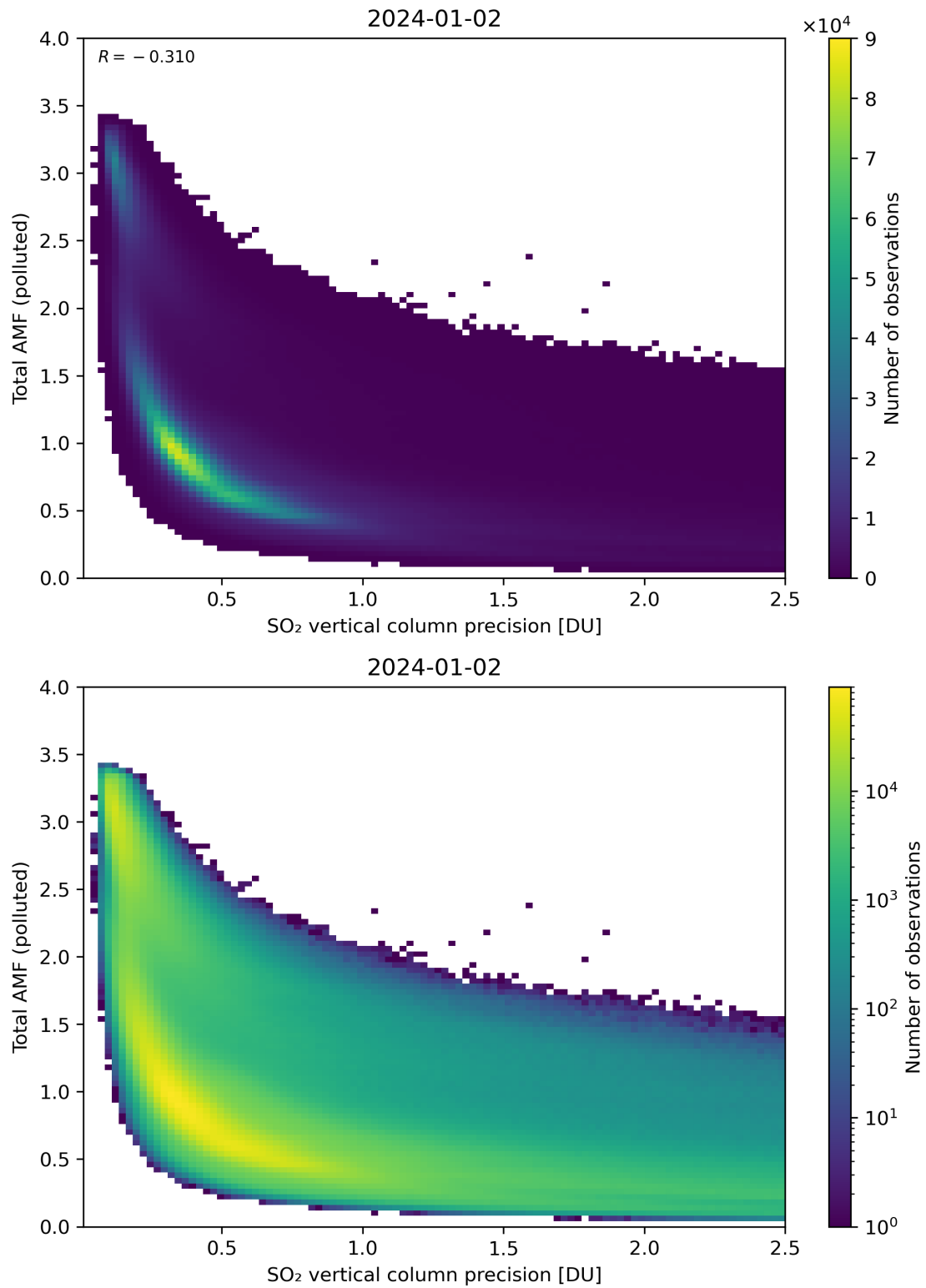
Figure 294: Scatter density plot of “SO 2 vertical column precision” against “Total AMF (polluted)” for 2024-01-01 to 2024-01-03.
