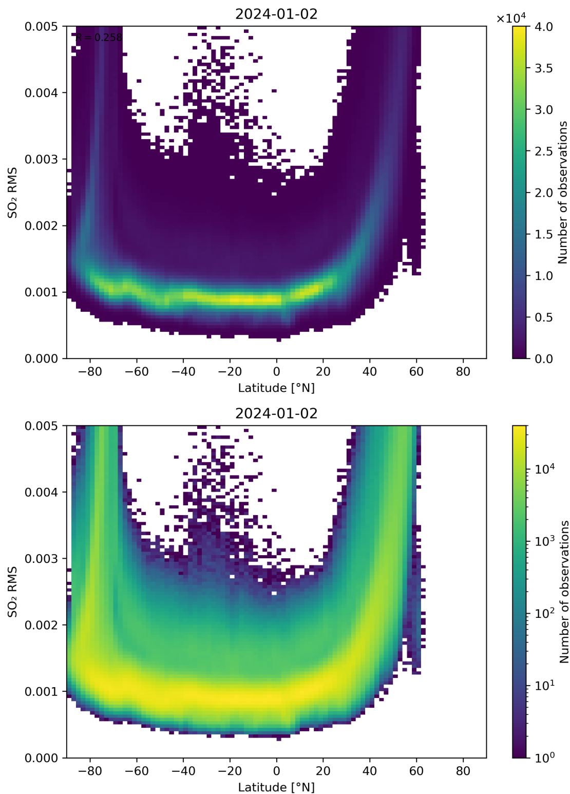
Figure 144: Scatter density plot of “Latitude” against “SO 2 RMS” for 2024-01-01 to 2024-01-03.
