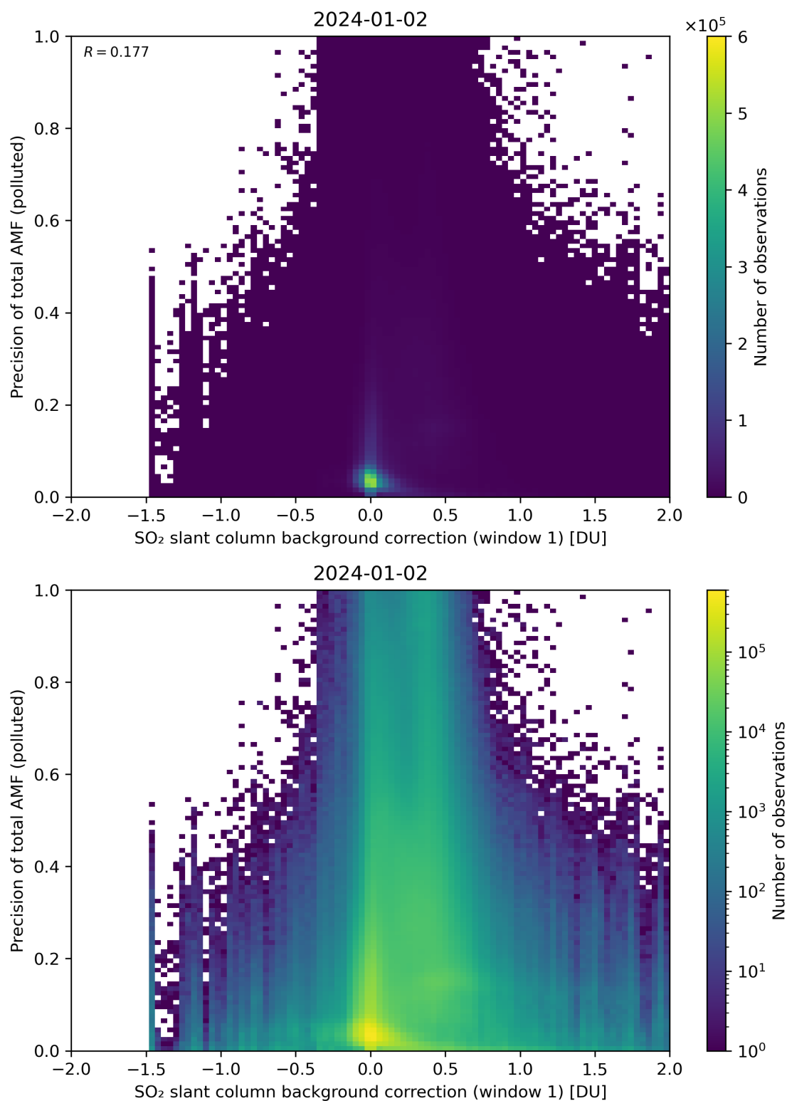
Figure 110: Scatter density plot of “SO 2 slant column background correction (window 1)” against “Precision of total AMF (polluted)” for 2024-01-01 to 2024-01-03.
