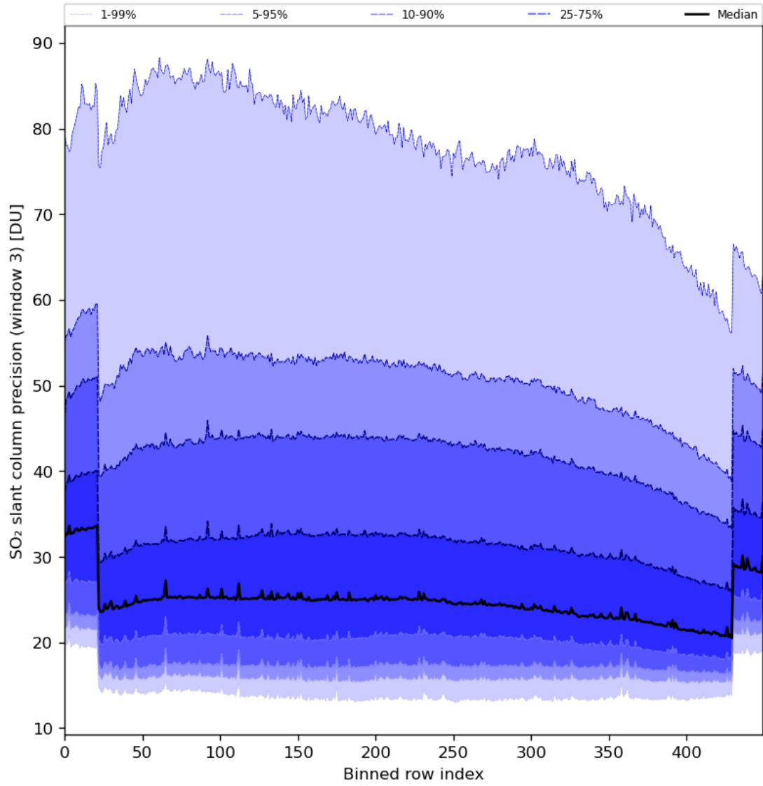
Figure 88: Along track statistics of “SO 2 slant column precision (window 3)” for 2024-01-01 to 2024-01-03
