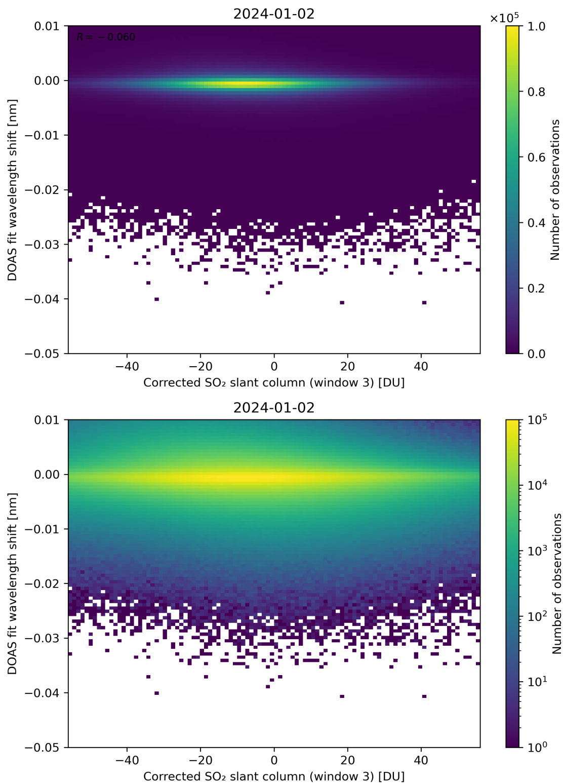
Figure 206: Scatter density plot of “Corrected SO 2 slant column (window 3)” against “DOAS fit wavelength shift” for 2024-01-01 to 2024-01-03.
