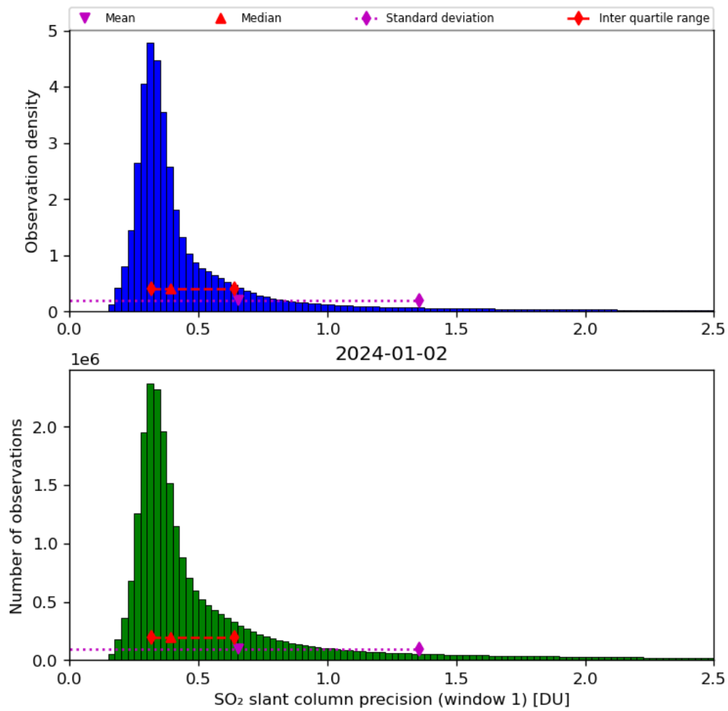
Figure 57: Histogram of “SO 2 slant column precision (window 1)” for 2024-01-01 to 2024-01-03
