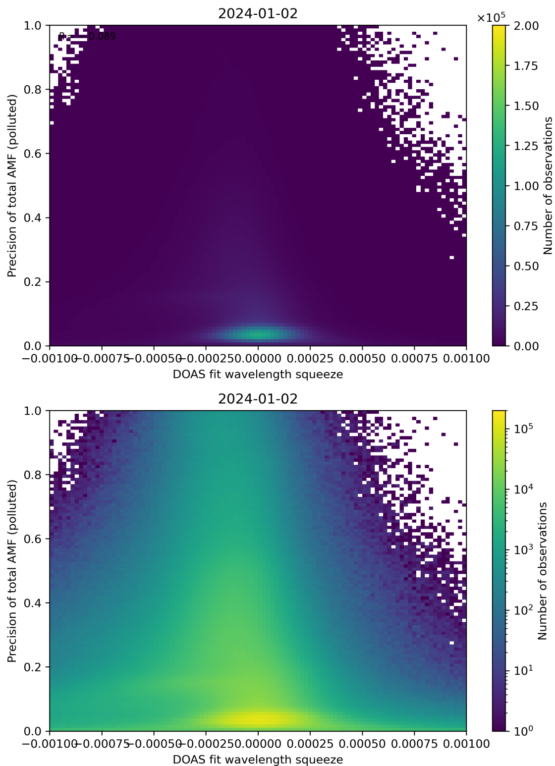
Figure 135: Scatter density plot of “DOAS fit wavelength squeeze” against “Precision of total AMF (polluted)” for 2024-01-01 to 2024-01-03.
