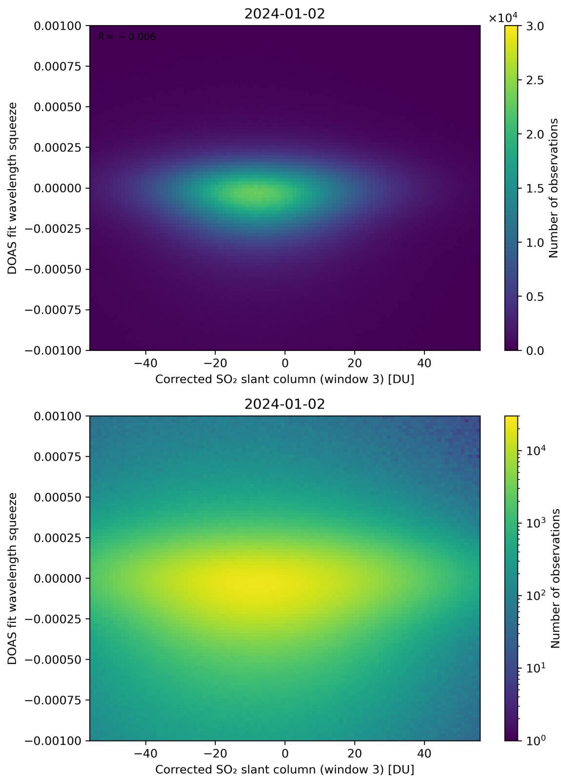
Figure 207: Scatter density plot of “Corrected SO 2 slant column (window 3)” against “DOAS fit wavelength squeeze” for 2024-01-01 to 2024-01-03.
