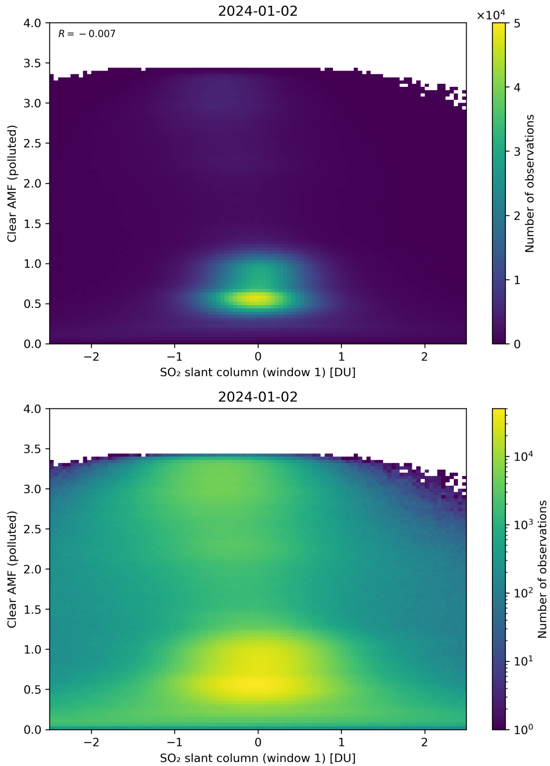
Figure 232: Scatter density plot of “SO 2 slant column (window 1)” against “Clear AMF (polluted)” for 2024-01-01 to 2024-01-03.
