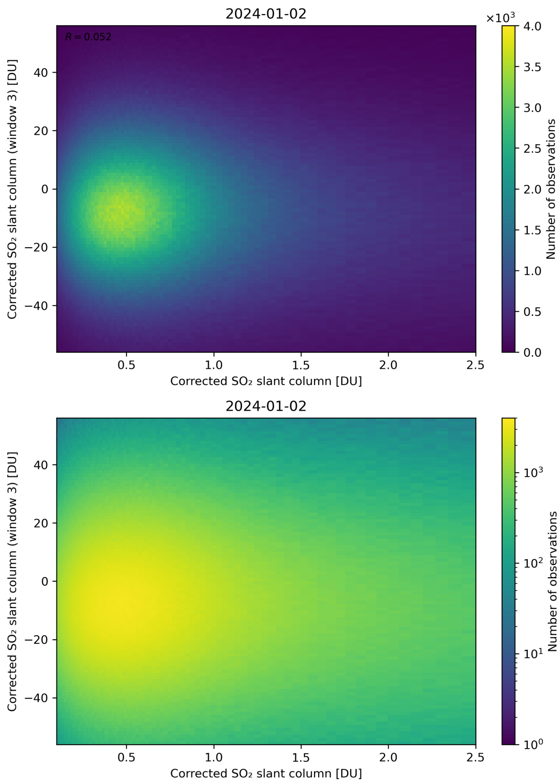
Figure 186: Scatter density plot of “Corrected SO 2 slant column” against “Corrected SO 2 slant column (window 3)” for 2024-01-01 to 2024-01-03.
