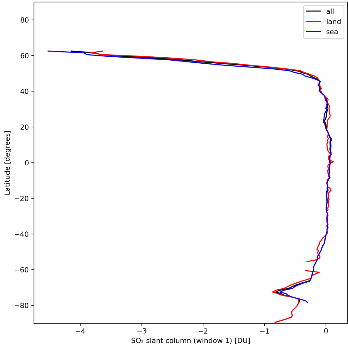
Figure 33: Zonal average of “SO 2 slant column (window 1)” for 2024-01-01 to 2024-01-03.
