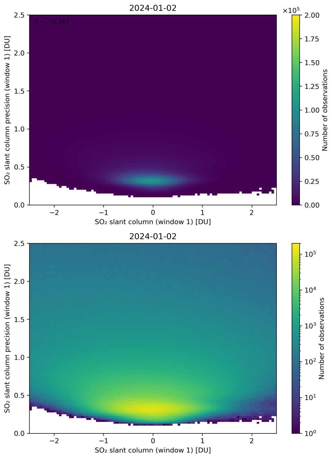
Figure 235: Scatter density plot of “SO 2 slant column (window 1)” against “SO 2 slant column precision (window 1)” for 2024-01-01 to 2024-01-03.
