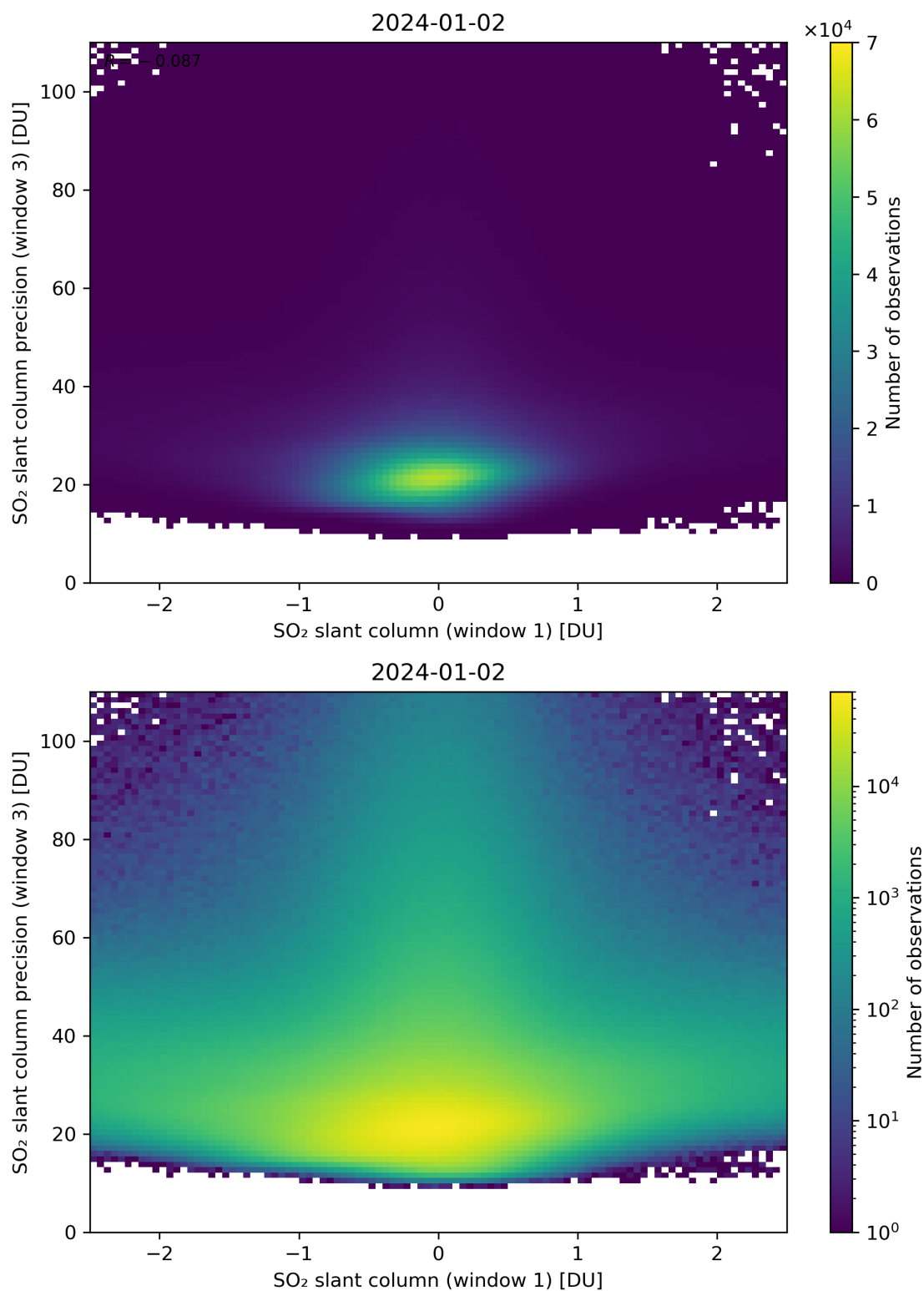
Figure 238: Scatter density plot of “SO 2 slant column (window 1)” against “SO 2 slant column precision (window 3)” for 2024-01-01 to 2024-01-03.
