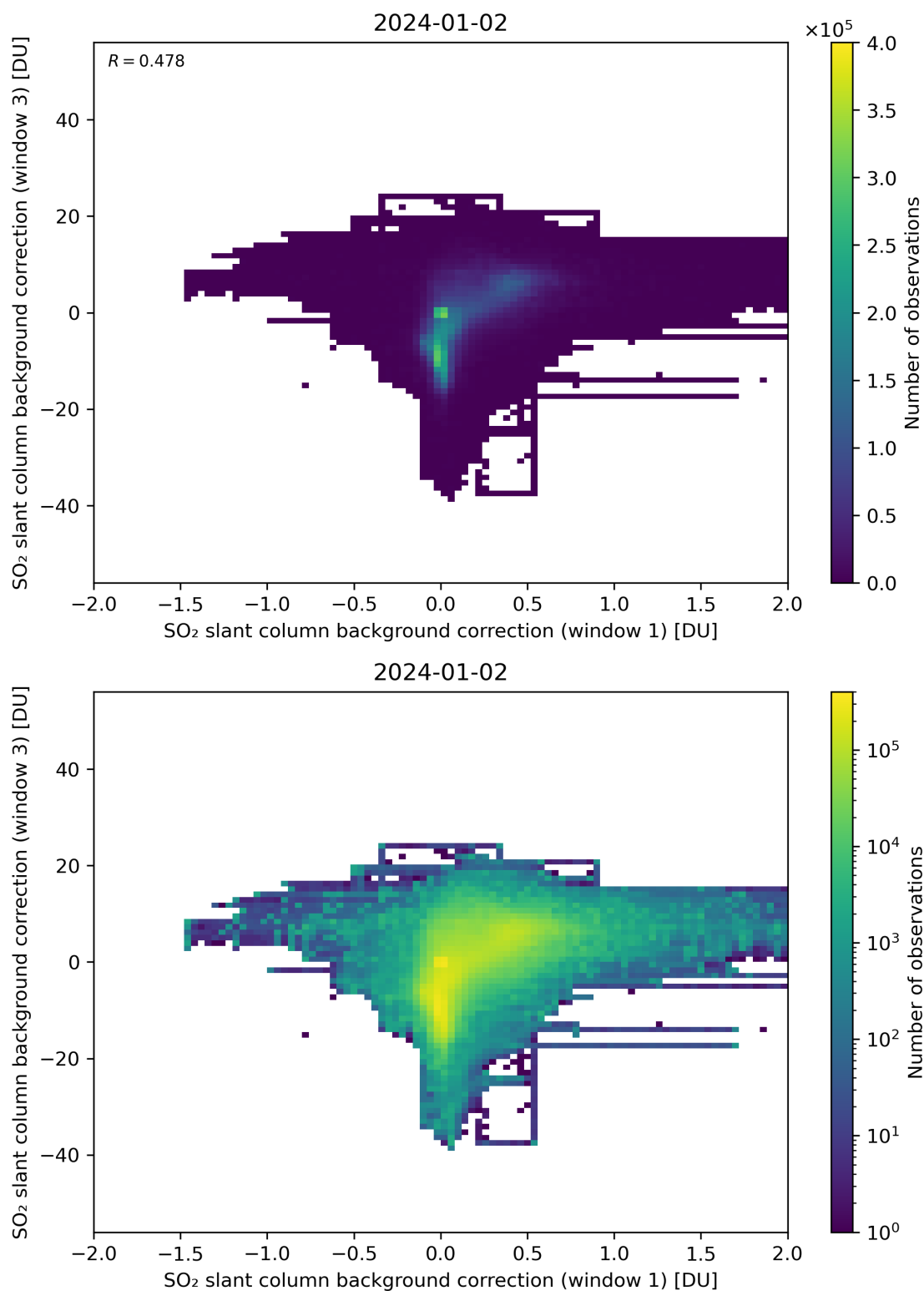
Figure 99: Scatter density plot of “SO 2 slant column background correction (window 1)” against “SO 2 slant column background correction (window 3)” for 2024-01-01 to 2024-01-03.
