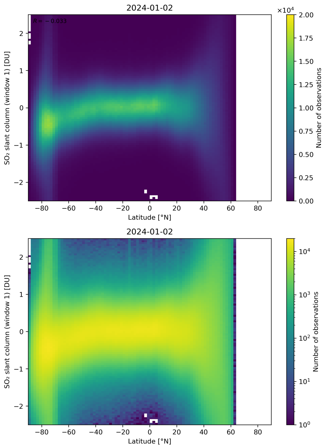
Figure 149: Scatter density plot of “Latitude” against “SO 2 slant column (window 1)” for 2024-01-01 to 2024-01-03.
