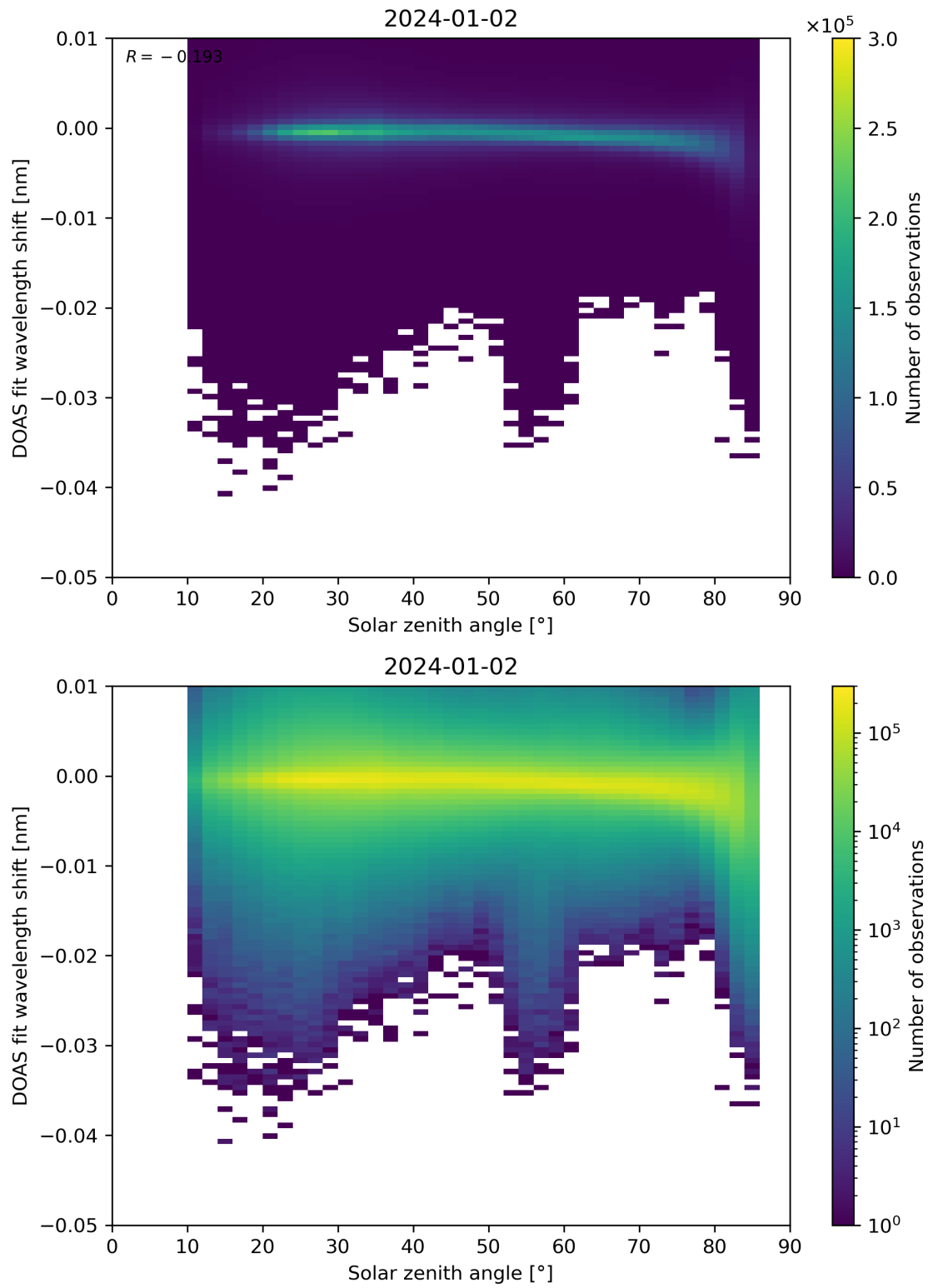
Figure 161: Scatter density plot of “Solar zenith angle” against “DOAS fit wavelength shift” for 2024-01-01 to 2024-01-03.
