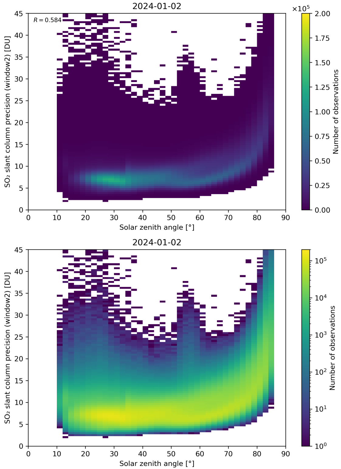
Figure 171: Scatter density plot of “Solar zenith angle” against “SO 2 slant column precision (window2)” for 2024-01-01 to 2024-01-03.
