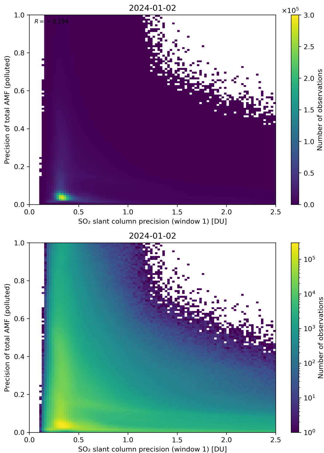
Figure 231: Scatter density plot of “SO 2 slant column precision (window 1)” against “Precision of total AMF (polluted)” for 2024-01-01 to 2024-01-03.
