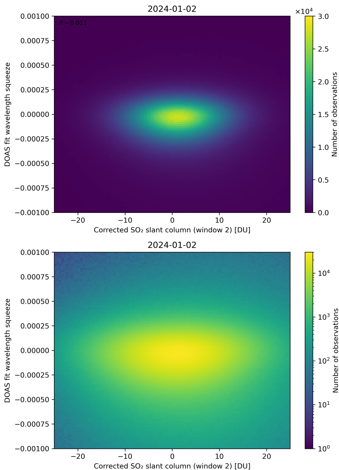
Figure 197: Scatter density plot of “Corrected SO 2 slant column (window 2)” against “DOAS fit wavelength squeeze” for 2024-01-01 to 2024-01-03.
