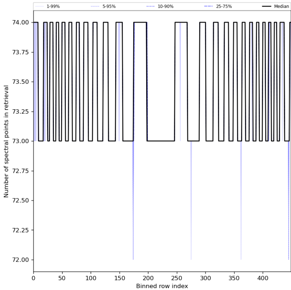
Figure 97: Along track statistics of “Number of spectral points in retrieval” for 2024-01-01 to 2024-01-03
