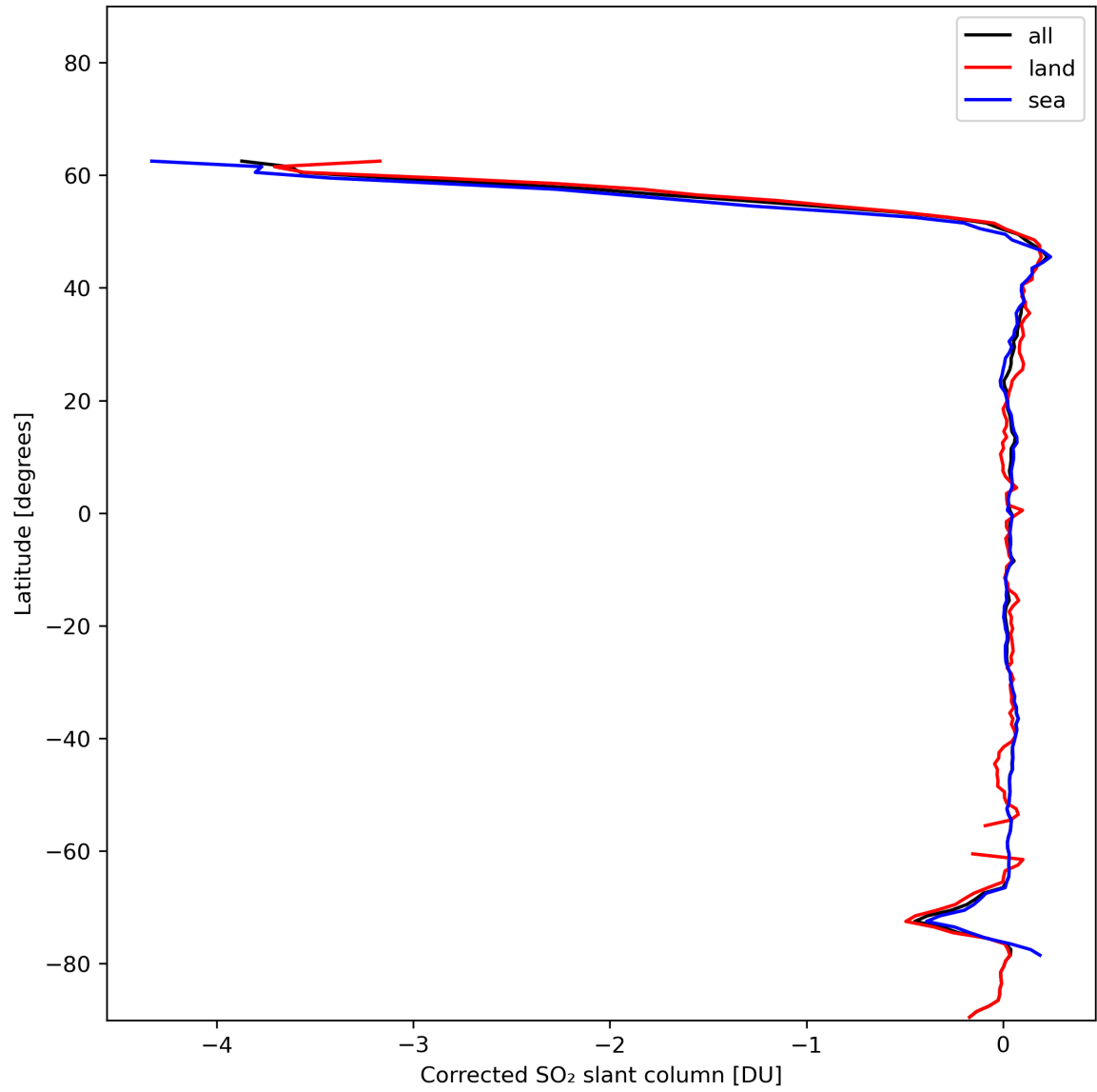
Figure 32: Zonal average of “Corrected SO 2 slant column” for 2024-01-01 to 2024-01-03.
