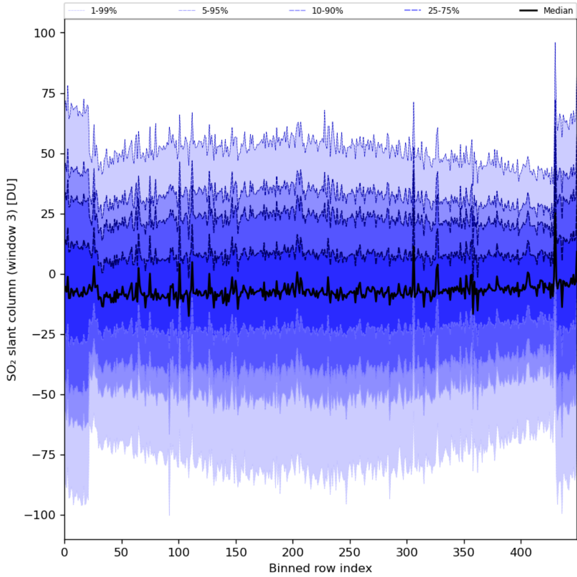
Figure 87: Along track statistics of “SO 2 slant column (window 3)” for 2024-01-01 to 2024-01-03
