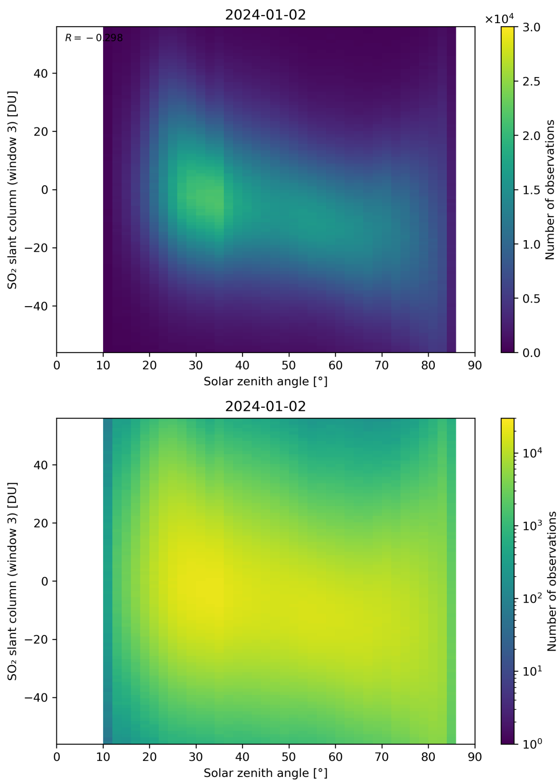
Figure 172: Scatter density plot of “Solar zenith angle” against “SO 2 slant column (window 3)” for 2024-01-01 to 2024-01-03.
