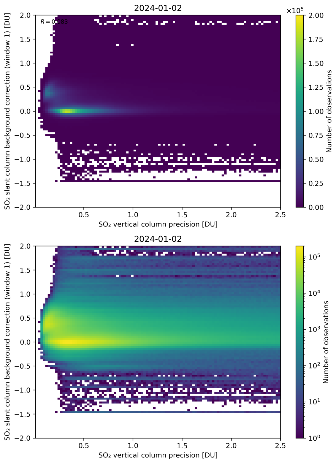
Figure 279: Scatter density plot of “SO 2 vertical column precision” against “SO 2 slant column background correction (window 1)” for 2024-01-01 to 2024-01-03.
