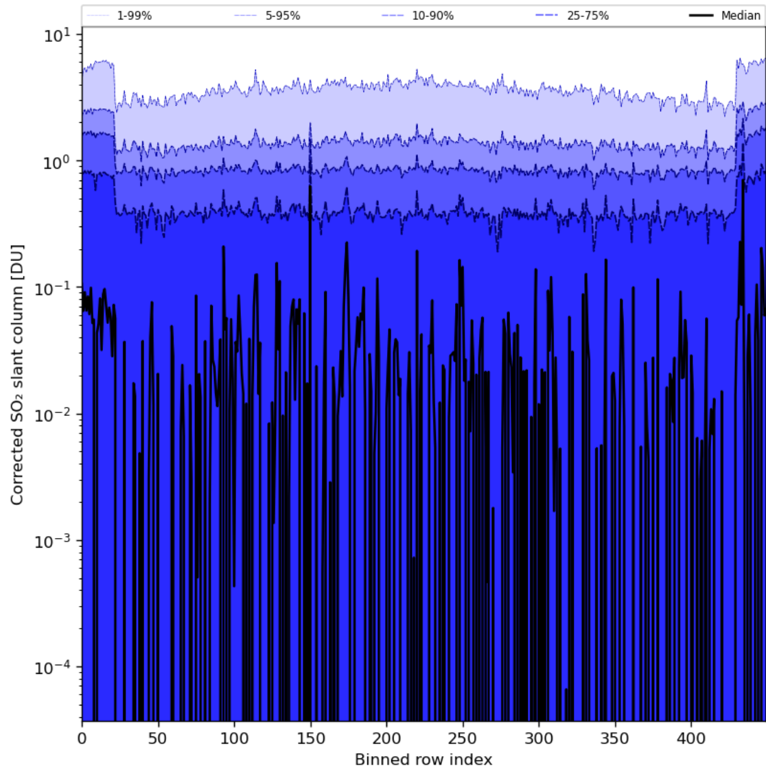
Figure 78: Along track statistics of "Corrected SO 2 slant column" for 2024-01-01 to 2024-01-03
