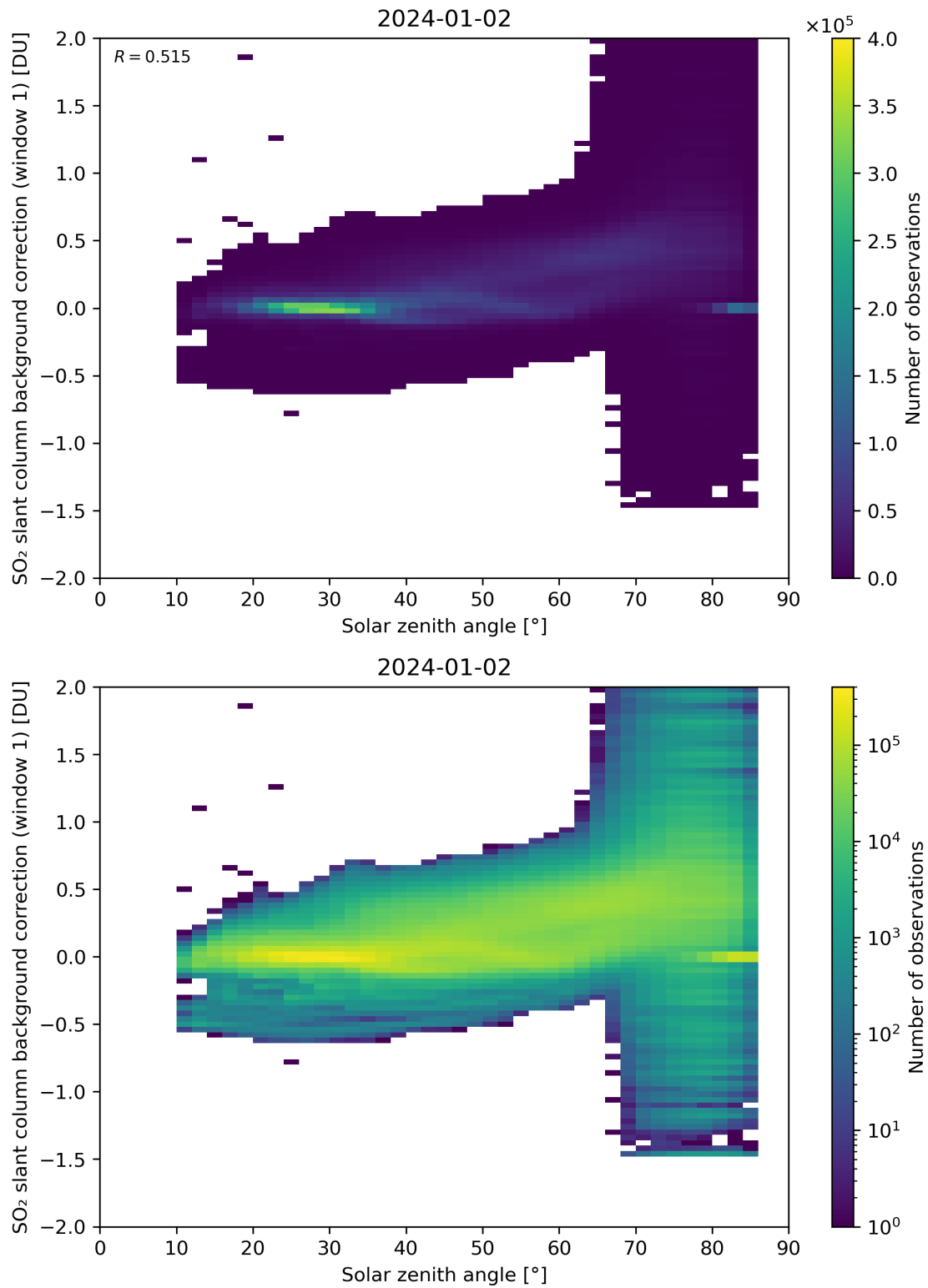
Figure 158: Scatter density plot of “Solar zenith angle” against “SO 2 slant column background correction (window 1)” for 2024-01-01 to 2024-01-03.
