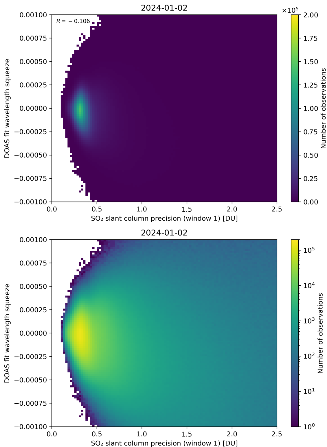
Figure 222: Scatter density plot of “SO 2 slant column precision (window 1)” against “DOAS fit wavelength squeeze” for 2024-01-01 to 2024-01-03.
