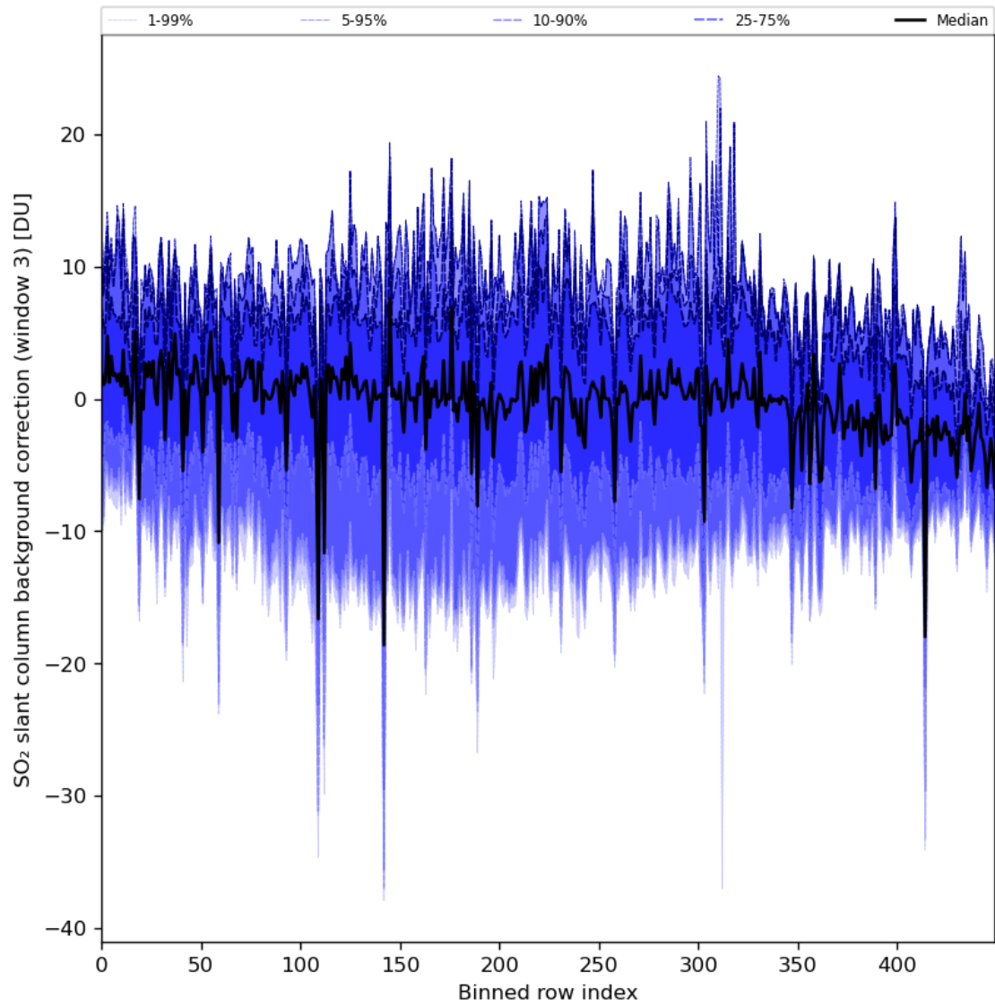
Figure 90: Along track statistics of “SO 2 slant column background correction (window 3)” for 2024-01-01 to 2024-01-03
