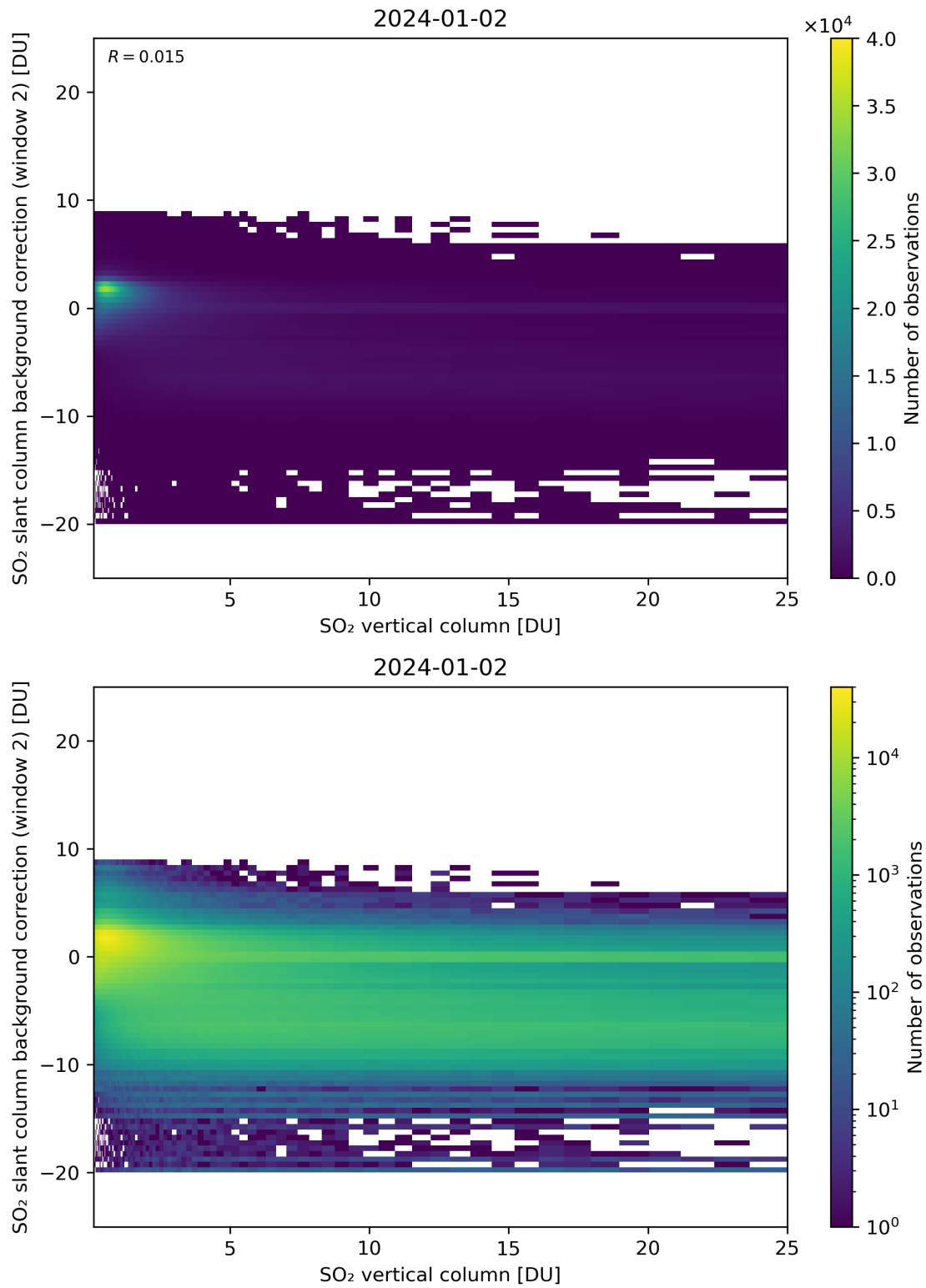
Figure 274: Scatter density plot of “SO 2 vertical column” against “SO 2 slant column background correction (window 2)” for 2024-01-01 to 2024-01-03.
