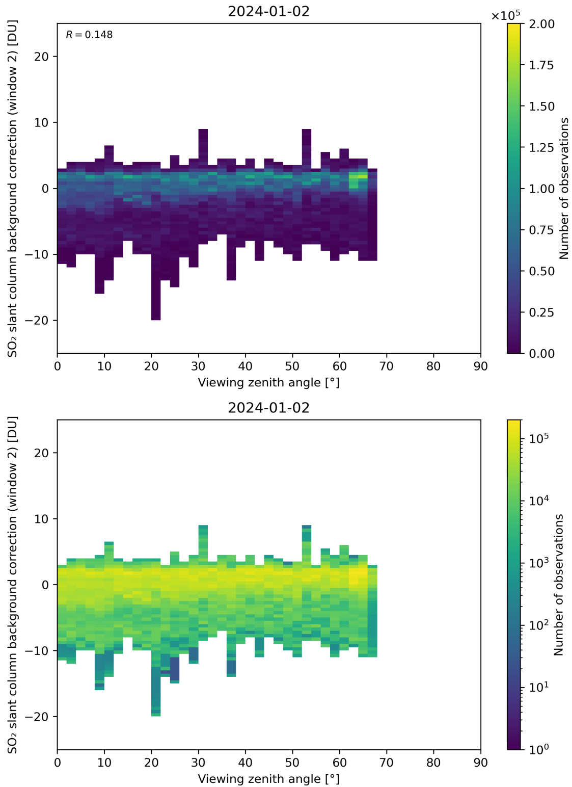
Figure 309: Scatter density plot of “Viewing zenith angle” against “SO 2 slant column background correction (window 2)” for 2024-01-01 to 2024-01-03.
