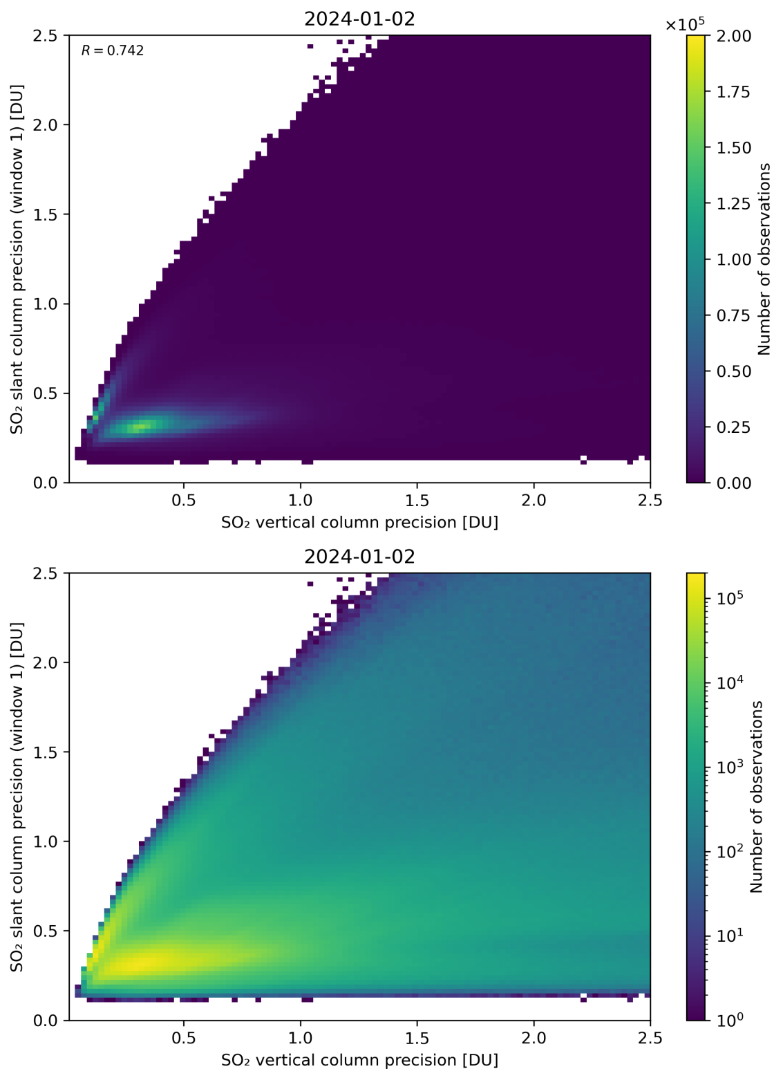
Figure 290: Scatter density plot of “SO 2 vertical column precision” against “SO 2 slant column precision (window 1)” for 2024-01-01 to 2024-01-03.
