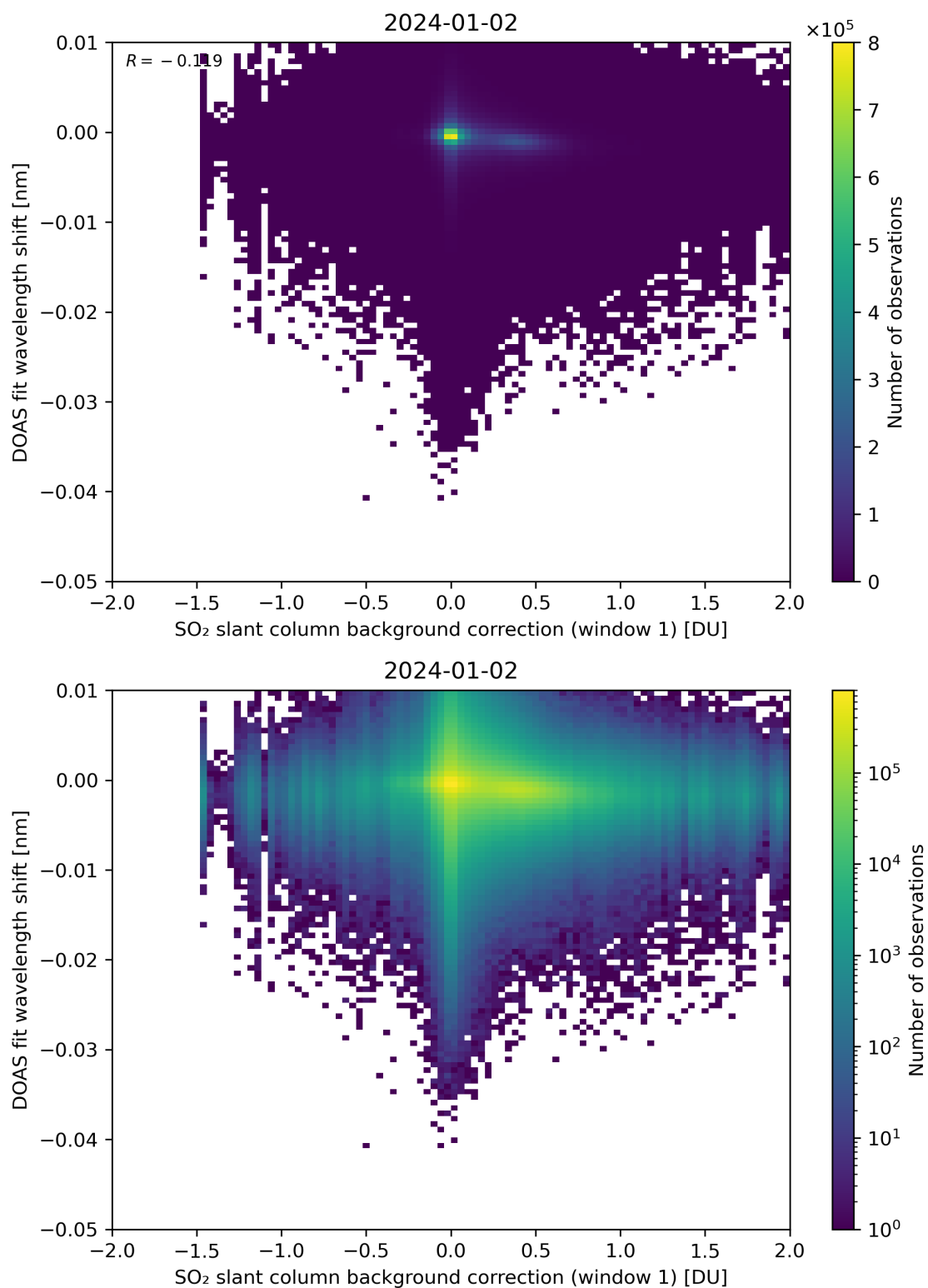
Figure 100: Scatter density plot of “SO 2 slant column background correction (window 1)” against “DOAS fit wavelength shift” for 2024-01-01 to 2024-01-03.
