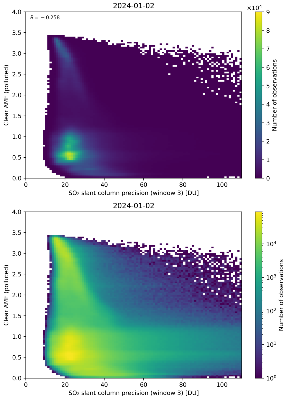
Figure 261: Scatter density plot of “SO 2 slant column precision (window 3)” against “Clear AMF (polluted)” for 2024-01-01 to 2024-01-03.
