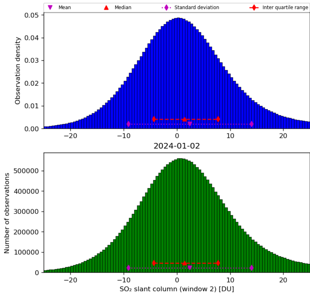
Figure 60: Histogram of “SO 2 slant column (window 2)” for 2024-01-01 to 2024-01-03
