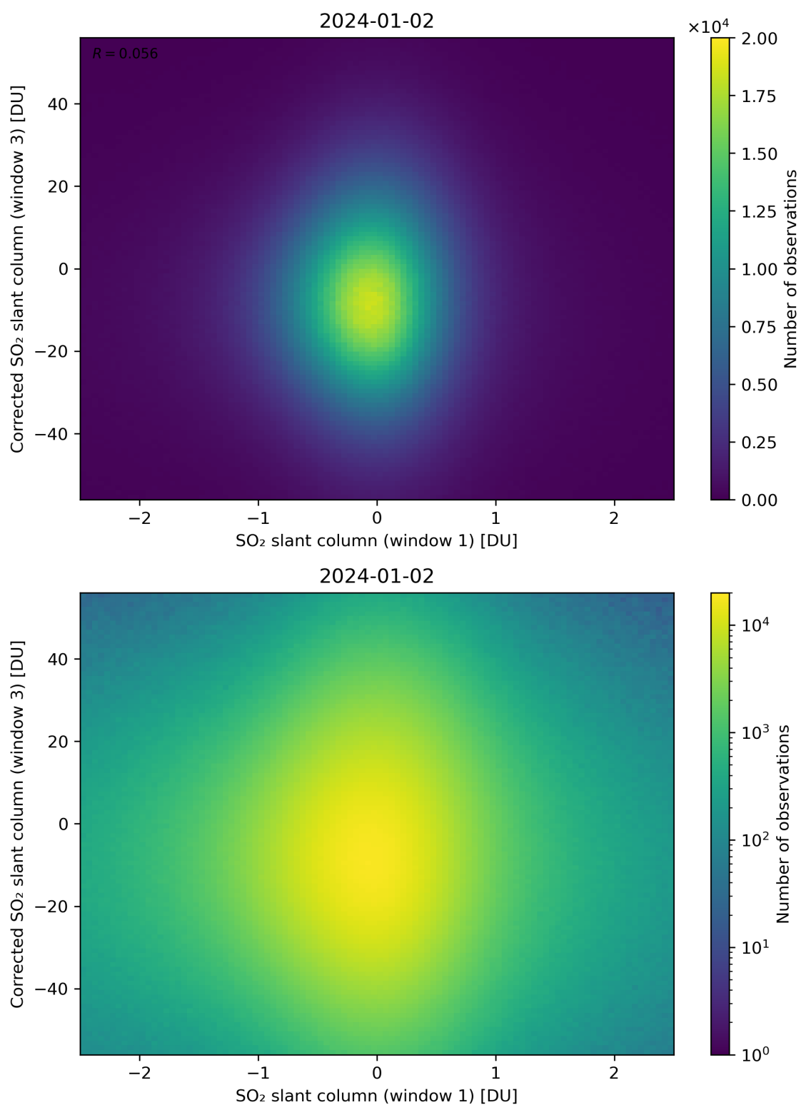
Figure 234: Scatter density plot of “SO 2 slant column (window 1)” against “Corrected SO 2 slant column (window 3)” for 2024-01-01 to 2024-01-03.
