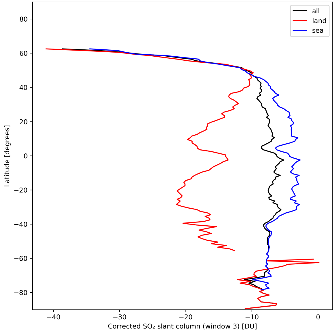
Figure 43: Zonal average of “Corrected SO 2 slant column (window 3)” for 2024-01-01 to 2024-01-03.
