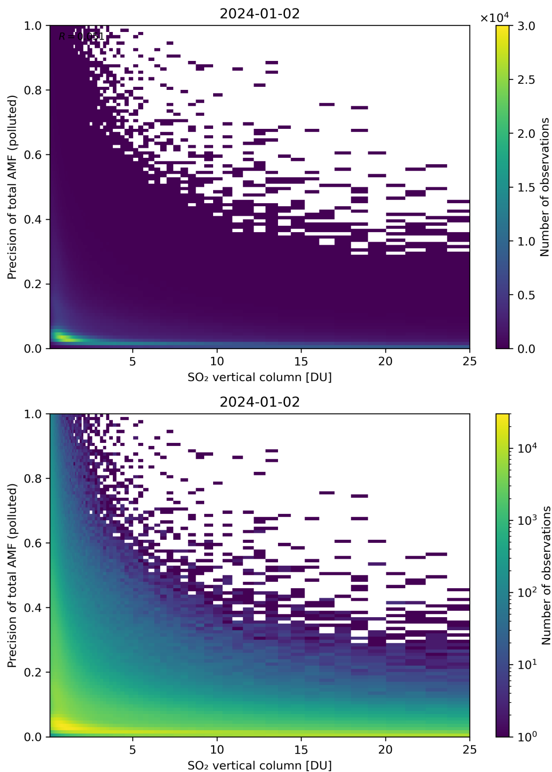
Figure 306: Scatter density plot of “SO 2 vertical column” against “Precision of total AMF (polluted)” for 2024-01-01 to 2024-01-03.
