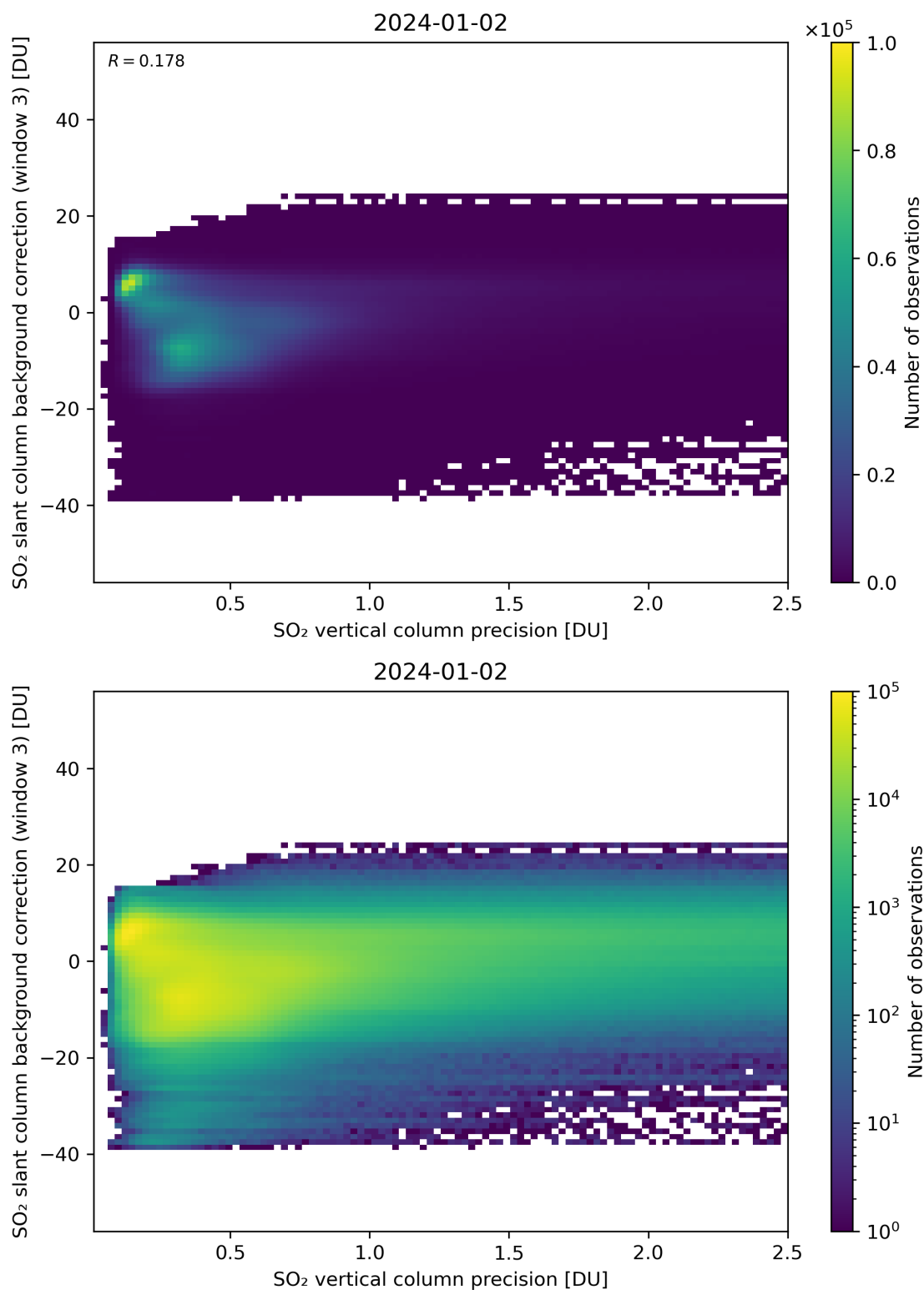
Figure 281: Scatter density plot of “SO 2 vertical column precision” against “SO 2 slant column background correction (window 3)” for 2024-01-01 to 2024-01-03.
