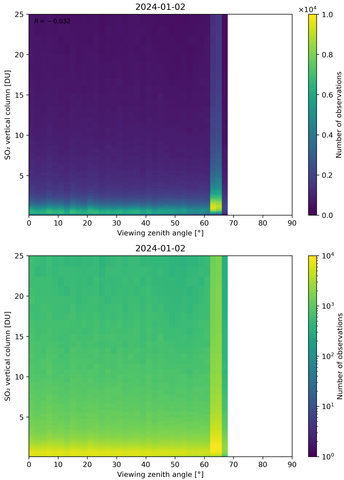
Figure 327: Scatter density plot of “Viewing zenith angle” against “SO 2 vertical column” for 2024-01-01 to 2024-01-03.
