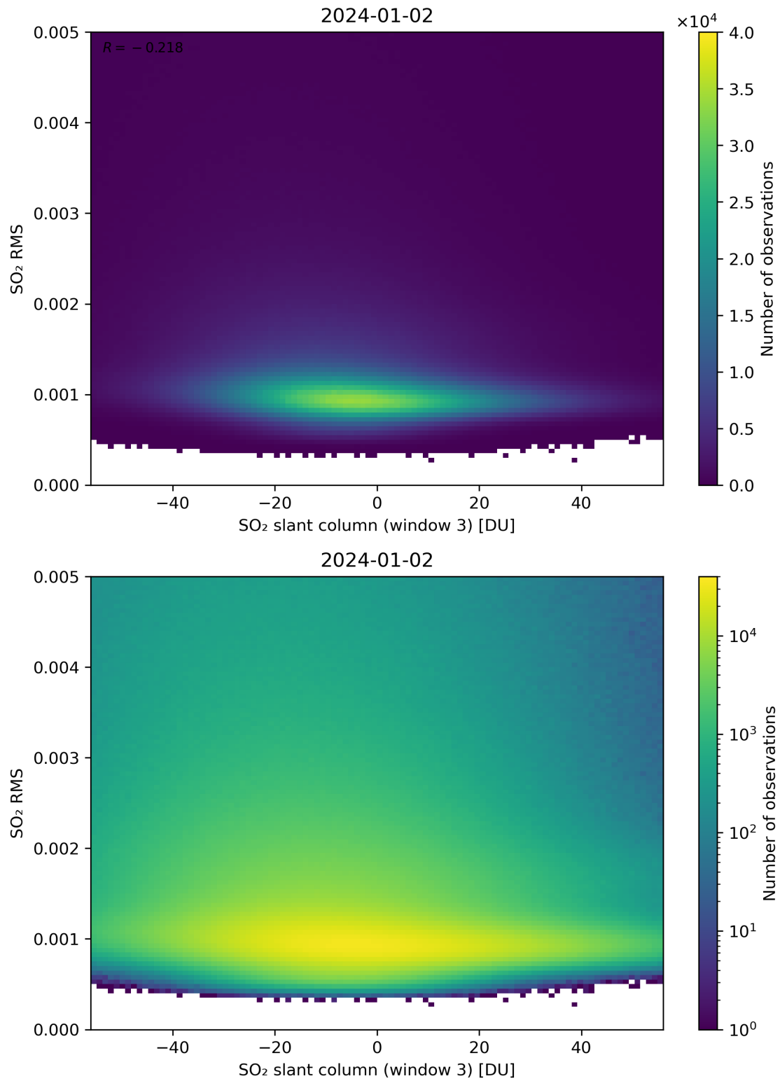
Figure 256: Scatter density plot of “SO 2 slant column (window 3)” against “SO 2 RMS” for 2024-01-01 to 2024-01-03.
