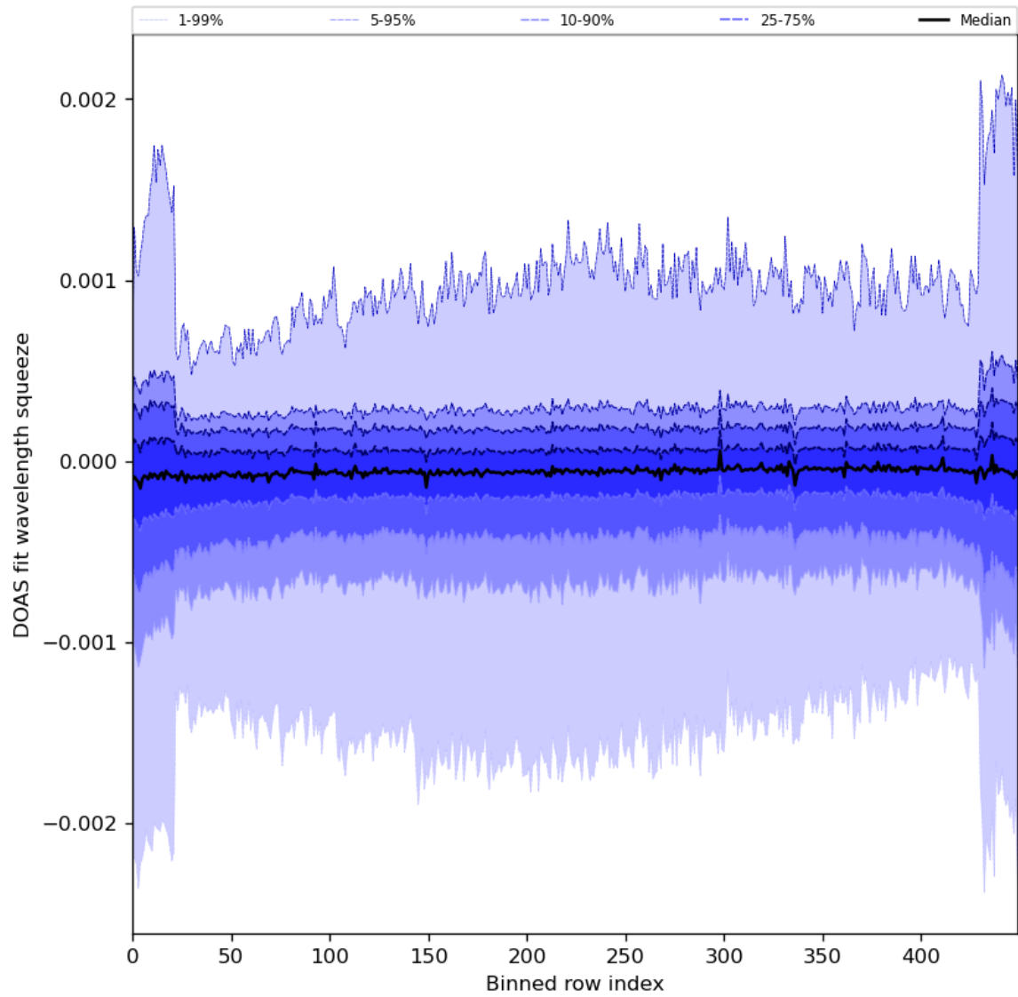
Figure 92: Along track statistics of “DOAS fit wavelength squeeze” for 2024-01-01 to 2024-01-03
