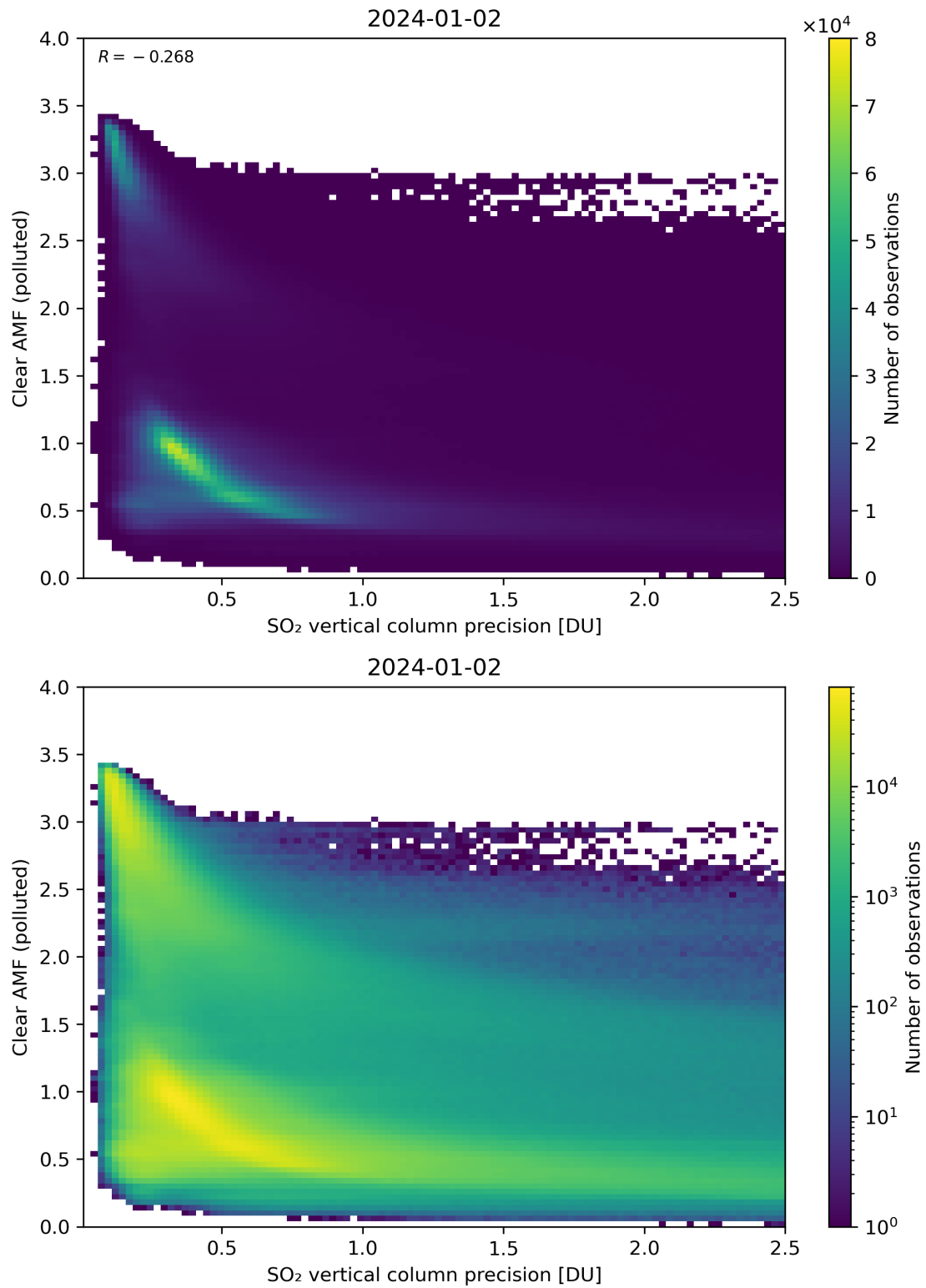
Figure 285: Scatter density plot of “SO 2 vertical column precision” against “Clear AMF (polluted)” for 2024-01-01 to 2024-01-03.
