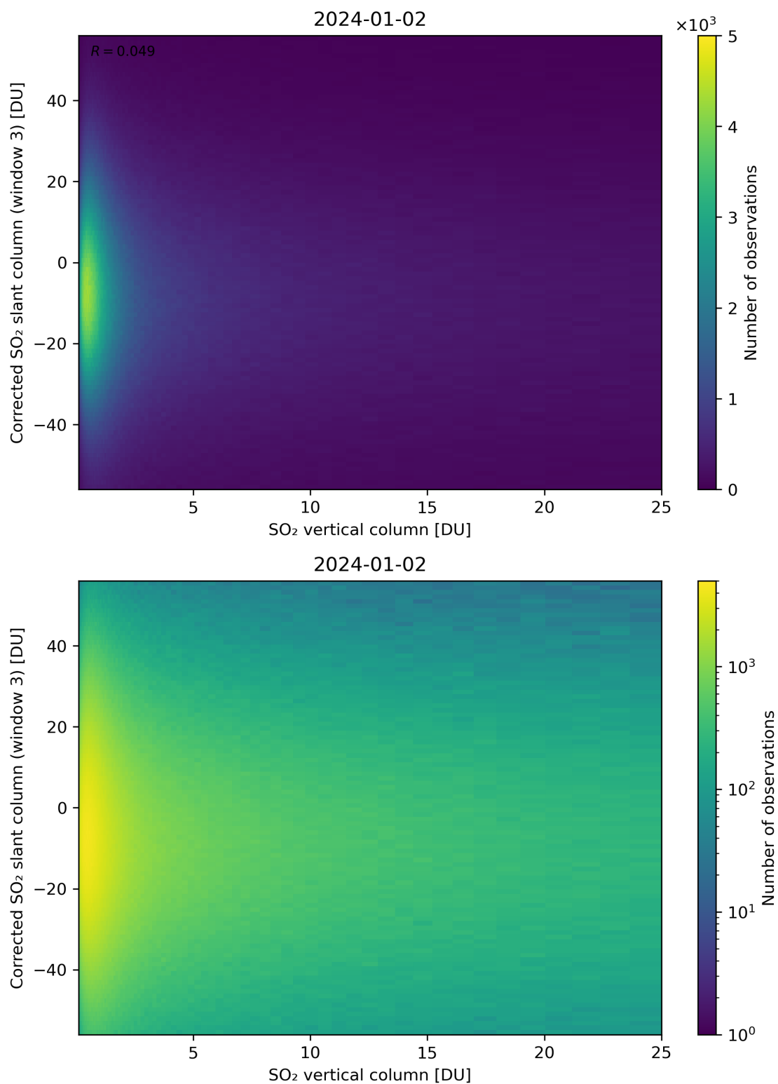
Figure 299: Scatter density plot of “SO 2 vertical column” against “Corrected SO 2 slant column (window 3)” for 2024-01-01 to 2024-01-03.
