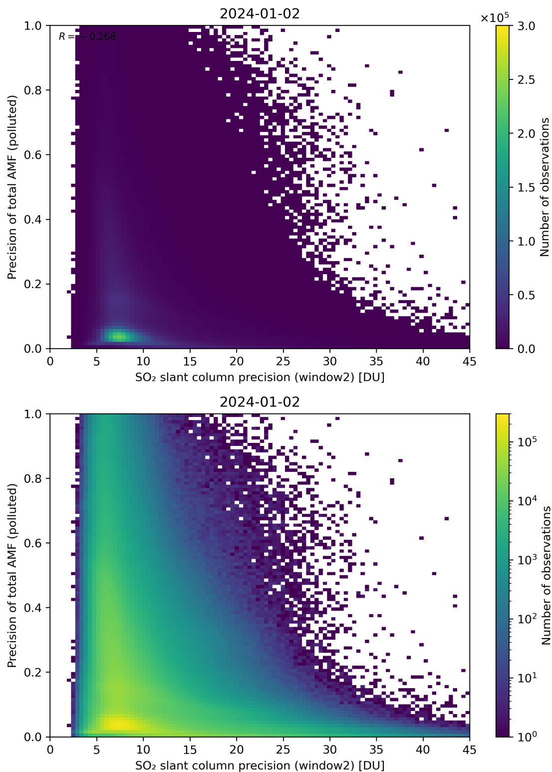
Figure 252: Scatter density plot of “SO 2 slant column precision (window2)” against “Precision of total AMF (polluted)” for 2024-01-01 to 2024-01-03.
