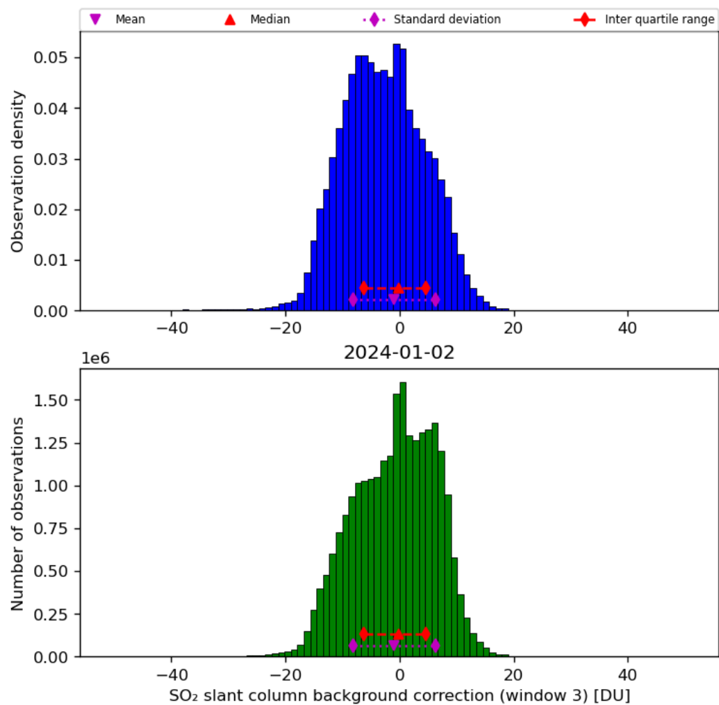
Figure 67: Histogram of “SO 2 slant column background correction (window 3)” for 2024-01-01 to 2024-01-03
