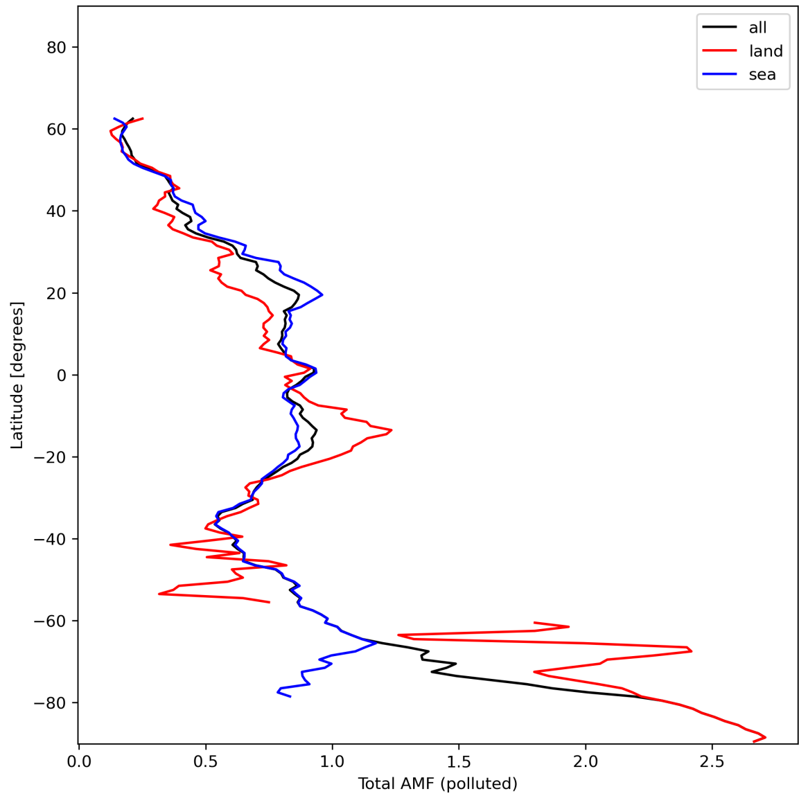
Figure 48: Zonal average of “Total AMF (polluted)” for 2024-01-01 to 2024-01-03.
