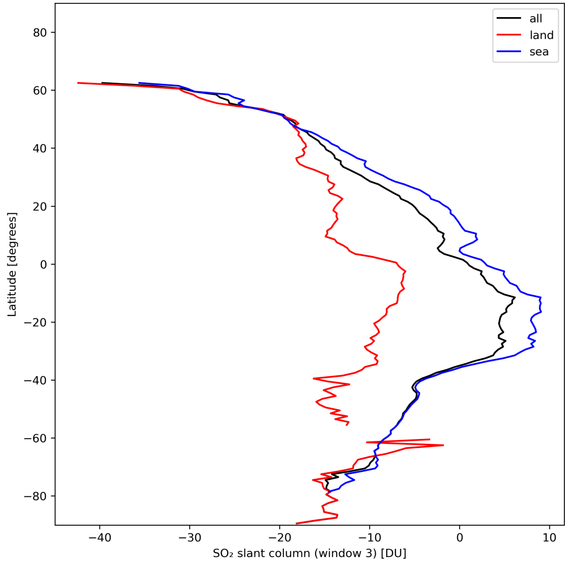
Figure 41: Zonal average of “SO 2 slant column (window 3)” for 2024-01-01 to 2024-01-03.
