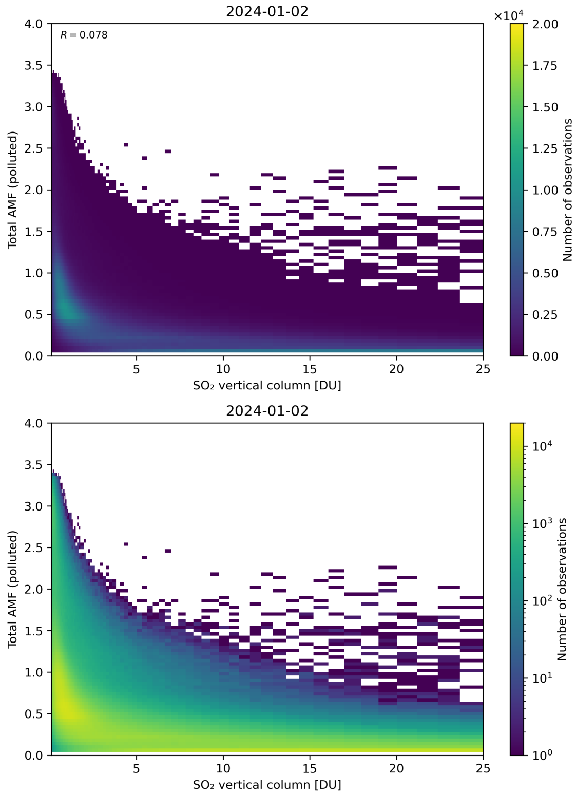
Figure 305: Scatter density plot of “SO 2 vertical column” against “Total AMF (polluted)” for 2024-01-01 to 2024-01-03.
