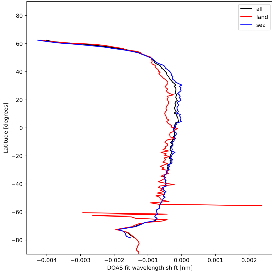
Figure 45: Zonal average of “DOAS fit wavelength shift” for 2024-01-01 to 2024-01-03.
