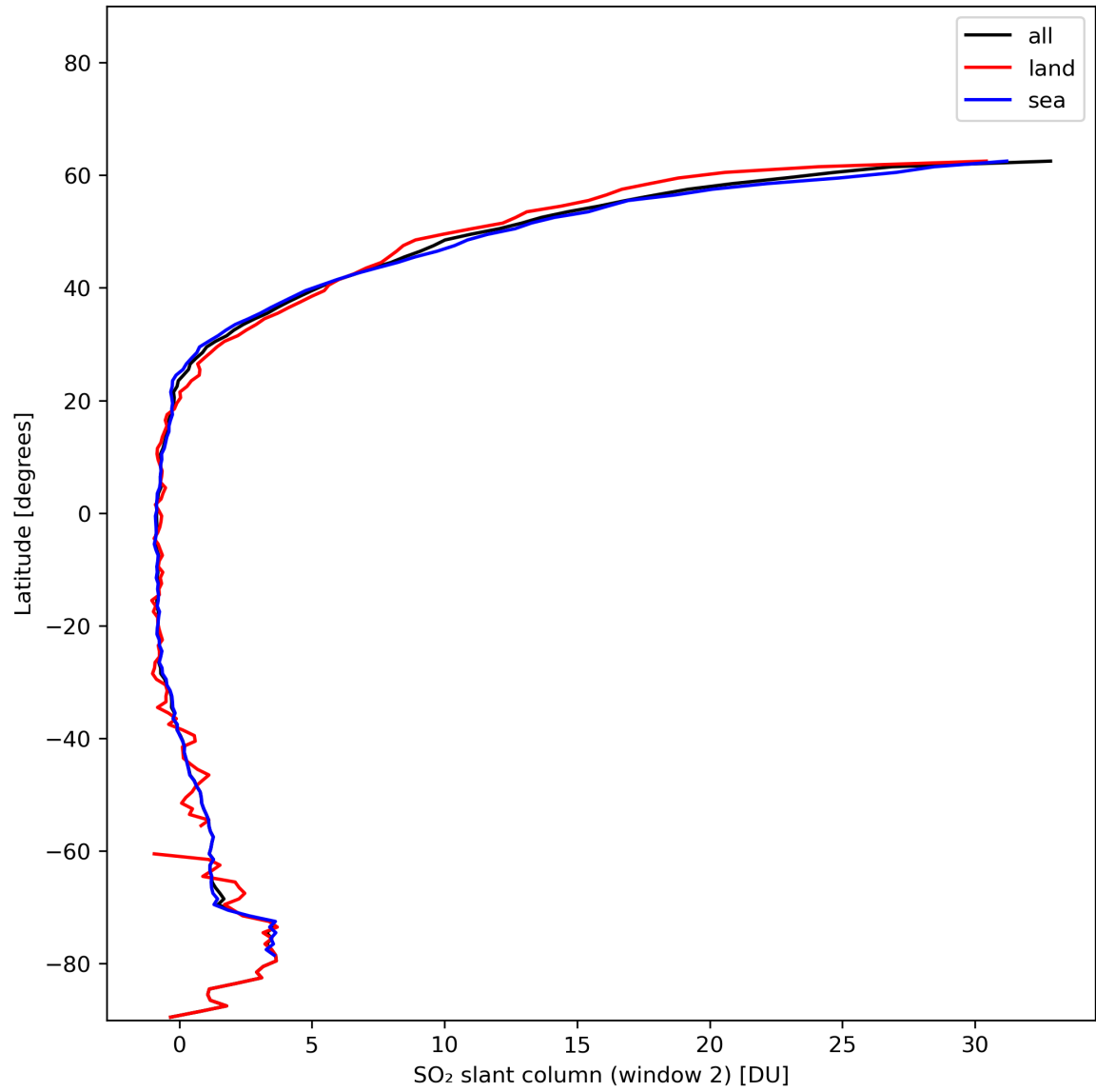
Figure 37: Zonal average of “SO 2 slant column (window 2)” for 2024-01-01 to 2024-01-03.
