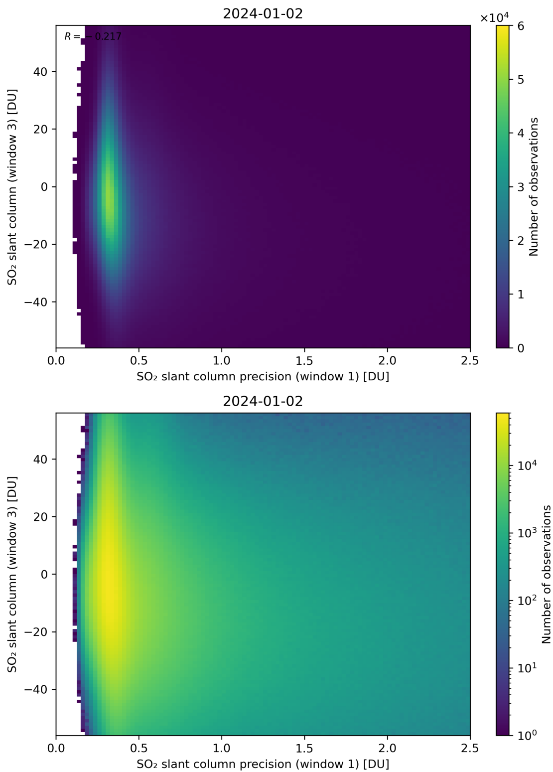
Figure 228: Scatter density plot of “SO 2 slant column precision (window 1)” against “SO 2 slant column (window 3)” for 2024-01-01 to 2024-01-03.
