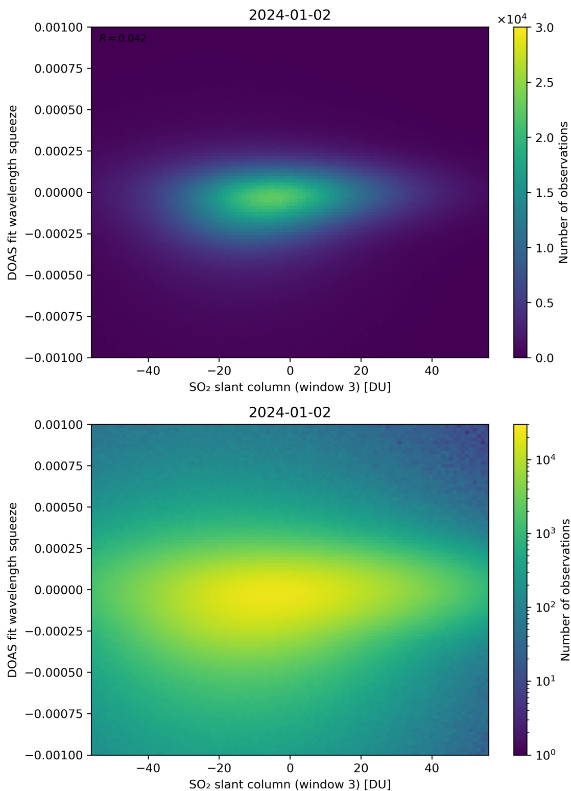
Figure 255: Scatter density plot of “SO 2 slant column (window 3)” against “DOAS fit wavelength squeeze” for 2024-01-01 to 2024-01-03.
