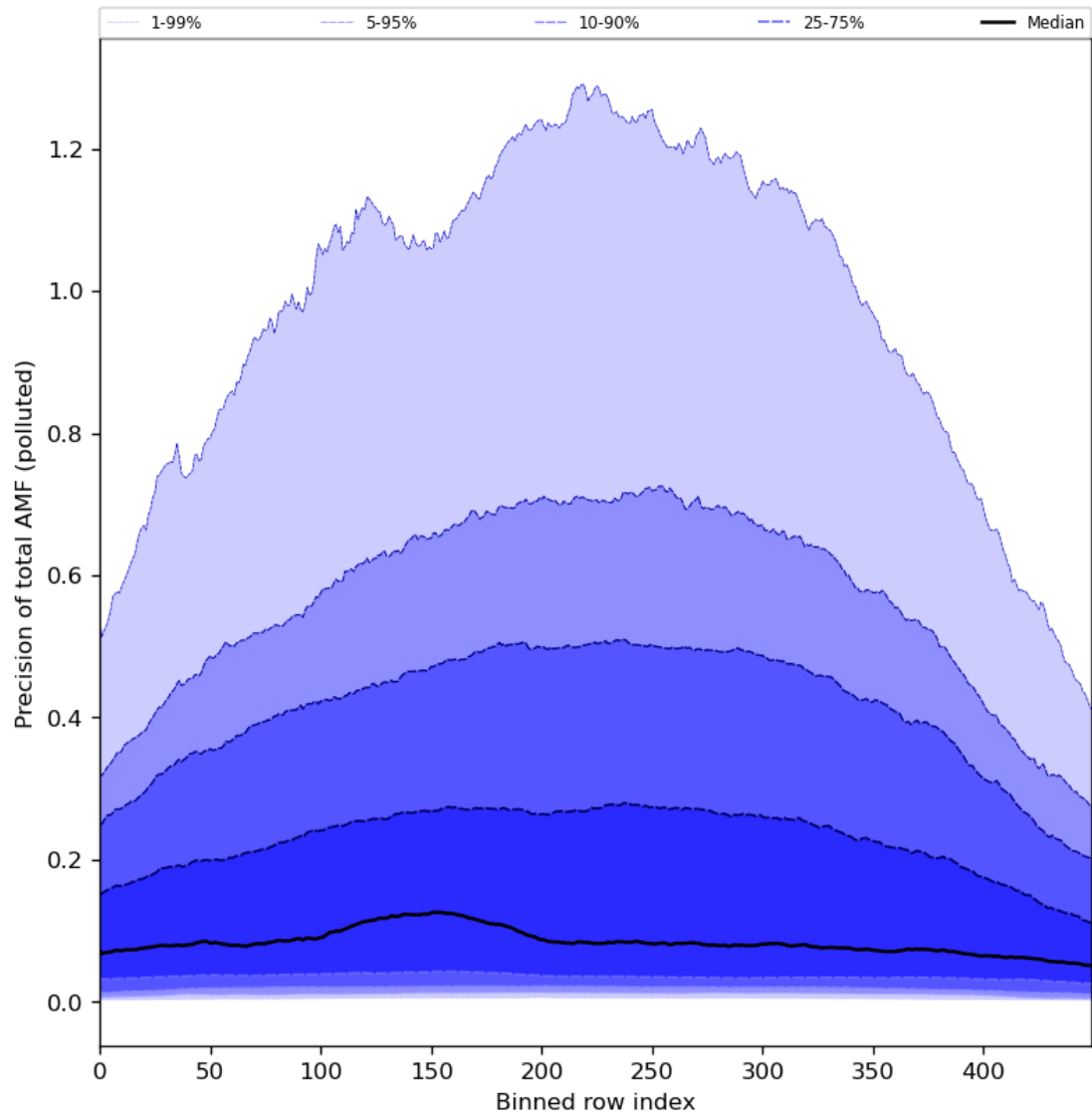
Figure 95: Along track statistics of “Precision of total AMF (polluted)” for 2024-01-01 to 2024-01-03
