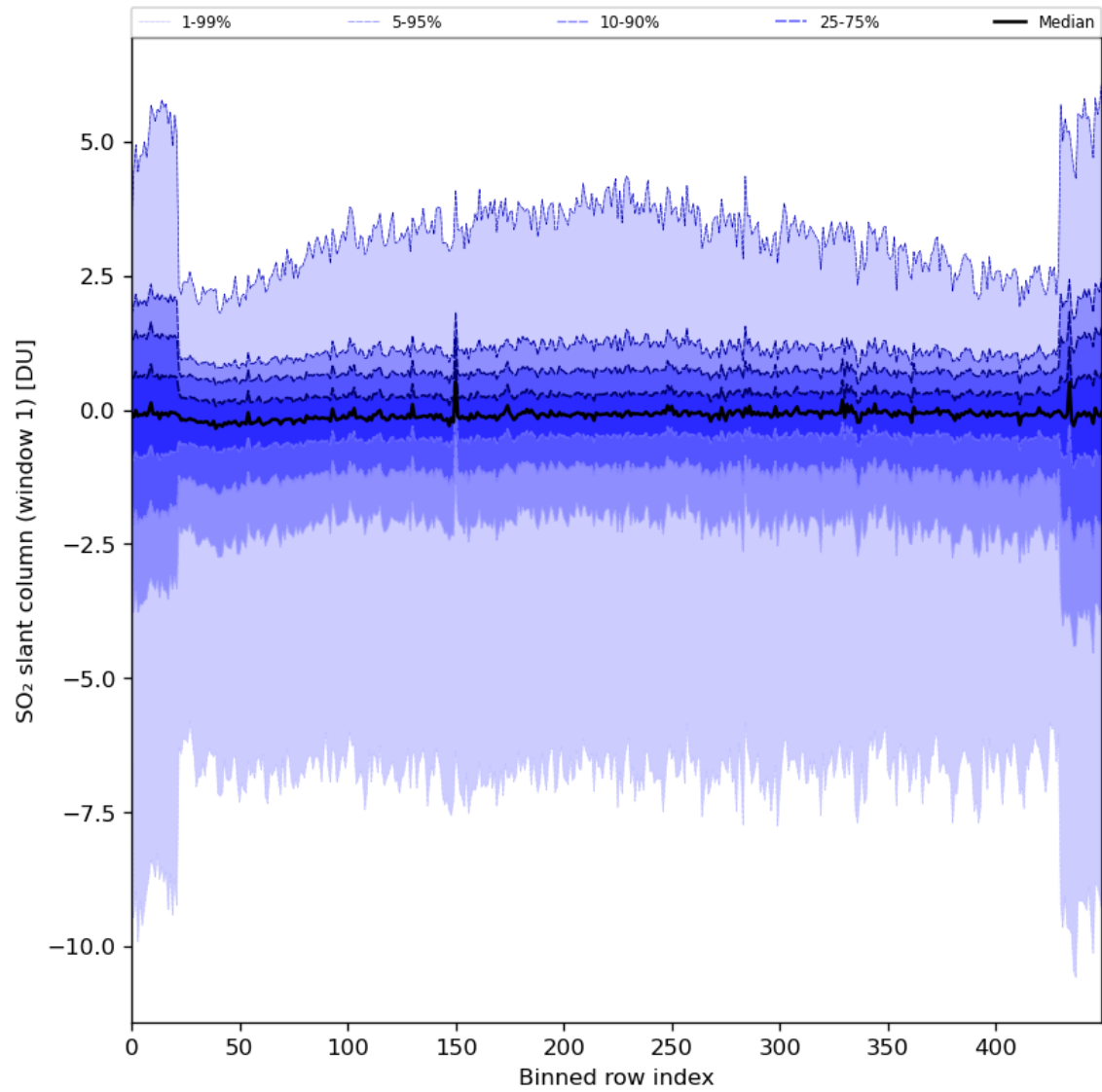
Figure 79: Along track statistics of “SO 2 slant column (window 1)” for 2024-01-01 to 2024-01-03
