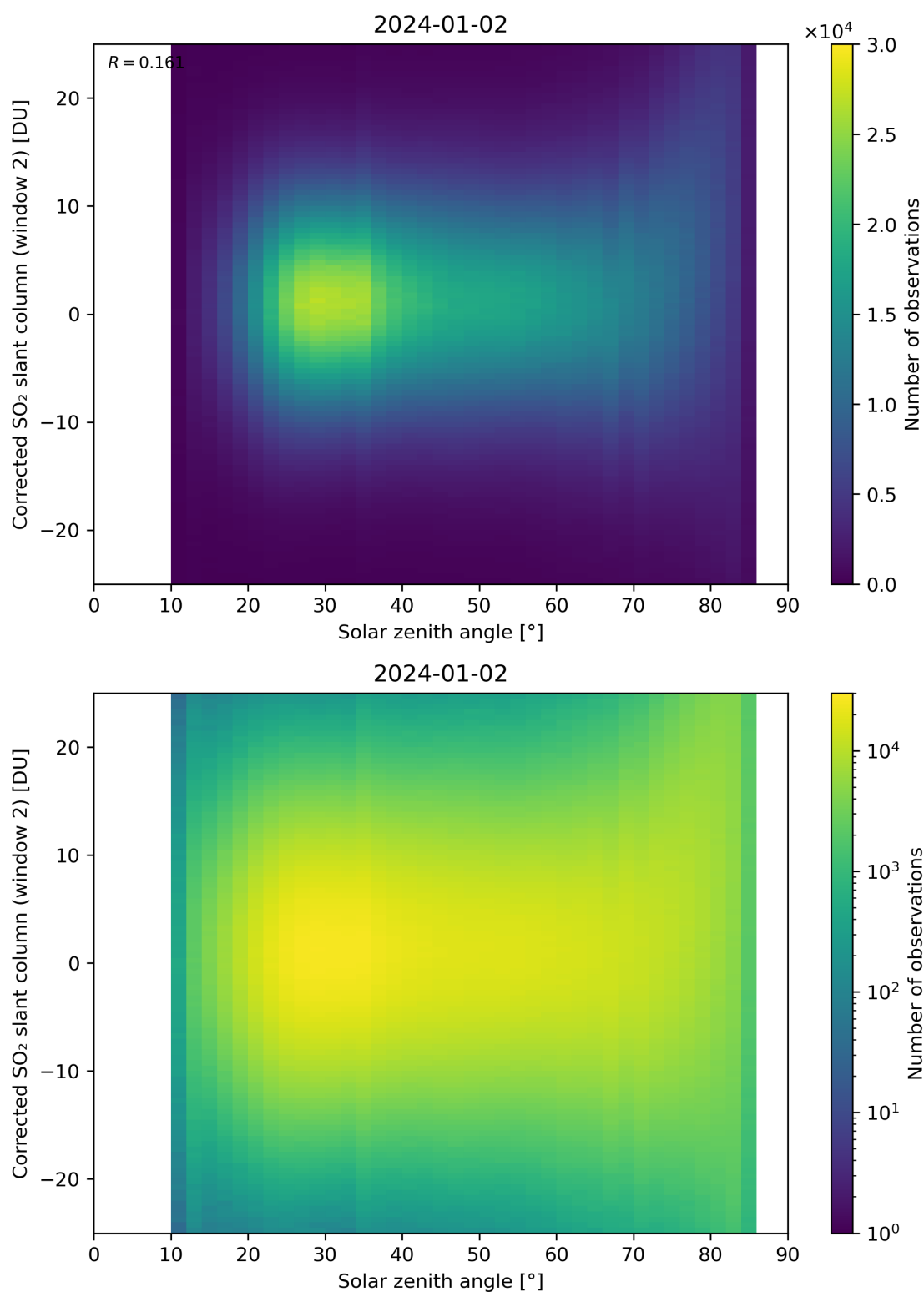
Figure 167: Scatter density plot of “Solar zenith angle” against “Corrected SO 2 slant column (window 2)” for 2024-01-01 to 2024-01-03.
