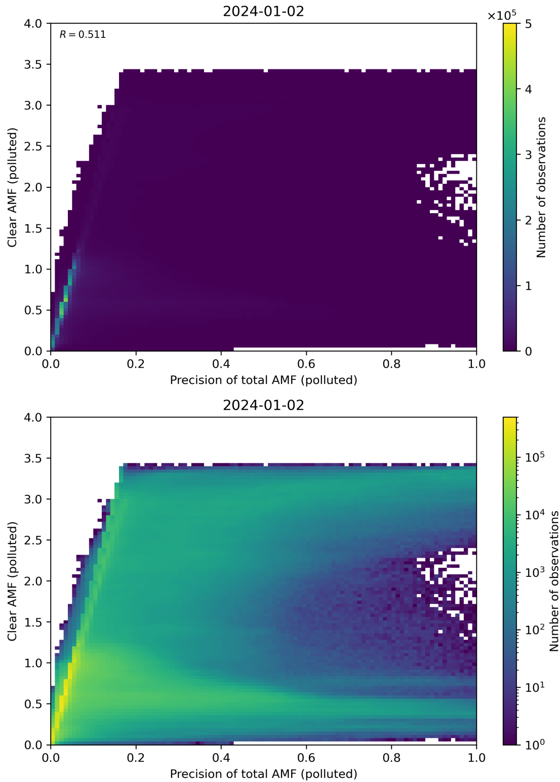
Figure 270: Scatter density plot of “Precision of total AMF (polluted)” against “Clear AMF (polluted)” for 2024-01-01 to 2024-01-03.
