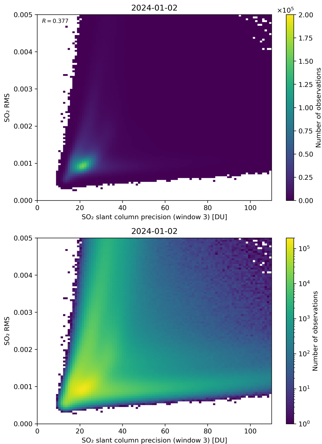
Figure 260: Scatter density plot of “SO 2 slant column precision (window 3)” against “SO 2 RMS” for 2024-01-01 to 2024-01-03.
