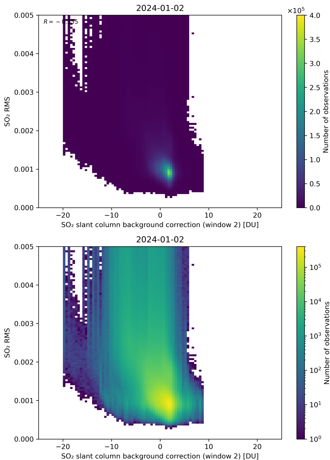
Figure 114: Scatter density plot of “SO 2 slant column background correction (window 2)” against “SO 2 RMS” for 2024-01-01 to 2024-01-03.
