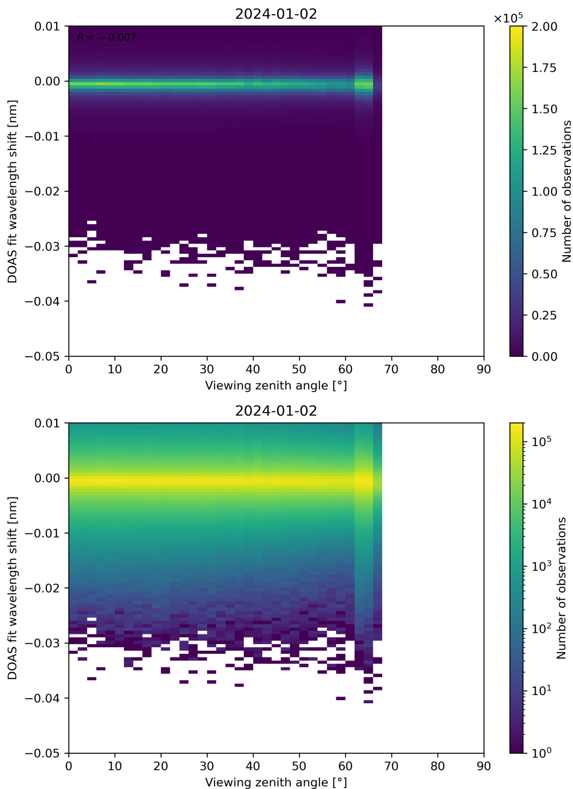
Figure 311: Scatter density plot of “Viewing zenith angle” against “DOAS fit wavelength shift” for 2024-01-01 to 2024-01-03.
