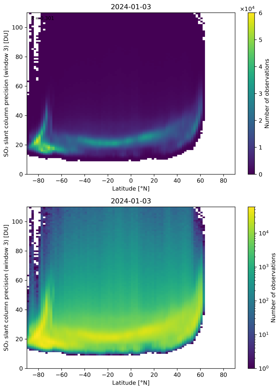
Figure 153: Scatter density plot of “Latitude” against “SO 2 slant column precision (window 3)” for 2024-01-02 to 2024-01-04.
