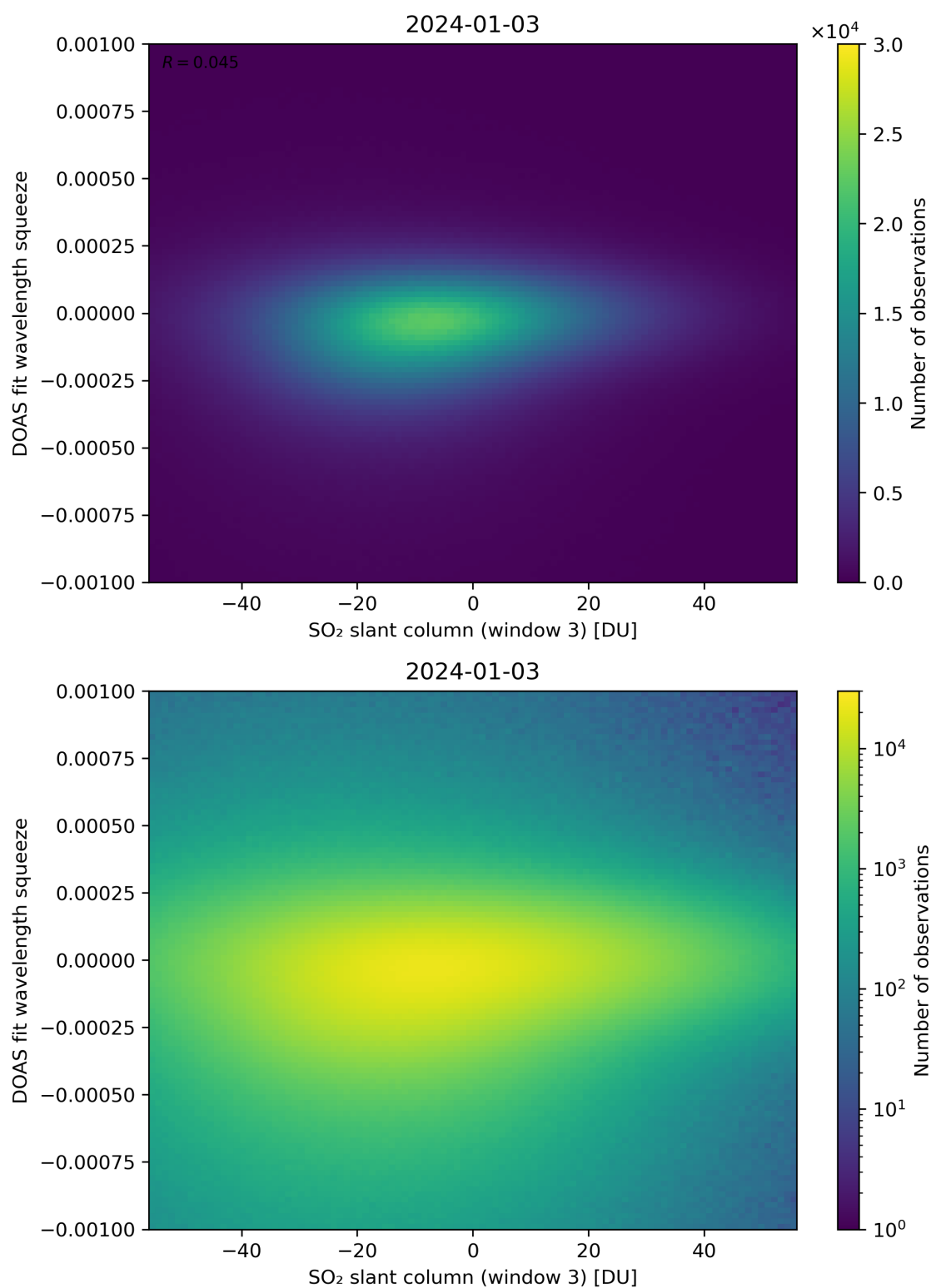
Figure 255: Scatter density plot of “SO 2 slant column (window 3)” against “DOAS fit wavelength squeeze” for 2024-01-02 to 2024-01-04.
