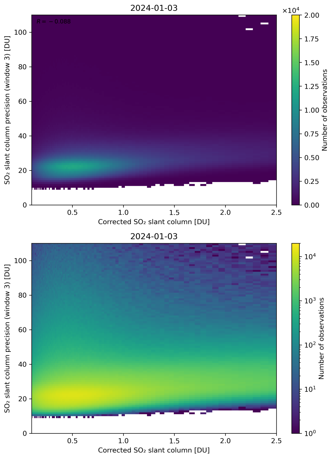
Figure 191: Scatter density plot of “Corrected SO 2 slant column” against “SO 2 slant column precision (window 3)” for 2024-01-02 to 2024-01-04.
