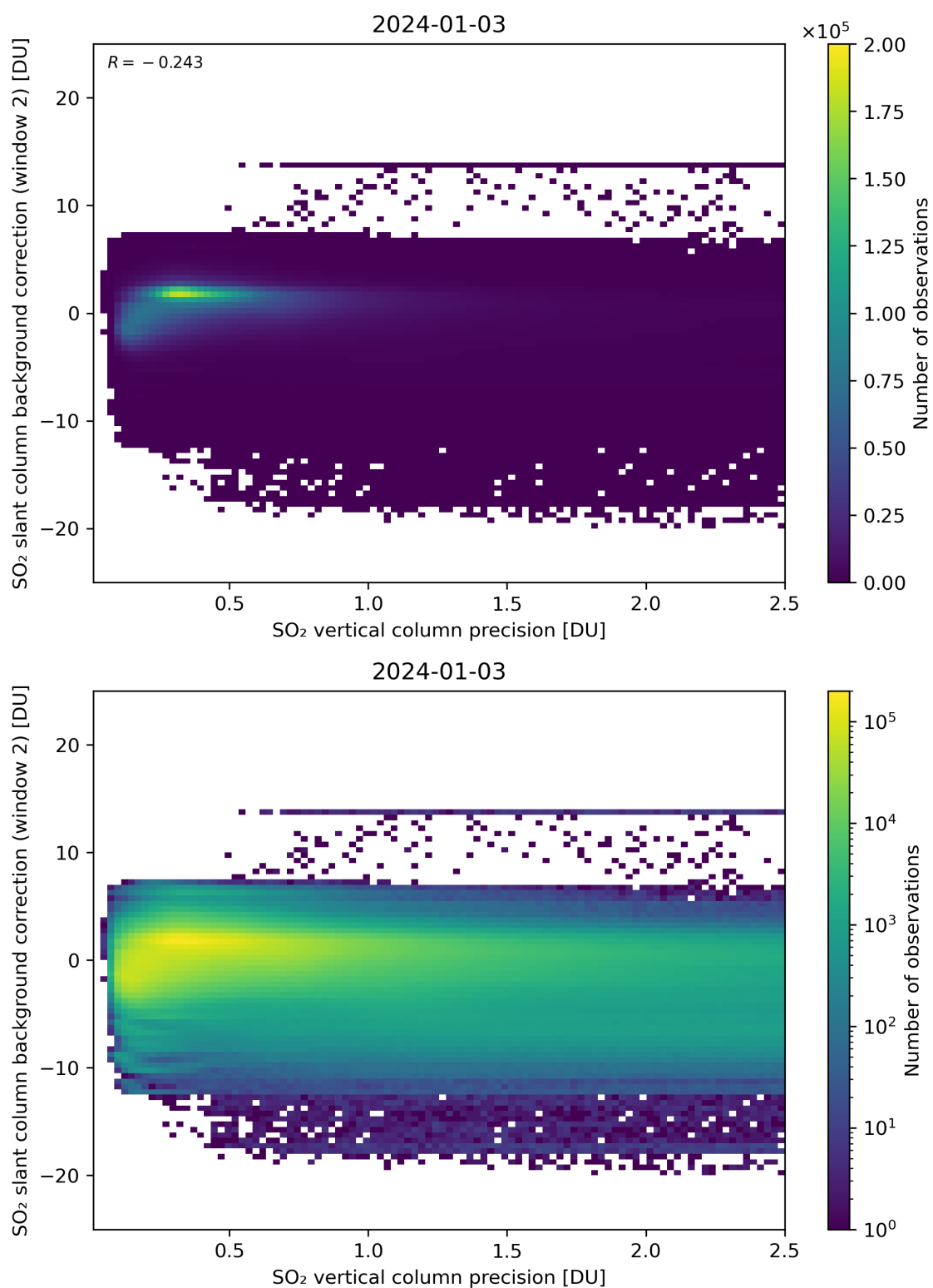
Figure 280: Scatter density plot of “SO 2 vertical column precision” against “SO 2 slant column background correction (window 2)” for 2024-01-02 to 2024-01-04.
