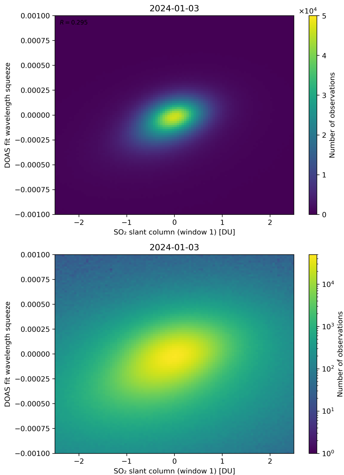
Figure 216: Scatter density plot of “SO 2 slant column (window 1)” against “DOAS fit wavelength squeeze” for 2024-01-02 to 2024-01-04.
