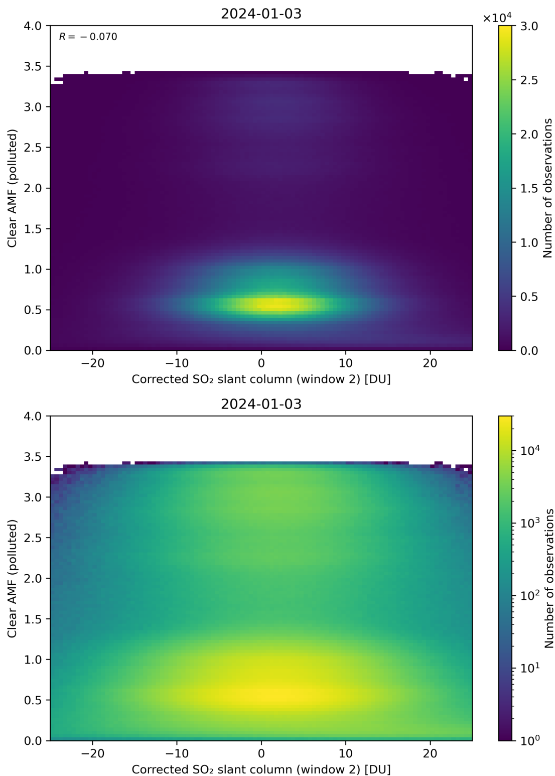
Figure 199: Scatter density plot of “Corrected SO 2 slant column (window 2)” against “Clear AMF (polluted)” for 2024-01-02 to 2024-01-04.
