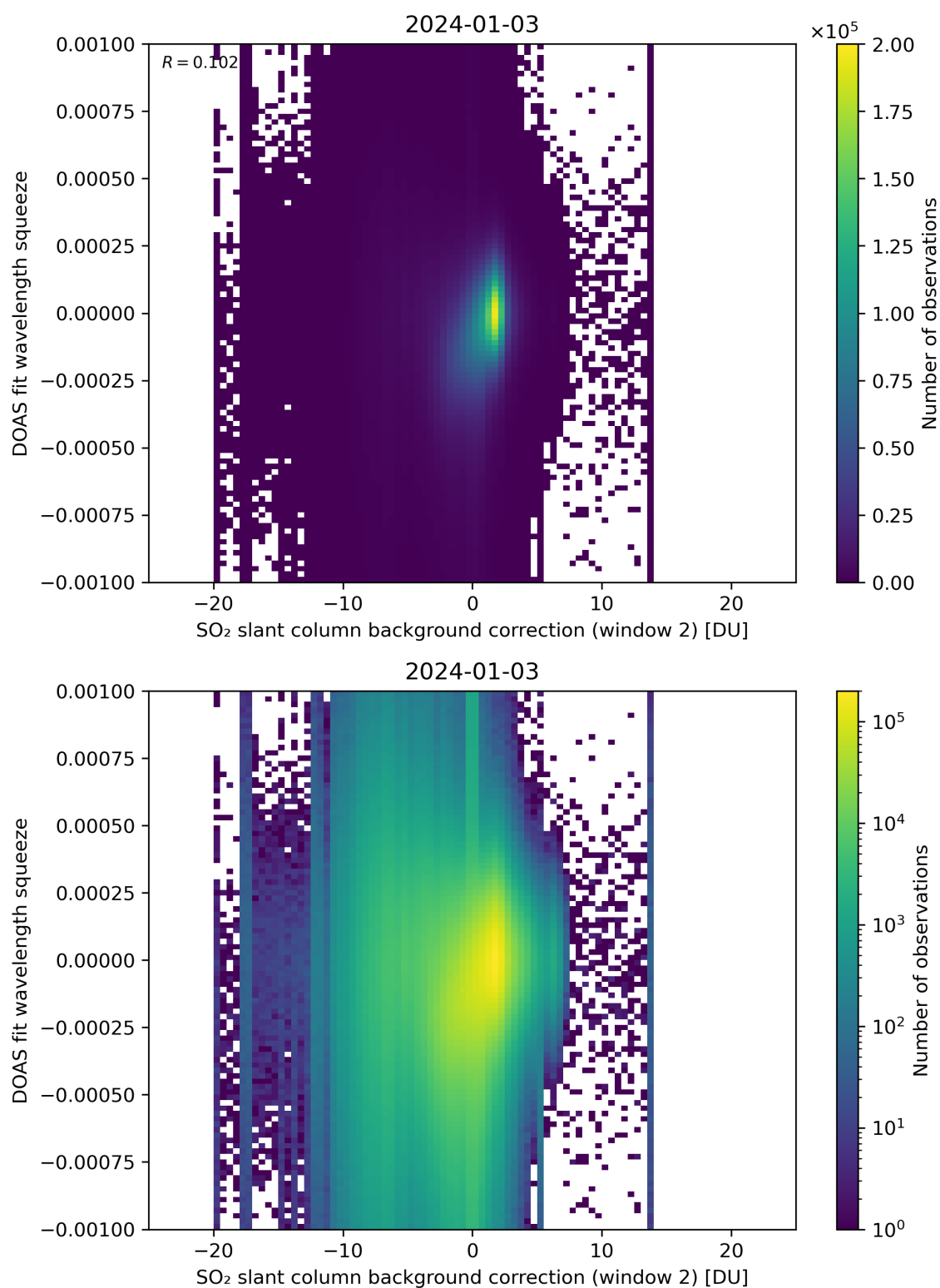
Figure 113: Scatter density plot of “SO 2 slant column background correction (window 2)” against “DOAS fit wavelength squeeze” for 2024-01-02 to 2024-01-04.
