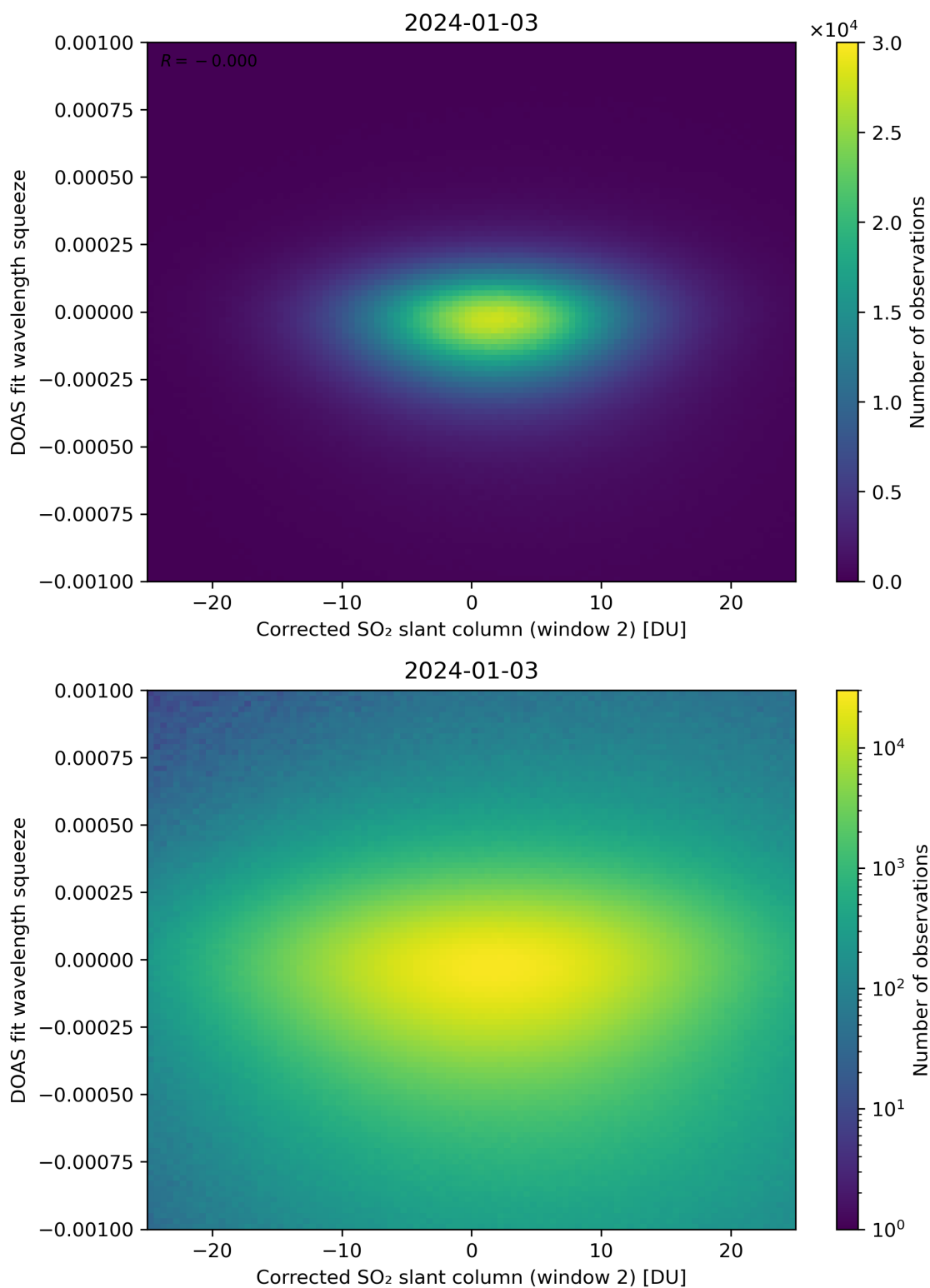
Figure 197: Scatter density plot of “Corrected SO 2 slant column (window 2)” against “DOAS fit wavelength squeeze” for 2024-01-02 to 2024-01-04.
