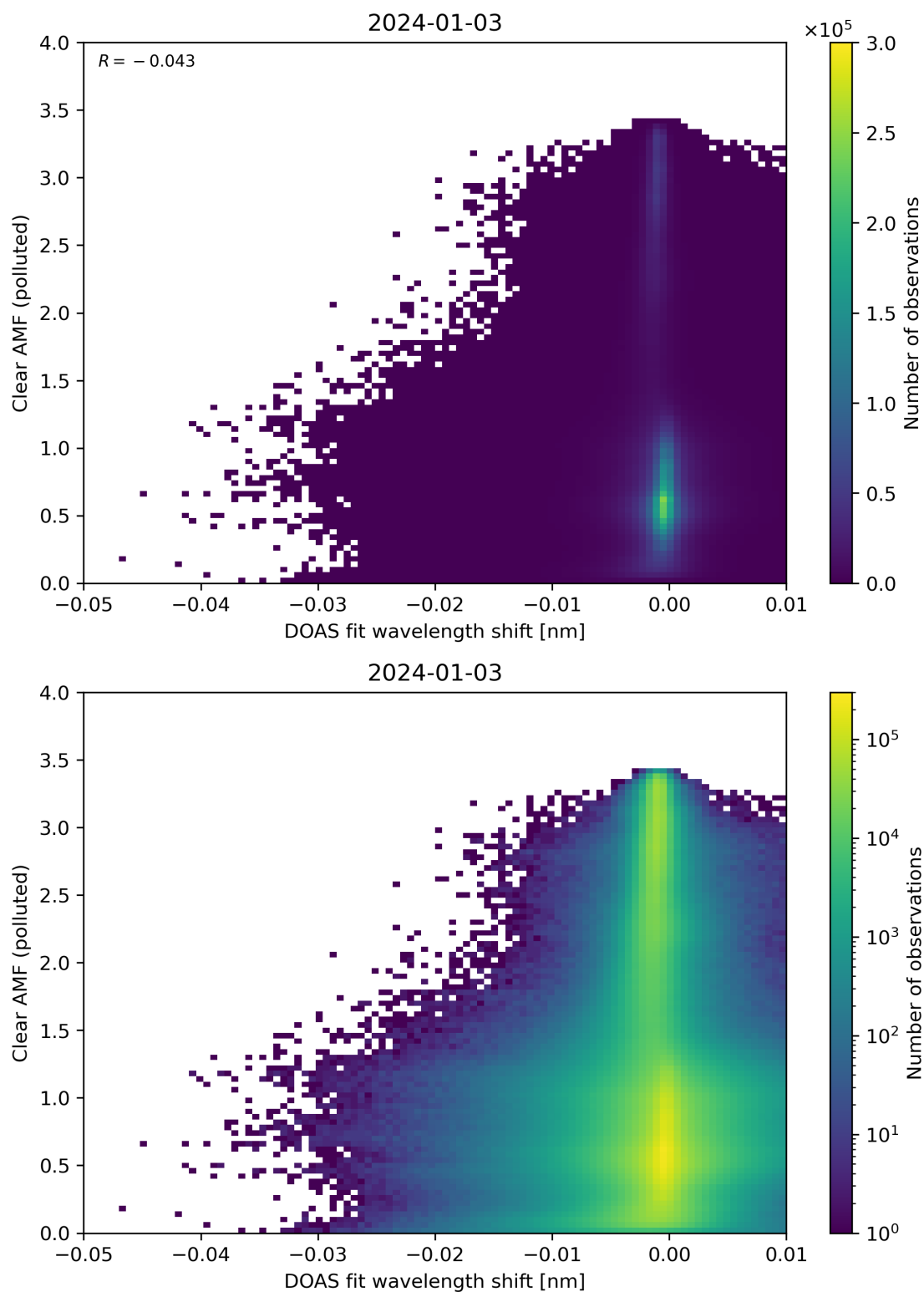
Figure 129: Scatter density plot of “DOAS fit wavelength shift” against “Clear AMF (polluted)” for 2024-01-02 to 2024-01-04.
