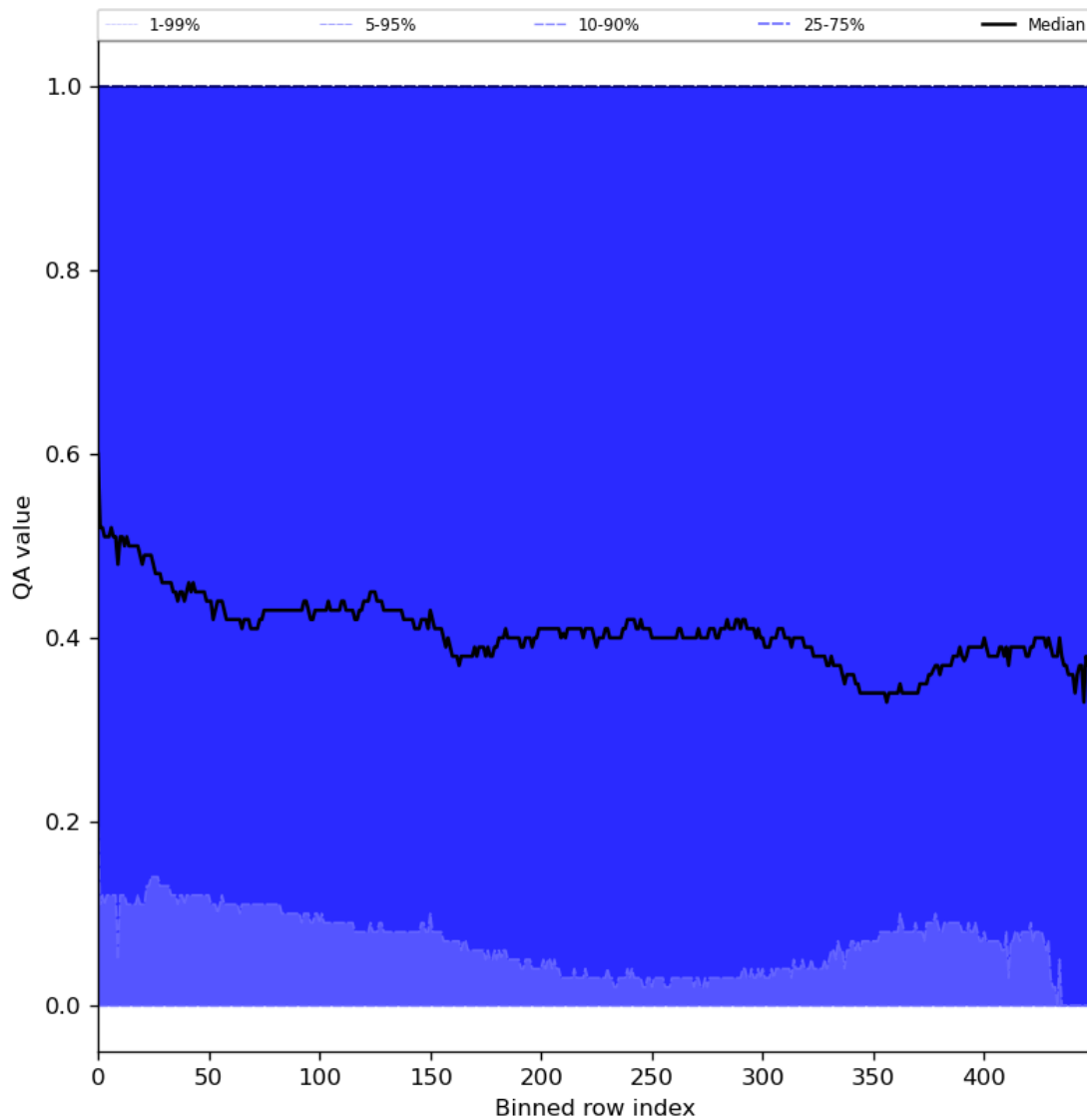
Figure 75: Along track statistics of “QA value” for 2024-01-02 to 2024-01-04
