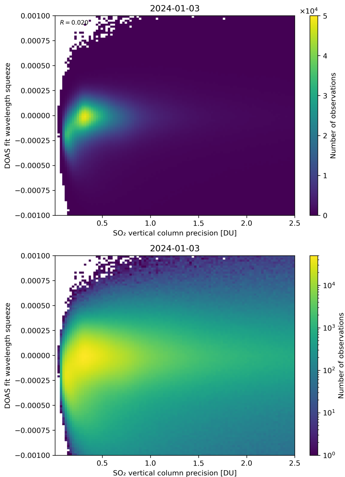
Figure 283: Scatter density plot of “SO 2 vertical column precision” against “DOAS fit wavelength squeeze” for 2024-01-02 to 2024-01-04.
