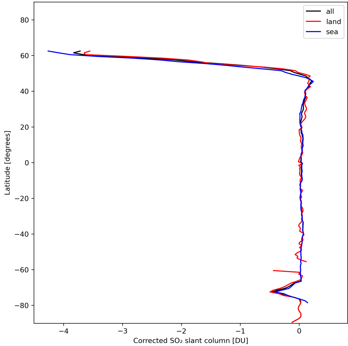
Figure 32: Zonal average of “Corrected SO 2 slant column” for 2024-01-02 to 2024-01-04.
