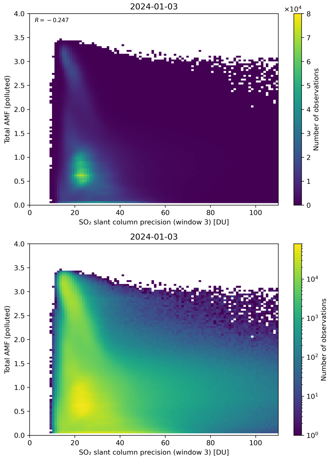
Figure 263: Scatter density plot of “SO 2 slant column precision (window 3)” against “Total AMF (polluted)” for 2024-01-02 to 2024-01-04.
