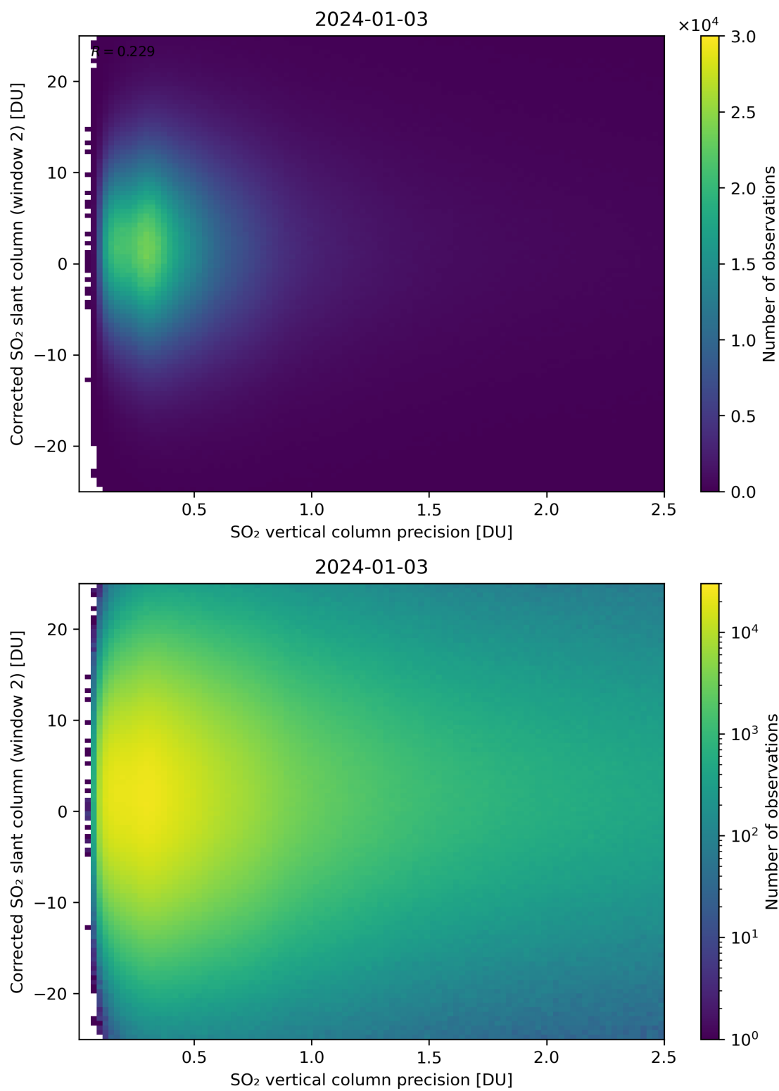
Figure 287: Scatter density plot of “SO 2 vertical column precision” against “Corrected SO 2 slant column (window 2)” for 2024-01-02 to 2024-01-04.
