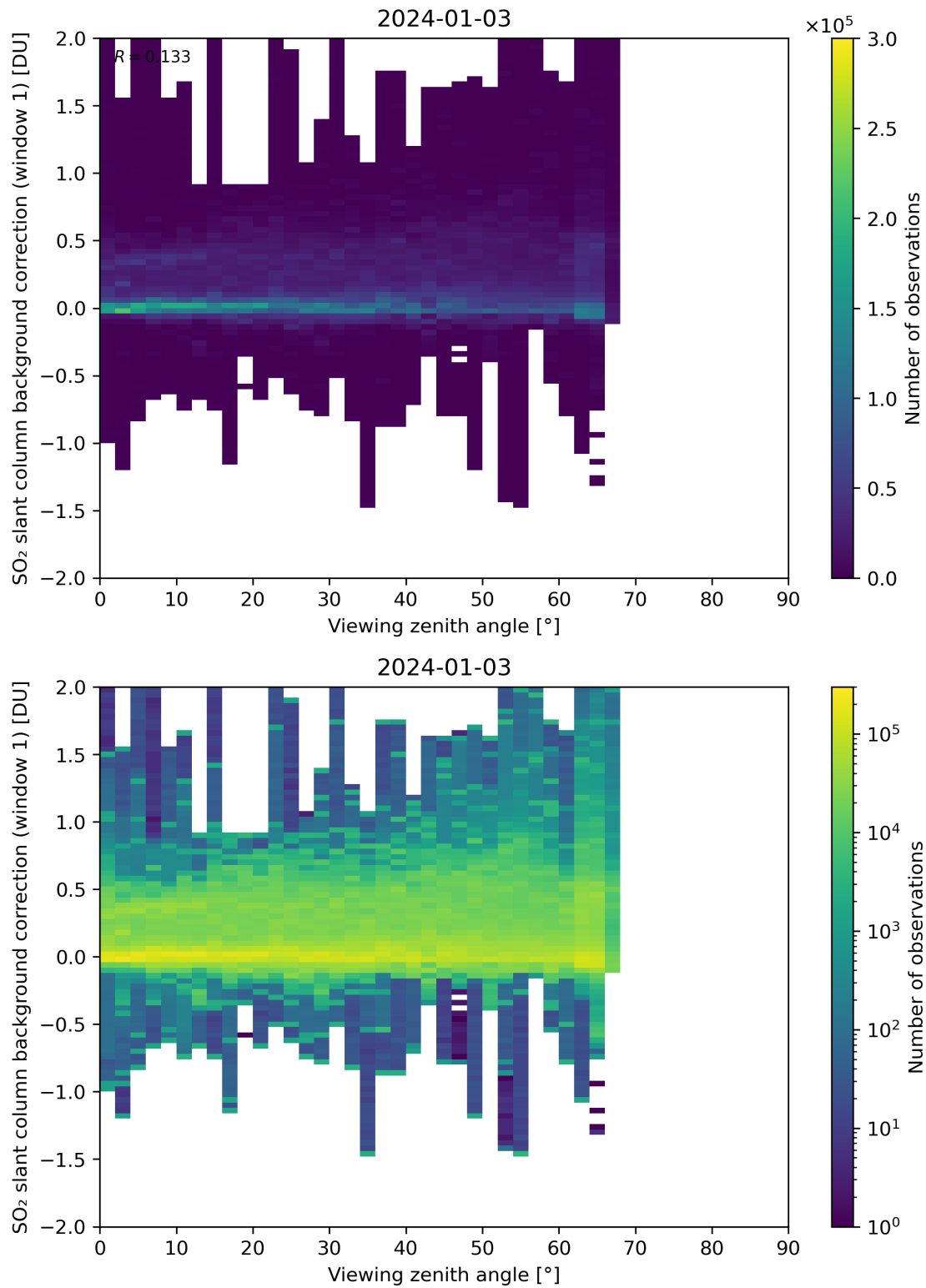
Figure 308: Scatter density plot of “Viewing zenith angle” against “SO 2 slant column background correction (window 1)” for 2024-01-02 to 2024-01-04.
