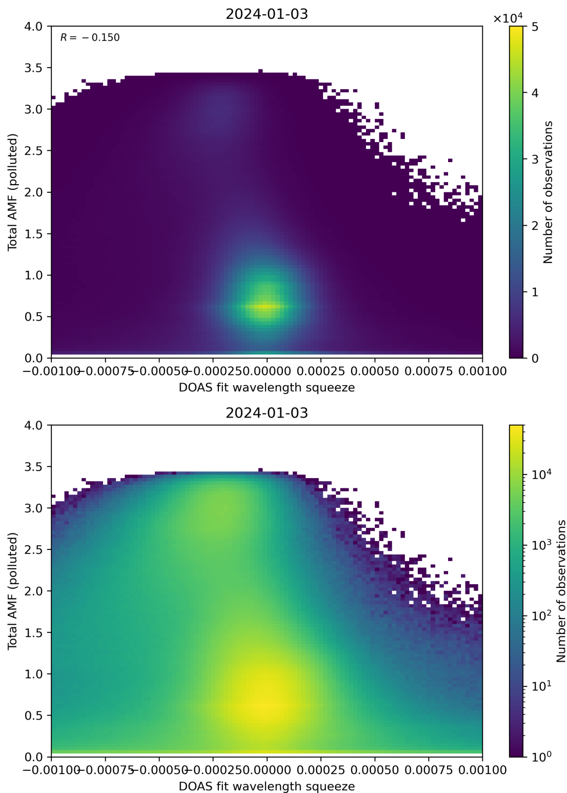
Figure 134: Scatter density plot of “DOAS fit wavelength squeeze” against “Total AMF (polluted)” for 2024-01-02 to 2024-01-04.
