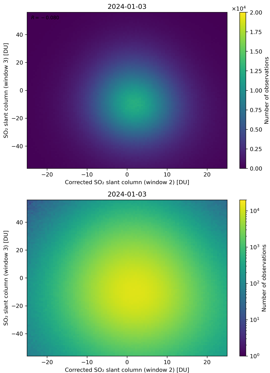
Figure 201: Scatter density plot of “Corrected SO 2 slant column (window 2)” against “SO 2 slant column (window 3)” for 2024-01-02 to 2024-01-04.
