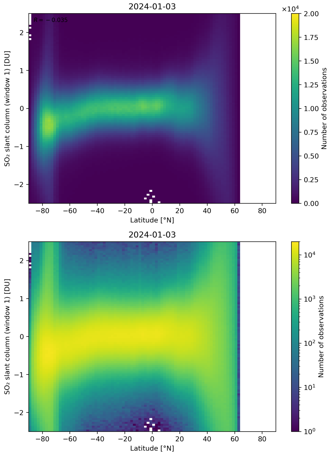
Figure 149: Scatter density plot of “Latitude” against “SO 2 slant column (window 1)” for 2024-01-02 to 2024-01-04.
