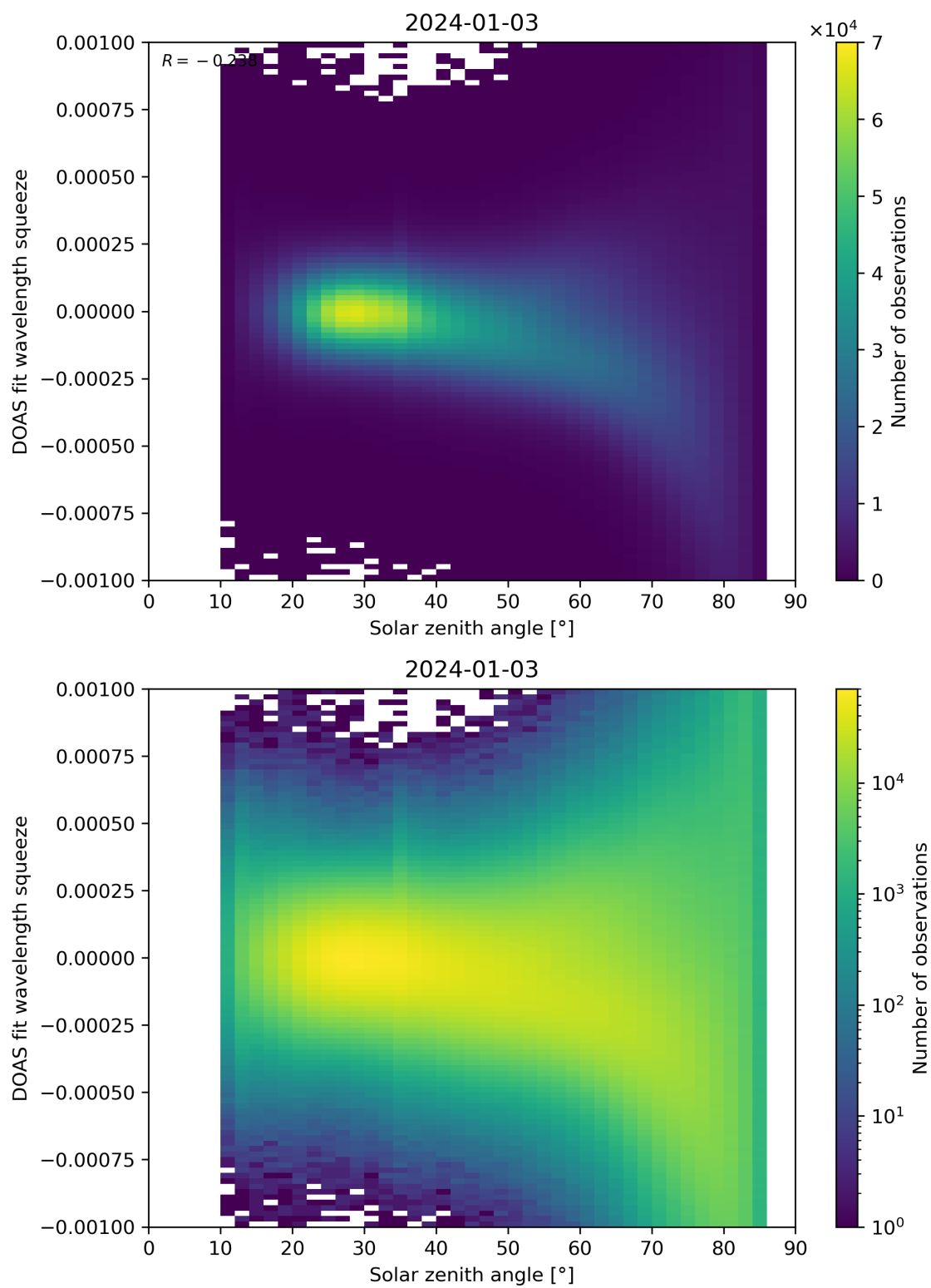
Figure 162: Scatter density plot of “Solar zenith angle” against “DOAS fit wavelength squeeze” for 2024-01-02 to 2024-01-04.
