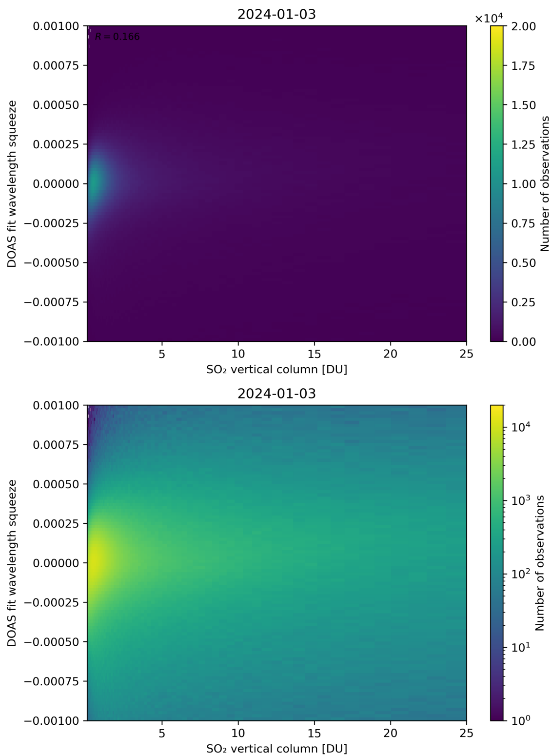
Figure 277: Scatter density plot of “SO 2 vertical column” against “DOAS fit wavelength squeeze” for 2024-01-02 to 2024-01-04.
