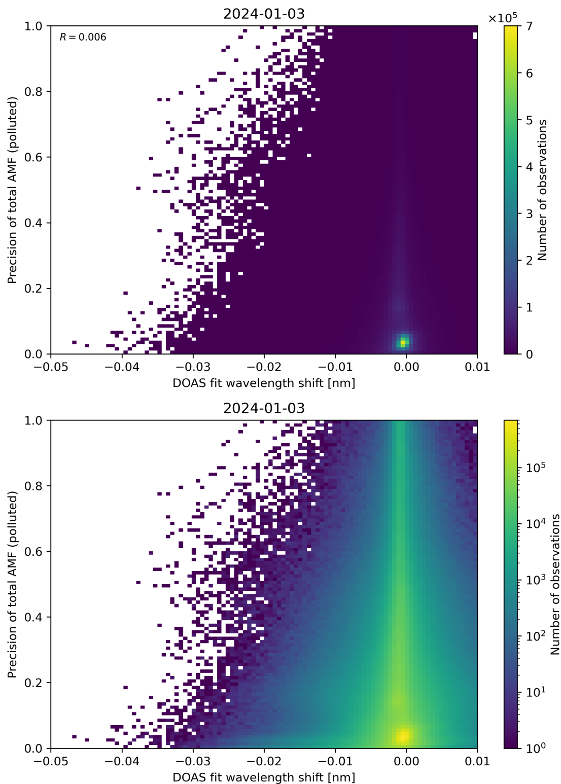
Figure 131: Scatter density plot of “DOAS fit wavelength shift” against “Precision of total AMF (polluted)” for 2024-01-02 to 2024-01-04.
