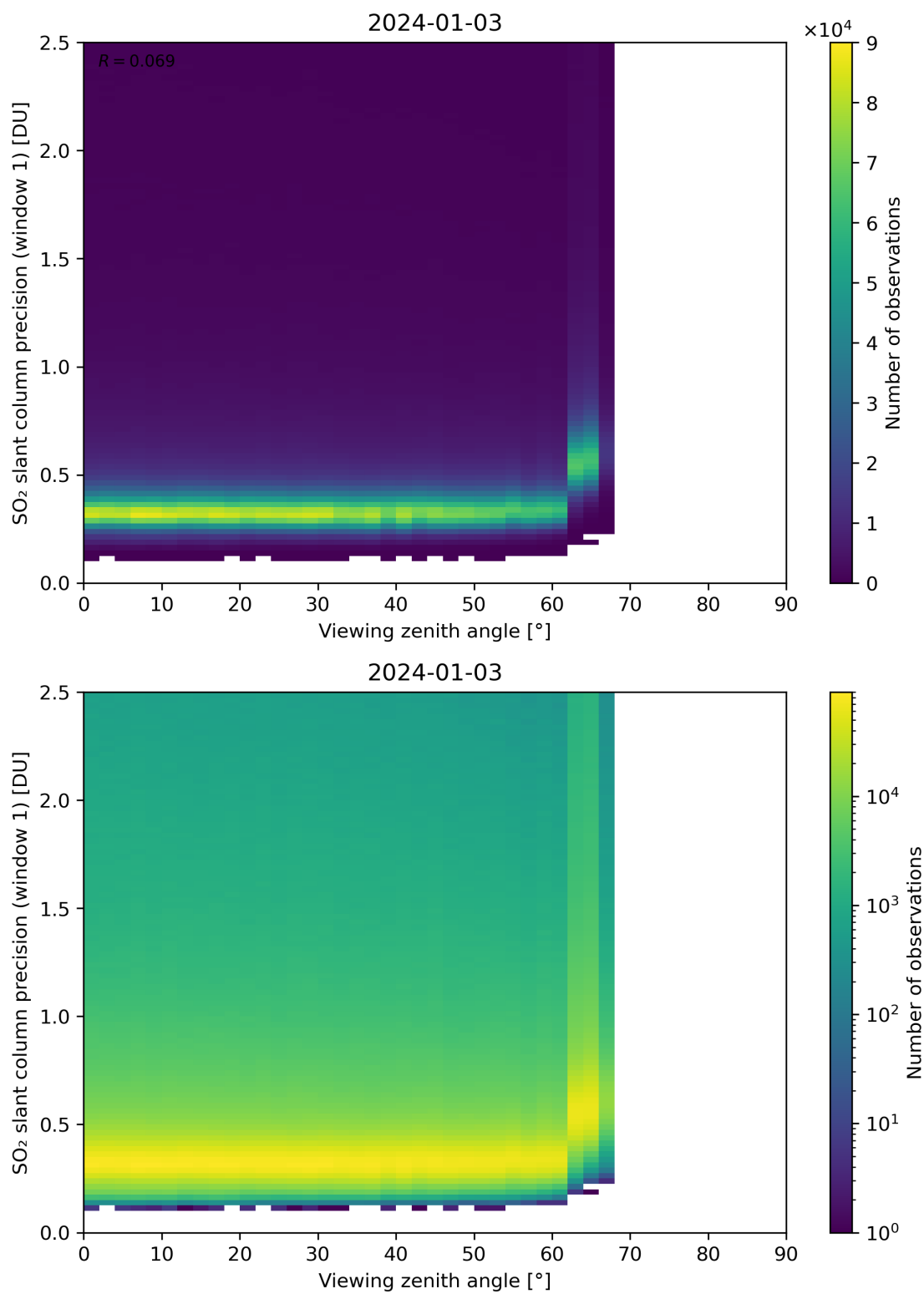
Figure 321: Scatter density plot of “Viewing zenith angle” against “SO 2 slant column precision (window 1)” for 2024-01-02 to 2024-01-04.
