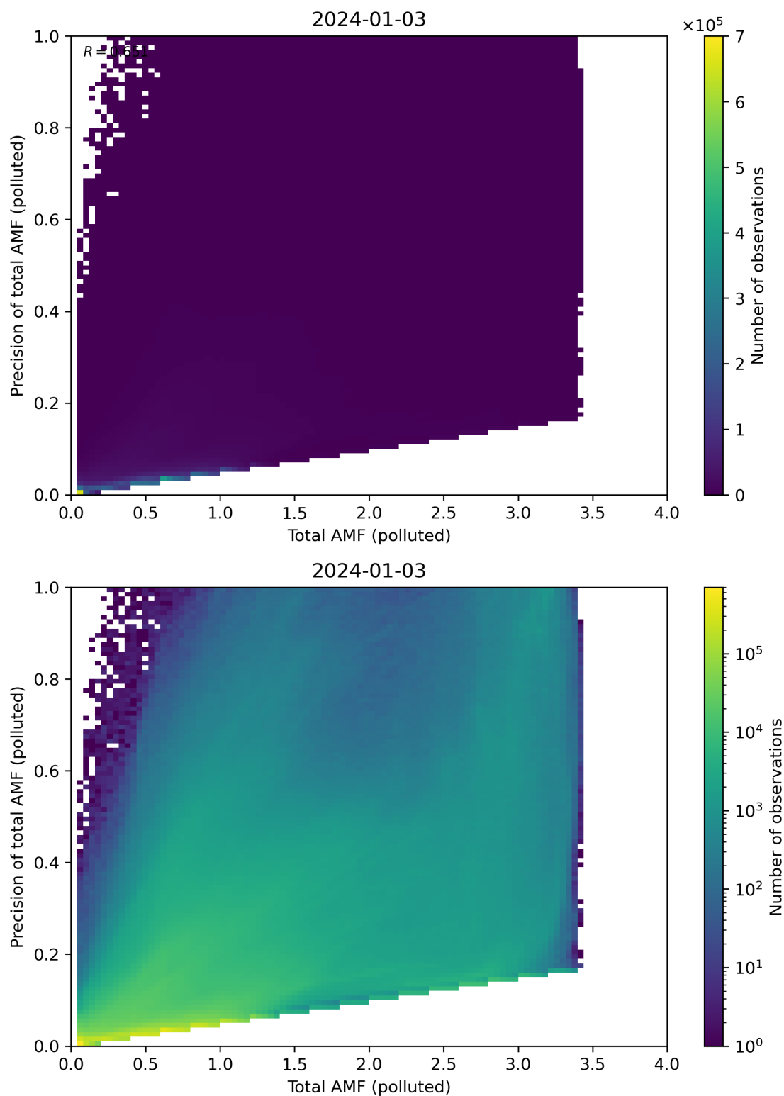
Figure 272: Scatter density plot of “Total AMF (polluted)” against “Precision of total AMF (polluted)” for 2024-01-02 to 2024-01-04.
