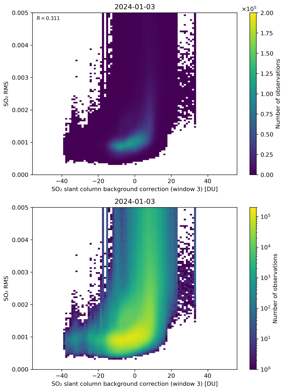
Figure 123: Scatter density plot of “SO 2 slant column background correction (window 3)” against “SO 2 RMS” for 2024-01-02 to 2024-01-04.
