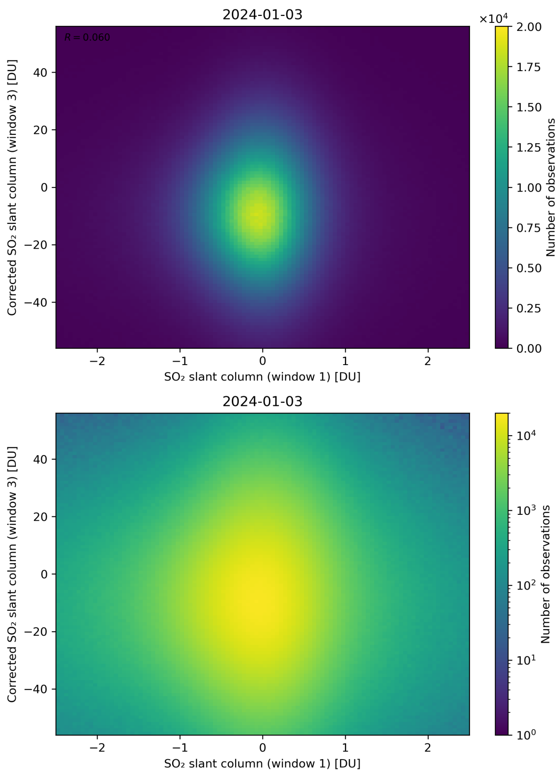
Figure 234: Scatter density plot of “SO 2 slant column (window 1)” against “Corrected SO 2 slant column (window 3)” for 2024-01-02 to 2024-01-04.
