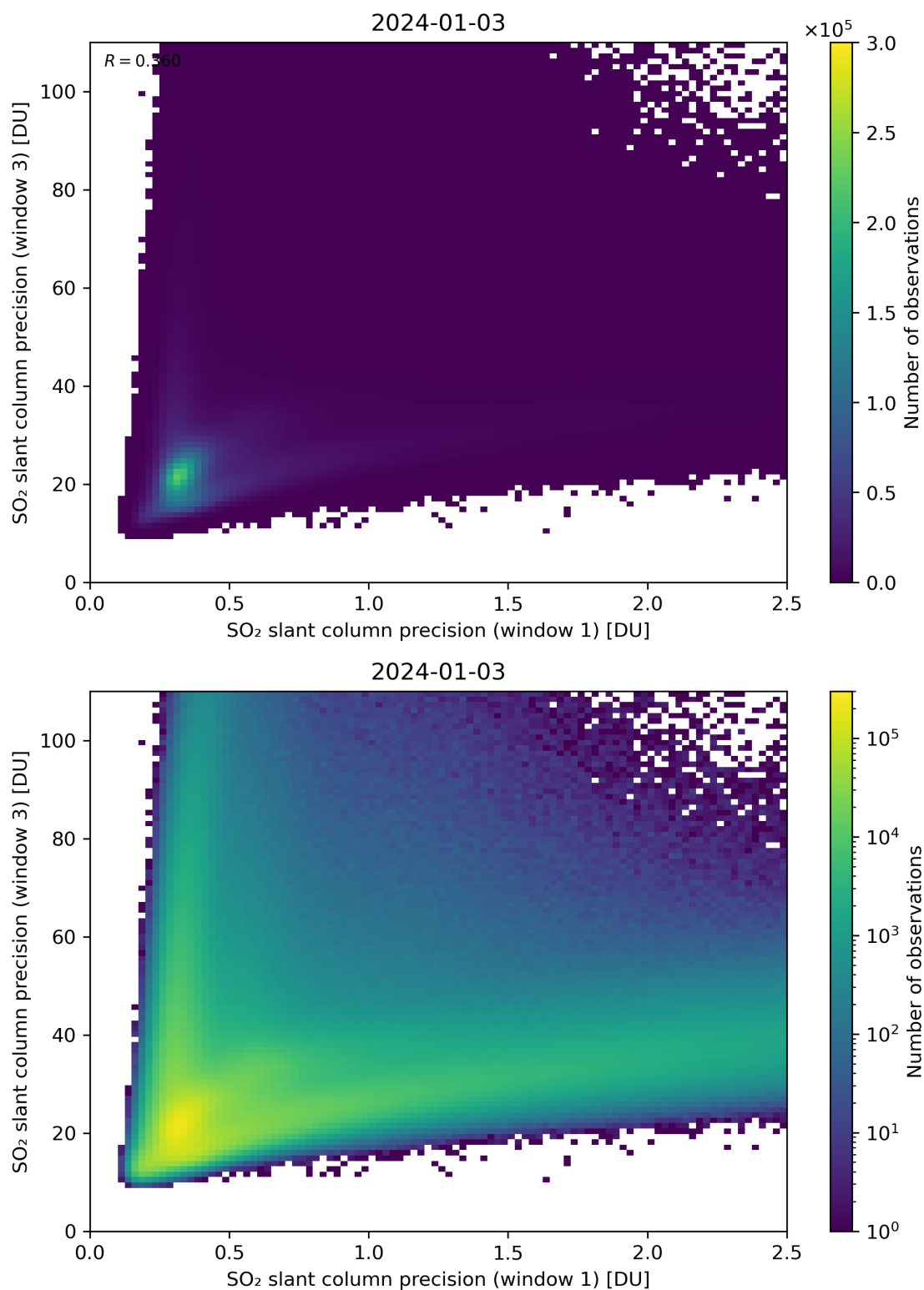
Figure 229: Scatter density plot of “SO 2 slant column precision (window 1)” against “SO 2 slant column precision (window 3)” for 2024-01-02 to 2024-01-04.
