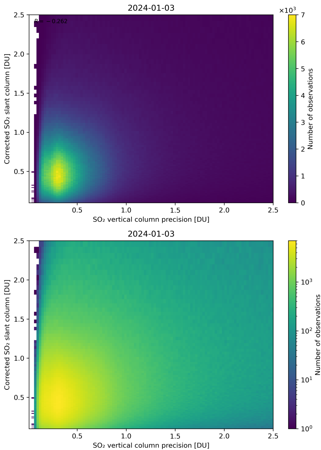
Figure 286: Scatter density plot of “SO 2 vertical column precision” against “Corrected SO 2 slant column” for 2024-01-02 to 2024-01-04.
