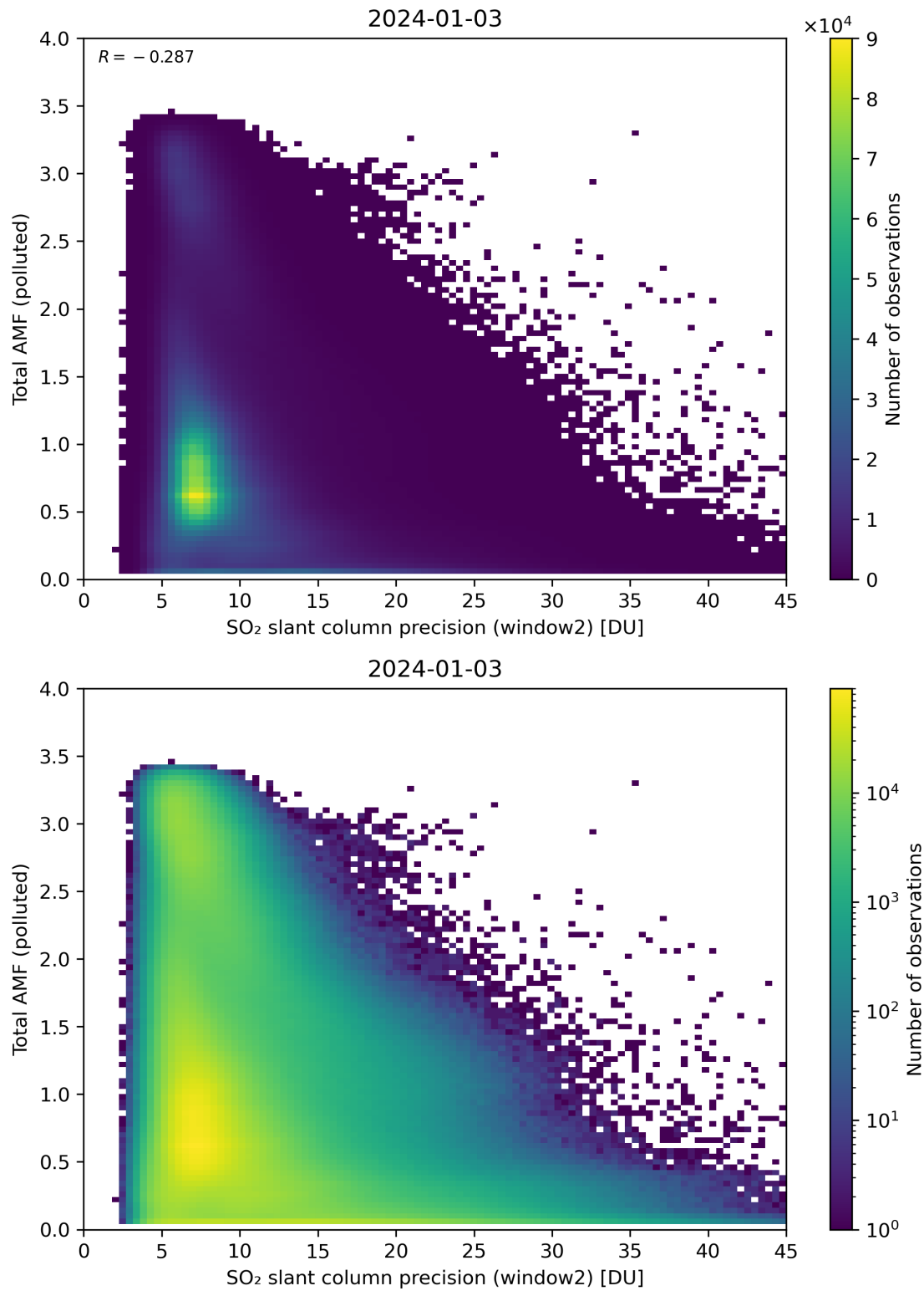
Figure 251: Scatter density plot of “SO 2 slant column precision (window2)” against “Total AMF (polluted)” for 2024-01-02 to 2024-01-04.
