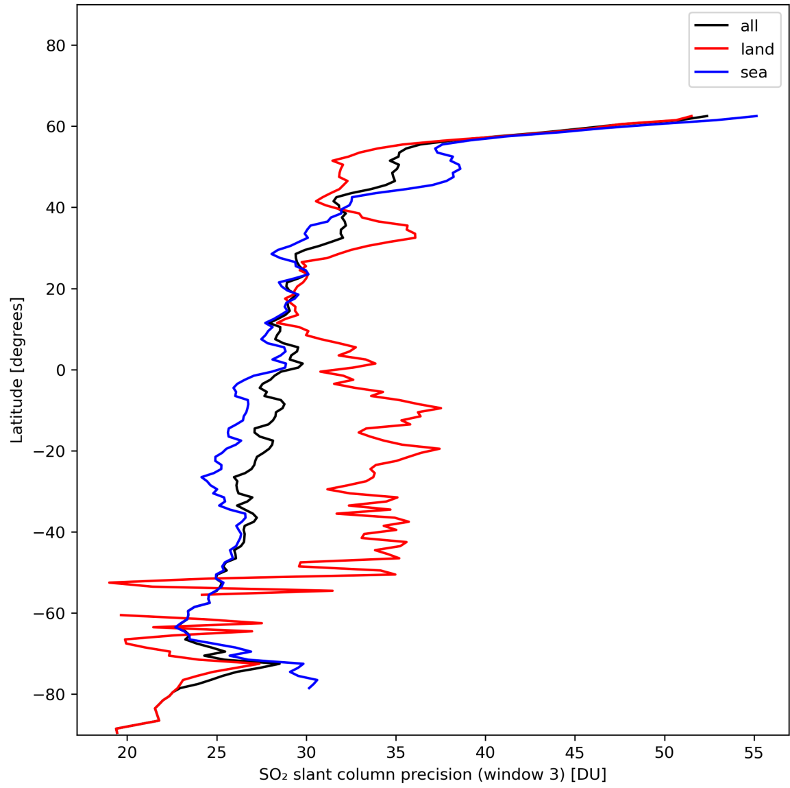
Figure 42: Zonal average of “SO 2 slant column precision (window 3)” for 2024-01-02 to 2024-01-04.
