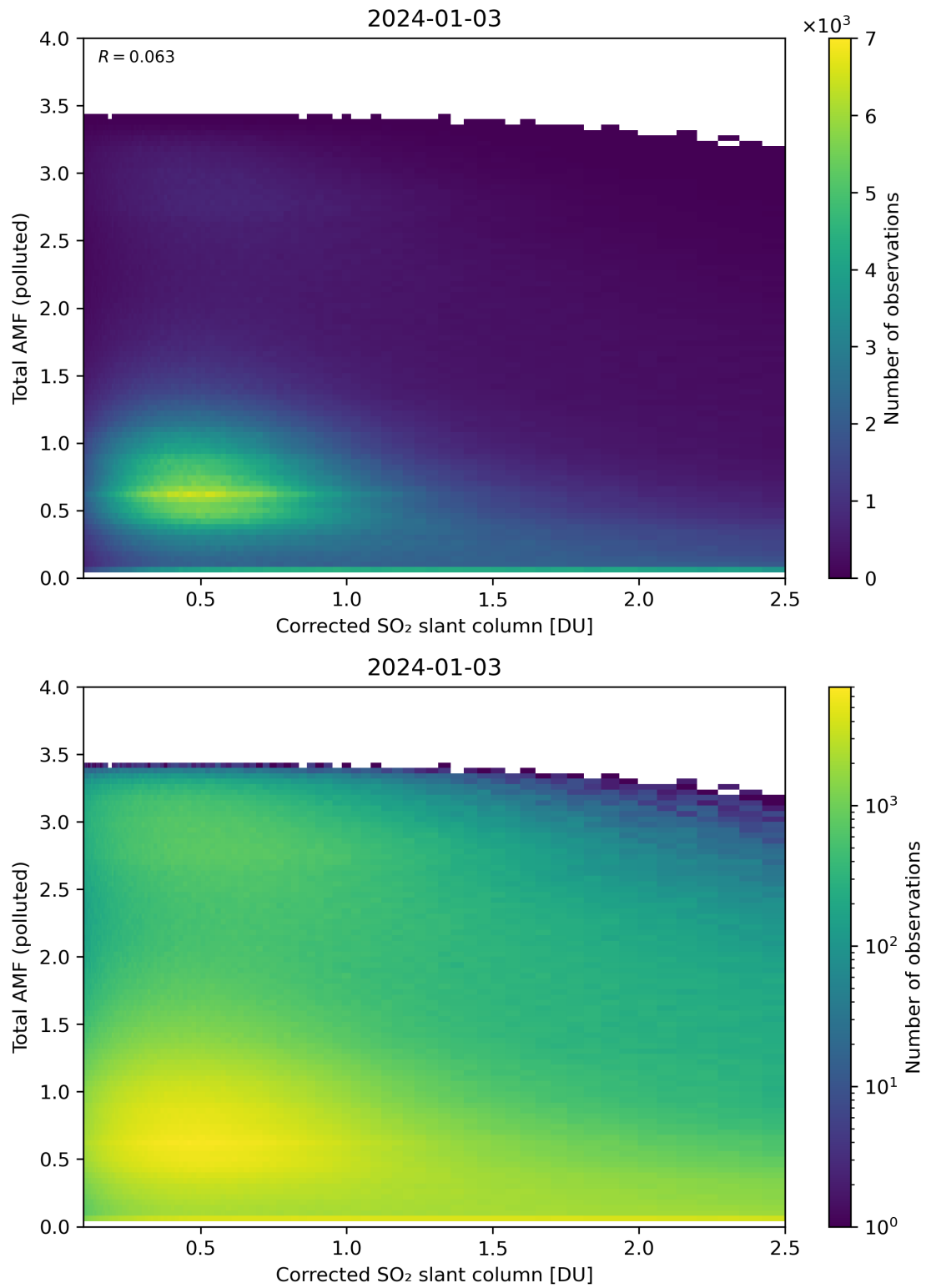
Figure 192: Scatter density plot of “Corrected SO 2 slant column” against “Total AMF (polluted)” for 2024-01-02 to 2024-01-04.
