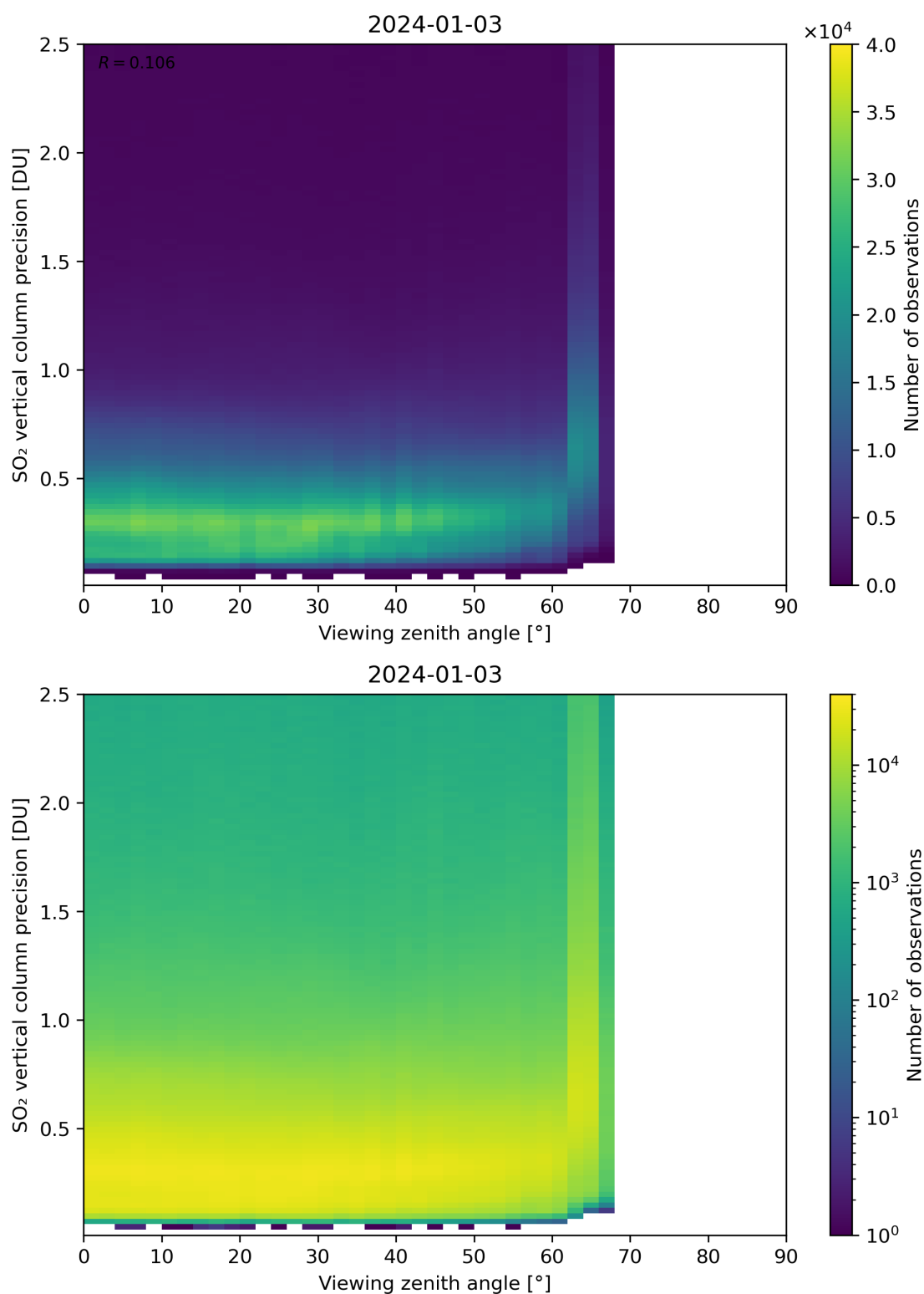
Figure 328: Scatter density plot of “Viewing zenith angle” against “SO 2 vertical column precision” for 2024-01-02 to 2024-01-04.
