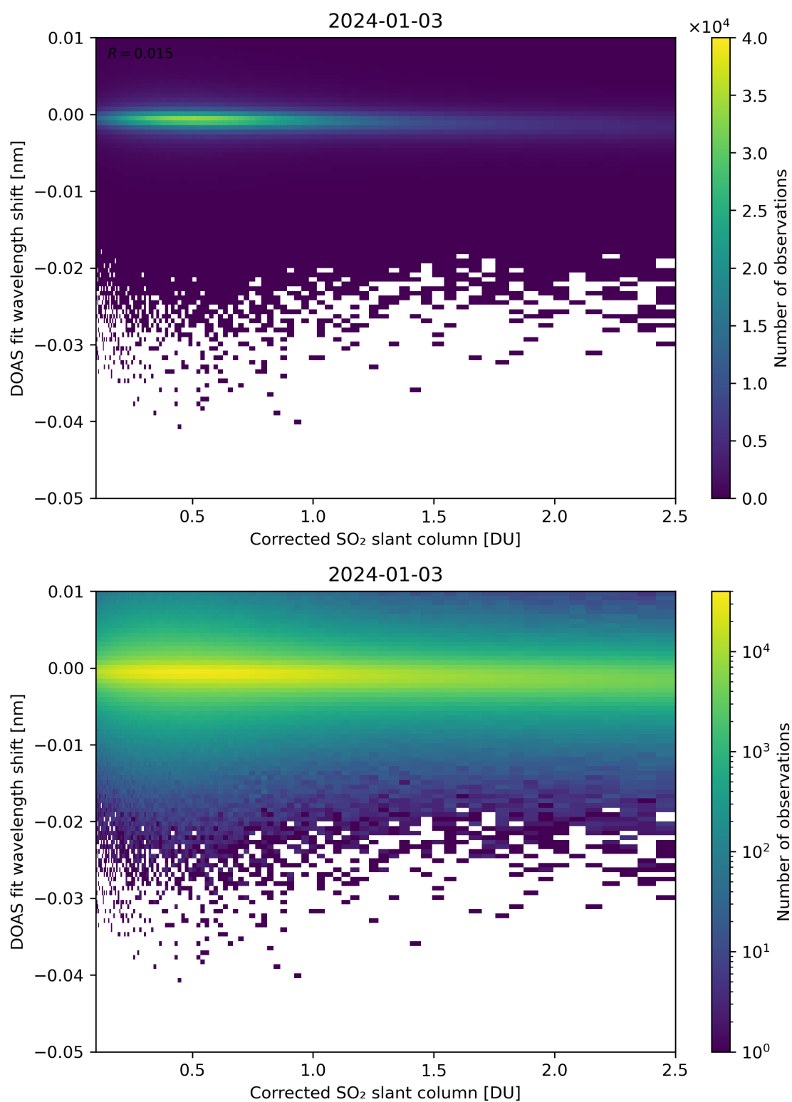
Figure 181: Scatter density plot of “Corrected SO 2 slant column” against “DOAS fit wavelength shift” for 2024-01-02 to 2024-01-04.
