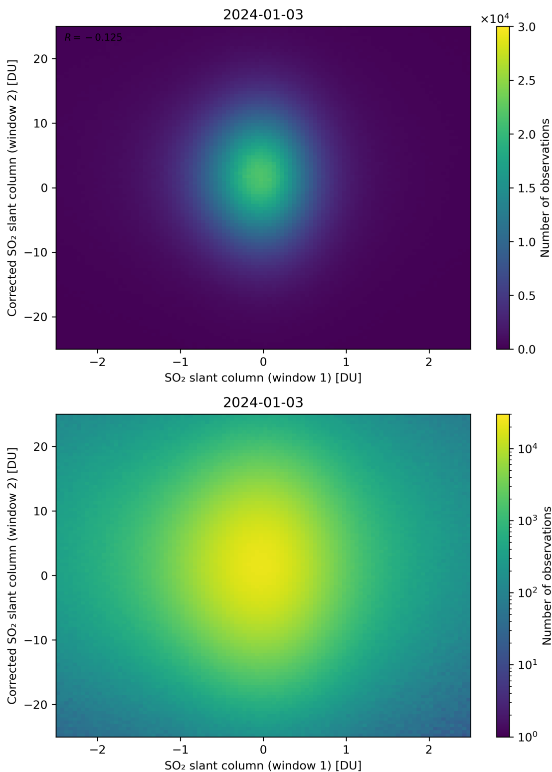
Figure 233: Scatter density plot of “SO 2 slant column (window 1)” against “Corrected SO 2 slant column (window 2)” for 2024-01-02 to 2024-01-04.
