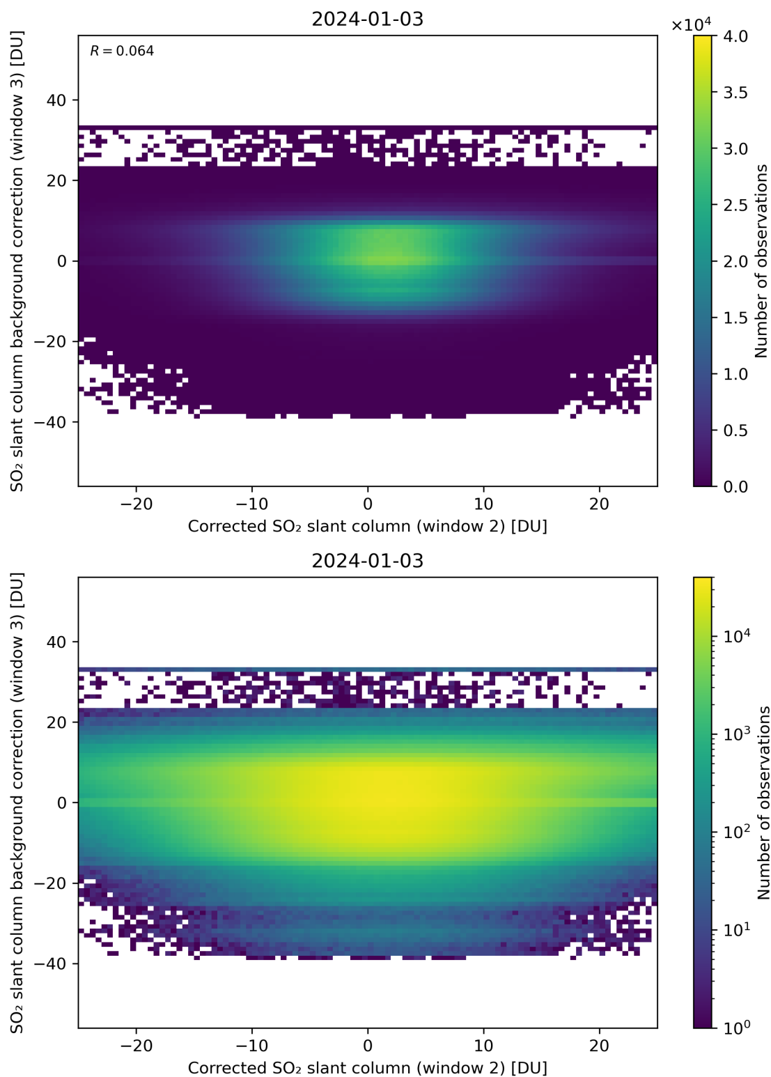
Figure 195: Scatter density plot of “Corrected SO 2 slant column (window 2)” against “SO 2 slant column background correction (window 3)” for 2024-01-02 to 2024-01-04.
