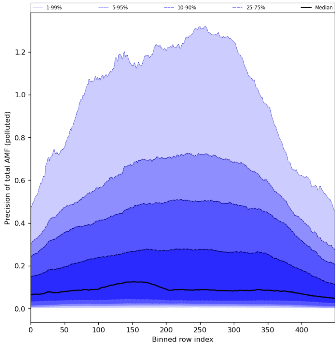
Figure 95: Along track statistics of “Precision of total AMF (polluted)” for 2024-01-02 to 2024-01-04
