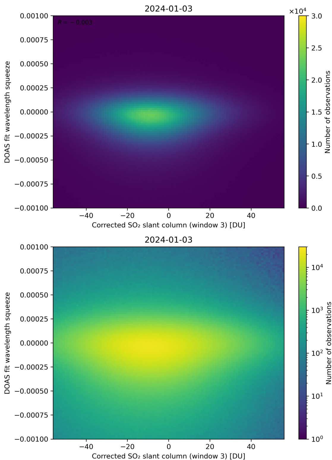
Figure 207: Scatter density plot of “Corrected SO 2 slant column (window 3)” against “DOAS fit wavelength squeeze” for 2024-01-02 to 2024-01-04.
