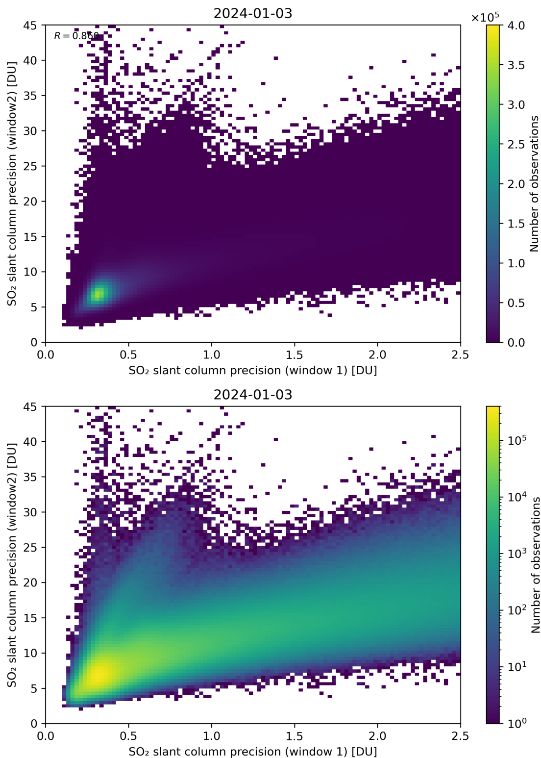
Figure 227: Scatter density plot of “SO 2 slant column precision (window 1)” against “SO 2 slant column precision (window 2)” for 2024-01-02 to 2024-01-04.
