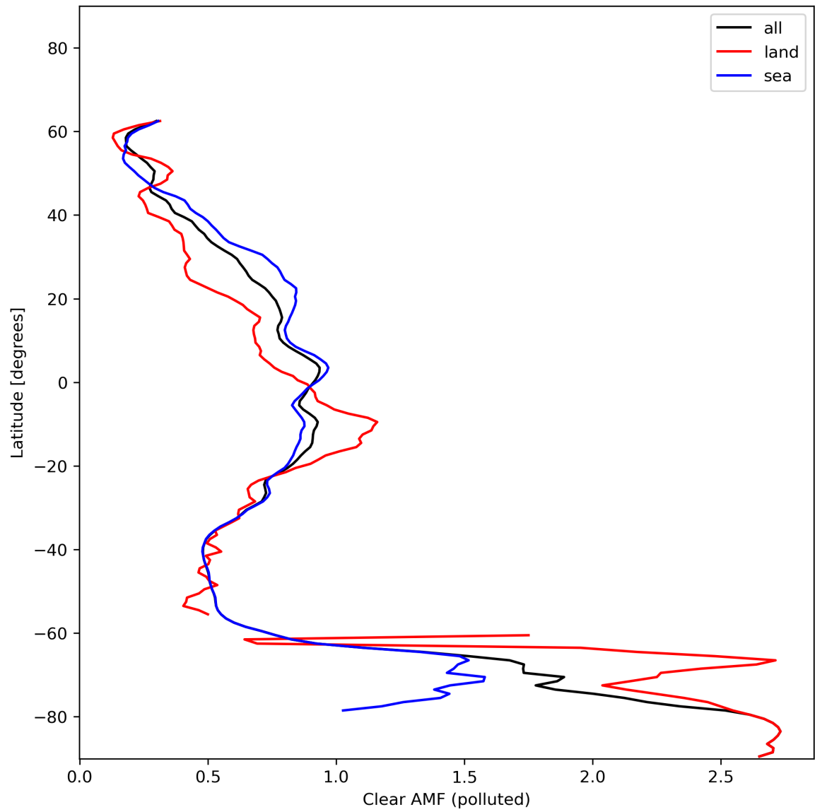
Figure 50: Zonal average of “Clear AMF (polluted)” for 2024-01-02 to 2024-01-04.
