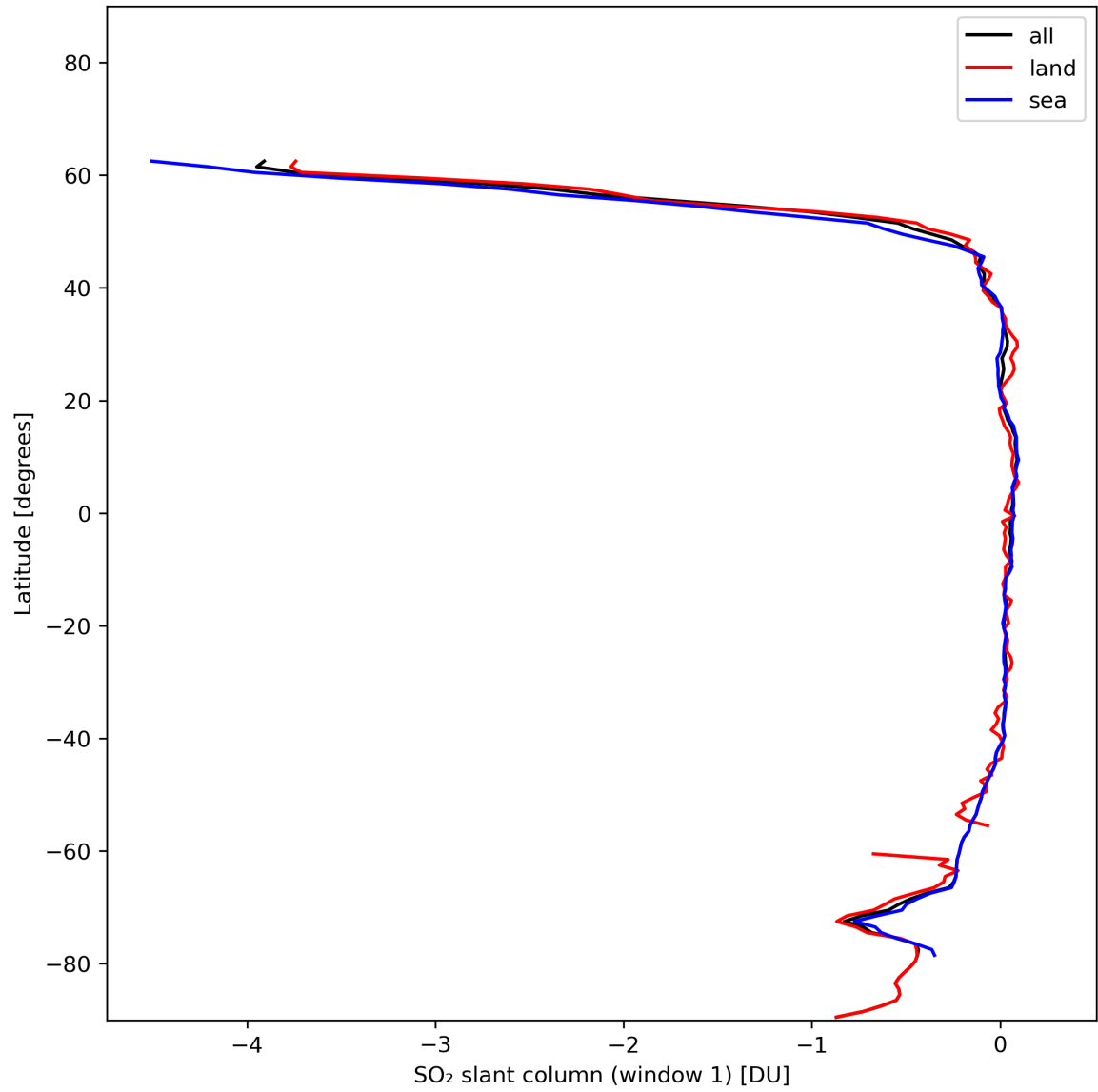
Figure 33: Zonal average of “SO 2 slant column (window 1)” for 2024-01-02 to 2024-01-04.
