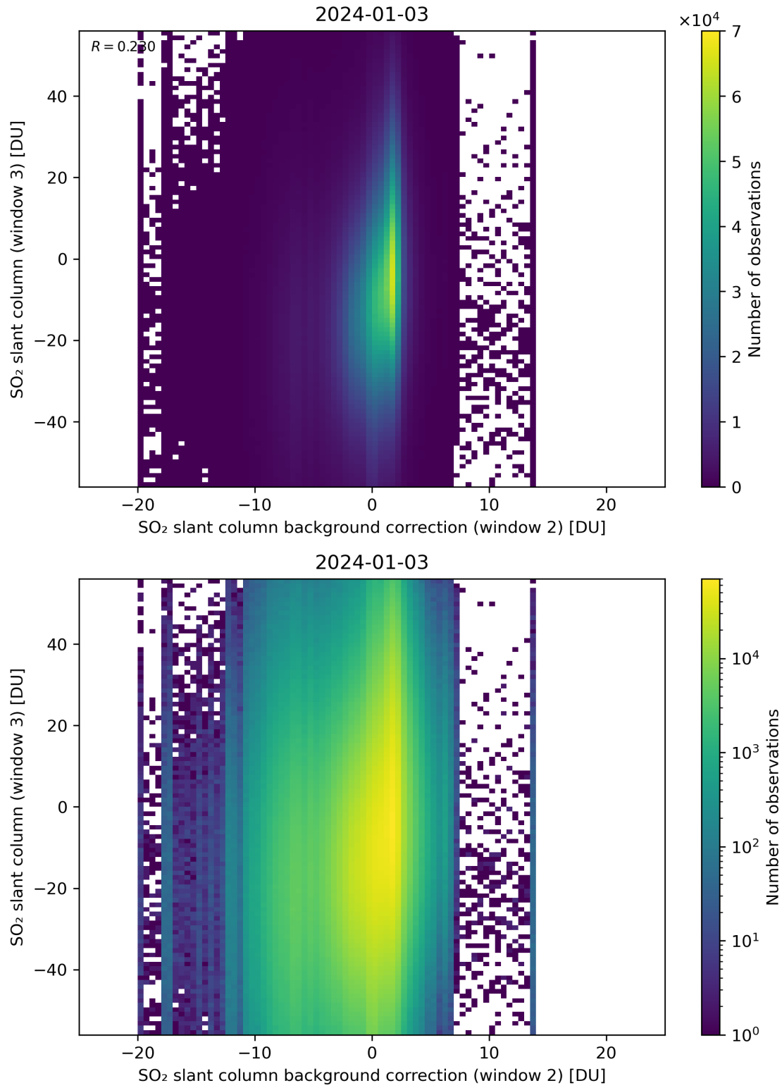
Figure 117: Scatter density plot of “SO 2 slant column background correction (window 2)” against “SO 2 slant column (window 3)” for 2024-01-02 to 2024-01-04.
