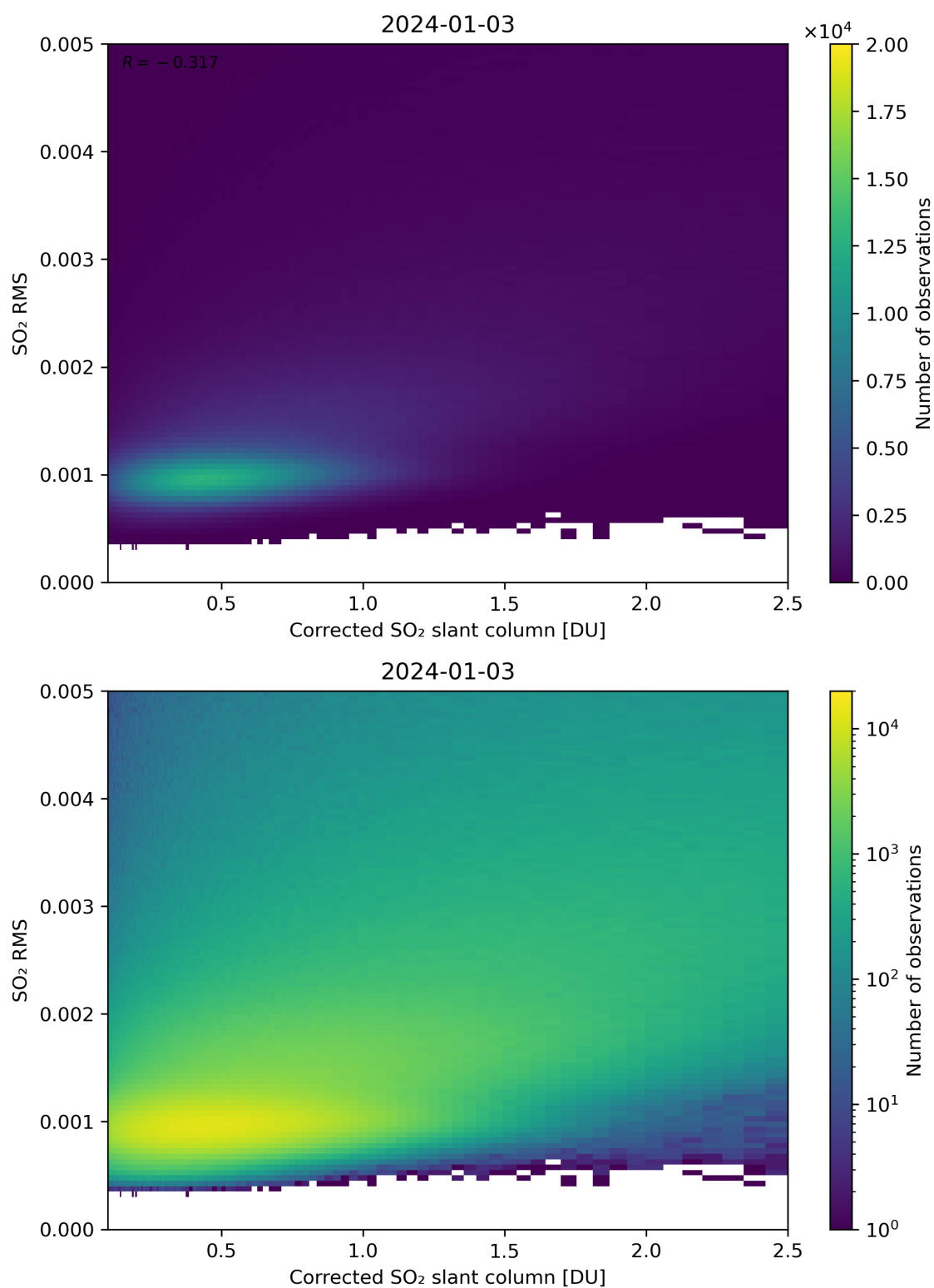
Figure 183: Scatter density plot of “Corrected SO 2 slant column” against “SO 2 RMS” for 2024-01-02 to 2024-01-04.
