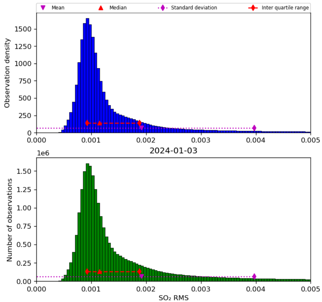
Figure 70: Histogram of “SO 2 RMS” for 2024-01-02 to 2024-01-04
