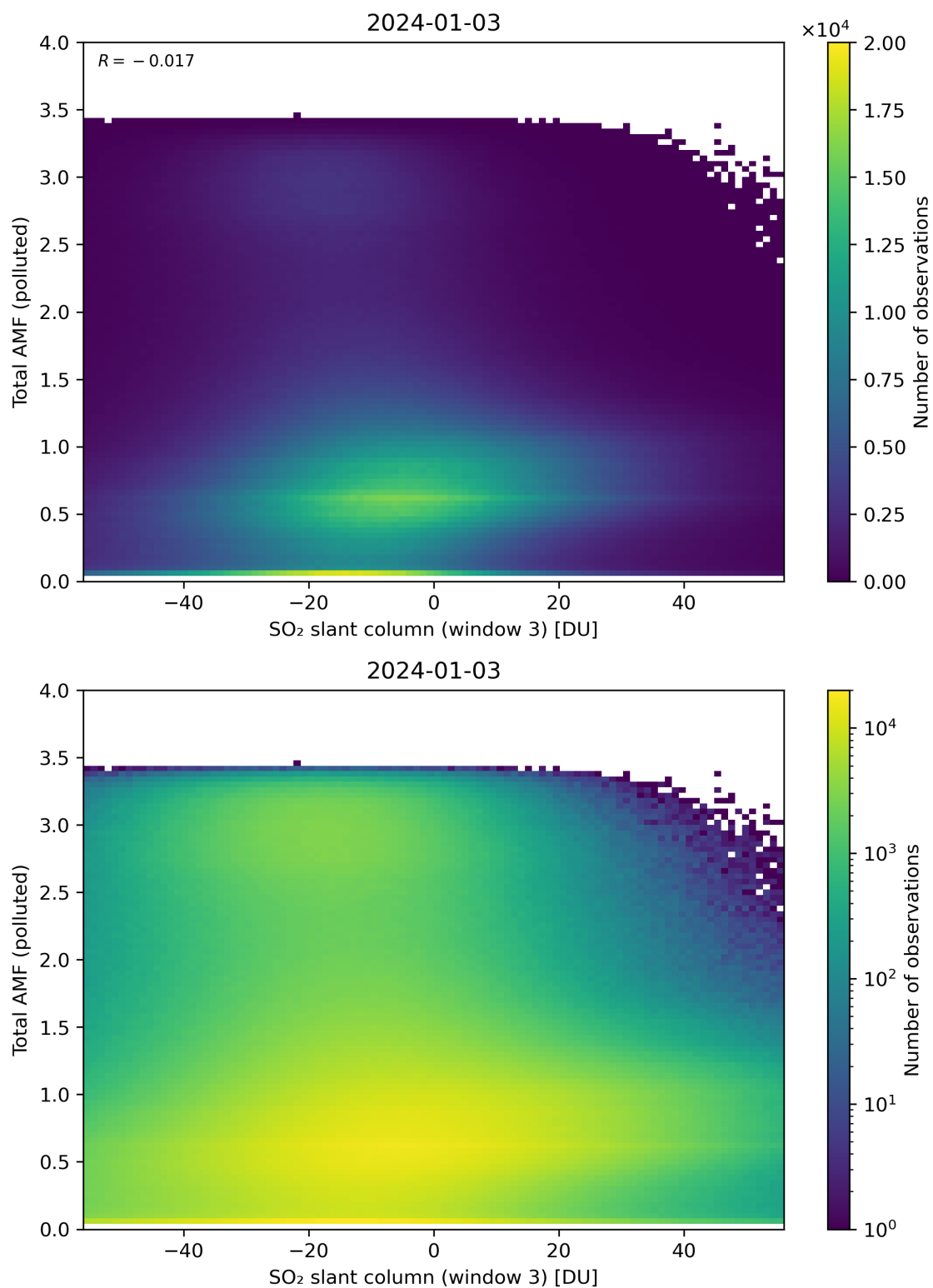
Figure 268: Scatter density plot of “SO 2 slant column (window 3)” against “Total AMF (polluted)” for 2024-01-02 to 2024-01-04.
