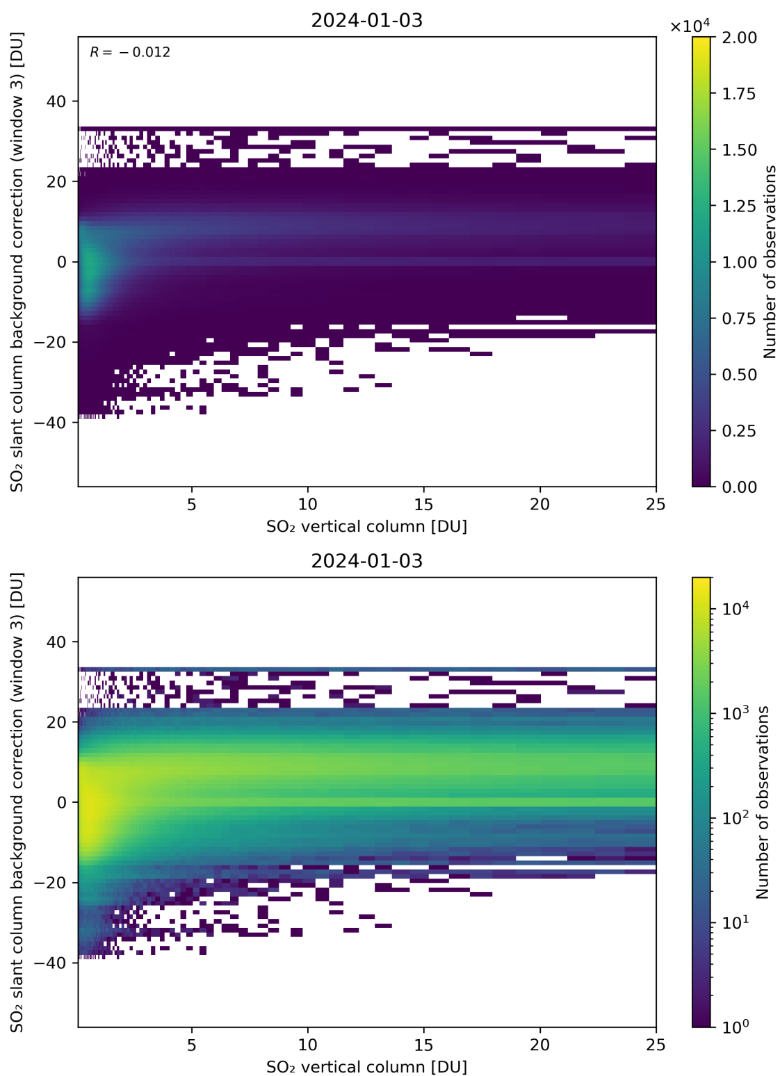
Figure 275: Scatter density plot of “SO 2 vertical column” against “SO 2 slant column background correction (window 3)” for 2024-01-02 to 2024-01-04.
