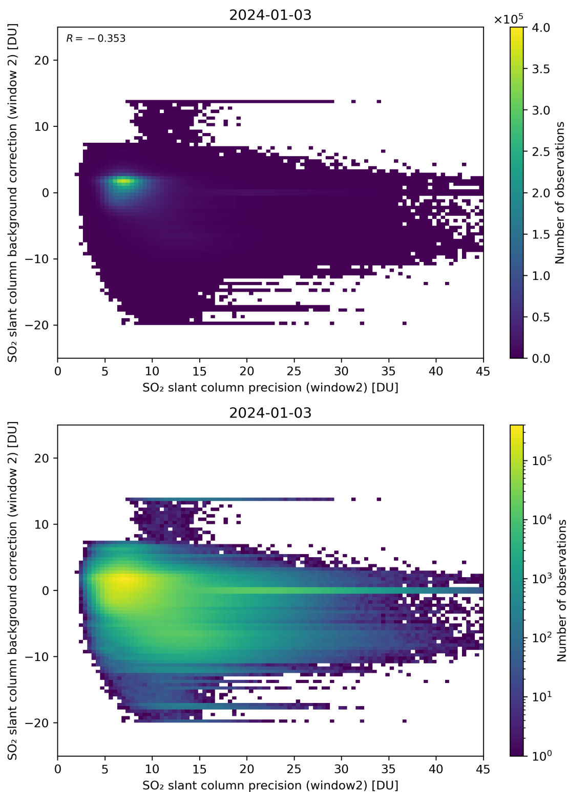
Figure 241: Scatter density plot of “SO 2 slant column precision (window2)” against “SO 2 slant column background correction (window 2)” for 2024-01-02 to 2024-01-04.
