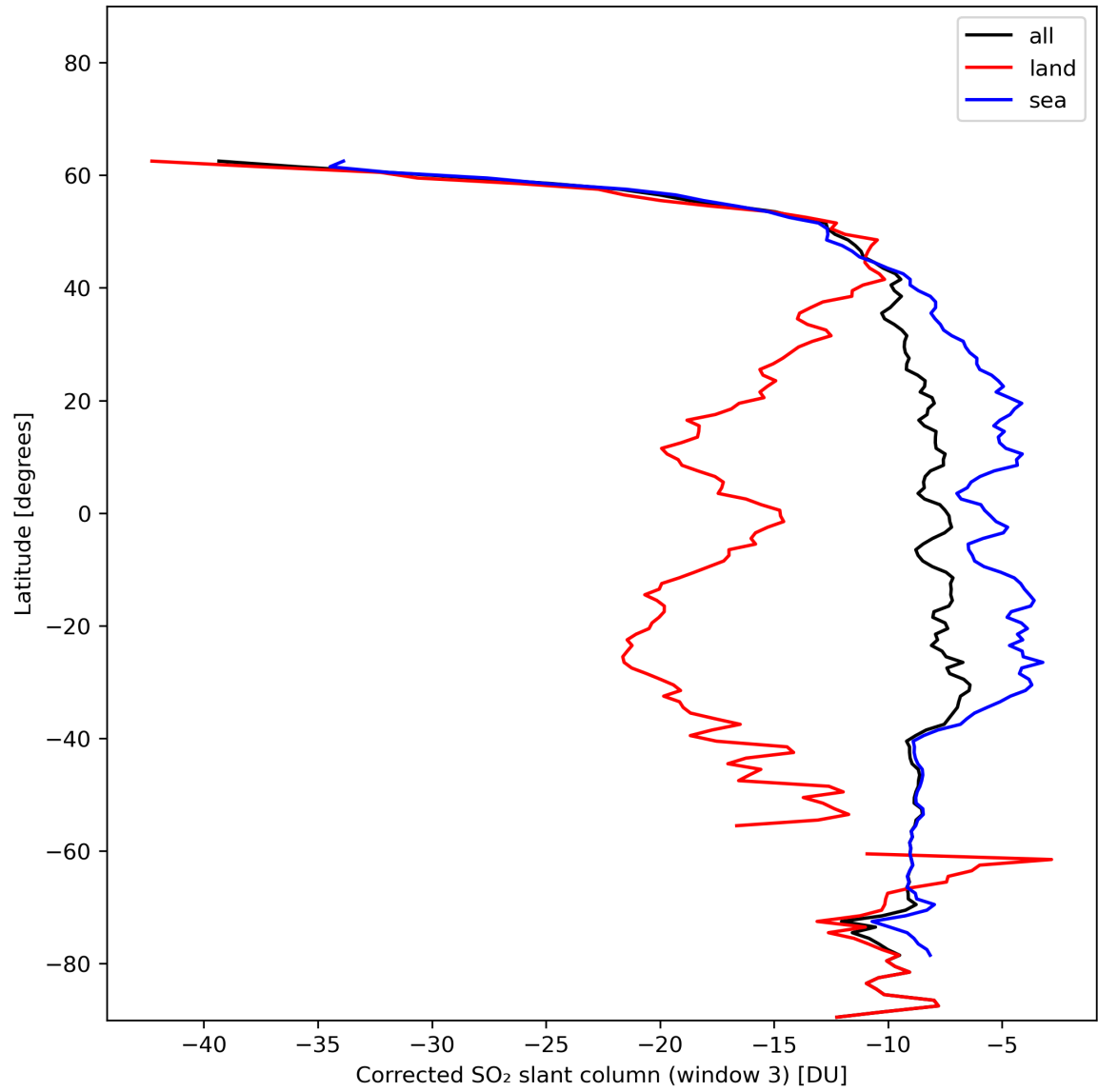
Figure 43: Zonal average of “Corrected SO 2 slant column (window 3)” for 2024-01-02 to 2024-01-04.
