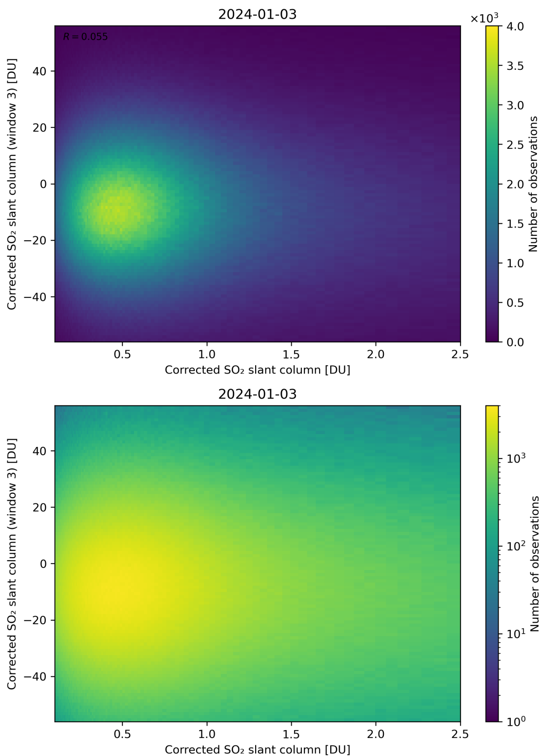
Figure 186: Scatter density plot of “Corrected SO 2 slant column” against “Corrected SO 2 slant column (window 3)” for 2024-01-02 to 2024-01-04.
