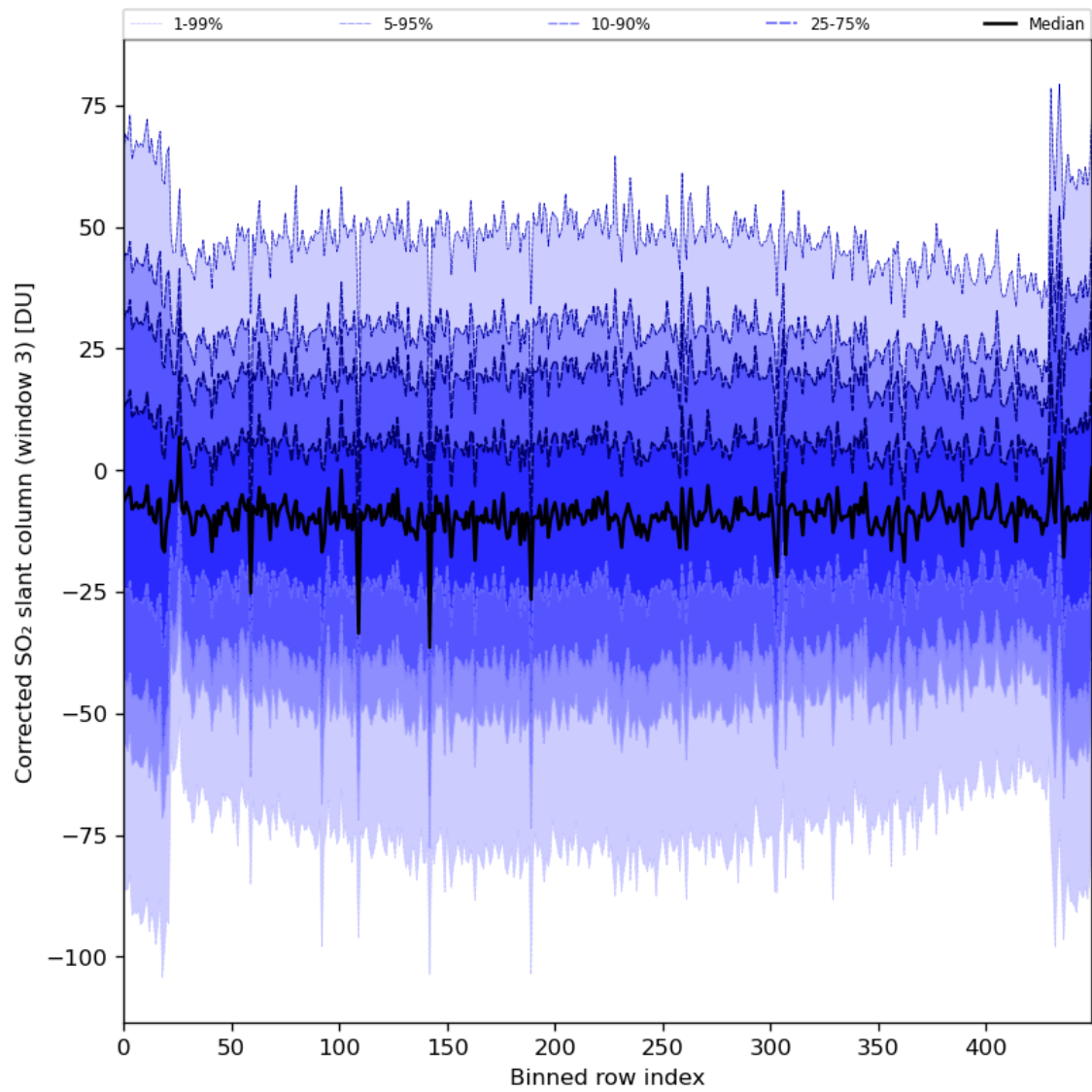
Figure 89: Along track statistics of “Corrected SO 2 slant column (window 3)” for 2024-01-02 to 2024-01-04
