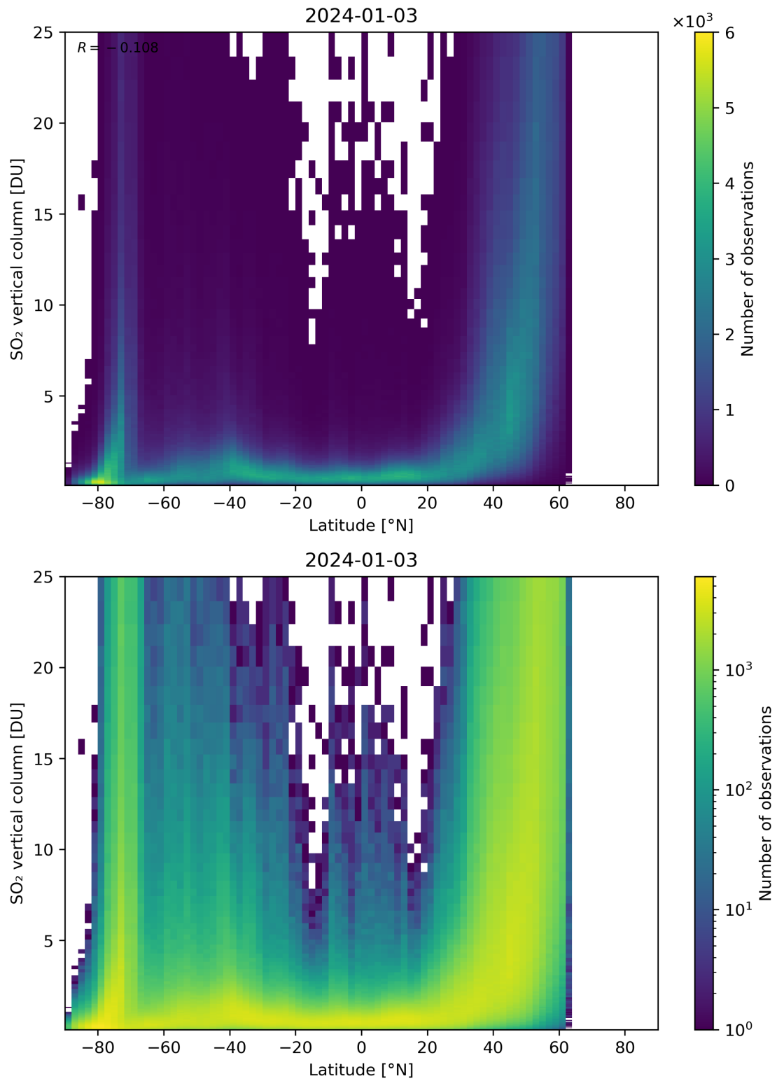
Figure 156: Scatter density plot of “Latitude” against “SO 2 vertical column” for 2024-01-02 to 2024-01-04.
