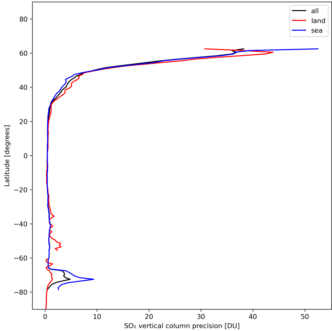
Figure 31: Zonal average of “SO 2 vertical column precision” for 2024-01-02 to 2024-01-04.
