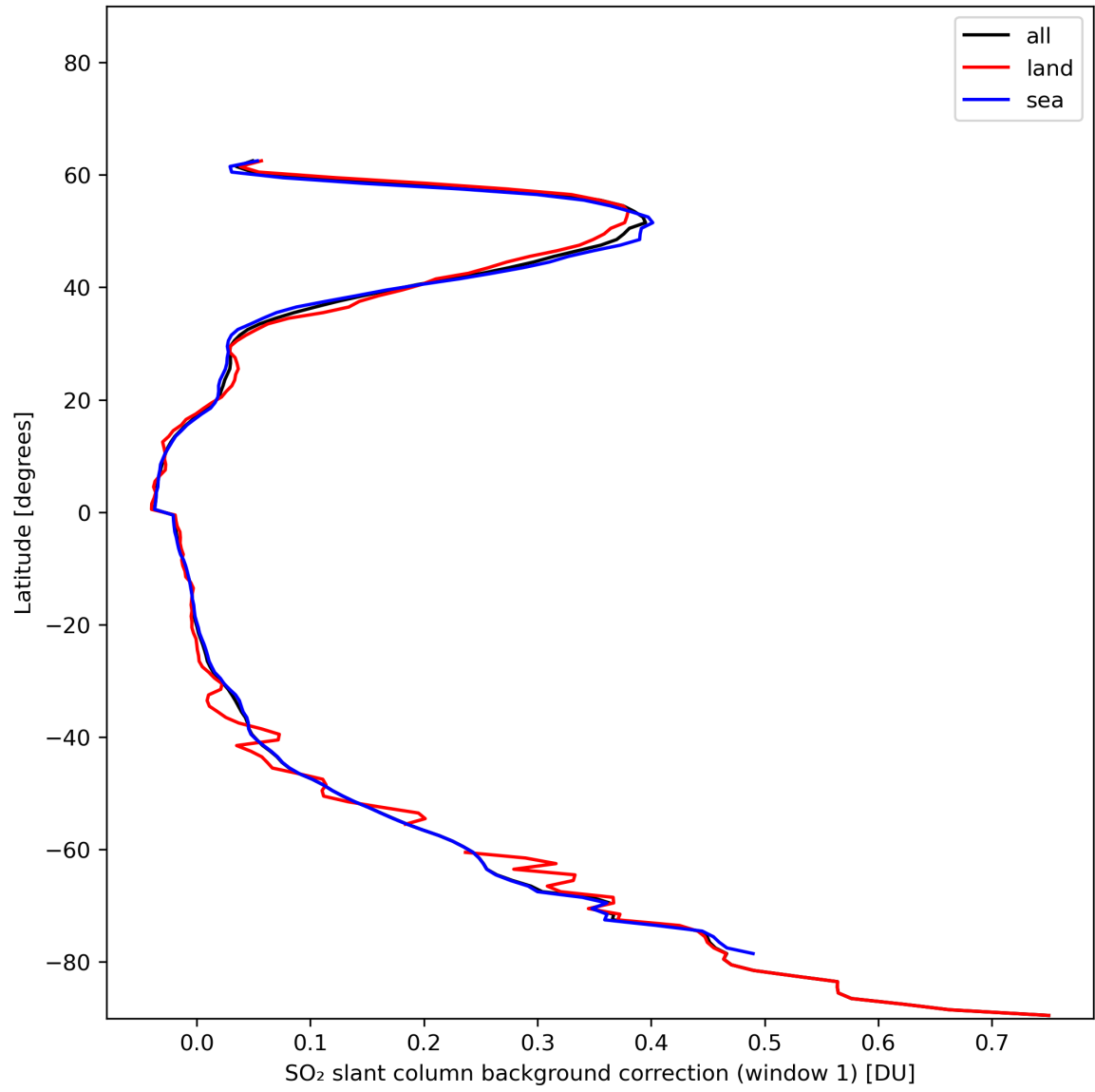
Figure 36: Zonal average of “SO 2 slant column background correction (window 1)” for 2024-01-02 to 2024-01-04.
