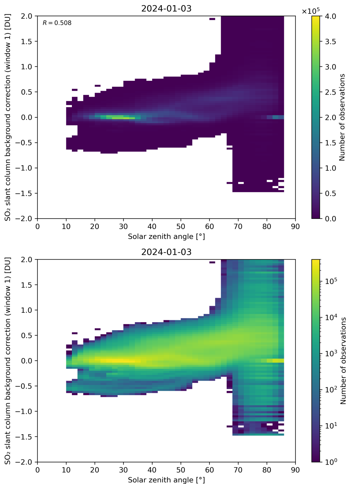
Figure 158: Scatter density plot of “Solar zenith angle” against “SO 2 slant column background correction (window 1)” for 2024-01-02 to 2024-01-04.
