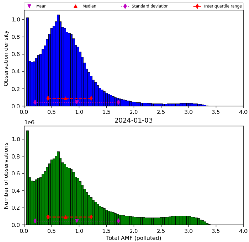
Figure 71: Histogram of “Total AMF (polluted)” for 2024-01-02 to 2024-01-04
