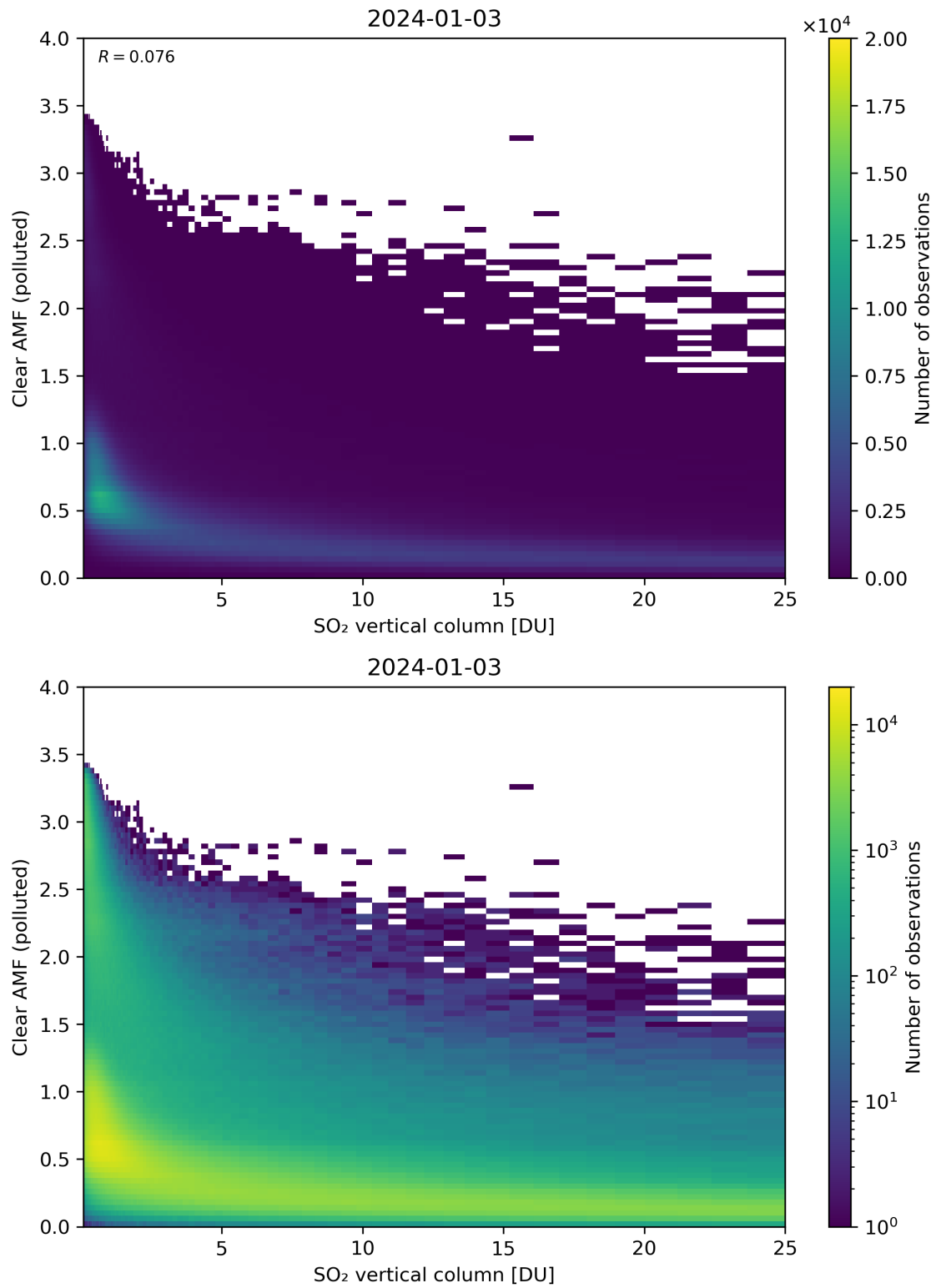
Figure 296: Scatter density plot of “SO 2 vertical column” against “Clear AMF (polluted)” for 2024-01-02 to 2024-01-04.
