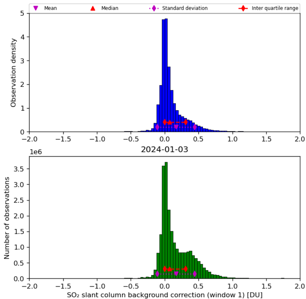
Figure 59: Histogram of “SO 2 slant column background correction (window 1)” for 2024-01-02 to 2024-01-04
