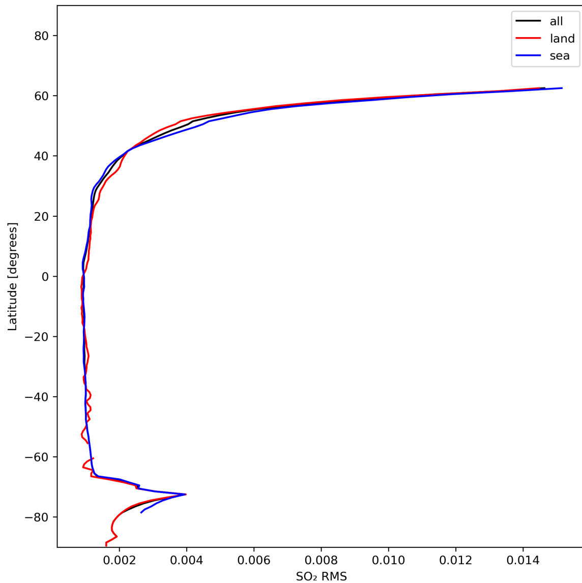
Figure 47: Zonal average of “SO 2 RMS” for 2024-01-02 to 2024-01-04.
