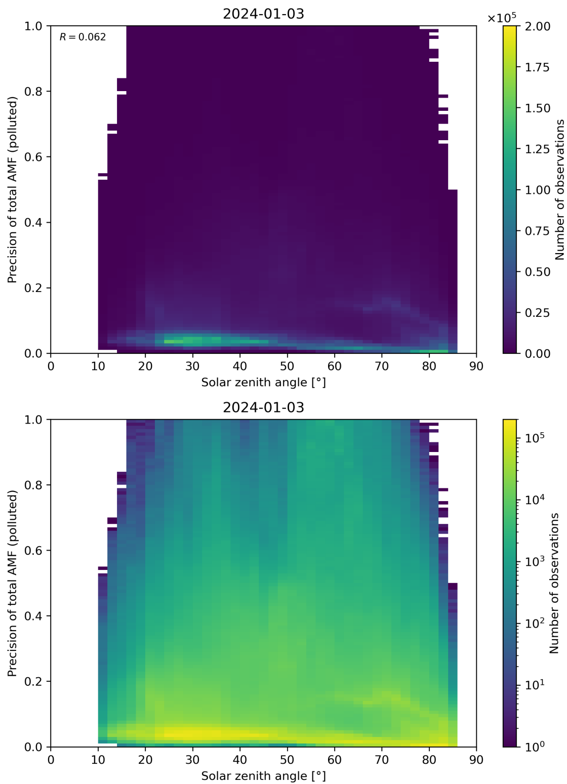
Figure 175: Scatter density plot of “Solar zenith angle” against “Precision of total AMF (polluted)” for 2024-01-02 to 2024-01-04.
