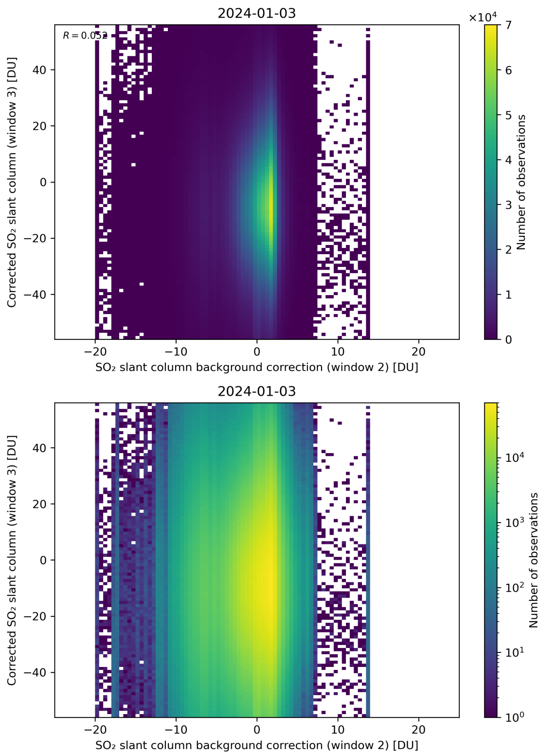
Figure 116: Scatter density plot of “SO 2 slant column background correction (window 2)” against “Corrected SO 2 slant column (window 3)” for 2024-01-02 to 2024-01-04.
