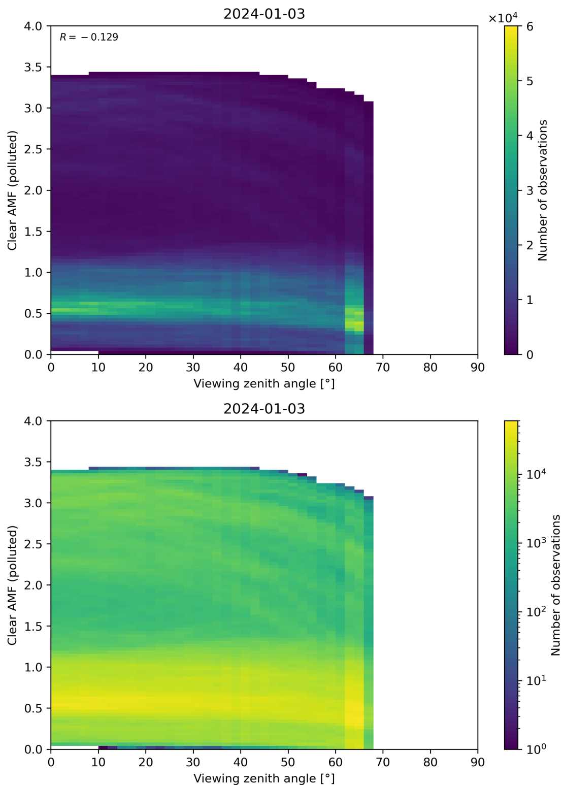
Figure 316: Scatter density plot of “Viewing zenith angle” against “Clear AMF (polluted)” for 2024-01-02 to 2024-01-04.
