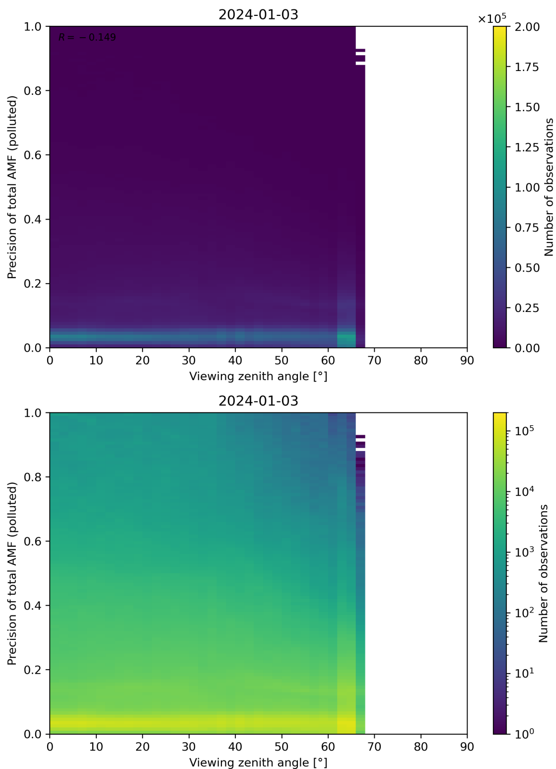
Figure 326: Scatter density plot of “Viewing zenith angle” against “Precision of total AMF (polluted)” for 2024-01-02 to 2024-01-04.
