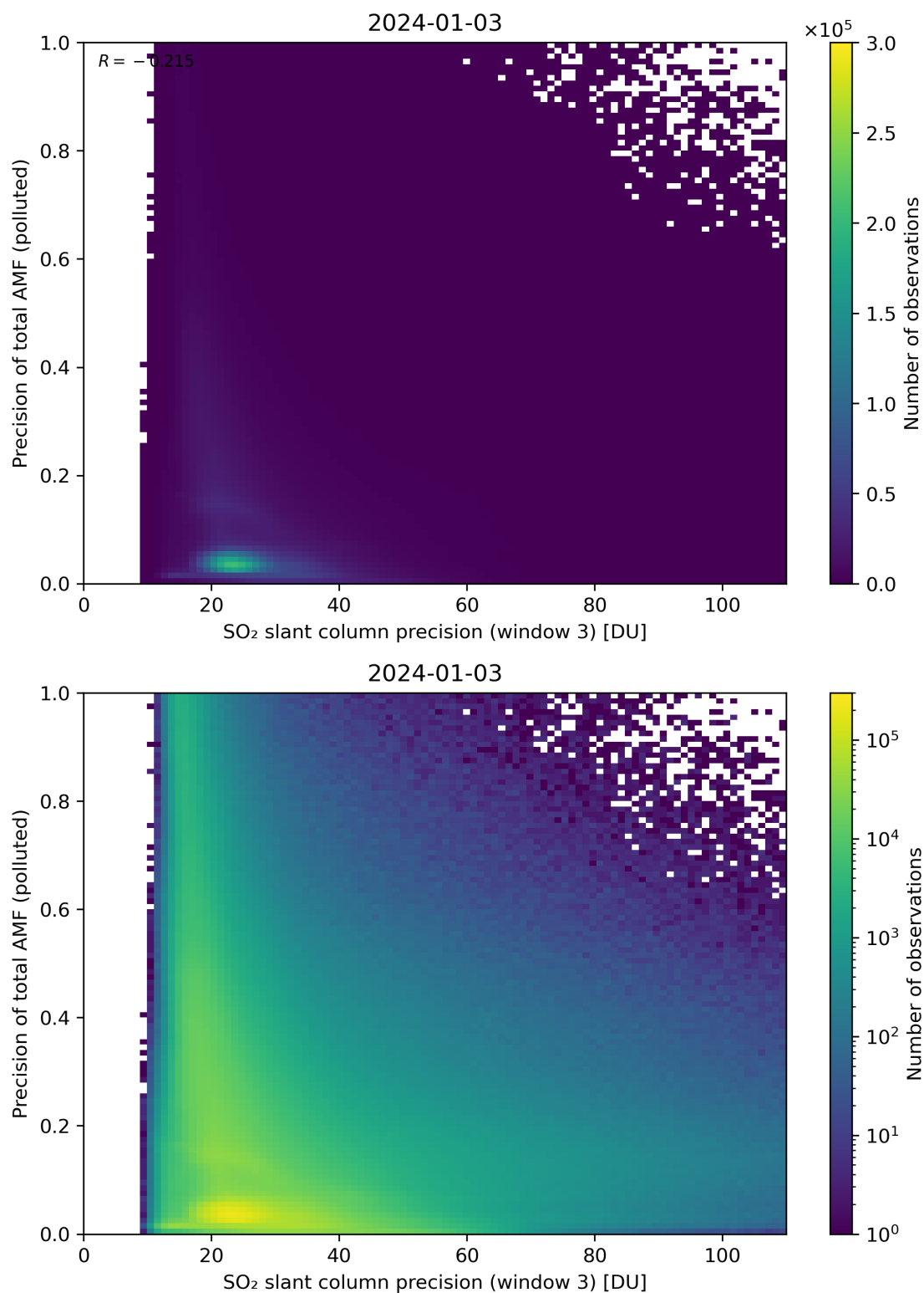
Figure 264: Scatter density plot of “SO 2 slant column precision (window 3)” against “Precision of total AMF (polluted)” for 2024-01-02 to 2024-01-04.
