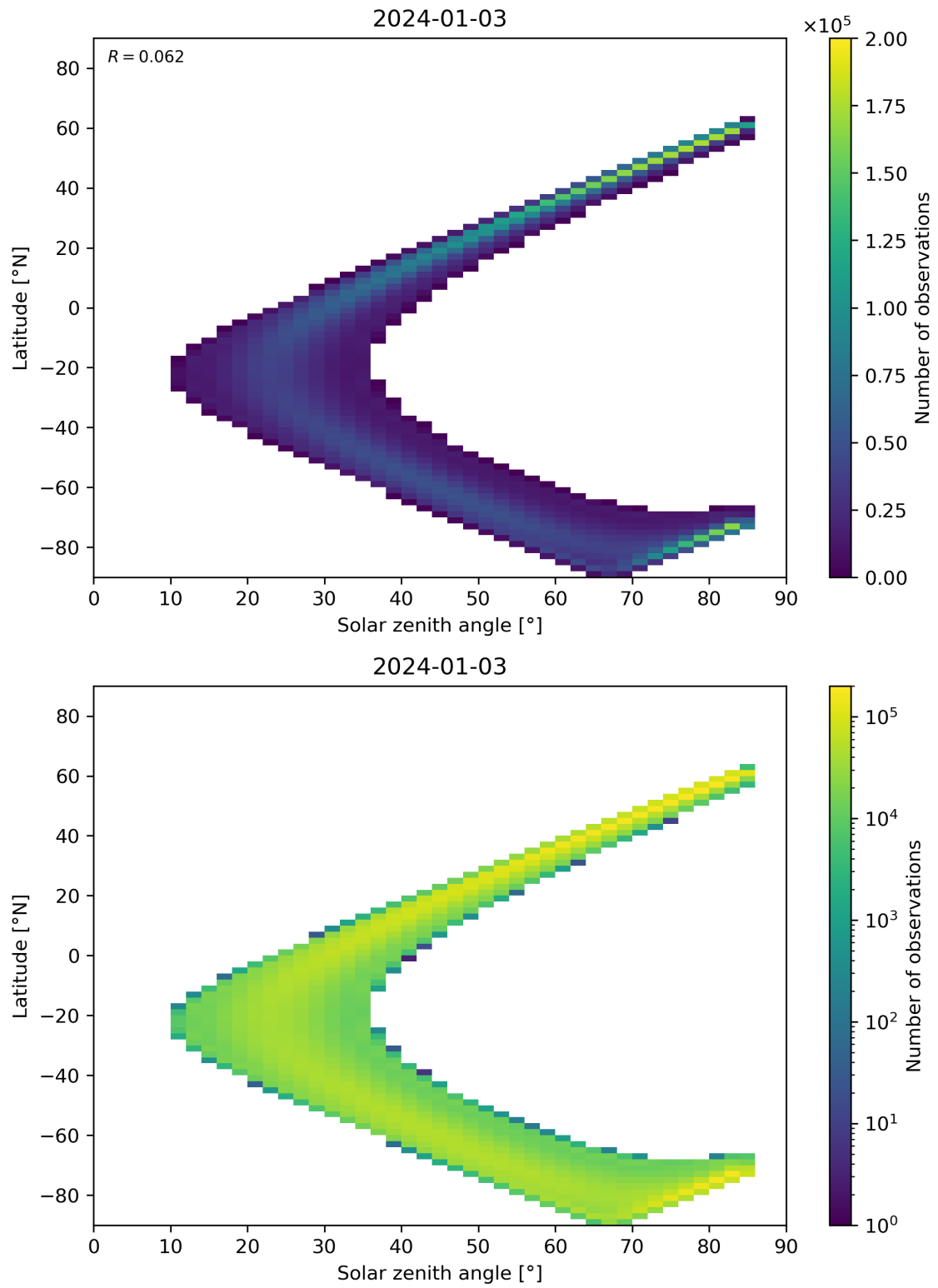
Figure 164: Scatter density plot of “Solar zenith angle” against “Latitude” for 2024-01-02 to 2024-01-04.
