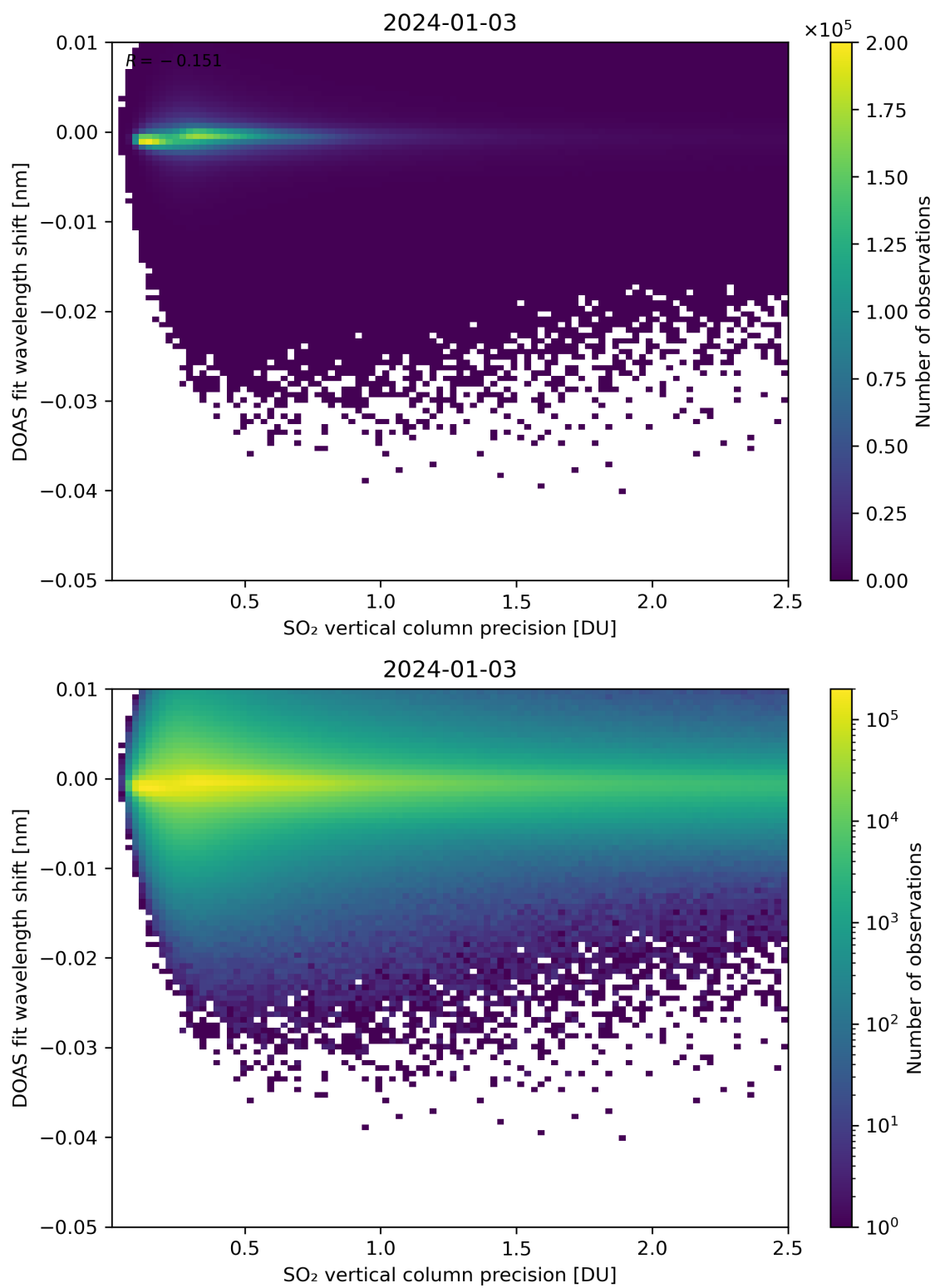
Figure 282: Scatter density plot of “SO 2 vertical column precision” against “DOAS fit wavelength shift” for 2024-01-02 to 2024-01-04.
