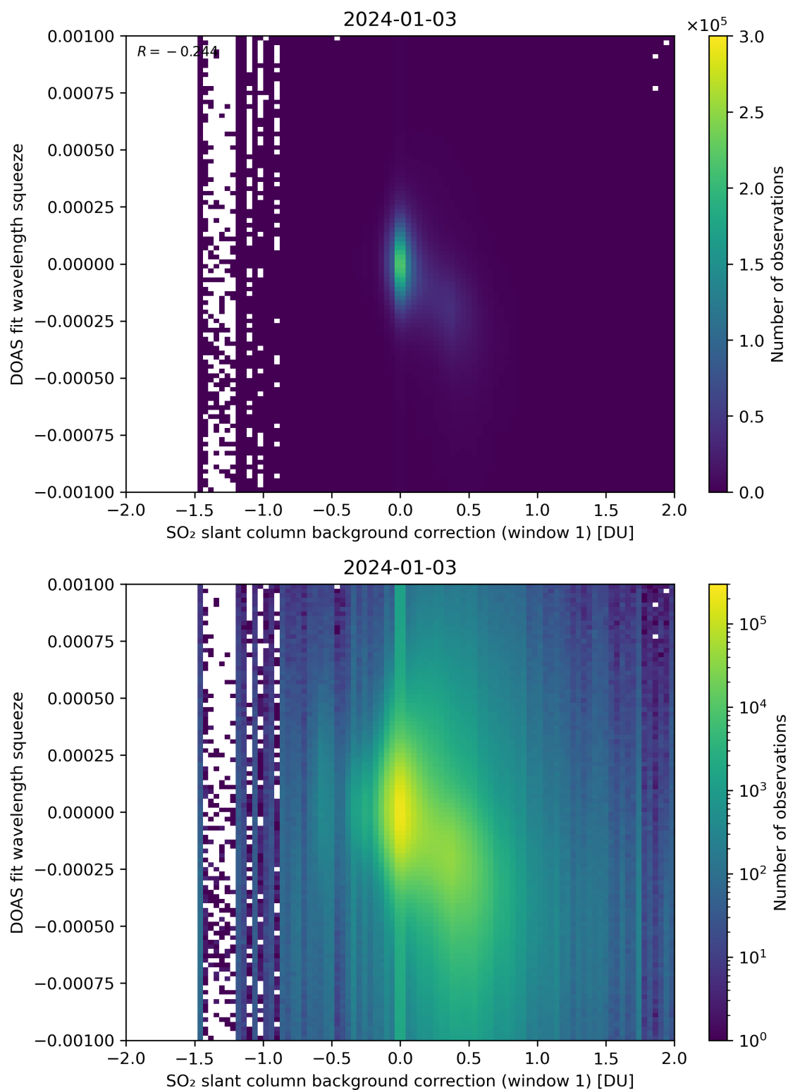
Figure 101: Scatter density plot of “SO 2 slant column background correction (window 1)” against “DOAS fit wavelength squeeze” for 2024-01-02 to 2024-01-04.
