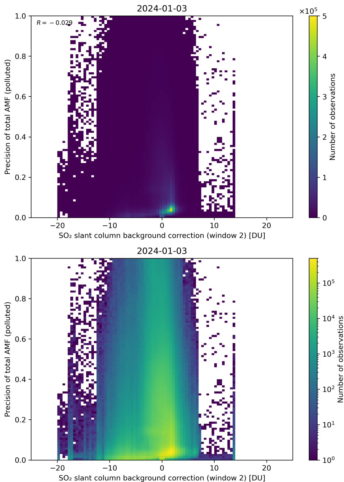
Figure 120: Scatter density plot of “SO 2 slant column background correction (window 2)” against “Precision of total AMF (polluted)” for 2024-01-02 to 2024-01-04.
