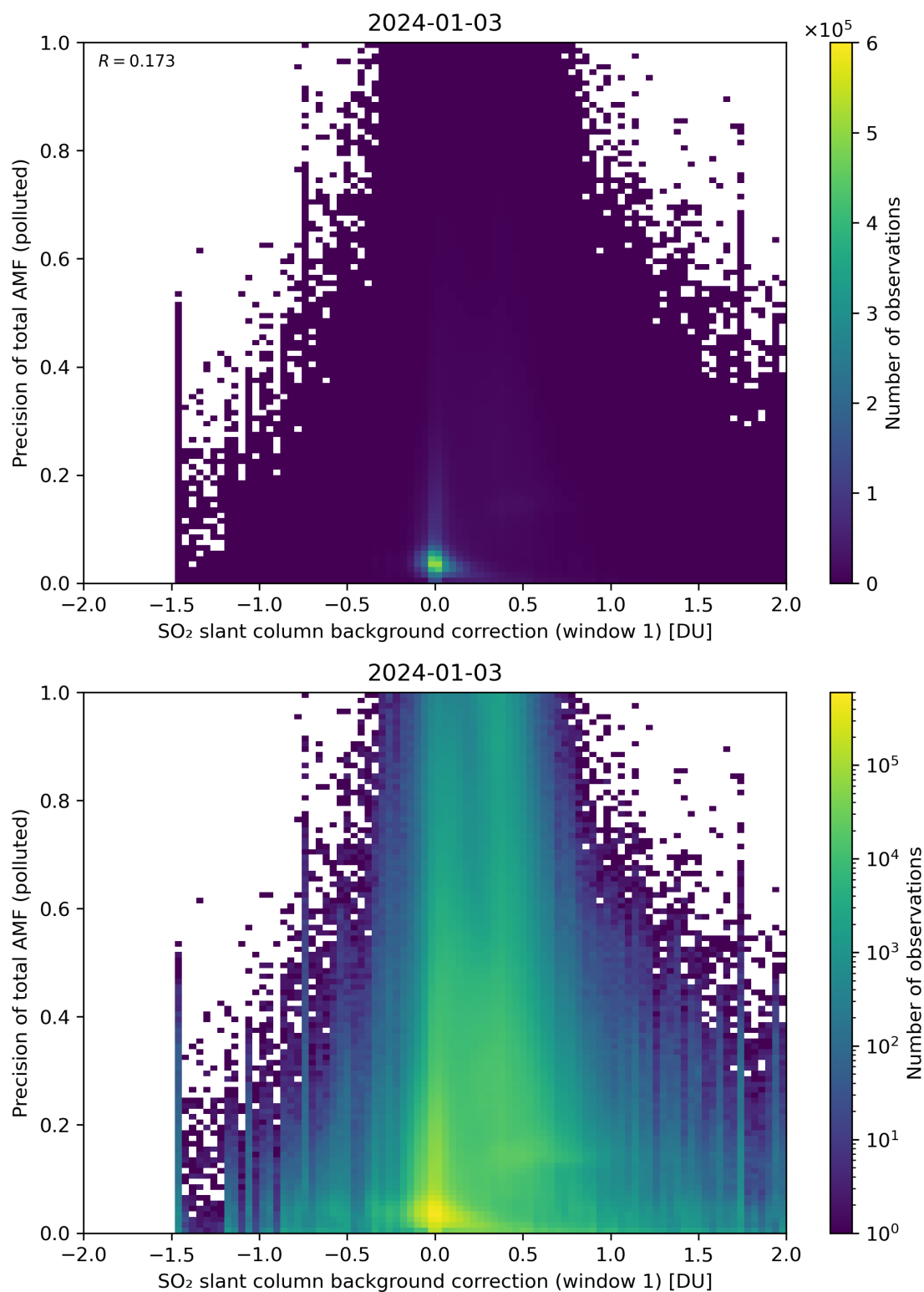
Figure 110: Scatter density plot of “SO 2 slant column background correction (window 1)” against “Precision of total AMF (polluted)” for 2024-01-02 to 2024-01-04.
