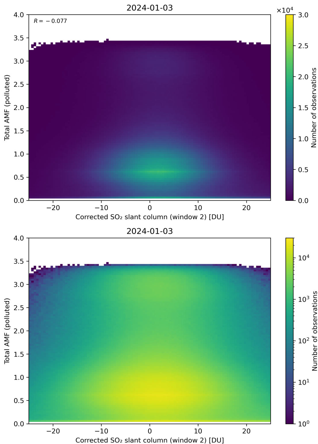
Figure 203: Scatter density plot of “Corrected SO 2 slant column (window 2)” against “Total AMF (polluted)” for 2024-01-02 to 2024-01-04.
