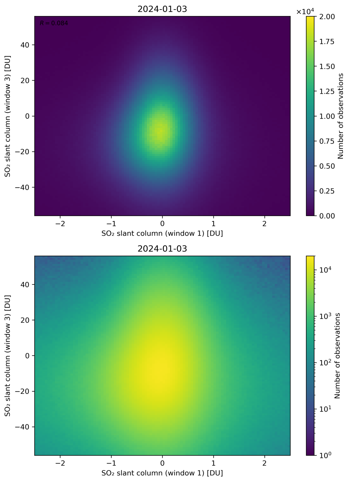
Figure 237: Scatter density plot of “SO 2 slant column (window 1)” against “SO 2 slant column (window 3)” for 2024-01-02 to 2024-01-04.
