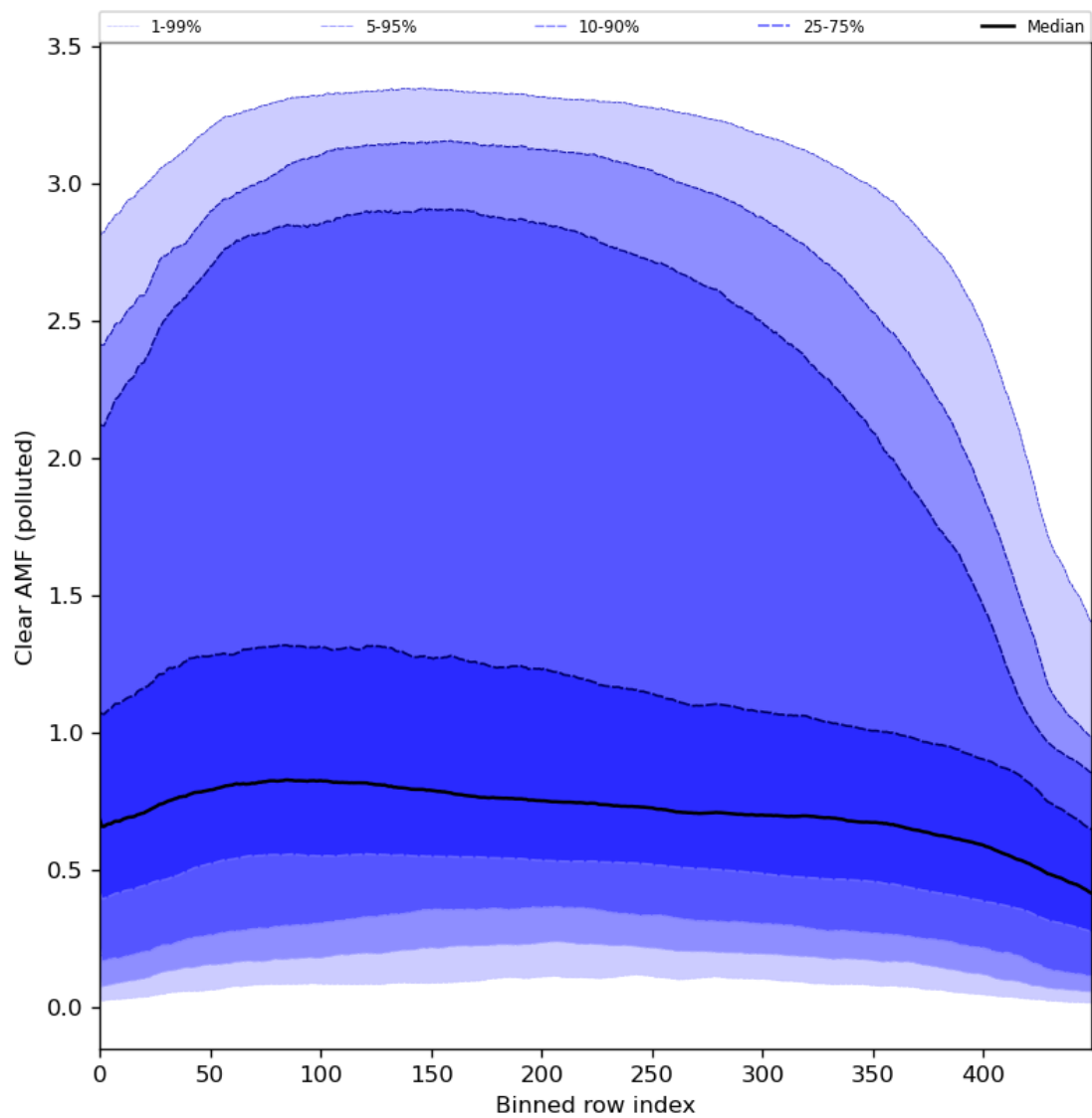
Figure 96: Along track statistics of “Clear AMF (polluted)” for 2024-01-02 to 2024-01-04
