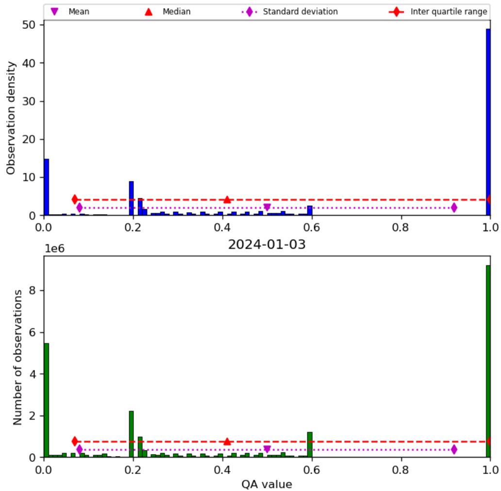
Figure 52: Histogram of “QA value” for 2024-01-02 to 2024-01-04
