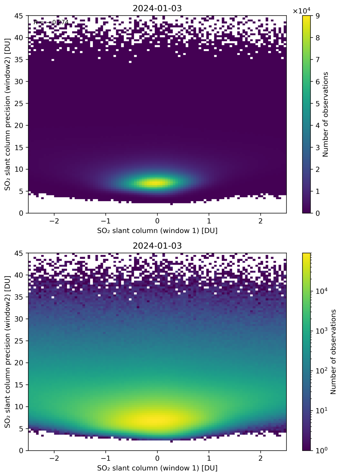
Figure 236: Scatter density plot of “SO 2 slant column (window 1)” against “SO 2 slant column precision (window2)” for 2024-01-02 to 2024-01-04.
