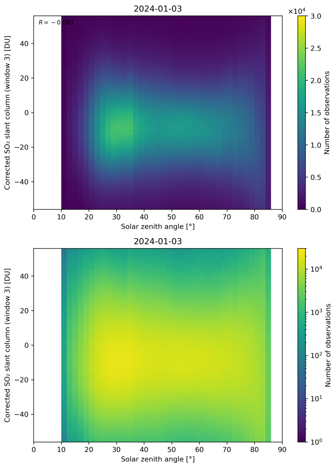
Figure 168: Scatter density plot of “Solar zenith angle” against “Corrected SO 2 slant column (window 3)” for 2024-01-02 to 2024-01-04.
