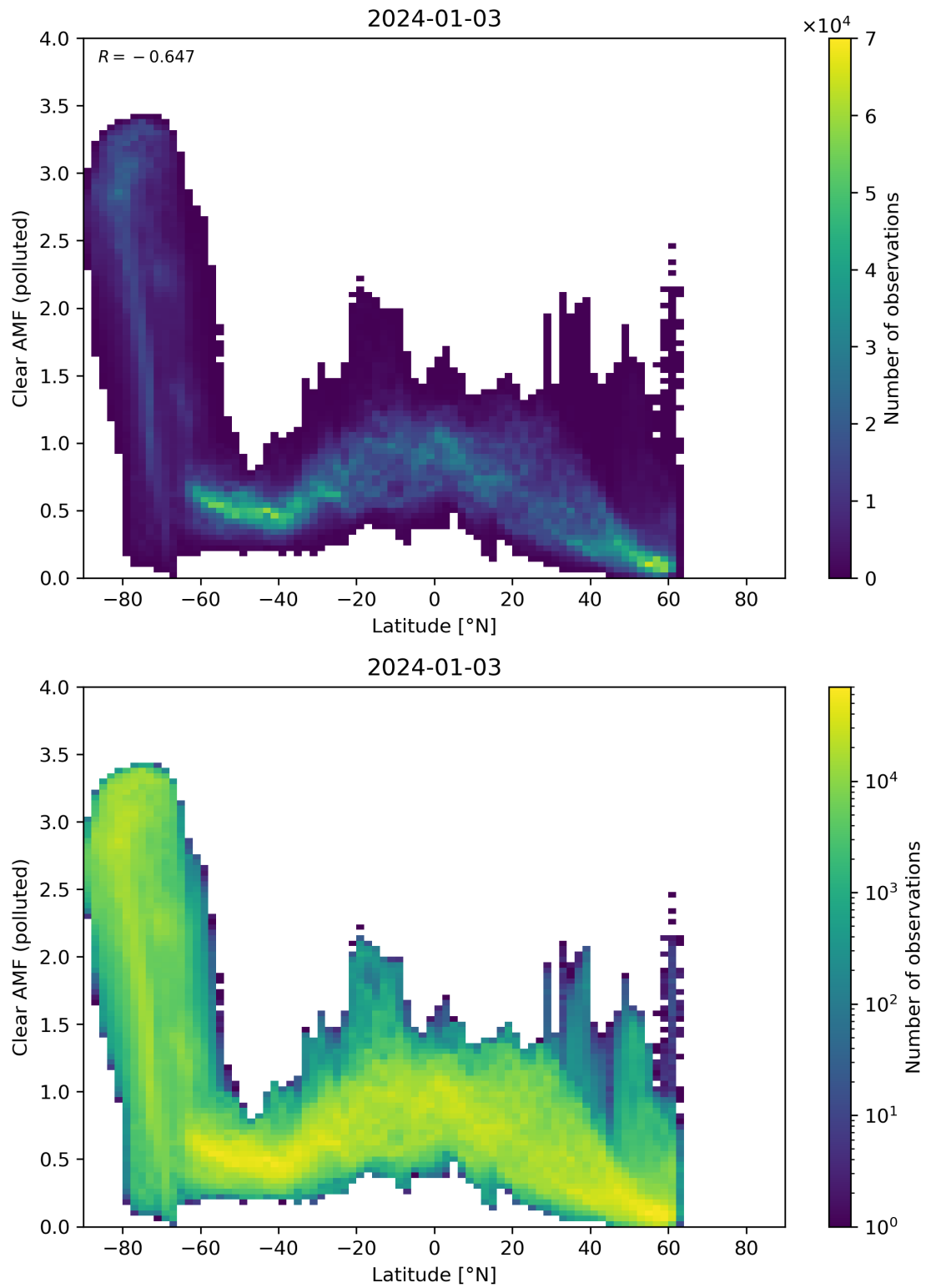
Figure 145: Scatter density plot of “Latitude” against “Clear AMF (polluted)” for 2024-01-02 to 2024-01-04.
