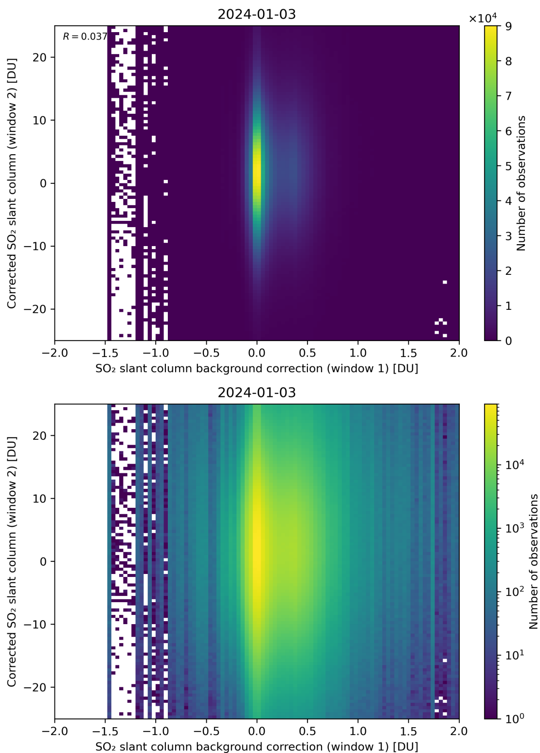
Figure 104: Scatter density plot of “SO 2 slant column background correction (window 1)” against “Corrected SO 2 slant column (window 2)” for 2024-01-02 to 2024-01-04.
