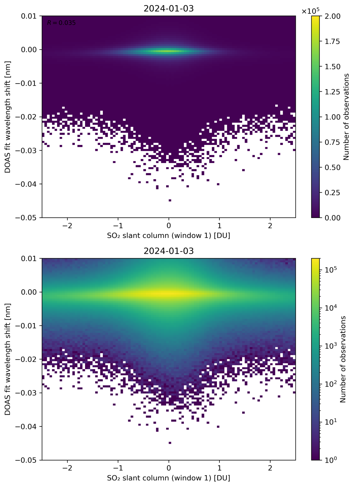
Figure 215: Scatter density plot of “SO 2 slant column (window 1)” against “DOAS fit wavelength shift” for 2024-01-02 to 2024-01-04.
