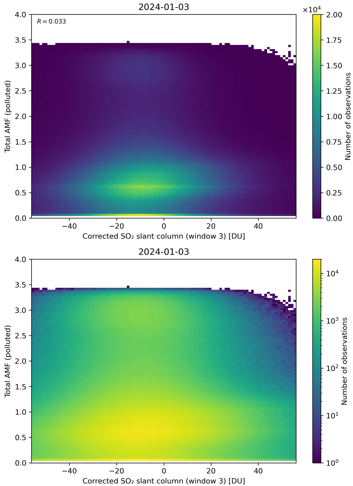
Figure 210: Scatter density plot of “Corrected SO 2 slant column (window 3)” against “Total AMF (polluted)” for 2024-01-02 to 2024-01-04.
