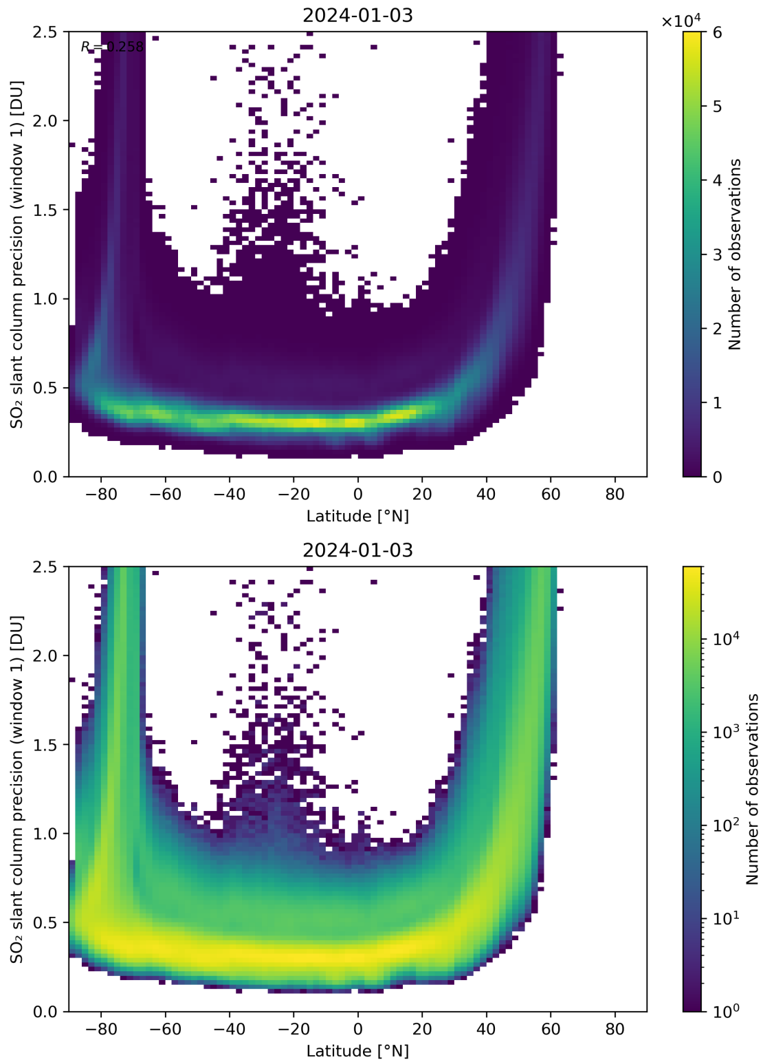
Figure 150: Scatter density plot of “Latitude” against “SO 2 slant column precision (window 1)” for 2024-01-02 to 2024-01-04.
