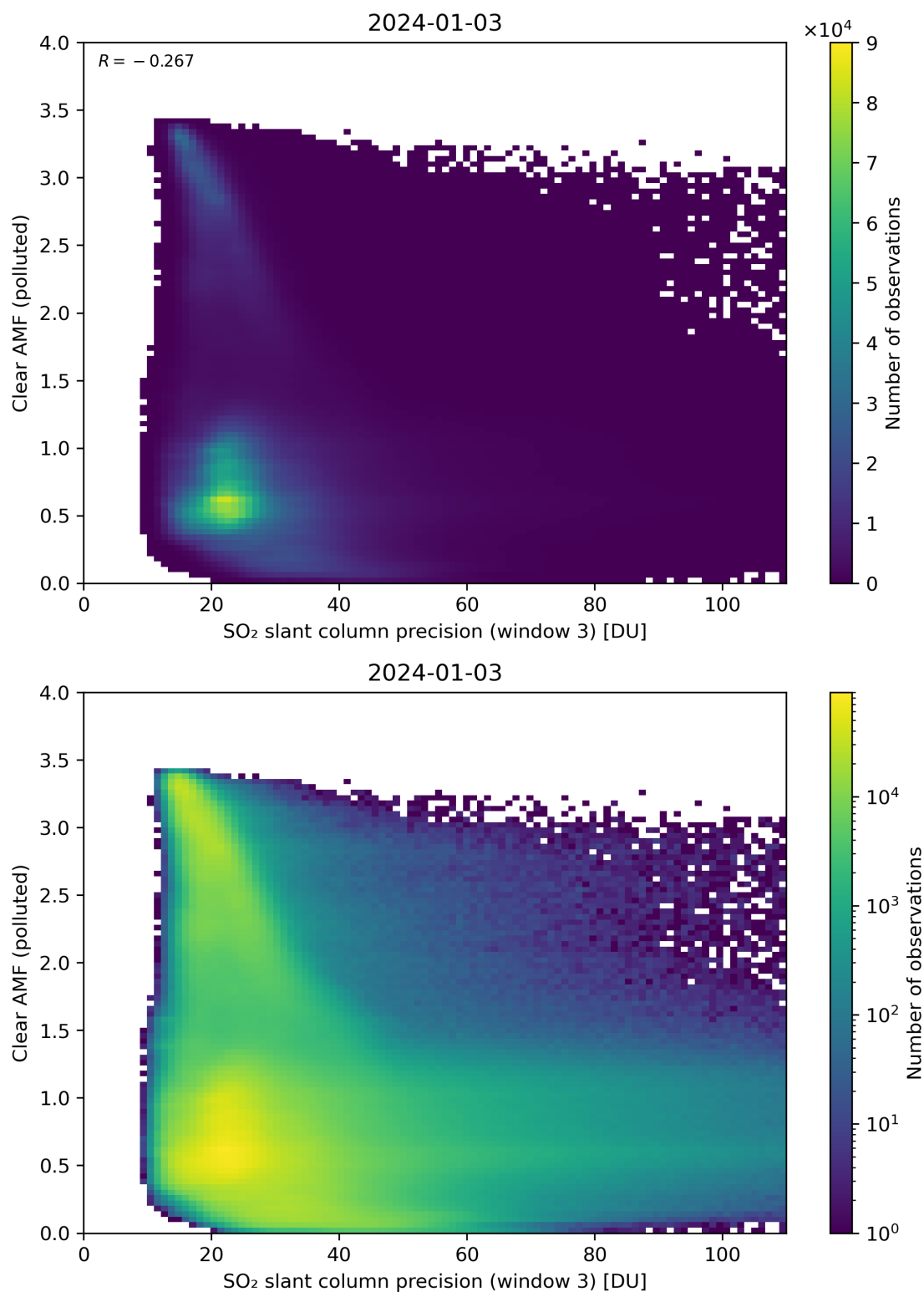
Figure 261: Scatter density plot of “SO 2 slant column precision (window 3)” against “Clear AMF (polluted)” for 2024-01-02 to 2024-01-04.
