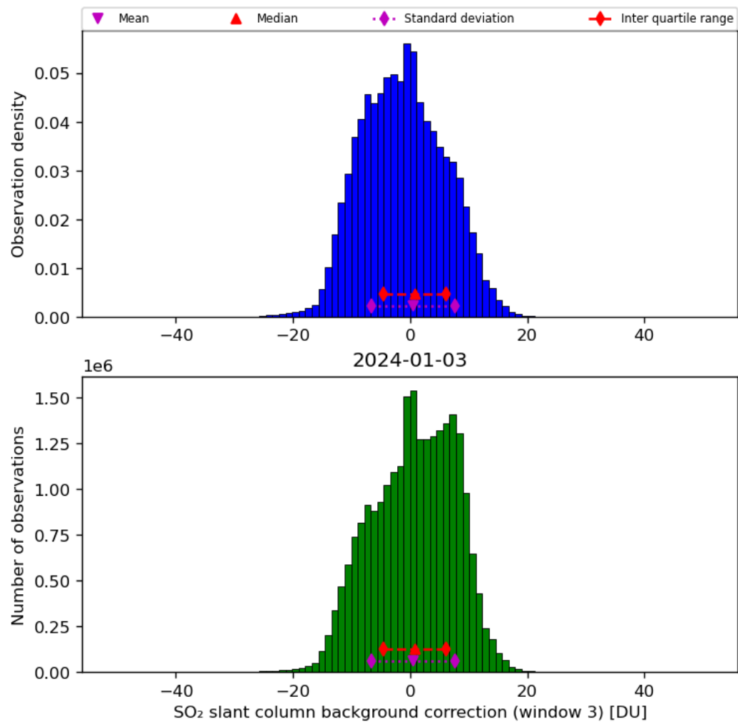
Figure 67: Histogram of “SO 2 slant column background correction (window 3)” for 2024-01-02 to 2024-01-04
