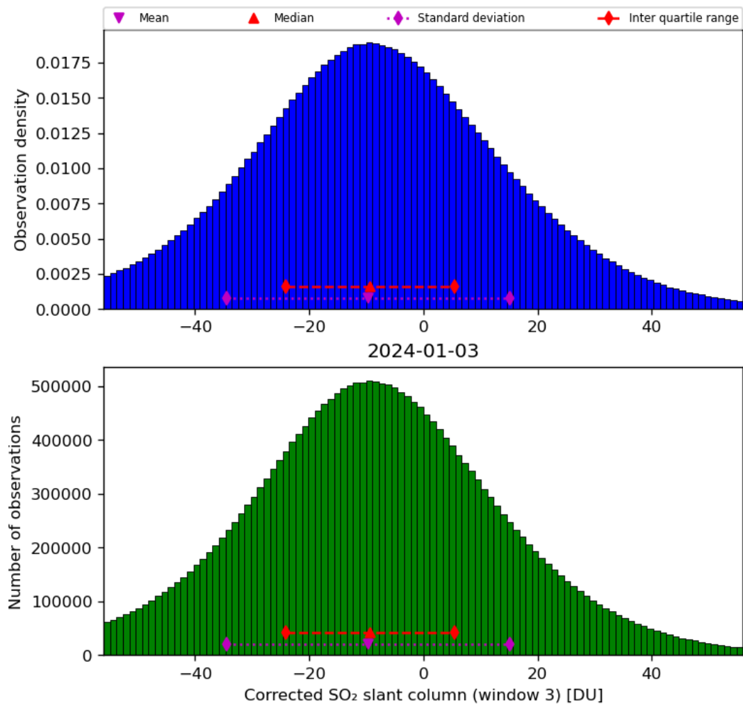
Figure 66: Histogram of “Corrected SO 2 slant column (window 3)” for 2024-01-02 to 2024-01-04
