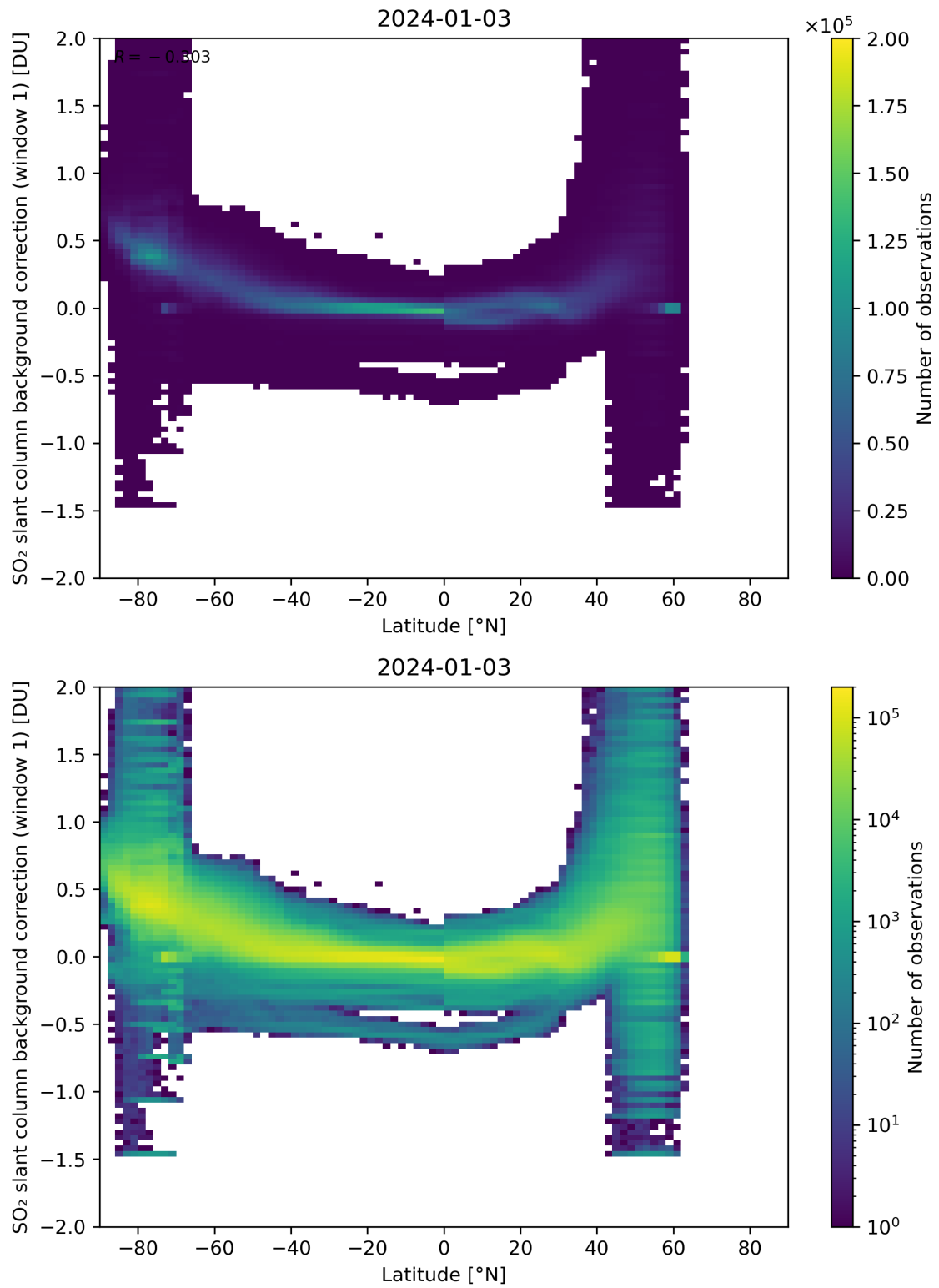
Figure 139: Scatter density plot of “Latitude” against “SO 2 slant column background correction (window 1)” for 2024-01-02 to 2024-01-04.
