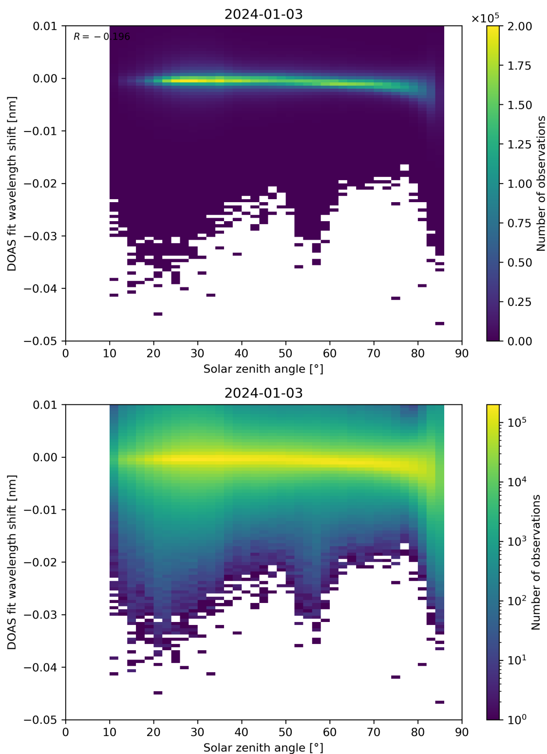
Figure 161: Scatter density plot of “Solar zenith angle” against “DOAS fit wavelength shift” for 2024-01-02 to 2024-01-04.
