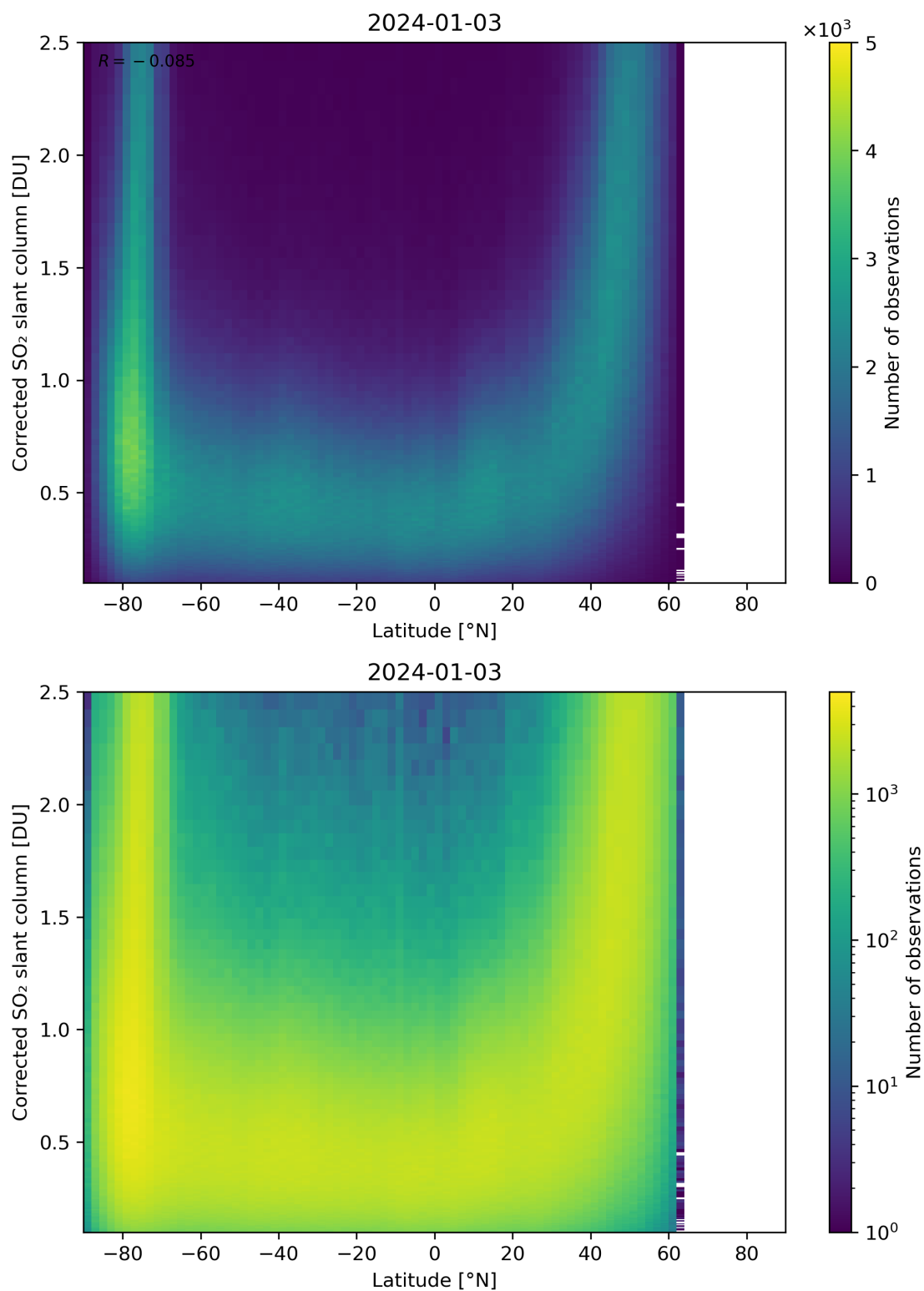
Figure 146: Scatter density plot of “Latitude” against “Corrected SO 2 slant column” for 2024-01-02 to 2024-01-04.
