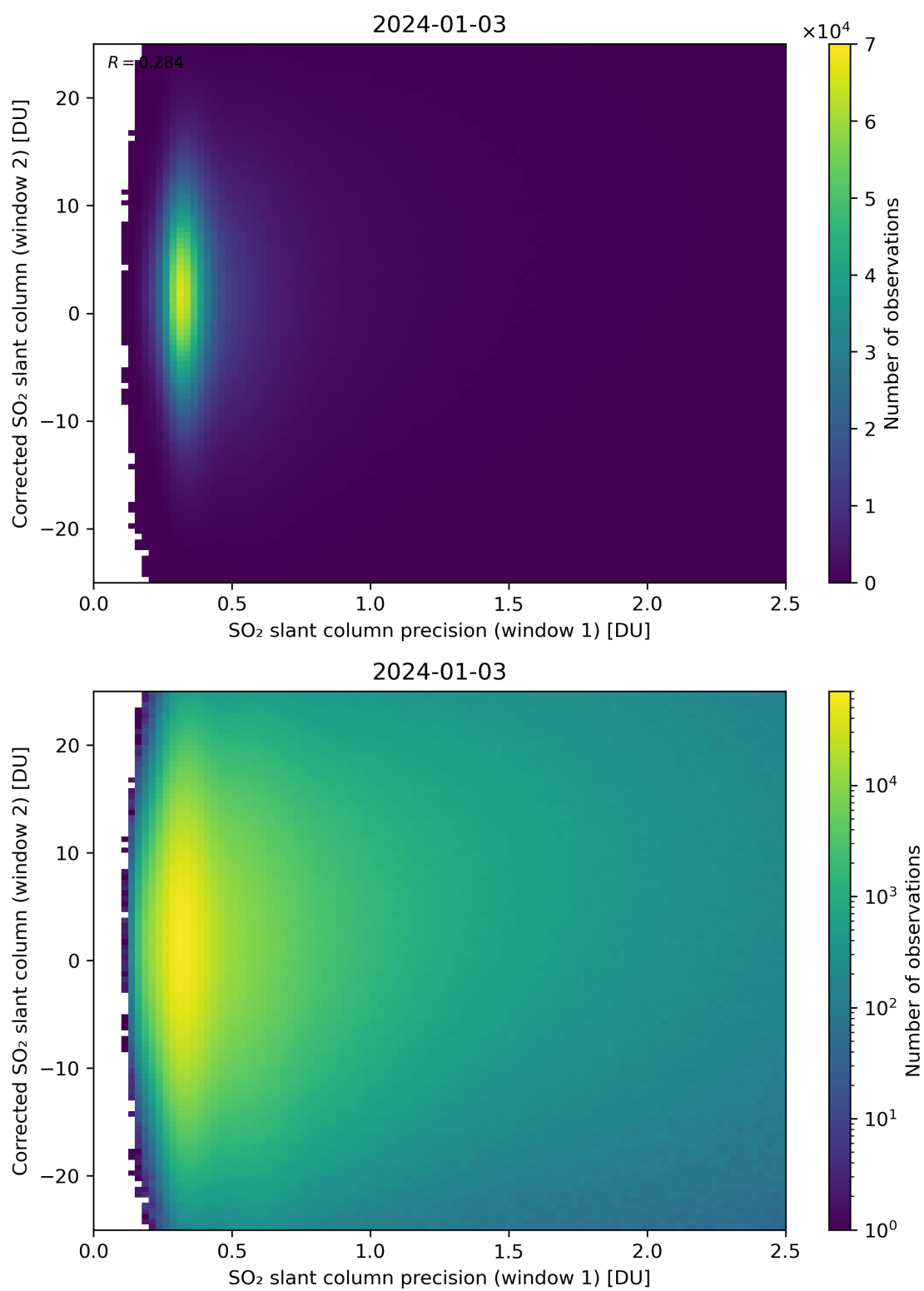
Figure 225: Scatter density plot of “SO 2 slant column precision (window 1)” against “Corrected SO 2 slant column (window 2)” for 2024-01-02 to 2024-01-04.
