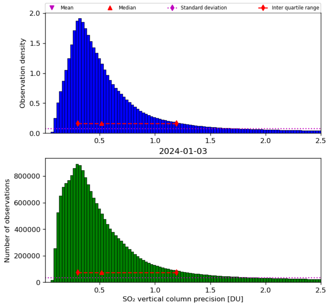
Figure 54: Histogram of “SO 2 vertical column precision” for 2024-01-02 to 2024-01-04
