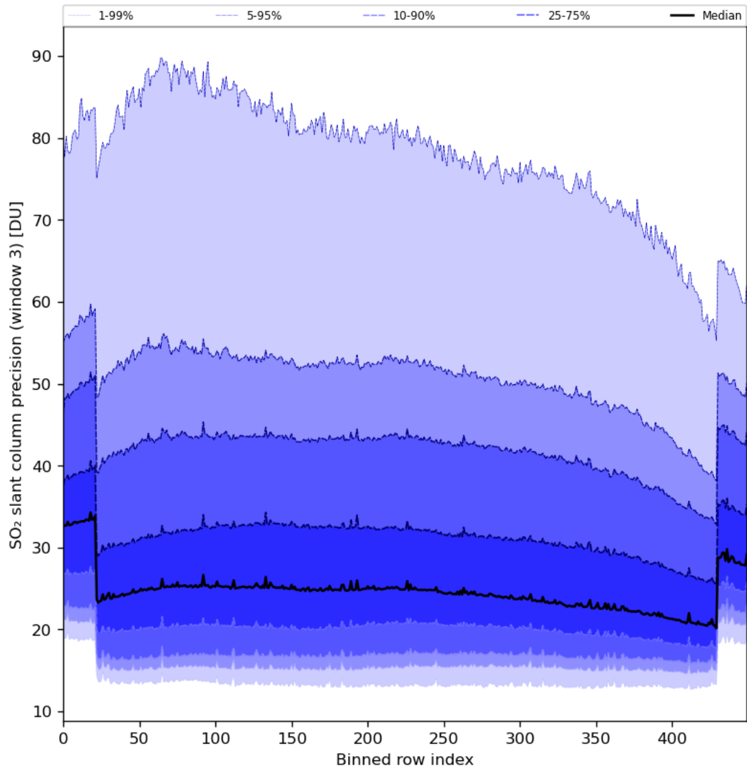
Figure 88: Along track statistics of “SO 2 slant column precision (window 3)” for 2024-01-02 to 2024-01-04
