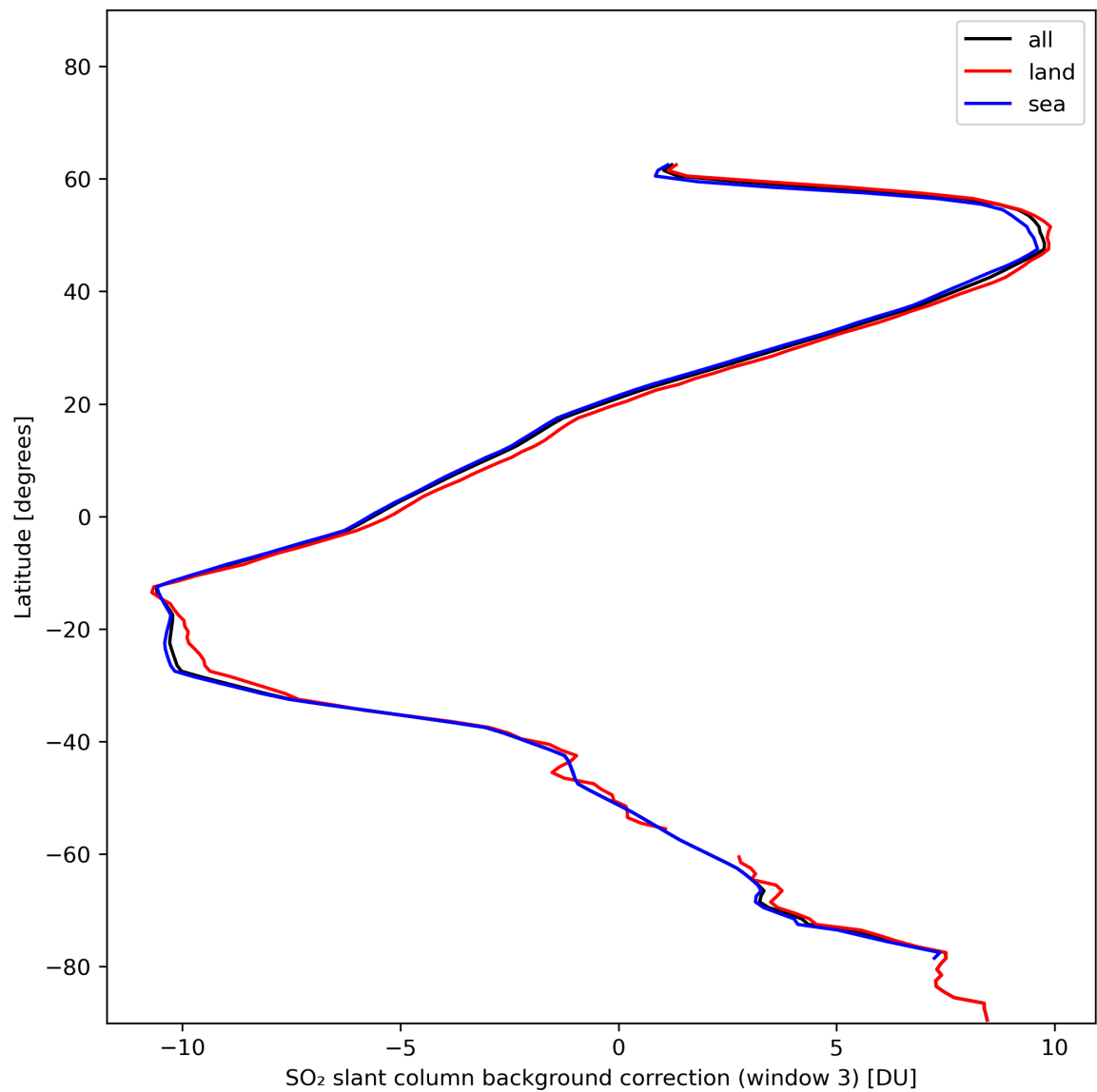
Figure 44: Zonal average of “SO 2 slant column background correction (window 3)” for 2024-01-02 to 2024-01-04.
