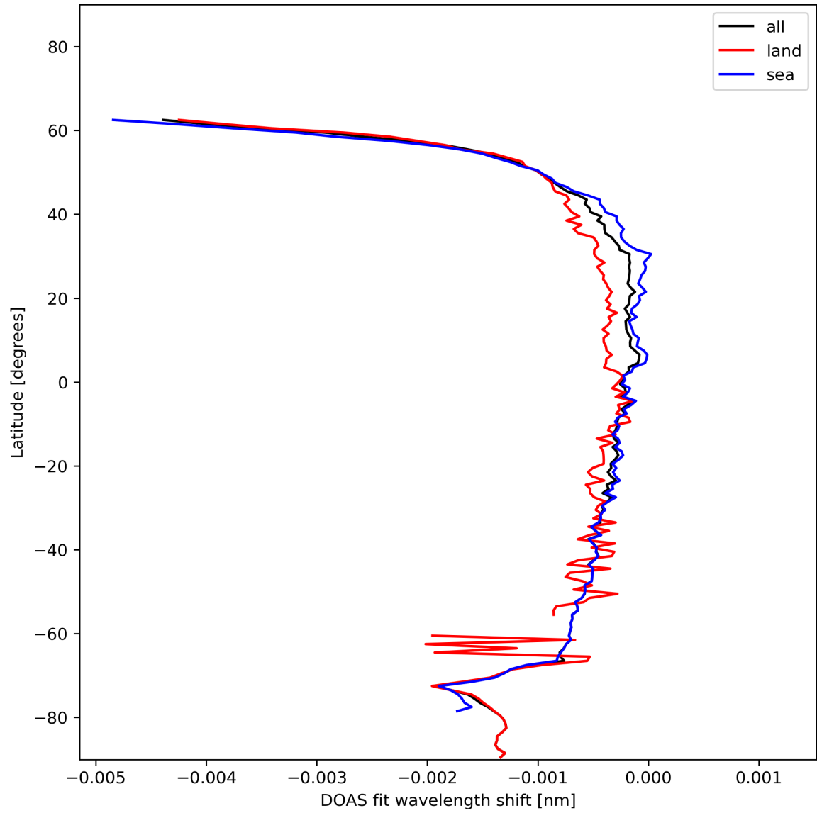
Figure 45: Zonal average of “DOAS fit wavelength shift” for 2024-01-02 to 2024-01-04.
