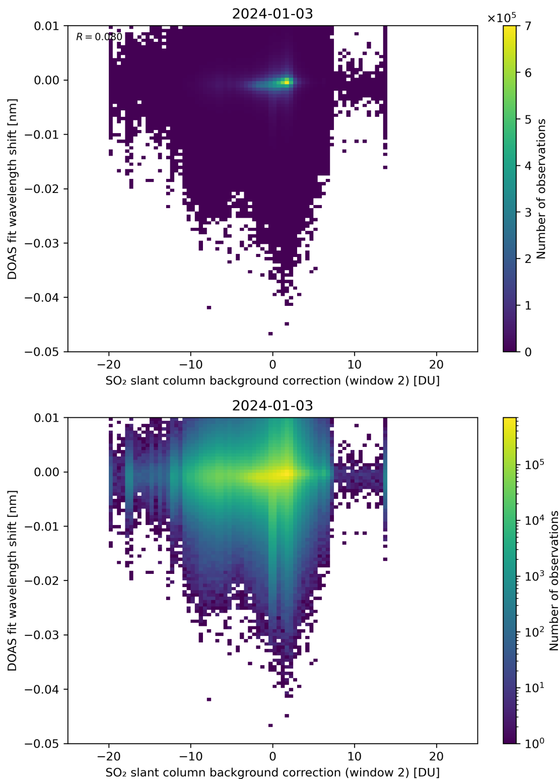
Figure 112: Scatter density plot of “SO 2 slant column background correction (window 2)” against “DOAS fit wavelength shift” for 2024-01-02 to 2024-01-04.
