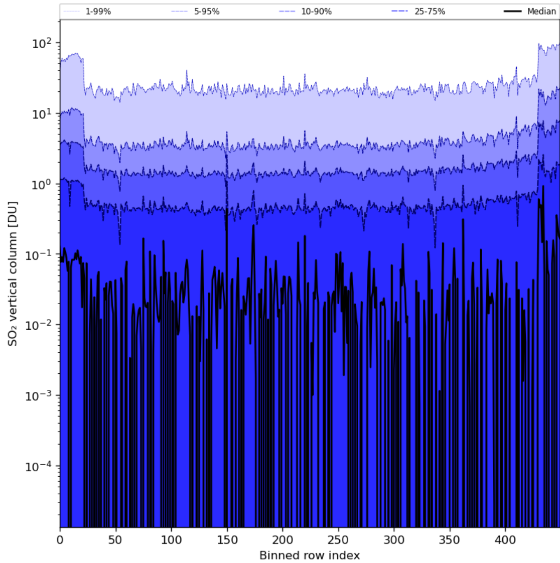
Figure 76: Along track statistics of “SO 2 vertical column” for 2024-01-02 to 2024-01-04
