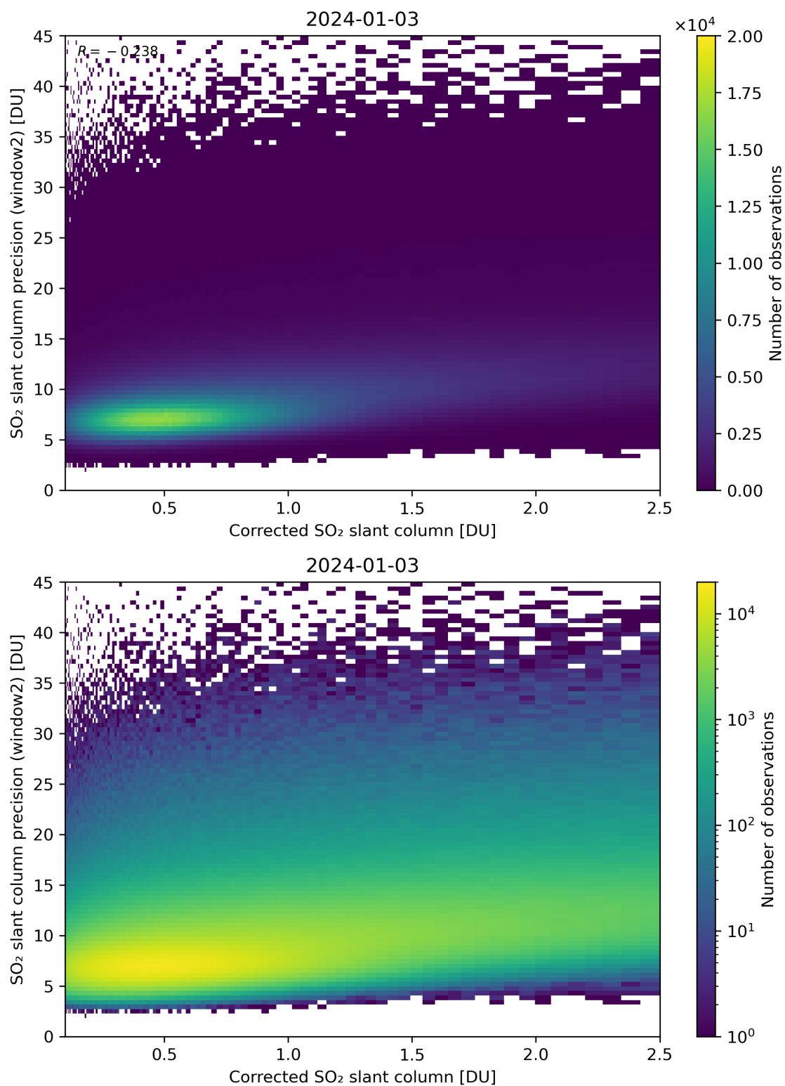
Figure 189: Scatter density plot of “Corrected SO 2 slant column” against “SO 2 slant column precision (window2)” for 2024-01-02 to 2024-01-04.
