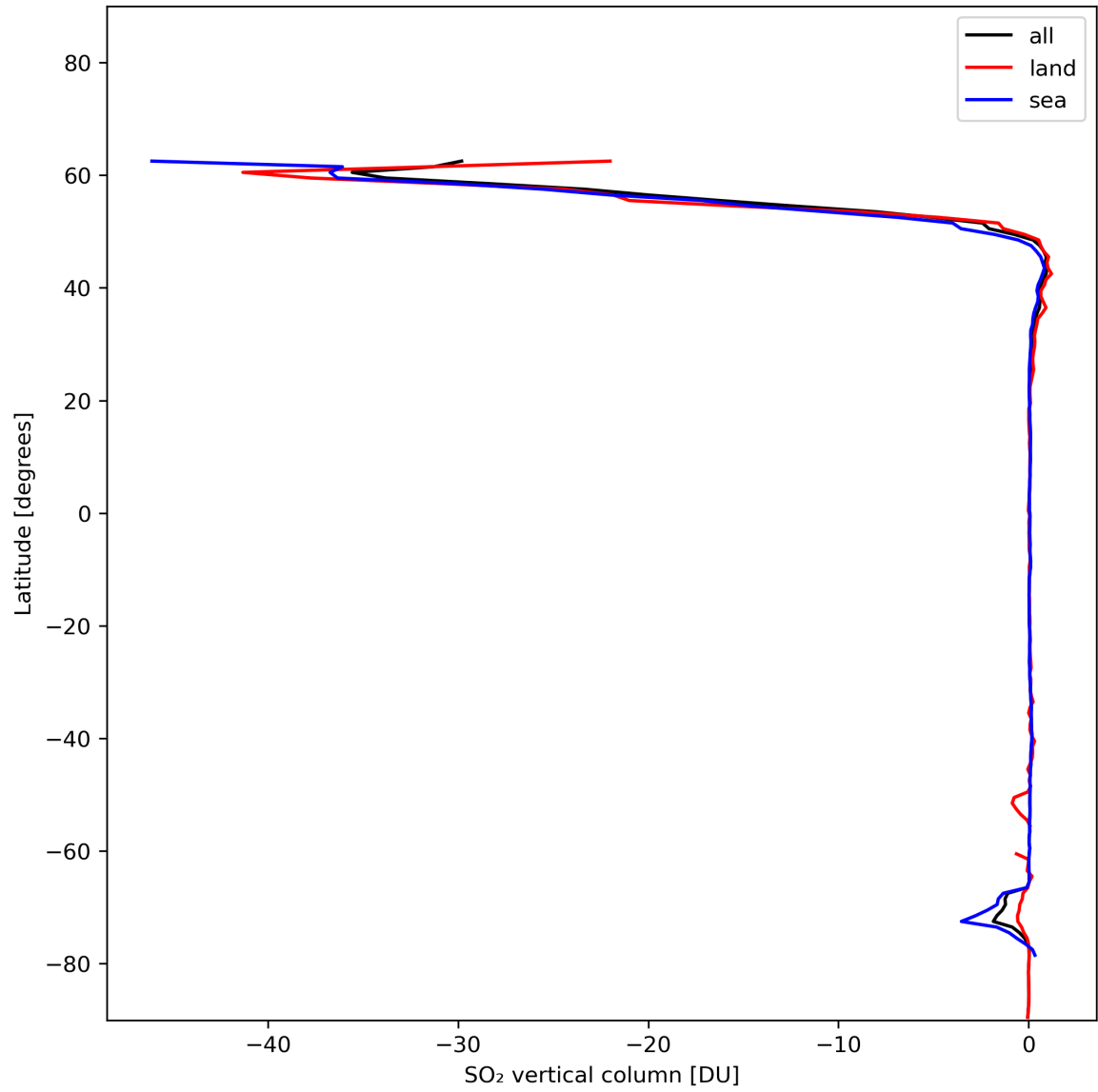
Figure 30: Zonal average of “SO 2 vertical column” for 2024-01-02 to 2024-01-04.
