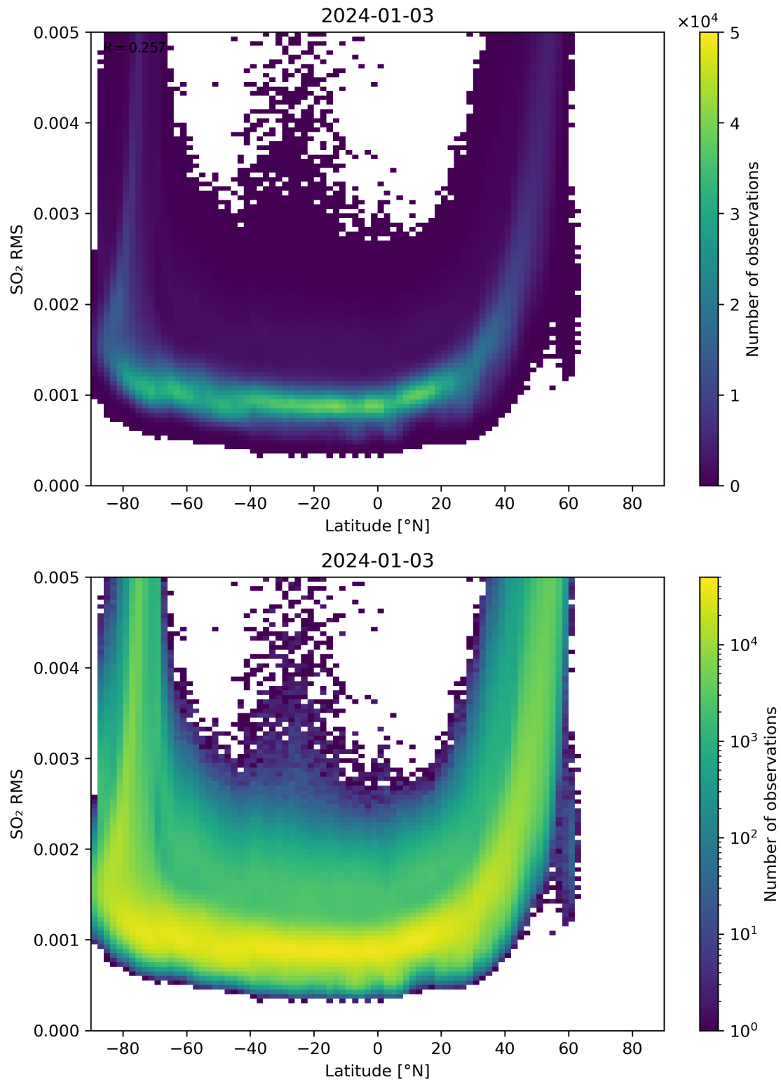
Figure 144: Scatter density plot of “Latitude” against “SO 2 RMS” for 2024-01-02 to 2024-01-04.
