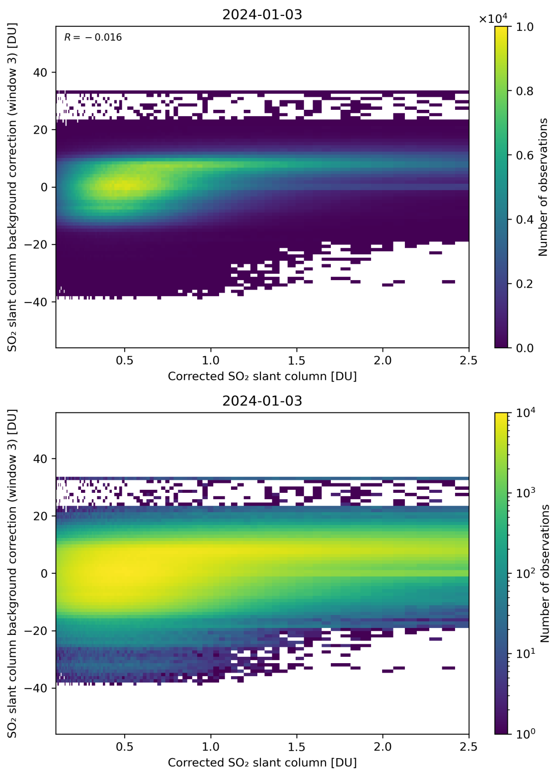
Figure 180: Scatter density plot of “Corrected SO 2 slant column” against “SO 2 slant column background correction (window 3)” for 2024-01-02 to 2024-01-04.
