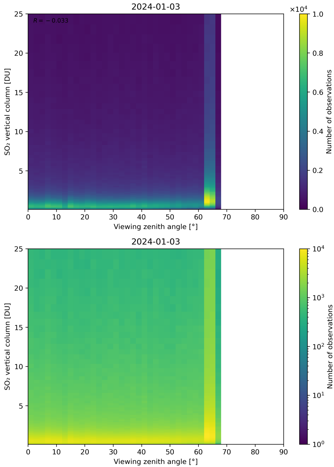
Figure 327: Scatter density plot of “Viewing zenith angle” against “SO 2 vertical column” for 2024-01-02 to 2024-01-04.
