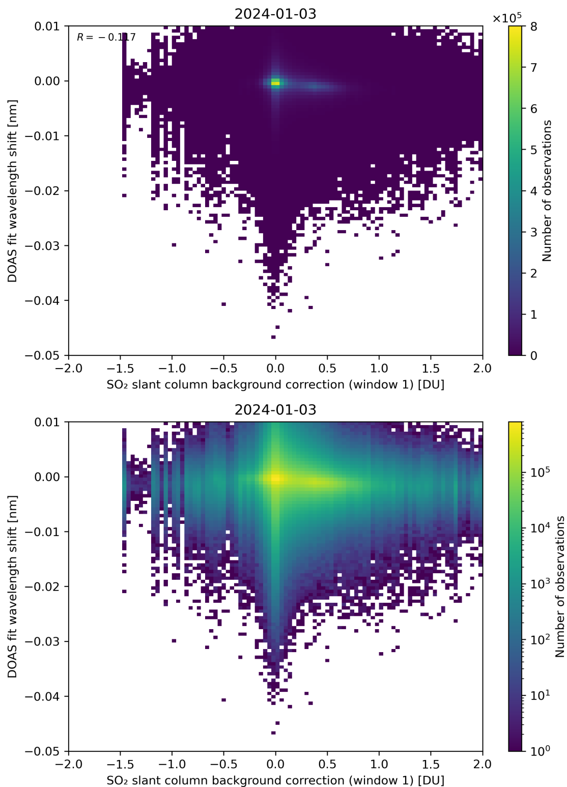
Figure 100: Scatter density plot of “SO 2 slant column background correction (window 1)” against “DOAS fit wavelength shift” for 2024-01-02 to 2024-01-04.
