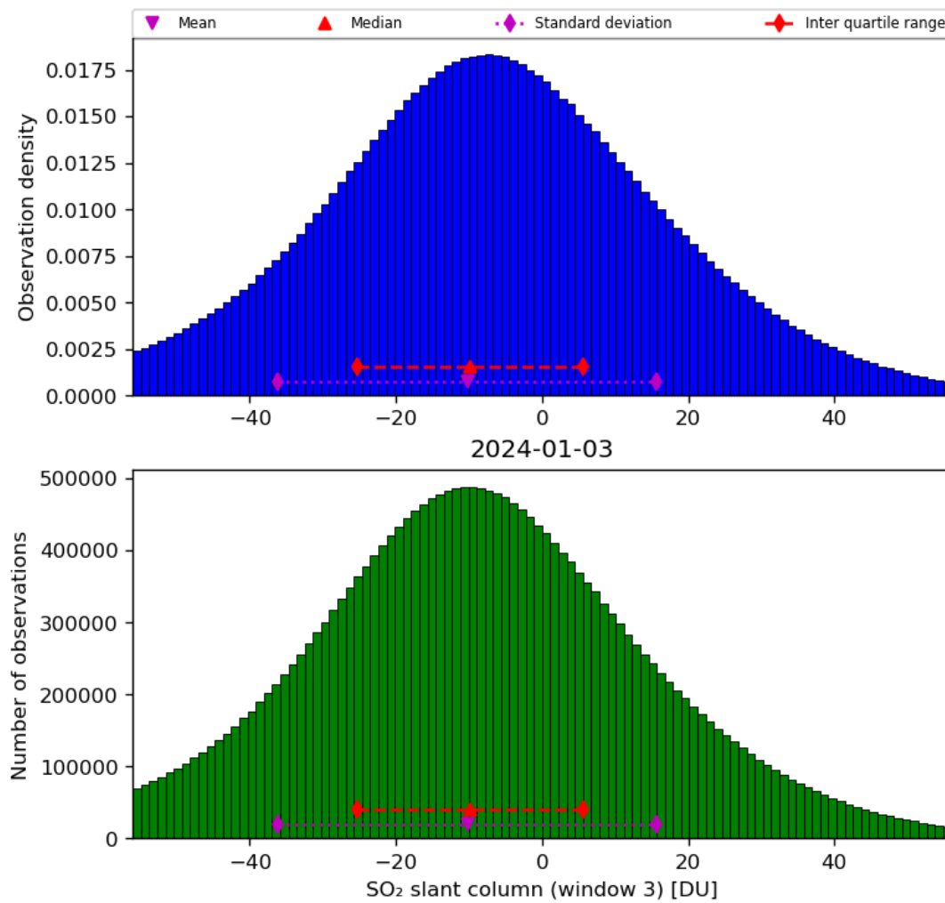
Figure 64: Histogram of “SO 2 slant column (window 3)” for 2024-01-02 to 2024-01-04
