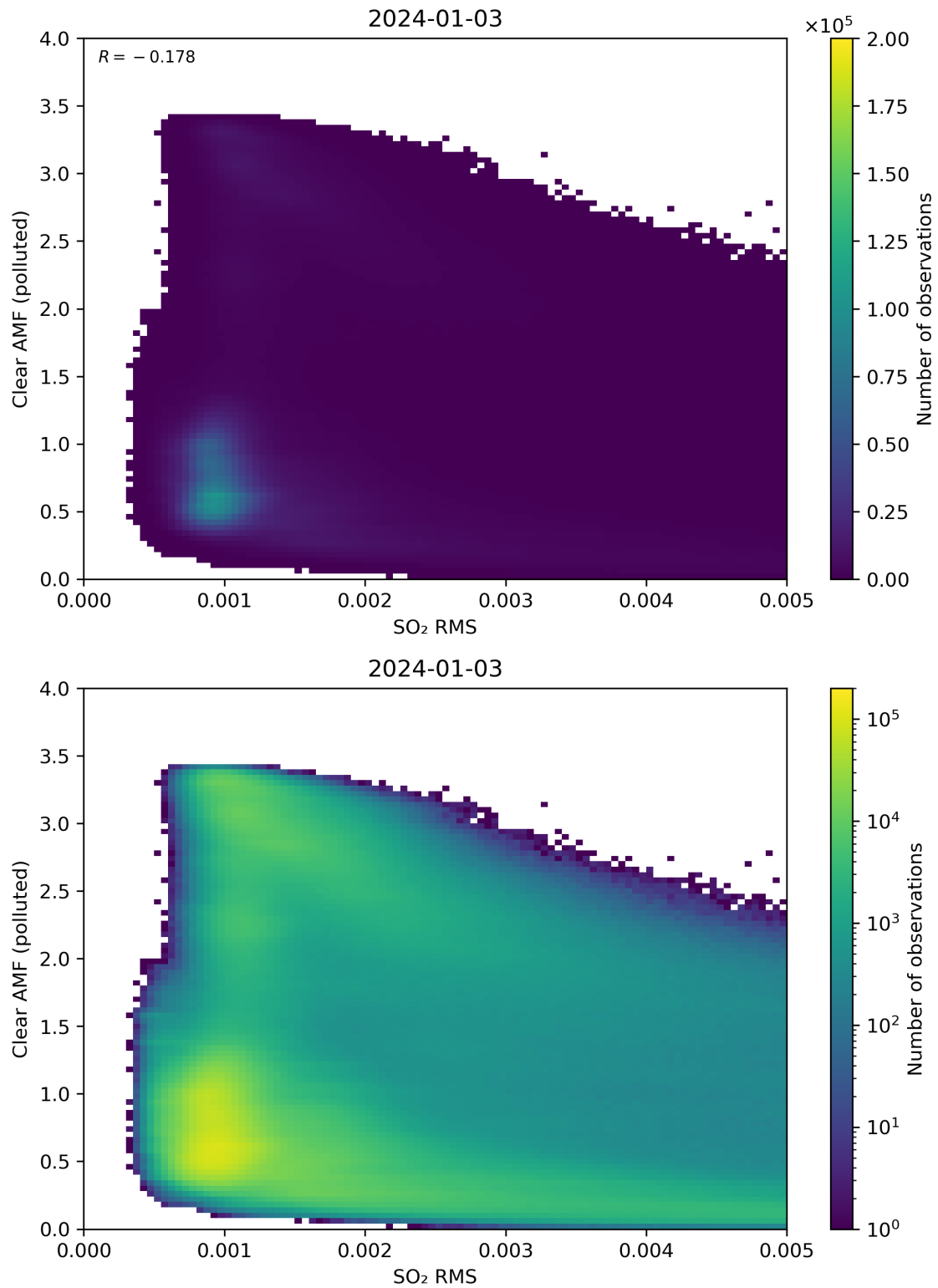
Figure 136: Scatter density plot of “SO 2 RMS” against “Clear AMF (polluted)” for 2024-01-02 to 2024-01-04.
