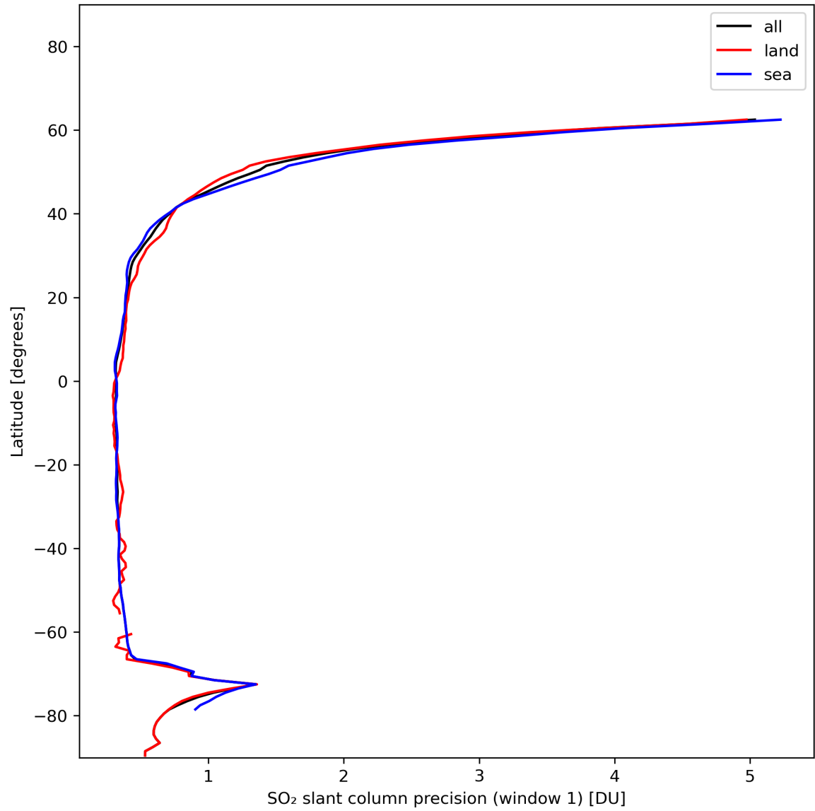
Figure 34: Zonal average of “SO 2 slant column precision (window 1)” for 2024-01-02 to 2024-01-04.
