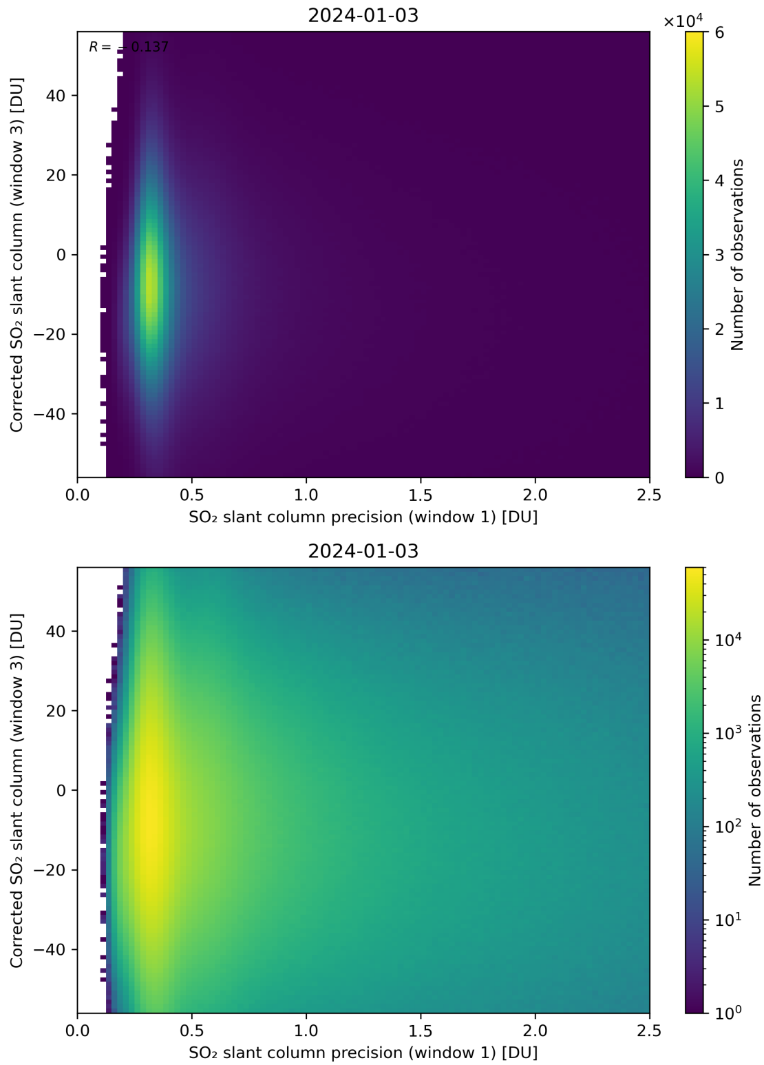
Figure 226: Scatter density plot of “SO 2 slant column precision (window 1)” against “Corrected SO 2 slant column (window 3)” for 2024-01-02 to 2024-01-04.
