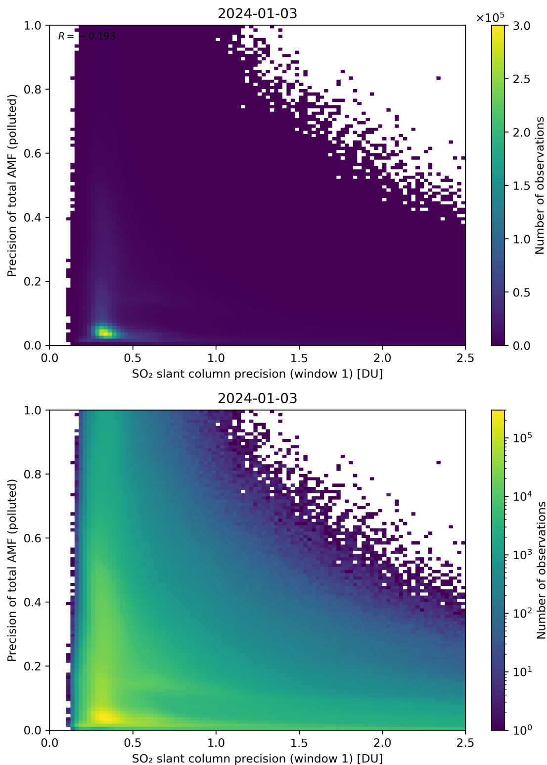
Figure 231: Scatter density plot of “SO 2 slant column precision (window 1)” against “Precision of total AMF (polluted)” for 2024-01-02 to 2024-01-04.
