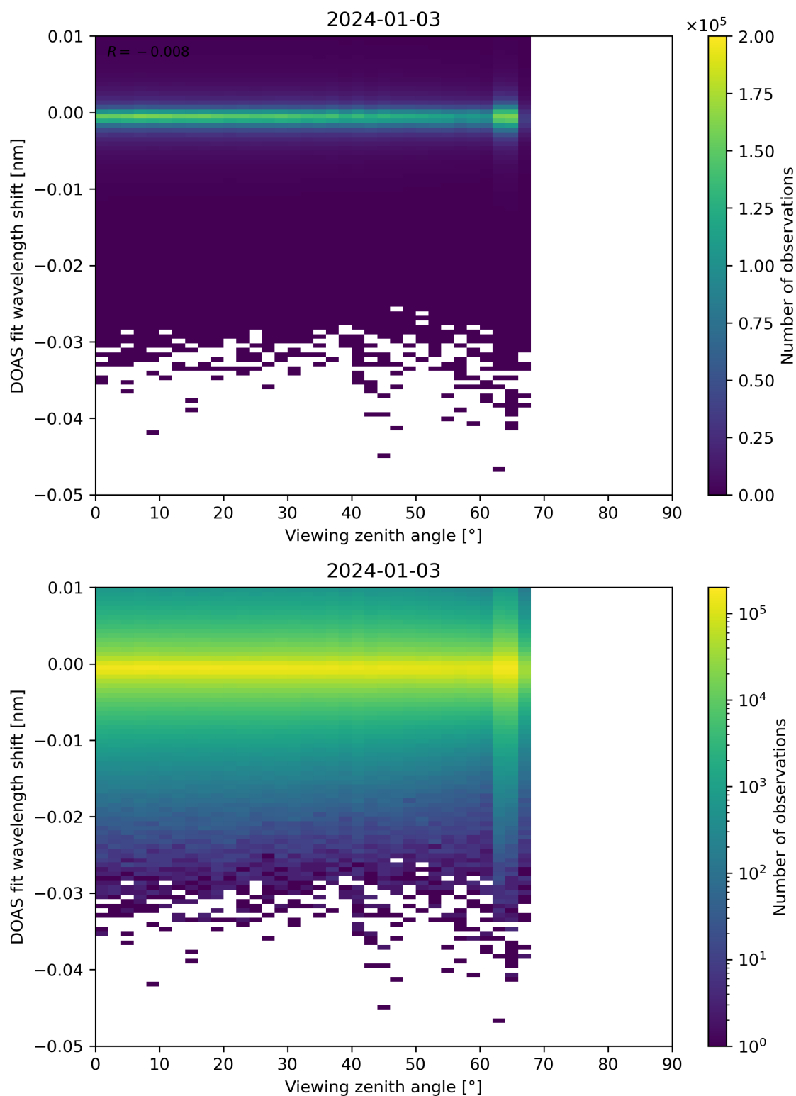
Figure 311: Scatter density plot of “Viewing zenith angle” against “DOAS fit wavelength shift” for 2024-01-02 to 2024-01-04.
