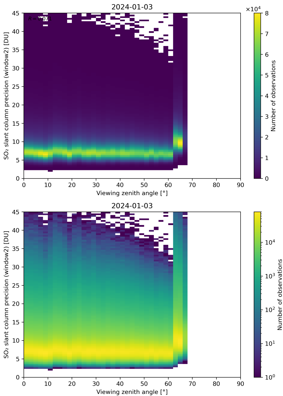
Figure 322: Scatter density plot of “Viewing zenith angle” against “SO 2 slant column precision (window2)” for 2024-01-02 to 2024-01-04.
