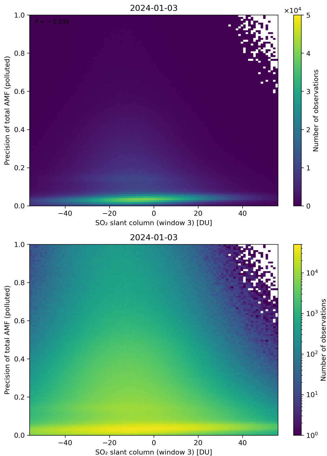
Figure 269: Scatter density plot of “SO 2 slant column (window 3)” against “Precision of total AMF (polluted)” for 2024-01-02 to 2024-01-04.
