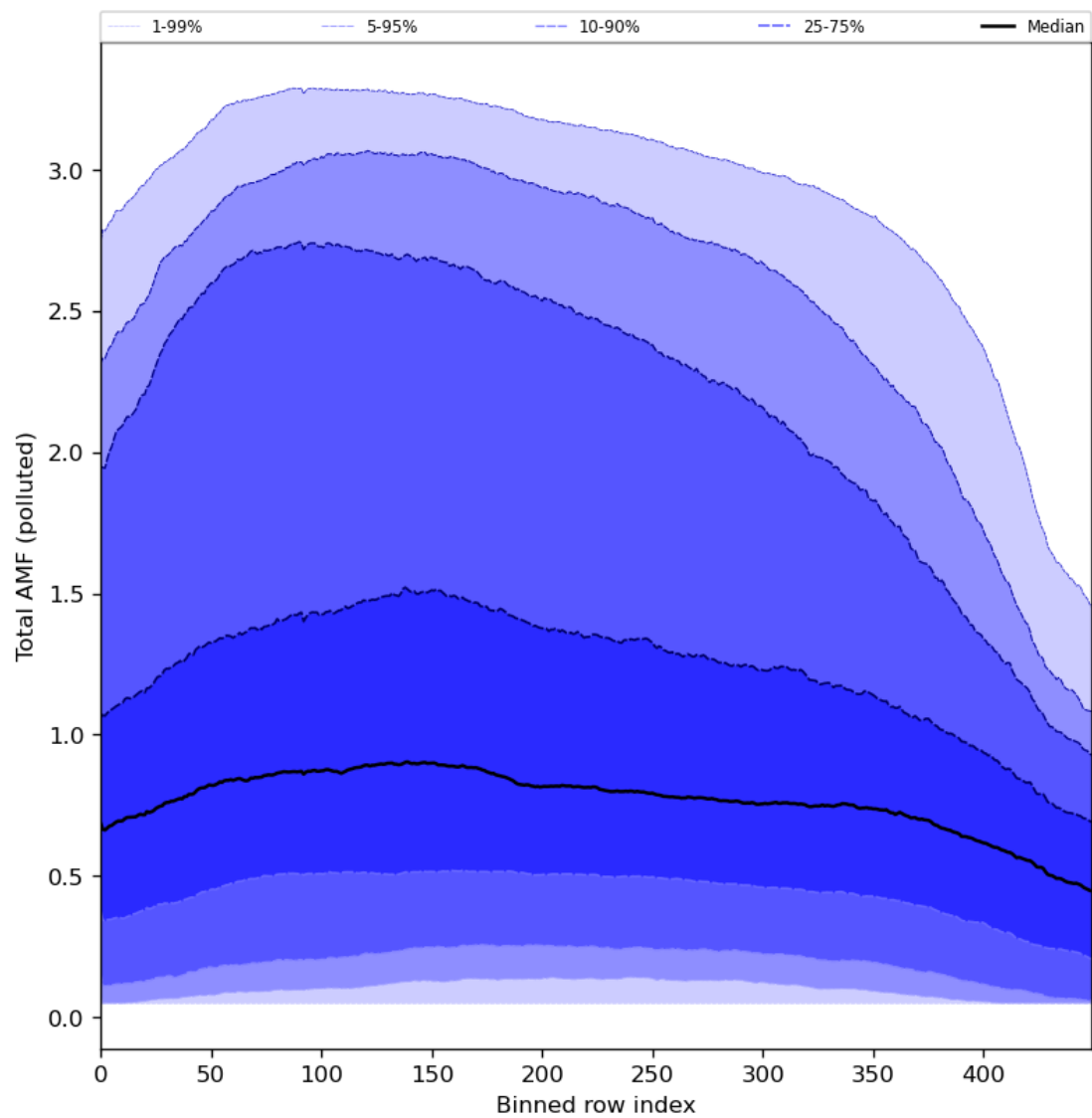
Figure 94: Along track statistics of “Total AMF (polluted)” for 2024-01-02 to 2024-01-04
