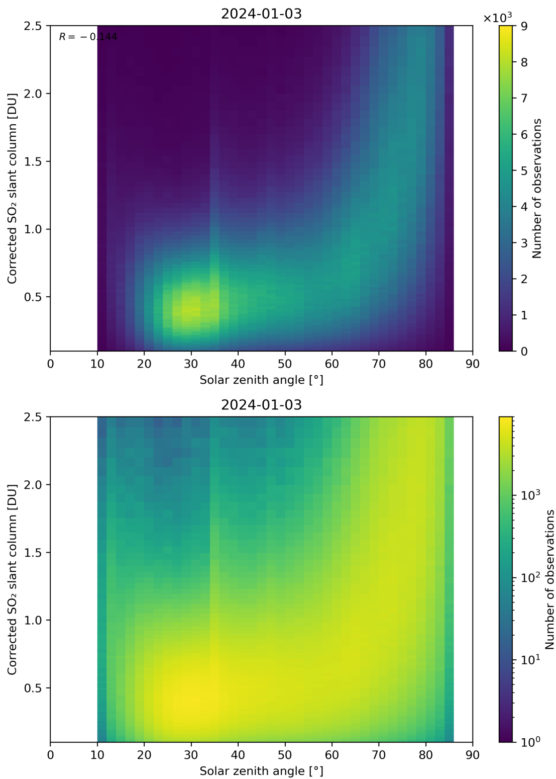
Figure 166: Scatter density plot of “Solar zenith angle” against “Corrected SO 2 slant column” for 2024-01-02 to 2024-01-04.
