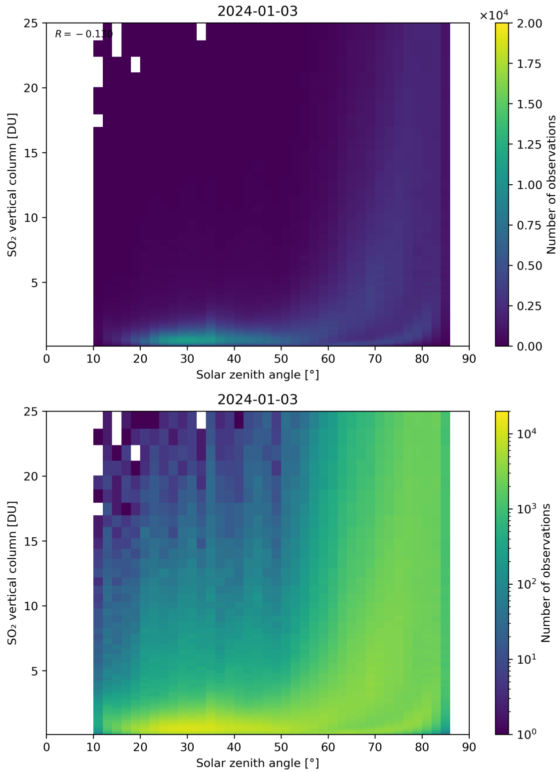
Figure 176: Scatter density plot of “Solar zenith angle” against “SO 2 vertical column” for 2024-01-02 to 2024-01-04.
