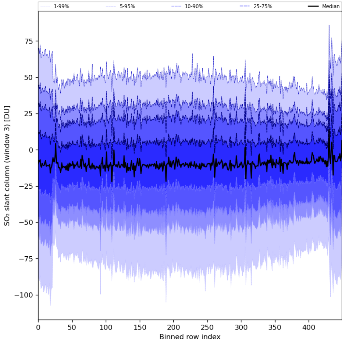
Figure 87: Along track statistics of “SO 2 slant column (window 3)” for 2024-01-02 to 2024-01-04
