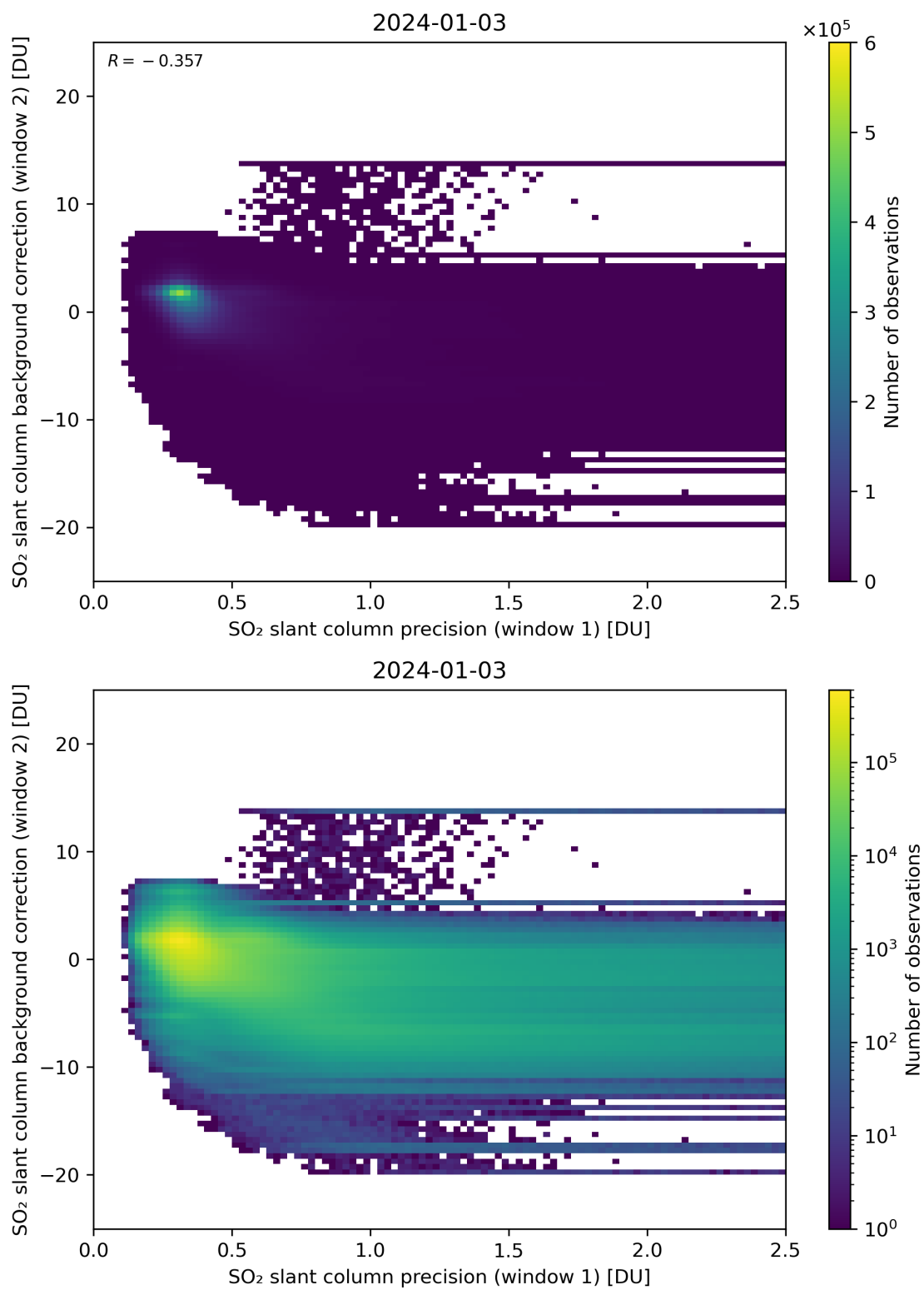
Figure 219: Scatter density plot of “SO 2 slant column precision (window 1)” against “SO 2 slant column background correction (window 2)” for 2024-01-02 to 2024-01-04.
