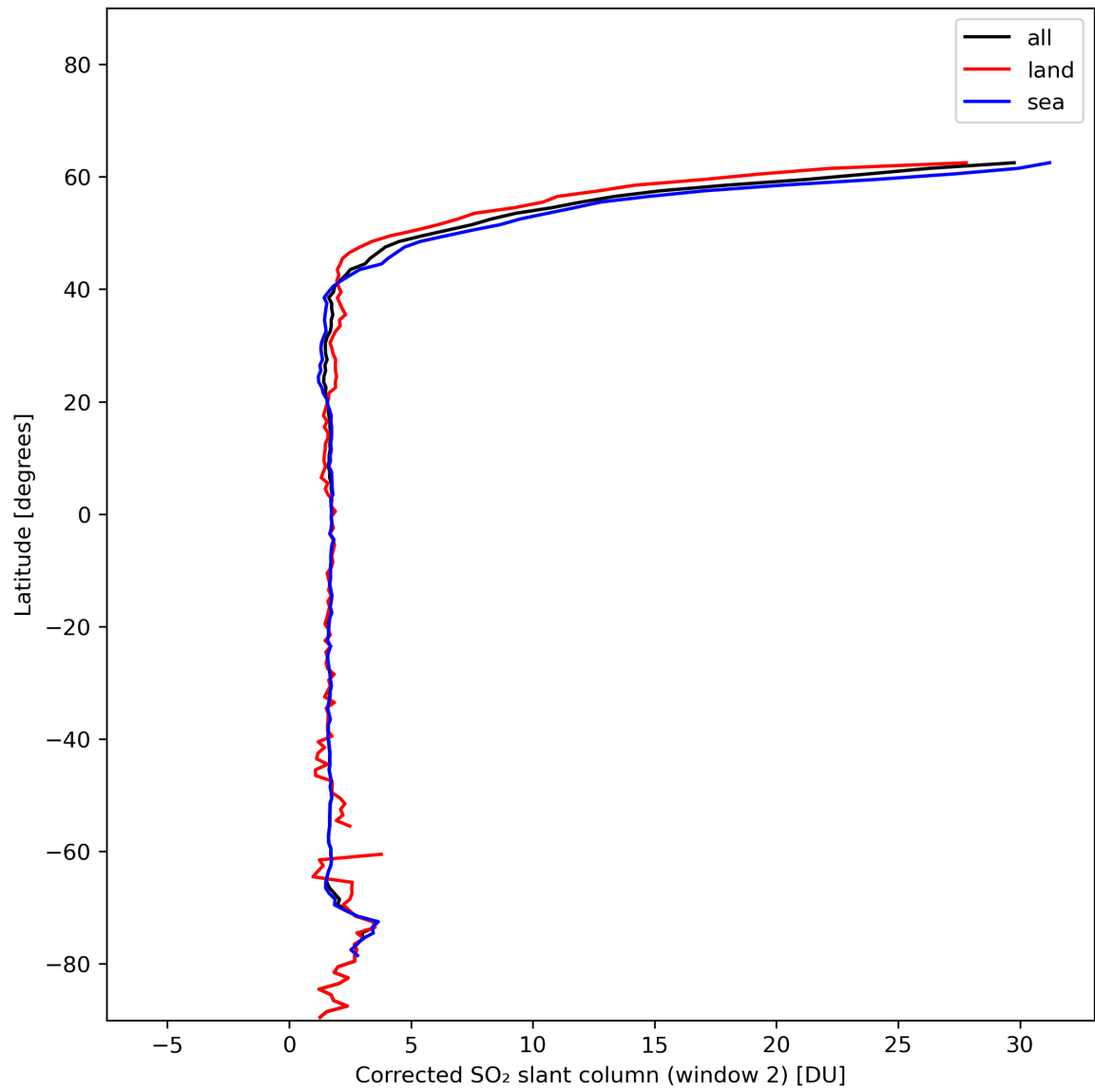
Figure 39: Zonal average of “Corrected SO 2 slant column (window 2)” for 2024-01-02 to 2024-01-04.
