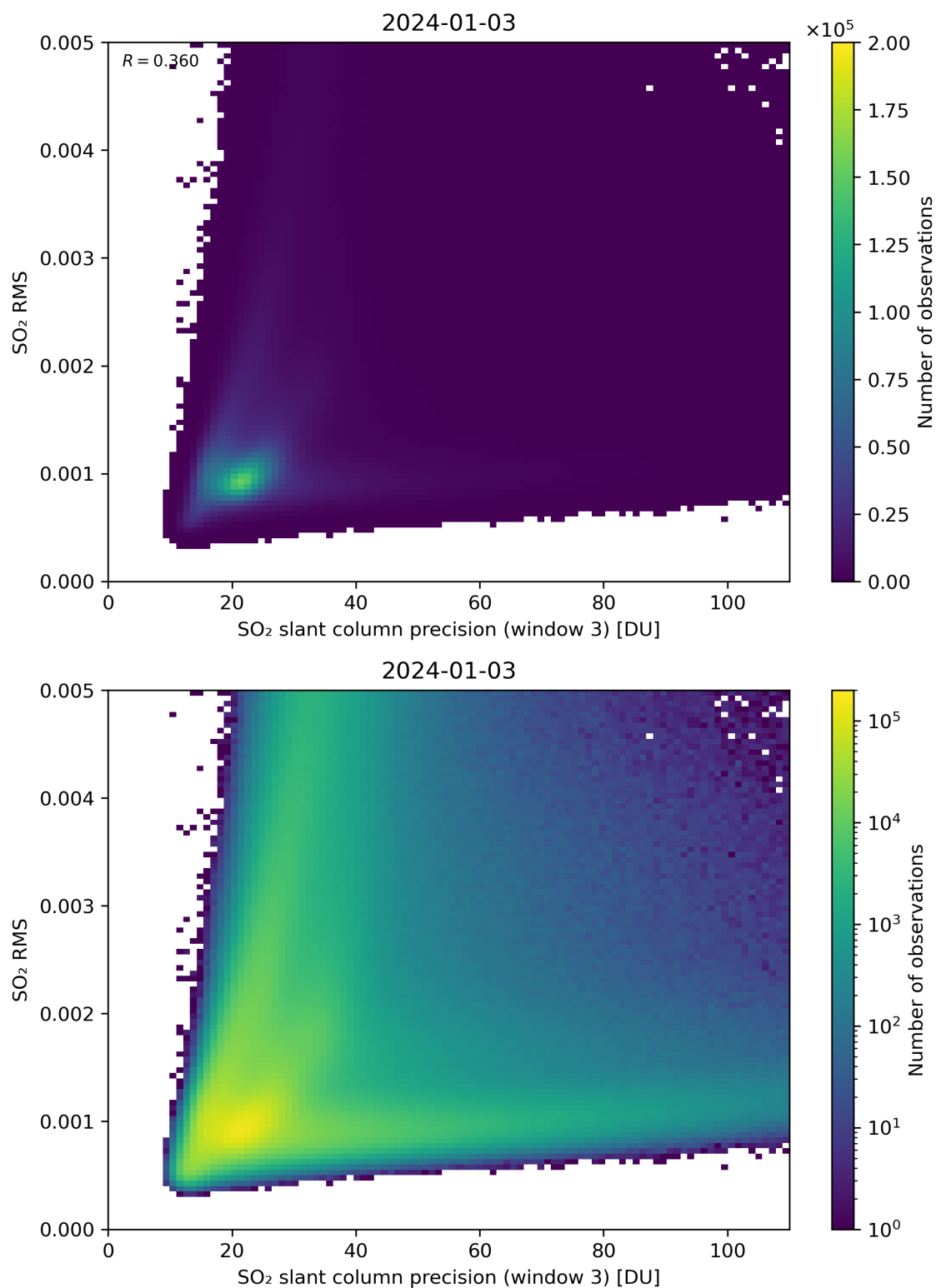
Figure 260: Scatter density plot of “SO 2 slant column precision (window 3)” against “SO 2 RMS” for 2024-01-02 to 2024-01-04.
