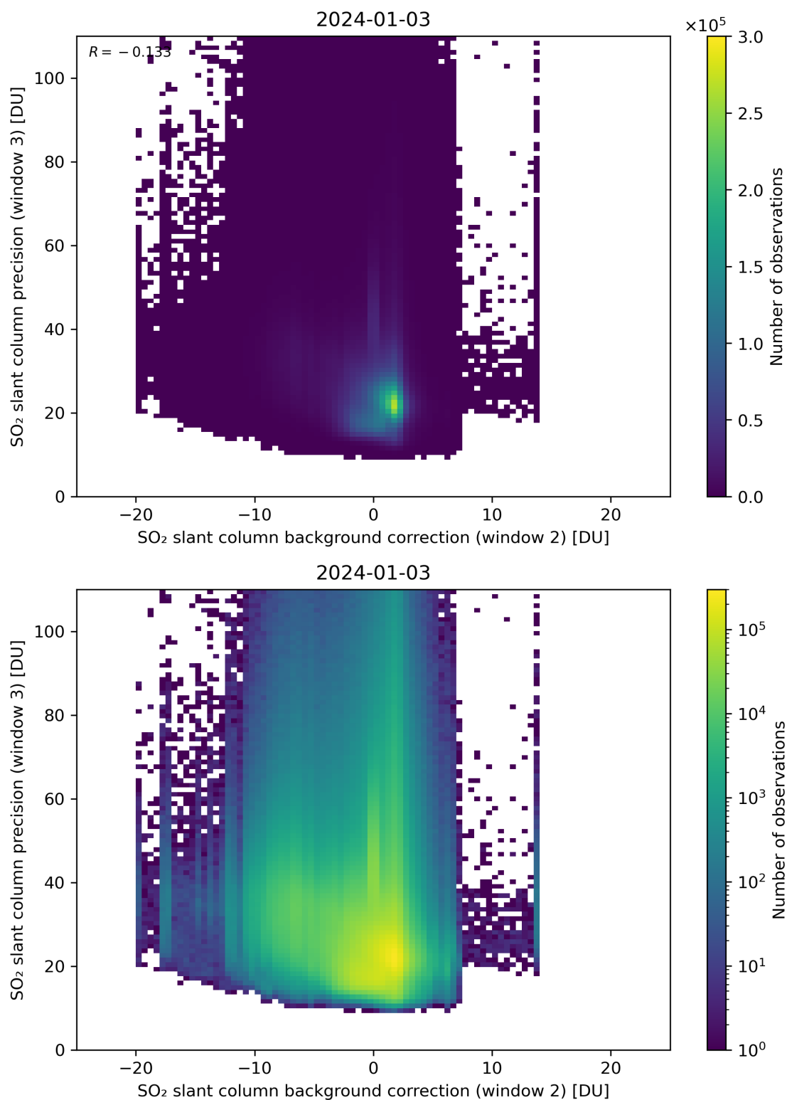
Figure 118: Scatter density plot of “SO 2 slant column background correction (window 2)” against “SO 2 slant column precision (window 3)” for 2024-01-02 to 2024-01-04.
