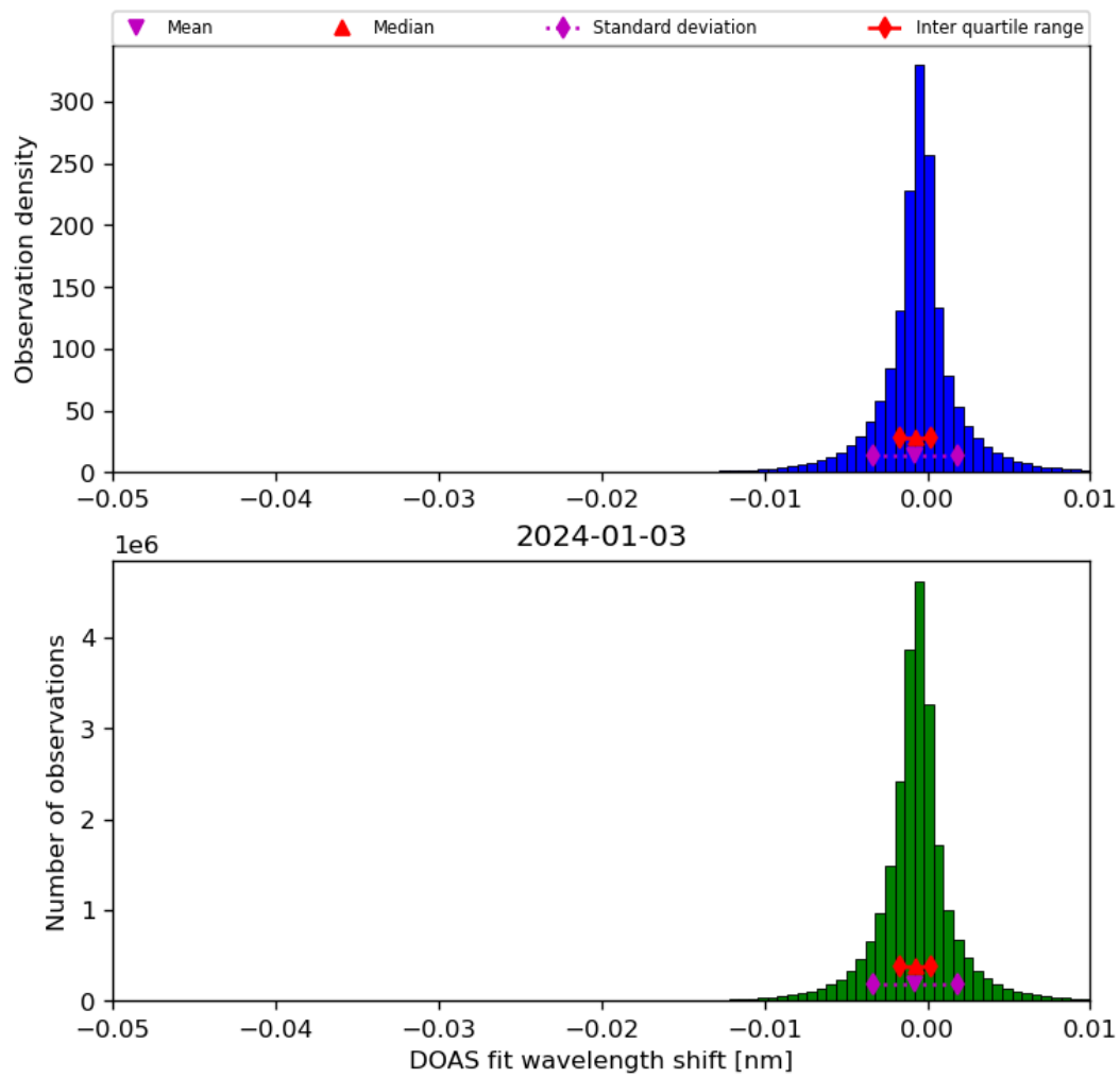
Figure 68: Histogram of “DOAS fit wavelength shift” for 2024-01-02 to 2024-01-04
