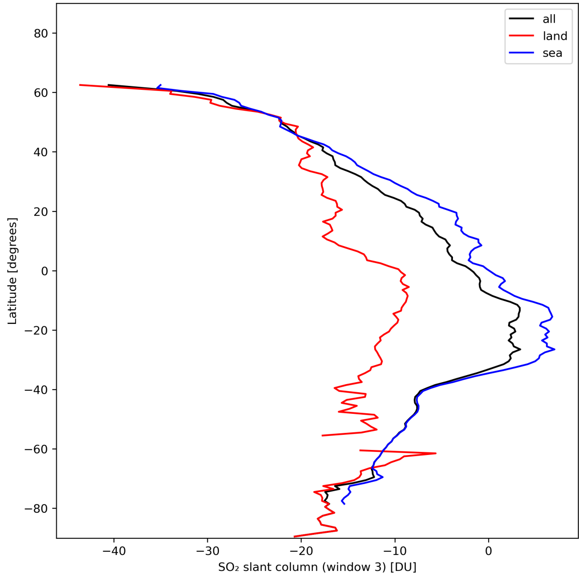
Figure 41: Zonal average of “SO 2 slant column (window 3)” for 2024-01-02 to 2024-01-04.
