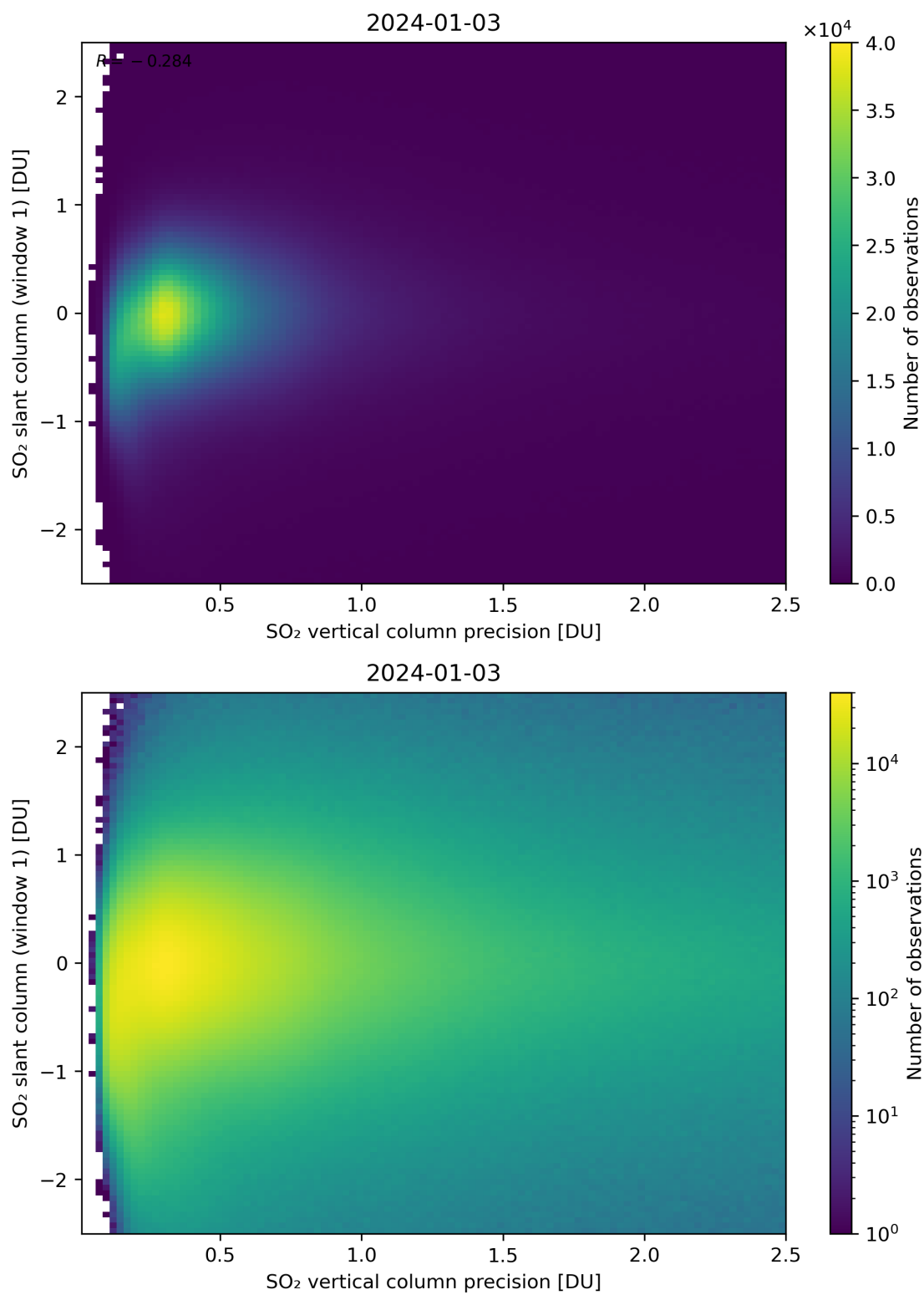
Figure 289: Scatter density plot of “SO 2 vertical column precision” against “SO 2 slant column (window 1)” for 2024-01-02 to 2024-01-04.
