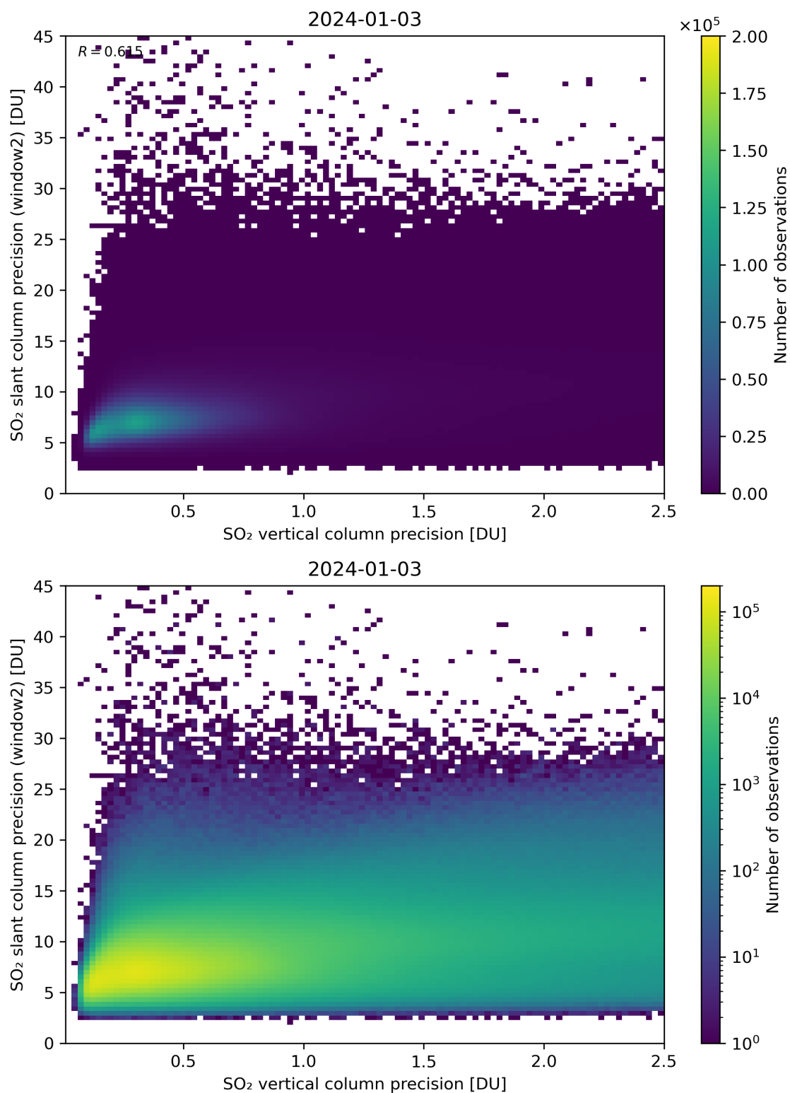
Figure 291: Scatter density plot of “SO 2 vertical column precision” against “SO 2 slant column precision (window2)” for 2024-01-02 to 2024-01-04.
