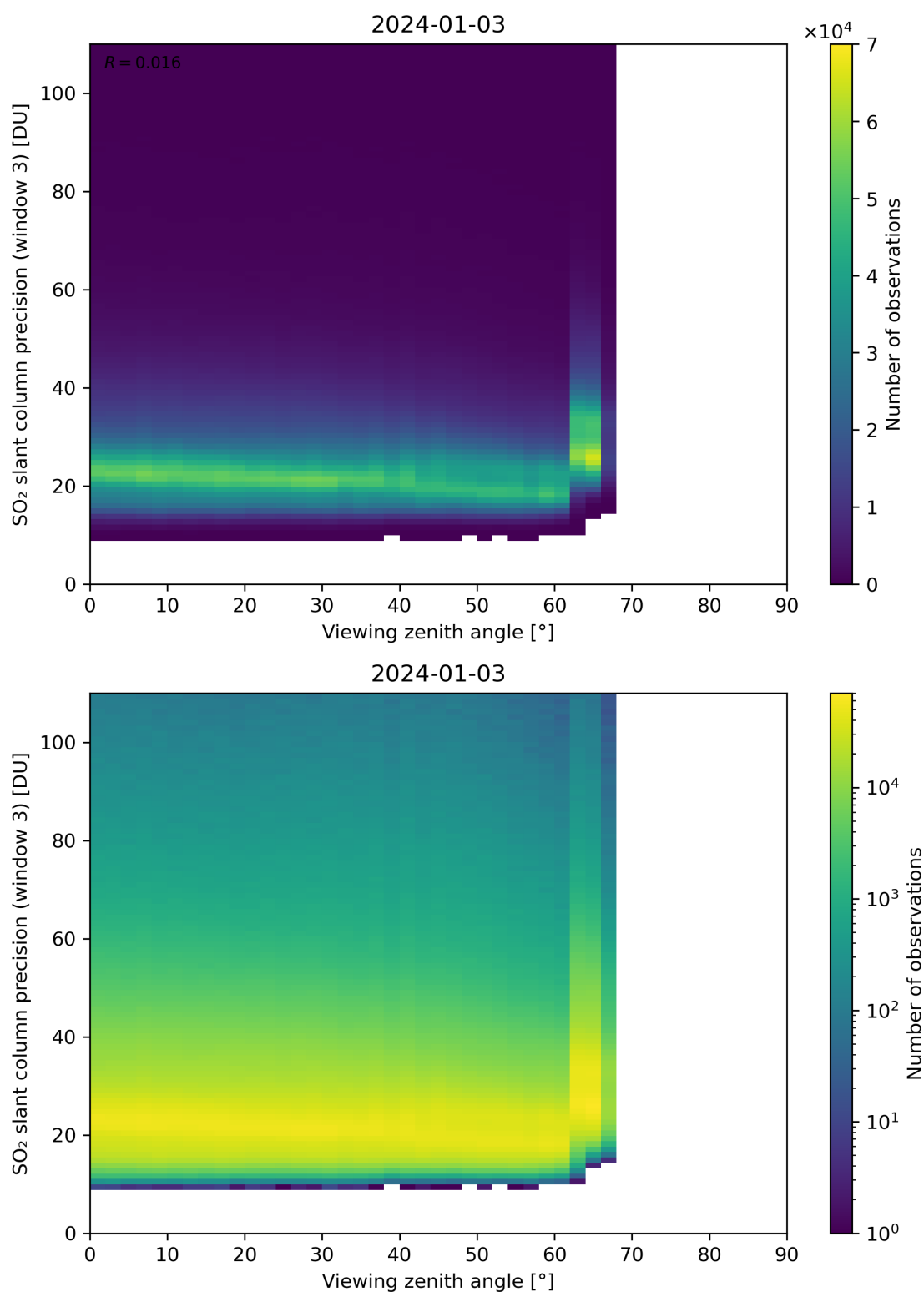
Figure 324: Scatter density plot of “Viewing zenith angle” against “SO 2 slant column precision (window 3)” for 2024-01-02 to 2024-01-04.
