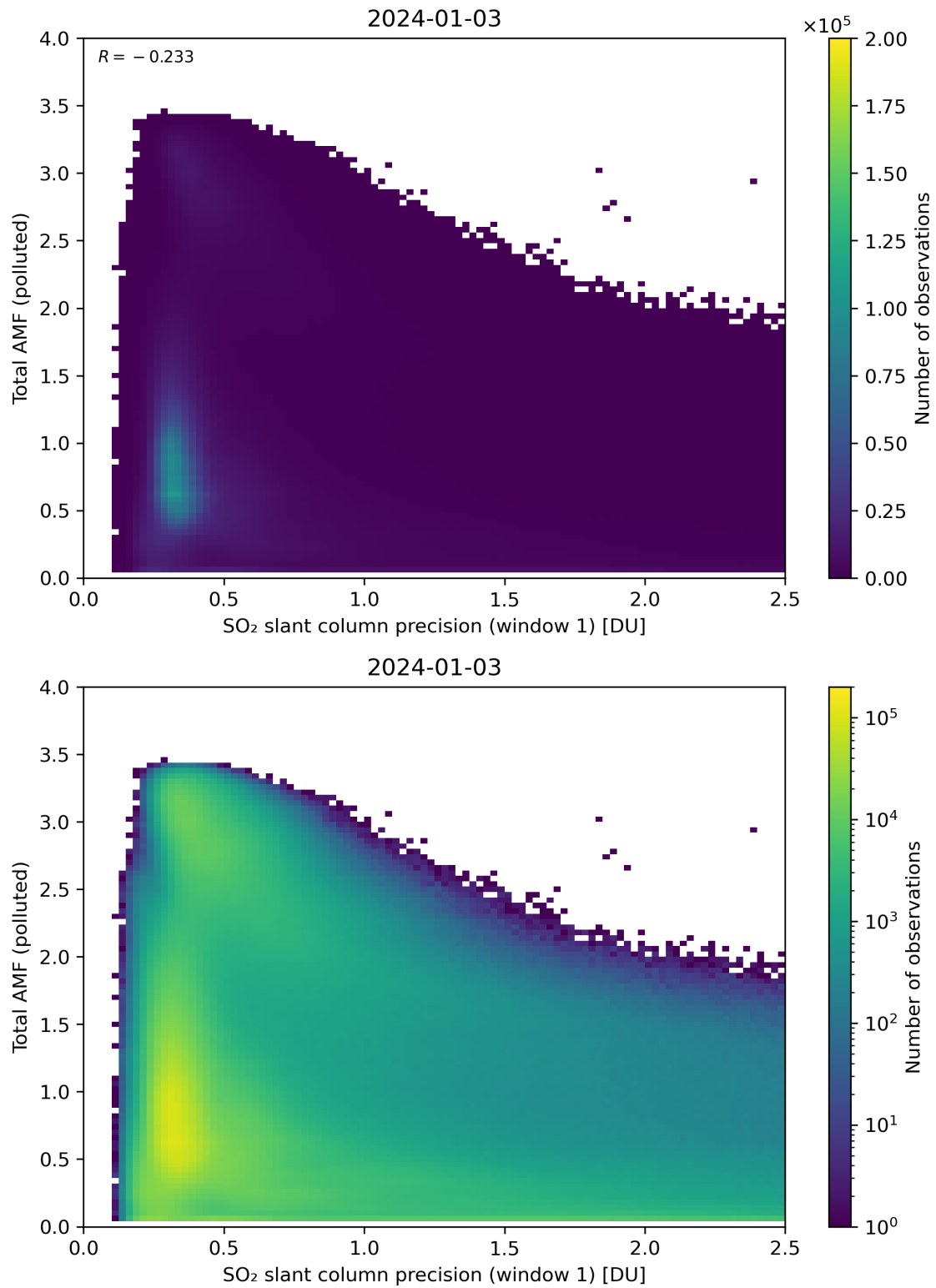
Figure 230: Scatter density plot of “SO 2 slant column precision (window 1)” against “Total AMF (polluted)” for 2024-01-02 to 2024-01-04.
