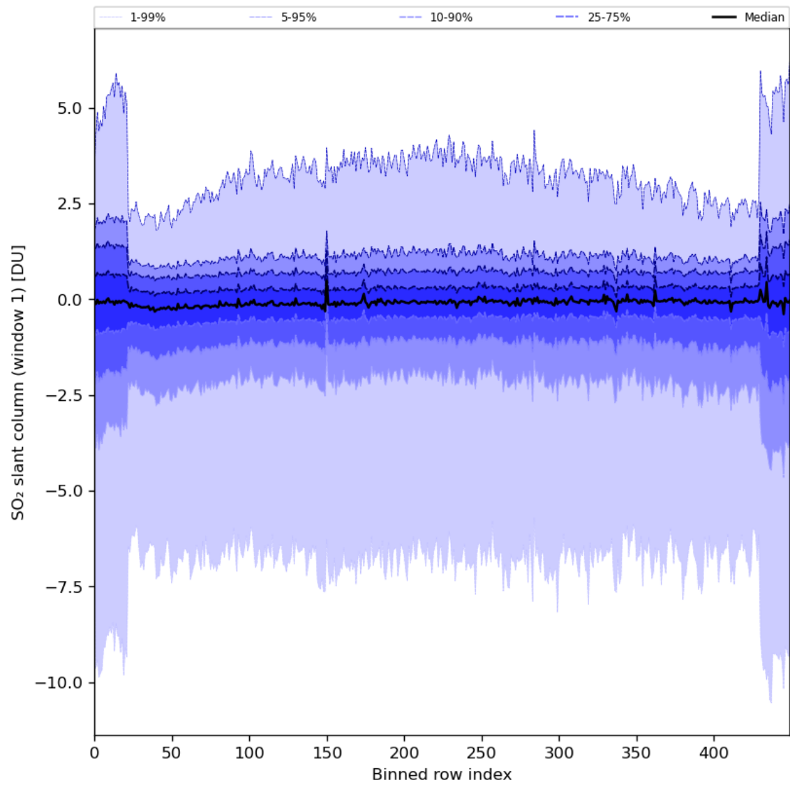
Figure 79: Along track statistics of “SO 2 slant column (window 1)” for 2024-01-02 to 2024-01-04
