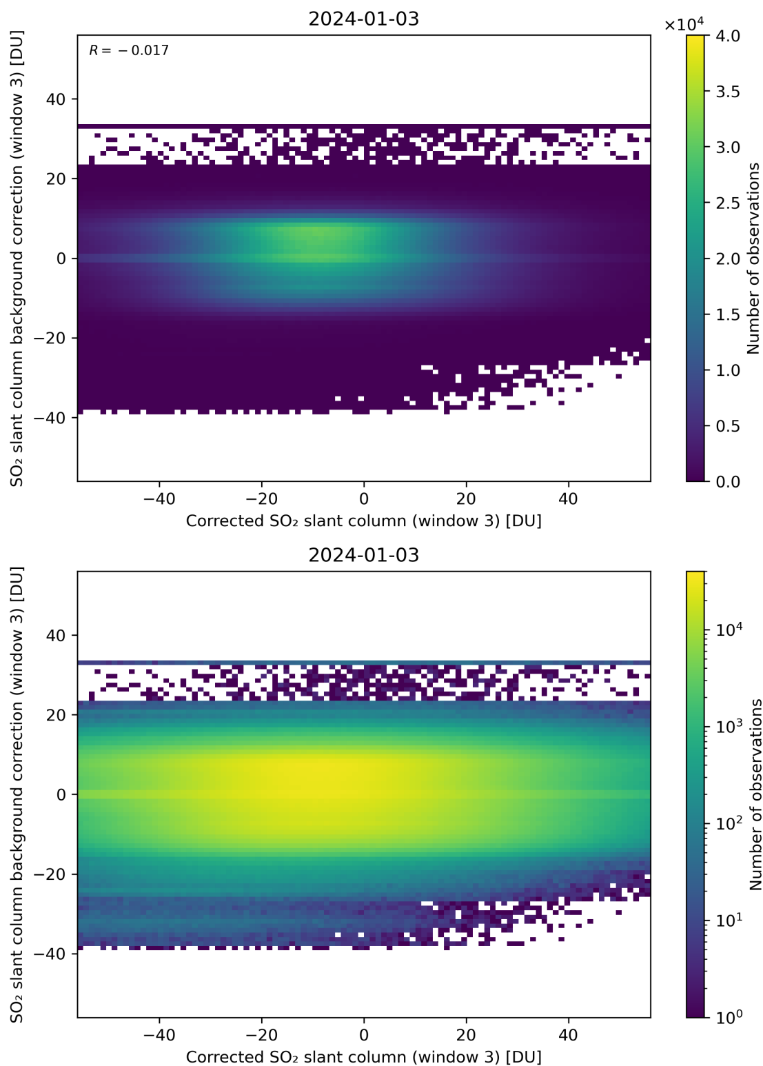
Figure 205: Scatter density plot of “Corrected SO 2 slant column (window 3)” against “SO 2 slant column background correction (window 3)” for 2024-01-02 to 2024-01-04.
