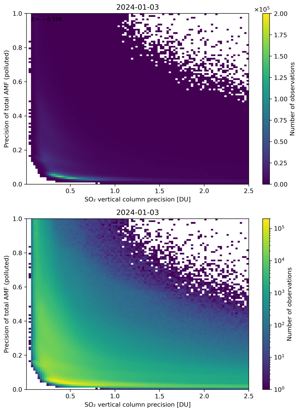
Figure 295: Scatter density plot of “SO 2 vertical column precision” against “Precision of total AMF (polluted)” for 2024-01-02 to 2024-01-04.
