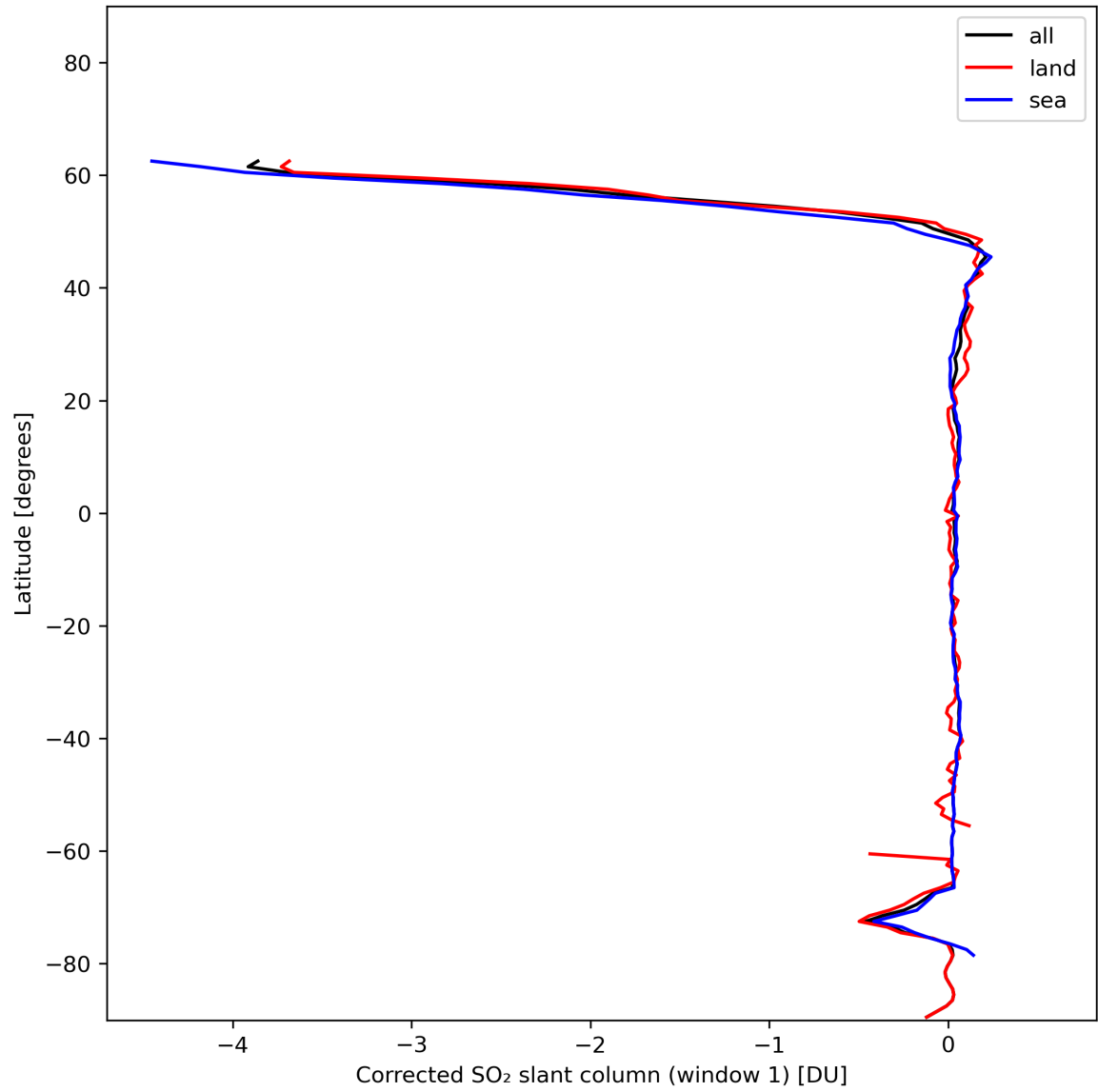
Figure 35: Zonal average of “Corrected SO 2 slant column (window 1)” for 2024-01-02 to 2024-01-04.
