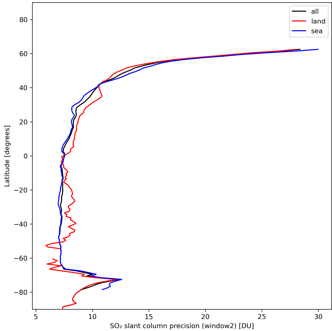
Figure 38: Zonal average of “SO 2 slant column precision (window2)” for 2024-01-02 to 2024-01-04.
