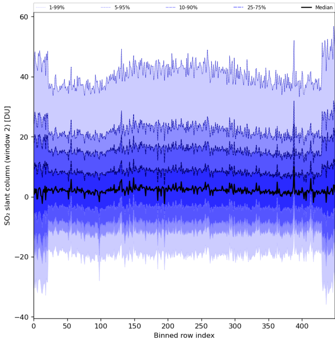
Figure 83: Along track statistics of “SO 2 slant column (window 2)” for 2024-01-02 to 2024-01-04
