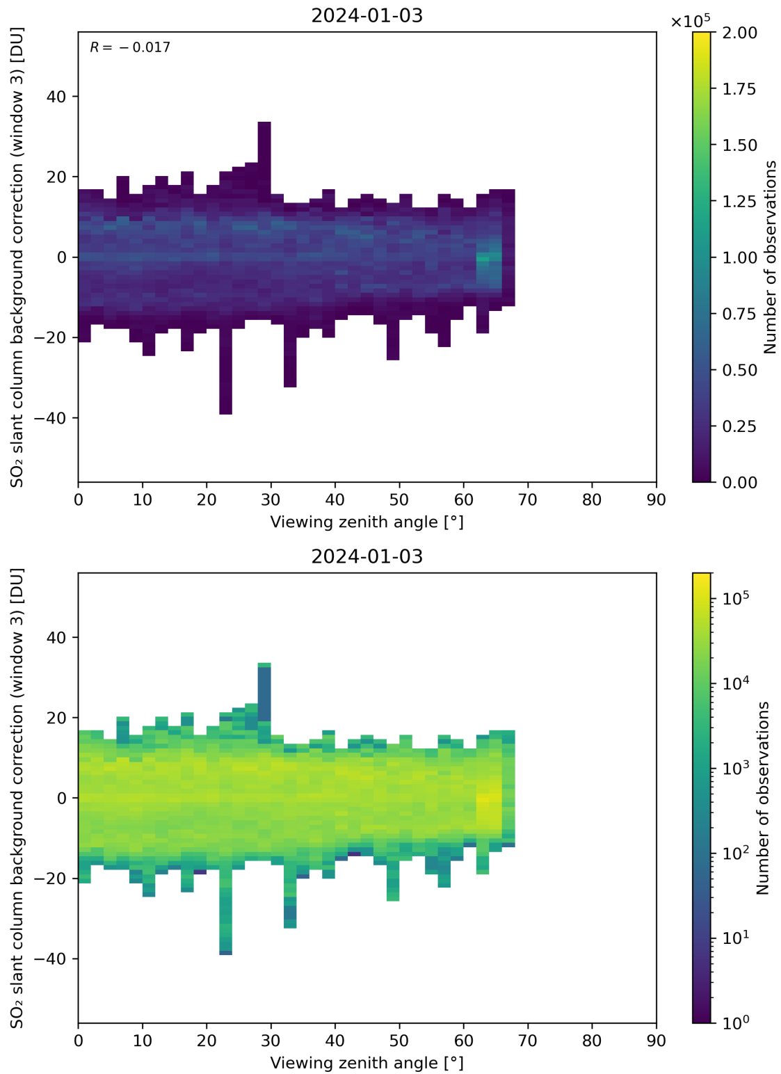
Figure 310: Scatter density plot of “Viewing zenith angle” against “SO 2 slant column background correction (window 3)” for 2024-01-02 to 2024-01-04.
