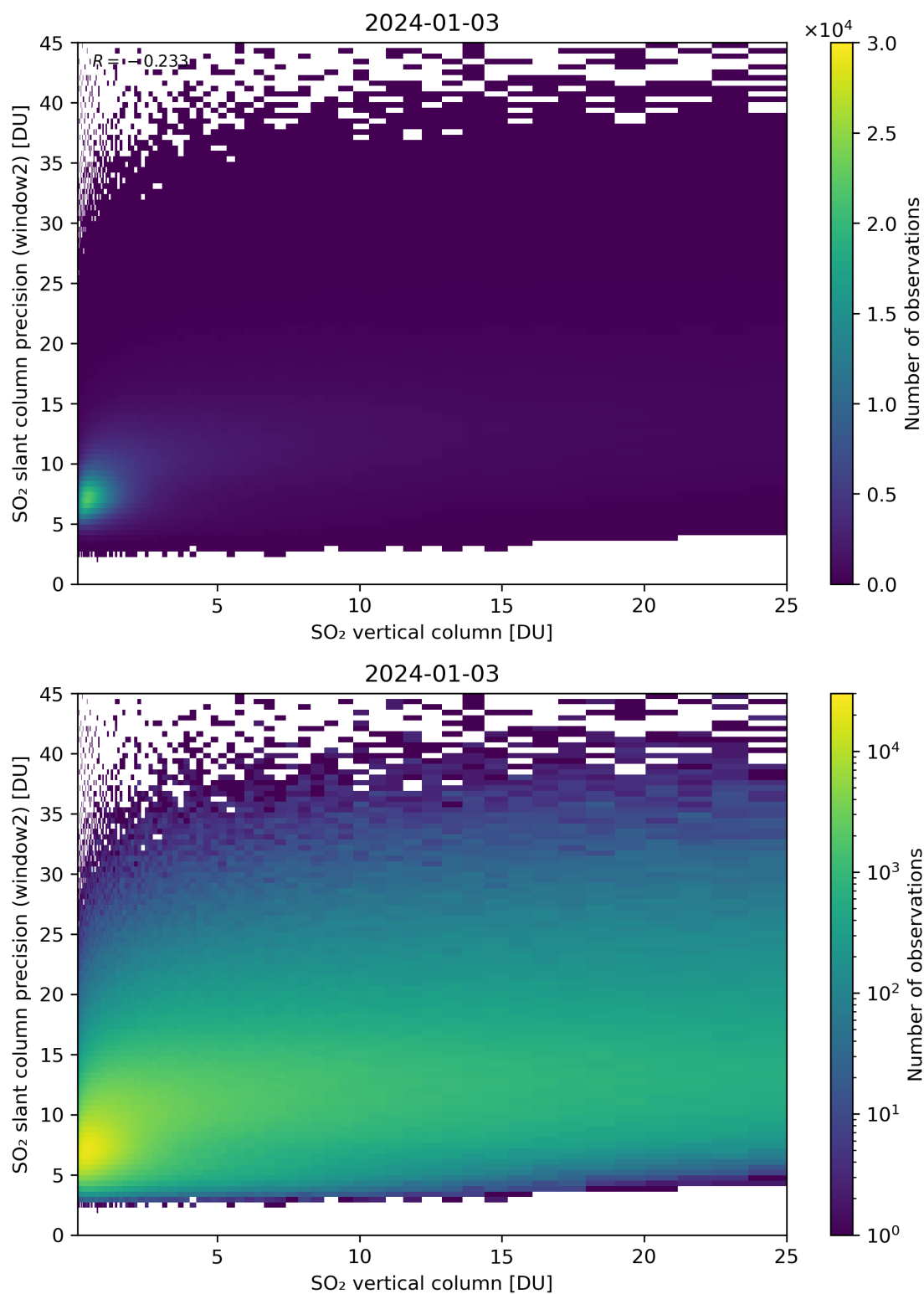
Figure 302: Scatter density plot of “SO 2 vertical column” against “SO 2 slant column precision (window2)” for 2024-01-02 to 2024-01-04.
