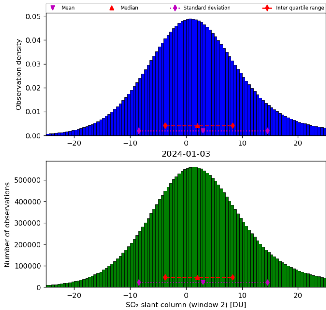
Figure 60: Histogram of “SO 2 slant column (window 2)” for 2024-01-02 to 2024-01-04
