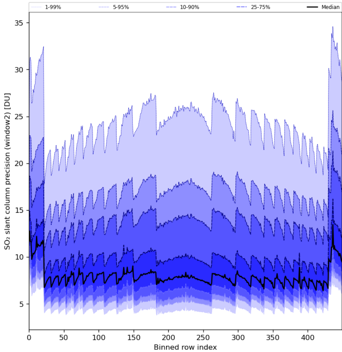
Figure 84: Along track statistics of “SO 2 slant column precision (window2)” for 2024-01-02 to 2024-01-04
