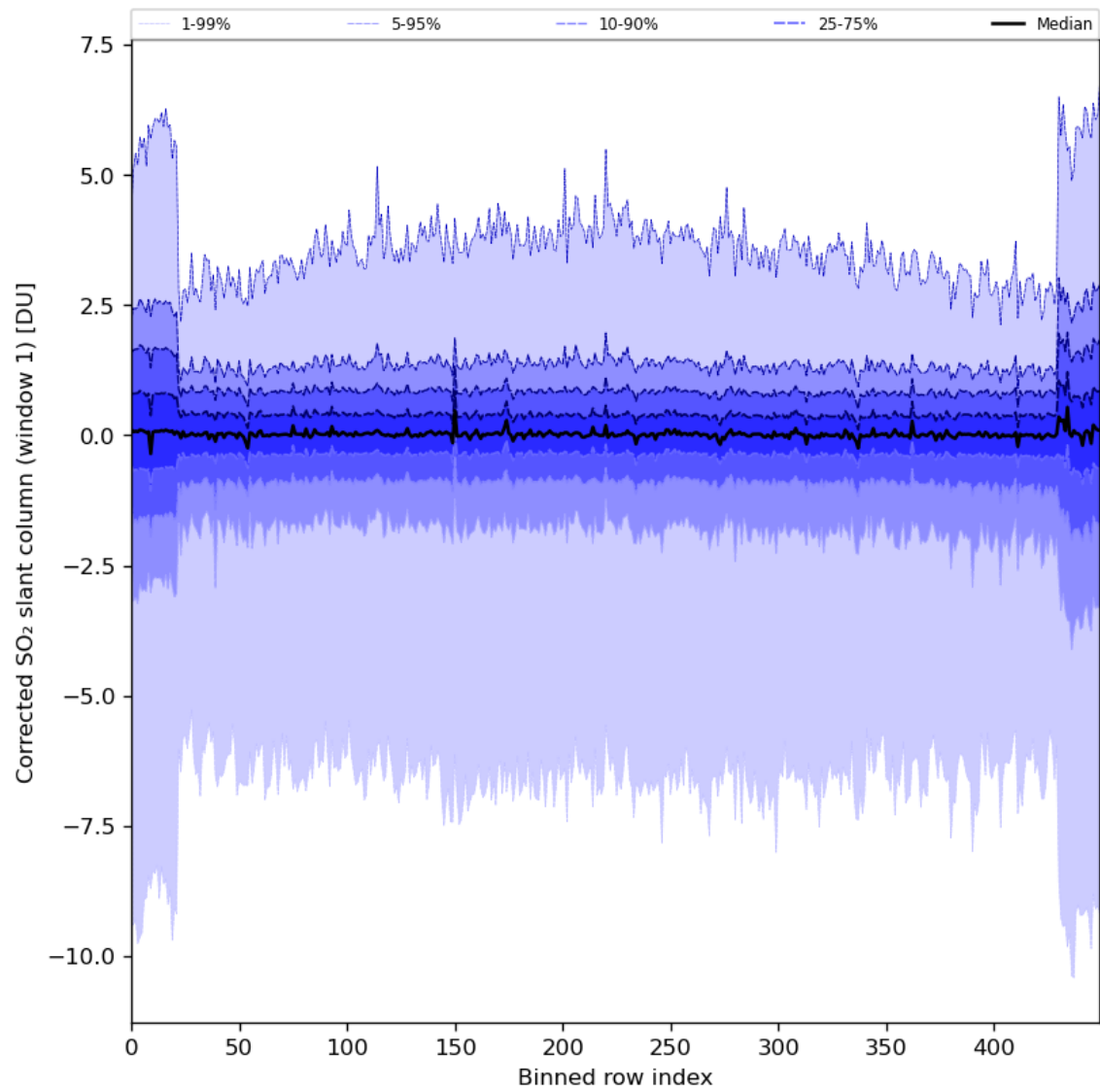
Figure 81: Along track statistics of “Corrected SO 2 slant column (window 1)” for 2024-01-02 to 2024-01-04
