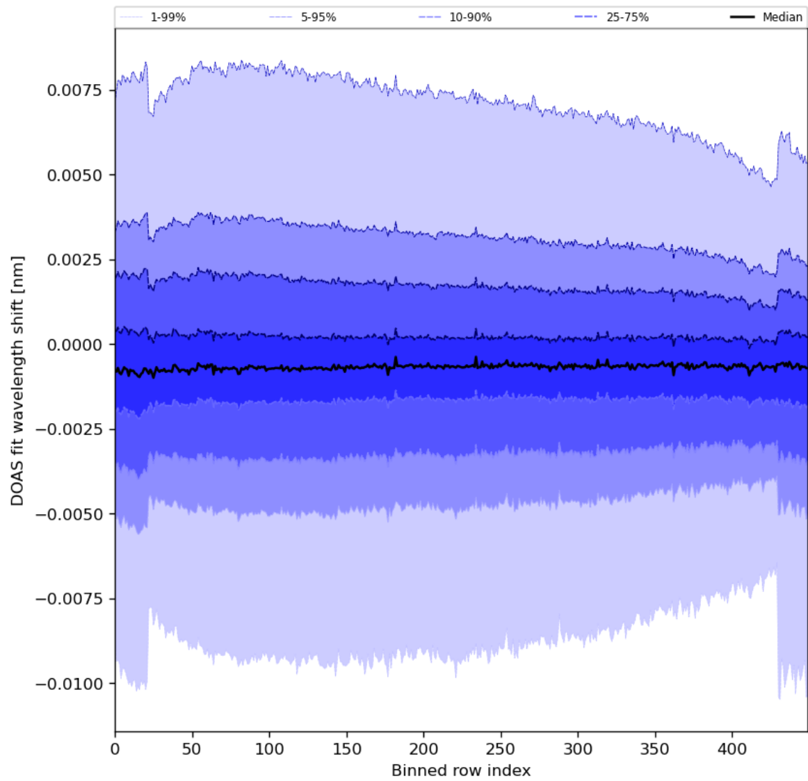
Figure 91: Along track statistics of “DOAS fit wavelength shift” for 2024-01-02 to 2024-01-04
