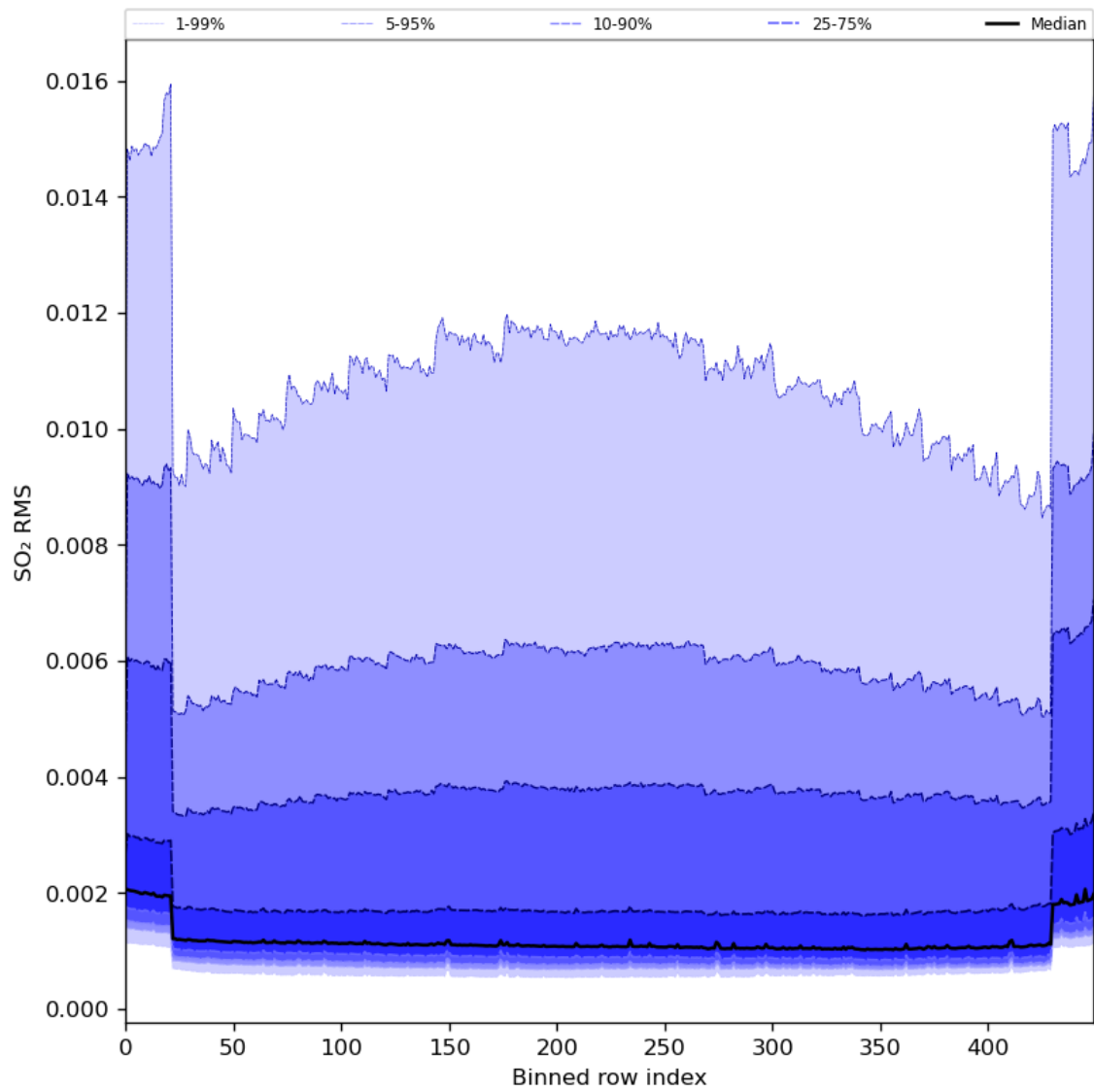
Figure 93: Along track statistics of “SO 2 RMS” for 2024-01-02 to 2024-01-04
