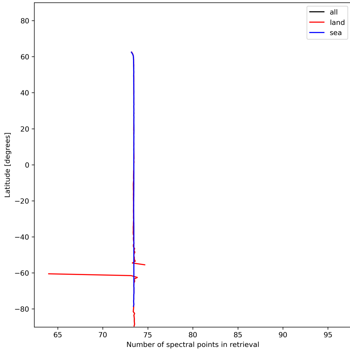
Figure 51: Zonal average of “Number of spectral points in retrieval” for 2024-01-02 to 2024-01-04.
