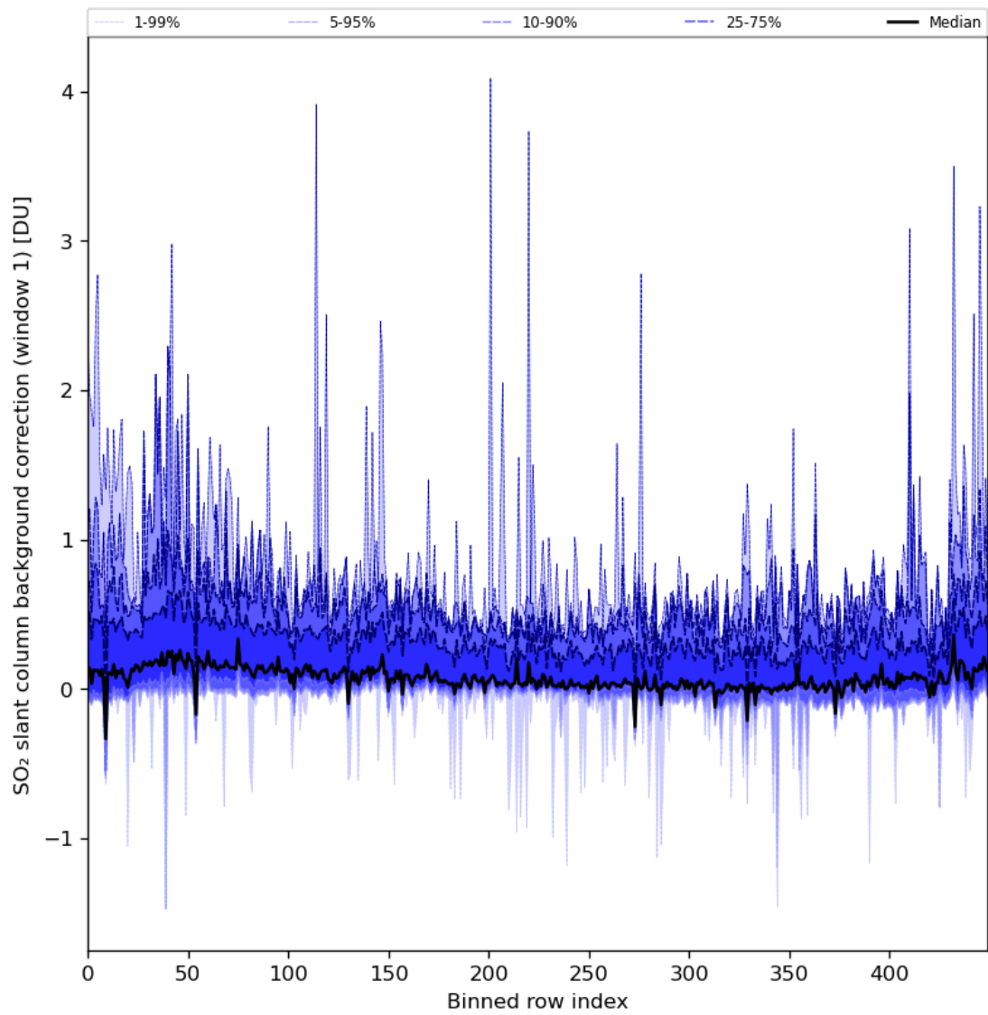
Figure 82: Along track statistics of “SO 2 slant column background correction (window 1)” for 2024-01-02 to 2024-01-04
