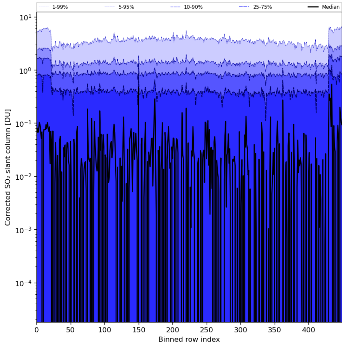
Figure 78: Along track statistics of “Corrected SO 2 slant column” for 2024-01-02 to 2024-01-04
