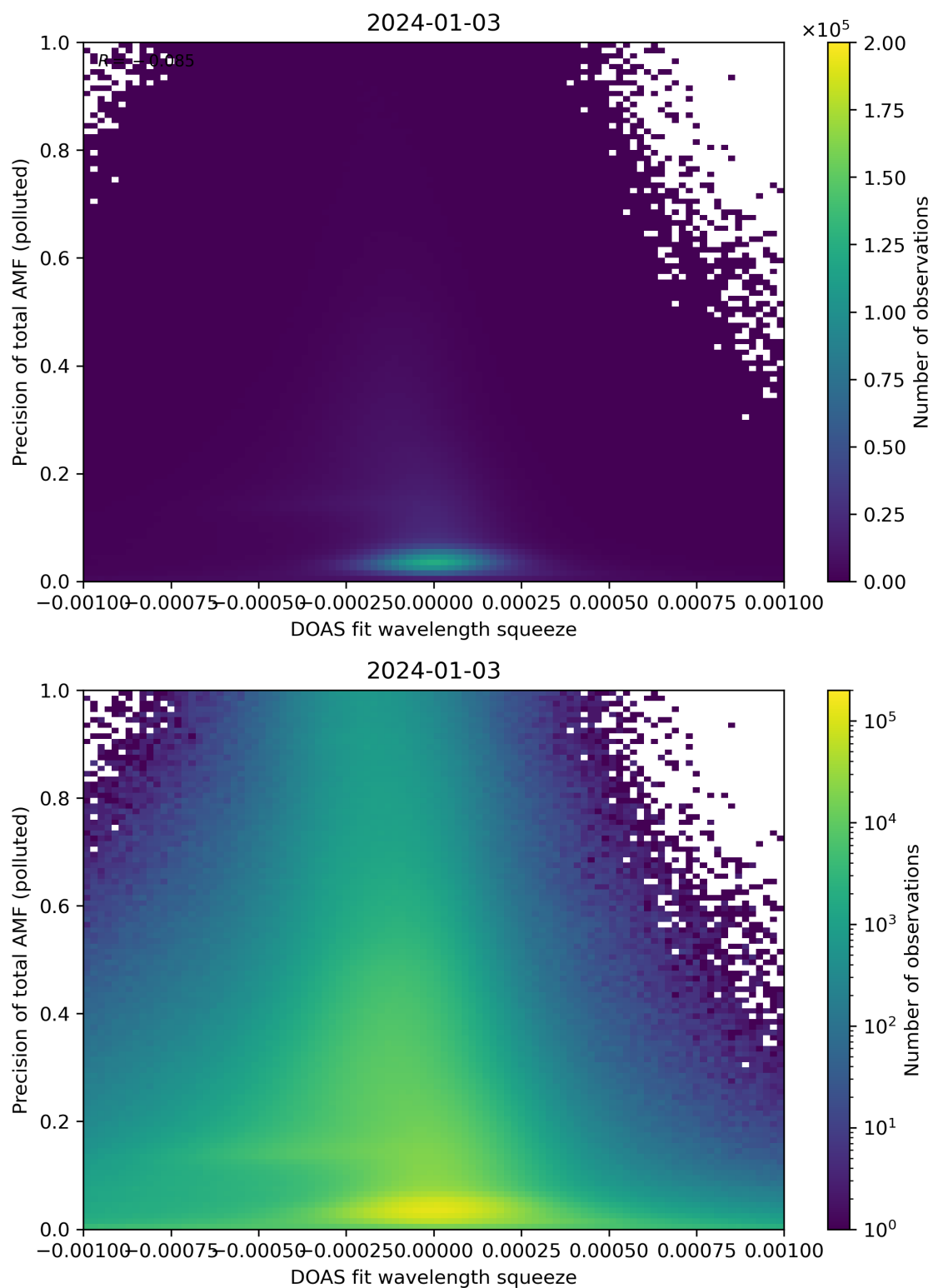
Figure 135: Scatter density plot of “DOAS fit wavelength squeeze” against “Precision of total AMF (polluted)” for 2024-01-02 to 2024-01-04.
