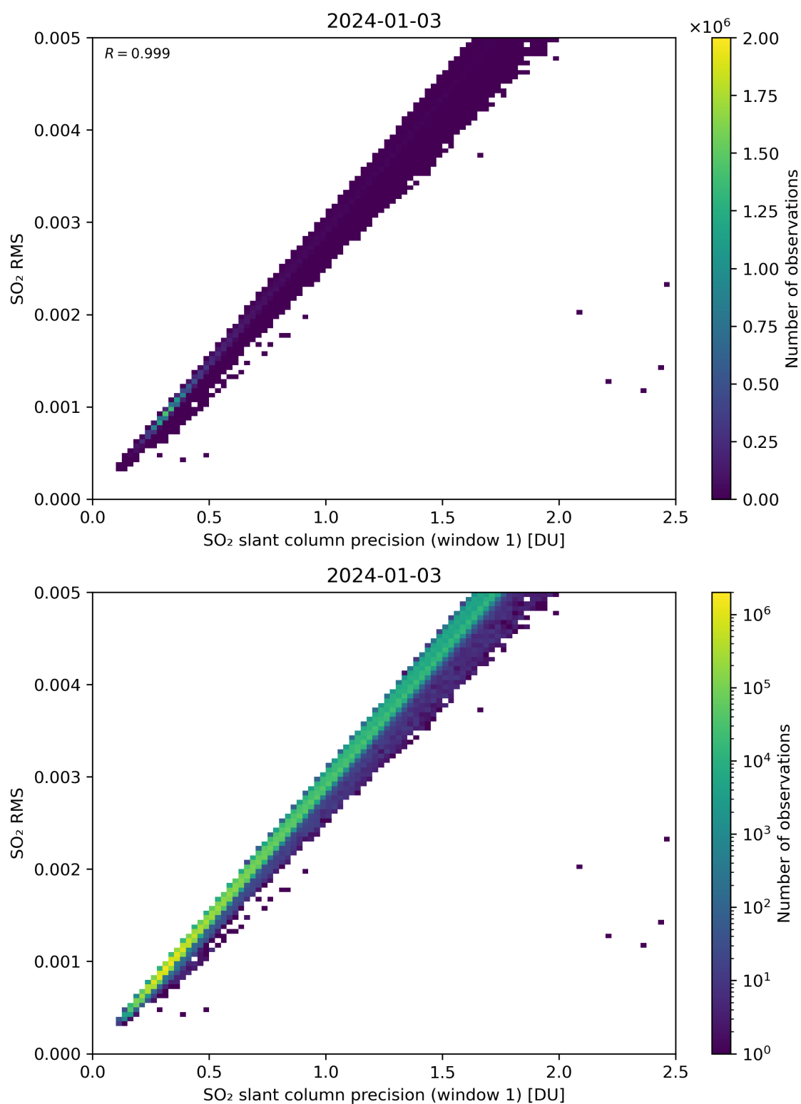
Figure 223: Scatter density plot of “SO 2 slant column precision (window 1)” against “SO 2 RMS” for 2024-01-02 to 2024-01-04.
