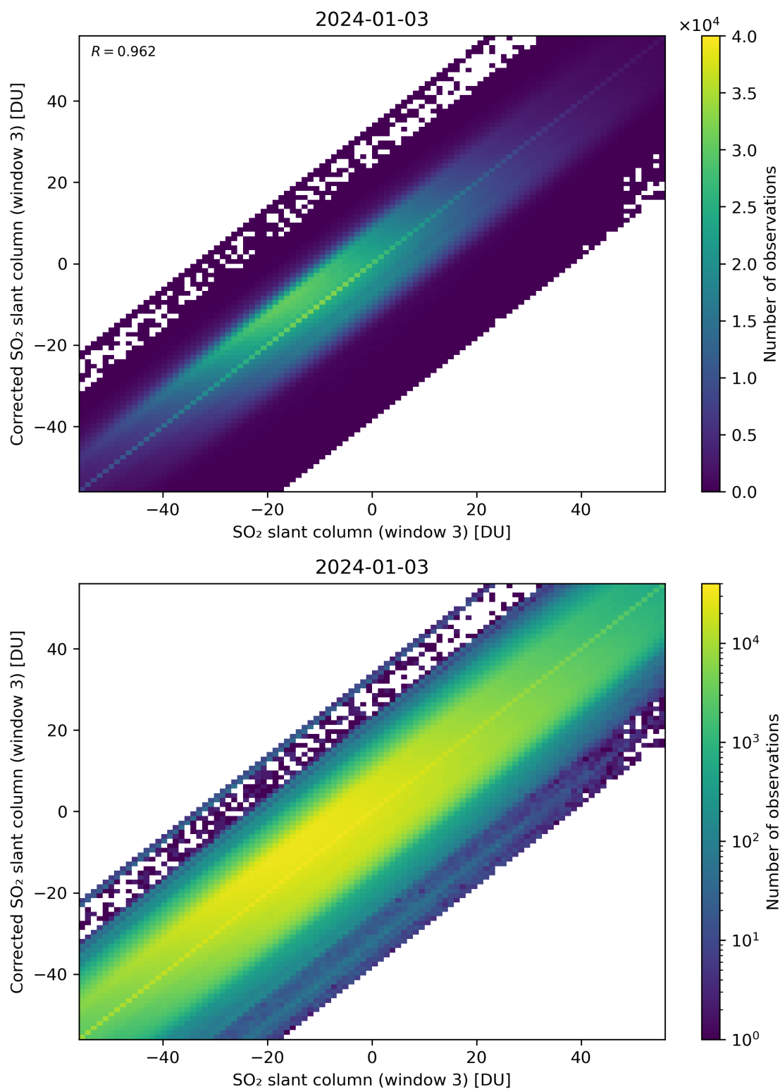
Figure 266: Scatter density plot of “SO 2 slant column (window 3)” against “Corrected SO 2 slant column (window 3)” for 2024-01-02 to 2024-01-04.
