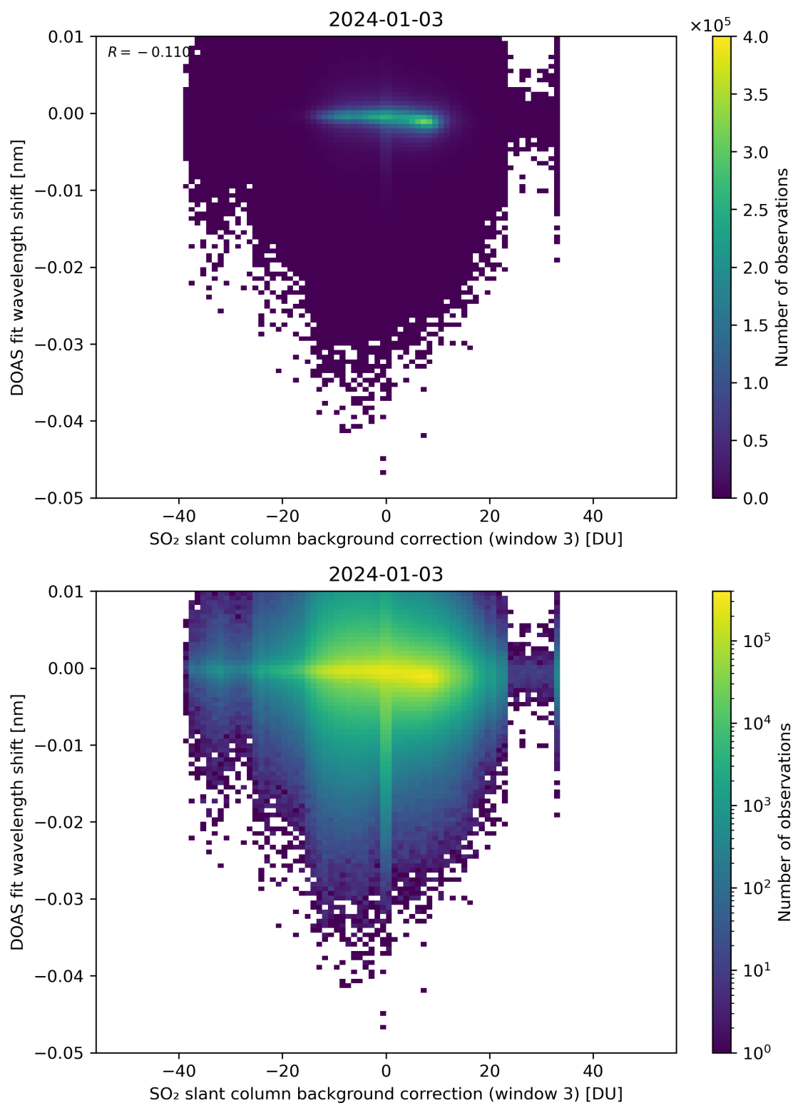
Figure 121: Scatter density plot of “SO 2 slant column background correction (window 3)” against “DOAS fit wavelength shift” for 2024-01-02 to 2024-01-04.
