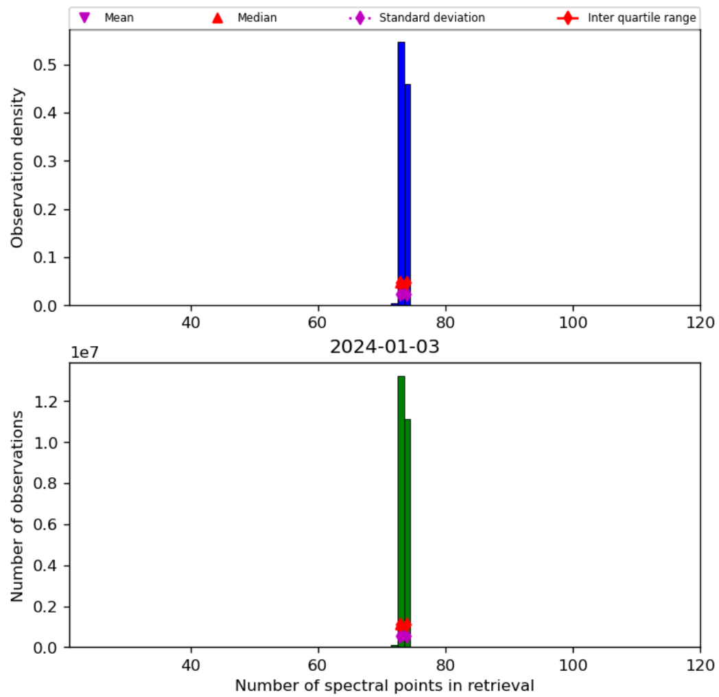
Figure 74: Histogram of “Number of spectral points in retrieval” for 2024-01-02 to 2024-01-04
