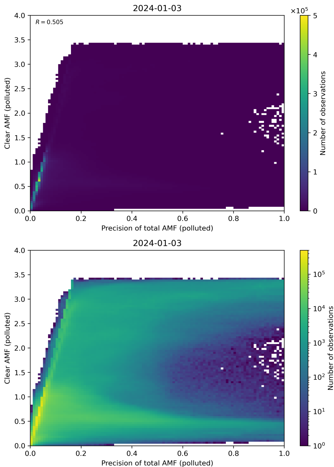
Figure 270: Scatter density plot of “Precision of total AMF (polluted)” against “Clear AMF (polluted)” for 2024-01-02 to 2024-01-04.
