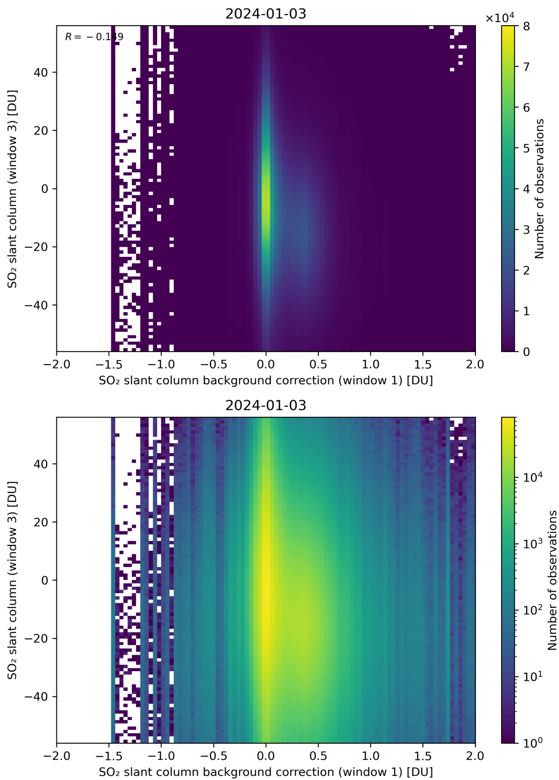
Figure 107: Scatter density plot of “SO 2 slant column background correction (window 1)” against “SO 2 slant column (window 3)” for 2024-01-02 to 2024-01-04.
