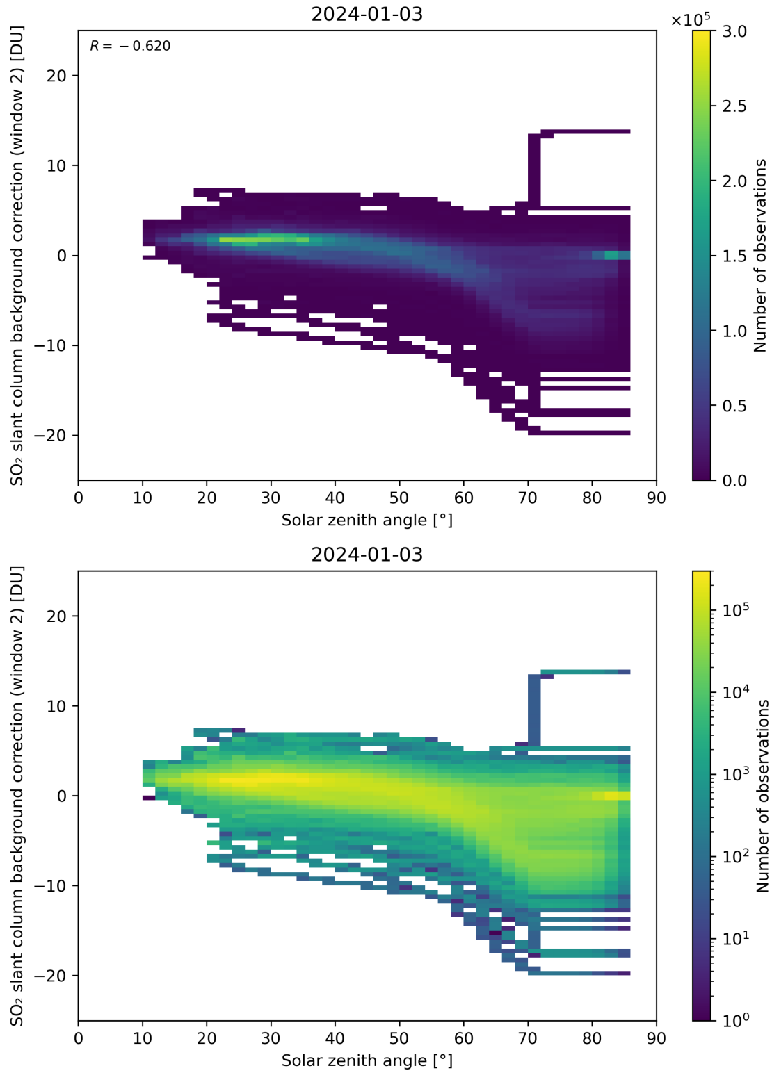
Figure 159: Scatter density plot of “Solar zenith angle” against “SO 2 slant column background correction (window 2)” for 2024-01-02 to 2024-01-04.
