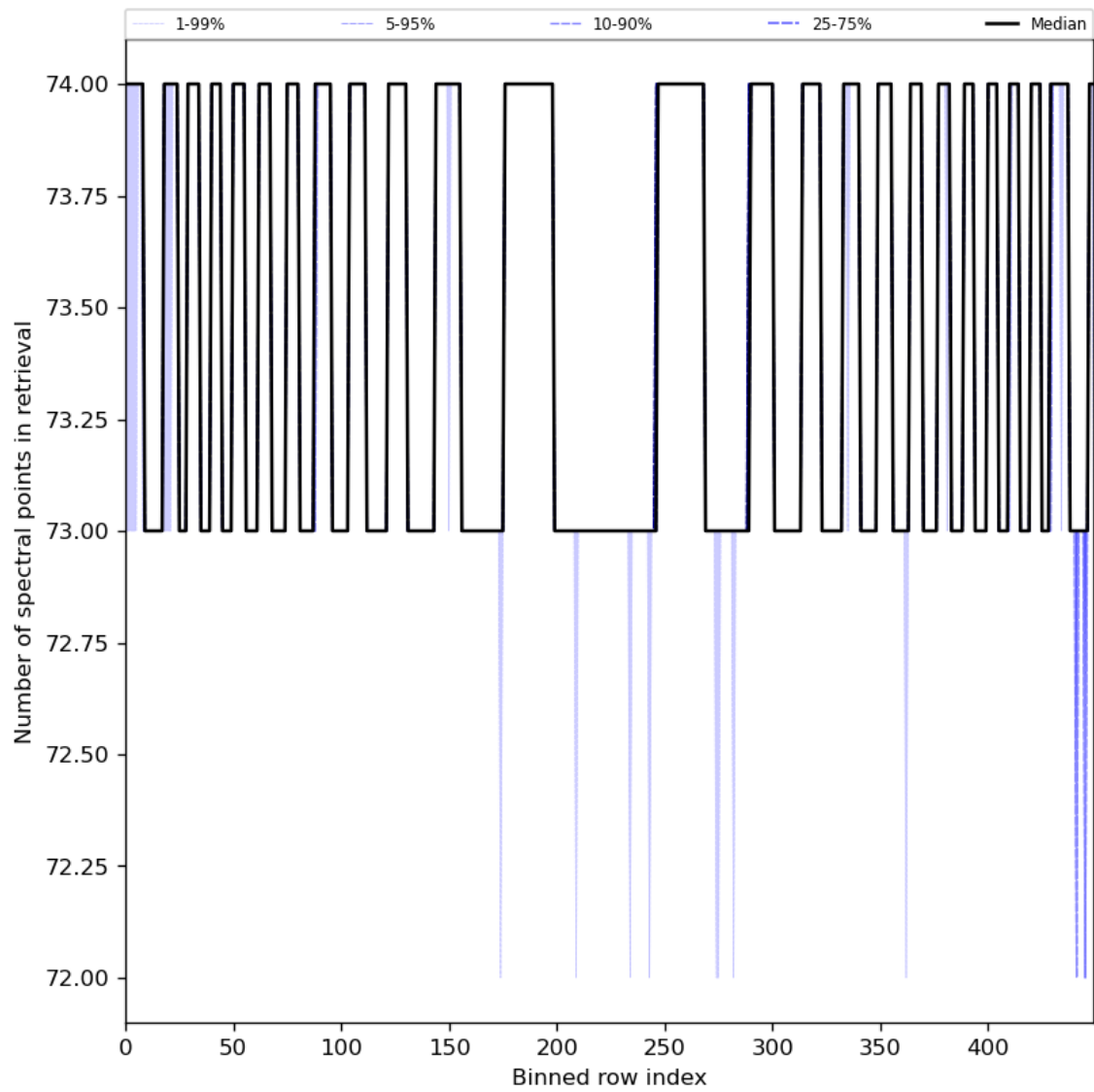
Figure 97: Along track statistics of “Number of spectral points in retrieval” for 2024-01-02 to 2024-01-04
