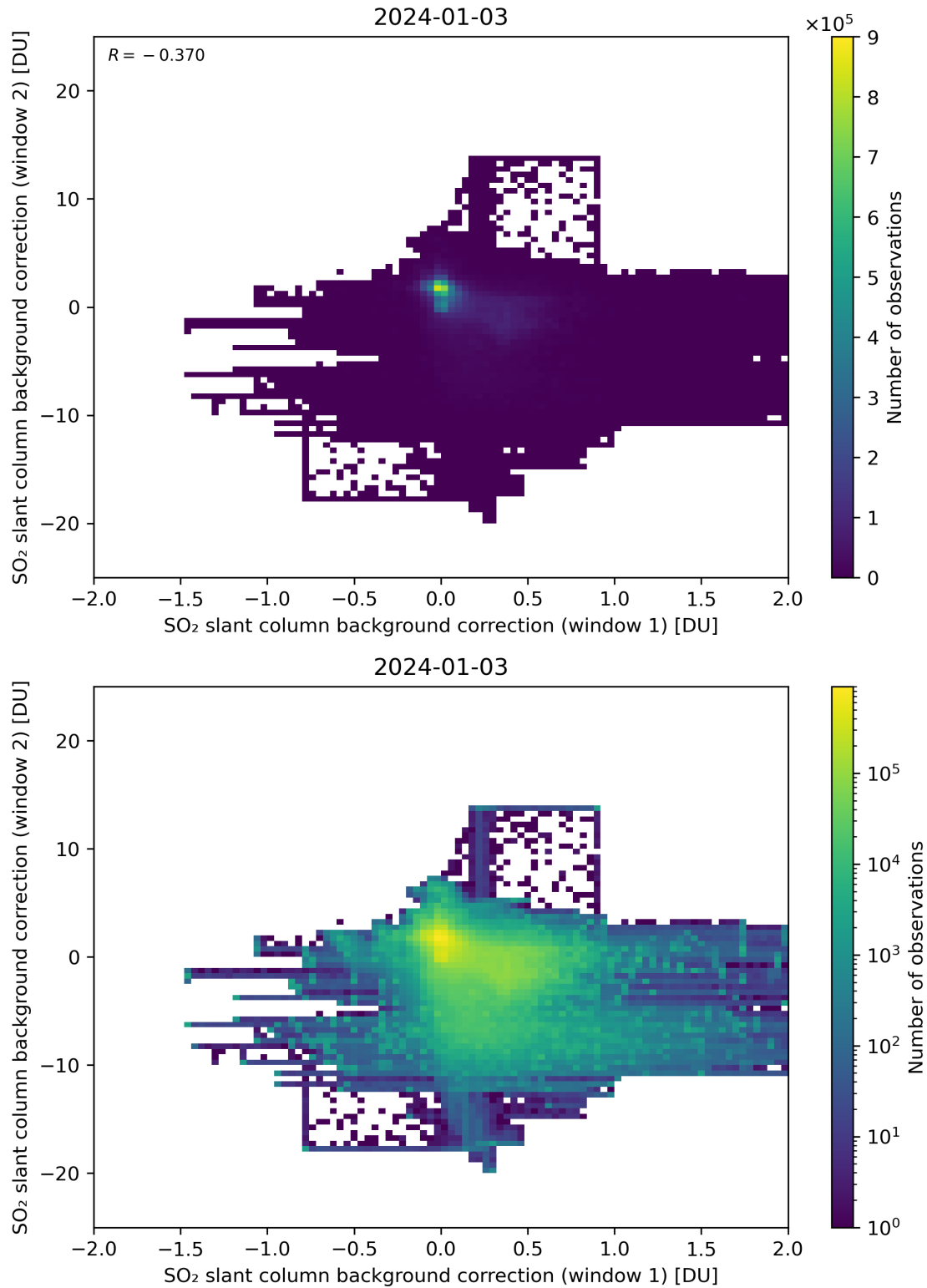
Figure 98: Scatter density plot of “SO 2 slant column background correction (window 1)” against “SO 2 slant column background correction (window 2)” for 2024-01-02 to 2024-01-04.
