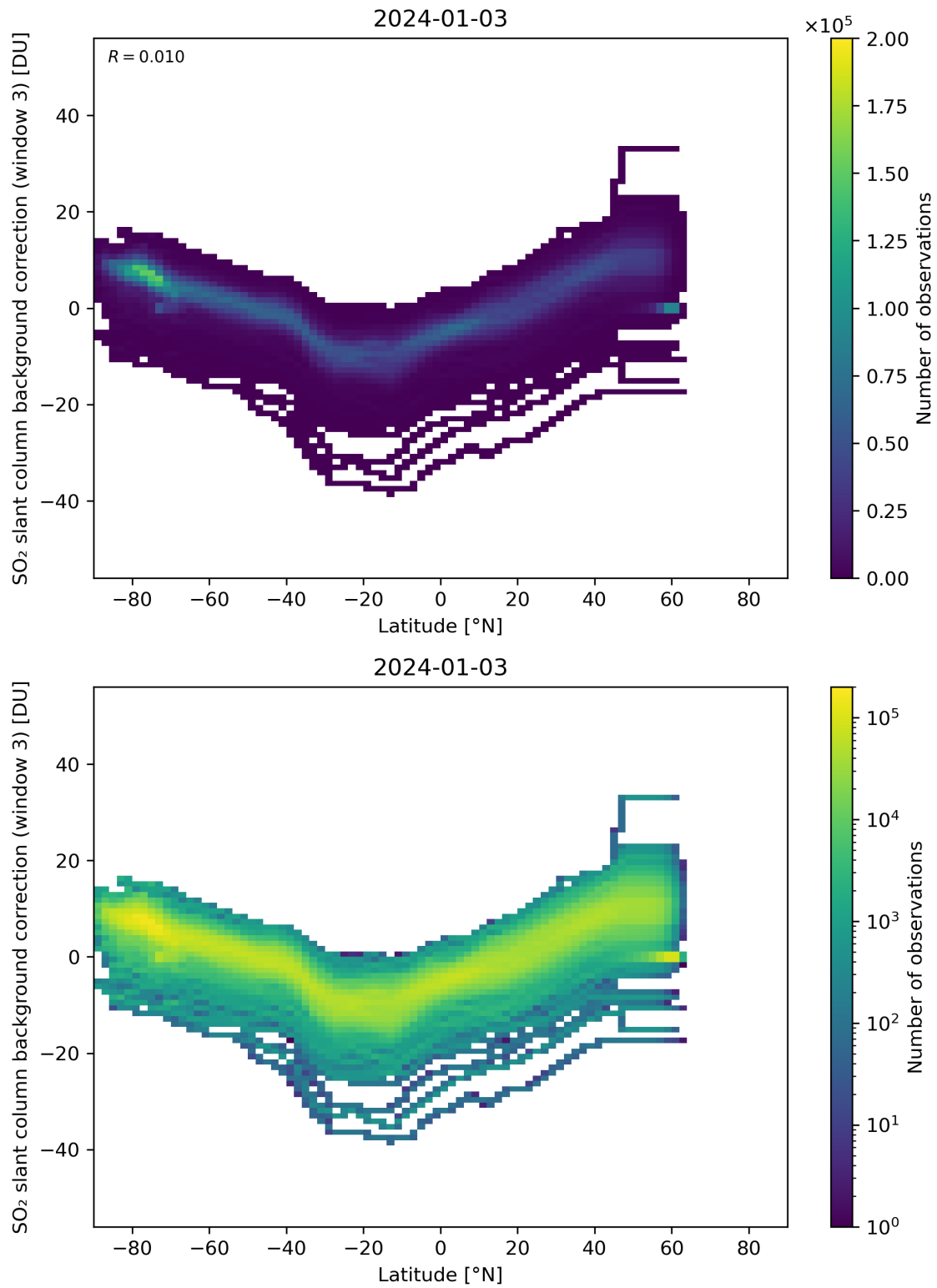
Figure 141: Scatter density plot of “Latitude” against “SO 2 slant column background correction (window 3)” for 2024-01-02 to 2024-01-04.
