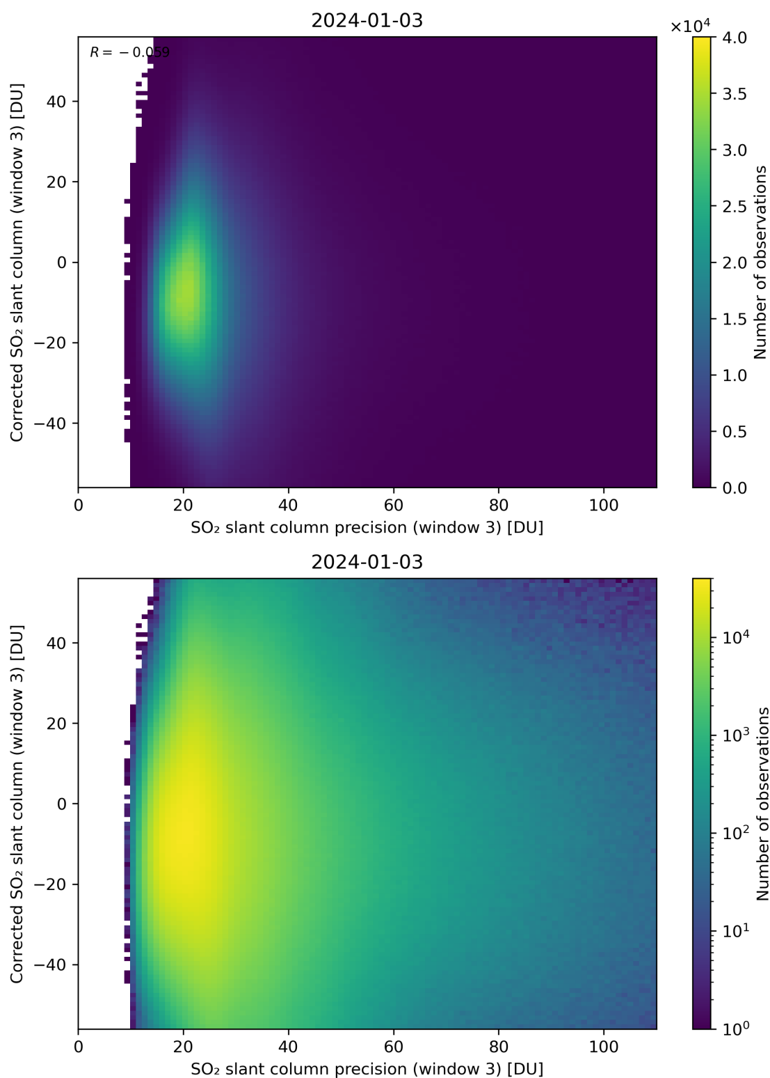
Figure 262: Scatter density plot of “SO 2 slant column precision (window 3)” against “Corrected SO 2 slant column (window 3)” for 2024-01-02 to 2024-01-04.
