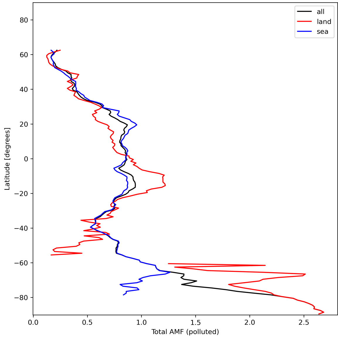
Figure 48: Zonal average of “Total AMF (polluted)” for 2024-01-02 to 2024-01-04.
