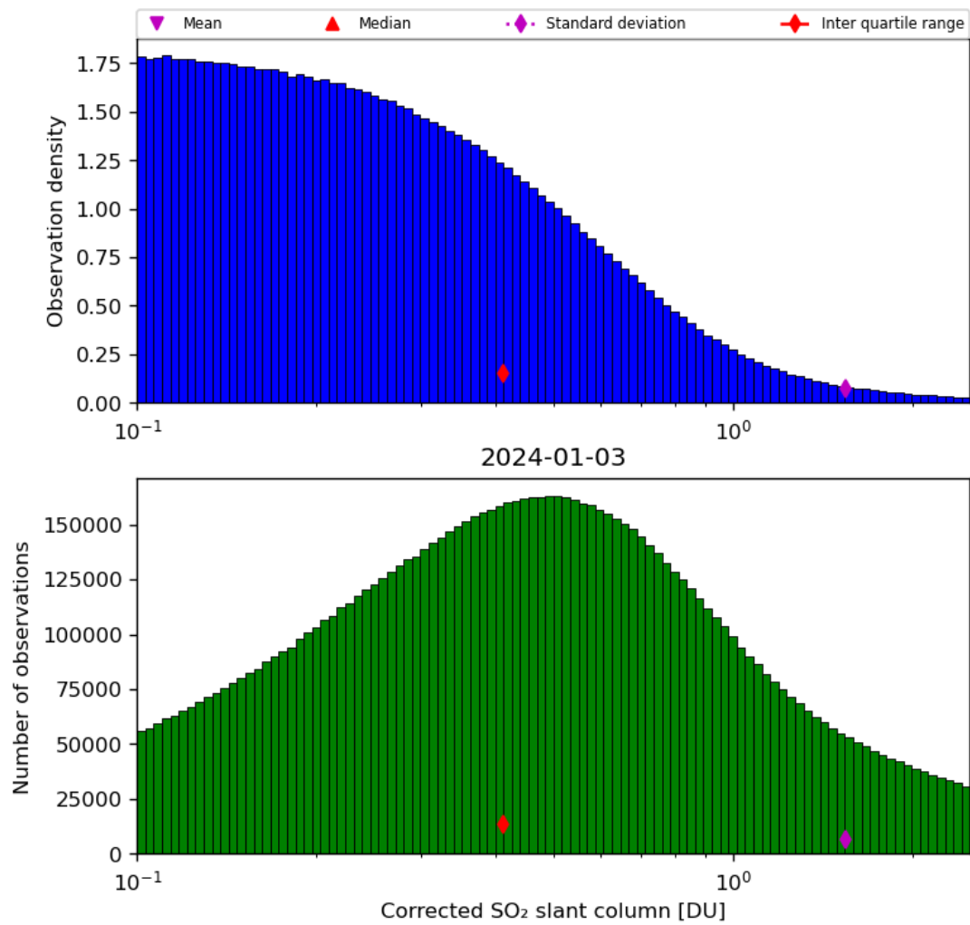
Figure 55: Histogram of “Corrected SO 2 slant column” for 2024-01-02 to 2024-01-04
