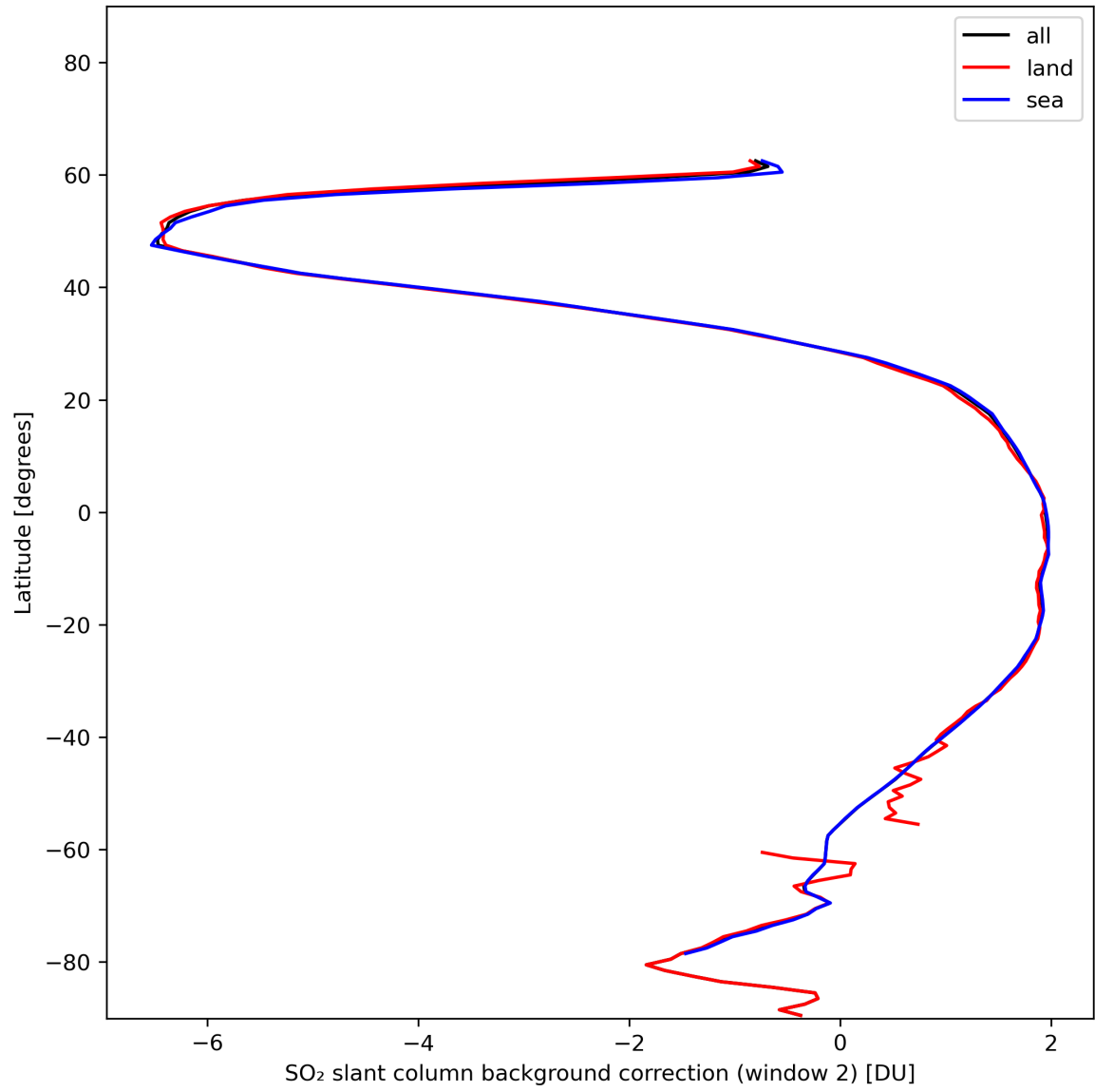
Figure 40: Zonal average of “SO 2 slant column background correction (window 2)” for 2024-01-02 to 2024-01-04.
