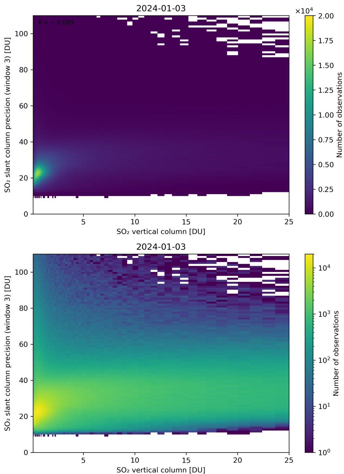
Figure 304: Scatter density plot of “SO 2 vertical column” against “SO 2 slant column precision (window 3)” for 2024-01-02 to 2024-01-04.
