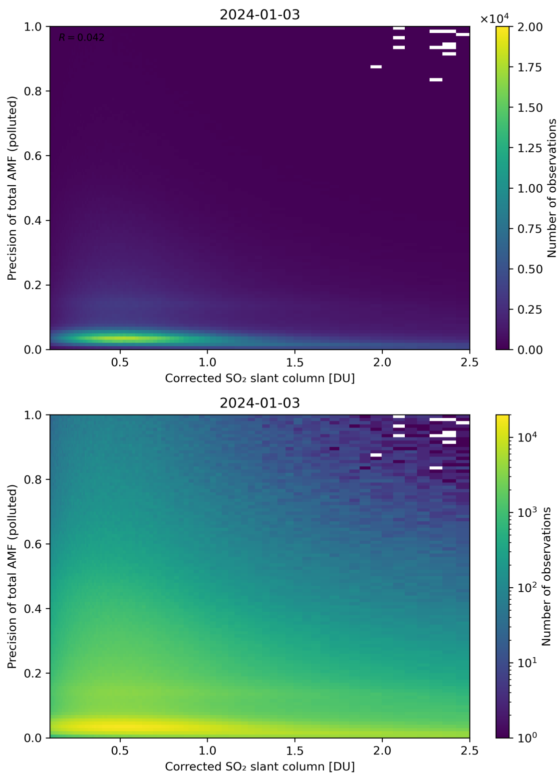
Figure 193: Scatter density plot of “Corrected SO 2 slant column” against “Precision of total AMF (polluted)” for 2024-01-02 to 2024-01-04.
