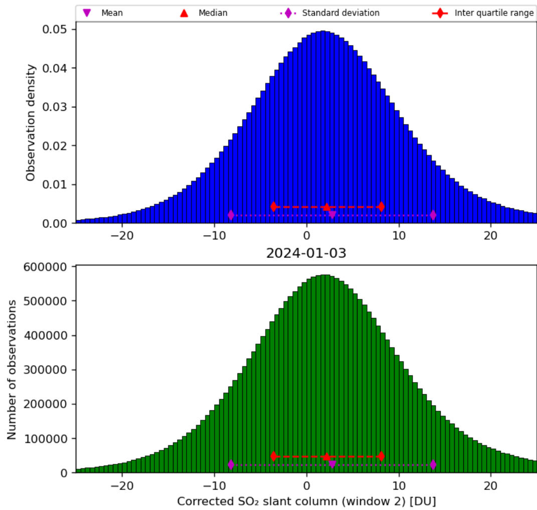
Figure 62: Histogram of “Corrected SO 2 slant column (window 2)” for 2024-01-02 to 2024-01-04
