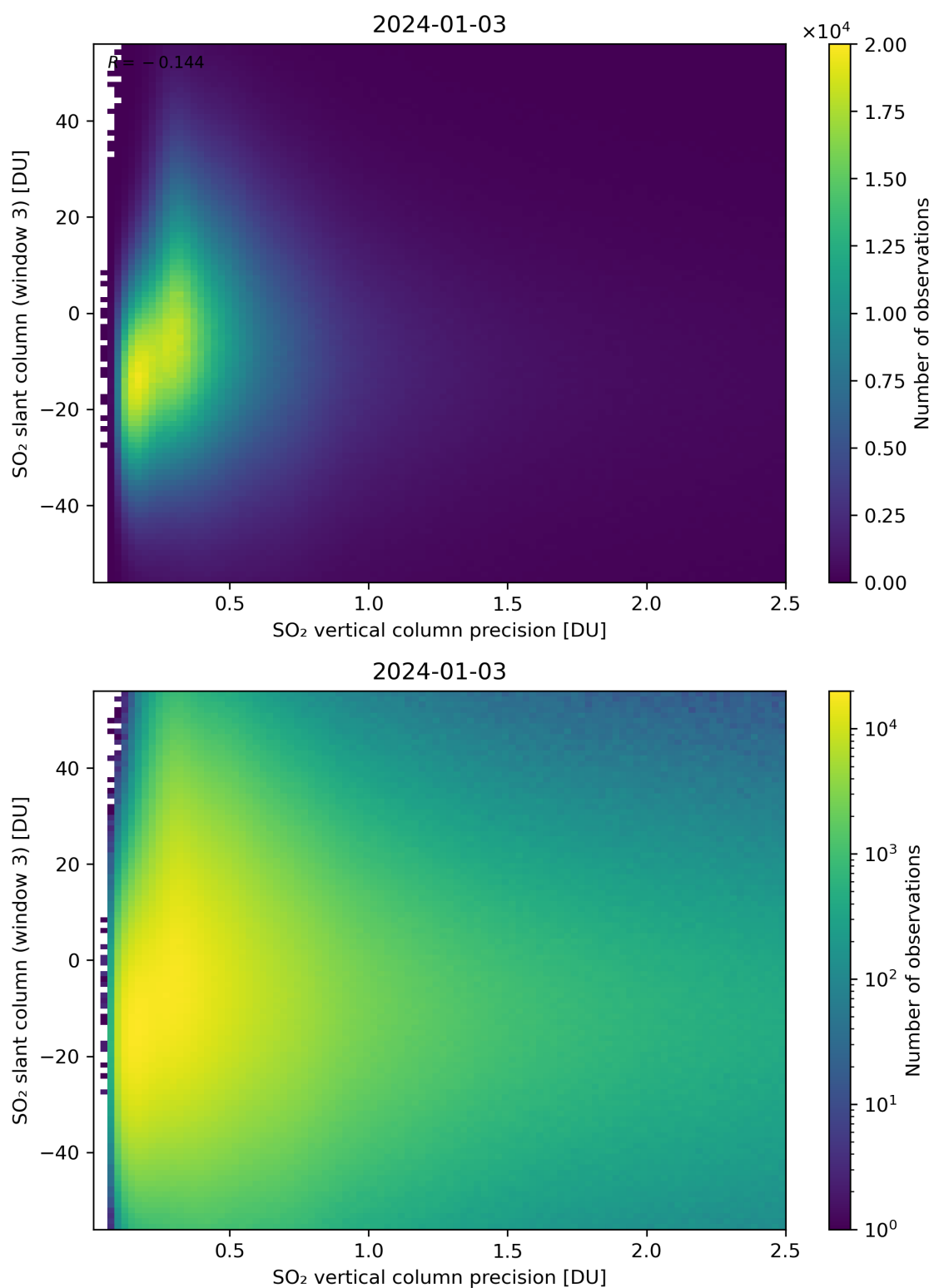
Figure 292: Scatter density plot of “SO 2 vertical column precision” against “SO 2 slant column (window 3)” for 2024-01-02 to 2024-01-04.
