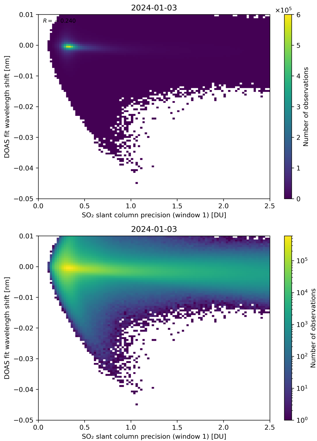
Figure 221: Scatter density plot of “SO 2 slant column precision (window 1)” against “DOAS fit wavelength shift” for 2024-01-02 to 2024-01-04.
