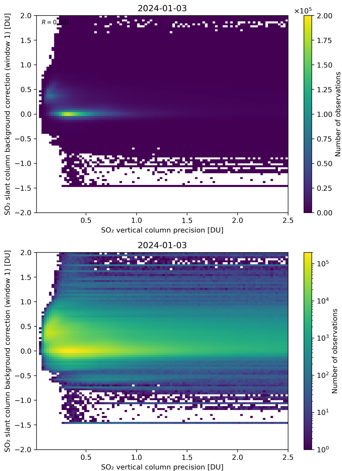
Figure 279: Scatter density plot of “SO 2 vertical column precision” against “SO 2 slant column background correction (window 1)” for 2024-01-02 to 2024-01-04.
