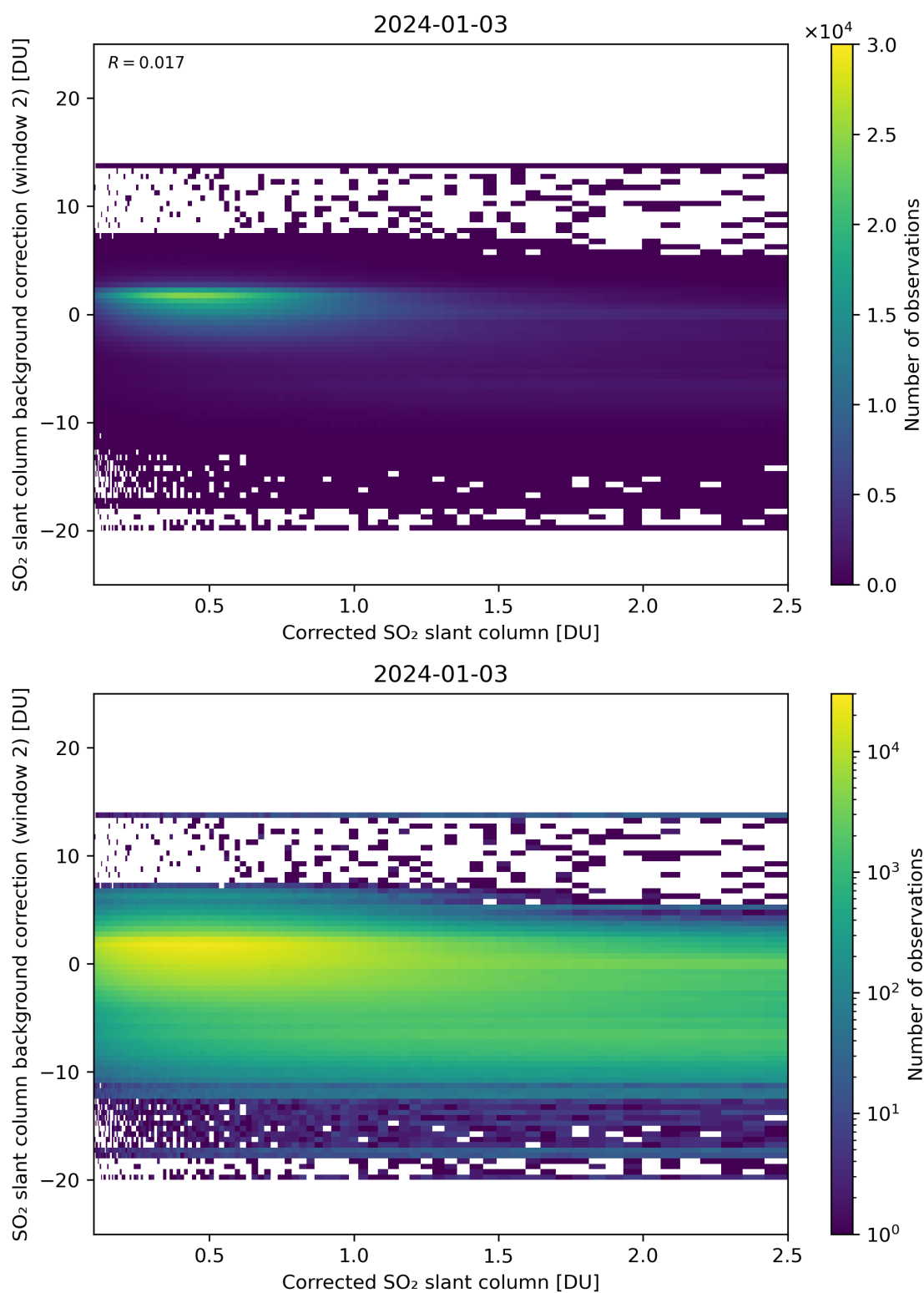
Figure 179: Scatter density plot of “Corrected SO 2 slant column” against “SO 2 slant column background correction (window 2)” for 2024-01-02 to 2024-01-04.
