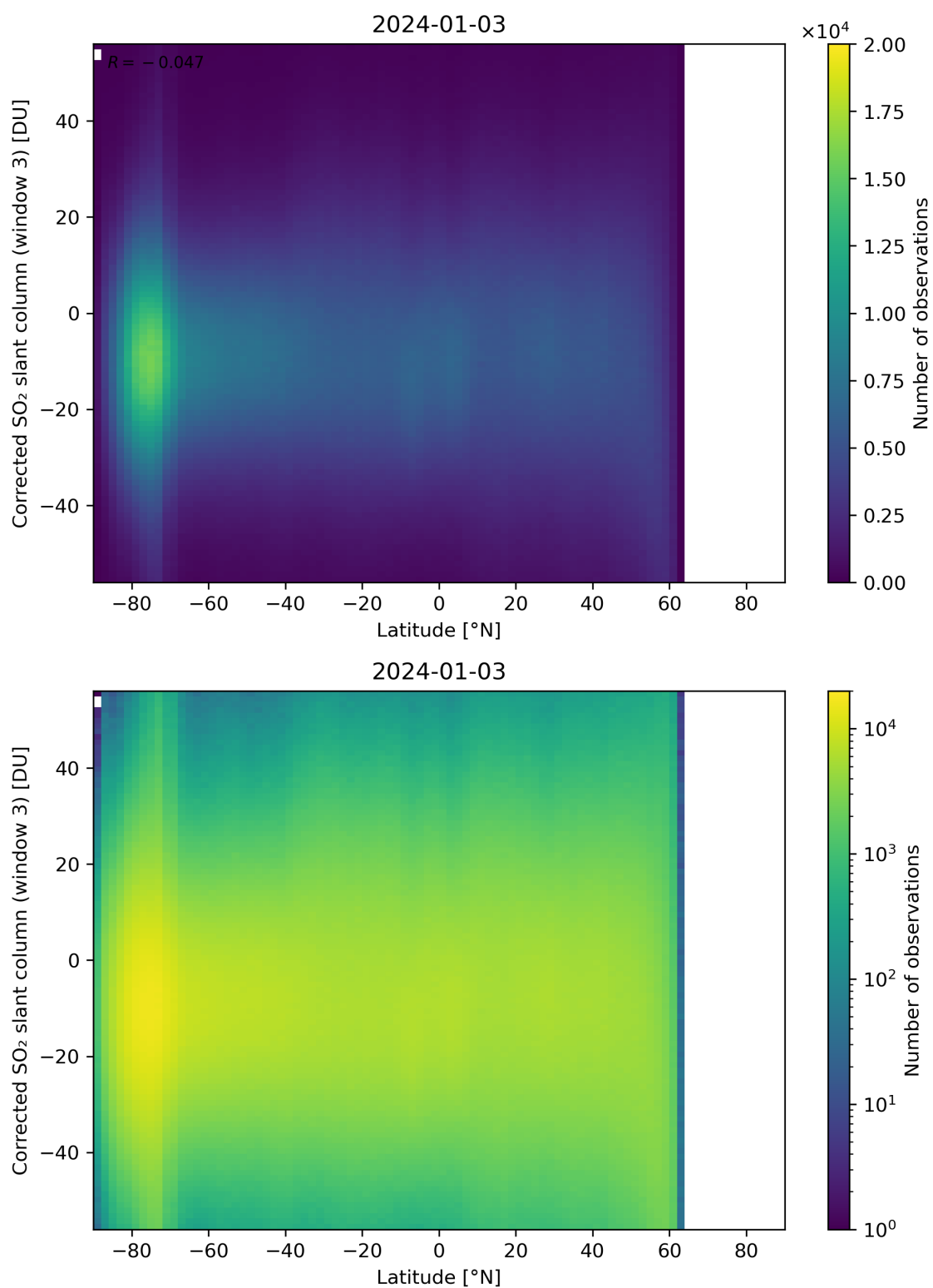
Figure 148: Scatter density plot of “Latitude” against “Corrected SO 2 slant column (window 3)” for 2024-01-02 to 2024-01-04.
