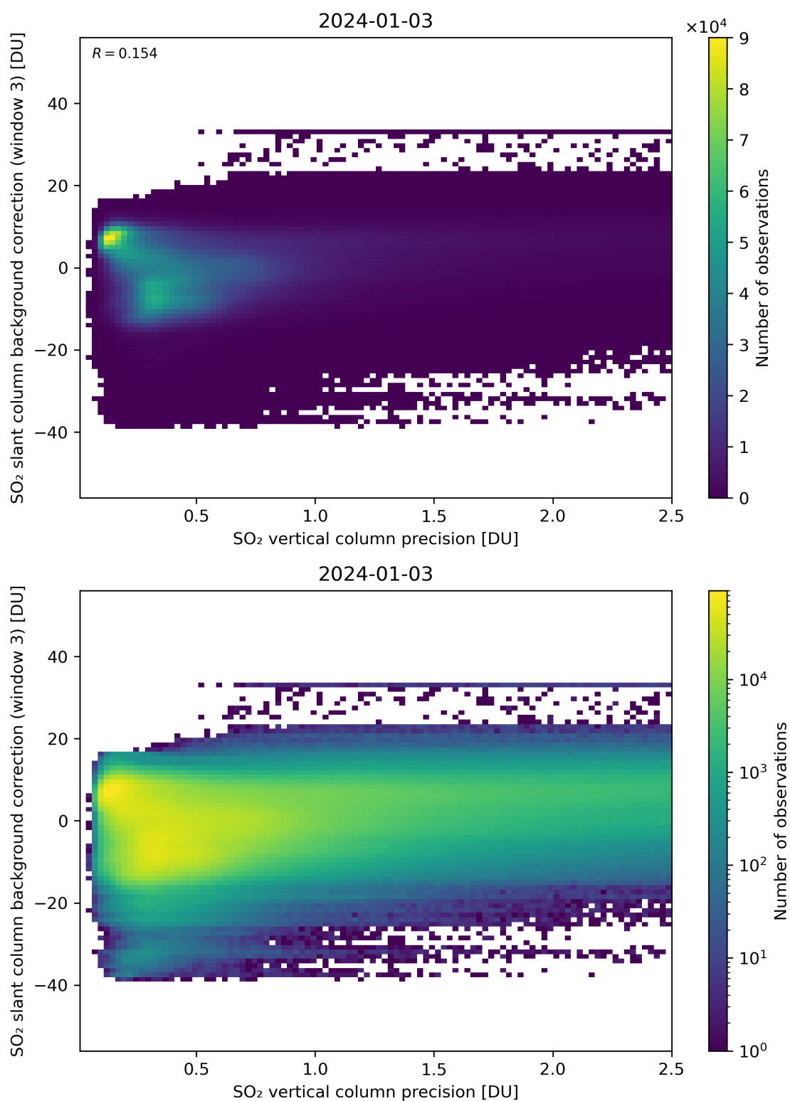
Figure 281: Scatter density plot of “SO 2 vertical column precision” against “SO 2 slant column background correction (window 3)” for 2024-01-02 to 2024-01-04.
