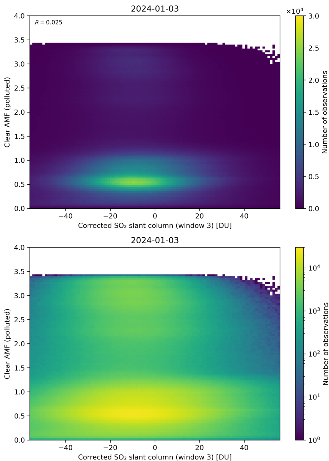
Figure 209: Scatter density plot of “Corrected SO 2 slant column (window 3)” against “Clear AMF (polluted)” for 2024-01-02 to 2024-01-04.
