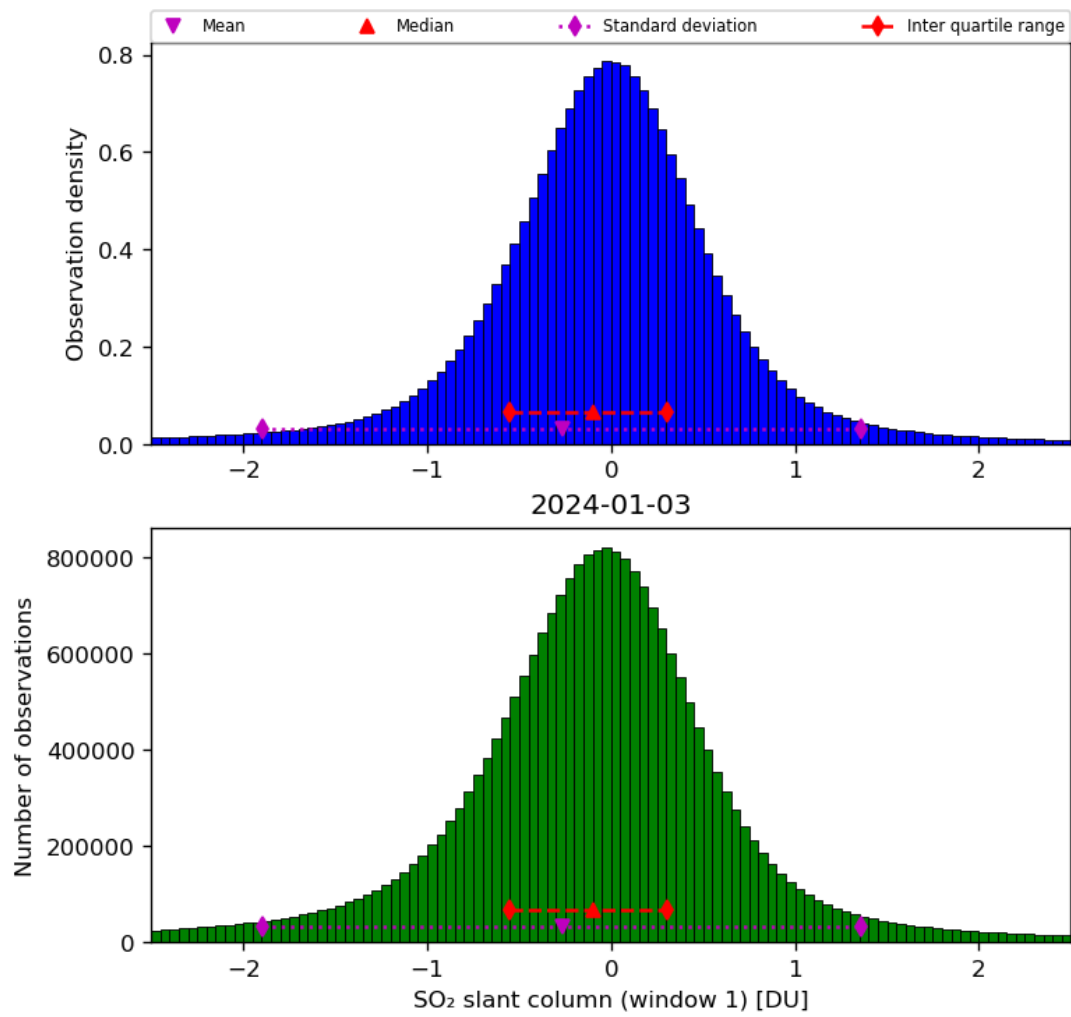
Figure 56: Histogram of “SO 2 slant column (window 1)” for 2024-01-02 to 2024-01-04
