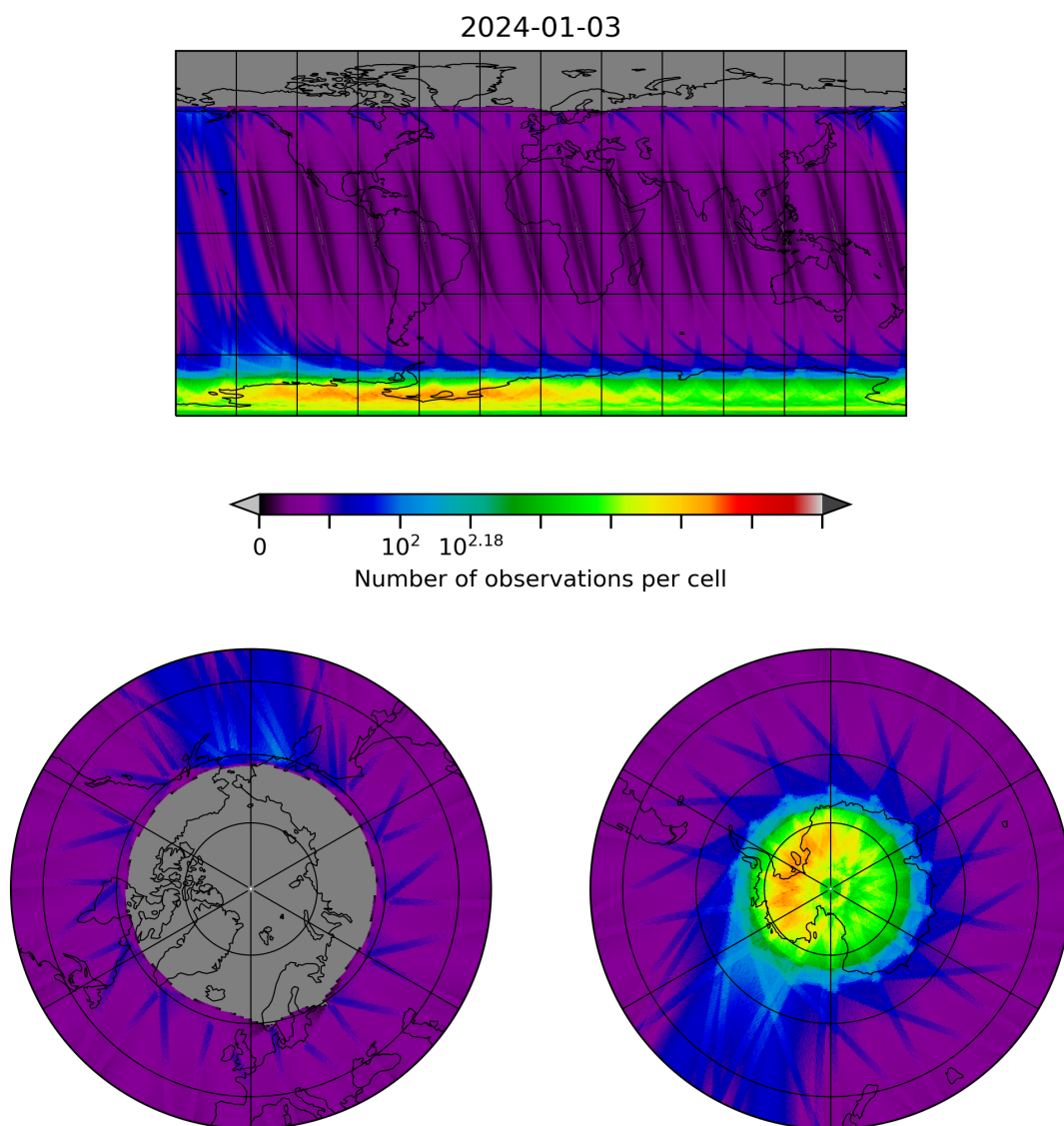
Figure 28: Map of the number of observations for 2024-01-02 to 2024-01-04
