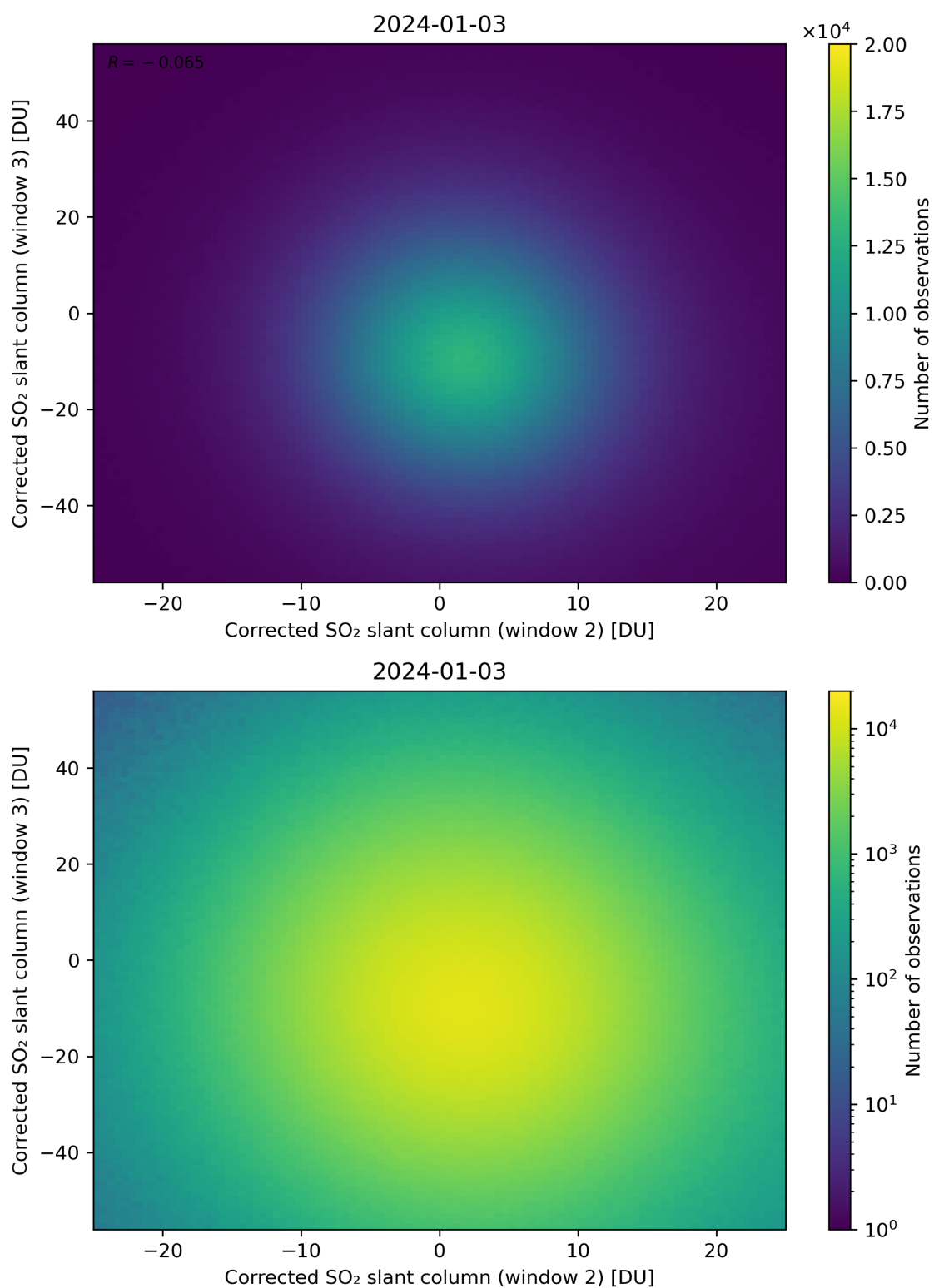
Figure 200: Scatter density plot of “Corrected SO 2 slant column (window 2)” against “Corrected SO 2 slant column (window 3)” for 2024-01-02 to 2024-01-04.
