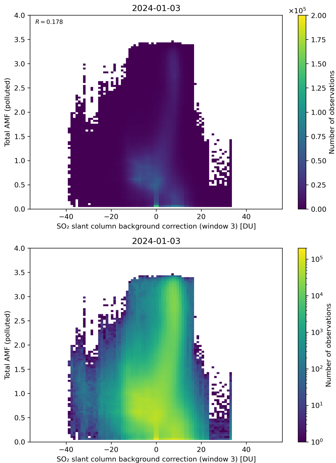
Figure 125: Scatter density plot of “SO 2 slant column background correction (window 3)” against “Total AMF (polluted)” for 2024-01-02 to 2024-01-04.
