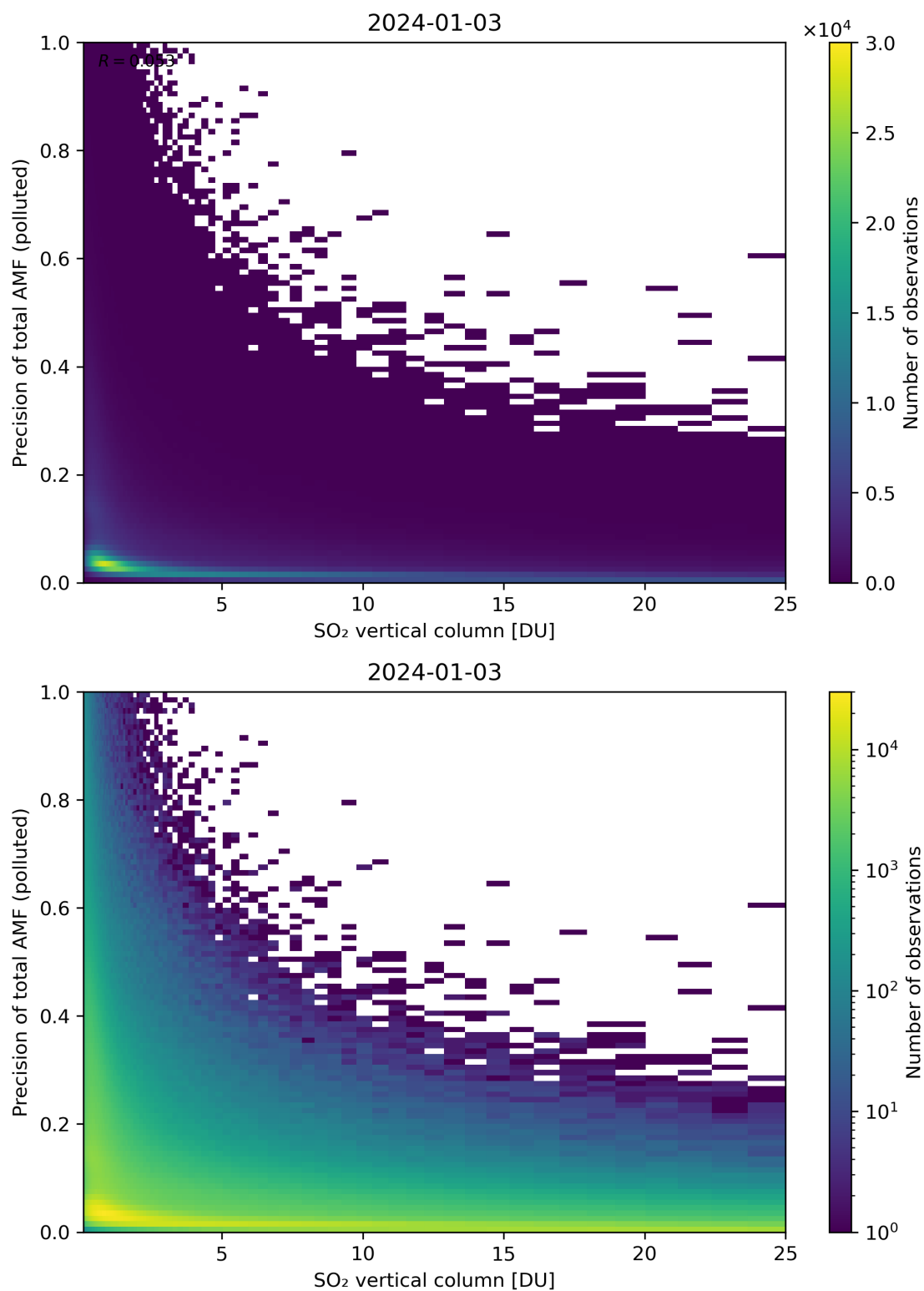
Figure 306: Scatter density plot of “SO 2 vertical column” against “Precision of total AMF (polluted)” for 2024-01-02 to 2024-01-04.
