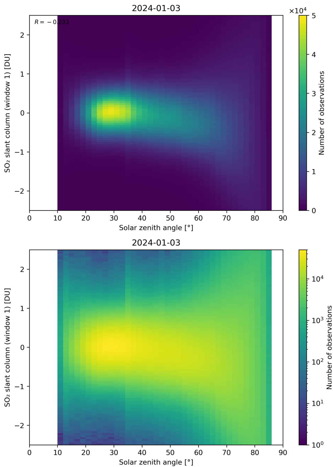
Figure 169: Scatter density plot of “Solar zenith angle” against “SO 2 slant column (window 1)” for 2024-01-02 to 2024-01-04.
