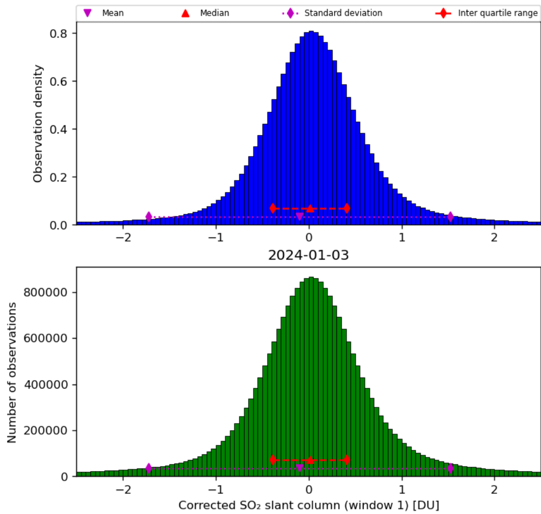
Figure 58: Histogram of “Corrected SO 2 slant column (window 1)” for 2024-01-02 to 2024-01-04
