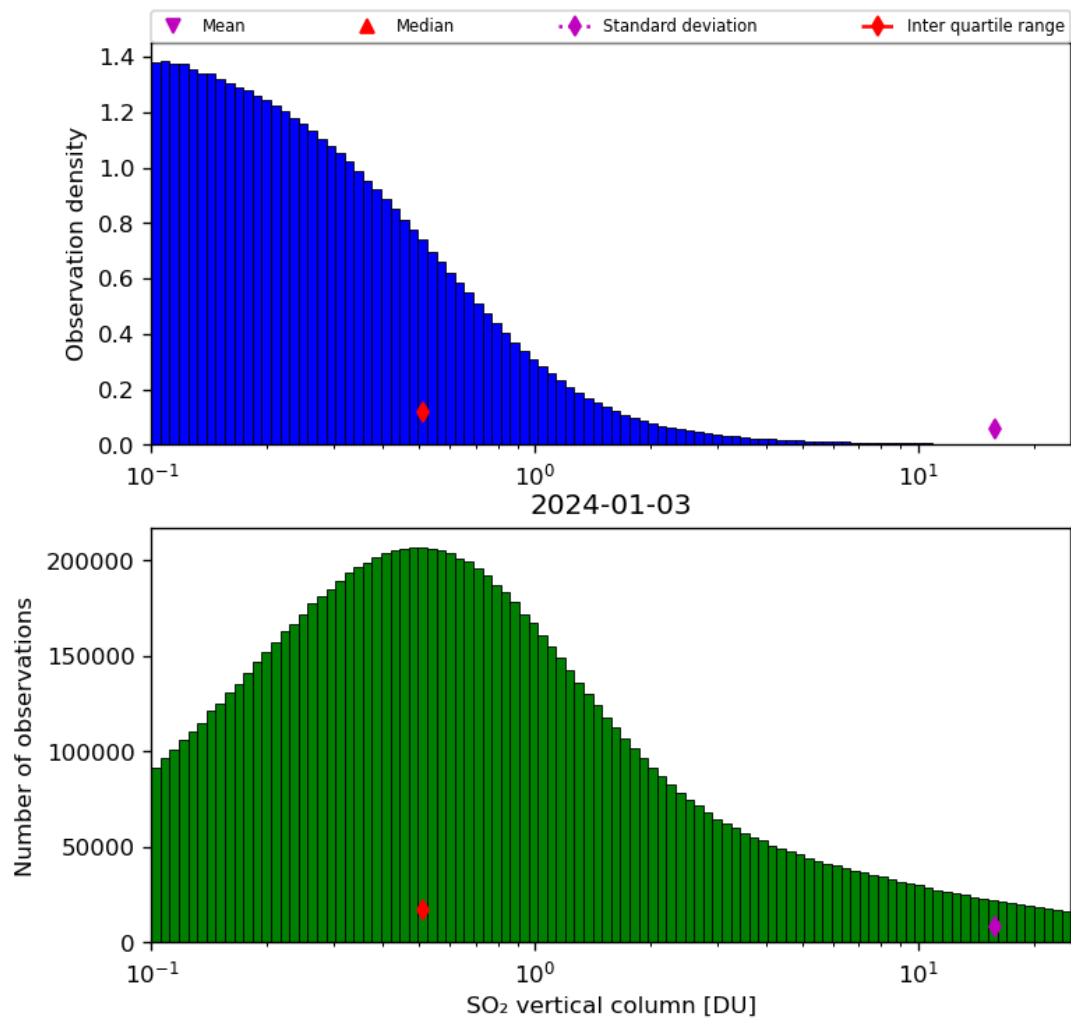
Figure 53: Histogram of “SO 2 vertical column” for 2024-01-02 to 2024-01-04
