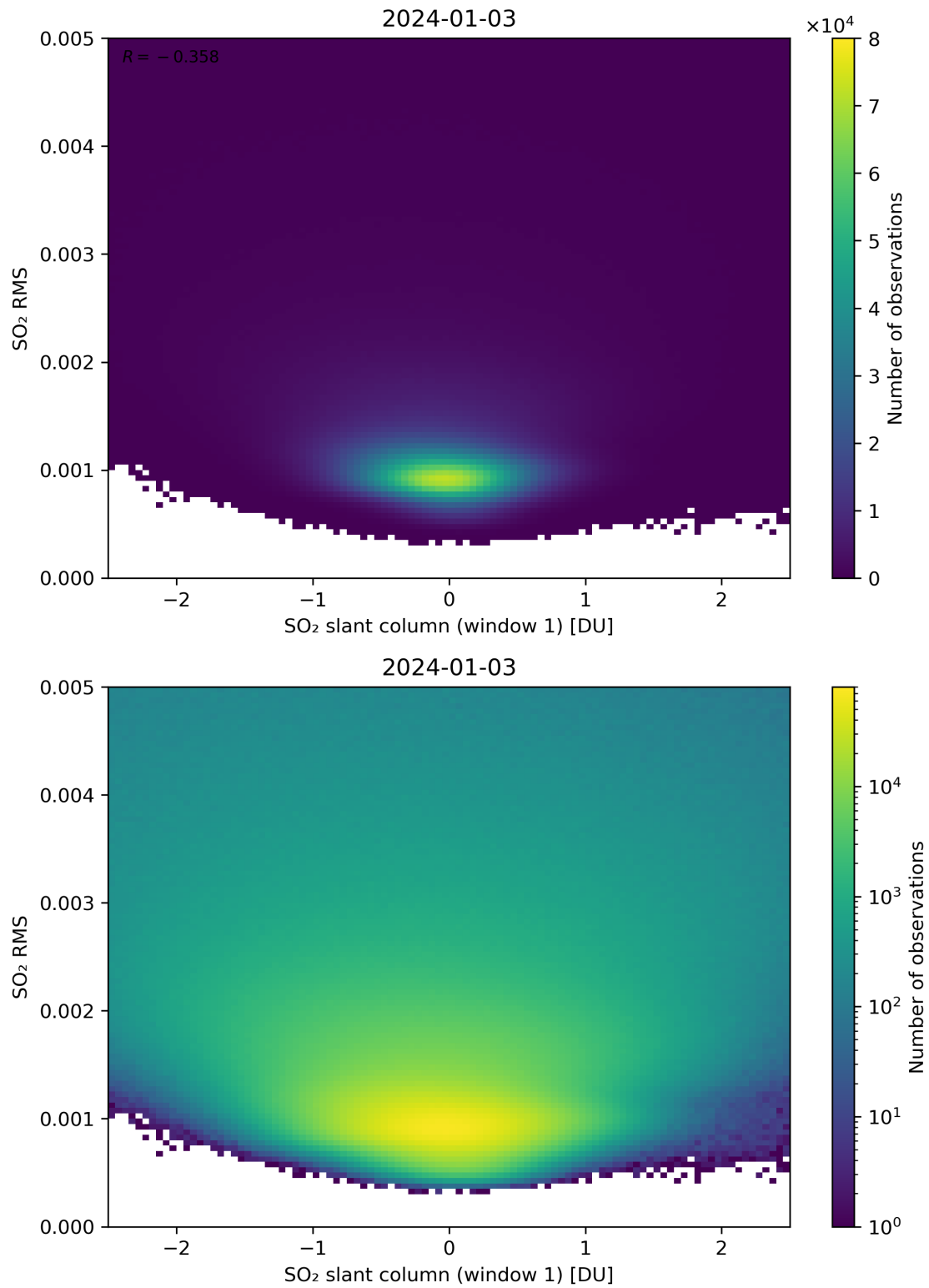
Figure 217: Scatter density plot of “SO 2 slant column (window 1)” against “SO 2 RMS” for 2024-01-02 to 2024-01-04.
