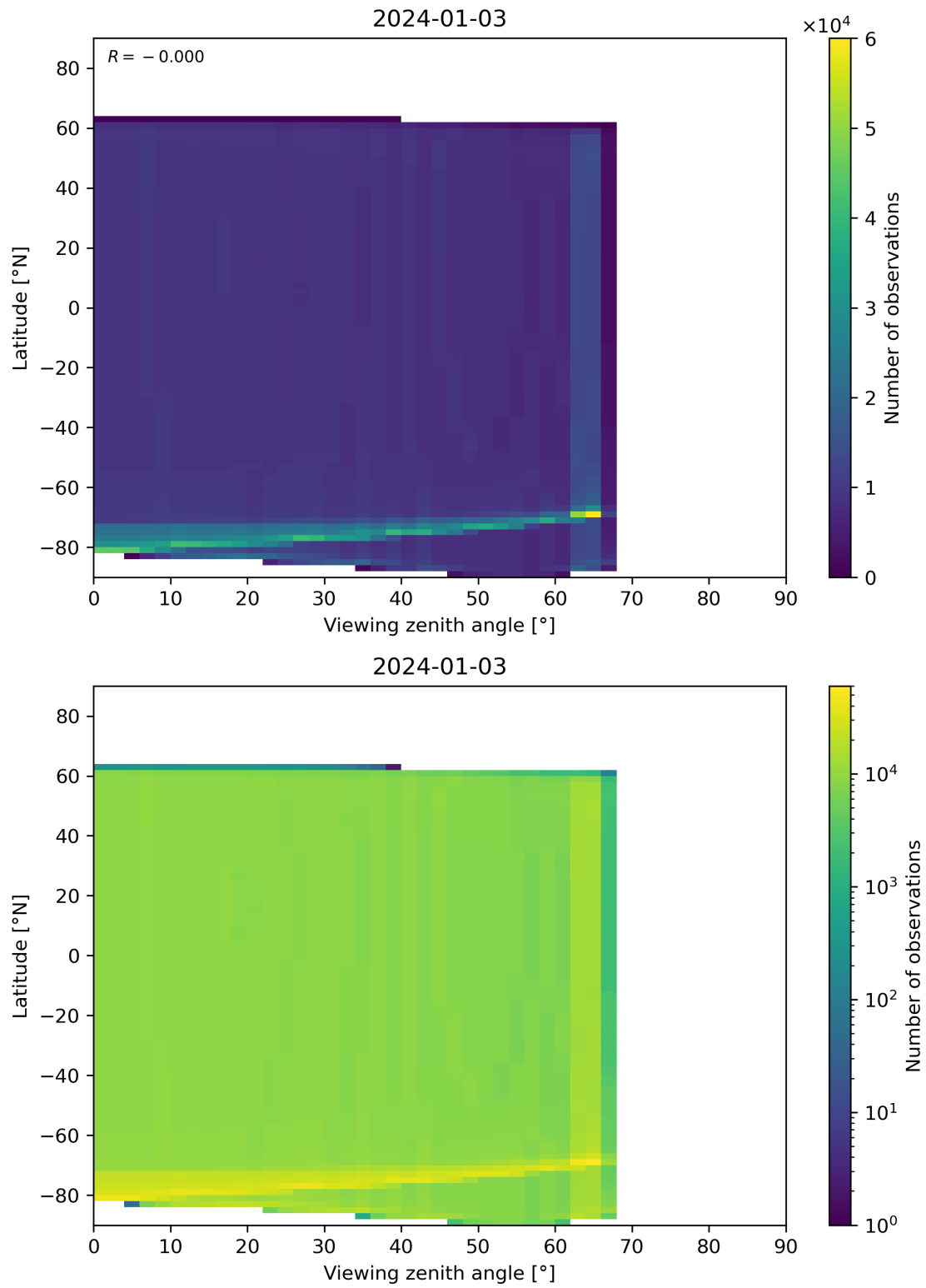
Figure 314: Scatter density plot of “Viewing zenith angle” against “Latitude” for 2024-01-02 to 2024-01-04.
