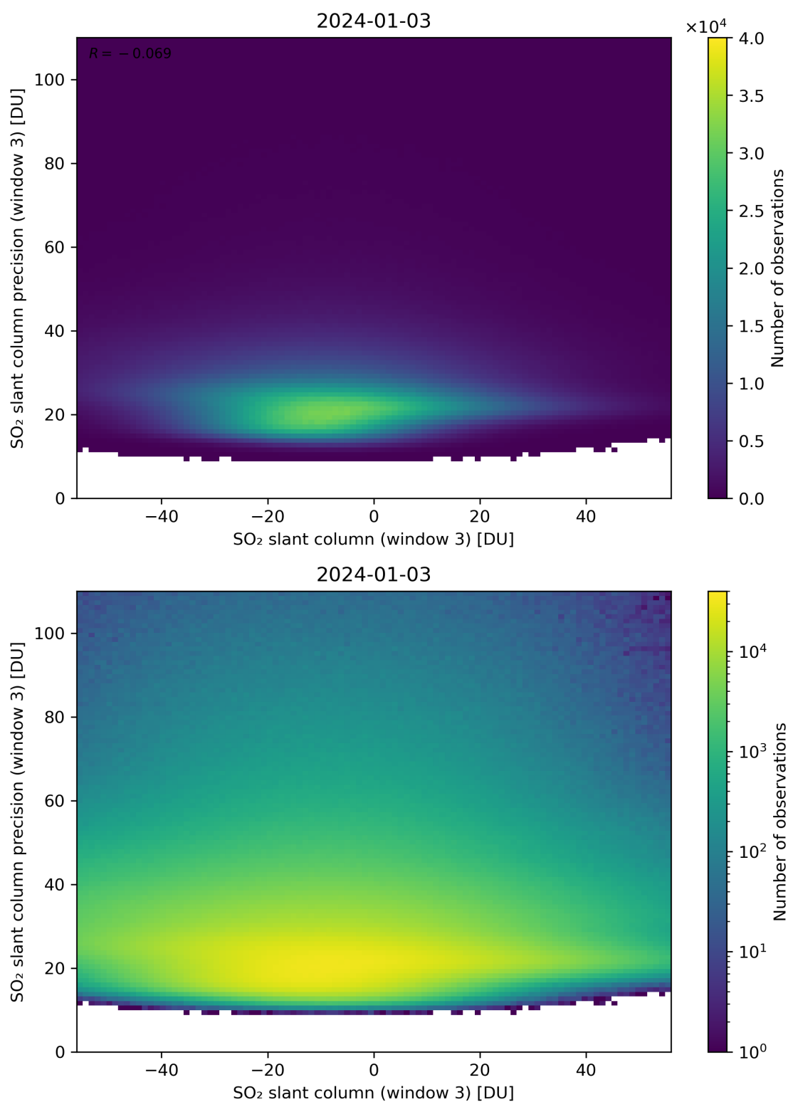
Figure 267: Scatter density plot of “SO 2 slant column (window 3)” against “SO 2 slant column precision (window 3)” for 2024-01-02 to 2024-01-04.
