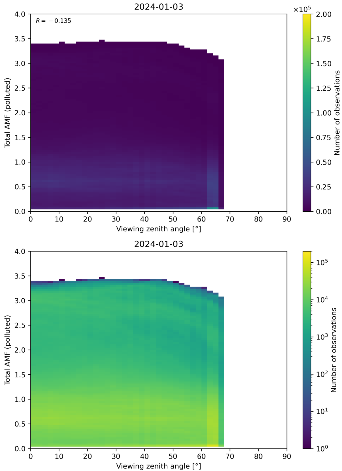
Figure 325: Scatter density plot of “Viewing zenith angle” against “Total AMF (polluted)” for 2024-01-02 to 2024-01-04.
