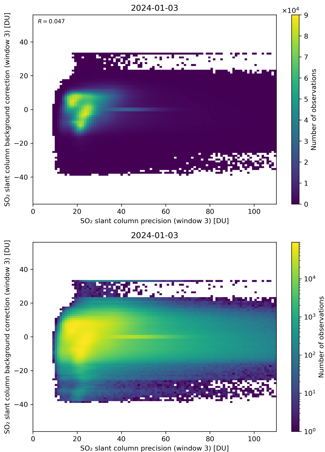
Figure 257: Scatter density plot of “SO 2 slant column precision (window 3)” against “SO 2 slant column background correction (window 3)” for 2024-01-02 to 2024-01-04.
