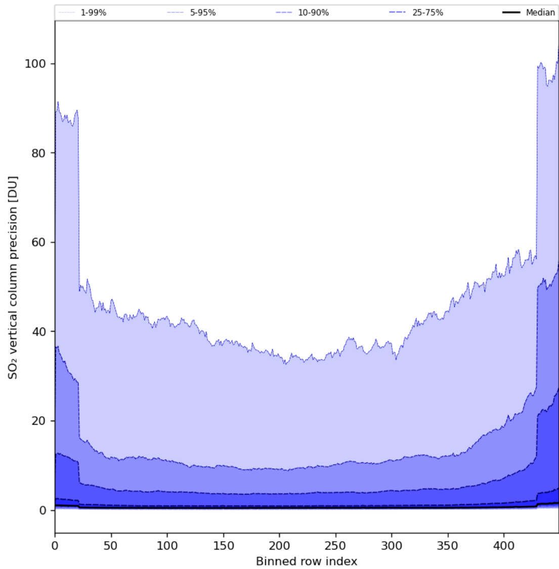
Figure 77: Along track statistics of “SO 2 vertical column precision” for 2024-01-02 to 2024-01-04
