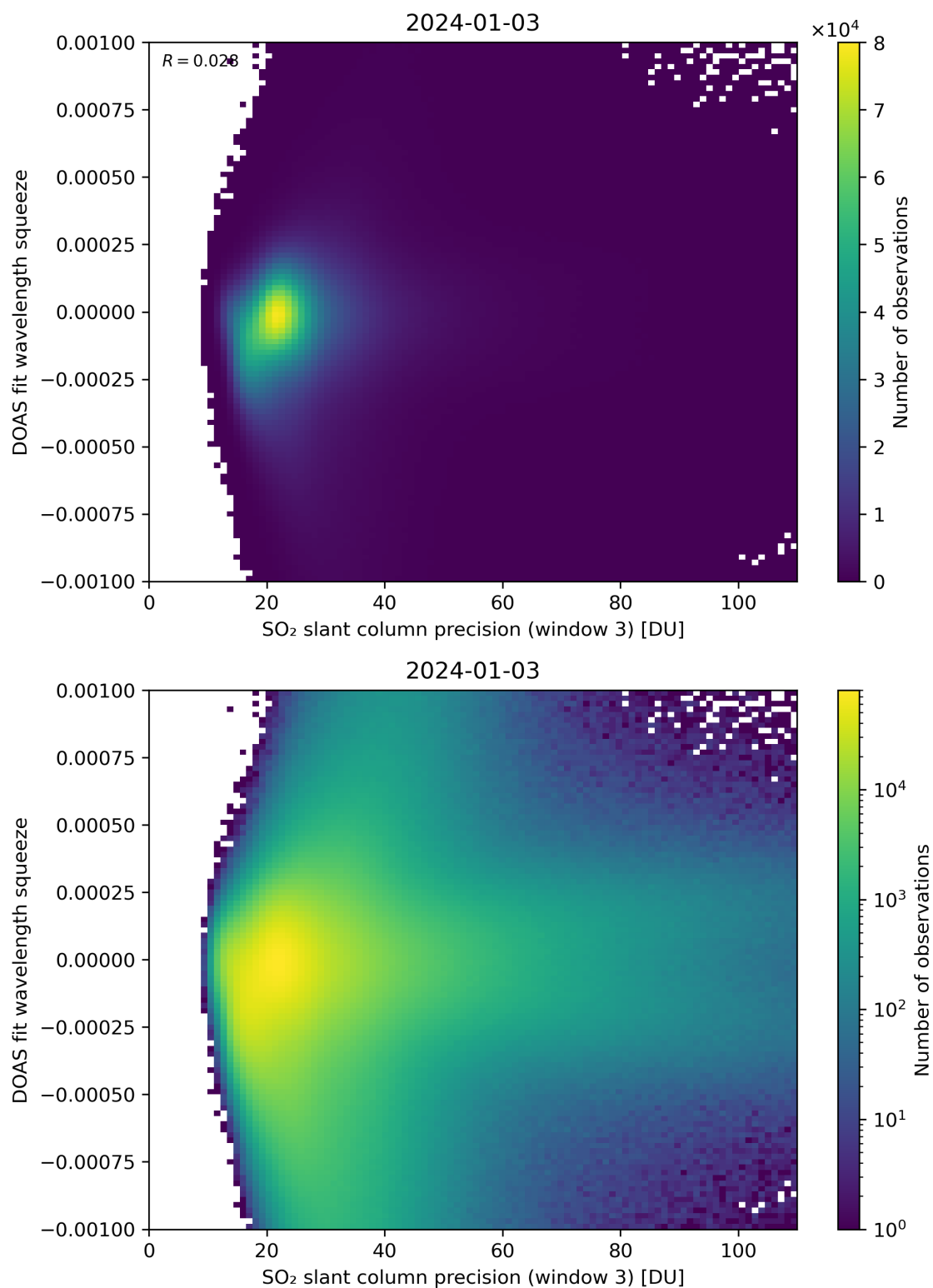
Figure 259: Scatter density plot of “SO 2 slant column precision (window 3)” against “DOAS fit wavelength squeeze” for 2024-01-02 to 2024-01-04.
