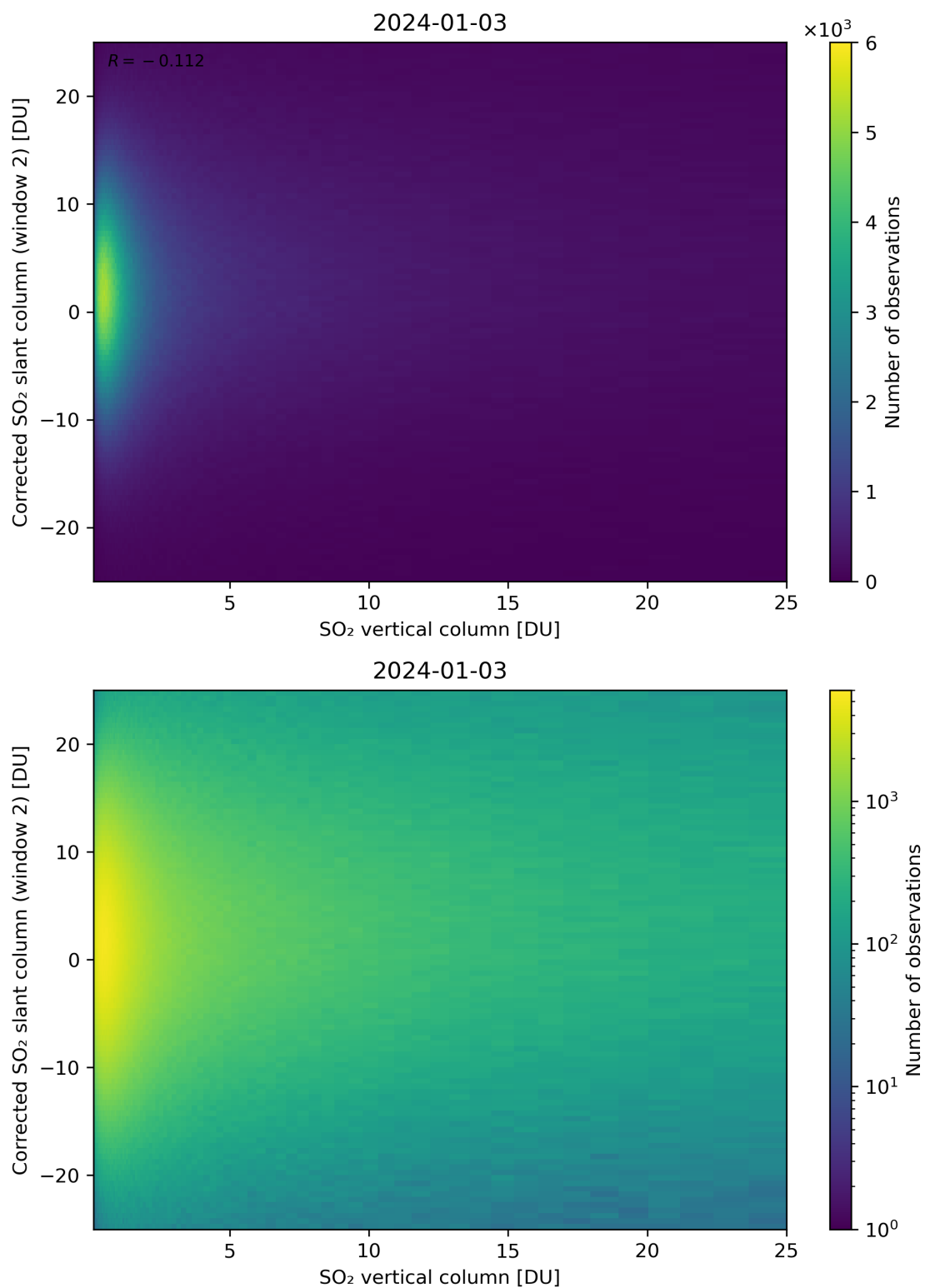
Figure 298: Scatter density plot of “SO 2 vertical column” against “Corrected SO 2 slant column (window 2)” for 2024-01-02 to 2024-01-04.
