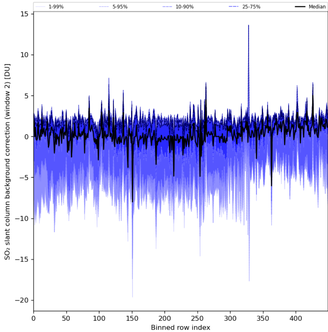
Figure 86: Along track statistics of “SO 2 slant column background correction (window 2)” for 2024-01-02 to 2024-01-04
