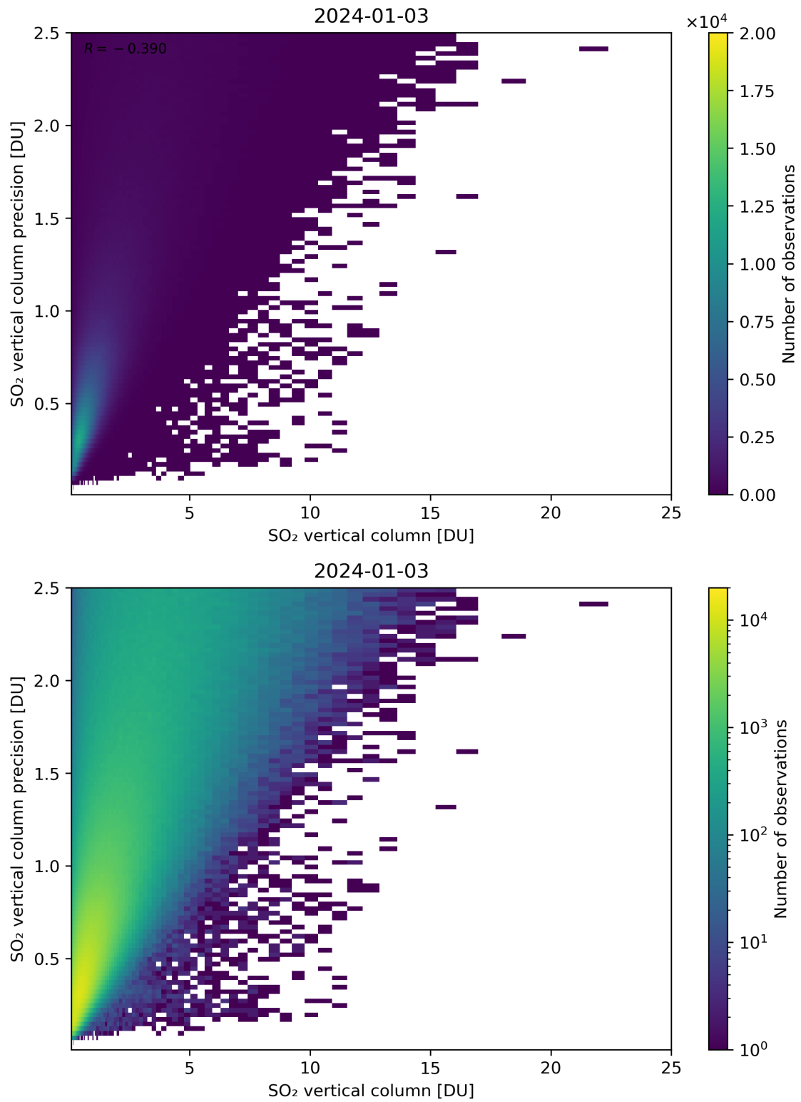
Figure 307: Scatter density plot of “SO 2 vertical column” against “SO 2 vertical column precision” for 2024-01-02 to 2024-01-04.
