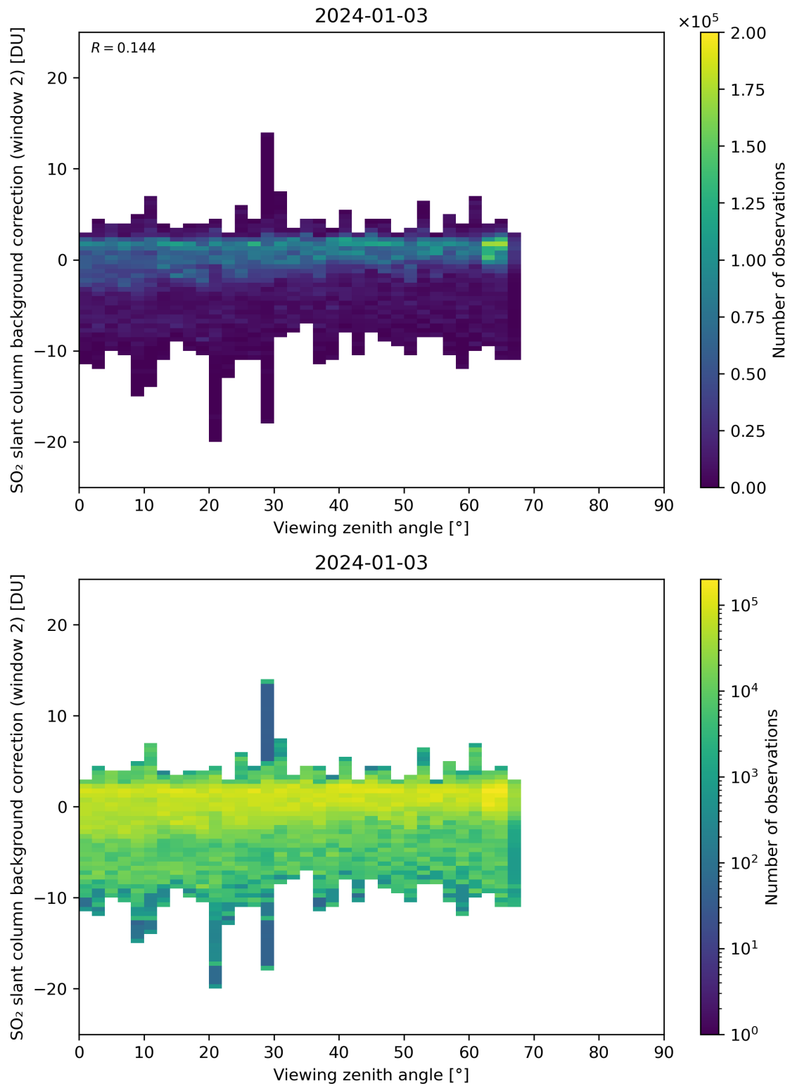
Figure 309: Scatter density plot of “Viewing zenith angle” against “SO 2 slant column background correction (window 2)” for 2024-01-02 to 2024-01-04.
