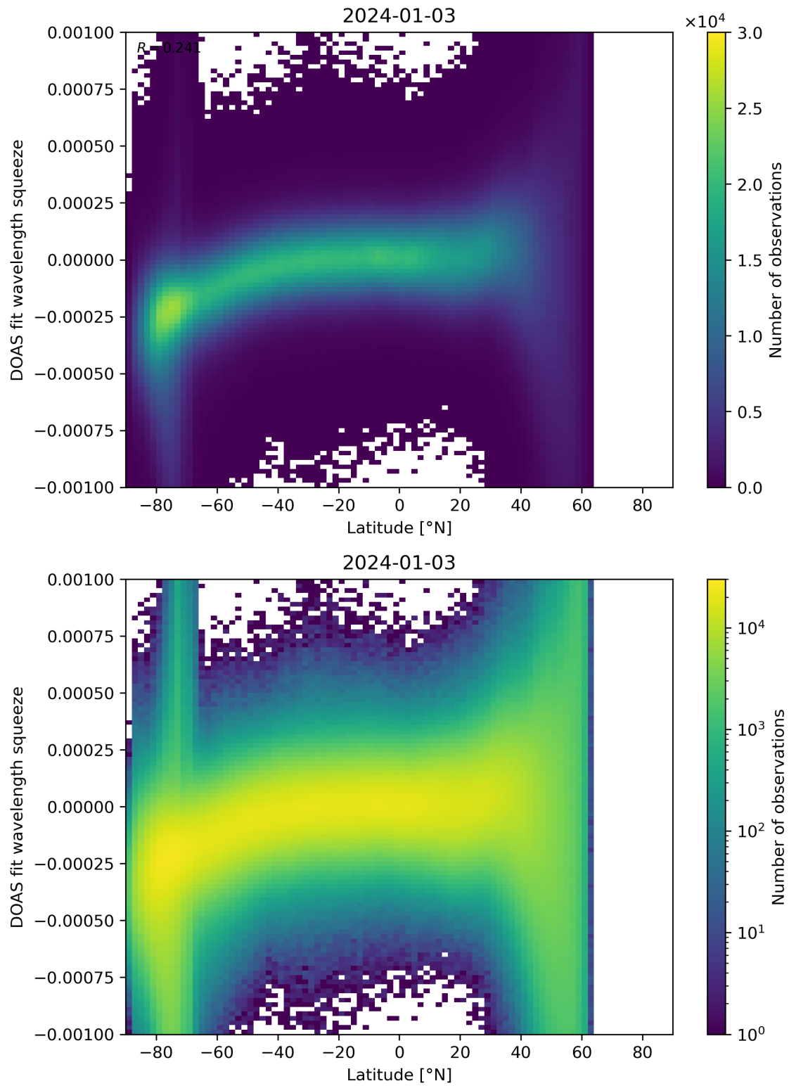
Figure 143: Scatter density plot of “Latitude” against “DOAS fit wavelength squeeze” for 2024-01-02 to 2024-01-04.
