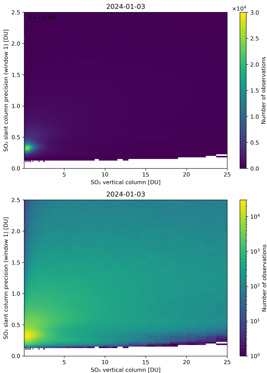
Figure 301: Scatter density plot of “SO 2 vertical column” against “SO 2 slant column precision (window 1)” for 2024-01-02 to 2024-01-04.
