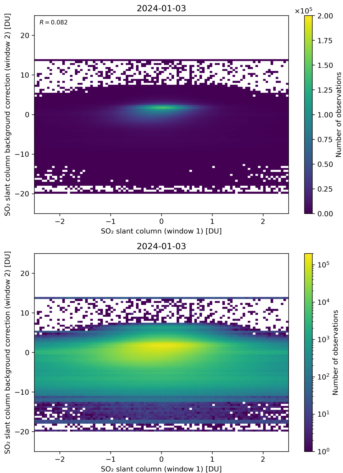
Figure 213: Scatter density plot of “SO 2 slant column (window 1)” against “SO 2 slant column background correction (window 2)” for 2024-01-02 to 2024-01-04.
