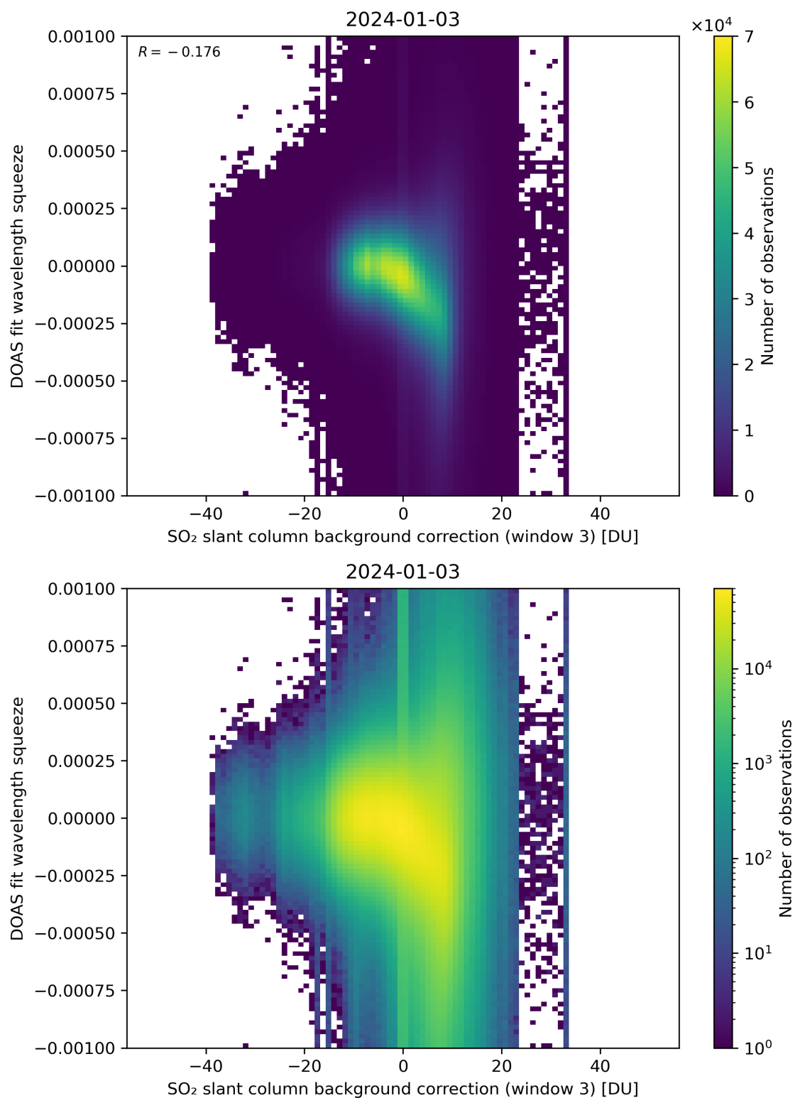
Figure 122: Scatter density plot of “SO 2 slant column background correction (window 3)” against “DOAS fit wavelength squeeze” for 2024-01-02 to 2024-01-04.
