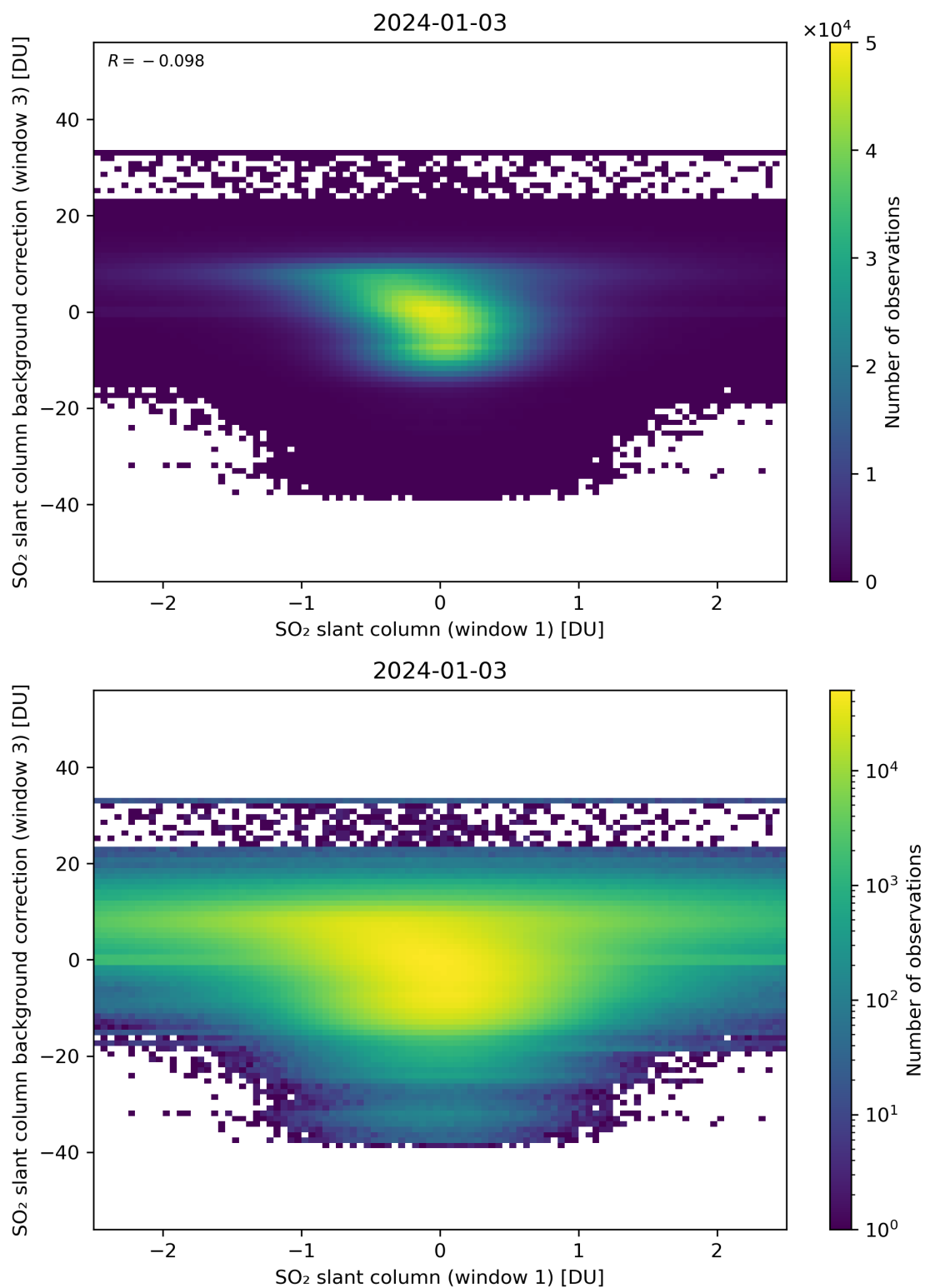
Figure 214: Scatter density plot of “SO 2 slant column (window 1)” against “SO 2 slant column background correction (window 3)” for 2024-01-02 to 2024-01-04.
