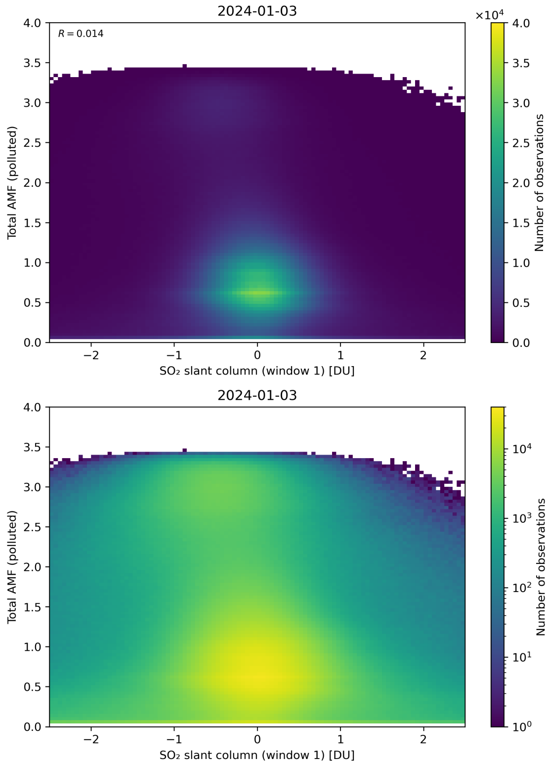
Figure 239: Scatter density plot of “SO 2 slant column (window 1)” against “Total AMF (polluted)” for 2024-01-02 to 2024-01-04.
