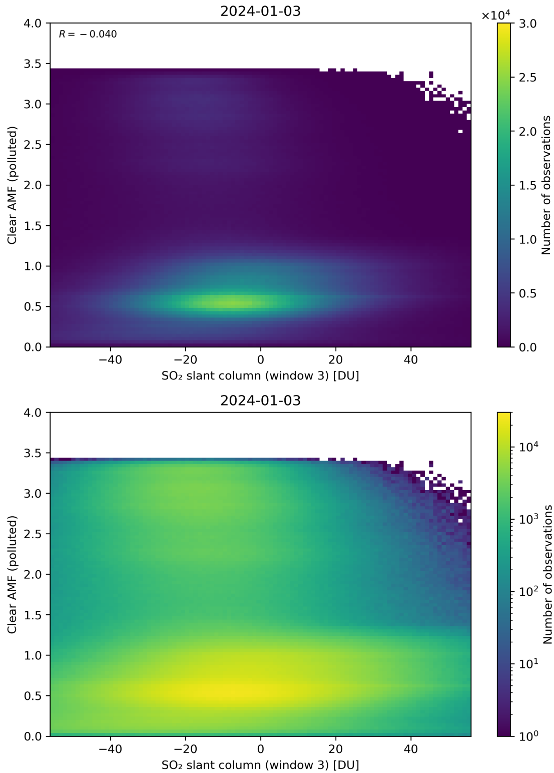
Figure 265: Scatter density plot of “SO 2 slant column (window 3)” against “Clear AMF (polluted)” for 2024-01-02 to 2024-01-04.
