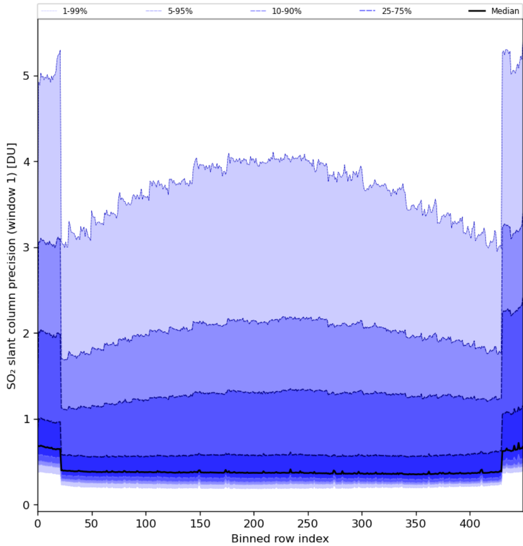
Figure 80: Along track statistics of “SO 2 slant column precision (window 1)” for 2024-01-02 to 2024-01-04
