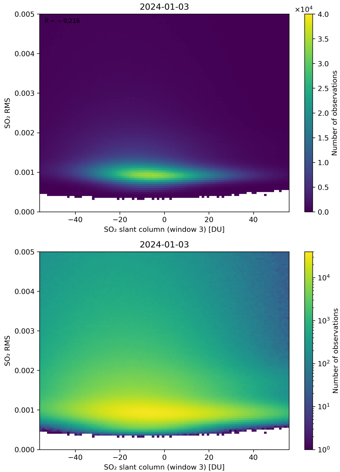
Figure 256: Scatter density plot of “SO 2 slant column (window 3)” against “SO 2 RMS” for 2024-01-02 to 2024-01-04.
