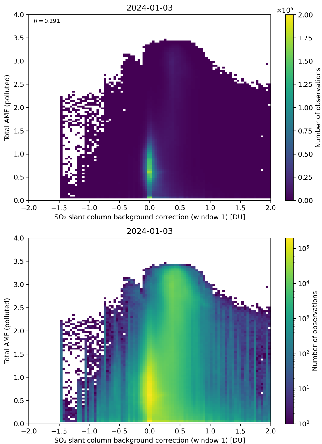
Figure 109: Scatter density plot of “SO 2 slant column background correction (window 1)” against “Total AMF (polluted)” for 2024-01-02 to 2024-01-04.
