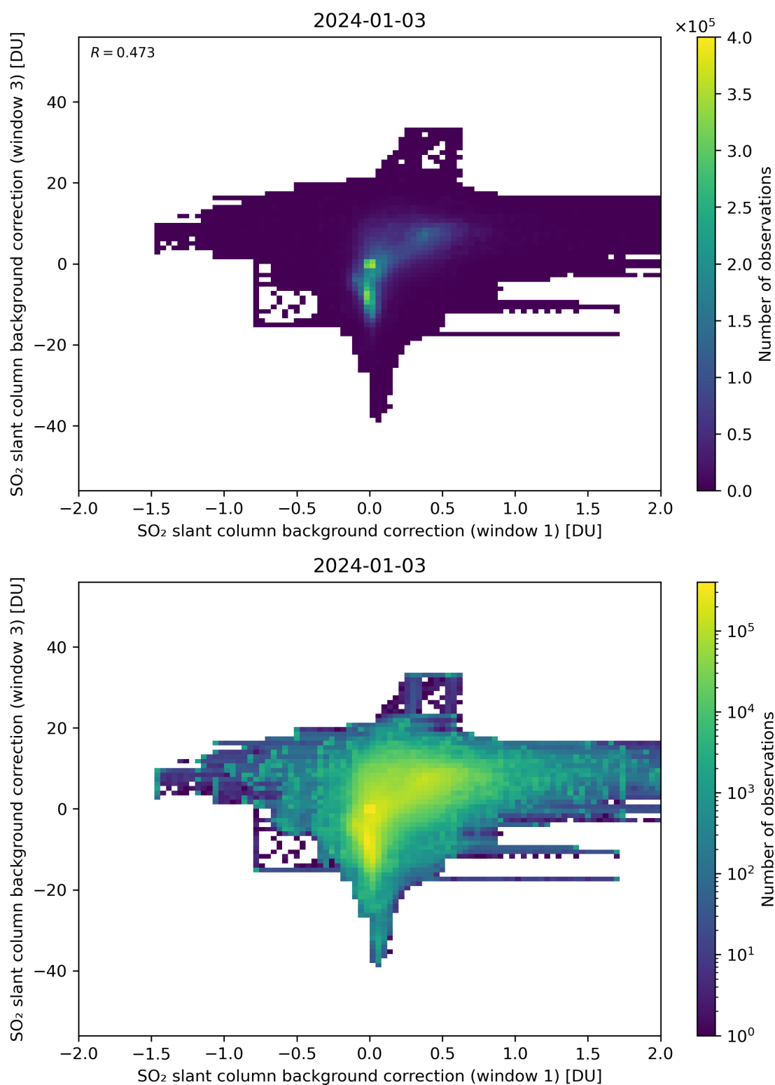
Figure 99: Scatter density plot of “SO 2 slant column background correction (window 1)” against “SO 2 slant column background correction (window 3)” for 2024-01-02 to 2024-01-04.
