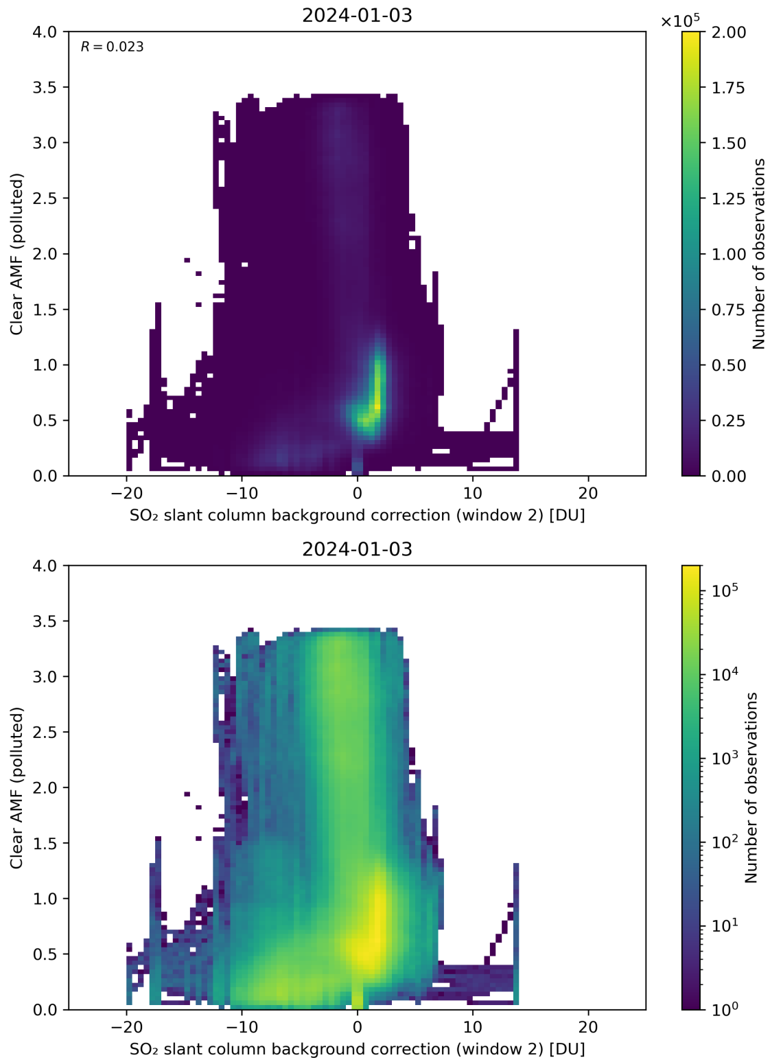
Figure 115: Scatter density plot of “SO 2 slant column background correction (window 2)” against “Clear AMF (polluted)” for 2024-01-02 to 2024-01-04.
