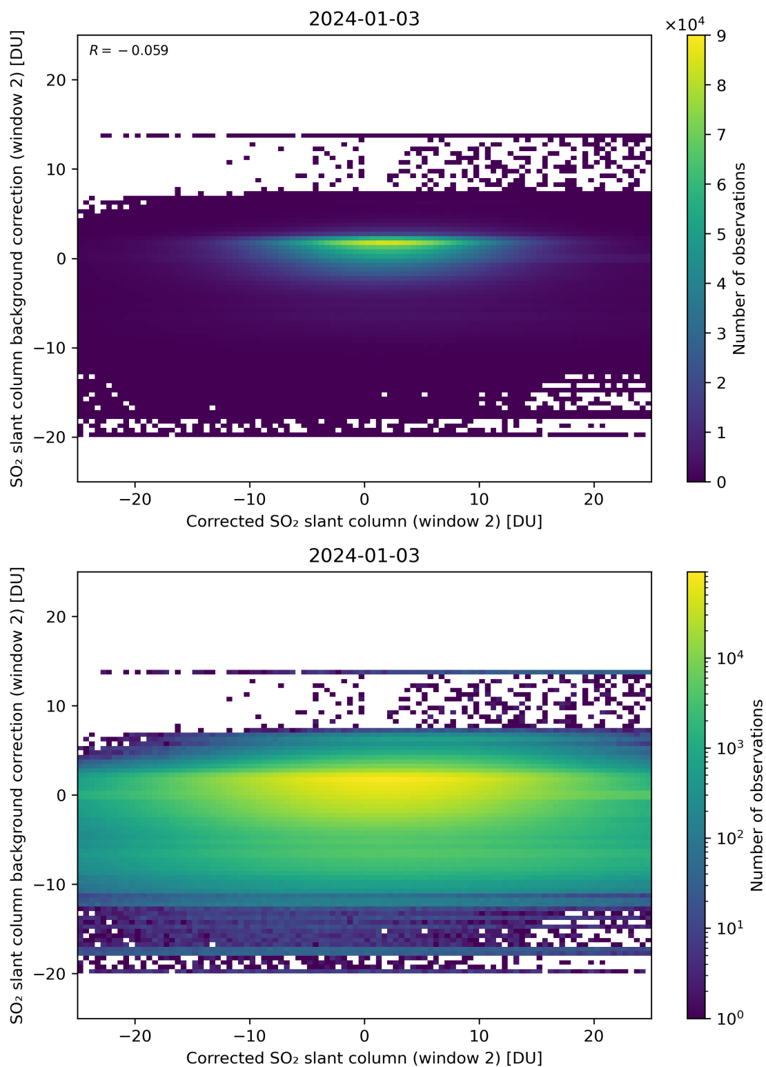
Figure 194: Scatter density plot of “Corrected SO 2 slant column (window 2)” against “SO 2 slant column background correction (window 2)” for 2024-01-02 to 2024-01-04.
