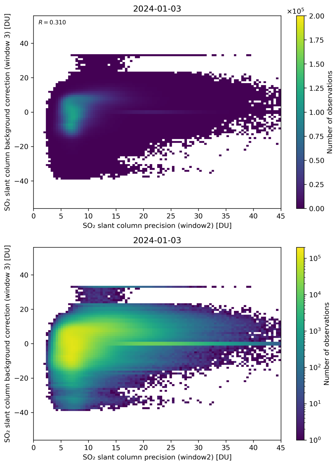
Figure 242: Scatter density plot of “SO 2 slant column precision (window2)” against “SO 2 slant column background correction (window 3)” for 2024-01-02 to 2024-01-04.
