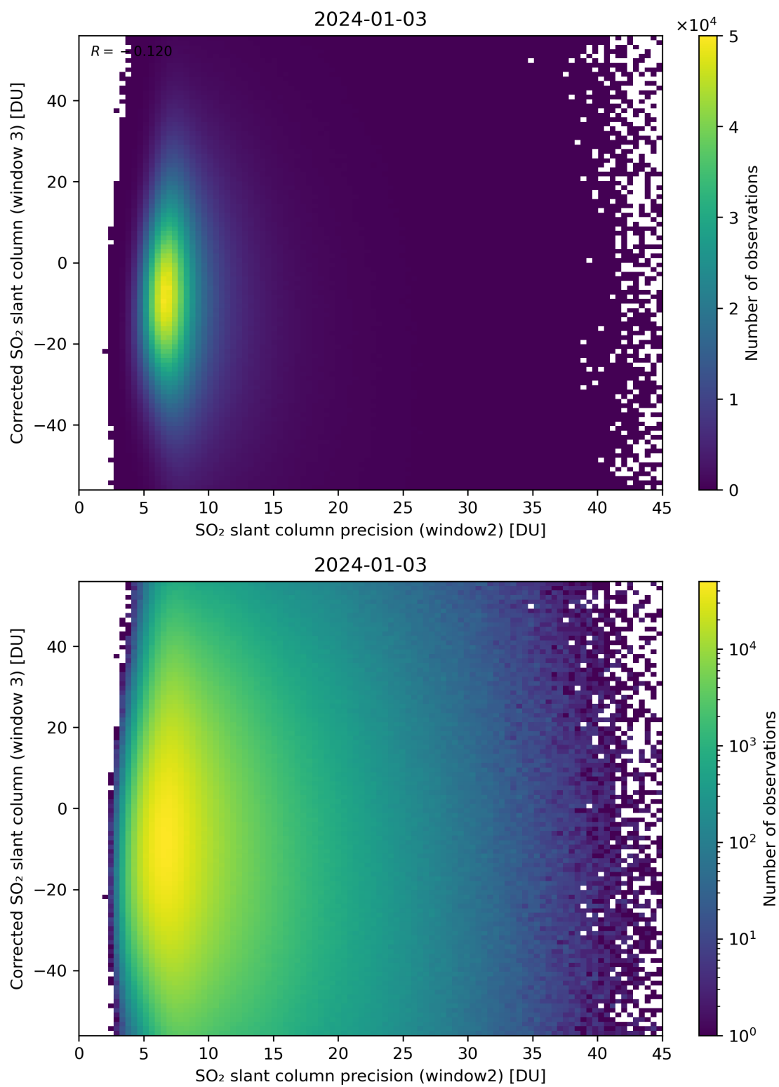
Figure 248: Scatter density plot of “SO 2 slant column precision (window2)” against “Corrected SO 2 slant column (window 3)” for 2024-01-02 to 2024-01-04.
