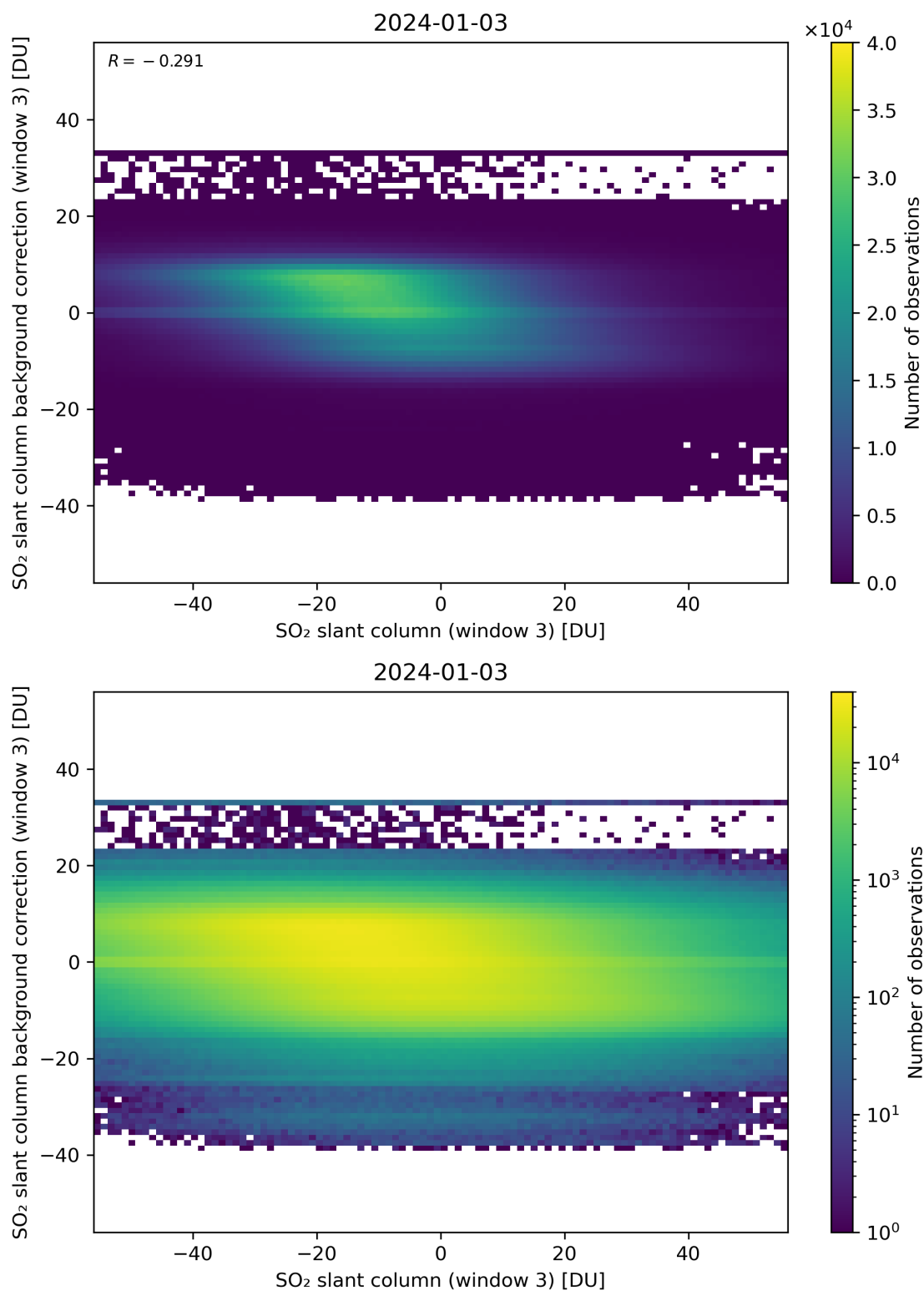
Figure 253: Scatter density plot of “SO 2 slant column (window 3)” against “SO 2 slant column background correction (window 3)” for 2024-01-02 to 2024-01-04.
