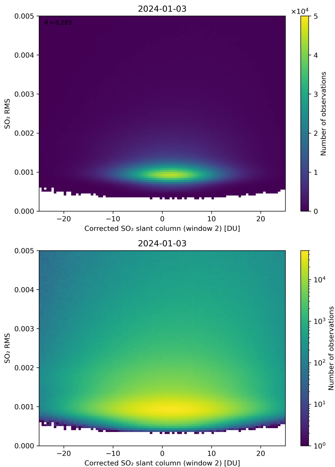
Figure 198: Scatter density plot of “Corrected SO 2 slant column (window 2)” against “SO 2 RMS” for 2024-01-02 to 2024-01-04.
