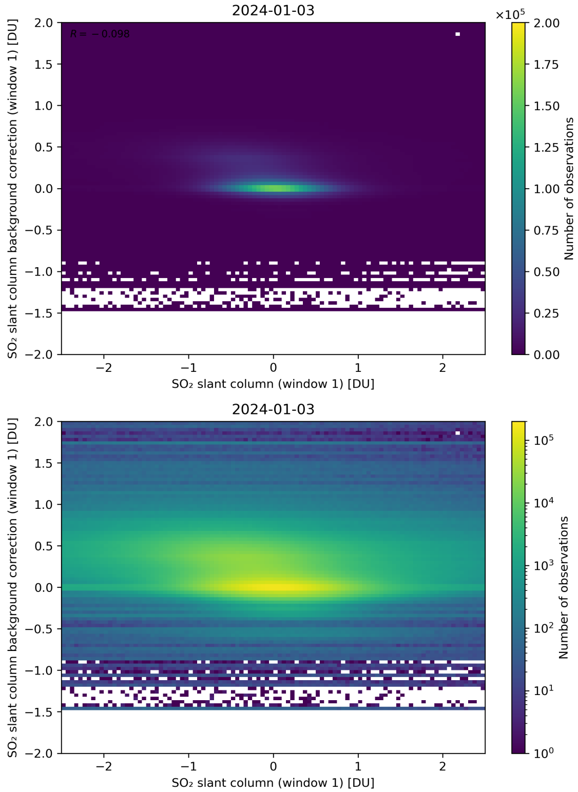
Figure 212: Scatter density plot of “SO 2 slant column (window 1)” against “SO 2 slant column background correction (window 1)” for 2024-01-02 to 2024-01-04.
