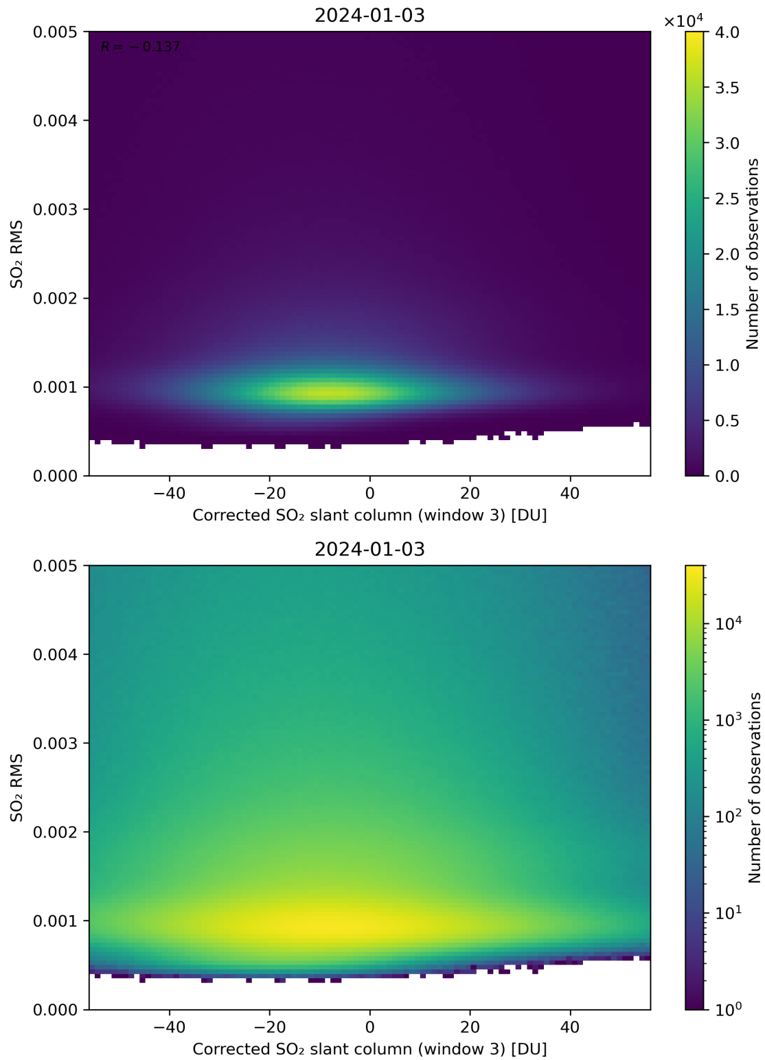
Figure 208: Scatter density plot of “Corrected SO 2 slant column (window 3)” against “SO 2 RMS” for 2024-01-02 to 2024-01-04.
