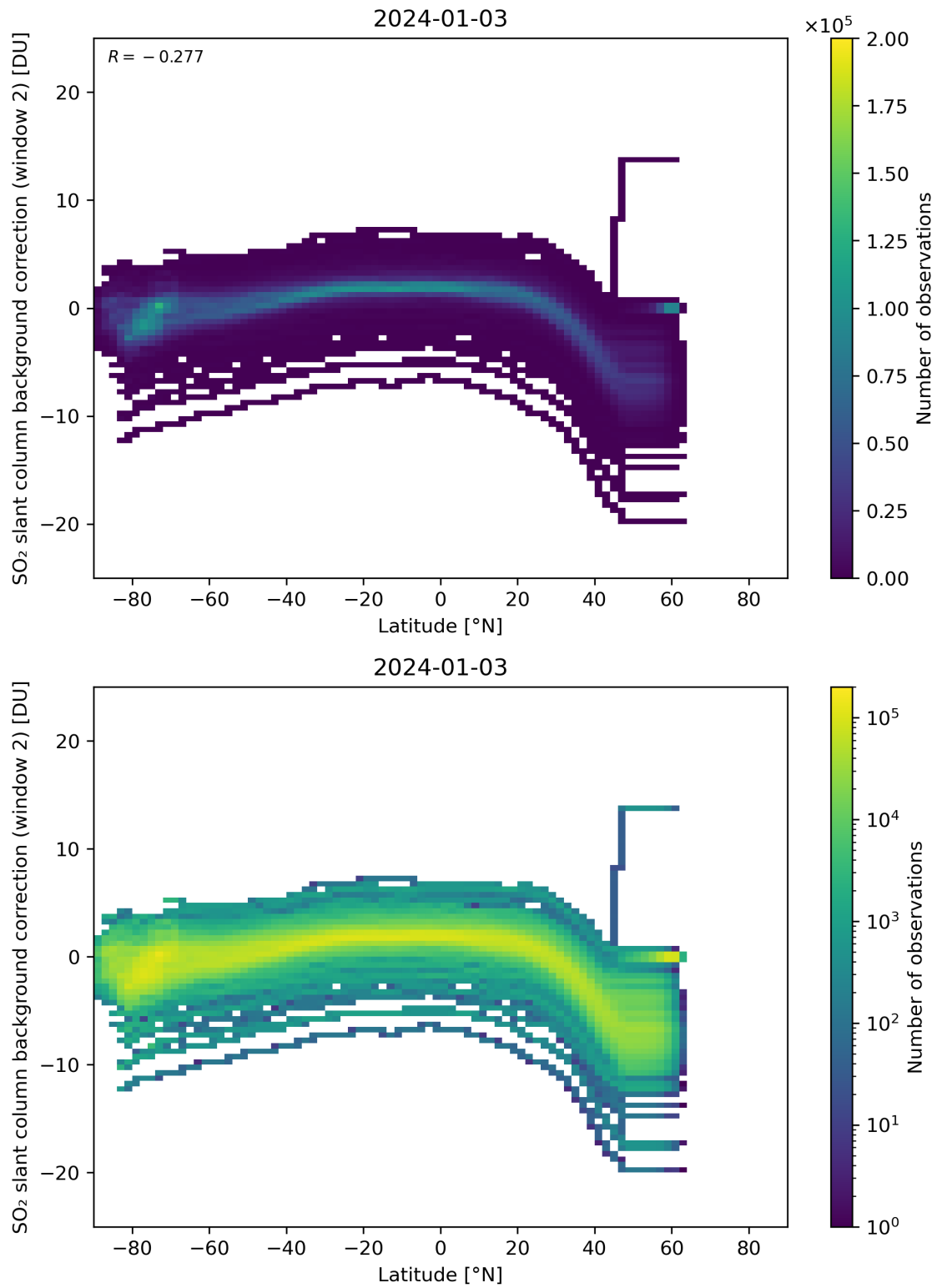
Figure 140: Scatter density plot of “Latitude” against “SO 2 slant column background correction (window 2)” for 2024-01-02 to 2024-01-04.
