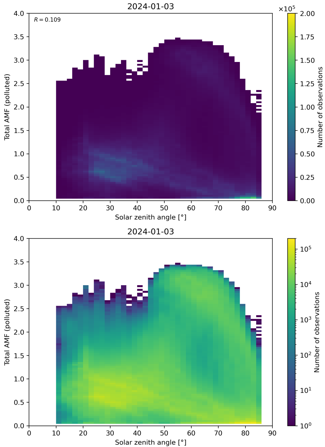
Figure 174: Scatter density plot of “Solar zenith angle” against “Total AMF (polluted)” for 2024-01-02 to 2024-01-04.
