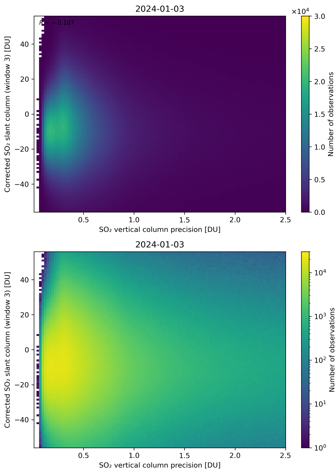
Figure 288: Scatter density plot of “SO 2 vertical column precision” against “Corrected SO 2 slant column (window 3)” for 2024-01-02 to 2024-01-04.
