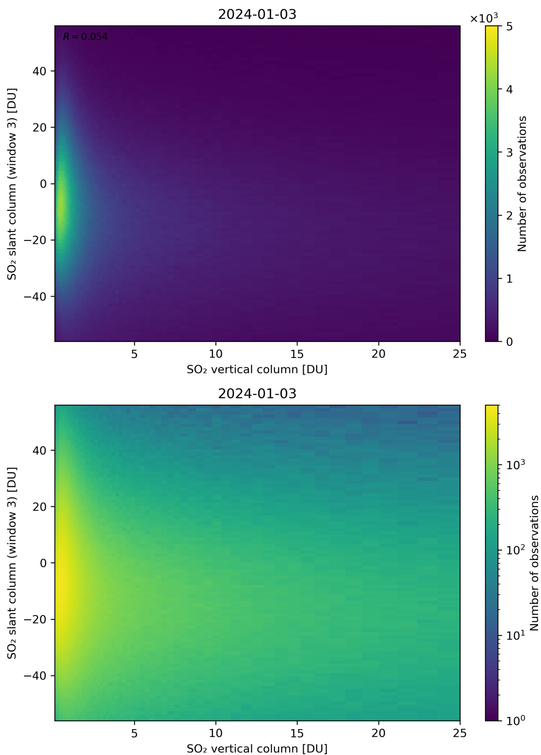
Figure 303: Scatter density plot of “SO 2 vertical column” against “SO 2 slant column (window 3)” for 2024-01-02 to 2024-01-04.
