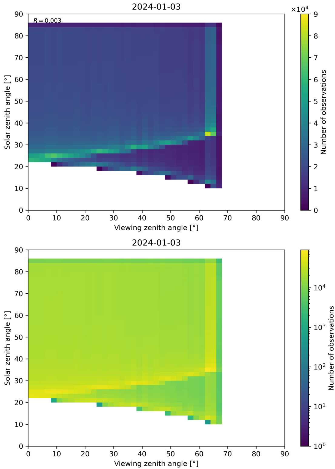
Figure 315: Scatter density plot of “Viewing zenith angle” against “Solar zenith angle” for 2024-01-02 to 2024-01-04.
