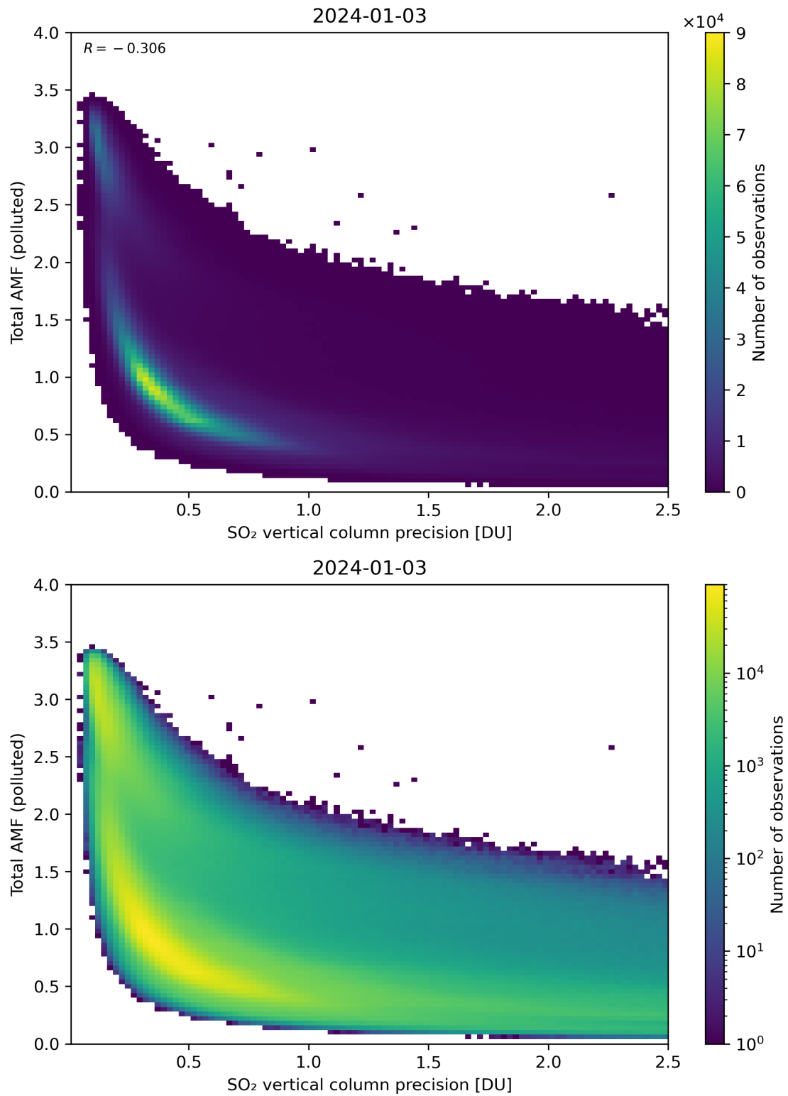
Figure 294: Scatter density plot of “SO 2 vertical column precision” against “Total AMF (polluted)” for 2024-01-02 to 2024-01-04.
