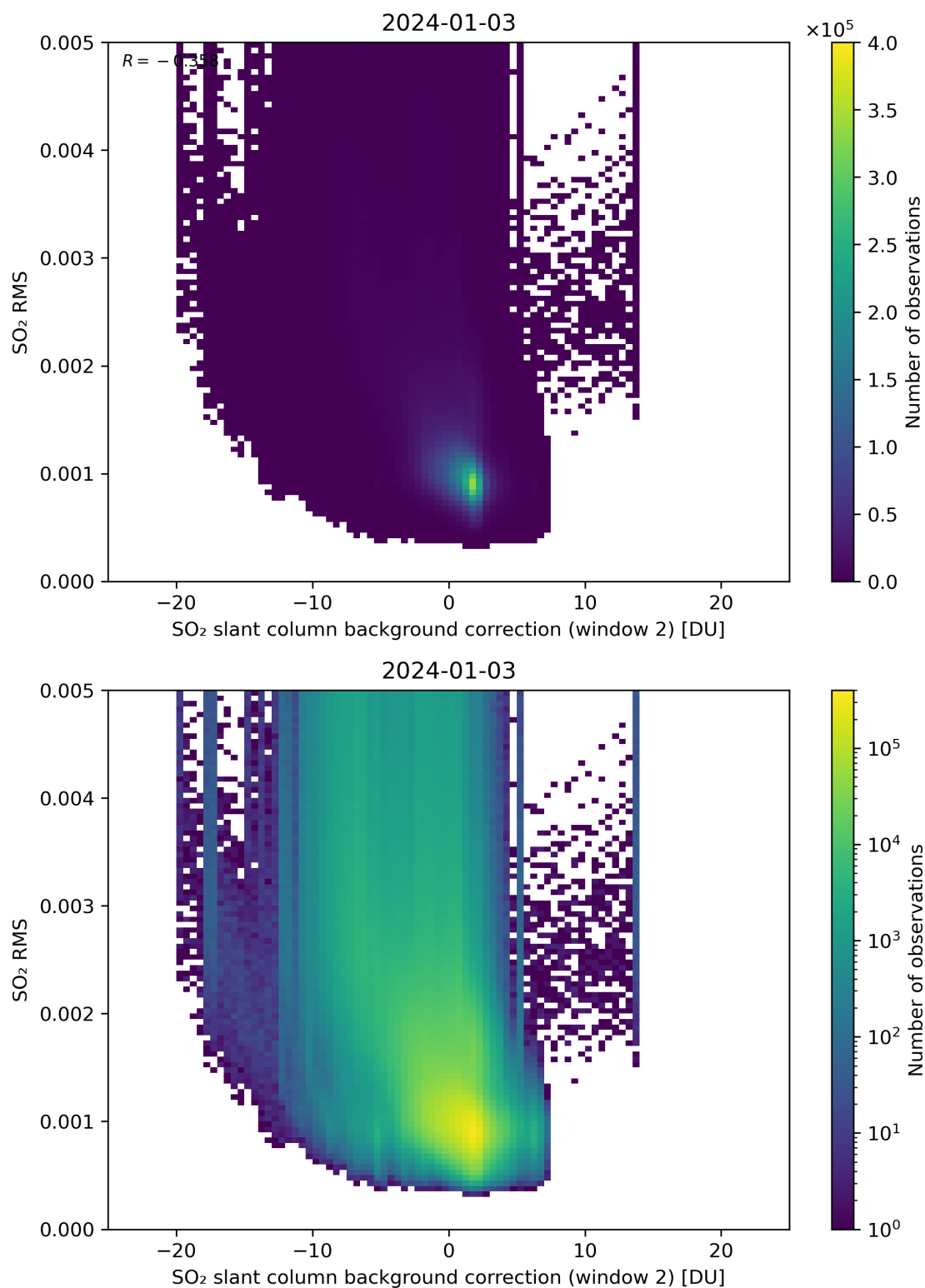
Figure 114: Scatter density plot of “SO 2 slant column background correction (window 2)” against “SO 2 RMS” for 2024-01-02 to 2024-01-04.
