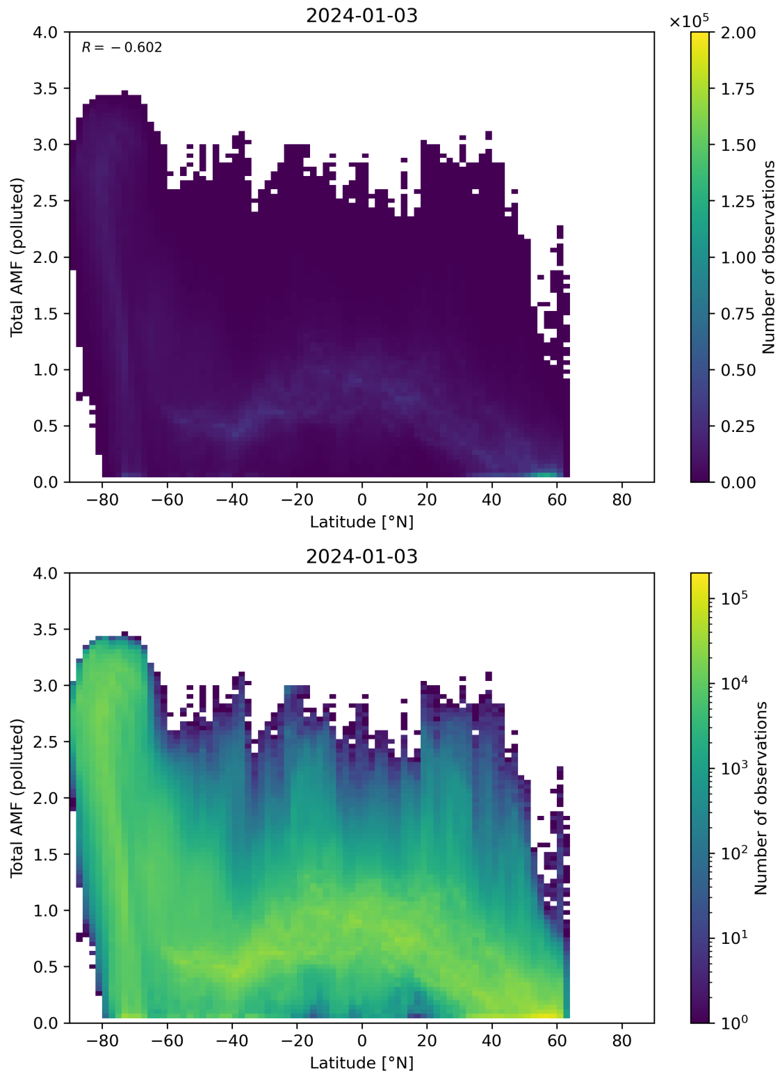
Figure 154: Scatter density plot of “Latitude” against “Total AMF (polluted)” for 2024-01-02 to 2024-01-04.
