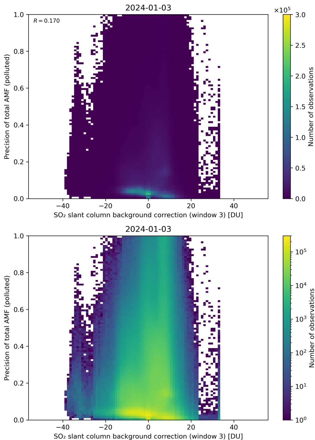
Figure 126: Scatter density plot of “SO 2 slant column background correction (window 3)” against “Precision of total AMF (polluted)” for 2024-01-02 to 2024-01-04.
