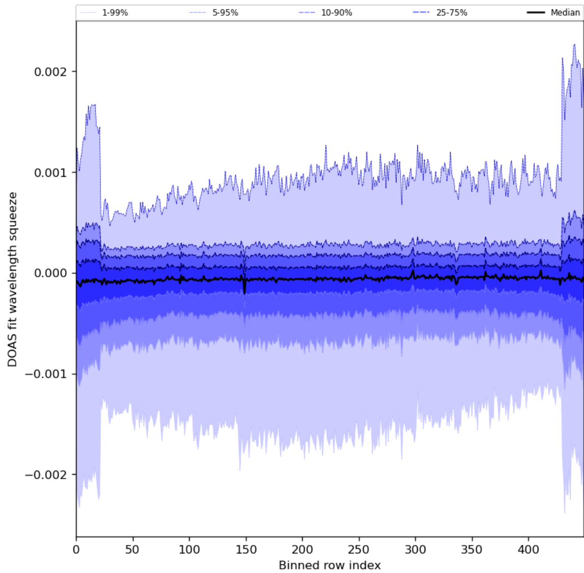
Figure 92: Along track statistics of “DOAS fit wavelength squeeze” for 2024-01-02 to 2024-01-04
