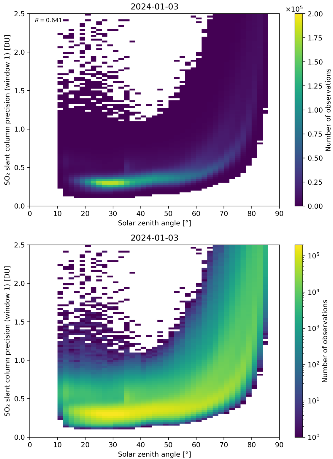
Figure 170: Scatter density plot of “Solar zenith angle” against “SO 2 slant column precision (window 1)” for 2024-01-02 to 2024-01-04.
