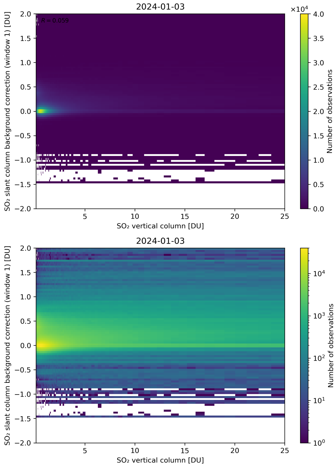
Figure 273: Scatter density plot of “SO 2 vertical column” against “SO 2 slant column background correction (window 1)” for 2024-01-02 to 2024-01-04.
