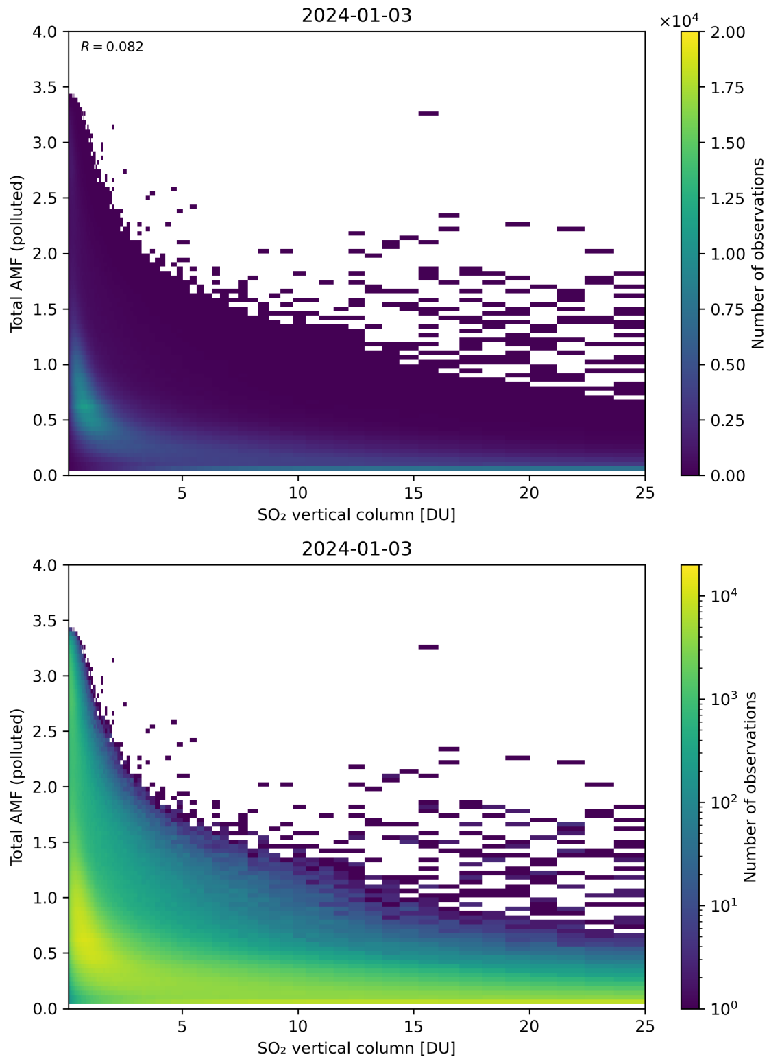
Figure 305: Scatter density plot of “SO 2 vertical column” against “Total AMF (polluted)” for 2024-01-02 to 2024-01-04.
