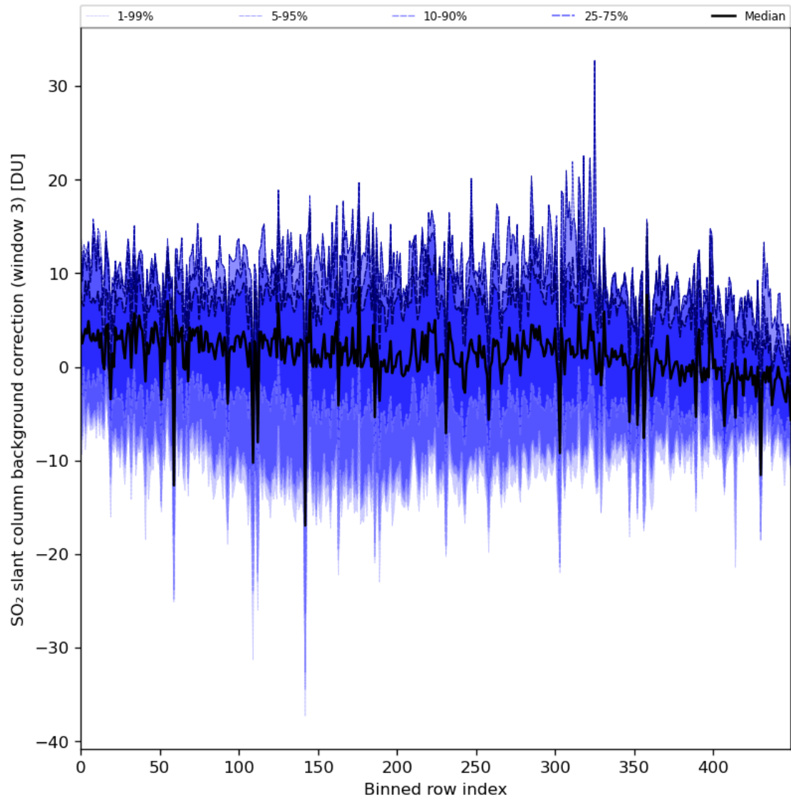
Figure 90: Along track statistics of “SO 2 slant column background correction (window 3)” for 2024-01-02 to 2024-01-04
