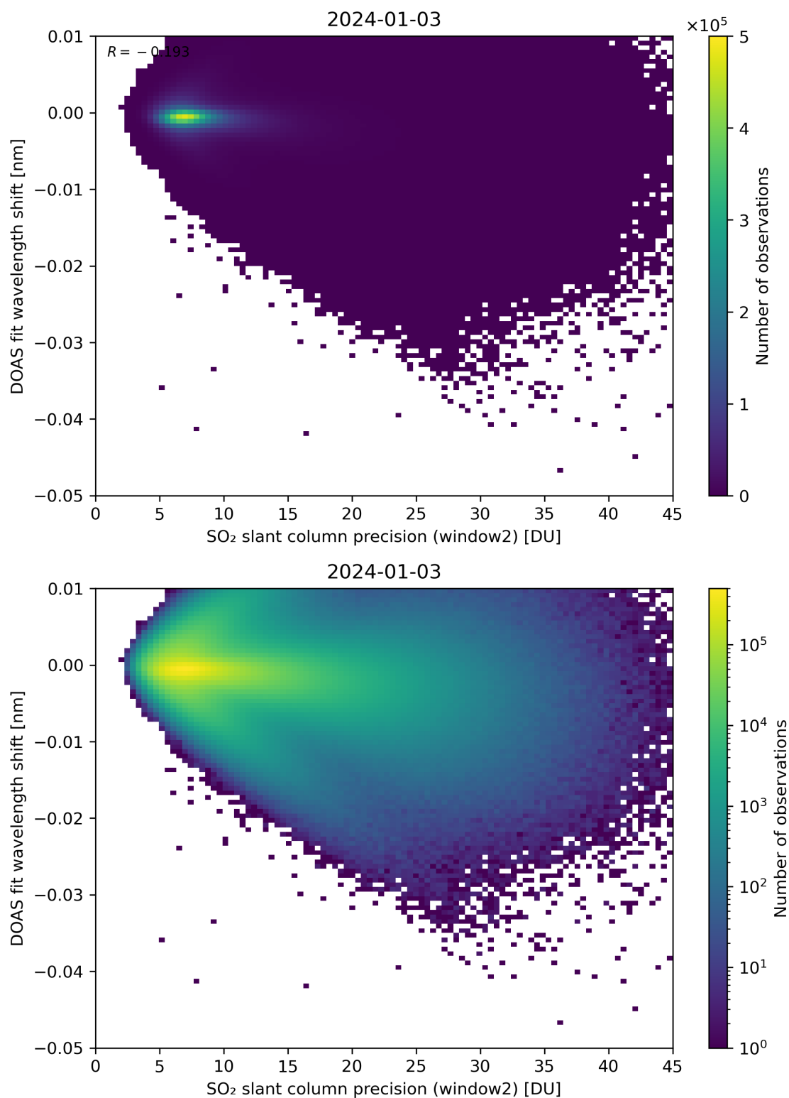
Figure 243: Scatter density plot of “SO 2 slant column precision (window2)” against “DOAS fit wavelength shift” for 2024-01-02 to 2024-01-04.
