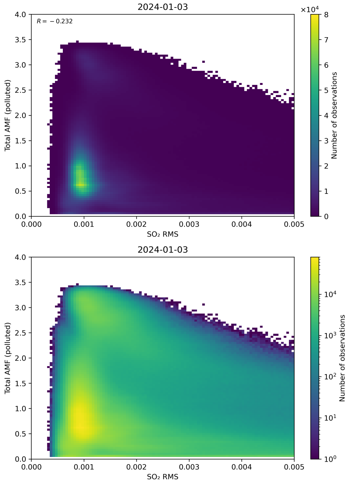
Figure 137: Scatter density plot of “SO 2 RMS” against “Total AMF (polluted)” for 2024-01-02 to 2024-01-04.
