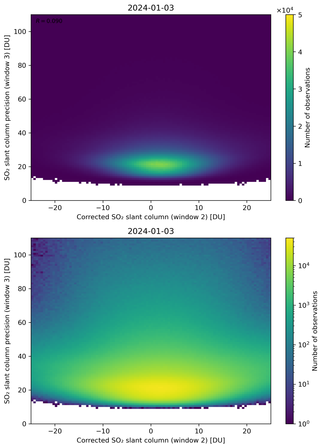
Figure 202: Scatter density plot of “Corrected SO 2 slant column (window 2)” against “SO 2 slant column precision (window 3)” for 2024-01-02 to 2024-01-04.
