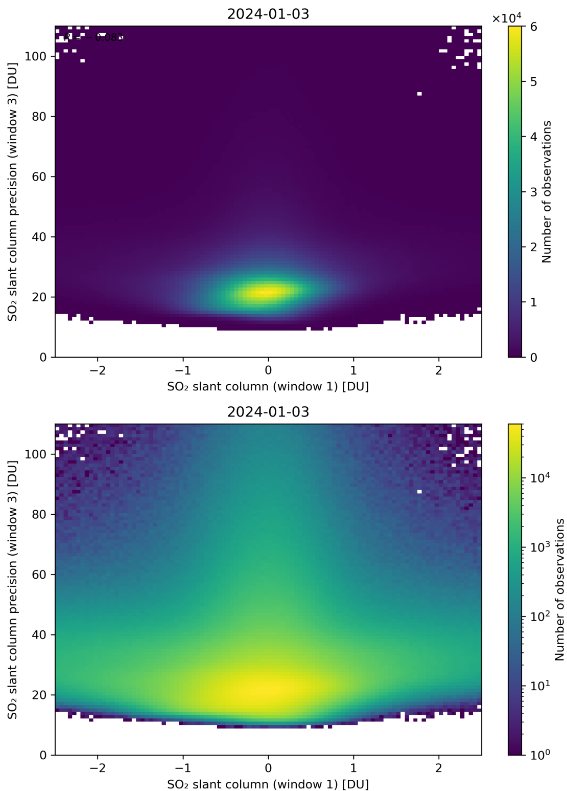
Figure 238: Scatter density plot of “SO 2 slant column (window 1)” against “SO 2 slant column precision (window 3)” for 2024-01-02 to 2024-01-04.
