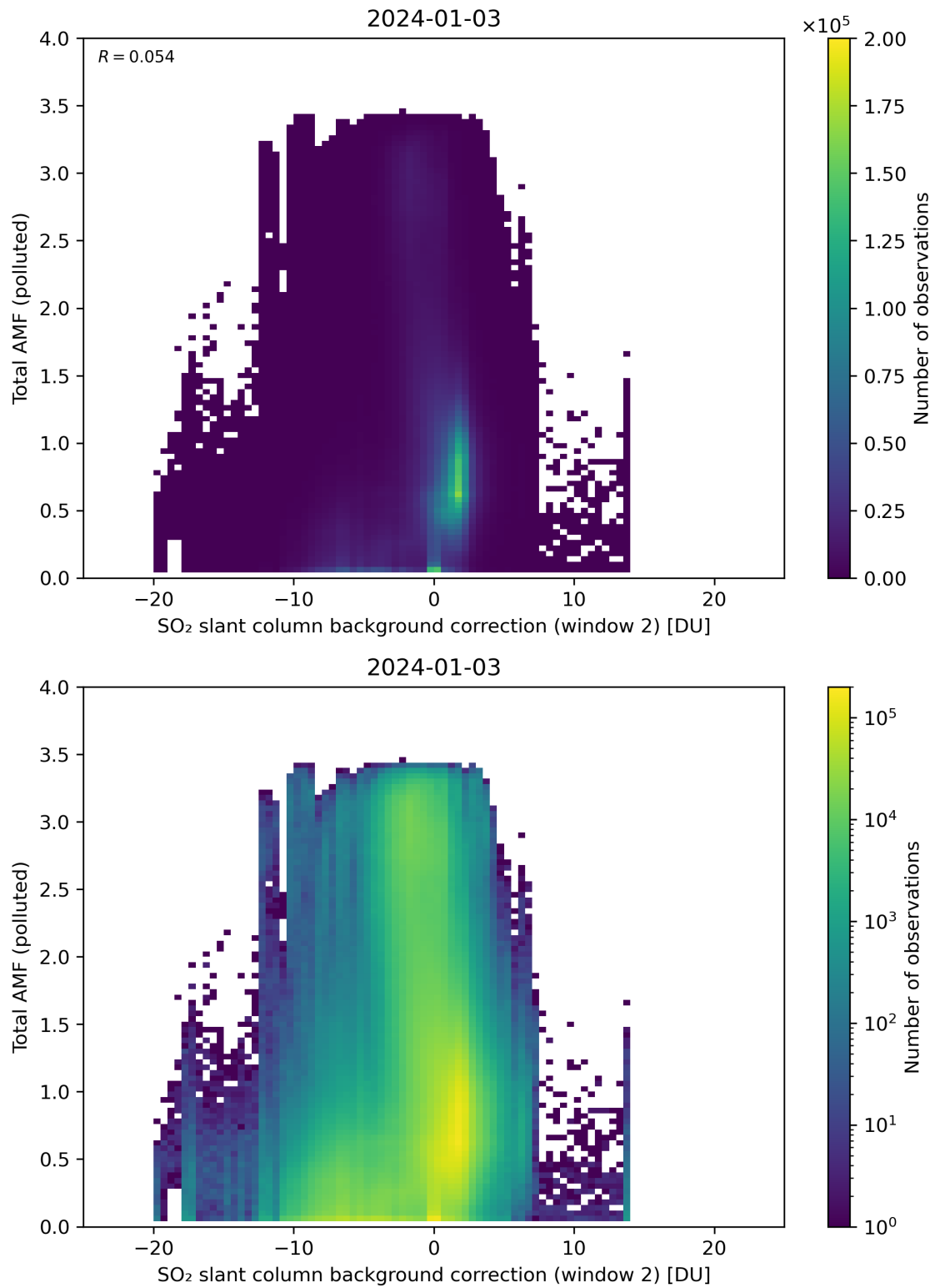
Figure 119: Scatter density plot of “SO 2 slant column background correction (window 2)” against “Total AMF (polluted)” for 2024-01-02 to 2024-01-04.
