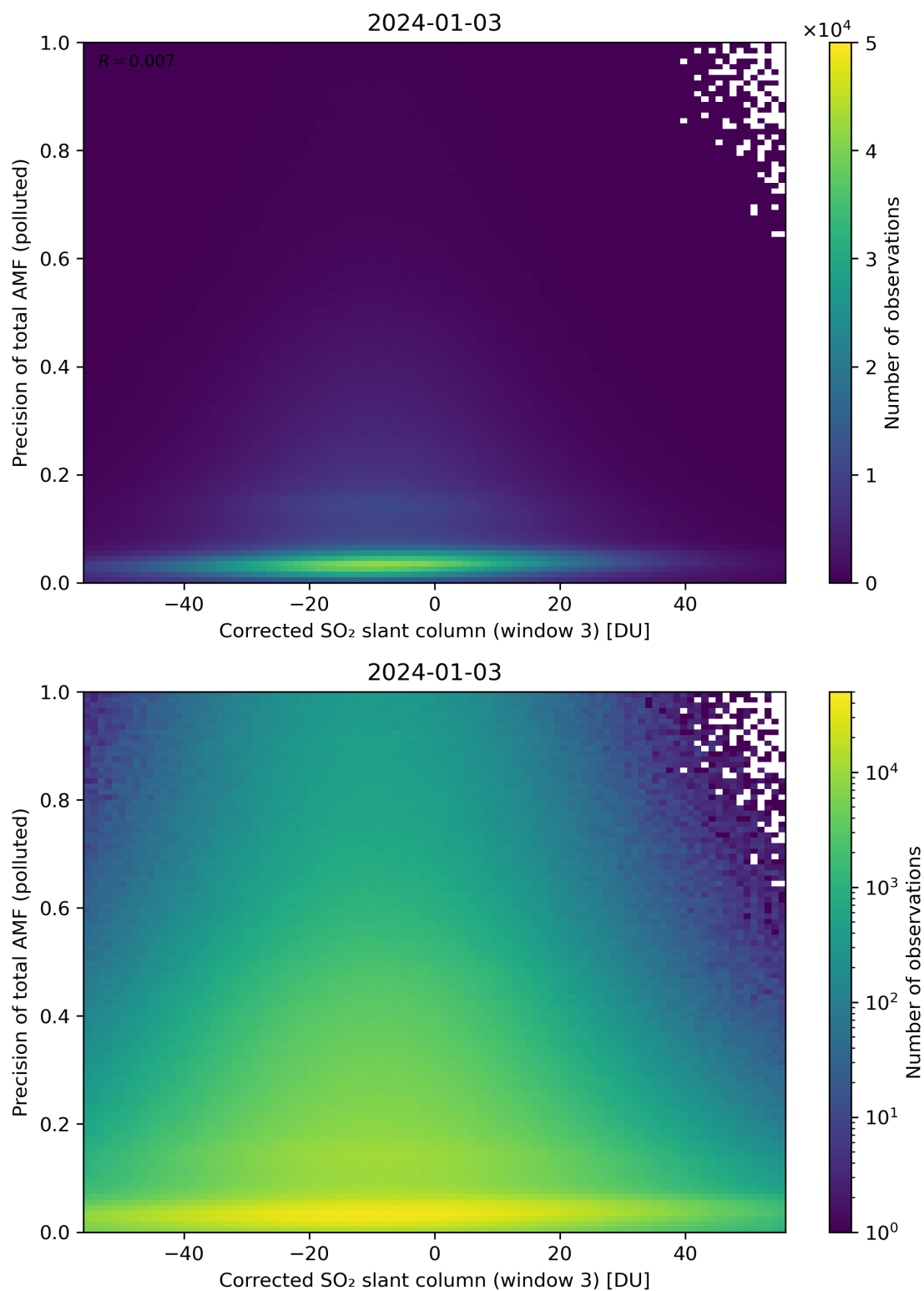
Figure 211: Scatter density plot of “Corrected SO 2 slant column (window 3)” against “Precision of total AMF (polluted)” for 2024-01-02 to 2024-01-04.
