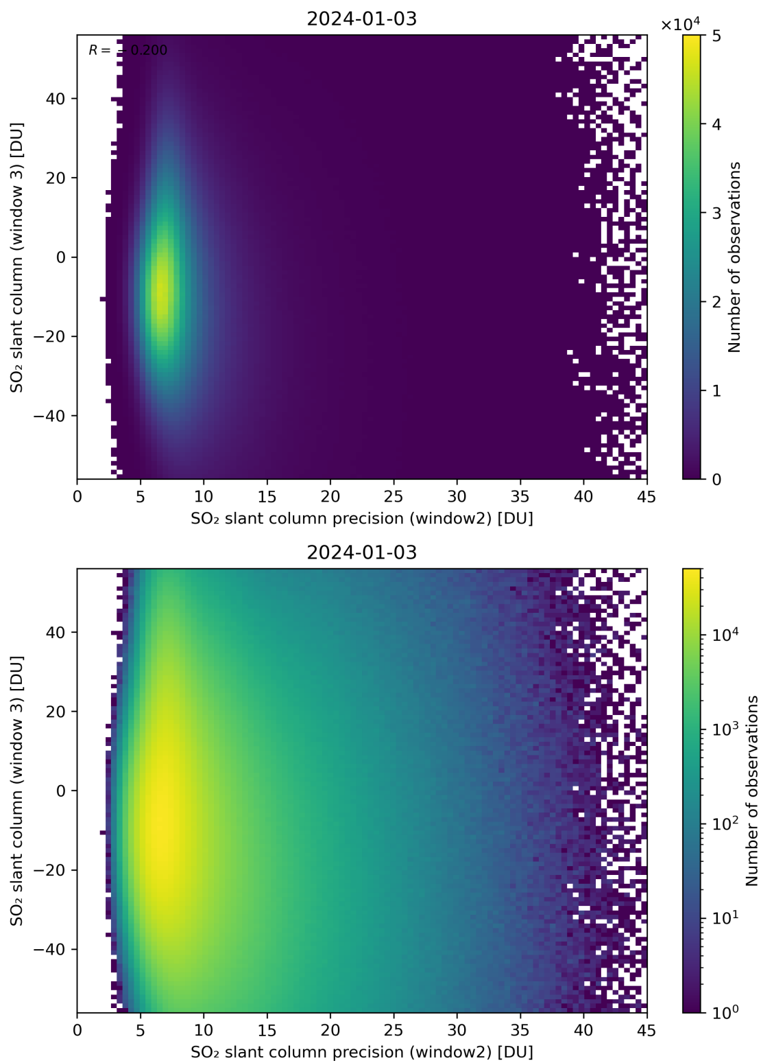
Figure 249: Scatter density plot of “SO 2 slant column precision (window2)” against “SO 2 slant column (window 3)” for 2024-01-02 to 2024-01-04.
