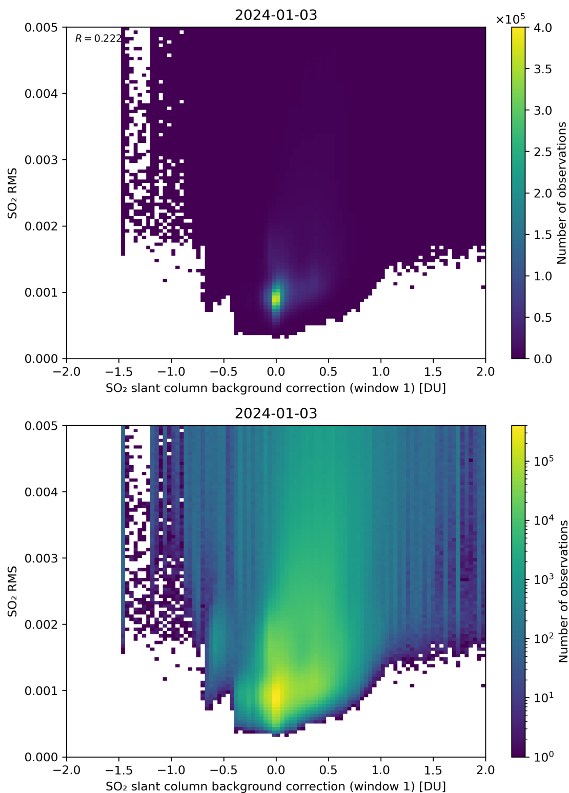
Figure 102: Scatter density plot of “SO 2 slant column background correction (window 1)” against “SO 2 RMS” for 2024-01-02 to 2024-01-04.
