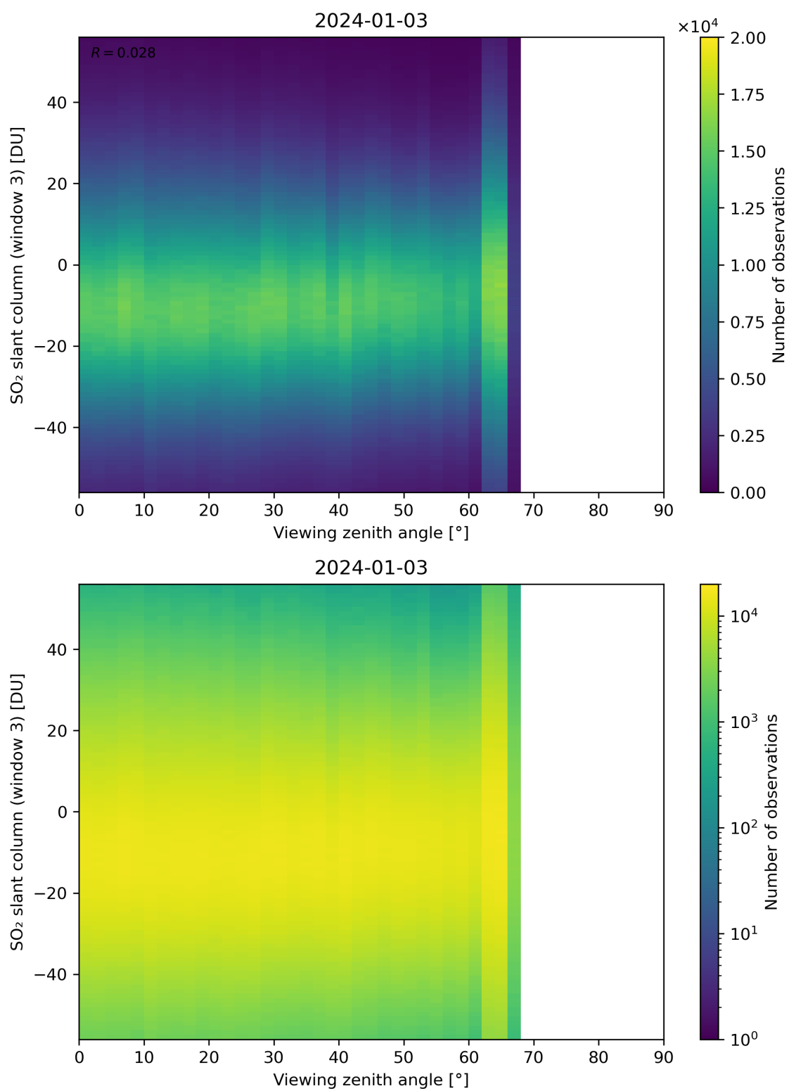
Figure 323: Scatter density plot of “Viewing zenith angle” against “SO 2 slant column (window 3)” for 2024-01-02 to 2024-01-04.
