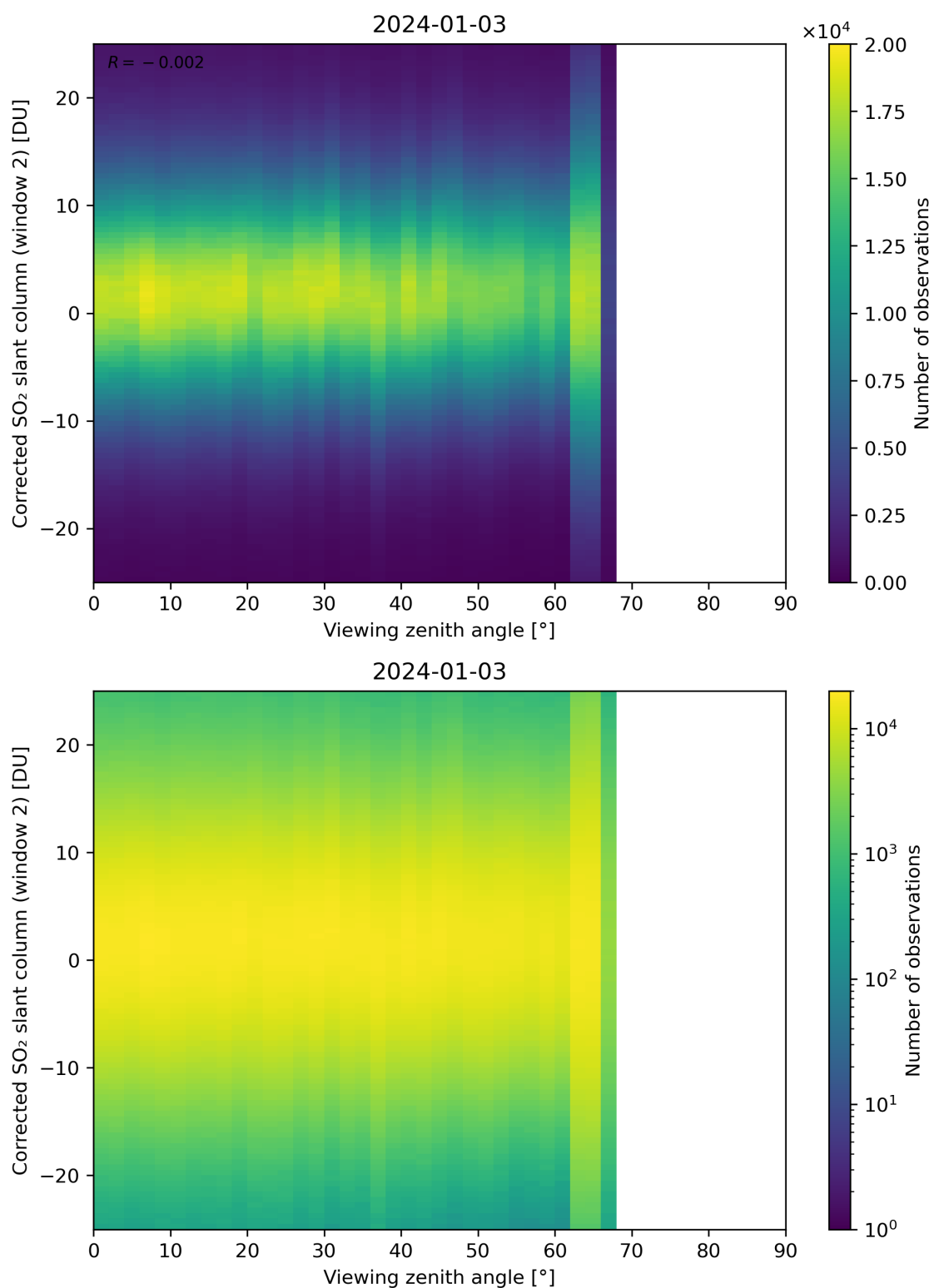
Figure 318: Scatter density plot of “Viewing zenith angle” against “Corrected SO 2 slant column (window 2)” for 2024-01-02 to 2024-01-04.
