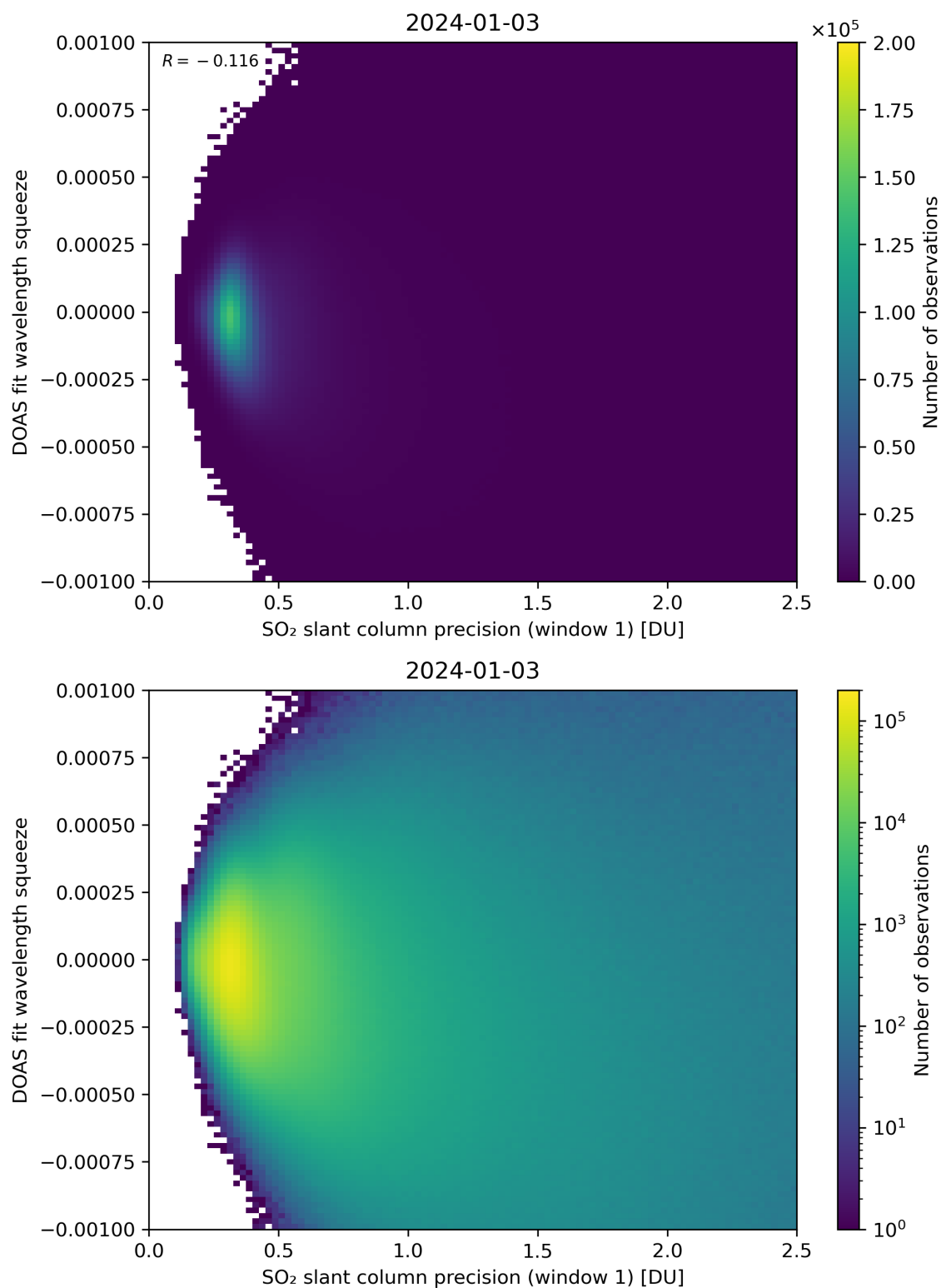
Figure 222: Scatter density plot of “SO 2 slant column precision (window 1)” against “DOAS fit wavelength squeeze” for 2024-01-02 to 2024-01-04.
