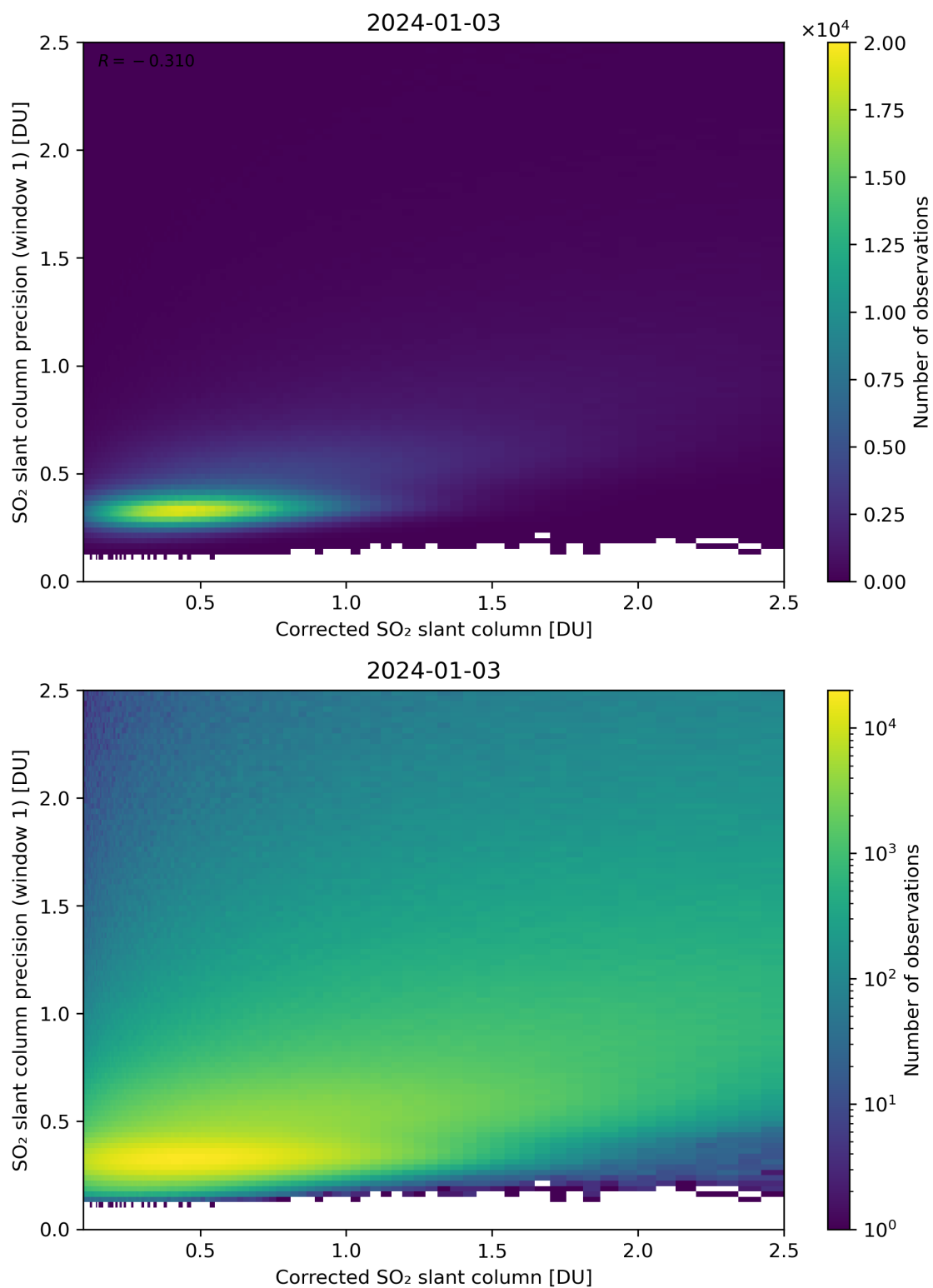
Figure 188: Scatter density plot of “Corrected SO 2 slant column” against “SO 2 slant column precision (window 1)” for 2024-01-02 to 2024-01-04.
