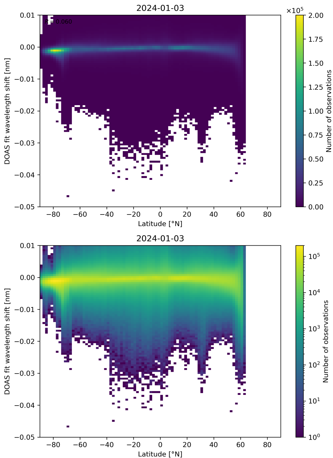
Figure 142: Scatter density plot of “Latitude” against “DOAS fit wavelength shift” for 2024-01-02 to 2024-01-04.
