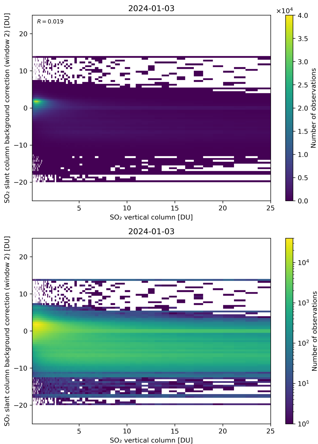
Figure 274: Scatter density plot of “SO 2 vertical column” against “SO 2 slant column background correction (window 2)” for 2024-01-02 to 2024-01-04.
