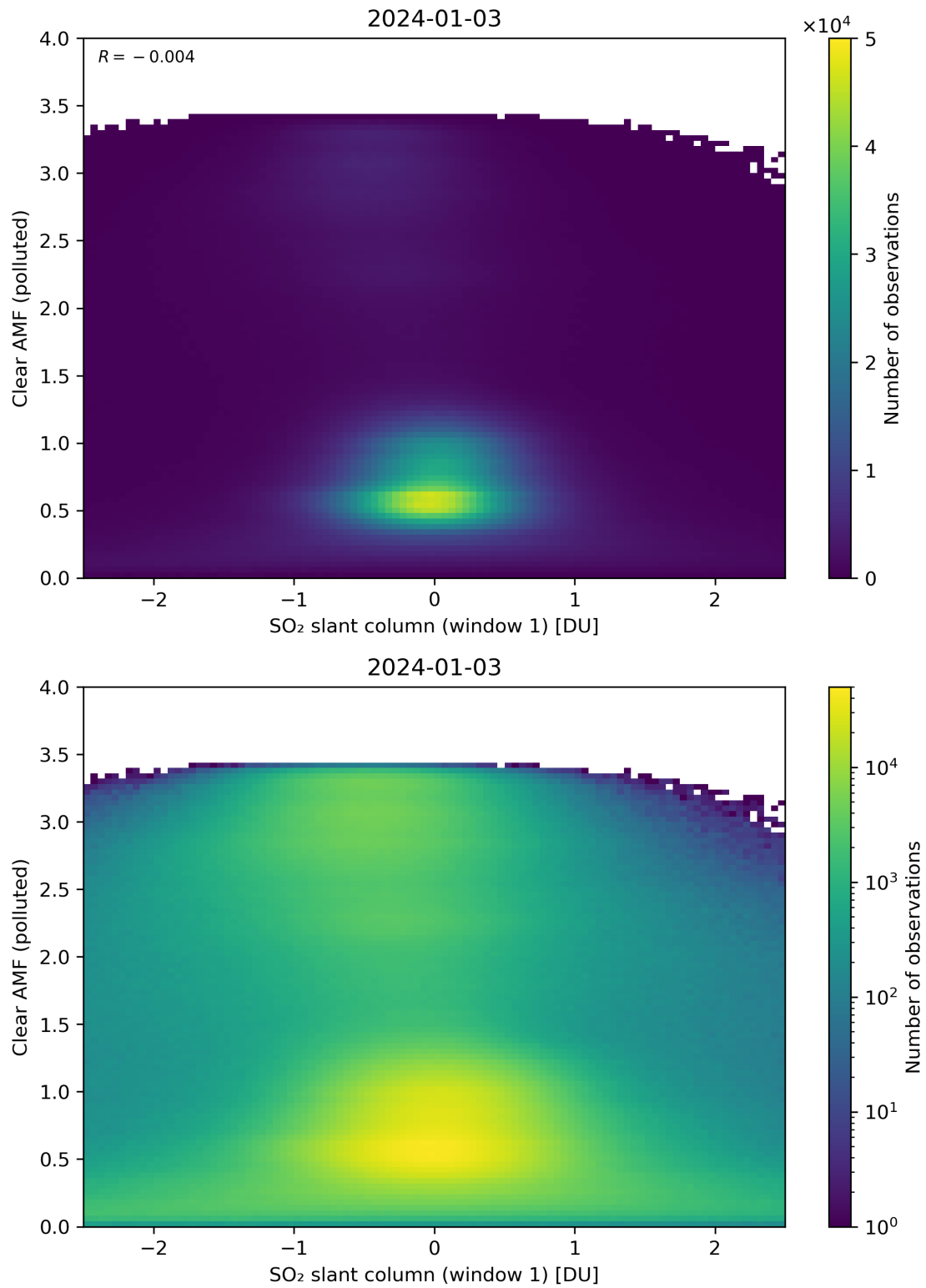
Figure 232: Scatter density plot of “SO 2 slant column (window 1)” against “Clear AMF (polluted)” for 2024-01-02 to 2024-01-04.
