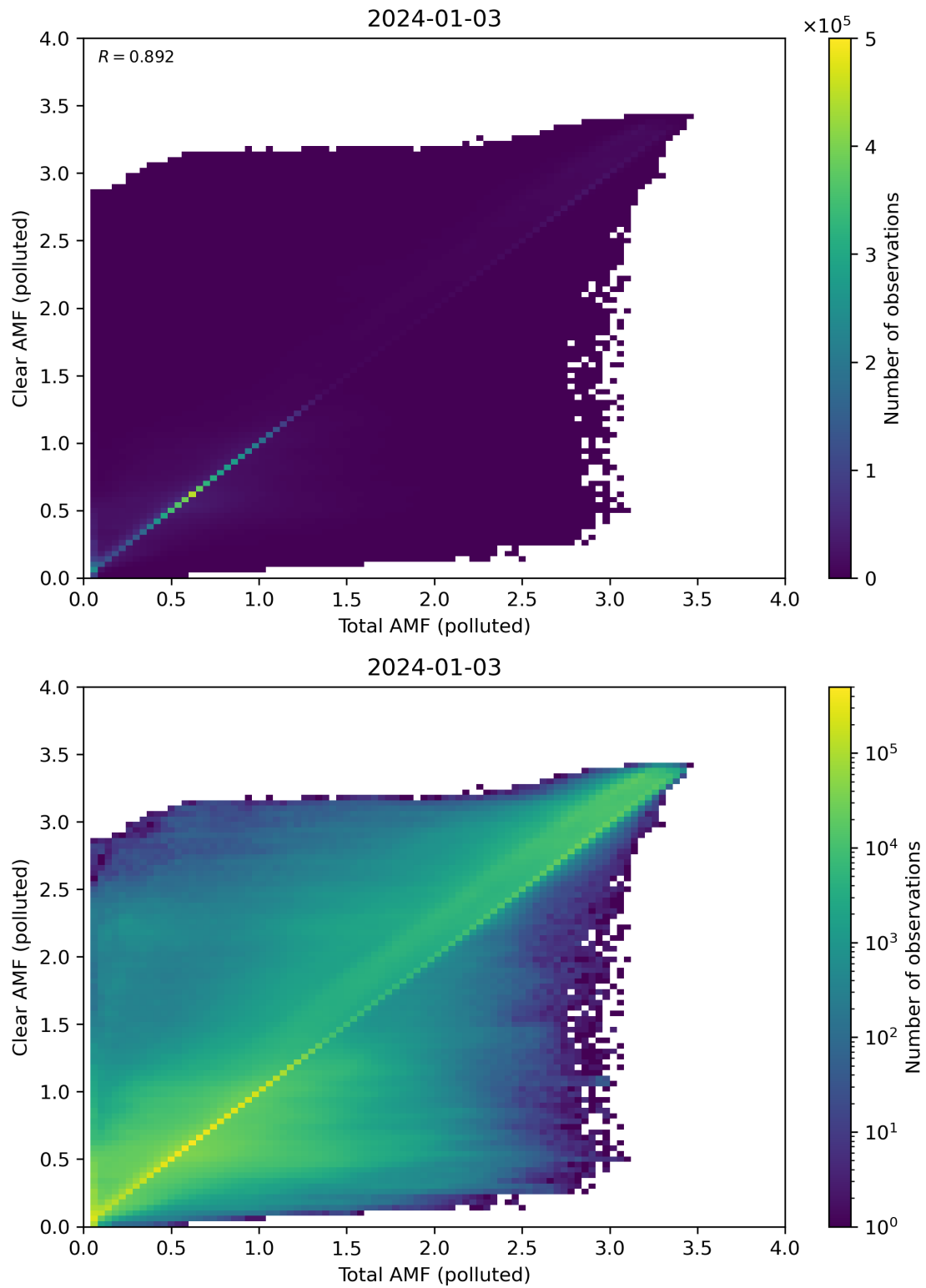
Figure 271: Scatter density plot of “Total AMF (polluted)” against “Clear AMF (polluted)” for 2024-01-02 to 2024-01-04.
