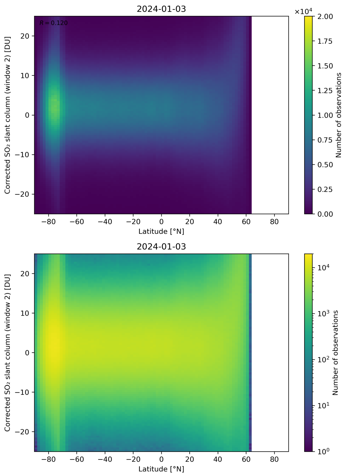
Figure 147: Scatter density plot of “Latitude” against “Corrected SO 2 slant column (window 2)” for 2024-01-02 to 2024-01-04.
