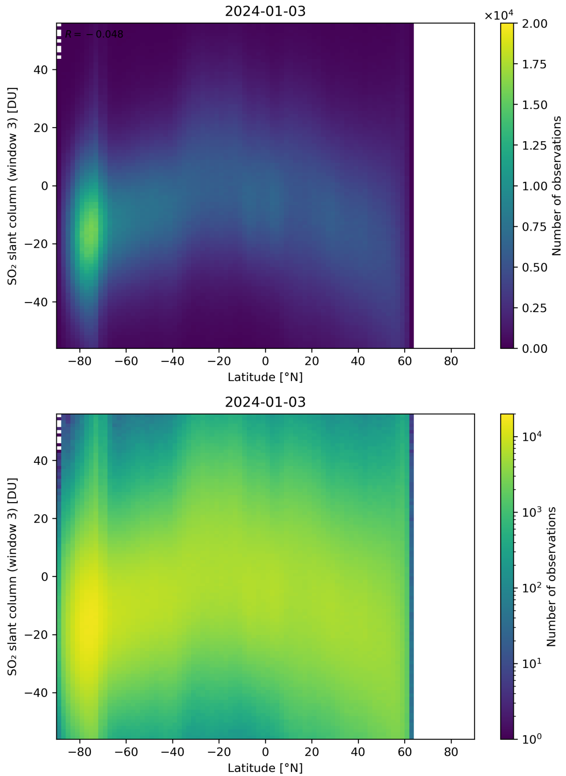
Figure 152: Scatter density plot of “Latitude” against “SO 2 slant column (window 3)” for 2024-01-02 to 2024-01-04.
