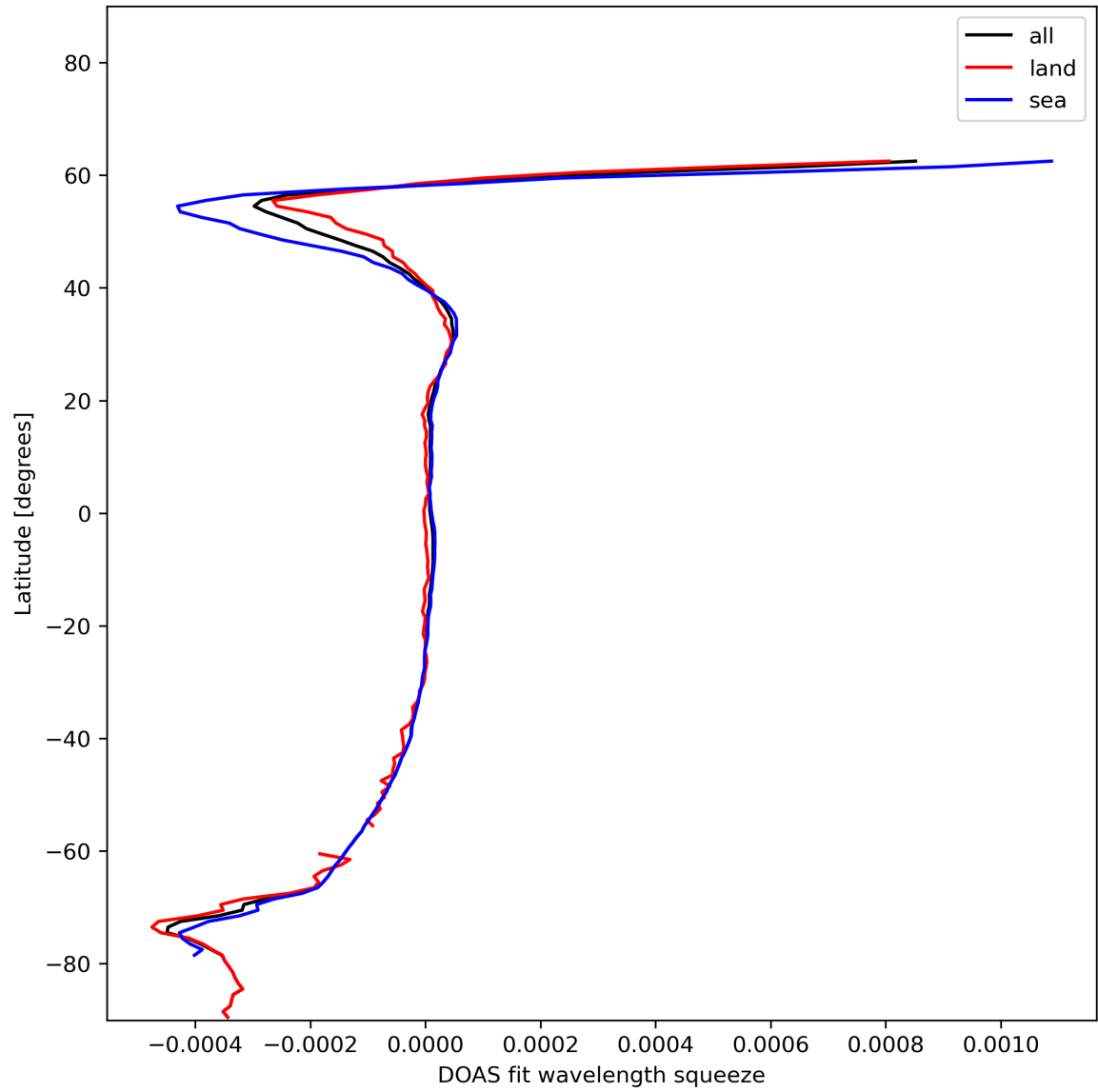
Figure 46: Zonal average of “DOAS fit wavelength squeeze” for 2024-01-02 to 2024-01-04.
