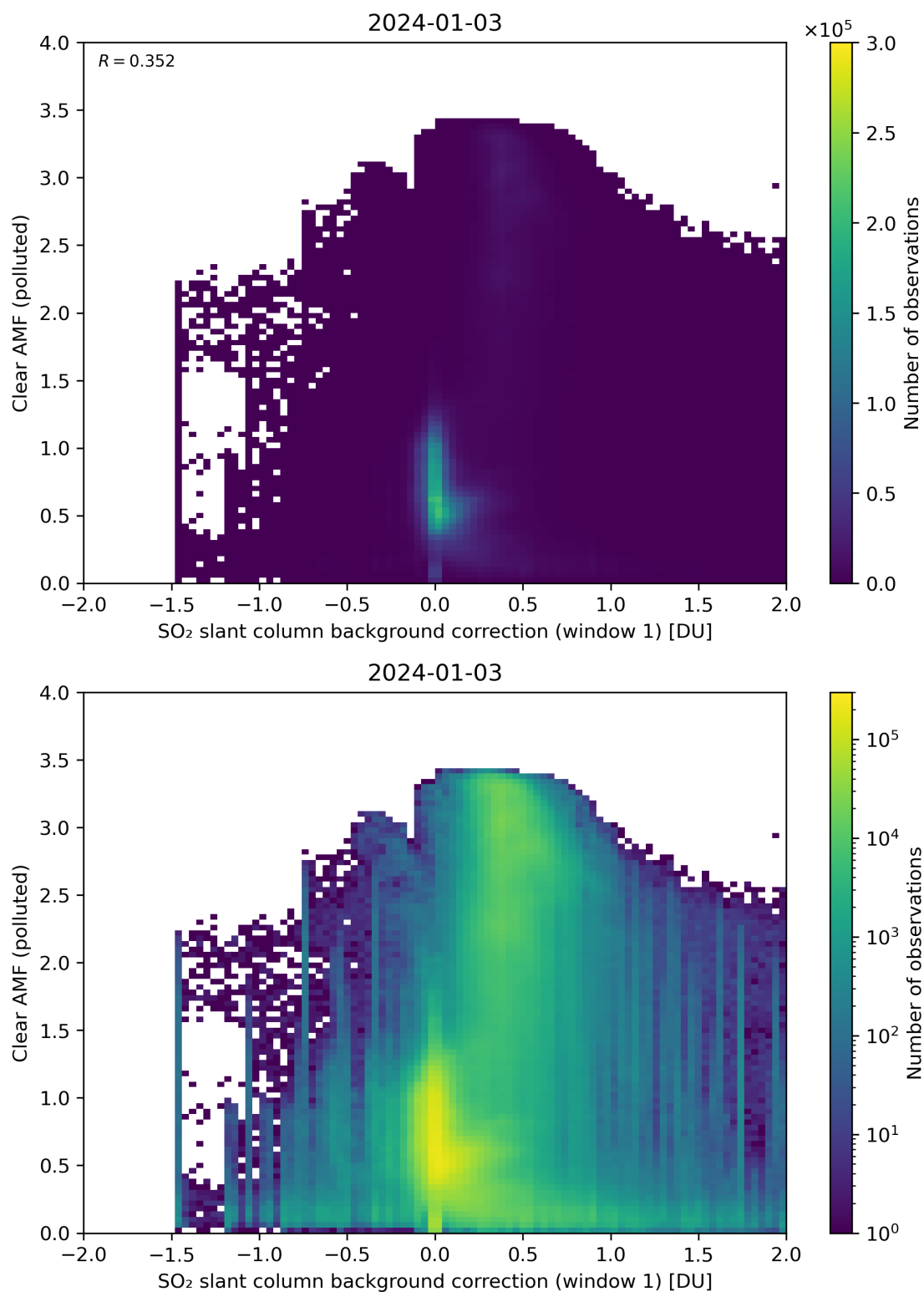
Figure 103: Scatter density plot of “SO 2 slant column background correction (window 1)” against “Clear AMF (polluted)” for 2024-01-02 to 2024-01-04.
