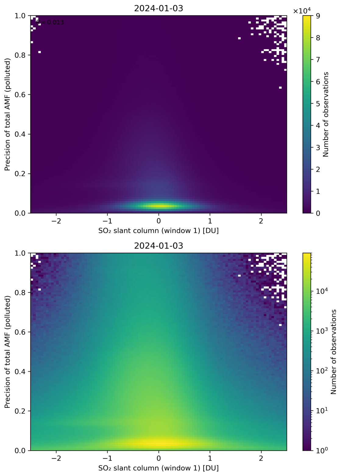
Figure 240: Scatter density plot of “SO 2 slant column (window 1)” against “Precision of total AMF (polluted)” for 2024-01-02 to 2024-01-04.
