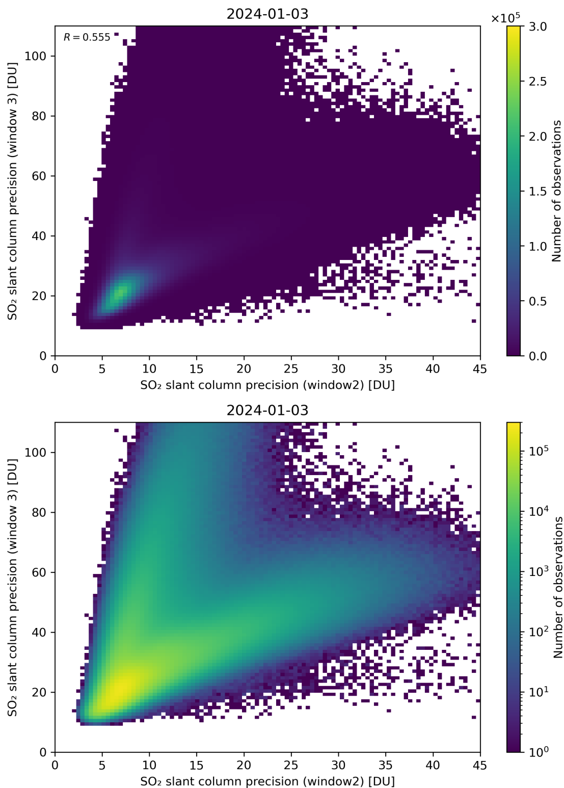
Figure 250: Scatter density plot of “SO 2 slant column precision (window2)” against “SO 2 slant column precision (window 3)” for 2024-01-02 to 2024-01-04.
