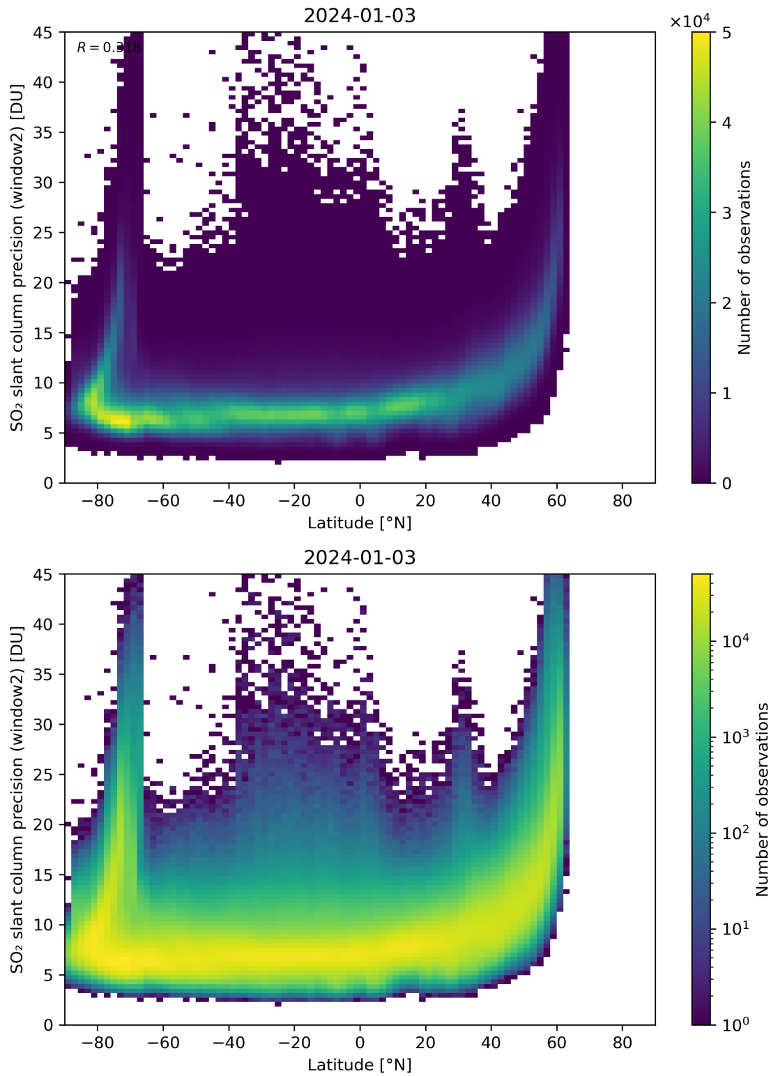
Figure 151: Scatter density plot of “Latitude” against “SO 2 slant column precision (window2)” for 2024-01-02 to 2024-01-04.
