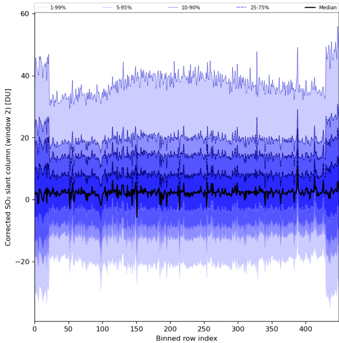
Figure 85: Along track statistics of “Corrected SO 2 slant column (window 2)” for 2024-01-02 to 2024-01-04
