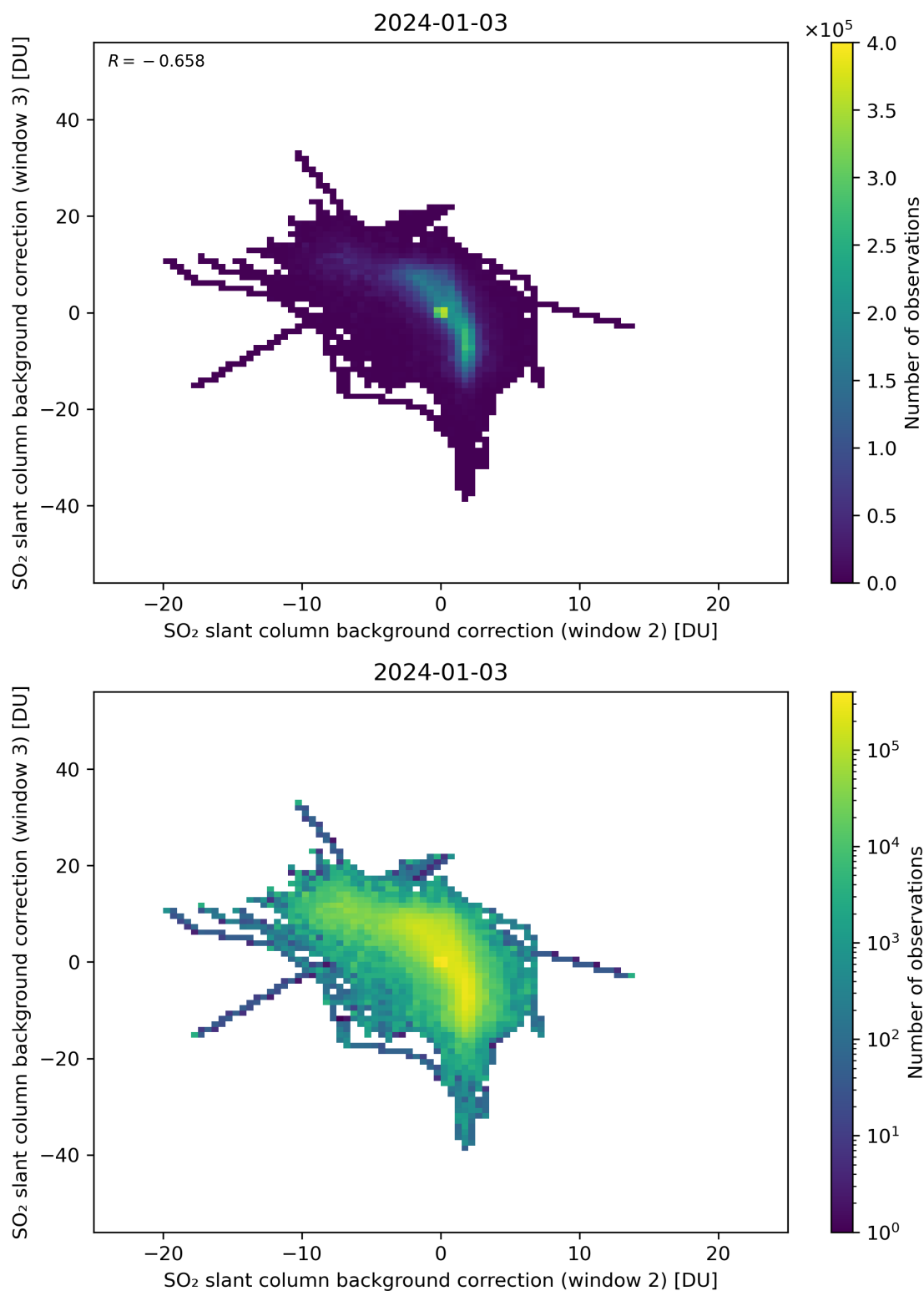
Figure 111: Scatter density plot of “SO 2 slant column background correction (window 2)” against “SO 2 slant column background correction (window 3)” for 2024-01-02 to 2024-01-04.
