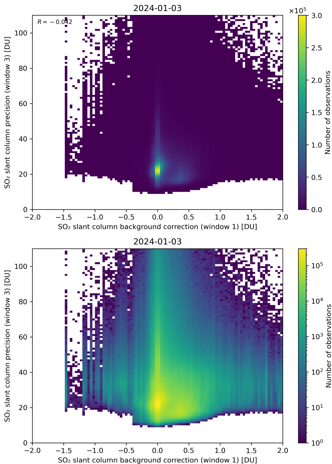
Figure 108: Scatter density plot of “SO 2 slant column background correction (window 1)” against “SO 2 slant column precision (window 3)” for 2024-01-02 to 2024-01-04.
