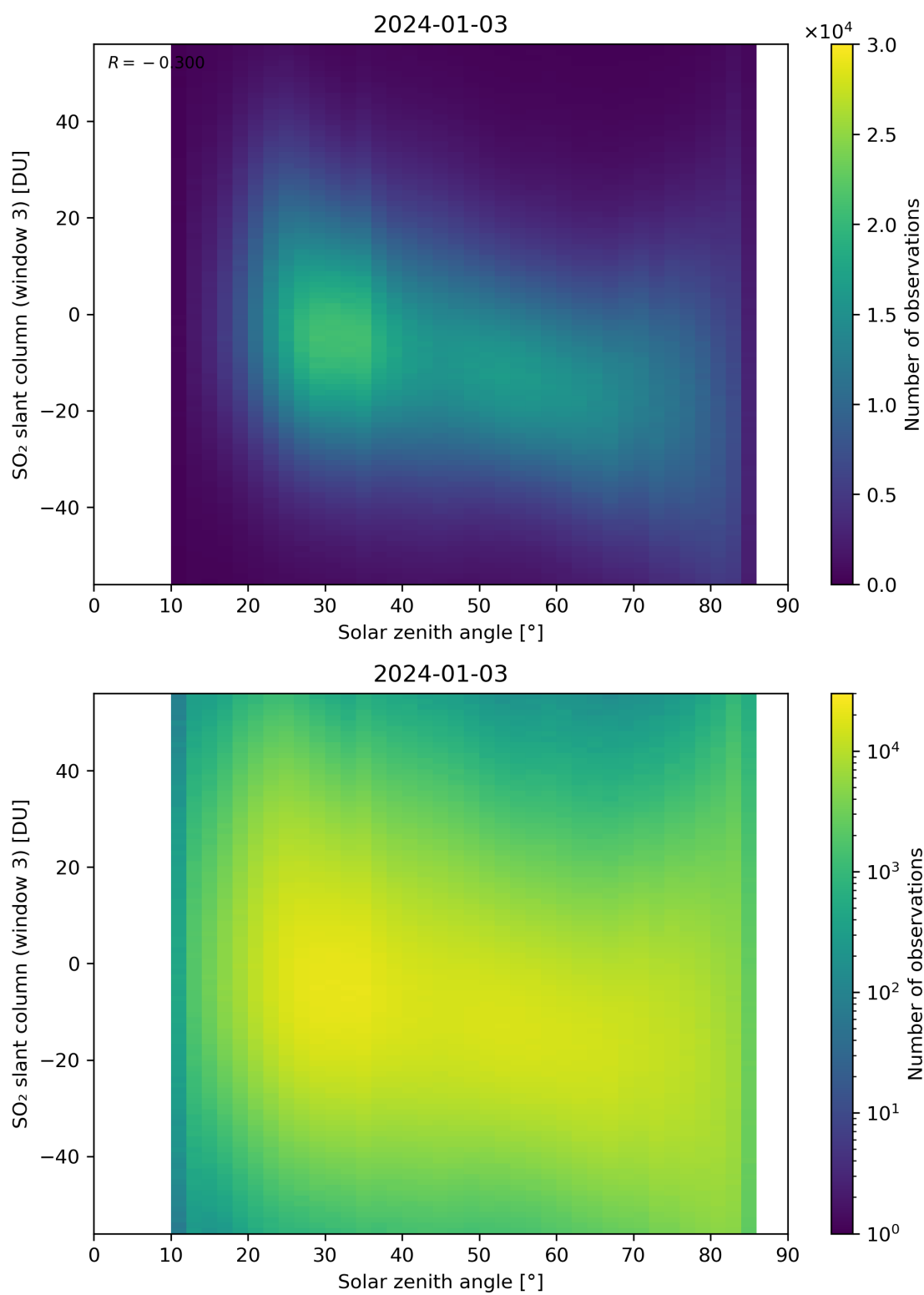
Figure 172: Scatter density plot of “Solar zenith angle” against “SO 2 slant column (window 3)” for 2024-01-02 to 2024-01-04.
