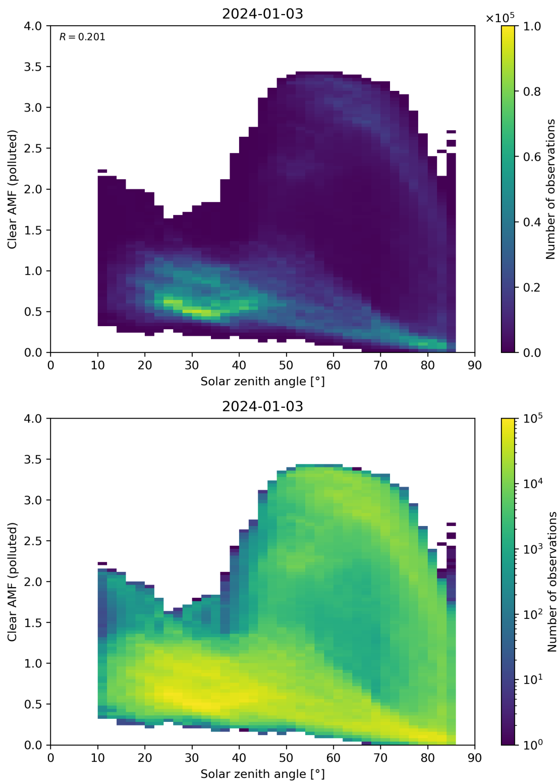
Figure 165: Scatter density plot of “Solar zenith angle” against “Clear AMF (polluted)” for 2024-01-02 to 2024-01-04.
