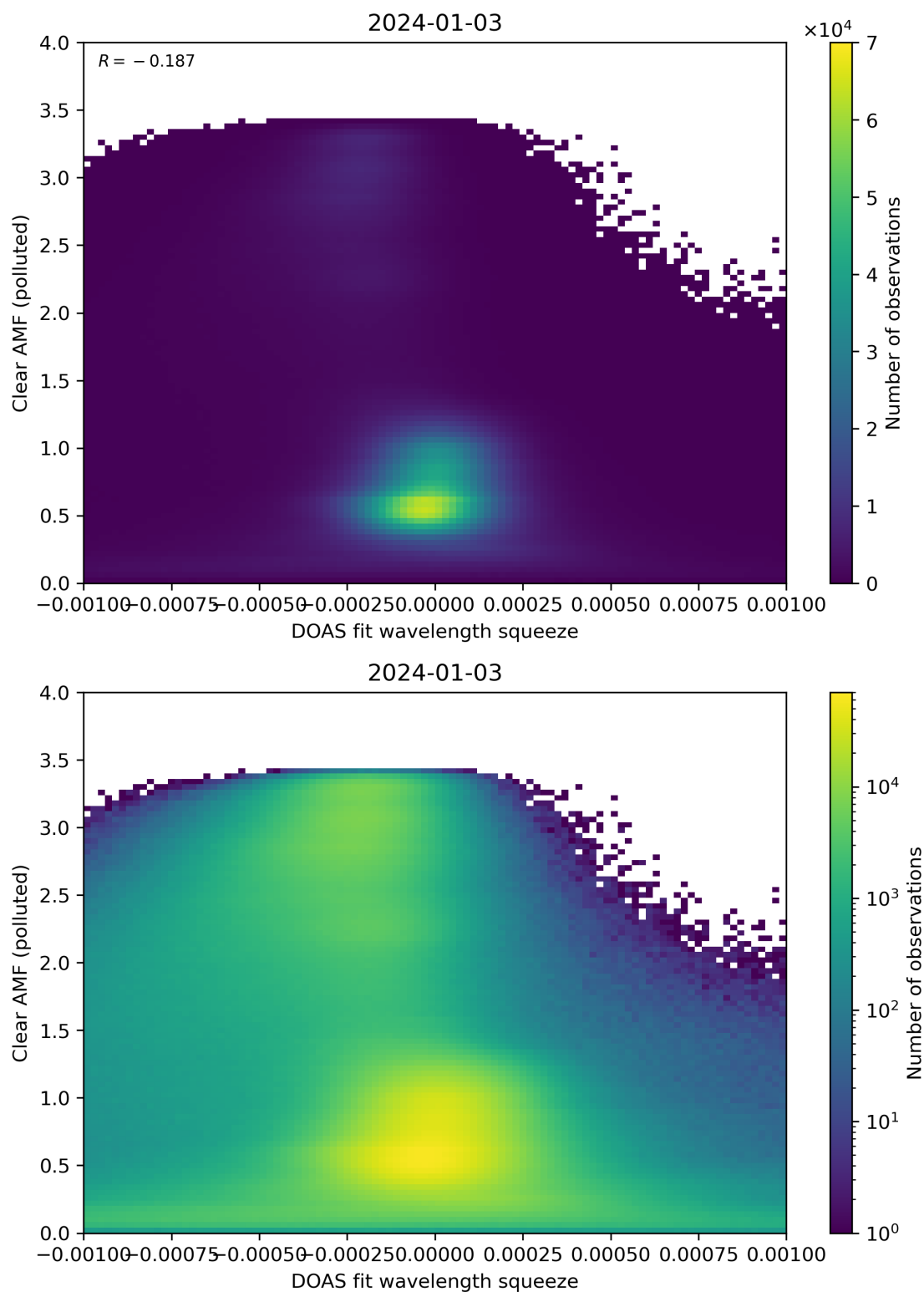
Figure 133: Scatter density plot of “DOAS fit wavelength squeeze” against “Clear AMF (polluted)” for 2024-01-02 to 2024-01-04.
