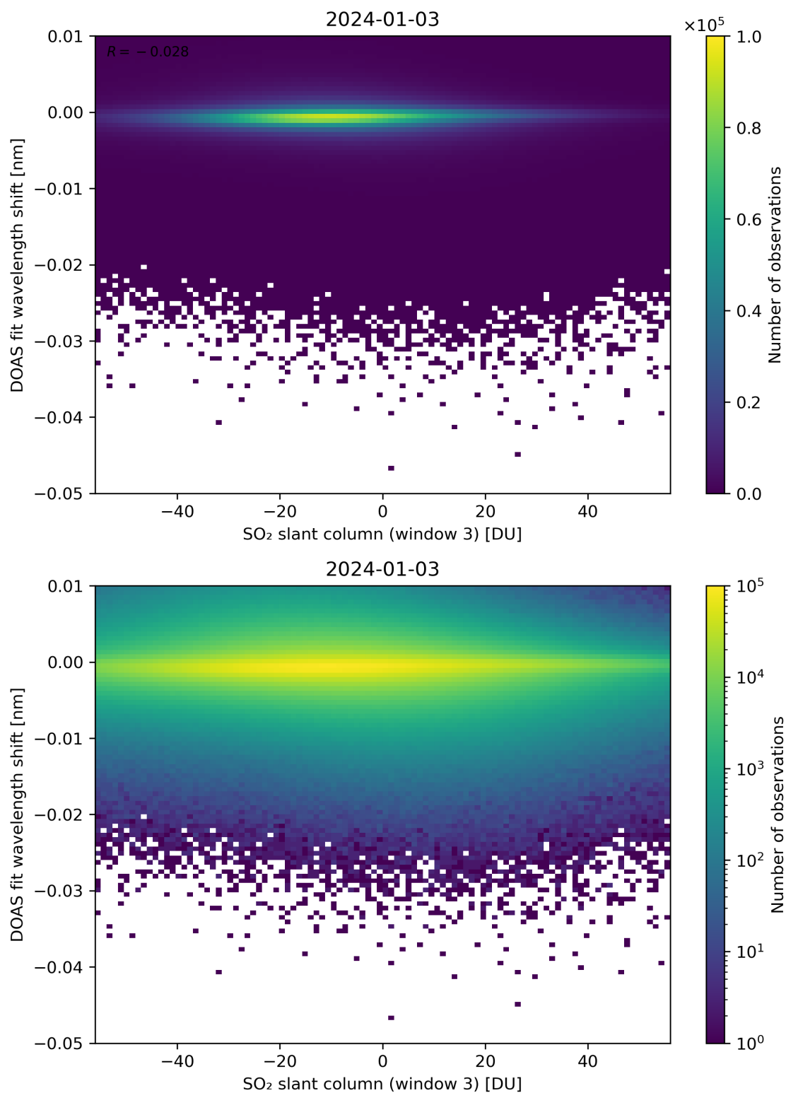
Figure 254: Scatter density plot of “SO 2 slant column (window 3)” against “DOAS fit wavelength shift” for 2024-01-02 to 2024-01-04.
