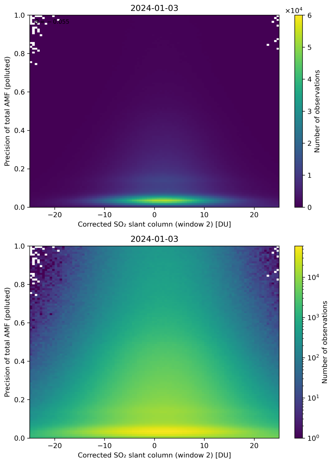
Figure 204: Scatter density plot of “Corrected SO 2 slant column (window 2)” against “Precision of total AMF (polluted)” for 2024-01-02 to 2024-01-04.
