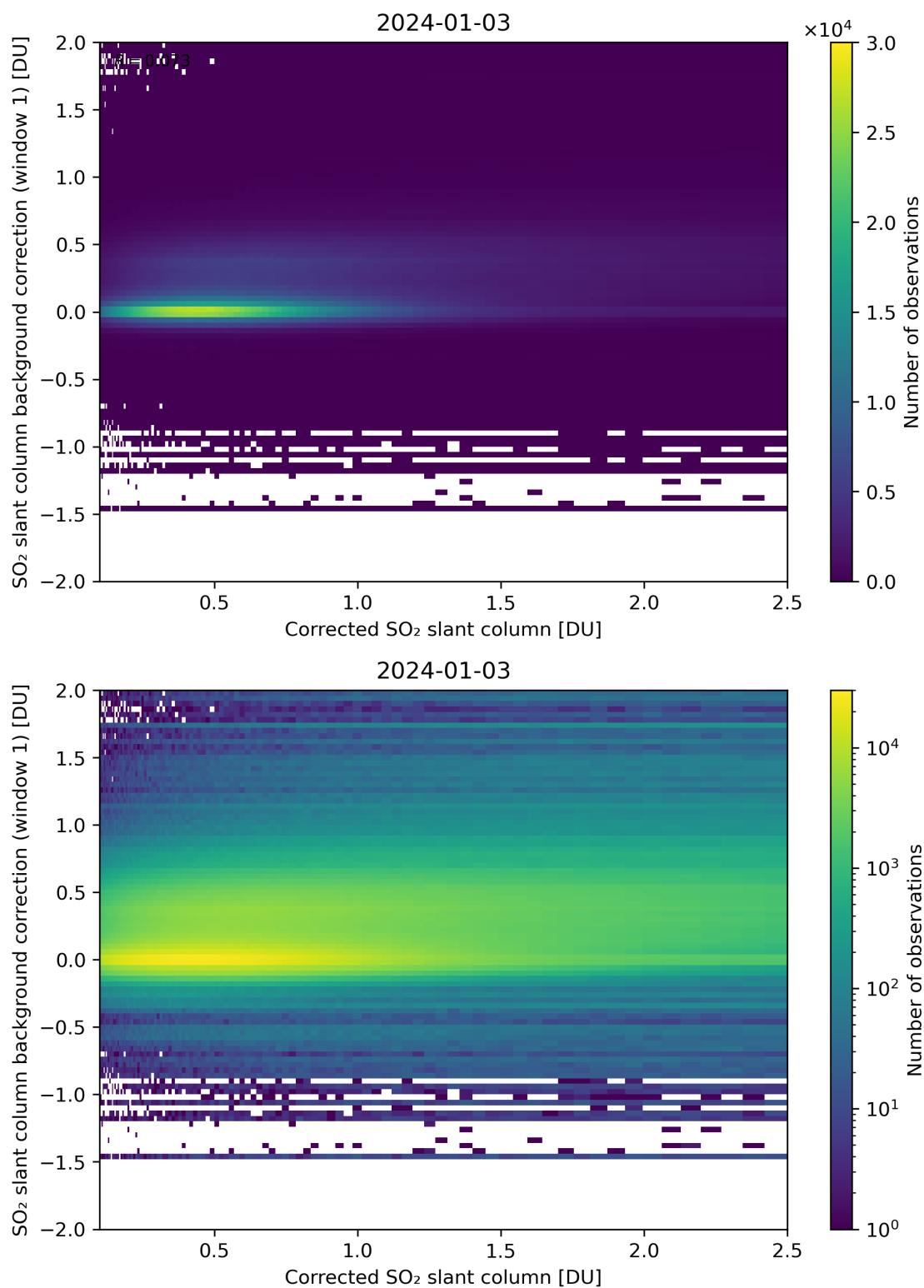
Figure 178: Scatter density plot of “Corrected SO 2 slant column” against “SO 2 slant column background correction (window 1)” for 2024-01-02 to 2024-01-04.
