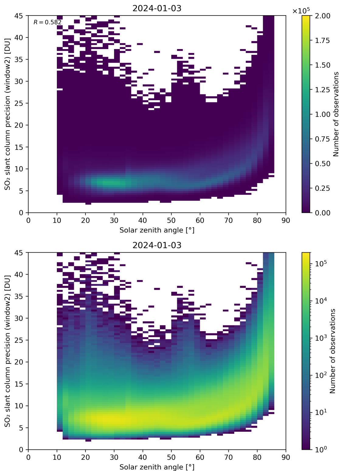
Figure 171: Scatter density plot of “Solar zenith angle” against “SO 2 slant column precision (window2)” for 2024-01-02 to 2024-01-04.
