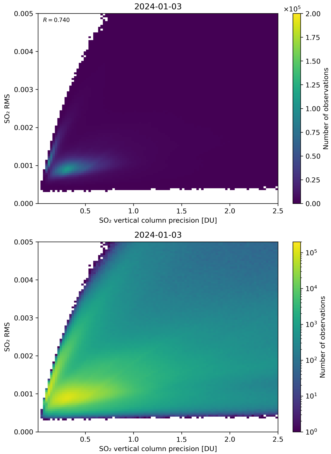
Figure 284: Scatter density plot of “SO 2 vertical column precision” against “SO 2 RMS” for 2024-01-02 to 2024-01-04.
