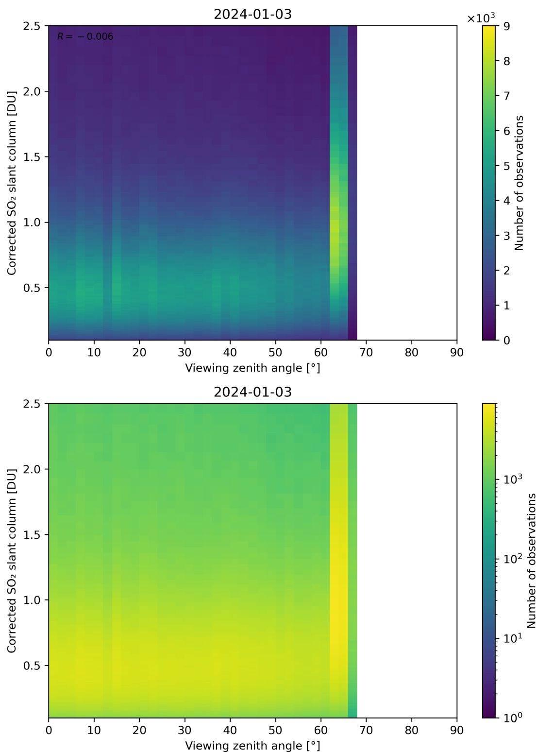
Figure 317: Scatter density plot of “Viewing zenith angle” against “Corrected SO 2 slant column” for 2024-01-02 to 2024-01-04.
