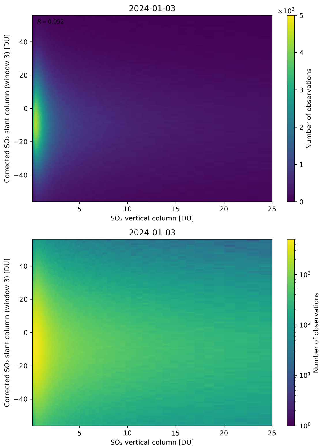
Figure 299: Scatter density plot of “SO 2 vertical column” against “Corrected SO 2 slant column (window 3)” for 2024-01-02 to 2024-01-04.
