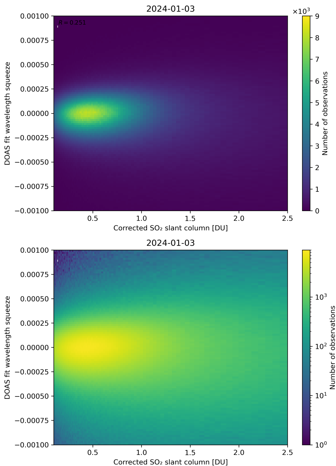
Figure 182: Scatter density plot of “Corrected SO 2 slant column” against “DOAS fit wavelength squeeze” for 2024-01-02 to 2024-01-04.
