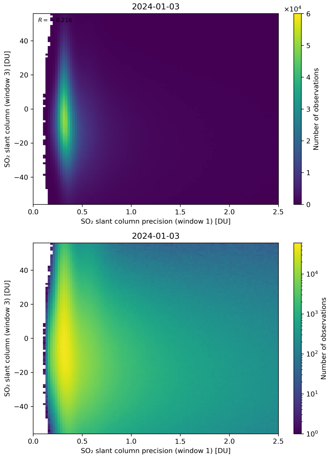
Figure 228: Scatter density plot of “SO 2 slant column precision (window 1)” against “SO 2 slant column (window 3)” for 2024-01-02 to 2024-01-04.
