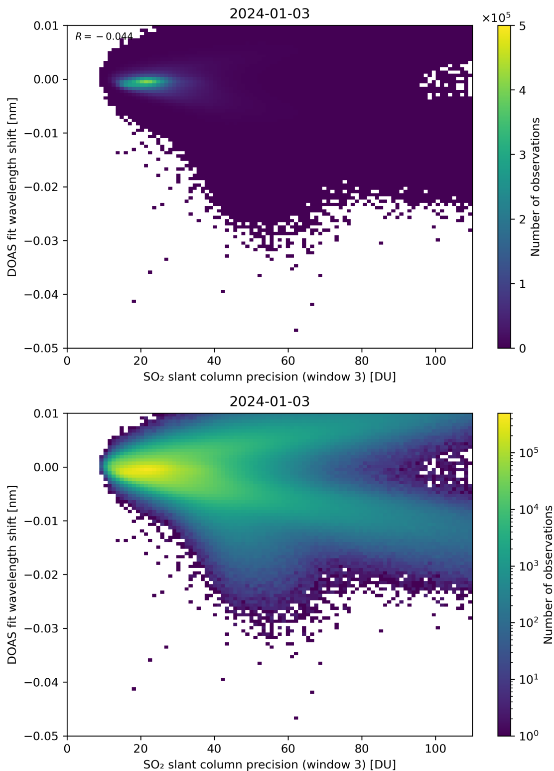
Figure 258: Scatter density plot of “SO 2 slant column precision (window 3)” against “DOAS fit wavelength shift” for 2024-01-02 to 2024-01-04.
