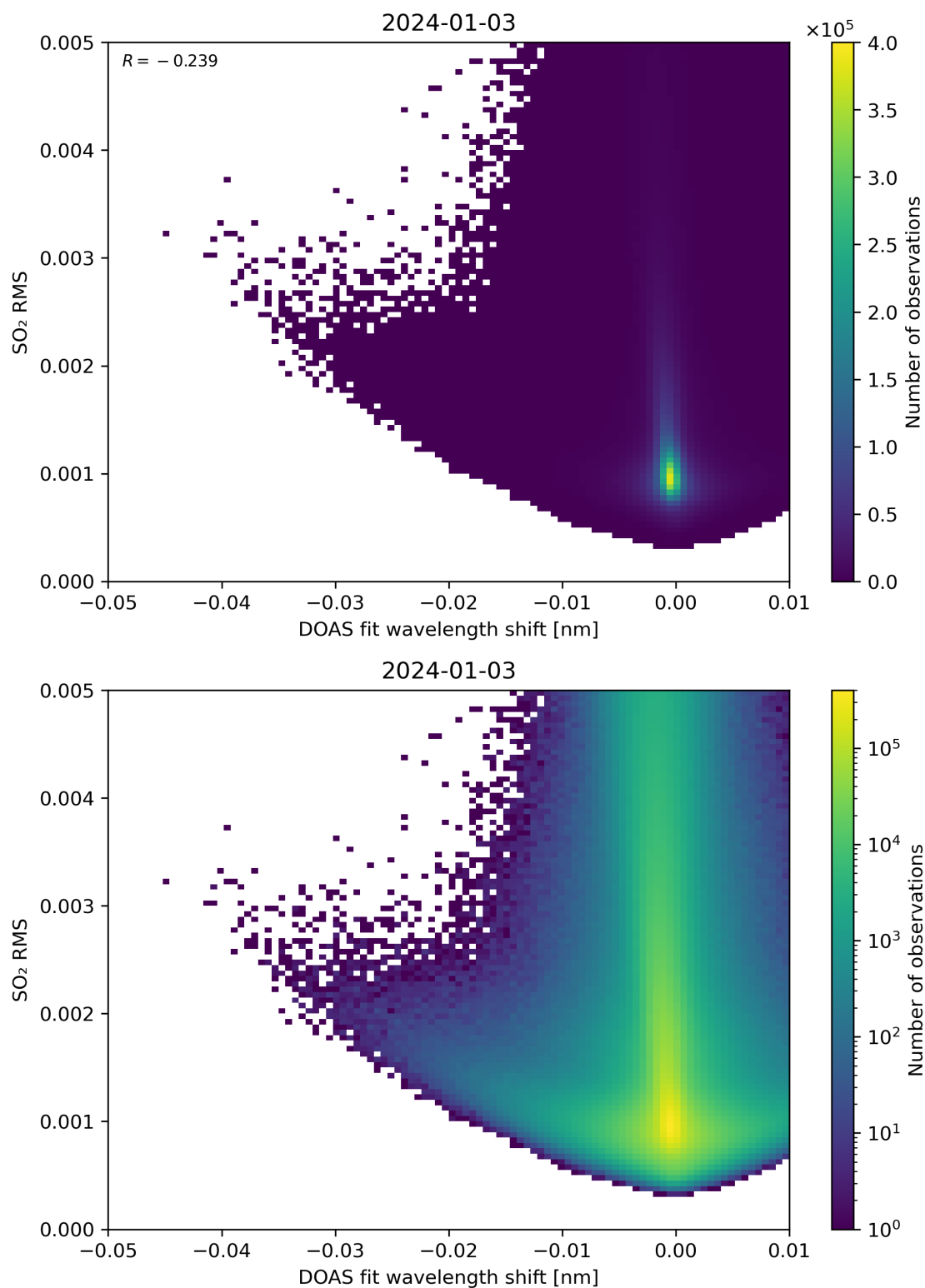
Figure 128: Scatter density plot of “DOAS fit wavelength shift” against “SO 2 RMS” for 2024-01-02 to 2024-01-04.
