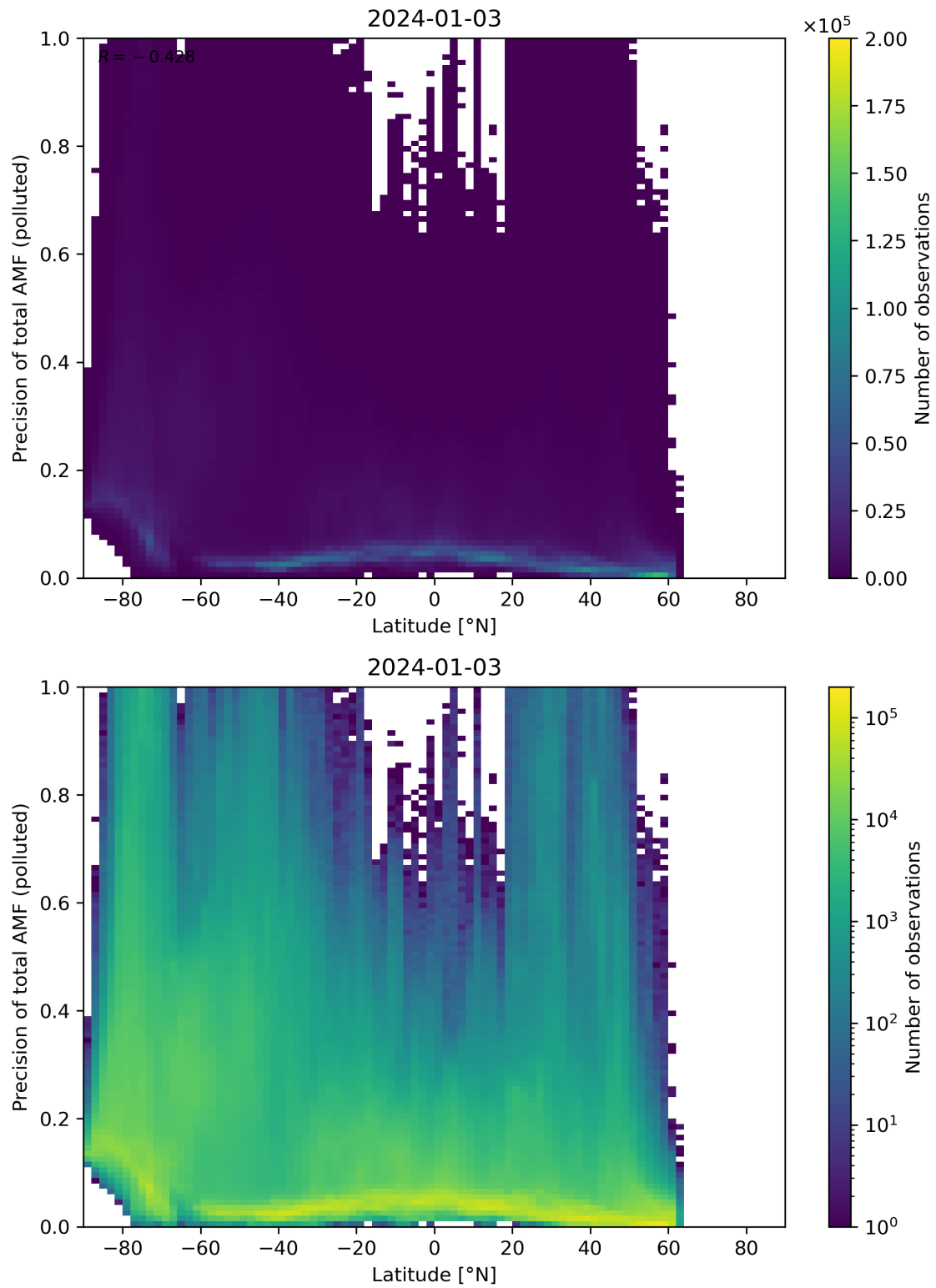
Figure 155: Scatter density plot of “Latitude” against “Precision of total AMF (polluted)” for 2024-01-02 to 2024-01-04.
