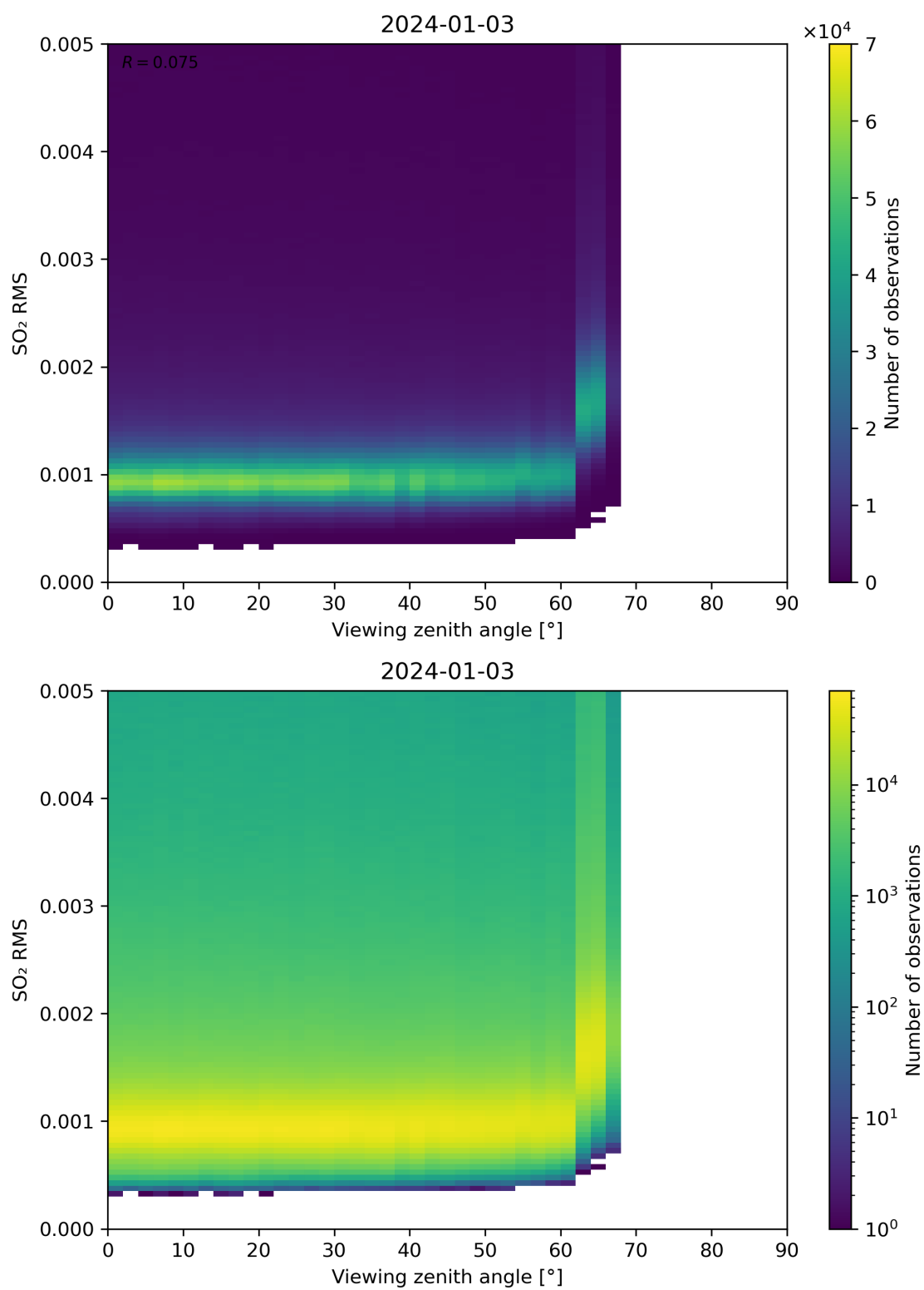
Figure 313: Scatter density plot of “Viewing zenith angle” against “SO 2 RMS” for 2024-01-02 to 2024-01-04.
