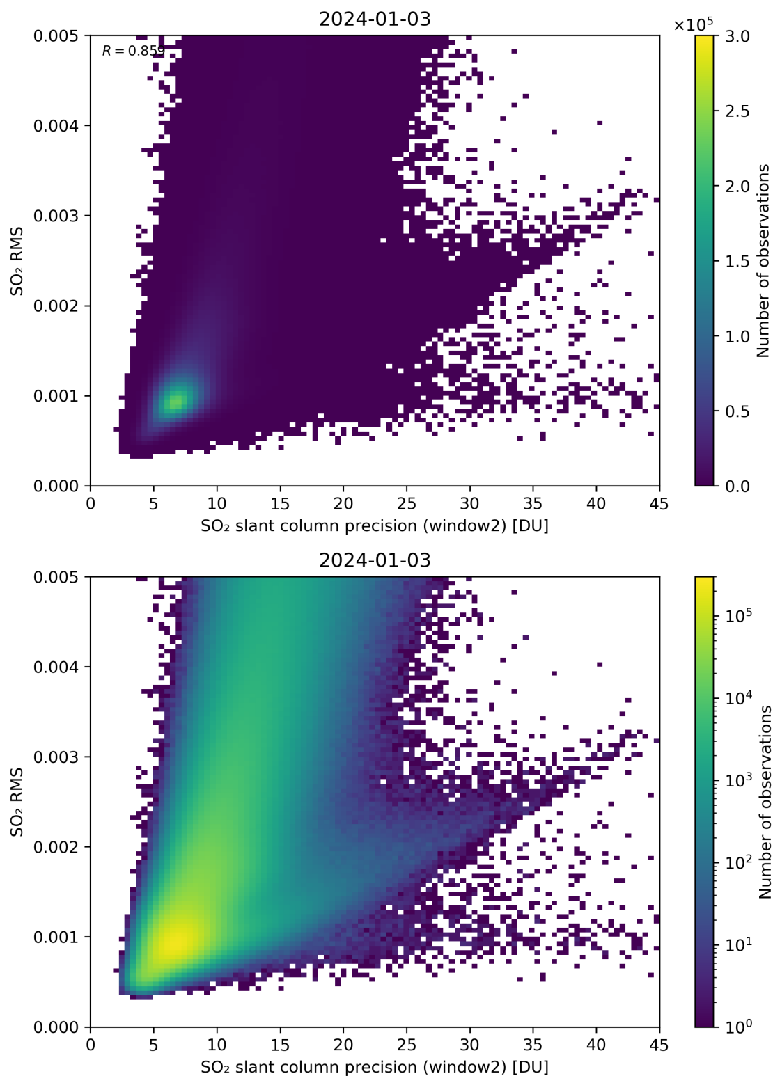
Figure 245: Scatter density plot of “SO 2 slant column precision (window2)” against “SO 2 RMS” for 2024-01-02 to 2024-01-04.
