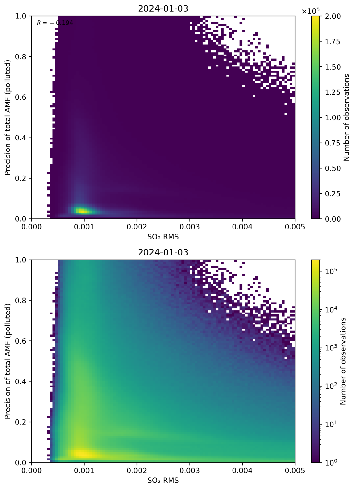
Figure 138: Scatter density plot of “SO 2 RMS” against “Precision of total AMF (polluted)” for 2024-01-02 to 2024-01-04.
