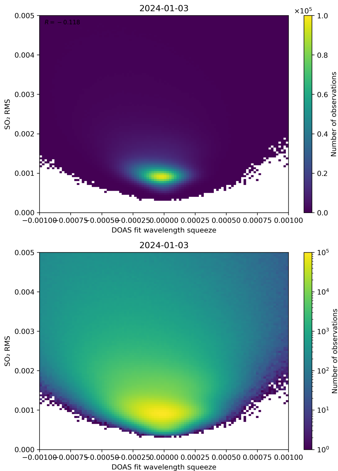
Figure 132: Scatter density plot of “DOAS fit wavelength squeeze” against “SO 2 RMS” for 2024-01-02 to 2024-01-04.
