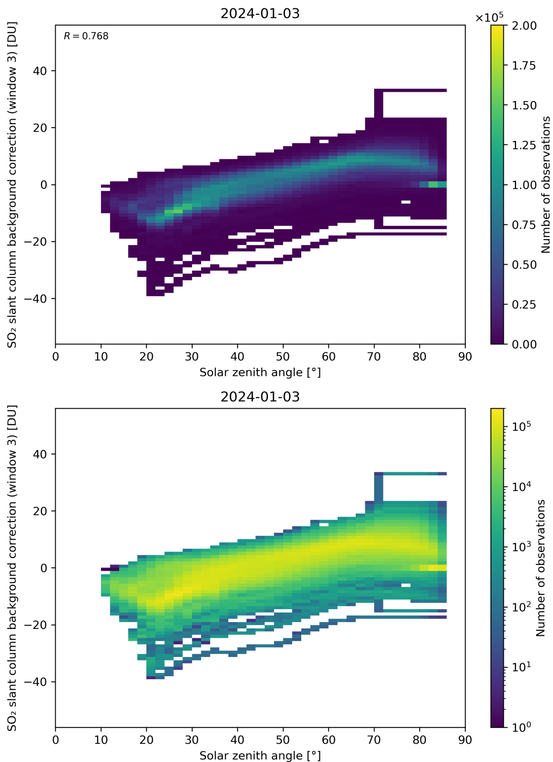
Figure 160: Scatter density plot of “Solar zenith angle” against “SO 2 slant column background correction (window 3)” for 2024-01-02 to 2024-01-04.
