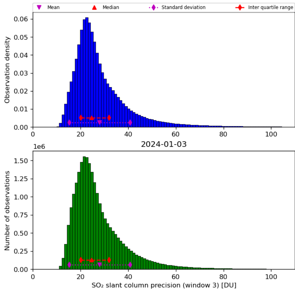
Figure 65: Histogram of “SO 2 slant column precision (window 3)” for 2024-01-02 to 2024-01-04
