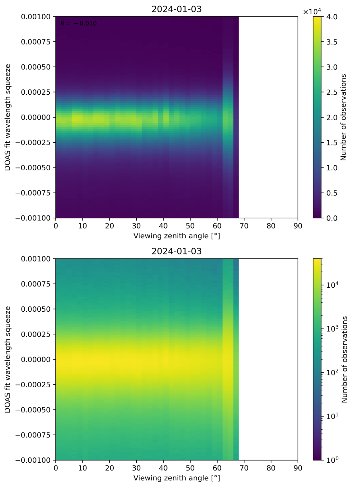
Figure 312: Scatter density plot of “Viewing zenith angle” against “DOAS fit wavelength squeeze” for 2024-01-02 to 2024-01-04.
