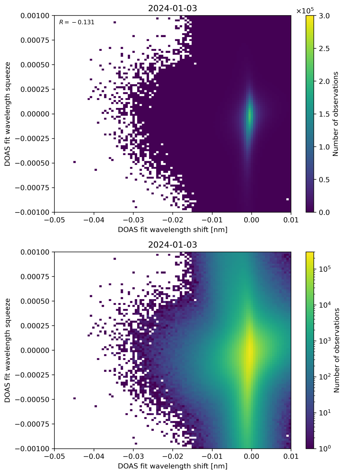
Figure 127: Scatter density plot of “DOAS fit wavelength shift” against “DOAS fit wavelength squeeze” for 2024-01-02 to 2024-01-04.
