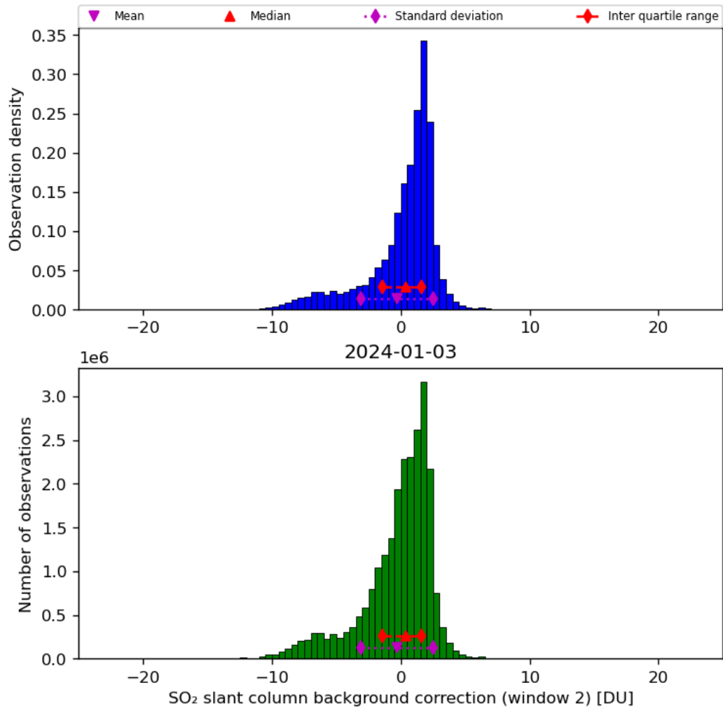
Figure 63: Histogram of “SO 2 slant column background correction (window 2)” for 2024-01-02 to 2024-01-04
