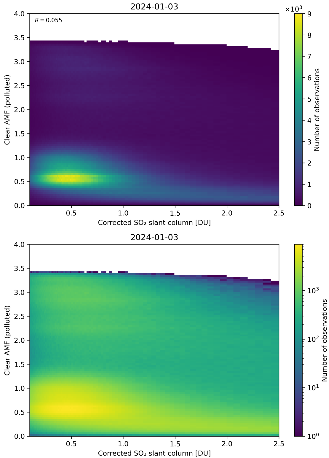
Figure 184: Scatter density plot of “Corrected SO 2 slant column” against “Clear AMF (polluted)” for 2024-01-02 to 2024-01-04.
