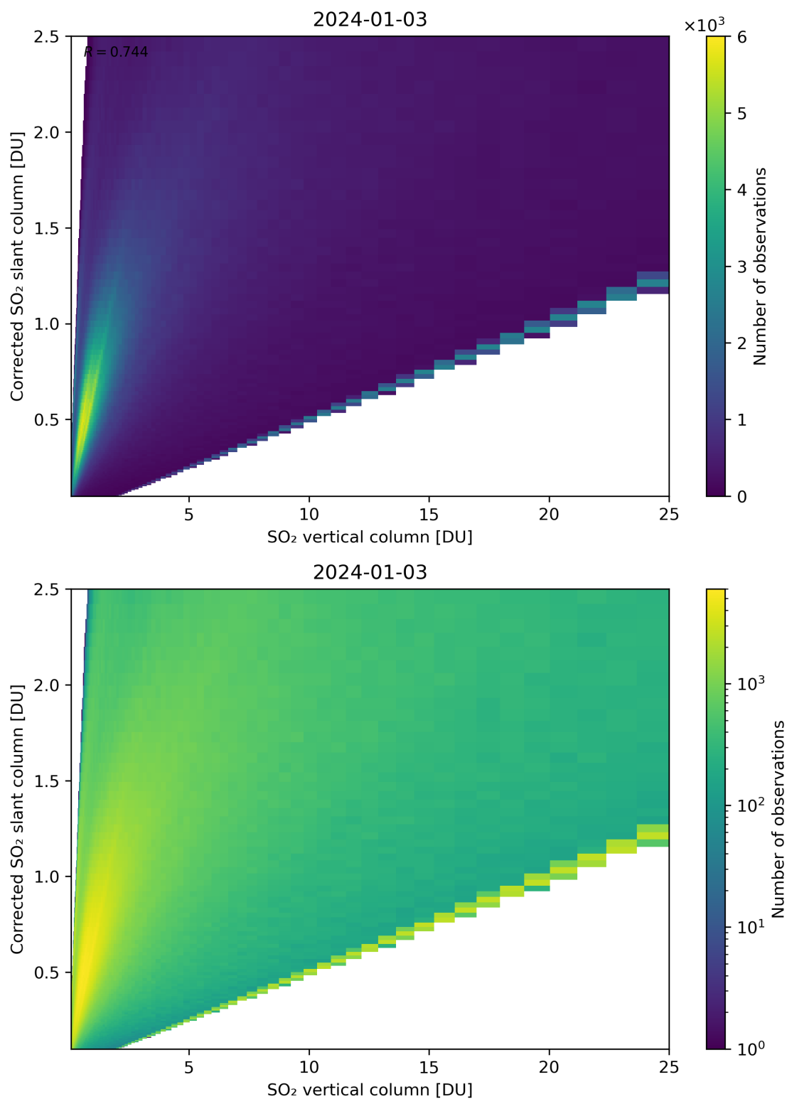
Figure 297: Scatter density plot of “SO 2 vertical column” against “Corrected SO 2 slant column” for 2024-01-02 to 2024-01-04.
