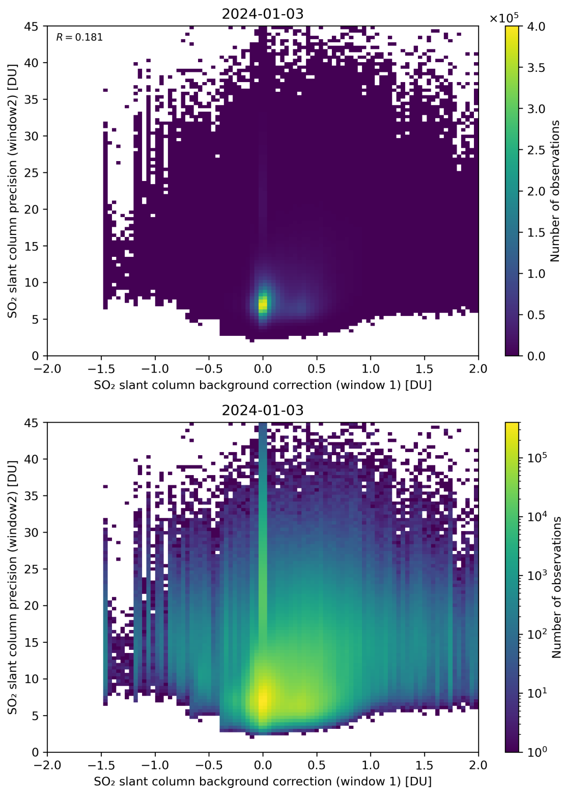
Figure 106: Scatter density plot of “SO 2 slant column background correction (window 1)” against “SO 2 slant column precision (window2)” for 2024-01-02 to 2024-01-04.
