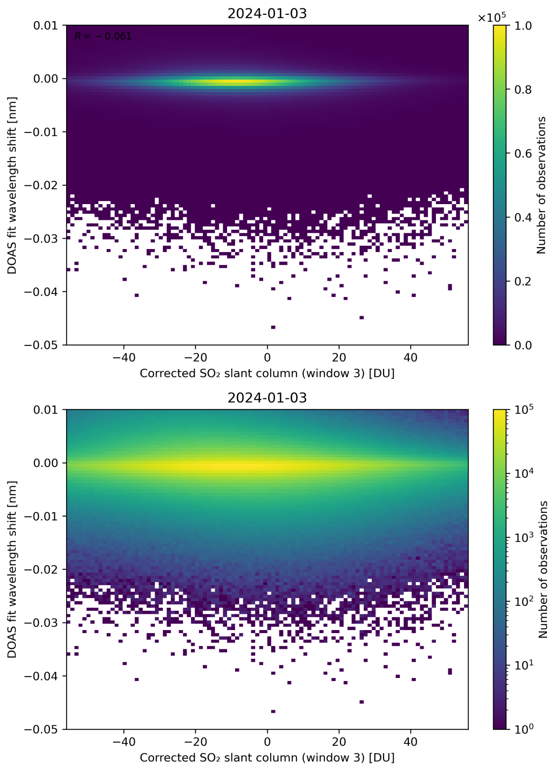
Figure 206: Scatter density plot of “Corrected SO 2 slant column (window 3)” against “DOAS fit wavelength shift” for 2024-01-02 to 2024-01-04.
