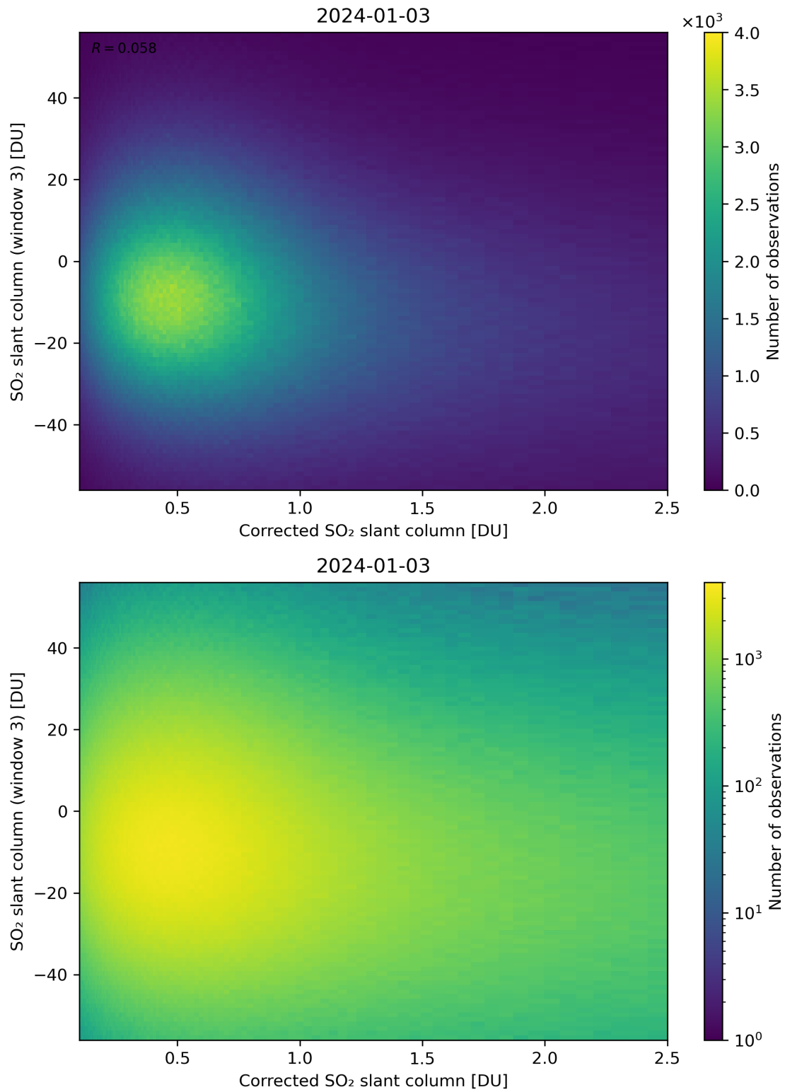
Figure 190: Scatter density plot of “Corrected SO 2 slant column” against “SO 2 slant column (window 3)” for 2024-01-02 to 2024-01-04.
