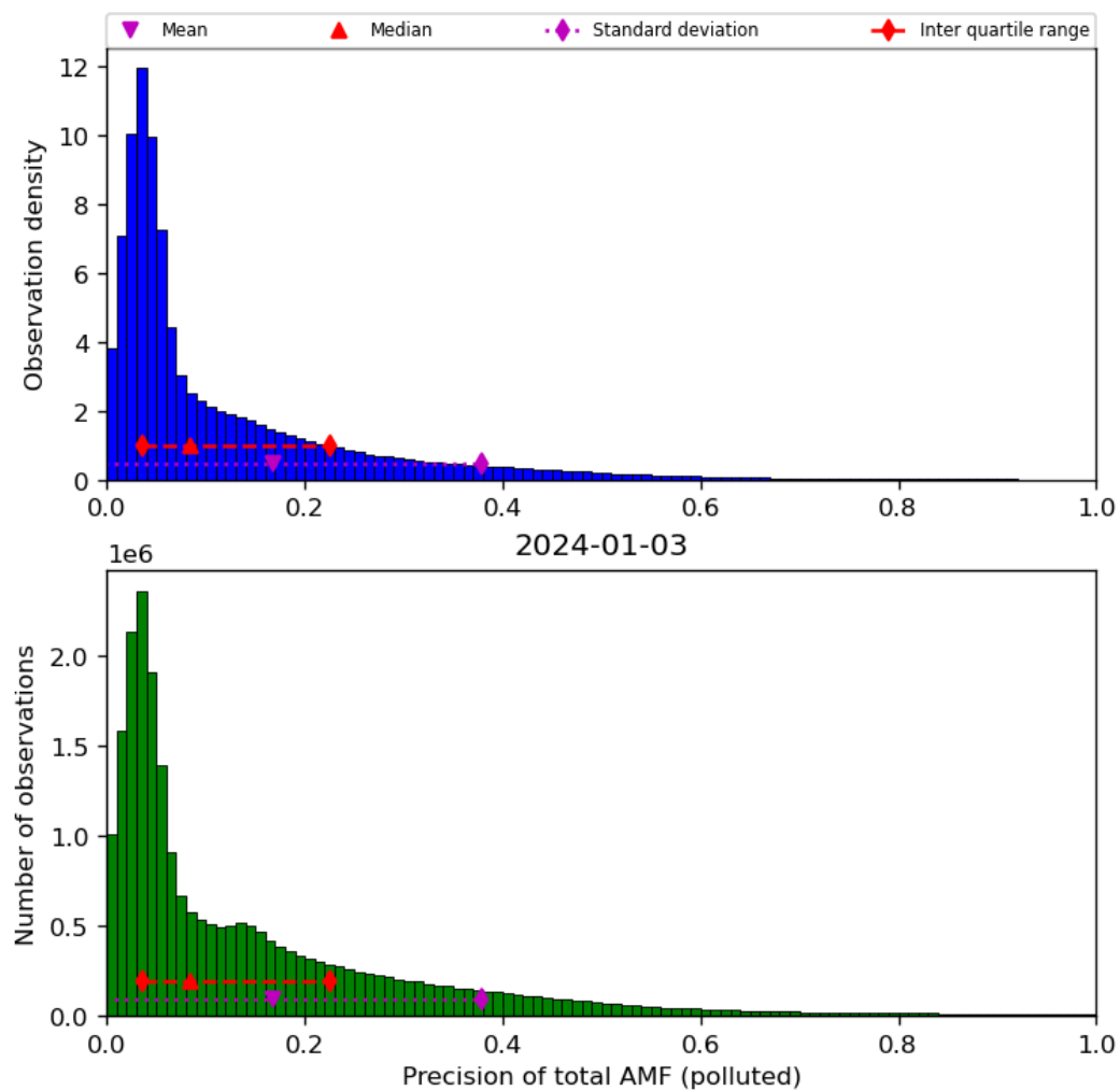
Figure 72: Histogram of “Precision of total AMF (polluted)” for 2024-01-02 to 2024-01-04
