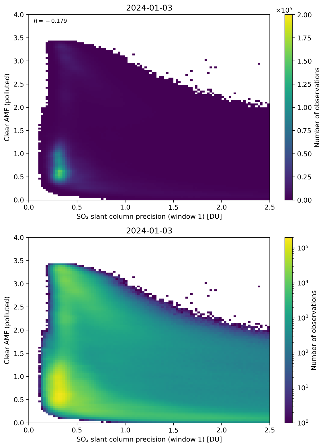
Figure 224: Scatter density plot of “SO 2 slant column precision (window 1)” against “Clear AMF (polluted)” for 2024-01-02 to 2024-01-04.
