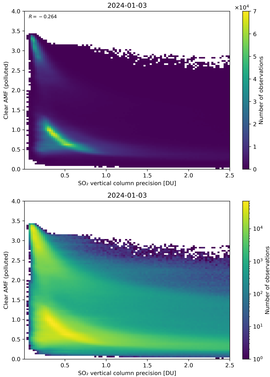
Figure 285: Scatter density plot of “SO 2 vertical column precision” against “Clear AMF (polluted)” for 2024-01-02 to 2024-01-04.
