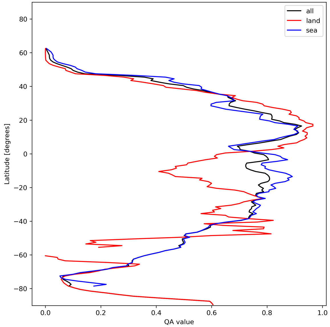
Figure 29: Zonal average of “QA value” for 2024-01-02 to 2024-01-04.
