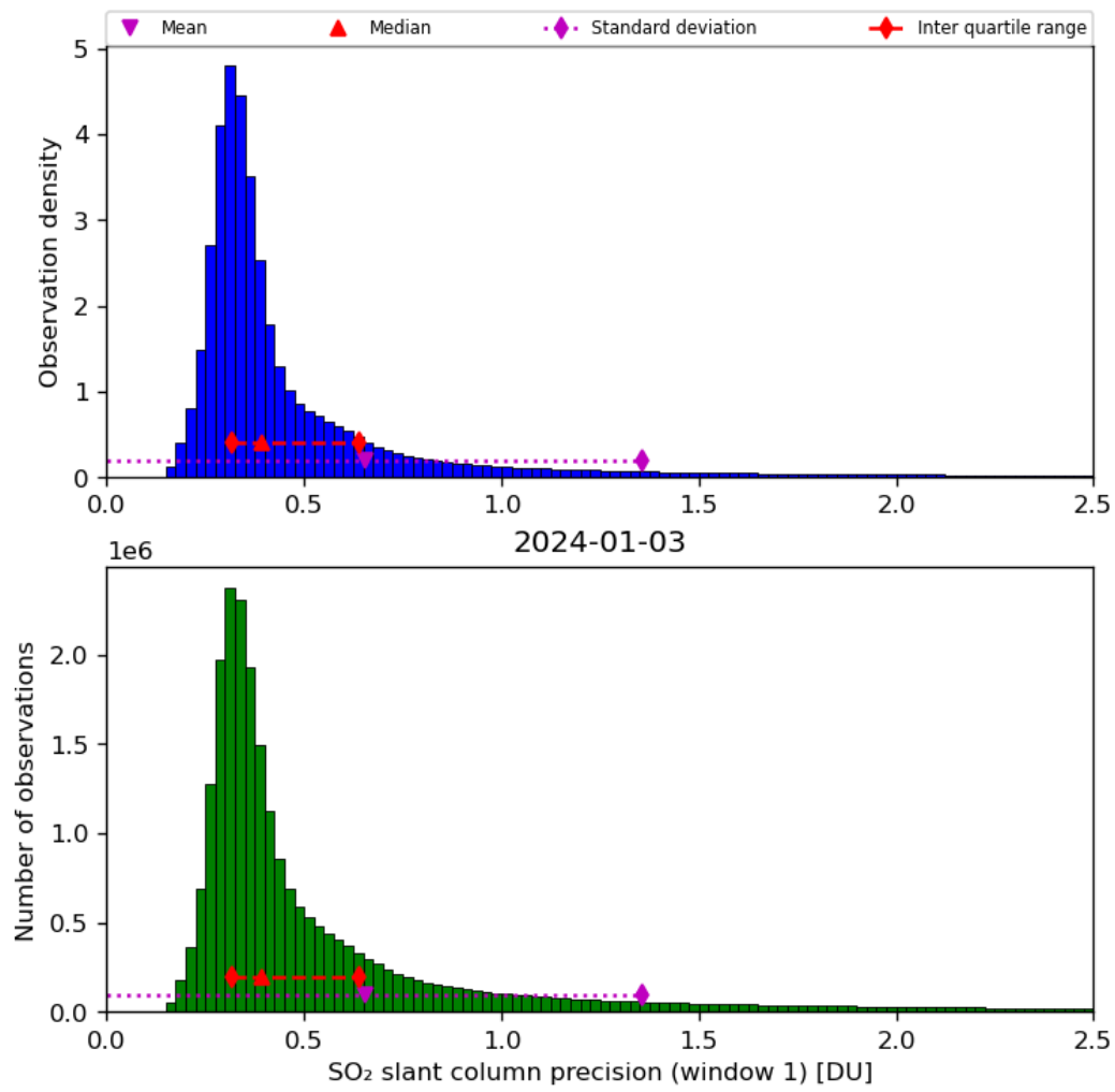
Figure 57: Histogram of “SO 2 slant column precision (window 1)” for 2024-01-02 to 2024-01-04
