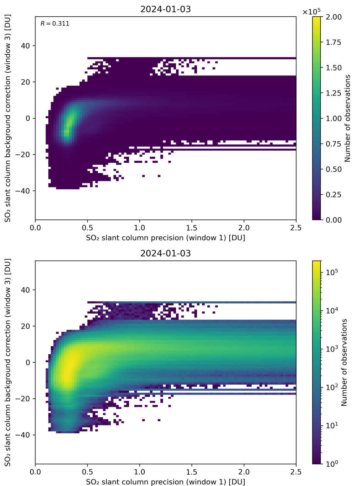
Figure 220: Scatter density plot of “SO 2 slant column precision (window 1)” against “SO 2 slant column background correction (window 3)” for 2024-01-02 to 2024-01-04.
