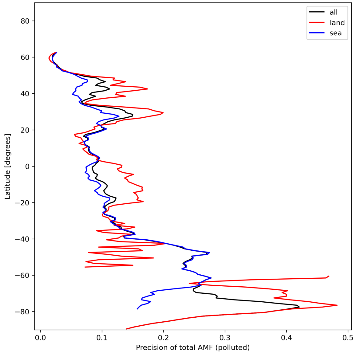
Figure 49: Zonal average of “Precision of total AMF (polluted)” for 2024-01-02 to 2024-01-04.
