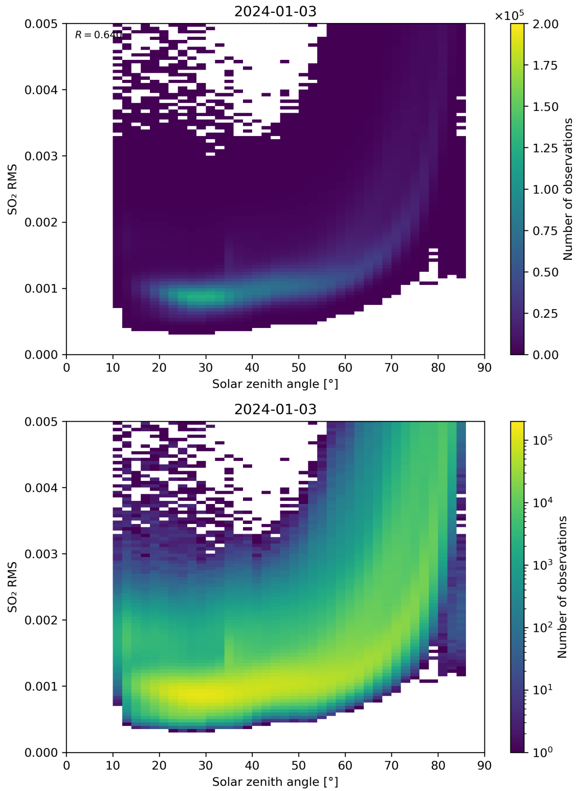
Figure 163: Scatter density plot of “Solar zenith angle” against “SO 2 RMS” for 2024-01-02 to 2024-01-04.
