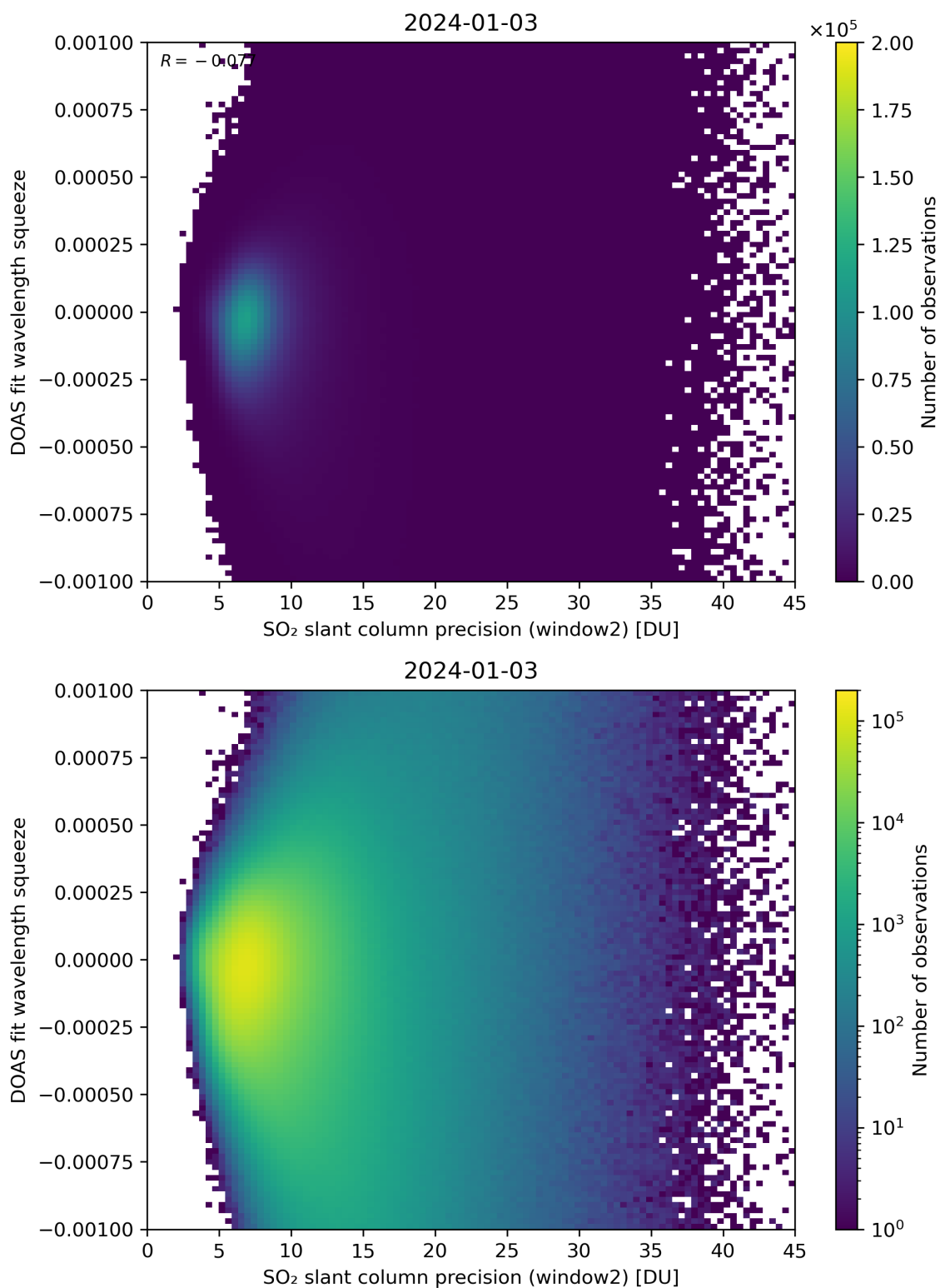
Figure 244: Scatter density plot of “SO 2 slant column precision (window2)” against “DOAS fit wavelength squeeze” for 2024-01-02 to 2024-01-04.
