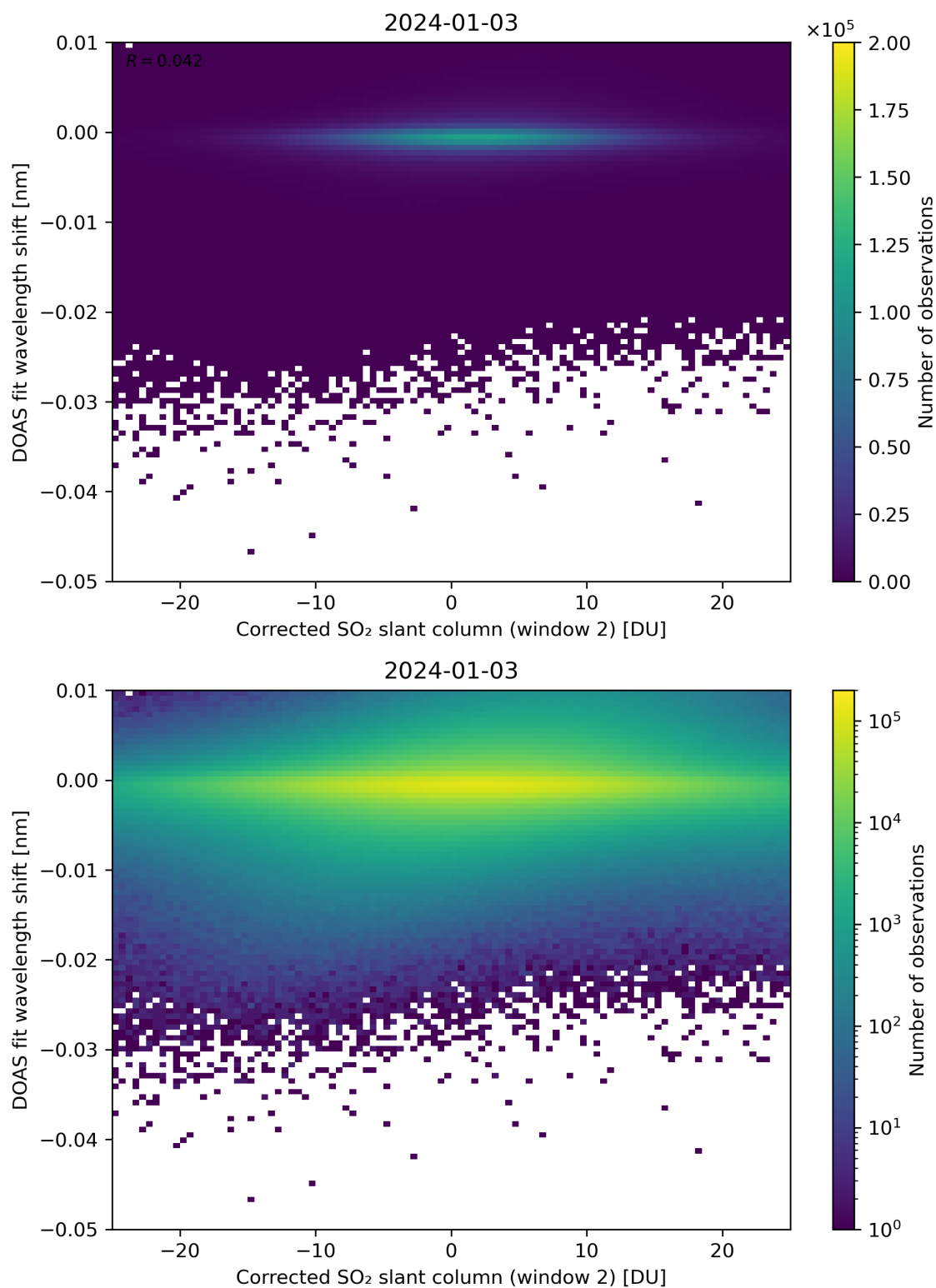
Figure 196: Scatter density plot of “Corrected SO 2 slant column (window 2)” against “DOAS fit wavelength shift” for 2024-01-02 to 2024-01-04.
