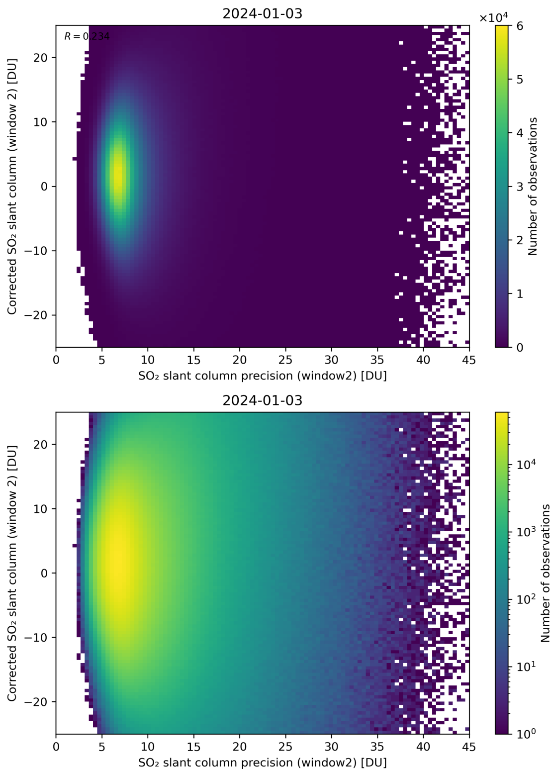
Figure 247: Scatter density plot of “SO 2 slant column precision (window2)” against “Corrected SO 2 slant column (window 2)” for 2024-01-02 to 2024-01-04.
