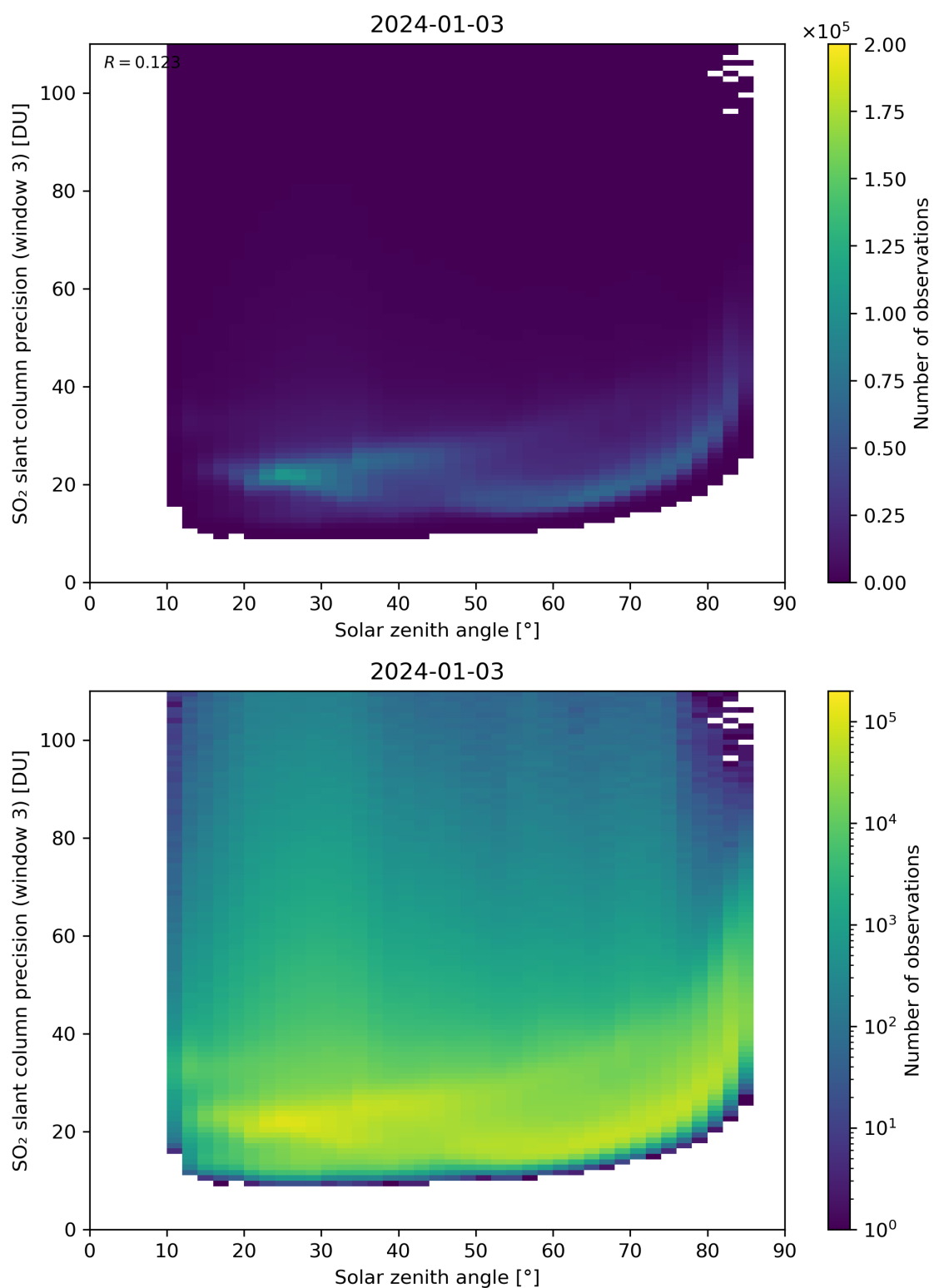
Figure 173: Scatter density plot of “Solar zenith angle” against “SO 2 slant column precision (window 3)” for 2024-01-02 to 2024-01-04.
