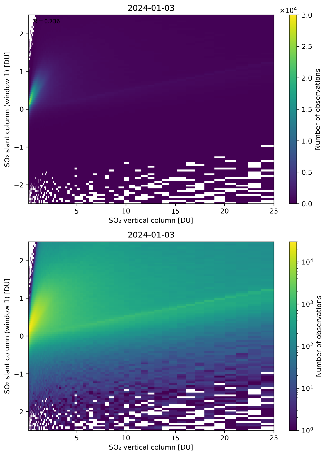
Figure 300: Scatter density plot of “SO 2 vertical column” against “SO 2 slant column (window 1)” for 2024-01-02 to 2024-01-04.
