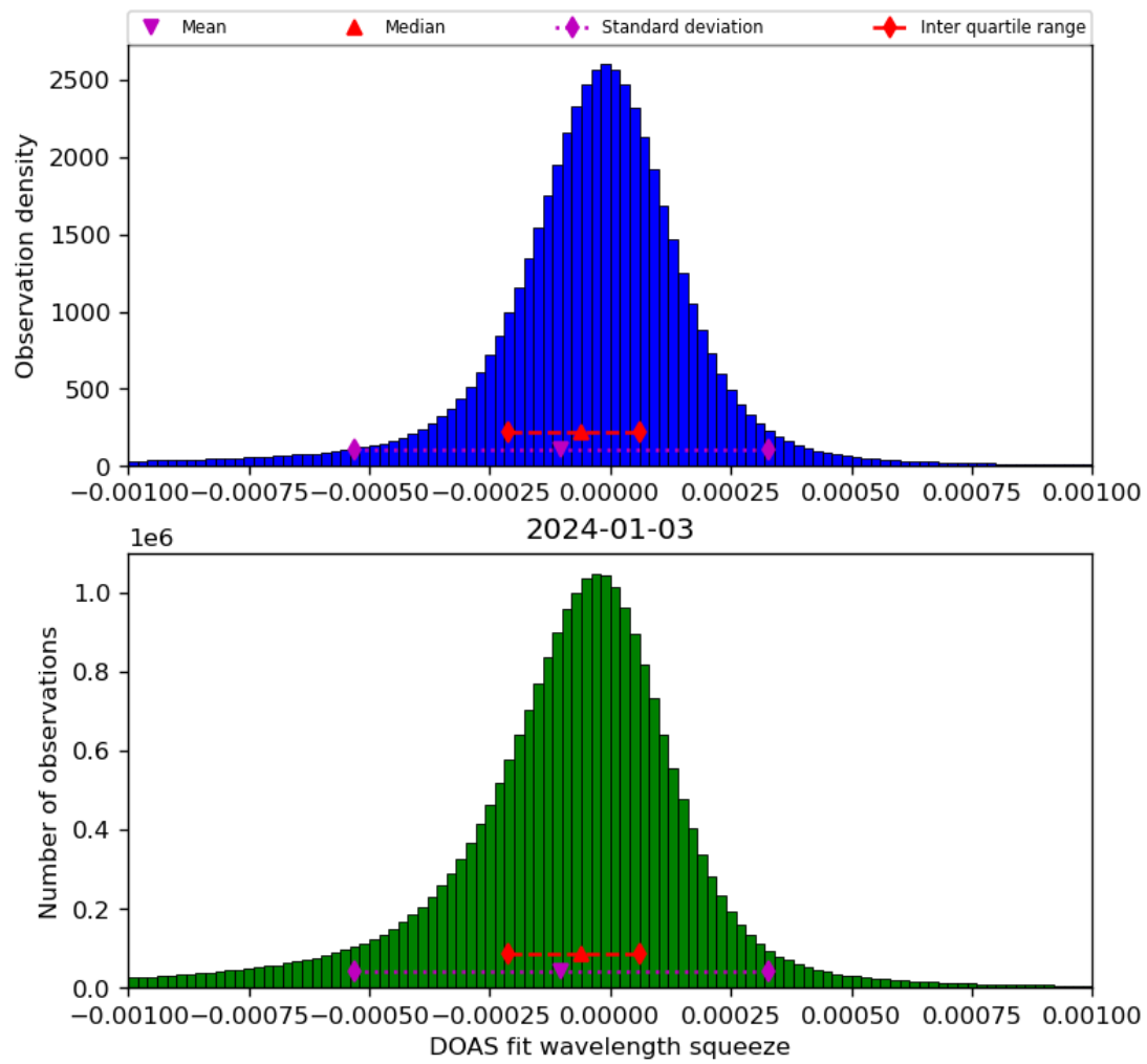
Figure 69: Histogram of “DOAS fit wavelength squeeze” for 2024-01-02 to 2024-01-04
