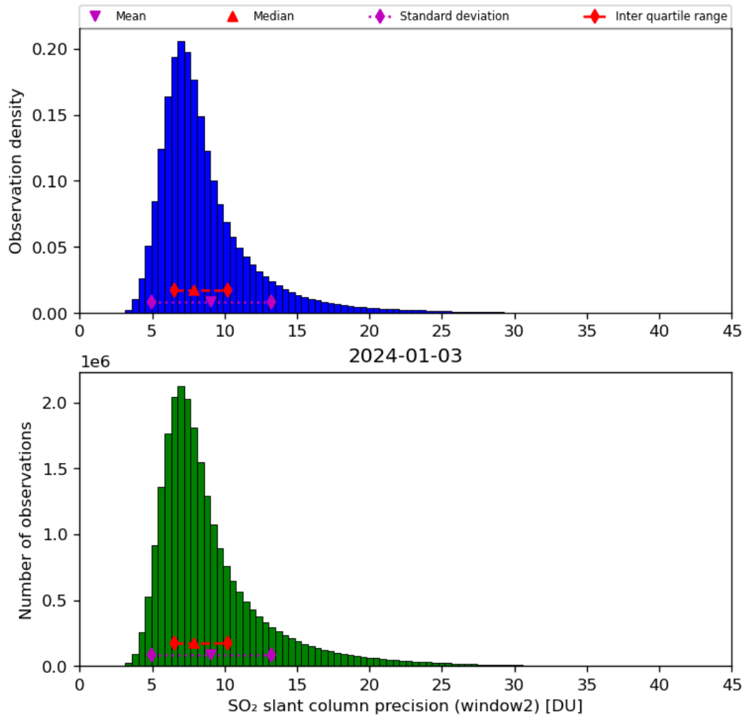
Figure 61: Histogram of “SO 2 slant column precision (window2)” for 2024-01-02 to 2024-01-04
