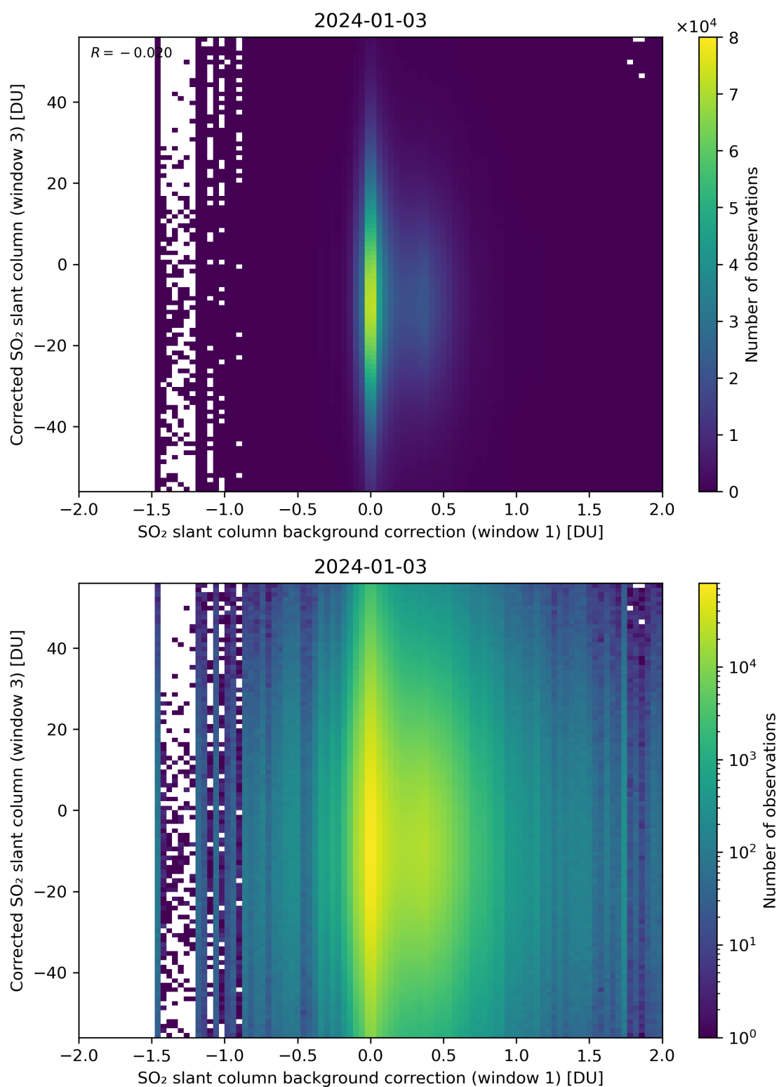
Figure 105: Scatter density plot of “SO 2 slant column background correction (window 1)” against “Corrected SO 2 slant column (window 3)” for 2024-01-02 to 2024-01-04.
