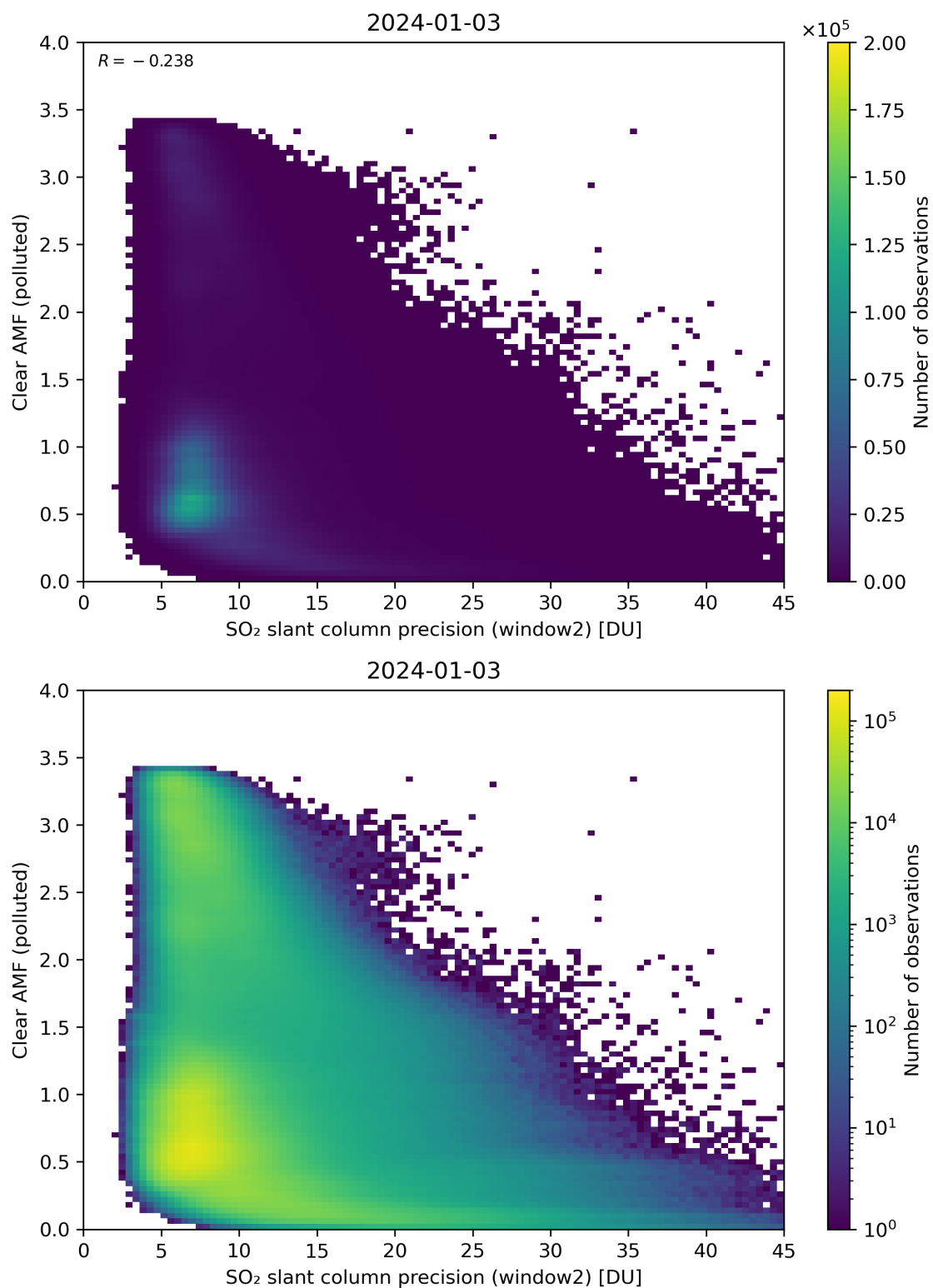
Figure 246: Scatter density plot of “SO 2 slant column precision (window2)” against “Clear AMF (polluted)” for 2024-01-02 to 2024-01-04.
