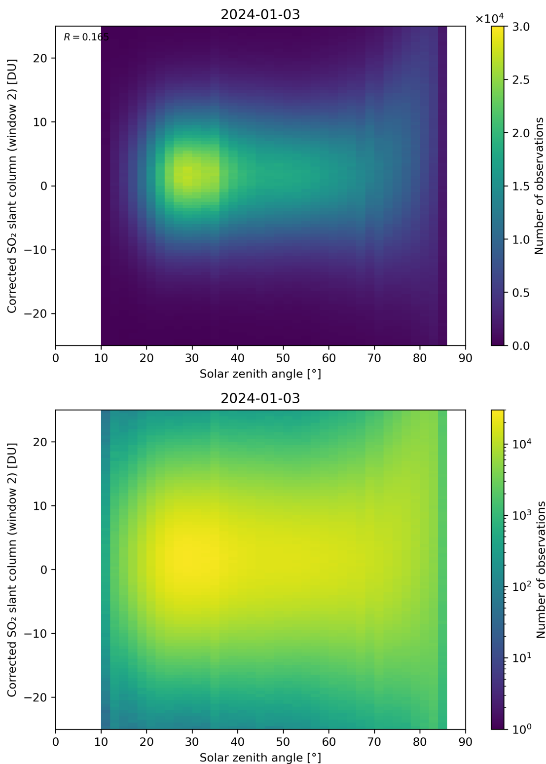
Figure 167: Scatter density plot of “Solar zenith angle” against “Corrected SO 2 slant column (window 2)” for 2024-01-02 to 2024-01-04.
