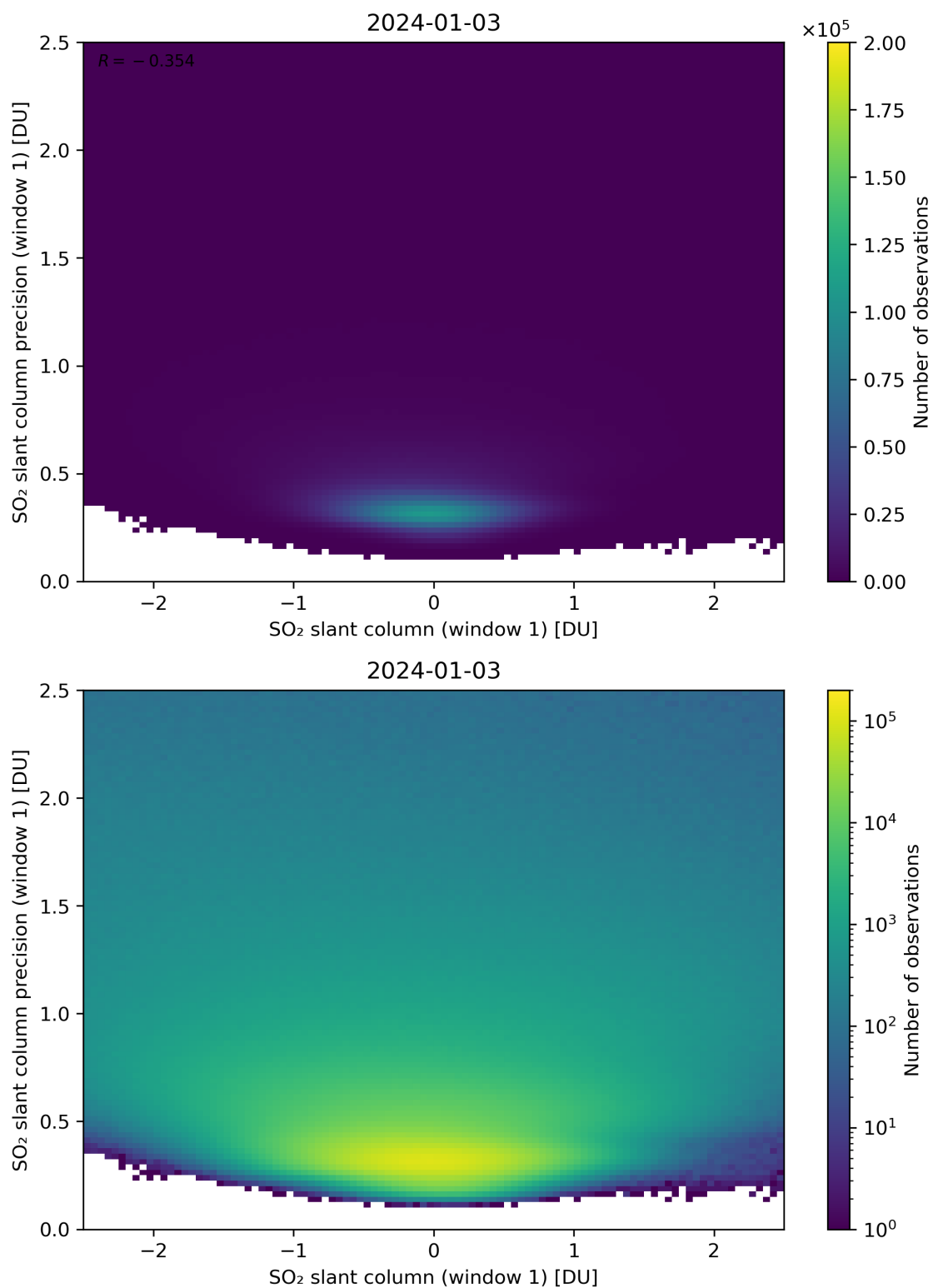
Figure 235: Scatter density plot of “SO 2 slant column (window 1)” against “SO 2 slant column precision (window 1)” for 2024-01-02 to 2024-01-04.
