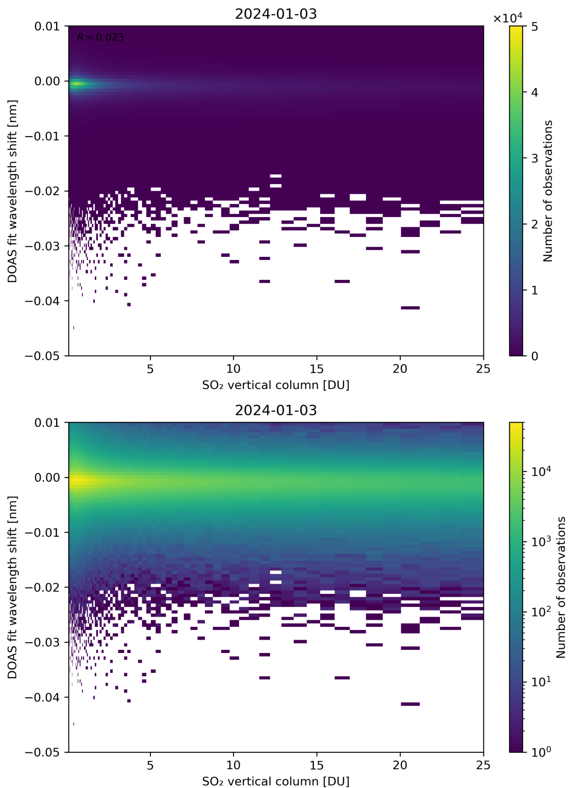
Figure 276: Scatter density plot of “SO 2 vertical column” against “DOAS fit wavelength shift” for 2024-01-02 to 2024-01-04.
