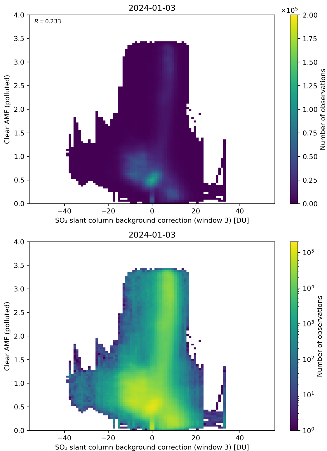
Figure 124: Scatter density plot of “SO 2 slant column background correction (window 3)” against “Clear AMF (polluted)” for 2024-01-02 to 2024-01-04.
