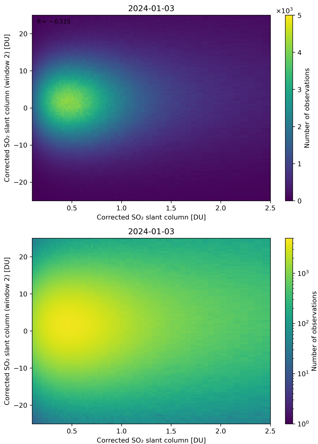
Figure 185: Scatter density plot of “Corrected SO 2 slant column” against “Corrected SO 2 slant column (window 2)” for 2024-01-02 to 2024-01-04.
