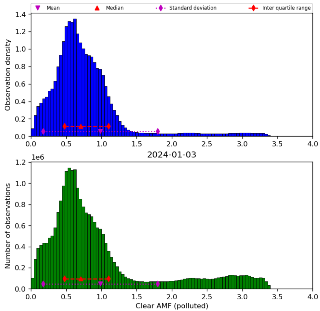
Figure 73: Histogram of “Clear AMF (polluted)” for 2024-01-02 to 2024-01-04
