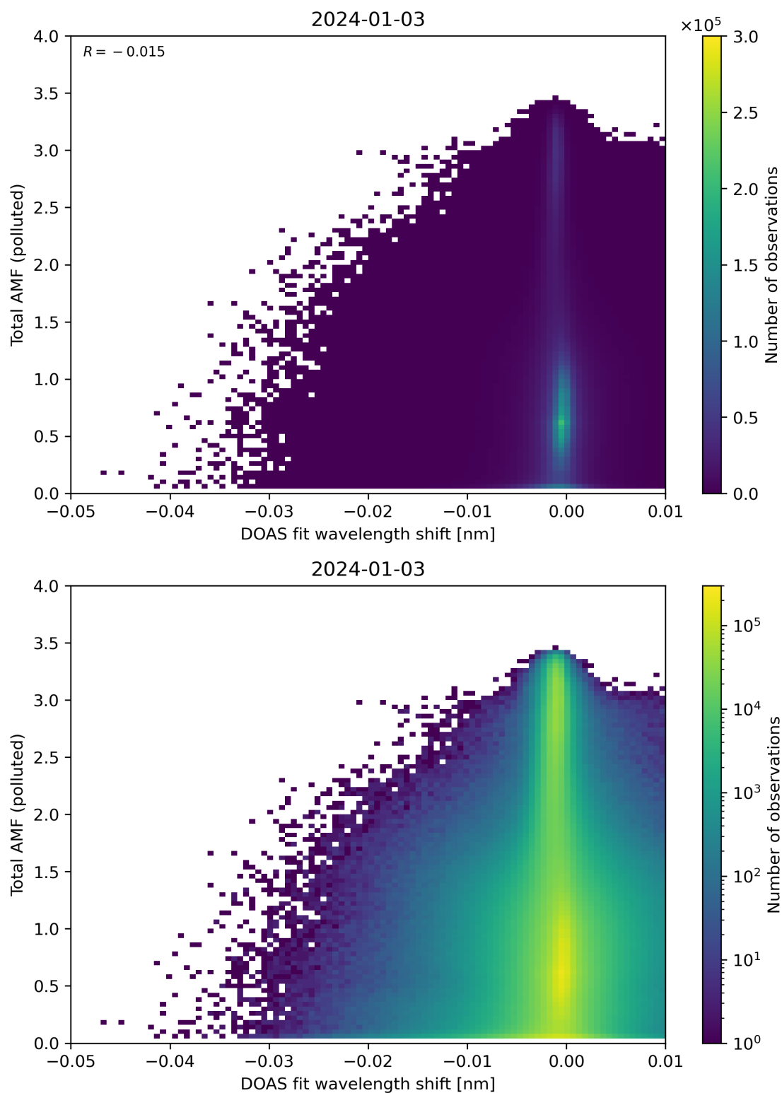
Figure 130: Scatter density plot of “DOAS fit wavelength shift” against “Total AMF (polluted)” for 2024-01-02 to 2024-01-04.
