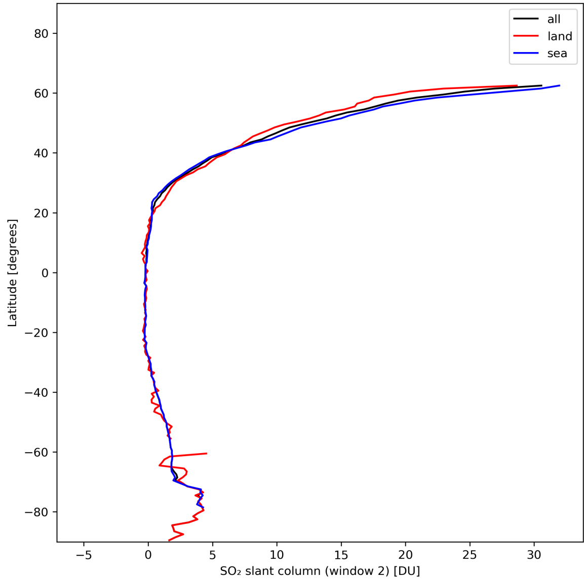
Figure 37: Zonal average of “SO 2 slant column (window 2)” for 2024-01-02 to 2024-01-04.
