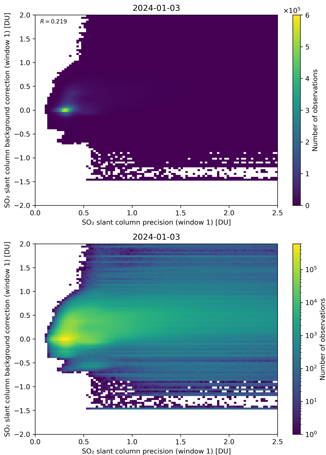
Figure 218: Scatter density plot of “SO 2 slant column precision (window 1)” against “SO 2 slant column background correction (window 1)” for 2024-01-02 to 2024-01-04.
