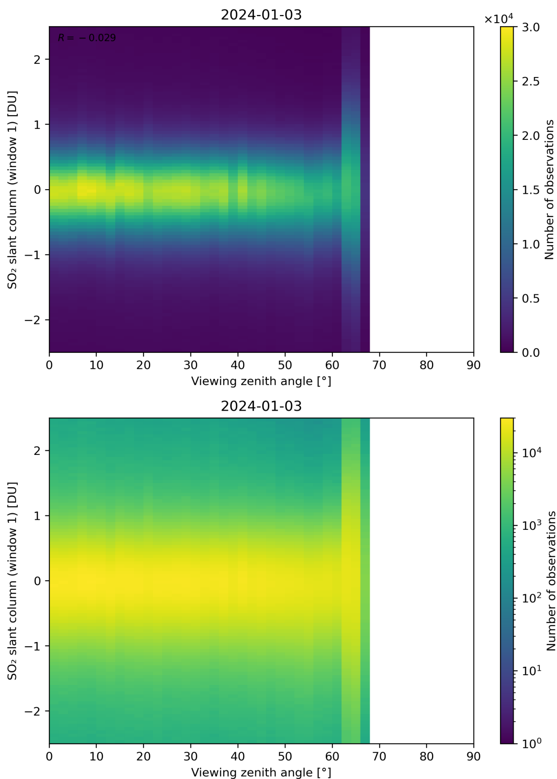
Figure 320: Scatter density plot of “Viewing zenith angle” against “SO 2 slant column (window 1)” for 2024-01-02 to 2024-01-04.
