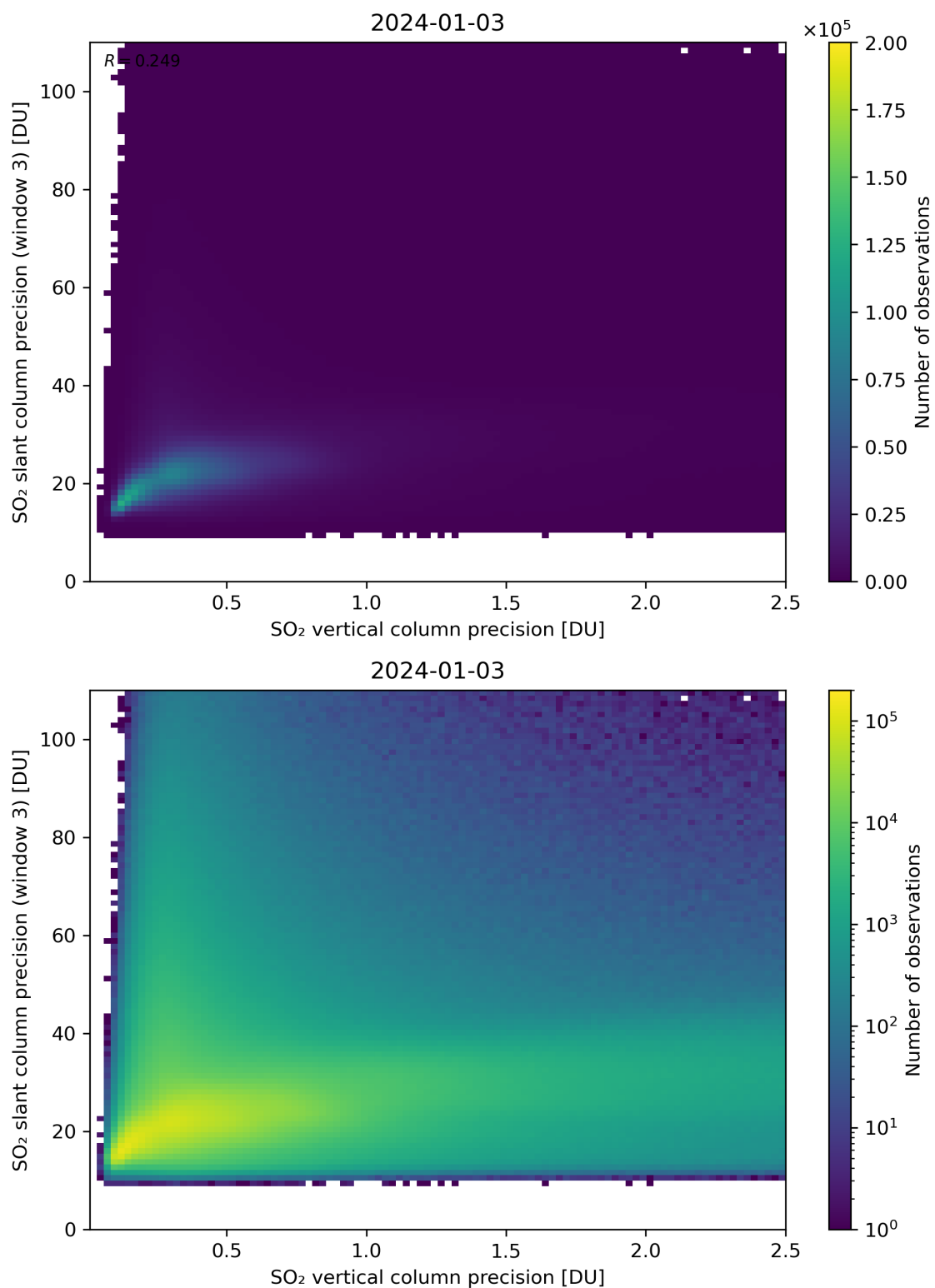
Figure 293: Scatter density plot of “SO 2 vertical column precision” against “SO 2 slant column precision (window 3)” for 2024-01-02 to 2024-01-04.
