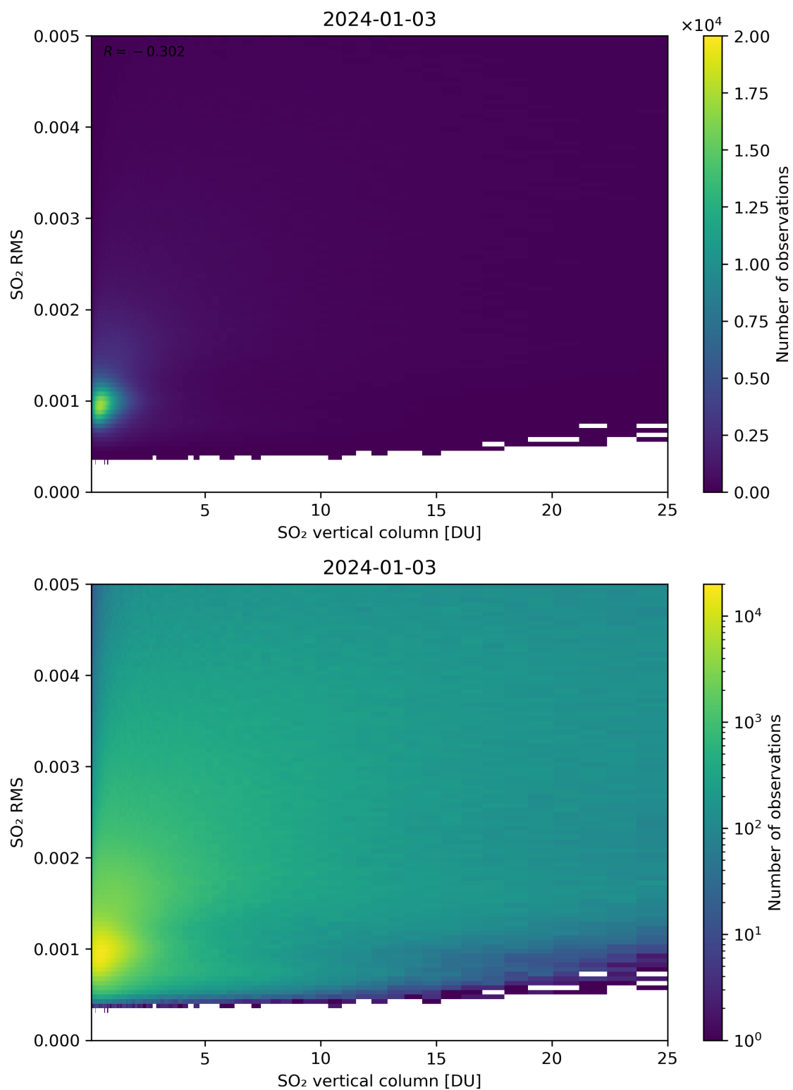
Figure 278: Scatter density plot of “SO 2 vertical column” against “SO 2 RMS” for 2024-01-02 to 2024-01-04.
