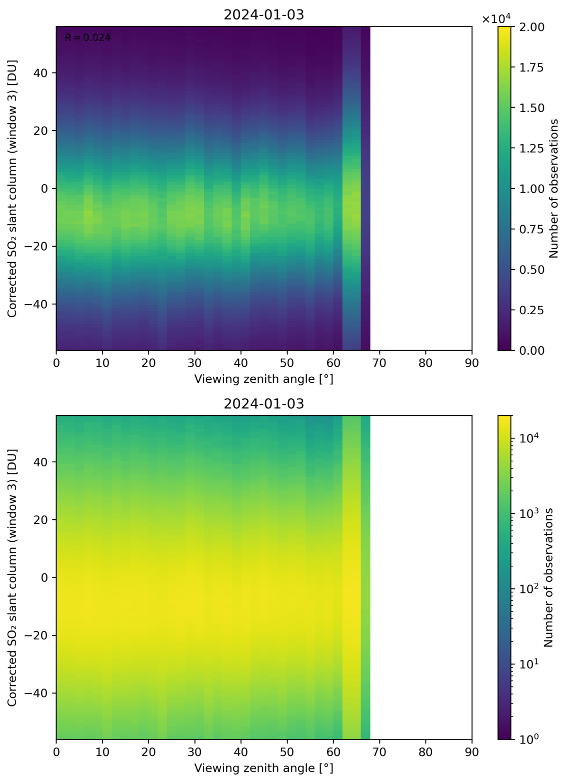
Figure 319: Scatter density plot of “Viewing zenith angle” against “Corrected SO 2 slant column (window 3)” for 2024-01-02 to 2024-01-04.
