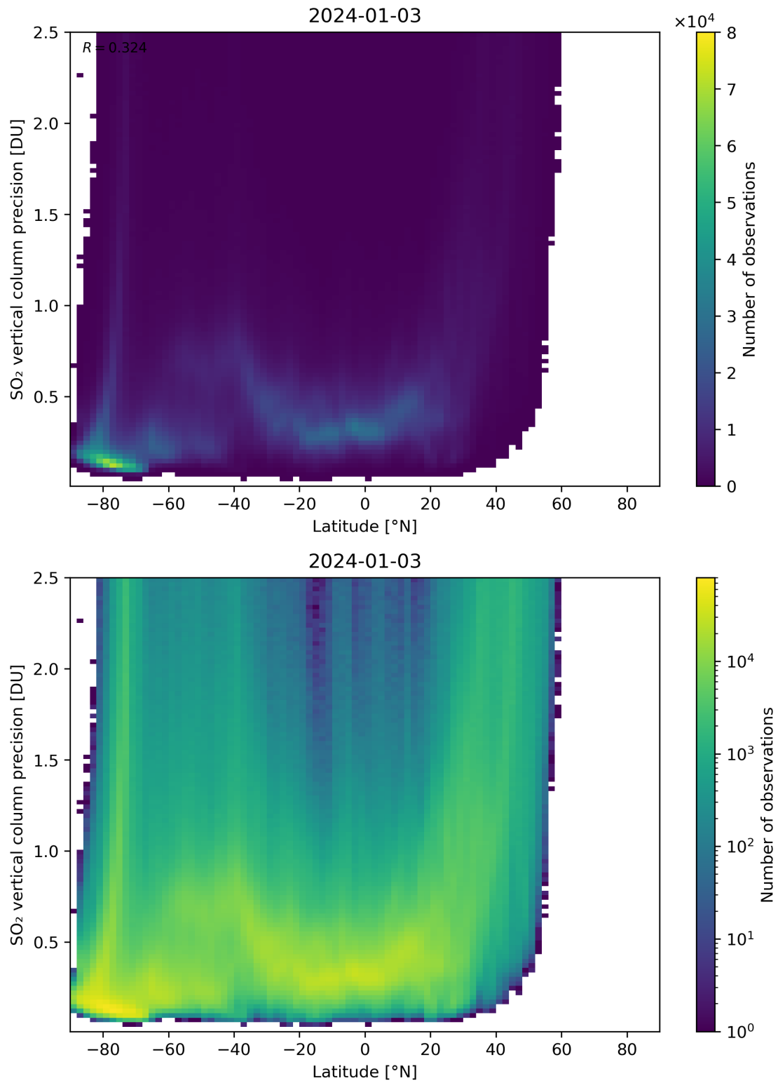
Figure 157: Scatter density plot of “Latitude” against “SO 2 vertical column precision” for 2024-01-02 to 2024-01-04.
