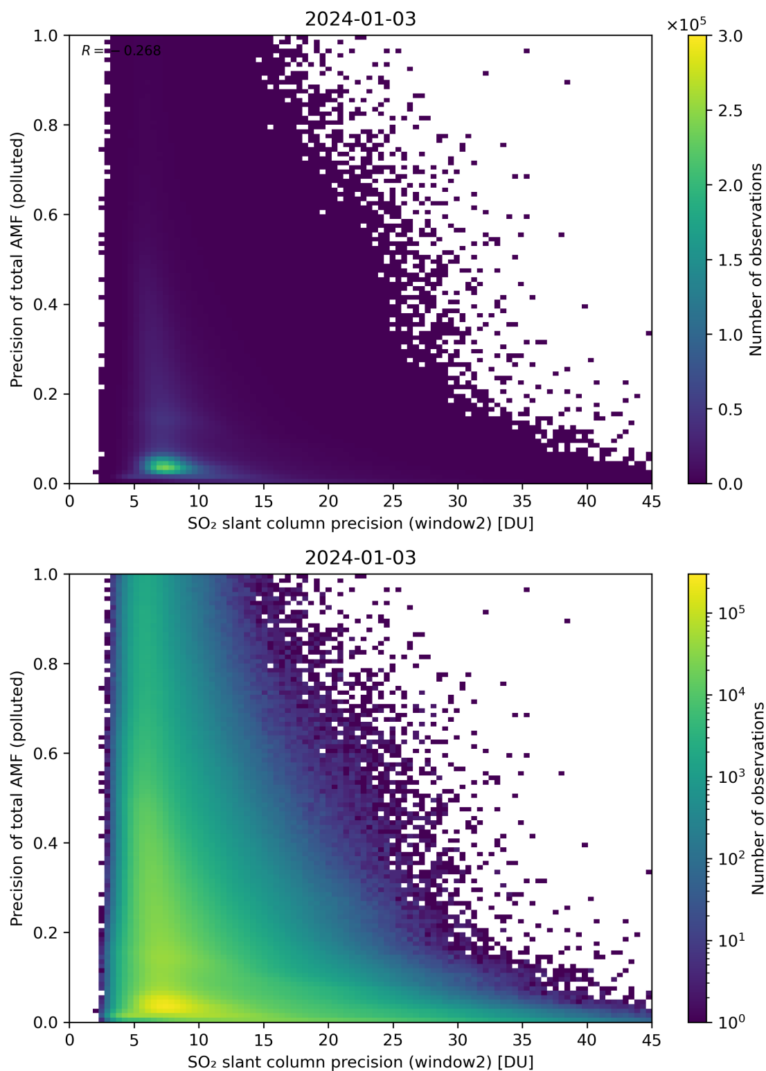
Figure 252: Scatter density plot of “SO 2 slant column precision (window2)” against “Precision of total AMF (polluted)” for 2024-01-02 to 2024-01-04.
