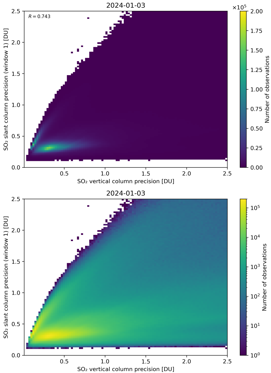
Figure 290: Scatter density plot of “SO 2 vertical column precision” against “SO 2 slant column precision (window 1)” for 2024-01-02 to 2024-01-04.
