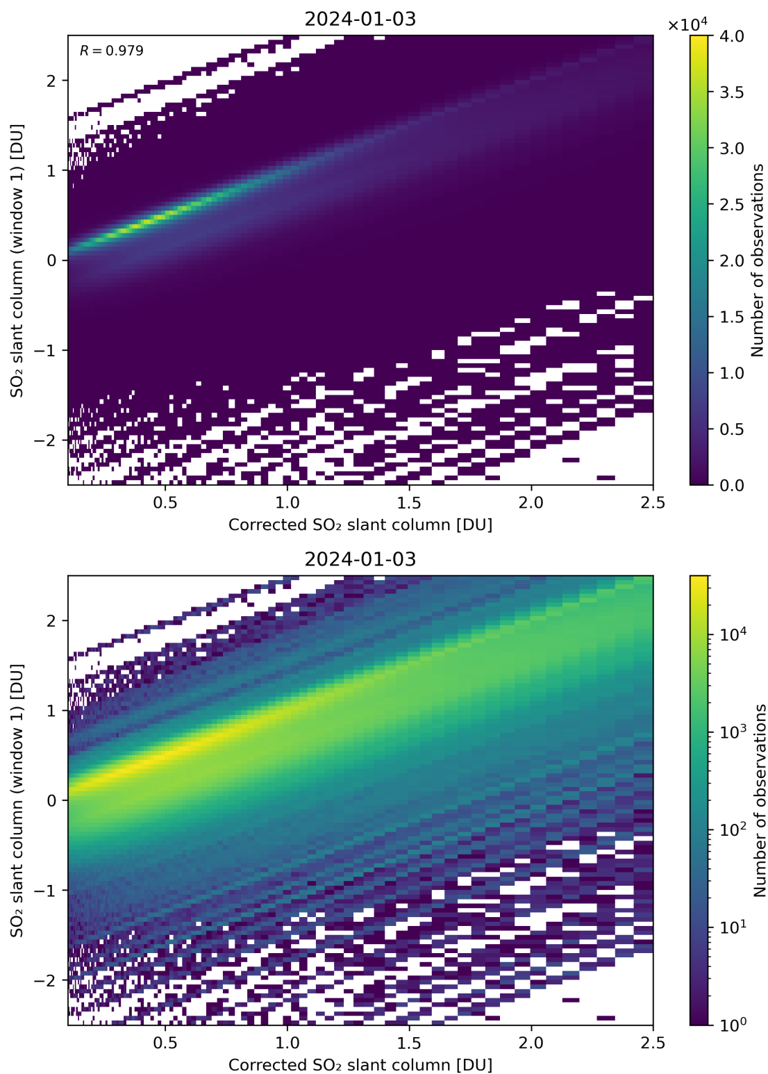
Figure 187: Scatter density plot of “Corrected SO 2 slant column” against “SO 2 slant column (window 1)” for 2024-01-02 to 2024-01-04.
