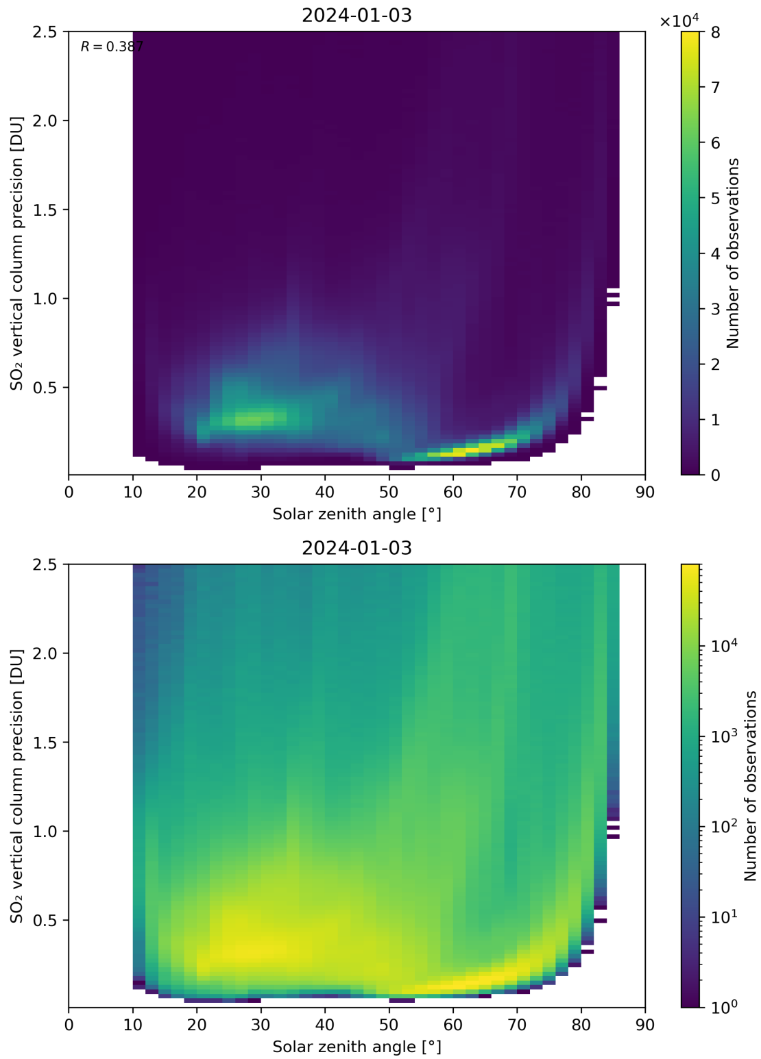
Figure 177: Scatter density plot of “Solar zenith angle” against “SO 2 vertical column precision” for 2024-01-02 to 2024-01-04.
