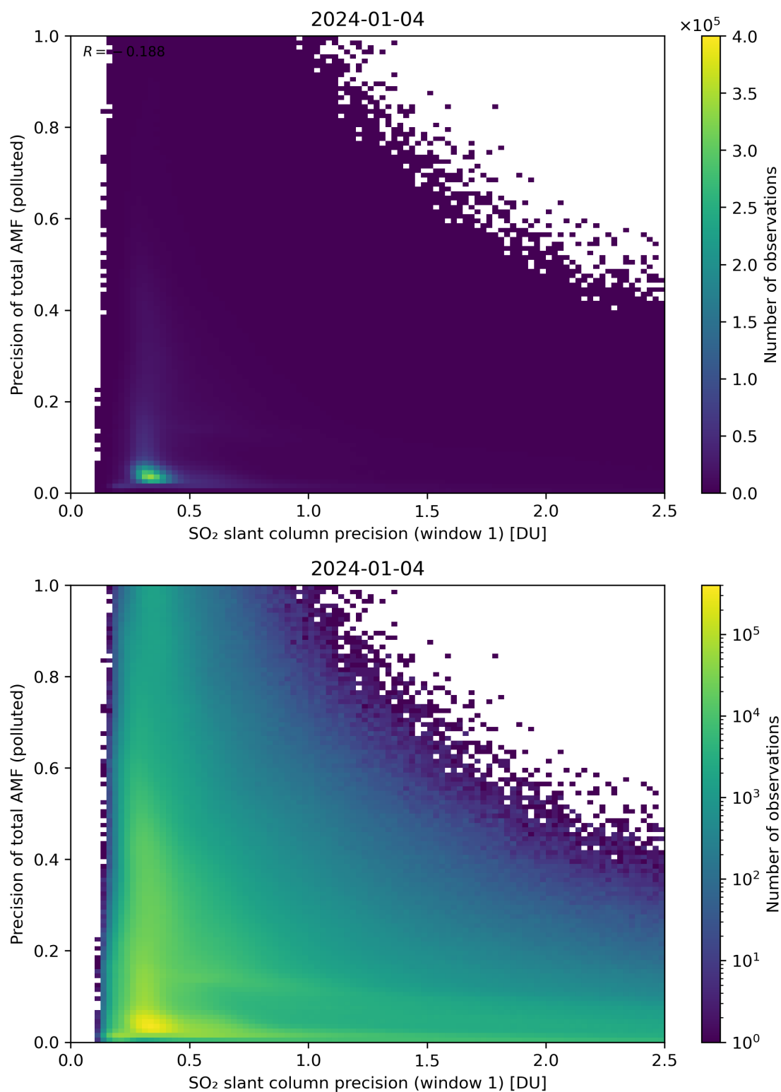
Figure 231: Scatter density plot of “SO 2 slant column precision (window 1)” against “Precision of total AMF (polluted)” for 2024-01-03 to 2024-01-05.
