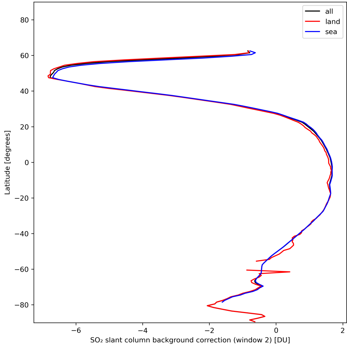
Figure 40: Zonal average of “SO 2 slant column background correction (window 2)” for 2024-01-03 to 2024-01-05.
