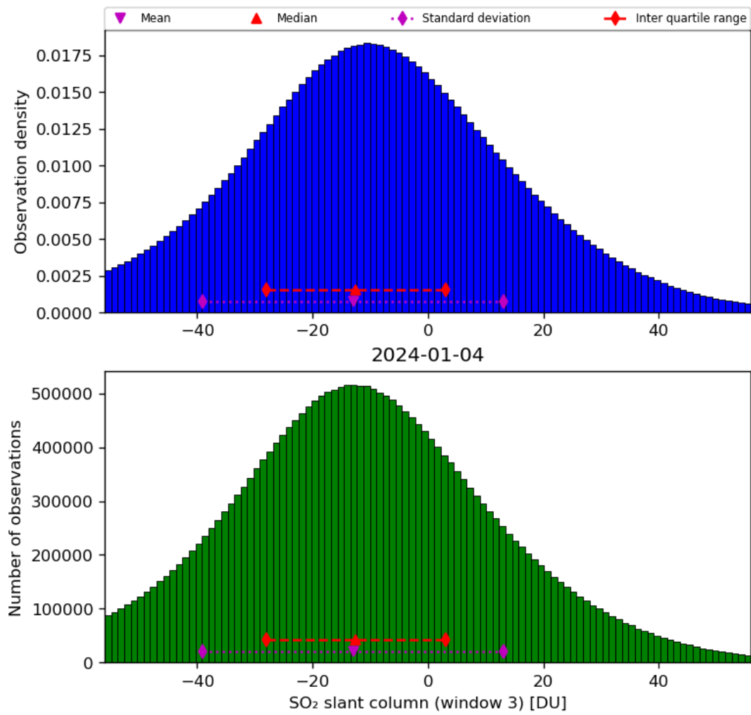
Figure 64: Histogram of “SO 2 slant column (window 3)” for 2024-01-03 to 2024-01-05
