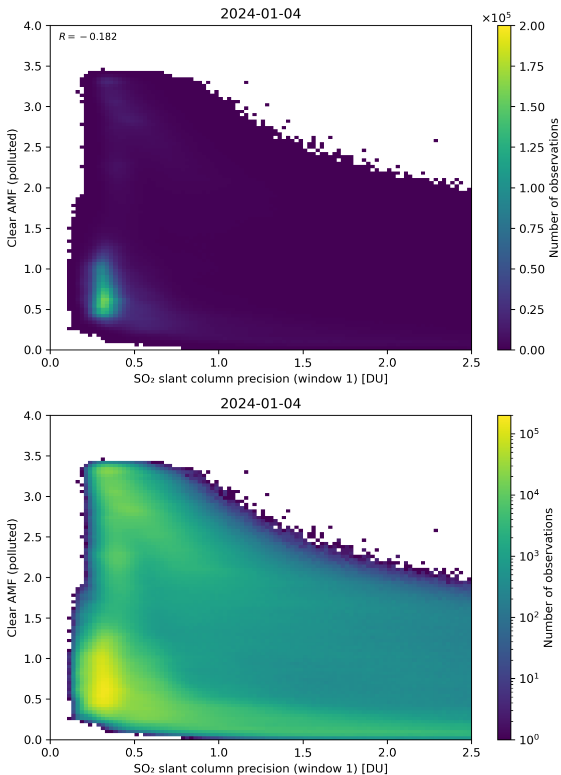
Figure 224: Scatter density plot of “SO 2 slant column precision (window 1)” against “Clear AMF (polluted)” for 2024-01-03 to 2024-01-05.
