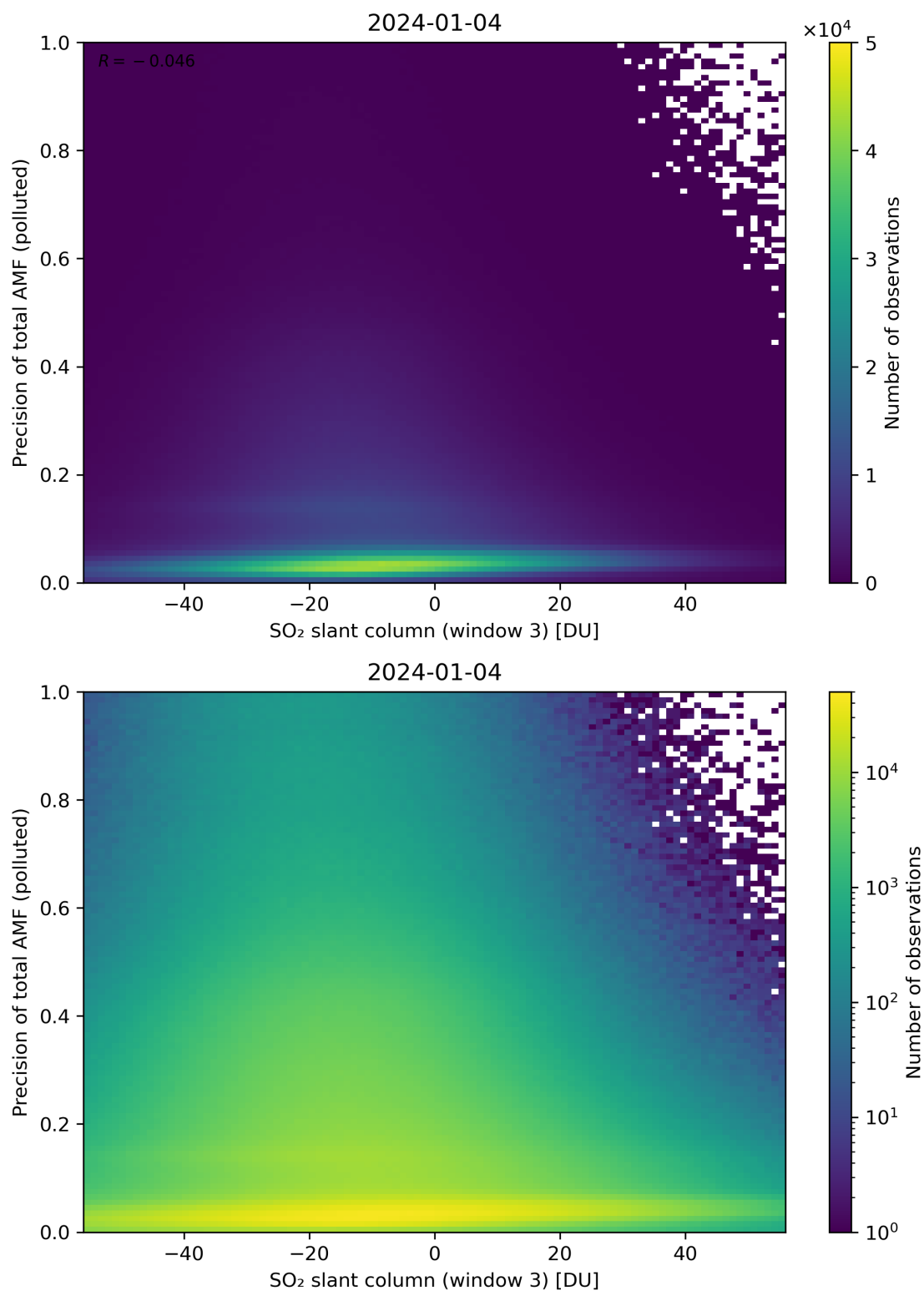
Figure 269: Scatter density plot of “SO 2 slant column (window 3)” against “Precision of total AMF (polluted)” for 2024-01-03 to 2024-01-05.
