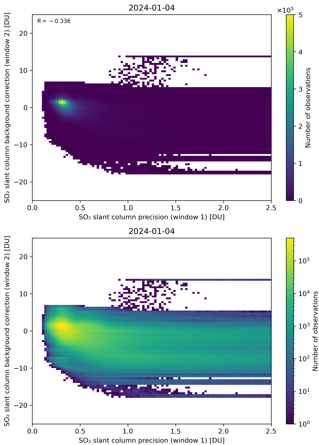
Figure 219: Scatter density plot of “SO 2 slant column precision (window 1)” against “SO 2 slant column background correction (window 2)” for 2024-01-03 to 2024-01-05.
