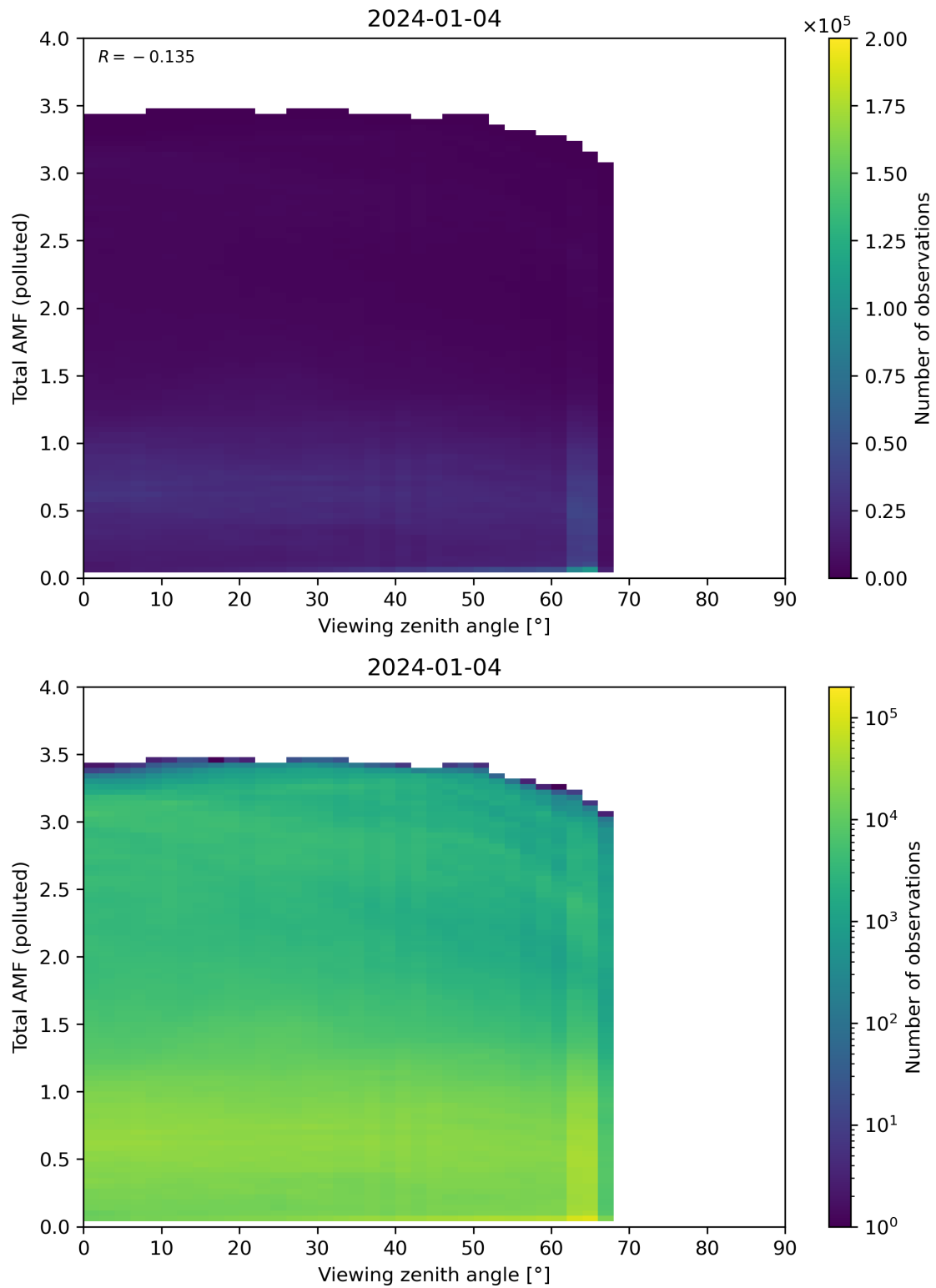
Figure 325: Scatter density plot of “Viewing zenith angle” against “Total AMF (polluted)” for 2024-01-03 to 2024-01-05.
