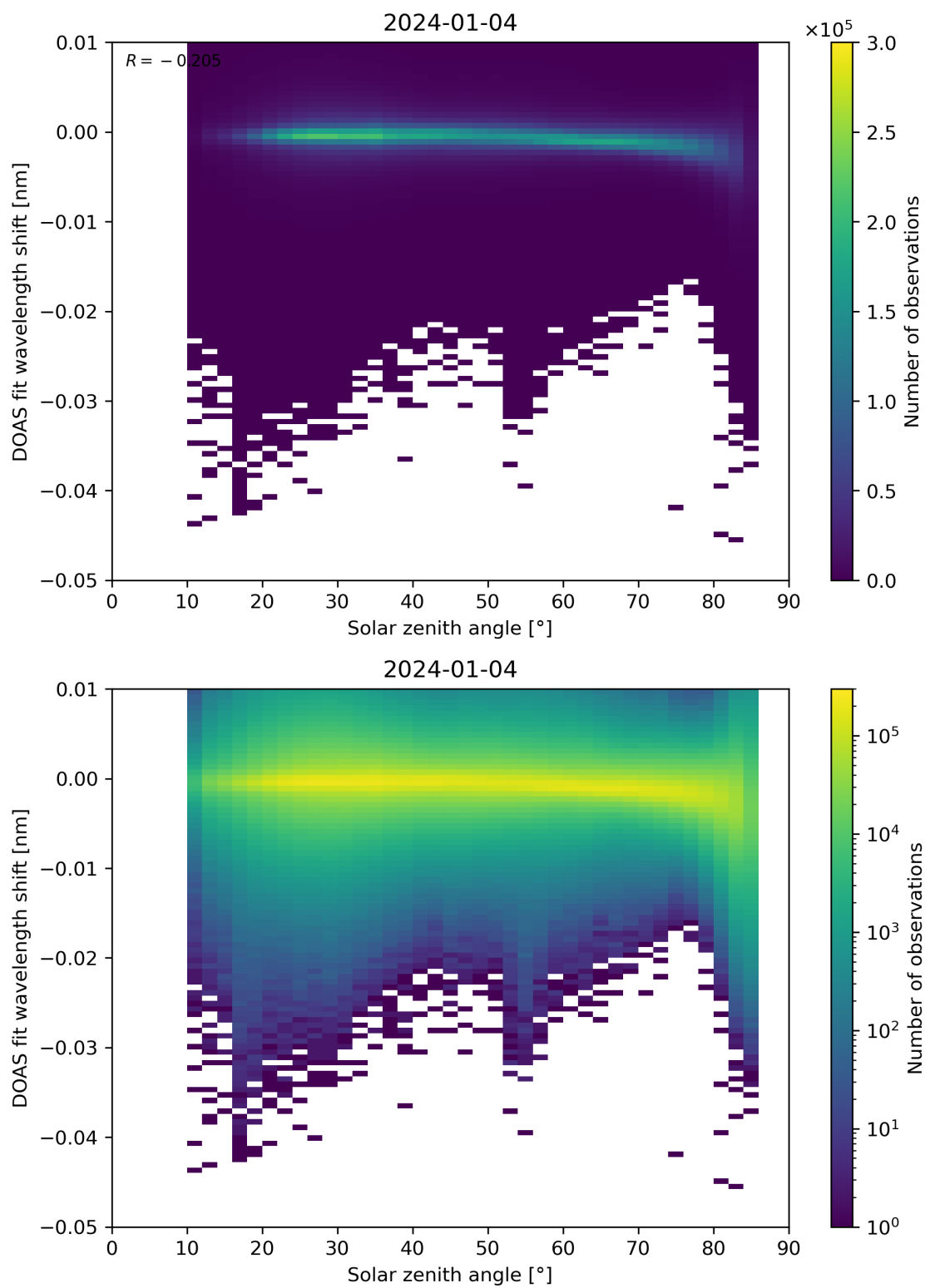
Figure 161: Scatter density plot of “Solar zenith angle” against “DOAS fit wavelength shift” for 2024-01-03 to 2024-01-05.
