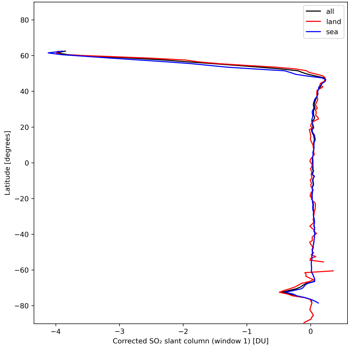
Figure 35: Zonal average of “Corrected SO 2 slant column (window 1)” for 2024-01-03 to 2024-01-05.
