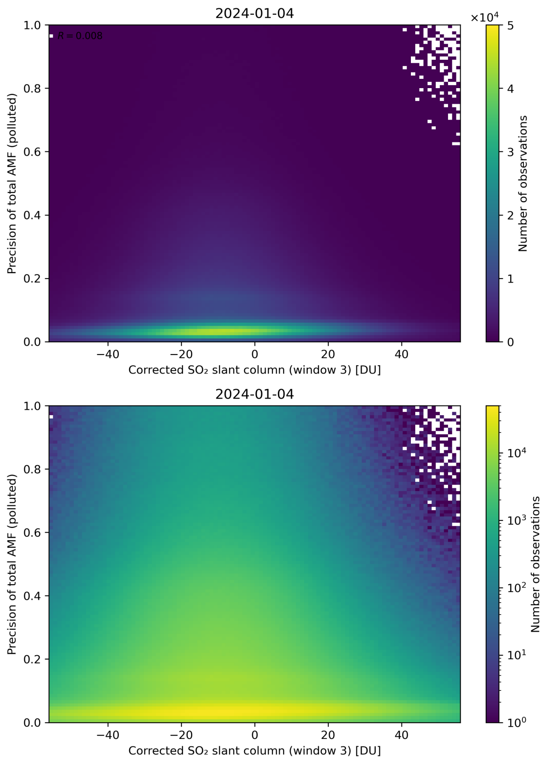
Figure 211: Scatter density plot of “Corrected SO 2 slant column (window 3)” against “Precision of total AMF (polluted)” for 2024-01-03 to 2024-01-05.
