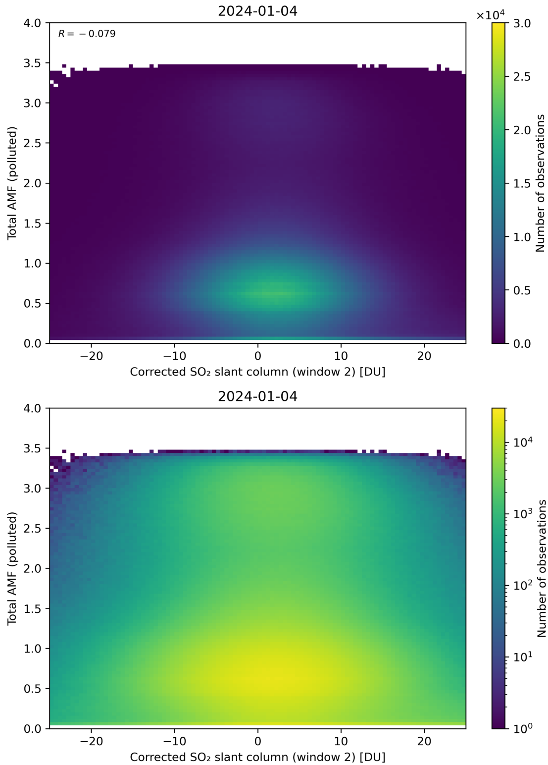
Figure 203: Scatter density plot of “Corrected SO 2 slant column (window 2)” against “Total AMF (polluted)” for 2024-01-03 to 2024-01-05.
