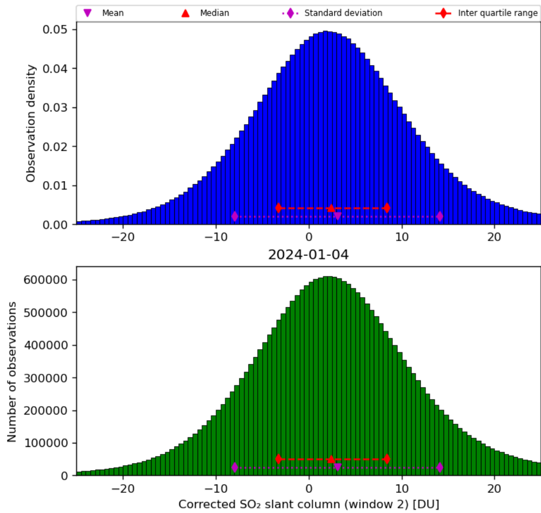
Figure 62: Histogram of “Corrected SO 2 slant column (window 2)” for 2024-01-03 to 2024-01-05
