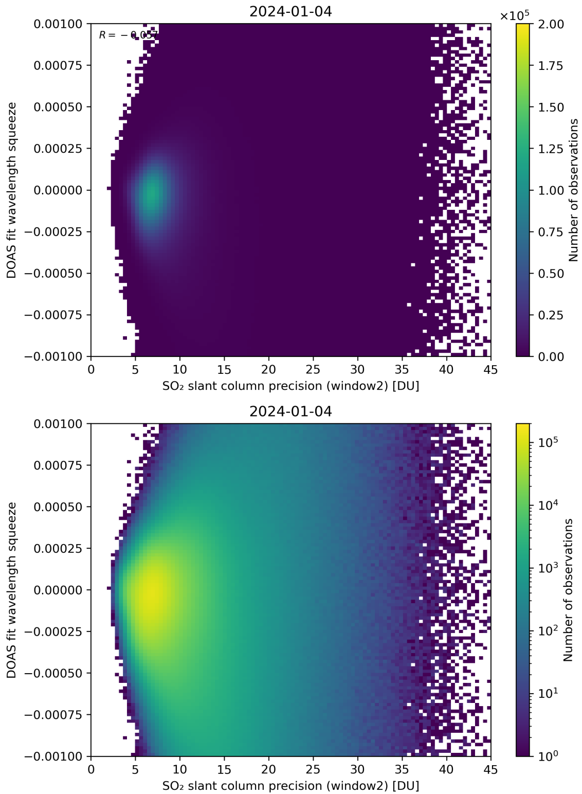
Figure 244: Scatter density plot of “SO 2 slant column precision (window2)” against “DOAS fit wavelength squeeze” for 2024-01-03 to 2024-01-05.
