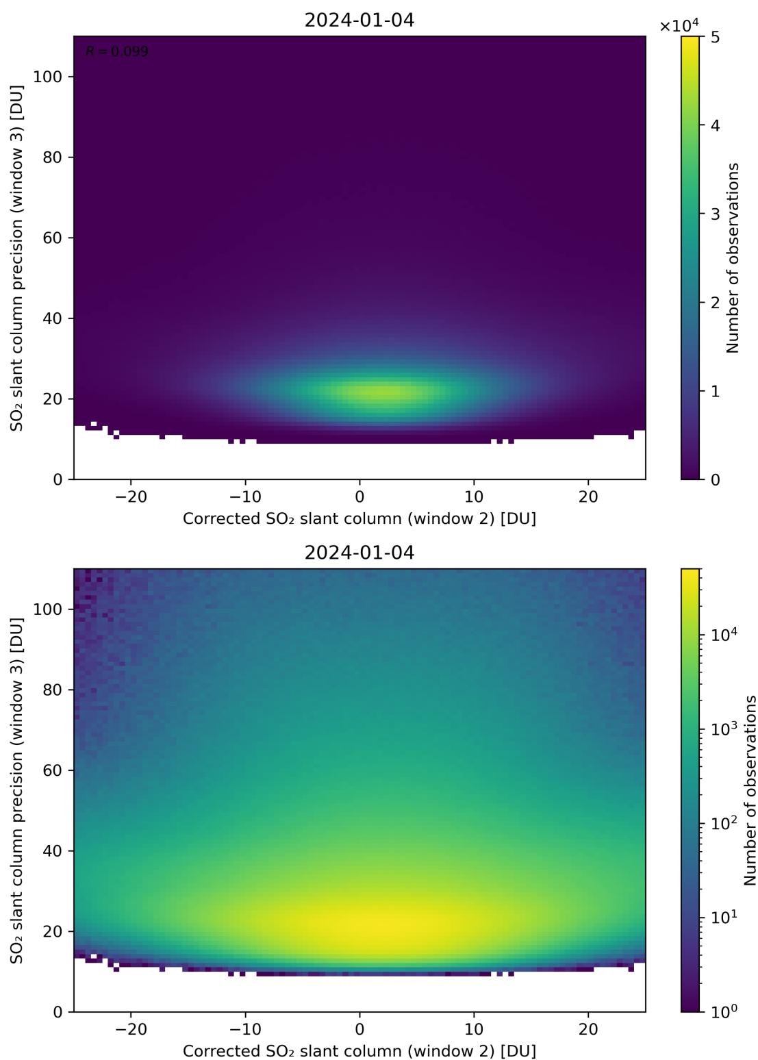
Figure 202: Scatter density plot of “Corrected SO 2 slant column (window 2)” against “SO 2 slant column precision (window 3)” for 2024-01-03 to 2024-01-05.
