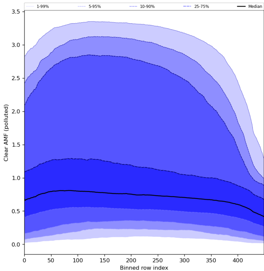
Figure 96: Along track statistics of “Clear AMF (polluted)” for 2024-01-03 to 2024-01-05
