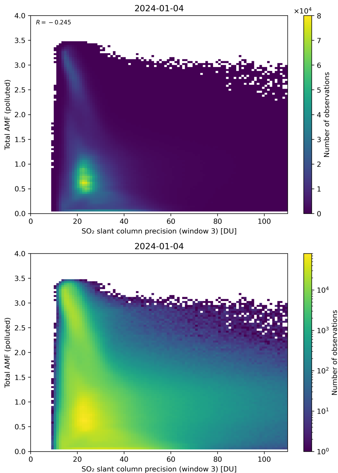
Figure 263: Scatter density plot of “SO 2 slant column precision (window 3)” against “Total AMF (polluted)” for 2024-01-03 to 2024-01-05.
