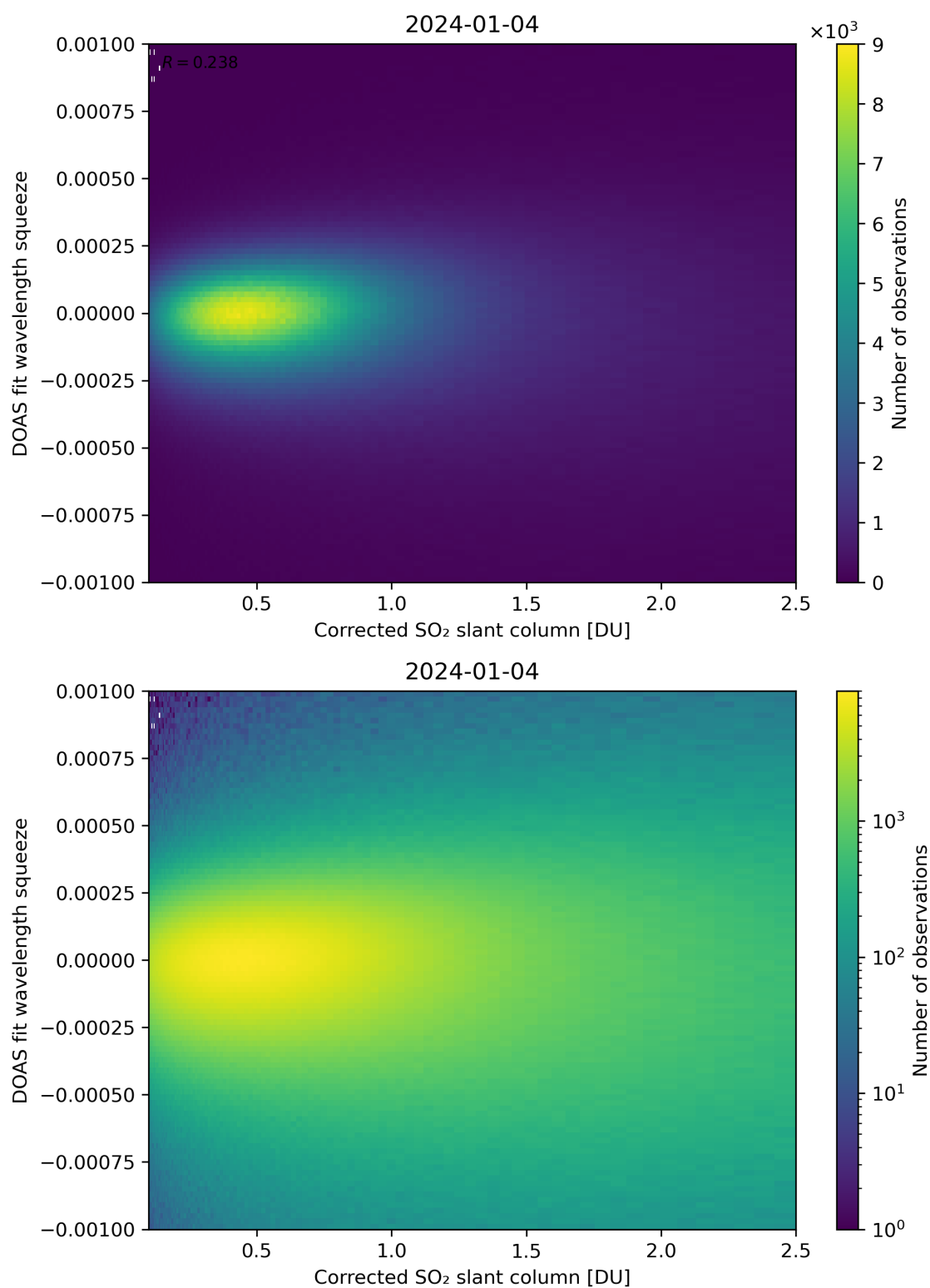
Figure 182: Scatter density plot of “Corrected SO 2 slant column” against “DOAS fit wavelength squeeze” for 2024-01-03 to 2024-01-05.
