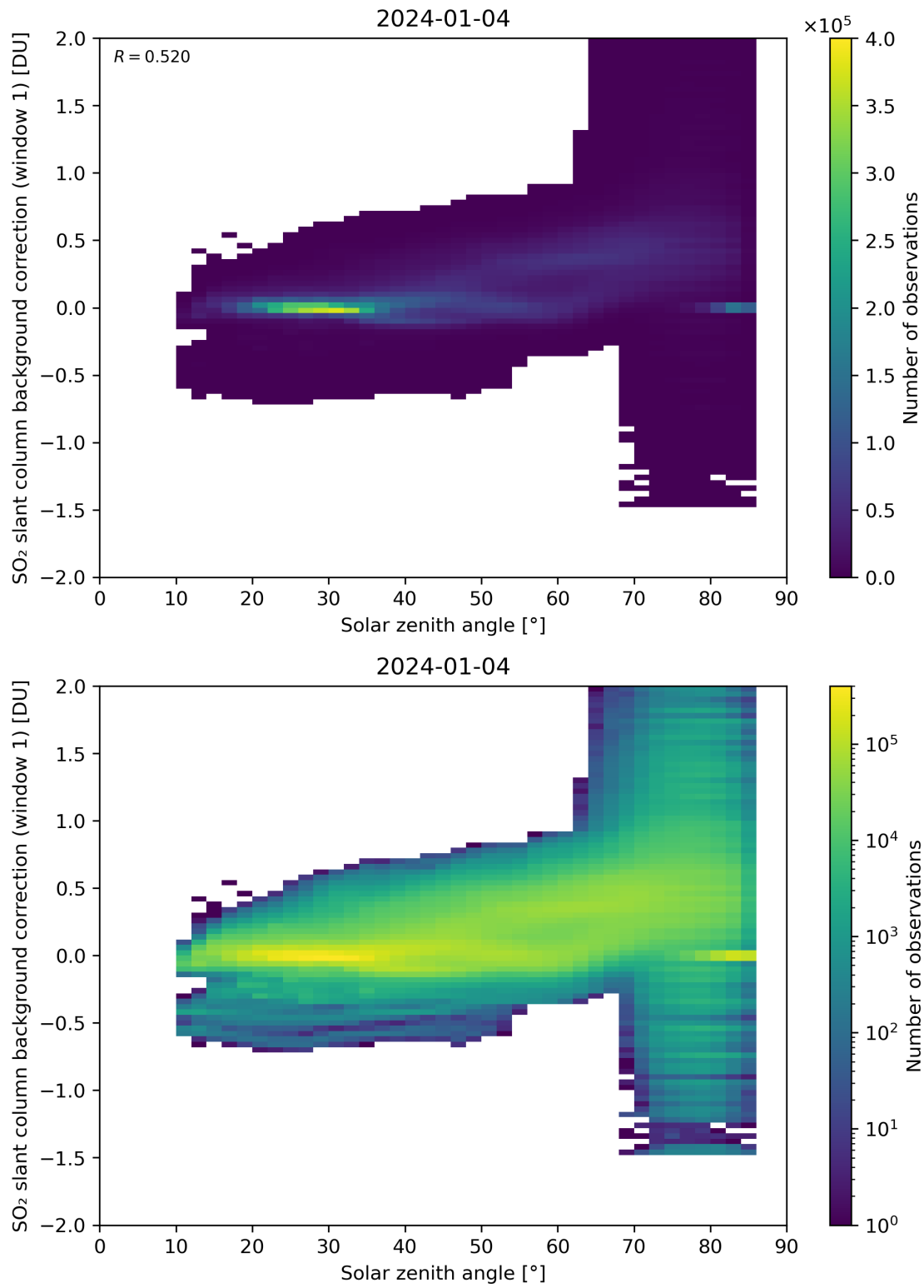
Figure 158: Scatter density plot of “Solar zenith angle” against “SO 2 slant column background correction (window 1)” for 2024-01-03 to 2024-01-05.
