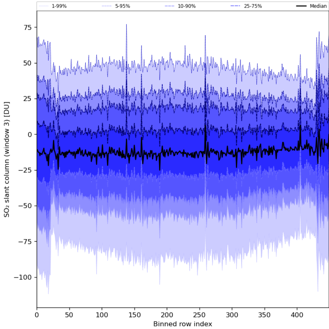
Figure 87: Along track statistics of “SO 2 slant column (window 3)” for 2024-01-03 to 2024-01-05
