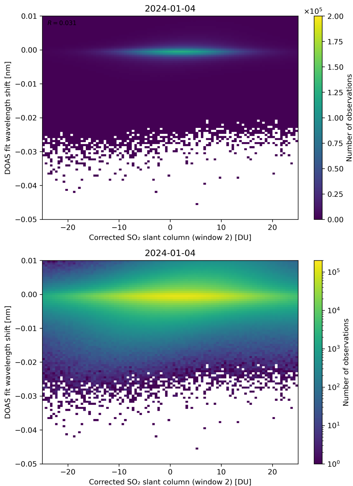
Figure 196: Scatter density plot of “Corrected SO 2 slant column (window 2)” against “DOAS fit wavelength shift” for 2024-01-03 to 2024-01-05.
