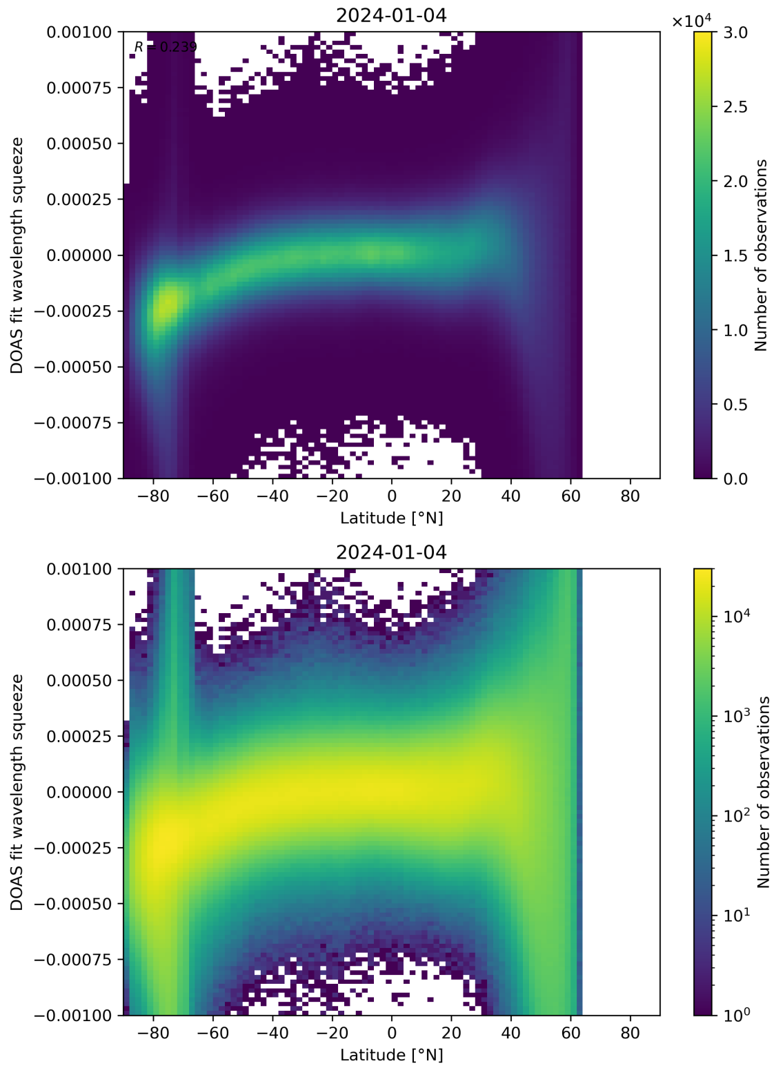
Figure 143: Scatter density plot of “Latitude” against “DOAS fit wavelength squeeze” for 2024-01-03 to 2024-01-05.
