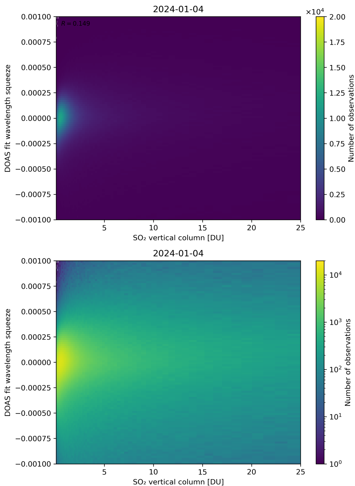
Figure 277: Scatter density plot of “SO 2 vertical column” against “DOAS fit wavelength squeeze” for 2024-01-03 to 2024-01-05.
