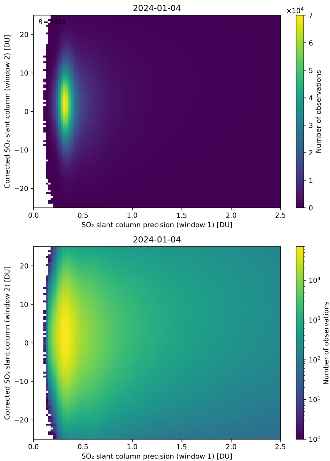
Figure 225: Scatter density plot of “SO 2 slant column precision (window 1)” against “Corrected SO 2 slant column (window 2)” for 2024-01-03 to 2024-01-05.
