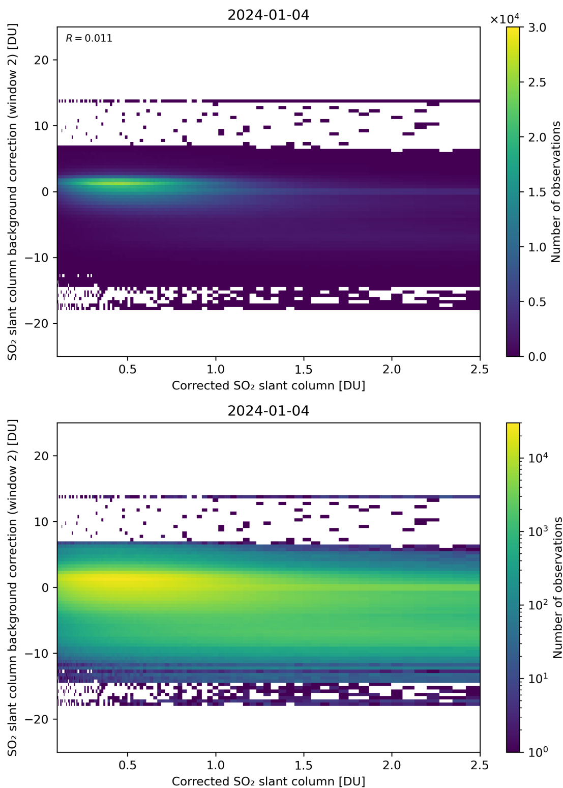
Figure 179: Scatter density plot of “Corrected SO 2 slant column” against “SO 2 slant column background correction (window 2)” for 2024-01-03 to 2024-01-05.
