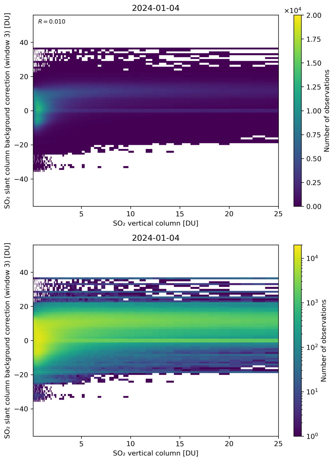
Figure 275: Scatter density plot of “SO 2 vertical column” against “SO 2 slant column background correction (window 3)” for 2024-01-03 to 2024-01-05.
