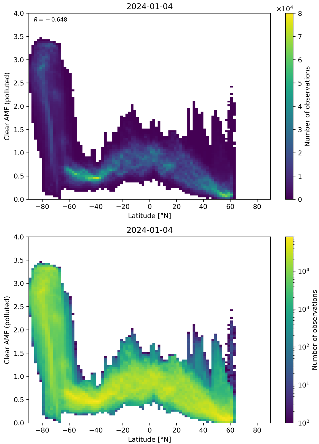
Figure 145: Scatter density plot of “Latitude” against “Clear AMF (polluted)” for 2024-01-03 to 2024-01-05.
