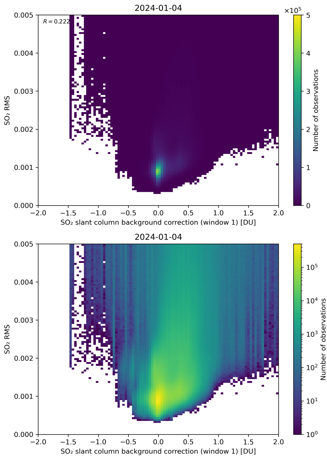
Figure 102: Scatter density plot of “SO 2 slant column background correction (window 1)” against “SO 2 RMS” for 2024-01-03 to 2024-01-05.
