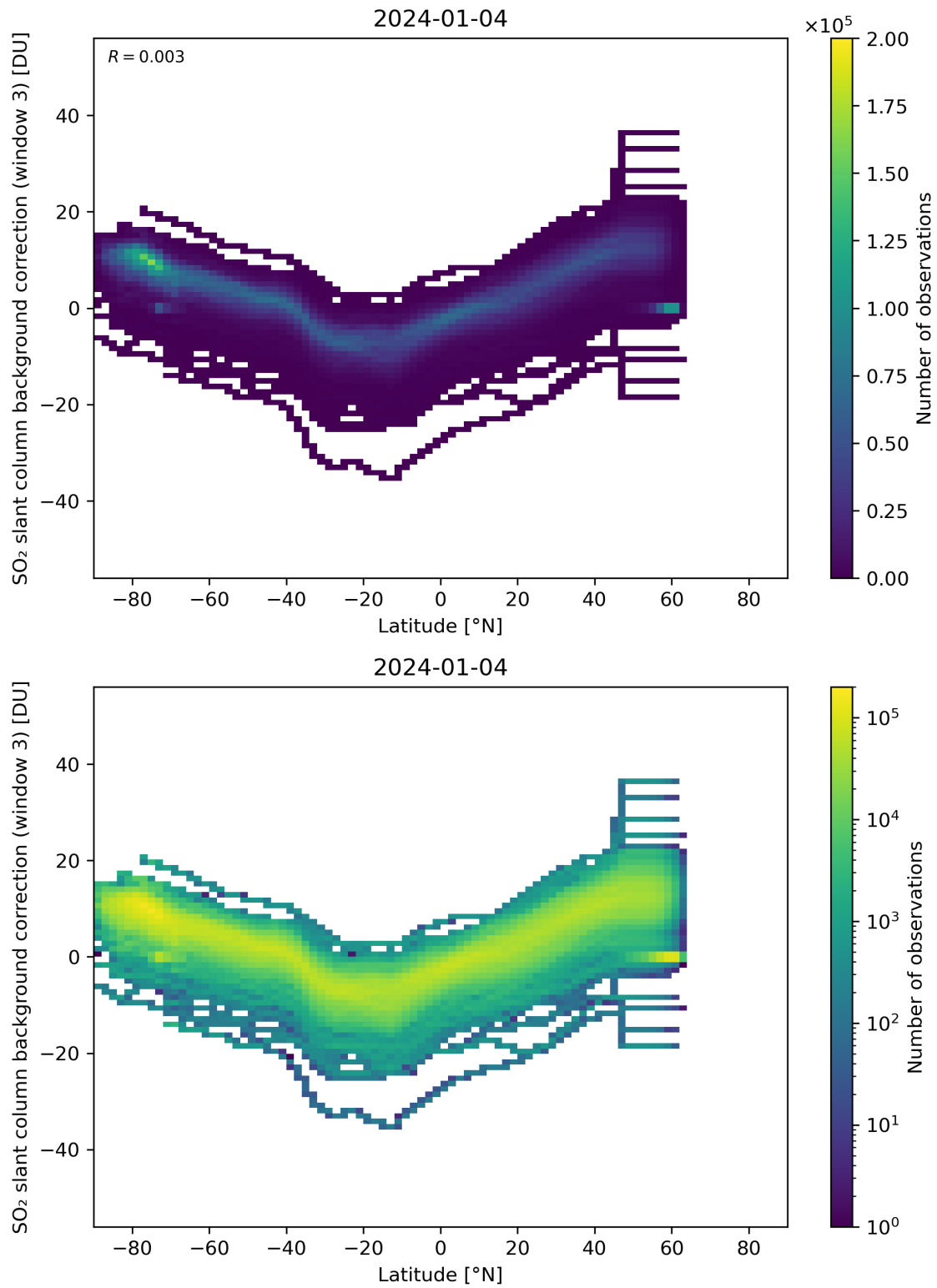
Figure 141: Scatter density plot of “Latitude” against “SO 2 slant column background correction (window 3)” for 2024-01-03 to 2024-01-05.
