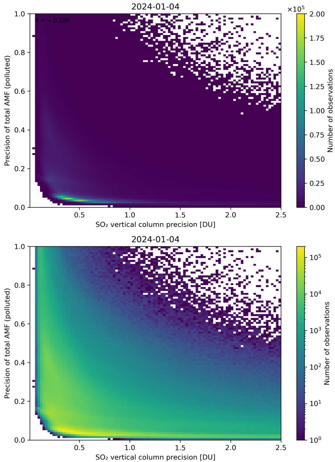
Figure 295: Scatter density plot of “SO 2 vertical column precision” against “Precision of total AMF (polluted)” for 2024-01-03 to 2024-01-05.
