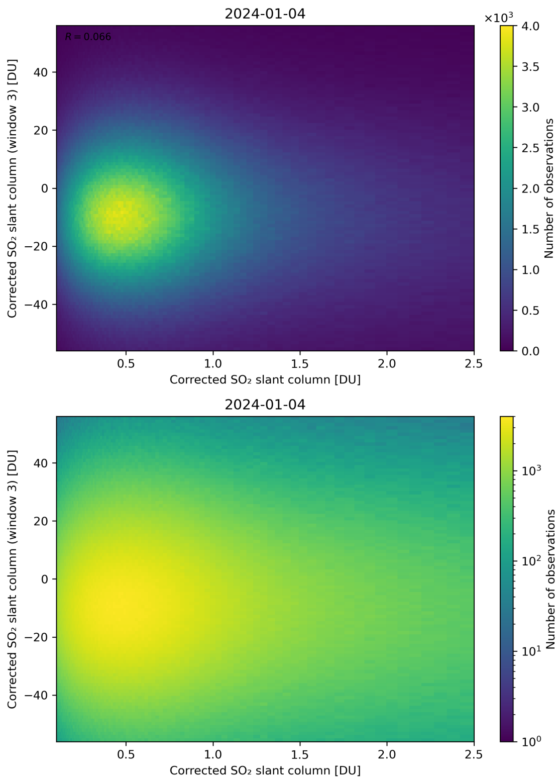
Figure 186: Scatter density plot of “Corrected SO 2 slant column” against “Corrected SO 2 slant column (window 3)” for 2024-01-03 to 2024-01-05.
