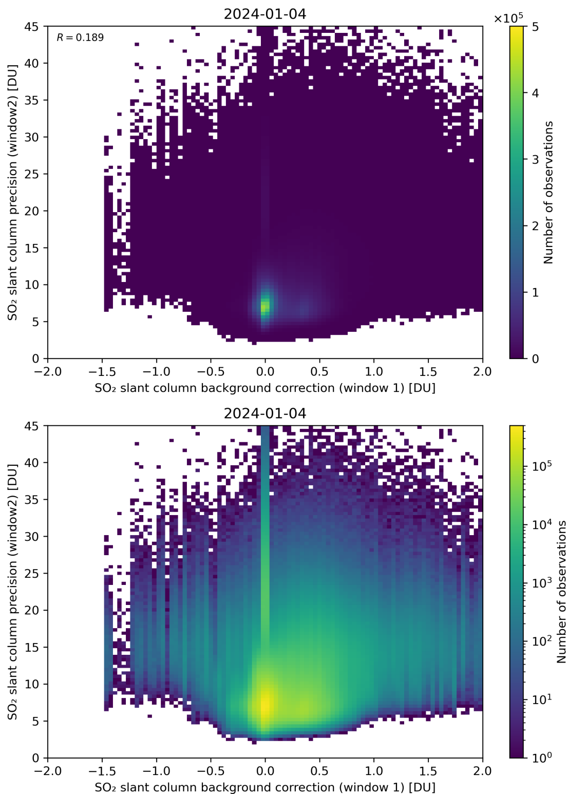
Figure 106: Scatter density plot of “SO 2 slant column background correction (window 1)” against “SO 2 slant column precision (window2)” for 2024-01-03 to 2024-01-05.
