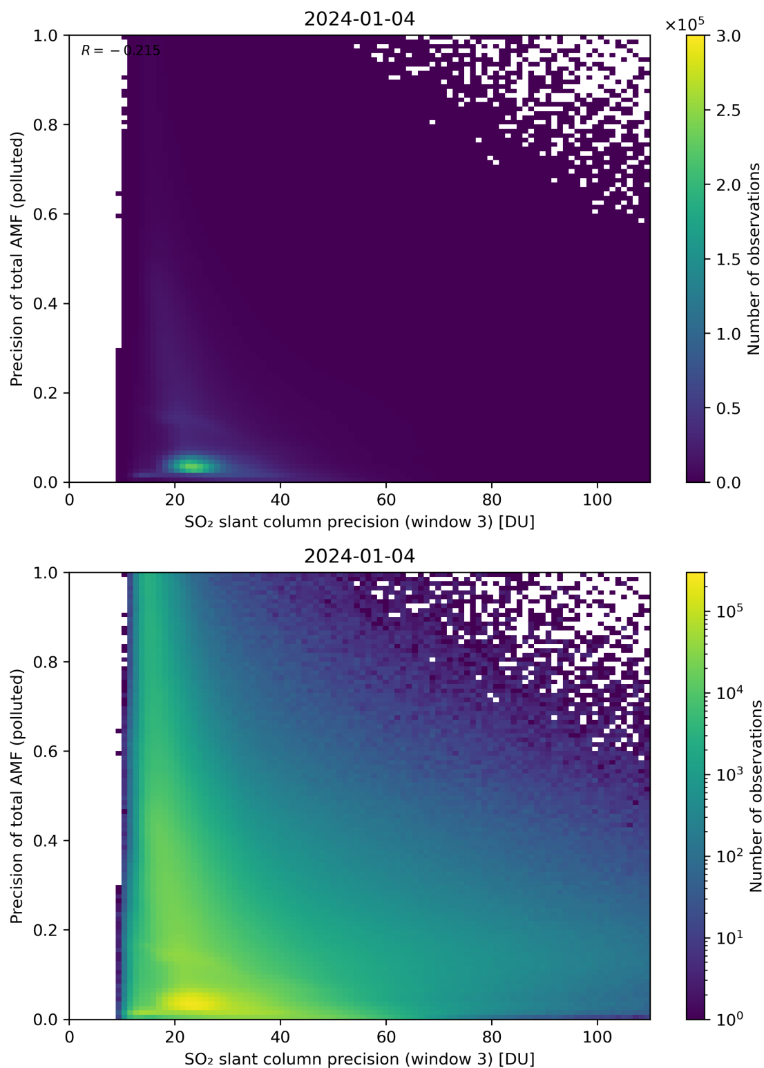
Figure 264: Scatter density plot of “SO 2 slant column precision (window 3)” against “Precision of total AMF (polluted)” for 2024-01-03 to 2024-01-05.
