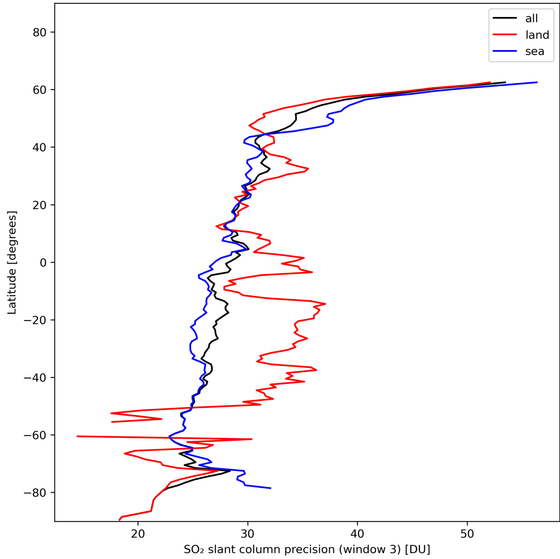
Figure 42: Zonal average of “SO 2 slant column precision (window 3)” for 2024-01-03 to 2024-01-05.
