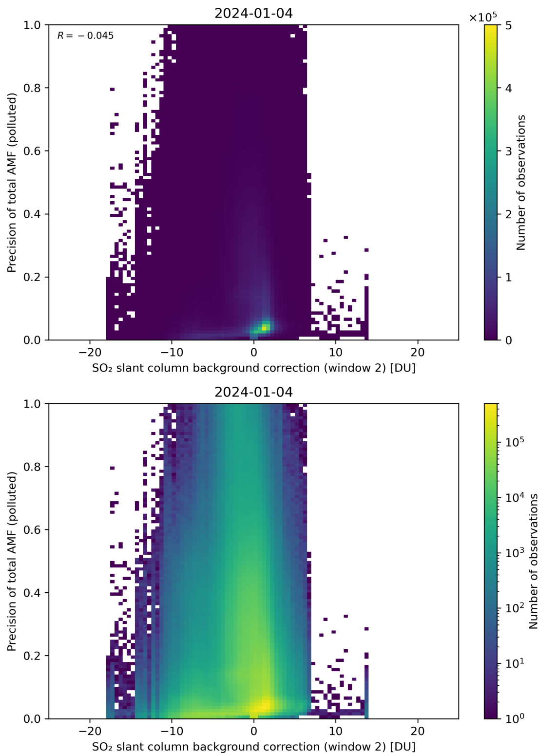
Figure 120: Scatter density plot of “SO 2 slant column background correction (window 2)” against “Precision of total AMF (polluted)” for 2024-01-03 to 2024-01-05.
