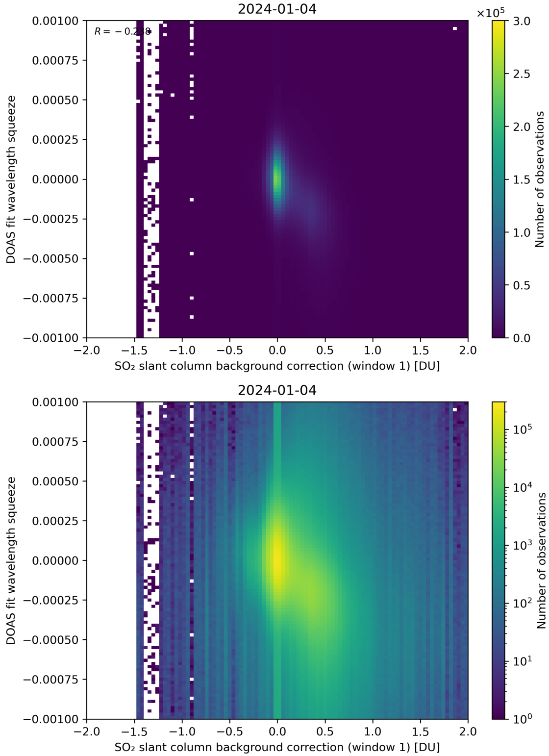
Figure 101: Scatter density plot of “SO 2 slant column background correction (window 1)” against “DOAS fit wavelength squeeze” for 2024-01-03 to 2024-01-05.
