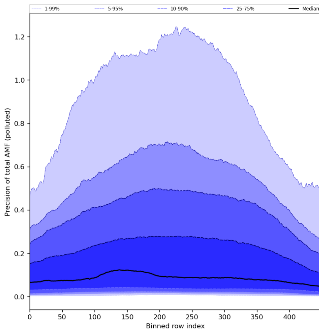
Figure 95: Along track statistics of “Precision of total AMF (polluted)” for 2024-01-03 to 2024-01-05
