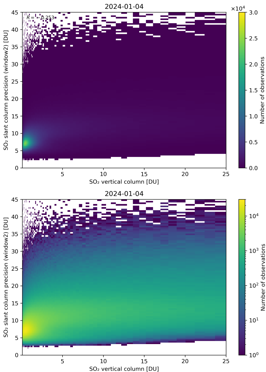
Figure 302: Scatter density plot of “SO 2 vertical column” against “SO 2 slant column precision (window2)” for 2024-01-03 to 2024-01-05.
