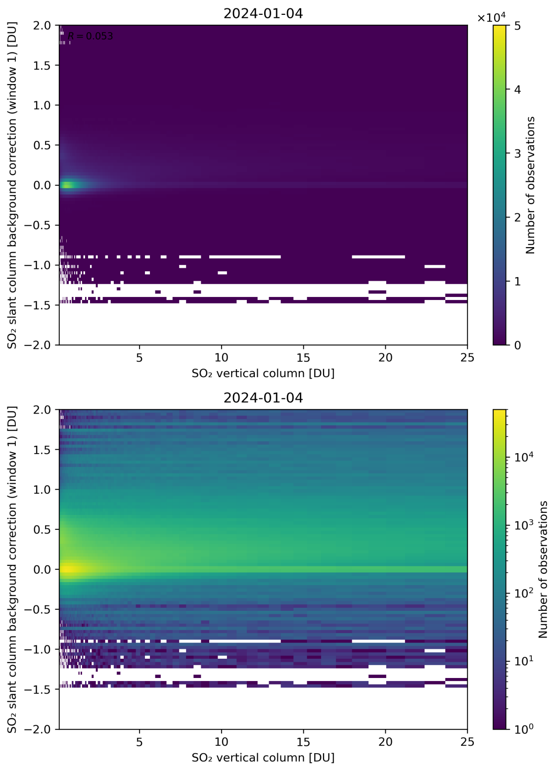
Figure 273: Scatter density plot of “SO 2 vertical column” against “SO 2 slant column background correction (window 1)” for 2024-01-03 to 2024-01-05.
