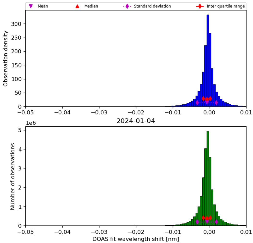
Figure 68: Histogram of “DOAS fit wavelength shift” for 2024-01-03 to 2024-01-05
