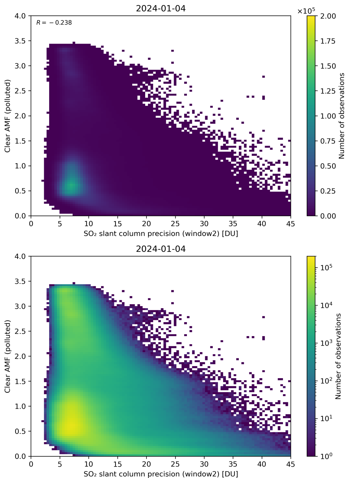
Figure 246: Scatter density plot of “SO 2 slant column precision (window2)” against “Clear AMF (polluted)” for 2024-01-03 to 2024-01-05.
