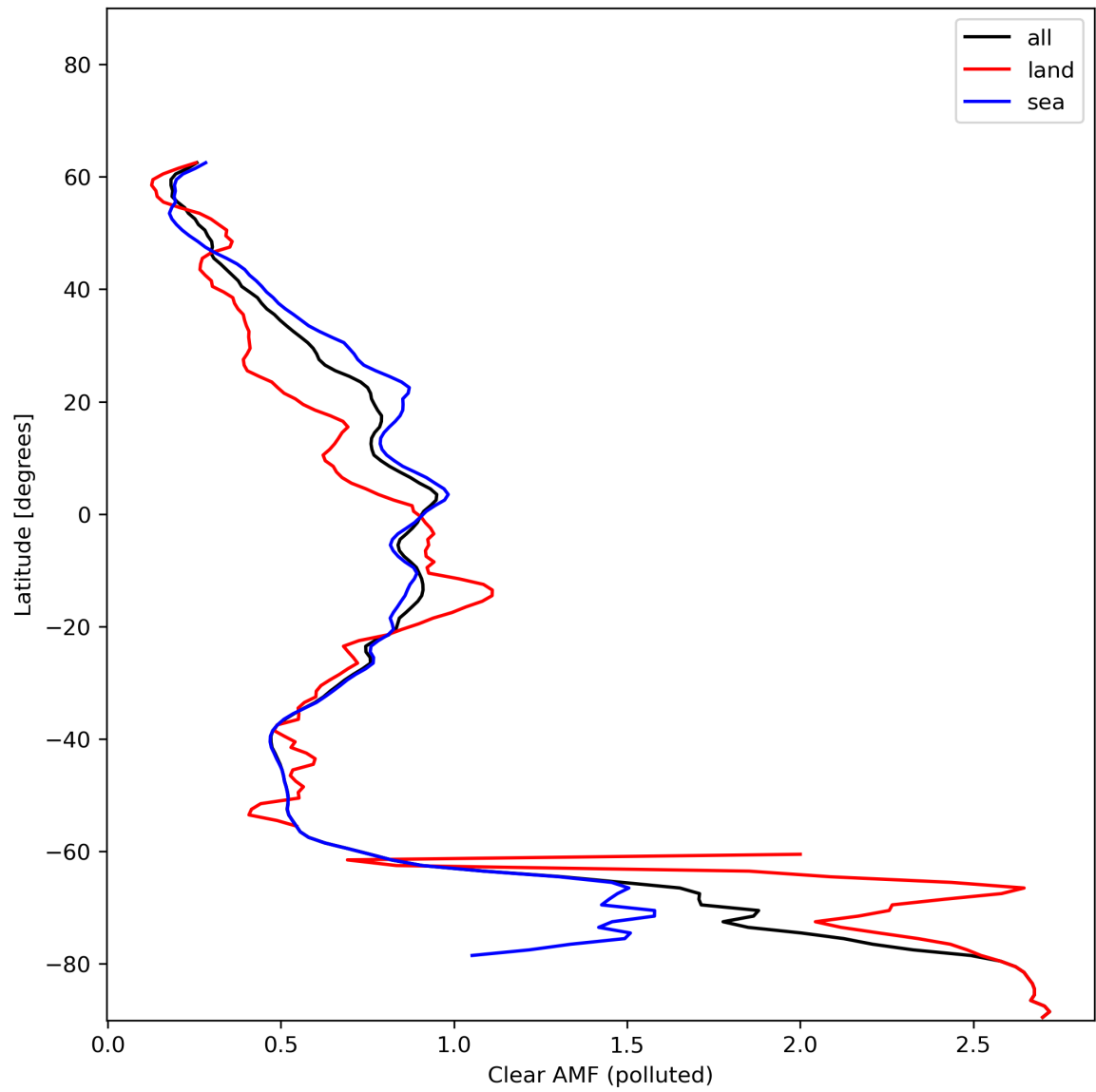
Figure 50: Zonal average of “Clear AMF (polluted)” for 2024-01-03 to 2024-01-05.
