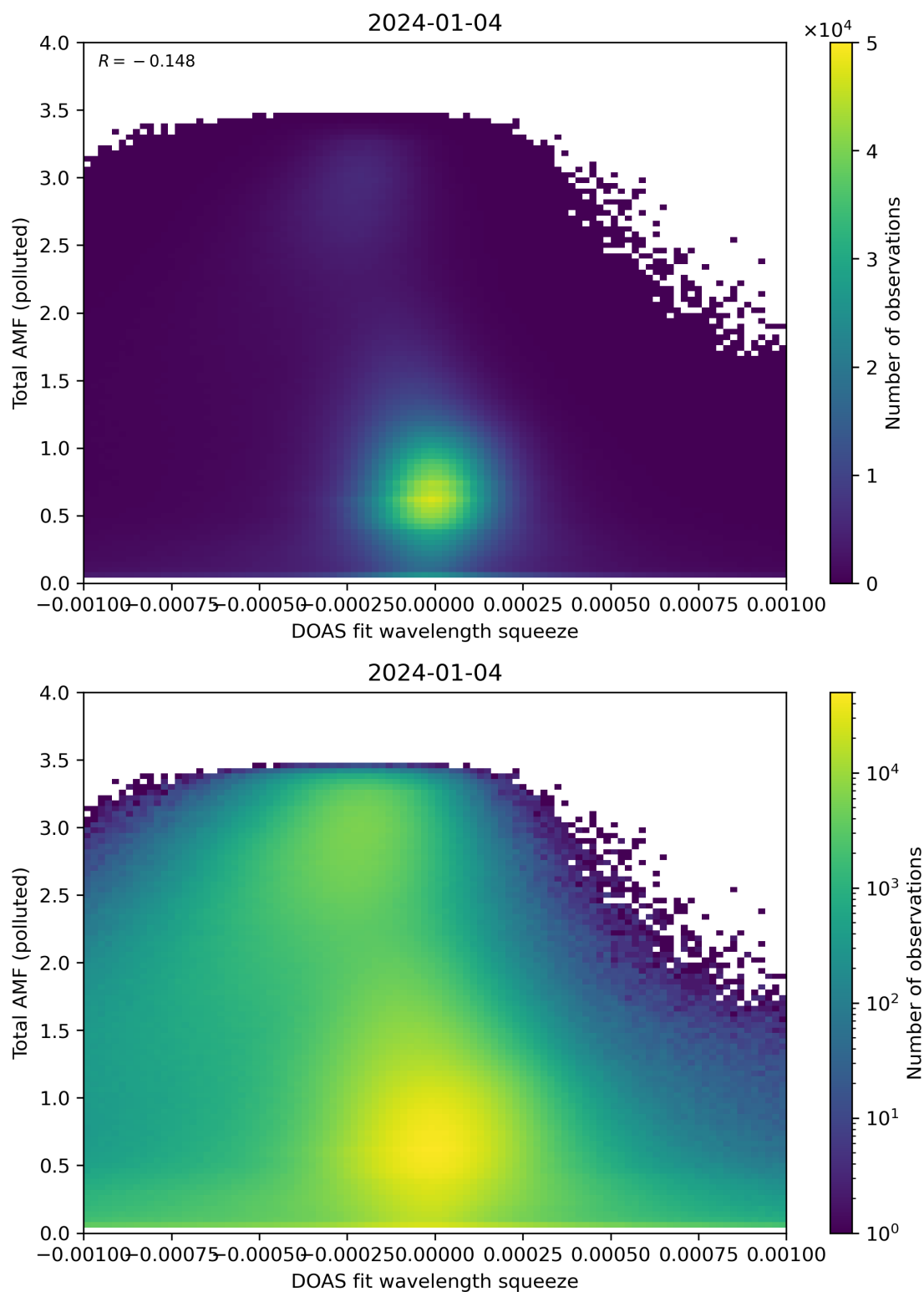
Figure 134: Scatter density plot of “DOAS fit wavelength squeeze” against “Total AMF (polluted)” for 2024-01-03 to 2024-01-05.
