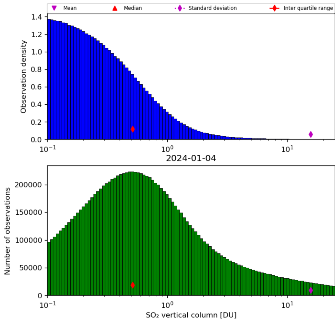
Figure 53: Histogram of “SO 2 vertical column” for 2024-01-03 to 2024-01-05
