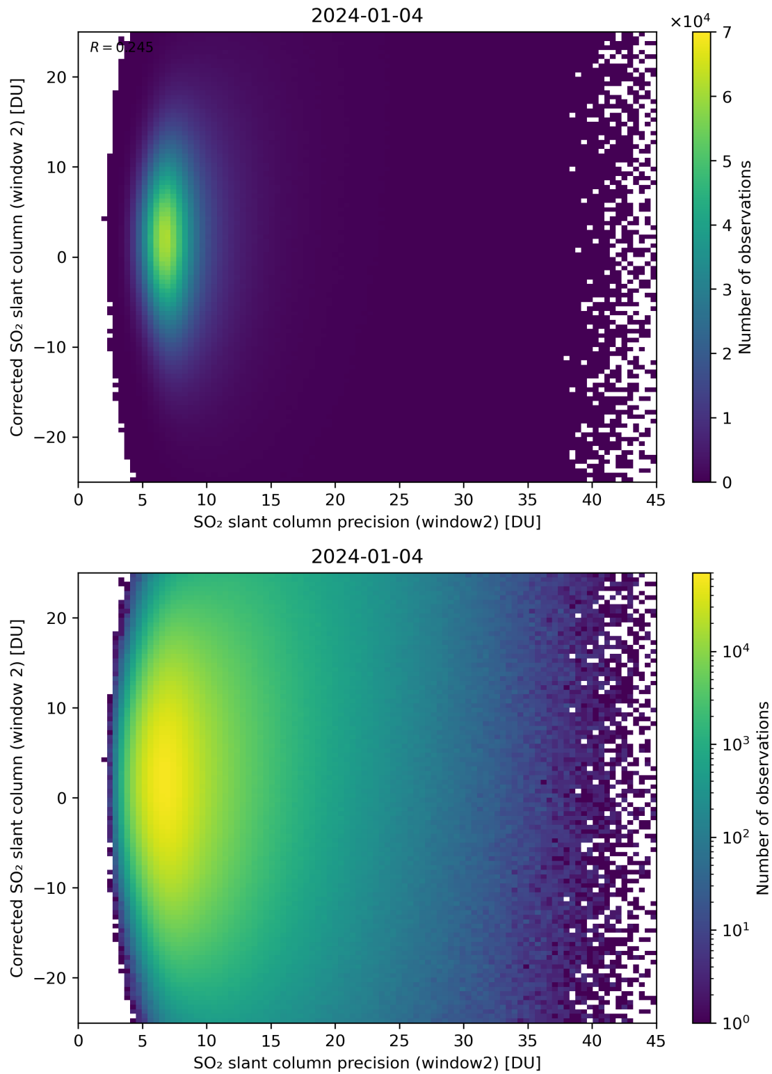
Figure 247: Scatter density plot of “SO 2 slant column precision (window2)” against “Corrected SO 2 slant column (window 2)” for 2024-01-03 to 2024-01-05.
