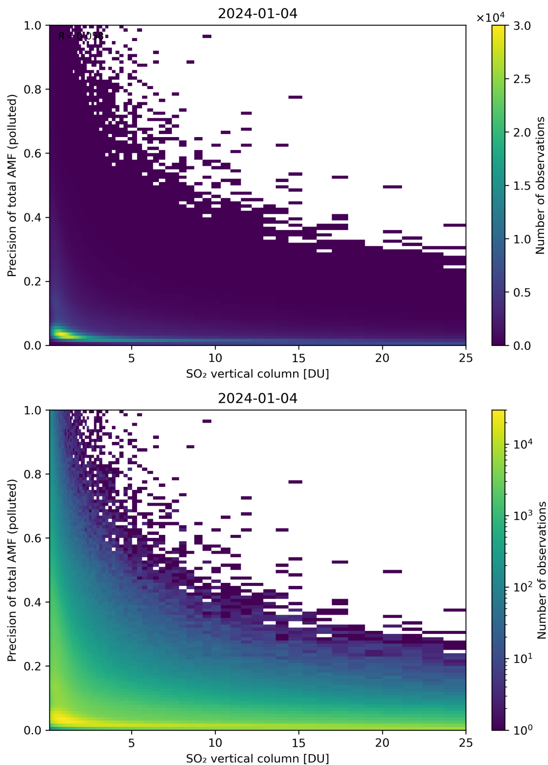
Figure 306: Scatter density plot of “SO 2 vertical column” against “Precision of total AMF (polluted)” for 2024-01-03 to 2024-01-05.
