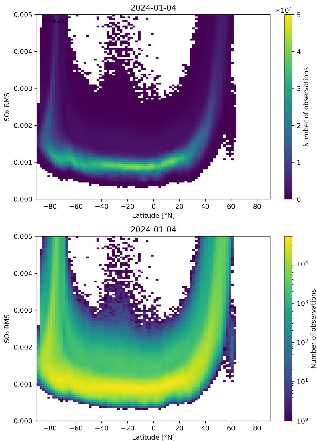
Figure 144: Scatter density plot of “Latitude” against “SO 2 RMS” for 2024-01-03 to 2024-01-05.
