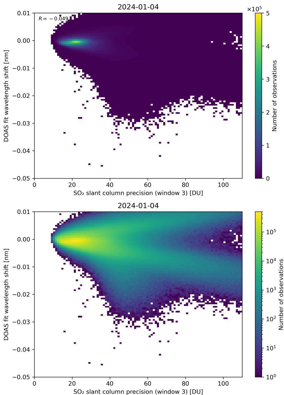
Figure 258: Scatter density plot of “SO 2 slant column precision (window 3)” against “DOAS fit wavelength shift” for 2024-01-03 to 2024-01-05.
