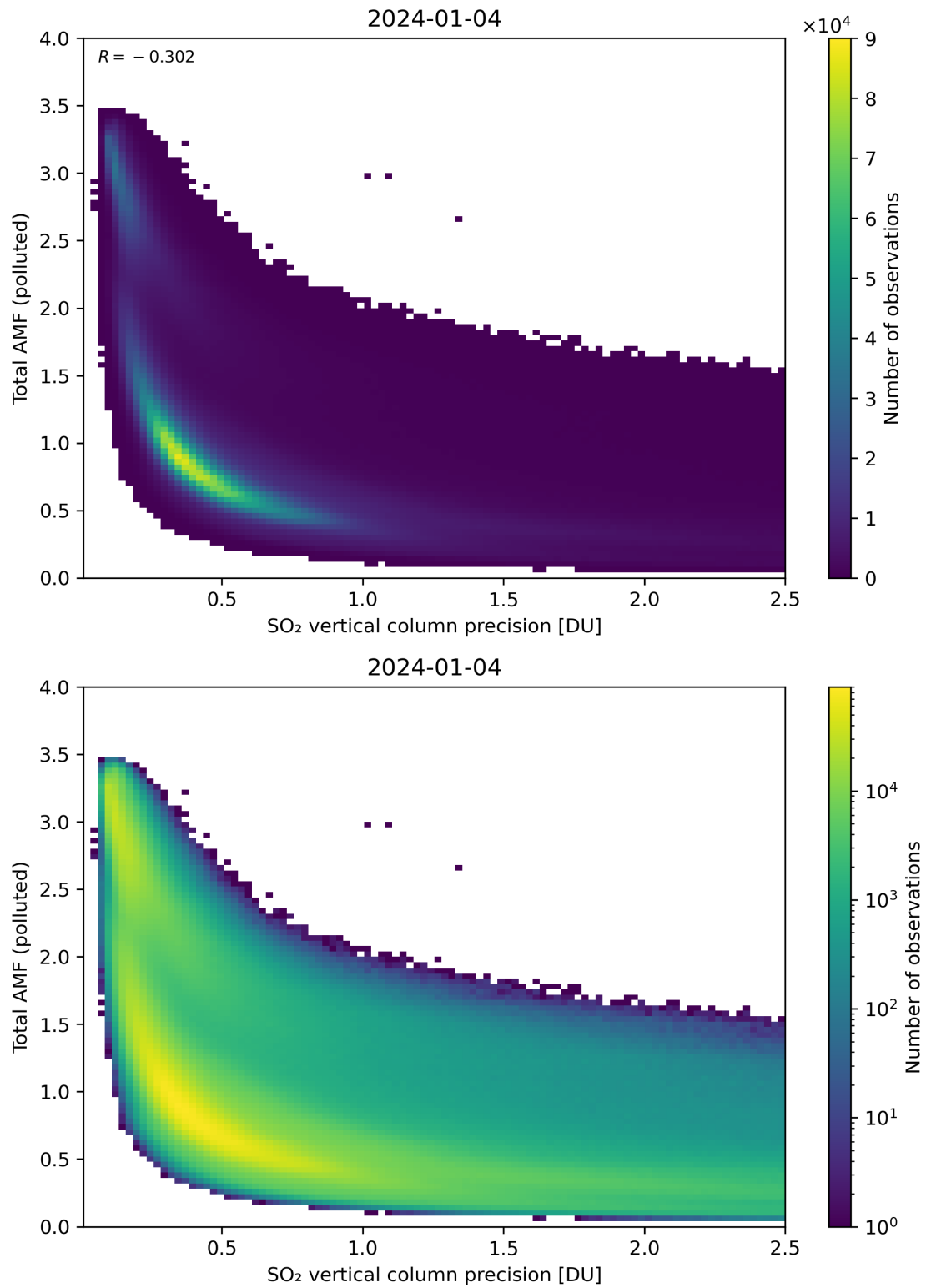
Figure 294: Scatter density plot of “SO 2 vertical column precision” against “Total AMF (polluted)” for 2024-01-03 to 2024-01-05.
