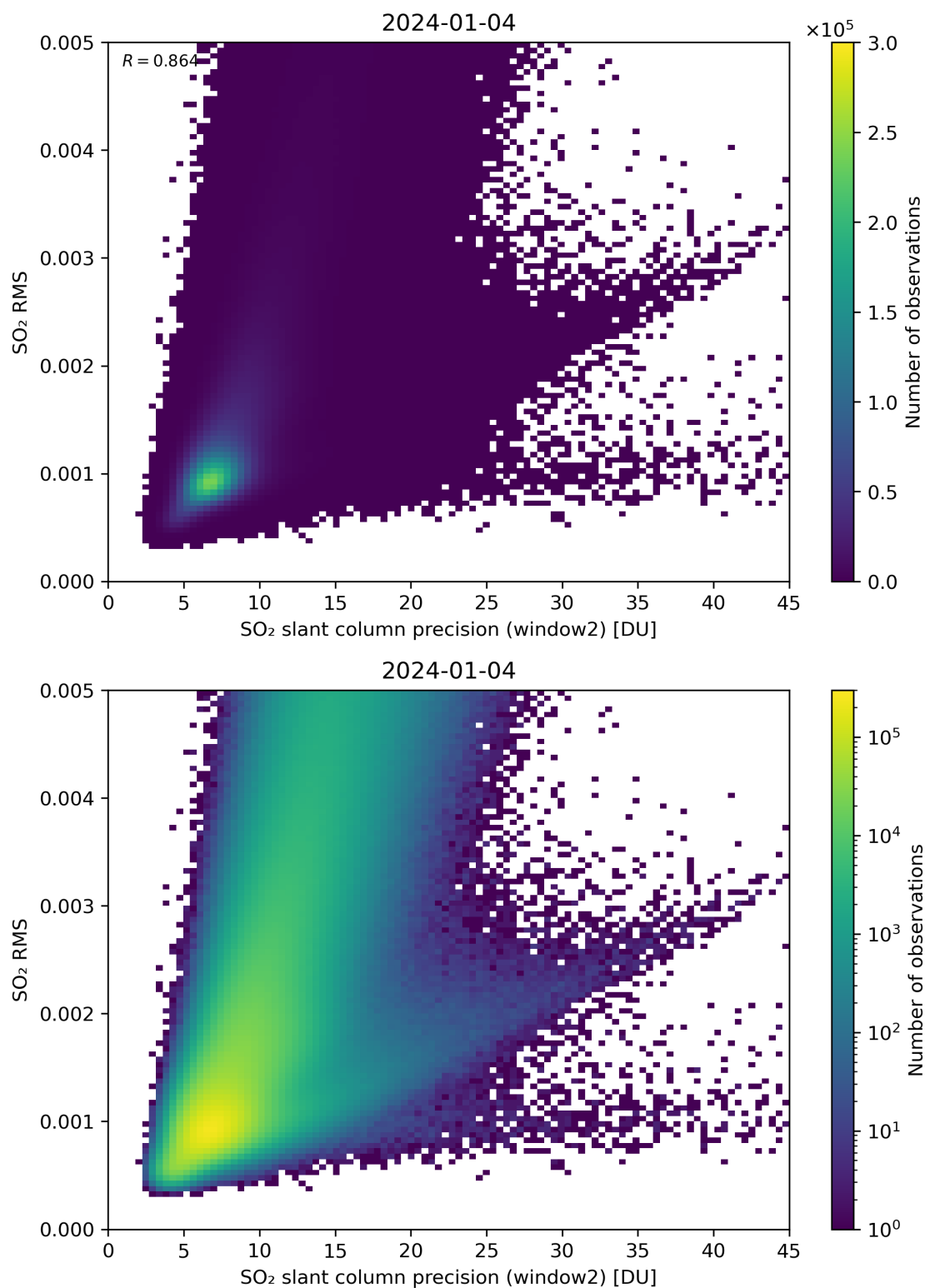
Figure 245: Scatter density plot of “SO 2 slant column precision (window2)” against “SO 2 RMS” for 2024-01-03 to 2024-01-05.
