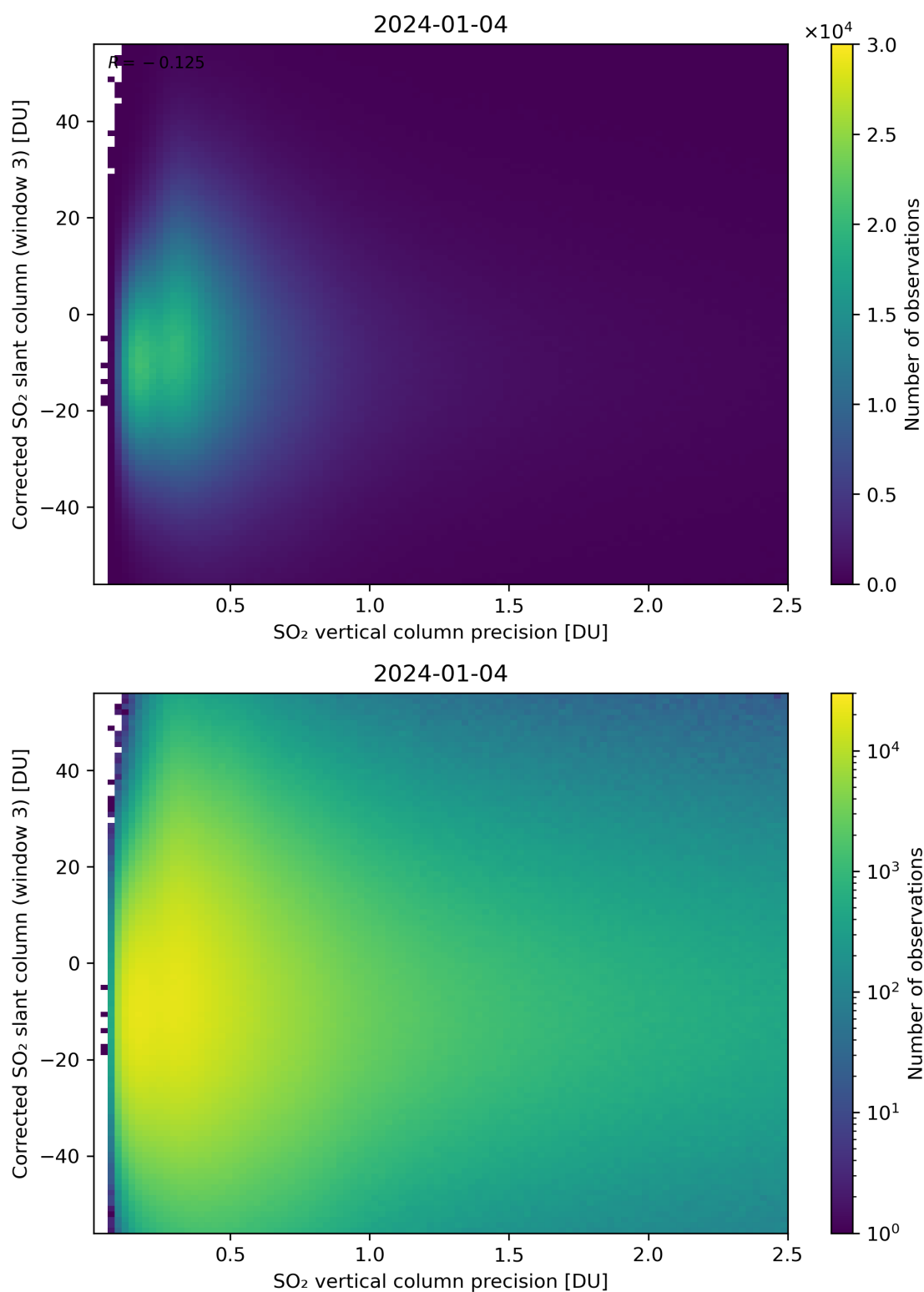
Figure 288: Scatter density plot of “SO 2 vertical column precision” against “Corrected SO 2 slant column (window 3)” for 2024-01-03 to 2024-01-05.
