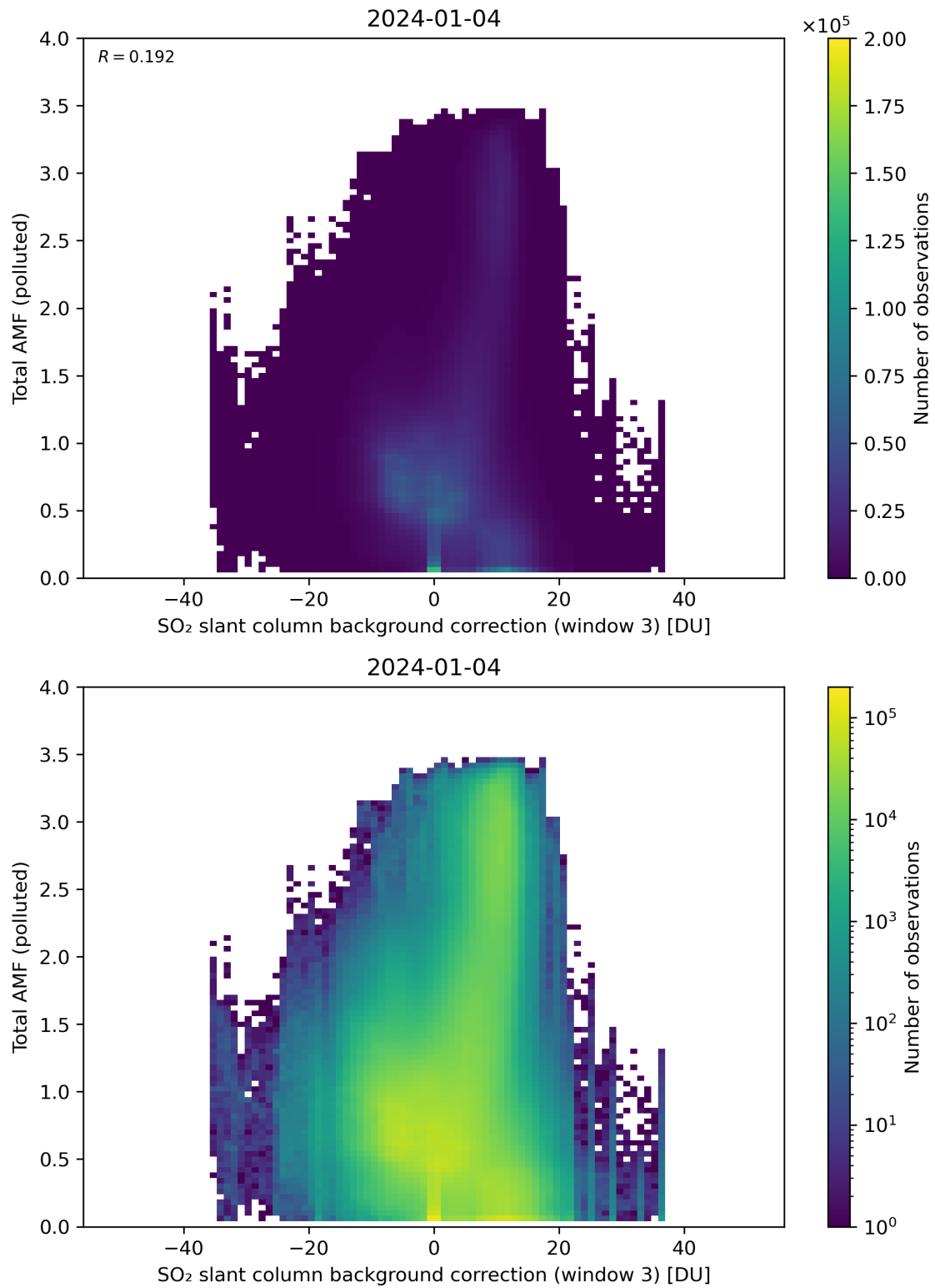
Figure 125: Scatter density plot of “SO 2 slant column background correction (window 3)” against “Total AMF (polluted)” for 2024-01-03 to 2024-01-05.
