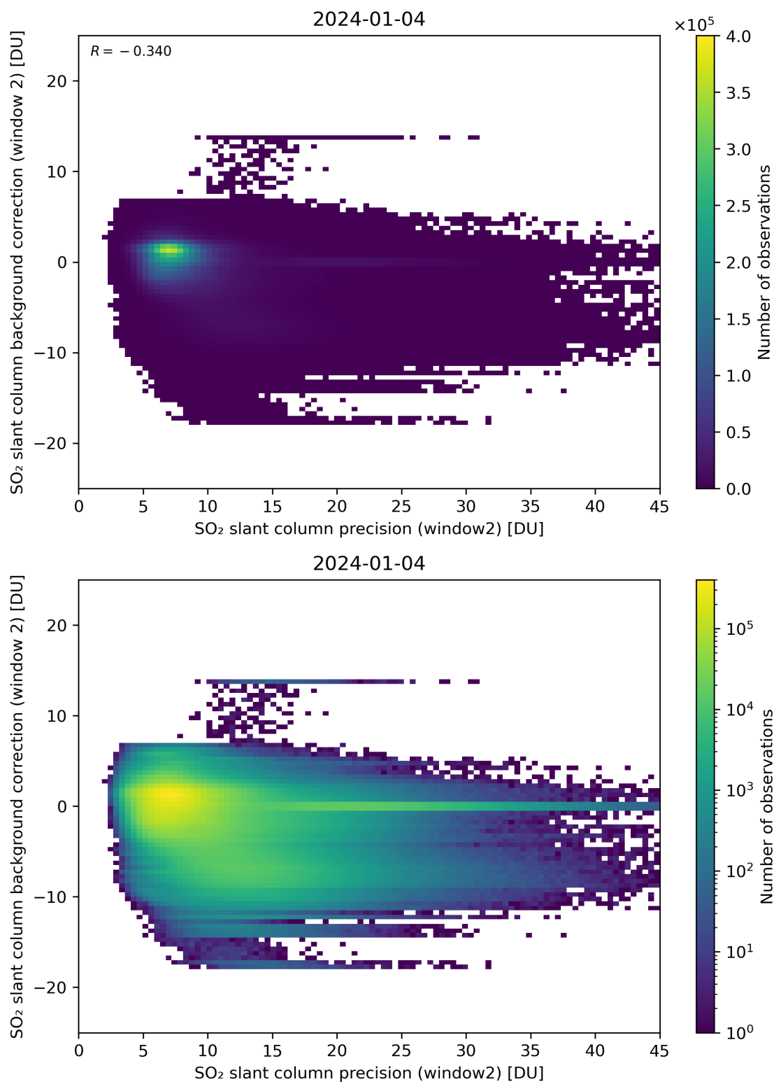
Figure 241: Scatter density plot of “SO 2 slant column precision (window2)” against “SO 2 slant column background correction (window 2)” for 2024-01-03 to 2024-01-05.
