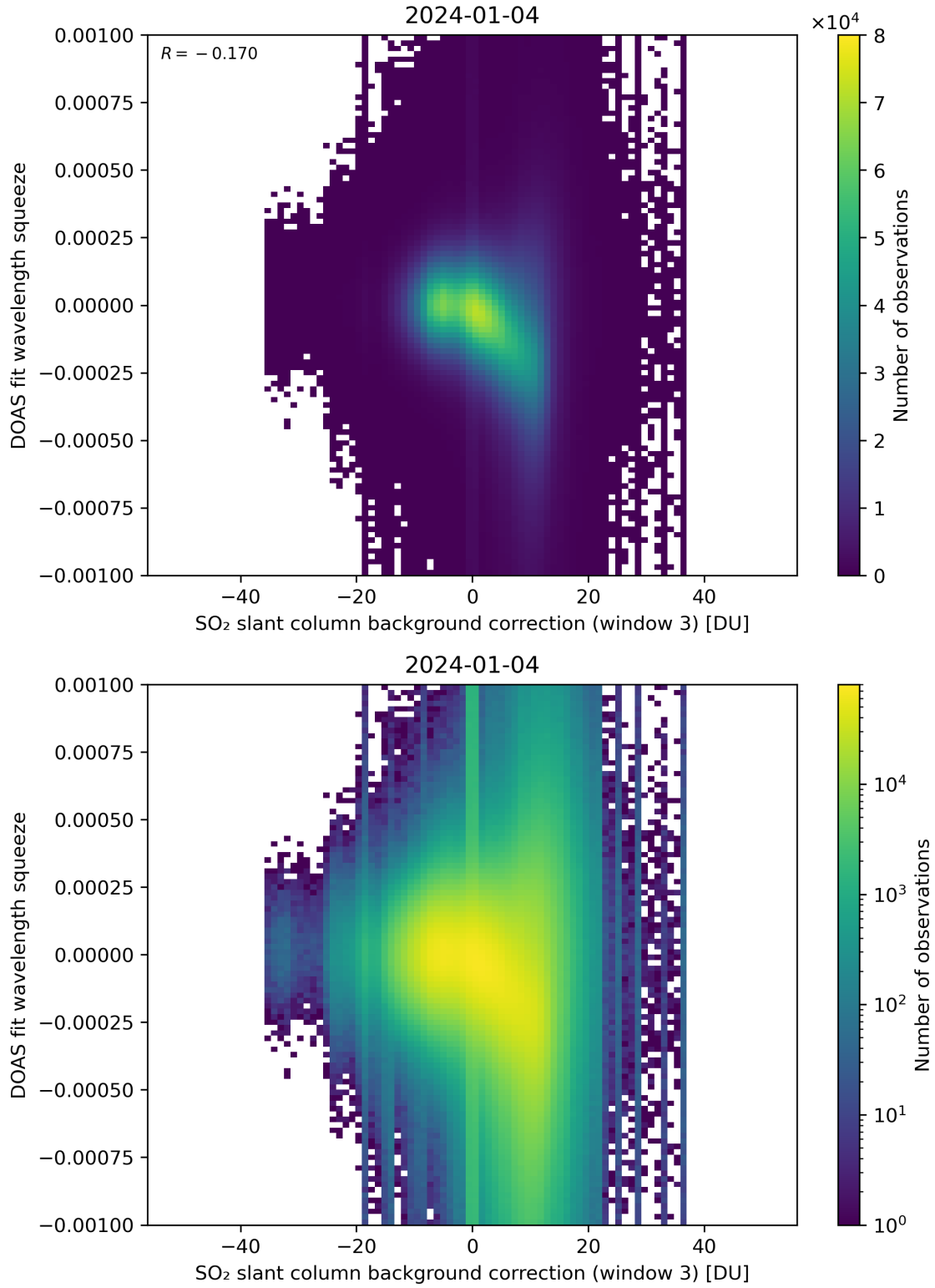
Figure 122: Scatter density plot of “SO 2 slant column background correction (window 3)” against “DOAS fit wavelength squeeze” for 2024-01-03 to 2024-01-05.
