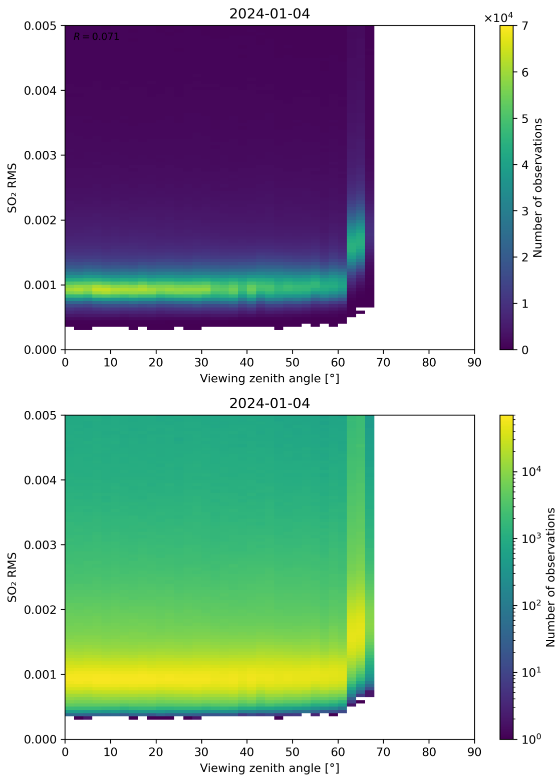
Figure 313: Scatter density plot of “Viewing zenith angle” against “SO 2 RMS” for 2024-01-03 to 2024-01-05.
