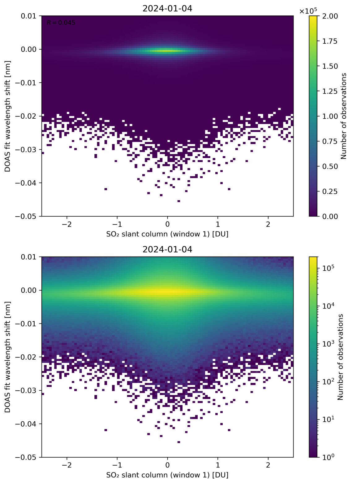
Figure 215: Scatter density plot of “SO 2 slant column (window 1)” against “DOAS fit wavelength shift” for 2024-01-03 to 2024-01-05.
