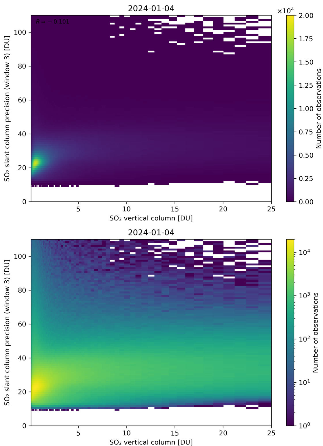
Figure 304: Scatter density plot of “SO 2 vertical column” against “SO 2 slant column precision (window 3)” for 2024-01-03 to 2024-01-05.
