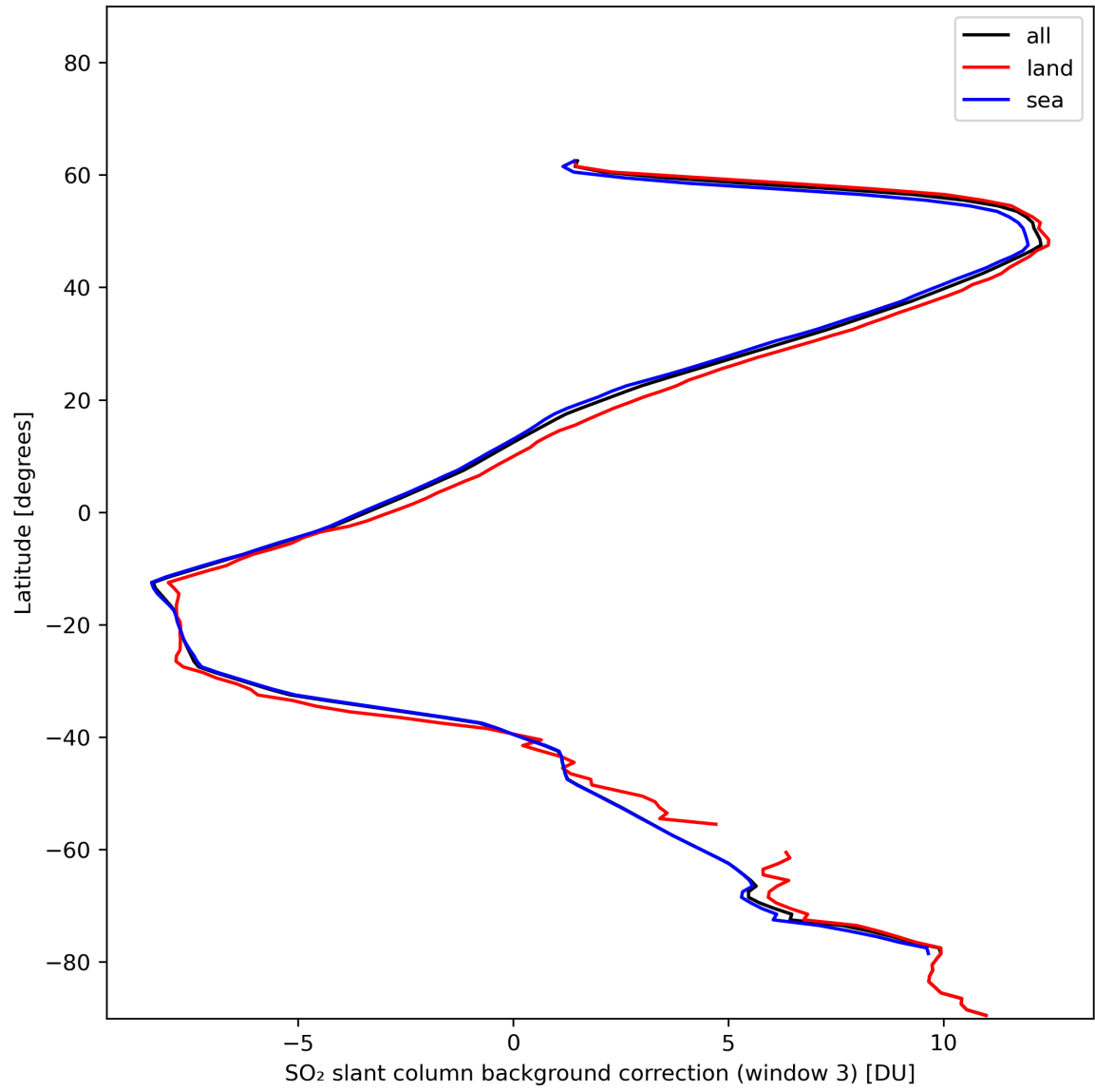
Figure 44: Zonal average of “SO 2 slant column background correction (window 3)” for 2024-01-03 to 2024-01-05.
