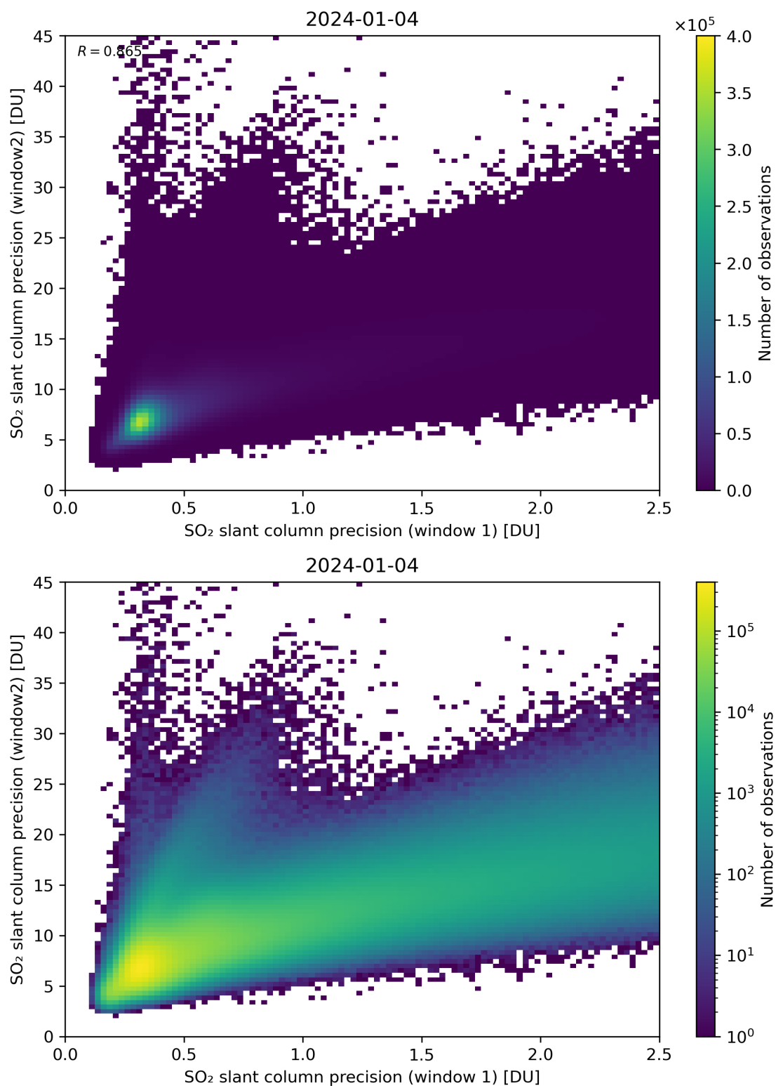
Figure 227: Scatter density plot of “SO 2 slant column precision (window 1)” against “SO 2 slant column precision (window2)” for 2024-01-03 to 2024-01-05.
