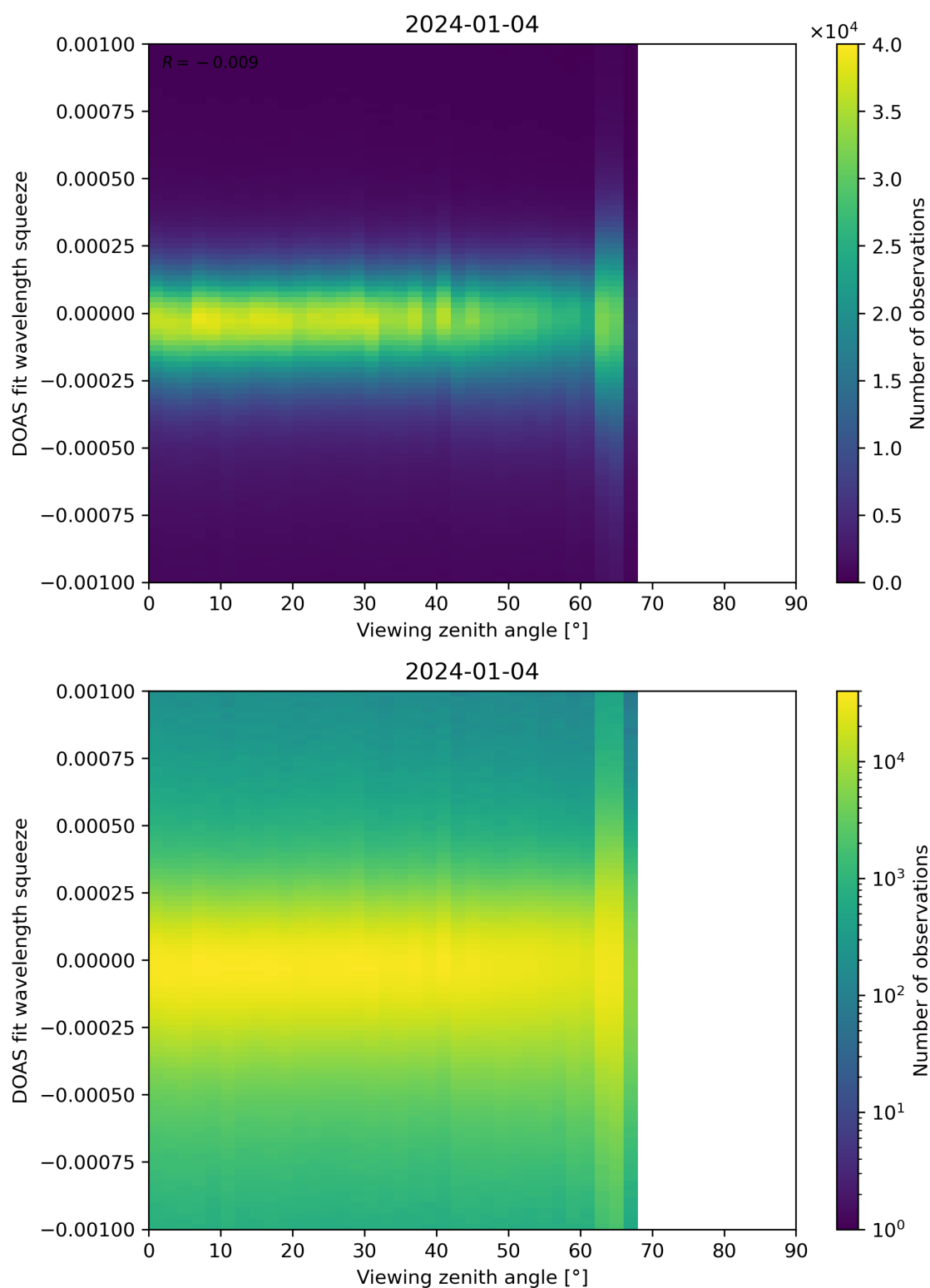
Figure 312: Scatter density plot of “Viewing zenith angle” against “DOAS fit wavelength squeeze” for 2024-01-03 to 2024-01-05.
