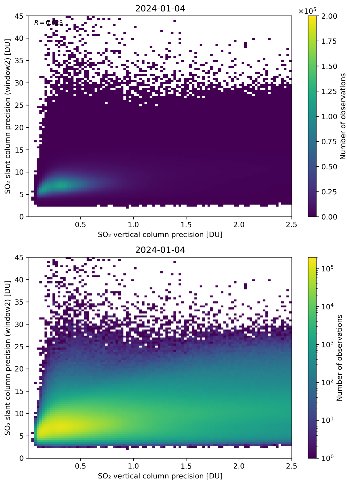
Figure 291: Scatter density plot of “SO 2 vertical column precision” against “SO 2 slant column precision (window2)” for 2024-01-03 to 2024-01-05.
