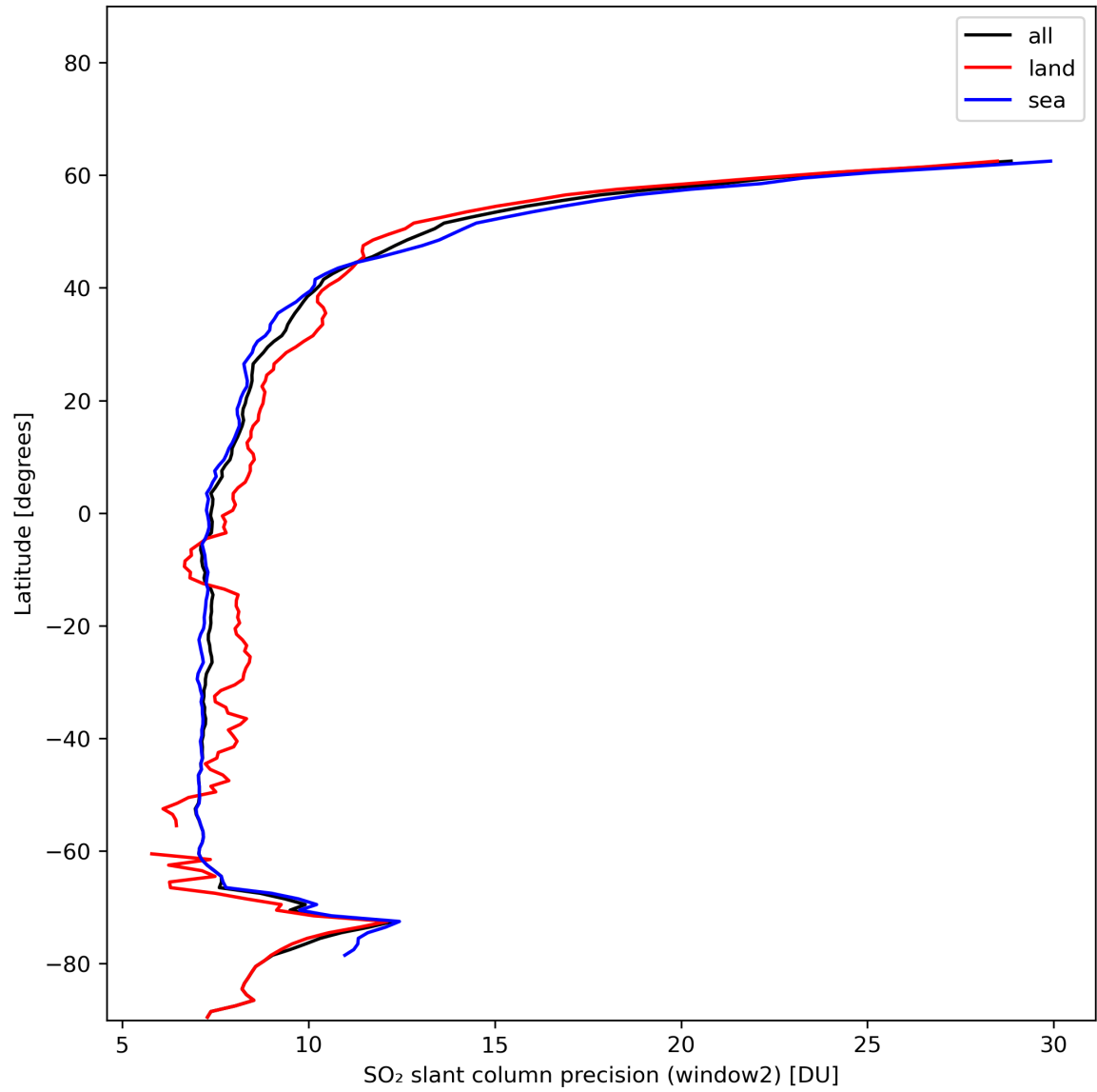
Figure 38: Zonal average of “SO 2 slant column precision (window2)” for 2024-01-03 to 2024-01-05.
