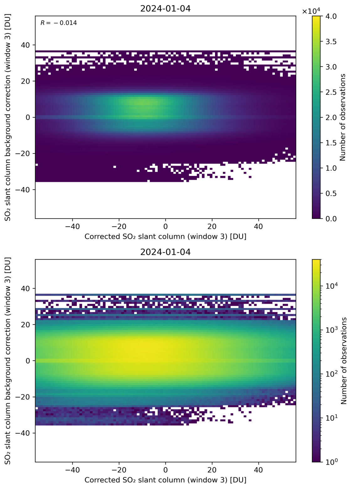
Figure 205: Scatter density plot of “Corrected SO 2 slant column (window 3)” against “SO 2 slant column background correction (window 3)” for 2024-01-03 to 2024-01-05.
