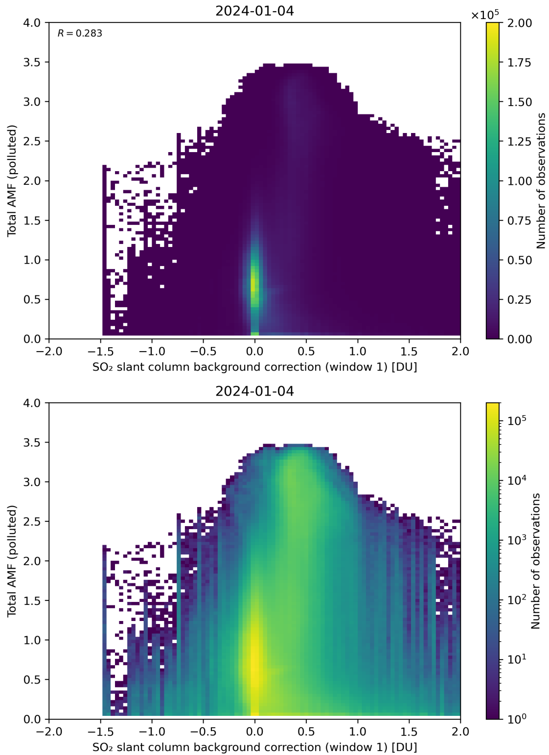
Figure 109: Scatter density plot of “SO 2 slant column background correction (window 1)” against “Total AMF (polluted)” for 2024-01-03 to 2024-01-05.
