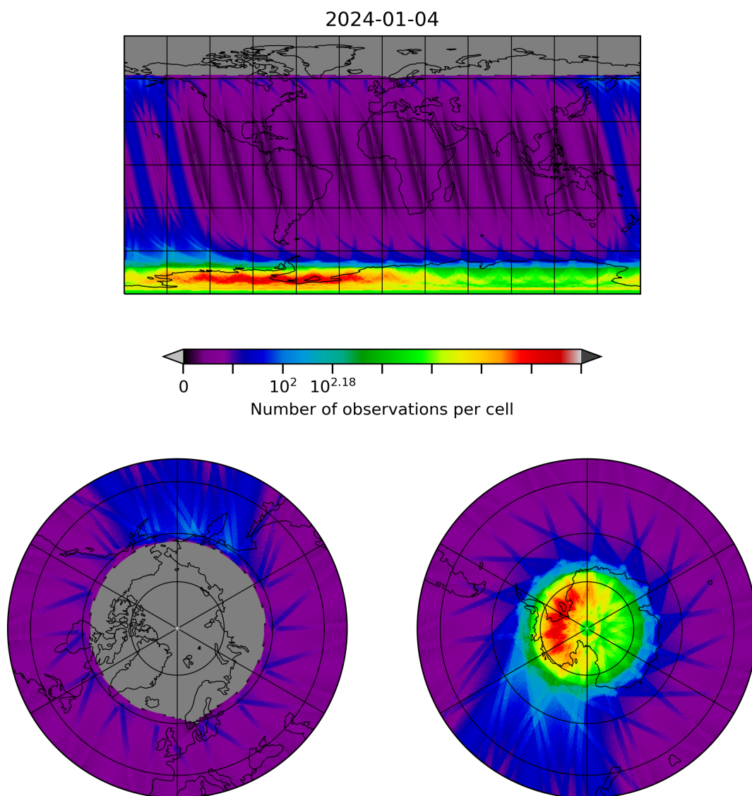
Figure 28: Map of the number of observations for 2024-01-03 to 2024-01-05
