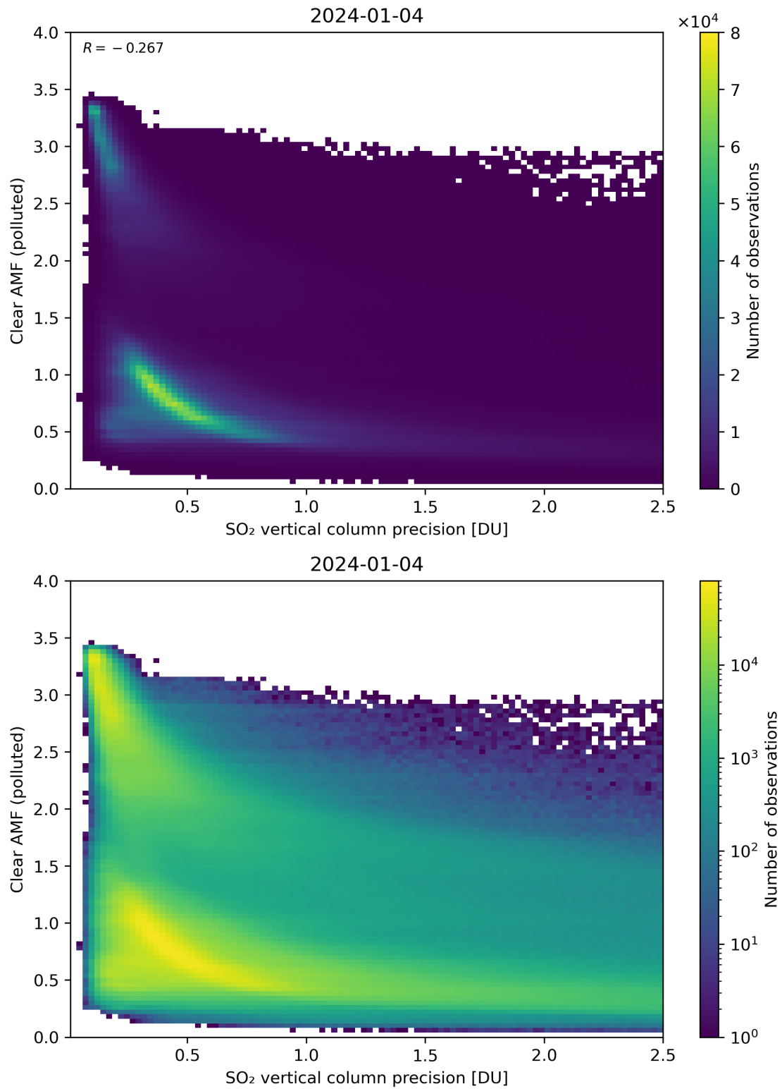
Figure 285: Scatter density plot of “SO 2 vertical column precision” against “Clear AMF (polluted)” for 2024-01-03 to 2024-01-05.
