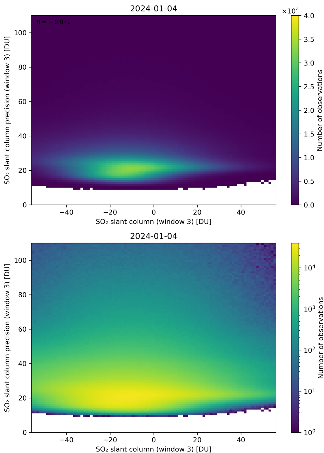
Figure 267: Scatter density plot of “SO 2 slant column (window 3)” against “SO 2 slant column precision (window 3)” for 2024-01-03 to 2024-01-05.
