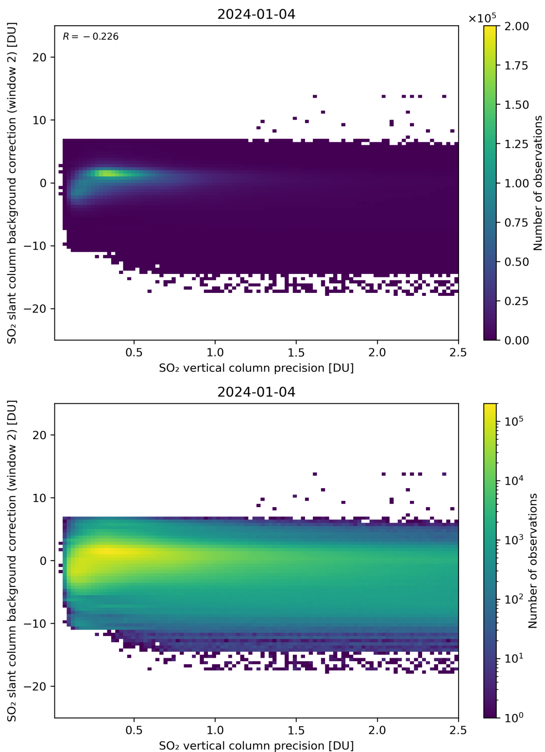
Figure 280: Scatter density plot of “SO 2 vertical column precision” against “SO 2 slant column background correction (window 2)” for 2024-01-03 to 2024-01-05.
