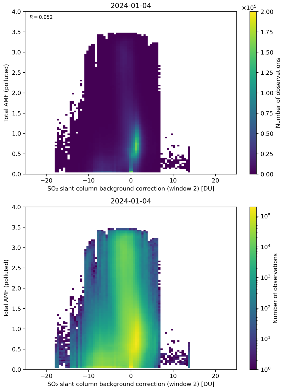
Figure 119: Scatter density plot of “SO 2 slant column background correction (window 2)” against “Total AMF (polluted)” for 2024-01-03 to 2024-01-05.
