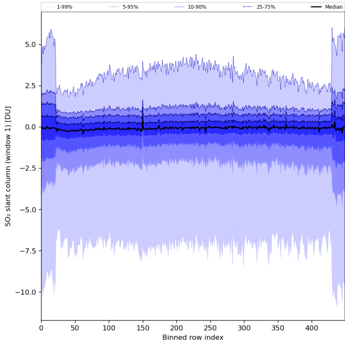
Figure 79: Along track statistics of “SO 2 slant column (window 1)” for 2024-01-03 to 2024-01-05
