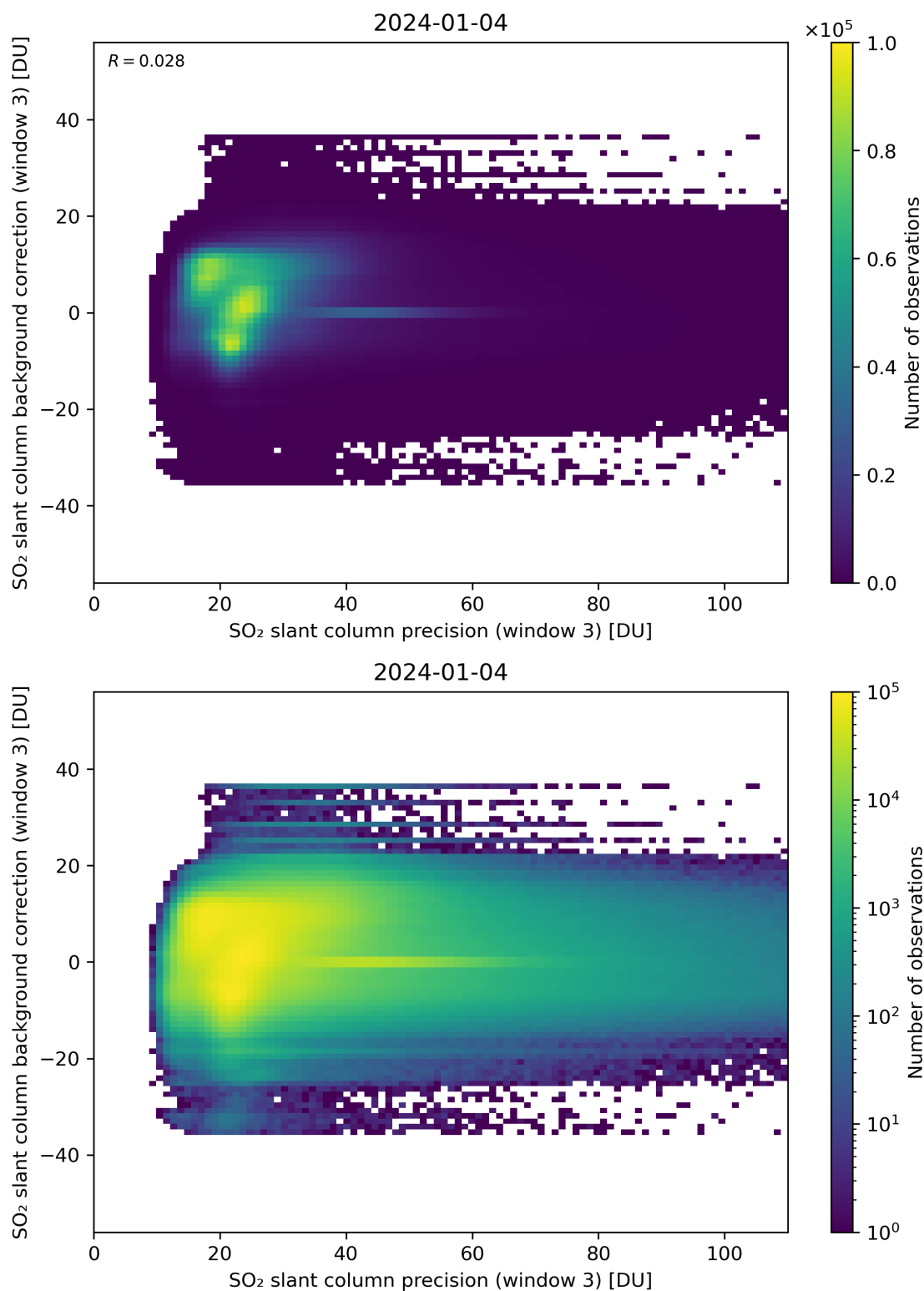
Figure 257: Scatter density plot of “SO 2 slant column precision (window 3)” against “SO 2 slant column background correction (window 3)” for 2024-01-03 to 2024-01-05.
