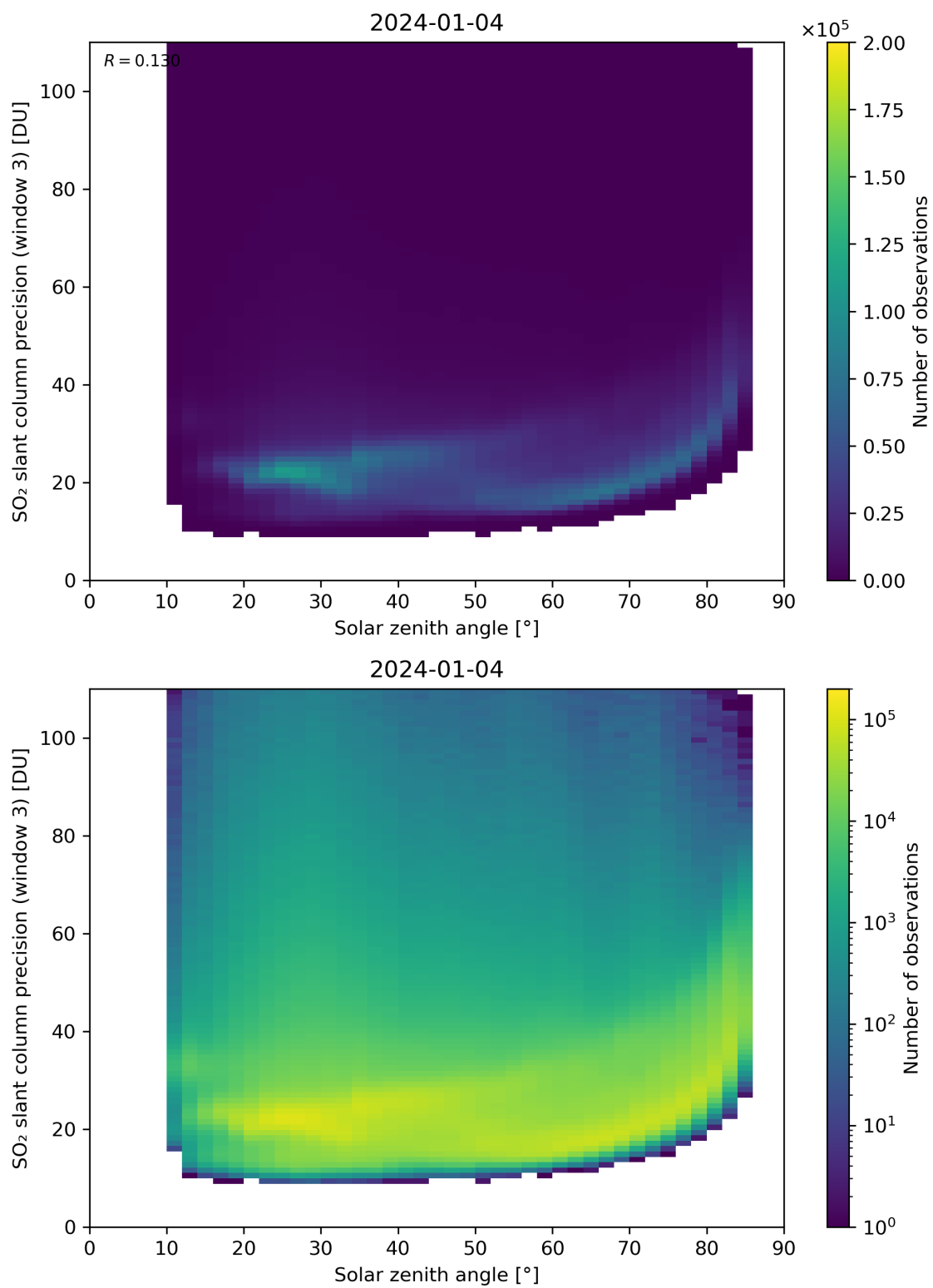
Figure 173: Scatter density plot of “Solar zenith angle” against “SO 2 slant column precision (window 3)” for 2024-01-03 to 2024-01-05.
