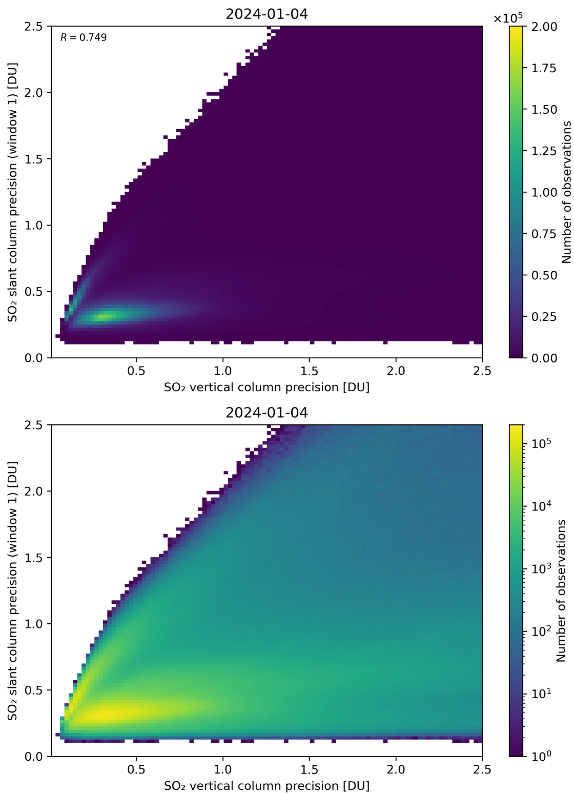
Figure 290: Scatter density plot of “SO 2 vertical column precision” against “SO 2 slant column precision (window 1)” for 2024-01-03 to 2024-01-05.
