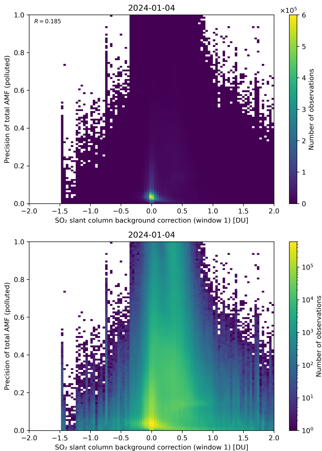
Figure 110: Scatter density plot of “SO 2 slant column background correction (window 1)” against “Precision of total AMF (polluted)” for 2024-01-03 to 2024-01-05.
