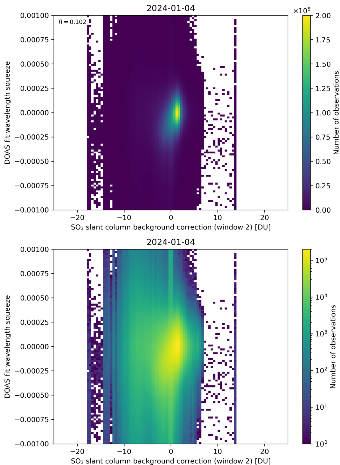
Figure 113: Scatter density plot of “SO 2 slant column background correction (window 2)” against “DOAS fit wavelength squeeze” for 2024-01-03 to 2024-01-05.
