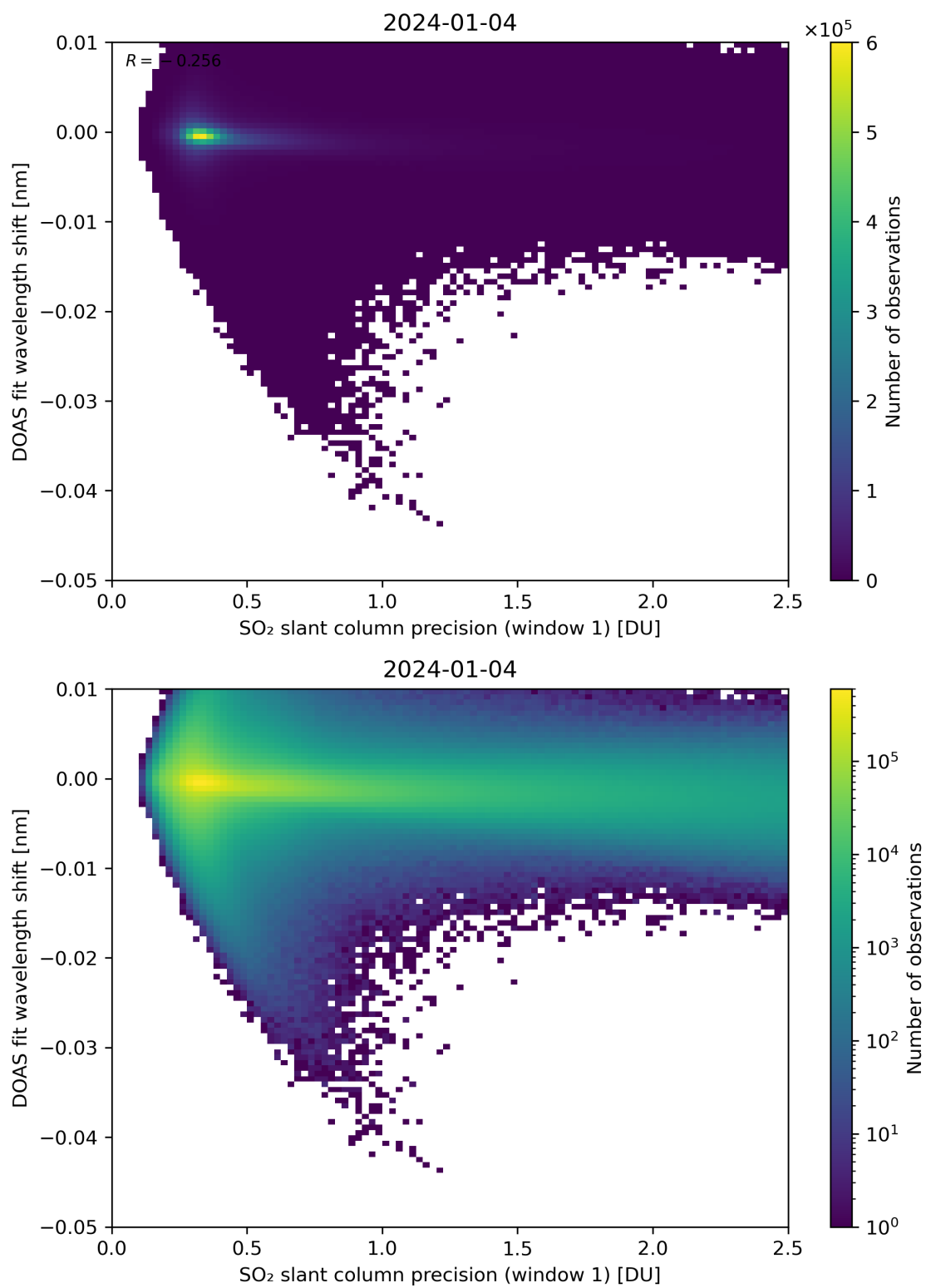
Figure 221: Scatter density plot of “SO 2 slant column precision (window 1)” against “DOAS fit wavelength shift” for 2024-01-03 to 2024-01-05.
