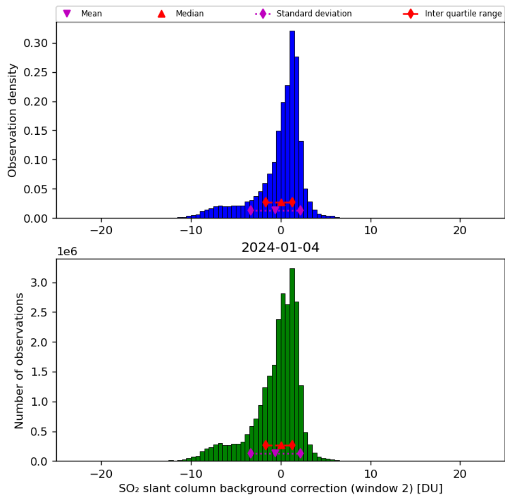
Figure 63: Histogram of “SO 2 slant column background correction (window 2)” for 2024-01-03 to 2024-01-05
