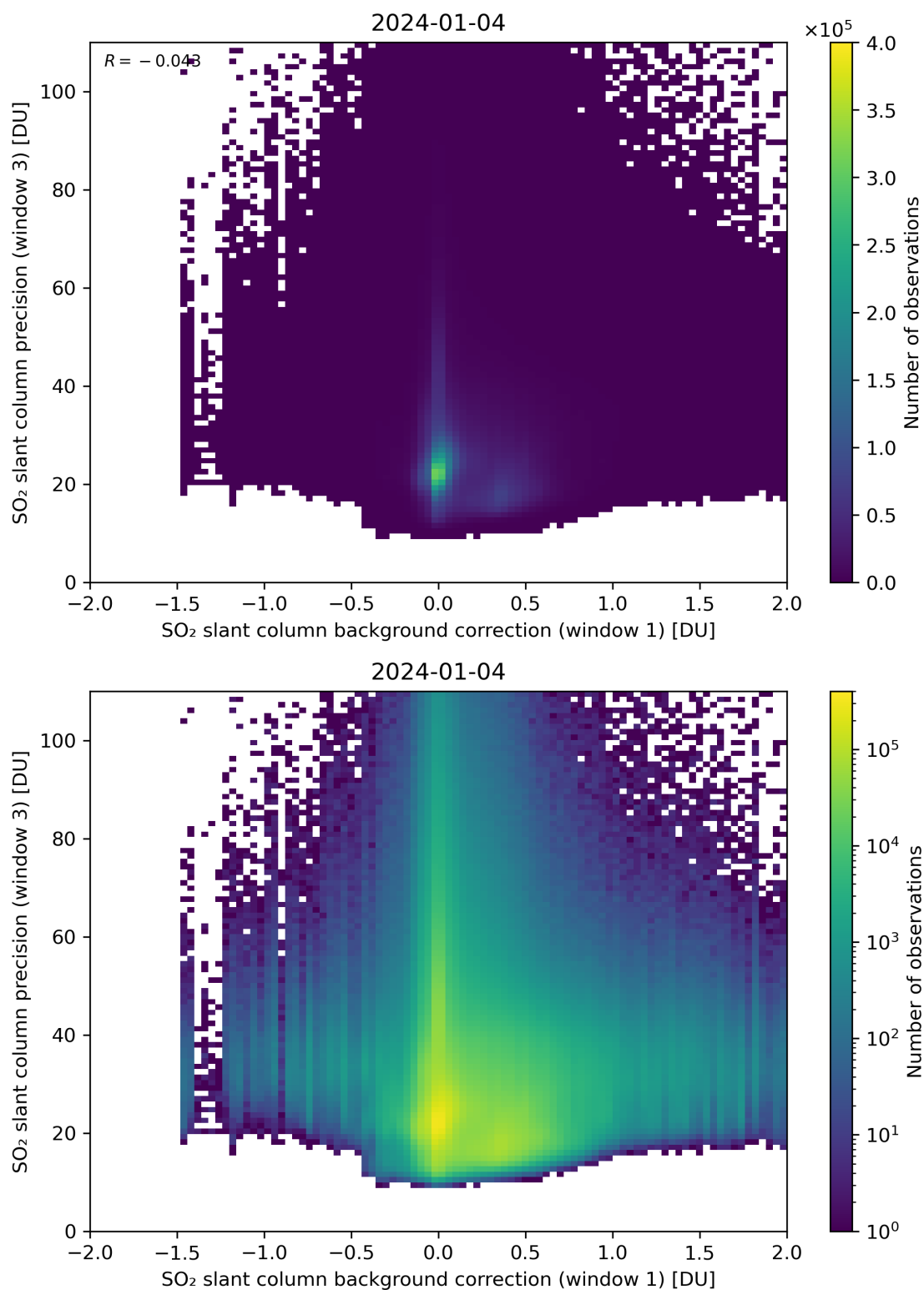
Figure 108: Scatter density plot of “SO 2 slant column background correction (window 1)” against “SO 2 slant column precision (window 3)” for 2024-01-03 to 2024-01-05.
