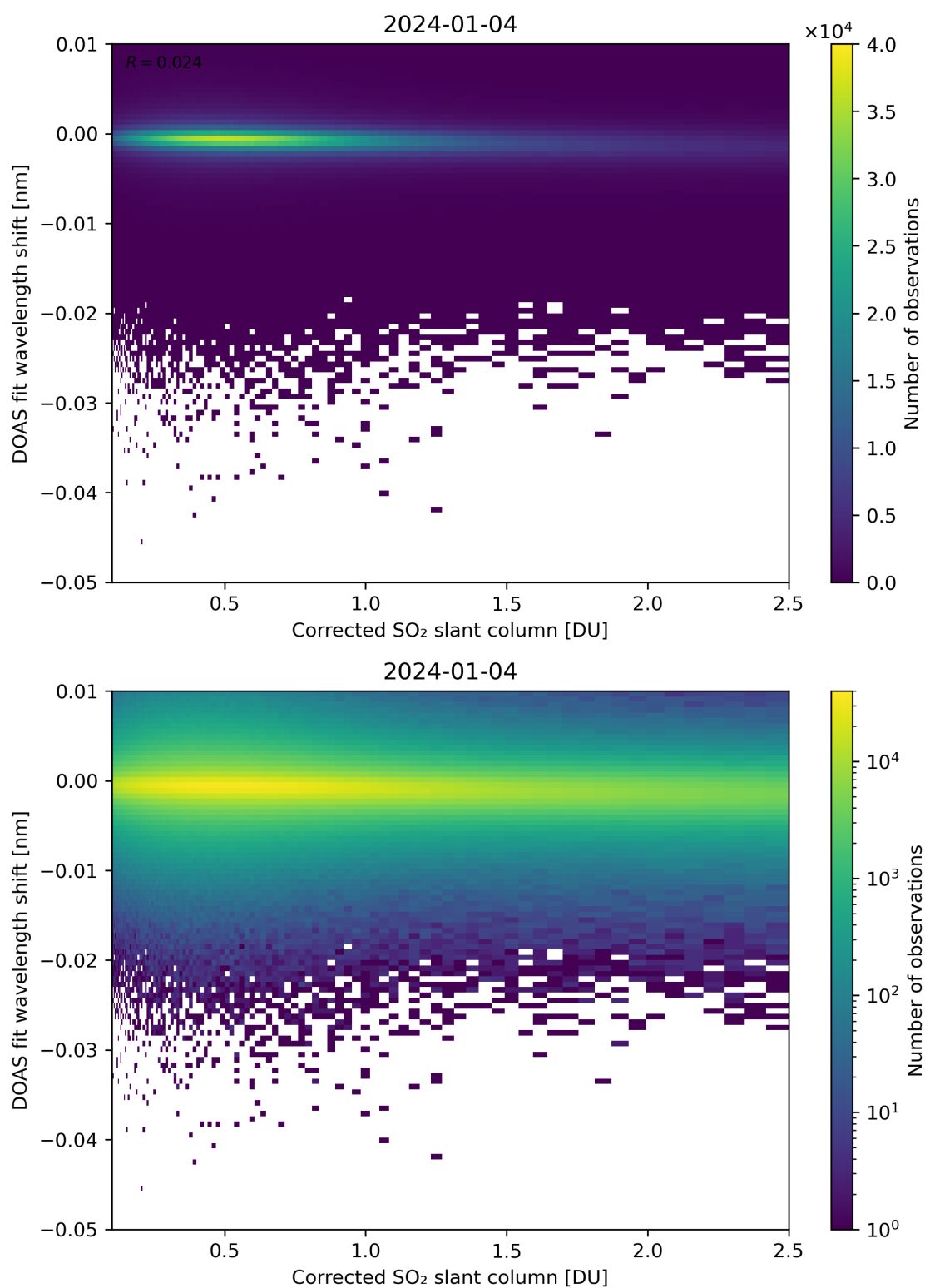
Figure 181: Scatter density plot of “Corrected SO 2 slant column” against “DOAS fit wavelength shift” for 2024-01-03 to 2024-01-05.
