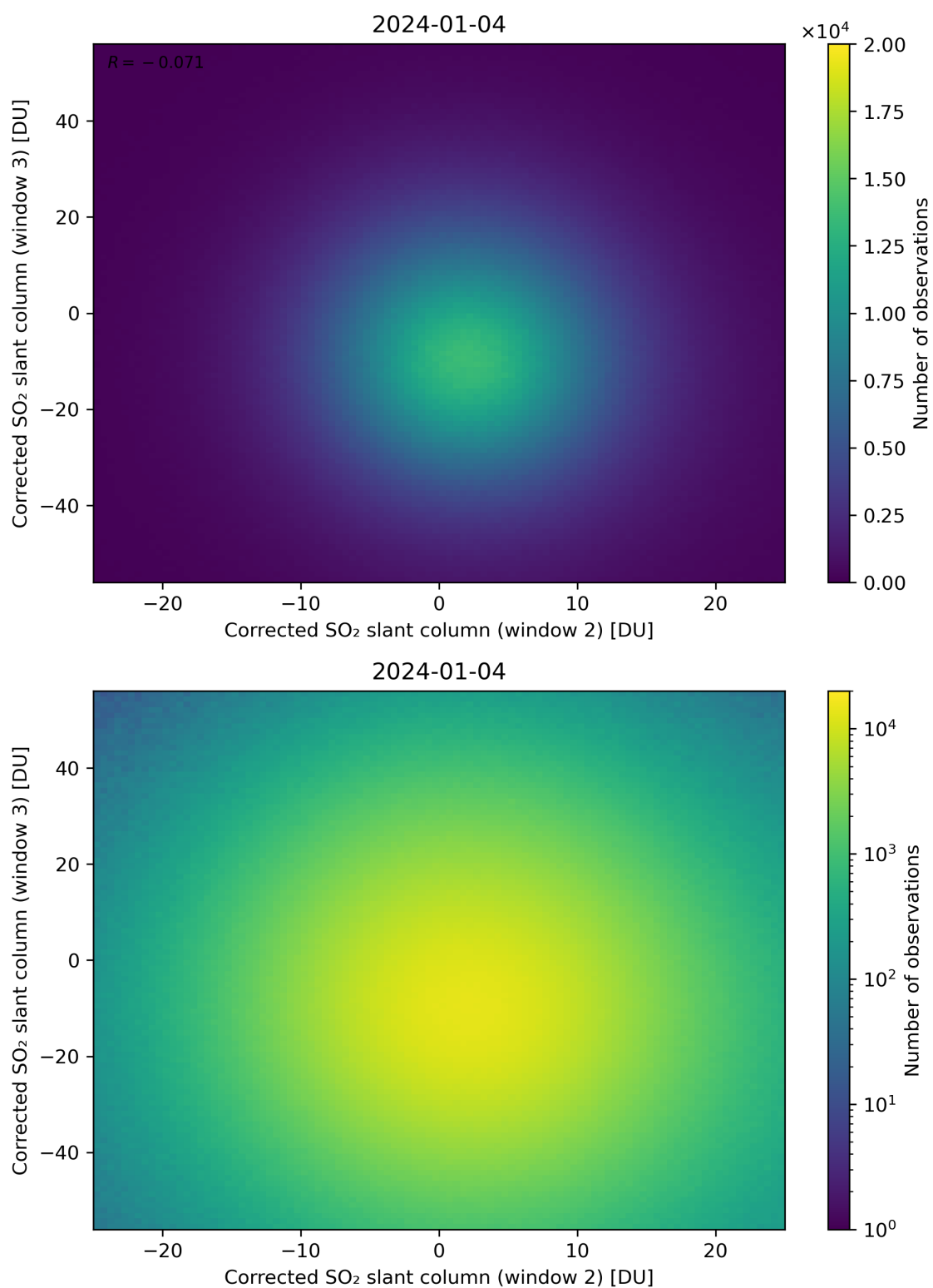
Figure 200: Scatter density plot of “Corrected SO 2 slant column (window 2)” against “Corrected SO 2 slant column (window 3)” for 2024-01-03 to 2024-01-05.
