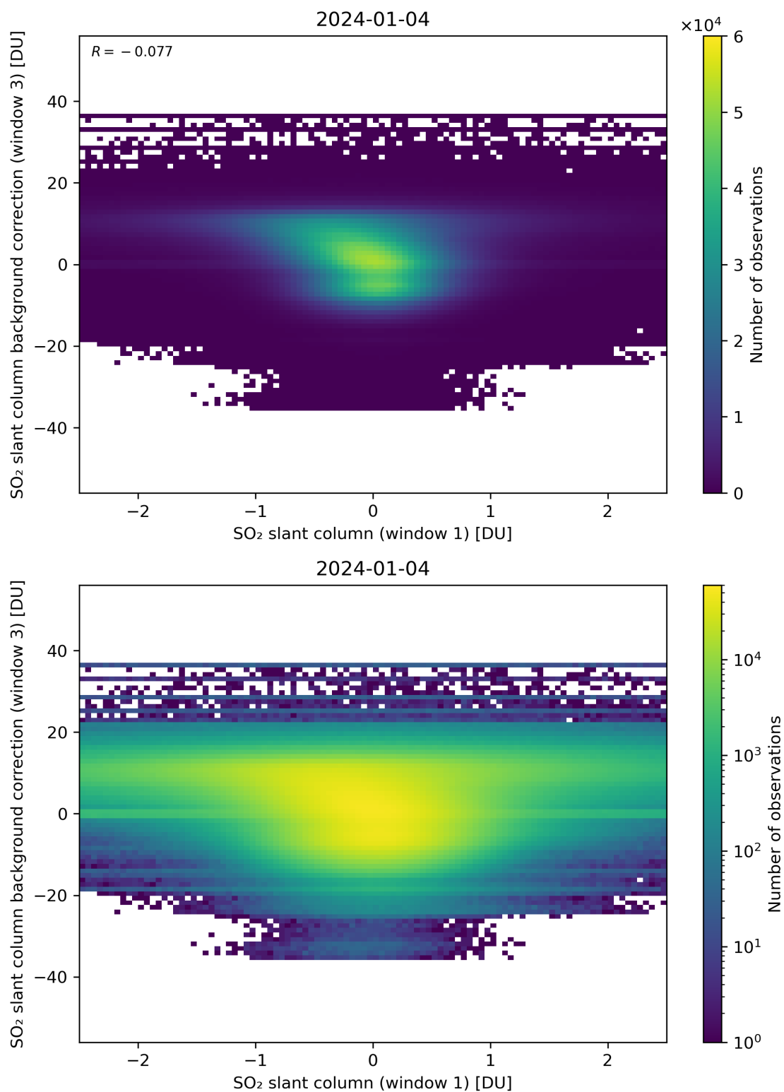
Figure 214: Scatter density plot of “SO 2 slant column (window 1)” against “SO 2 slant column background correction (window 3)” for 2024-01-03 to 2024-01-05.
