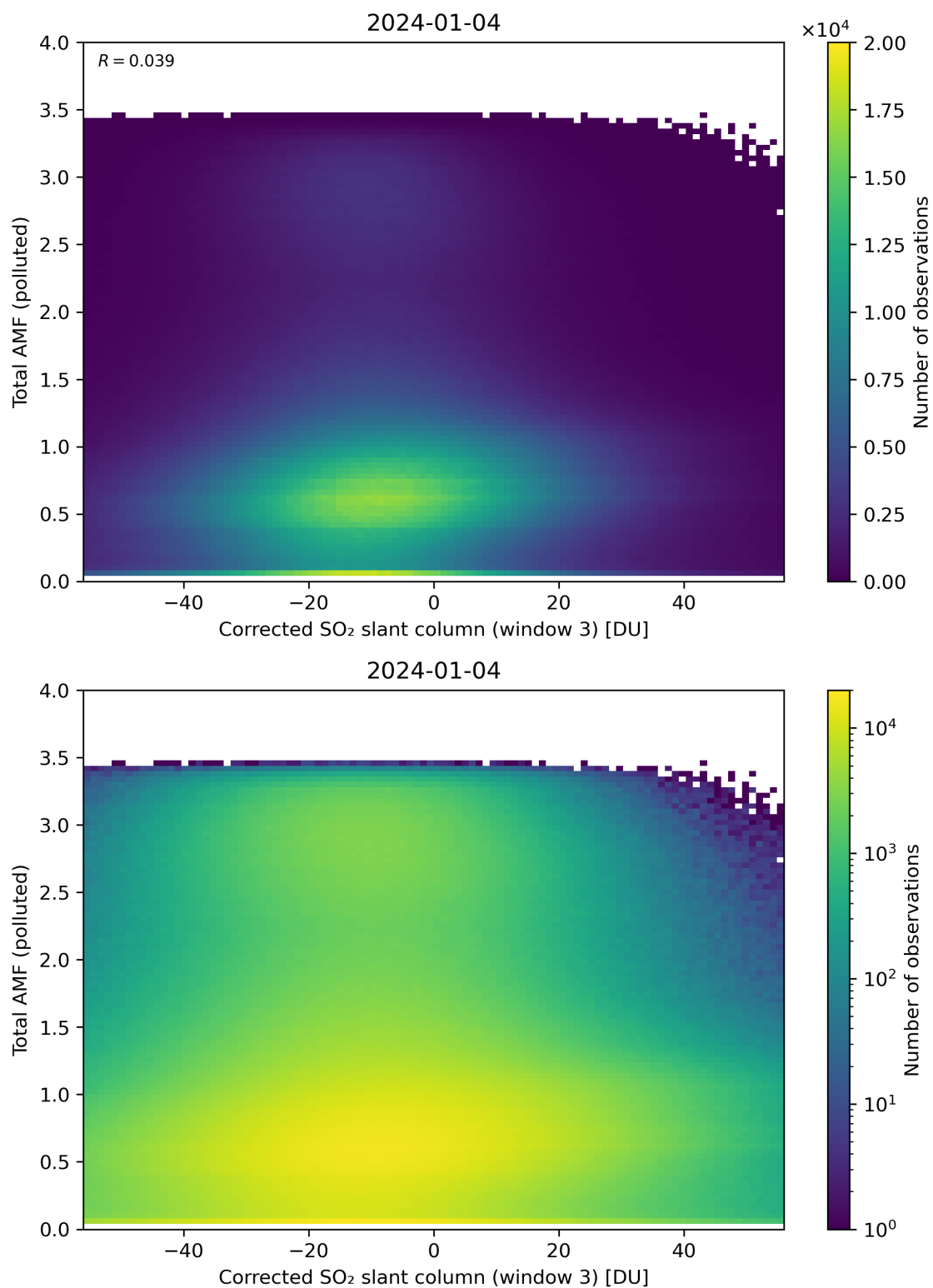
Figure 210: Scatter density plot of “Corrected SO 2 slant column (window 3)” against “Total AMF (polluted)” for 2024-01-03 to 2024-01-05.
