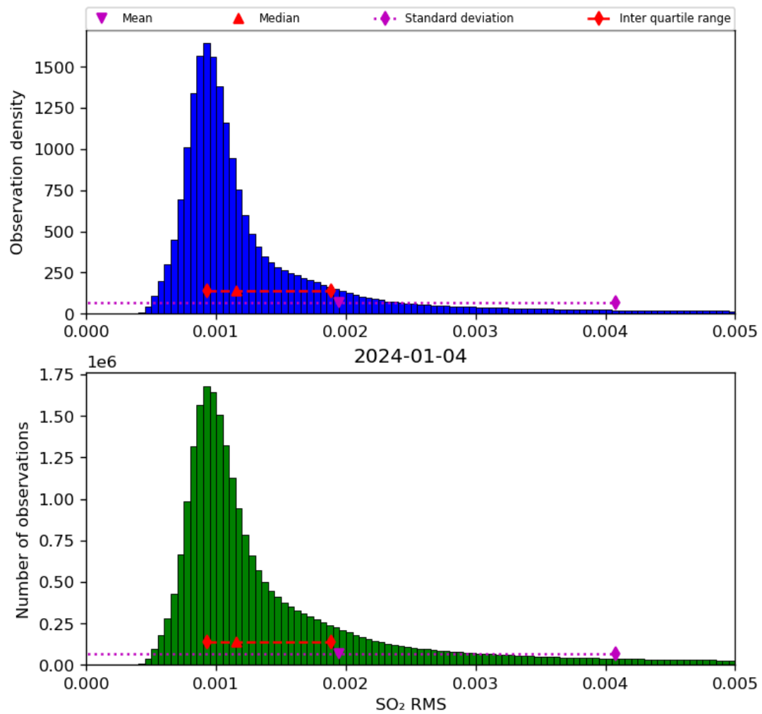
Figure 70: Histogram of “SO 2 RMS” for 2024-01-03 to 2024-01-05
