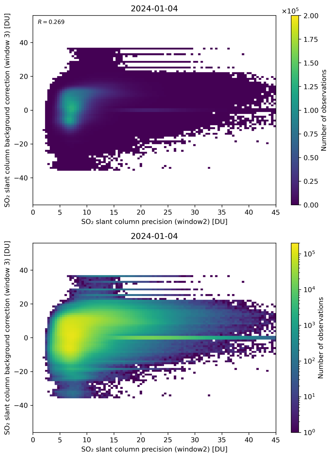
Figure 242: Scatter density plot of “SO 2 slant column precision (window2)” against “SO 2 slant column background correction (window 3)” for 2024-01-03 to 2024-01-05.
