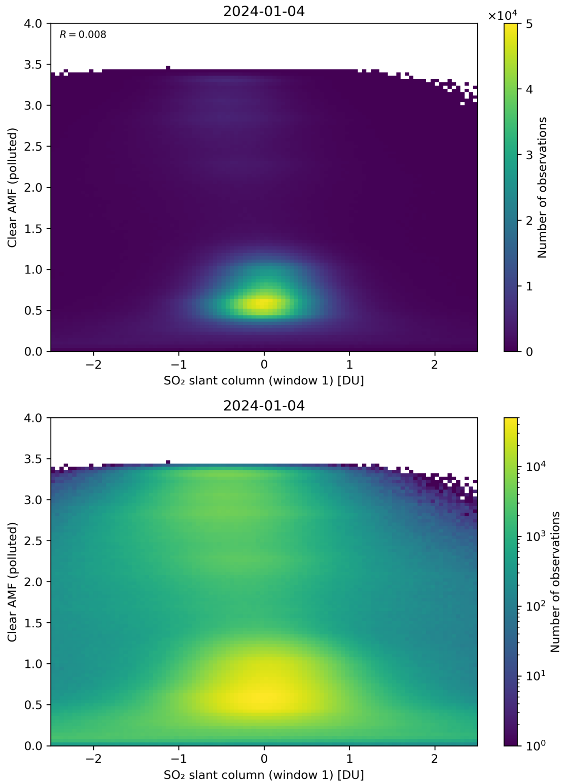
Figure 232: Scatter density plot of “SO 2 slant column (window 1)” against “Clear AMF (polluted)” for 2024-01-03 to 2024-01-05.
