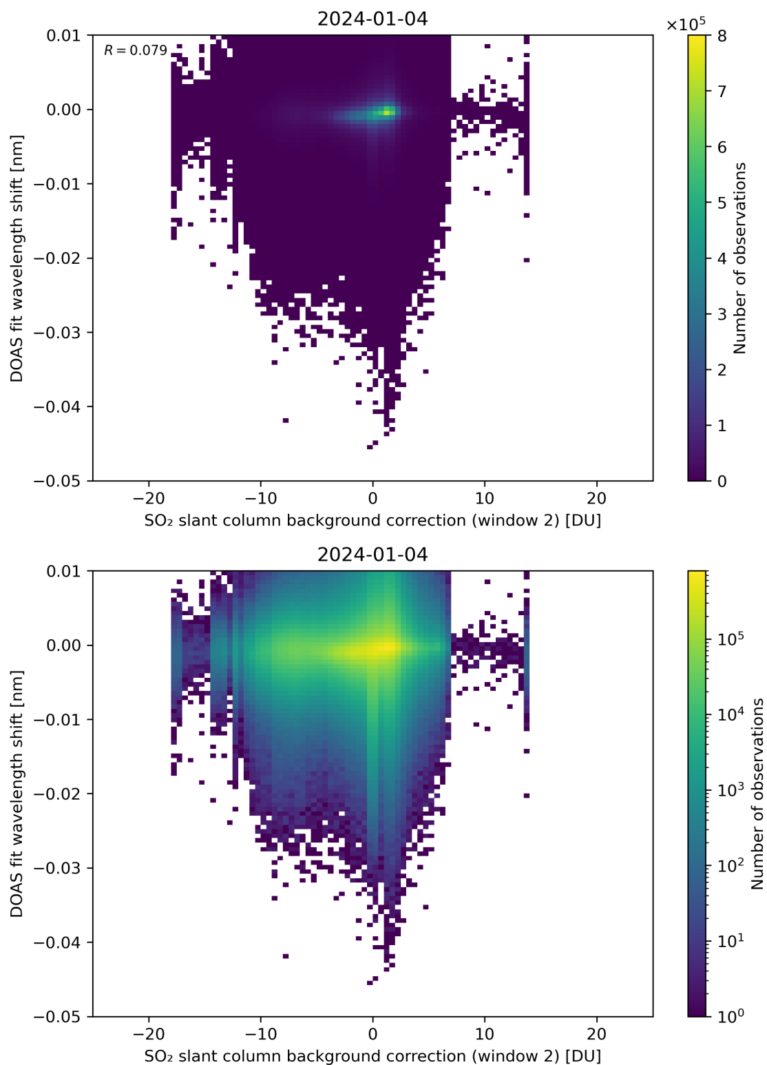
Figure 112: Scatter density plot of “SO 2 slant column background correction (window 2)” against “DOAS fit wavelength shift” for 2024-01-03 to 2024-01-05.
