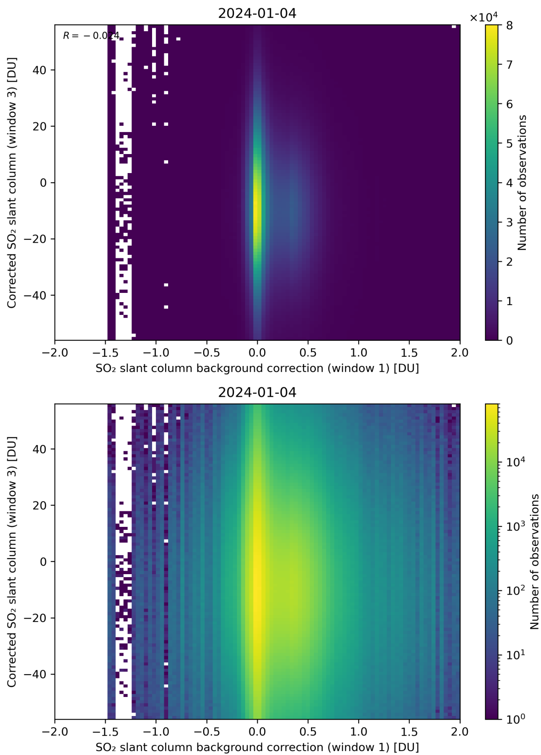
Figure 105: Scatter density plot of “SO 2 slant column background correction (window 1)” against “Corrected SO 2 slant column (window 3)” for 2024-01-03 to 2024-01-05.
