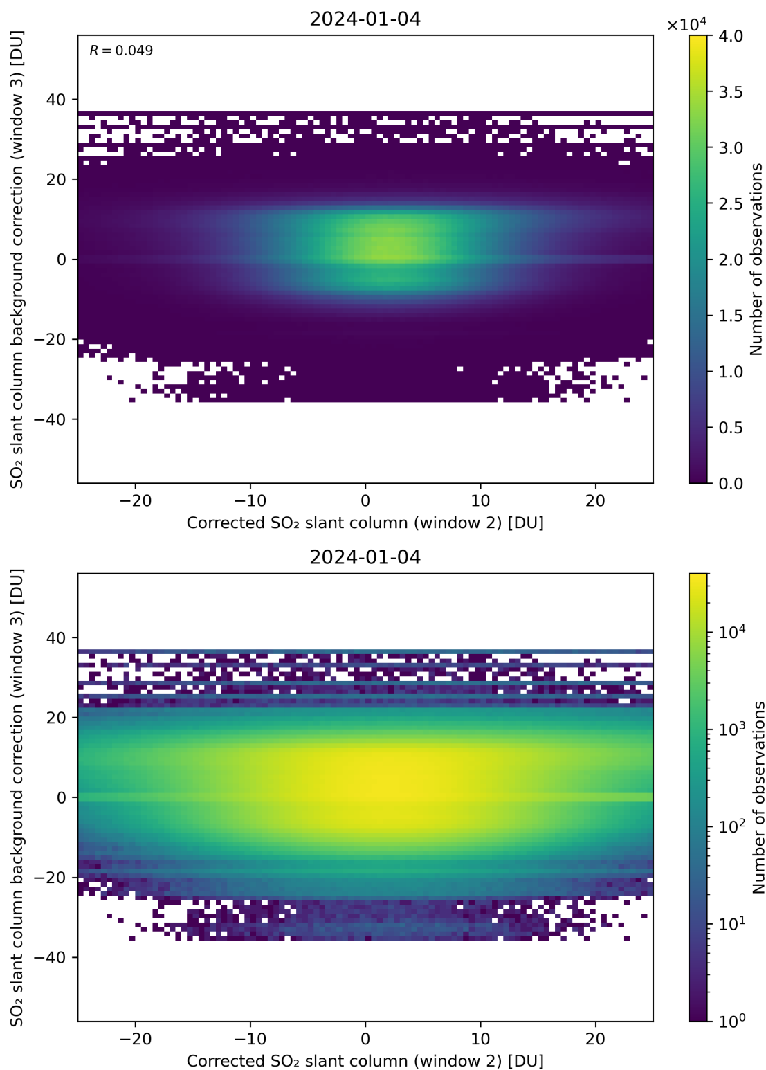
Figure 195: Scatter density plot of “Corrected SO 2 slant column (window 2)” against “SO 2 slant column background correction (window 3)” for 2024-01-03 to 2024-01-05.
