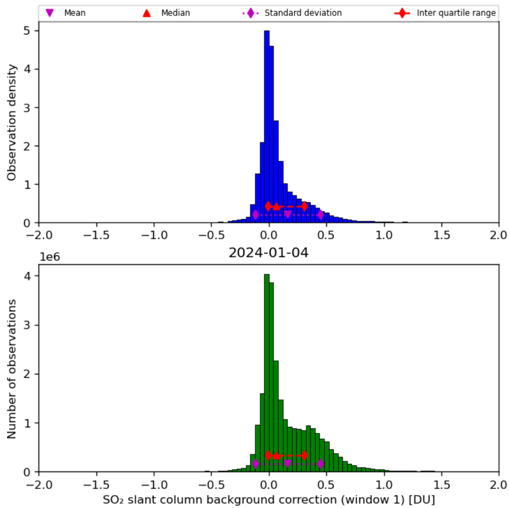
Figure 59: Histogram of “SO 2 slant column background correction (window 1)” for 2024-01-03 to 2024-01-05
