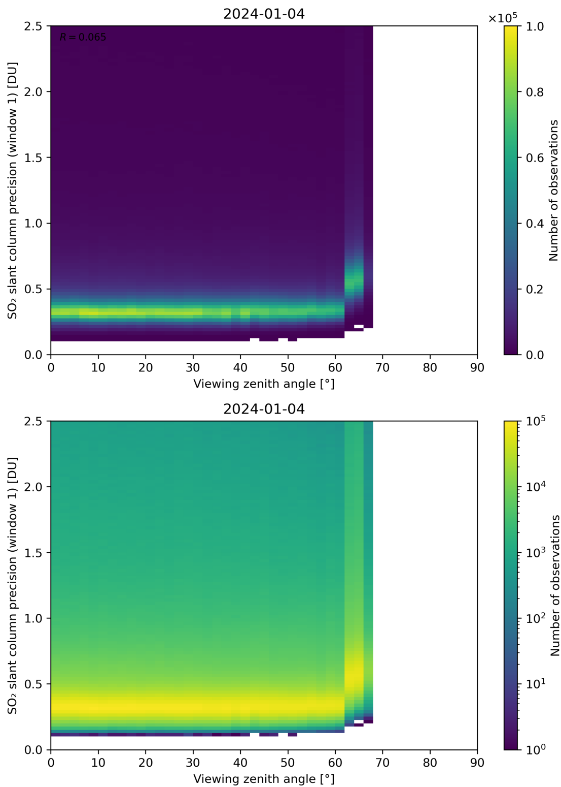
Figure 321: Scatter density plot of “Viewing zenith angle” against “SO 2 slant column precision (window 1)” for 2024-01-03 to 2024-01-05.
