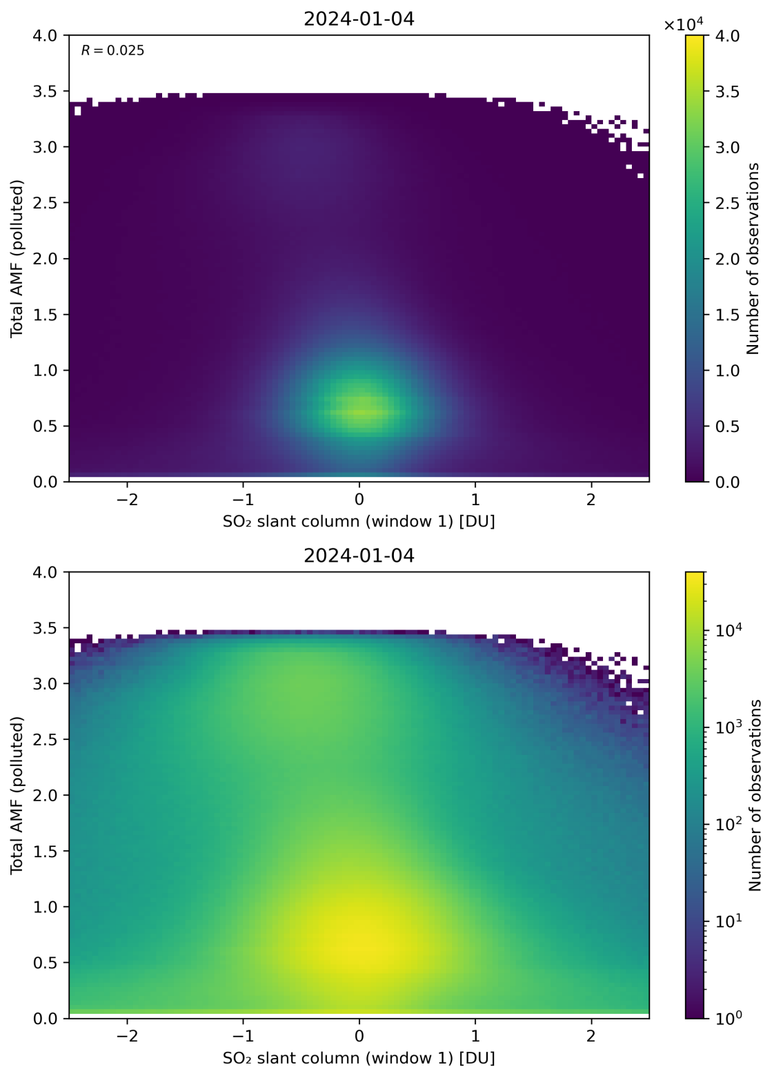
Figure 239: Scatter density plot of “SO 2 slant column (window 1)” against “Total AMF (polluted)” for 2024-01-03 to 2024-01-05.
