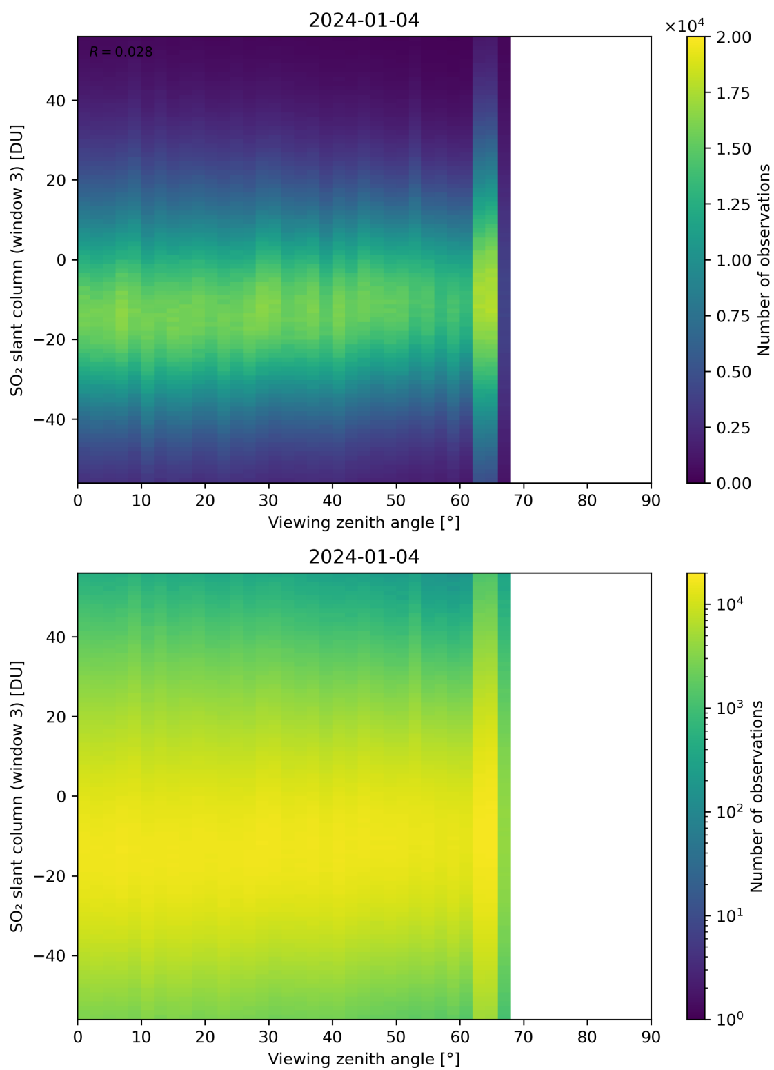
Figure 323: Scatter density plot of “Viewing zenith angle” against “SO 2 slant column (window 3)” for 2024-01-03 to 2024-01-05.
