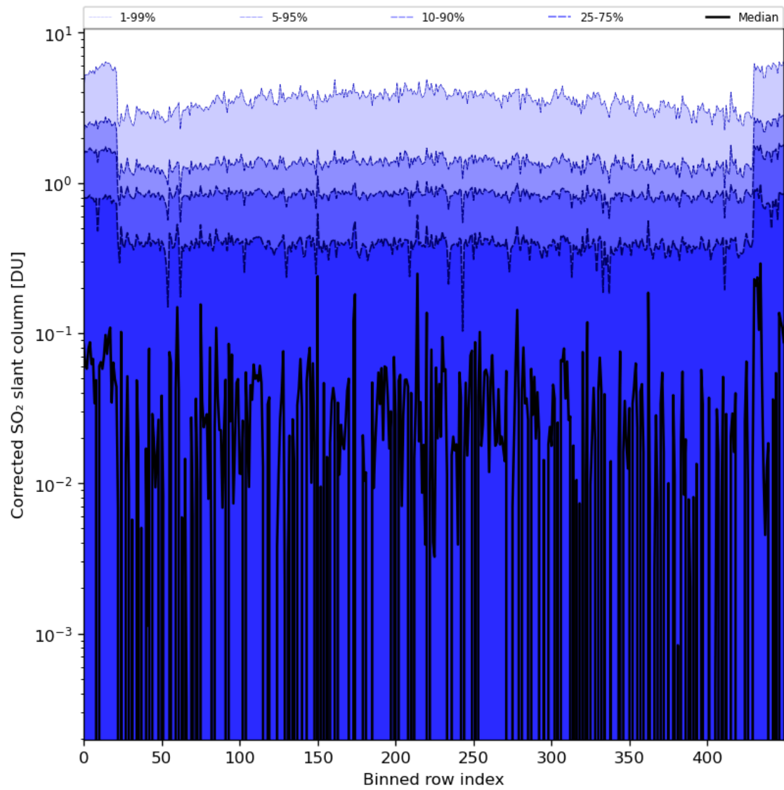
Figure 78: Along track statistics of “Corrected SO 2 slant column” for 2024-01-03 to 2024-01-05
