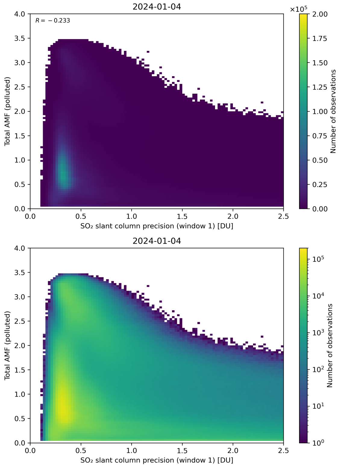
Figure 230: Scatter density plot of “SO 2 slant column precision (window 1)” against “Total AMF (polluted)” for 2024-01-03 to 2024-01-05.
