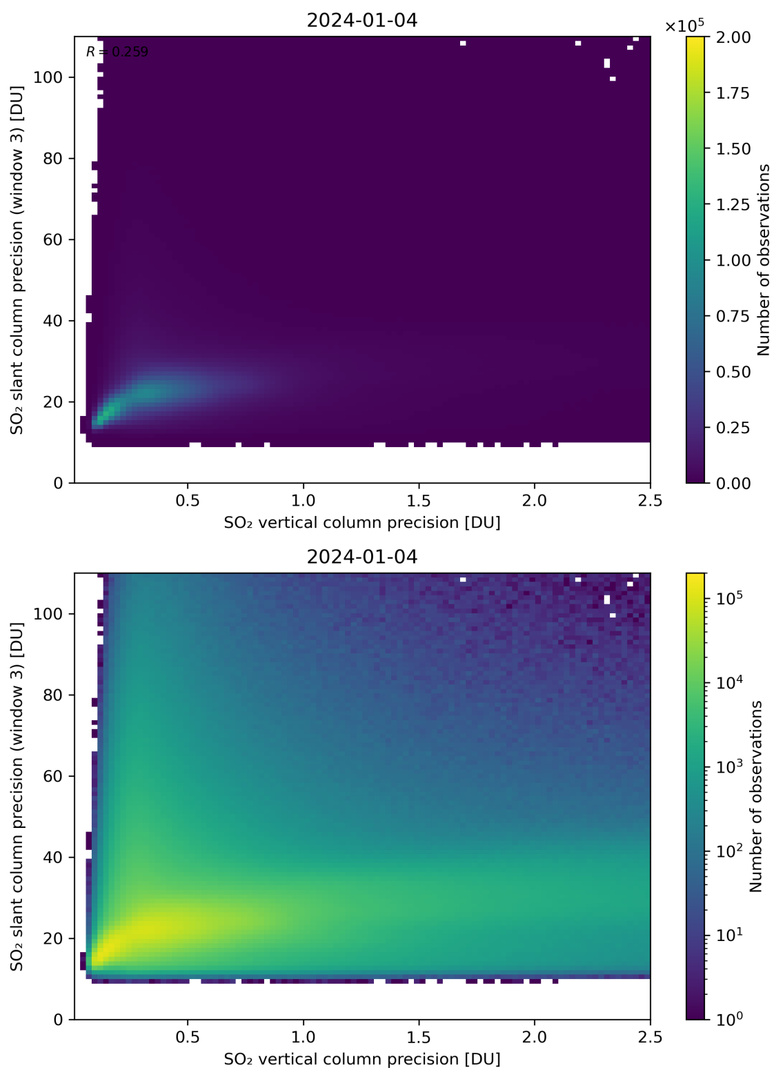
Figure 293: Scatter density plot of “SO 2 vertical column precision” against “SO 2 slant column precision (window 3)” for 2024-01-03 to 2024-01-05.
