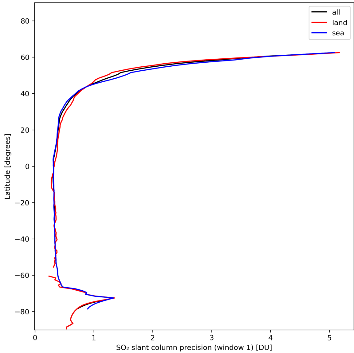
Figure 34: Zonal average of “SO 2 slant column precision (window 1)” for 2024-01-03 to 2024-01-05.
