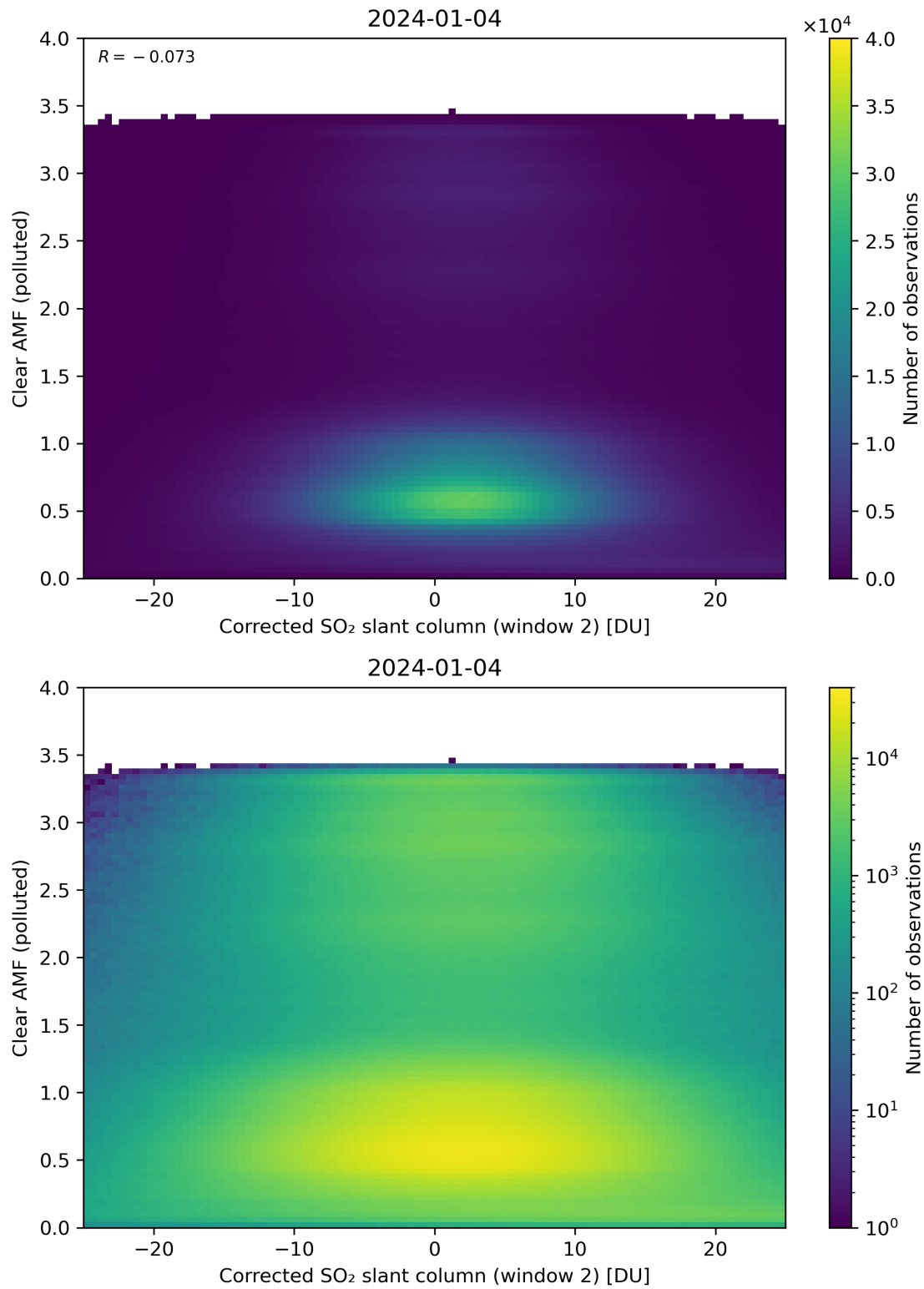
Figure 199: Scatter density plot of “Corrected SO 2 slant column (window 2)” against “Clear AMF (polluted)” for 2024-01-03 to 2024-01-05.
