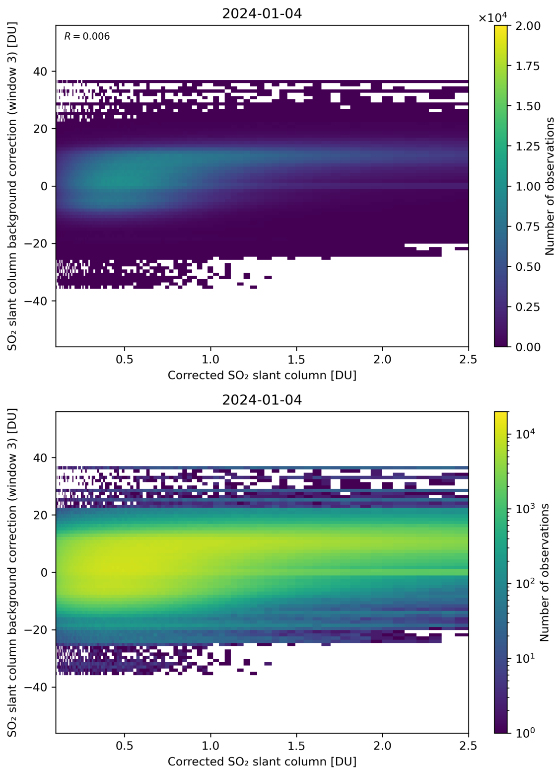
Figure 180: Scatter density plot of “Corrected SO 2 slant column” against “SO 2 slant column background correction (window 3)” for 2024-01-03 to 2024-01-05.
