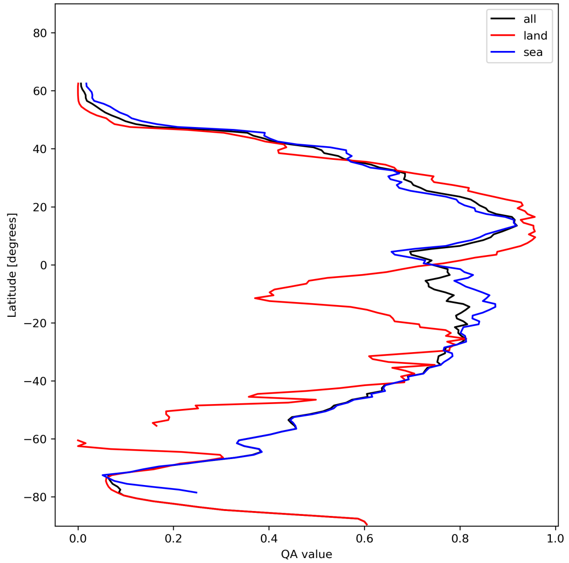
Figure 29: Zonal average of “QA value” for 2024-01-03 to 2024-01-05.
