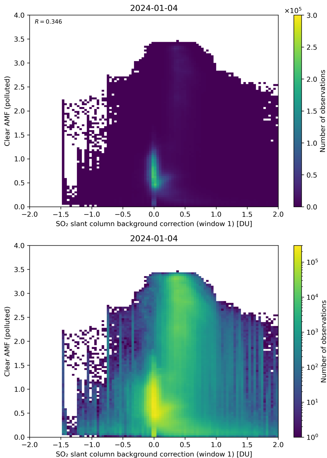
Figure 103: Scatter density plot of “SO 2 slant column background correction (window 1)” against “Clear AMF (polluted)” for 2024-01-03 to 2024-01-05.
