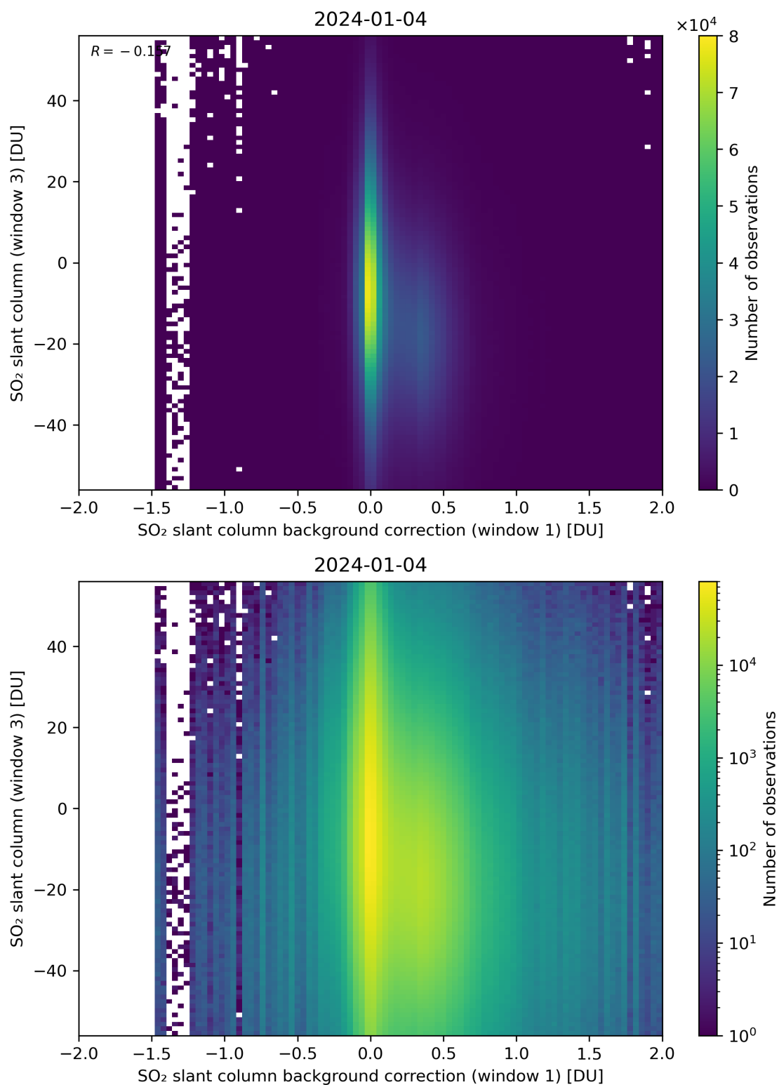
Figure 107: Scatter density plot of “SO 2 slant column background correction (window 1)” against “SO 2 slant column (window 3)” for 2024-01-03 to 2024-01-05.
