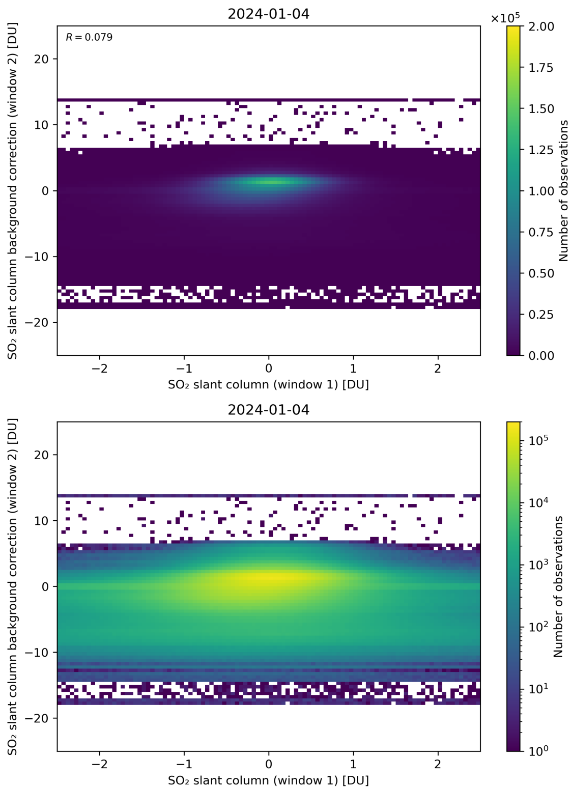
Figure 213: Scatter density plot of “SO 2 slant column (window 1)” against “SO 2 slant column background correction (window 2)” for 2024-01-03 to 2024-01-05.
