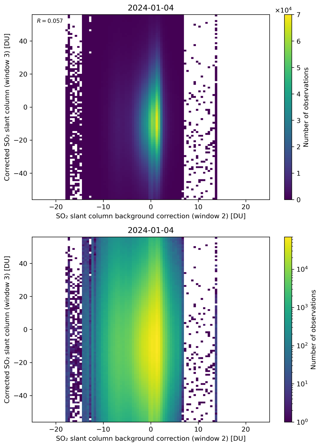
Figure 116: Scatter density plot of “SO 2 slant column background correction (window 2)” against “Corrected SO 2 slant column (window 3)” for 2024-01-03 to 2024-01-05.
