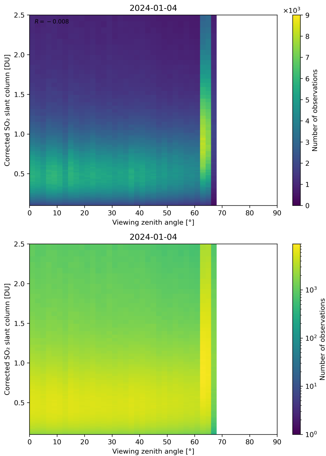
Figure 317: Scatter density plot of “Viewing zenith angle” against “Corrected SO 2 slant column” for 2024-01-03 to 2024-01-05.
