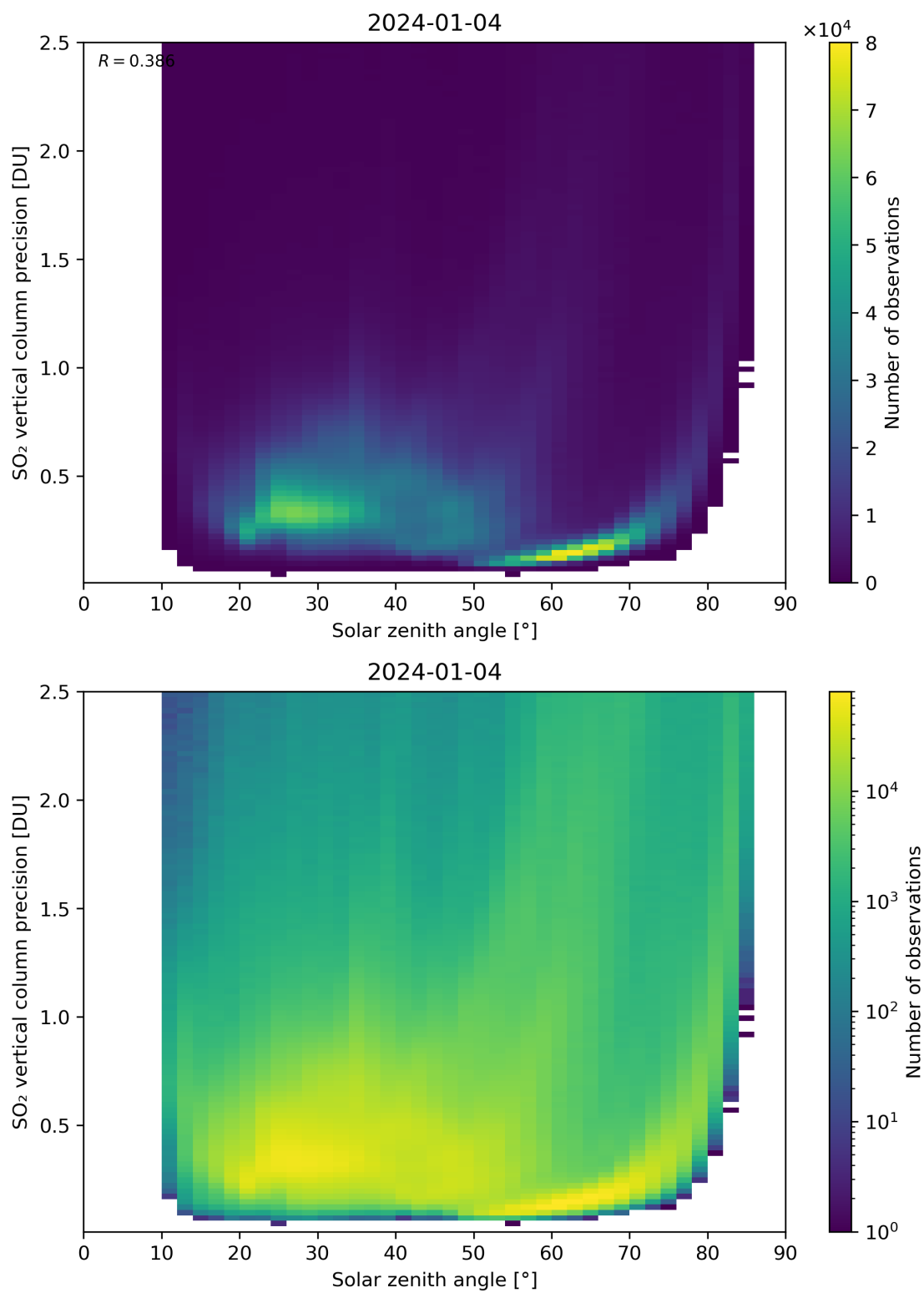
Figure 177: Scatter density plot of “Solar zenith angle” against “SO 2 vertical column precision” for 2024-01-03 to 2024-01-05.
