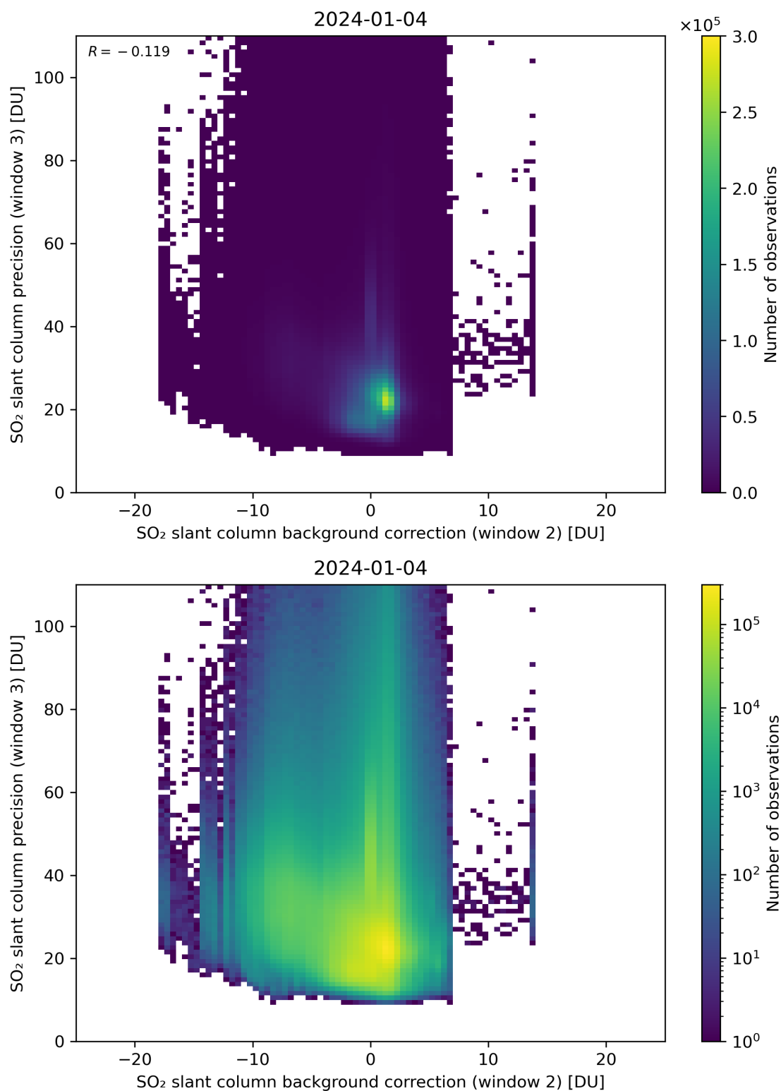
Figure 118: Scatter density plot of “SO 2 slant column background correction (window 2)” against “SO 2 slant column precision (window 3)” for 2024-01-03 to 2024-01-05.
