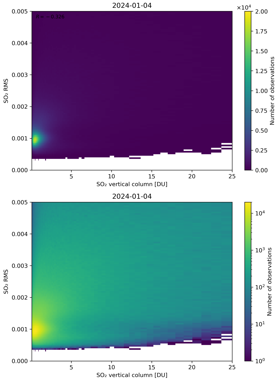
Figure 278: Scatter density plot of “SO 2 vertical column” against “SO 2 RMS” for 2024-01-03 to 2024-01-05.
