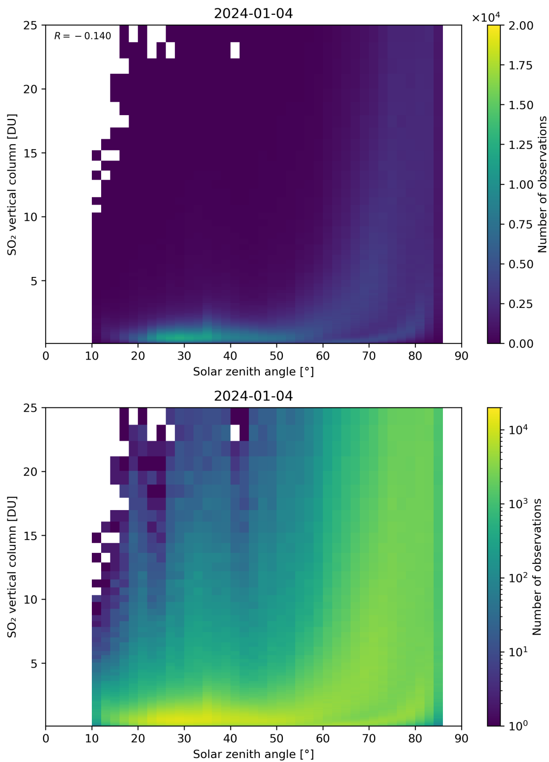
Figure 176: Scatter density plot of “Solar zenith angle” against “SO 2 vertical column” for 2024-01-03 to 2024-01-05.
