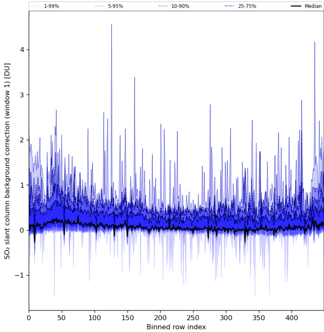
Figure 82: Along track statistics of “SO 2 slant column background correction (window 1)” for 2024-01-03 to 2024-01-05
