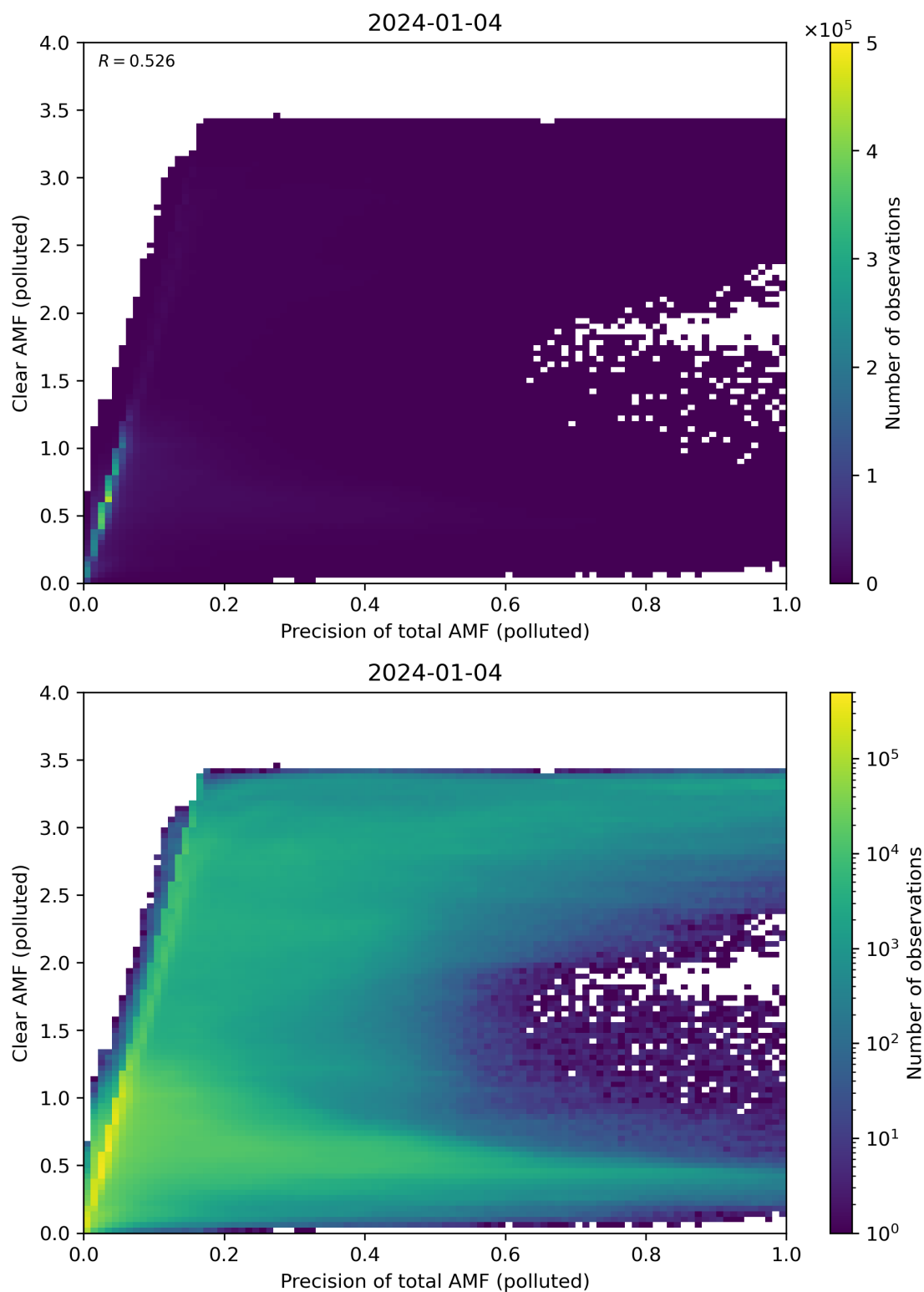
Figure 270: Scatter density plot of “Precision of total AMF (polluted)” against “Clear AMF (polluted)” for 2024-01-03 to 2024-01-05.
