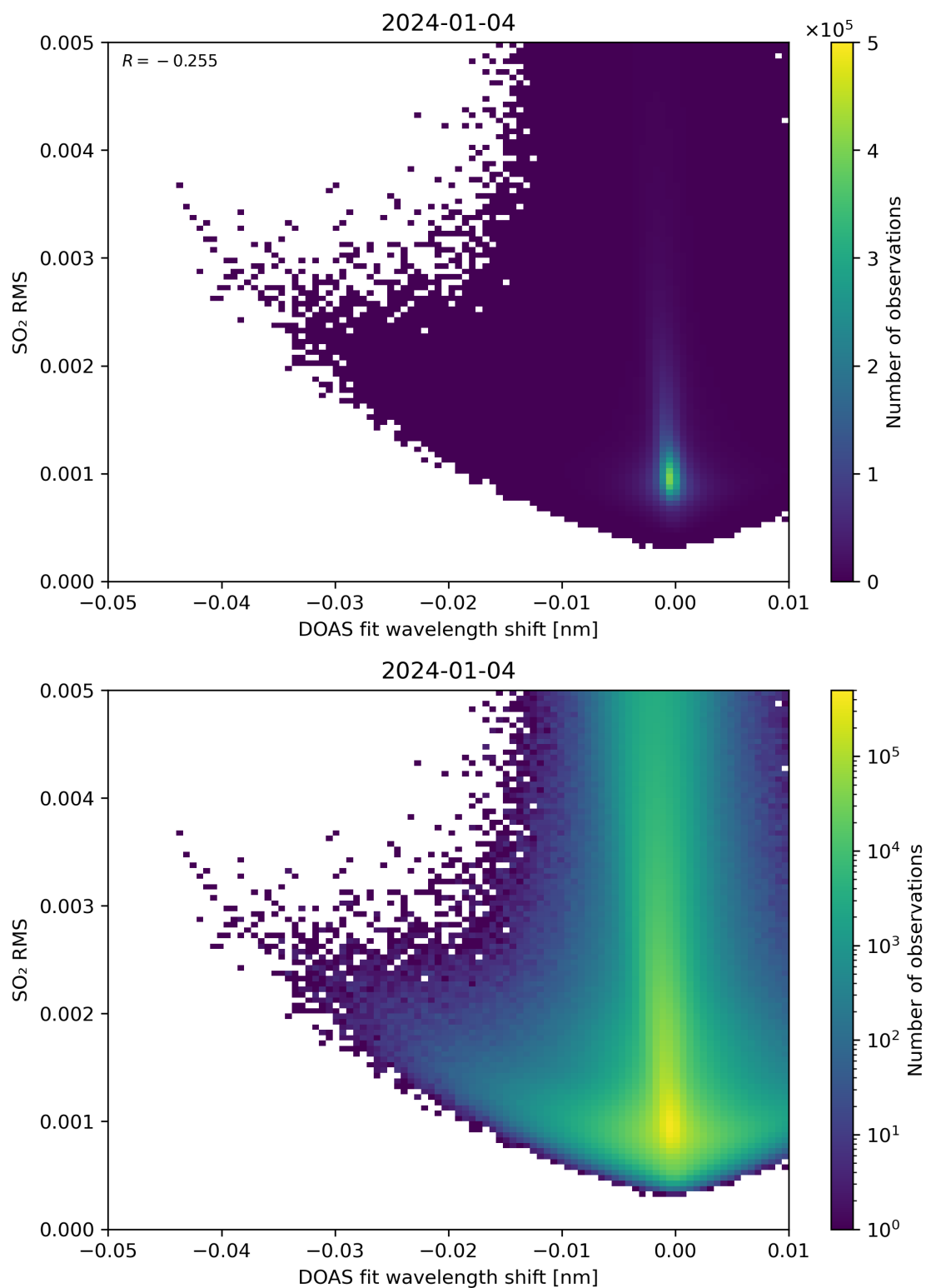
Figure 128: Scatter density plot of “DOAS fit wavelength shift” against “SO 2 RMS” for 2024-01-03 to 2024-01-05.
