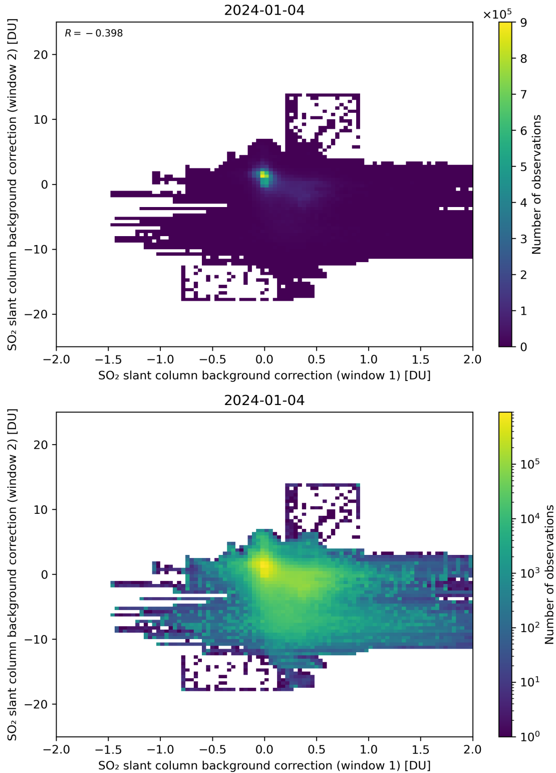
Figure 98: Scatter density plot of “SO 2 slant column background correction (window 1)” against “SO 2 slant column background correction (window 2)” for 2024-01-03 to 2024-01-05.
