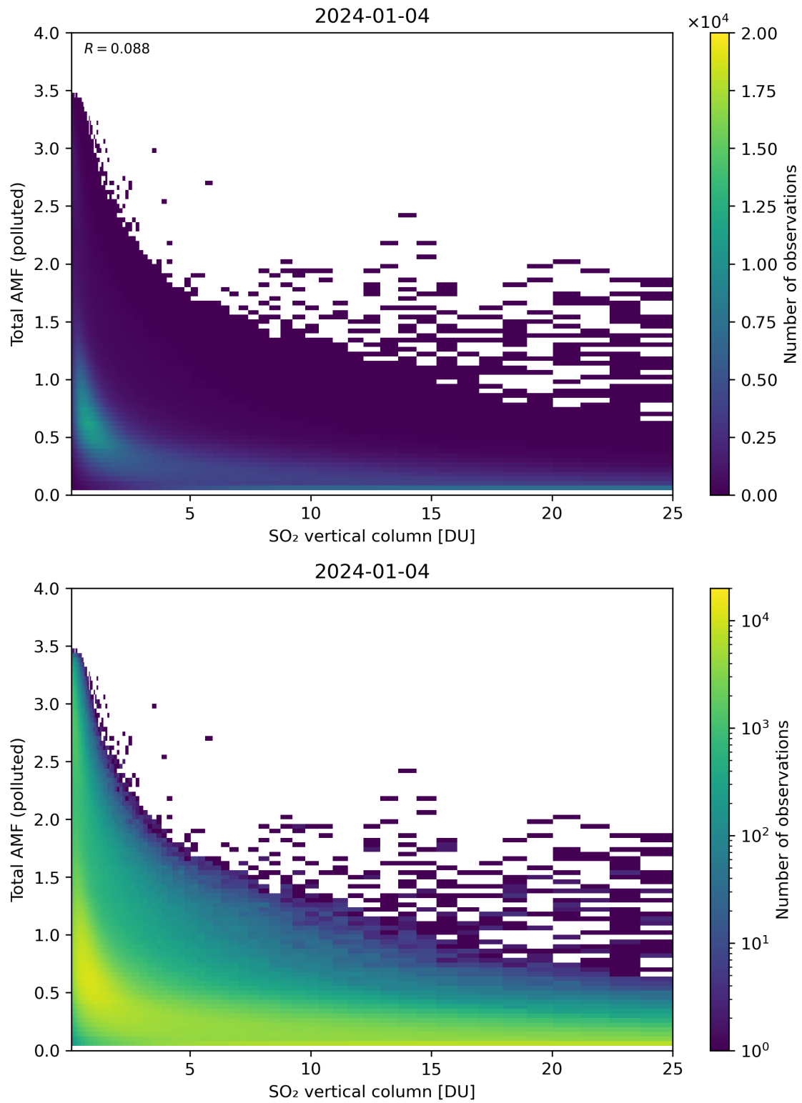
Figure 305: Scatter density plot of “SO 2 vertical column” against “Total AMF (polluted)” for 2024-01-03 to 2024-01-05.
