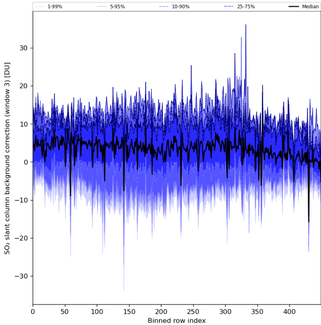
Figure 90: Along track statistics of “SO 2 slant column background correction (window 3)” for 2024-01-03 to 2024-01-05
