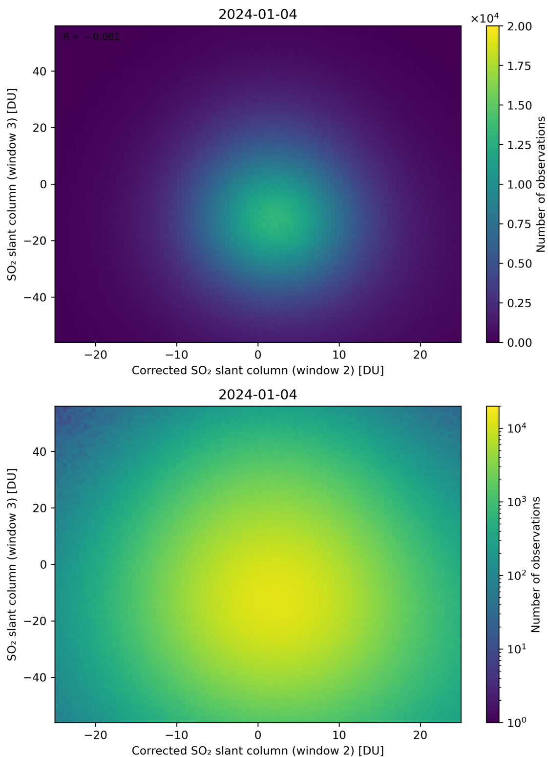
Figure 201: Scatter density plot of “Corrected SO 2 slant column (window 2)” against “SO 2 slant column (window 3)” for 2024-01-03 to 2024-01-05.
