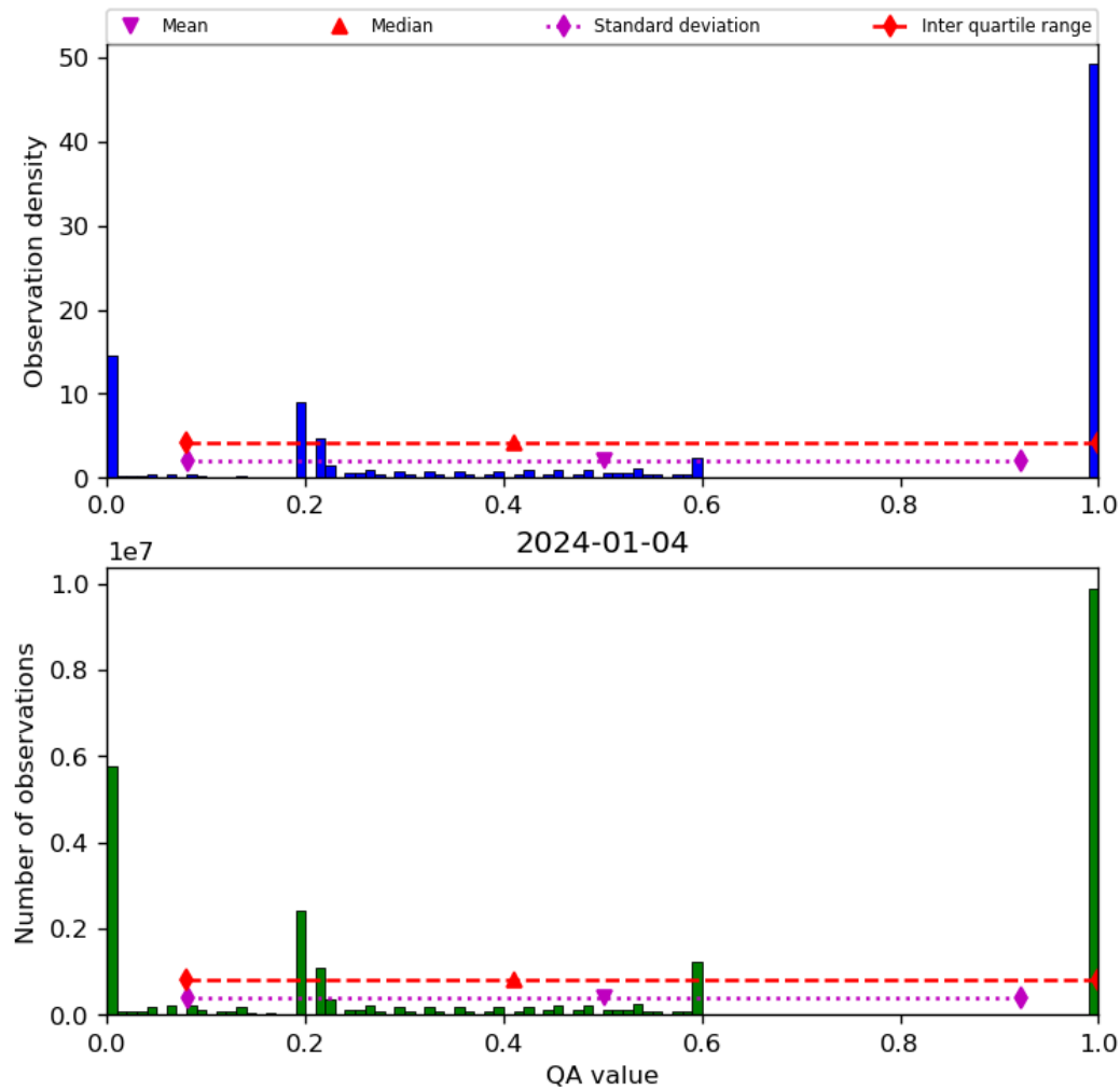
Figure 52: Histogram of “QA value” for 2024-01-03 to 2024-01-05
