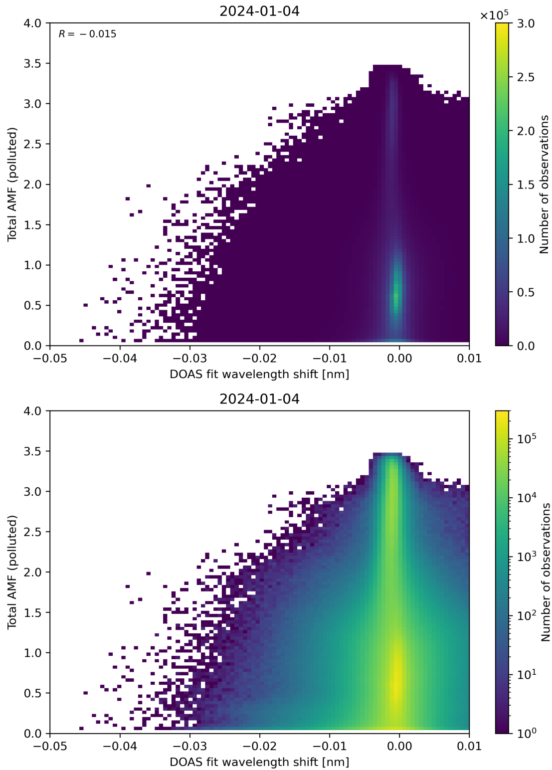
Figure 130: Scatter density plot of “DOAS fit wavelength shift” against “Total AMF (polluted)” for 2024-01-03 to 2024-01-05.
