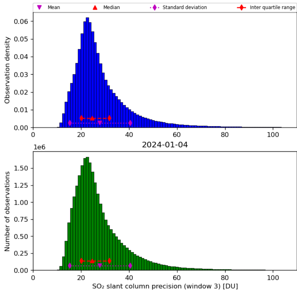
Figure 65: Histogram of “SO 2 slant column precision (window 3)” for 2024-01-03 to 2024-01-05
