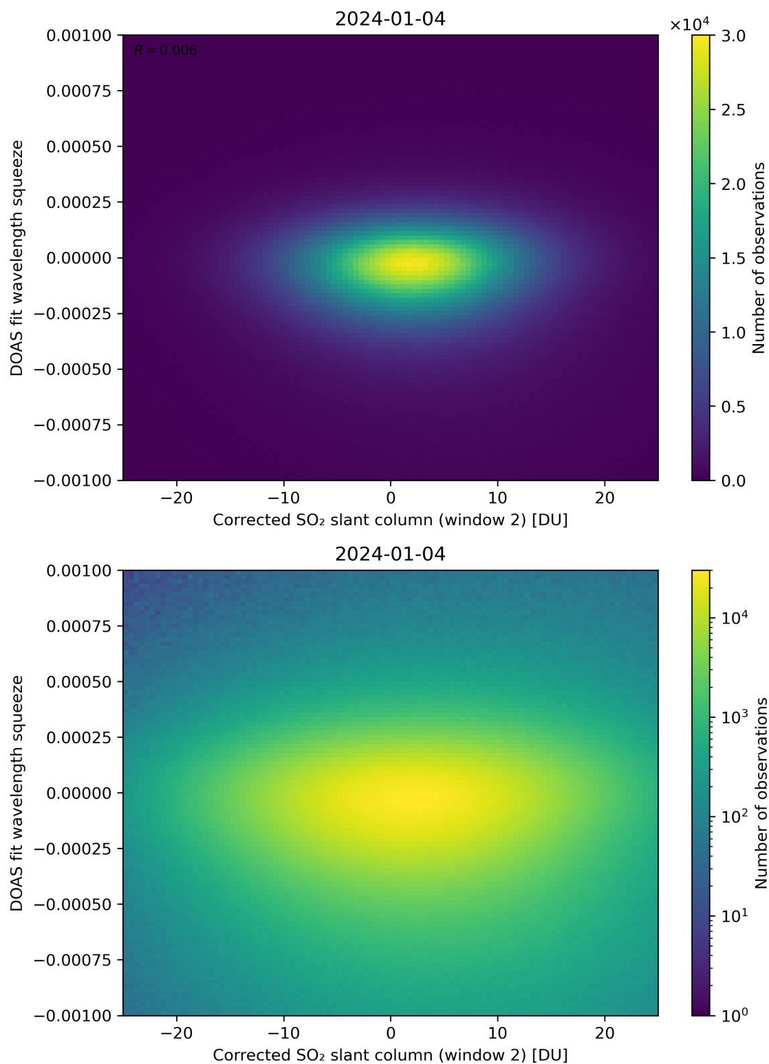
Figure 197: Scatter density plot of “Corrected SO 2 slant column (window 2)” against “DOAS fit wavelength squeeze” for 2024-01-03 to 2024-01-05.
