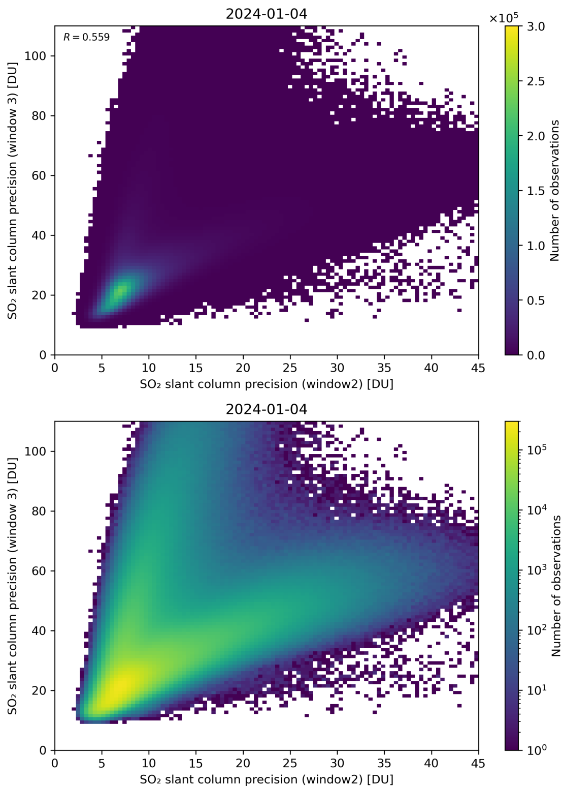
Figure 250: Scatter density plot of “SO 2 slant column precision (window2)” against “SO 2 slant column precision (window 3)” for 2024-01-03 to 2024-01-05.
