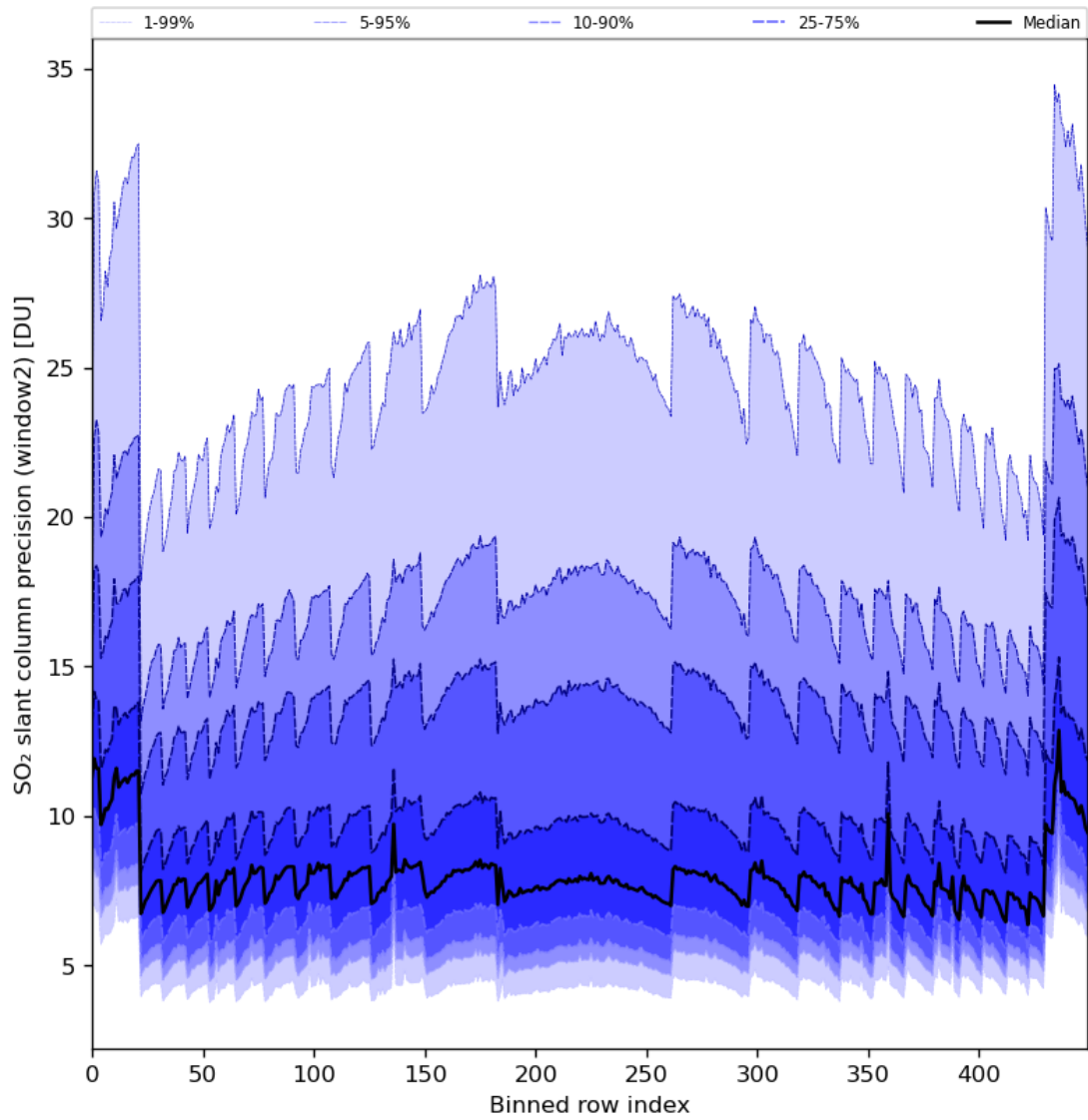
Figure 84: Along track statistics of “SO 2 slant column precision (window2)” for 2024-01-03 to 2024-01-05
