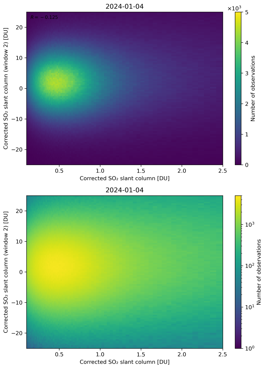
Figure 185: Scatter density plot of “Corrected SO 2 slant column” against “Corrected SO 2 slant column (window 2)” for 2024-01-03 to 2024-01-05.
