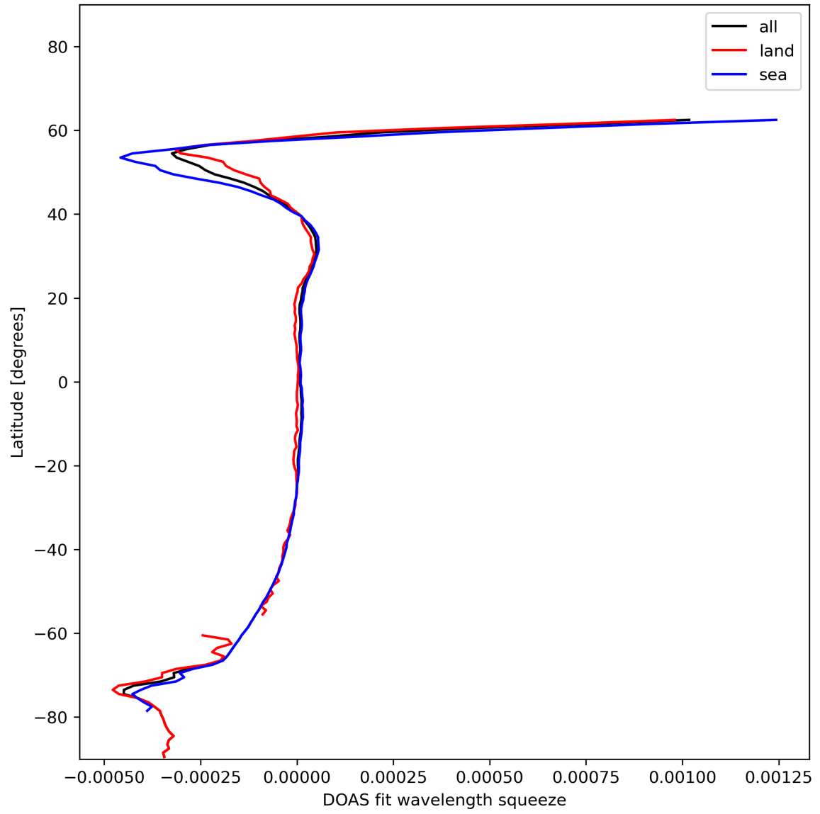
Figure 46: Zonal average of “DOAS fit wavelength squeeze” for 2024-01-03 to 2024-01-05.
