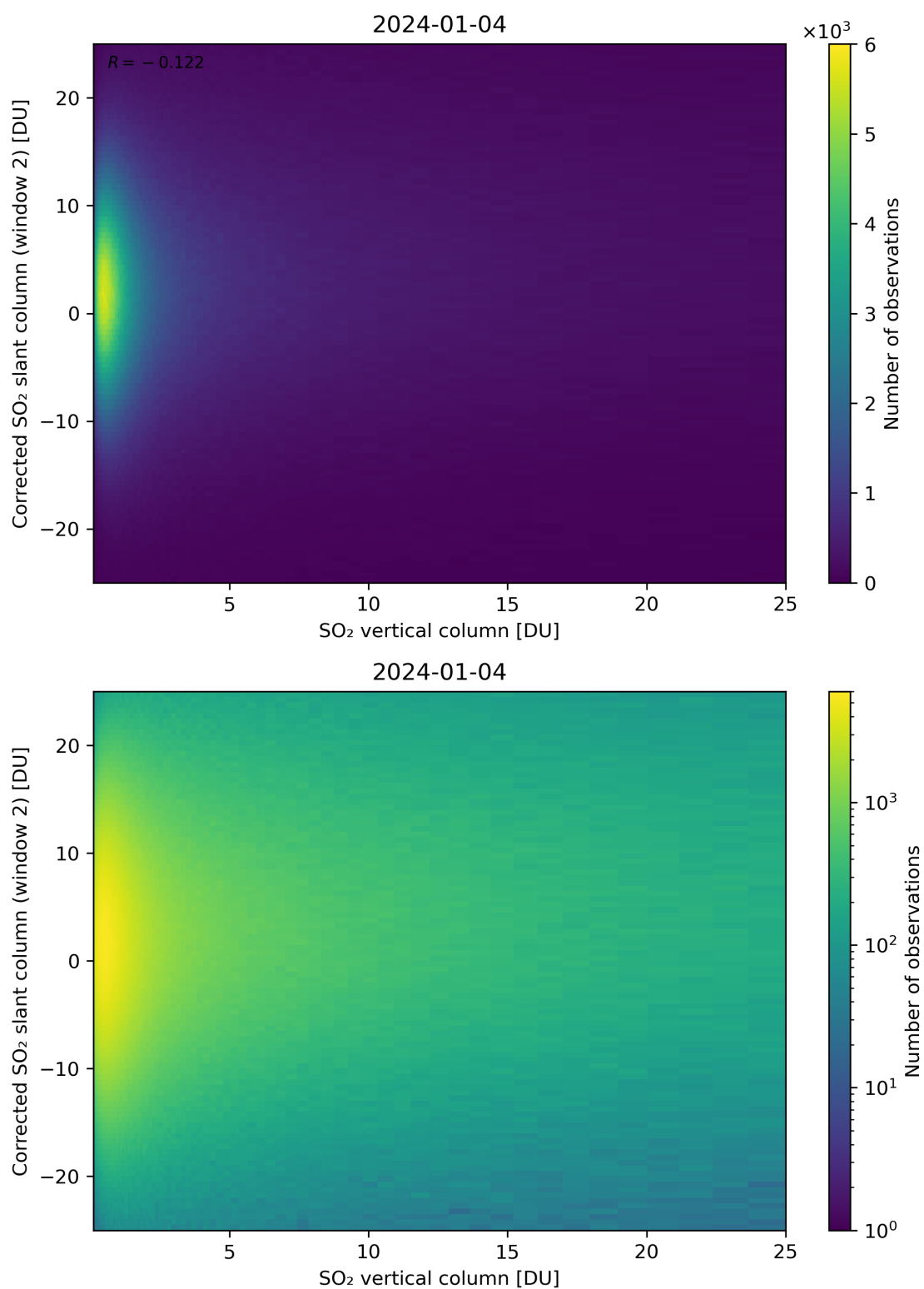
Figure 298: Scatter density plot of “SO 2 vertical column” against “Corrected SO 2 slant column (window 2)” for 2024-01-03 to 2024-01-05.
