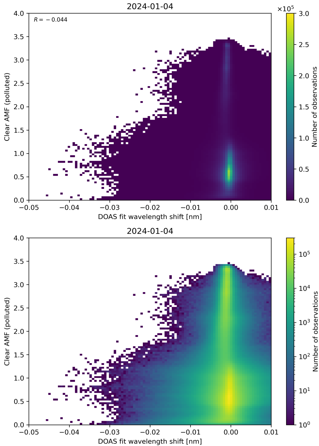
Figure 129: Scatter density plot of “DOAS fit wavelength shift” against “Clear AMF (polluted)” for 2024-01-03 to 2024-01-05.
