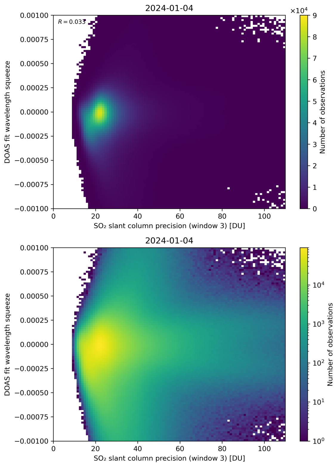
Figure 259: Scatter density plot of “SO 2 slant column precision (window 3)” against “DOAS fit wavelength squeeze” for 2024-01-03 to 2024-01-05.
