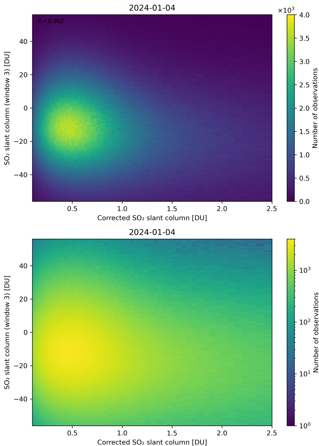
Figure 190: Scatter density plot of “Corrected SO 2 slant column” against “SO 2 slant column (window 3)” for 2024-01-03 to 2024-01-05.
