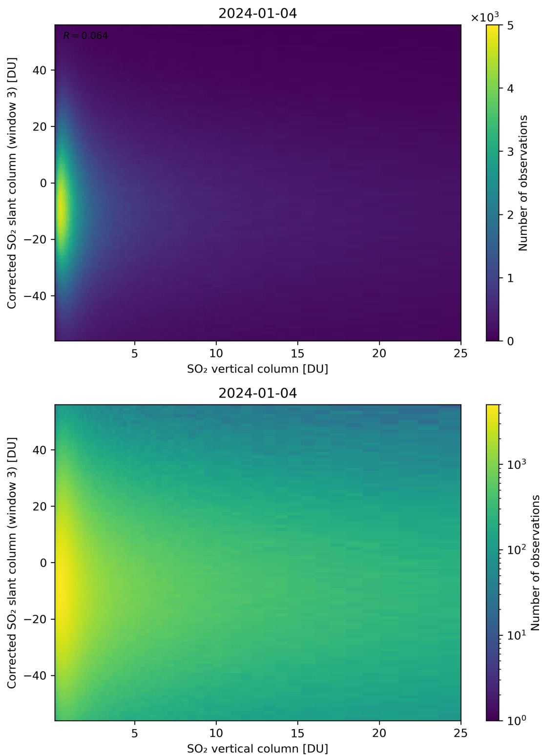
Figure 299: Scatter density plot of “SO 2 vertical column” against “Corrected SO 2 slant column (window 3)” for 2024-01-03 to 2024-01-05.
