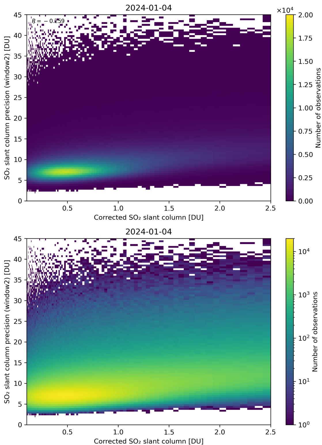
Figure 189: Scatter density plot of “Corrected SO 2 slant column” against “SO 2 slant column precision (window2)” for 2024-01-03 to 2024-01-05.
