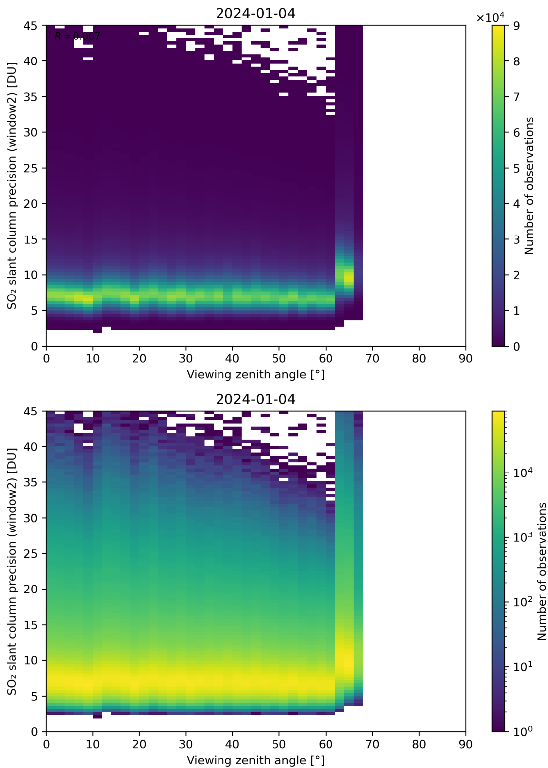
Figure 322: Scatter density plot of “Viewing zenith angle” against “SO 2 slant column precision (window2)” for 2024-01-03 to 2024-01-05.
