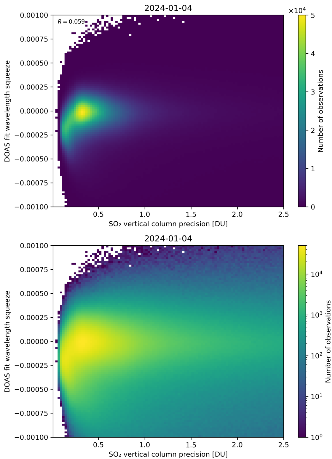
Figure 283: Scatter density plot of “SO 2 vertical column precision” against “DOAS fit wavelength squeeze” for 2024-01-03 to 2024-01-05.
