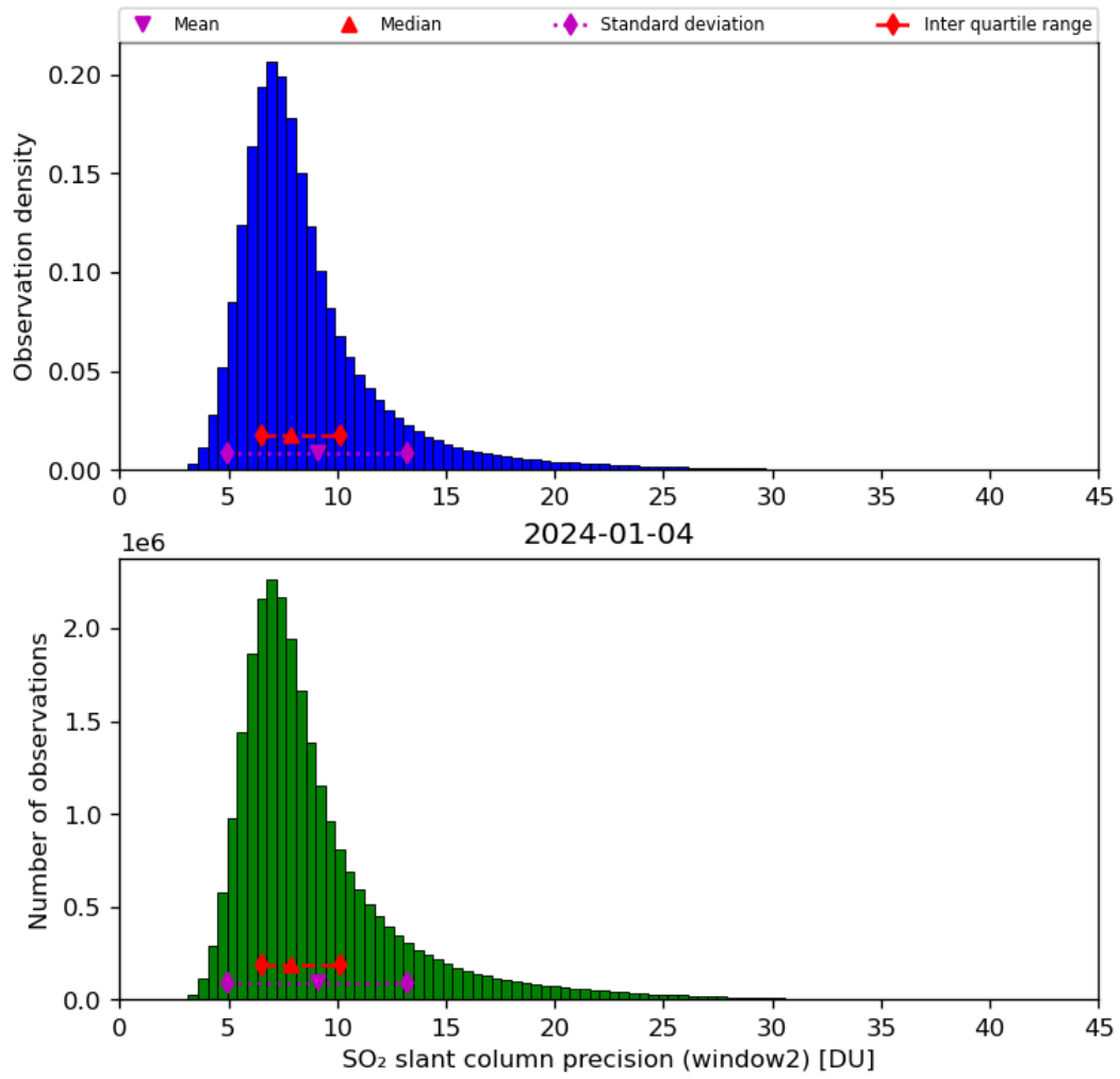
Figure 61: Histogram of “SO 2 slant column precision (window2)” for 2024-01-03 to 2024-01-05
