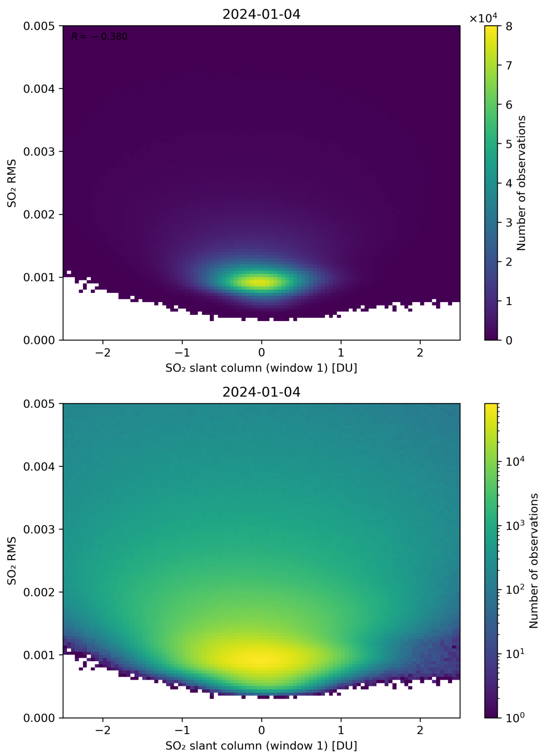
Figure 217: Scatter density plot of “SO 2 slant column (window 1)” against “SO 2 RMS” for 2024-01-03 to 2024-01-05.
