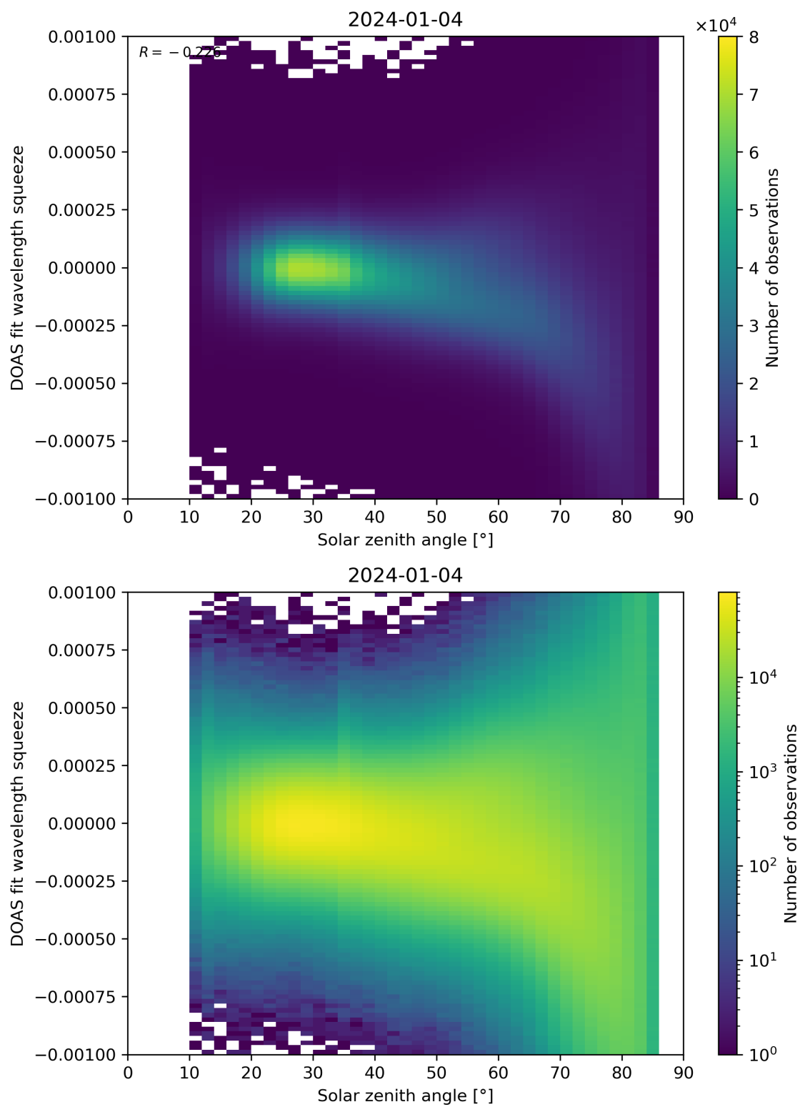
Figure 162: Scatter density plot of “Solar zenith angle” against “DOAS fit wavelength squeeze” for 2024-01-03 to 2024-01-05.
