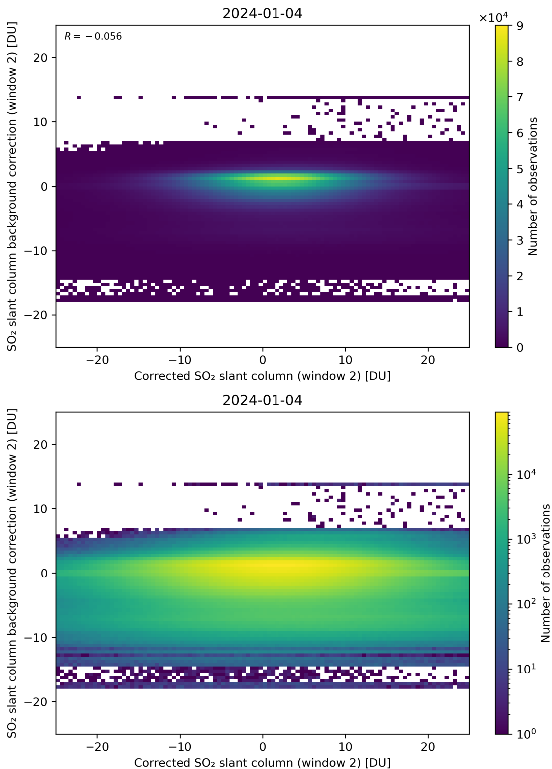
Figure 194: Scatter density plot of “Corrected SO 2 slant column (window 2)” against “SO 2 slant column background correction (window 2)” for 2024-01-03 to 2024-01-05.
