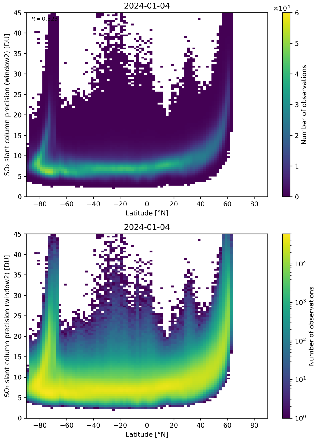
Figure 151: Scatter density plot of “Latitude” against “SO 2 slant column precision (window2)” for 2024-01-03 to 2024-01-05.
