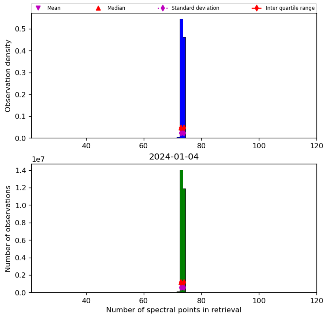
Figure 74: Histogram of “Number of spectral points in retrieval” for 2024-01-03 to 2024-01-05
