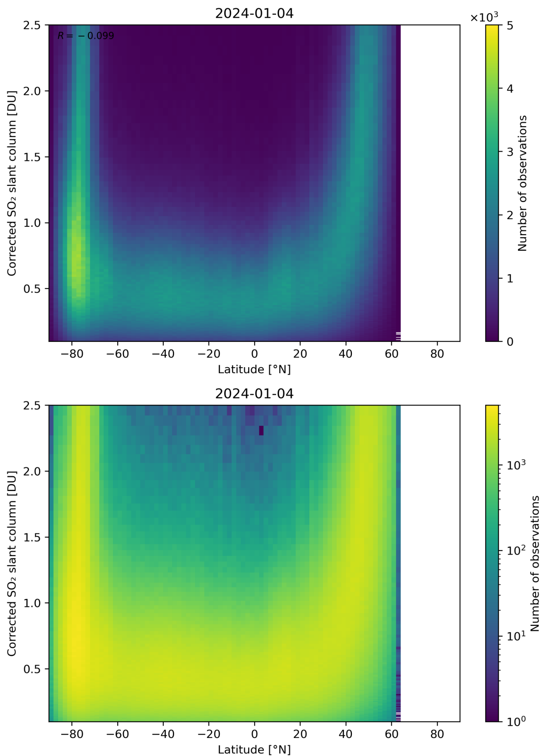
Figure 146: Scatter density plot of “Latitude” against “Corrected SO 2 slant column” for 2024-01-03 to 2024-01-05.
