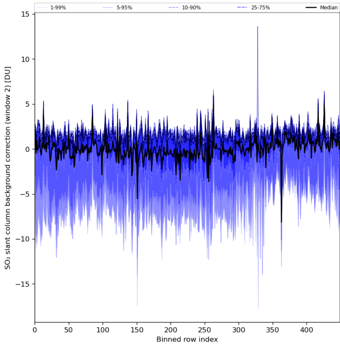
Figure 86: Along track statistics of “SO 2 slant column background correction (window 2)” for 2024-01-03 to 2024-01-05
