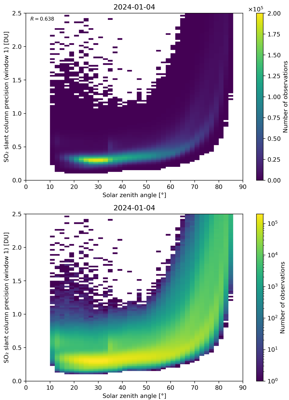
Figure 170: Scatter density plot of “Solar zenith angle” against “SO 2 slant column precision (window 1)” for 2024-01-03 to 2024-01-05.
