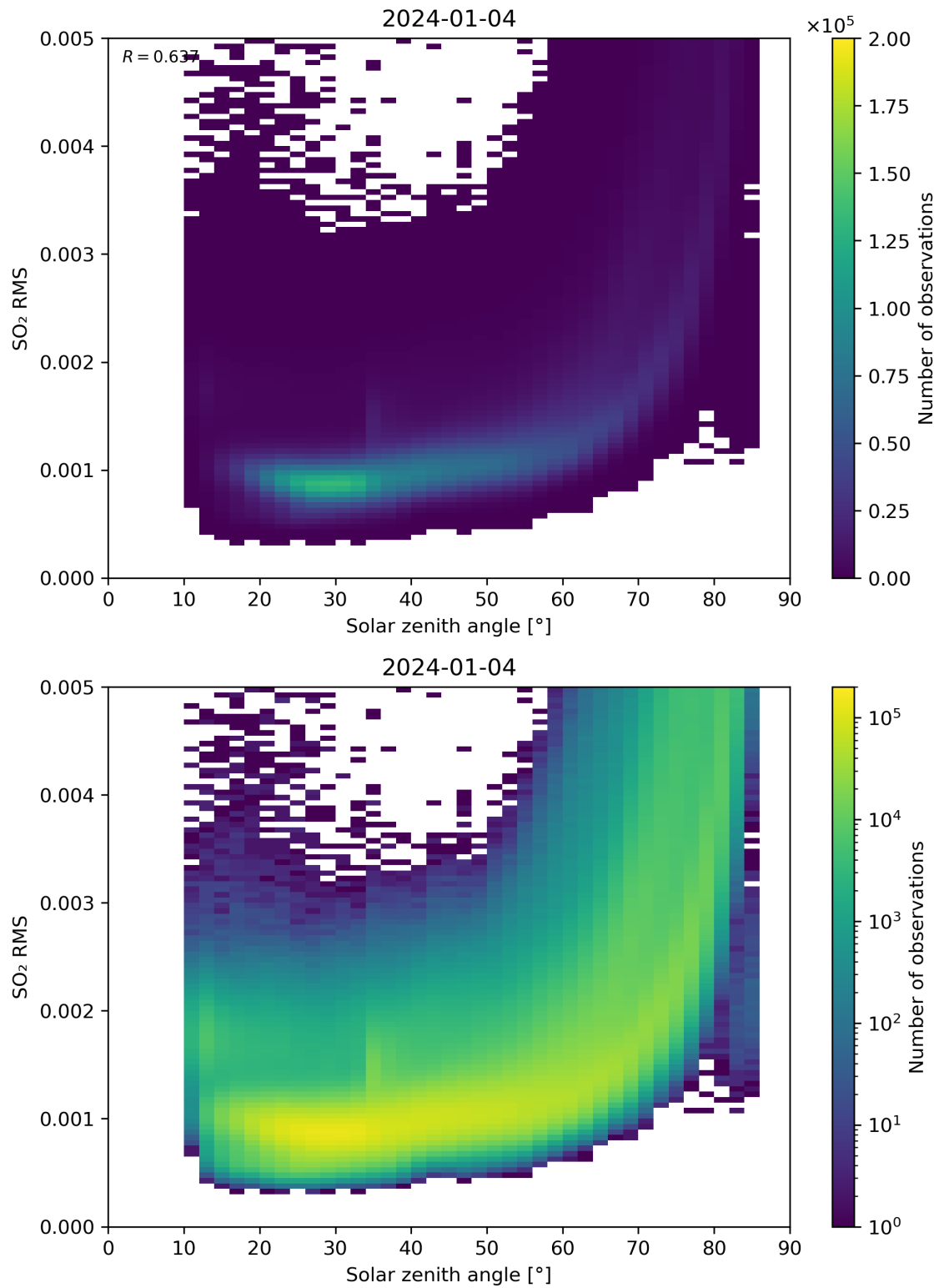
Figure 163: Scatter density plot of “Solar zenith angle” against “SO 2 RMS” for 2024-01-03 to 2024-01-05.
