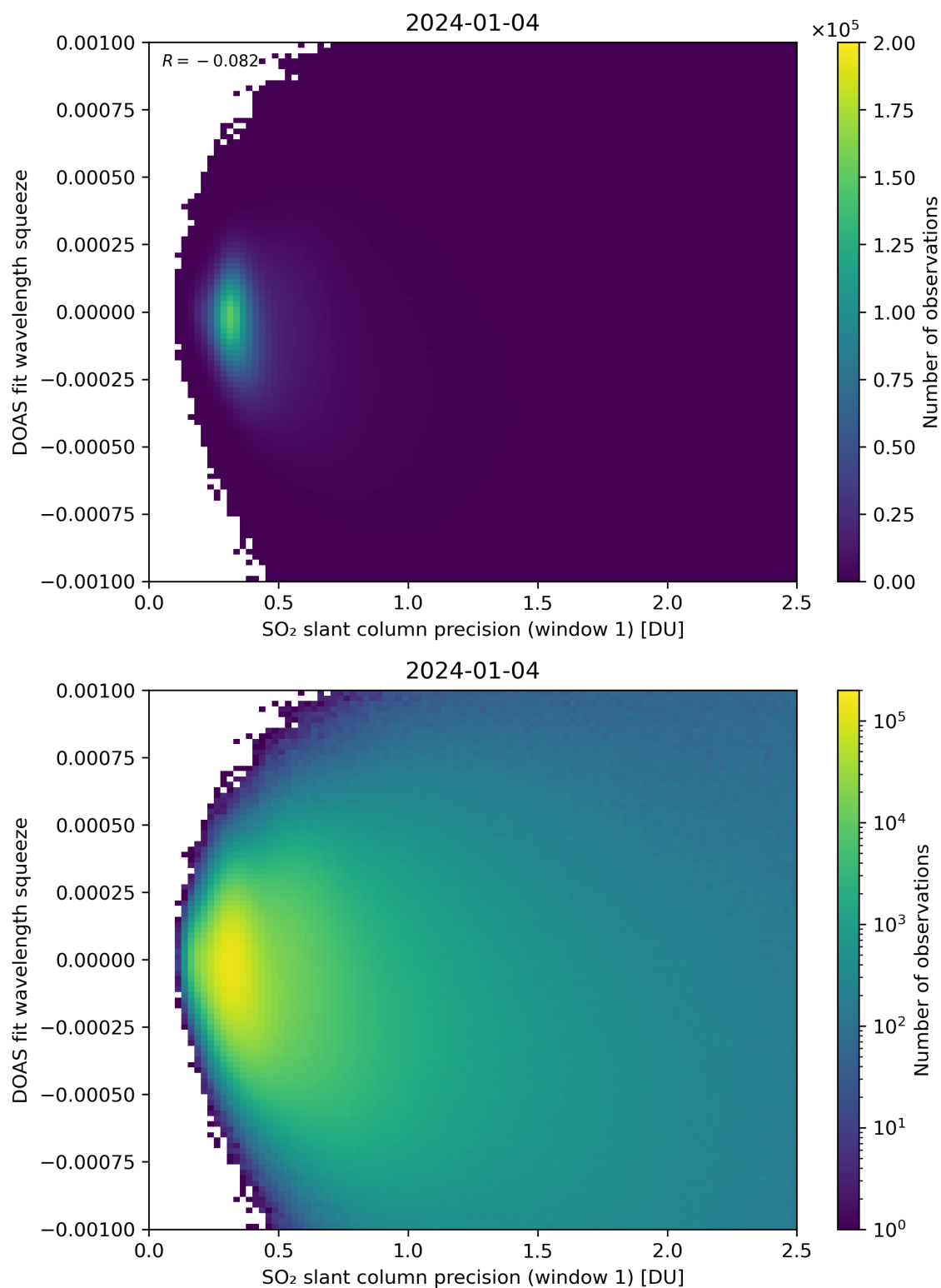
Figure 222: Scatter density plot of “SO 2 slant column precision (window 1)” against “DOAS fit wavelength squeeze” for 2024-01-03 to 2024-01-05.
