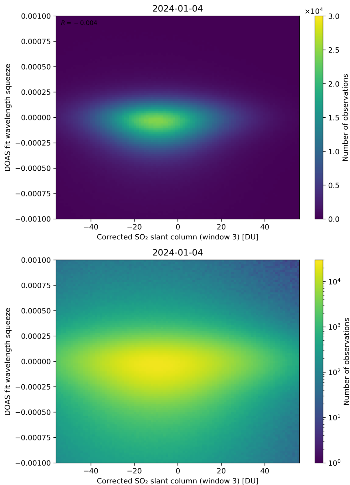
Figure 207: Scatter density plot of “Corrected SO 2 slant column (window 3)” against “DOAS fit wavelength squeeze” for 2024-01-03 to 2024-01-05.
