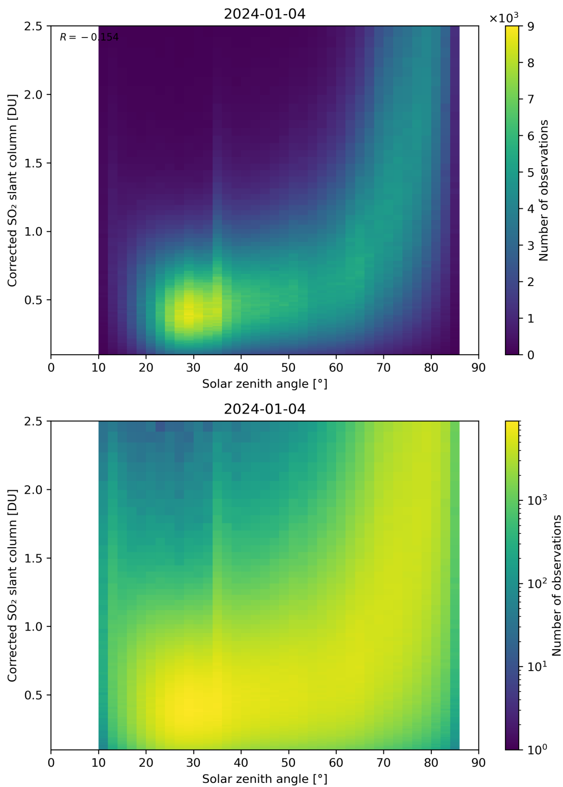
Figure 166: Scatter density plot of “Solar zenith angle” against “Corrected SO 2 slant column” for 2024-01-03 to 2024-01-05.
