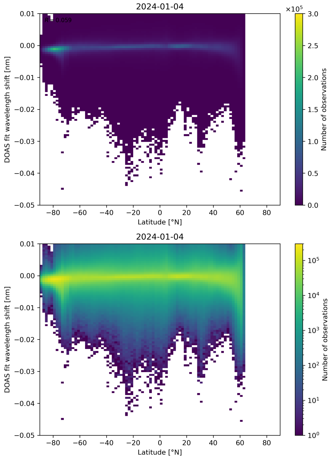
Figure 142: Scatter density plot of “Latitude” against “DOAS fit wavelength shift” for 2024-01-03 to 2024-01-05.
