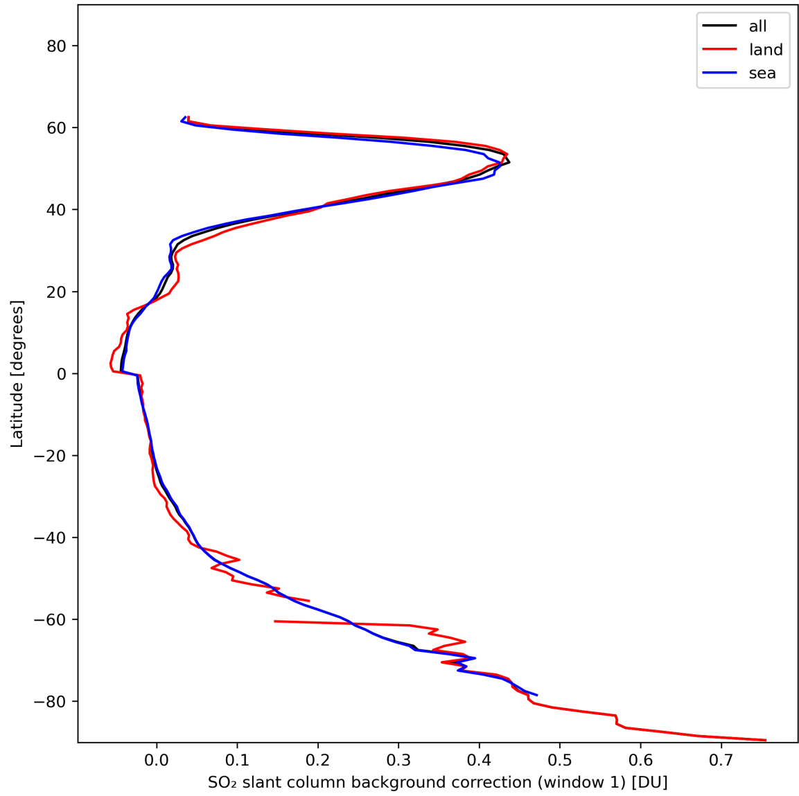
Figure 36: Zonal average of "SO 2 slant column background correction (window 1)" for 2024-01-03 to 2024-01-05.
