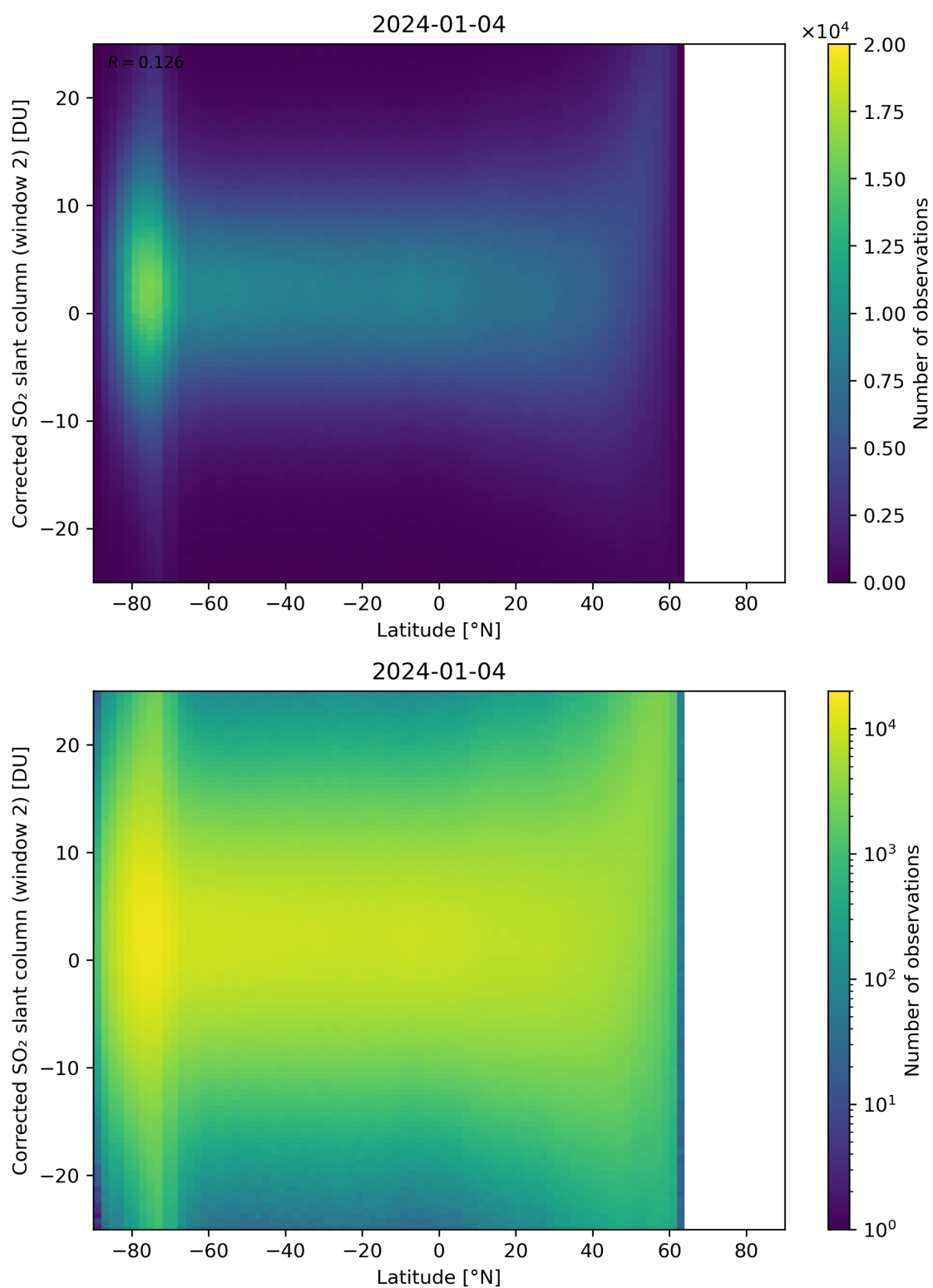
Figure 147: Scatter density plot of “Latitude” against “Corrected SO 2 slant column (window 2)” for 2024-01-03 to 2024-01-05.
