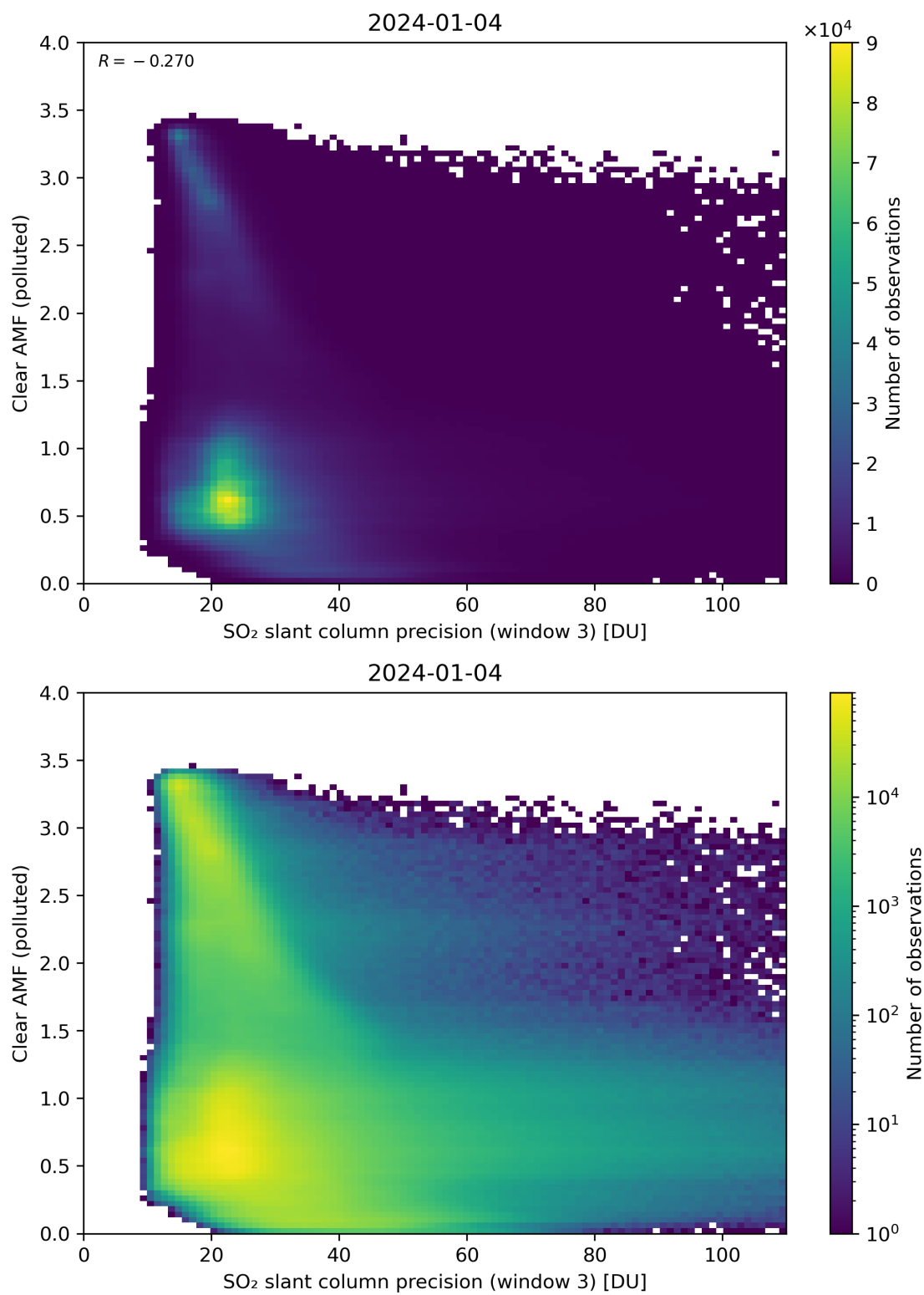
Figure 261: Scatter density plot of “SO 2 slant column precision (window 3)” against “Clear AMF (polluted)” for 2024-01-03 to 2024-01-05.
