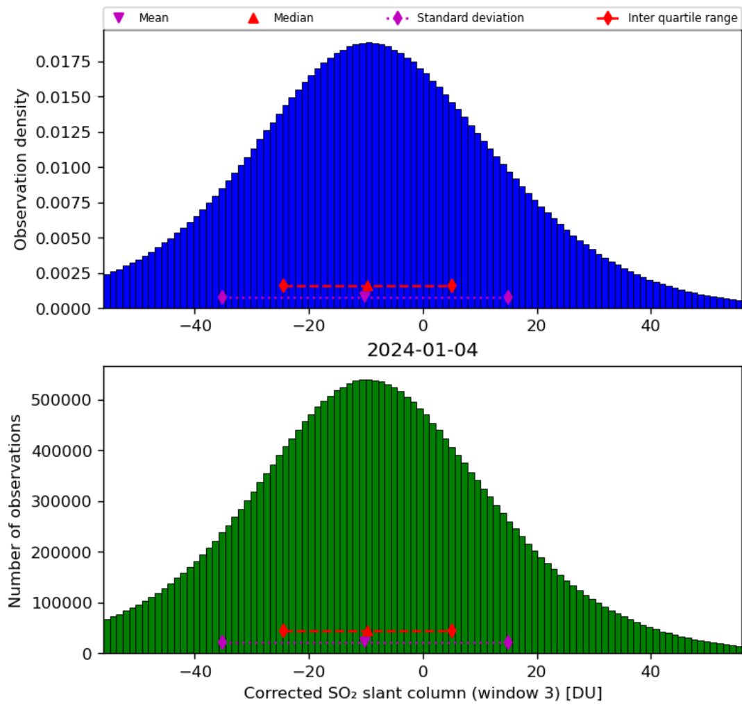
Figure 66: Histogram of “Corrected SO 2 slant column (window 3)” for 2024-01-03 to 2024-01-05
