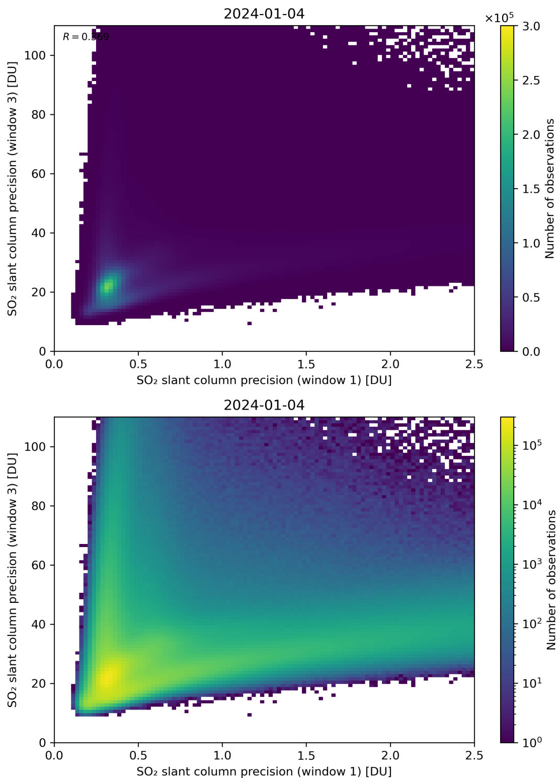
Figure 229: Scatter density plot of “SO 2 slant column precision (window 1)” against “SO 2 slant column precision (window 3)” for 2024-01-03 to 2024-01-05.
