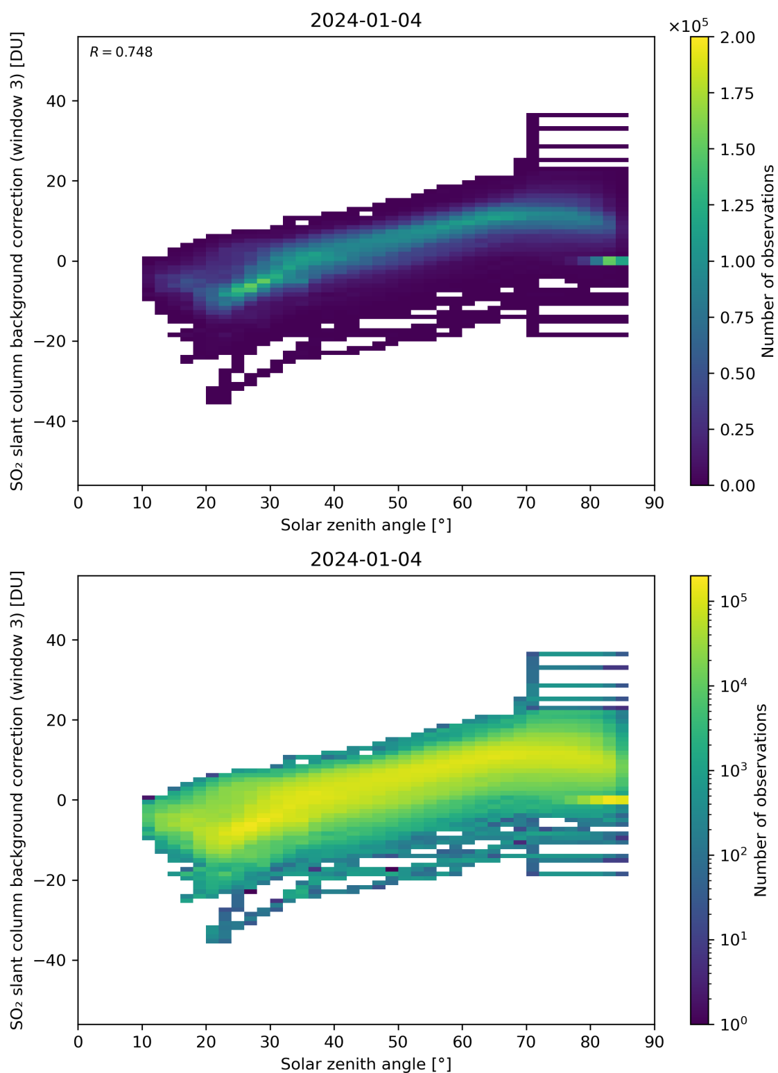
Figure 160: Scatter density plot of “Solar zenith angle” against “SO 2 slant column background correction (window 3)” for 2024-01-03 to 2024-01-05.
