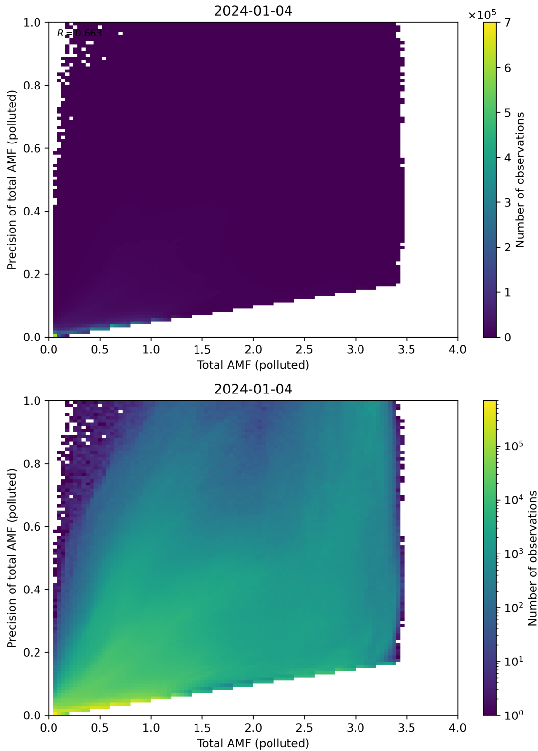
Figure 272: Scatter density plot of “Total AMF (polluted)” against “Precision of total AMF (polluted)” for 2024-01-03 to 2024-01-05.
