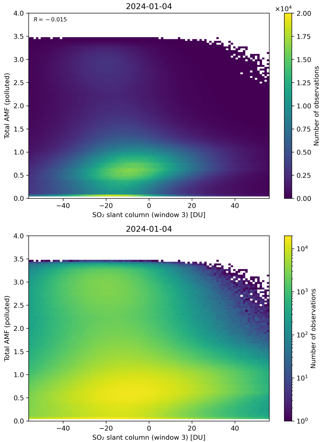
Figure 268: Scatter density plot of “SO 2 slant column (window 3)” against “Total AMF (polluted)” for 2024-01-03 to 2024-01-05.
