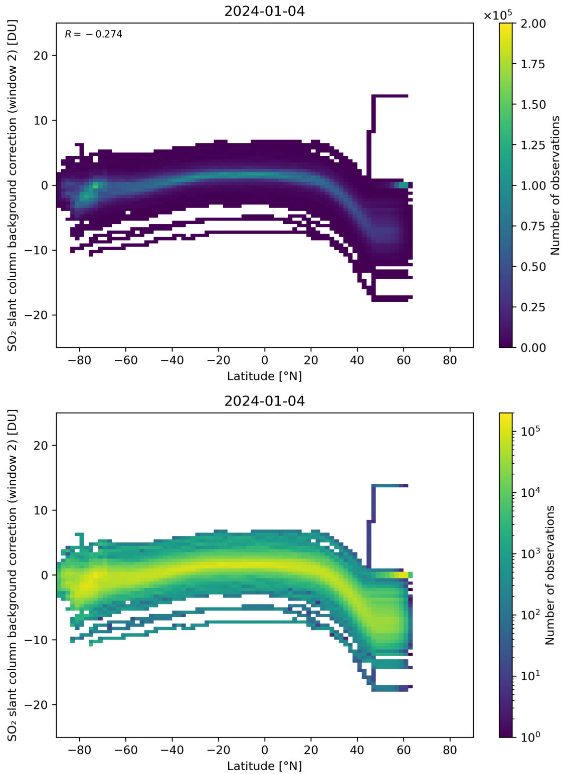
Figure 140: Scatter density plot of “Latitude” against “SO 2 slant column background correction (window 2)” for 2024-01-03 to 2024-01-05.
