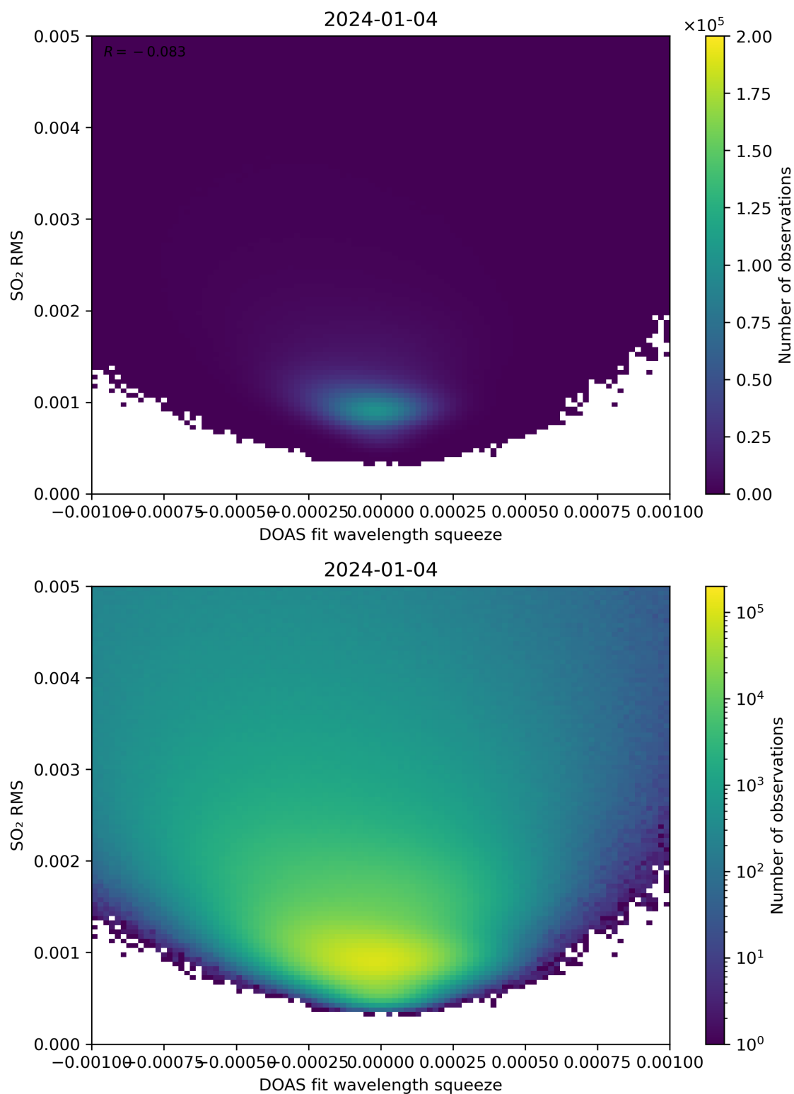
Figure 132: Scatter density plot of “DOAS fit wavelength squeeze” against “SO 2 RMS” for 2024-01-03 to 2024-01-05.
