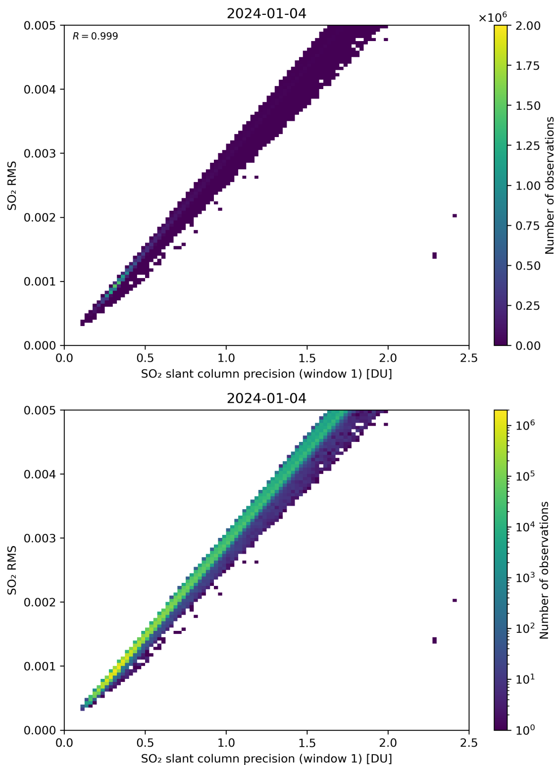
Figure 223: Scatter density plot of “SO 2 slant column precision (window 1)” against “SO 2 RMS” for 2024-01-03 to 2024-01-05.
