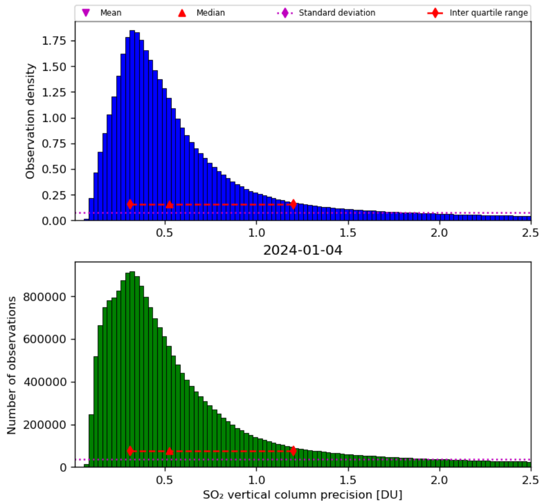
Figure 54: Histogram of “SO 2 vertical column precision” for 2024-01-03 to 2024-01-05
