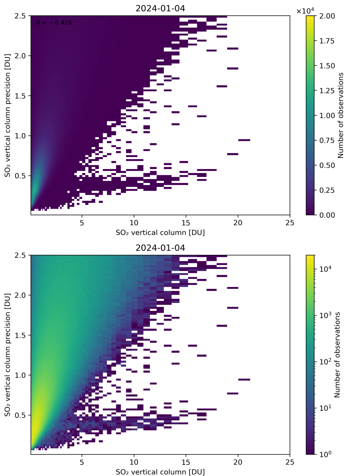
Figure 307: Scatter density plot of “SO 2 vertical column” against “SO 2 vertical column precision” for 2024-01-03 to 2024-01-05.
