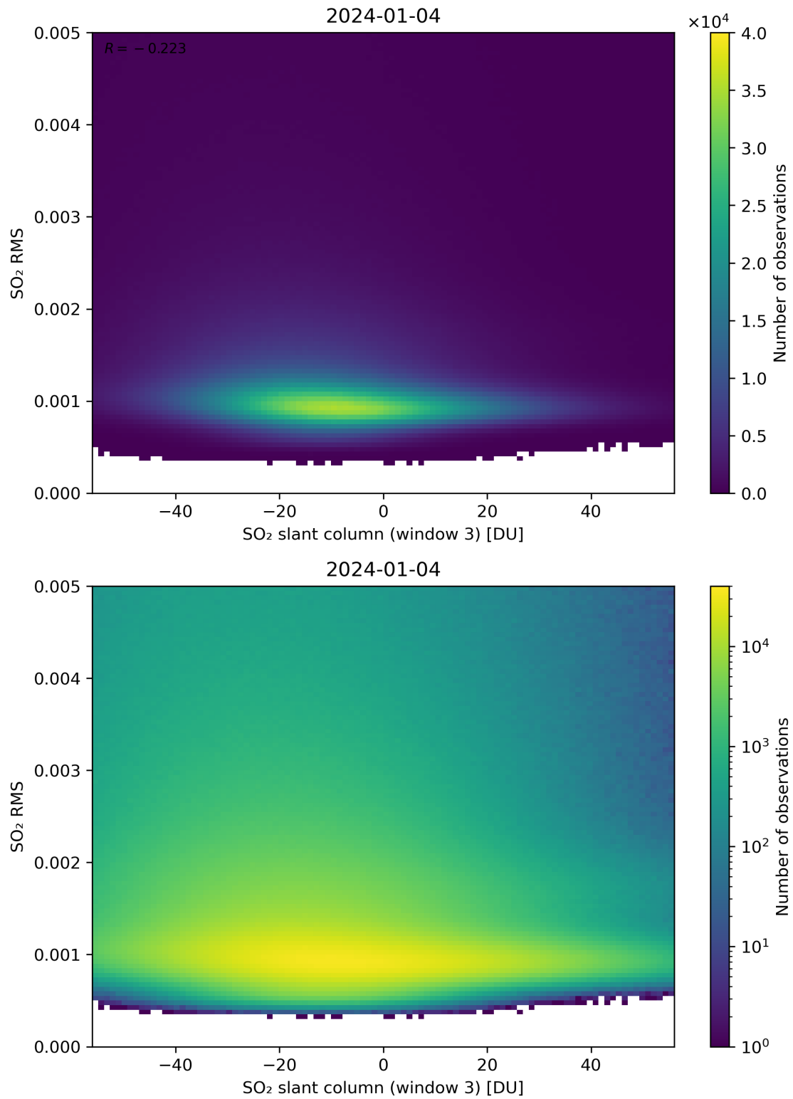
Figure 256: Scatter density plot of “SO 2 slant column (window 3)” against “SO 2 RMS” for 2024-01-03 to 2024-01-05.
