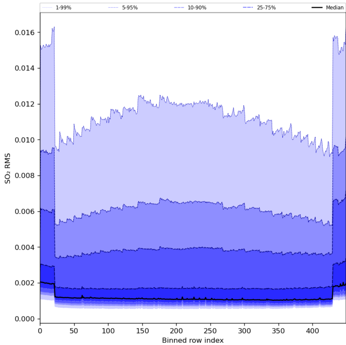
Figure 93: Along track statistics of “SO 2 RMS” for 2024-01-03 to 2024-01-05
