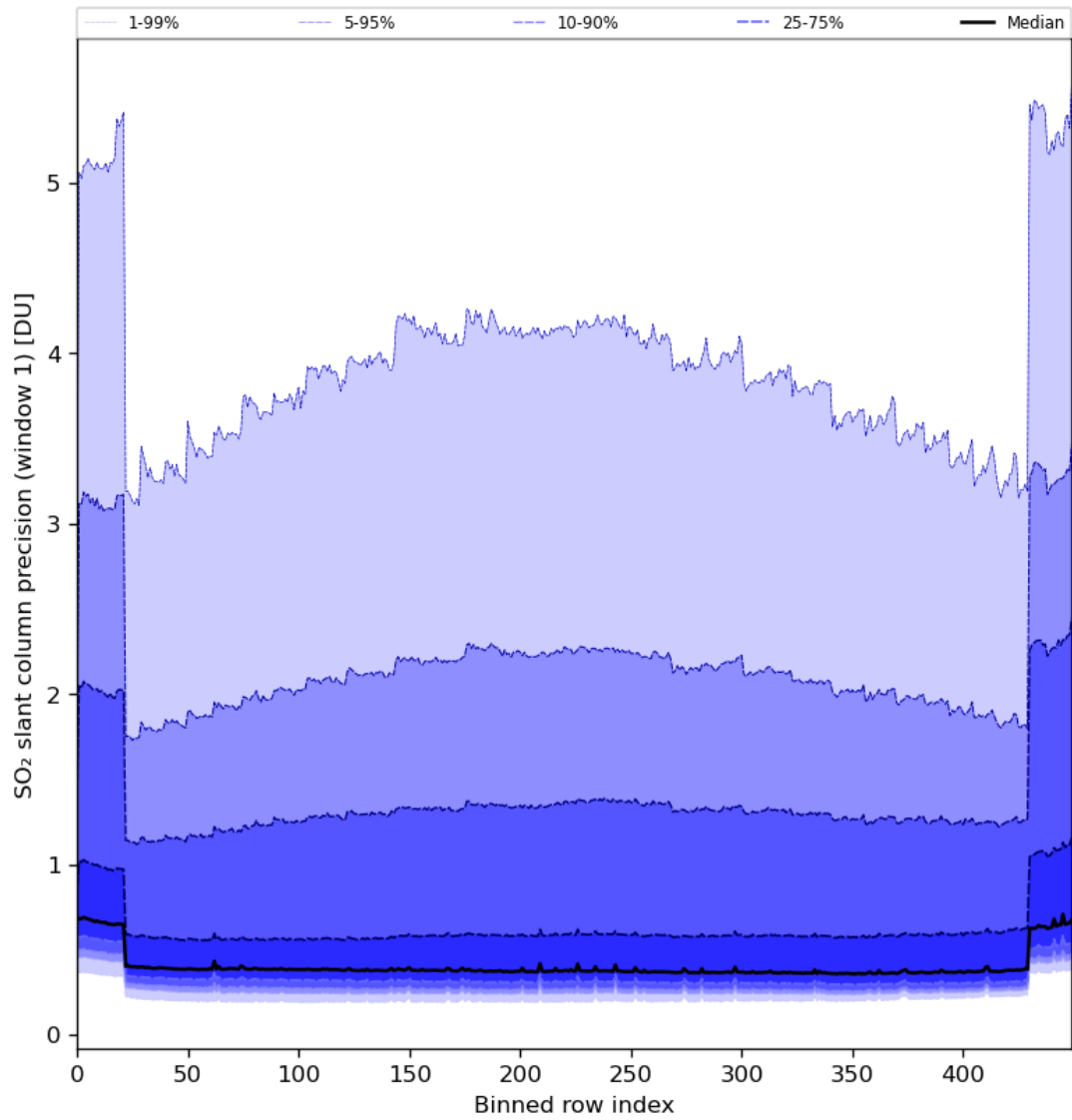
Figure 80: Along track statistics of “SO 2 slant column precision (window 1)” for 2024-01-03 to 2024-01-05
