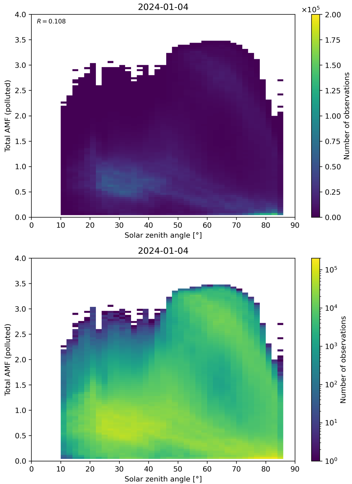
Figure 174: Scatter density plot of “Solar zenith angle” against “Total AMF (polluted)” for 2024-01-03 to 2024-01-05.
