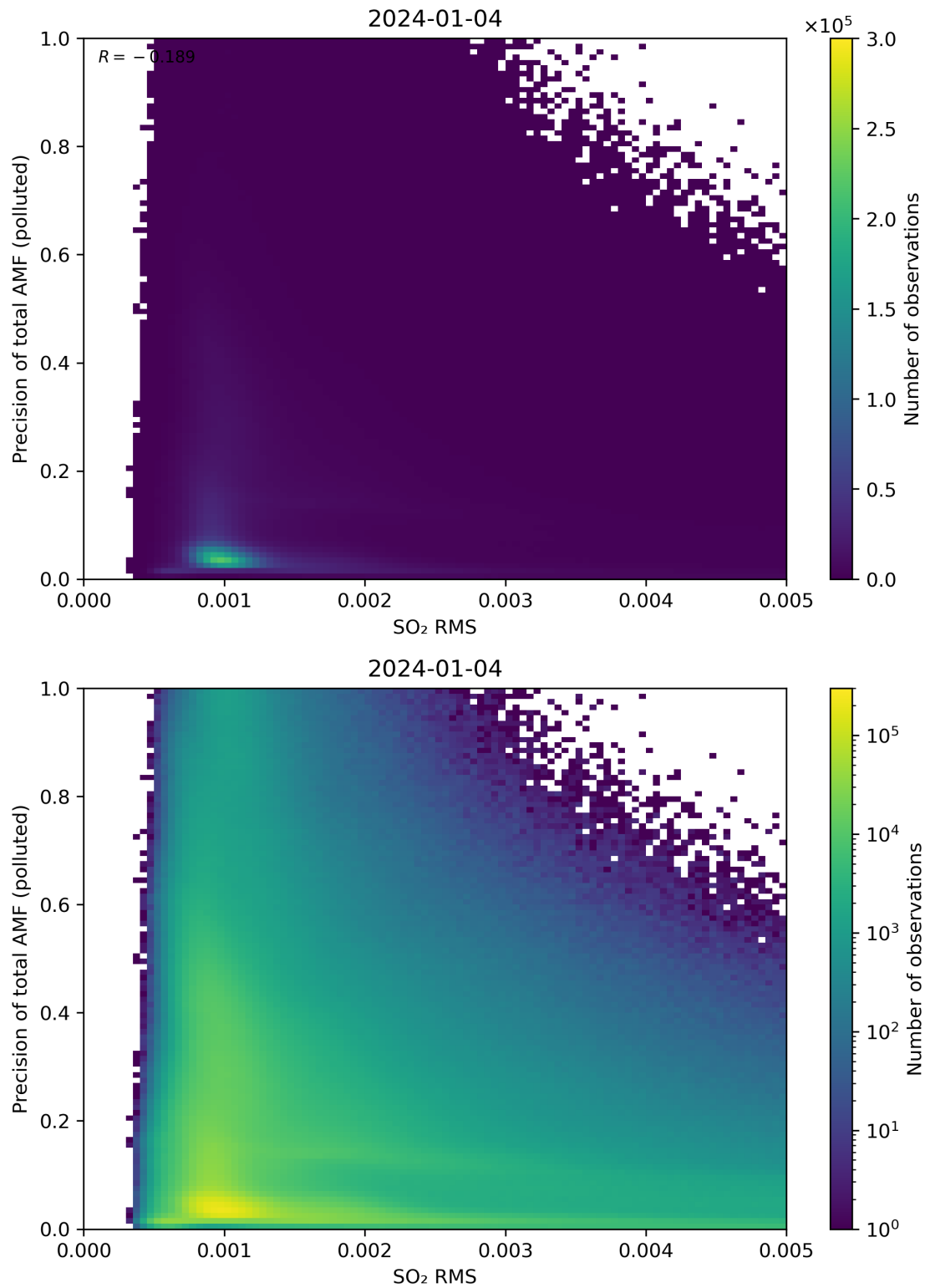
Figure 138: Scatter density plot of “SO 2 RMS” against “Precision of total AMF (polluted)” for 2024-01-03 to 2024-01-05.
