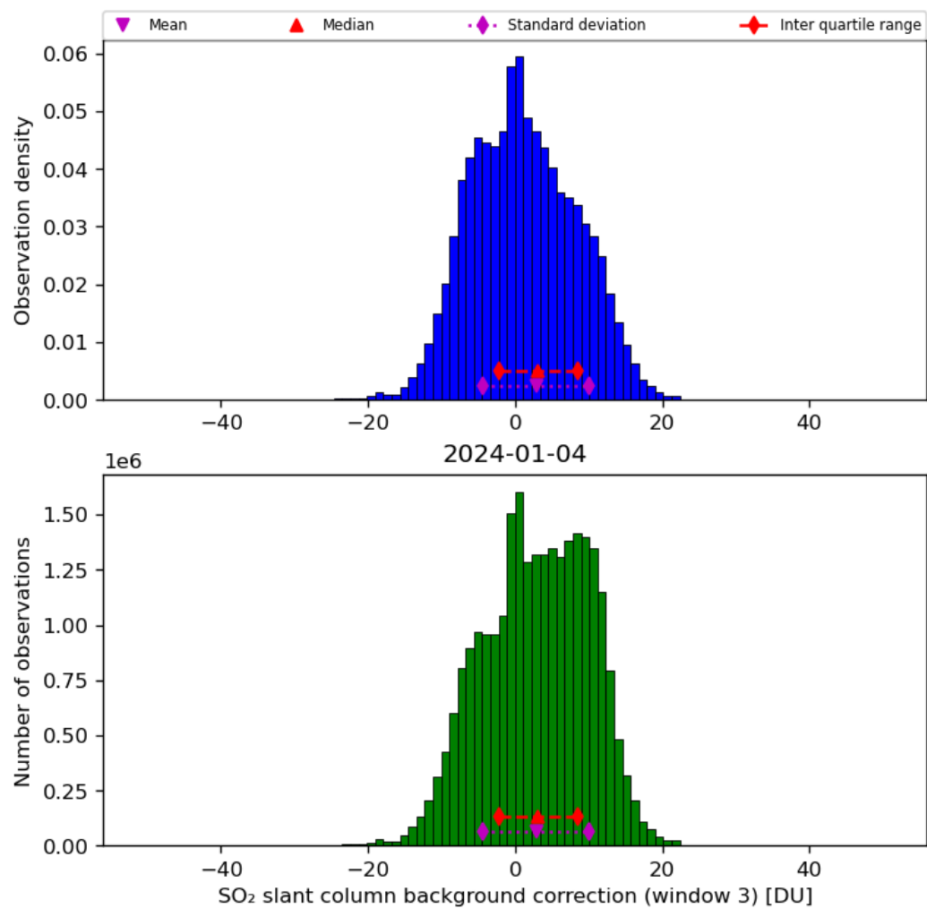
Figure 67: Histogram of “SO 2 slant column background correction (window 3)” for 2024-01-03 to 2024-01-05
