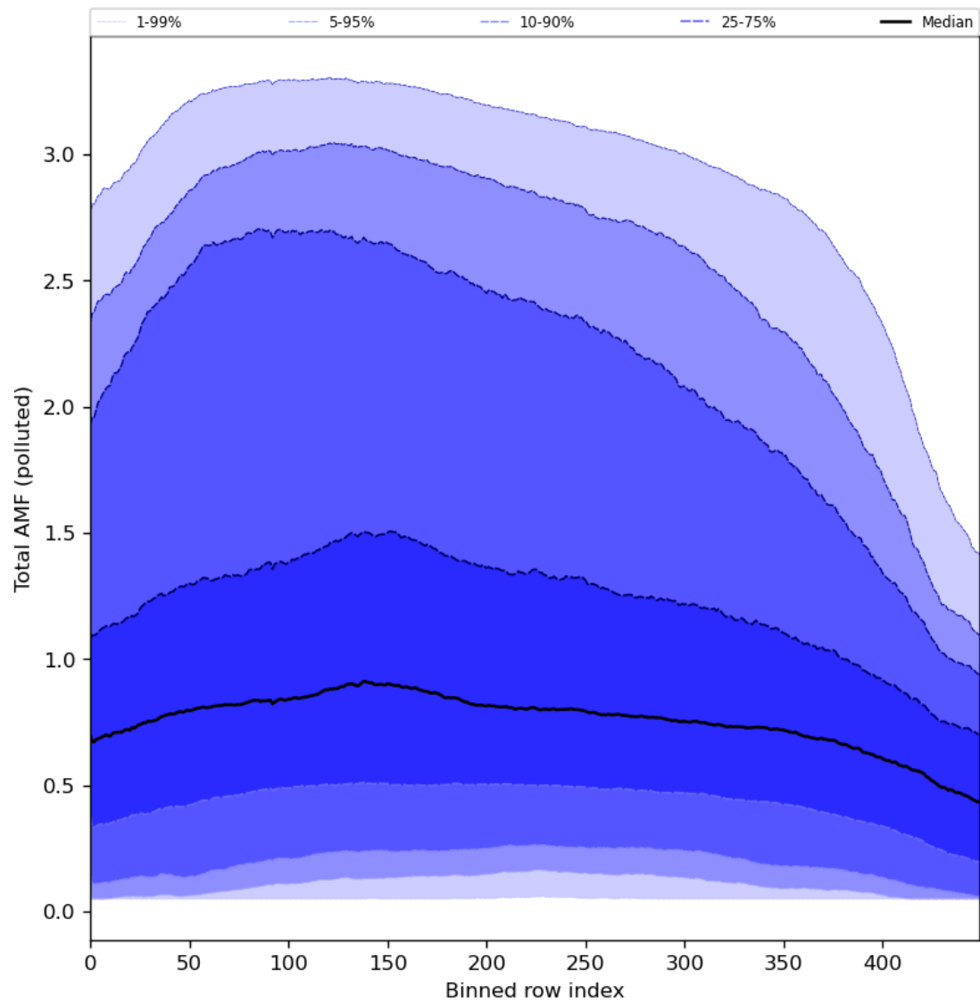
Figure 94: Along track statistics of “Total AMF (polluted)” for 2024-01-03 to 2024-01-05
