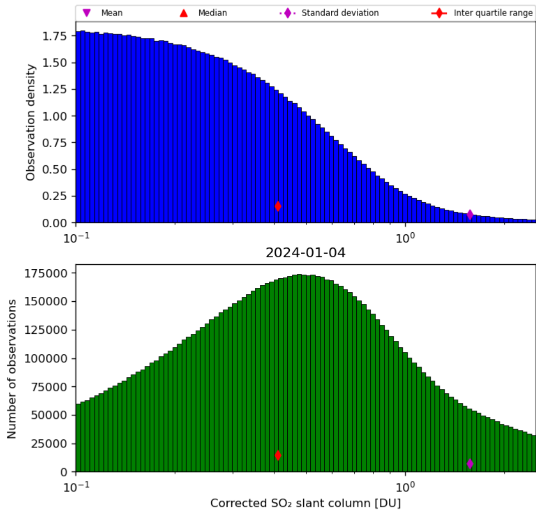
Figure 55: Histogram of “Corrected SO 2 slant column” for 2024-01-03 to 2024-01-05
