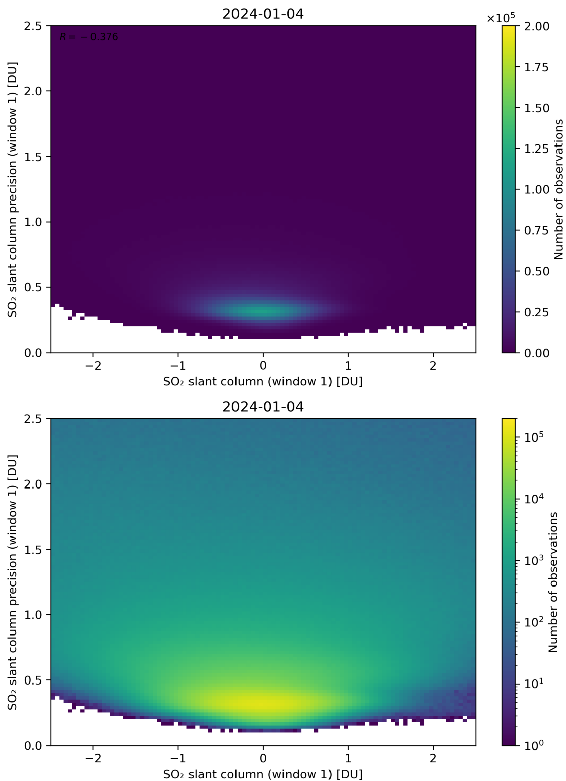
Figure 235: Scatter density plot of “SO 2 slant column (window 1)” against “SO 2 slant column precision (window 1)” for 2024-01-03 to 2024-01-05.
