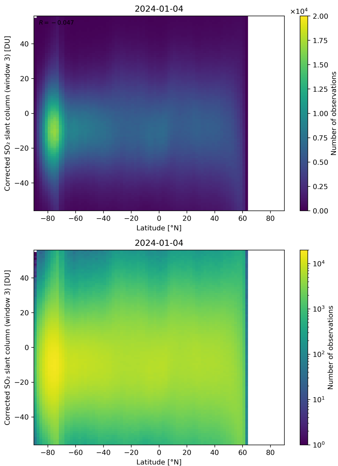
Figure 148: Scatter density plot of “Latitude” against “Corrected SO 2 slant column (window 3)” for 2024-01-03 to 2024-01-05.
