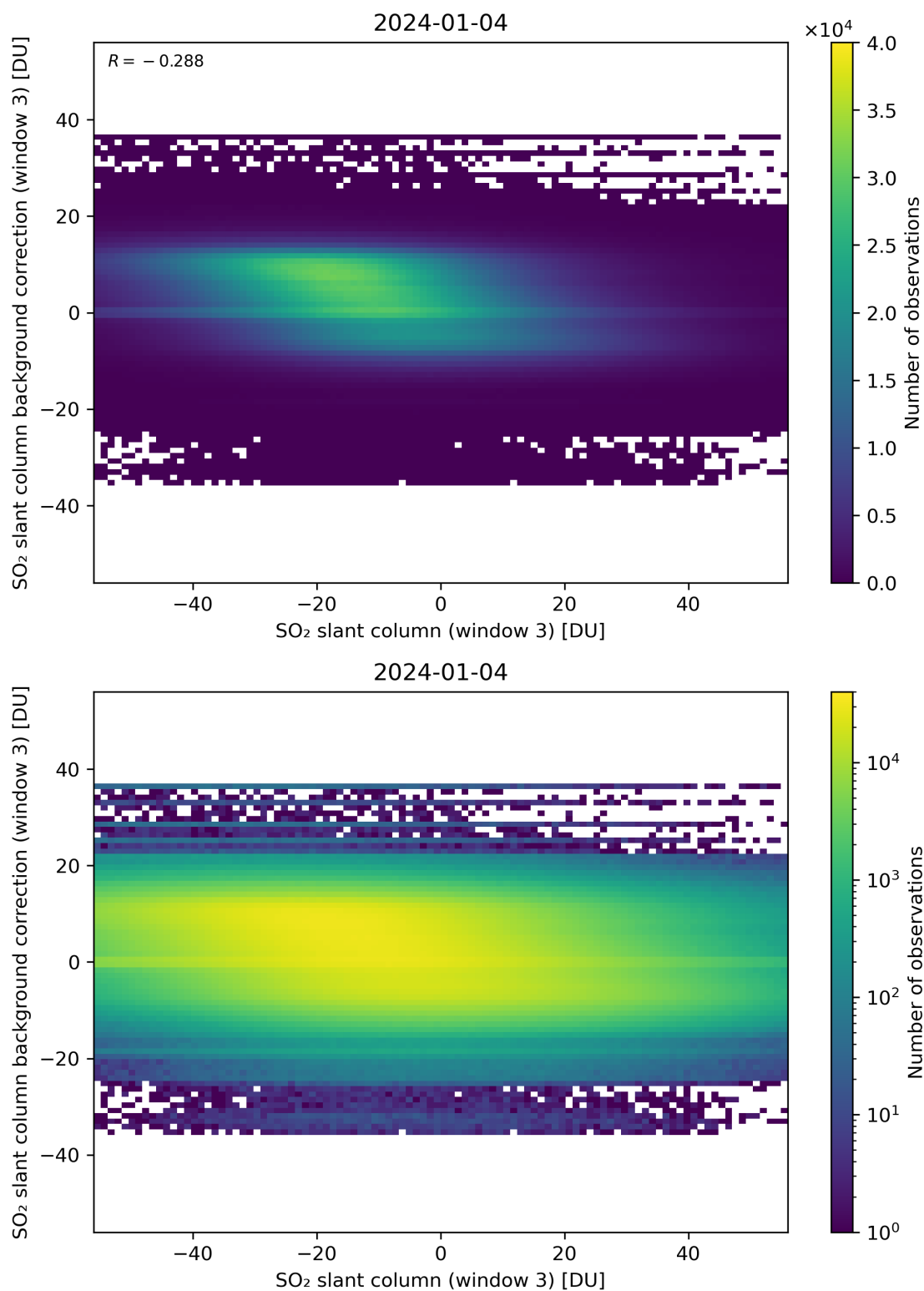
Figure 253: Scatter density plot of “SO 2 slant column (window 3)” against “SO 2 slant column background correction (window 3)” for 2024-01-03 to 2024-01-05.
