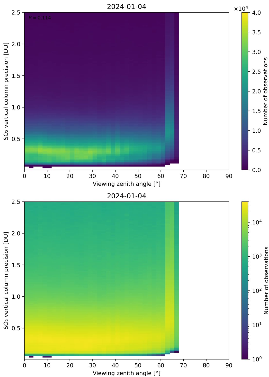
Figure 328: Scatter density plot of “Viewing zenith angle” against “SO 2 vertical column precision” for 2024-01-03 to 2024-01-05.
