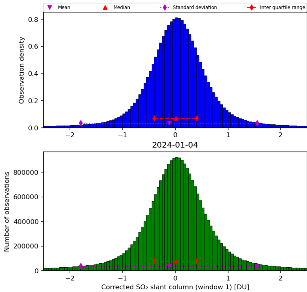
Figure 58: Histogram of “Corrected SO 2 slant column (window 1)” for 2024-01-03 to 2024-01-05
