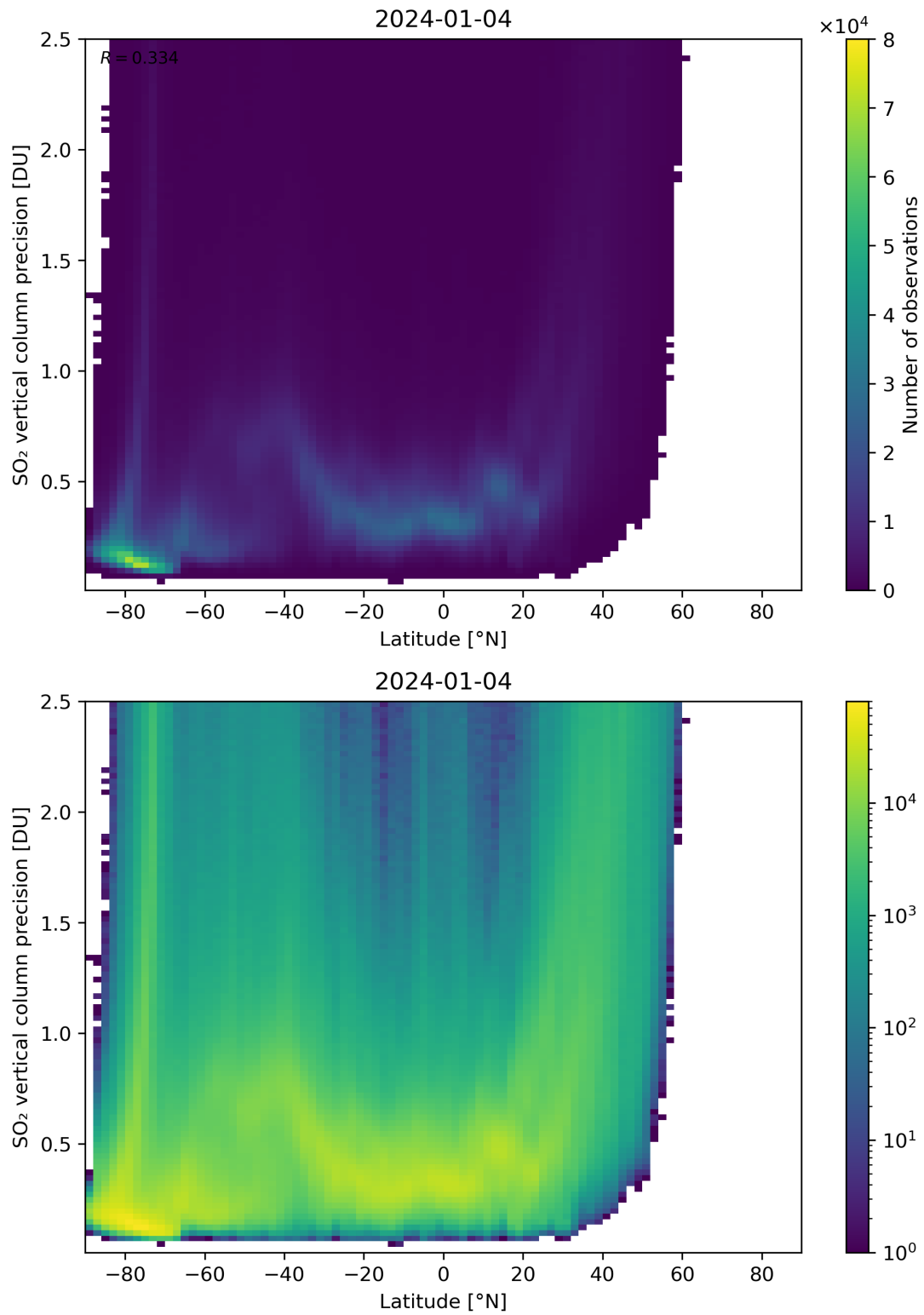
Figure 157: Scatter density plot of “Latitude” against “SO 2 vertical column precision” for 2024-01-03 to 2024-01-05.
