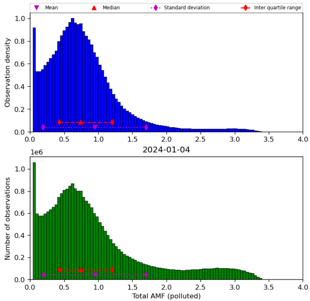
Figure 71: Histogram of “Total AMF (polluted)” for 2024-01-03 to 2024-01-05
