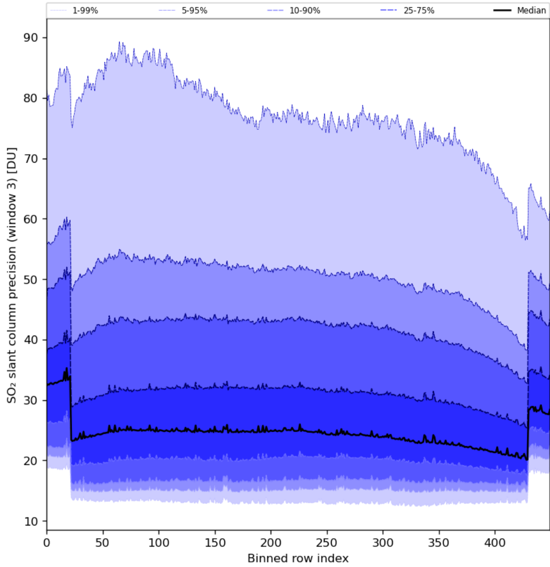
Figure 88: Along track statistics of “SO 2 slant column precision (window 3)” for 2024-01-03 to 2024-01-05
