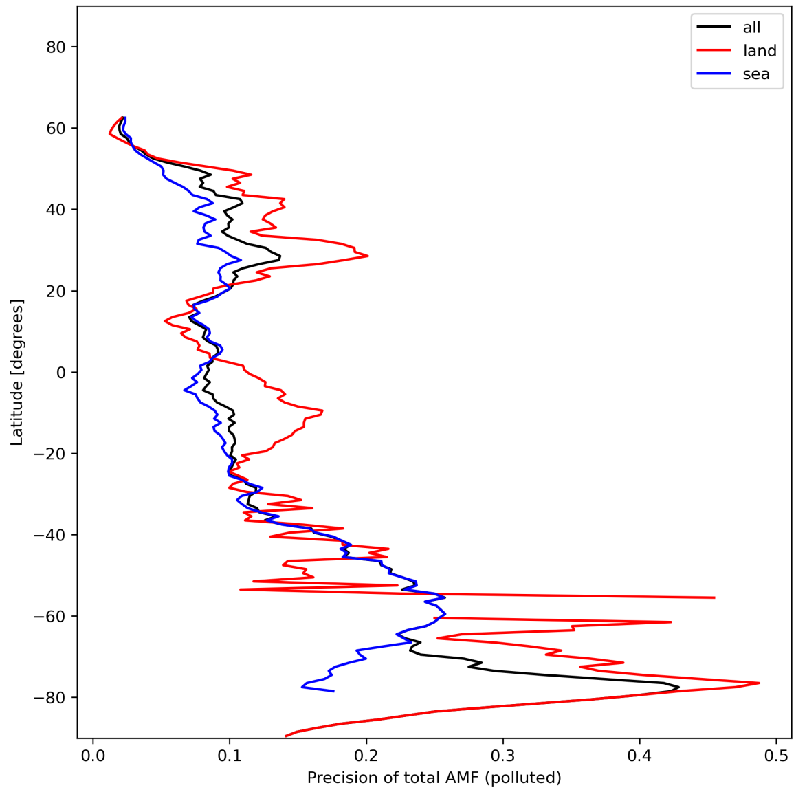
Figure 49: Zonal average of “Precision of total AMF (polluted)” for 2024-01-03 to 2024-01-05.
