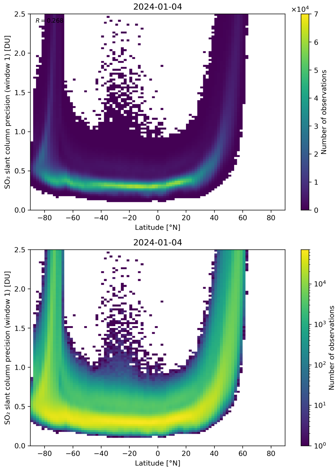
Figure 150: Scatter density plot of “Latitude” against “SO 2 slant column precision (window 1)” for 2024-01-03 to 2024-01-05.
