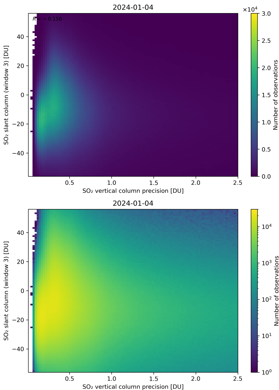
Figure 292: Scatter density plot of “SO 2 vertical column precision” against “SO 2 slant column (window 3)” for 2024-01-03 to 2024-01-05.
