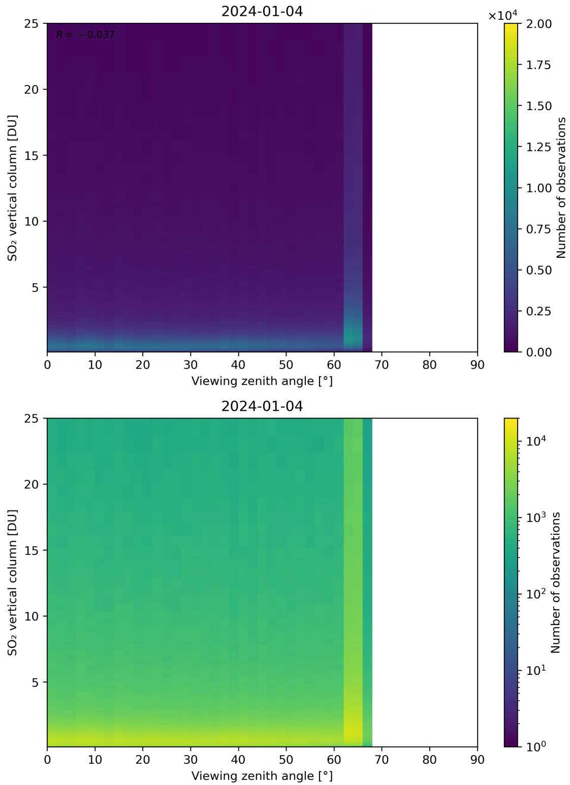
Figure 327: Scatter density plot of “Viewing zenith angle” against “SO 2 vertical column” for 2024-01-03 to 2024-01-05.
