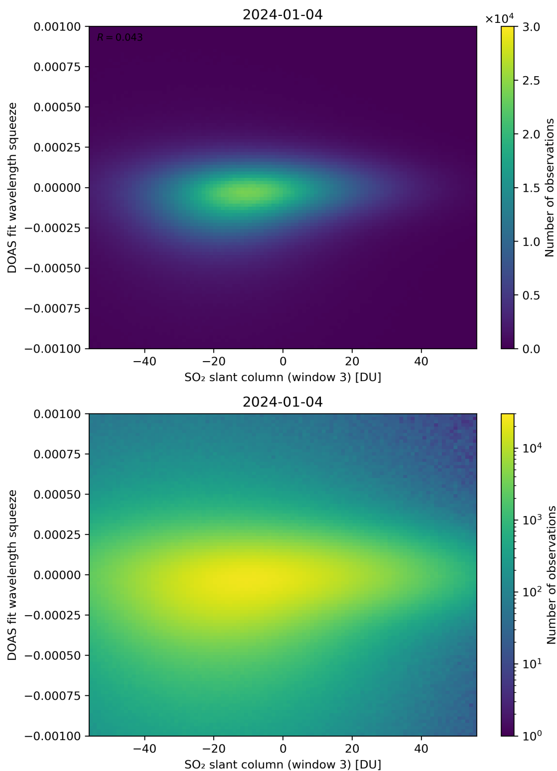
Figure 255: Scatter density plot of “SO 2 slant column (window 3)” against “DOAS fit wavelength squeeze” for 2024-01-03 to 2024-01-05.
