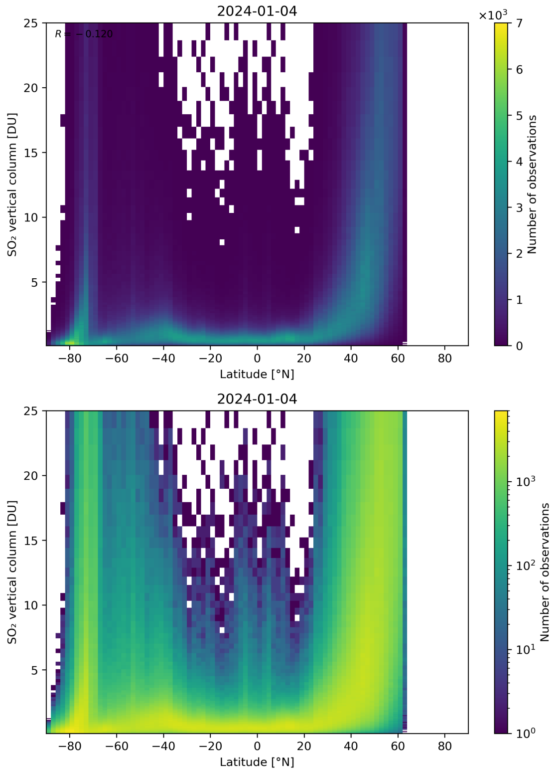
Figure 156: Scatter density plot of “Latitude” against “SO 2 vertical column” for 2024-01-03 to 2024-01-05.
