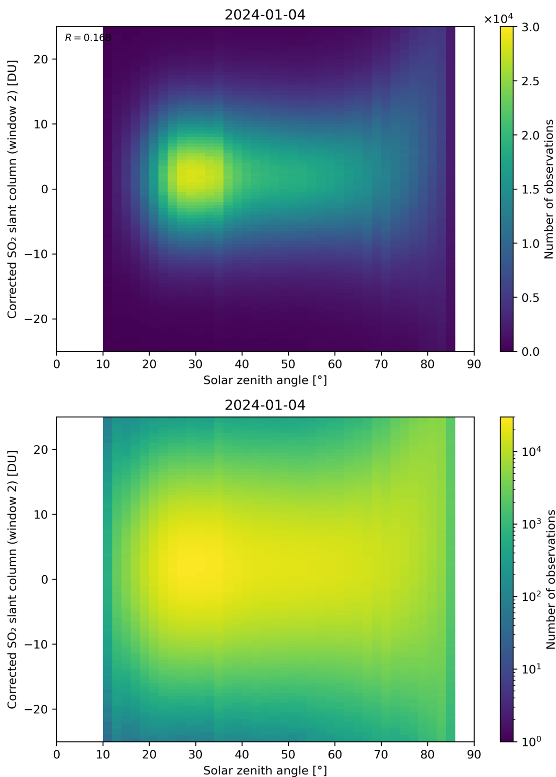
Figure 167: Scatter density plot of “Solar zenith angle” against “Corrected SO 2 slant column (window 2)” for 2024-01-03 to 2024-01-05.
