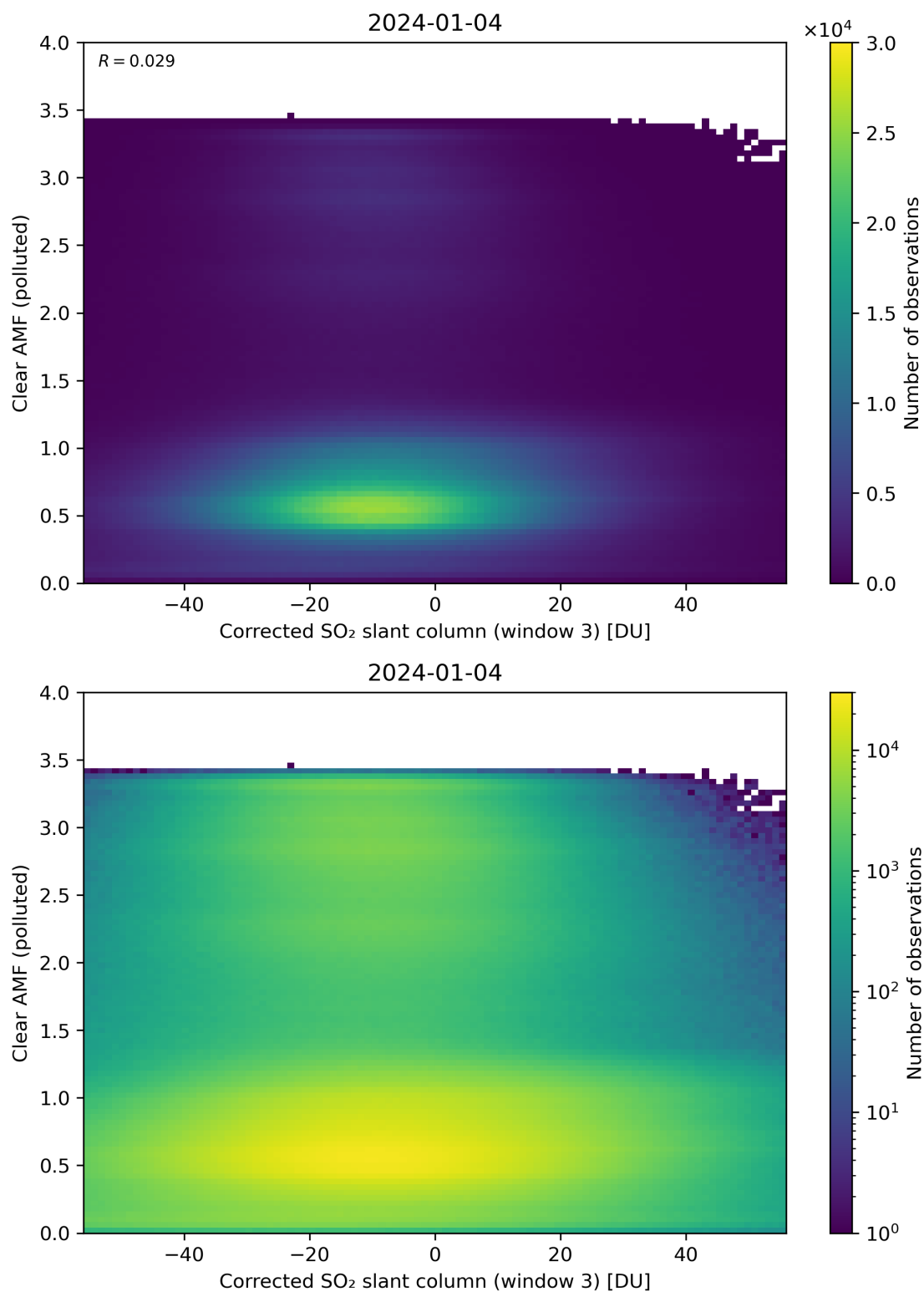
Figure 209: Scatter density plot of “Corrected SO 2 slant column (window 3)” against “Clear AMF (polluted)” for 2024-01-03 to 2024-01-05.
