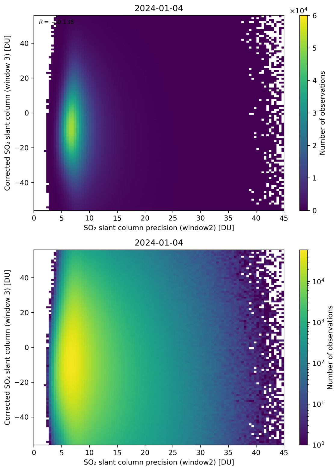
Figure 248: Scatter density plot of “SO 2 slant column precision (window2)” against “Corrected SO 2 slant column (window 3)” for 2024-01-03 to 2024-01-05.
