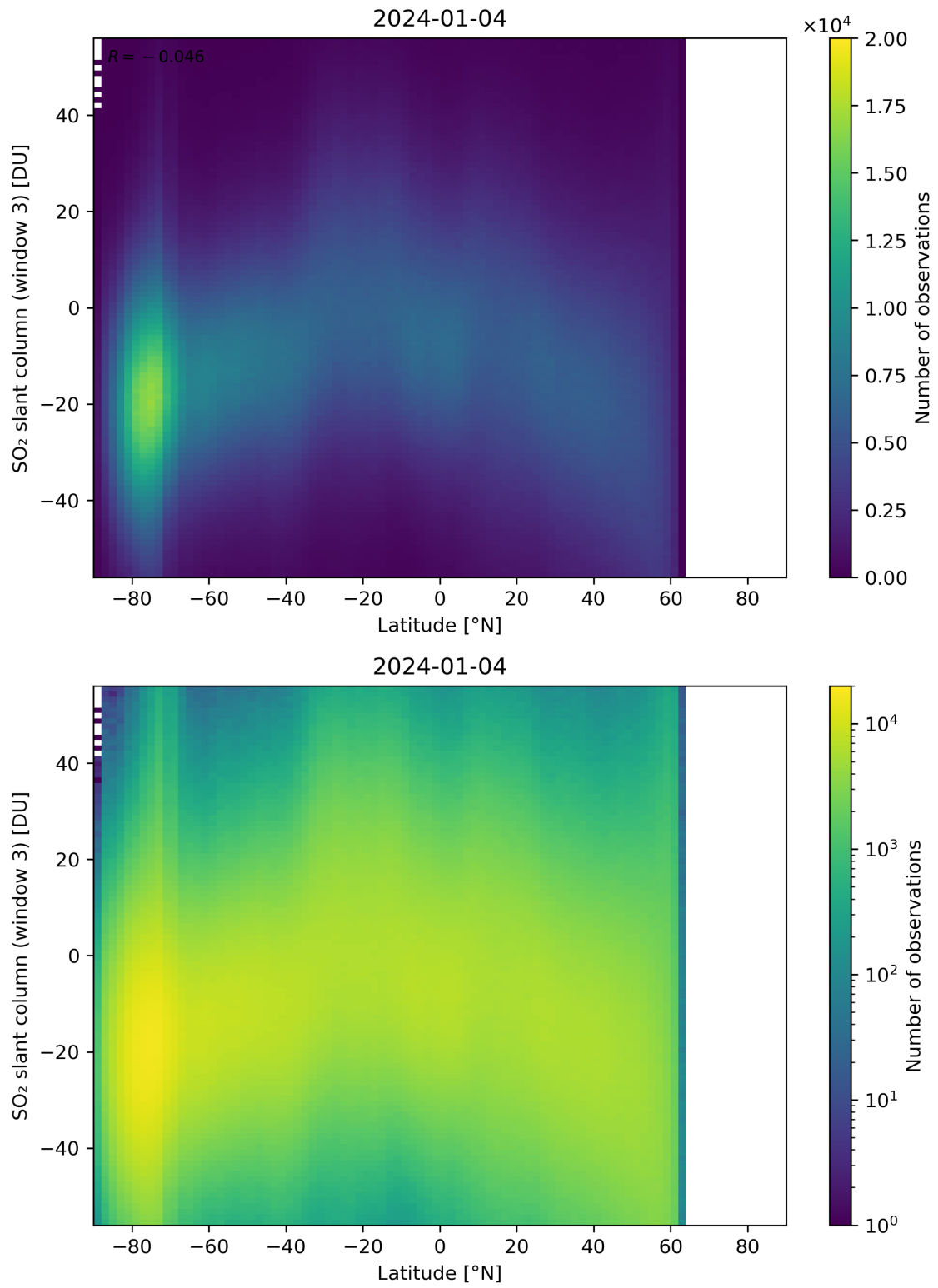
Figure 152: Scatter density plot of “Latitude” against “SO 2 slant column (window 3)” for 2024-01-03 to 2024-01-05.
