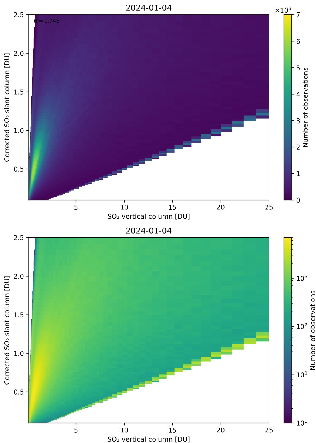
Figure 297: Scatter density plot of “SO 2 vertical column” against “Corrected SO 2 slant column” for 2024-01-03 to 2024-01-05.
