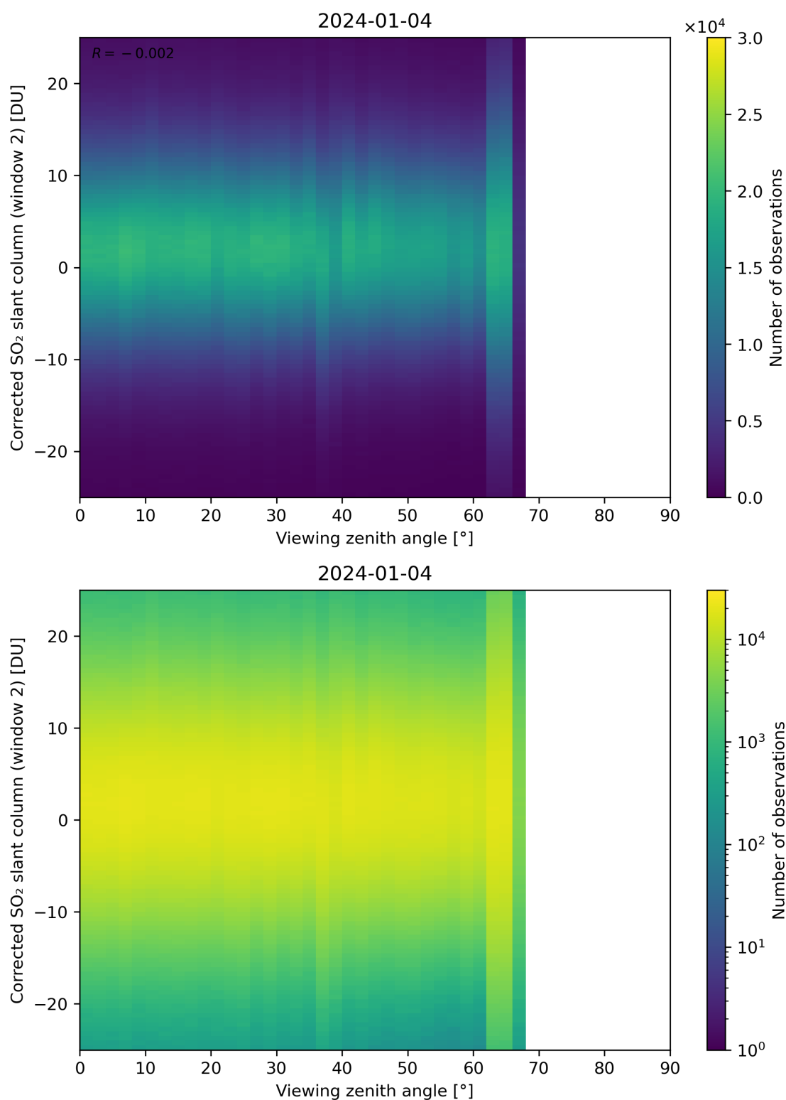
Figure 318: Scatter density plot of “Viewing zenith angle” against “Corrected SO 2 slant column (window 2)” for 2024-01-03 to 2024-01-05.
