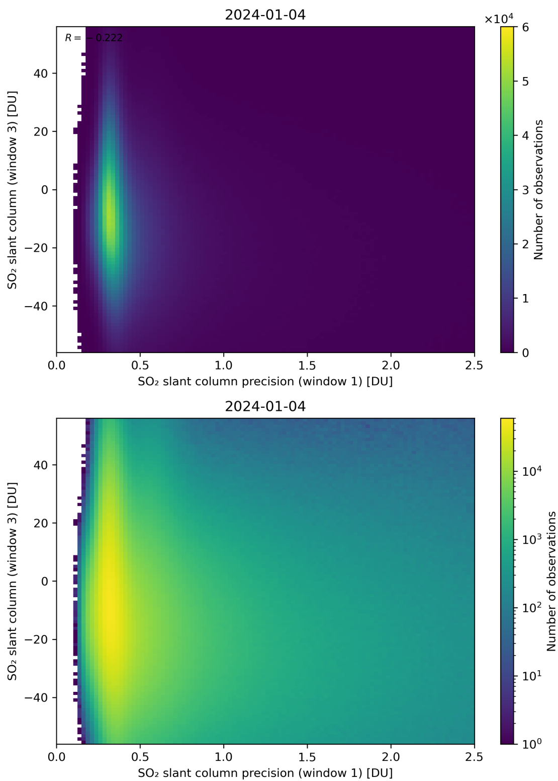
Figure 228: Scatter density plot of “SO 2 slant column precision (window 1)” against “SO 2 slant column (window 3)” for 2024-01-03 to 2024-01-05.
