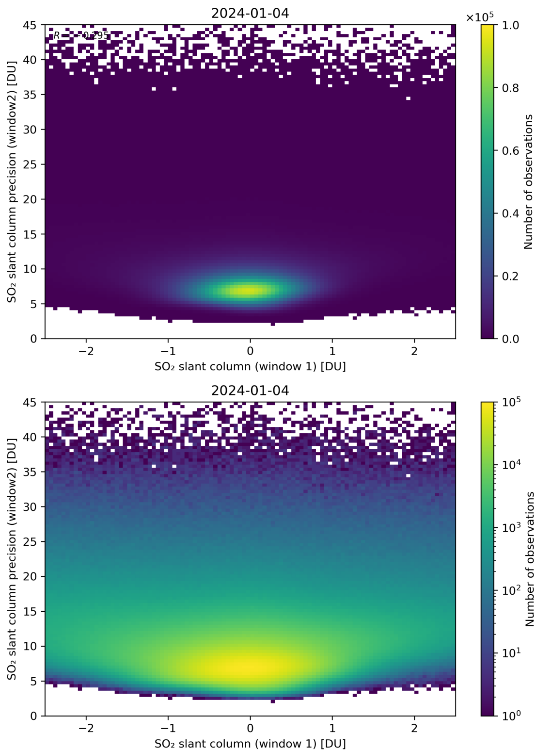
Figure 236: Scatter density plot of “SO 2 slant column (window 1)” against “SO 2 slant column precision (window2)” for 2024-01-03 to 2024-01-05.
