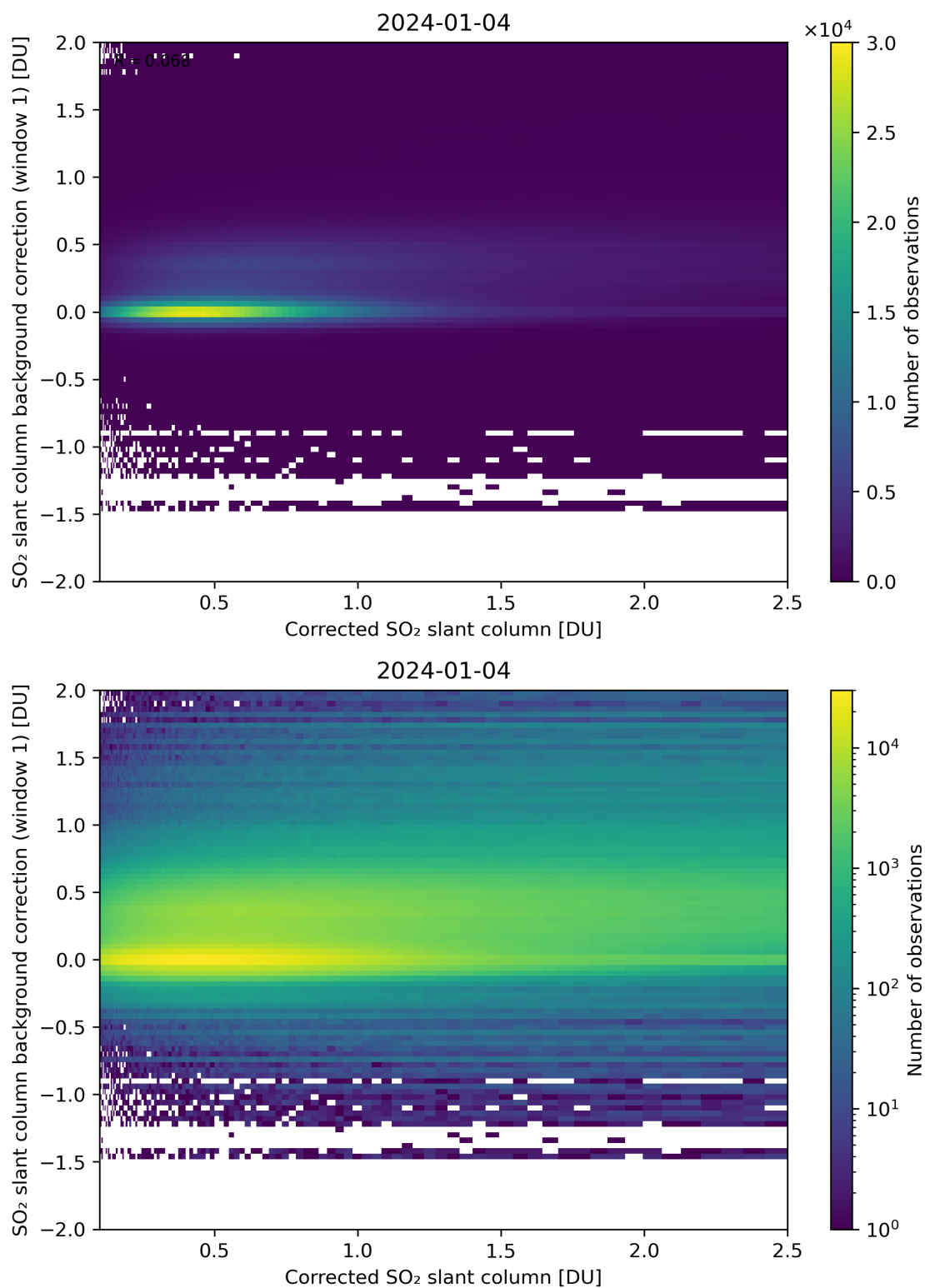
Figure 178: Scatter density plot of “Corrected SO 2 slant column” against “SO 2 slant column background correction (window 1)” for 2024-01-03 to 2024-01-05.
