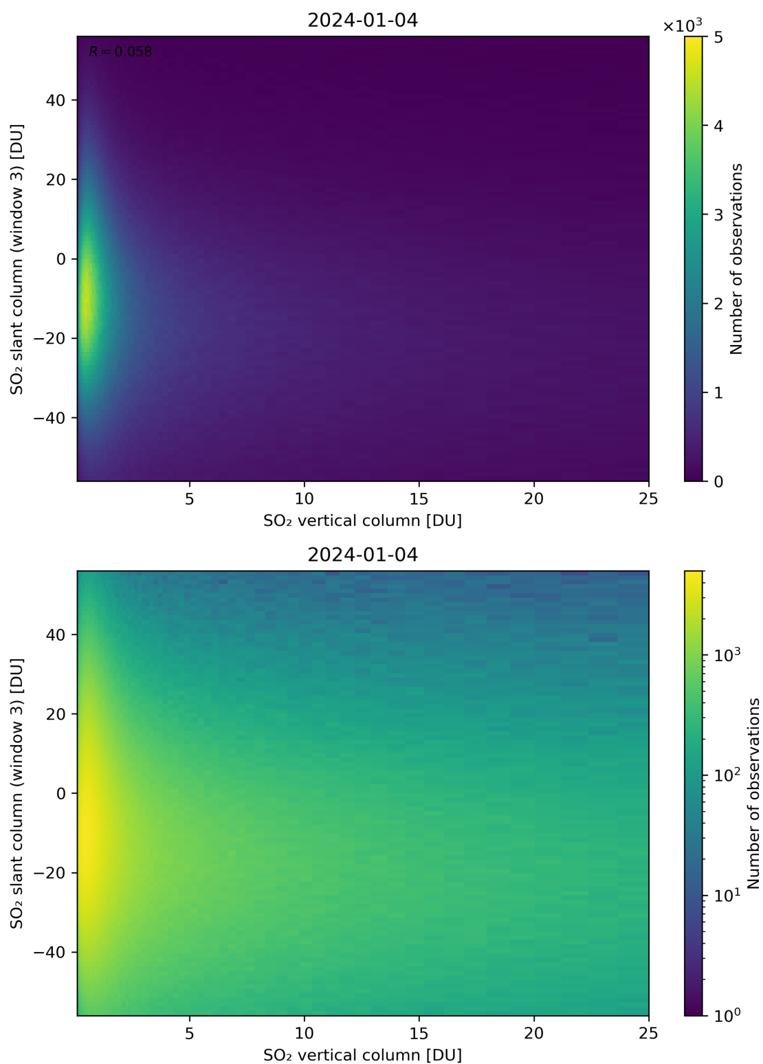
Figure 303: Scatter density plot of “SO 2 vertical column” against “SO 2 slant column (window 3)” for 2024-01-03 to 2024-01-05.
