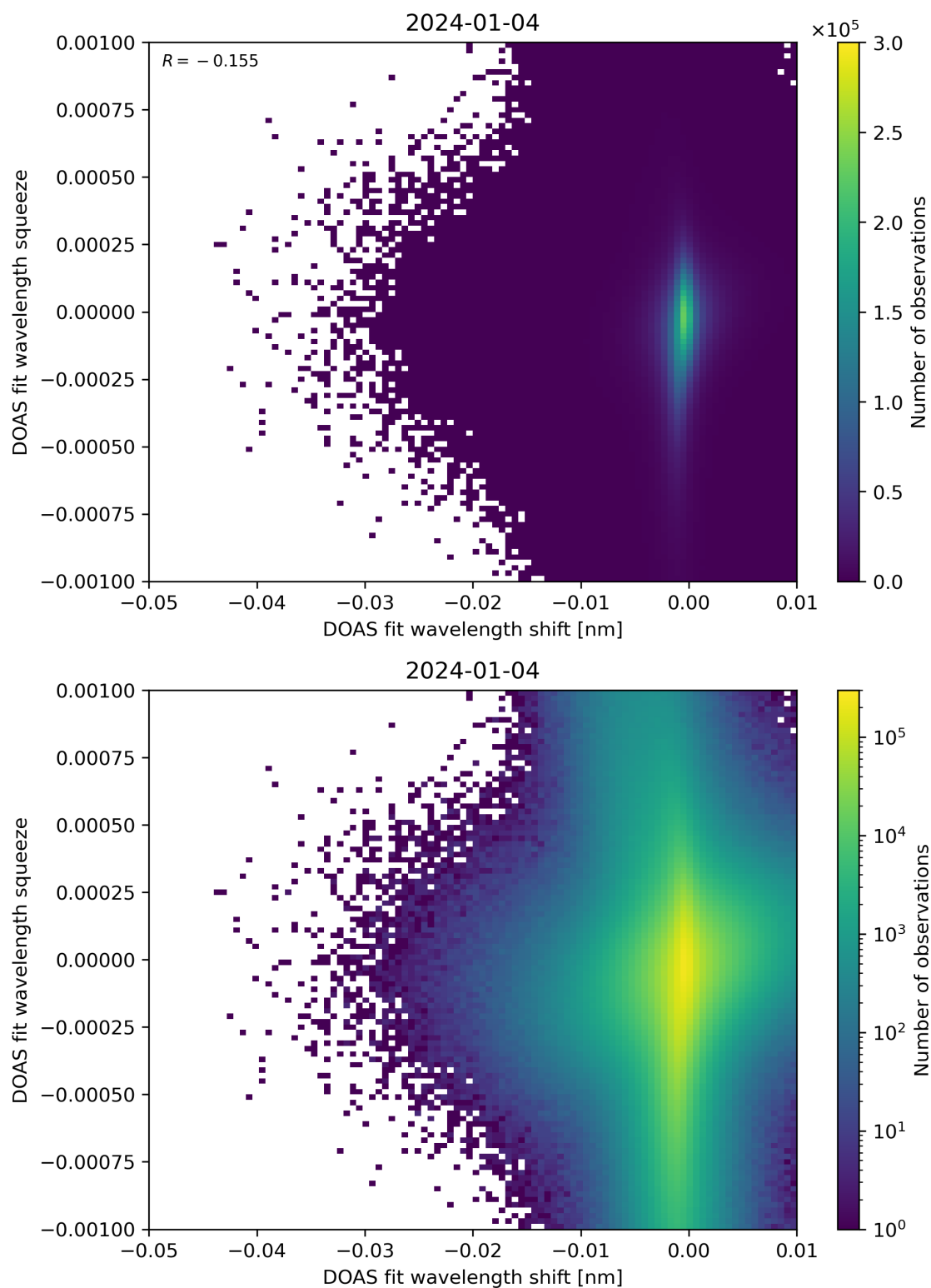
Figure 127: Scatter density plot of “DOAS fit wavelength shift” against “DOAS fit wavelength squeeze” for 2024-01-03 to 2024-01-05.
