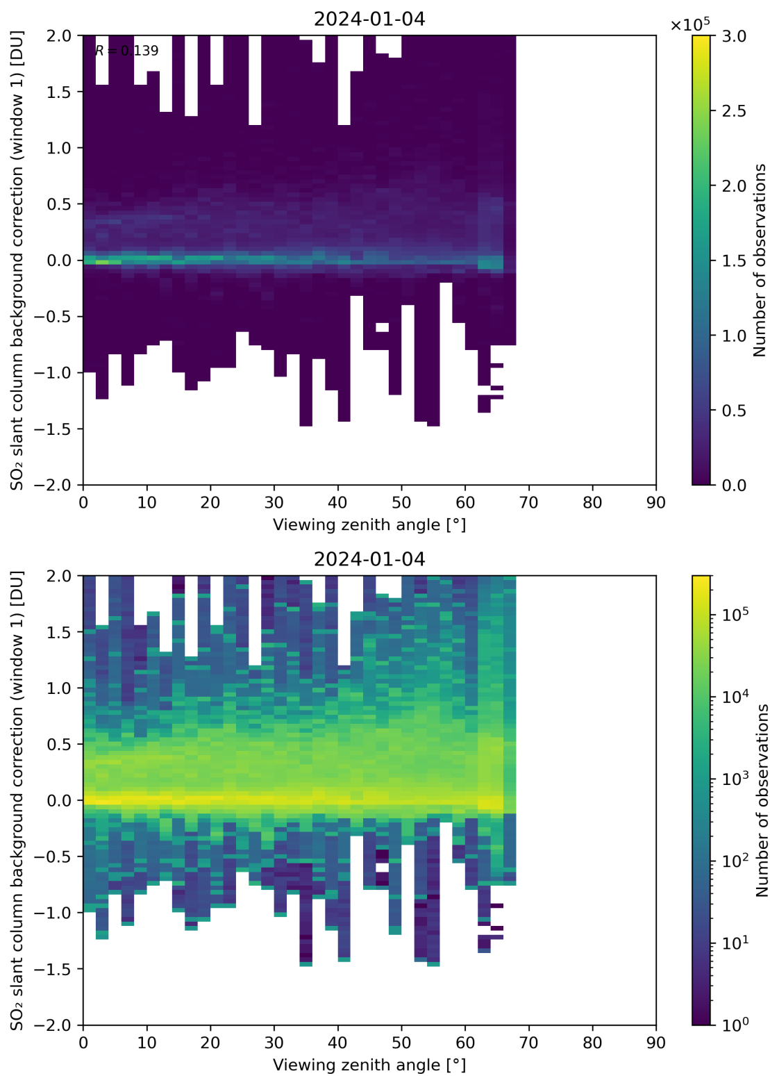
Figure 308: Scatter density plot of “Viewing zenith angle” against “SO 2 slant column background correction (window 1)” for 2024-01-03 to 2024-01-05.
