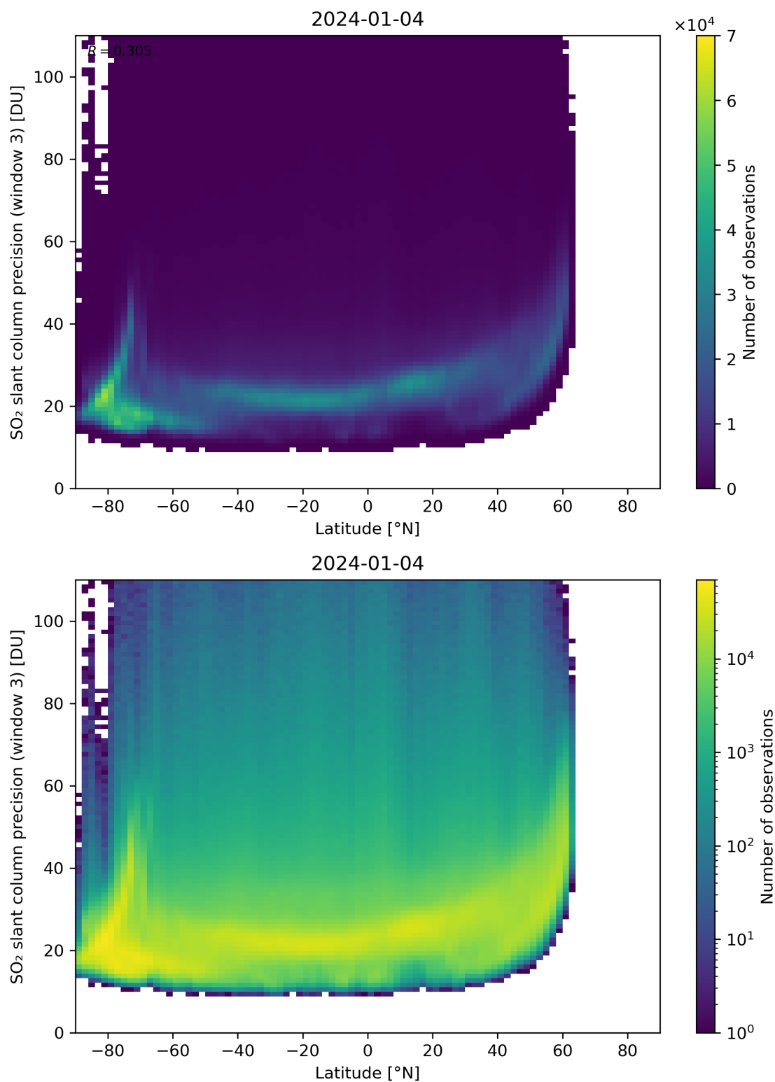
Figure 153: Scatter density plot of “Latitude” against “SO 2 slant column precision (window 3)” for 2024-01-03 to 2024-01-05.
