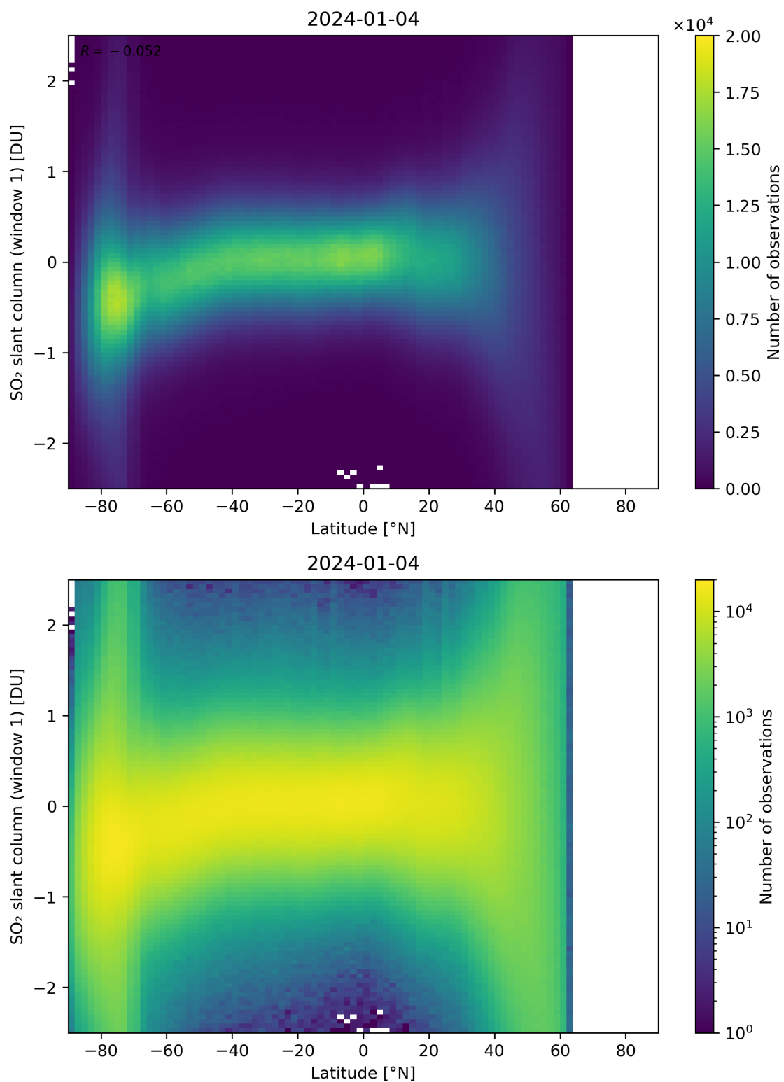
Figure 149: Scatter density plot of “Latitude” against “SO 2 slant column (window 1)” for 2024-01-03 to 2024-01-05.
