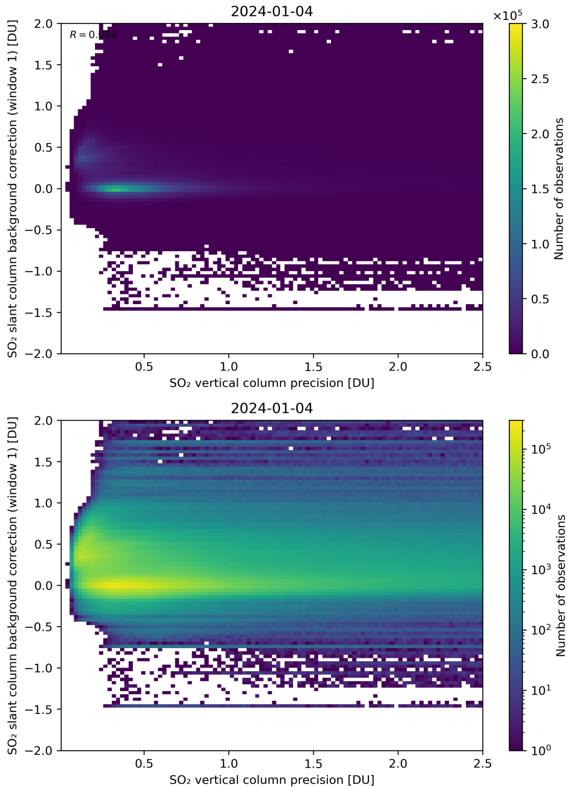
Figure 279: Scatter density plot of “SO 2 vertical column precision” against “SO 2 slant column background correction (window 1)” for 2024-01-03 to 2024-01-05.
