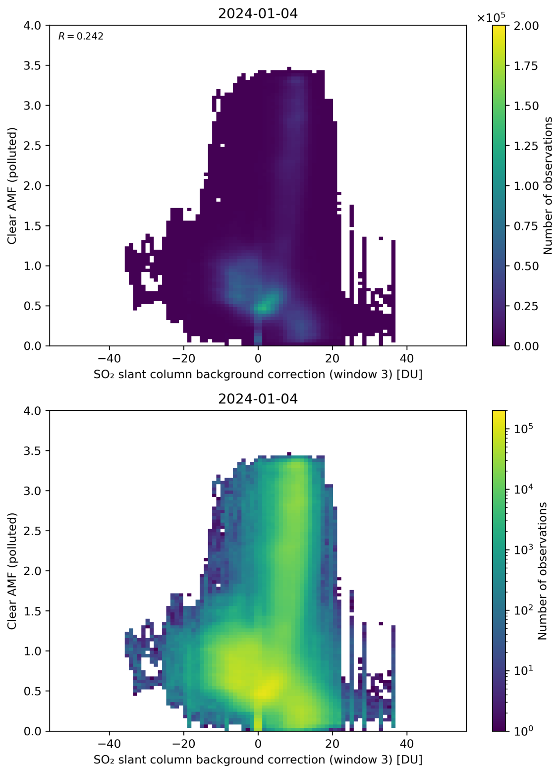
Figure 124: Scatter density plot of “SO 2 slant column background correction (window 3)” against “Clear AMF (polluted)” for 2024-01-03 to 2024-01-05.
