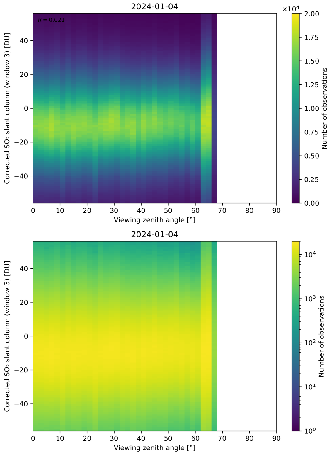
Figure 319: Scatter density plot of “Viewing zenith angle” against “Corrected SO 2 slant column (window 3)” for 2024-01-03 to 2024-01-05.
