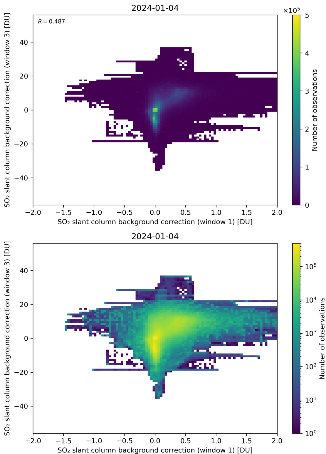
Figure 99: Scatter density plot of “SO 2 slant column background correction (window 1)” against “SO 2 slant column background correction (window 3)” for 2024-01-03 to 2024-01-05.
