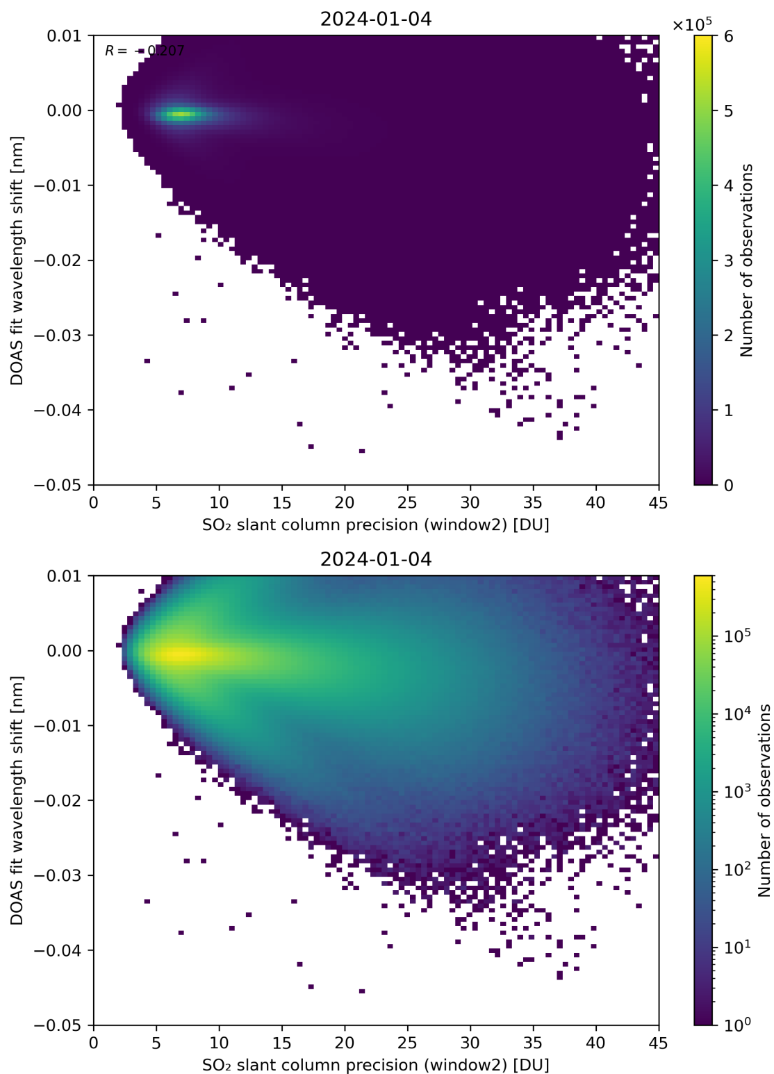
Figure 243: Scatter density plot of “SO 2 slant column precision (window2)” against “DOAS fit wavelength shift” for 2024-01-03 to 2024-01-05.
