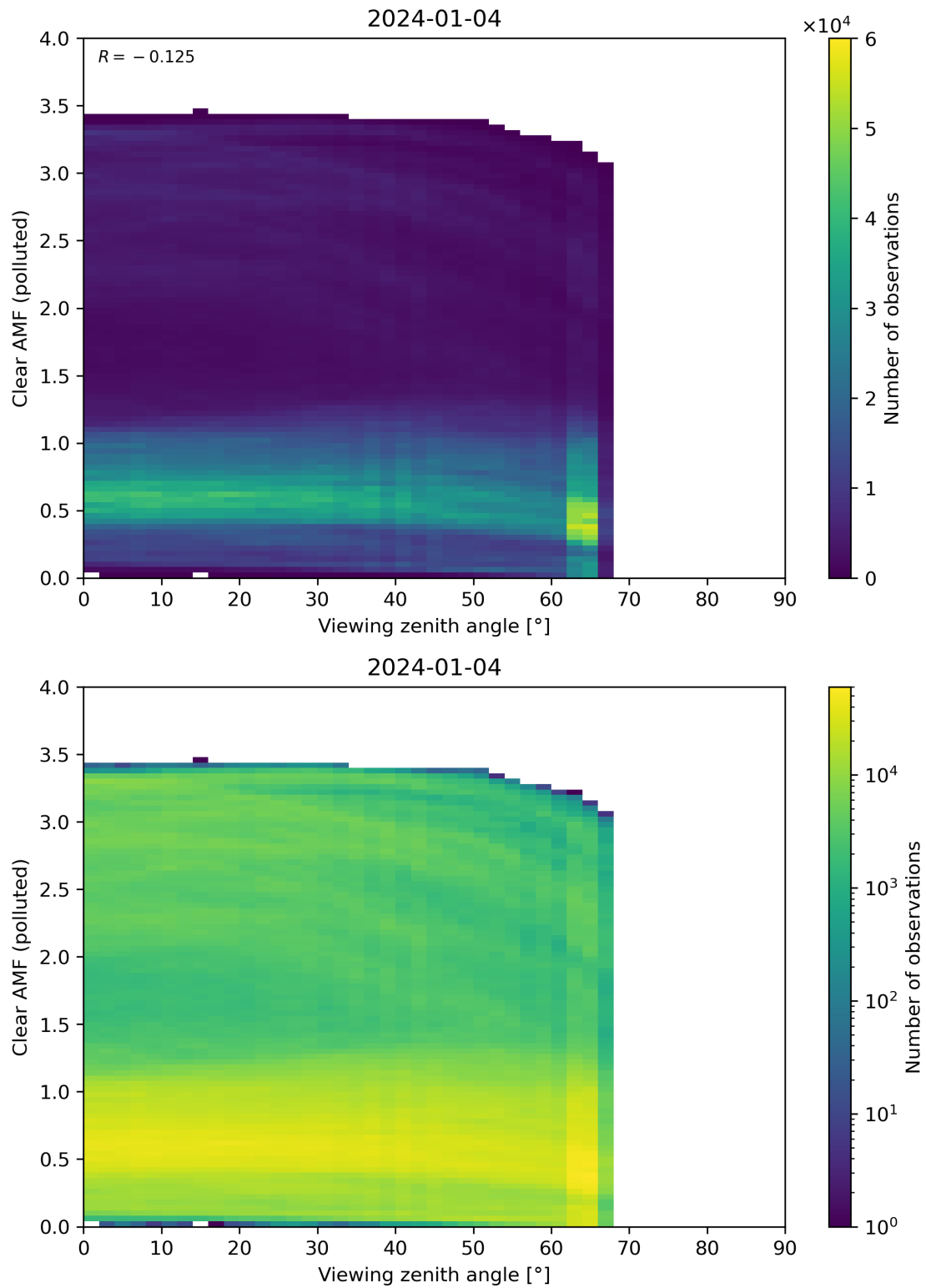
Figure 316: Scatter density plot of “Viewing zenith angle” against “Clear AMF (polluted)” for 2024-01-03 to 2024-01-05.
