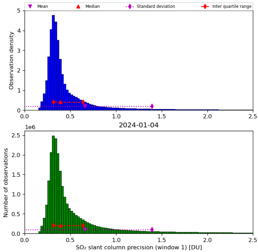
Figure 57: Histogram of “SO 2 slant column precision (window 1)” for 2024-01-03 to 2024-01-05
