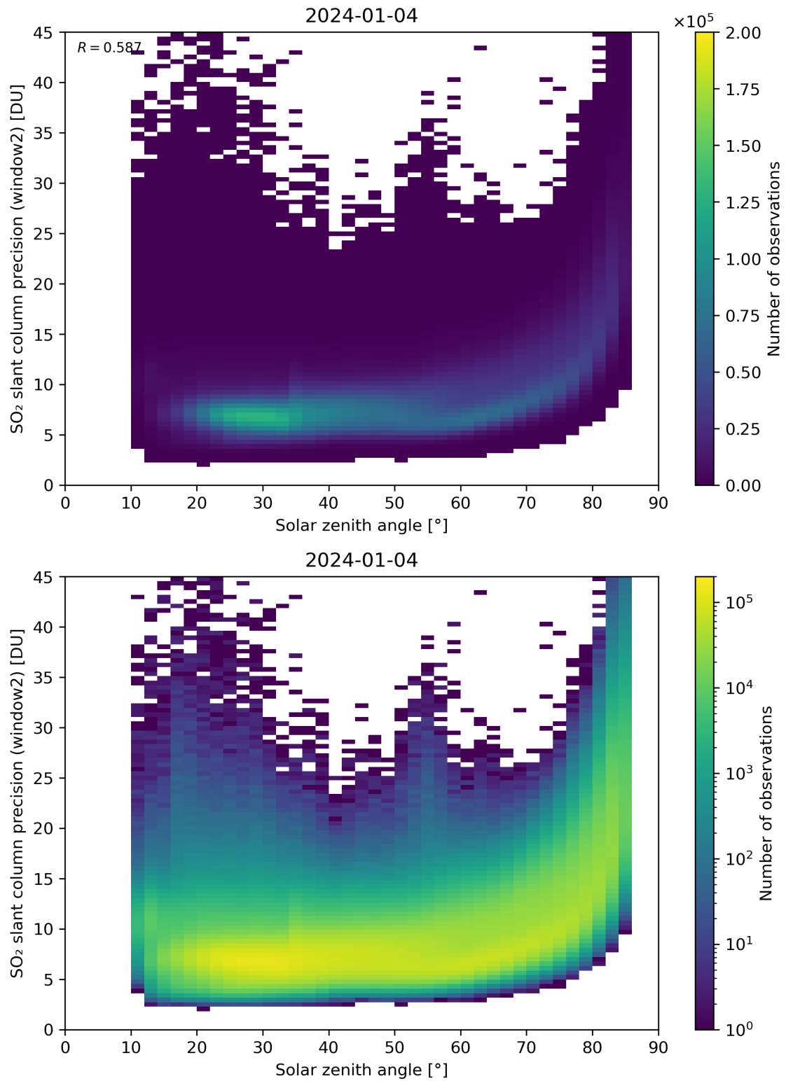
Figure 171: Scatter density plot of “Solar zenith angle” against “SO 2 slant column precision (window2)” for 2024-01-03 to 2024-01-05.
