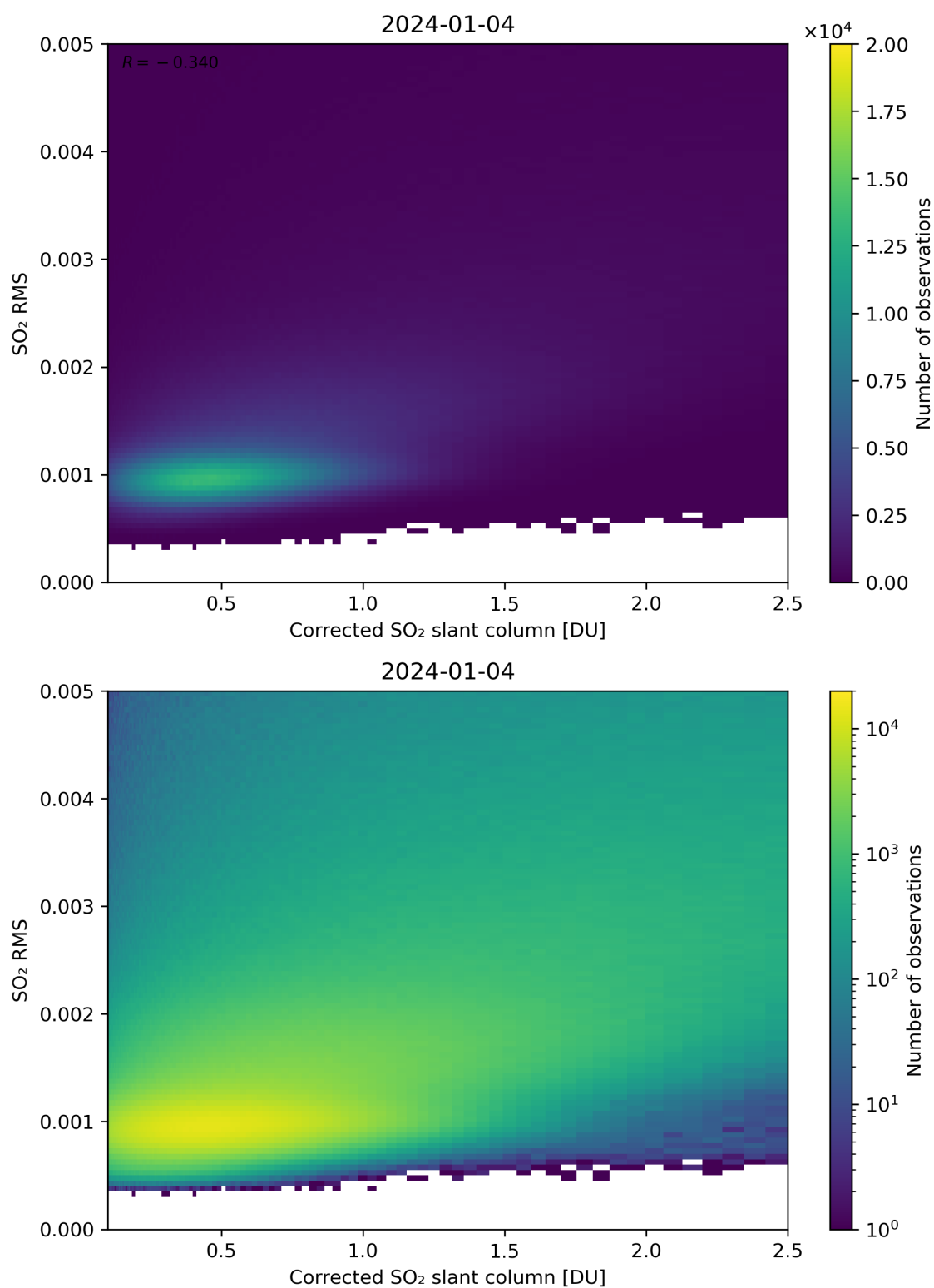
Figure 183: Scatter density plot of “Corrected SO 2 slant column” against “SO 2 RMS” for 2024-01-03 to 2024-01-05.
