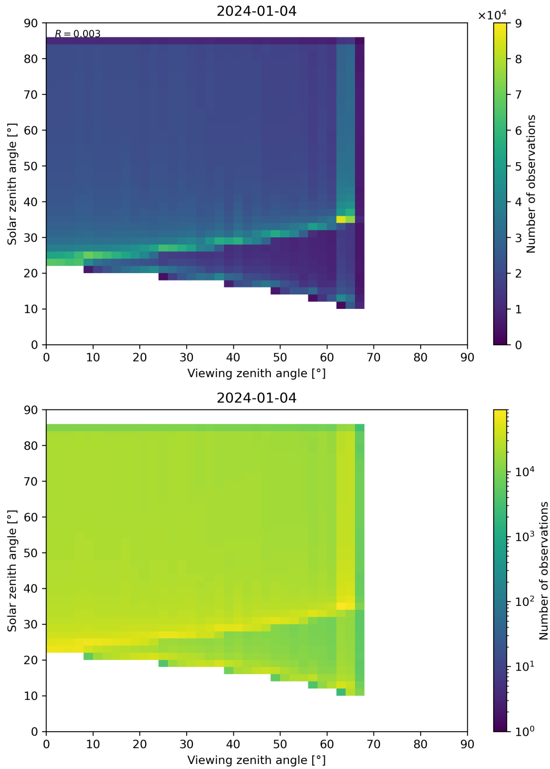
Figure 315: Scatter density plot of “Viewing zenith angle” against “Solar zenith angle” for 2024-01-03 to 2024-01-05.
