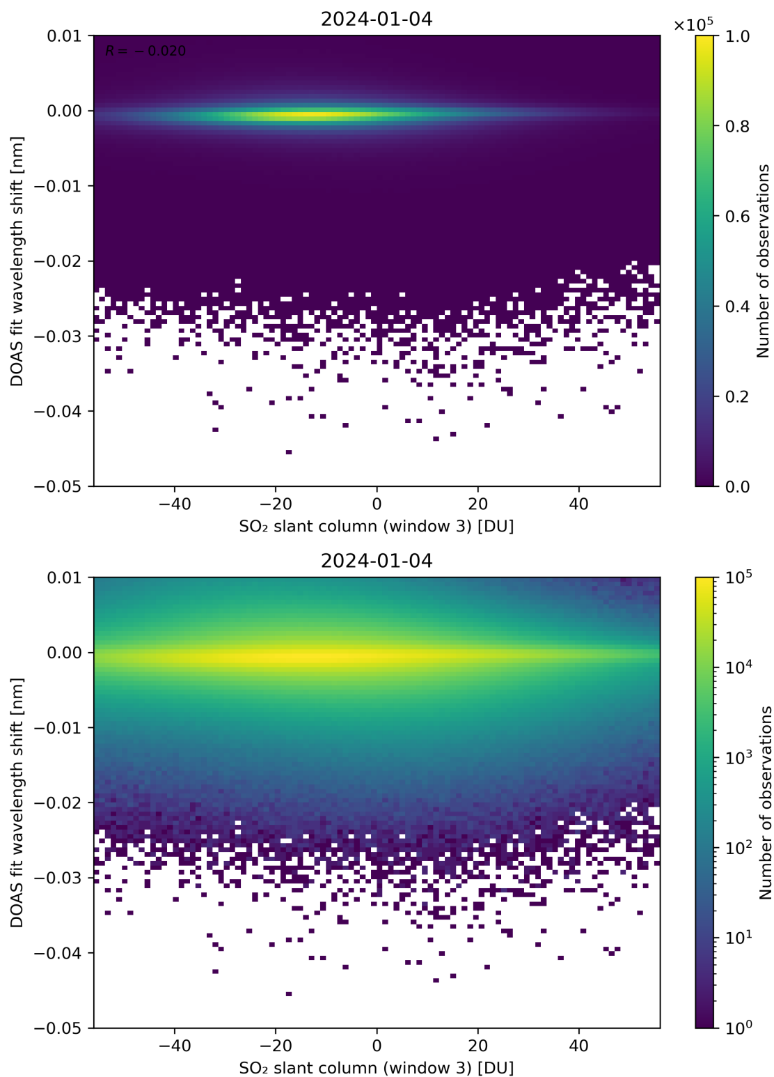
Figure 254: Scatter density plot of “SO 2 slant column (window 3)” against “DOAS fit wavelength shift” for 2024-01-03 to 2024-01-05.
