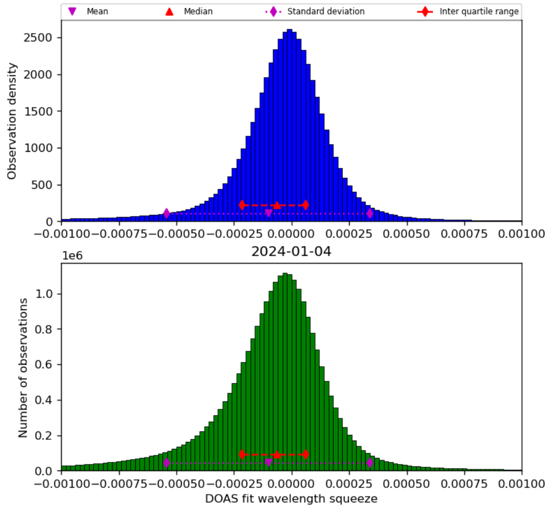
Figure 69: Histogram of “DOAS fit wavelength squeeze” for 2024-01-03 to 2024-01-05
