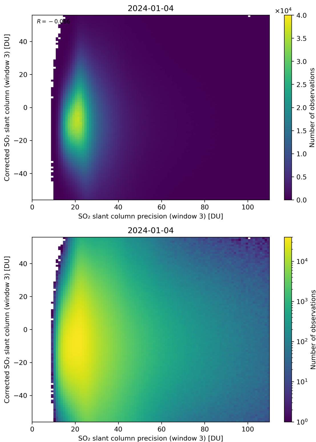
Figure 262: Scatter density plot of “SO 2 slant column precision (window 3)” against “Corrected SO 2 slant column (window 3)” for 2024-01-03 to 2024-01-05.
