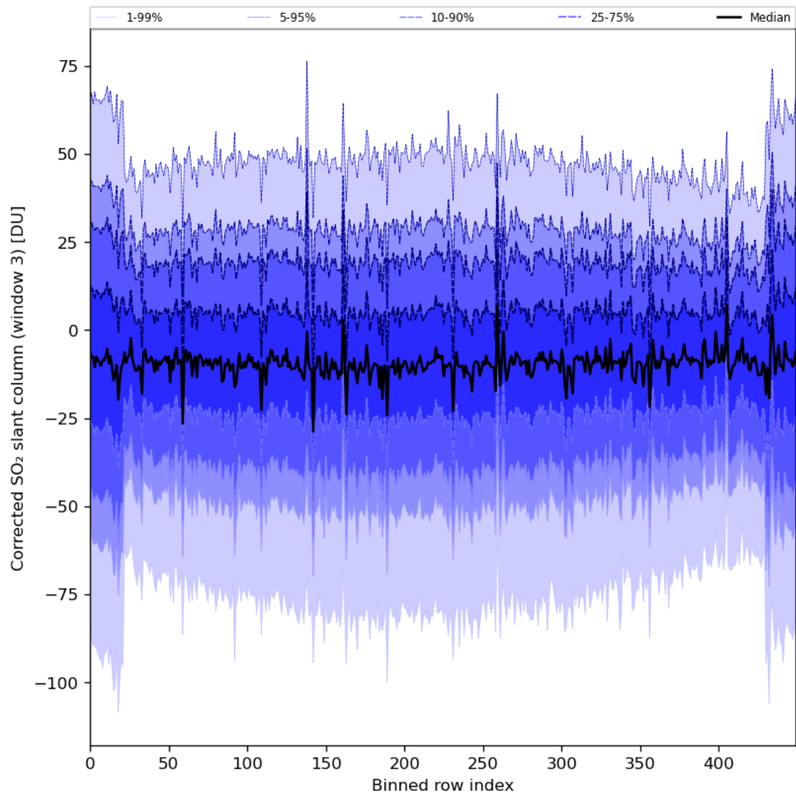
Figure 89: Along track statistics of "Corrected SO 2 slant column (window 3)" for 2024-01-03 to 2024-01-05
