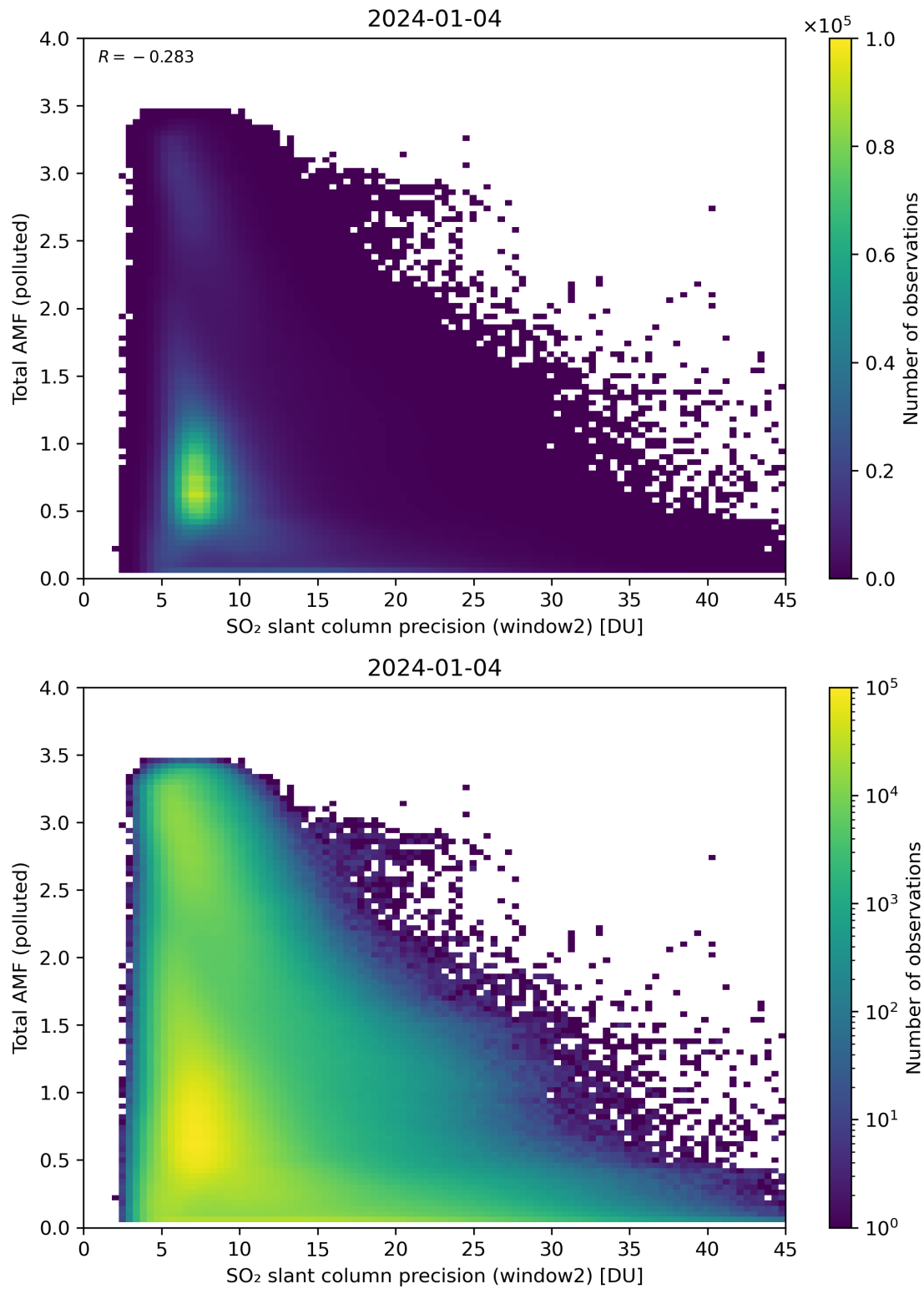
Figure 251: Scatter density plot of “SO 2 slant column precision (window2)” against “Total AMF (polluted)” for 2024-01-03 to 2024-01-05.
