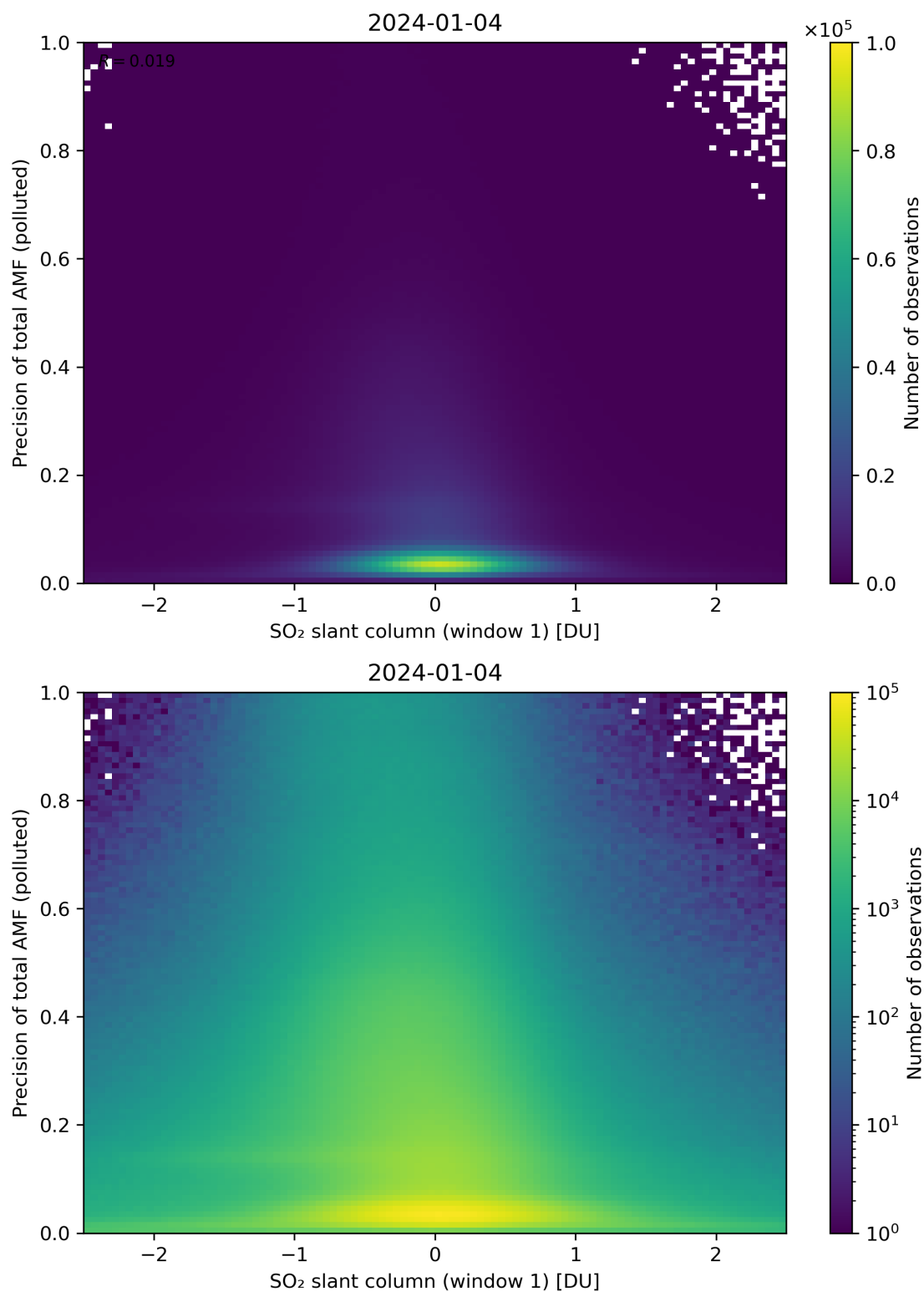
Figure 240: Scatter density plot of “SO 2 slant column (window 1)” against “Precision of total AMF (polluted)” for 2024-01-03 to 2024-01-05.
