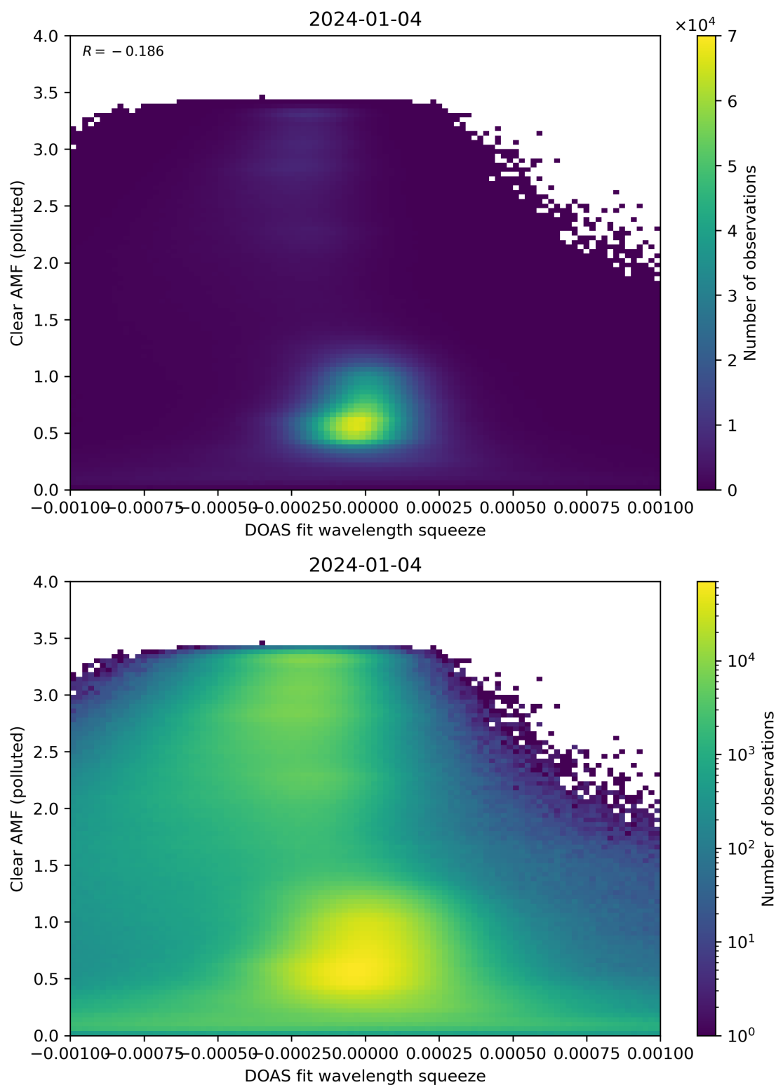
Figure 133: Scatter density plot of “DOAS fit wavelength squeeze” against “Clear AMF (polluted)” for 2024-01-03 to 2024-01-05.
