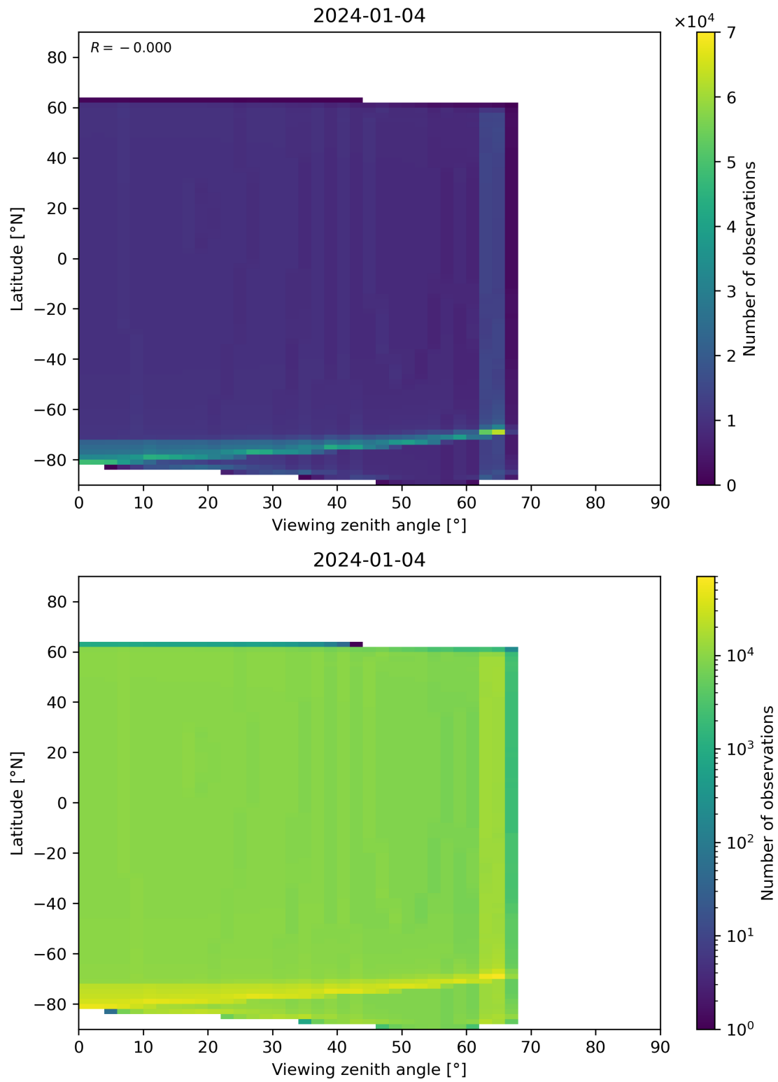
Figure 314: Scatter density plot of “Viewing zenith angle” against “Latitude” for 2024-01-03 to 2024-01-05.
