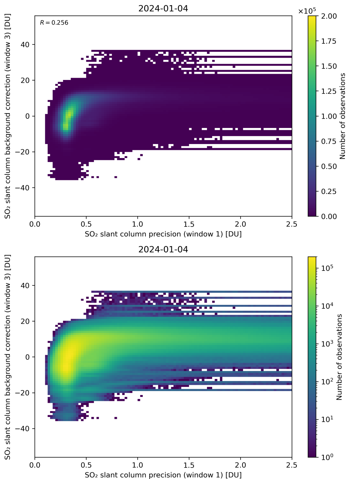
Figure 220: Scatter density plot of “SO 2 slant column precision (window 1)” against “SO 2 slant column background correction (window 3)” for 2024-01-03 to 2024-01-05.
