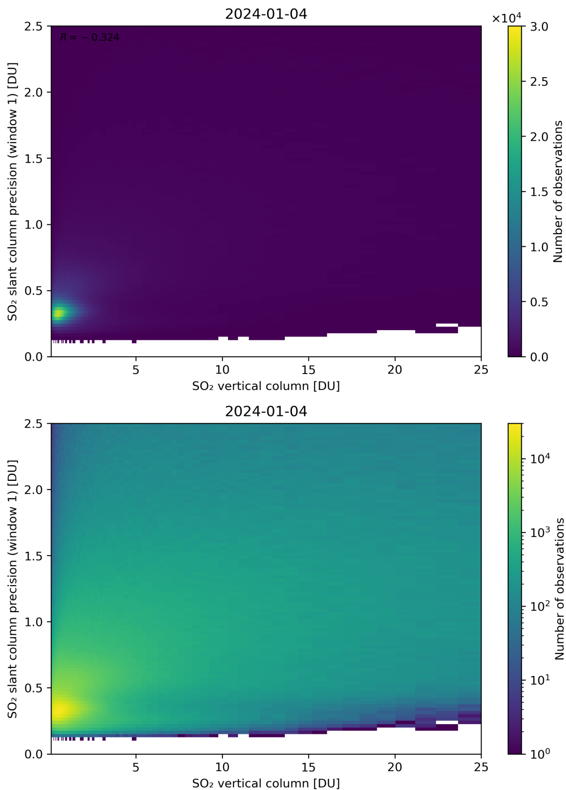
Figure 301: Scatter density plot of “SO 2 vertical column” against “SO 2 slant column precision (window 1)” for 2024-01-03 to 2024-01-05.
