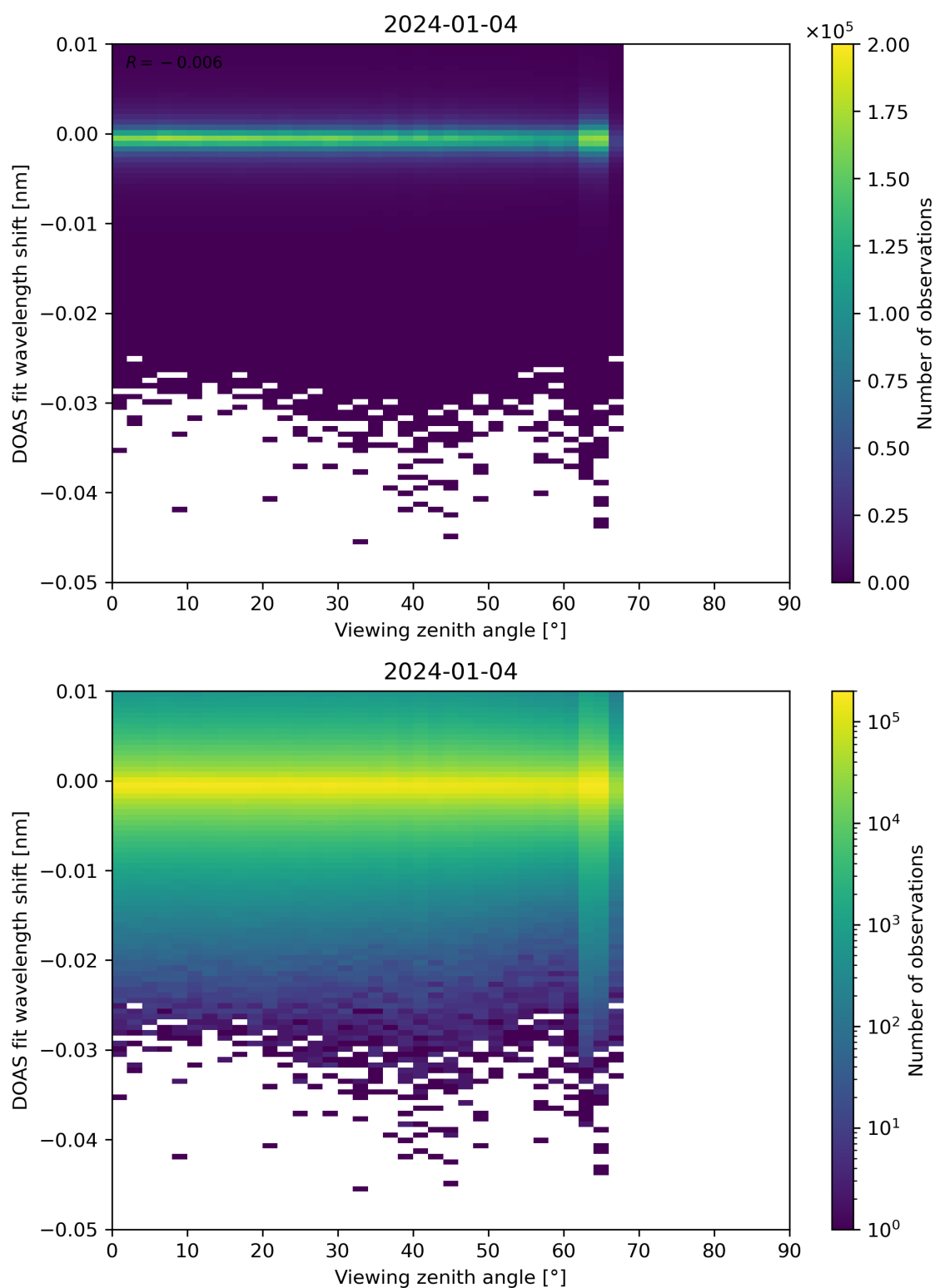
Figure 311: Scatter density plot of “Viewing zenith angle” against “DOAS fit wavelength shift” for 2024-01-03 to 2024-01-05.
