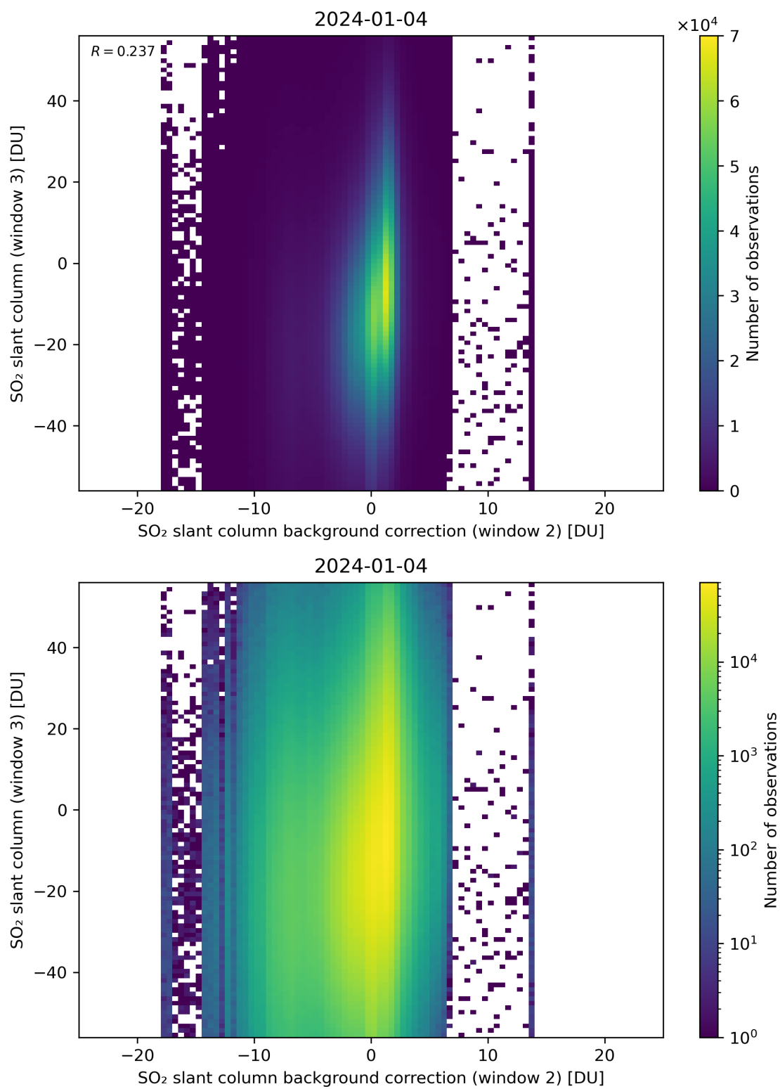
Figure 117: Scatter density plot of “SO 2 slant column background correction (window 2)” against “SO 2 slant column (window 3)” for 2024-01-03 to 2024-01-05.
