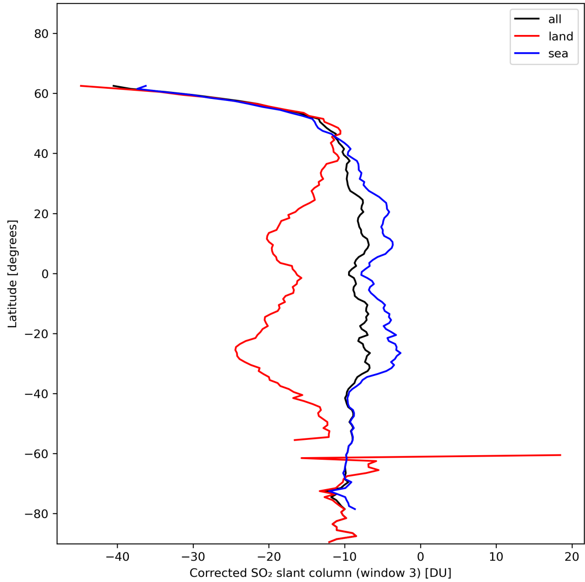
Figure 43: Zonal average of “Corrected SO 2 slant column (window 3)” for 2024-01-03 to 2024-01-05.
