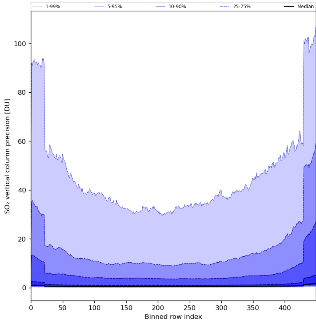
Figure 77: Along track statistics of “SO 2 vertical column precision” for 2024-01-03 to 2024-01-05
