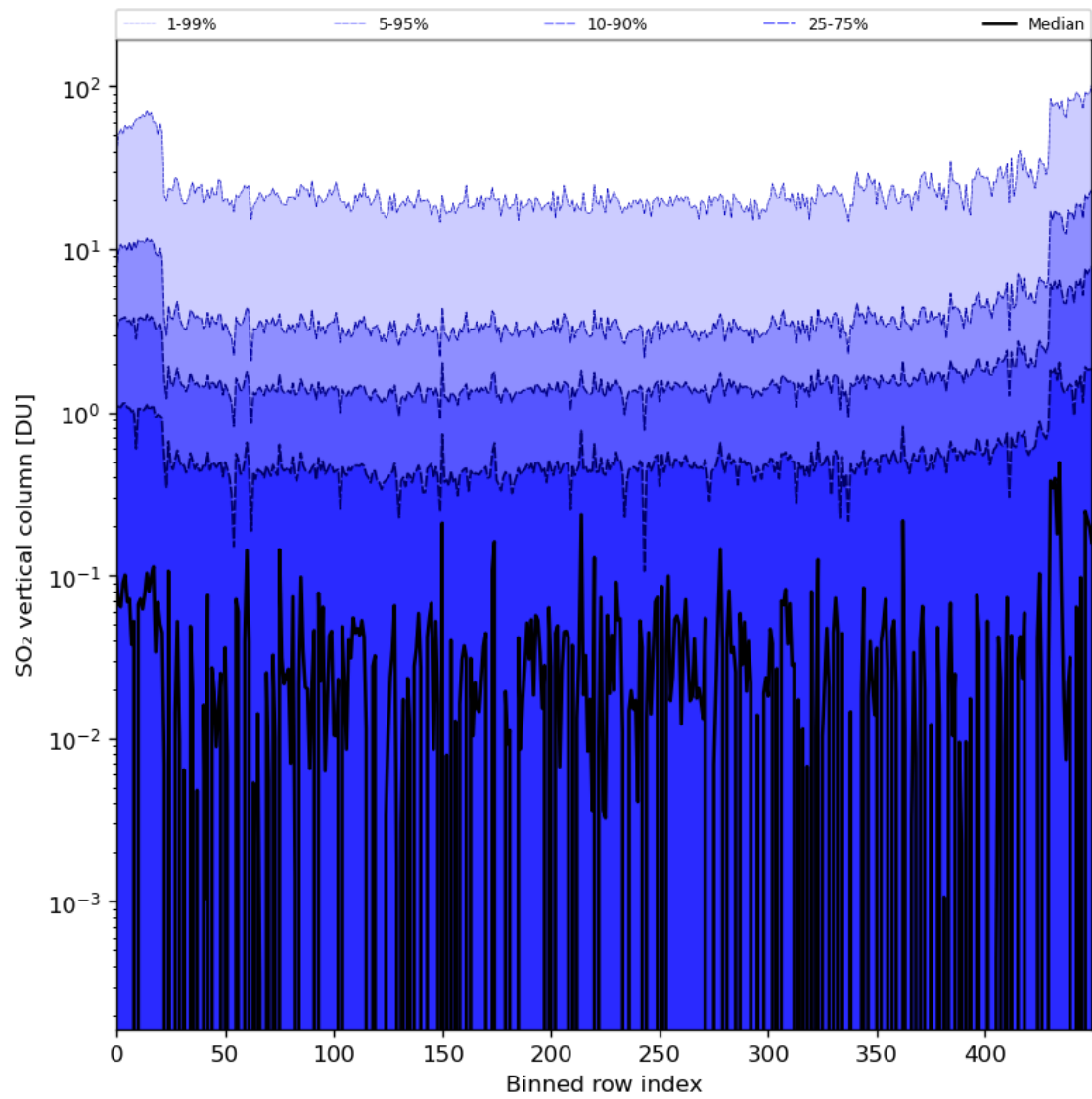
Figure 76: Along track statistics of “SO 2 vertical column” for 2024-01-03 to 2024-01-05
