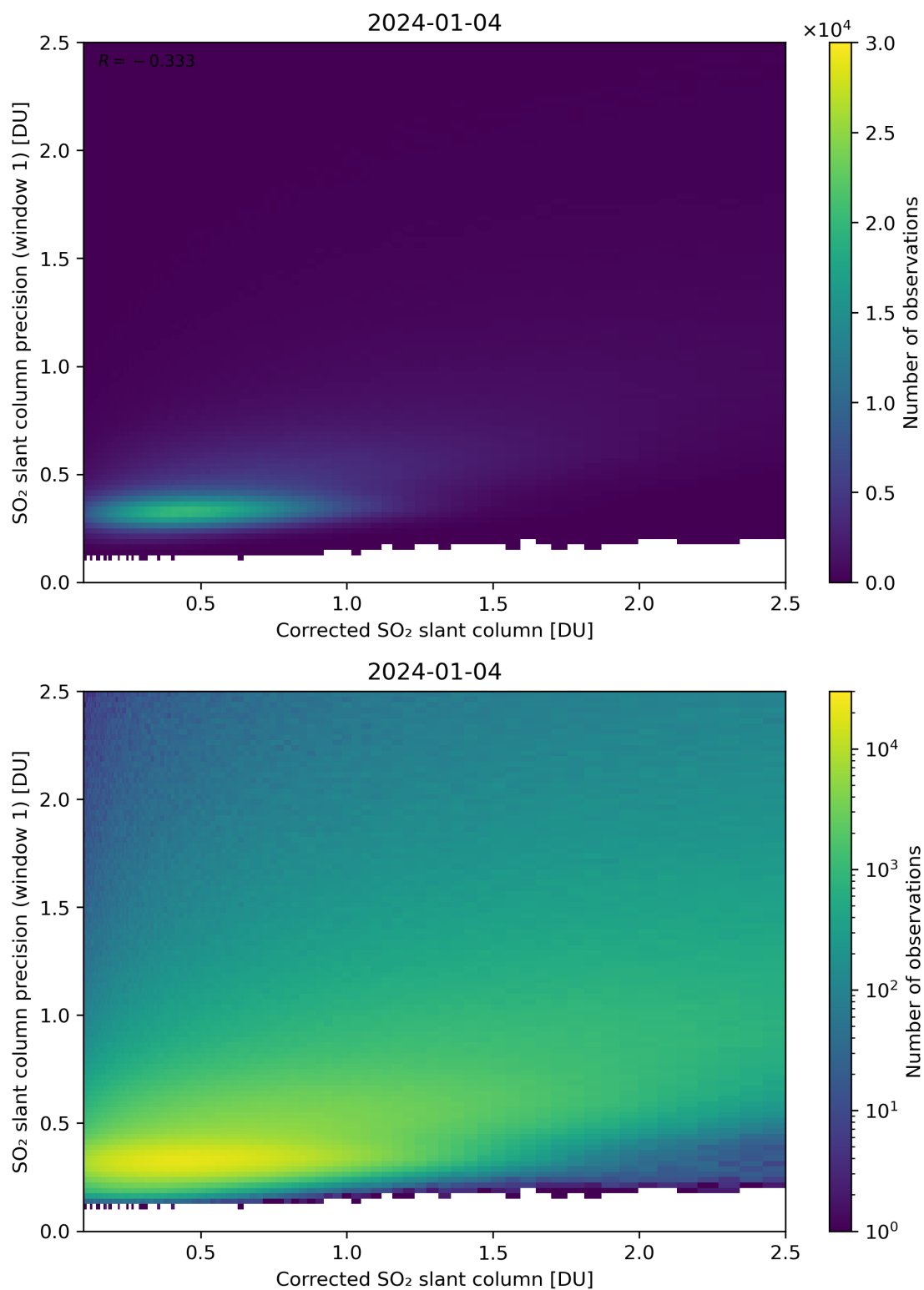
Figure 188: Scatter density plot of “Corrected SO 2 slant column” against “SO 2 slant column precision (window 1)” for 2024-01-03 to 2024-01-05.
