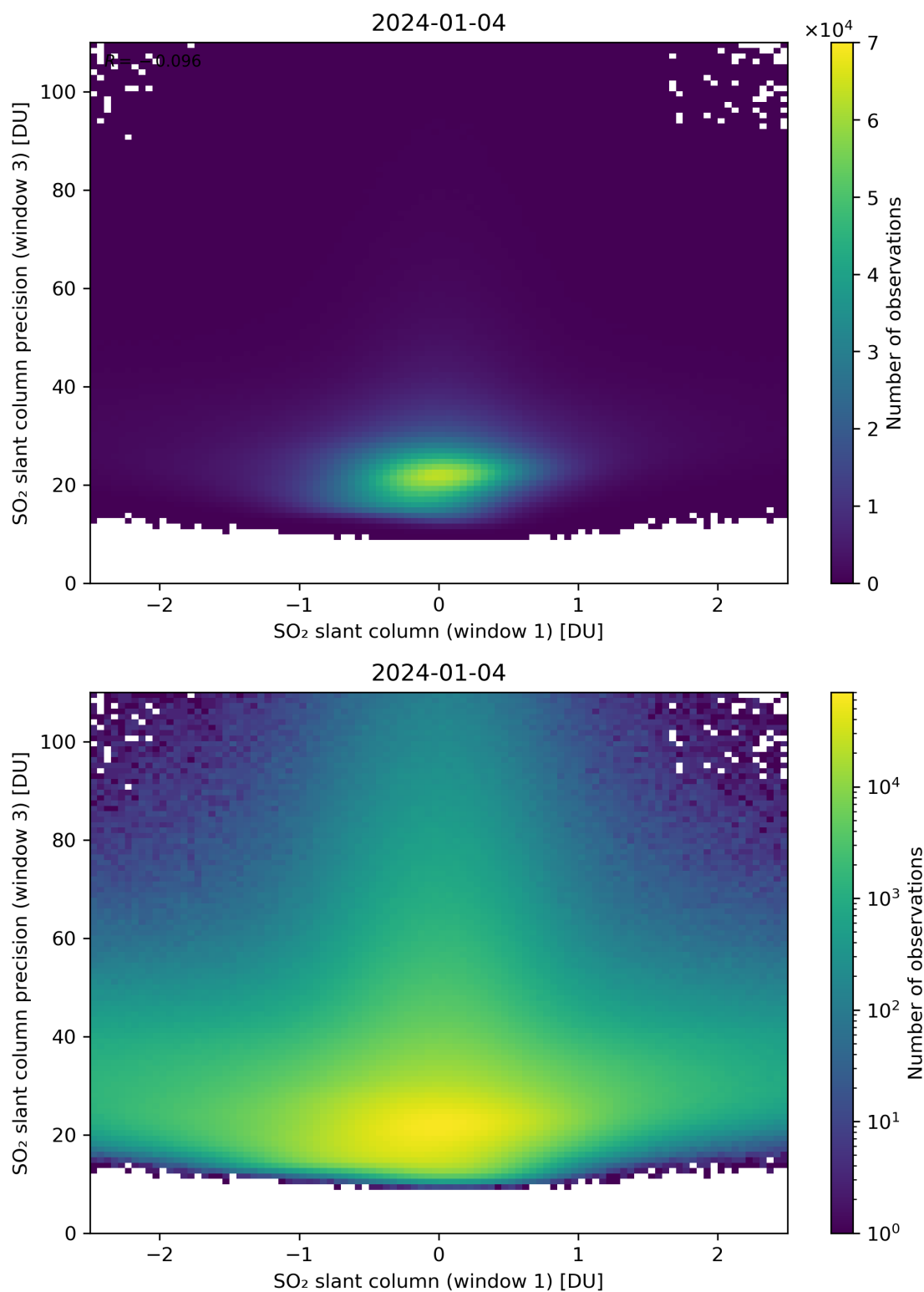
Figure 238: Scatter density plot of “SO 2 slant column (window 1)” against “SO 2 slant column precision (window 3)” for 2024-01-03 to 2024-01-05.
