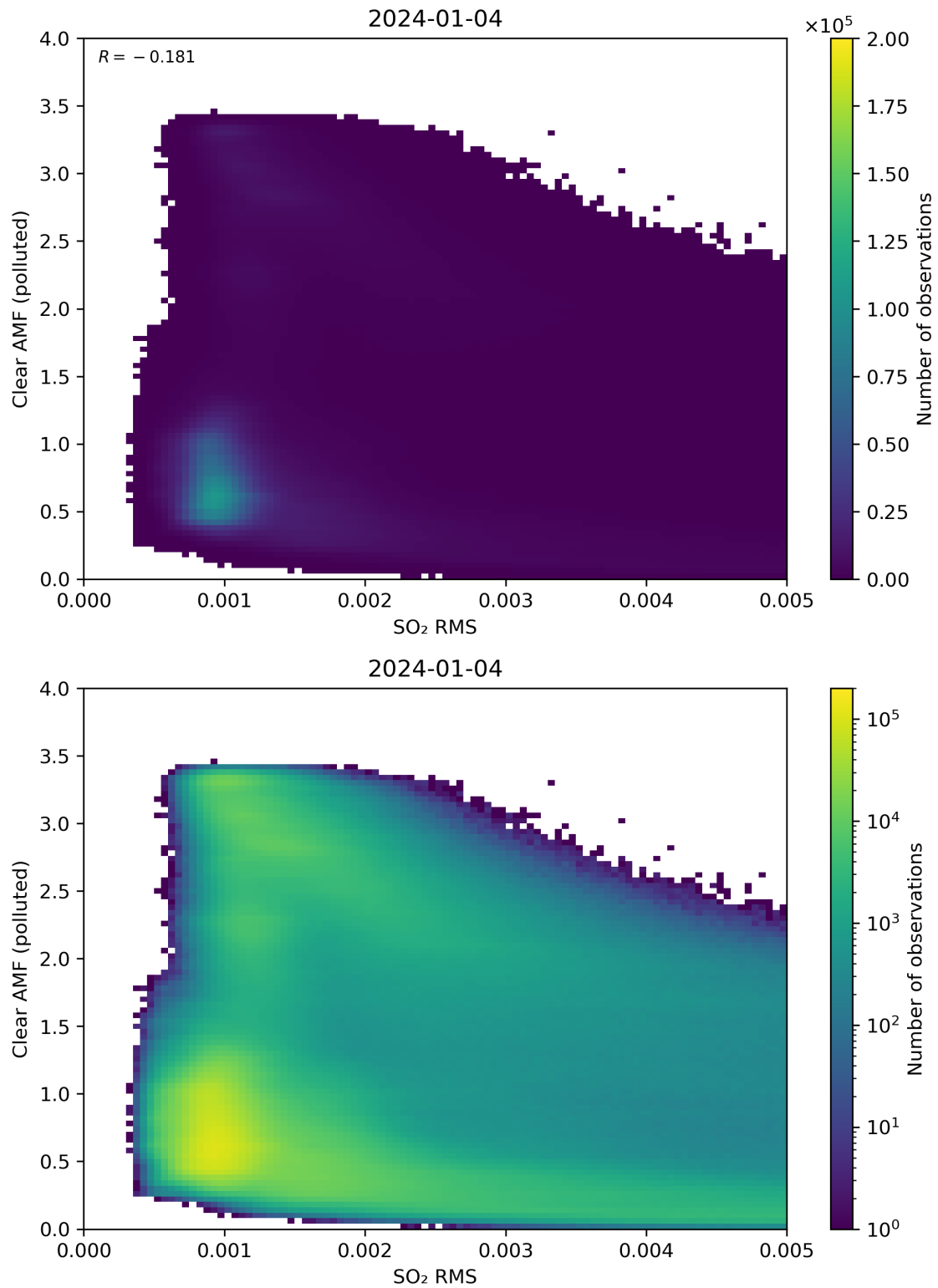
Figure 136: Scatter density plot of “SO 2 RMS” against “Clear AMF (polluted)” for 2024-01-03 to 2024-01-05.
