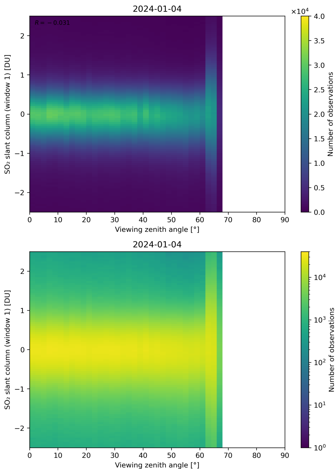
Figure 320: Scatter density plot of “Viewing zenith angle” against “SO 2 slant column (window 1)” for 2024-01-03 to 2024-01-05.
