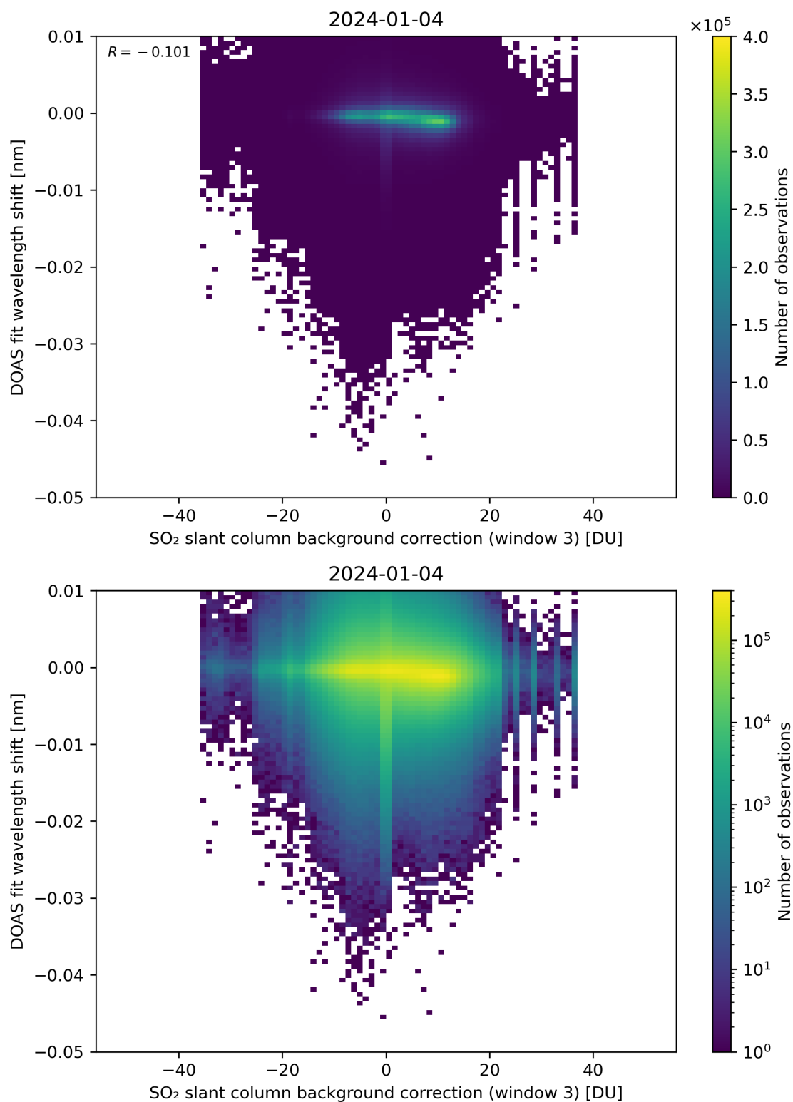
Figure 121: Scatter density plot of “SO 2 slant column background correction (window 3)” against “DOAS fit wavelength shift” for 2024-01-03 to 2024-01-05.
