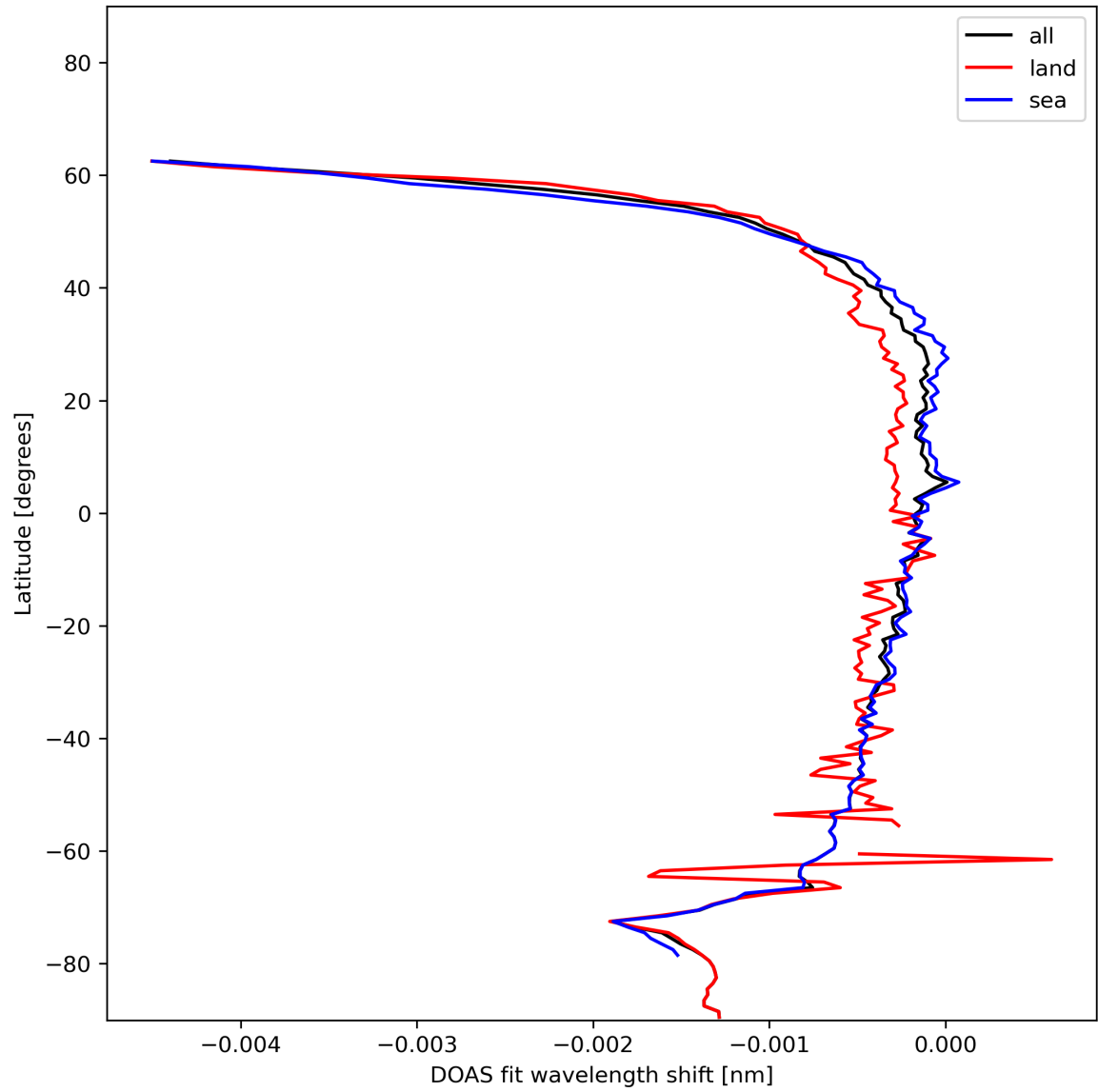
Figure 45: Zonal average of “DOAS fit wavelength shift” for 2024-01-03 to 2024-01-05.
