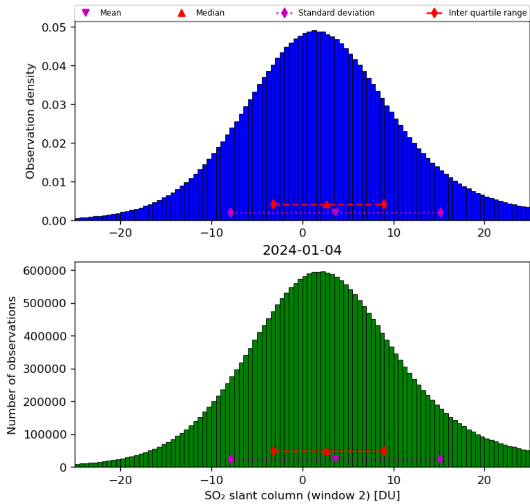
Figure 60: Histogram of “SO 2 slant column (window 2)” for 2024-01-03 to 2024-01-05
