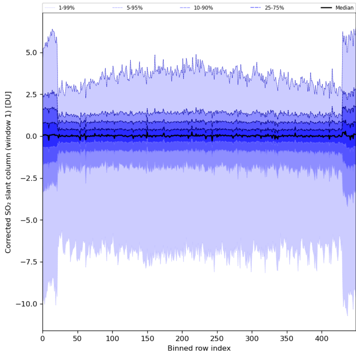
Figure 81: Along track statistics of “Corrected SO 2 slant column (window 1)” for 2024-01-03 to 2024-01-05
