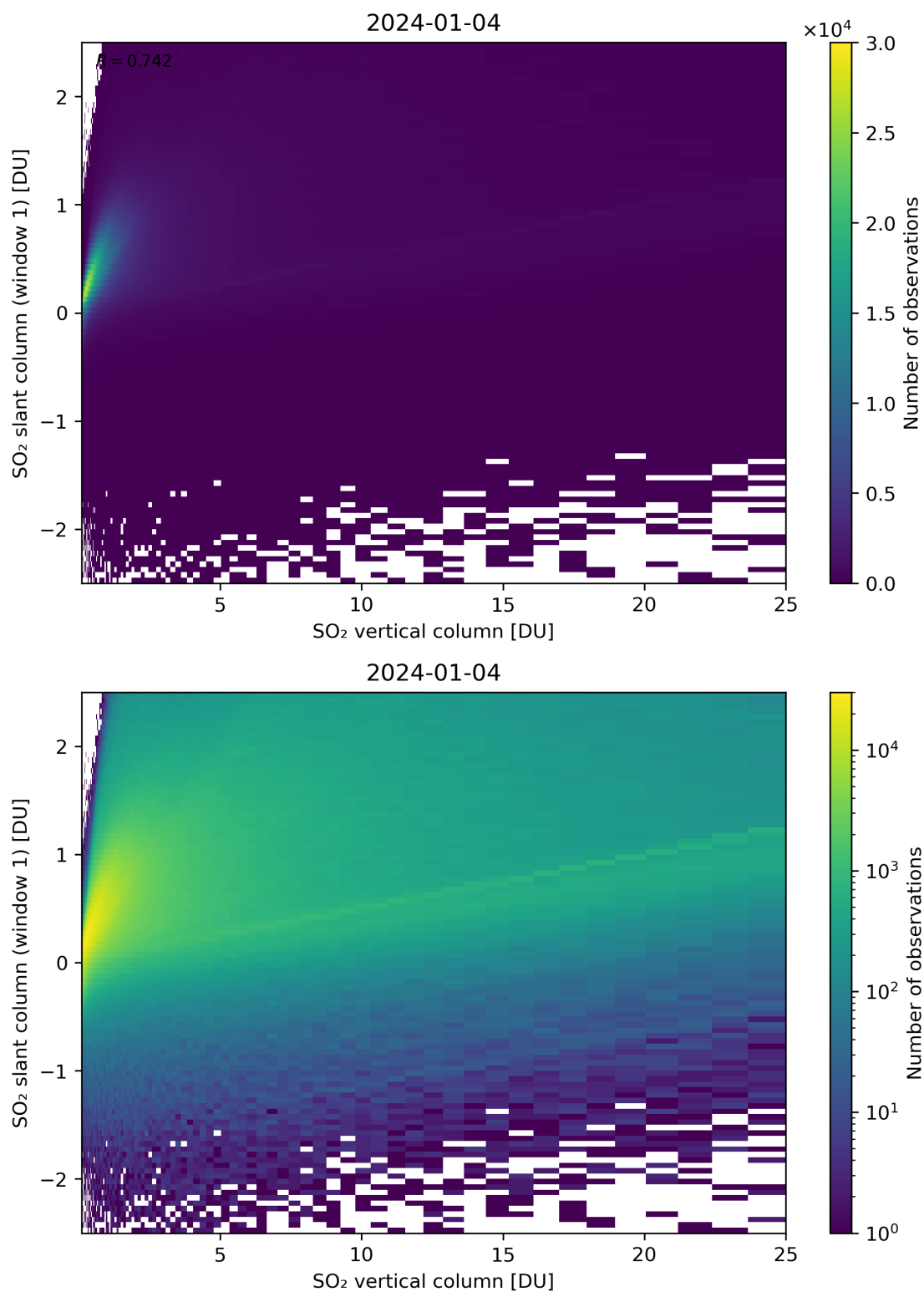
Figure 300: Scatter density plot of “SO 2 vertical column” against “SO 2 slant column (window 1)” for 2024-01-03 to 2024-01-05.
