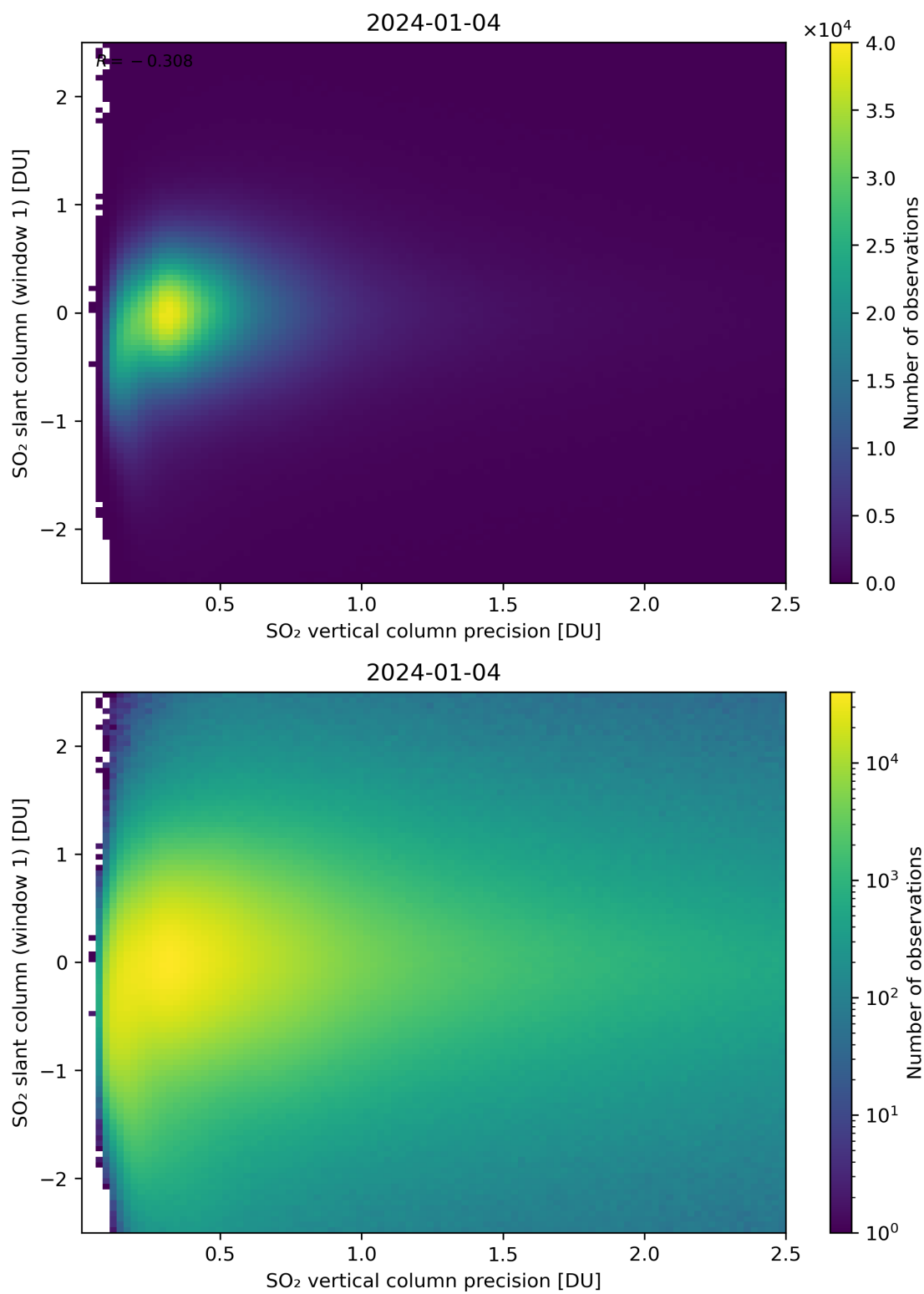
Figure 289: Scatter density plot of “SO 2 vertical column precision” against “SO 2 slant column (window 1)” for 2024-01-03 to 2024-01-05.
