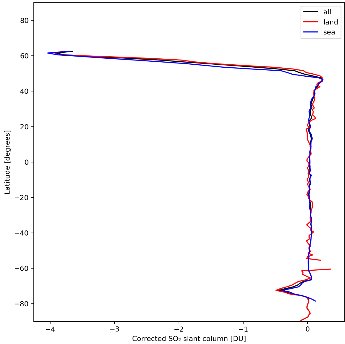
Figure 32: Zonal average of “Corrected SO 2 slant column” for 2024-01-03 to 2024-01-05.
