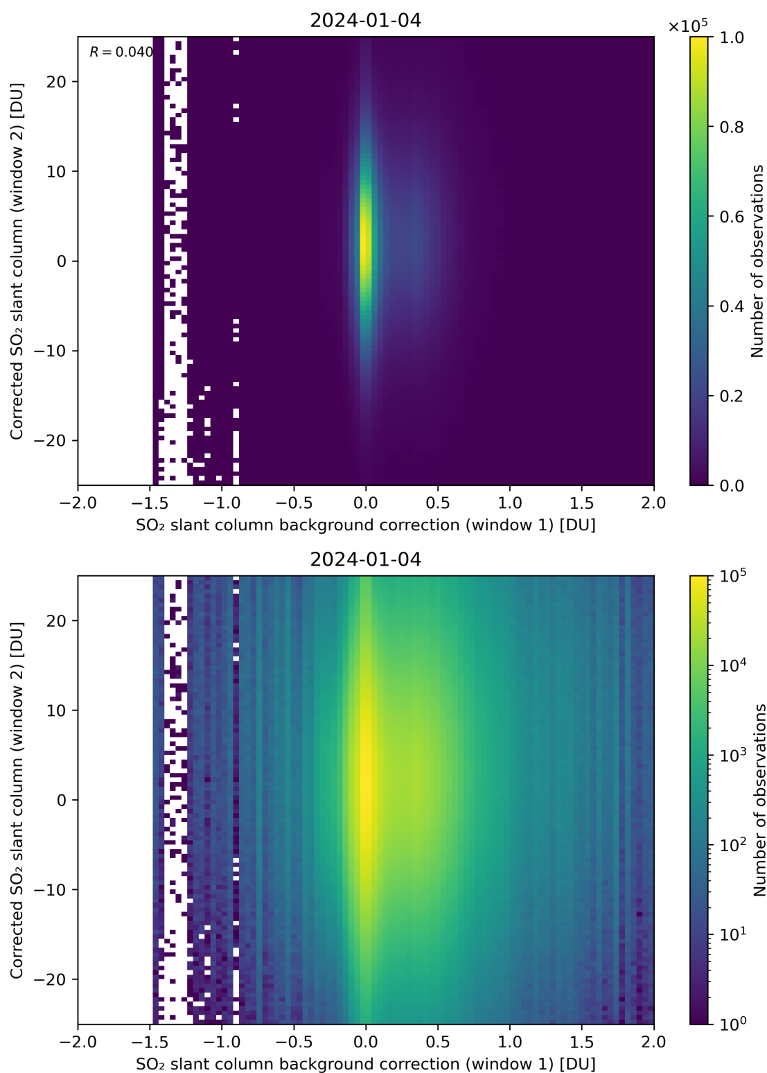
Figure 104: Scatter density plot of “SO 2 slant column background correction (window 1)” against “Corrected SO 2 slant column (window 2)” for 2024-01-03 to 2024-01-05.
