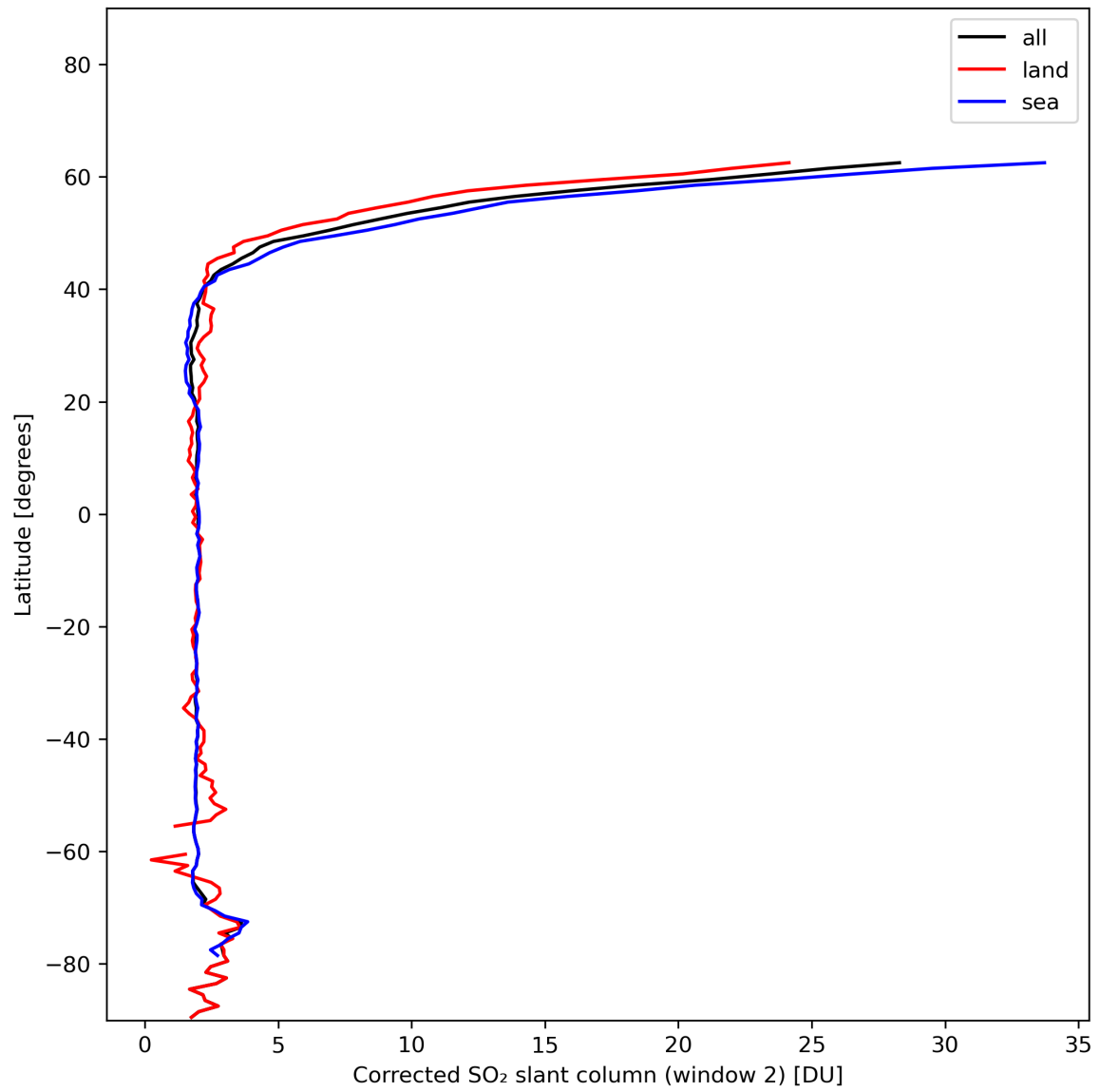
Figure 39: Zonal average of “Corrected SO 2 slant column (window 2)” for 2024-01-03 to 2024-01-05.
