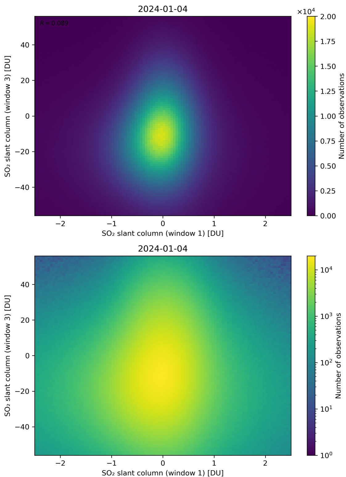
Figure 237: Scatter density plot of “SO 2 slant column (window 1)” against “SO 2 slant column (window 3)” for 2024-01-03 to 2024-01-05.
