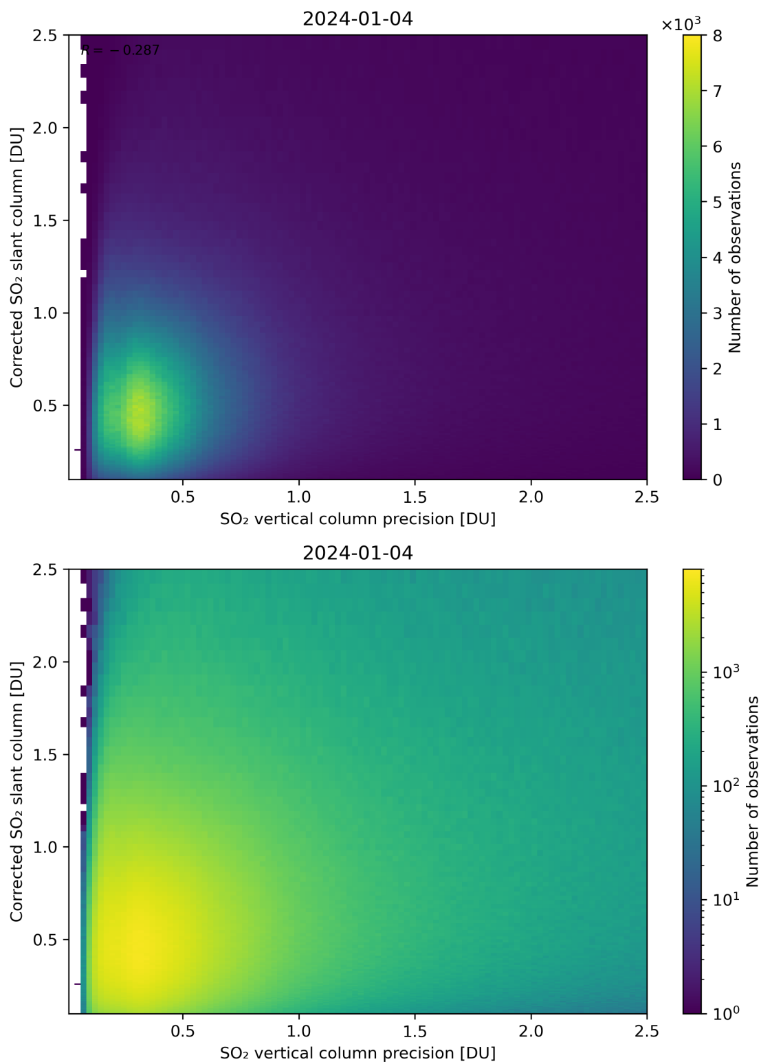
Figure 286: Scatter density plot of “SO 2 vertical column precision” against “Corrected SO 2 slant column” for 2024-01-03 to 2024-01-05.
