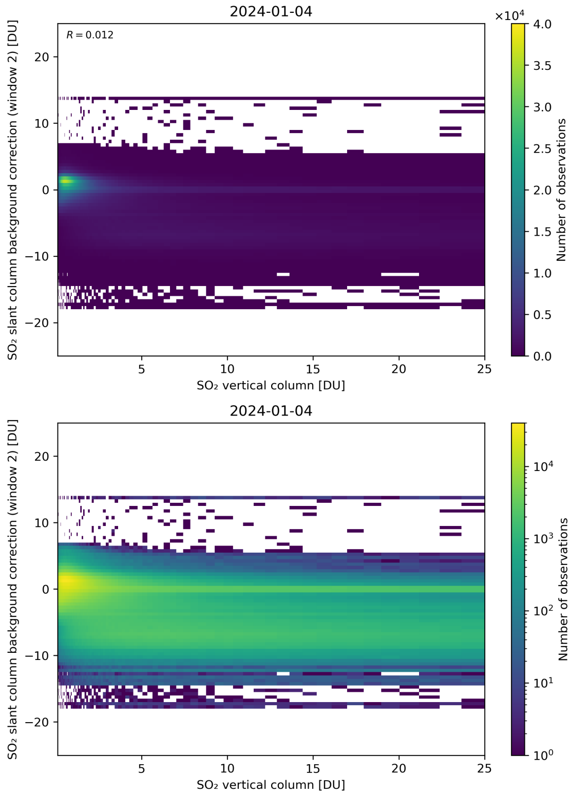
Figure 274: Scatter density plot of “SO 2 vertical column” against “SO 2 slant column background correction (window 2)” for 2024-01-03 to 2024-01-05.
