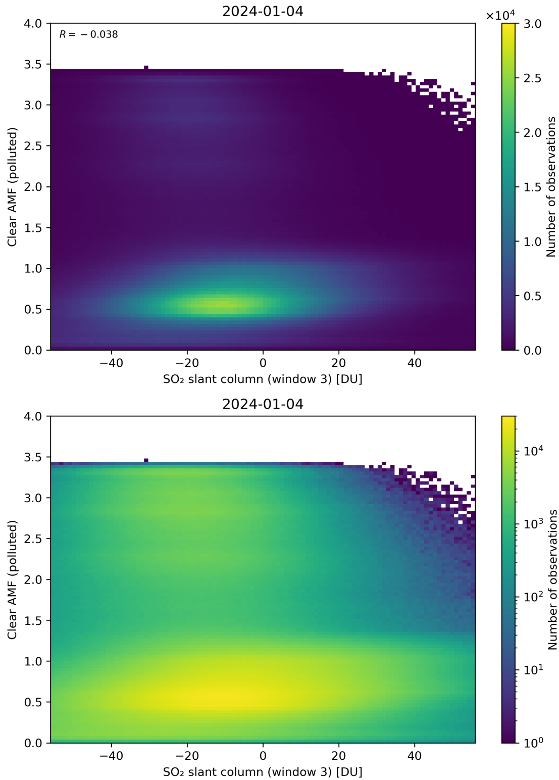
Figure 265: Scatter density plot of “SO 2 slant column (window 3)” against “Clear AMF (polluted)” for 2024-01-03 to 2024-01-05.
