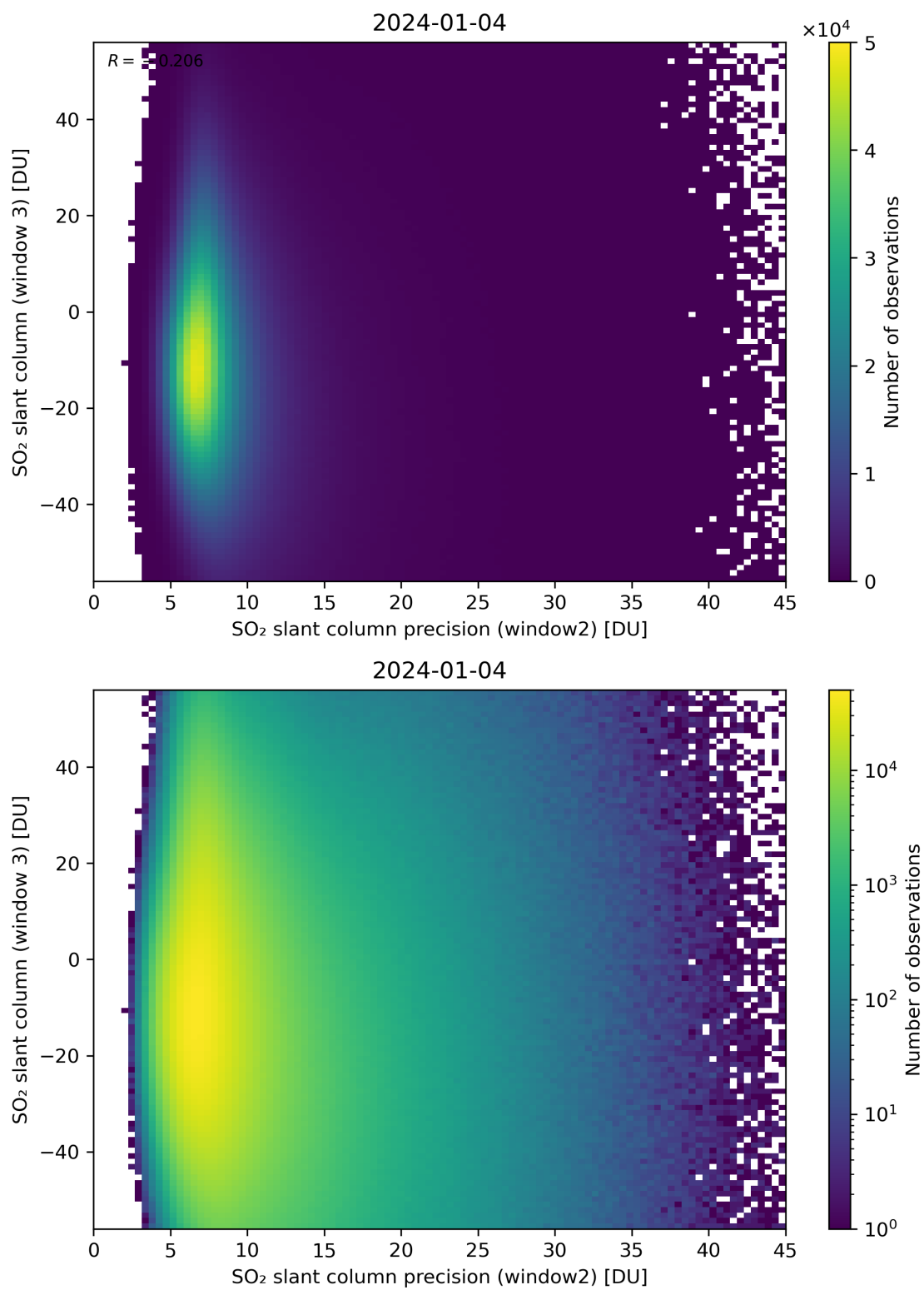
Figure 249: Scatter density plot of “SO 2 slant column precision (window2)” against “SO 2 slant column (window 3)” for 2024-01-03 to 2024-01-05.
