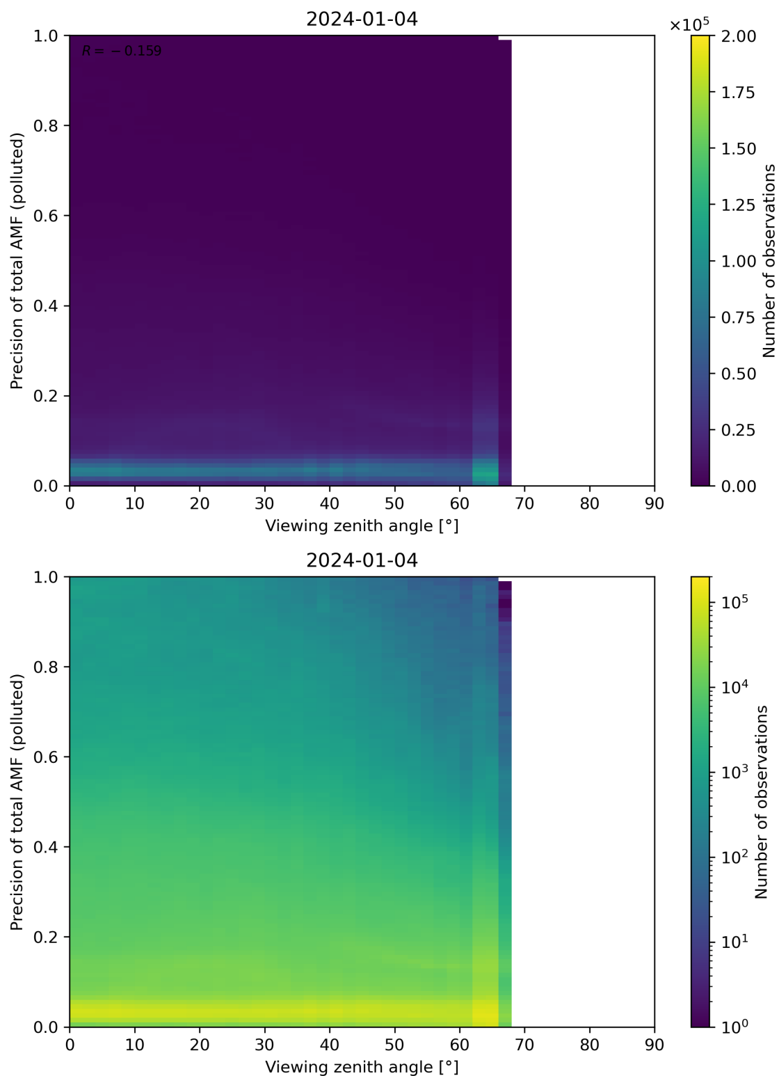
Figure 326: Scatter density plot of “Viewing zenith angle” against “Precision of total AMF (polluted)” for 2024-01-03 to 2024-01-05.
