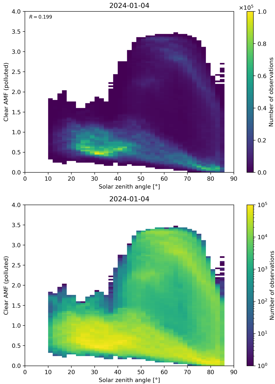
Figure 165: Scatter density plot of “Solar zenith angle” against “Clear AMF (polluted)” for 2024-01-03 to 2024-01-05.
