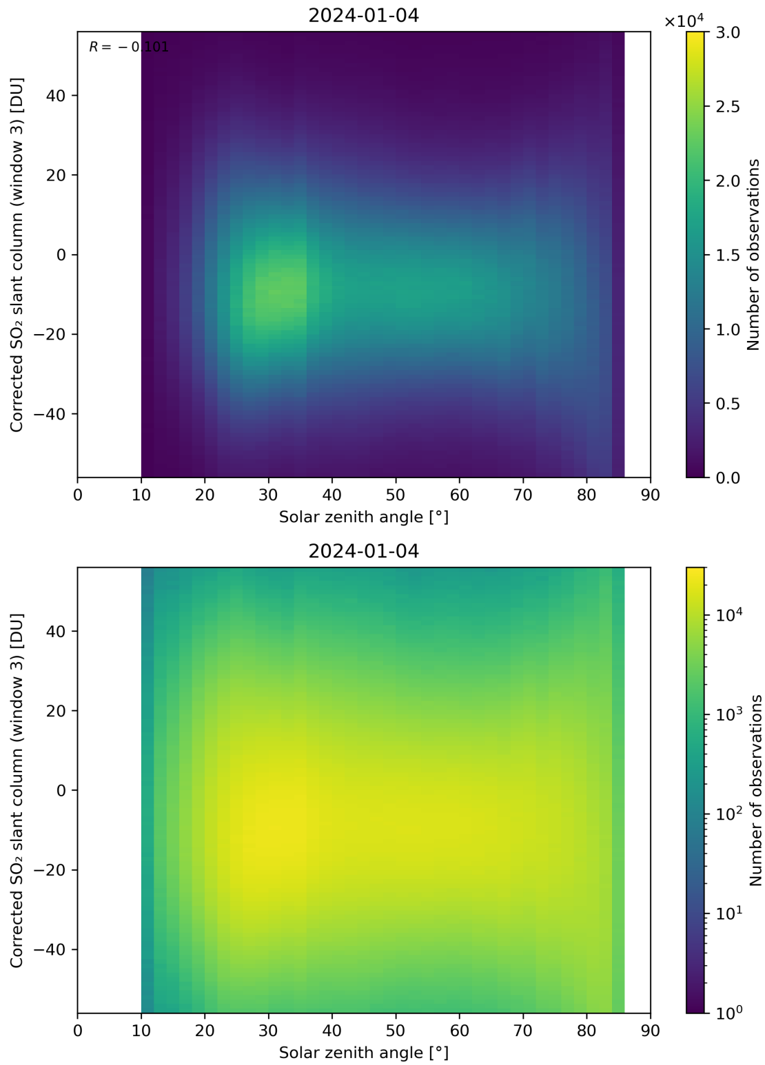
Figure 168: Scatter density plot of “Solar zenith angle” against “Corrected SO 2 slant column (window 3)” for 2024-01-03 to 2024-01-05.
