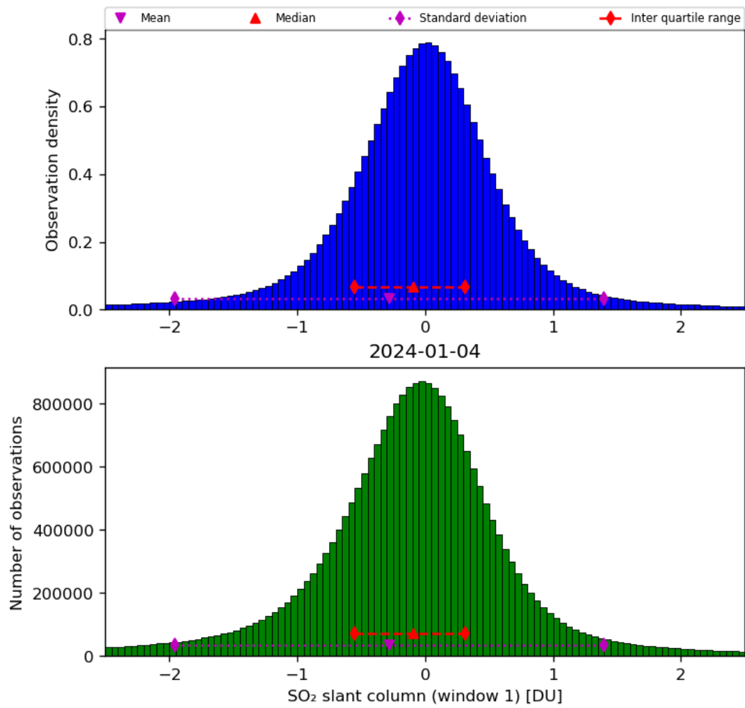
Figure 56: Histogram of “SO 2 slant column (window 1)” for 2024-01-03 to 2024-01-05
