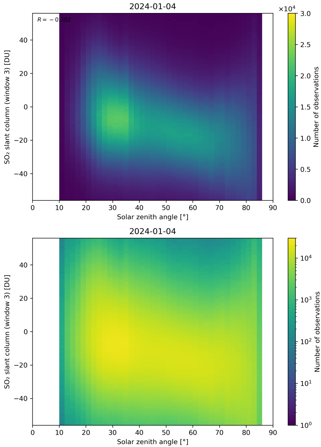
Figure 172: Scatter density plot of “Solar zenith angle” against “SO 2 slant column (window 3)” for 2024-01-03 to 2024-01-05.
