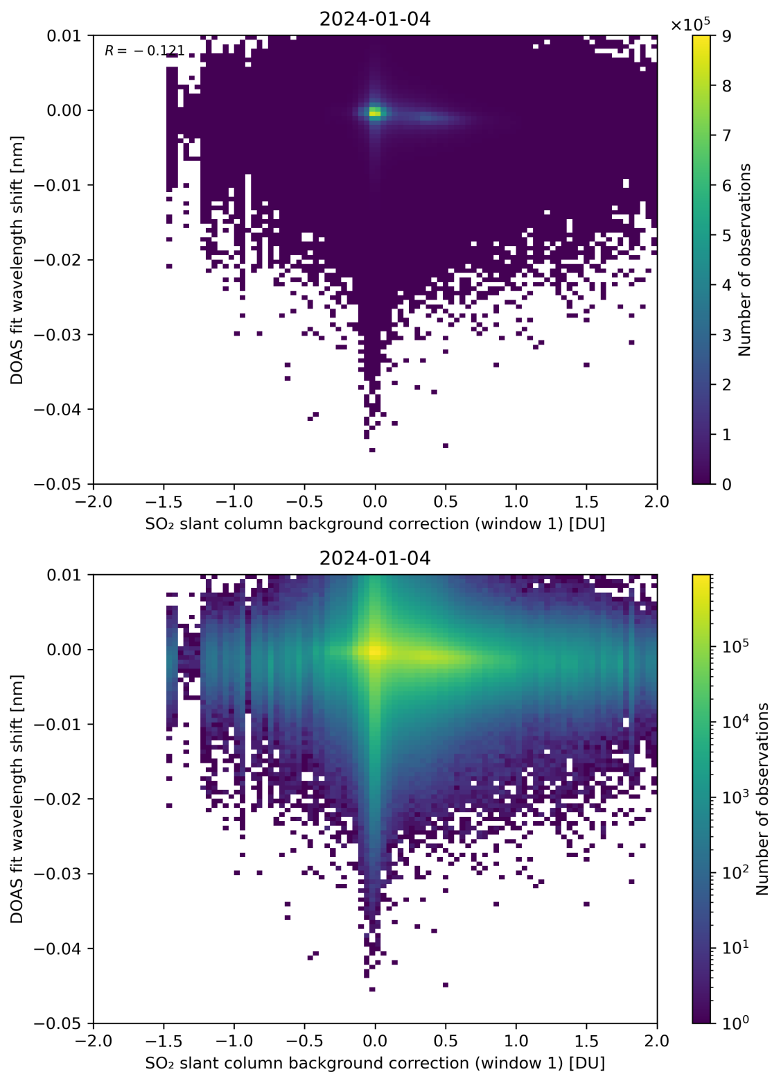
Figure 100: Scatter density plot of “SO 2 slant column background correction (window 1)” against “DOAS fit wavelength shift” for 2024-01-03 to 2024-01-05.
