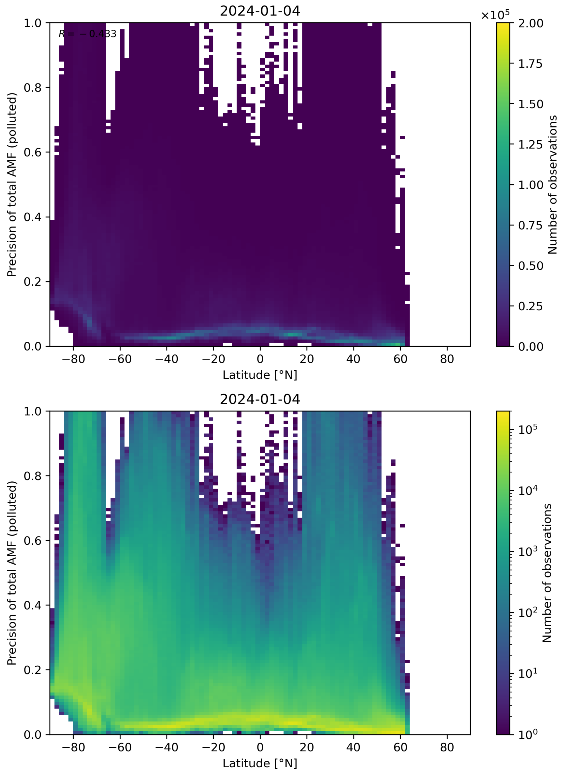
Figure 155: Scatter density plot of “Latitude” against “Precision of total AMF (polluted)” for 2024-01-03 to 2024-01-05.
