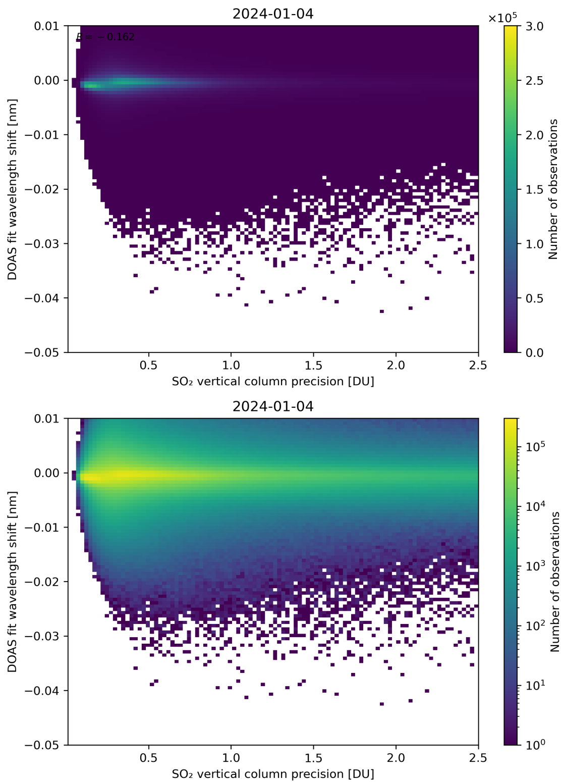
Figure 282: Scatter density plot of “SO 2 vertical column precision” against “DOAS fit wavelength shift” for 2024-01-03 to 2024-01-05.
