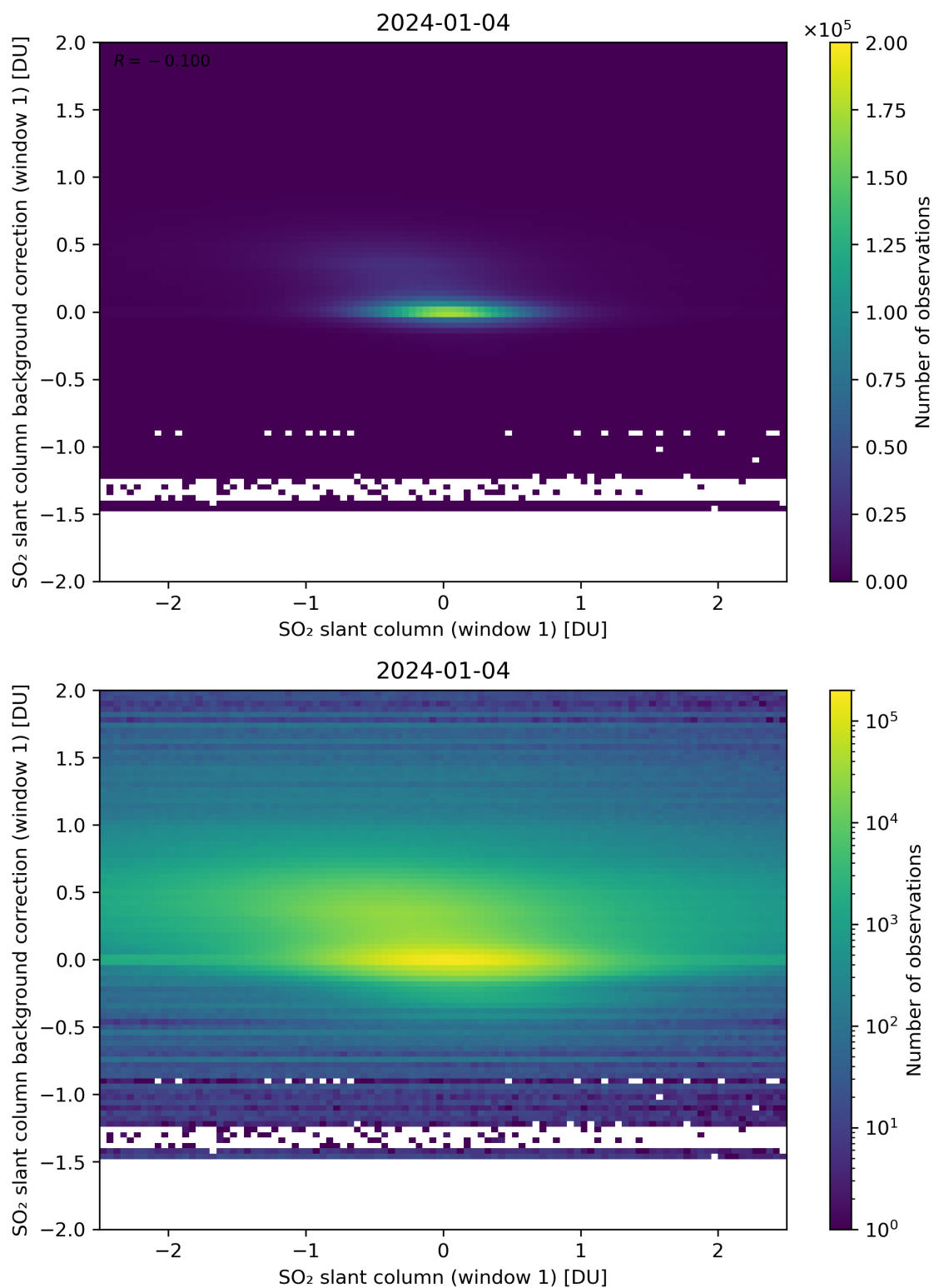
Figure 212: Scatter density plot of “SO 2 slant column (window 1)” against “SO 2 slant column background correction (window 1)” for 2024-01-03 to 2024-01-05.
