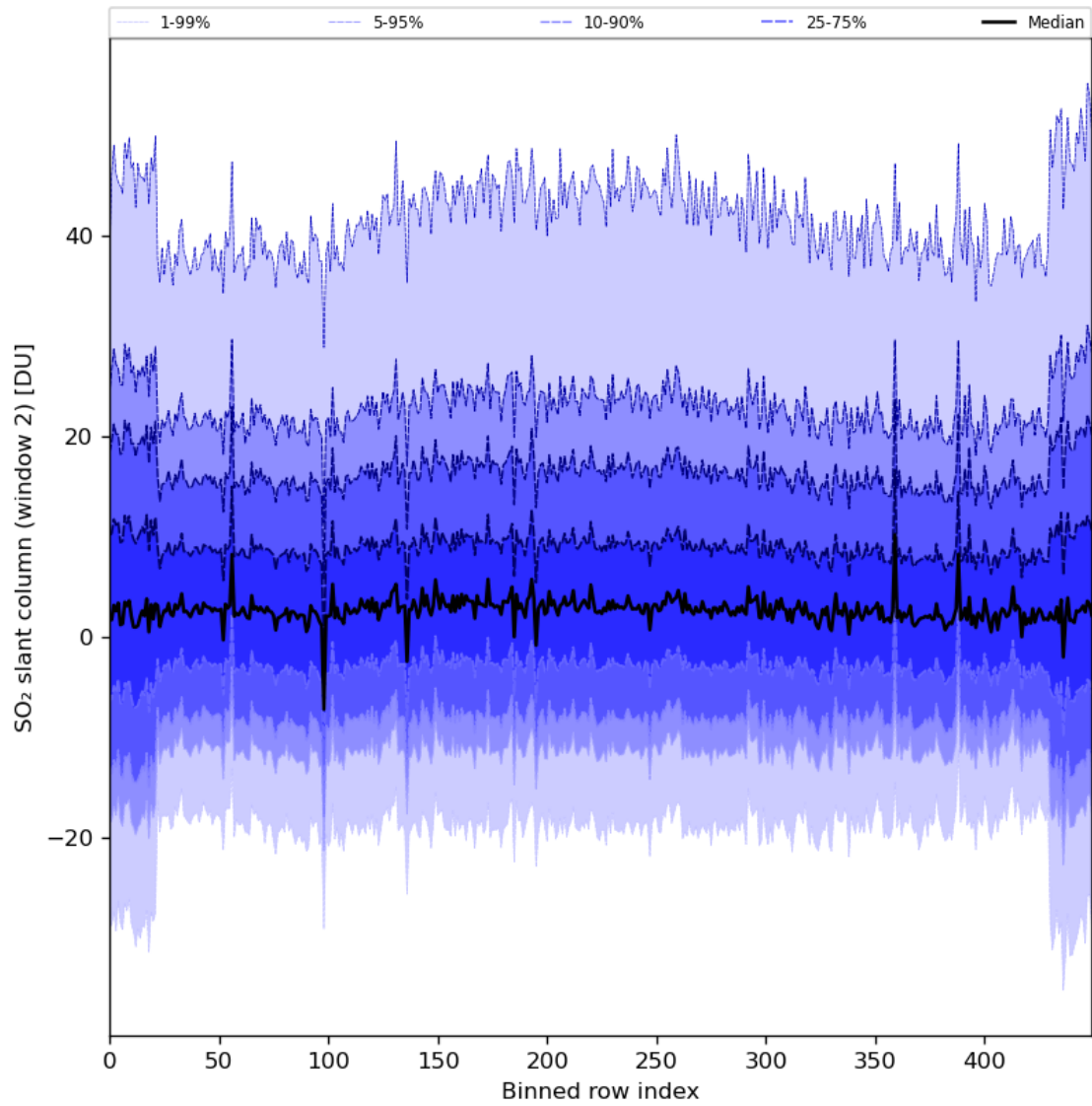
Figure 83: Along track statistics of “SO 2 slant column (window 2)” for 2024-01-03 to 2024-01-05
