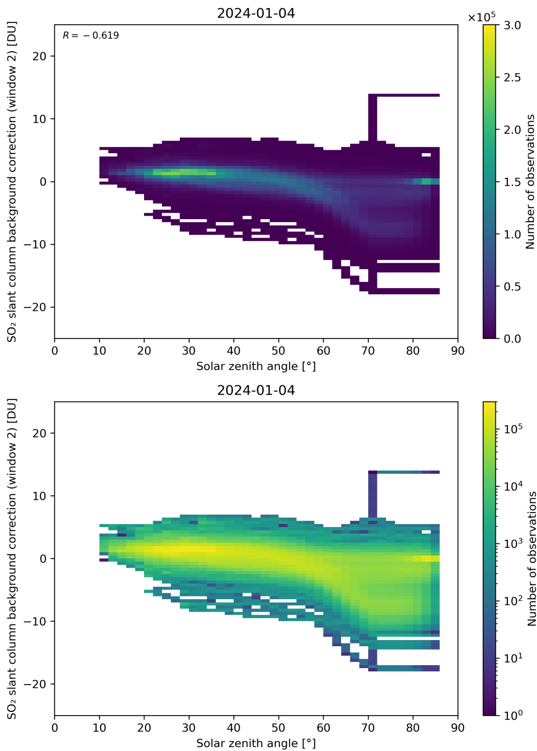
Figure 159: Scatter density plot of “Solar zenith angle” against “SO 2 slant column background correction (window 2)” for 2024-01-03 to 2024-01-05.
