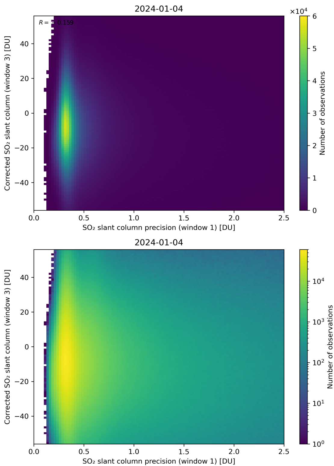
Figure 226: Scatter density plot of “SO 2 slant column precision (window 1)” against “Corrected SO 2 slant column (window 3)” for 2024-01-03 to 2024-01-05.
