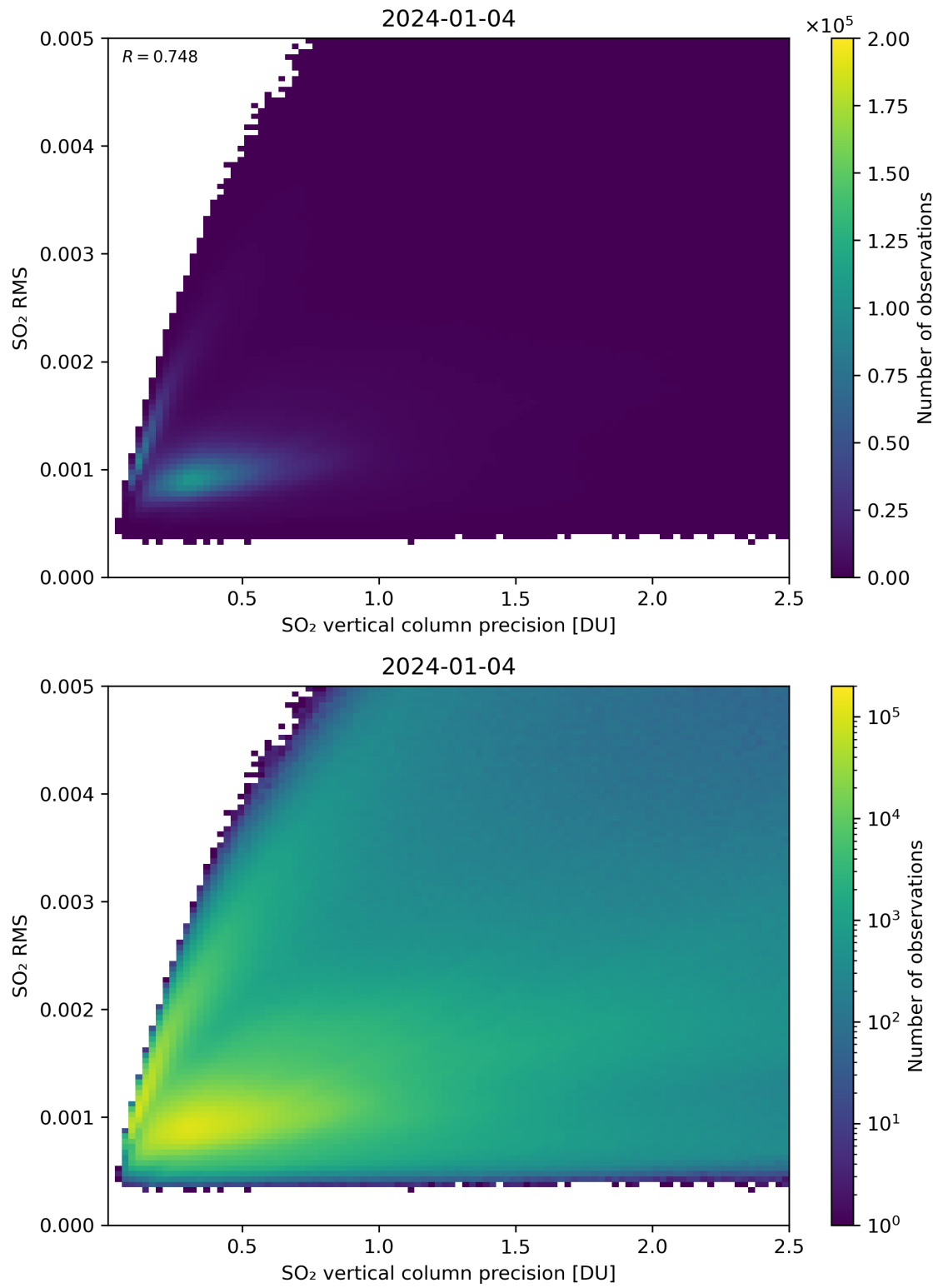
Figure 284: Scatter density plot of “SO 2 vertical column precision” against “SO 2 RMS” for 2024-01-03 to 2024-01-05.
