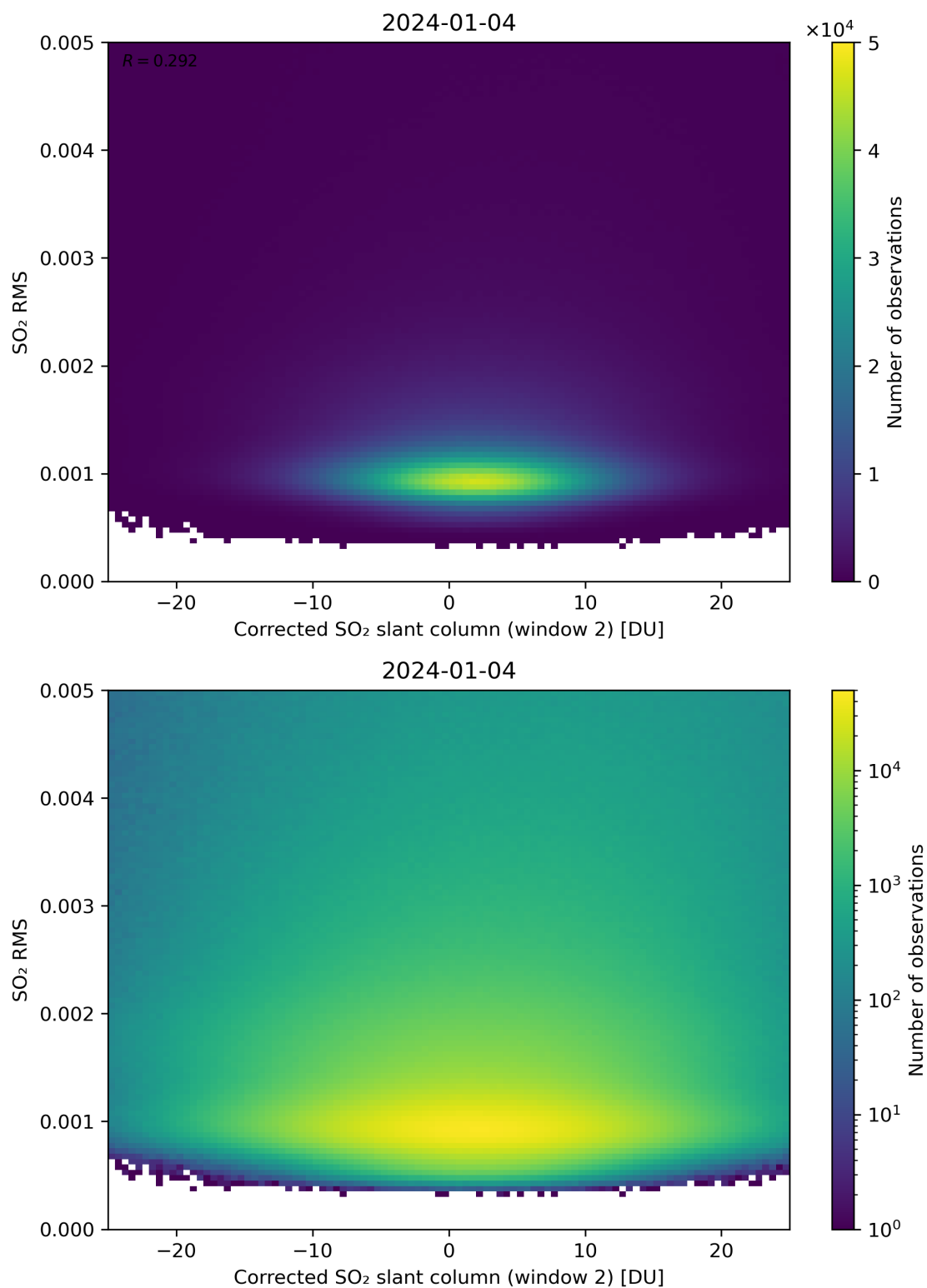
Figure 198: Scatter density plot of “Corrected SO 2 slant column (window 2)” against “SO 2 RMS” for 2024-01-03 to 2024-01-05.
