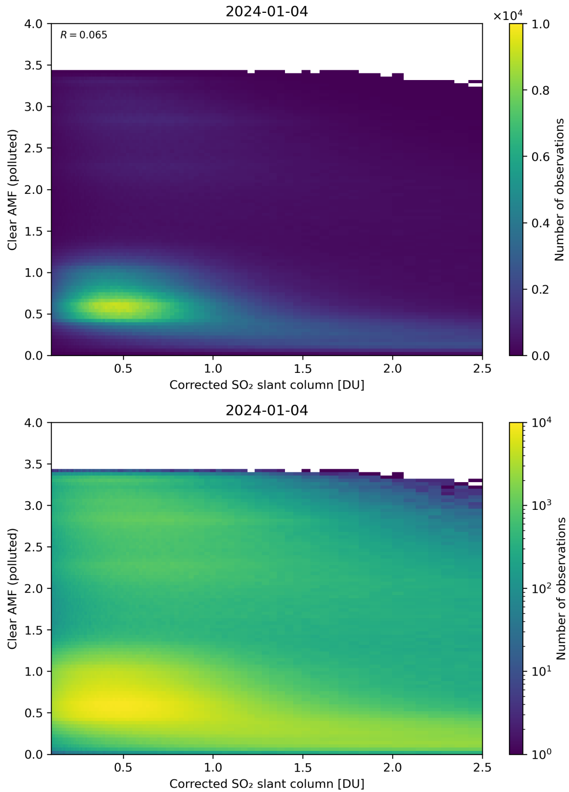
Figure 184: Scatter density plot of “Corrected SO 2 slant column” against “Clear AMF (polluted)” for 2024-01-03 to 2024-01-05.
