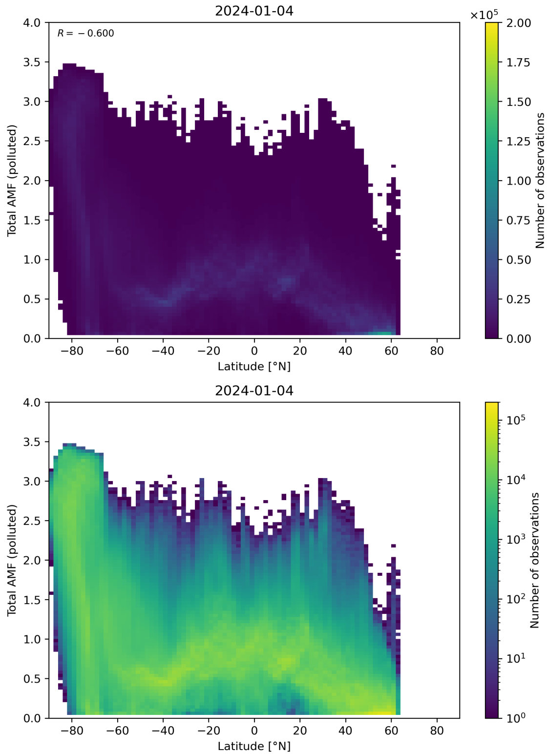
Figure 154: Scatter density plot of “Latitude” against “Total AMF (polluted)” for 2024-01-03 to 2024-01-05.
