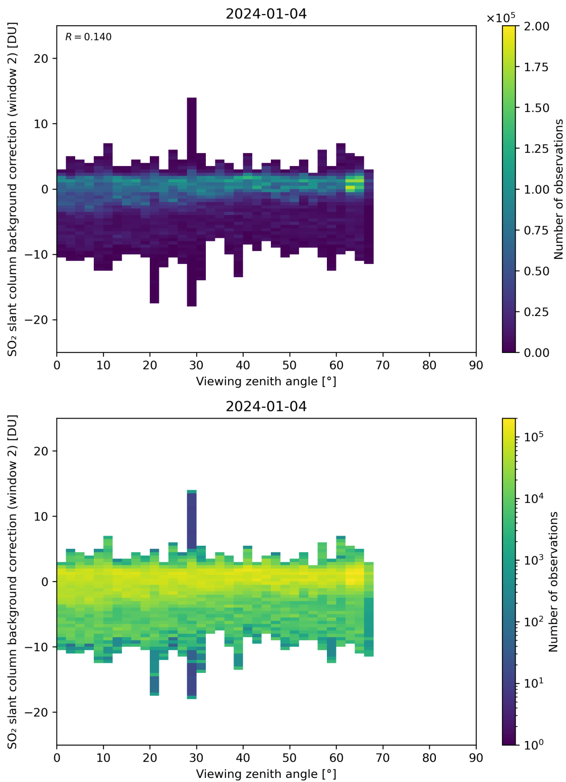
Figure 309: Scatter density plot of “Viewing zenith angle” against “SO 2 slant column background correction (window 2)” for 2024-01-03 to 2024-01-05.
