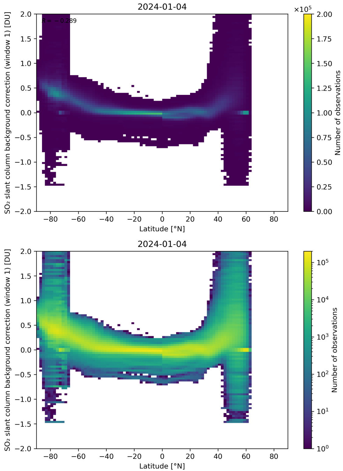
Figure 139: Scatter density plot of “Latitude” against “SO 2 slant column background correction (window 1)” for 2024-01-03 to 2024-01-05.
