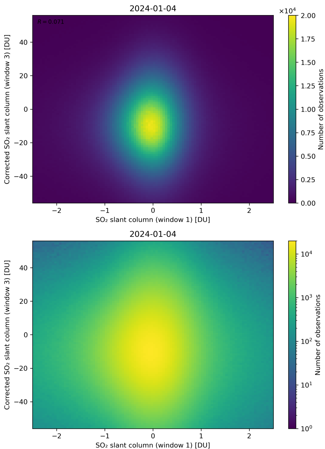
Figure 234: Scatter density plot of “SO 2 slant column (window 1)” against “Corrected SO 2 slant column (window 3)” for 2024-01-03 to 2024-01-05.
