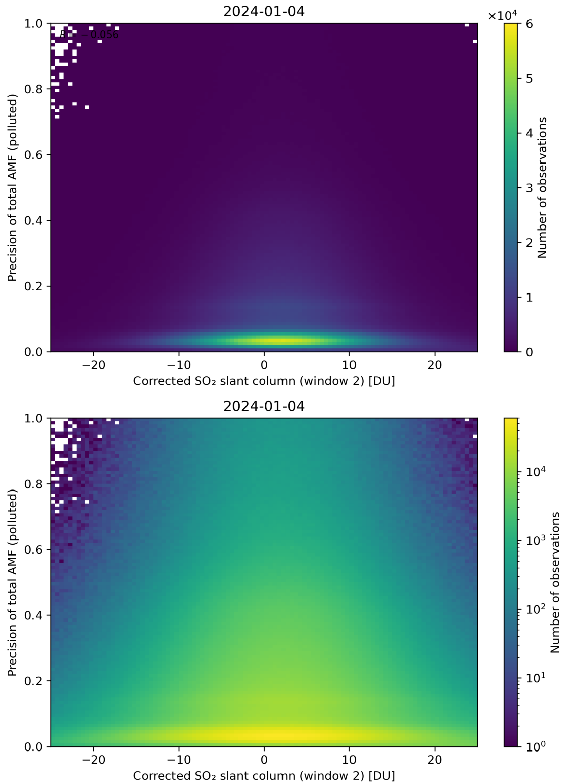
Figure 204: Scatter density plot of “Corrected SO 2 slant column (window 2)” against “Precision of total AMF (polluted)” for 2024-01-03 to 2024-01-05.
