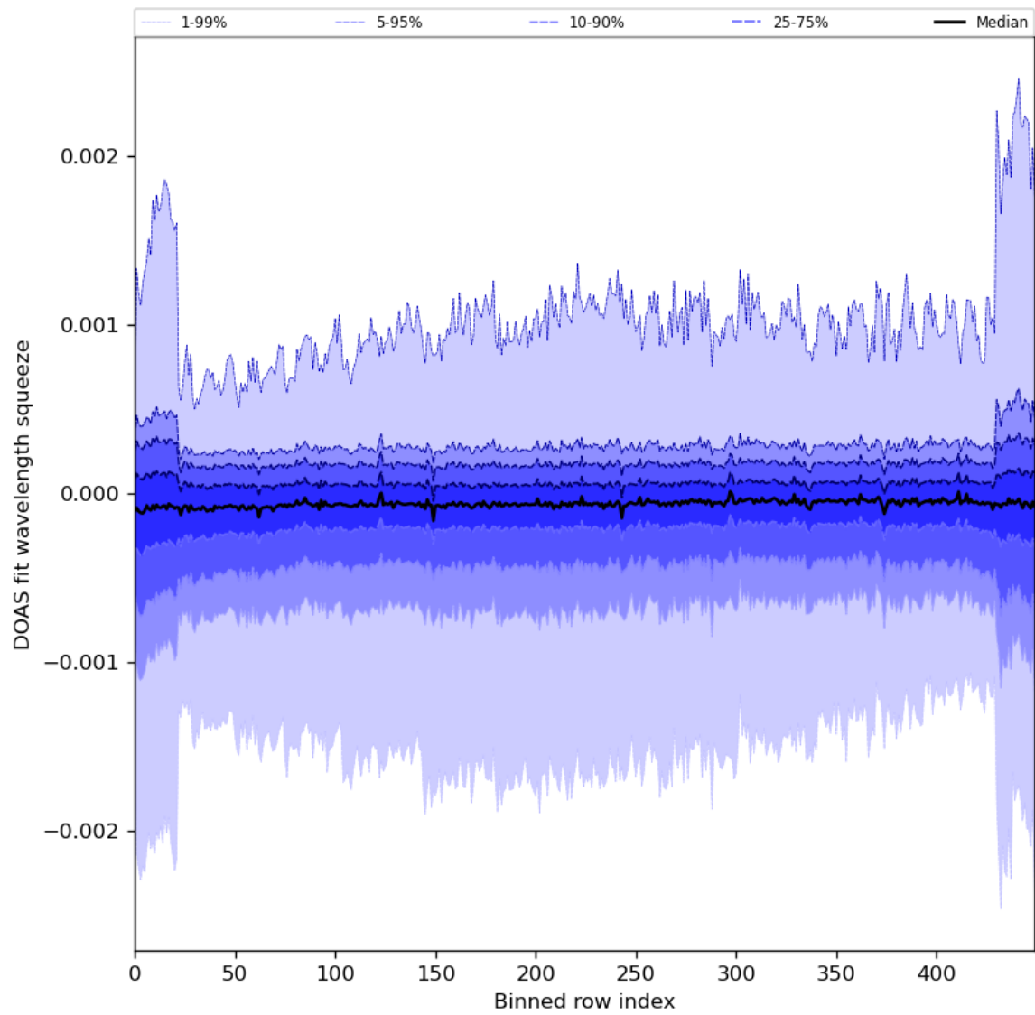
Figure 92: Along track statistics of “DOAS fit wavelength squeeze” for 2024-01-03 to 2024-01-05
