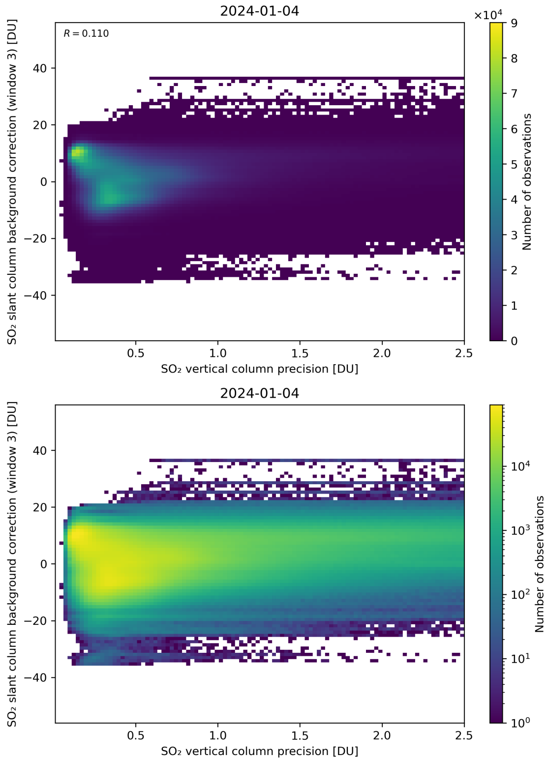
Figure 281: Scatter density plot of “SO 2 vertical column precision” against “SO 2 slant column background correction (window 3)” for 2024-01-03 to 2024-01-05.
