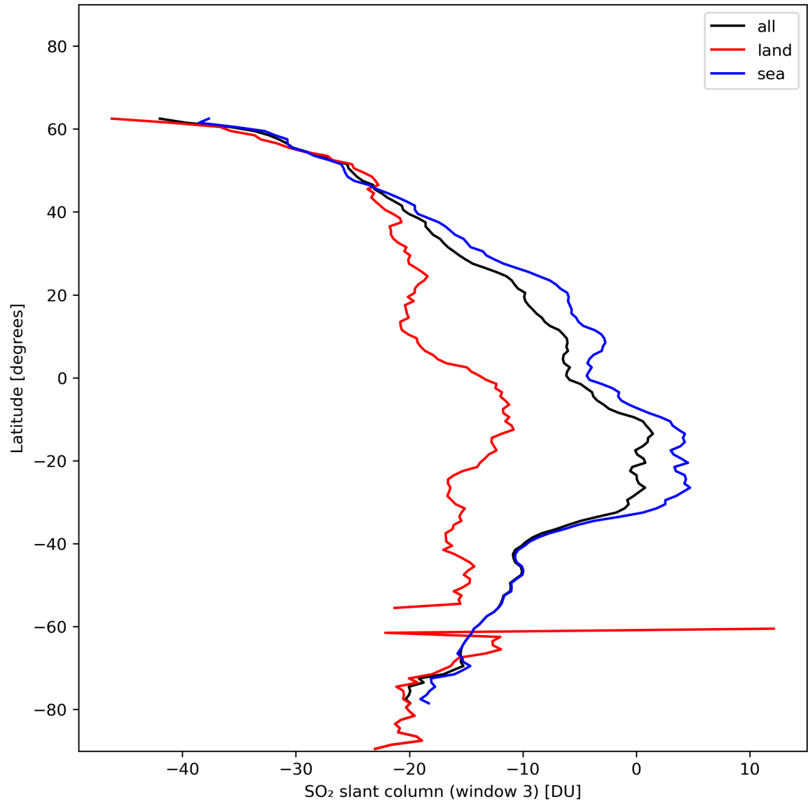
Figure 41: Zonal average of “SO 2 slant column (window 3)” for 2024-01-03 to 2024-01-05.
