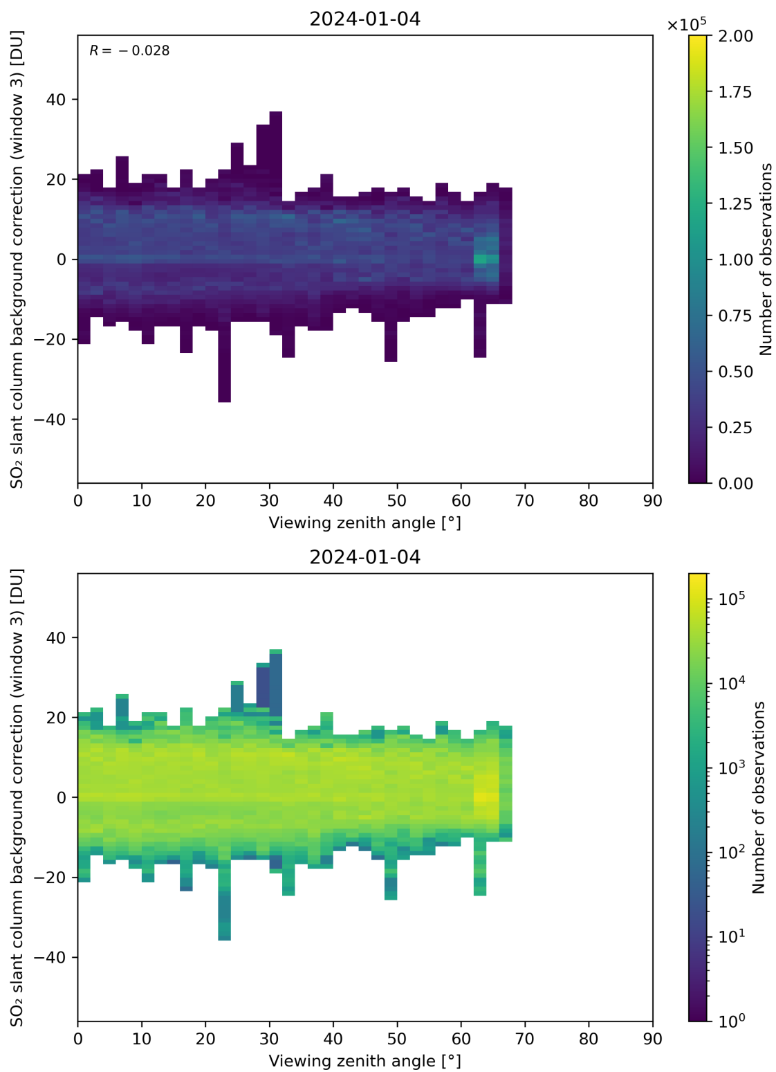
Figure 310: Scatter density plot of “Viewing zenith angle” against “SO 2 slant column background correction (window 3)” for 2024-01-03 to 2024-01-05.
