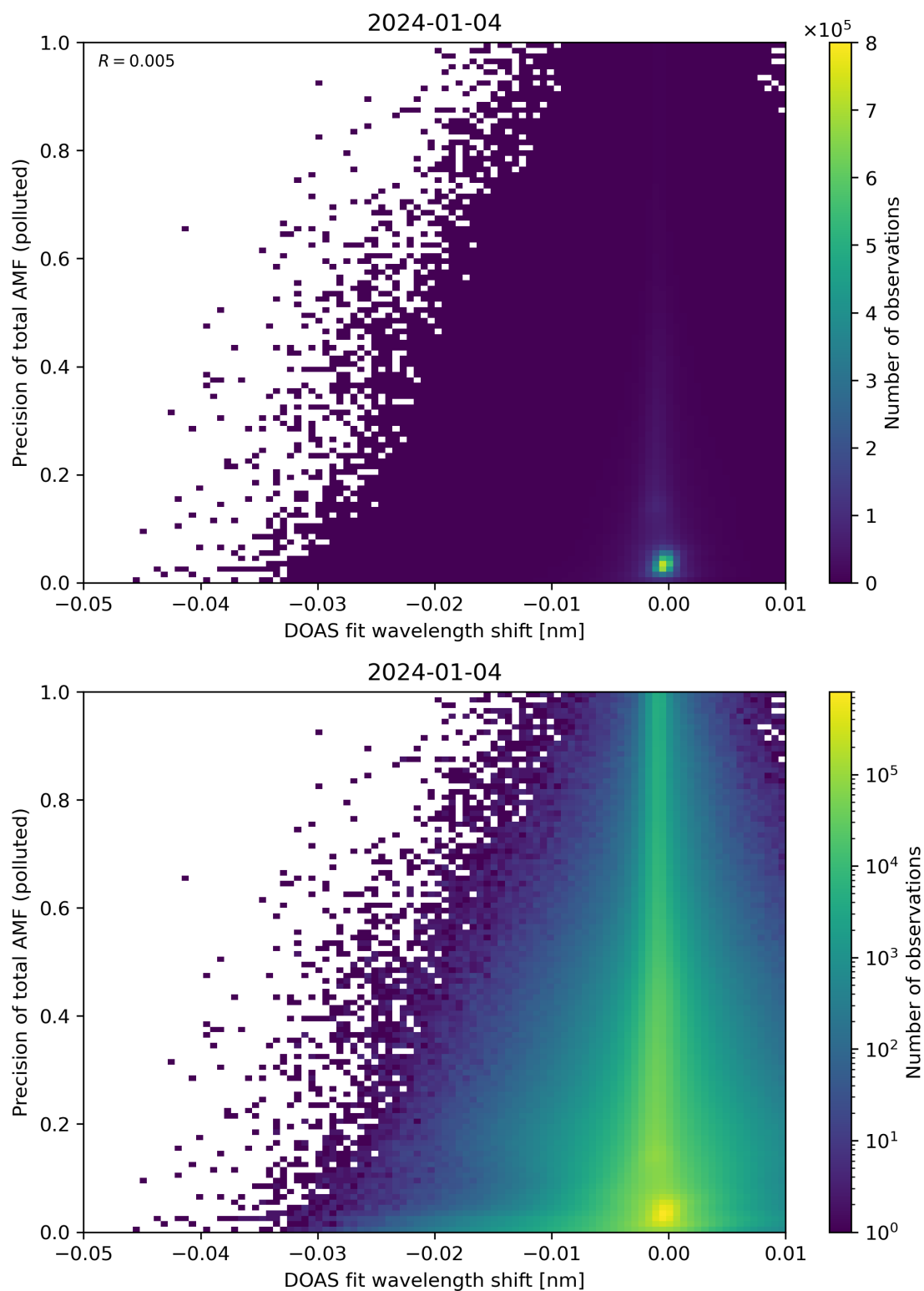
Figure 131: Scatter density plot of “DOAS fit wavelength shift” against “Precision of total AMF (polluted)” for 2024-01-03 to 2024-01-05.
