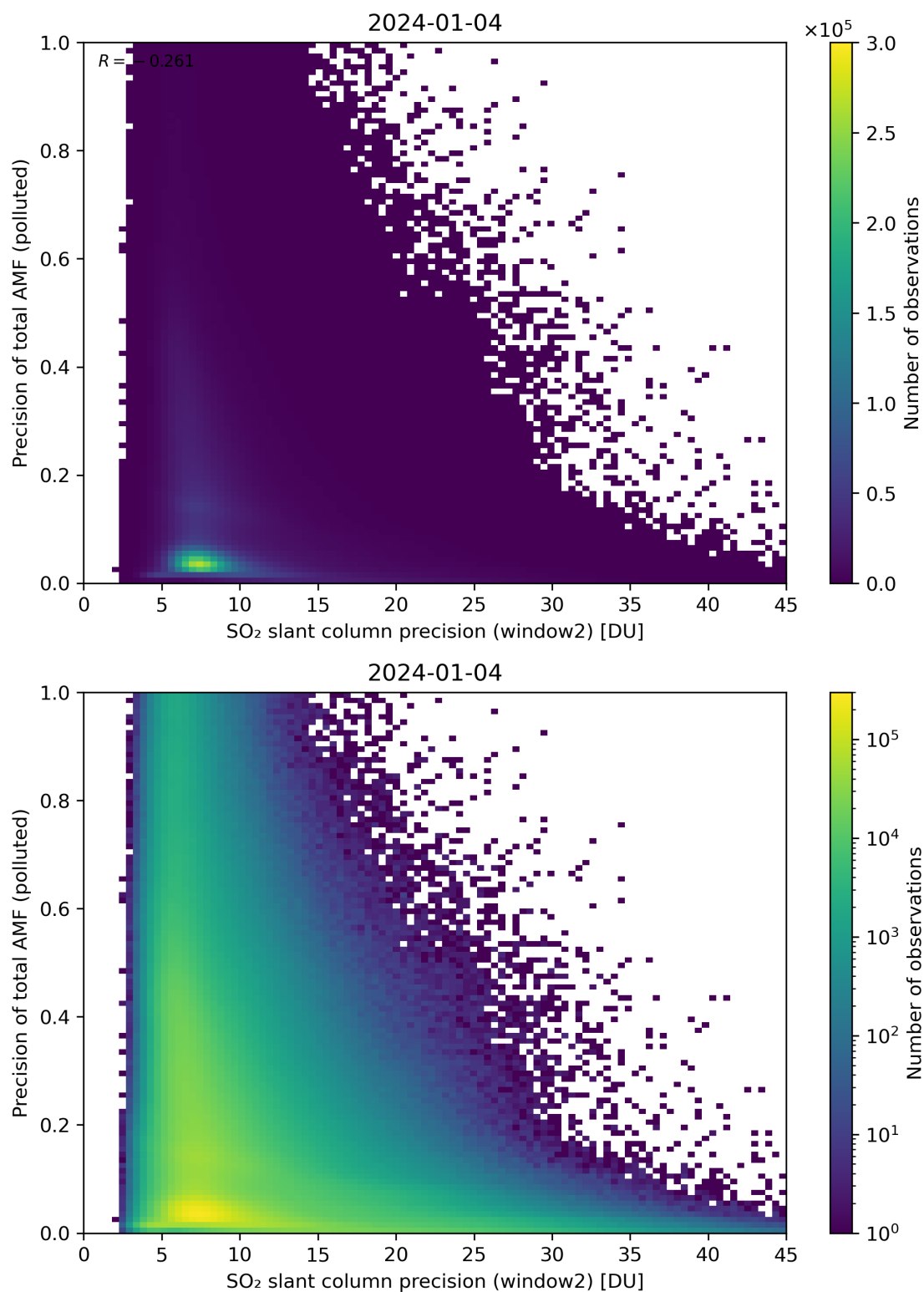
Figure 252: Scatter density plot of “SO 2 slant column precision (window2)” against “Precision of total AMF (polluted)” for 2024-01-03 to 2024-01-05.
