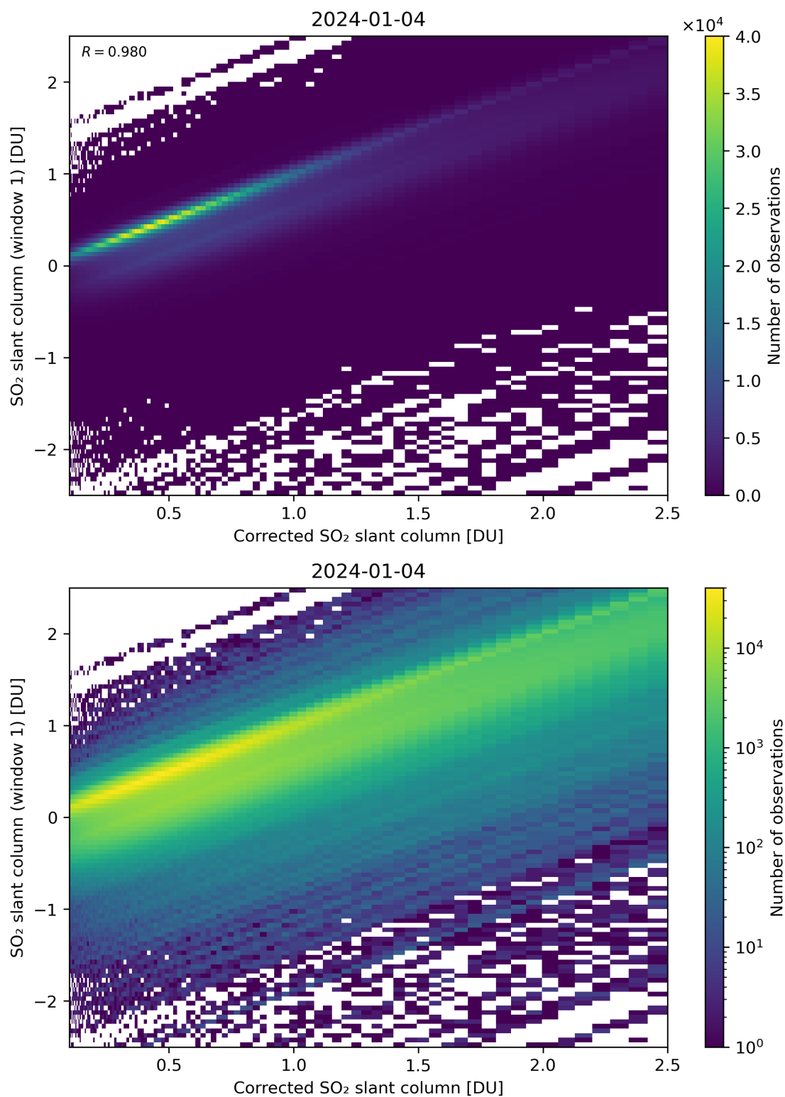
Figure 187: Scatter density plot of “Corrected SO 2 slant column” against “SO 2 slant column (window 1)” for 2024-01-03 to 2024-01-05.
