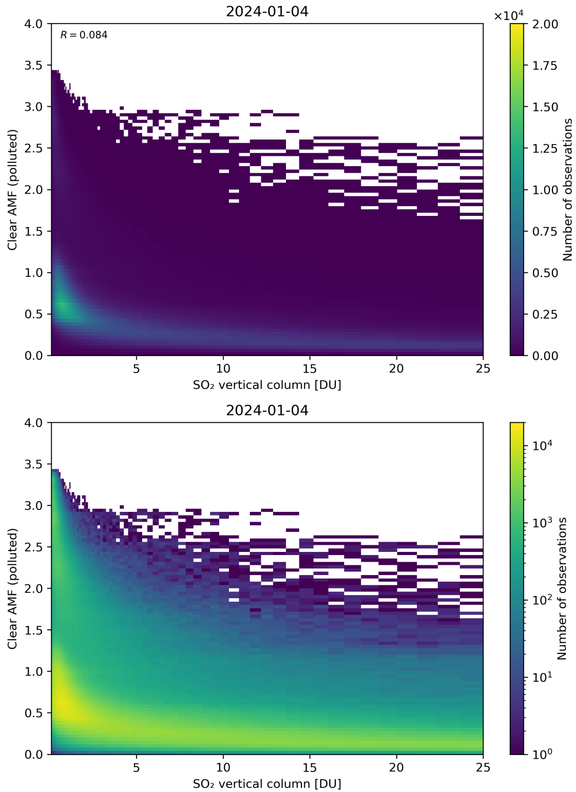
Figure 296: Scatter density plot of “SO 2 vertical column” against “Clear AMF (polluted)” for 2024-01-03 to 2024-01-05.
