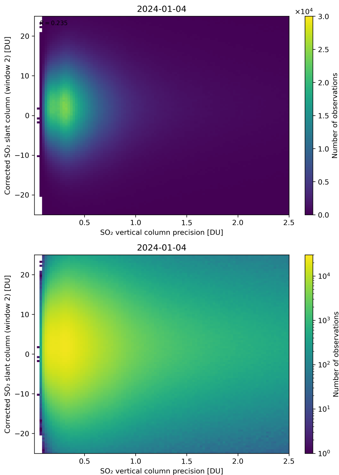
Figure 287: Scatter density plot of “SO 2 vertical column precision” against “Corrected SO 2 slant column (window 2)” for 2024-01-03 to 2024-01-05.
