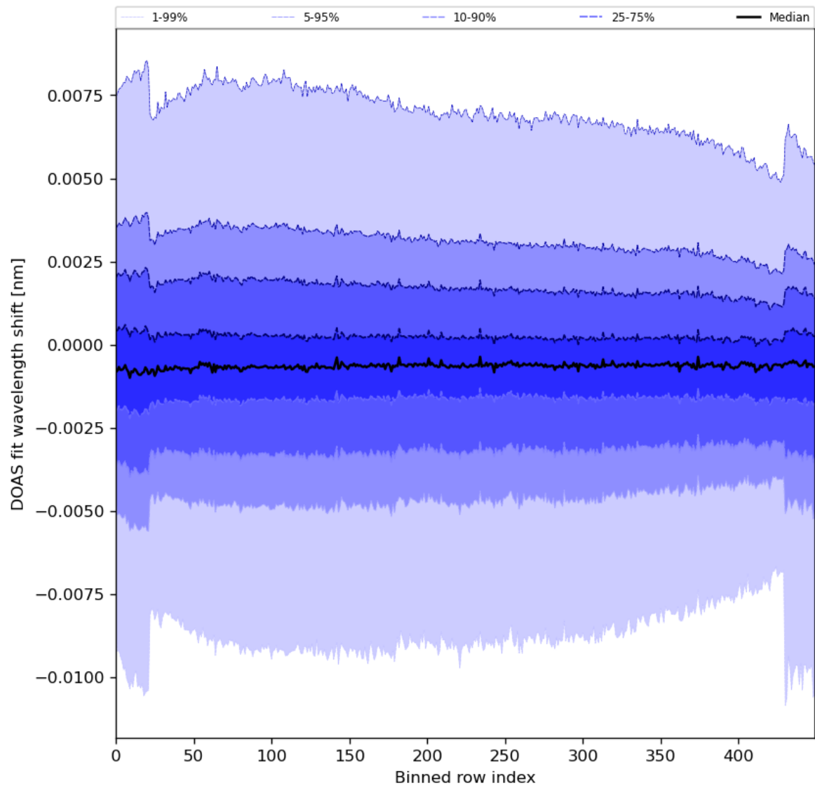
Figure 91: Along track statistics of “DOAS fit wavelength shift” for 2024-01-03 to 2024-01-05
