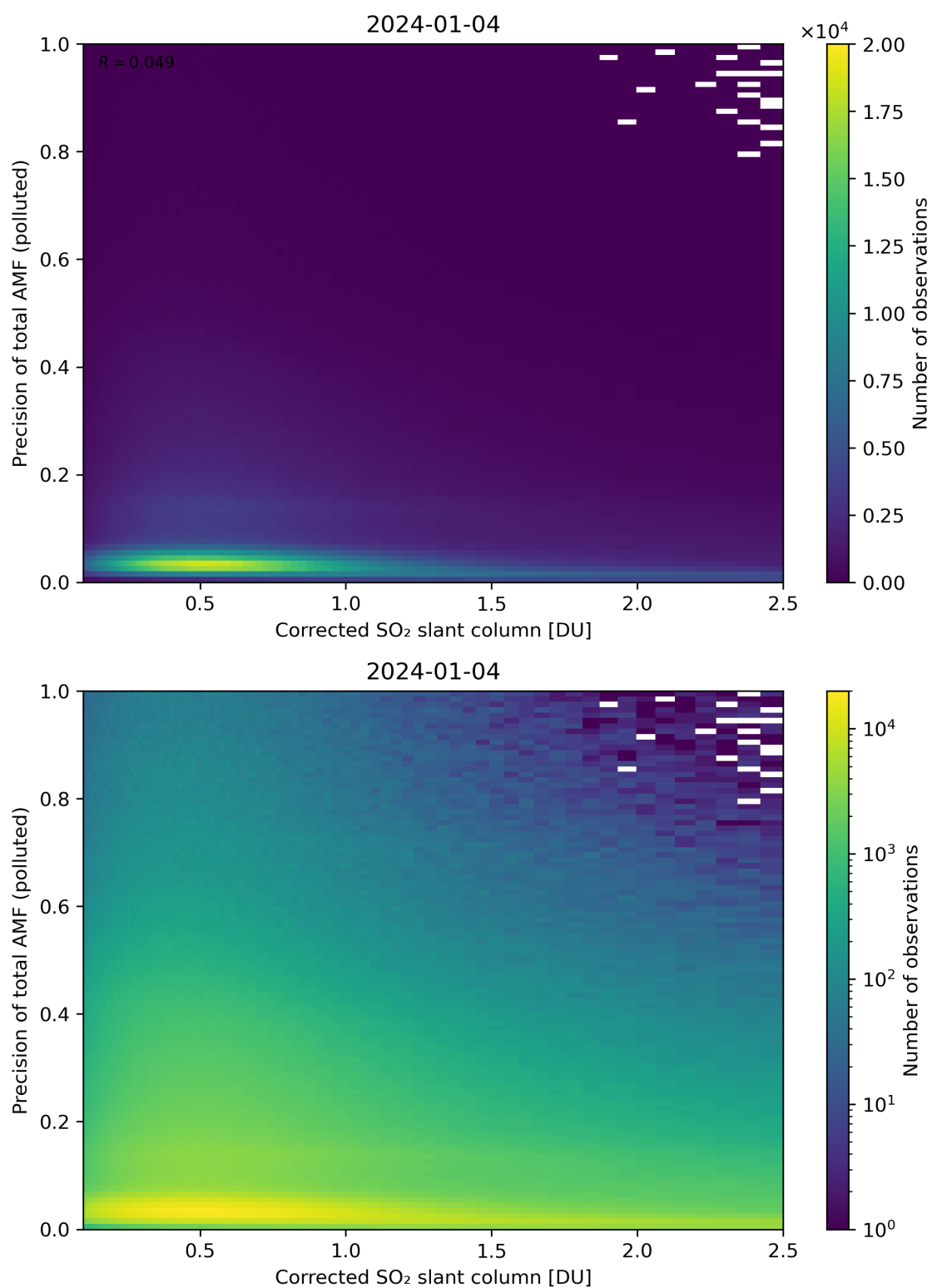
Figure 193: Scatter density plot of “Corrected SO 2 slant column” against “Precision of total AMF (polluted)” for 2024-01-03 to 2024-01-05.
