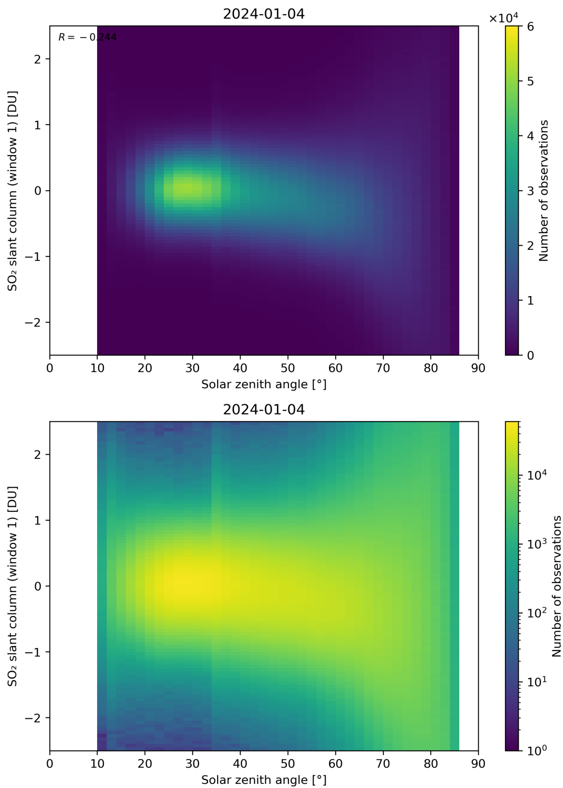
Figure 169: Scatter density plot of “Solar zenith angle” against “SO 2 slant column (window 1)” for 2024-01-03 to 2024-01-05.
