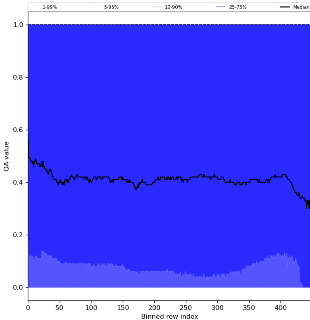
Figure 75: Along track statistics of “QA value” for 2024-01-03 to 2024-01-05
