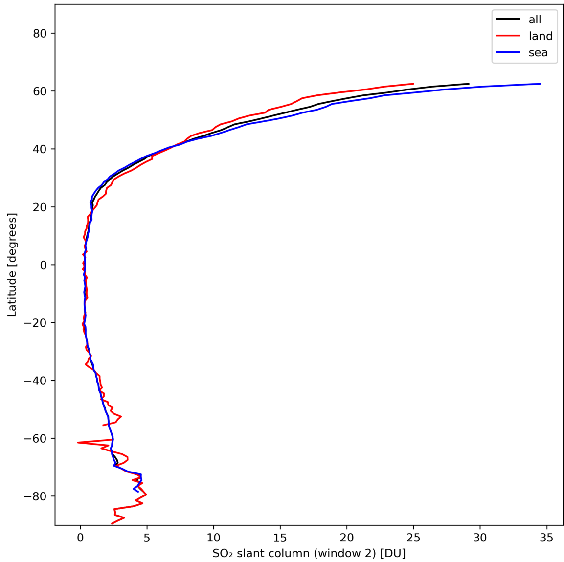
Figure 37: Zonal average of “SO 2 slant column (window 2)” for 2024-01-03 to 2024-01-05.
