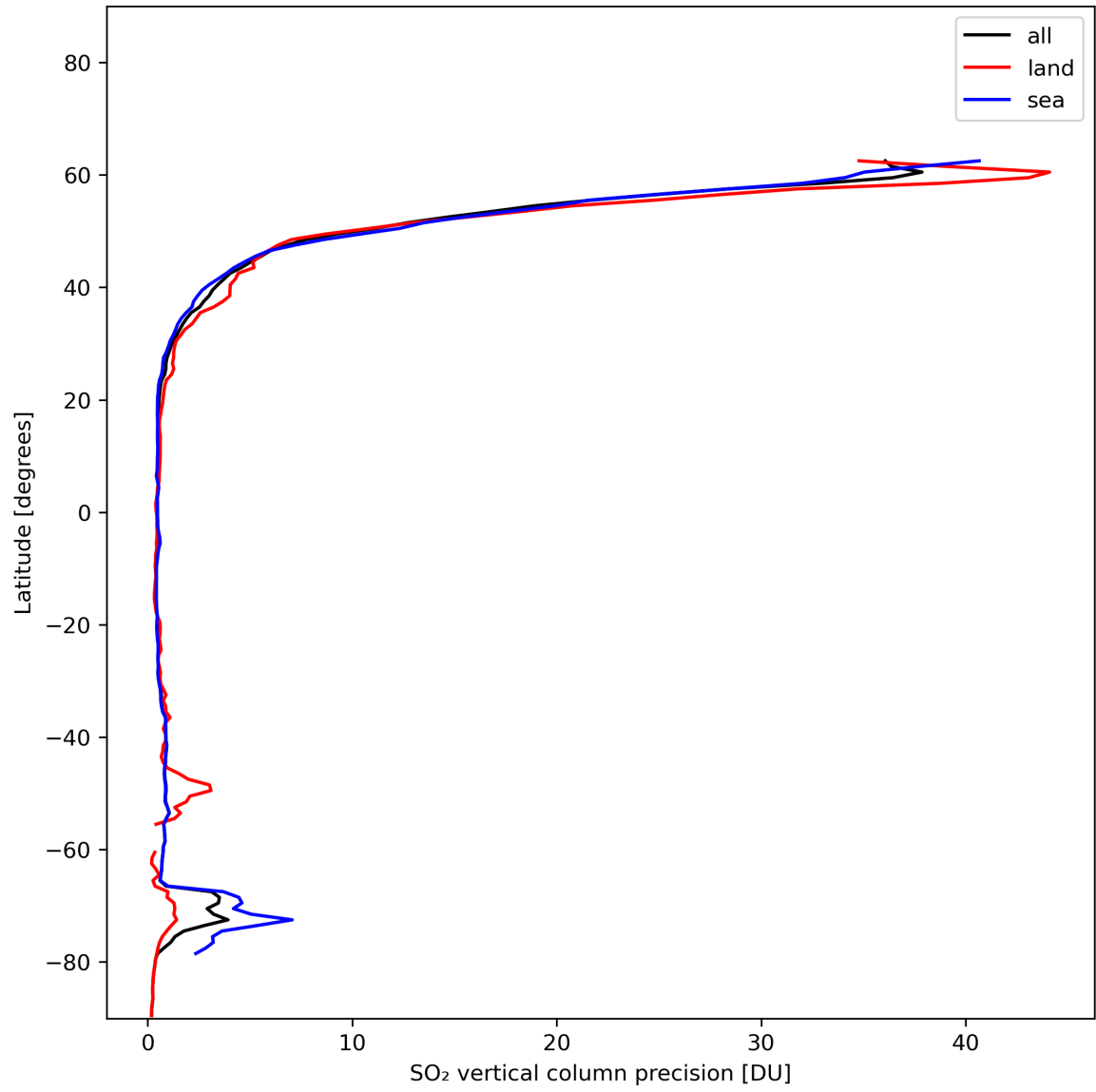
Figure 31: Zonal average of “SO 2 vertical column precision” for 2024-01-03 to 2024-01-05.
