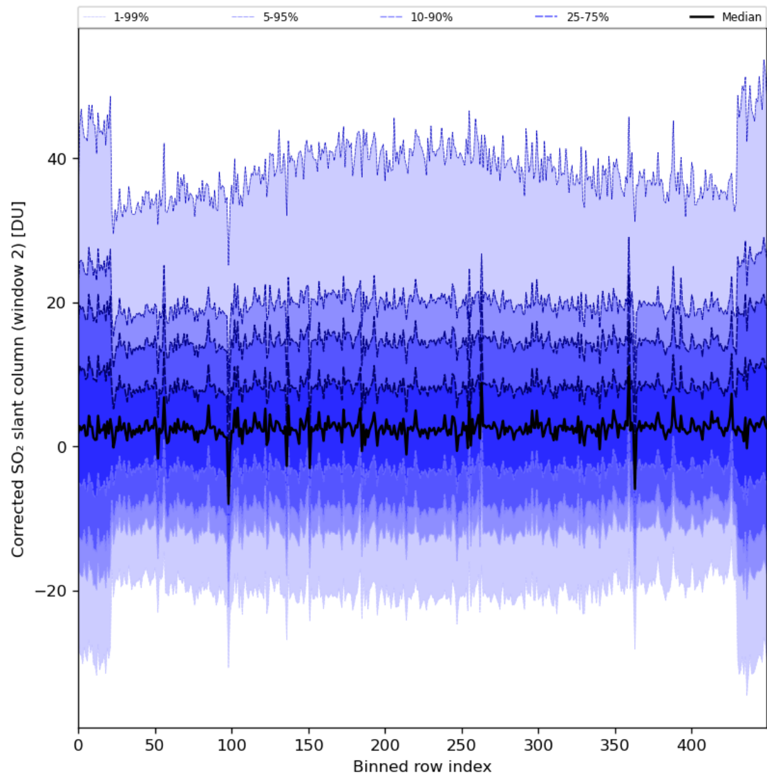
Figure 85: Along track statistics of “Corrected SO 2 slant column (window 2)” for 2024-01-03 to 2024-01-05
