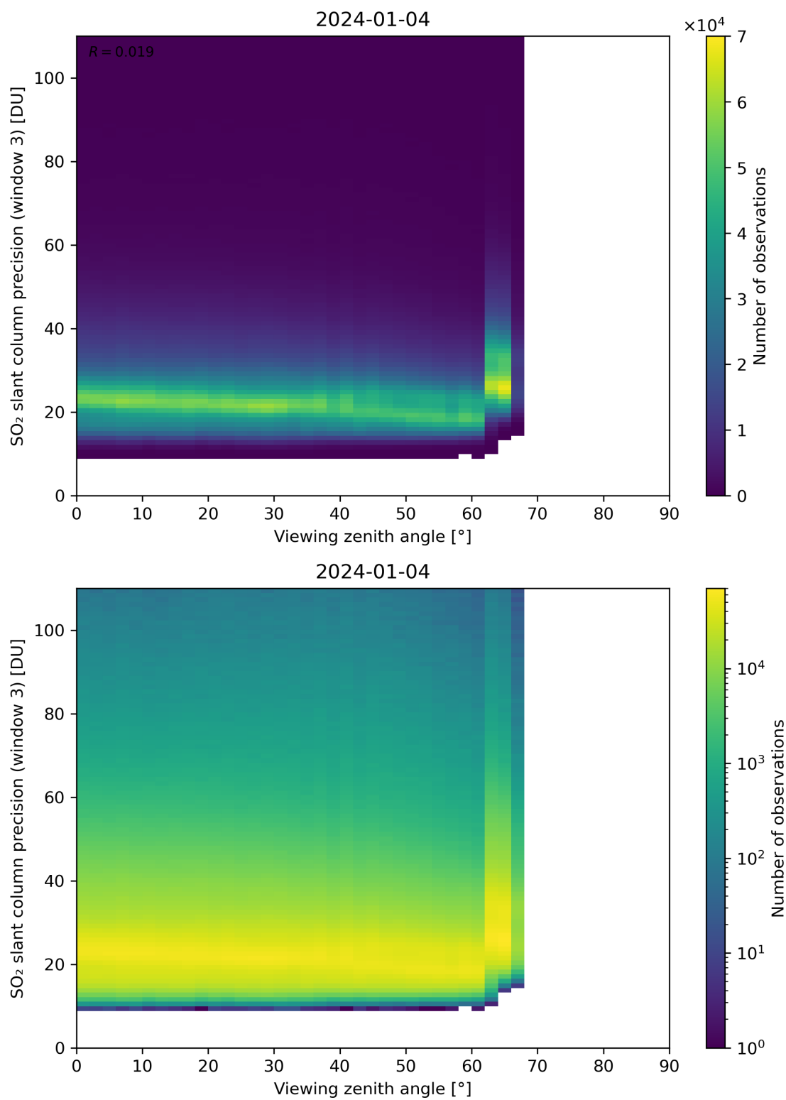
Figure 324: Scatter density plot of “Viewing zenith angle” against “SO 2 slant column precision (window 3)” for 2024-01-03 to 2024-01-05.
