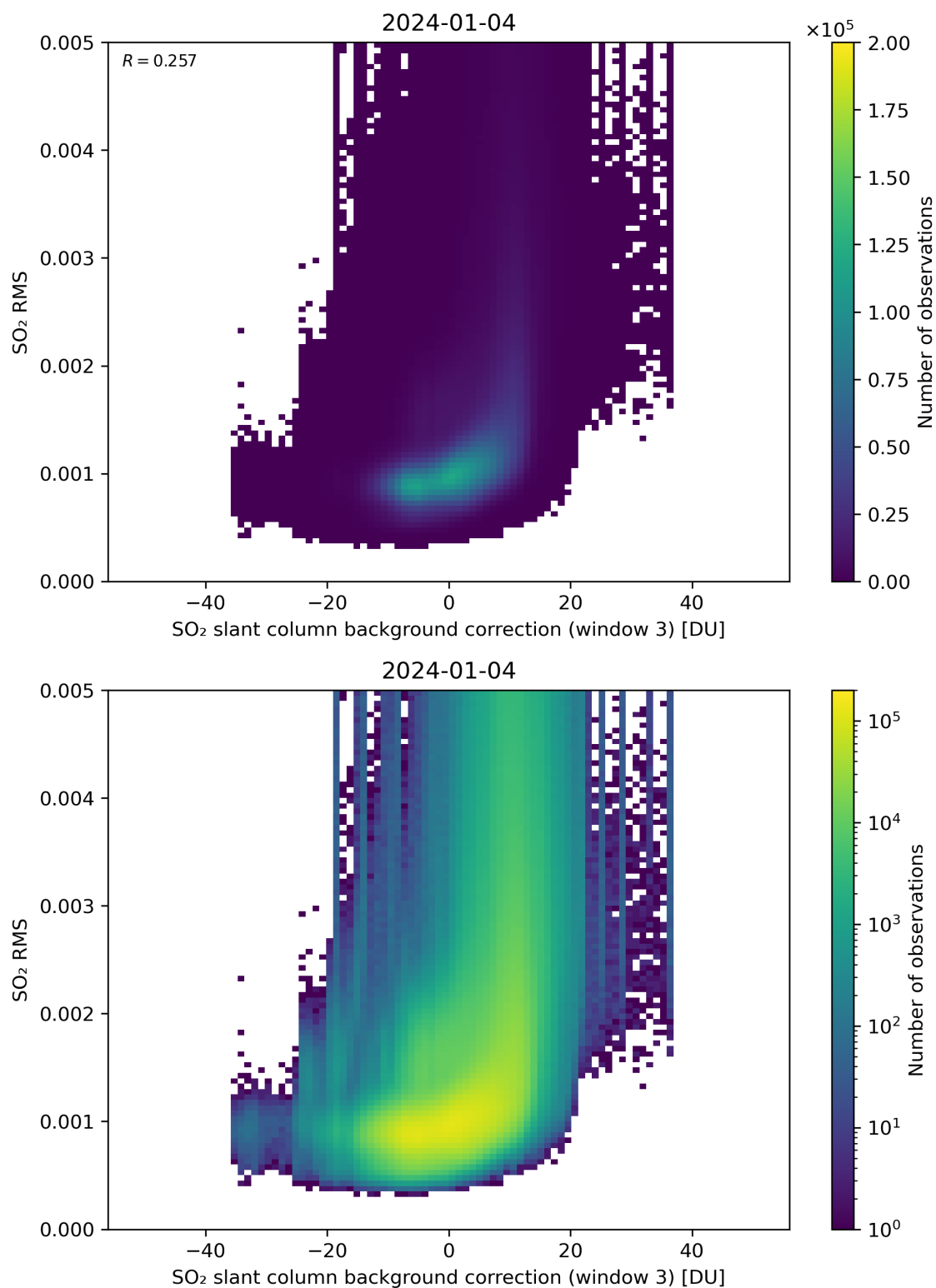
Figure 123: Scatter density plot of “SO 2 slant column background correction (window 3)” against “SO 2 RMS” for 2024-01-03 to 2024-01-05.
