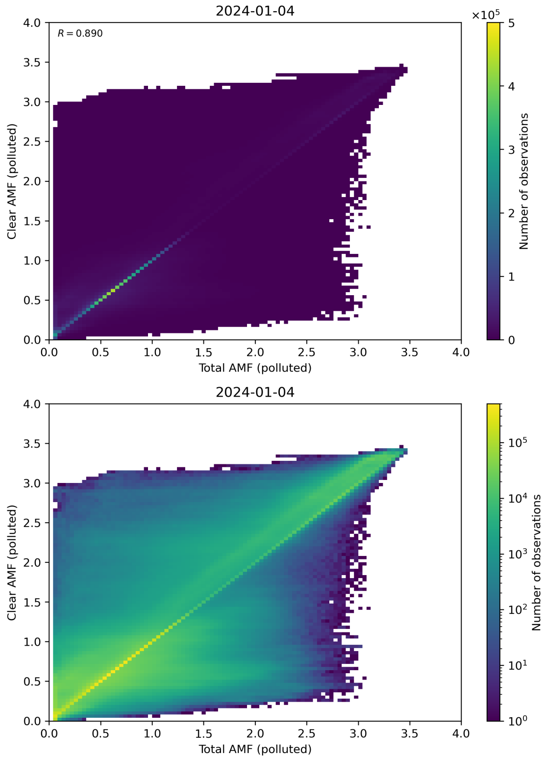
Figure 271: Scatter density plot of “Total AMF (polluted)” against “Clear AMF (polluted)” for 2024-01-03 to 2024-01-05.
