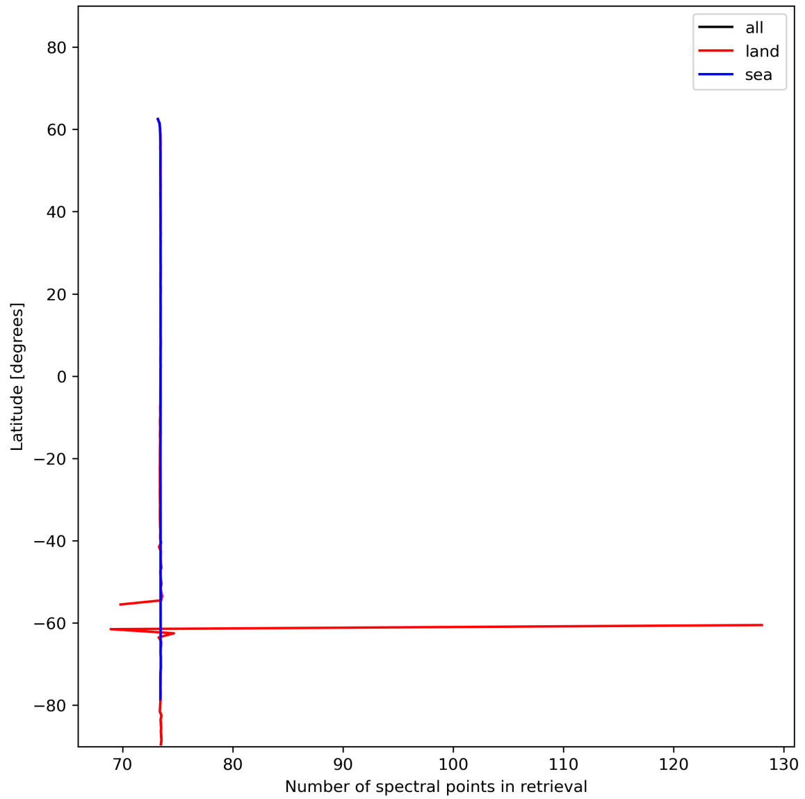
Figure 51: Zonal average of “Number of spectral points in retrieval” for 2024-01-03 to 2024-01-05.
