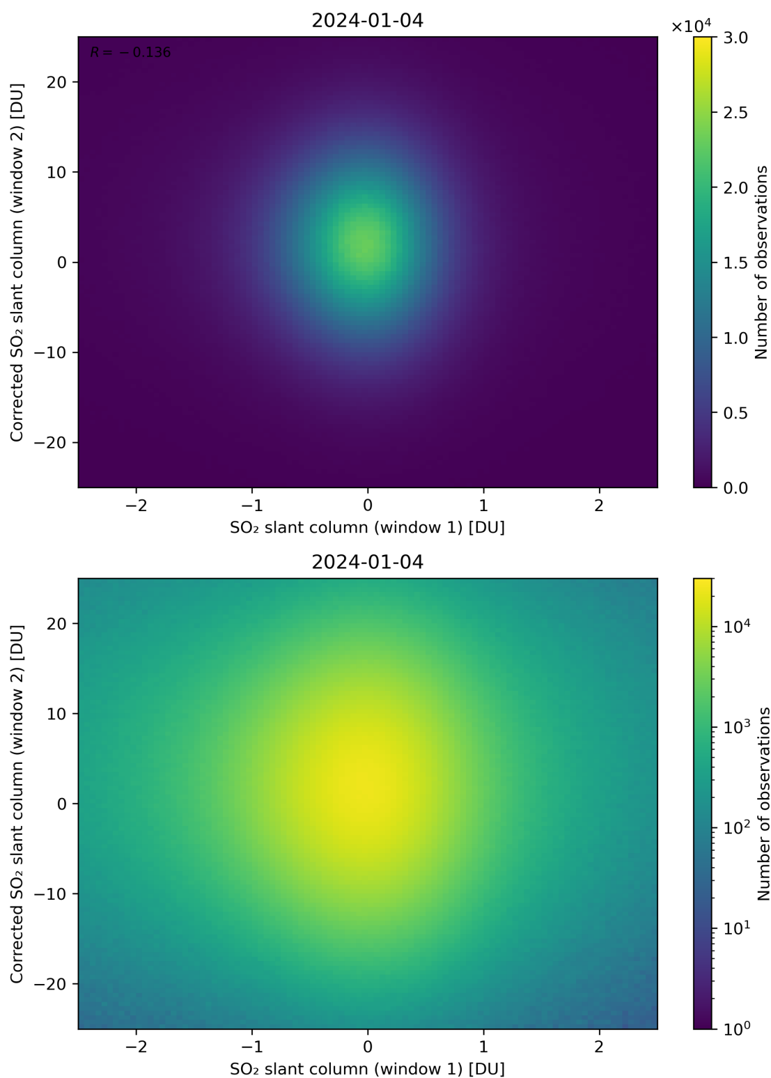
Figure 233: Scatter density plot of “SO 2 slant column (window 1)” against “Corrected SO 2 slant column (window 2)” for 2024-01-03 to 2024-01-05.
