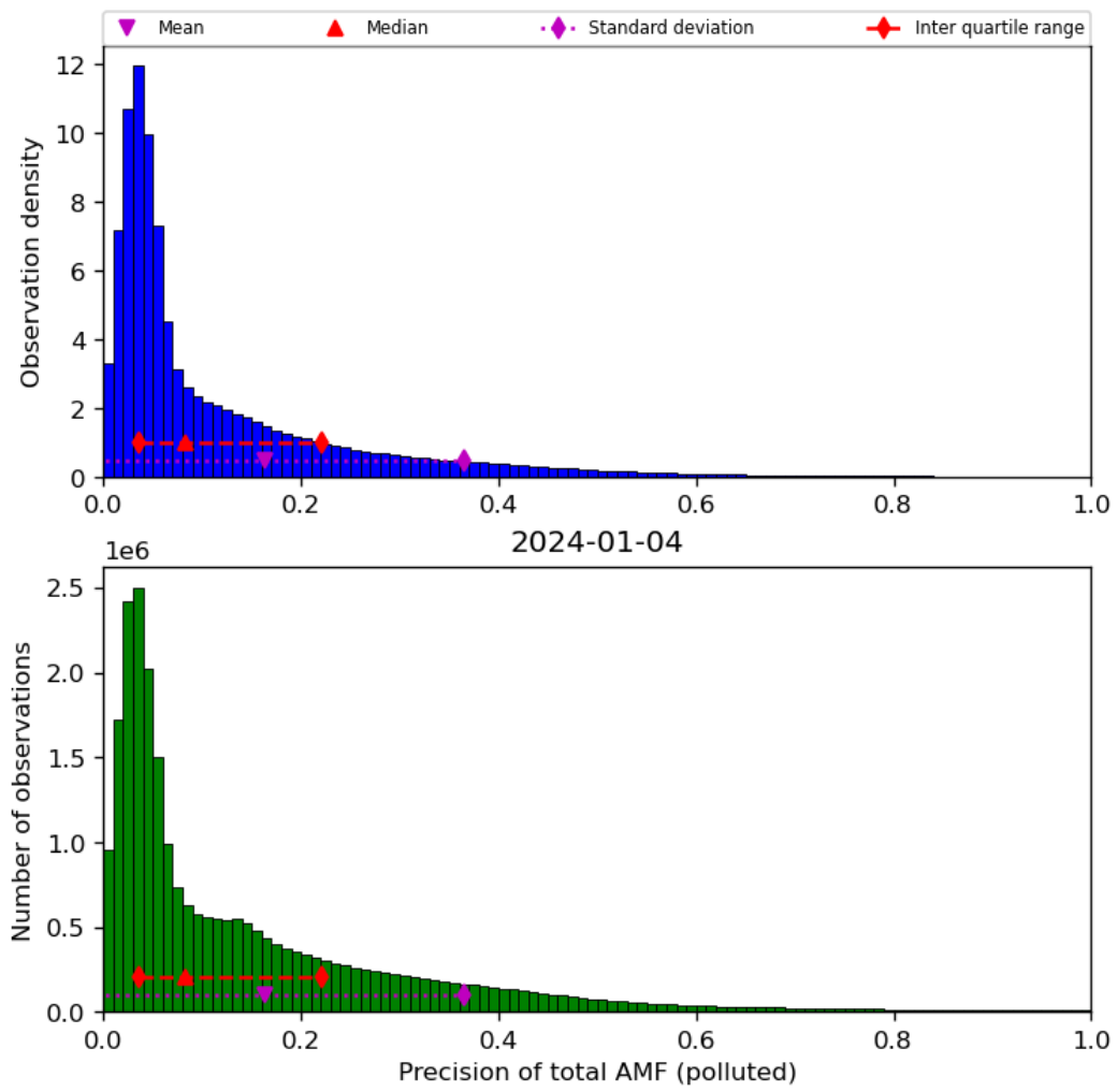
Figure 72: Histogram of “Precision of total AMF (polluted)” for 2024-01-03 to 2024-01-05
