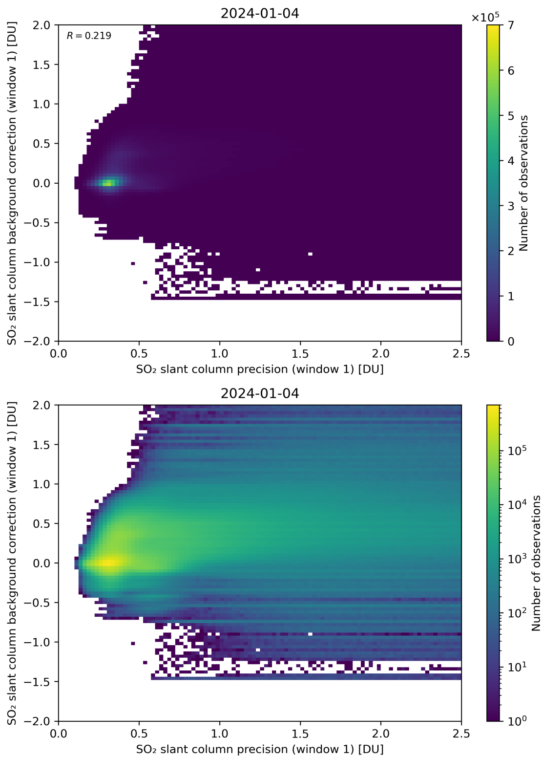
Figure 218: Scatter density plot of “SO 2 slant column precision (window 1)” against “SO 2 slant column background correction (window 1)” for 2024-01-03 to 2024-01-05.
