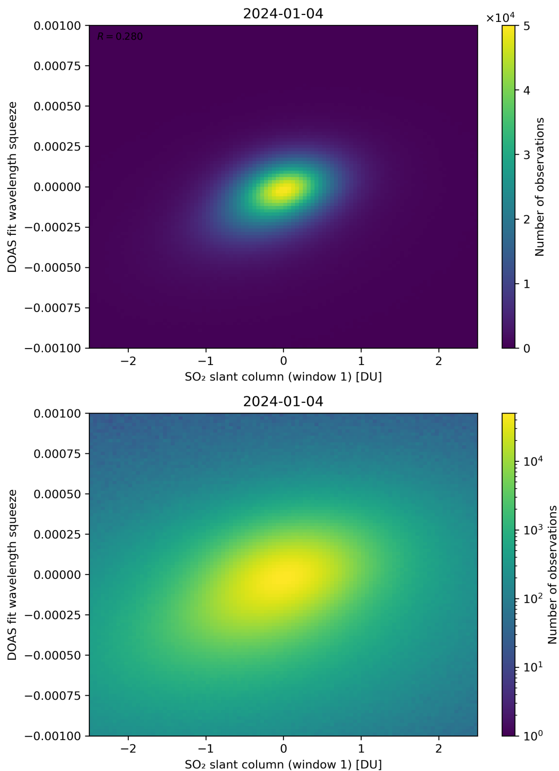
Figure 216: Scatter density plot of “SO 2 slant column (window 1)” against “DOAS fit wavelength squeeze” for 2024-01-03 to 2024-01-05.
