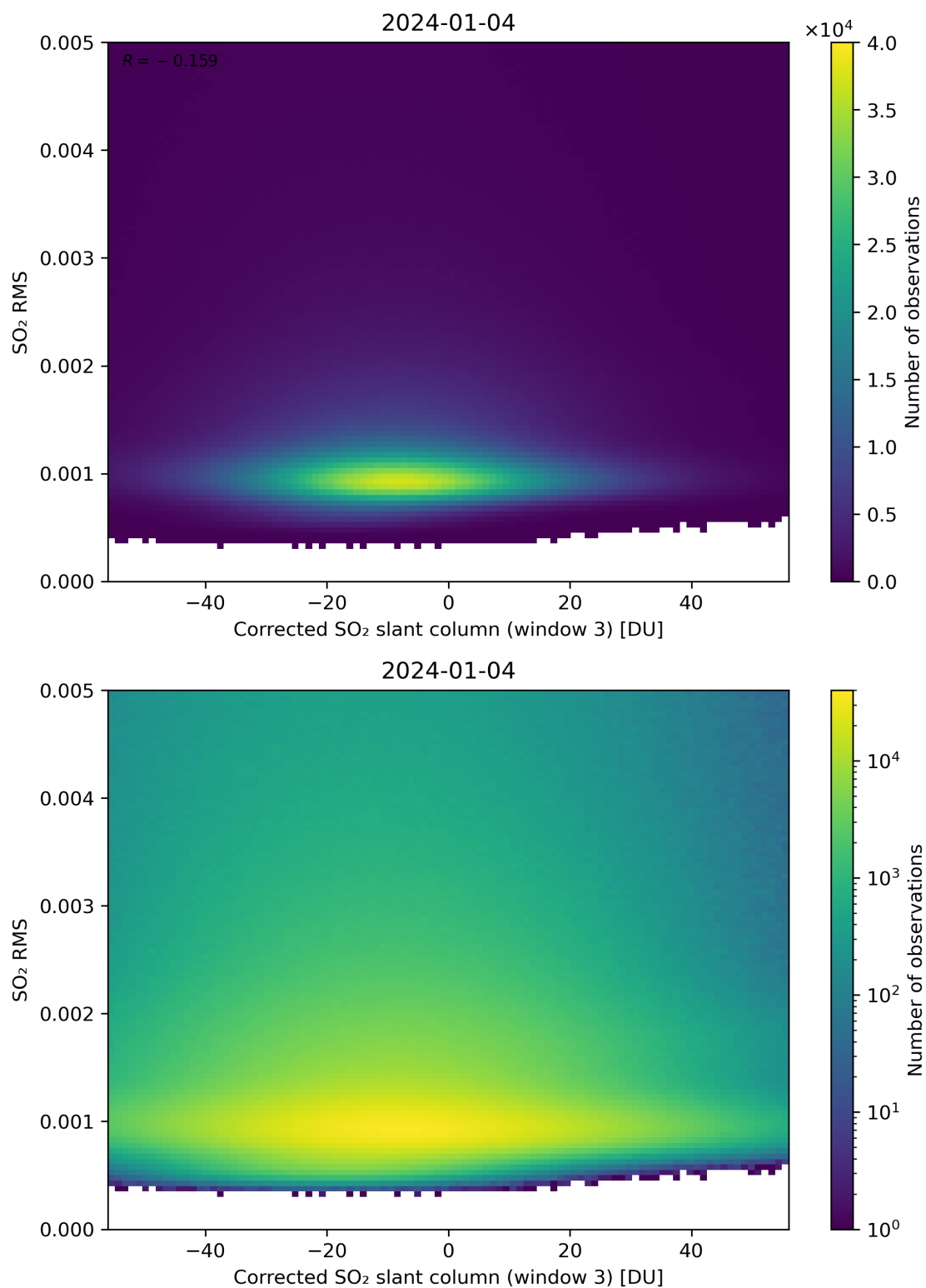
Figure 208: Scatter density plot of “Corrected SO 2 slant column (window 3)” against “SO 2 RMS” for 2024-01-03 to 2024-01-05.
