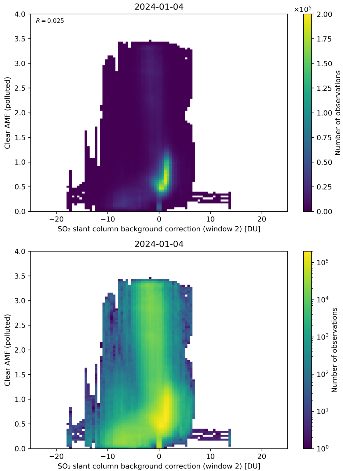
Figure 115: Scatter density plot of “SO 2 slant column background correction (window 2)” against “Clear AMF (polluted)” for 2024-01-03 to 2024-01-05.
