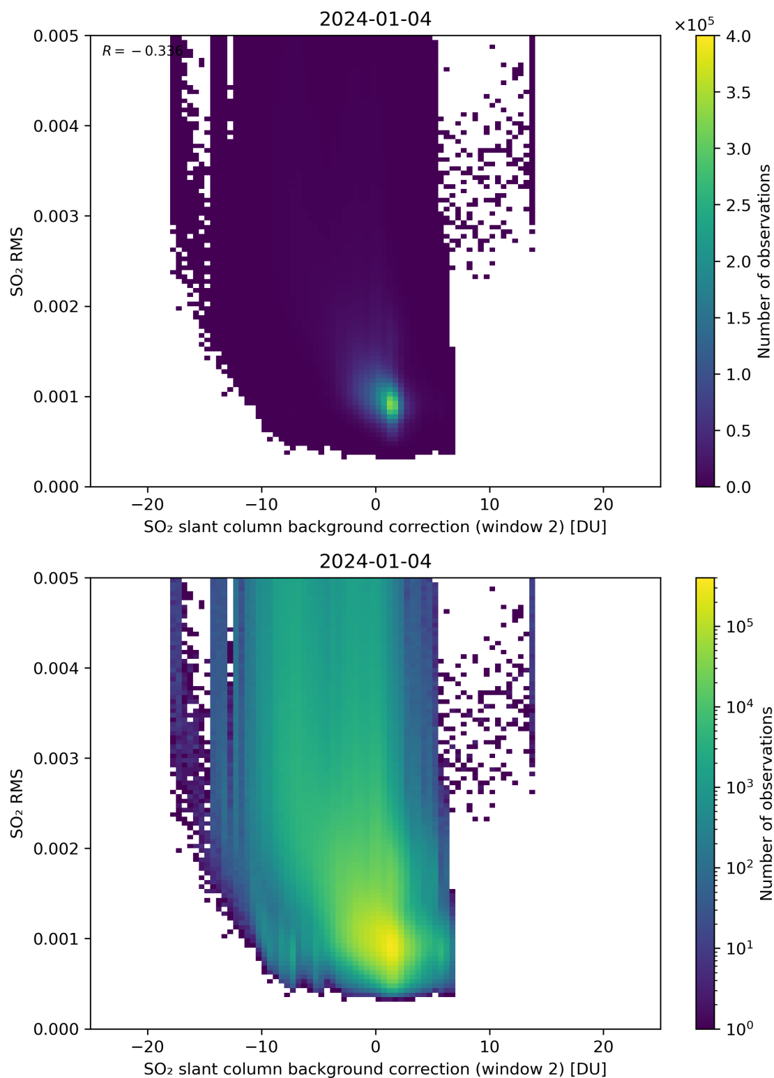
Figure 114: Scatter density plot of “SO 2 slant column background correction (window 2)” against “SO 2 RMS” for 2024-01-03 to 2024-01-05.
