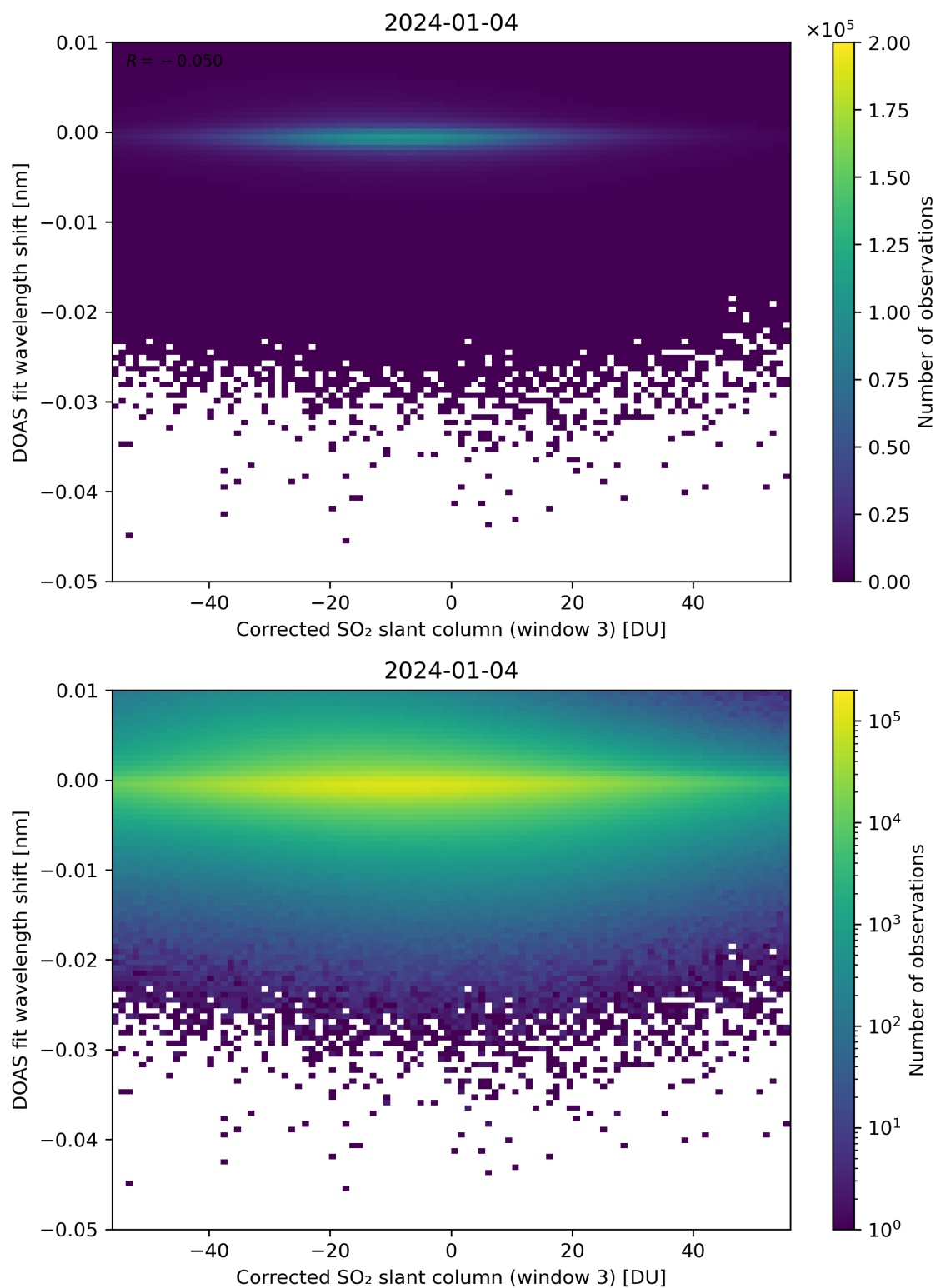
Figure 206: Scatter density plot of “Corrected SO 2 slant column (window 3)” against “DOAS fit wavelength shift” for 2024-01-03 to 2024-01-05.
