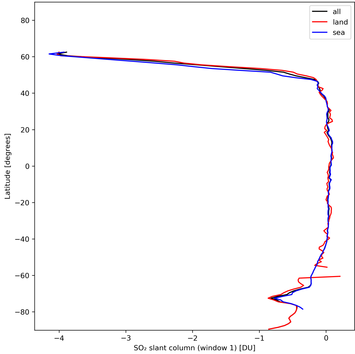
Figure 33: Zonal average of “SO 2 slant column (window 1)” for 2024-01-03 to 2024-01-05.
