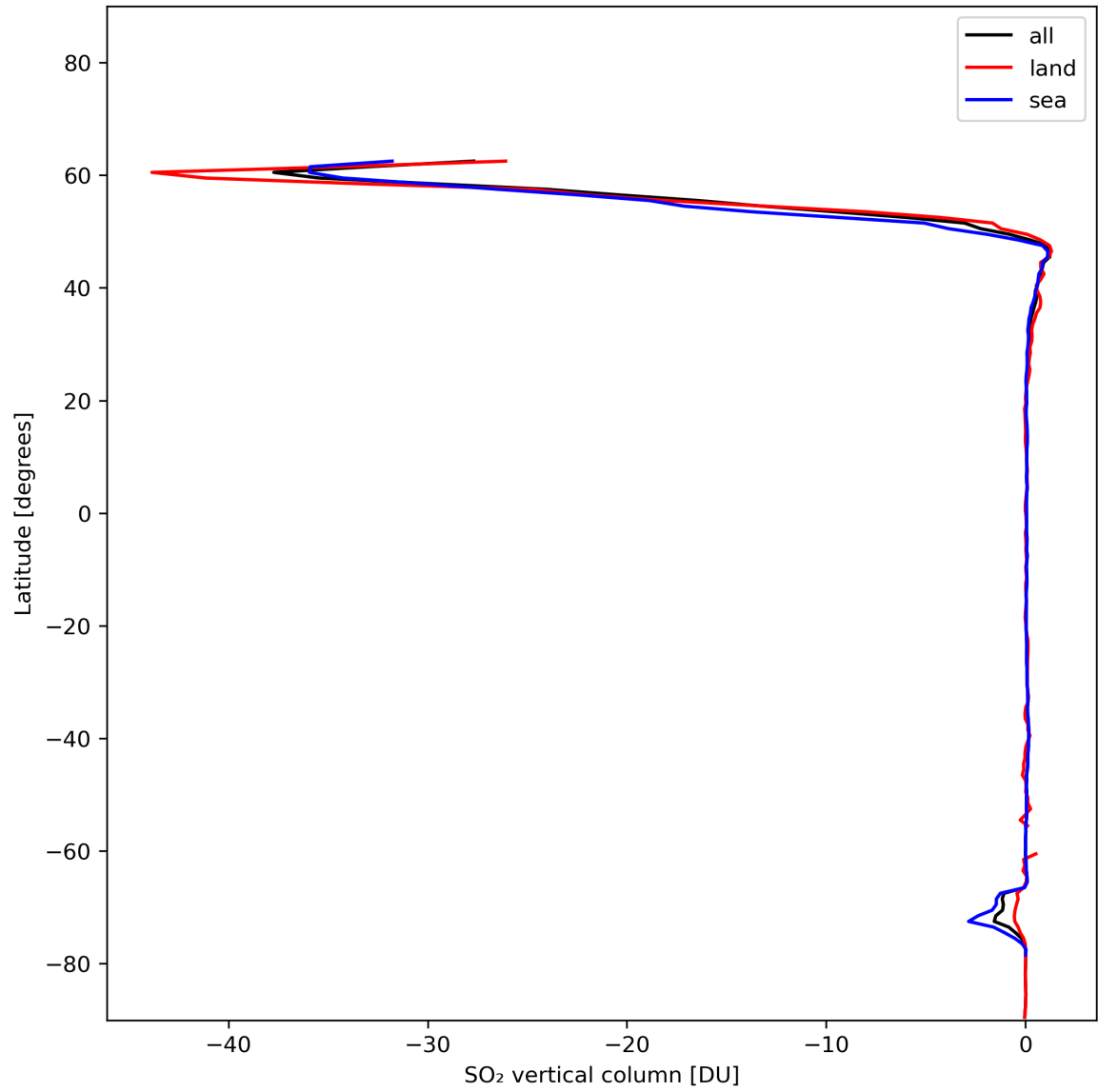
Figure 30: Zonal average of “SO 2 vertical column” for 2024-01-03 to 2024-01-05.
