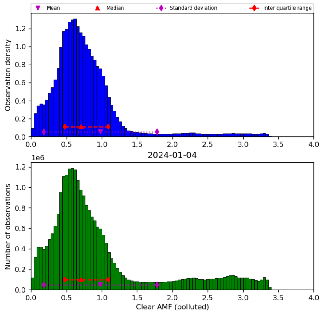
Figure 73: Histogram of “Clear AMF (polluted)” for 2024-01-03 to 2024-01-05
