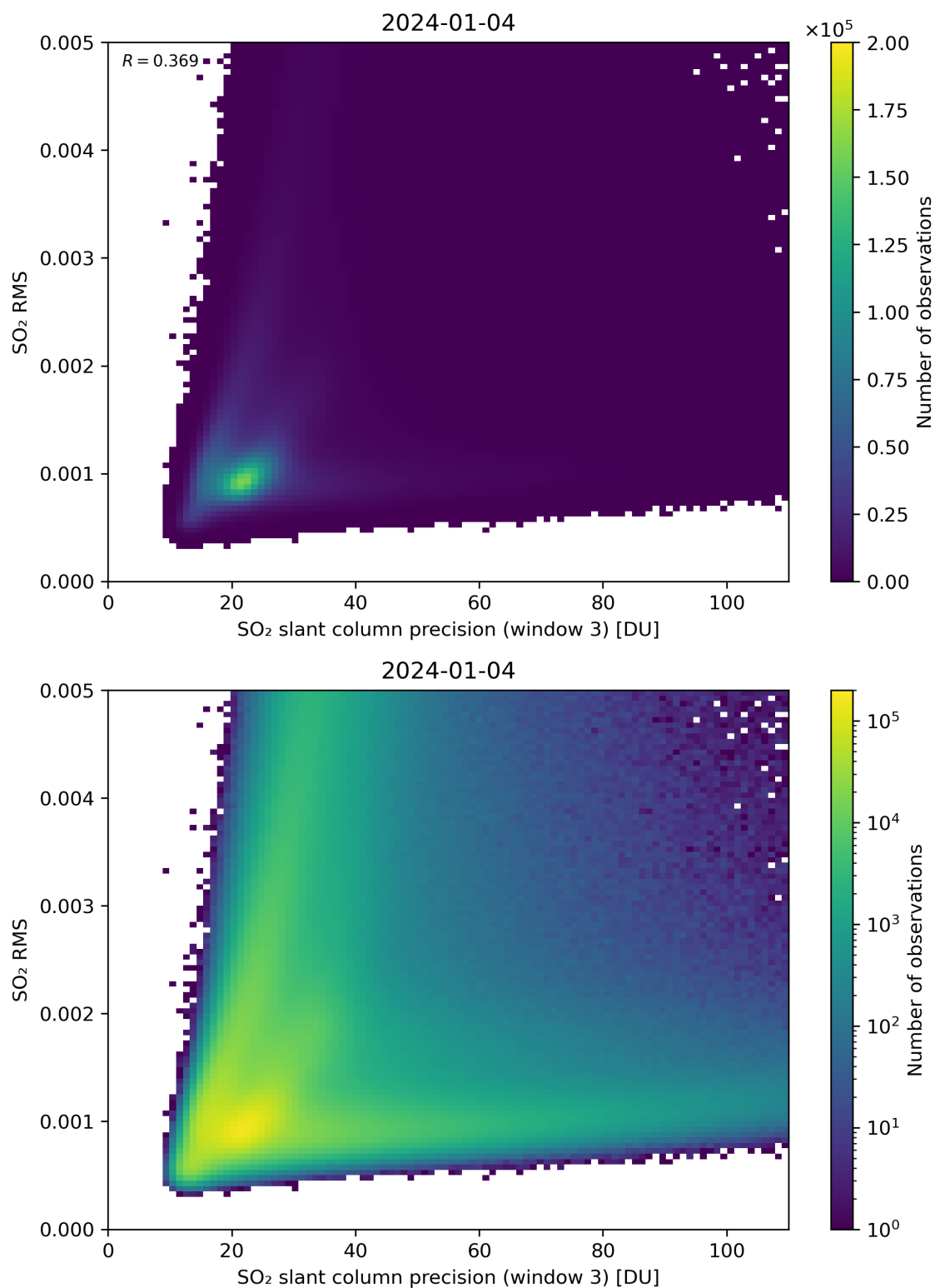
Figure 260: Scatter density plot of “SO 2 slant column precision (window 3)” against “SO 2 RMS” for 2024-01-03 to 2024-01-05.
