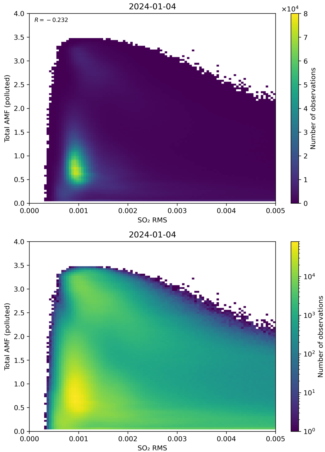
Figure 137: Scatter density plot of “SO 2 RMS” against “Total AMF (polluted)” for 2024-01-03 to 2024-01-05.
