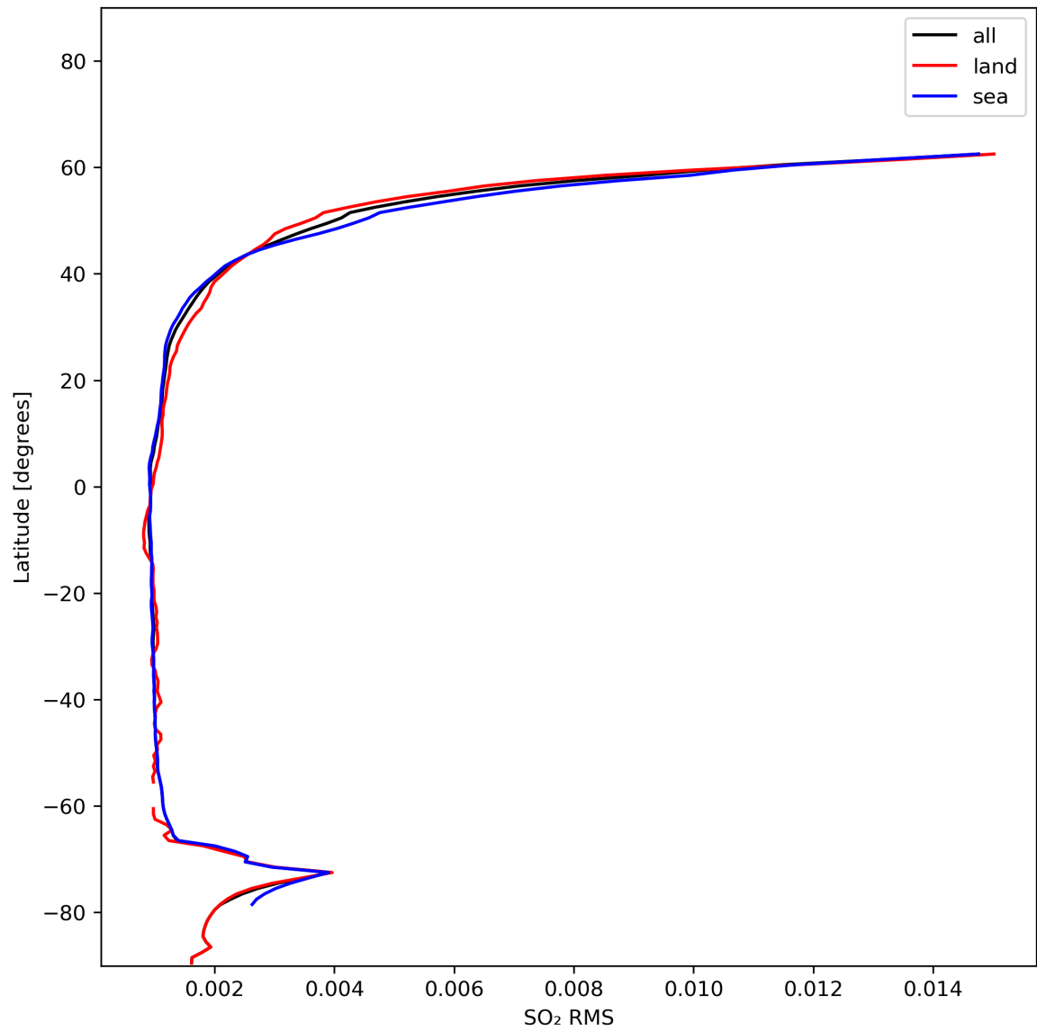
Figure 47: Zonal average of “SO 2 RMS” for 2024-01-03 to 2024-01-05.
