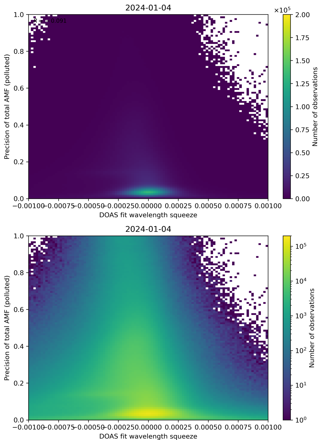
Figure 135: Scatter density plot of “DOAS fit wavelength squeeze” against “Precision of total AMF (polluted)” for 2024-01-03 to 2024-01-05.
