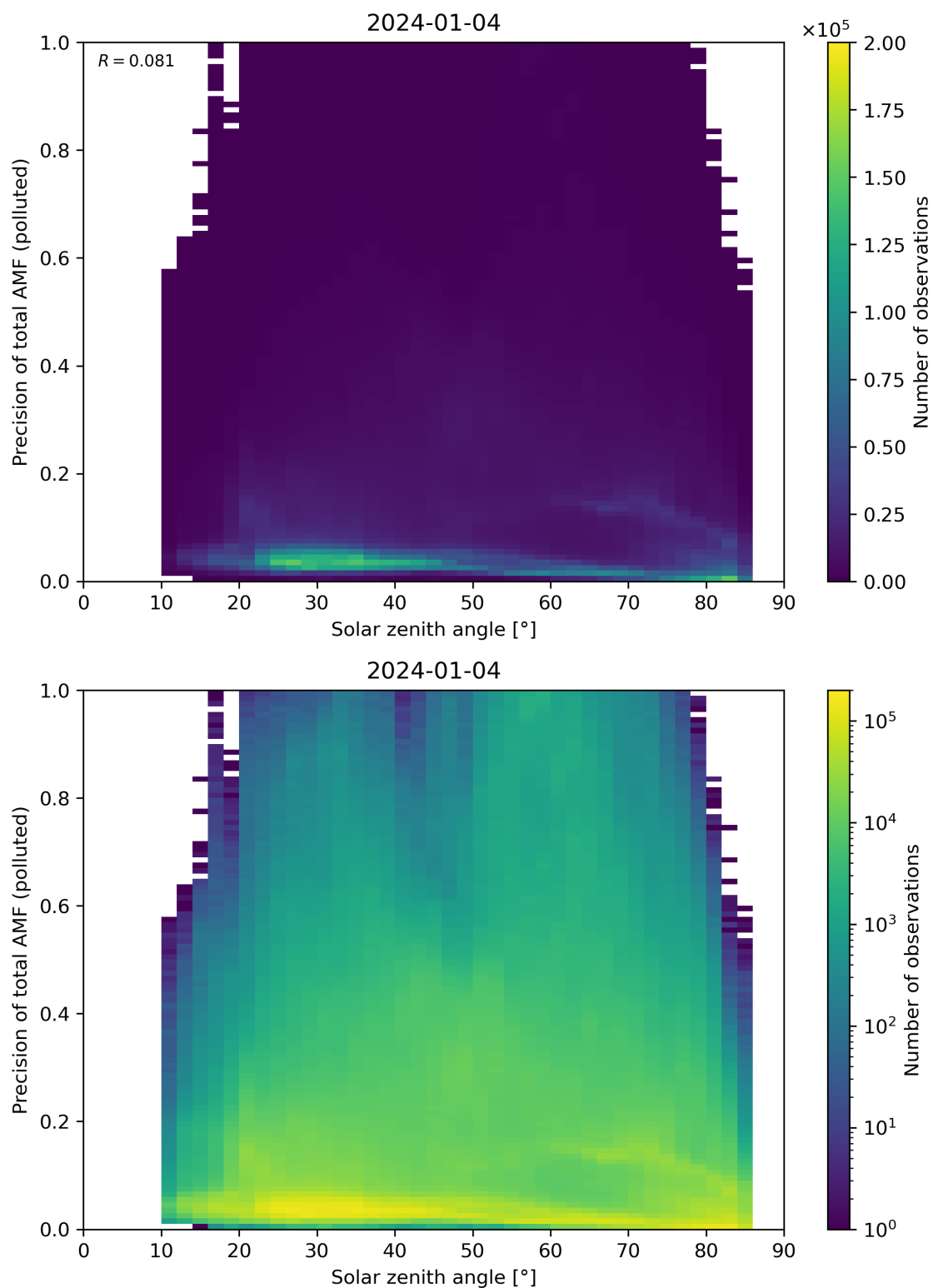
Figure 175: Scatter density plot of “Solar zenith angle” against “Precision of total AMF (polluted)” for 2024-01-03 to 2024-01-05.
