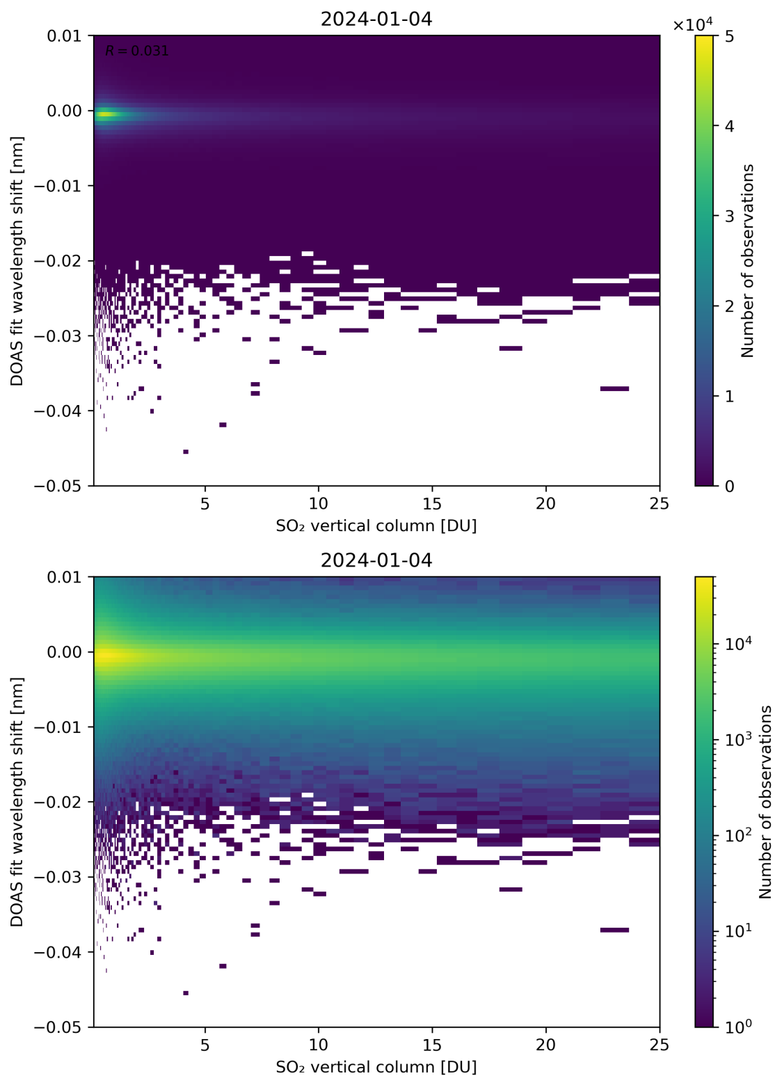
Figure 276: Scatter density plot of “SO 2 vertical column” against “DOAS fit wavelength shift” for 2024-01-03 to 2024-01-05.
