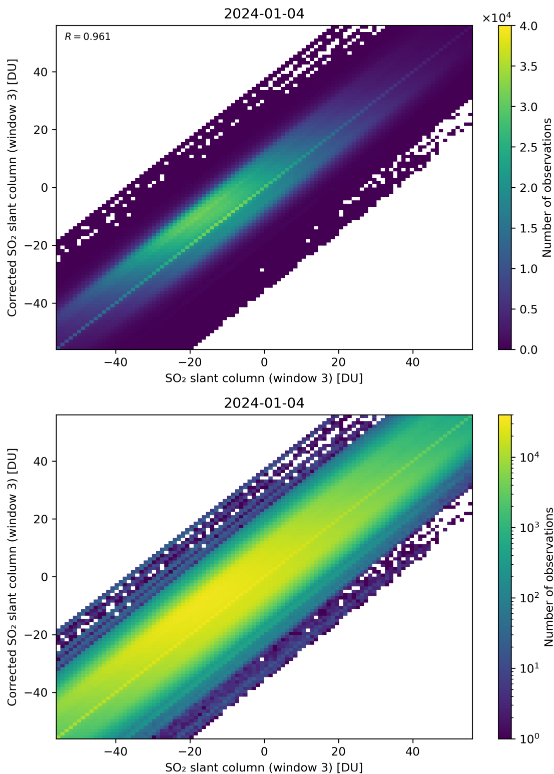
Figure 266: Scatter density plot of “SO 2 slant column (window 3)” against “Corrected SO 2 slant column (window 3)” for 2024-01-03 to 2024-01-05.
