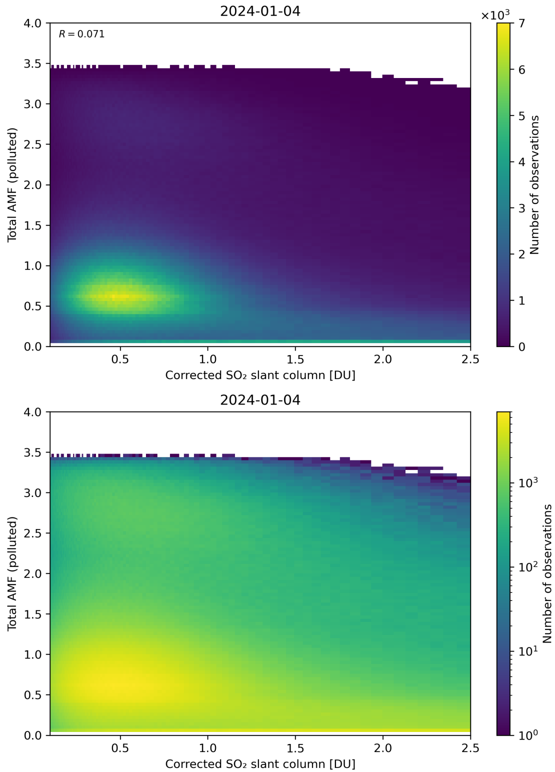
Figure 192: Scatter density plot of “Corrected SO 2 slant column” against “Total AMF (polluted)” for 2024-01-03 to 2024-01-05.
