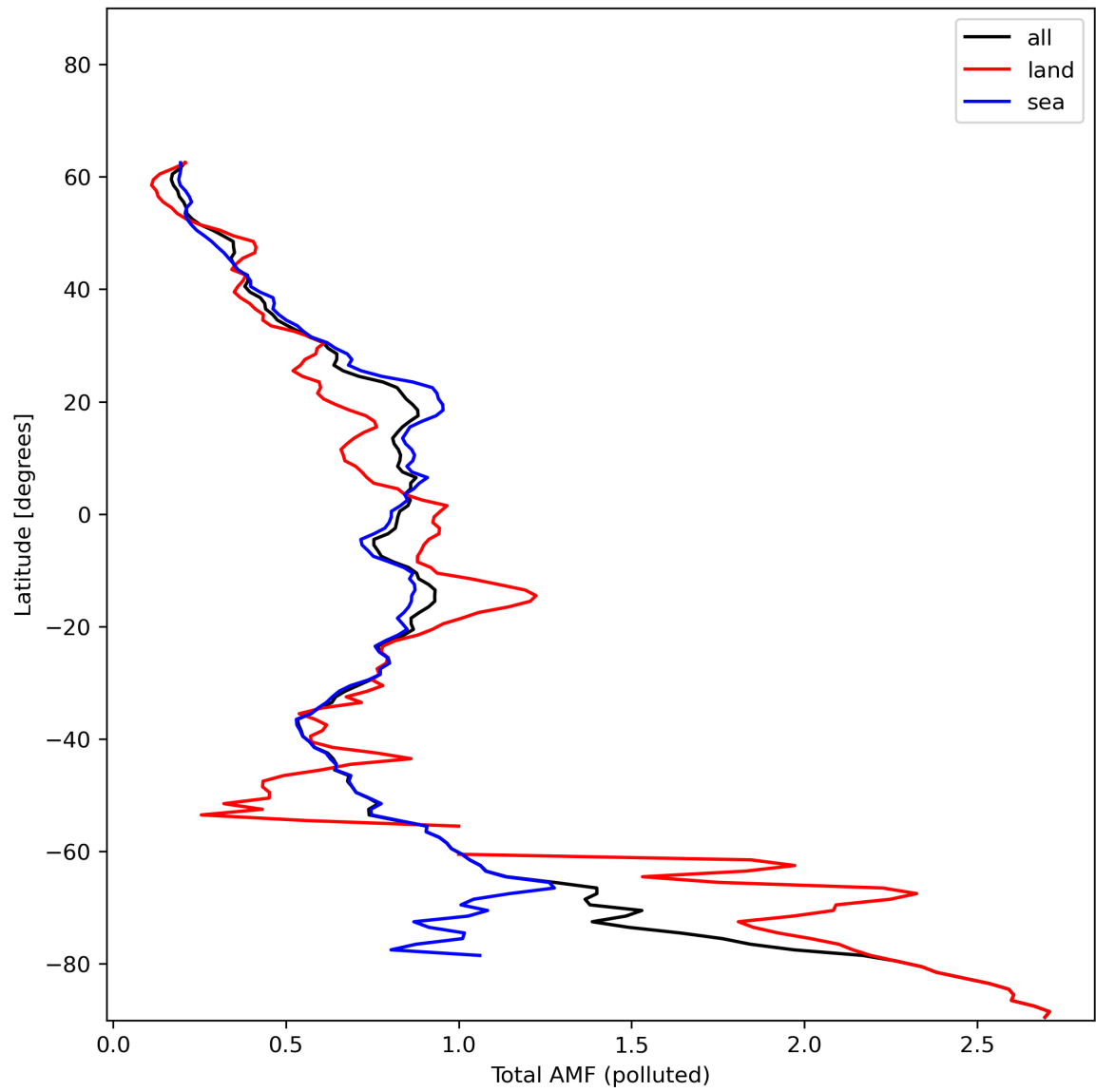
Figure 48: Zonal average of “Total AMF (polluted)” for 2024-01-03 to 2024-01-05.
