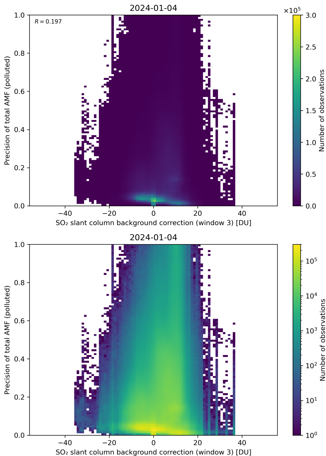
Figure 126: Scatter density plot of “SO 2 slant column background correction (window 3)” against “Precision of total AMF (polluted)” for 2024-01-03 to 2024-01-05.
