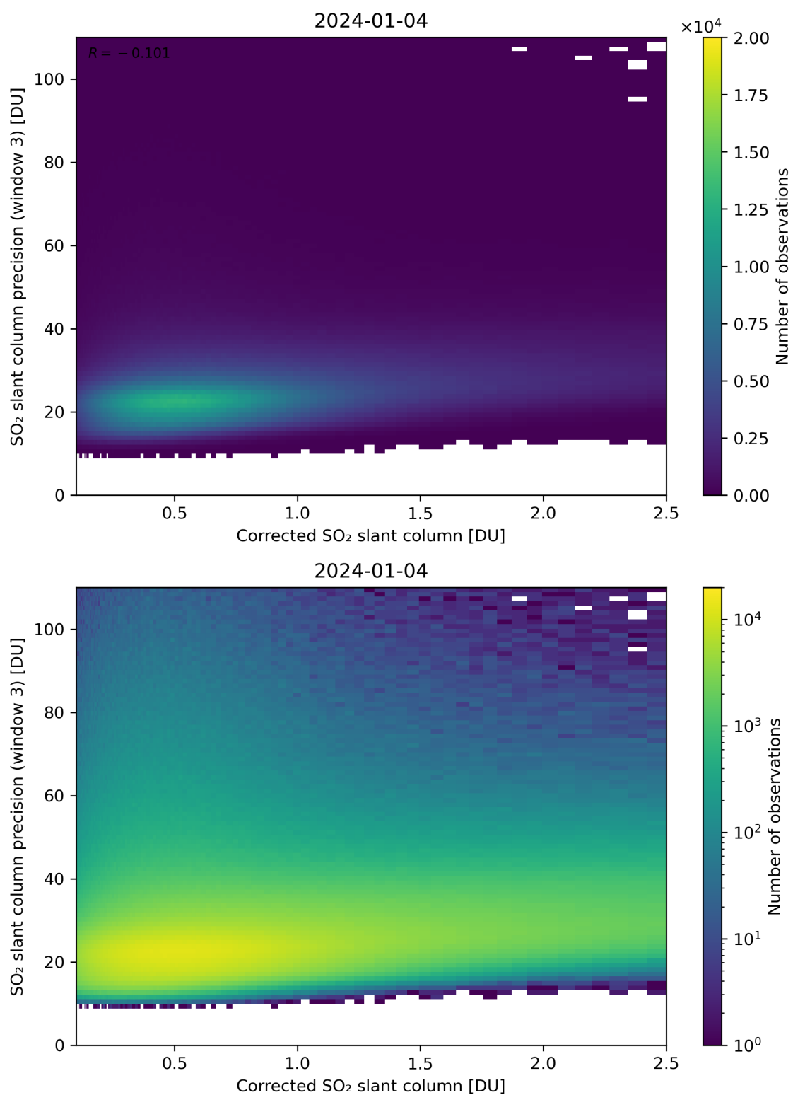
Figure 191: Scatter density plot of “Corrected SO 2 slant column” against “SO 2 slant column precision (window 3)” for 2024-01-03 to 2024-01-05.
