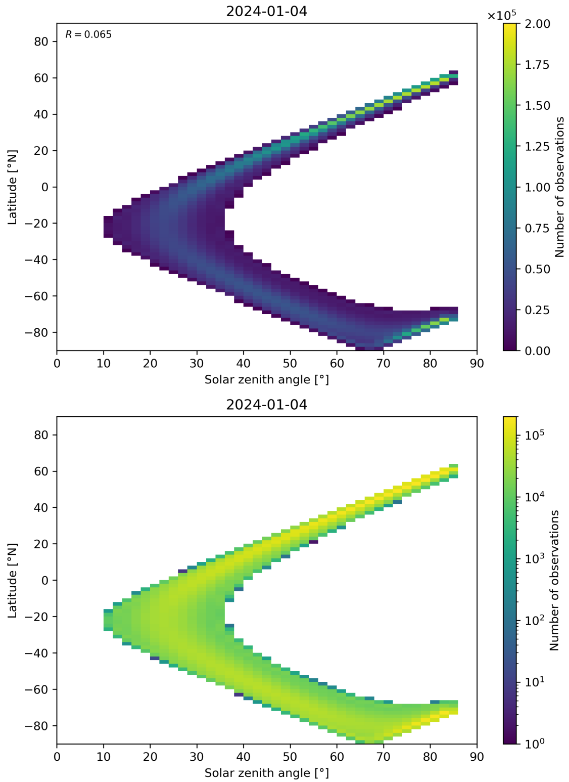
Figure 164: Scatter density plot of “Solar zenith angle” against “Latitude” for 2024-01-03 to 2024-01-05.
