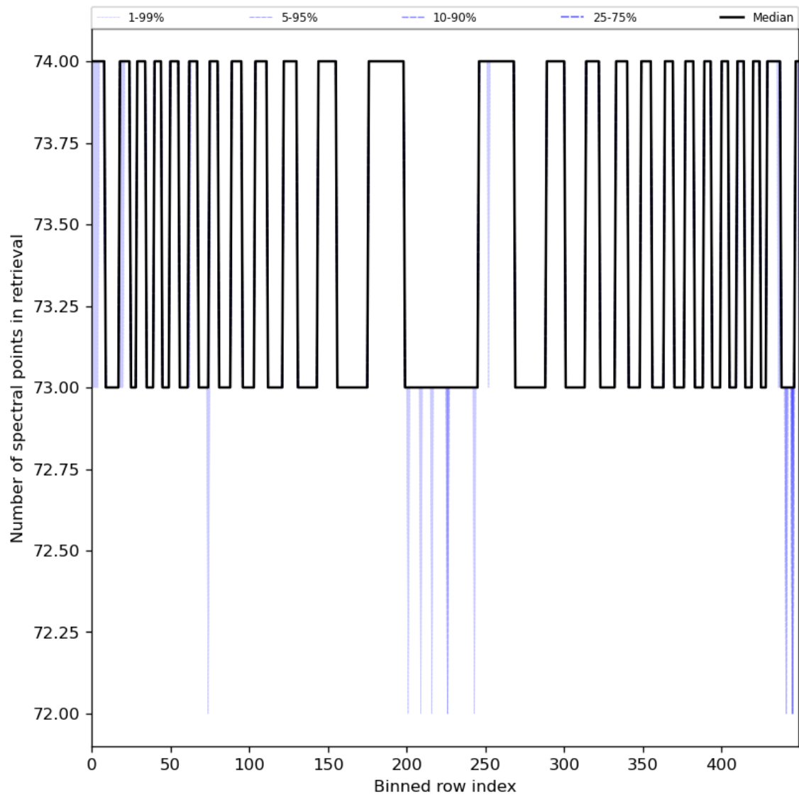
Figure 97: Along track statistics of “Number of spectral points in retrieval” for 2024-01-03 to 2024-01-05
