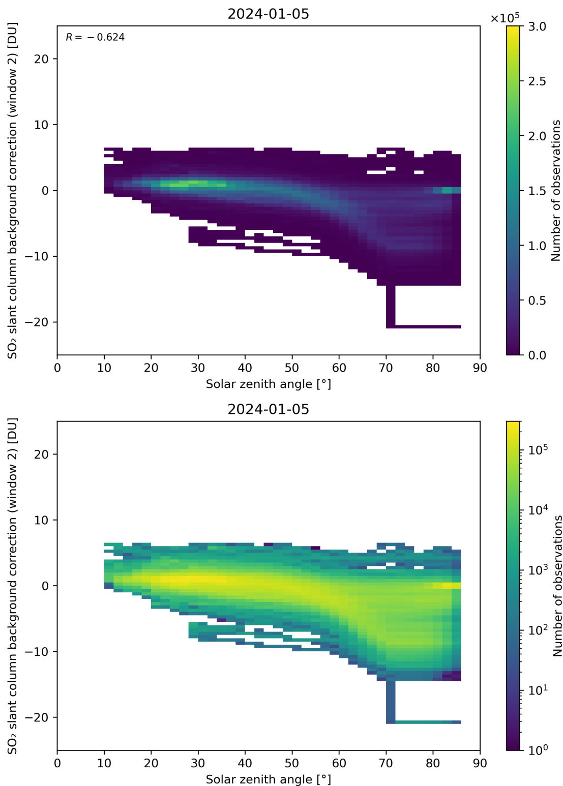
Figure 159: Scatter density plot of “Solar zenith angle” against “SO 2 slant column background correction (window 2)” for 2024-01-05 to 2024-01-06.
