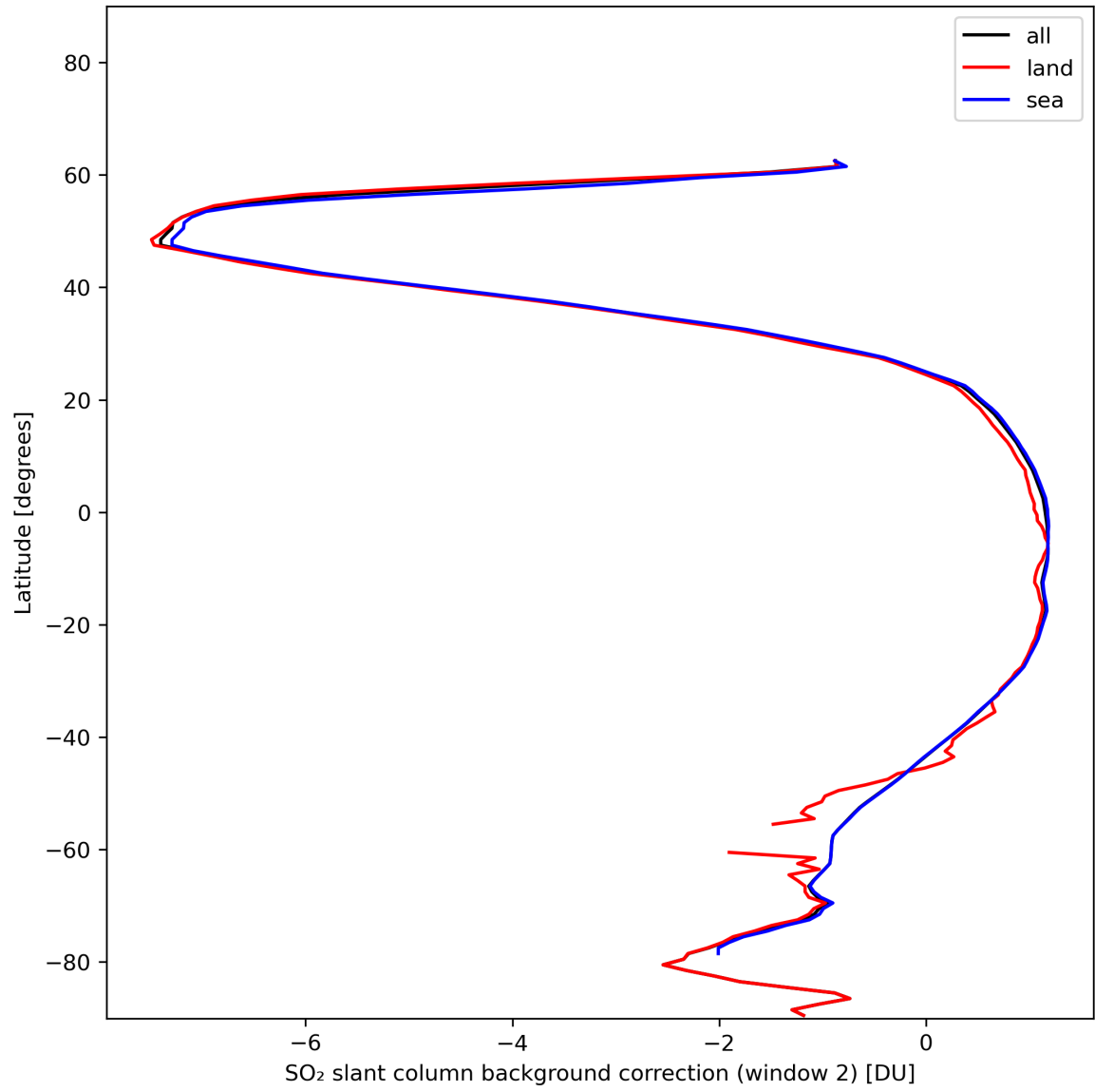
Figure 40: Zonal average of “SO 2 slant column background correction (window 2)” for 2024-01-05 to 2024-01-06.
