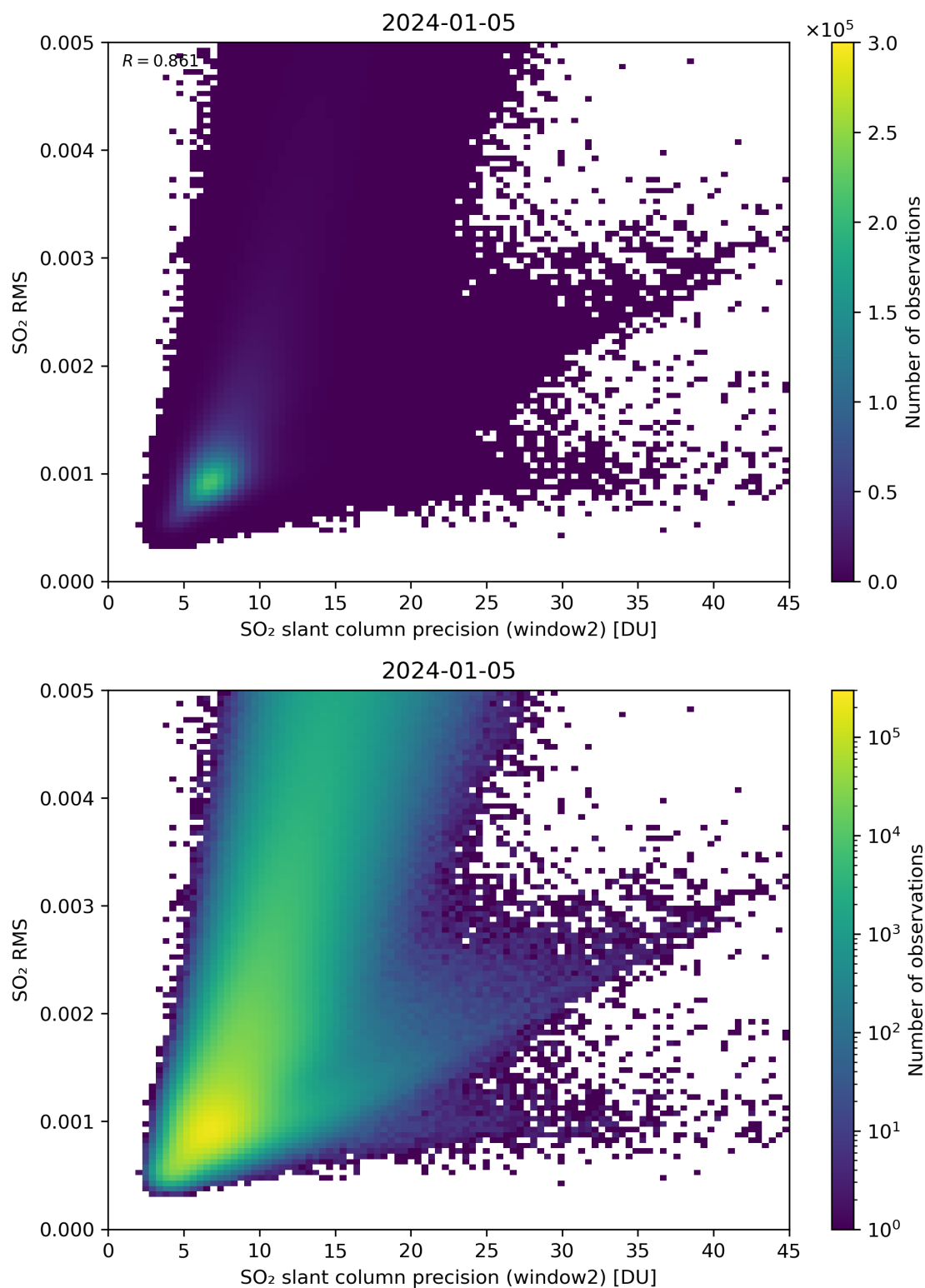
Figure 245: Scatter density plot of “SO 2 slant column precision (window2)” against “SO 2 RMS” for 2024-01-05 to 2024-01-06.
