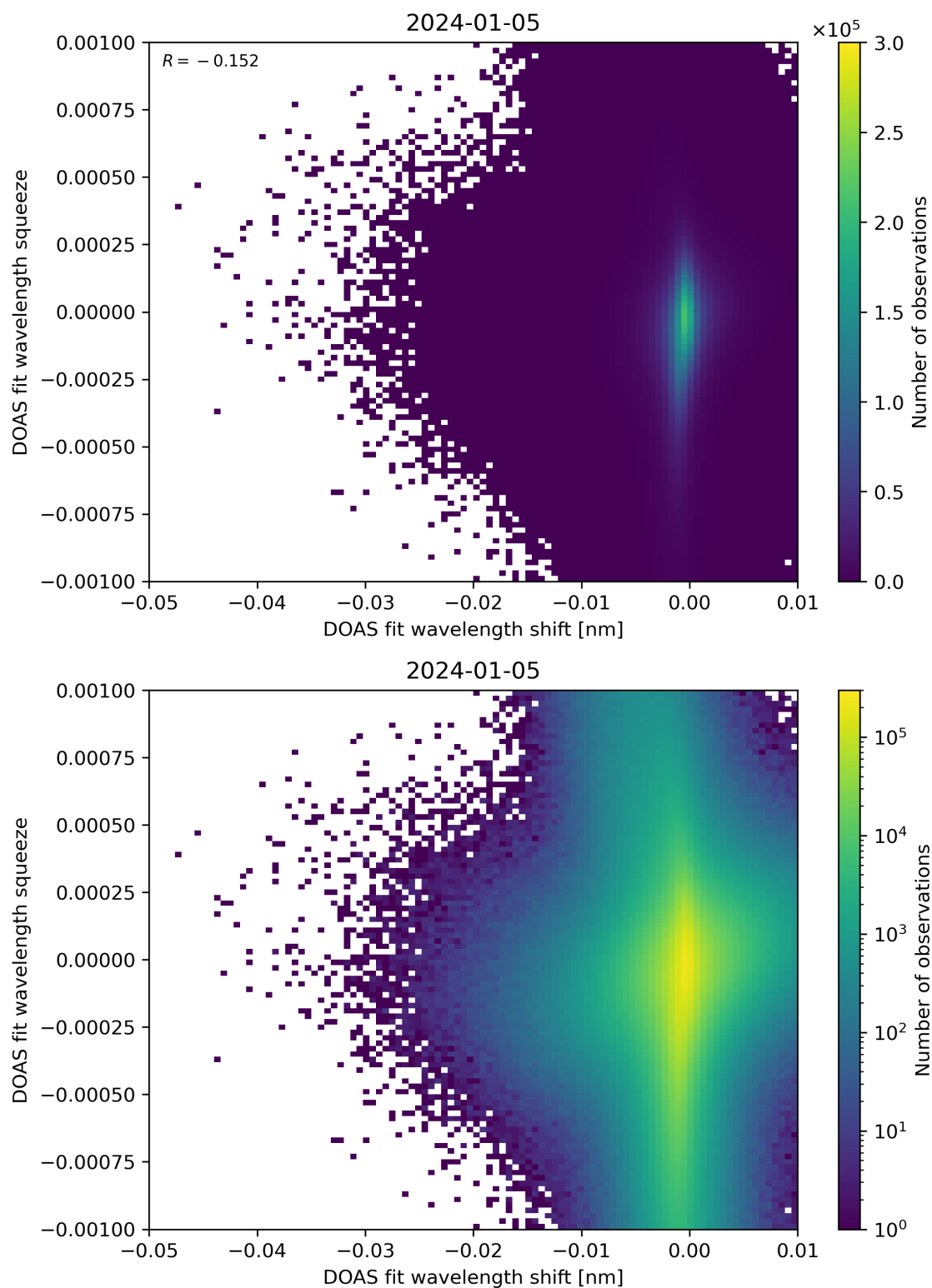
Figure 127: Scatter density plot of “DOAS fit wavelength shift” against “DOAS fit wavelength squeeze” for 2024-01-05 to 2024-01-06.
