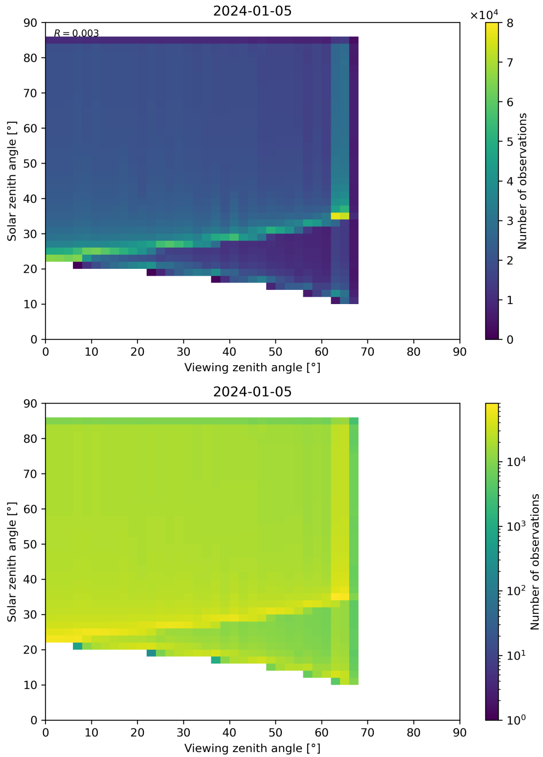
Figure 315: Scatter density plot of “Viewing zenith angle” against “Solar zenith angle” for 2024-01-05 to 2024-01-06.
