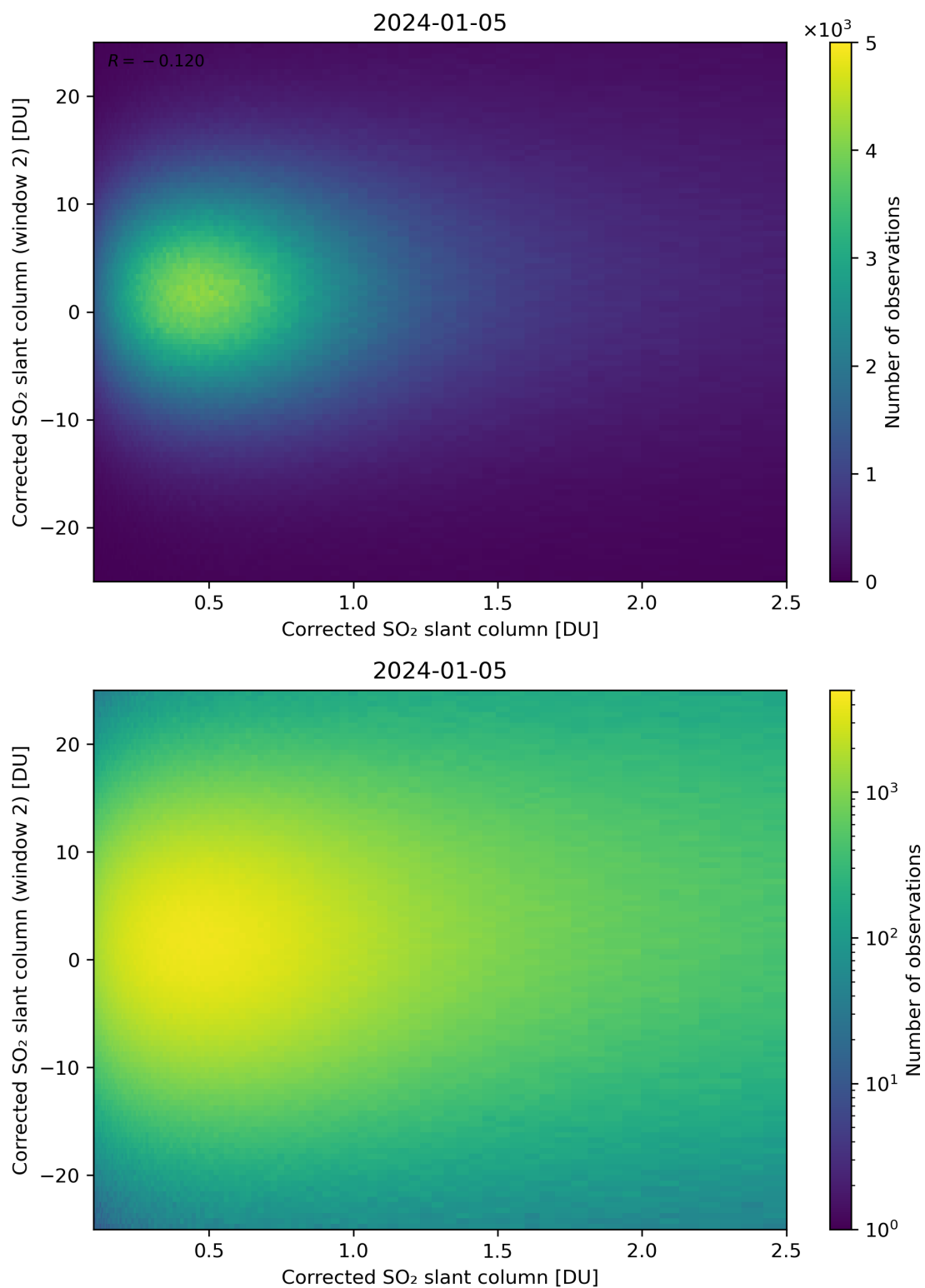
Figure 185: Scatter density plot of “Corrected SO 2 slant column” against “Corrected SO 2 slant column (window 2)” for 2024-01-05 to 2024-01-06.
