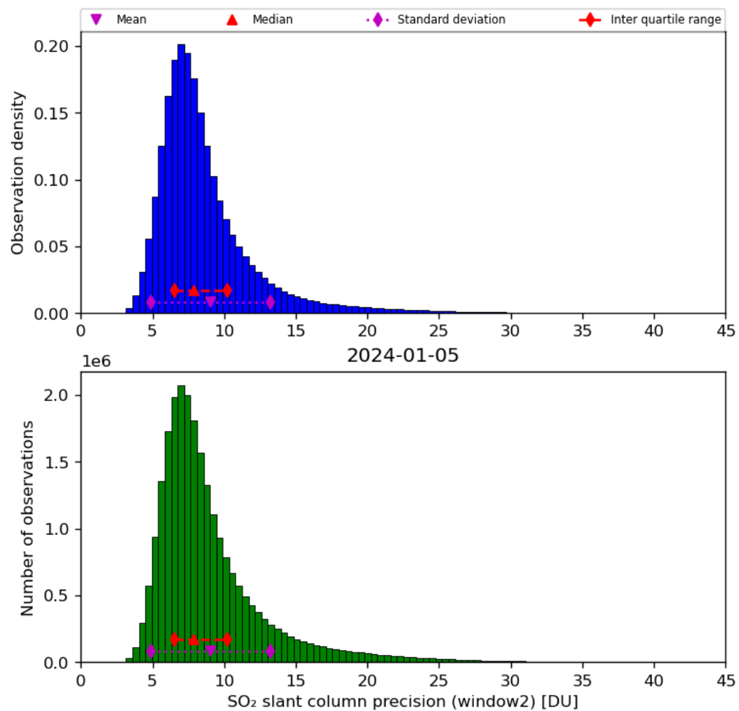
Figure 61: Histogram of “SO 2 slant column precision (window2)” for 2024-01-05 to 2024-01-06
