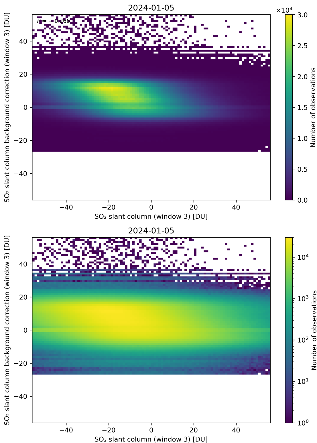
Figure 253: Scatter density plot of “SO 2 slant column (window 3)” against “SO 2 slant column background correction (window 3)” for 2024-01-05 to 2024-01-06.
