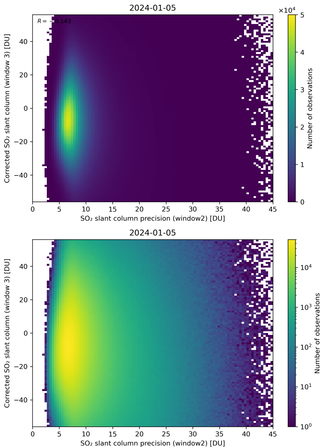
Figure 248: Scatter density plot of “SO 2 slant column precision (window2)” against “Corrected SO 2 slant column (window 3)” for 2024-01-05 to 2024-01-06.
