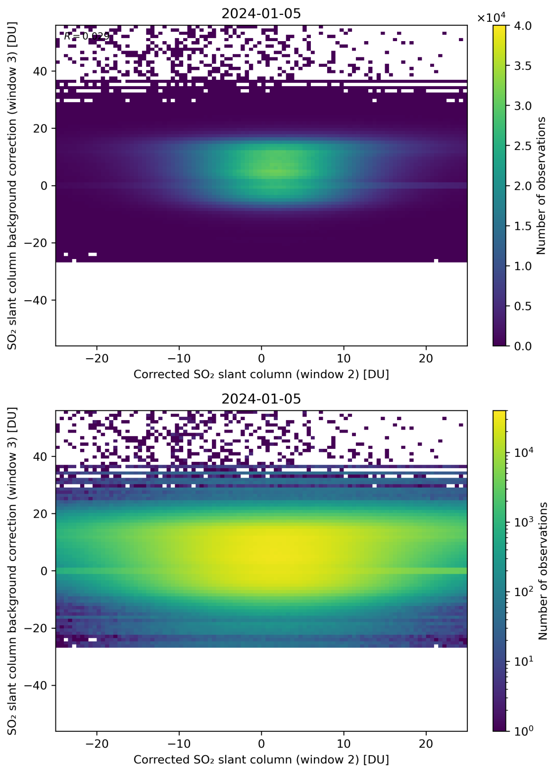
Figure 195: Scatter density plot of “Corrected SO 2 slant column (window 2)” against “SO 2 slant column background correction (window 3)” for 2024-01-05 to 2024-01-06.
