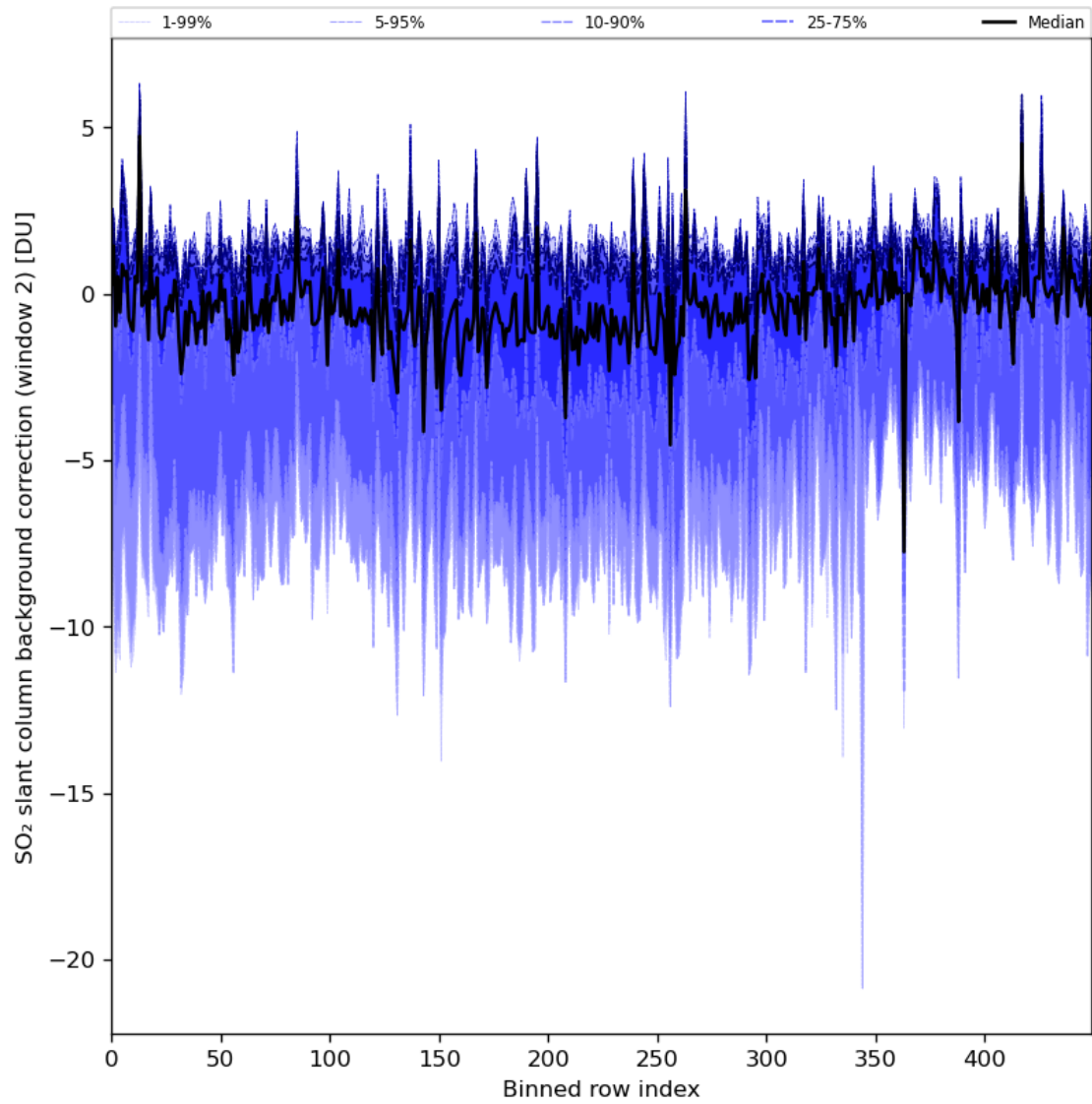
Figure 86: Along track statistics of “SO 2 slant column background correction (window 2)” for 2024-01-05 to 2024-01-06
