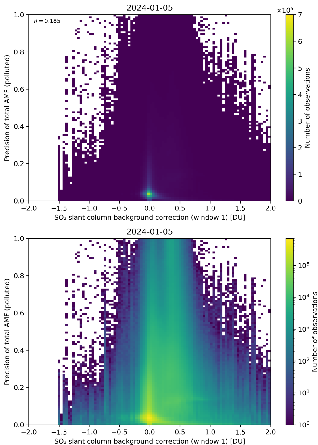
Figure 110: Scatter density plot of “SO 2 slant column background correction (window 1)” against “Precision of total AMF (polluted)” for 2024-01-05 to 2024-01-06.
