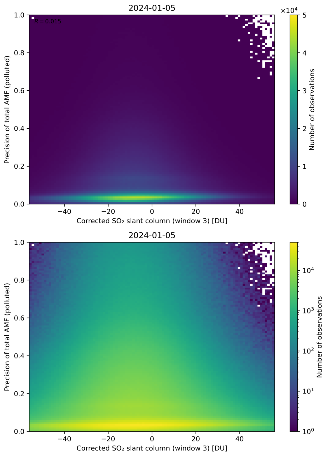
Figure 211: Scatter density plot of “Corrected SO 2 slant column (window 3)” against “Precision of total AMF (polluted)” for 2024-01-05 to 2024-01-06.
