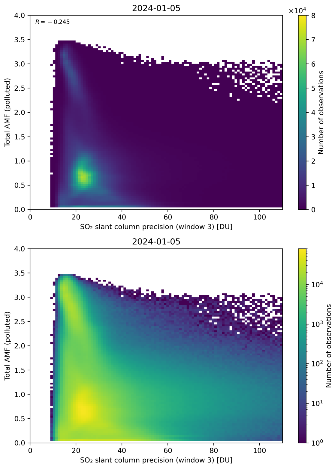
Figure 263: Scatter density plot of “SO 2 slant column precision (window 3)” against “Total AMF (polluted)” for 2024-01-05 to 2024-01-06.
