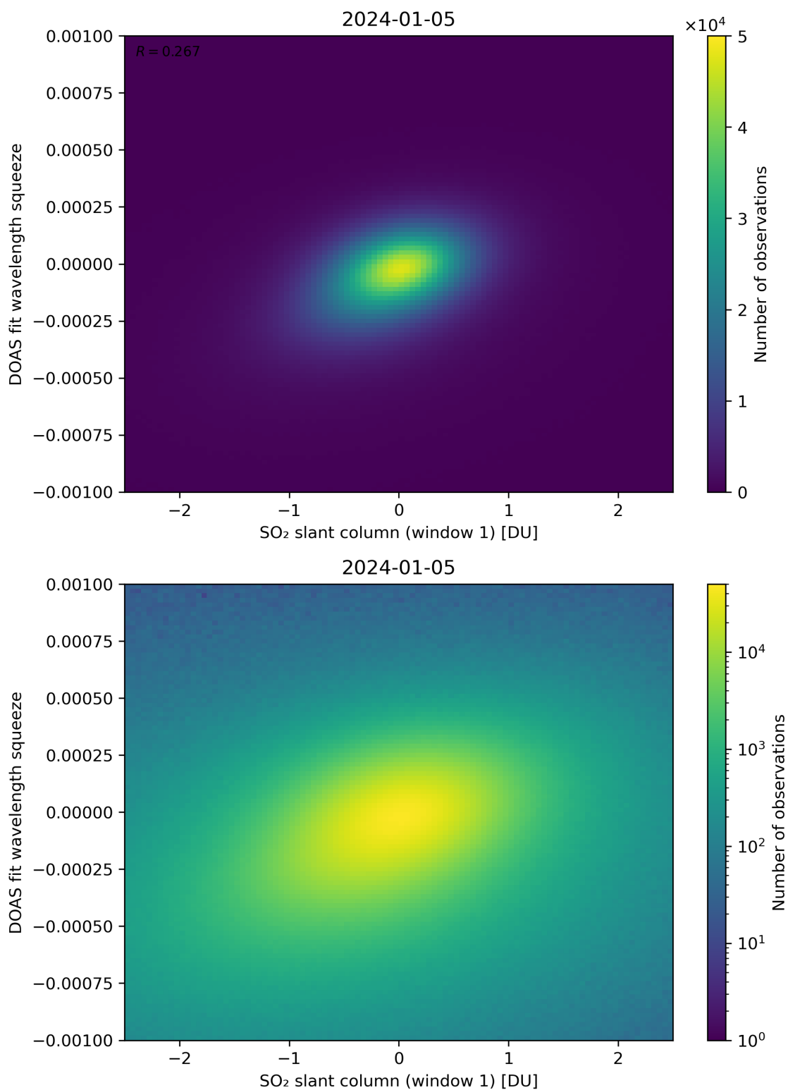
Figure 216: Scatter density plot of “SO 2 slant column (window 1)” against “DOAS fit wavelength squeeze” for 2024-01-05 to 2024-01-06.
