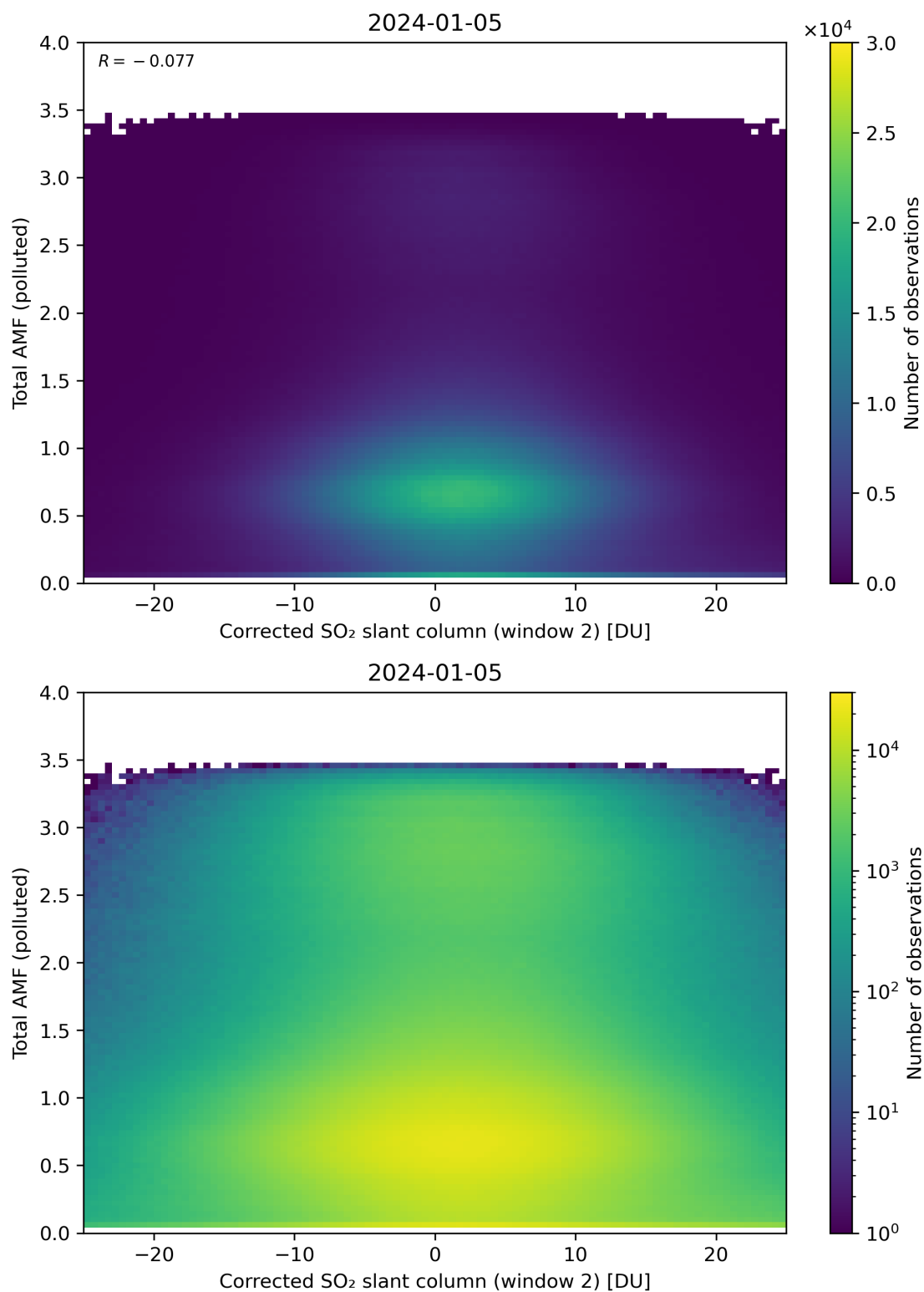
Figure 203: Scatter density plot of “Corrected SO 2 slant column (window 2)” against “Total AMF (polluted)” for 2024-01-05 to 2024-01-06.
