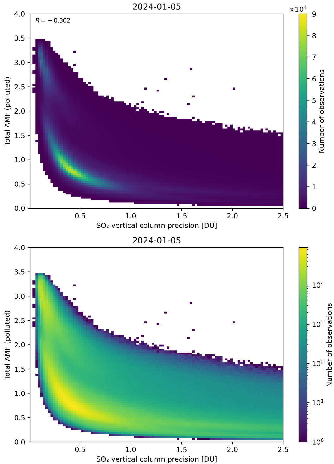
Figure 294: Scatter density plot of “SO 2 vertical column precision” against “Total AMF (polluted)” for 2024-01-05 to 2024-01-06.
