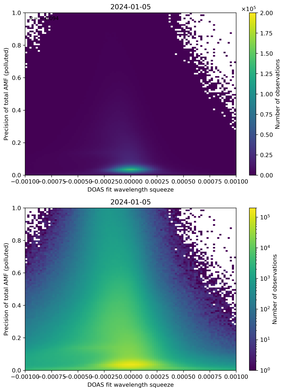
Figure 135: Scatter density plot of “DOAS fit wavelength squeeze” against “Precision of total AMF (polluted)” for 2024-01-05 to 2024-01-06.
