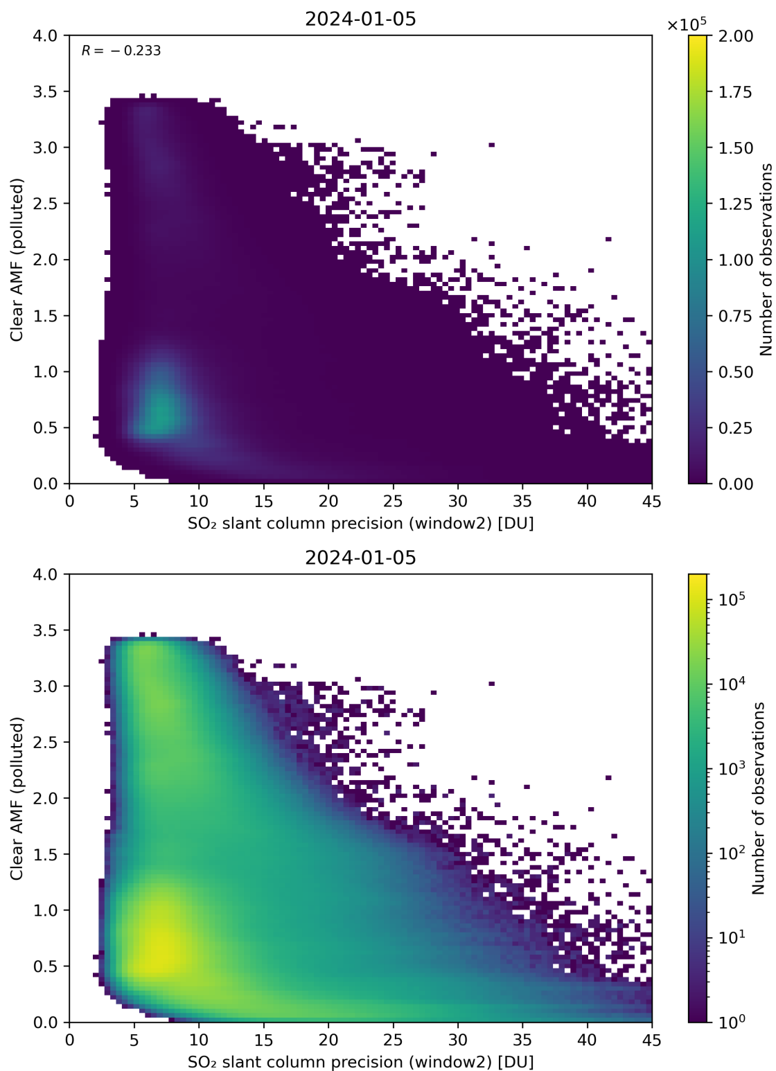
Figure 246: Scatter density plot of “SO 2 slant column precision (window2)” against “Clear AMF (polluted)” for 2024-01-05 to 2024-01-06.
