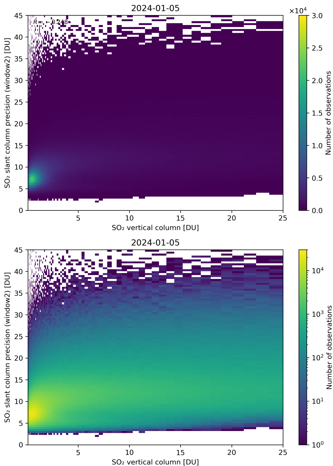
Figure 302: Scatter density plot of “SO 2 vertical column” against “SO 2 slant column precision (window2)” for 2024-01-05 to 2024-01-06.
