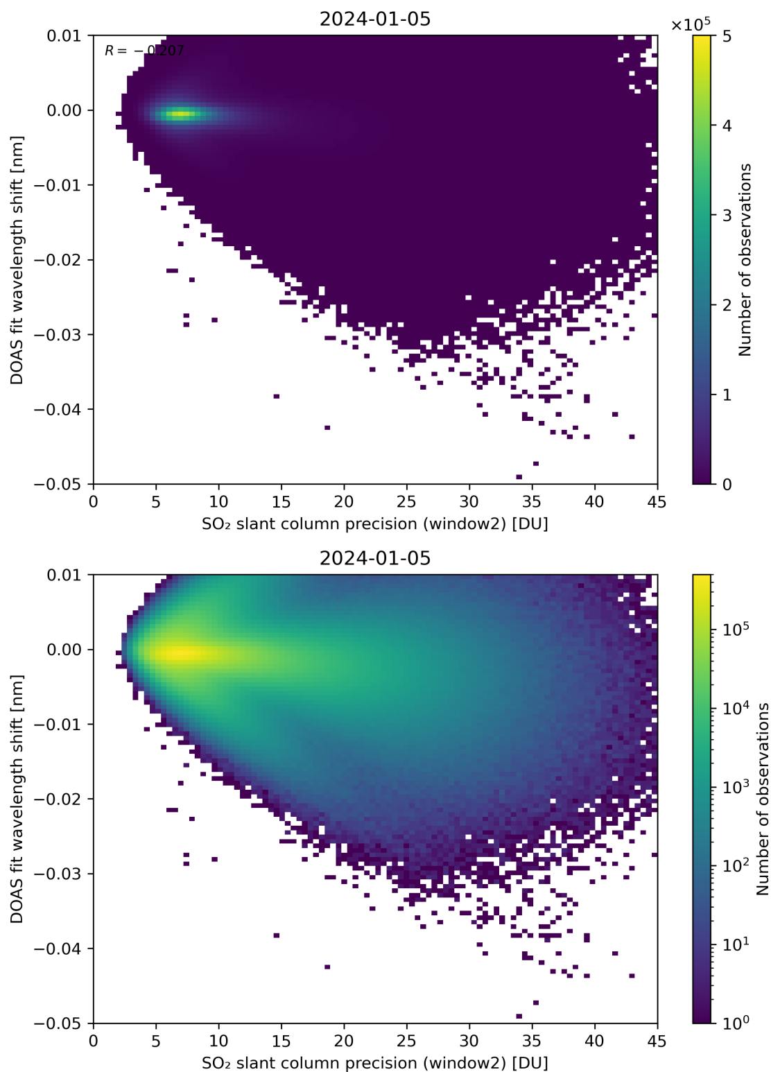
Figure 243: Scatter density plot of “SO 2 slant column precision (window2)” against “DOAS fit wavelength shift” for 2024-01-05 to 2024-01-06.
