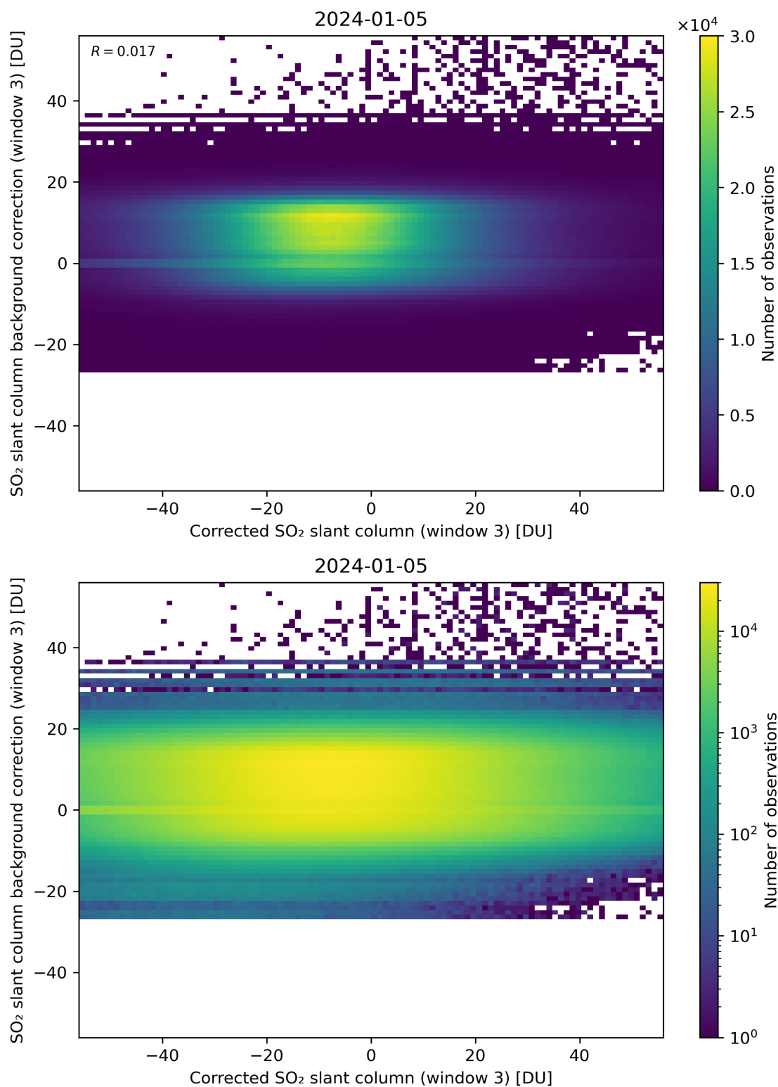
Figure 205: Scatter density plot of “Corrected SO 2 slant column (window 3)” against “SO 2 slant column background correction (window 3)” for 2024-01-05 to 2024-01-06.
