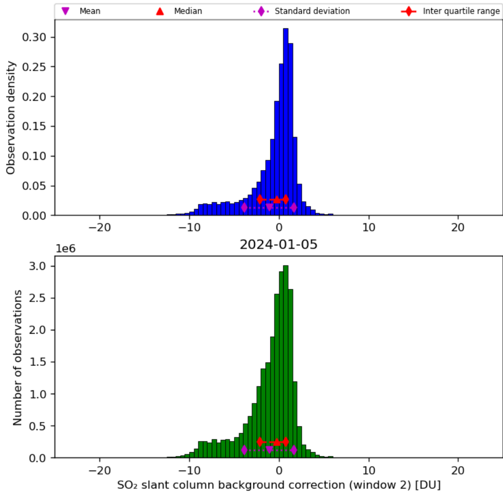
Figure 63: Histogram of “SO 2 slant column background correction (window 2)” for 2024-01-05 to 2024-01-06
