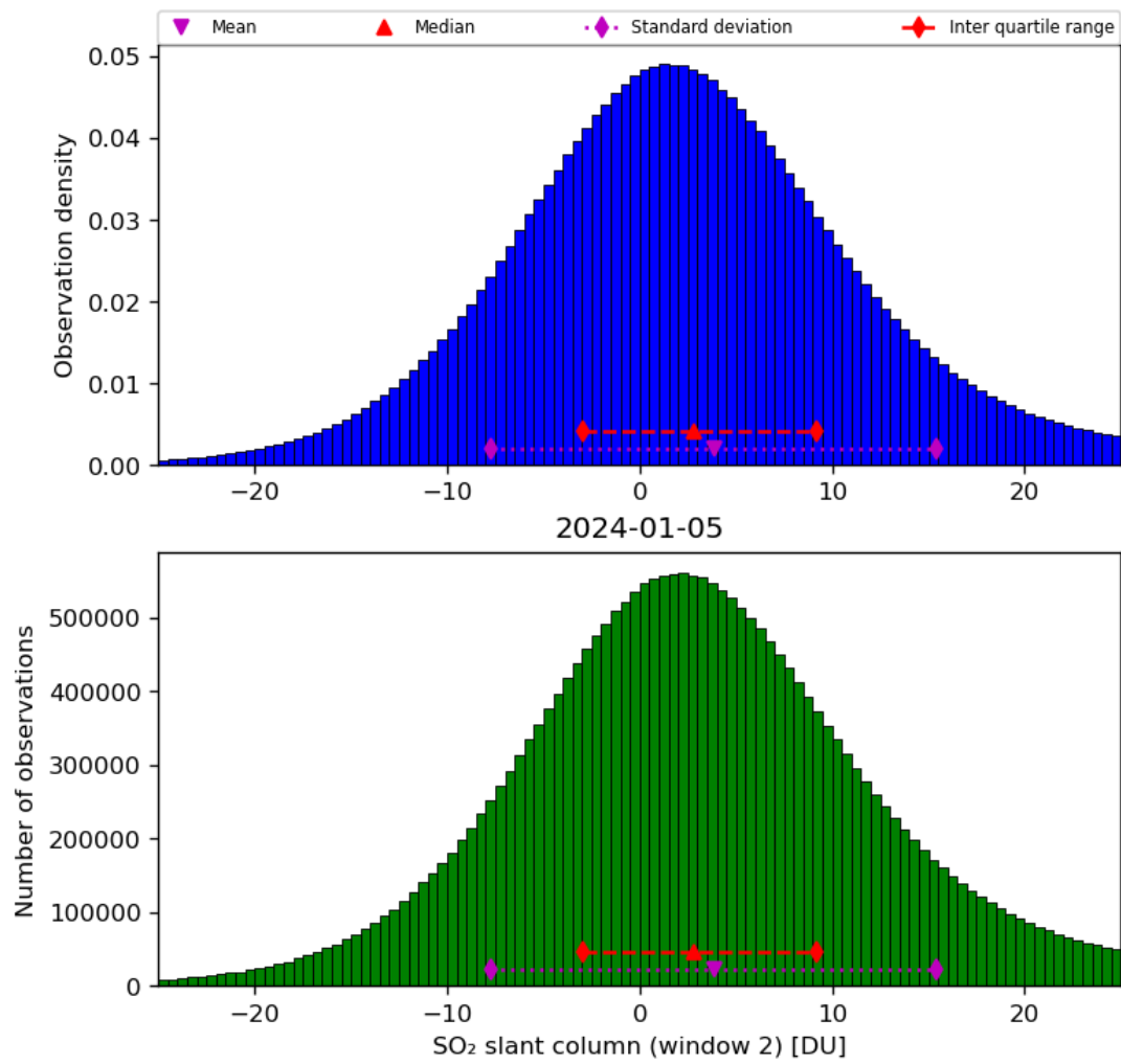
Figure 60: Histogram of “SO 2 slant column (window 2)” for 2024-01-05 to 2024-01-06
