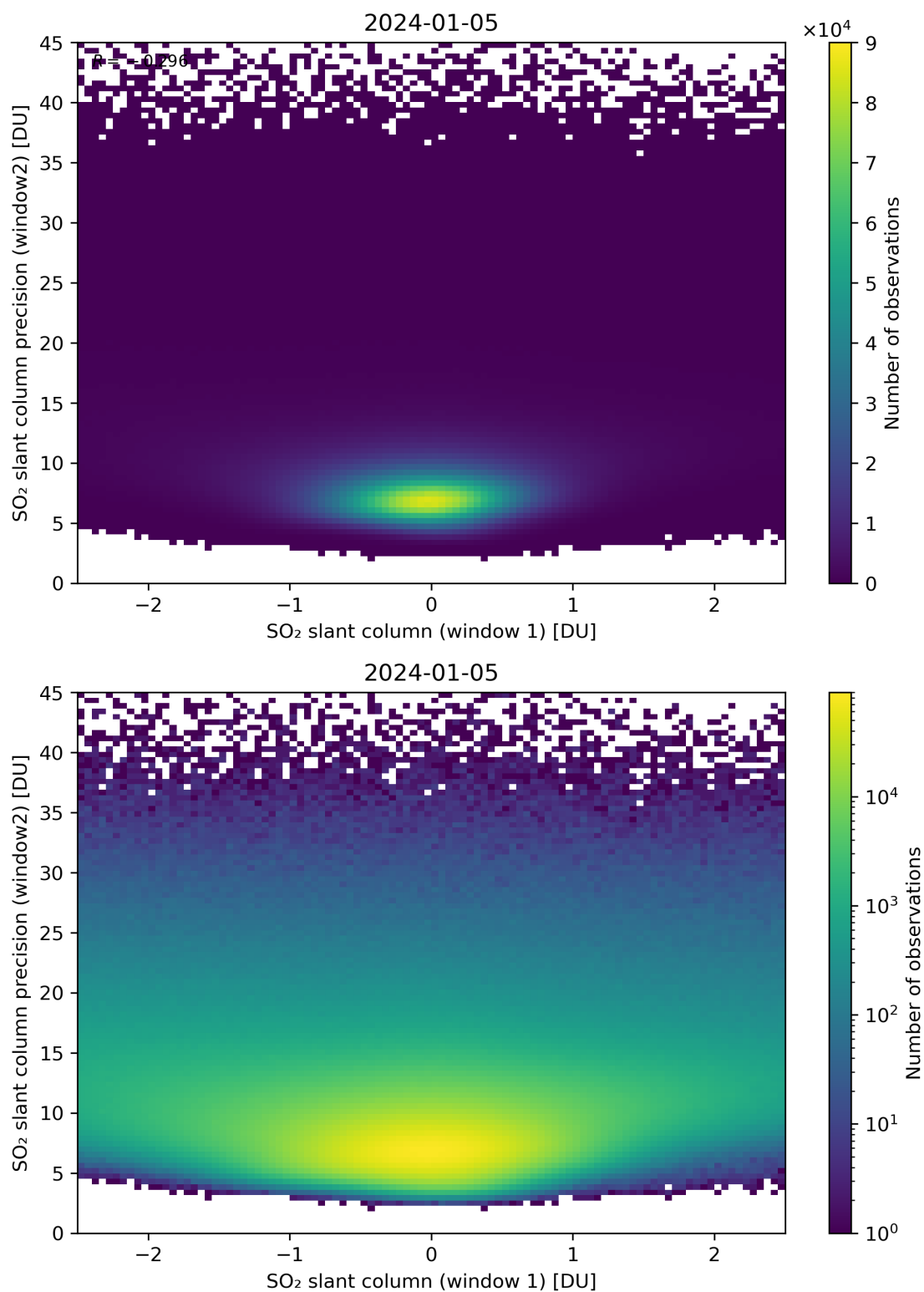
Figure 236: Scatter density plot of “SO 2 slant column (window 1)” against “SO 2 slant column precision (window2)” for 2024-01-05 to 2024-01-06.
