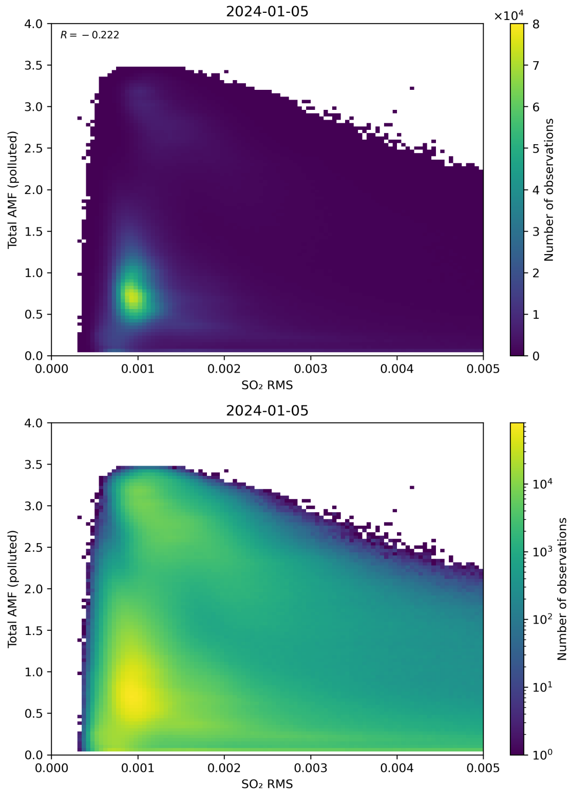
Figure 137: Scatter density plot of “SO 2 RMS” against “Total AMF (polluted)” for 2024-01-05 to 2024-01-06.
