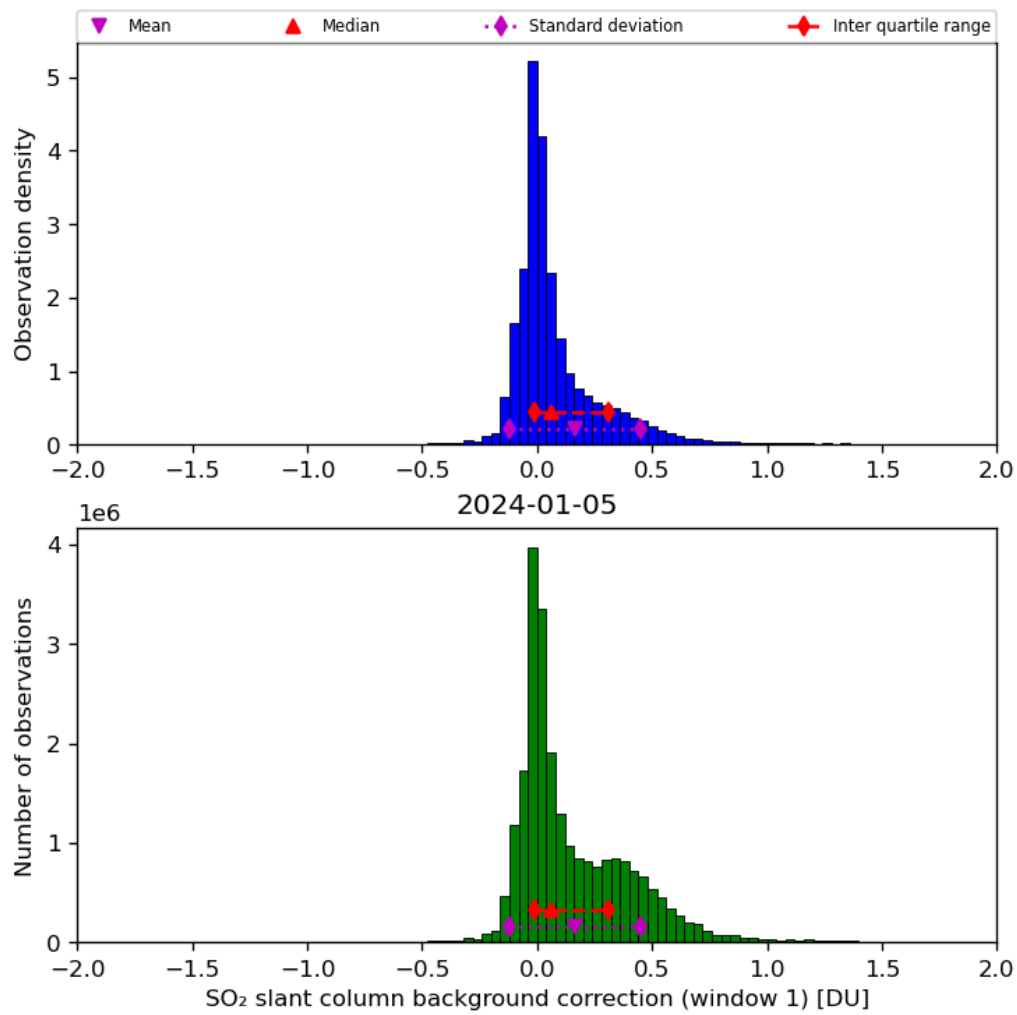
Figure 59: Histogram of “SO 2 slant column background correction (window 1)” for 2024-01-05 to 2024-01-06
