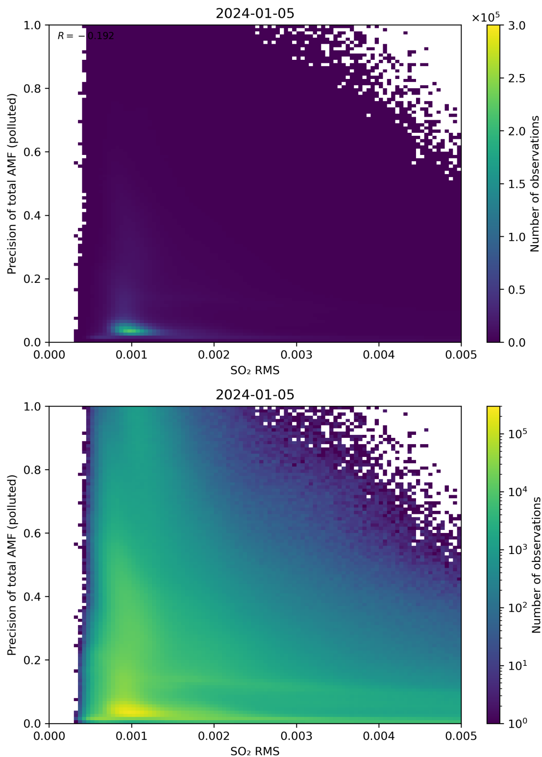
Figure 138: Scatter density plot of “SO 2 RMS” against “Precision of total AMF (polluted)” for 2024-01-05 to 2024-01-06.
