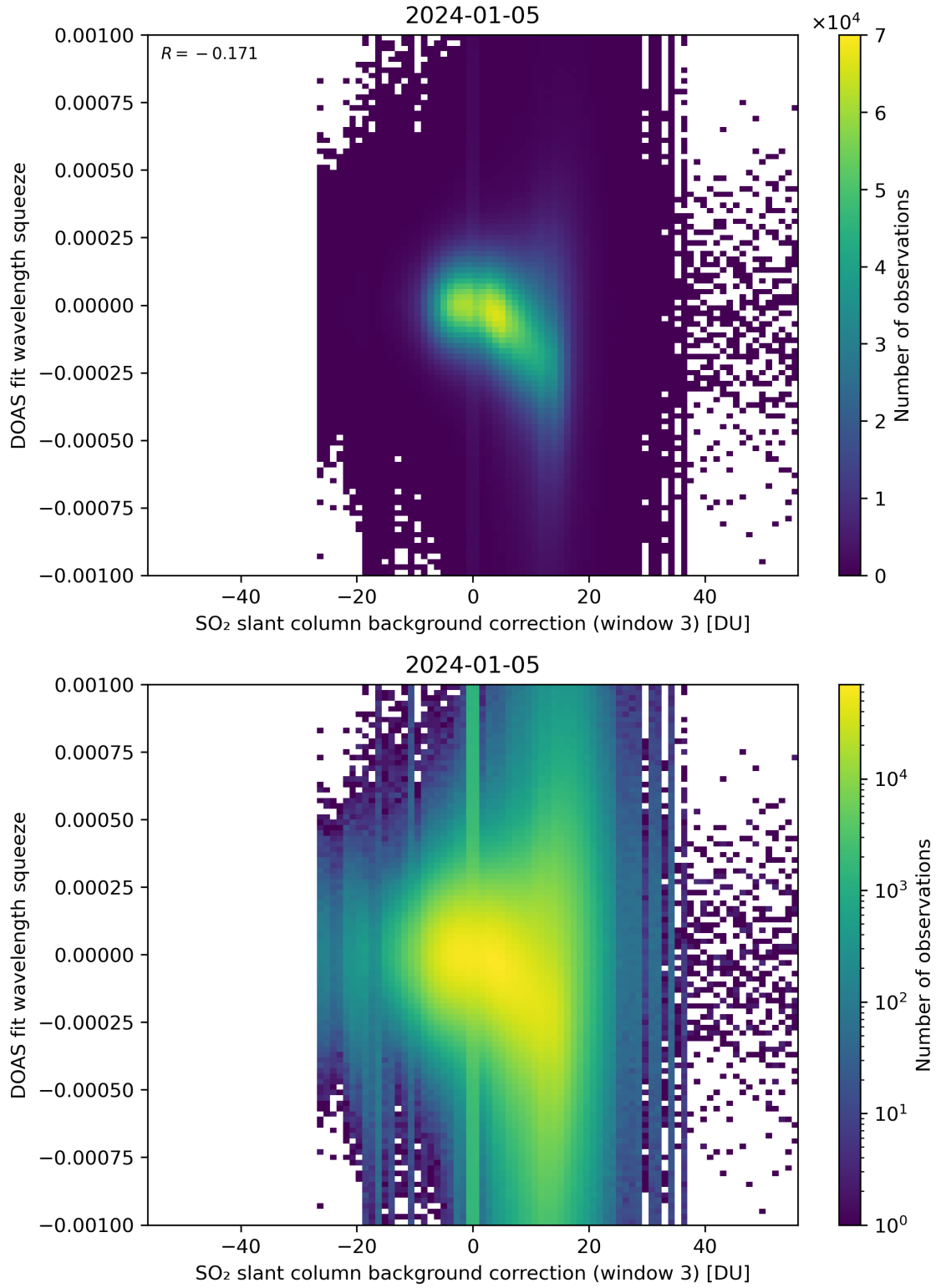
Figure 122: Scatter density plot of “SO 2 slant column background correction (window 3)” against “DOAS fit wavelength squeeze” for 2024-01-05 to 2024-01-06.
