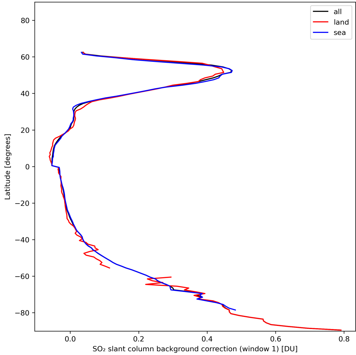
Figure 36: Zonal average of "SO 2 slant column background correction (window 1)" for 2024-01-05 to 2024-01-06.
