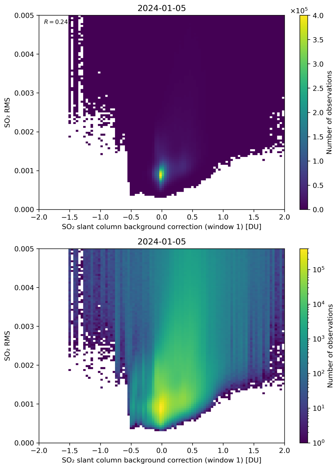
Figure 102: Scatter density plot of “SO 2 slant column background correction (window 1)” against “SO 2 RMS” for 2024-01-05 to 2024-01-06.
