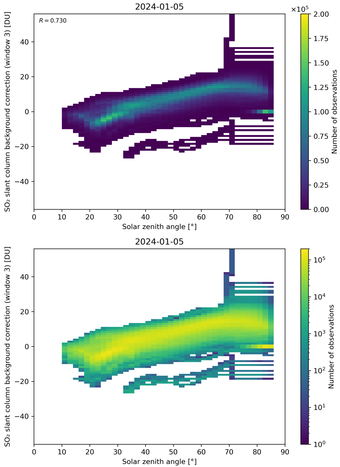
Figure 160: Scatter density plot of “Solar zenith angle” against “SO 2 slant column background correction (window 3)” for 2024-01-05 to 2024-01-06.
