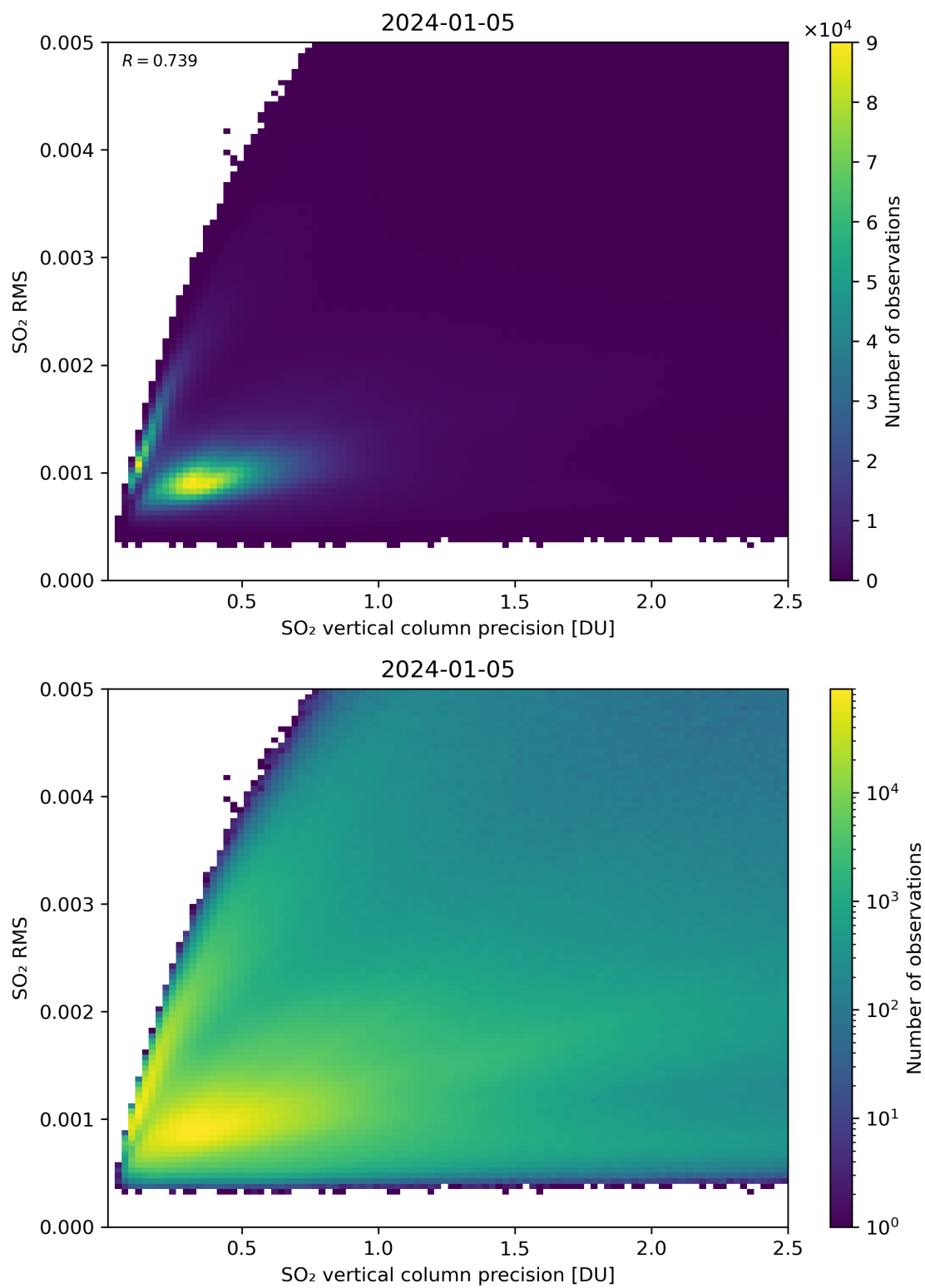
Figure 284: Scatter density plot of “SO 2 vertical column precision” against “SO 2 RMS” for 2024-01-05 to 2024-01-06.
