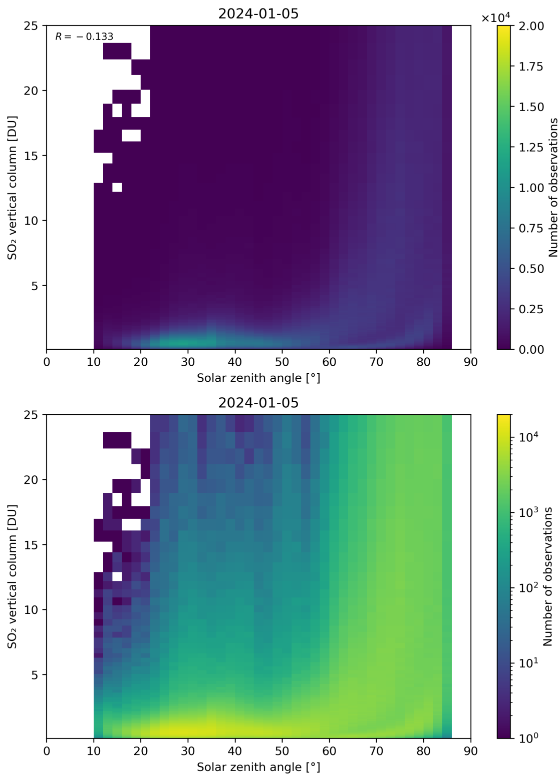
Figure 176: Scatter density plot of “Solar zenith angle” against “SO 2 vertical column” for 2024-01-05 to 2024-01-06.
