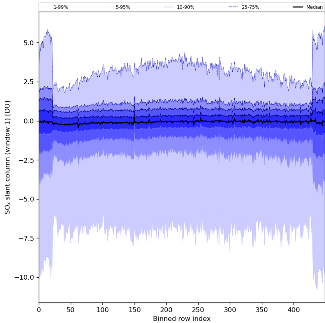
Figure 79: Along track statistics of “SO 2 slant column (window 1)” for 2024-01-05 to 2024-01-06
