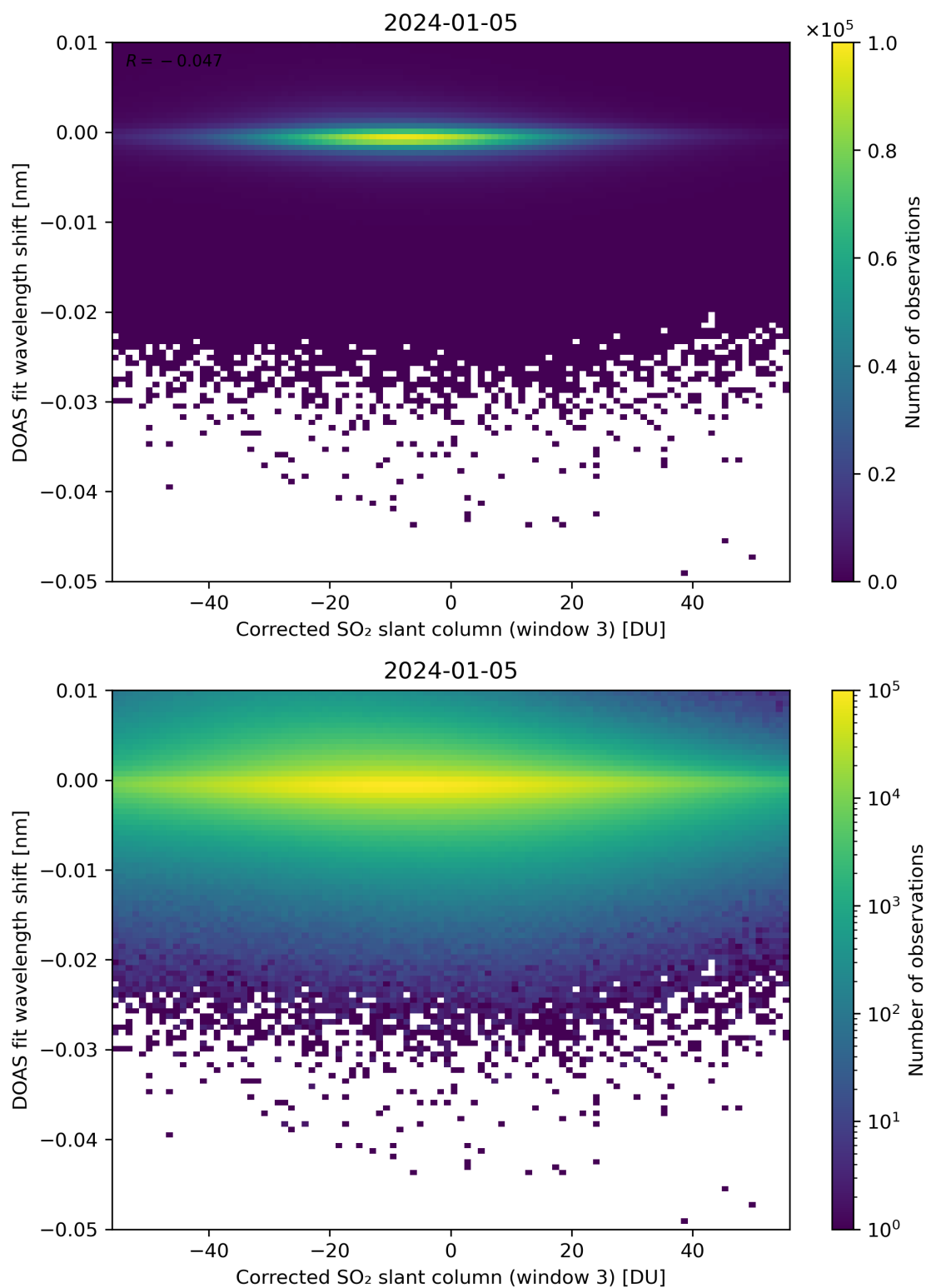
Figure 206: Scatter density plot of “Corrected SO 2 slant column (window 3)” against “DOAS fit wavelength shift” for 2024-01-05 to 2024-01-06.
