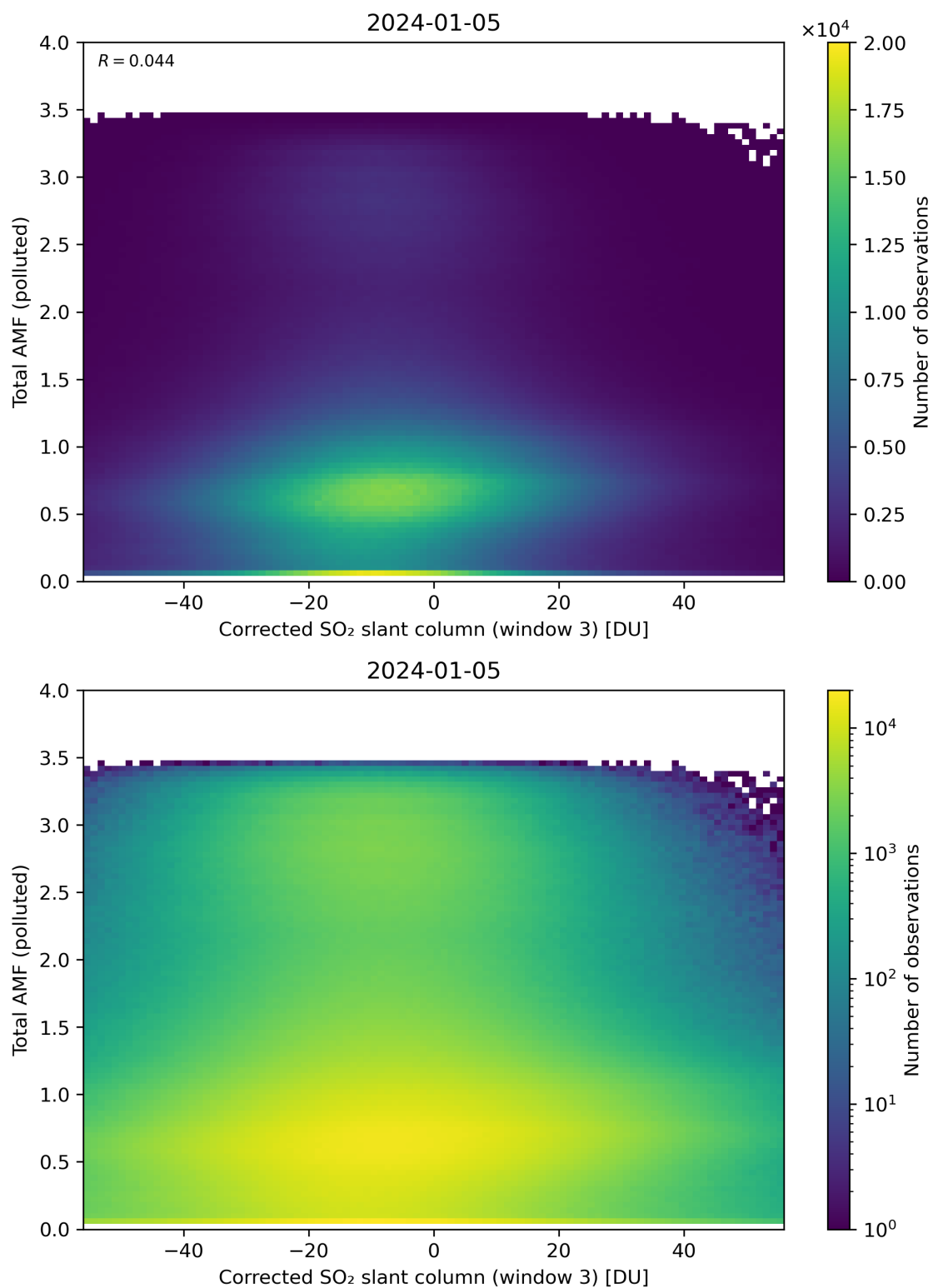
Figure 210: Scatter density plot of “Corrected SO 2 slant column (window 3)” against “Total AMF (polluted)” for 2024-01-05 to 2024-01-06.
