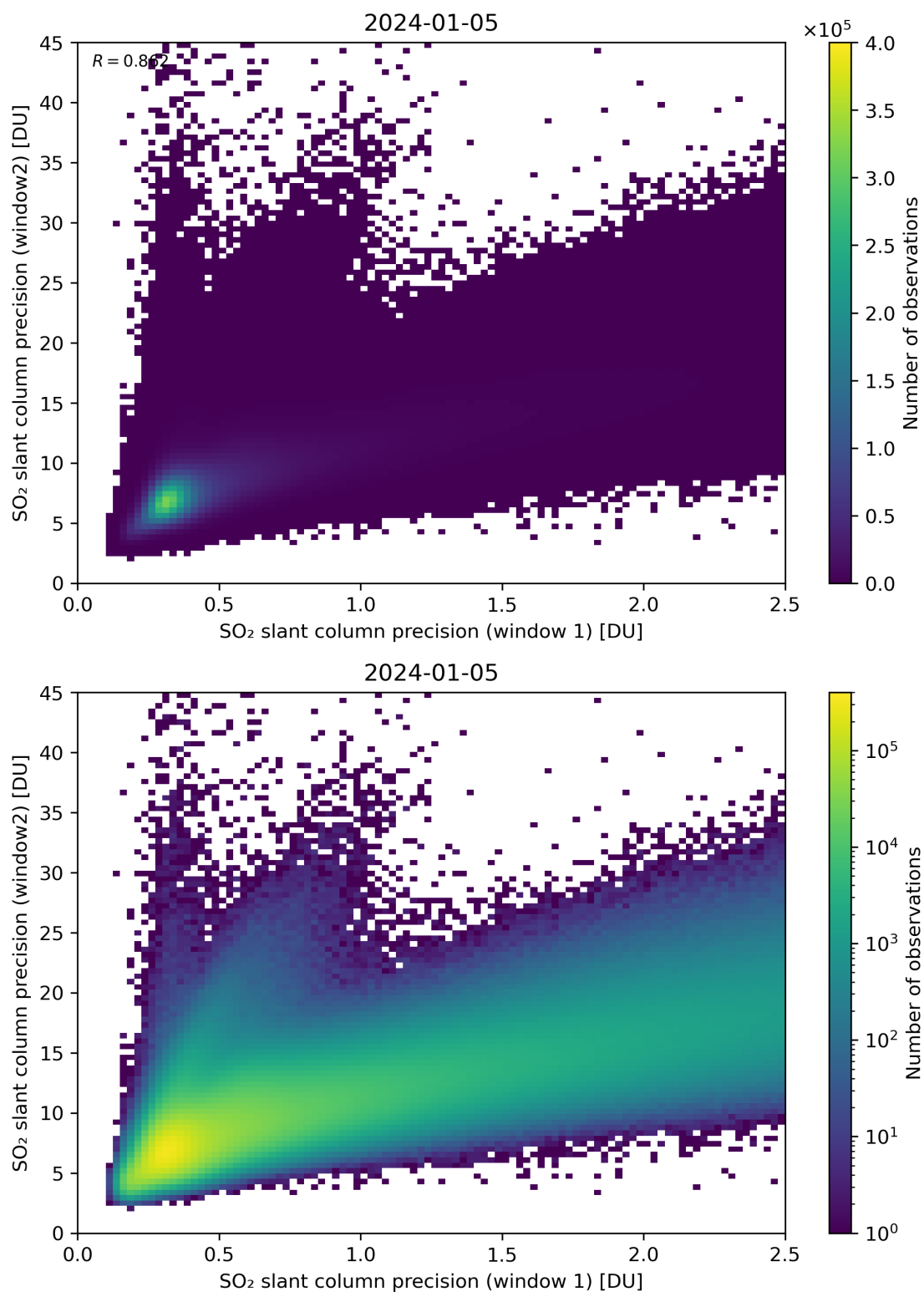
Figure 227: Scatter density plot of “SO 2 slant column precision (window 1)” against “SO 2 slant column precision (window2)” for 2024-01-05 to 2024-01-06.
