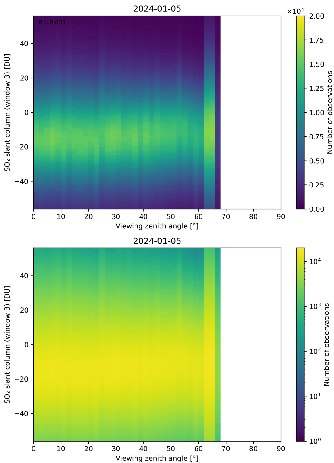
Figure 323: Scatter density plot of “Viewing zenith angle” against “SO 2 slant column (window 3)” for 2024-01-05 to 2024-01-06.
