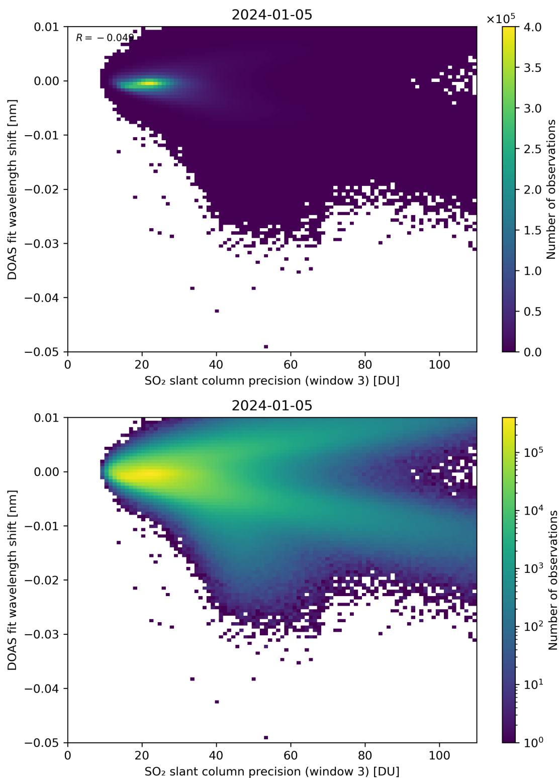
Figure 258: Scatter density plot of “SO 2 slant column precision (window 3)” against “DOAS fit wavelength shift” for 2024-01-05 to 2024-01-06.
