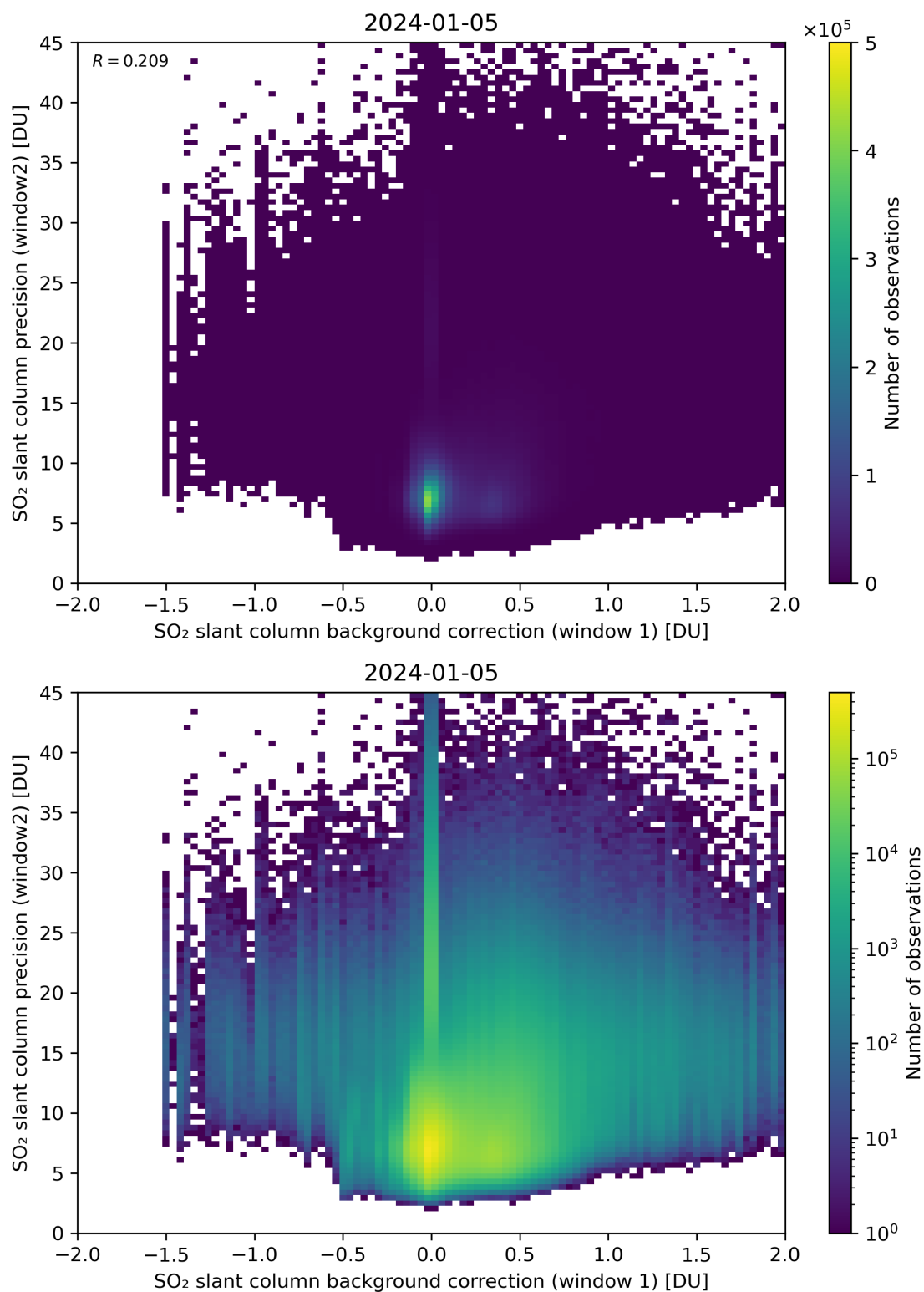
Figure 106: Scatter density plot of “SO 2 slant column background correction (window 1)” against “SO 2 slant column precision (window2)” for 2024-01-05 to 2024-01-06.
