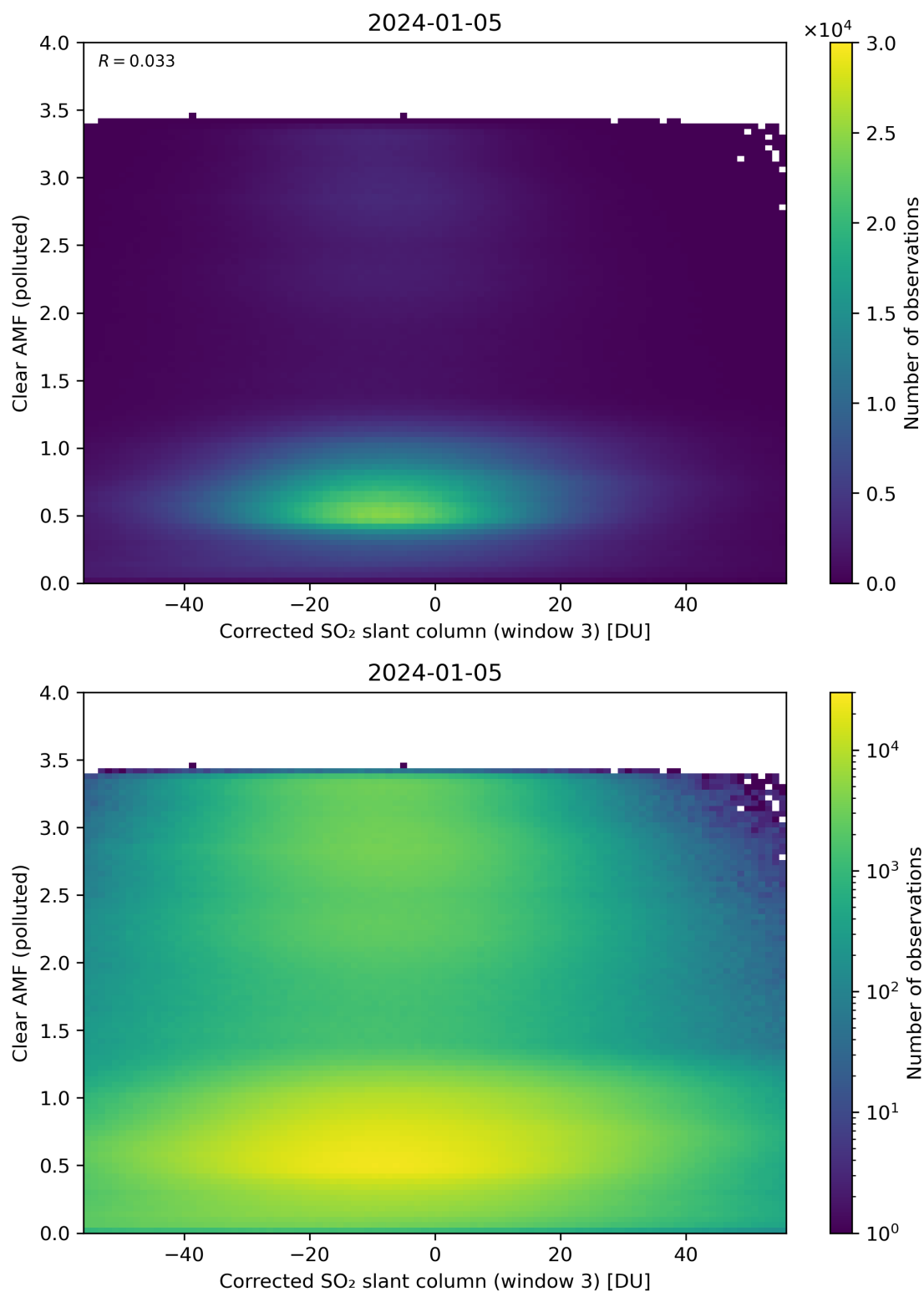
Figure 209: Scatter density plot of “Corrected SO 2 slant column (window 3)” against “Clear AMF (polluted)” for 2024-01-05 to 2024-01-06.
