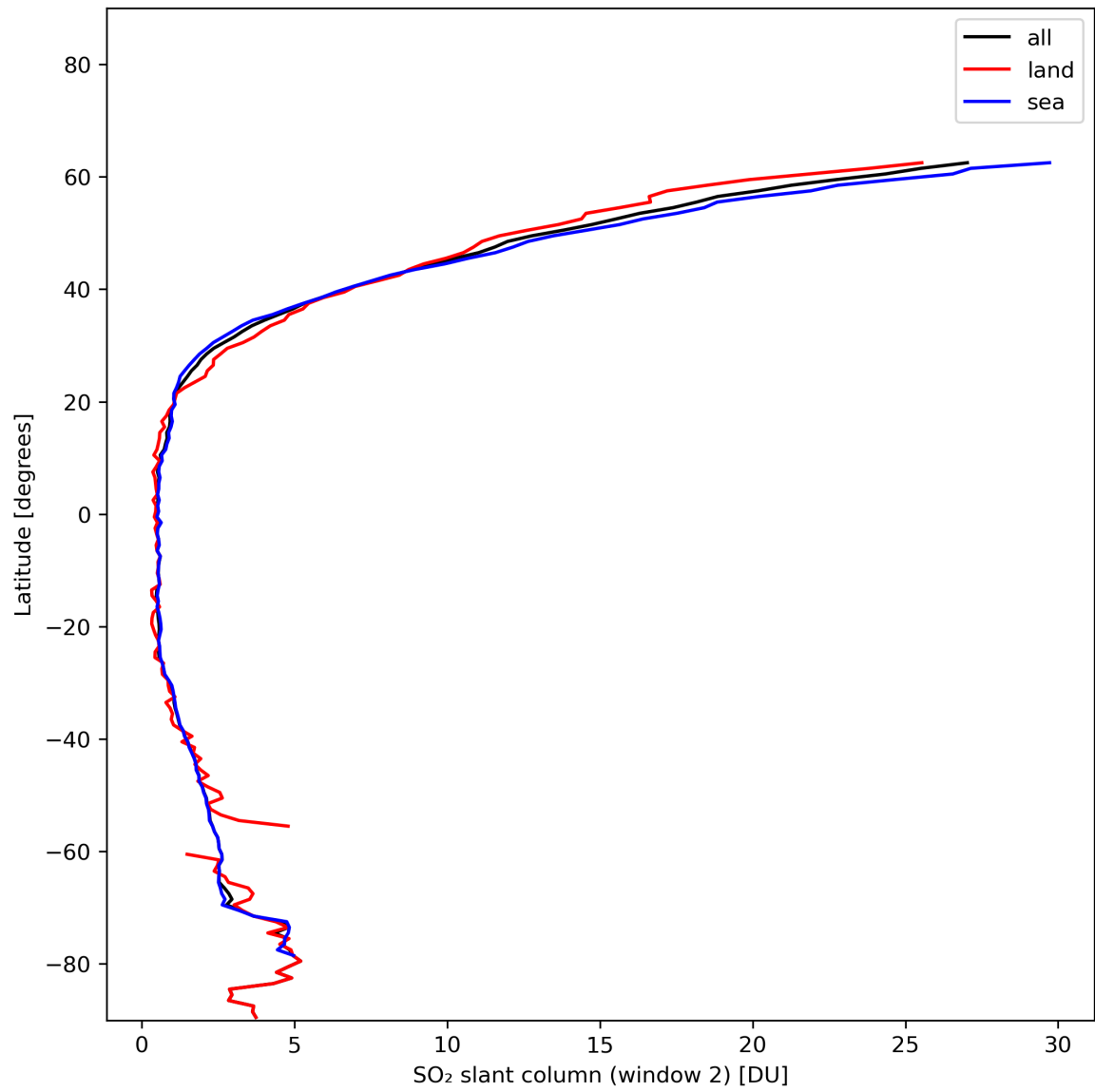
Figure 37: Zonal average of “SO 2 slant column (window 2)” for 2024-01-05 to 2024-01-06.
