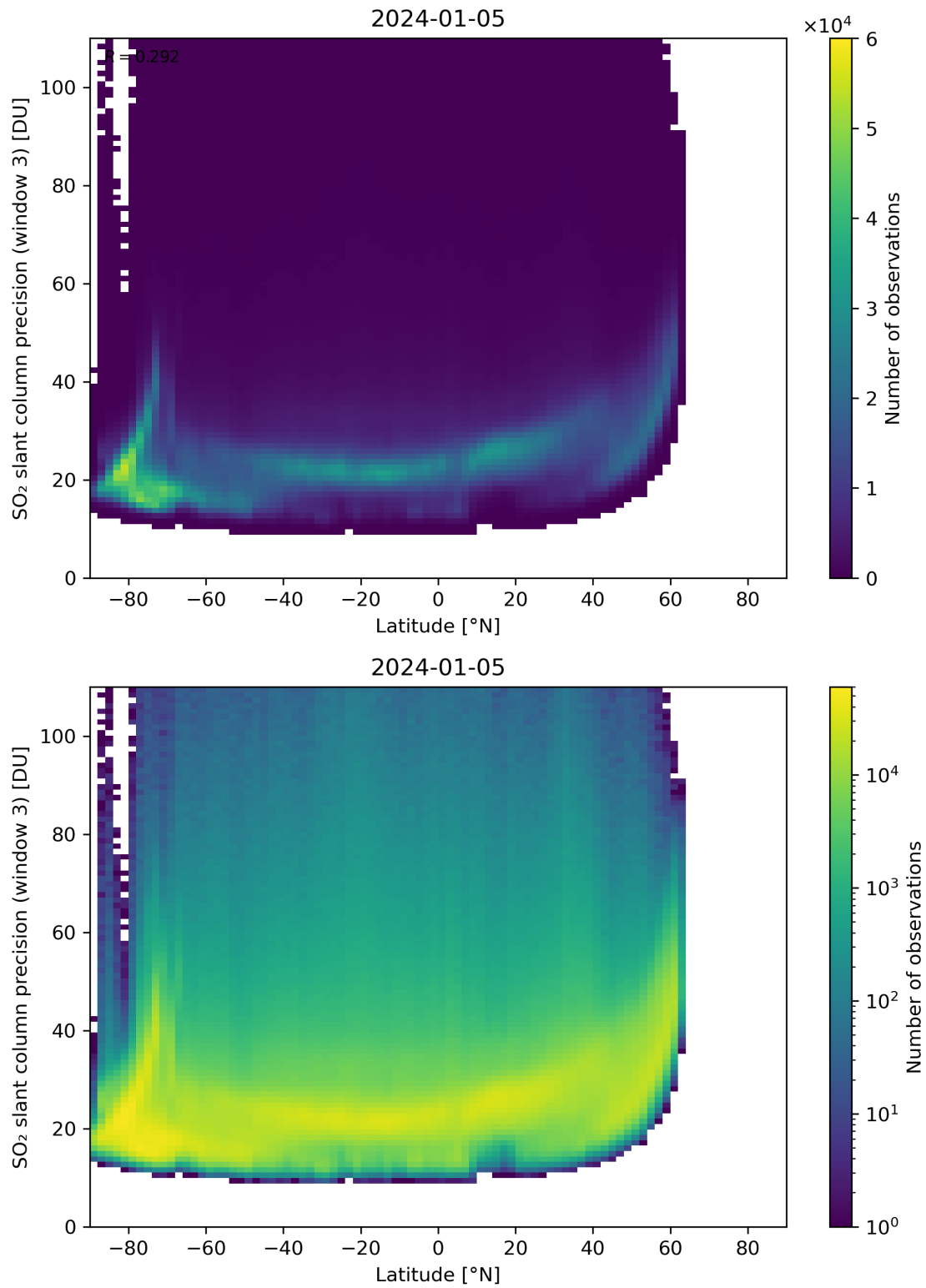
Figure 153: Scatter density plot of “Latitude” against “SO 2 slant column precision (window 3)” for 2024-01-05 to 2024-01-06.
