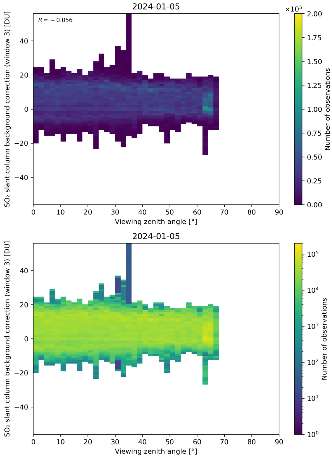
Figure 310: Scatter density plot of “Viewing zenith angle” against “SO 2 slant column background correction (window 3)” for 2024-01-05 to 2024-01-06.
