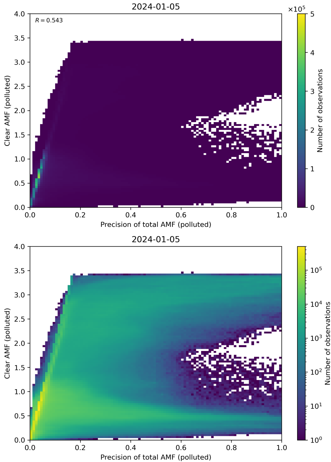
Figure 270: Scatter density plot of “Precision of total AMF (polluted)” against “Clear AMF (polluted)” for 2024-01-05 to 2024-01-06.
