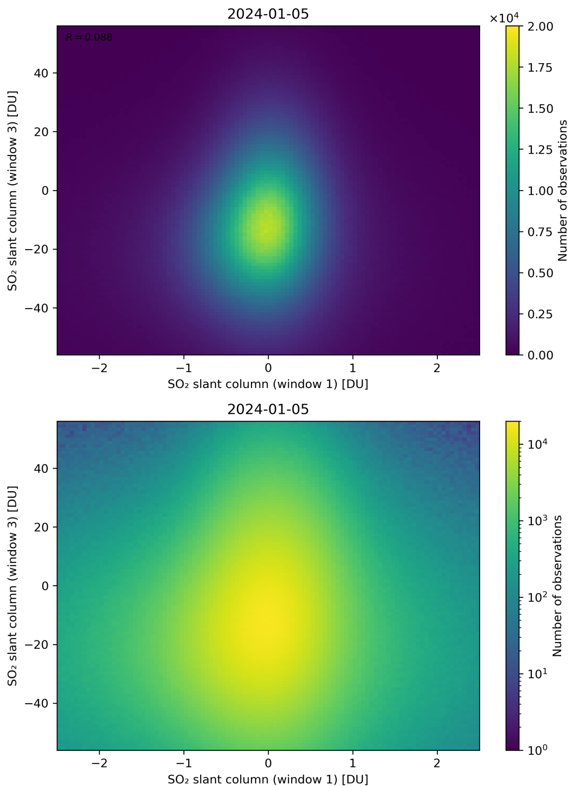
Figure 237: Scatter density plot of “SO 2 slant column (window 1)” against “SO 2 slant column (window 3)” for 2024-01-05 to 2024-01-06.
