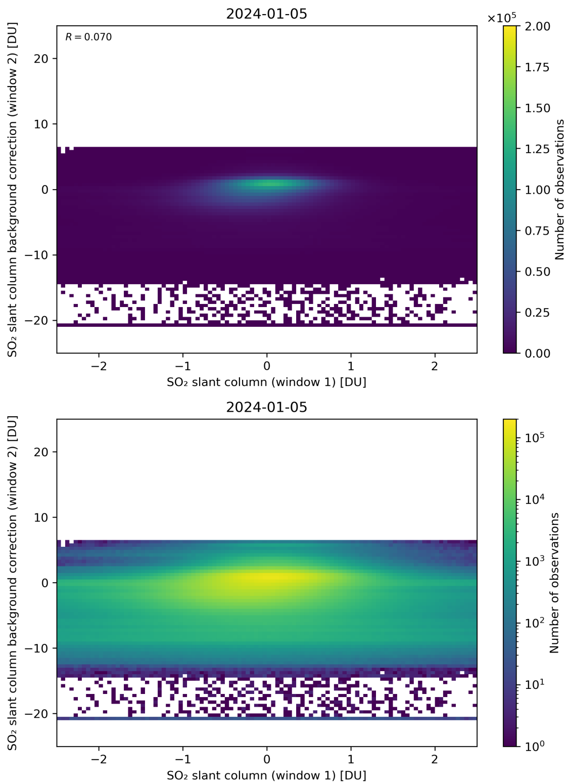
Figure 213: Scatter density plot of “SO 2 slant column (window 1)” against “SO 2 slant column background correction (window 2)” for 2024-01-05 to 2024-01-06.
