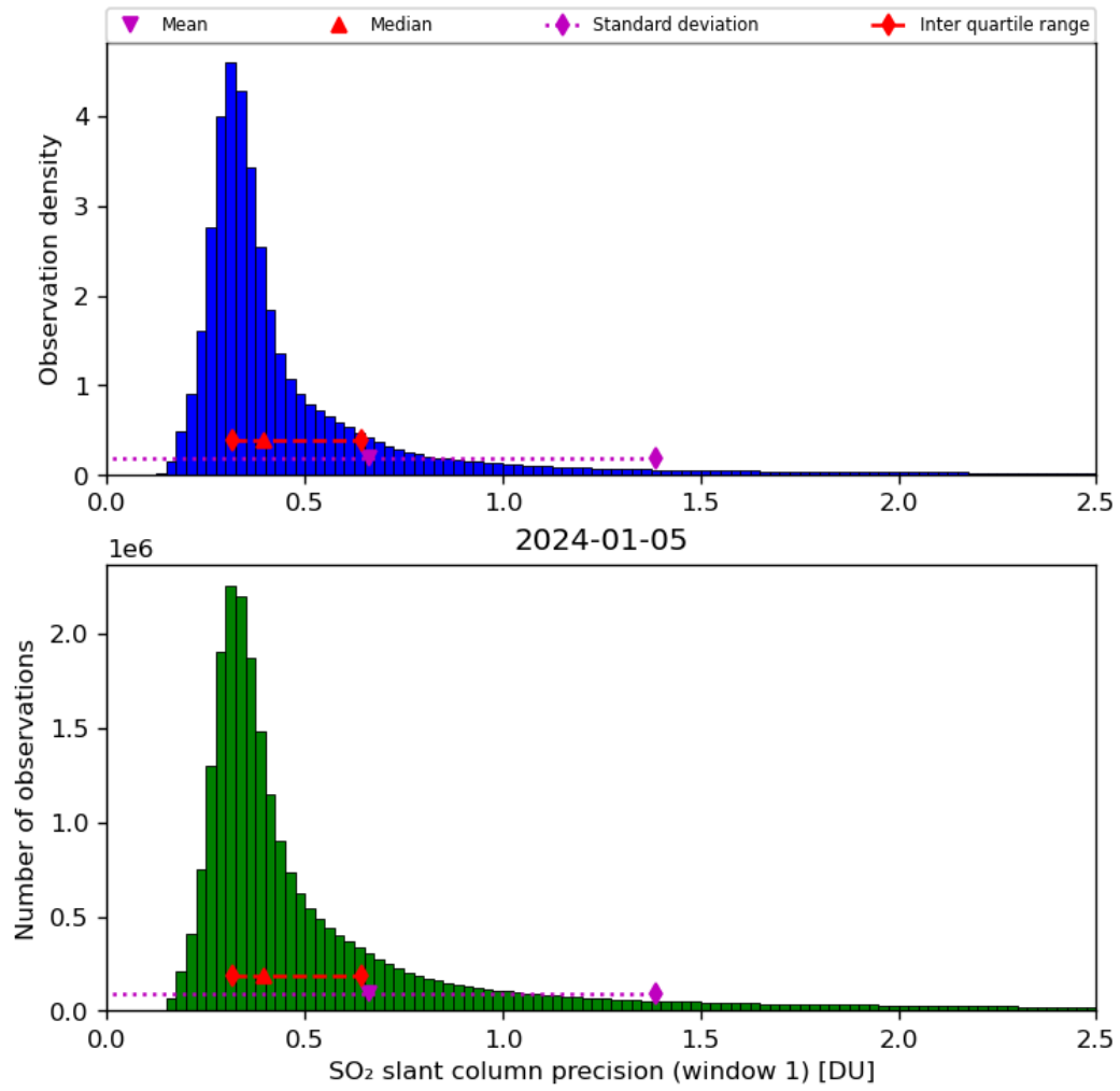
Figure 57: Histogram of “SO 2 slant column precision (window 1)” for 2024-01-05 to 2024-01-06
