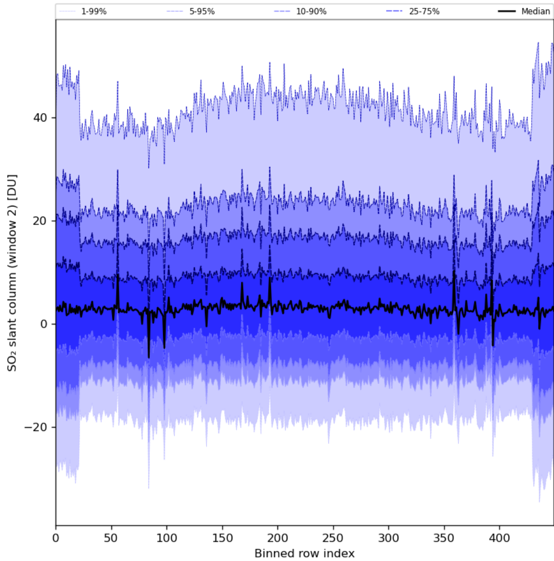
Figure 83: Along track statistics of “SO 2 slant column (window 2)” for 2024-01-05 to 2024-01-06
