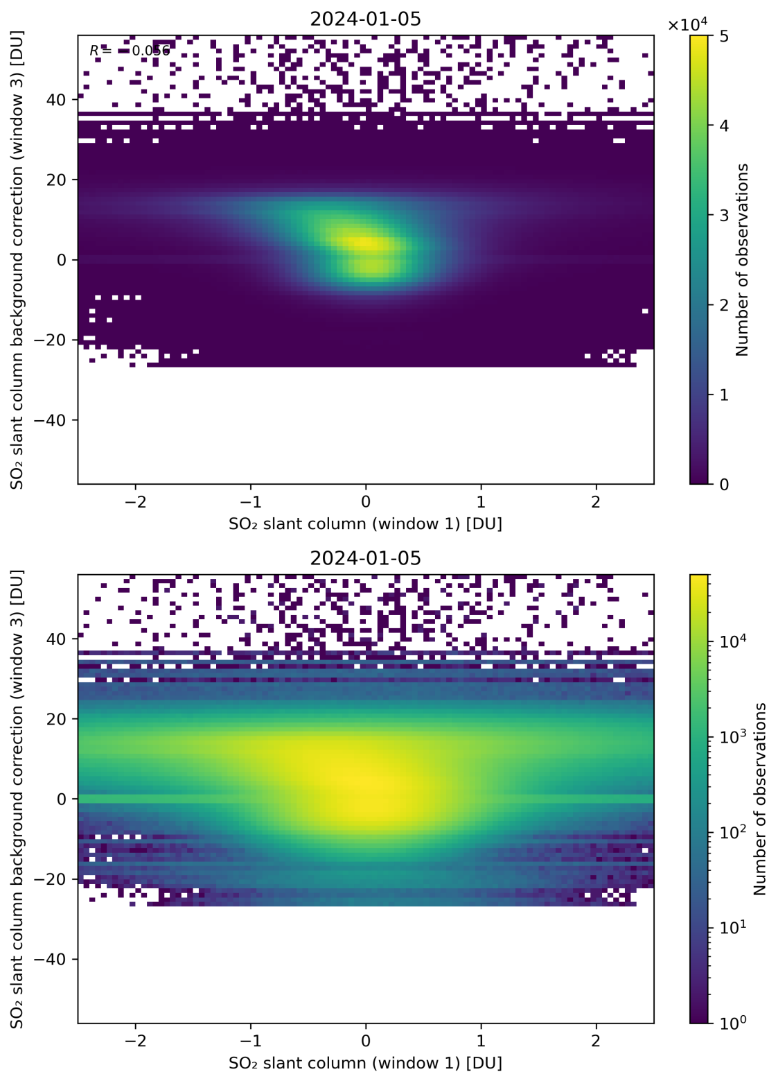
Figure 214: Scatter density plot of “SO 2 slant column (window 1)” against “SO 2 slant column background correction (window 3)” for 2024-01-05 to 2024-01-06.
