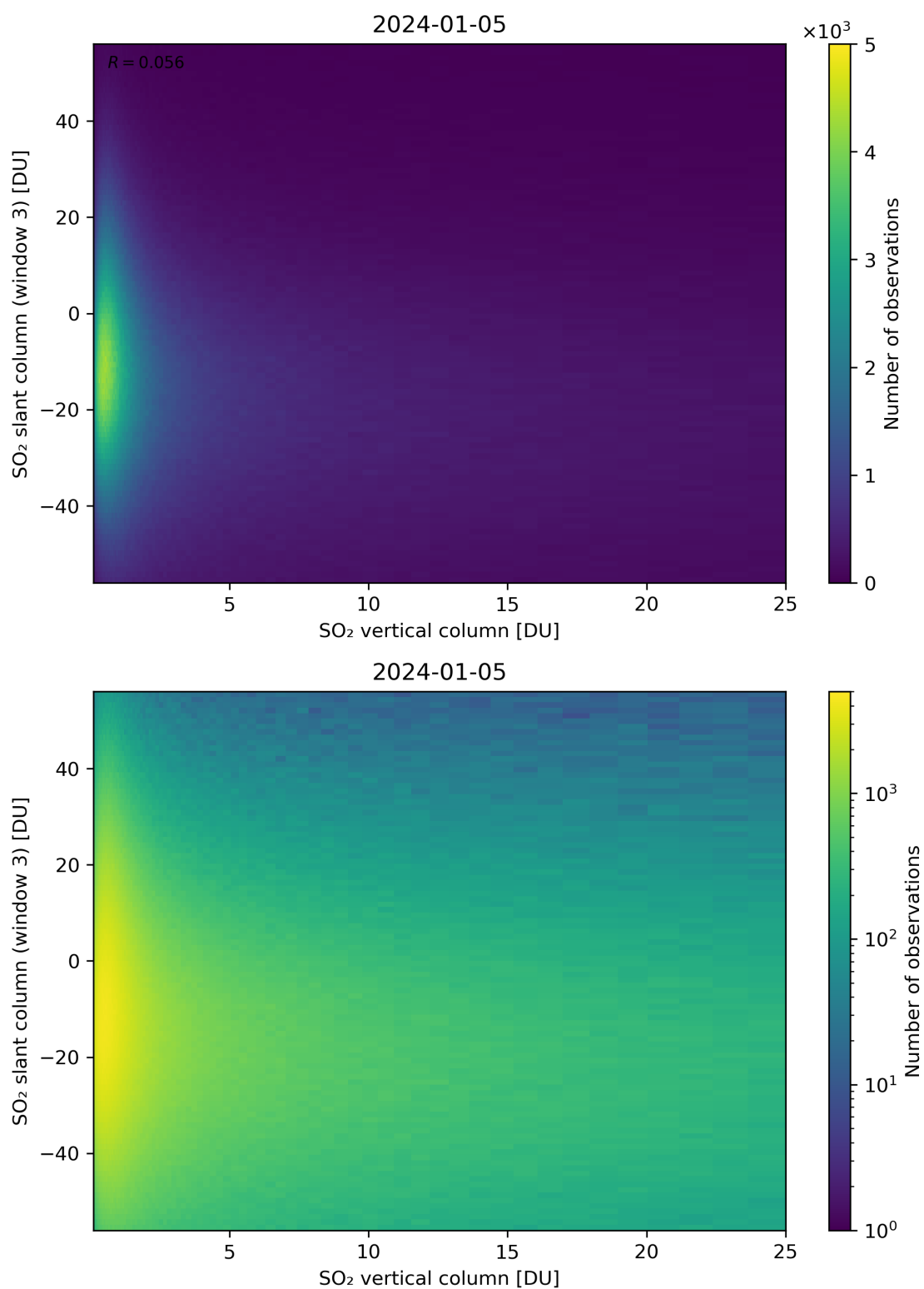
Figure 303: Scatter density plot of “SO 2 vertical column” against “SO 2 slant column (window 3)” for 2024-01-05 to 2024-01-06.
