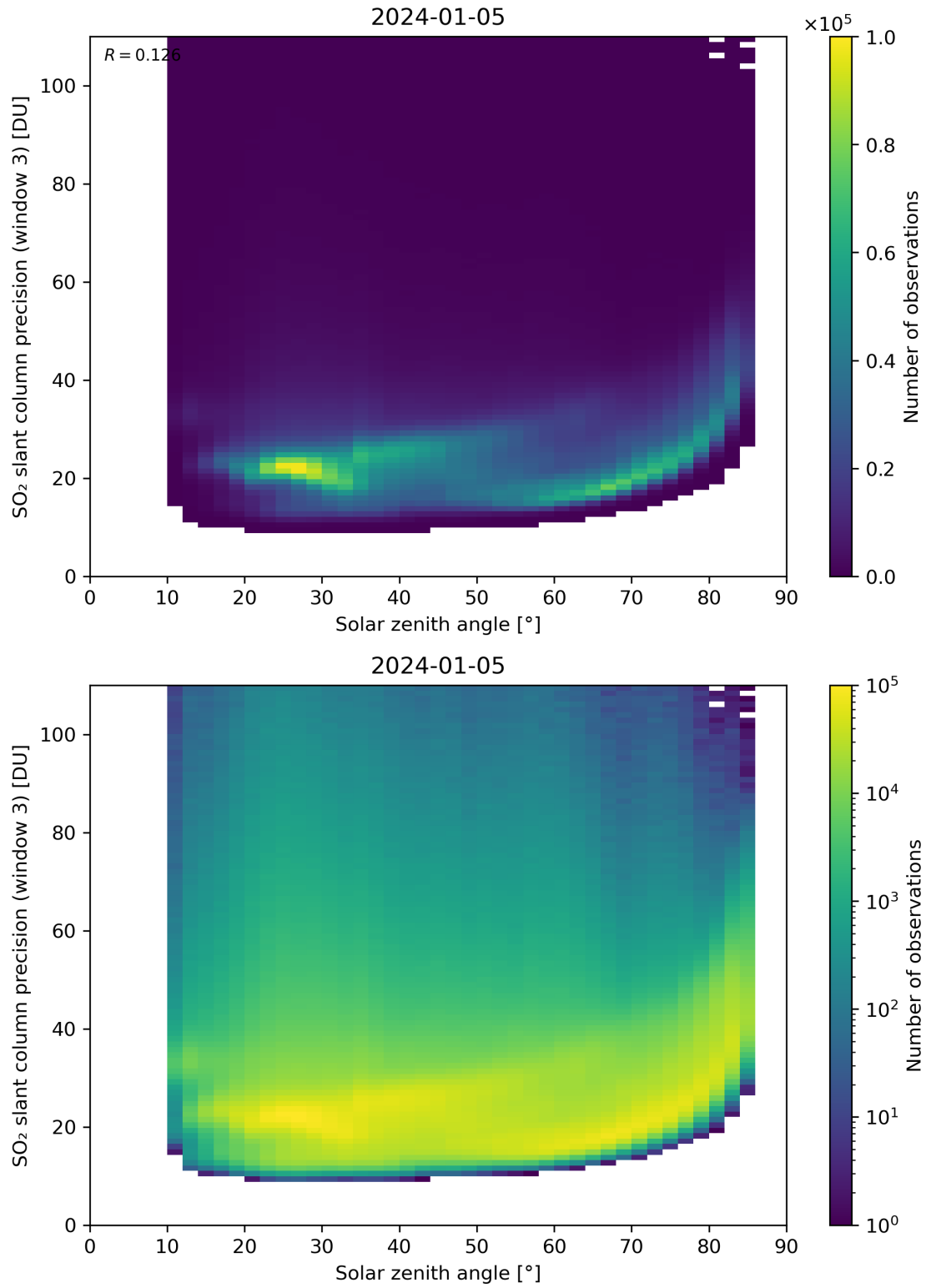
Figure 173: Scatter density plot of “Solar zenith angle” against “SO 2 slant column precision (window 3)” for 2024-01-05 to 2024-01-06.
