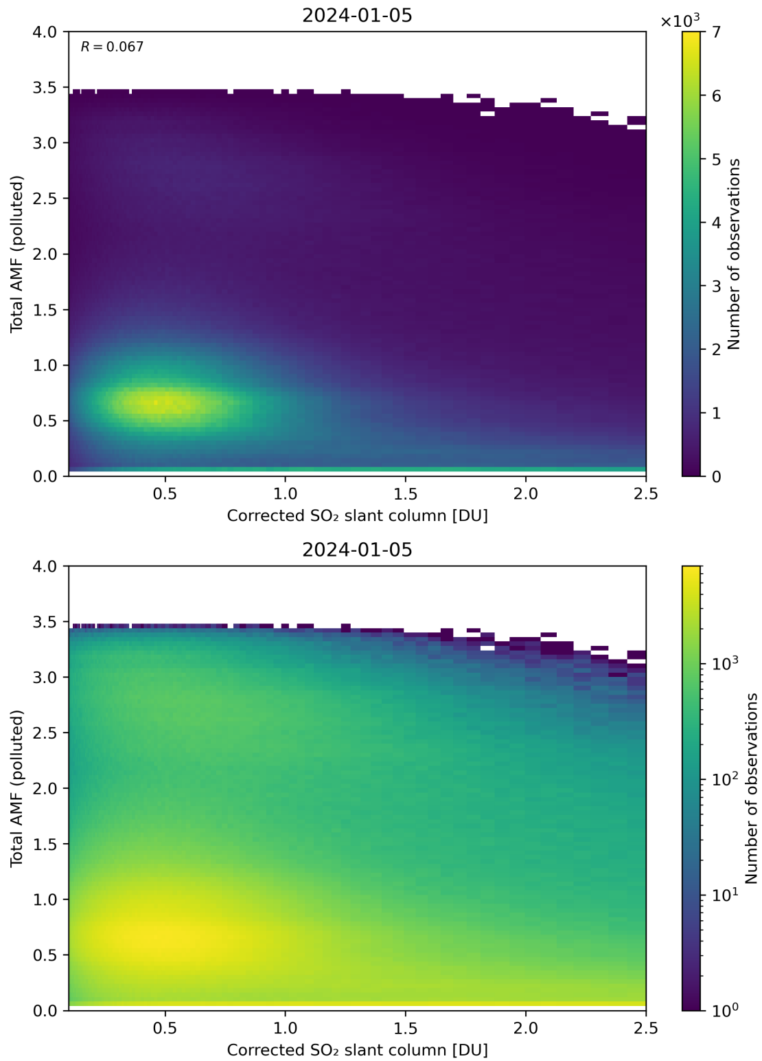
Figure 192: Scatter density plot of “Corrected SO 2 slant column” against “Total AMF (polluted)” for 2024-01-05 to 2024-01-06.
