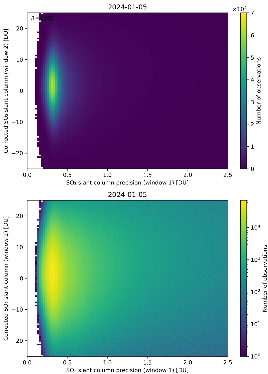
Figure 225: Scatter density plot of “SO 2 slant column precision (window 1)” against “Corrected SO 2 slant column (window 2)” for 2024-01-05 to 2024-01-06.
