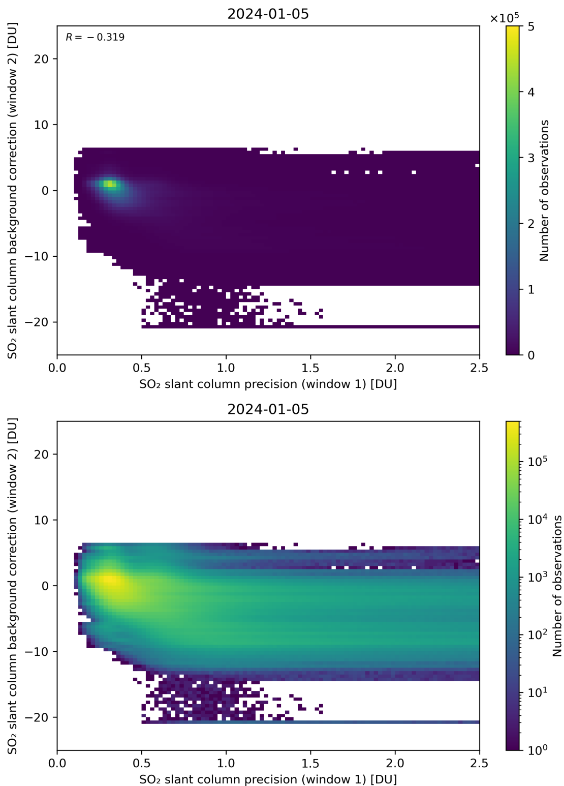
Figure 219: Scatter density plot of “SO 2 slant column precision (window 1)” against “SO 2 slant column background correction (window 2)” for 2024-01-05 to 2024-01-06.
