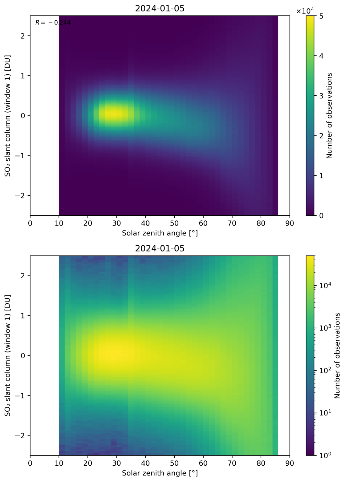
Figure 169: Scatter density plot of “Solar zenith angle” against “SO 2 slant column (window 1)” for 2024-01-05 to 2024-01-06.
