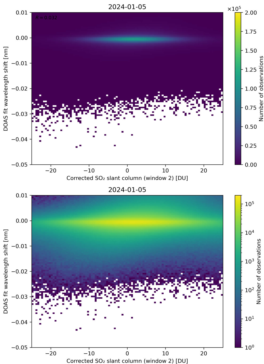
Figure 196: Scatter density plot of “Corrected SO 2 slant column (window 2)” against “DOAS fit wavelength shift” for 2024-01-05 to 2024-01-06.
