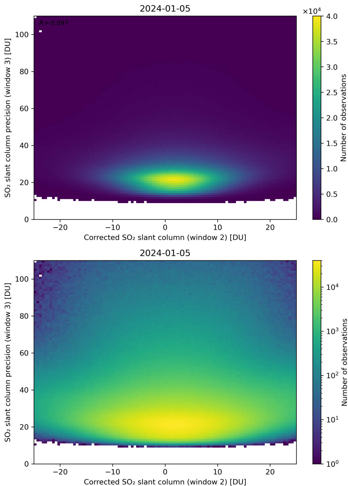
Figure 202: Scatter density plot of “Corrected SO 2 slant column (window 2)” against “SO 2 slant column precision (window 3)” for 2024-01-05 to 2024-01-06.
