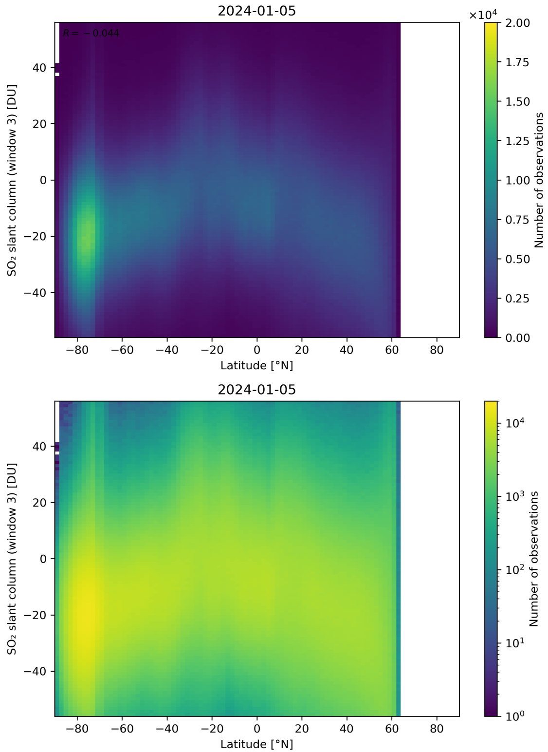
Figure 152: Scatter density plot of “Latitude” against “SO 2 slant column (window 3)” for 2024-01-05 to 2024-01-06.
