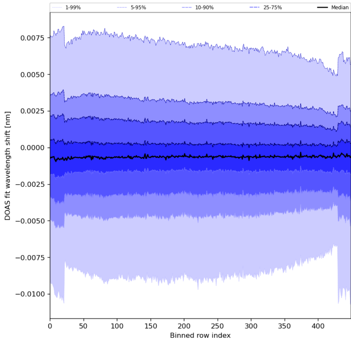
Figure 91: Along track statistics of “DOAS fit wavelength shift” for 2024-01-05 to 2024-01-06
