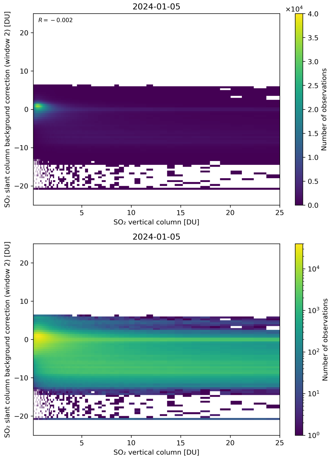
Figure 274: Scatter density plot of “SO 2 vertical column” against “SO 2 slant column background correction (window 2)” for 2024-01-05 to 2024-01-06.
