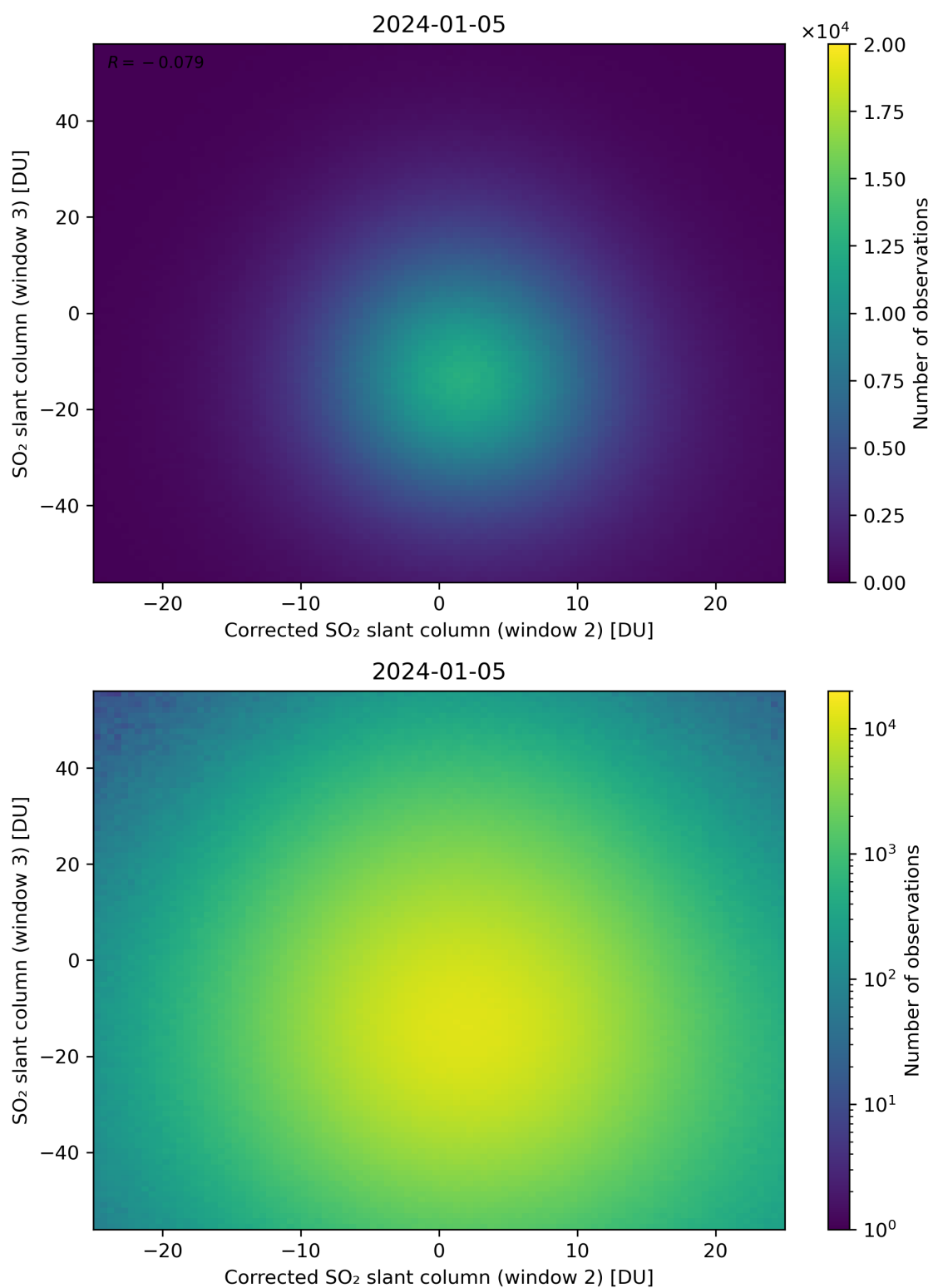
Figure 201: Scatter density plot of “Corrected SO 2 slant column (window 2)” against “SO 2 slant column (window 3)” for 2024-01-05 to 2024-01-06.
