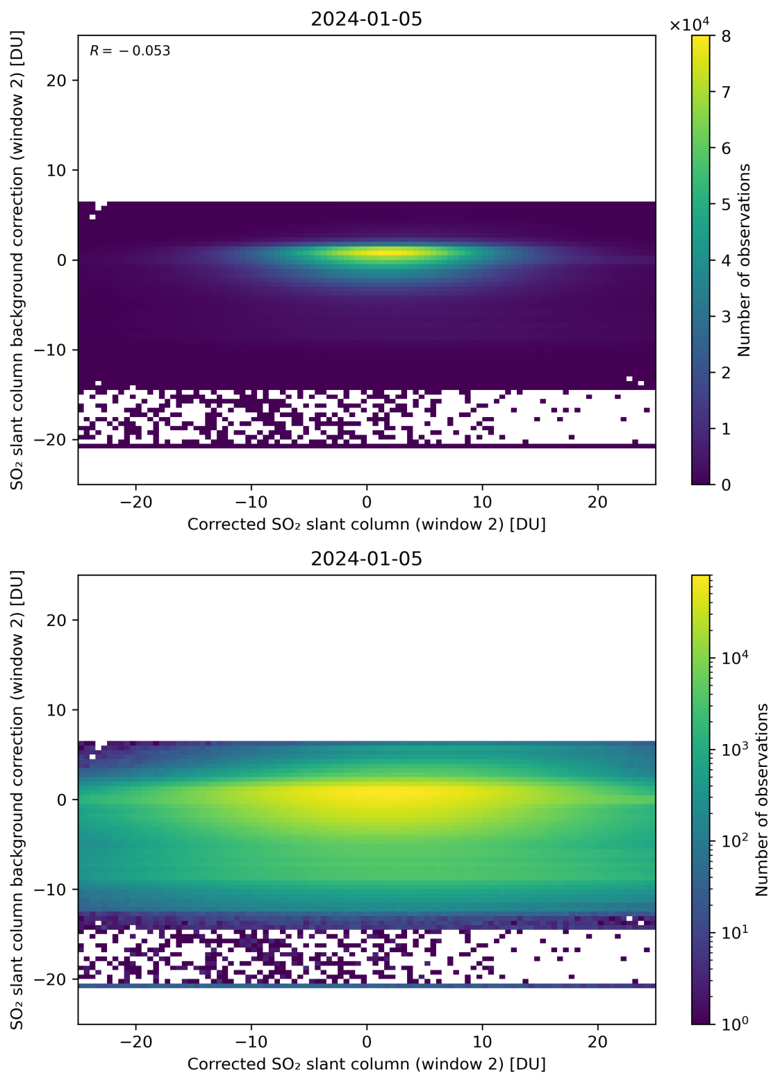
Figure 194: Scatter density plot of “Corrected SO 2 slant column (window 2)” against “SO 2 slant column background correction (window 2)” for 2024-01-05 to 2024-01-06.
