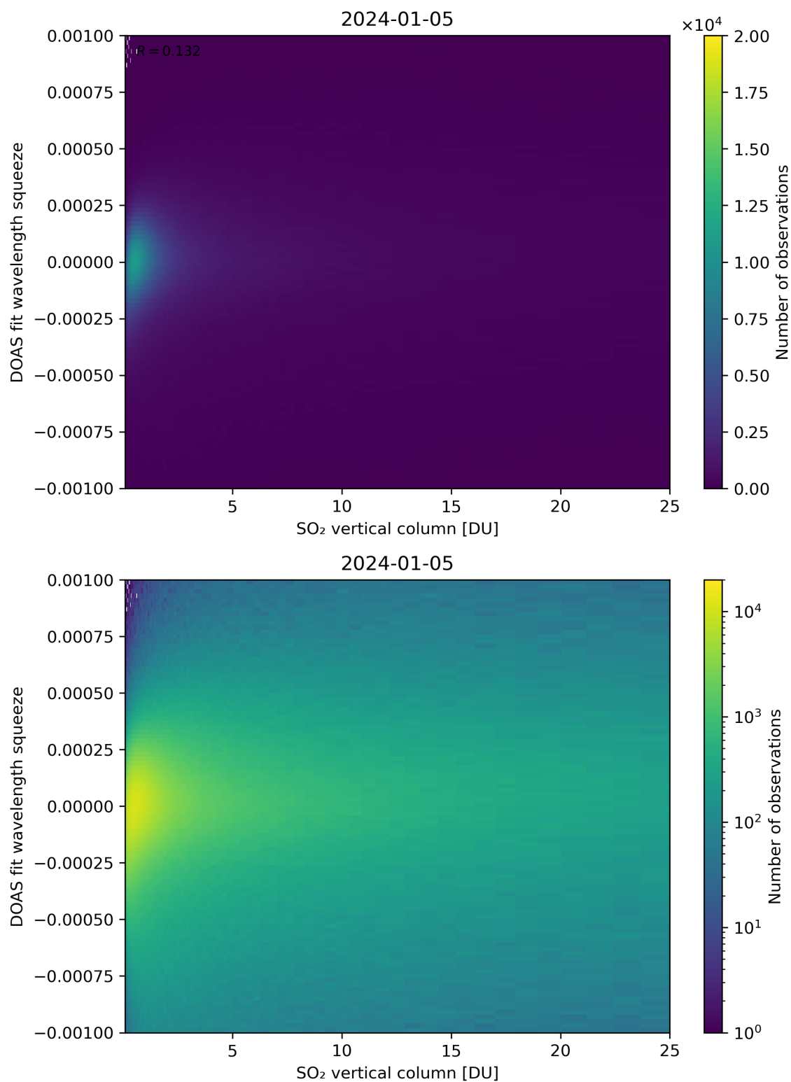
Figure 277: Scatter density plot of “SO 2 vertical column” against “DOAS fit wavelength squeeze” for 2024-01-05 to 2024-01-06.
