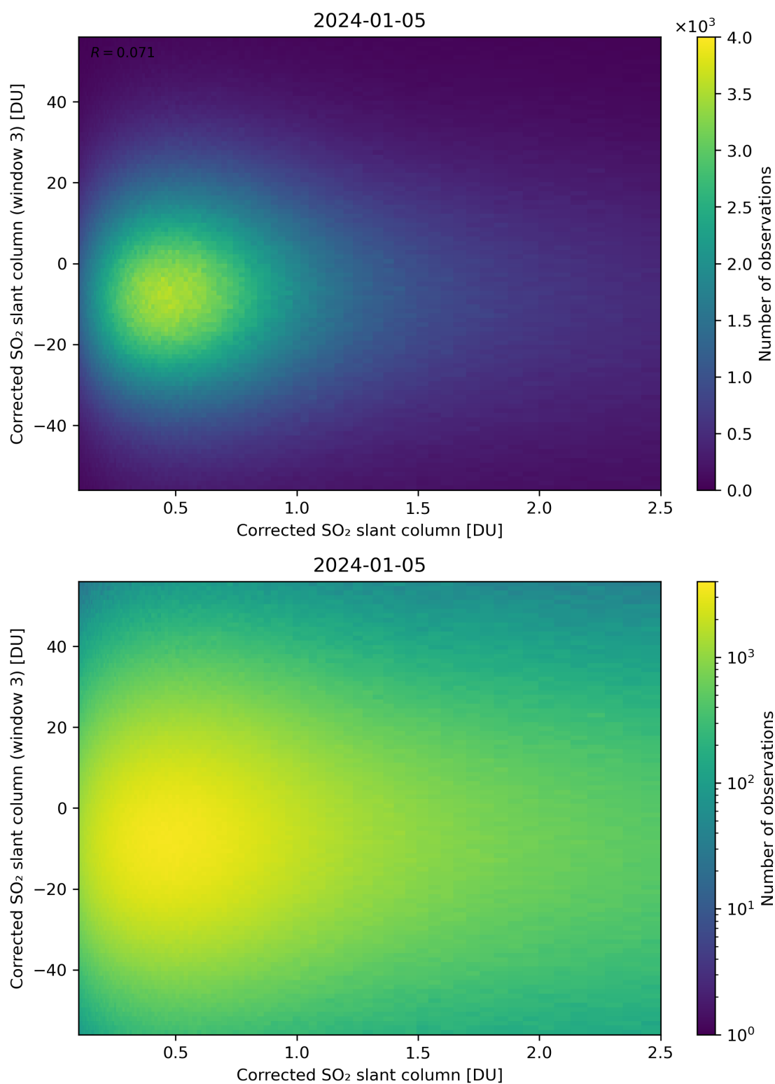
Figure 186: Scatter density plot of “Corrected SO 2 slant column” against “Corrected SO 2 slant column (window 3)” for 2024-01-05 to 2024-01-06.
