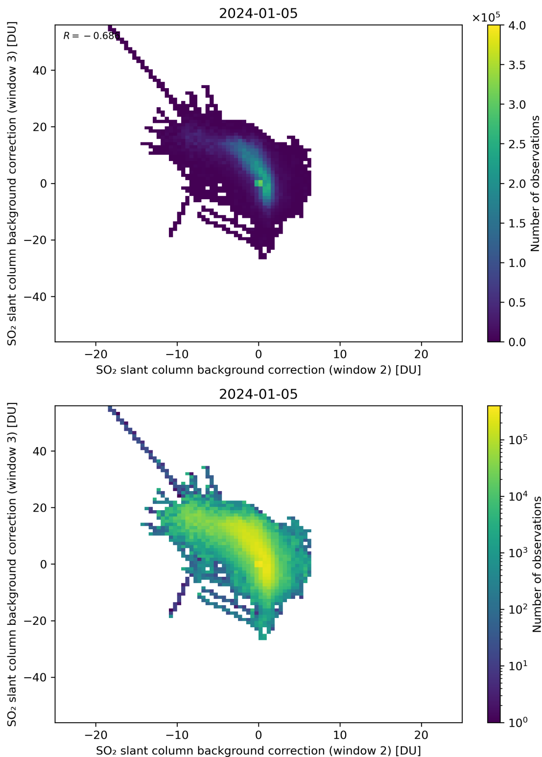
Figure 111: Scatter density plot of “SO 2 slant column background correction (window 2)” against “SO 2 slant column background correction (window 3)” for 2024-01-05 to 2024-01-06.
