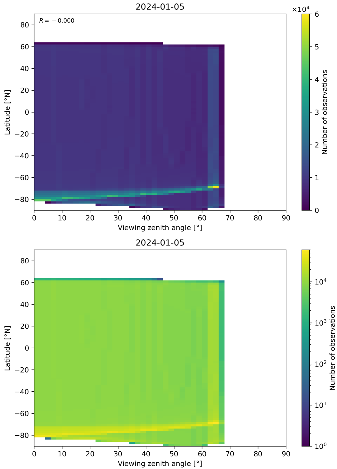
Figure 314: Scatter density plot of “Viewing zenith angle” against “Latitude” for 2024-01-05 to 2024-01-06.
