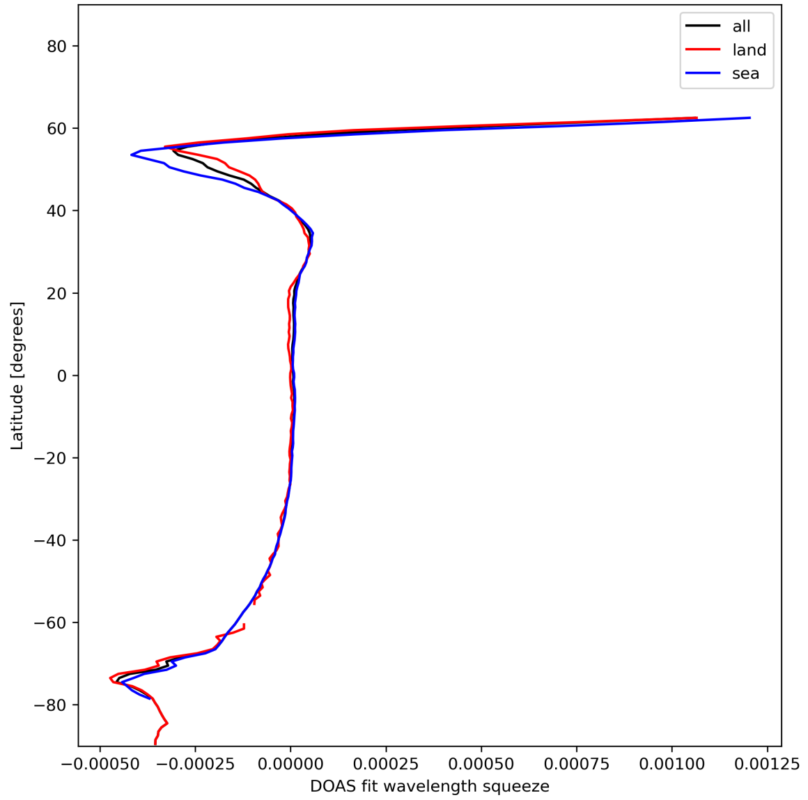
Figure 46: Zonal average of “DOAS fit wavelength squeeze” for 2024-01-05 to 2024-01-06.
