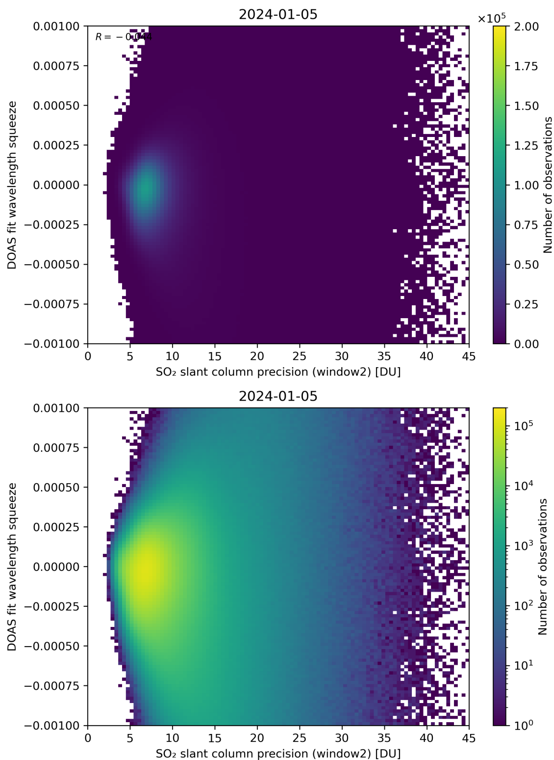
Figure 244: Scatter density plot of “SO 2 slant column precision (window2)” against “DOAS fit wavelength squeeze” for 2024-01-05 to 2024-01-06.
