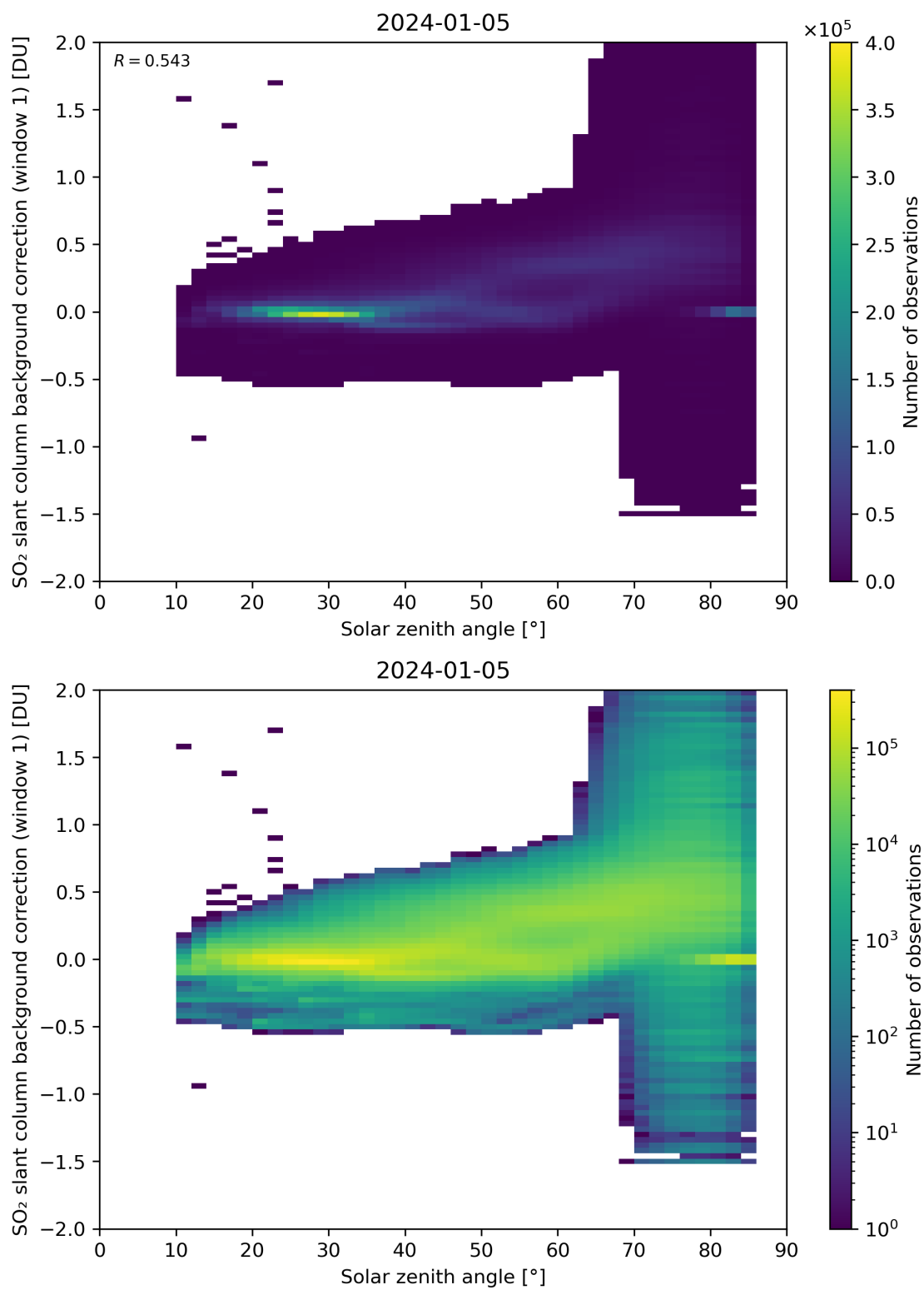
Figure 158: Scatter density plot of “Solar zenith angle” against “SO 2 slant column background correction (window 1)” for 2024-01-05 to 2024-01-06.
