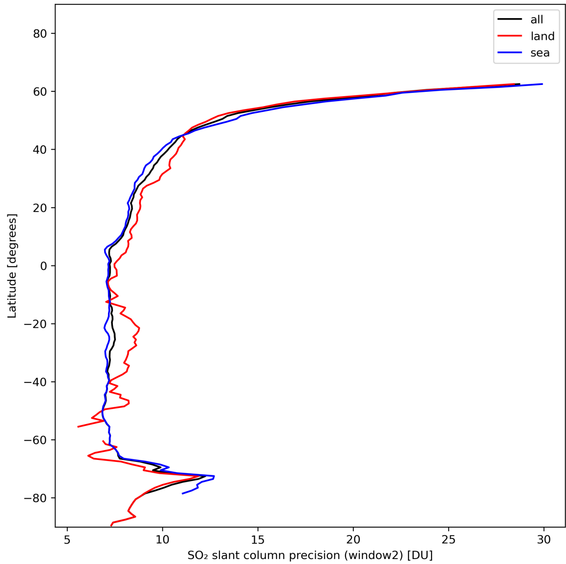
Figure 38: Zonal average of “SO 2 slant column precision (window2)” for 2024-01-05 to 2024-01-06.
