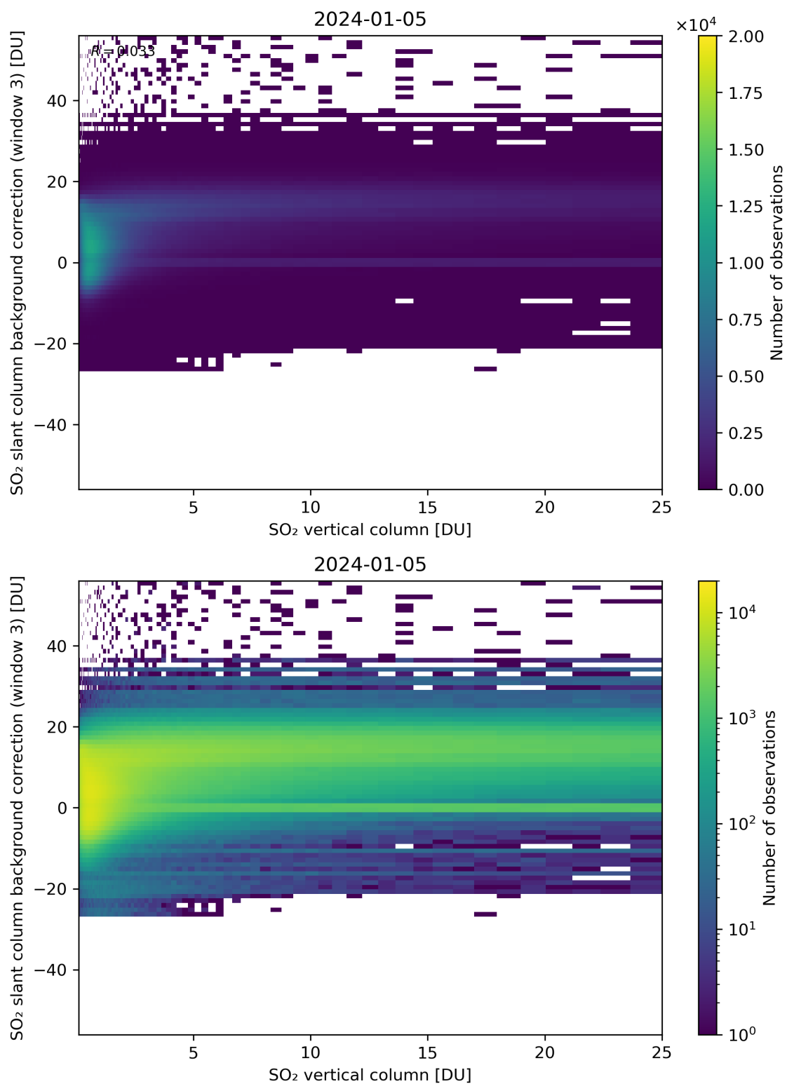
Figure 275: Scatter density plot of “SO 2 vertical column” against “SO 2 slant column background correction (window 3)” for 2024-01-05 to 2024-01-06.
