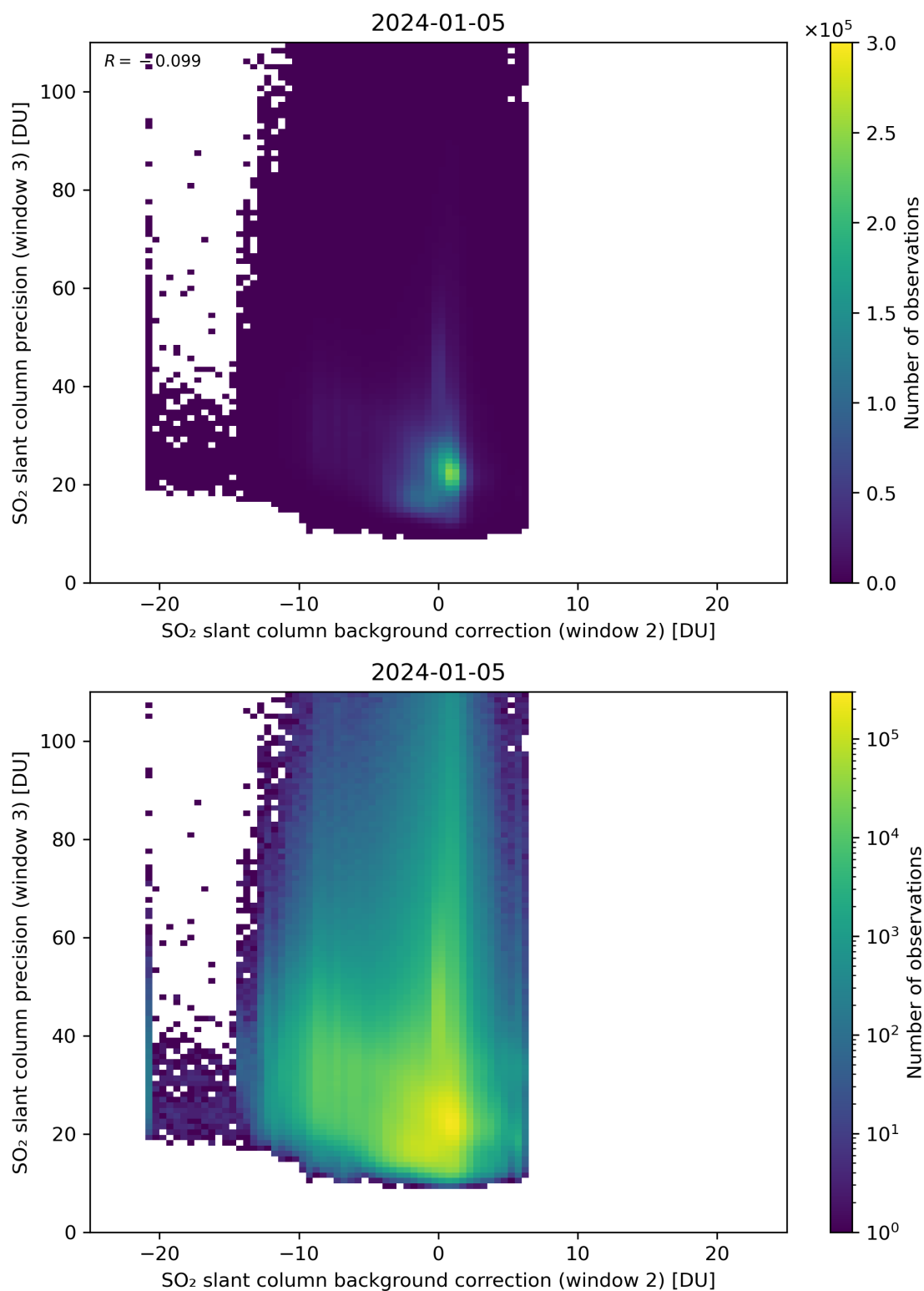
Figure 118: Scatter density plot of “SO 2 slant column background correction (window 2)” against “SO 2 slant column precision (window 3)” for 2024-01-05 to 2024-01-06.
