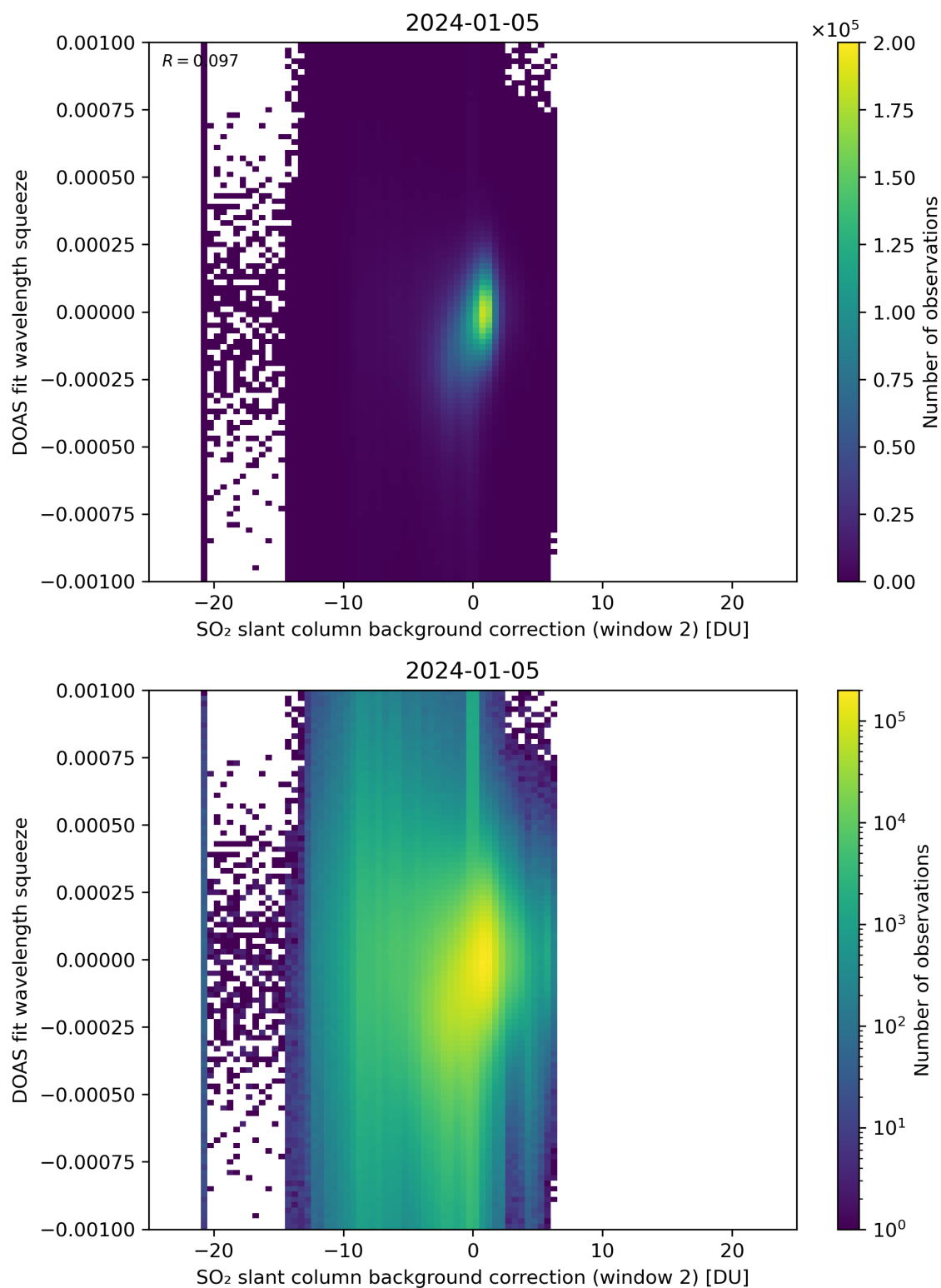
Figure 113: Scatter density plot of “SO 2 slant column background correction (window 2)” against “DOAS fit wavelength squeeze” for 2024-01-05 to 2024-01-06.
