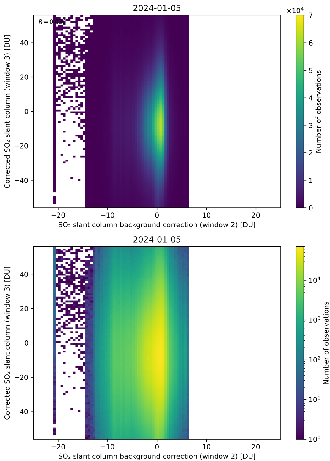
Figure 116: Scatter density plot of “SO 2 slant column background correction (window 2)” against “Corrected SO 2 slant column (window 3)” for 2024-01-05 to 2024-01-06.
