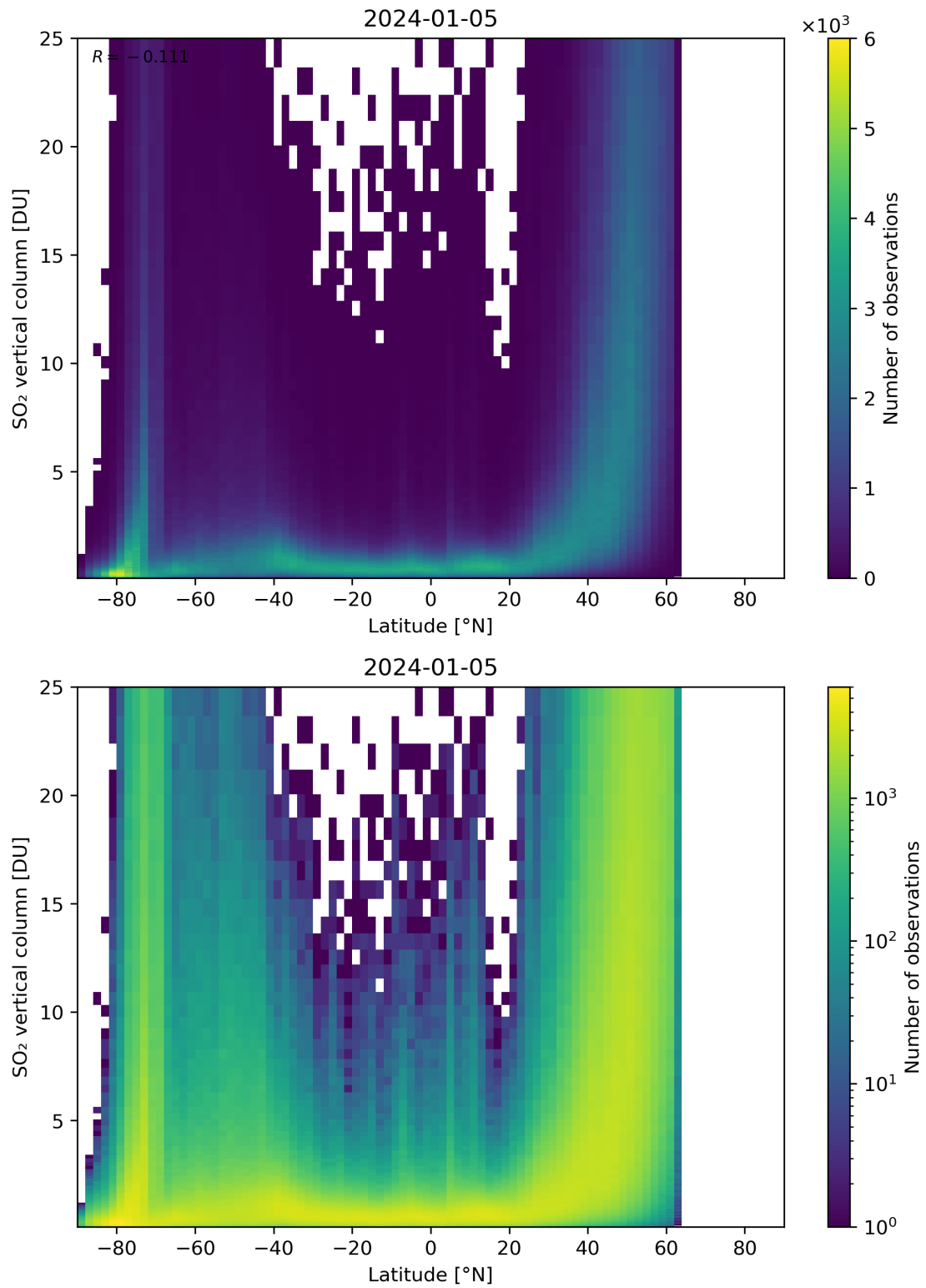
Figure 156: Scatter density plot of “Latitude” against “SO 2 vertical column” for 2024-01-05 to 2024-01-06.
