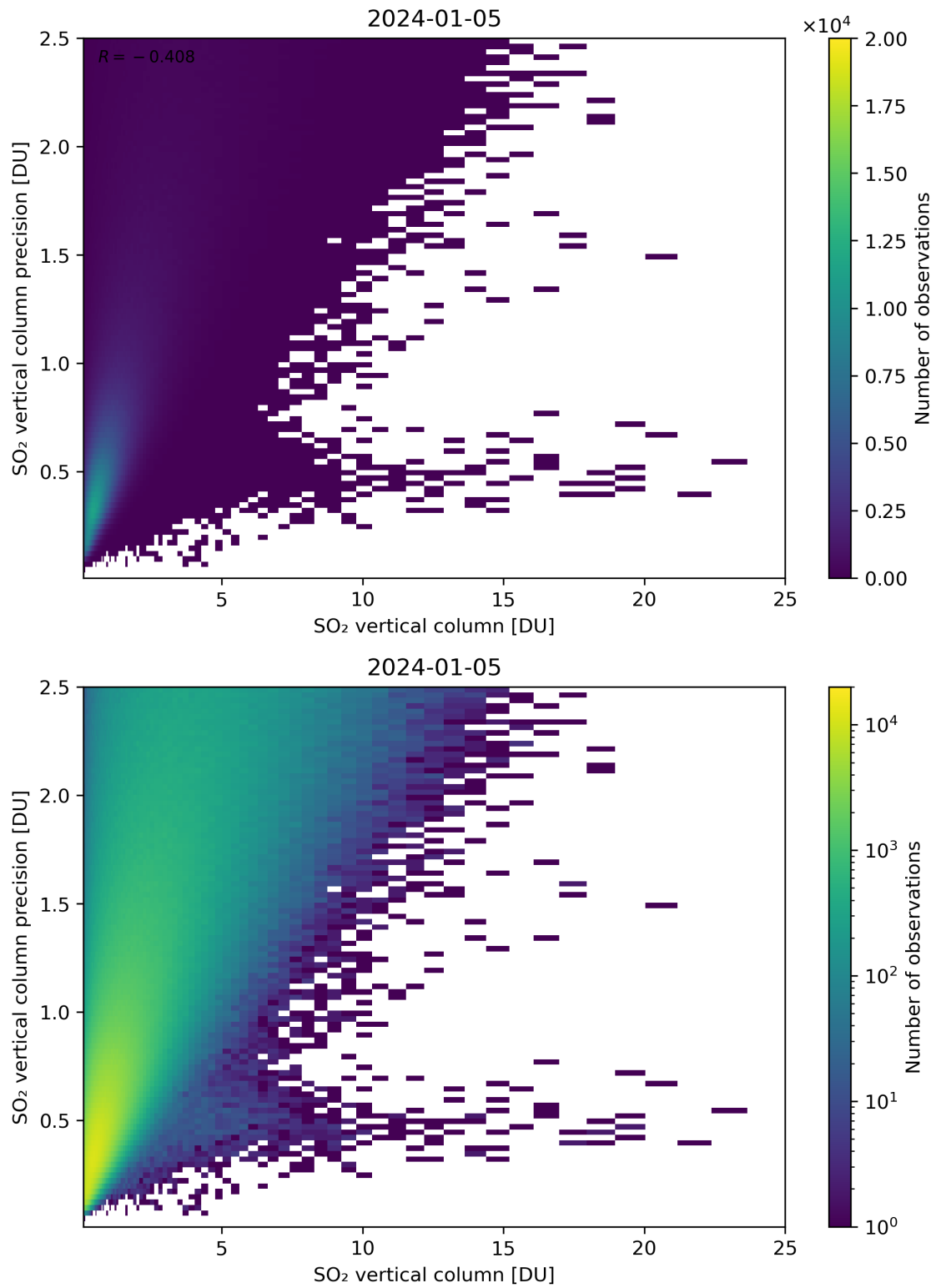
Figure 307: Scatter density plot of “SO 2 vertical column” against “SO 2 vertical column precision” for 2024-01-05 to 2024-01-06.
