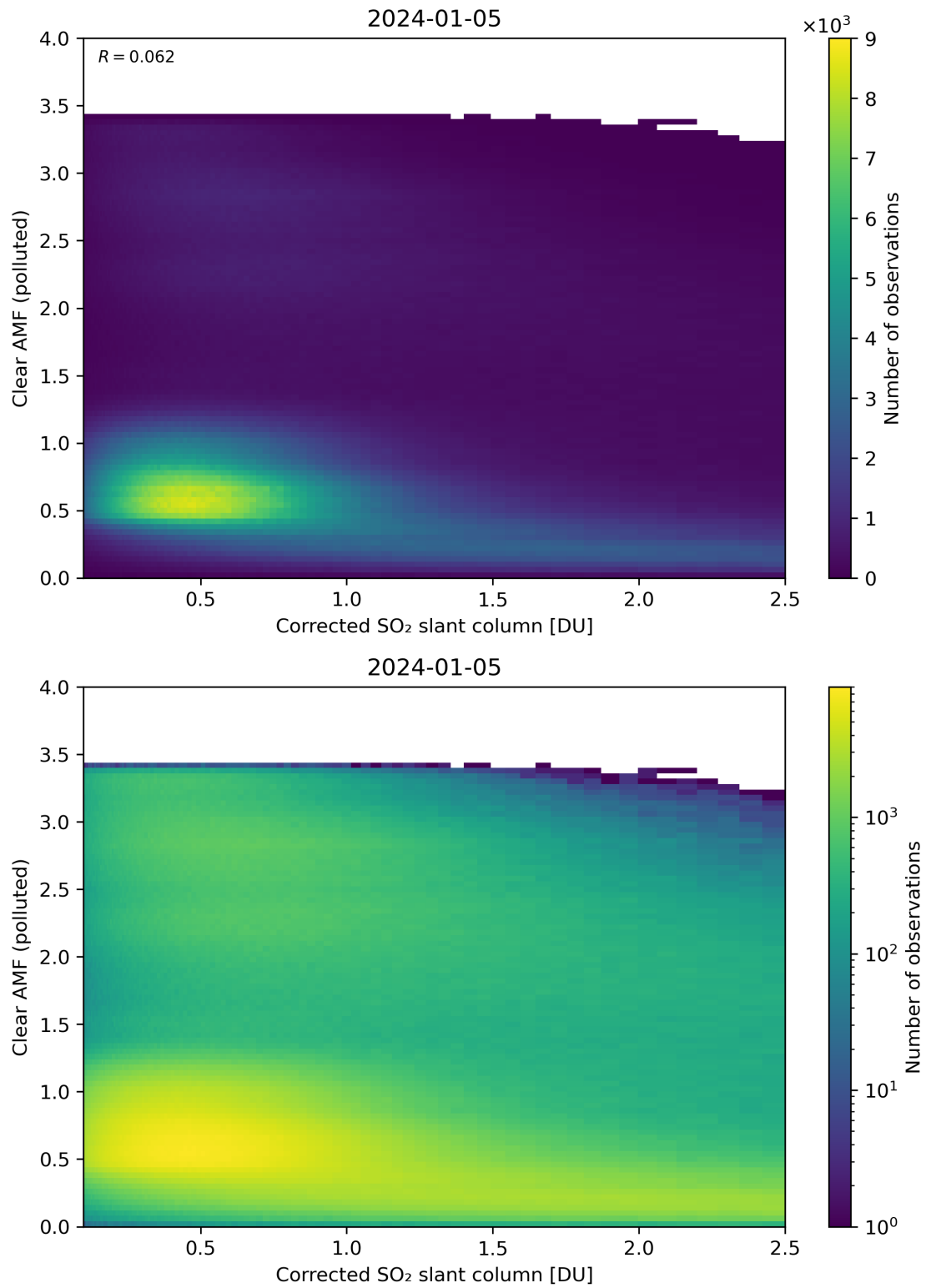
Figure 184: Scatter density plot of “Corrected SO 2 slant column” against “Clear AMF (polluted)” for 2024-01-05 to 2024-01-06.
