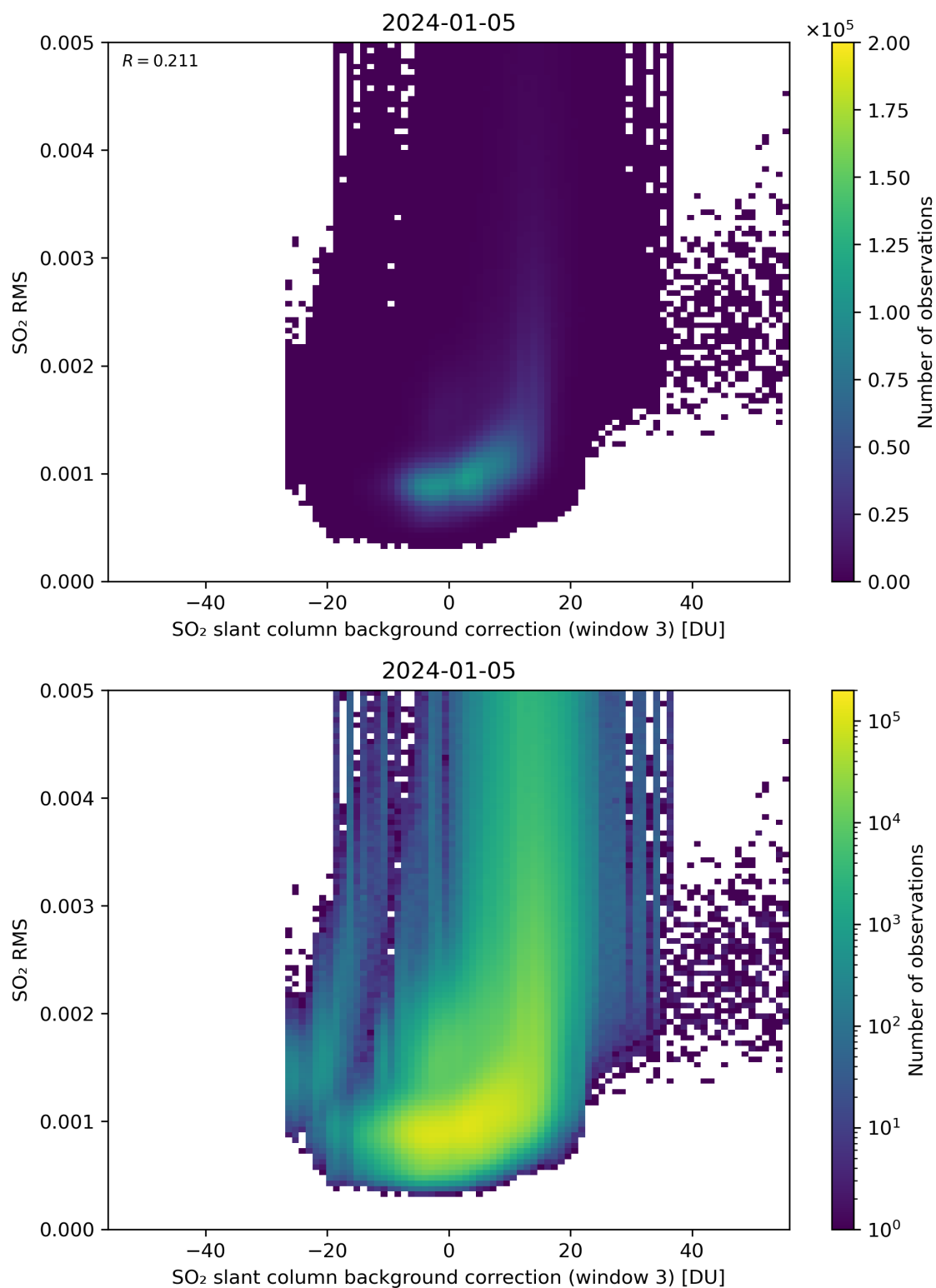
Figure 123: Scatter density plot of “SO 2 slant column background correction (window 3)” against “SO 2 RMS” for 2024-01-05 to 2024-01-06.
