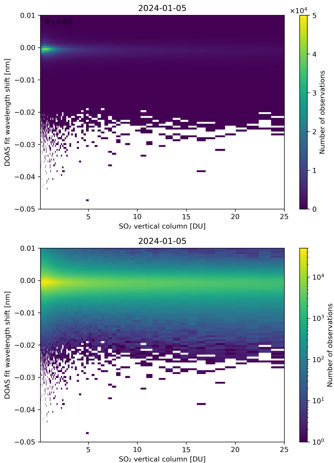
Figure 276: Scatter density plot of “SO 2 vertical column” against “DOAS fit wavelength shift” for 2024-01-05 to 2024-01-06.
