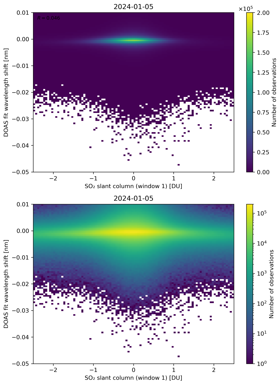
Figure 215: Scatter density plot of “SO 2 slant column (window 1)” against “DOAS fit wavelength shift” for 2024-01-05 to 2024-01-06.
