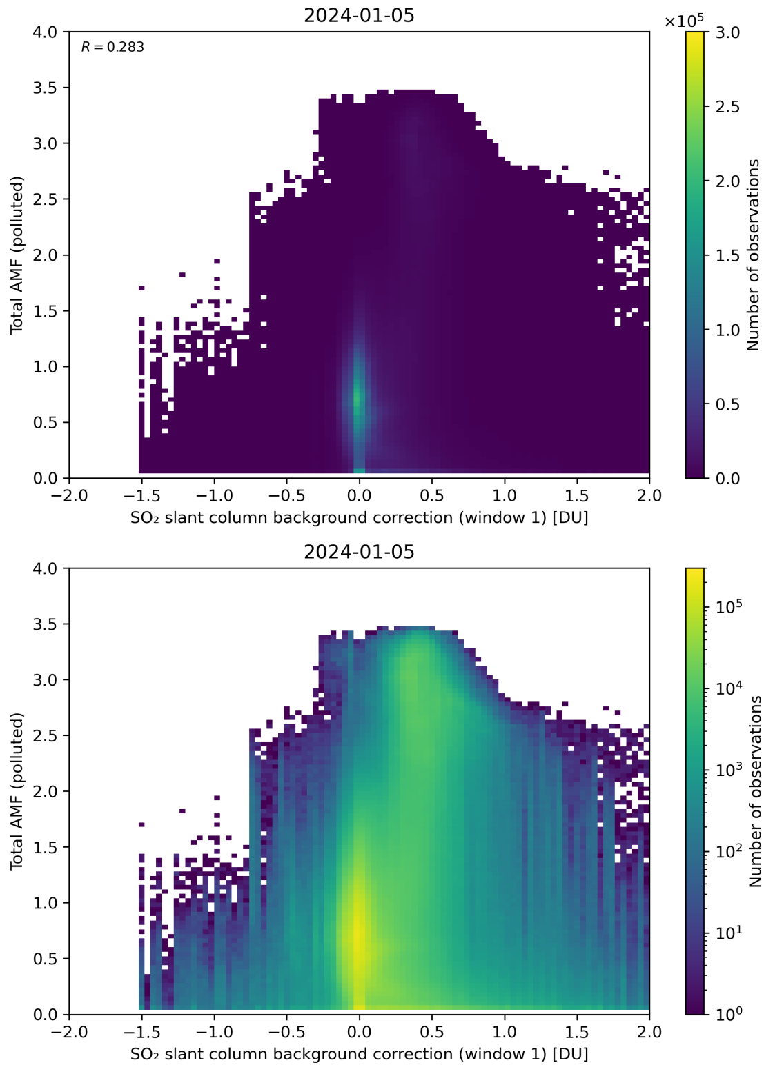
Figure 109: Scatter density plot of “SO 2 slant column background correction (window 1)” against “Total AMF (polluted)” for 2024-01-05 to 2024-01-06.
