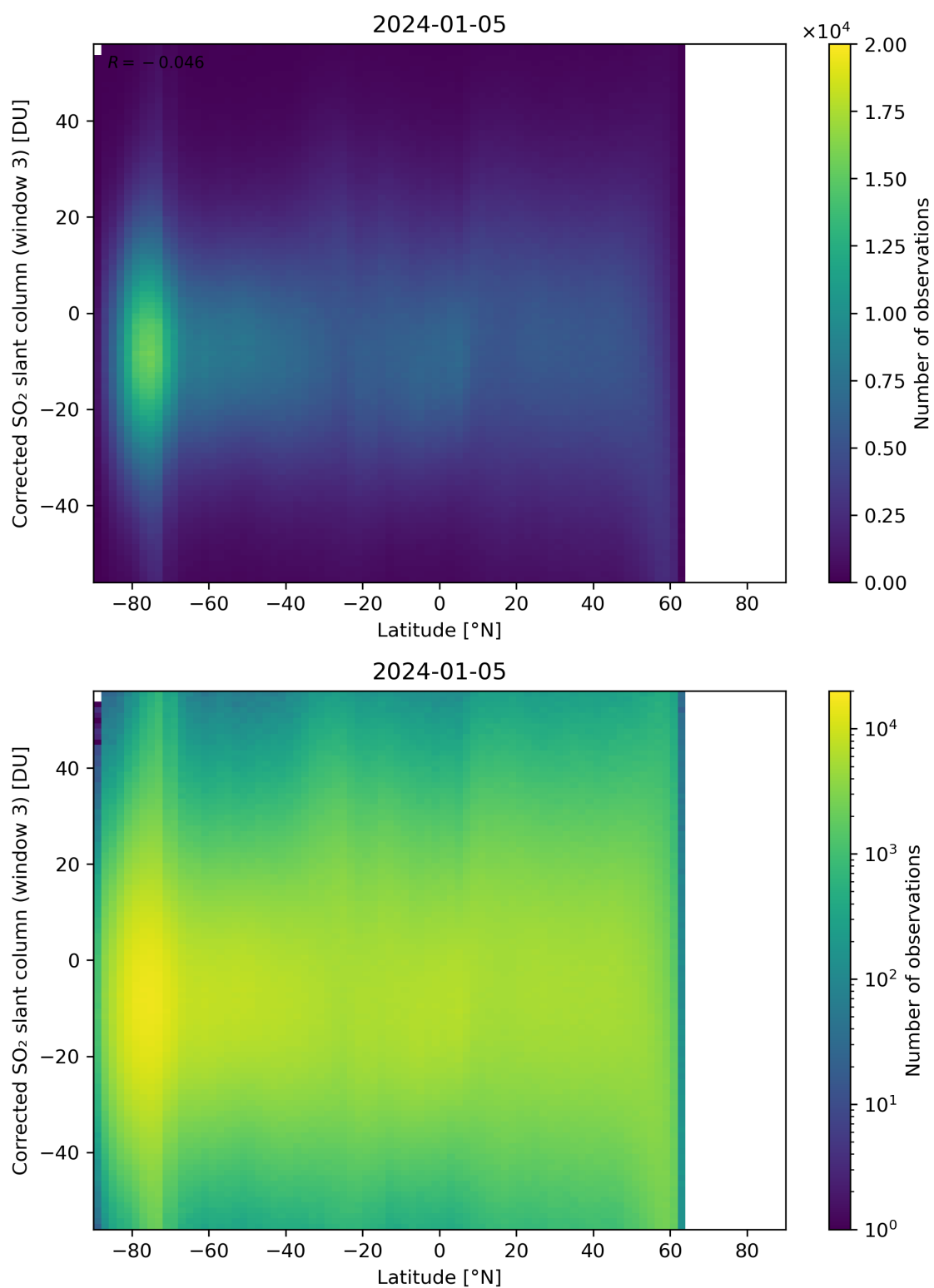
Figure 148: Scatter density plot of “Latitude” against “Corrected SO 2 slant column (window 3)” for 2024-01-05 to 2024-01-06.
