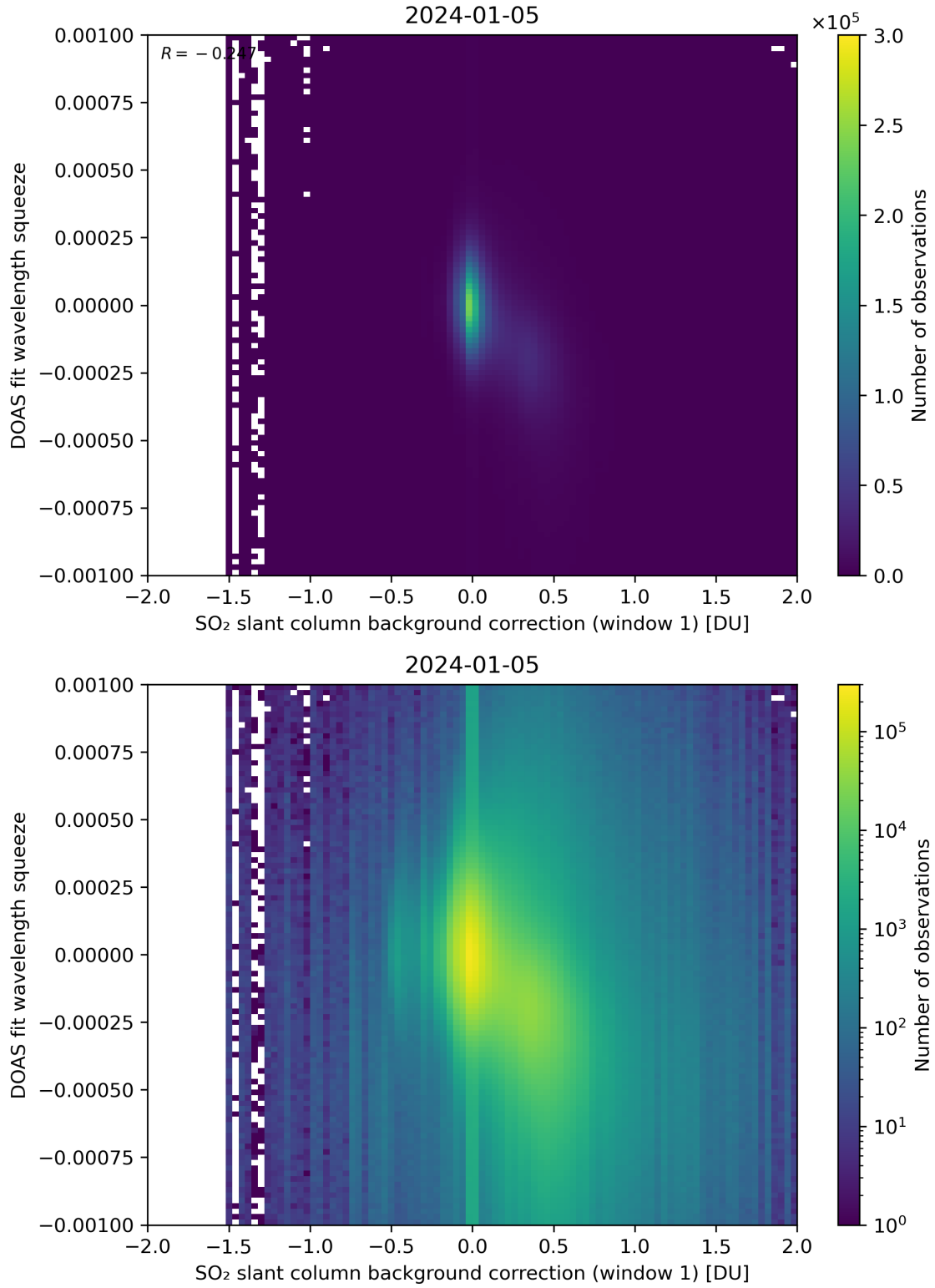
Figure 101: Scatter density plot of “SO 2 slant column background correction (window 1)” against “DOAS fit wavelength squeeze” for 2024-01-05 to 2024-01-06.
