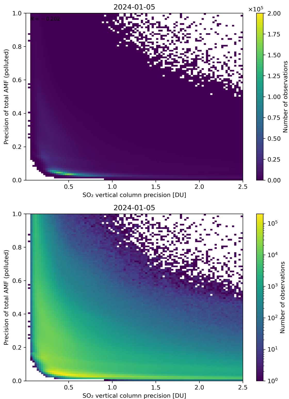
Figure 295: Scatter density plot of “SO 2 vertical column precision” against “Precision of total AMF (polluted)” for 2024-01-05 to 2024-01-06.
