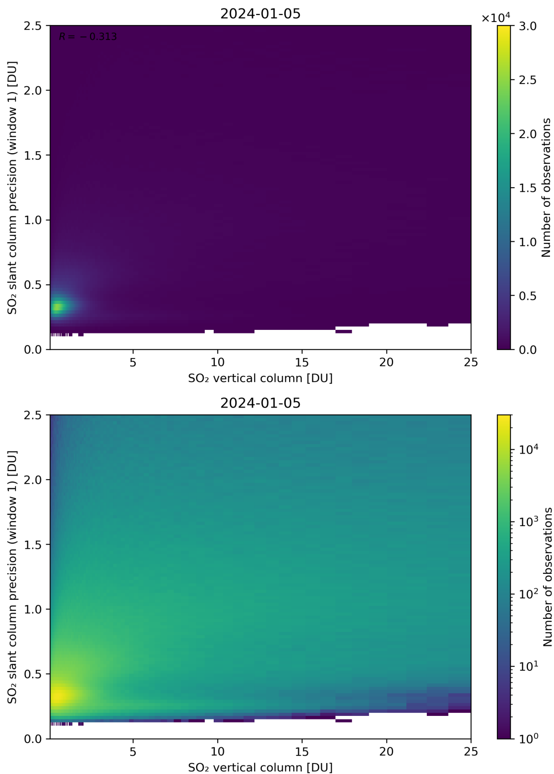
Figure 301: Scatter density plot of “SO 2 vertical column” against “SO 2 slant column precision (window 1)” for 2024-01-05 to 2024-01-06.
