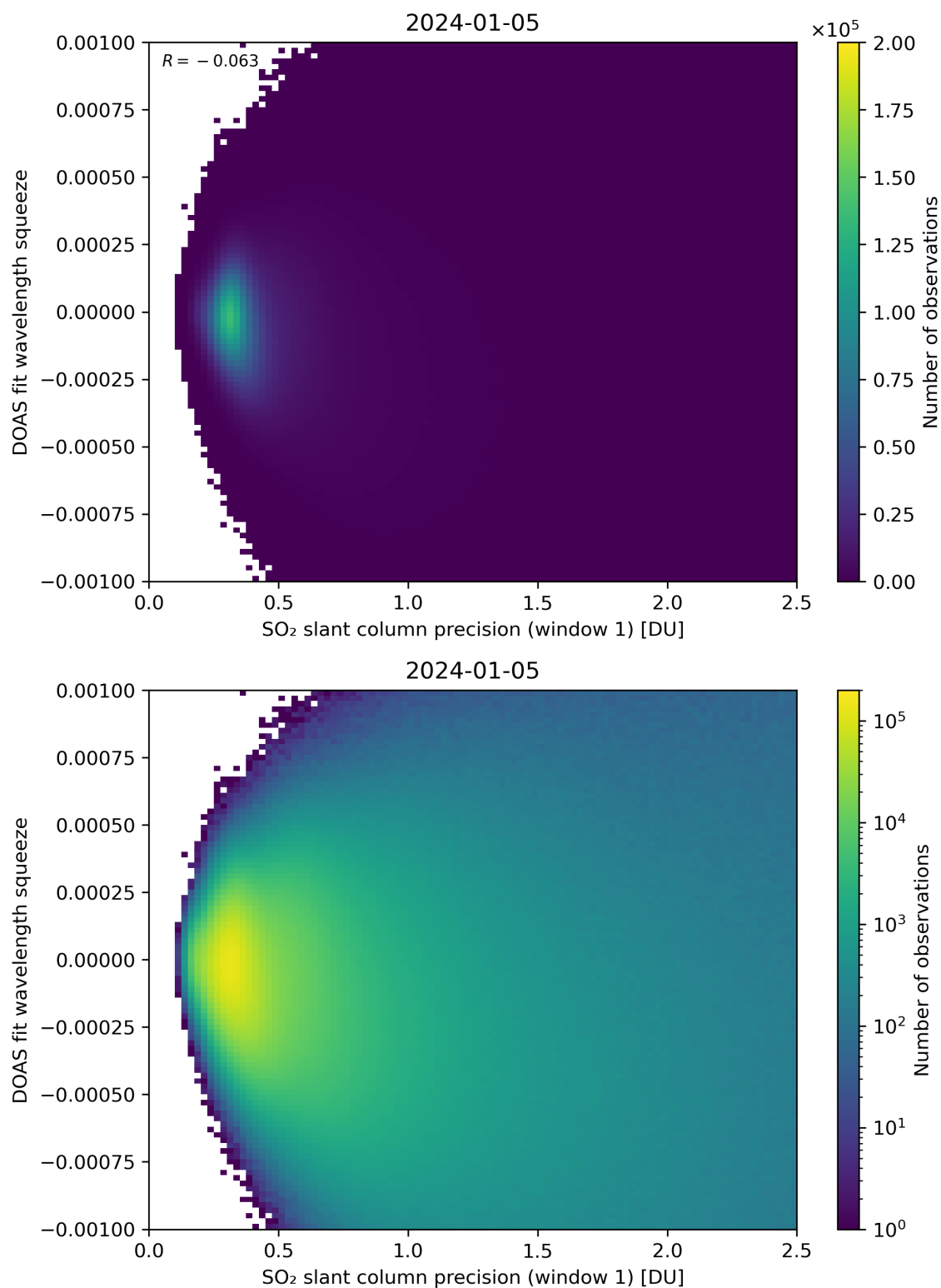
Figure 222: Scatter density plot of “SO 2 slant column precision (window 1)” against “DOAS fit wavelength squeeze” for 2024-01-05 to 2024-01-06.
