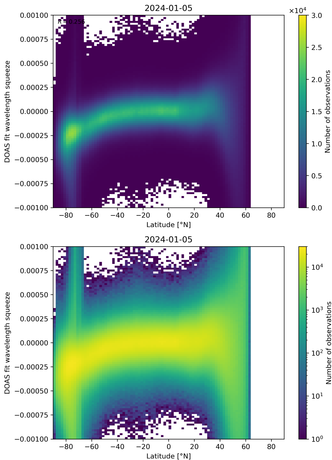
Figure 143: Scatter density plot of “Latitude” against “DOAS fit wavelength squeeze” for 2024-01-05 to 2024-01-06.
