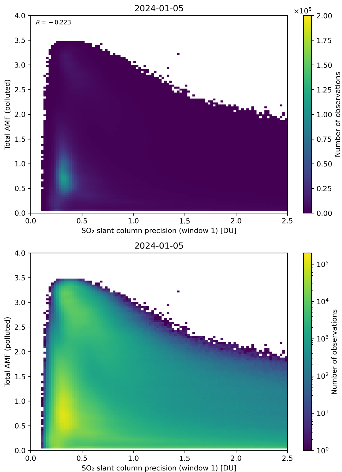
Figure 230: Scatter density plot of “SO 2 slant column precision (window 1)” against “Total AMF (polluted)” for 2024-01-05 to 2024-01-06.
