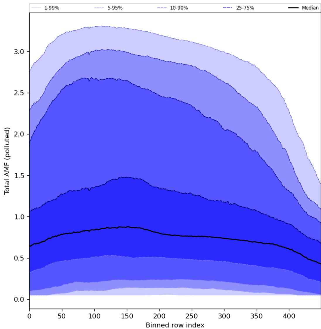
Figure 94: Along track statistics of “Total AMF (polluted)” for 2024-01-05 to 2024-01-06
