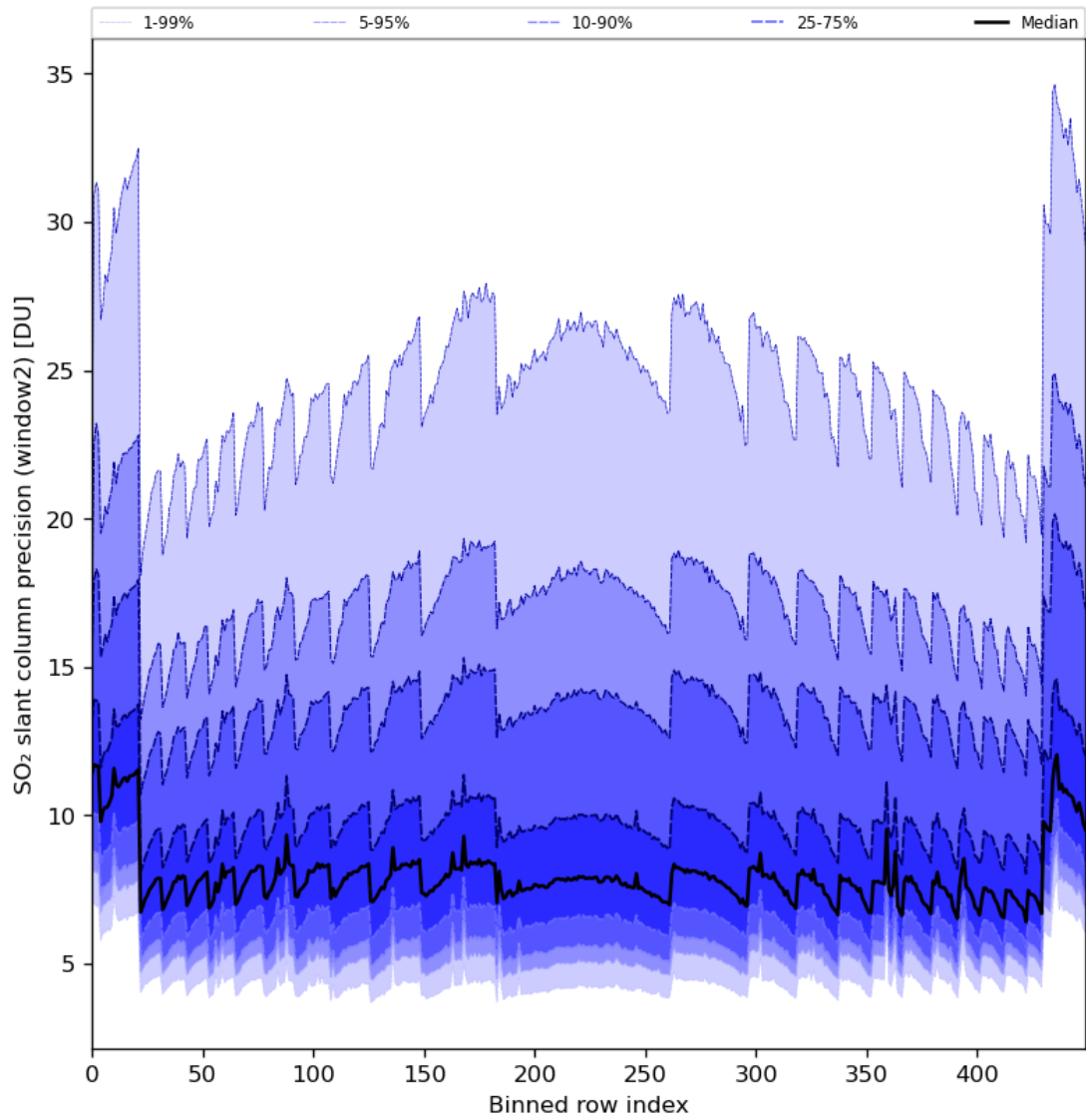
Figure 84: Along track statistics of “SO 2 slant column precision (window2)” for 2024-01-05 to 2024-01-06
