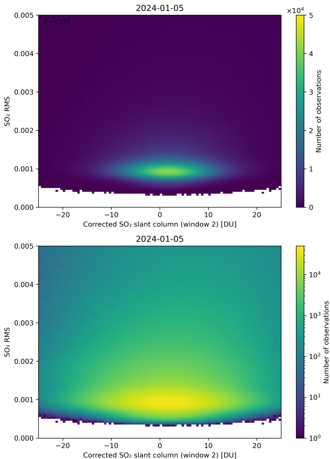
Figure 198: Scatter density plot of “Corrected SO 2 slant column (window 2)” against “SO 2 RMS” for 2024-01-05 to 2024-01-06.
