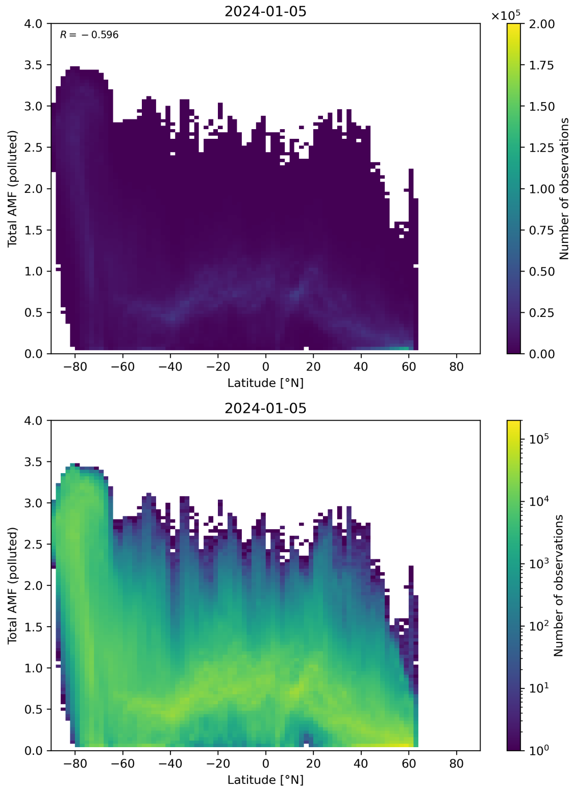
Figure 154: Scatter density plot of “Latitude” against “Total AMF (polluted)” for 2024-01-05 to 2024-01-06.
