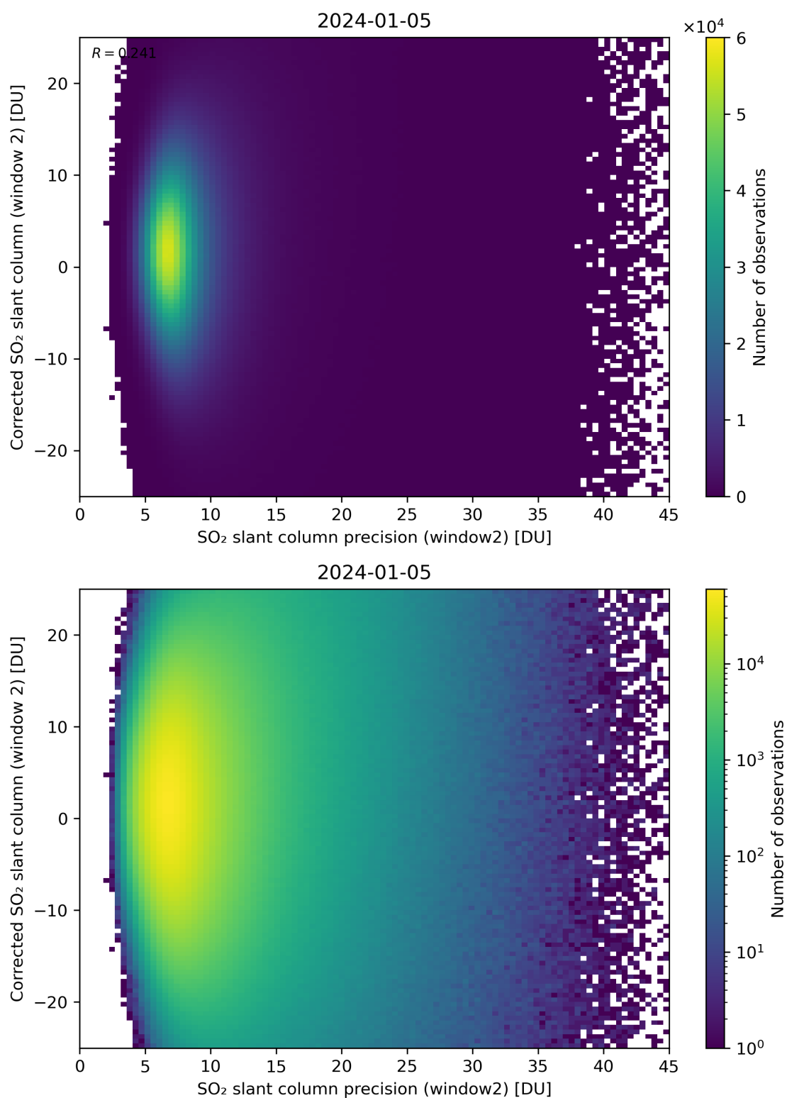
Figure 247: Scatter density plot of “SO 2 slant column precision (window2)” against “Corrected SO 2 slant column (window 2)” for 2024-01-05 to 2024-01-06.
