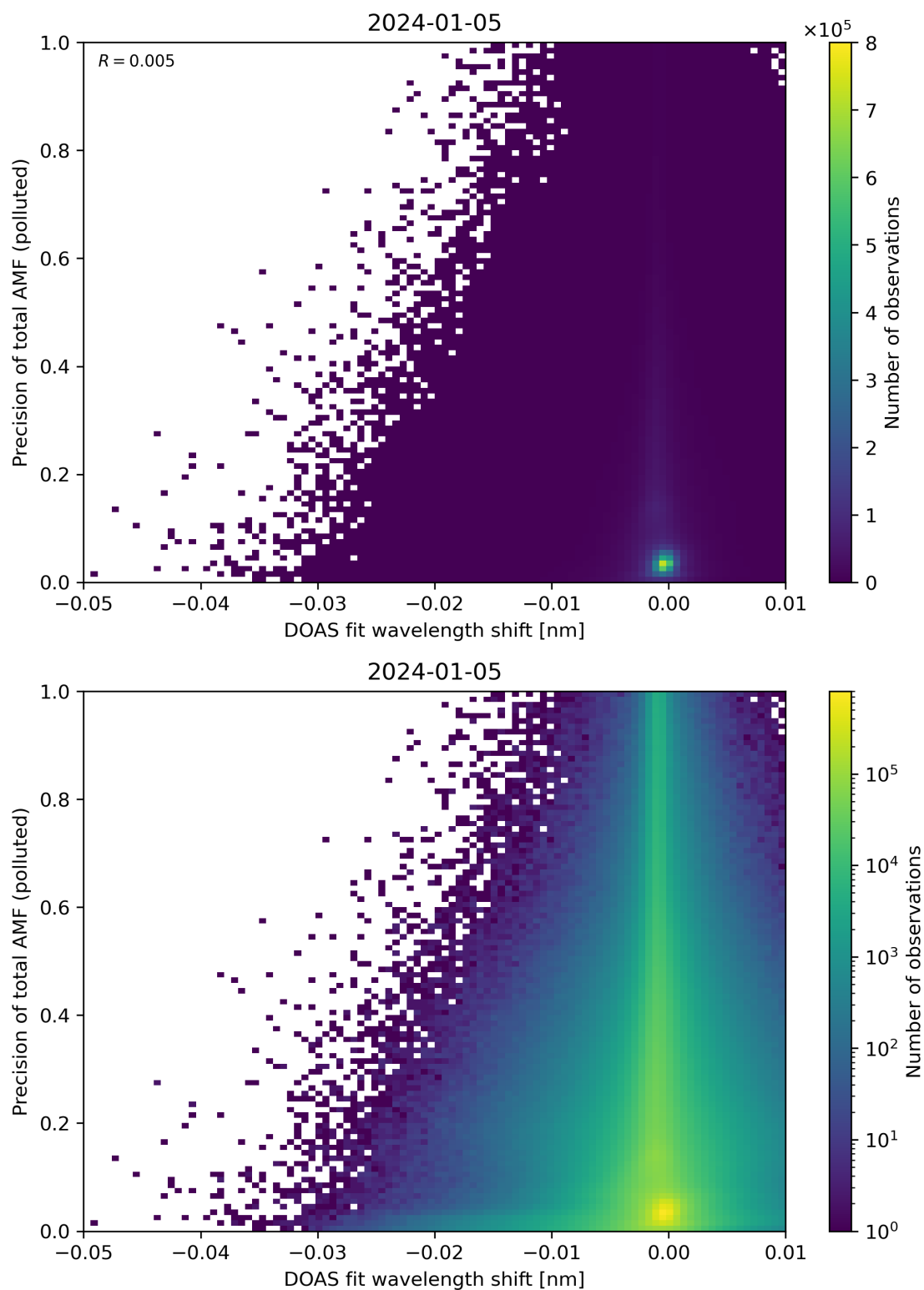
Figure 131: Scatter density plot of “DOAS fit wavelength shift” against “Precision of total AMF (polluted)” for 2024-01-05 to 2024-01-06.
