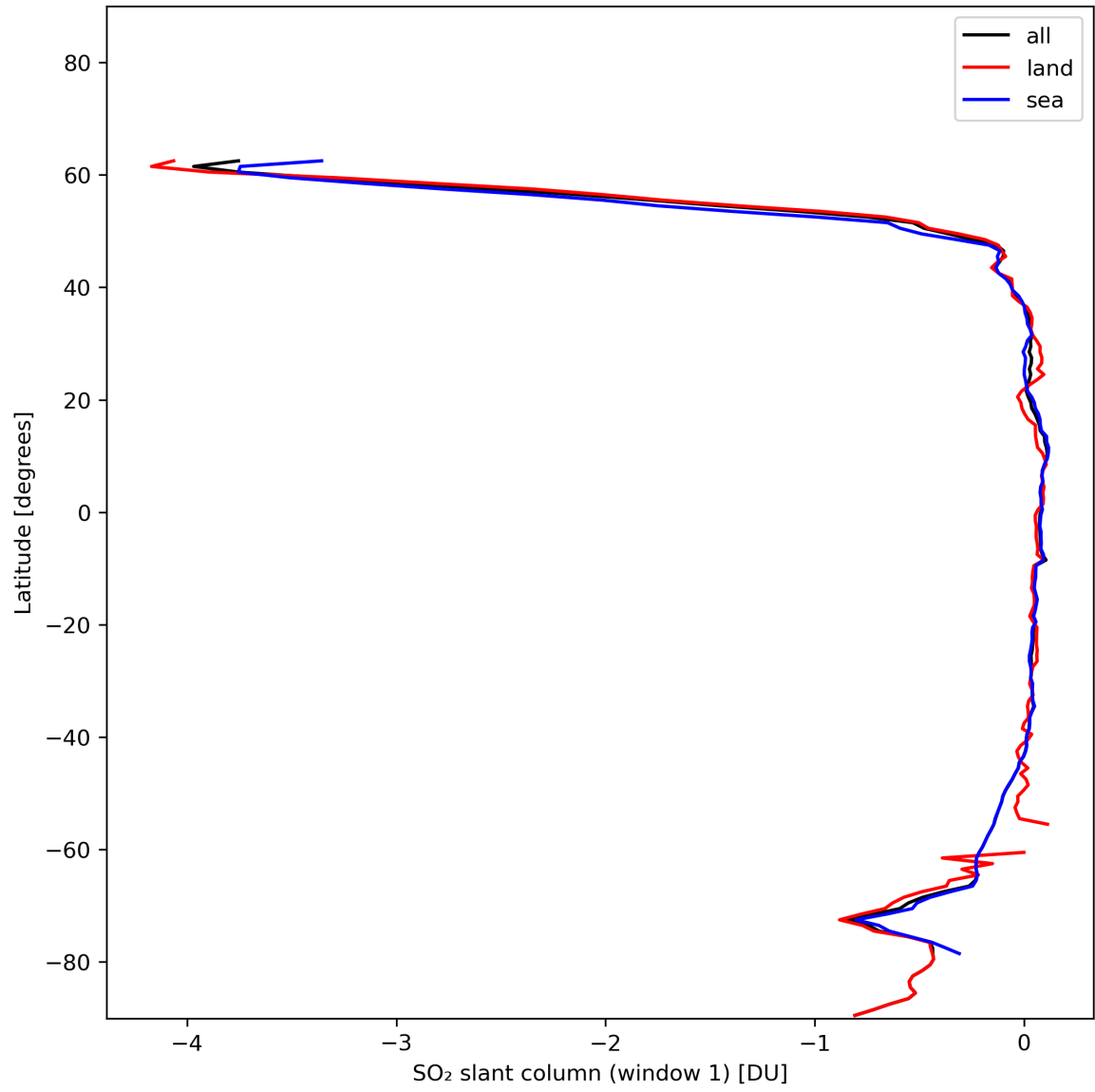
Figure 33: Zonal average of “SO 2 slant column (window 1)” for 2024-01-05 to 2024-01-06.
