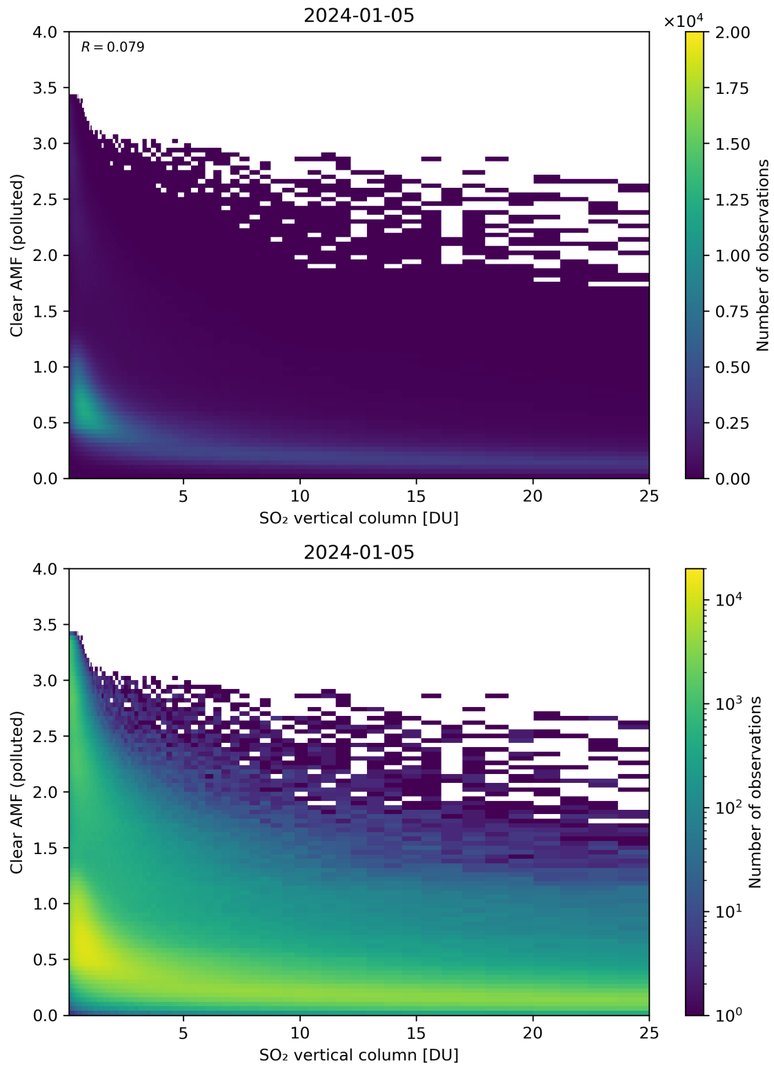
Figure 296: Scatter density plot of “SO 2 vertical column” against “Clear AMF (polluted)” for 2024-01-05 to 2024-01-06.
