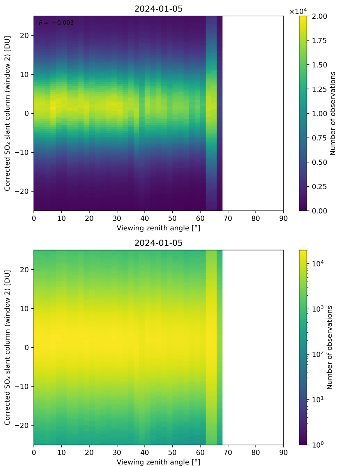
Figure 318: Scatter density plot of “Viewing zenith angle” against “Corrected SO 2 slant column (window 2)” for 2024-01-05 to 2024-01-06.
