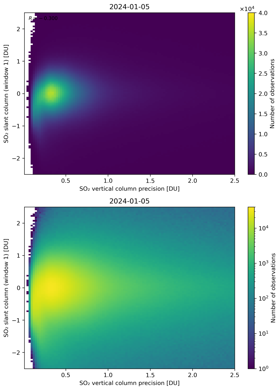
Figure 289: Scatter density plot of “SO 2 vertical column precision” against “SO 2 slant column (window 1)” for 2024-01-05 to 2024-01-06.
