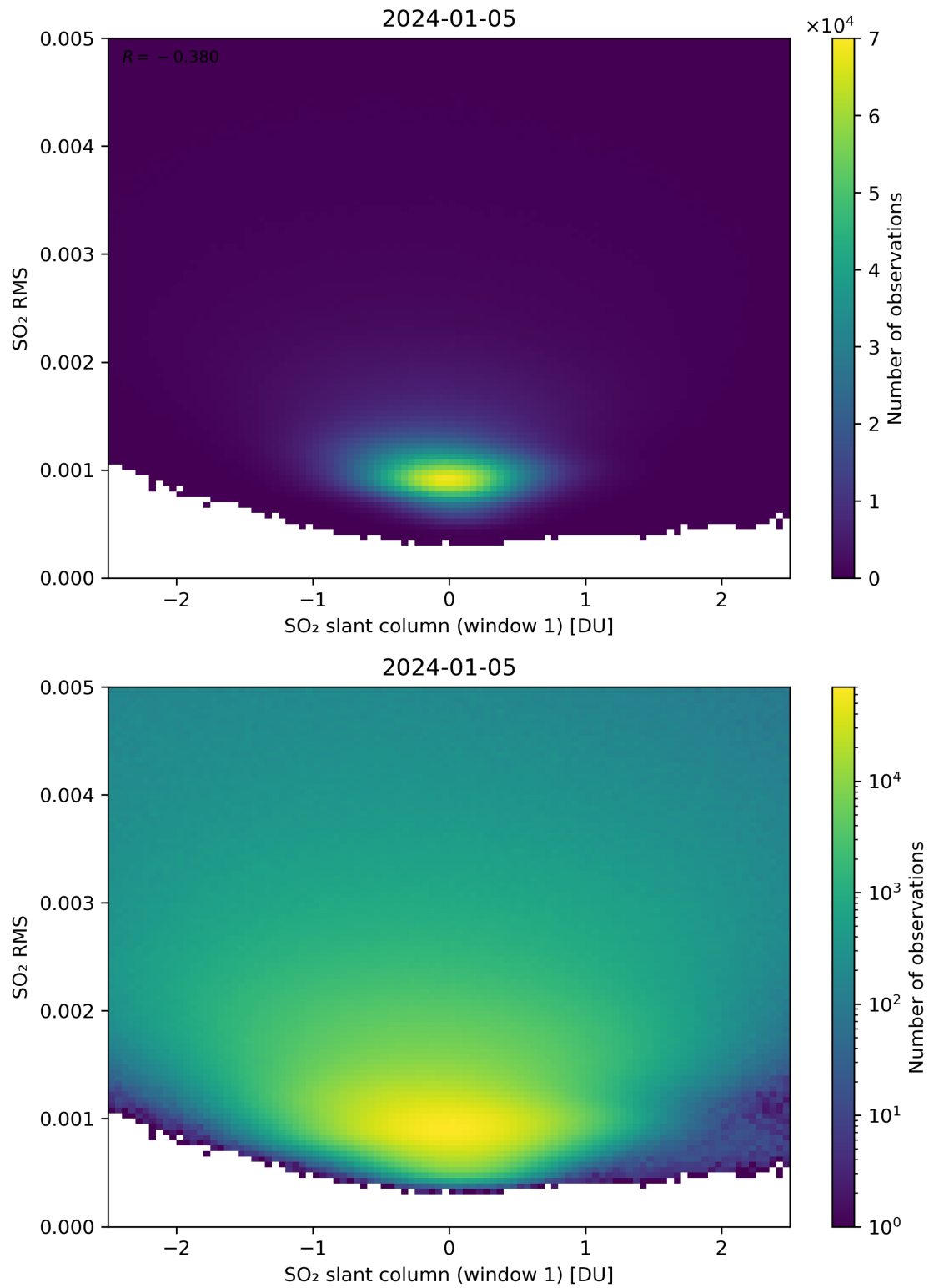
Figure 217: Scatter density plot of “SO 2 slant column (window 1)” against “SO 2 RMS” for 2024-01-05 to 2024-01-06.
