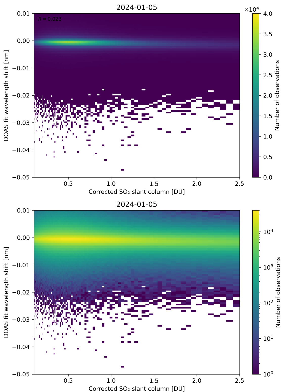
Figure 181: Scatter density plot of “Corrected SO 2 slant column” against “DOAS fit wavelength shift” for 2024-01-05 to 2024-01-06.
