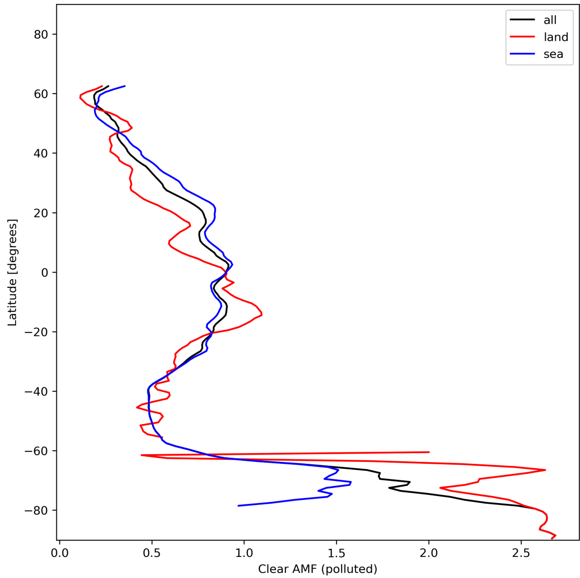
Figure 50: Zonal average of “Clear AMF (polluted)” for 2024-01-05 to 2024-01-06.
