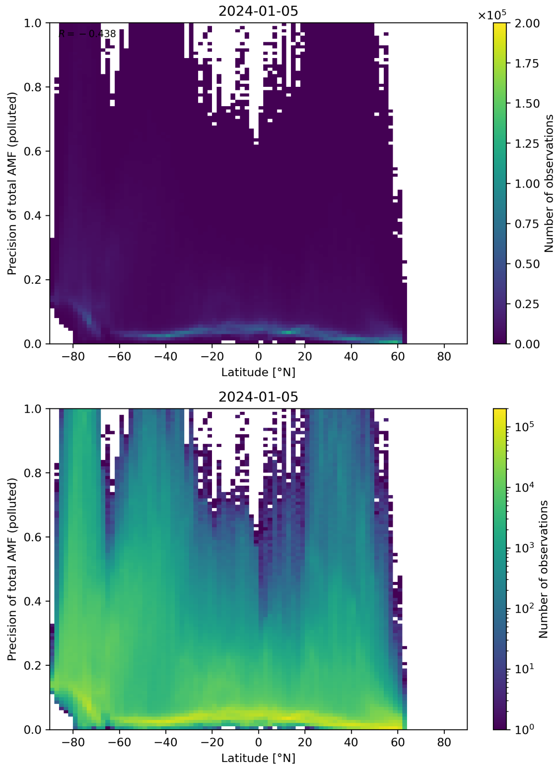
Figure 155: Scatter density plot of “Latitude” against “Precision of total AMF (polluted)” for 2024-01-05 to 2024-01-06.
