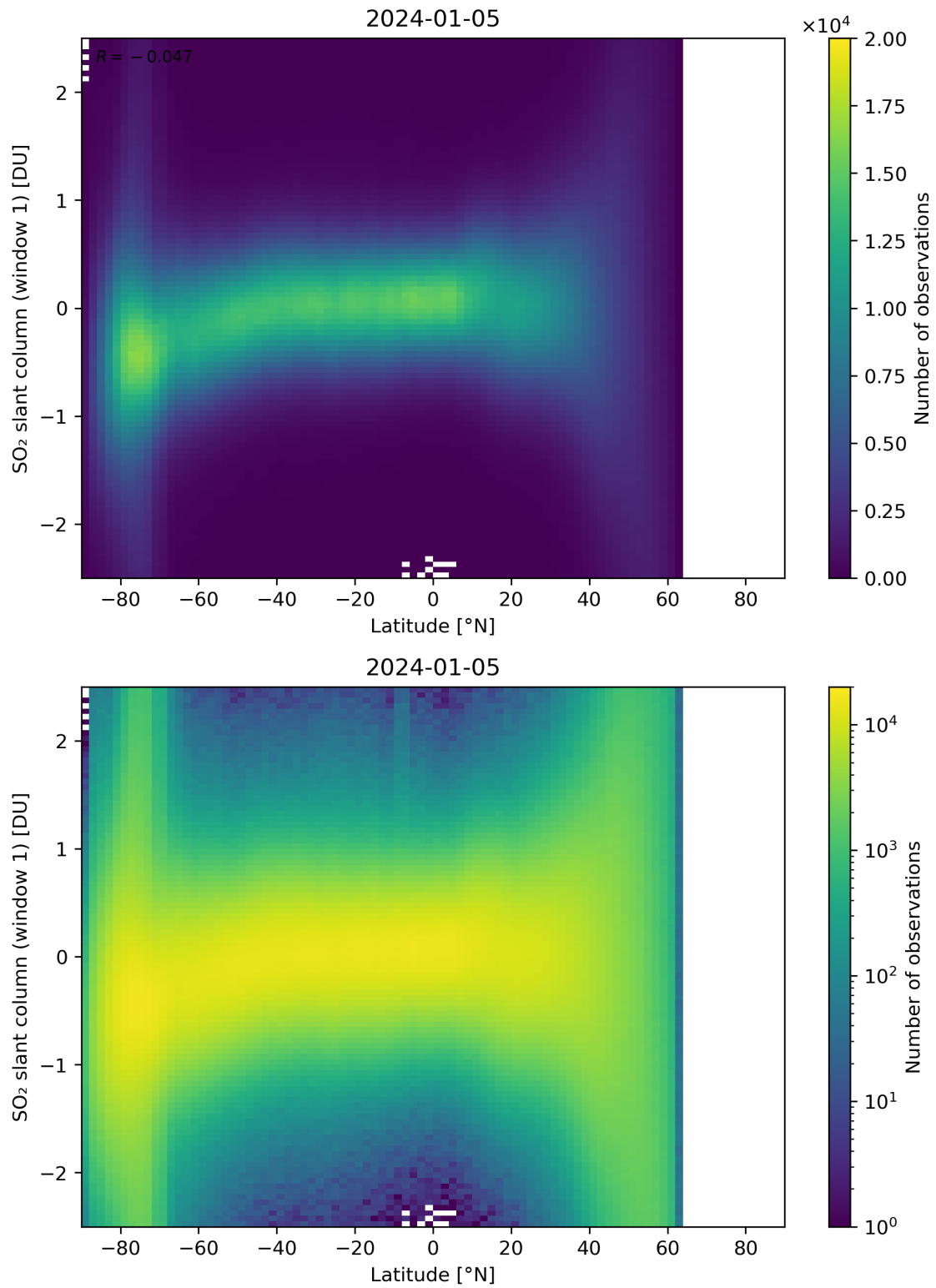
Figure 149: Scatter density plot of “Latitude” against “SO 2 slant column (window 1)” for 2024-01-05 to 2024-01-06.
