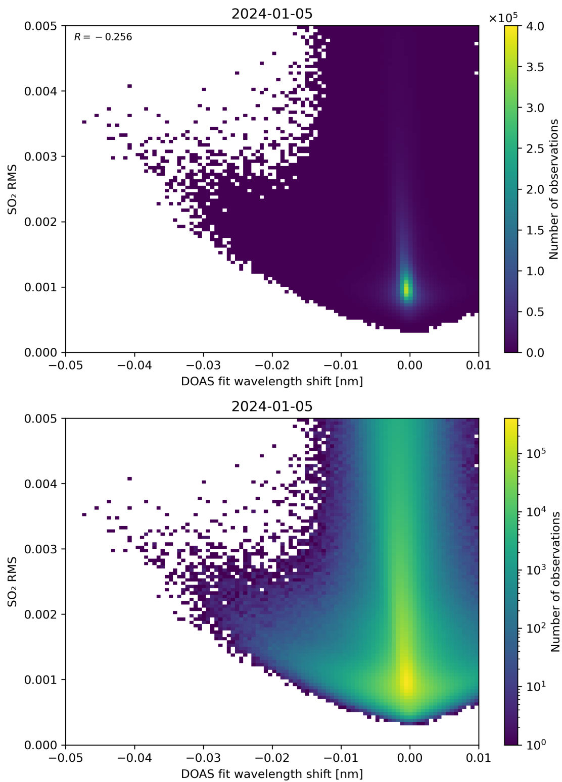
Figure 128: Scatter density plot of “DOAS fit wavelength shift” against “SO 2 RMS” for 2024-01-05 to 2024-01-06.
