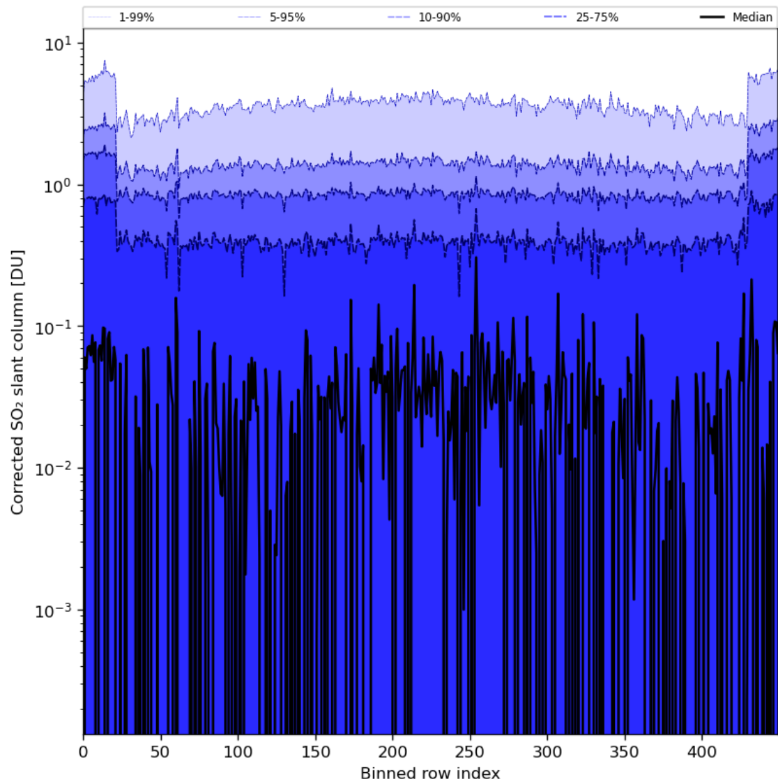
Figure 78: Along track statistics of “Corrected SO 2 slant column” for 2024-01-05 to 2024-01-06
