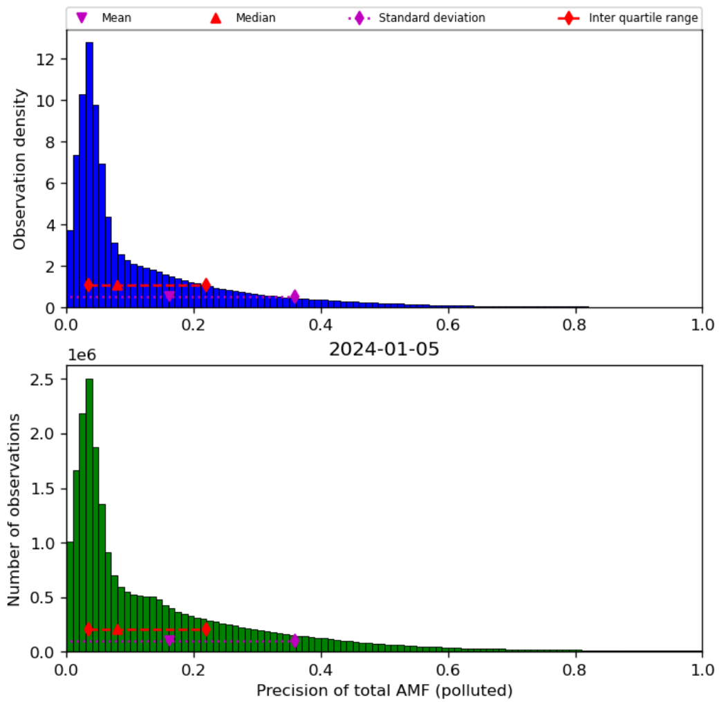
Figure 72: Histogram of “Precision of total AMF (polluted)” for 2024-01-05 to 2024-01-06
