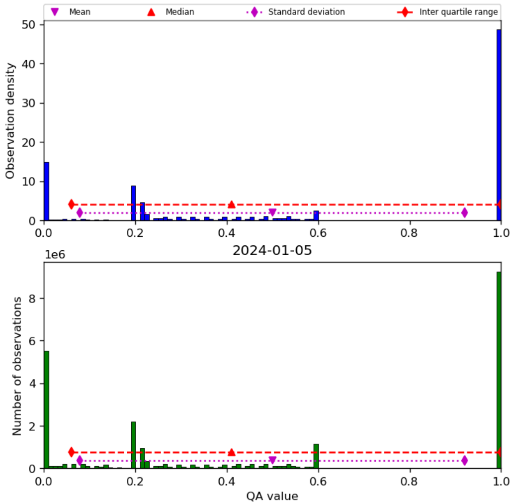
Figure 52: Histogram of “QA value” for 2024-01-05 to 2024-01-06
