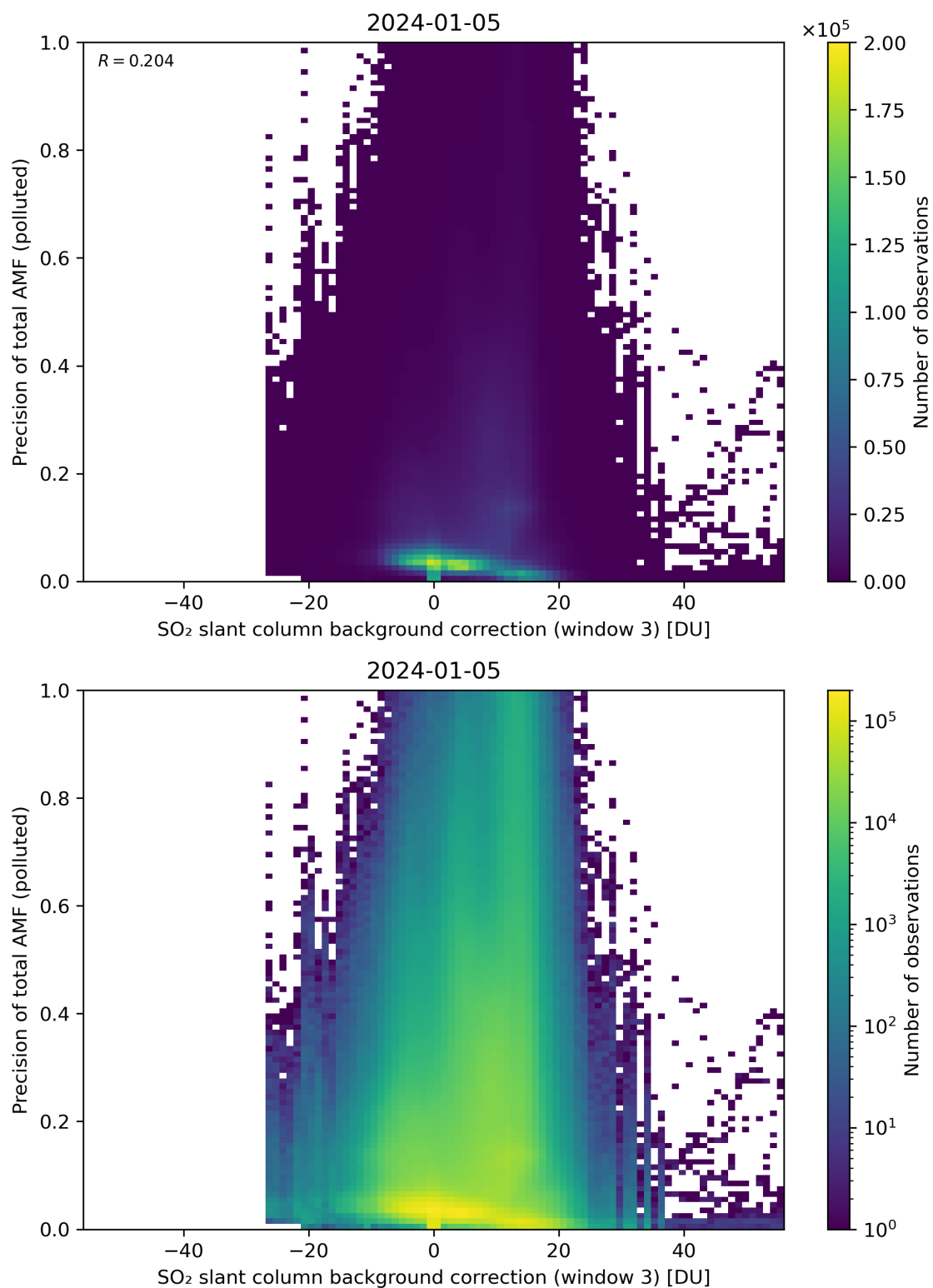
Figure 126: Scatter density plot of “SO 2 slant column background correction (window 3)” against “Precision of total AMF (polluted)” for 2024-01-05 to 2024-01-06.
