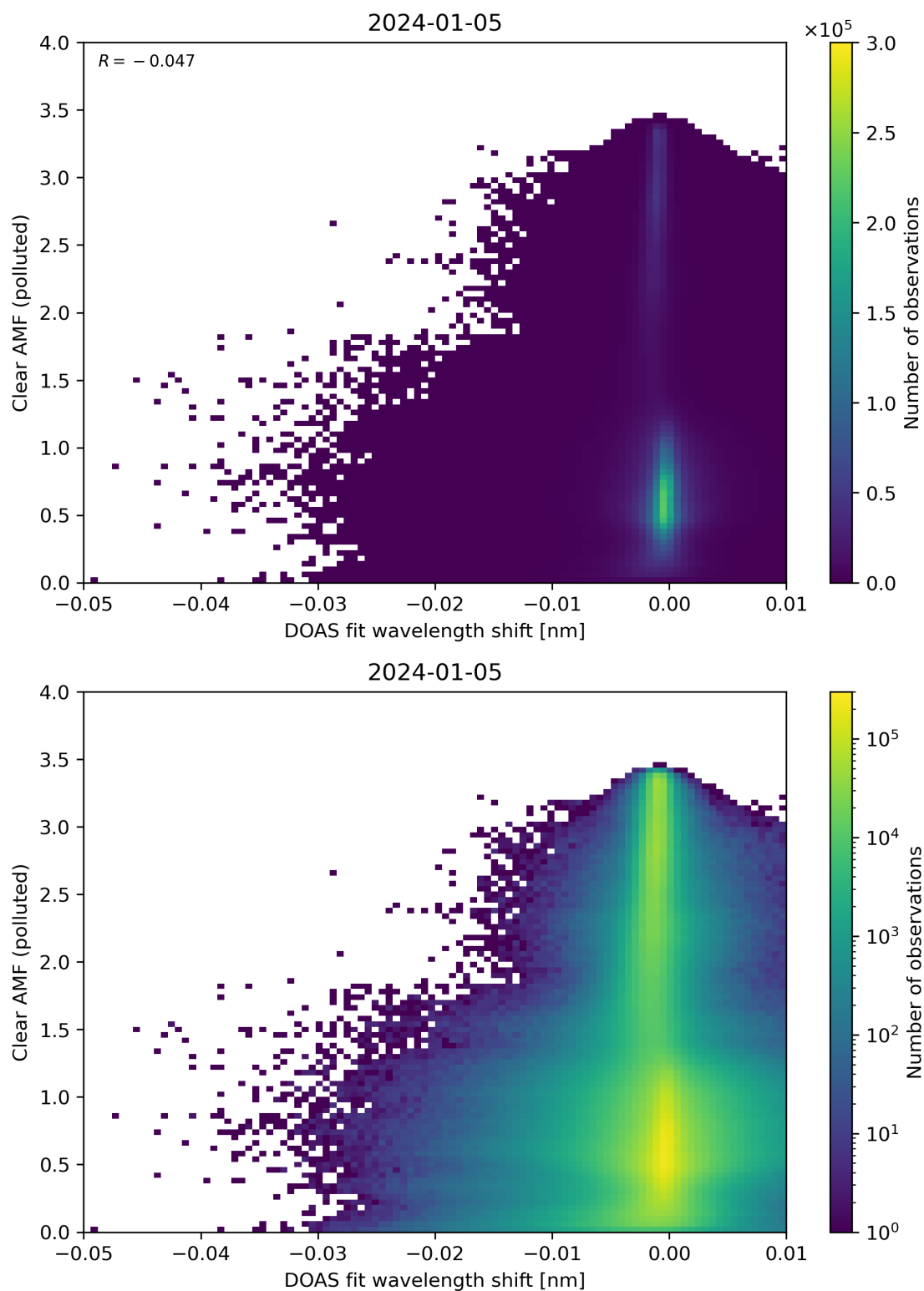
Figure 129: Scatter density plot of “DOAS fit wavelength shift” against “Clear AMF (polluted)” for 2024-01-05 to 2024-01-06.
