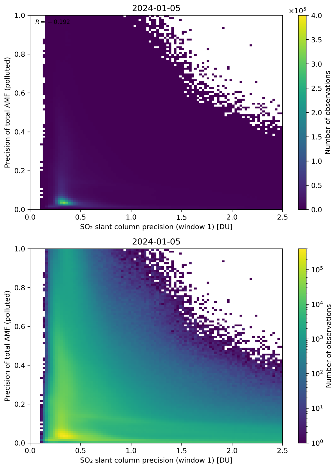
Figure 231: Scatter density plot of “SO 2 slant column precision (window 1)” against “Precision of total AMF (polluted)” for 2024-01-05 to 2024-01-06.
