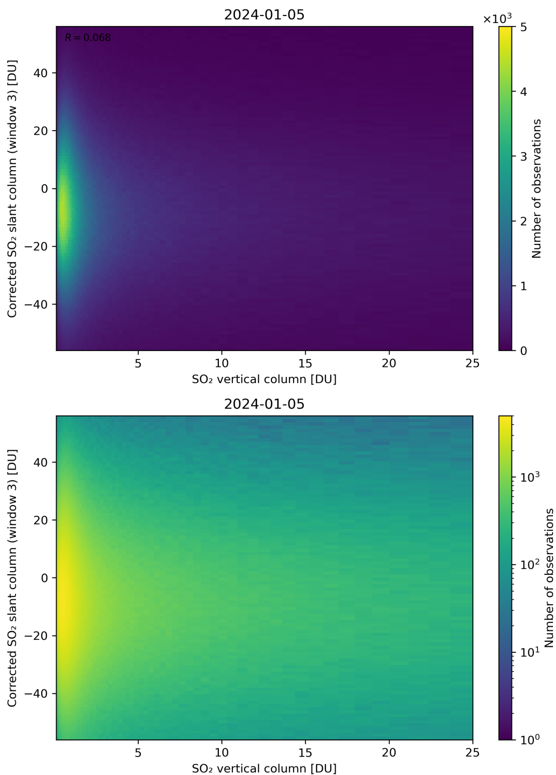
Figure 299: Scatter density plot of “SO 2 vertical column” against “Corrected SO 2 slant column (window 3)” for 2024-01-05 to 2024-01-06.
