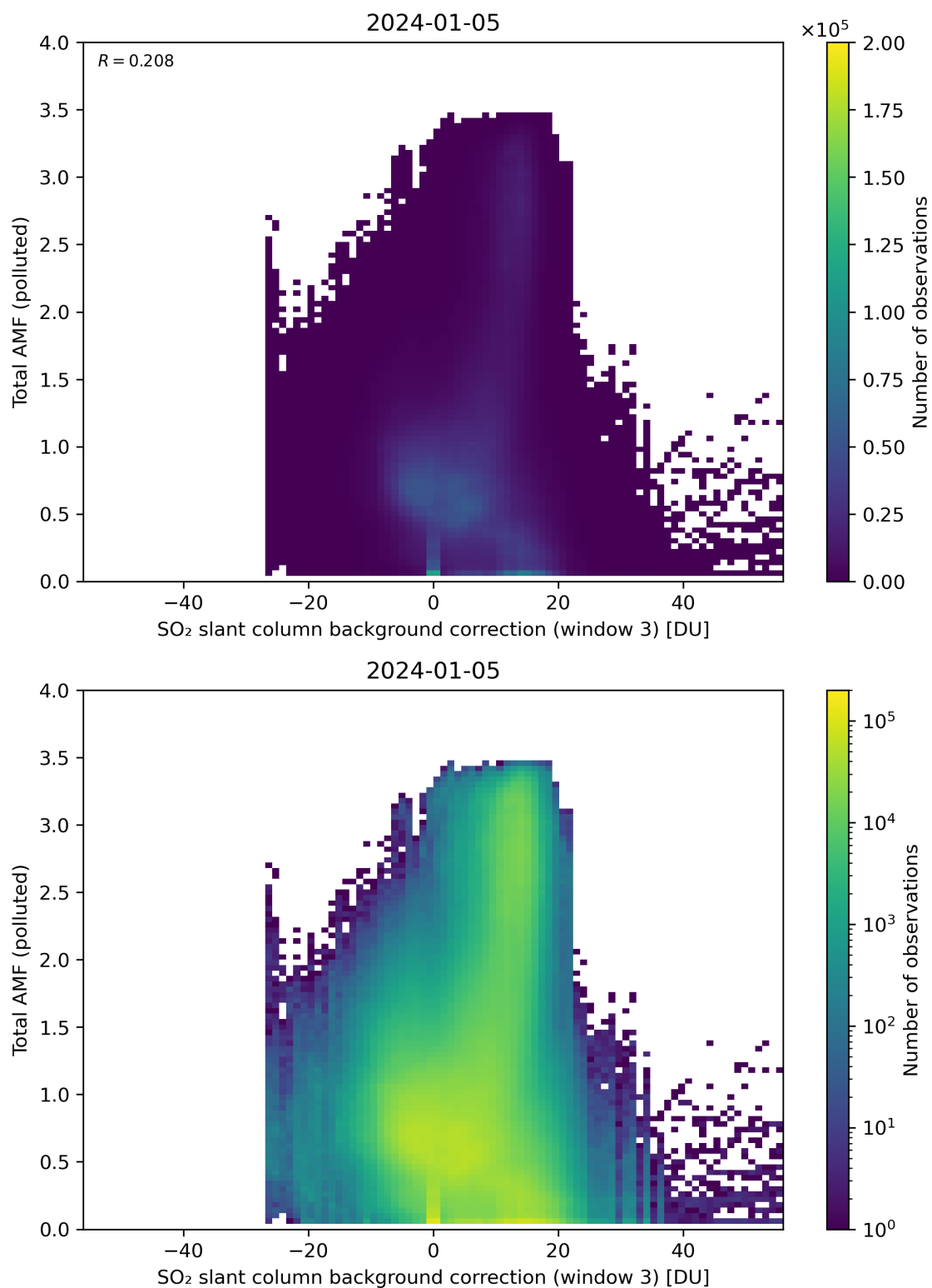
Figure 125: Scatter density plot of “SO 2 slant column background correction (window 3)” against “Total AMF (polluted)” for 2024-01-05 to 2024-01-06.
