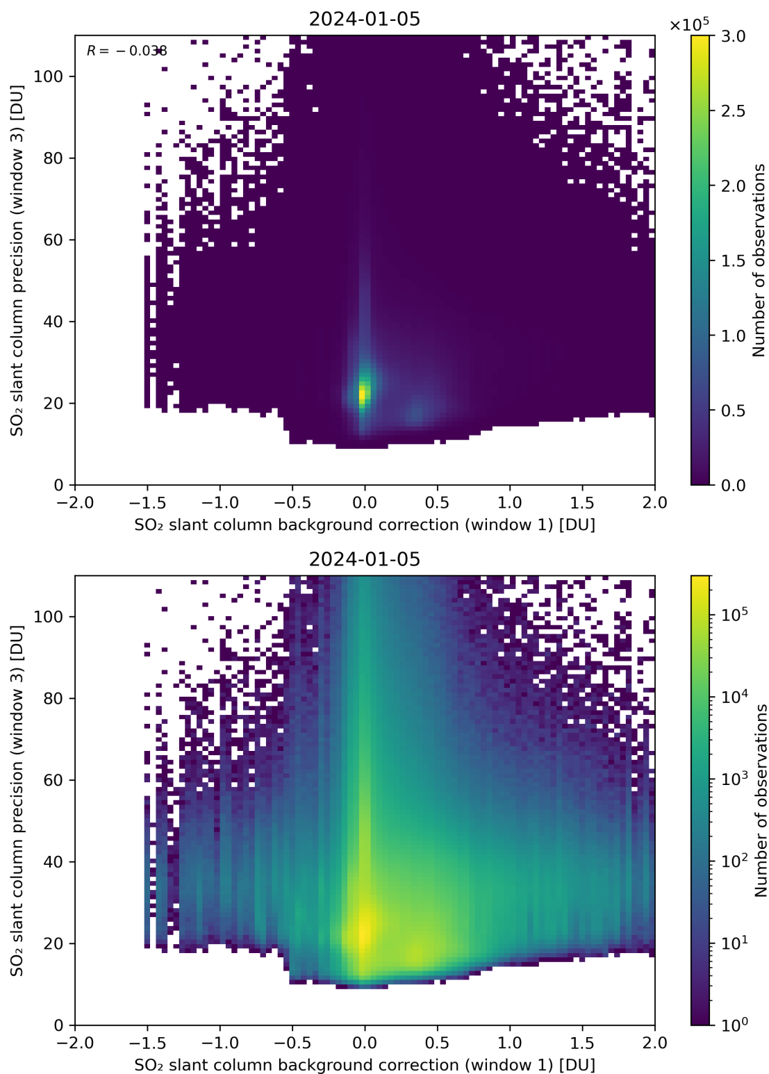
Figure 108: Scatter density plot of “SO 2 slant column background correction (window 1)” against “SO 2 slant column precision (window 3)” for 2024-01-05 to 2024-01-06.
