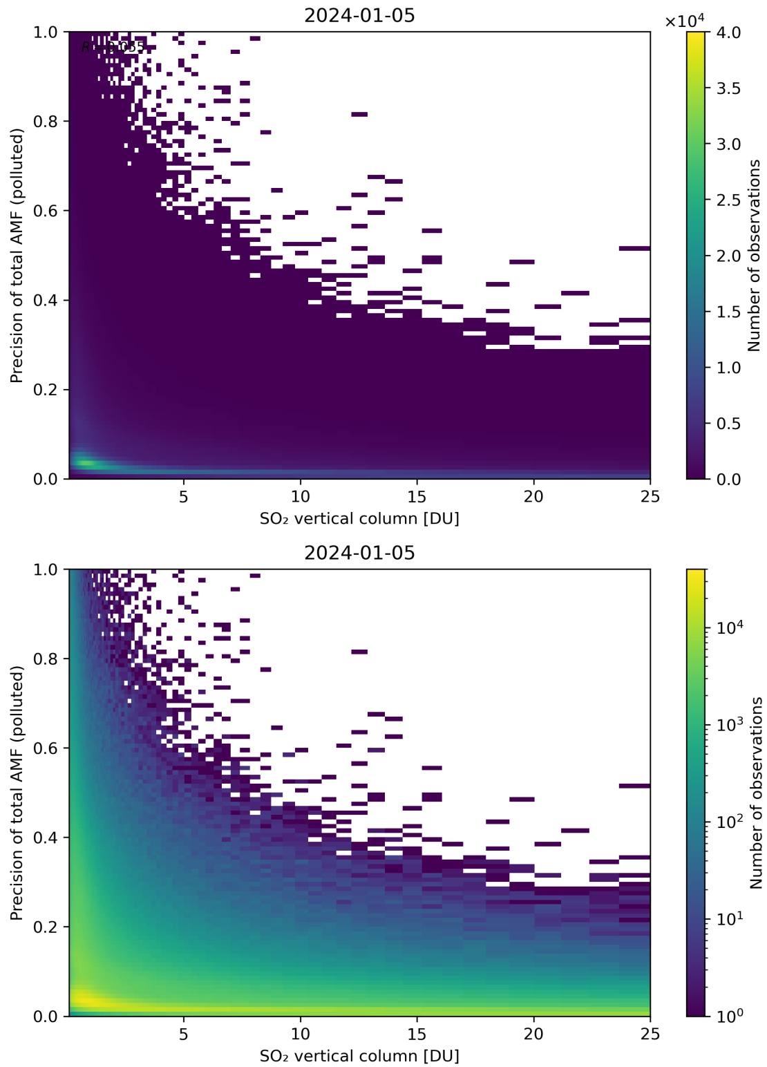
Figure 306: Scatter density plot of “SO 2 vertical column” against “Precision of total AMF (polluted)” for 2024-01-05 to 2024-01-06.
