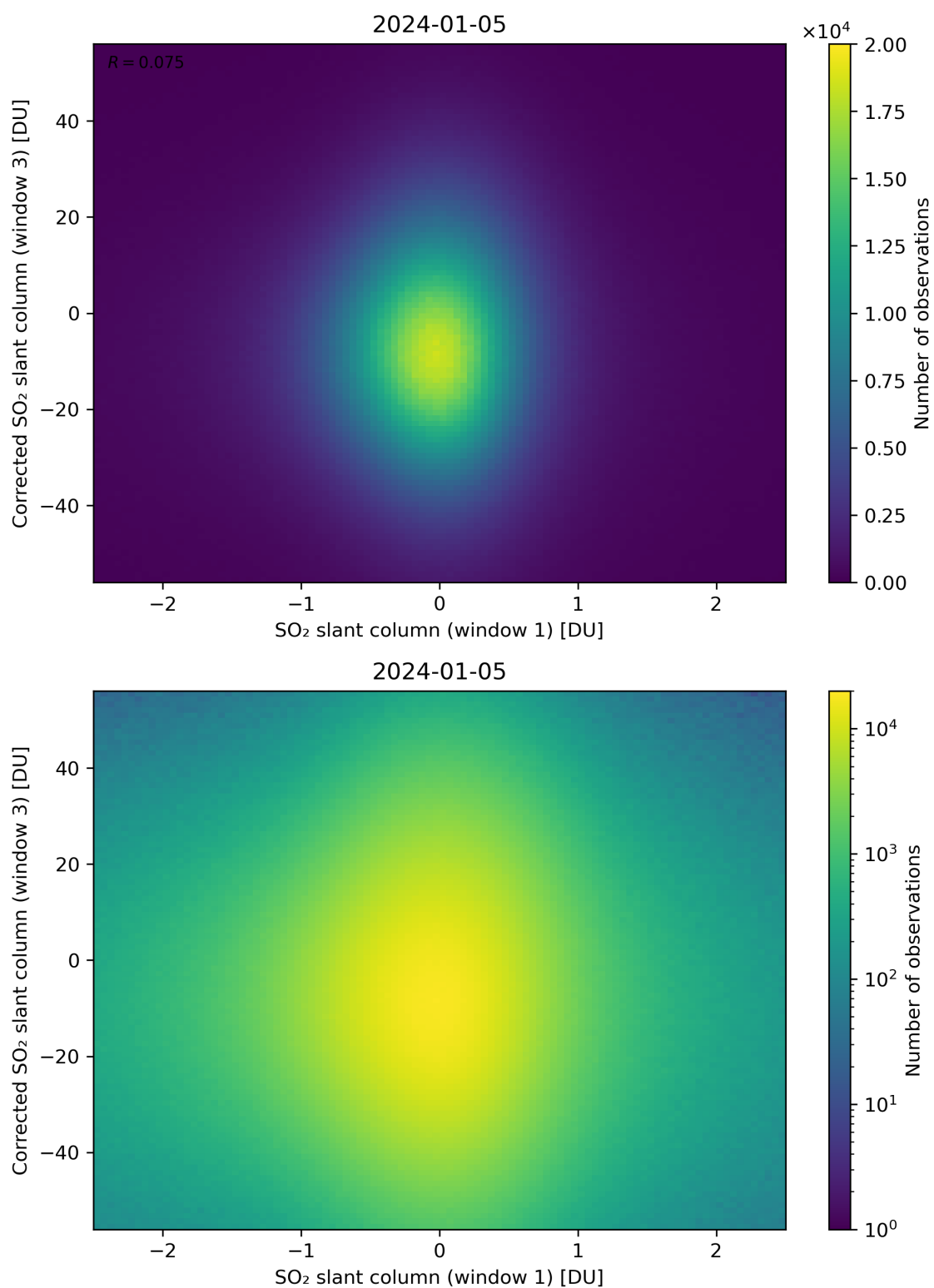
Figure 234: Scatter density plot of “SO 2 slant column (window 1)” against “Corrected SO 2 slant column (window 3)” for 2024-01-05 to 2024-01-06.
