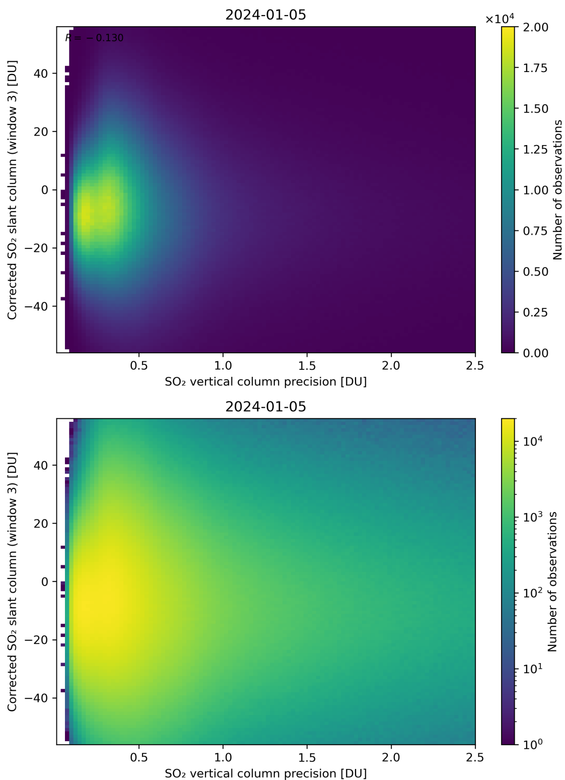
Figure 288: Scatter density plot of “SO 2 vertical column precision” against “Corrected SO 2 slant column (window 3)” for 2024-01-05 to 2024-01-06.
