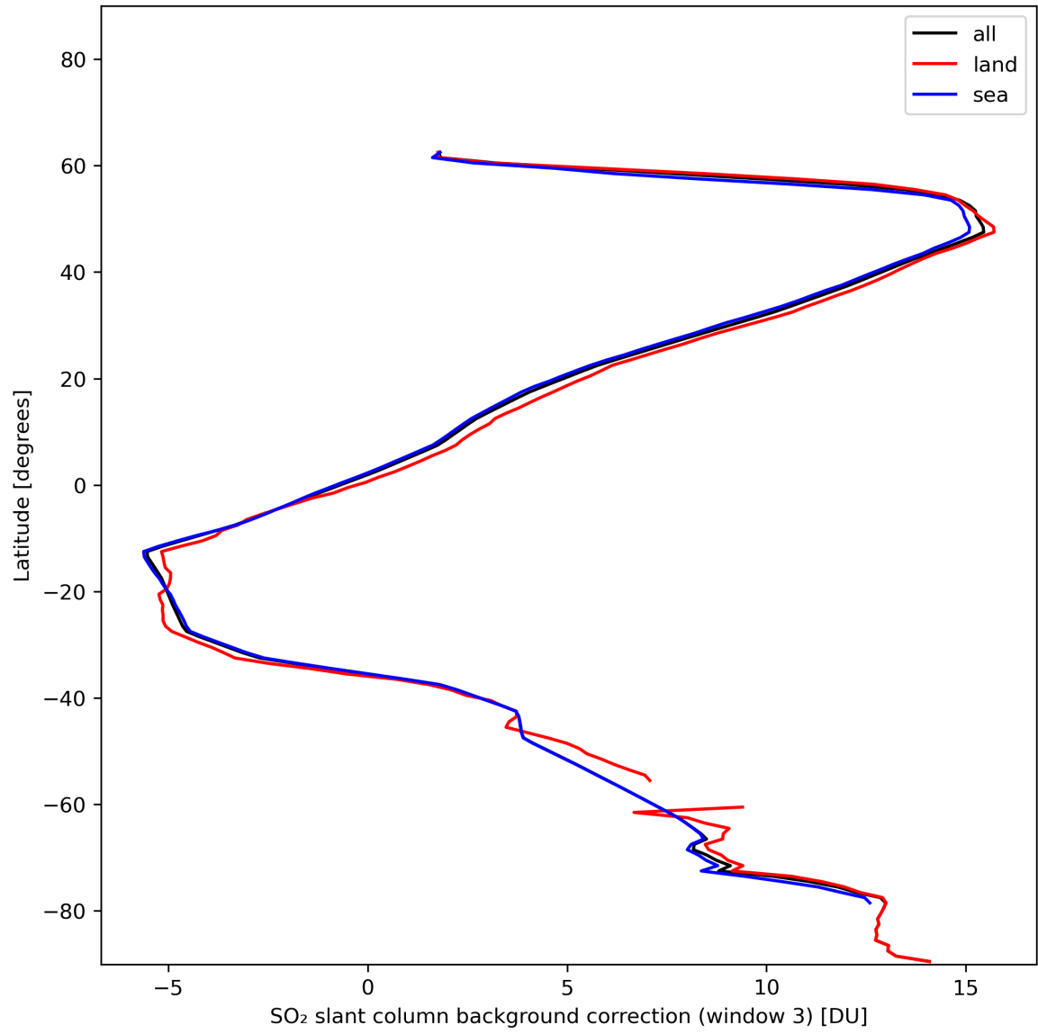
Figure 44: Zonal average of “SO 2 slant column background correction (window 3)” for 2024-01-05 to 2024-01-06.
