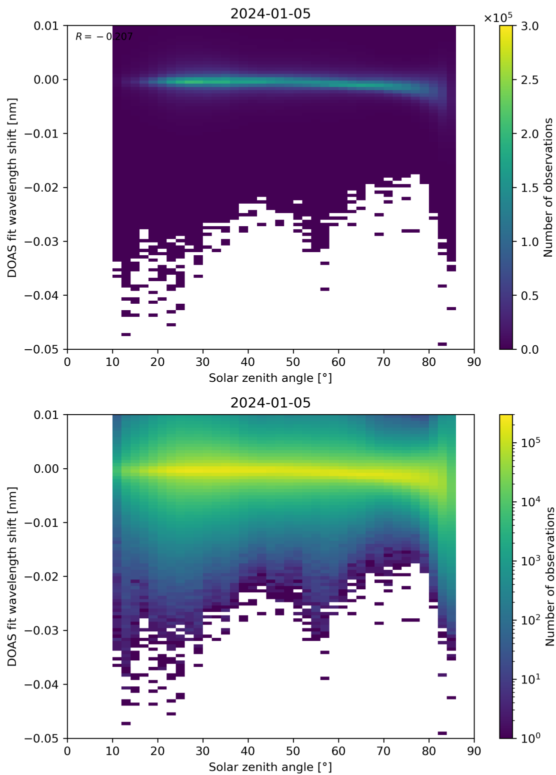
Figure 161: Scatter density plot of “Solar zenith angle” against “DOAS fit wavelength shift” for 2024-01-05 to 2024-01-06.
