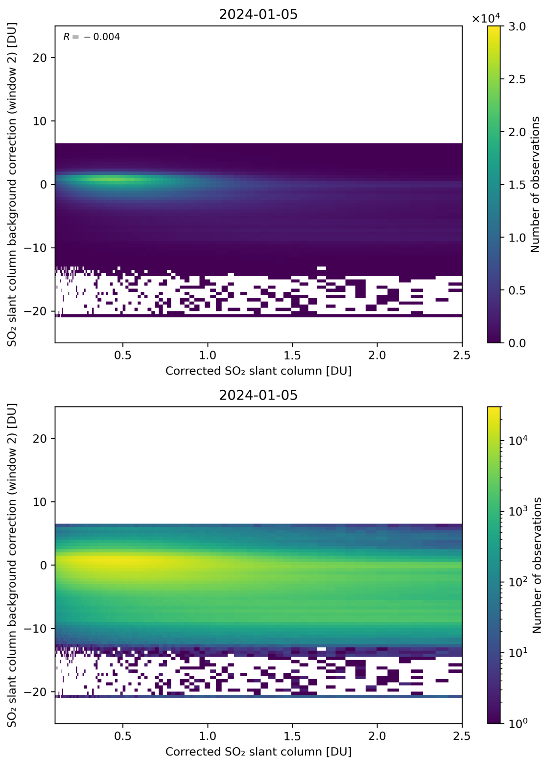
Figure 179: Scatter density plot of “Corrected SO 2 slant column” against “SO 2 slant column background correction (window 2)” for 2024-01-05 to 2024-01-06.
