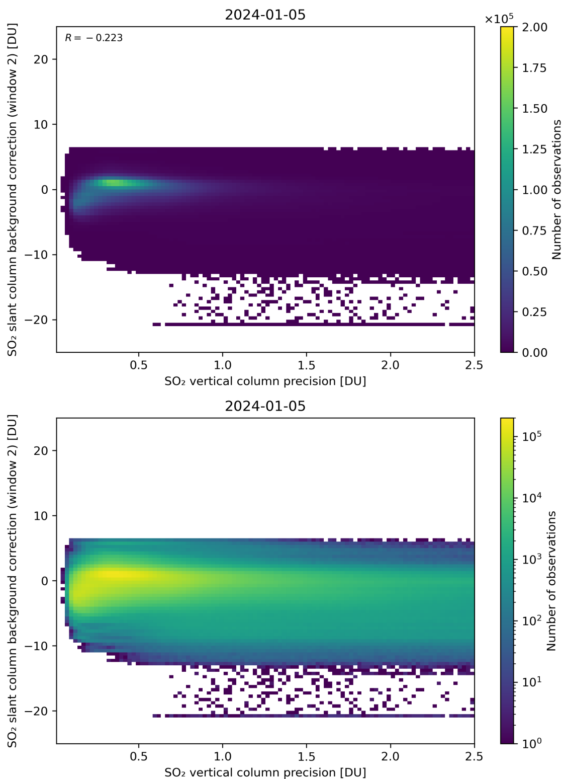
Figure 280: Scatter density plot of “SO 2 vertical column precision” against “SO 2 slant column background correction (window 2)” for 2024-01-05 to 2024-01-06.
