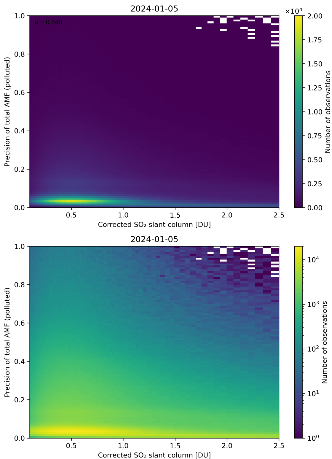
Figure 193: Scatter density plot of “Corrected SO 2 slant column” against “Precision of total AMF (polluted)” for 2024-01-05 to 2024-01-06.
