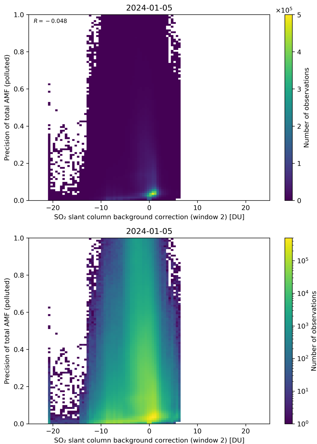
Figure 120: Scatter density plot of “SO 2 slant column background correction (window 2)” against “Precision of total AMF (polluted)” for 2024-01-05 to 2024-01-06.
