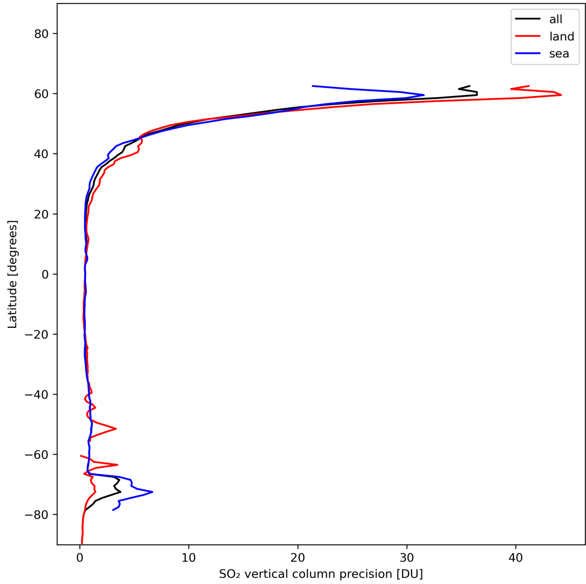
Figure 31: Zonal average of “SO 2 vertical column precision” for 2024-01-05 to 2024-01-06.
