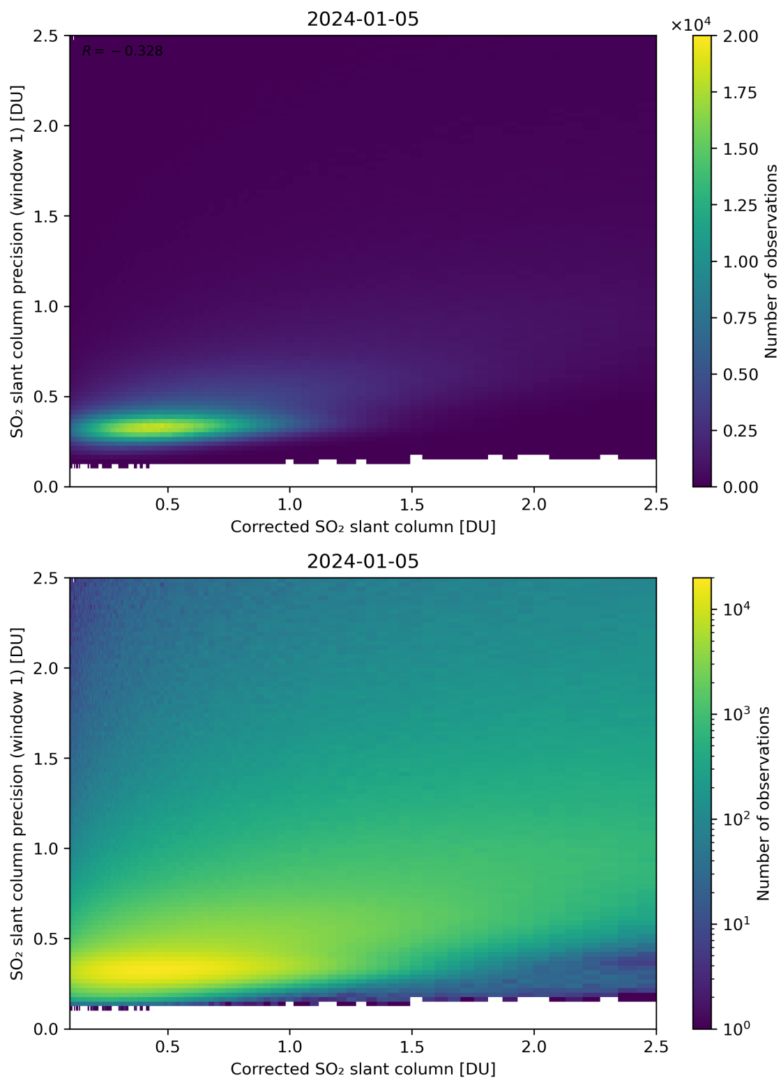
Figure 188: Scatter density plot of “Corrected SO 2 slant column” against “SO 2 slant column precision (window 1)” for 2024-01-05 to 2024-01-06.
