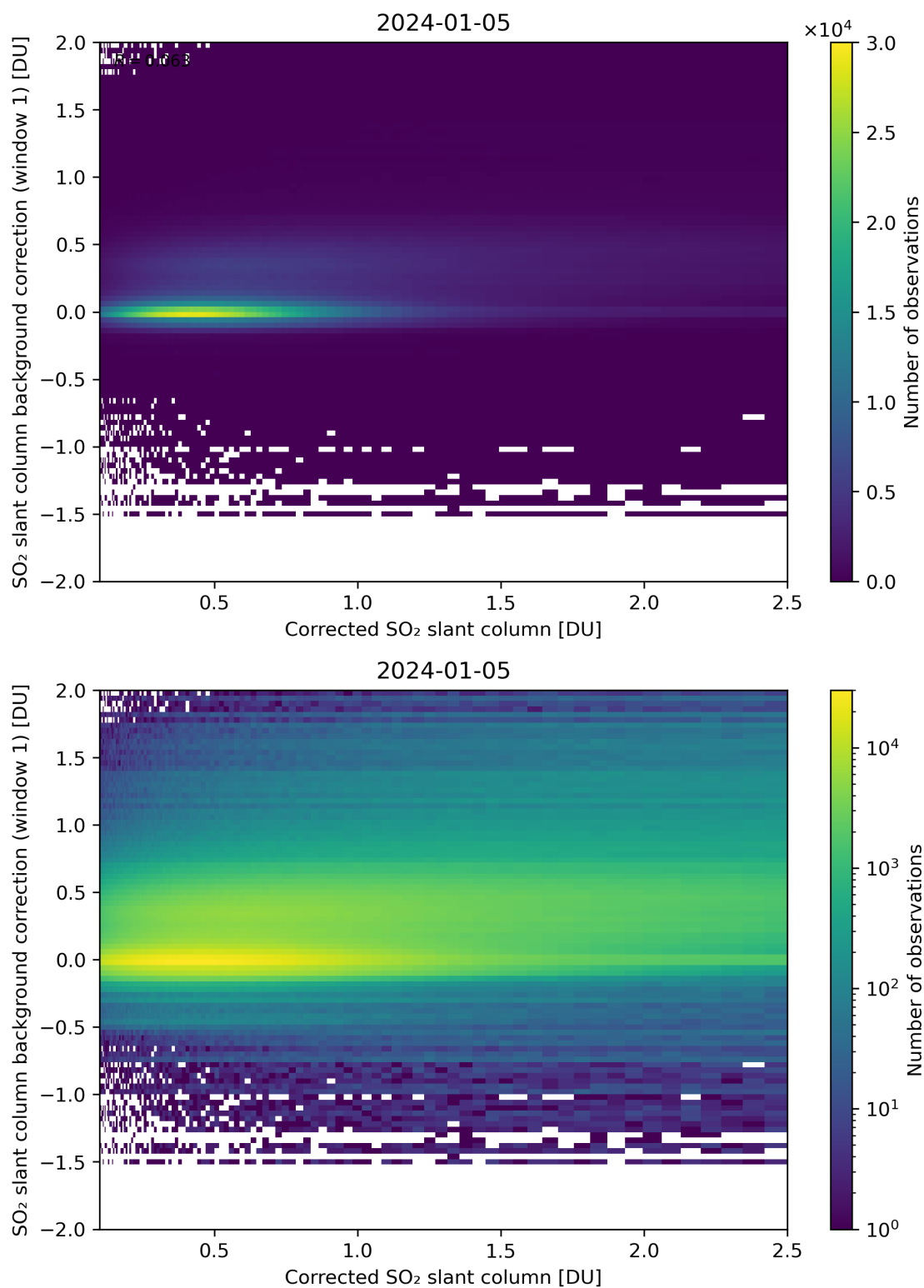
Figure 178: Scatter density plot of “Corrected SO 2 slant column” against “SO 2 slant column background correction (window 1)” for 2024-01-05 to 2024-01-06.
