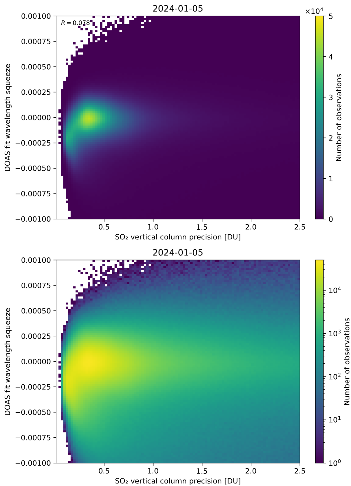
Figure 283: Scatter density plot of “SO 2 vertical column precision” against “DOAS fit wavelength squeeze” for 2024-01-05 to 2024-01-06.
