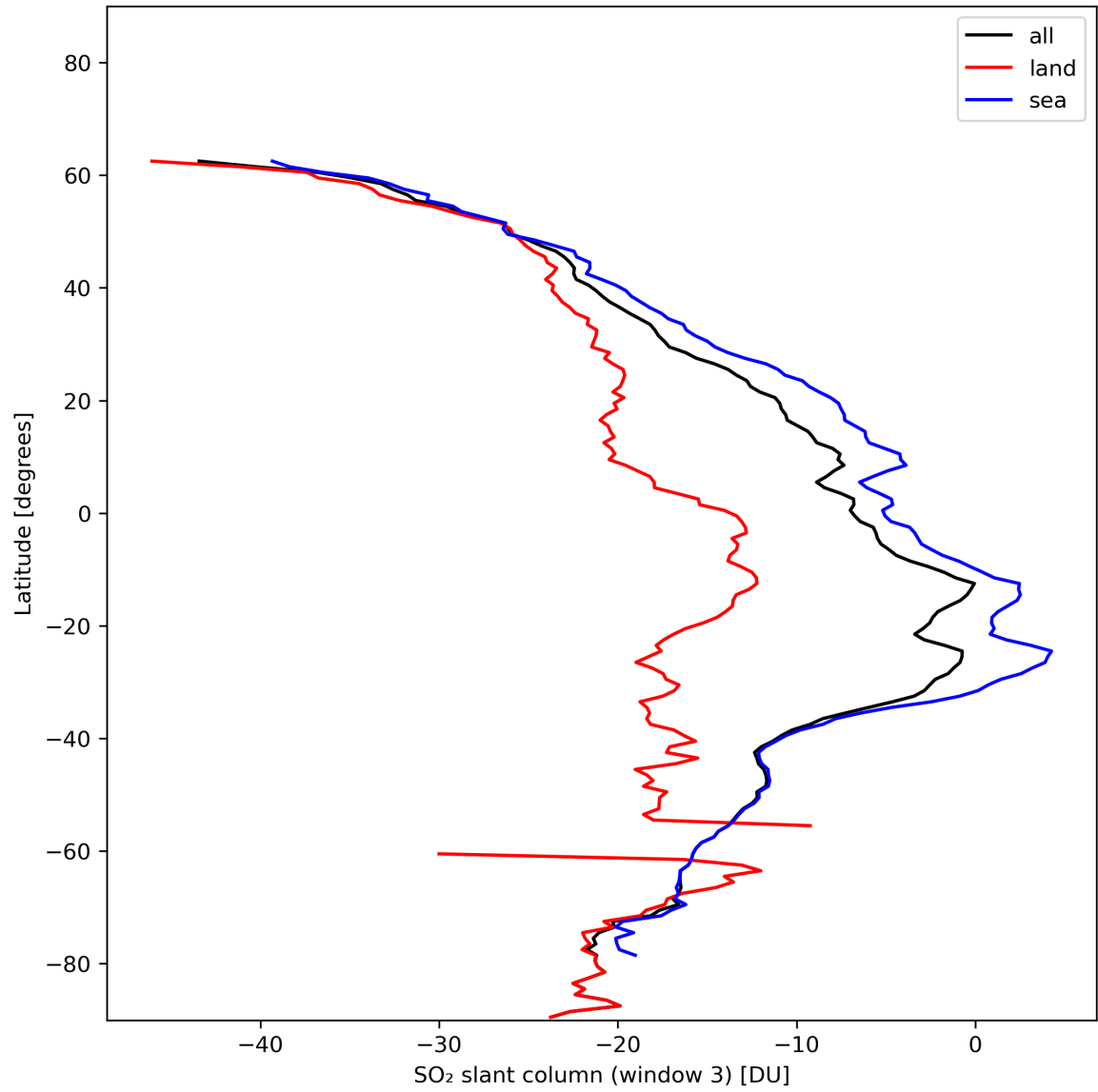
Figure 41: Zonal average of “SO 2 slant column (window 3)” for 2024-01-05 to 2024-01-06.
