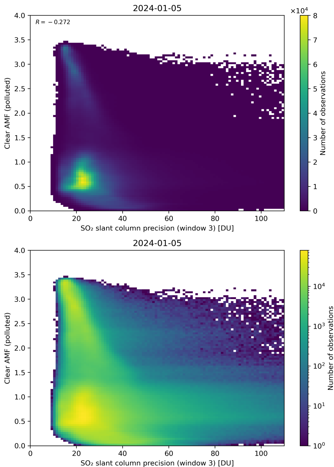
Figure 261: Scatter density plot of “SO 2 slant column precision (window 3)” against “Clear AMF (polluted)” for 2024-01-05 to 2024-01-06.
