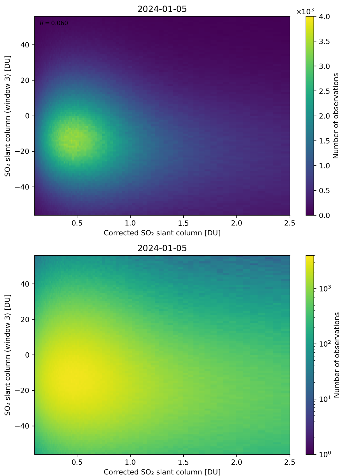
Figure 190: Scatter density plot of “Corrected SO 2 slant column” against “SO 2 slant column (window 3)” for 2024-01-05 to 2024-01-06.
