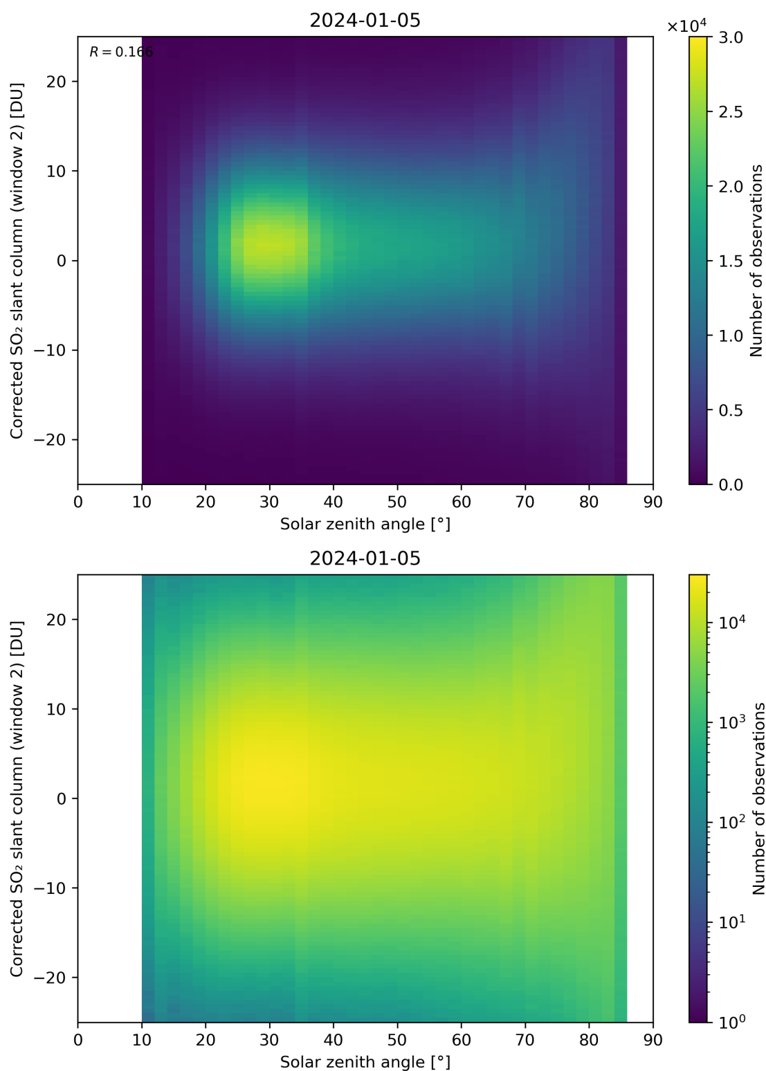
Figure 167: Scatter density plot of “Solar zenith angle” against “Corrected SO 2 slant column (window 2)” for 2024-01-05 to 2024-01-06.
