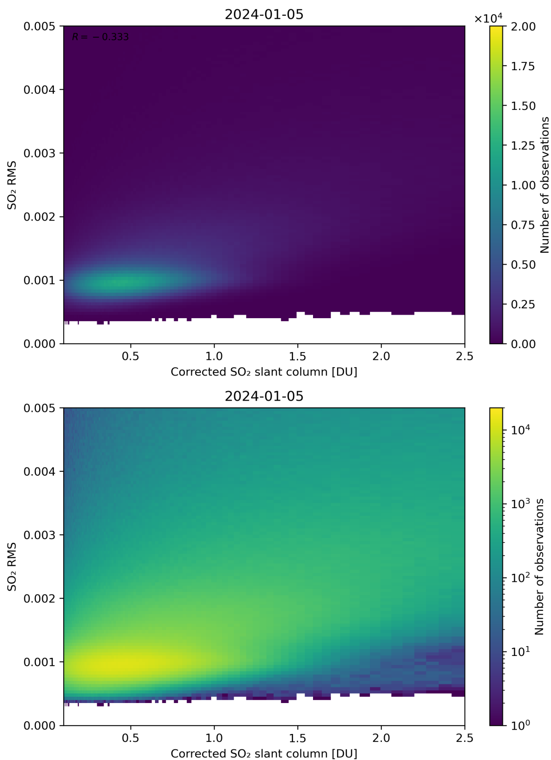
Figure 183: Scatter density plot of “Corrected SO 2 slant column” against “SO 2 RMS” for 2024-01-05 to 2024-01-06.
