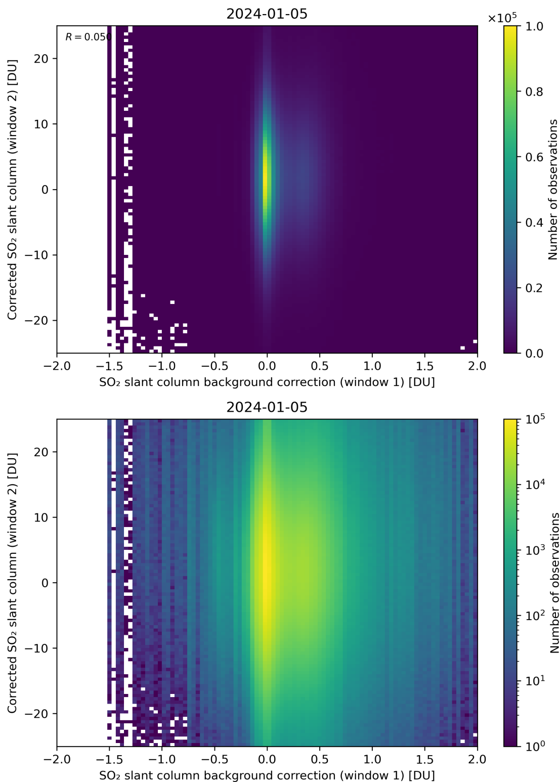
Figure 104: Scatter density plot of “SO 2 slant column background correction (window 1)” against “Corrected SO 2 slant column (window 2)” for 2024-01-05 to 2024-01-06.
