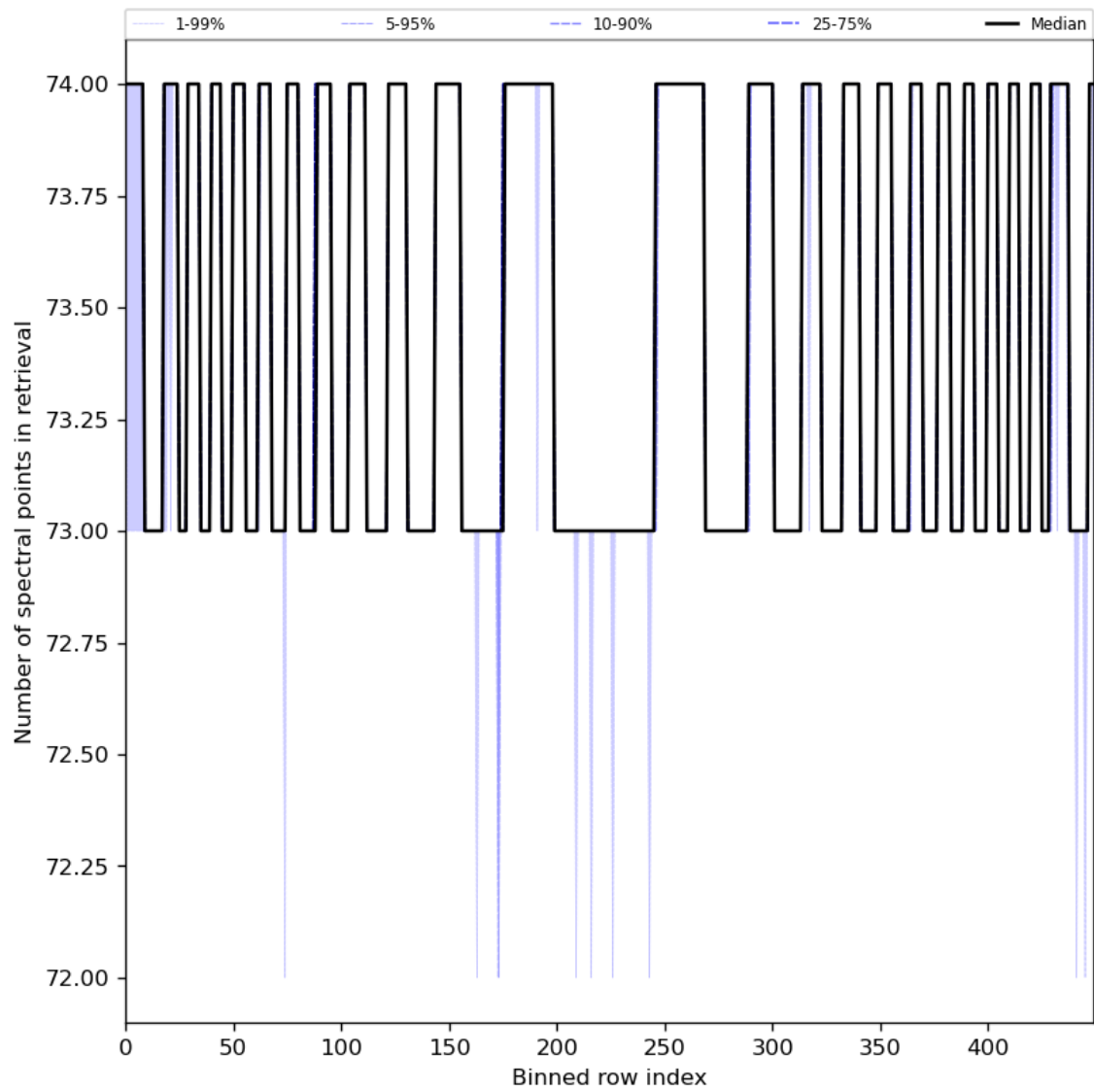
Figure 97: Along track statistics of “Number of spectral points in retrieval” for 2024-01-05 to 2024-01-06
