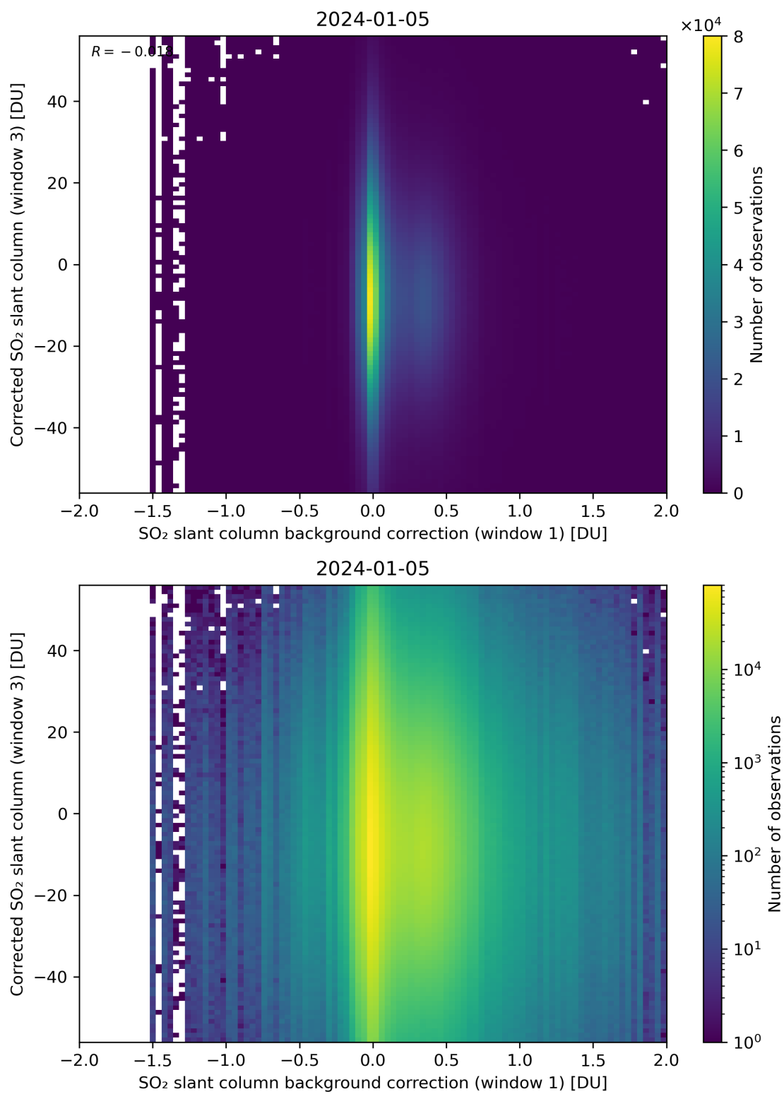
Figure 105: Scatter density plot of “SO 2 slant column background correction (window 1)” against “Corrected SO 2 slant column (window 3)” for 2024-01-05 to 2024-01-06.
