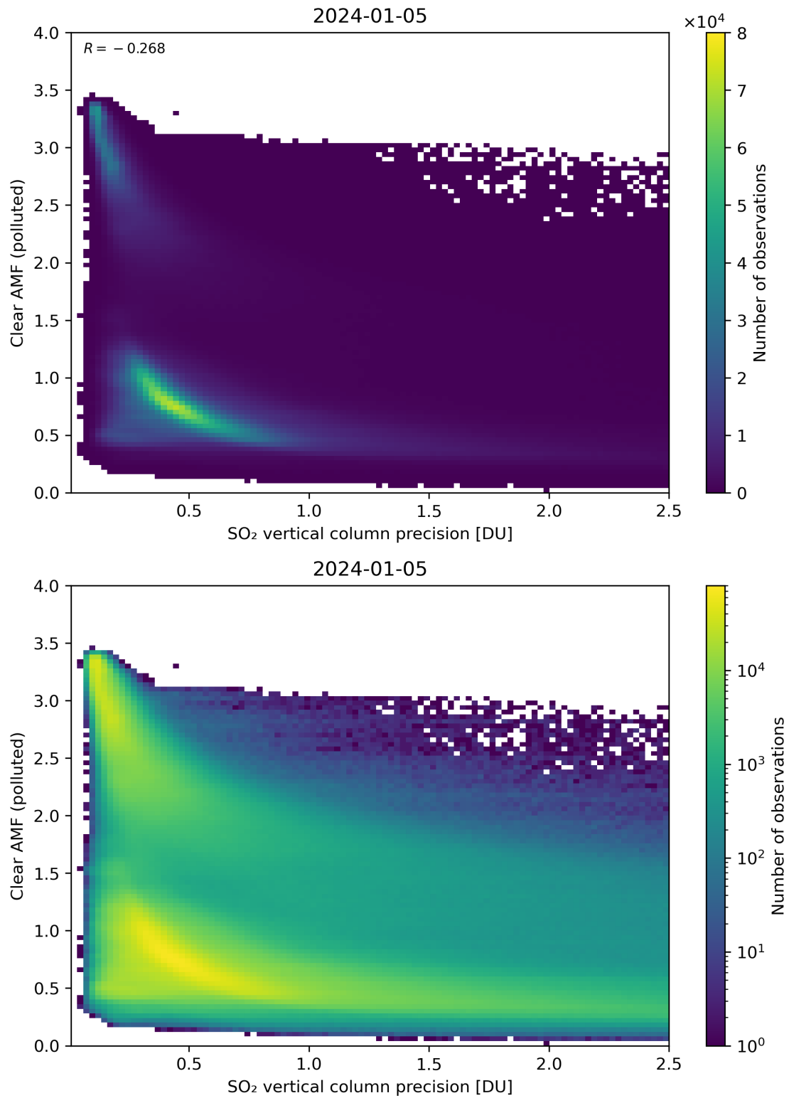
Figure 285: Scatter density plot of “SO 2 vertical column precision” against “Clear AMF (polluted)” for 2024-01-05 to 2024-01-06.
