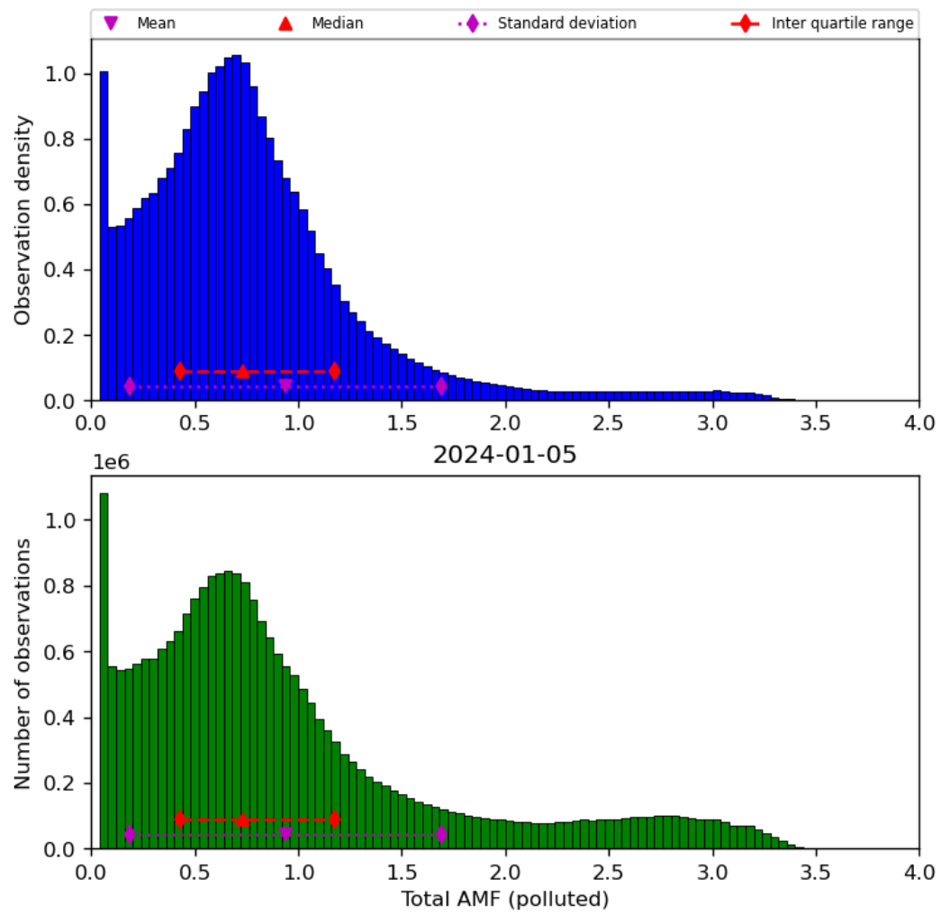
Figure 71: Histogram of “Total AMF (polluted)” for 2024-01-05 to 2024-01-06
