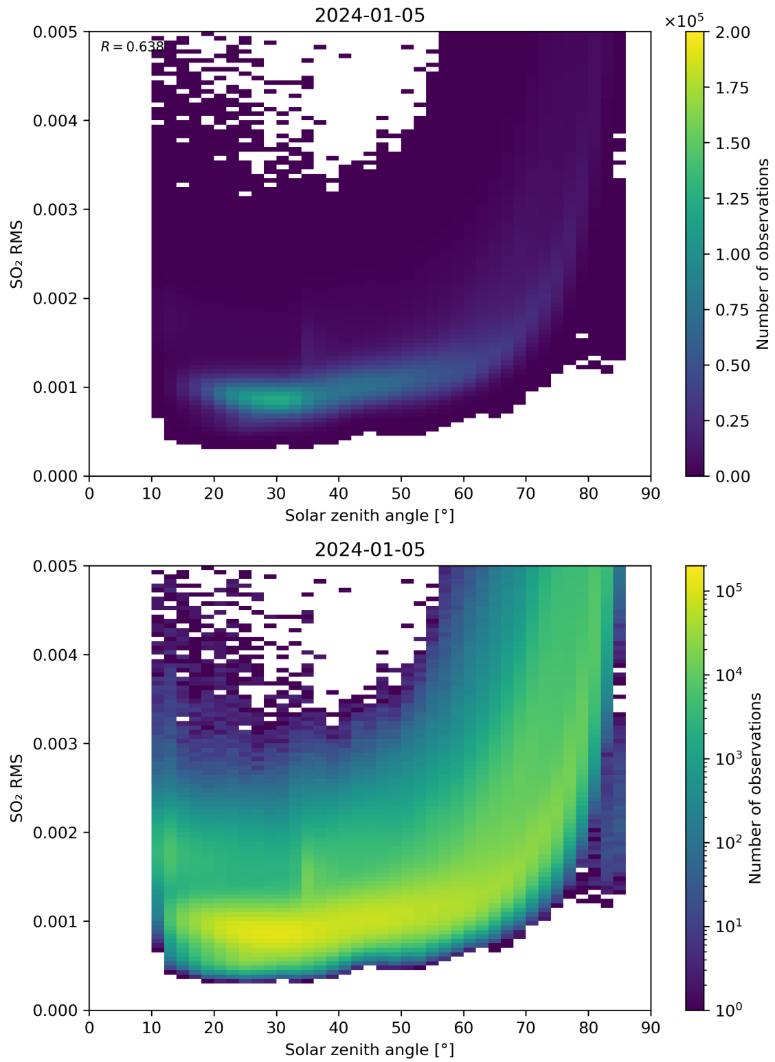
Figure 163: Scatter density plot of “Solar zenith angle” against “SO 2 RMS” for 2024-01-05 to 2024-01-06.
