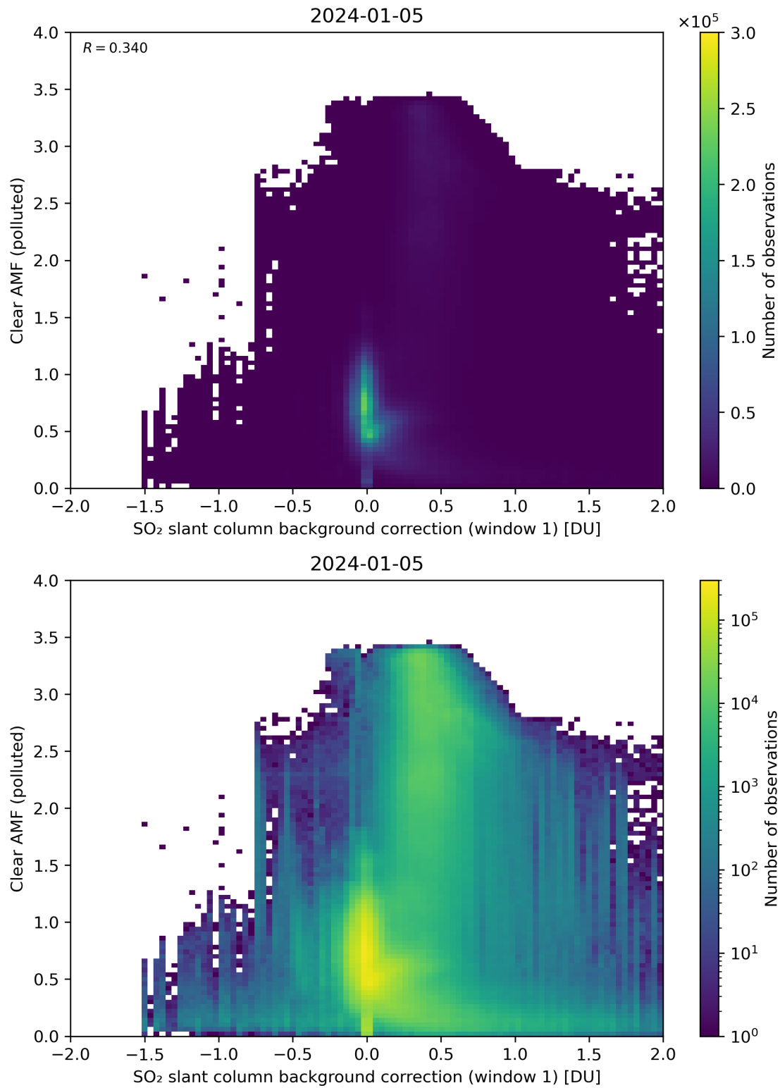
Figure 103: Scatter density plot of “SO 2 slant column background correction (window 1)” against “Clear AMF (polluted)” for 2024-01-05 to 2024-01-06.
