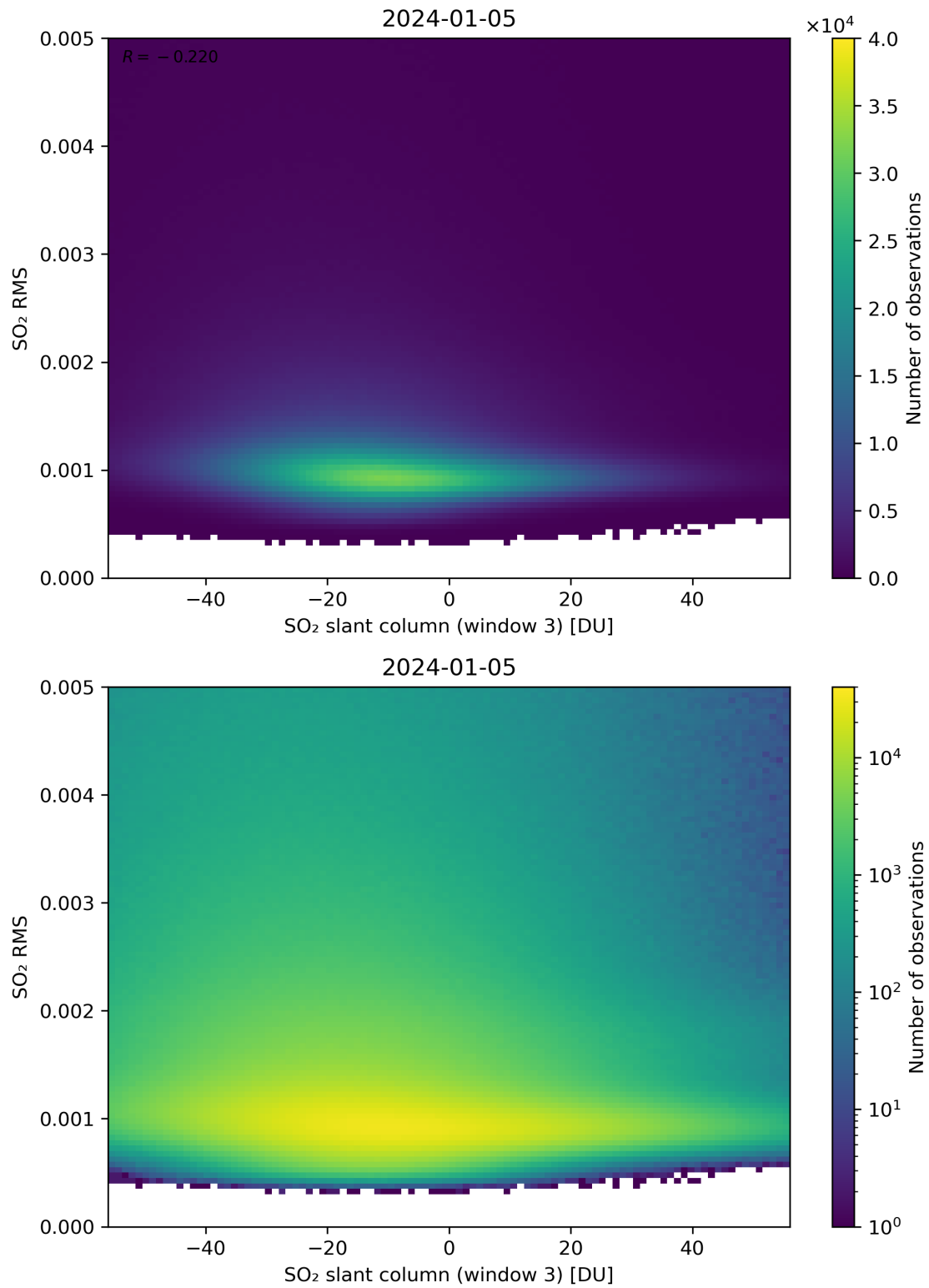
Figure 256: Scatter density plot of “SO 2 slant column (window 3)” against “SO 2 RMS” for 2024-01-05 to 2024-01-06.
