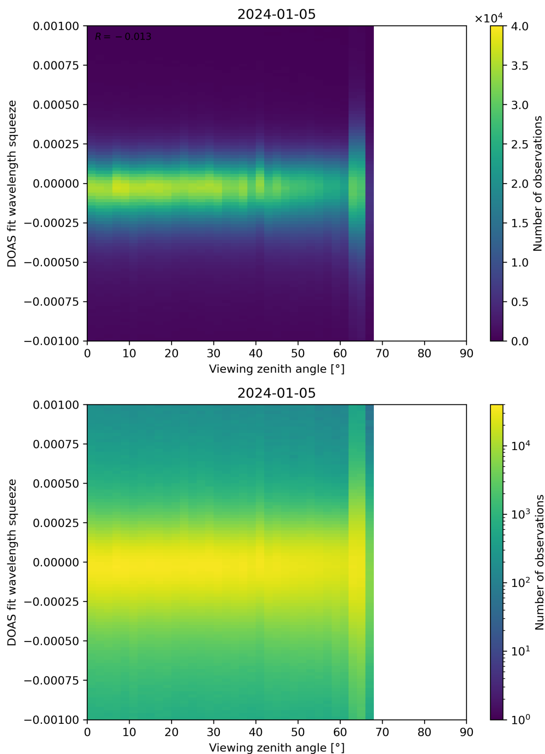
Figure 312: Scatter density plot of “Viewing zenith angle” against “DOAS fit wavelength squeeze” for 2024-01-05 to 2024-01-06.
