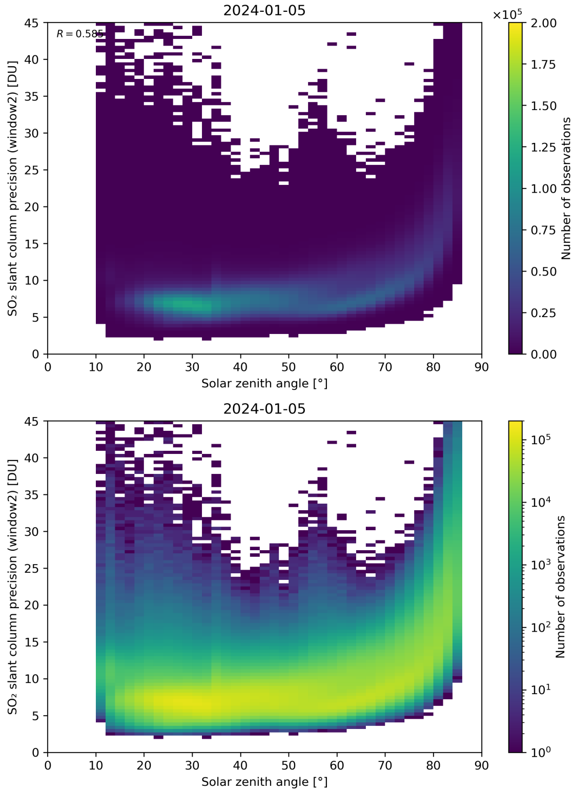
Figure 171: Scatter density plot of “Solar zenith angle” against “SO 2 slant column precision (window2)” for 2024-01-05 to 2024-01-06.
