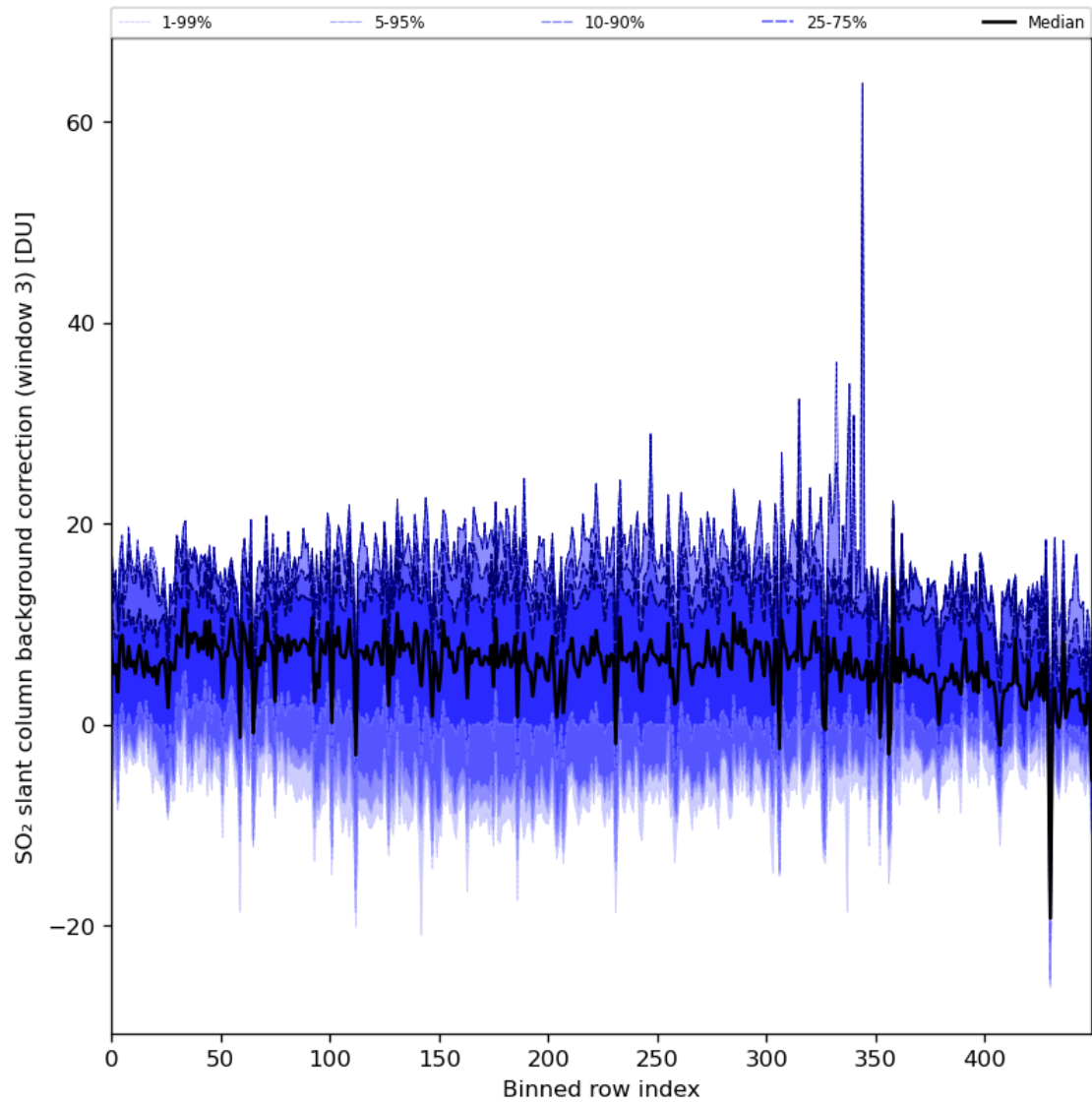
Figure 90: Along track statistics of “SO 2 slant column background correction (window 3)” for 2024-01-05 to 2024-01-06
