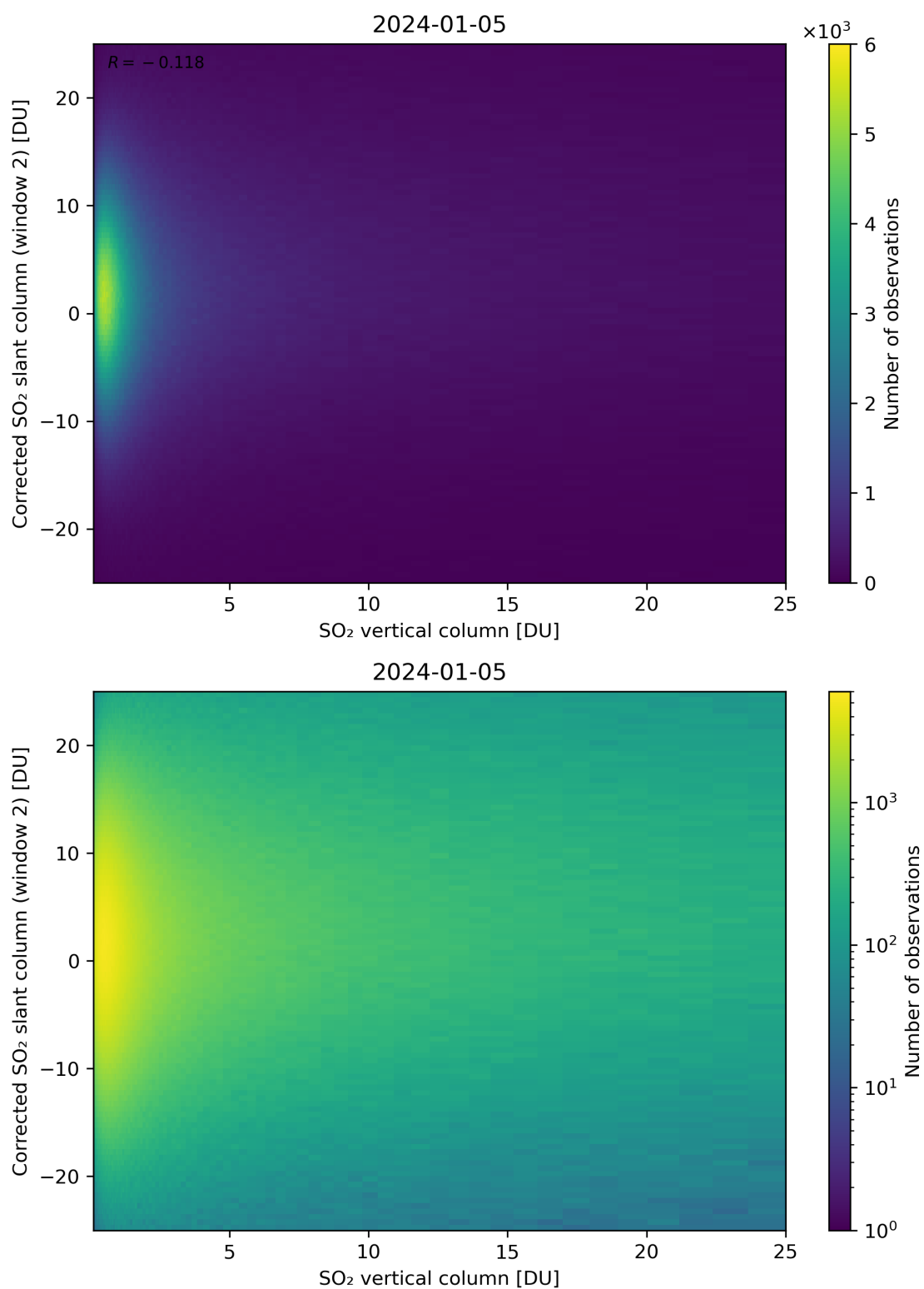
Figure 298: Scatter density plot of “SO 2 vertical column” against “Corrected SO 2 slant column (window 2)” for 2024-01-05 to 2024-01-06.
