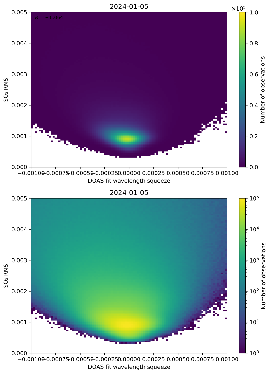
Figure 132: Scatter density plot of “DOAS fit wavelength squeeze” against “SO 2 RMS” for 2024-01-05 to 2024-01-06.
