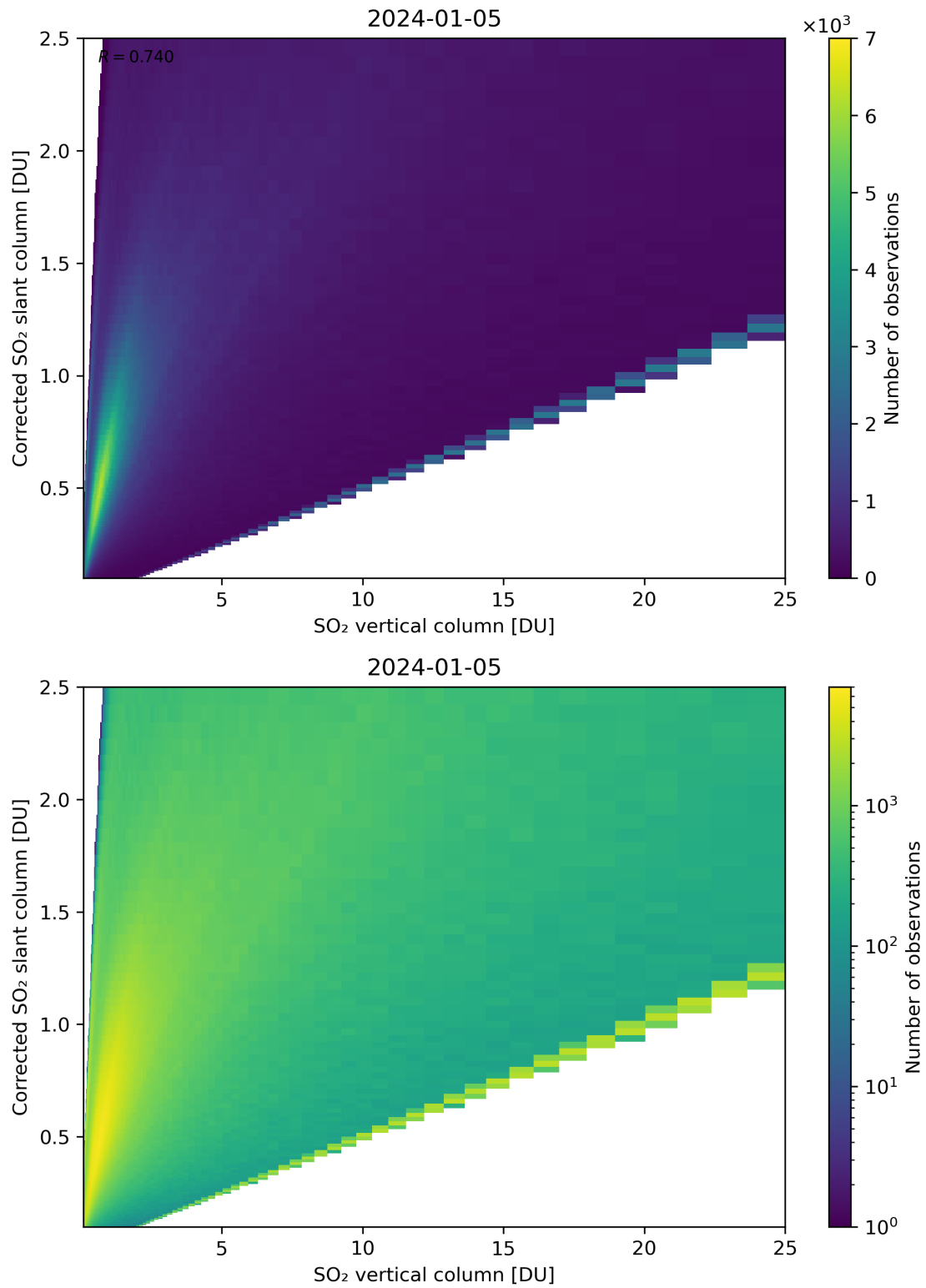
Figure 297: Scatter density plot of “SO 2 vertical column” against “Corrected SO 2 slant column” for 2024-01-05 to 2024-01-06.
