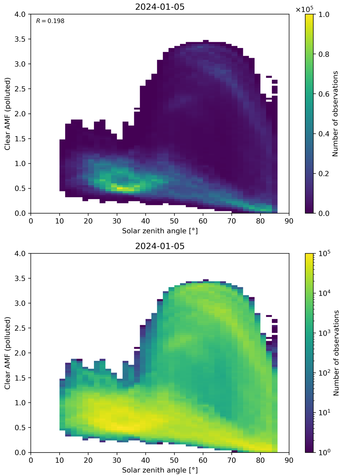
Figure 165: Scatter density plot of “Solar zenith angle” against “Clear AMF (polluted)” for 2024-01-05 to 2024-01-06.
