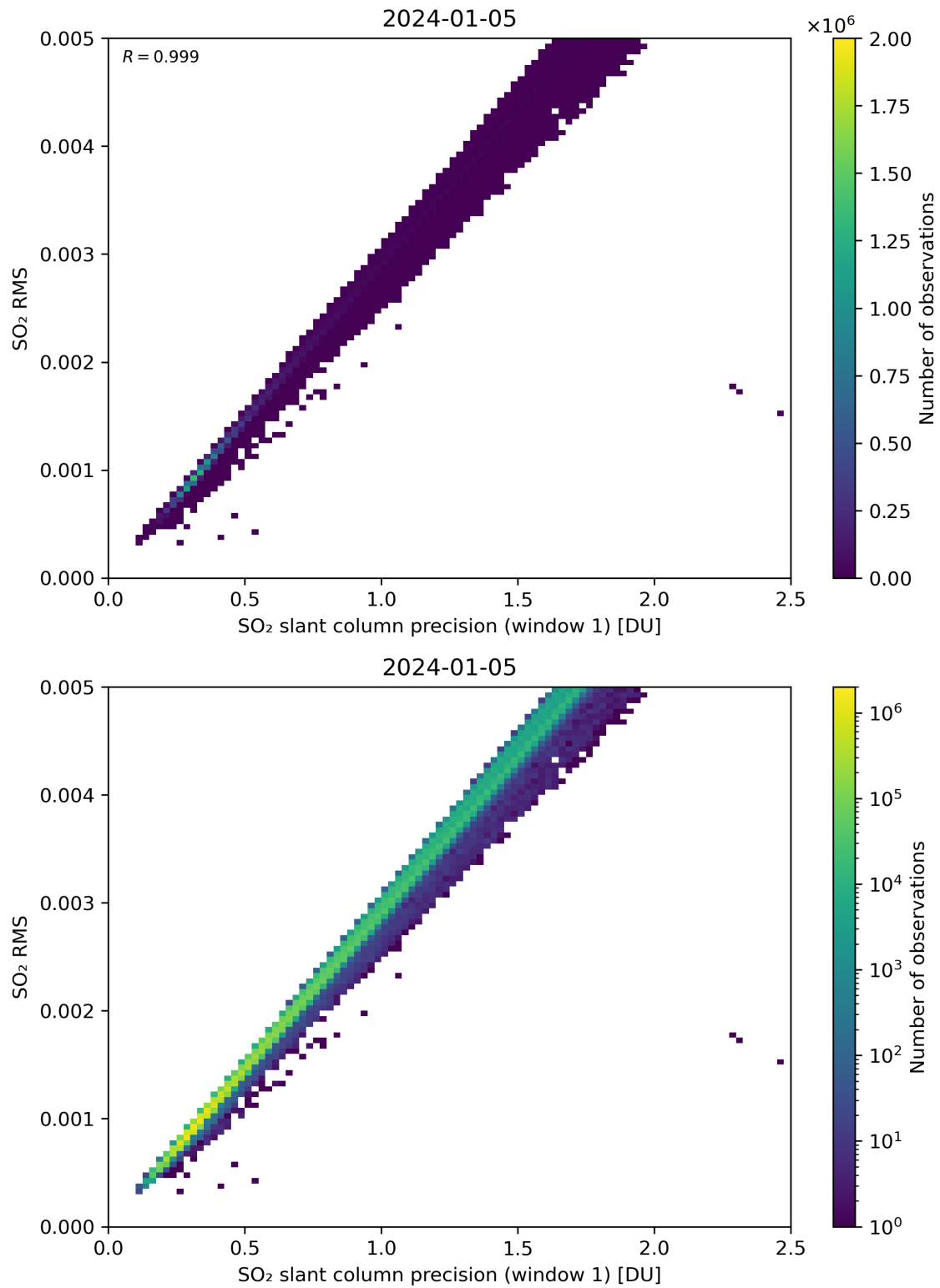
Figure 223: Scatter density plot of “SO 2 slant column precision (window 1)” against “SO 2 RMS” for 2024-01-05 to 2024-01-06.
