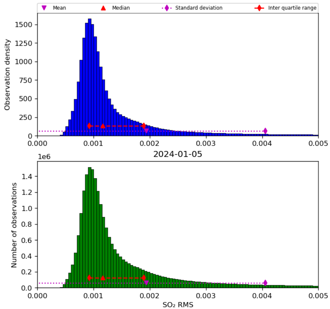
Figure 70: Histogram of “SO 2 RMS” for 2024-01-05 to 2024-01-06
