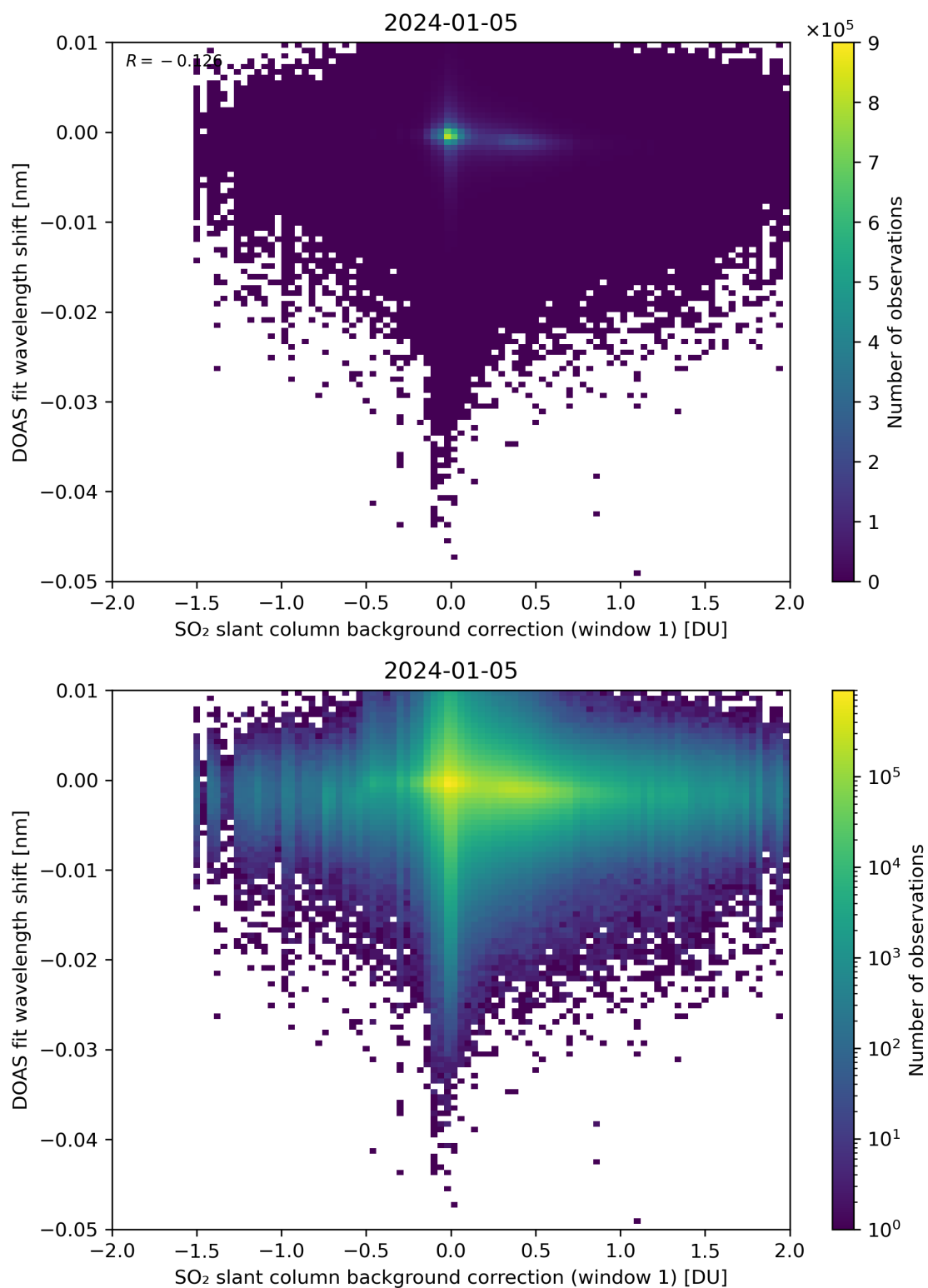
Figure 100: Scatter density plot of “SO 2 slant column background correction (window 1)” against “DOAS fit wavelength shift” for 2024-01-05 to 2024-01-06.
