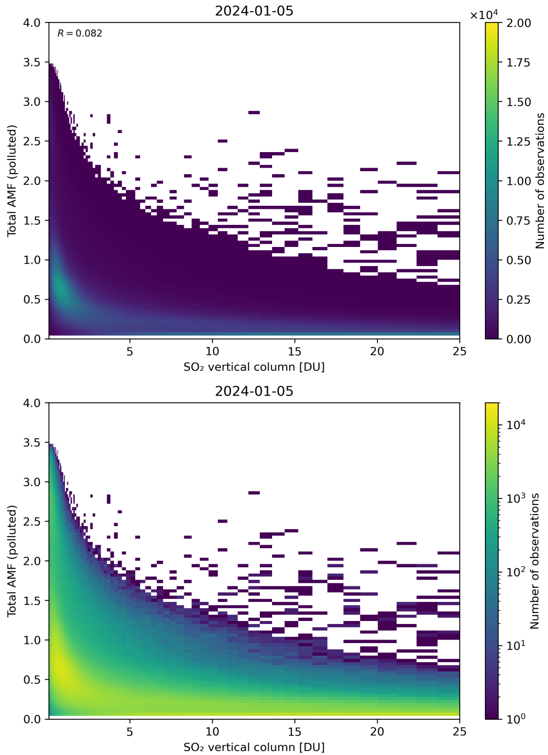
Figure 305: Scatter density plot of “SO 2 vertical column” against “Total AMF (polluted)” for 2024-01-05 to 2024-01-06.
