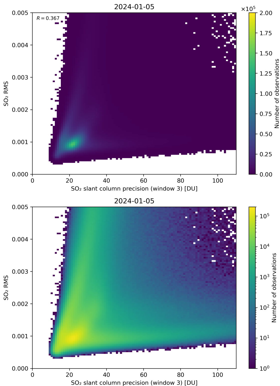
Figure 260: Scatter density plot of “SO 2 slant column precision (window 3)” against “SO 2 RMS” for 2024-01-05 to 2024-01-06.
