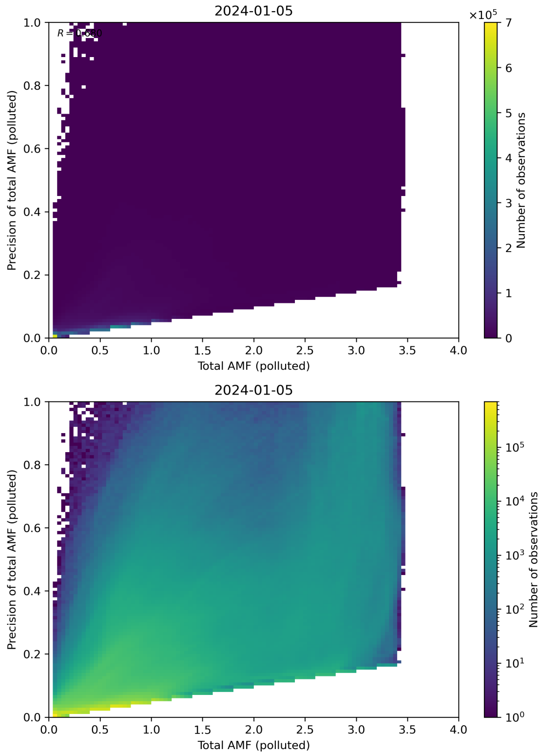
Figure 272: Scatter density plot of “Total AMF (polluted)” against “Precision of total AMF (polluted)” for 2024-01-05 to 2024-01-06.
