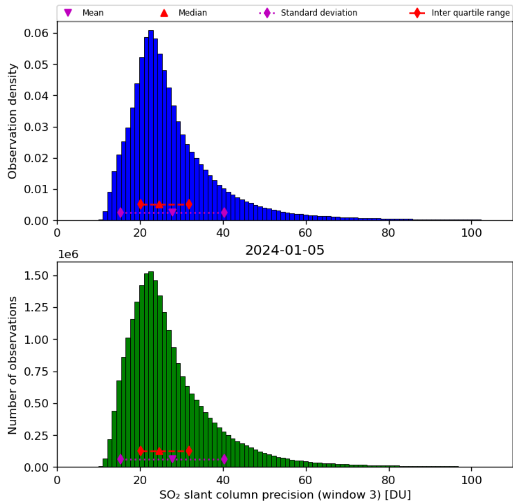
Figure 65: Histogram of “SO 2 slant column precision (window 3)” for 2024-01-05 to 2024-01-06
