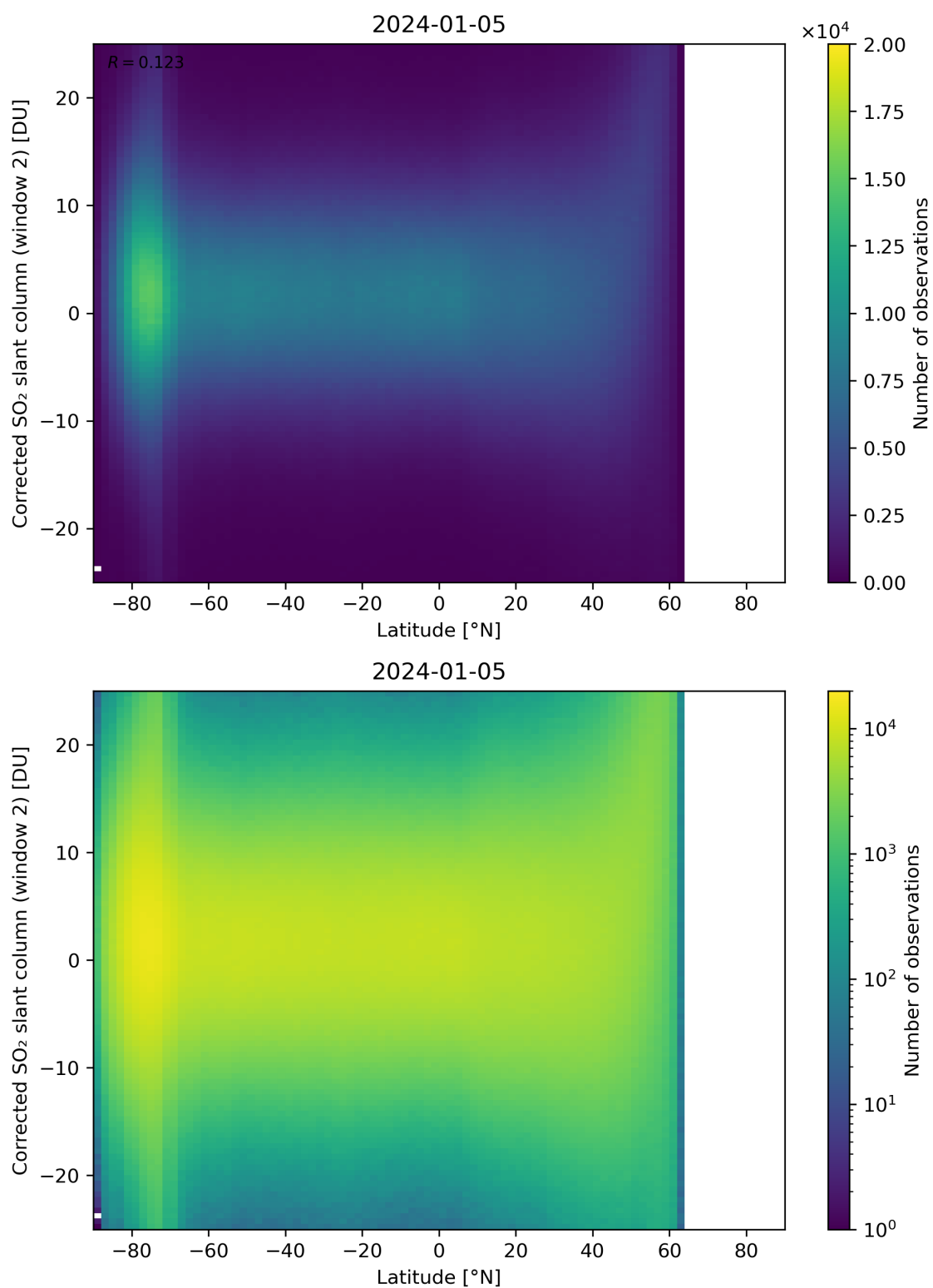
Figure 147: Scatter density plot of “Latitude” against “Corrected SO 2 slant column (window 2)” for 2024-01-05 to 2024-01-06.
