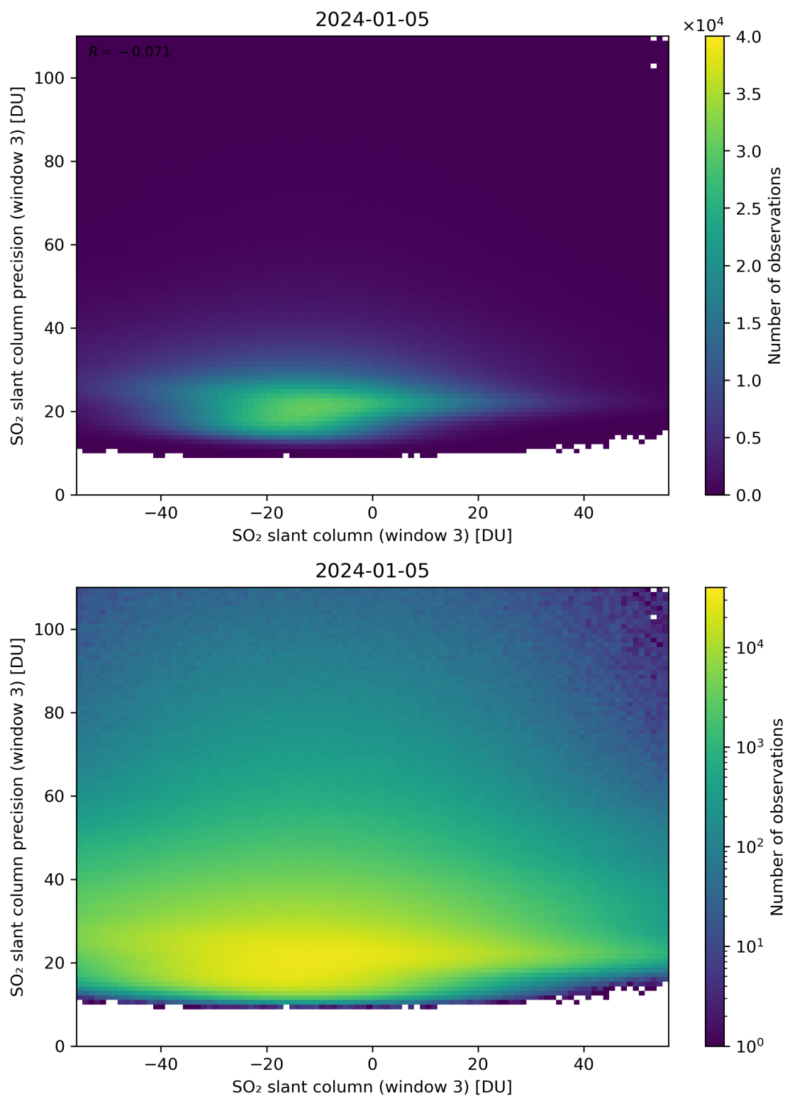
Figure 267: Scatter density plot of “SO 2 slant column (window 3)” against “SO 2 slant column precision (window 3)” for 2024-01-05 to 2024-01-06.
