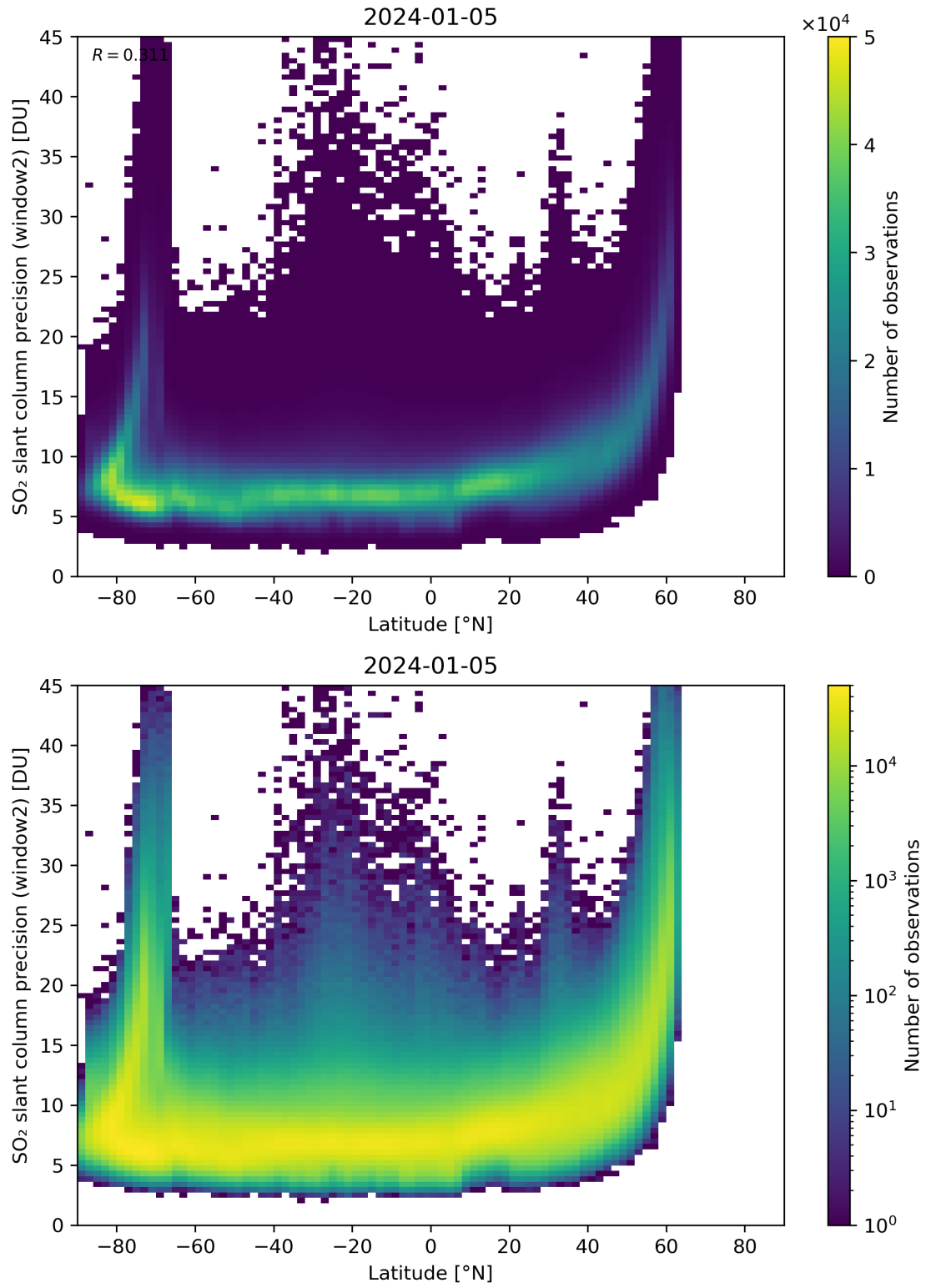
Figure 151: Scatter density plot of “Latitude” against “SO 2 slant column precision (window2)” for 2024-01-05 to 2024-01-06.
