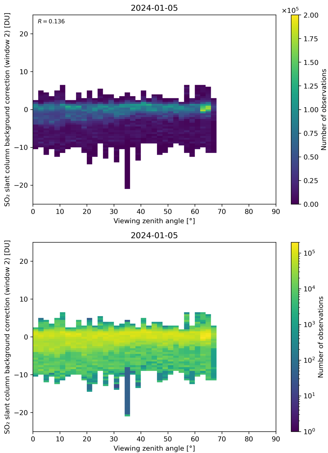
Figure 309: Scatter density plot of “Viewing zenith angle” against “SO 2 slant column background correction (window 2)” for 2024-01-05 to 2024-01-06.
