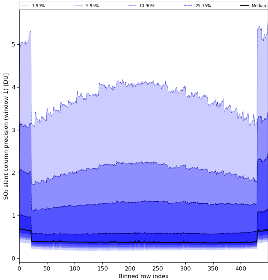
Figure 80: Along track statistics of “SO 2 slant column precision (window 1)” for 2024-01-05 to 2024-01-06
