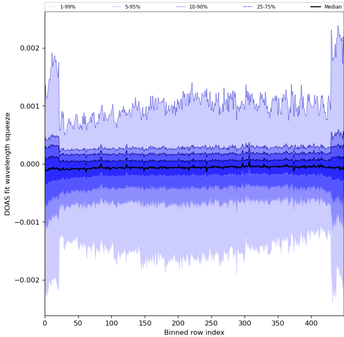
Figure 92: Along track statistics of “DOAS fit wavelength squeeze” for 2024-01-05 to 2024-01-06
