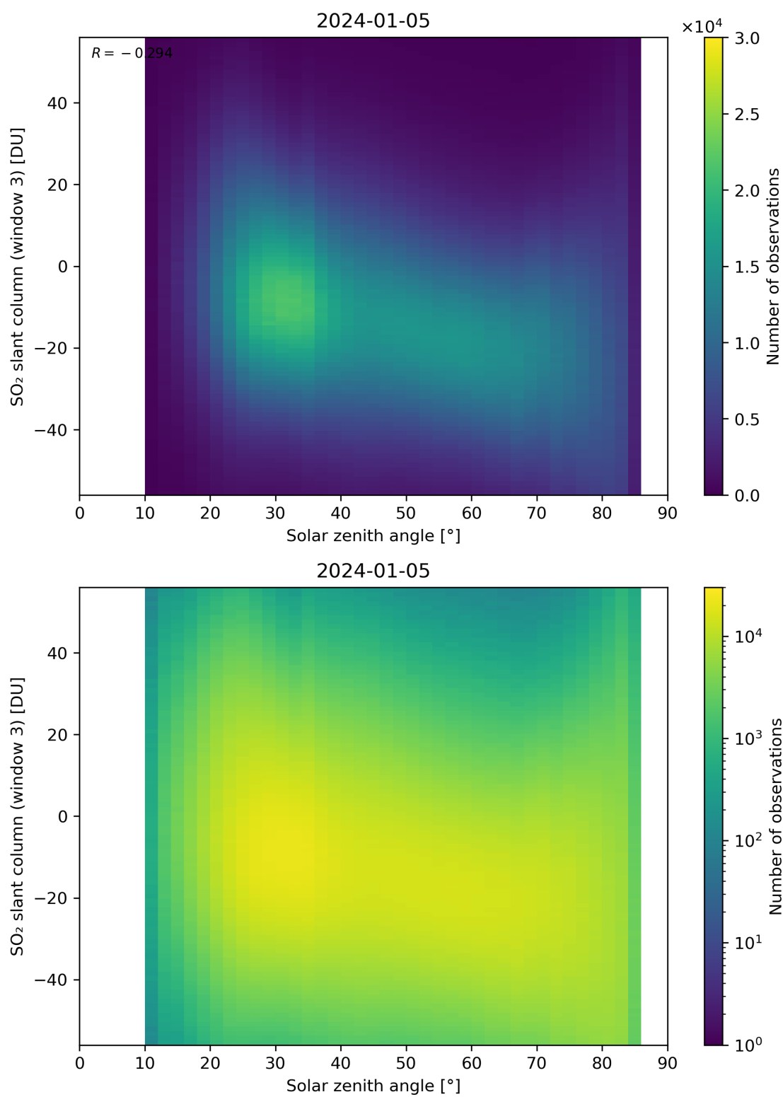
Figure 172: Scatter density plot of “Solar zenith angle” against “SO 2 slant column (window 3)” for 2024-01-05 to 2024-01-06.
