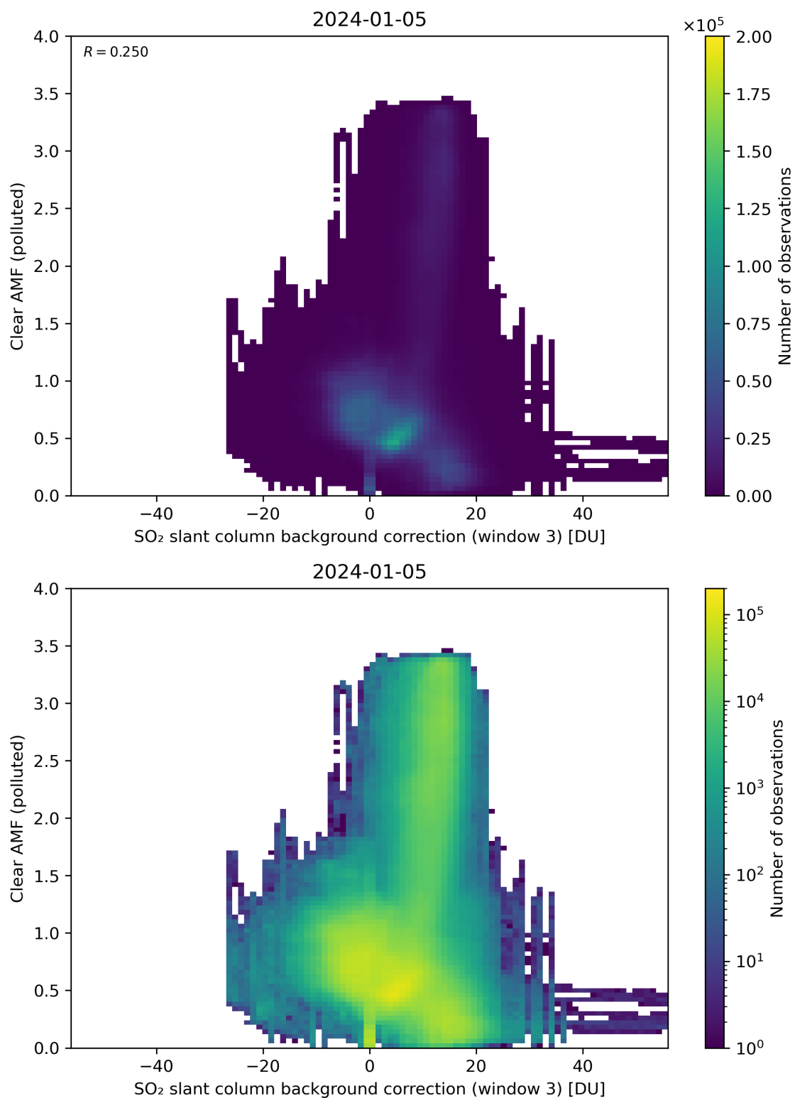
Figure 124: Scatter density plot of “SO 2 slant column background correction (window 3)” against “Clear AMF (polluted)” for 2024-01-05 to 2024-01-06.
