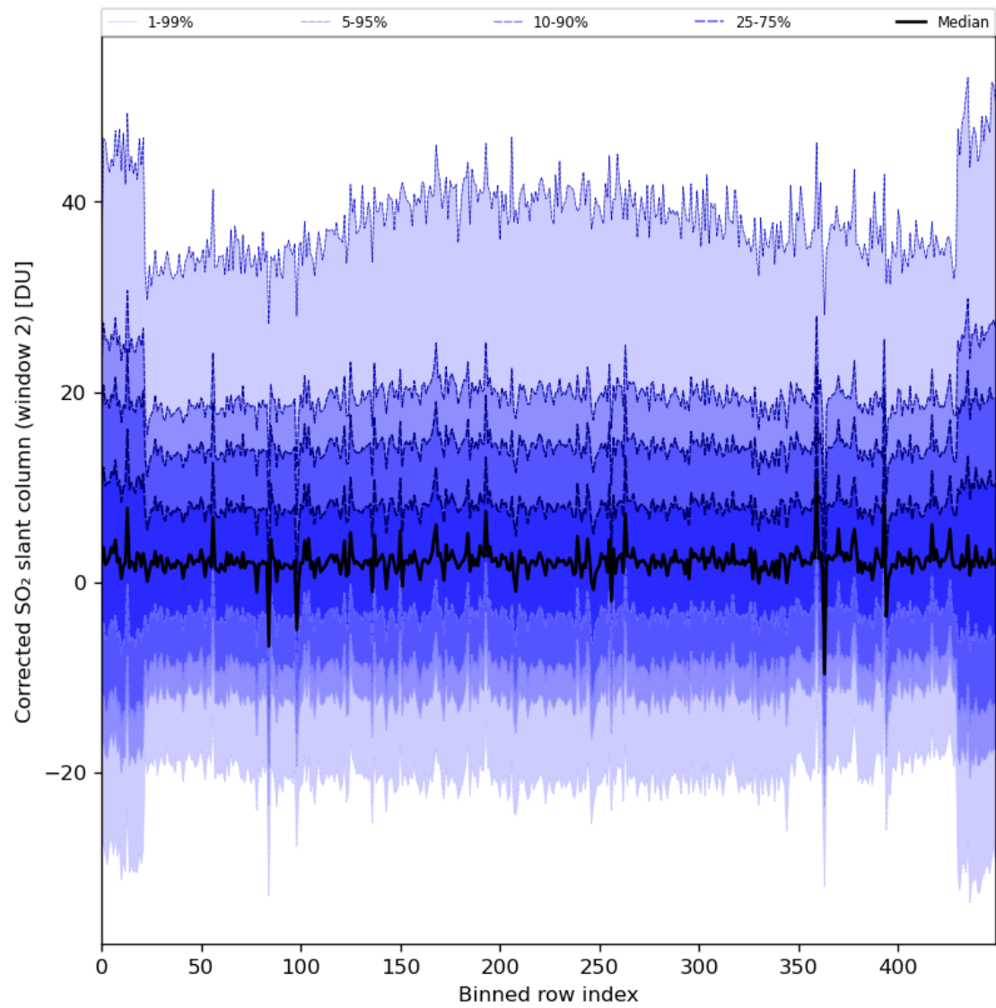
Figure 85: Along track statistics of “Corrected SO 2 slant column (window 2)” for 2024-01-05 to 2024-01-06
