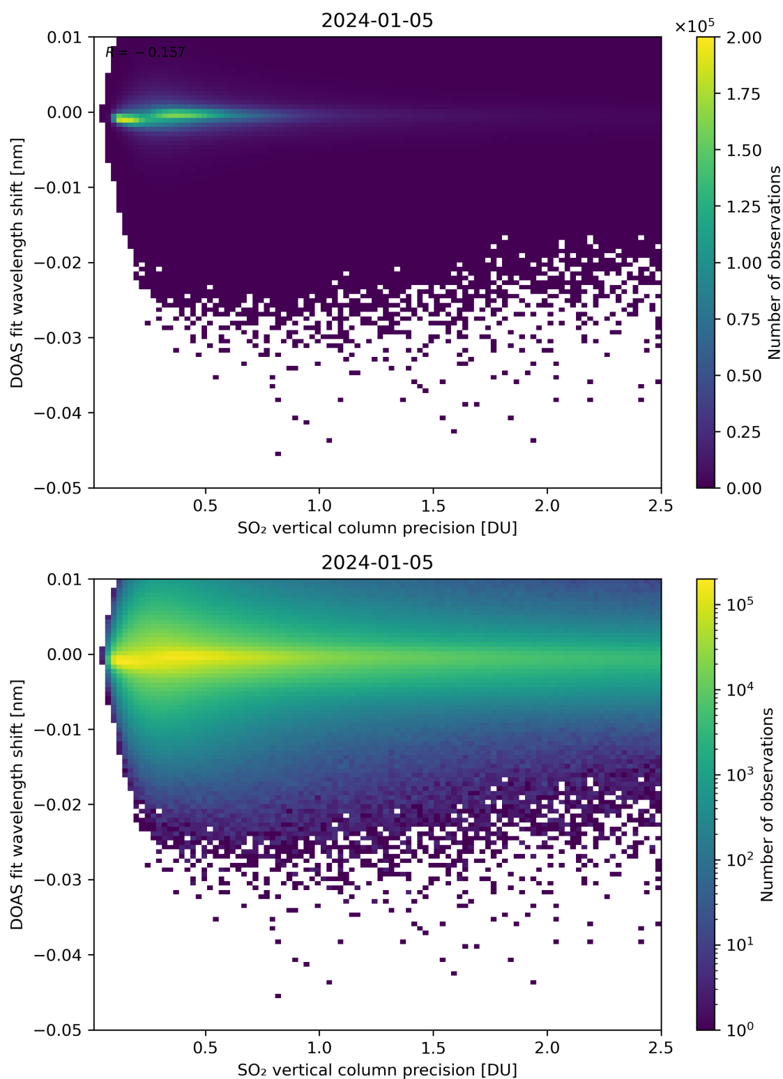
Figure 282: Scatter density plot of “SO 2 vertical column precision” against “DOAS fit wavelength shift” for 2024-01-05 to 2024-01-06.
