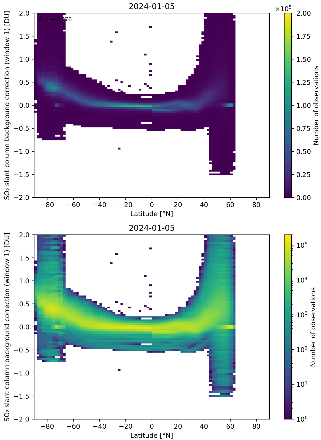
Figure 139: Scatter density plot of “Latitude” against “SO 2 slant column background correction (window 1)” for 2024-01-05 to 2024-01-06.
