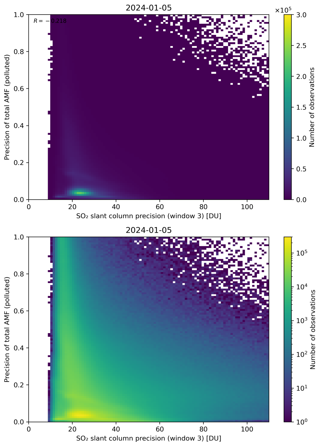
Figure 264: Scatter density plot of “SO 2 slant column precision (window 3)” against “Precision of total AMF (polluted)” for 2024-01-05 to 2024-01-06.
