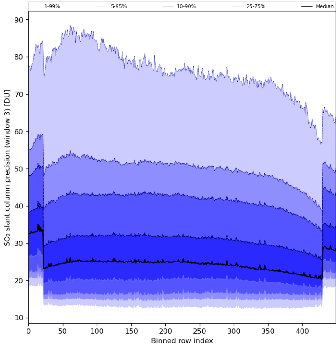
Figure 88: Along track statistics of “SO 2 slant column precision (window 3)” for 2024-01-05 to 2024-01-06
