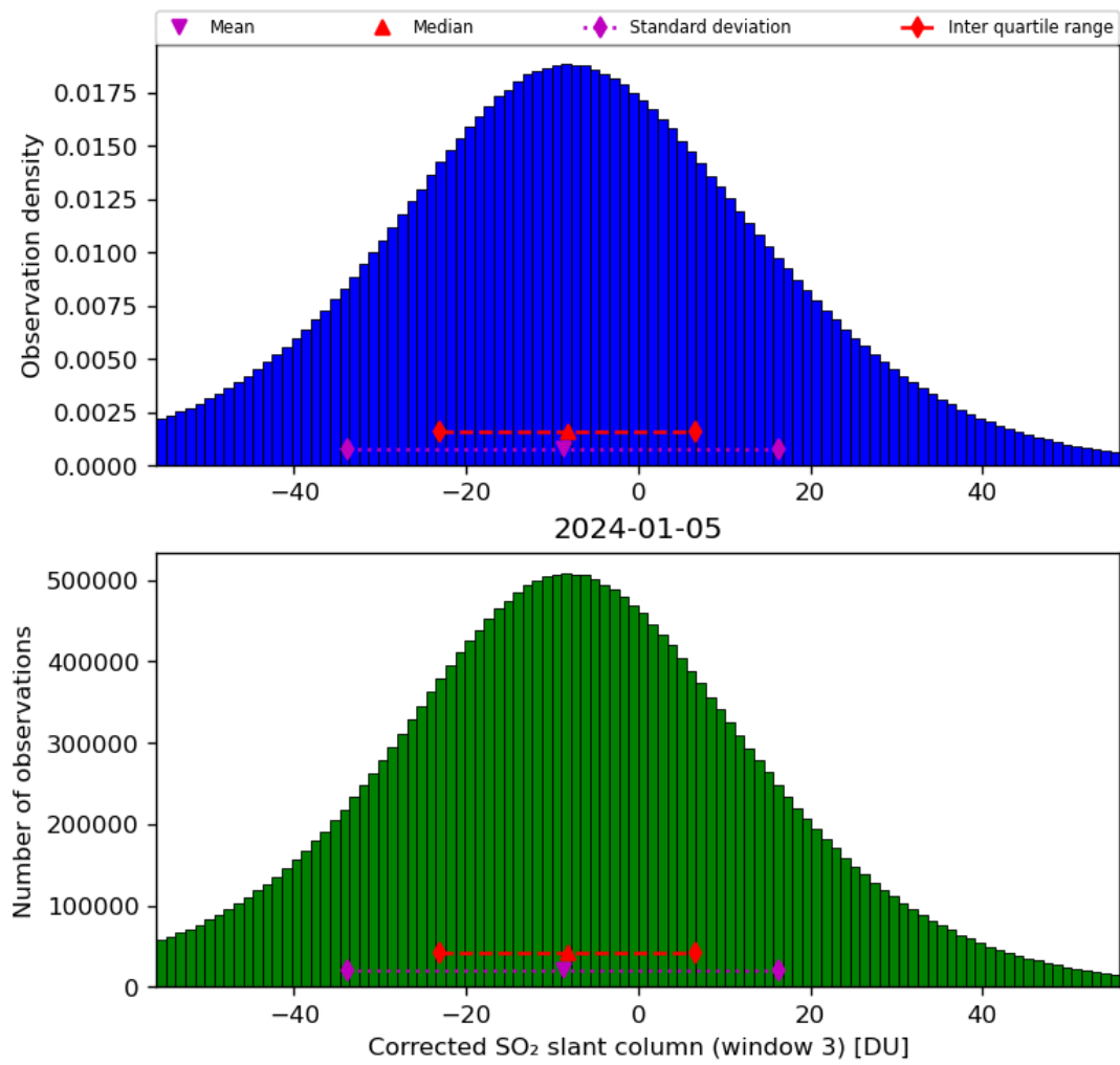
Figure 66: Histogram of “Corrected SO 2 slant column (window 3)” for 2024-01-05 to 2024-01-06
