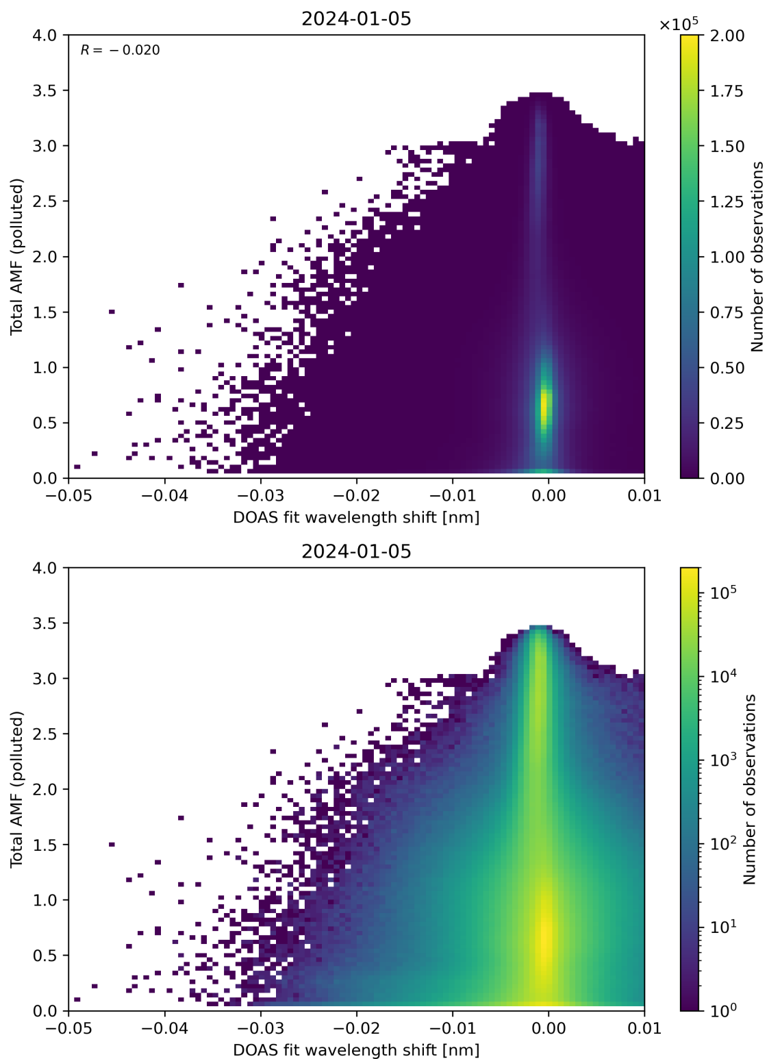
Figure 130: Scatter density plot of “DOAS fit wavelength shift” against “Total AMF (polluted)” for 2024-01-05 to 2024-01-06.
