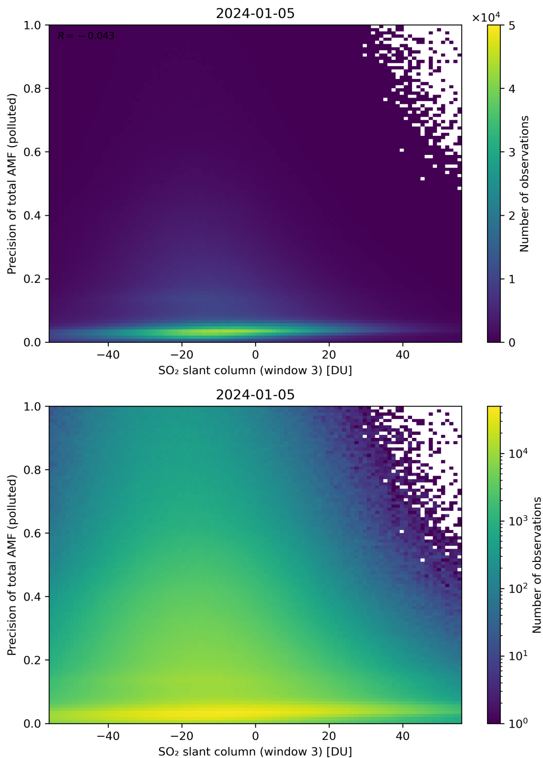
Figure 269: Scatter density plot of “SO 2 slant column (window 3)” against “Precision of total AMF (polluted)” for 2024-01-05 to 2024-01-06.
