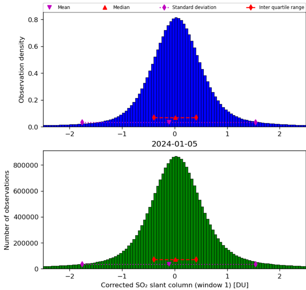
Figure 58: Histogram of “Corrected SO 2 slant column (window 1)” for 2024-01-05 to 2024-01-06
