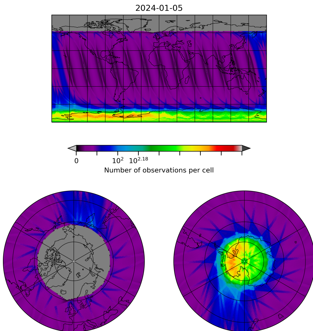
Figure 28: Map of the number of observations for 2024-01-05 to 2024-01-06
