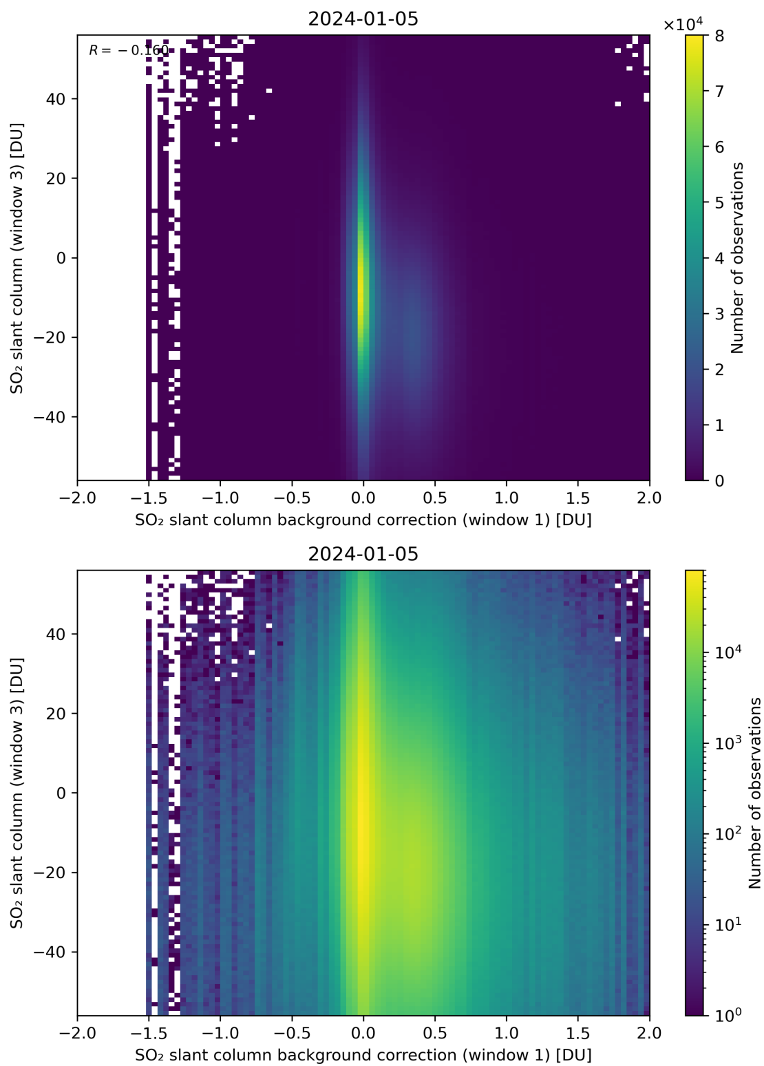
Figure 107: Scatter density plot of “SO 2 slant column background correction (window 1)” against “SO 2 slant column (window 3)” for 2024-01-05 to 2024-01-06.
