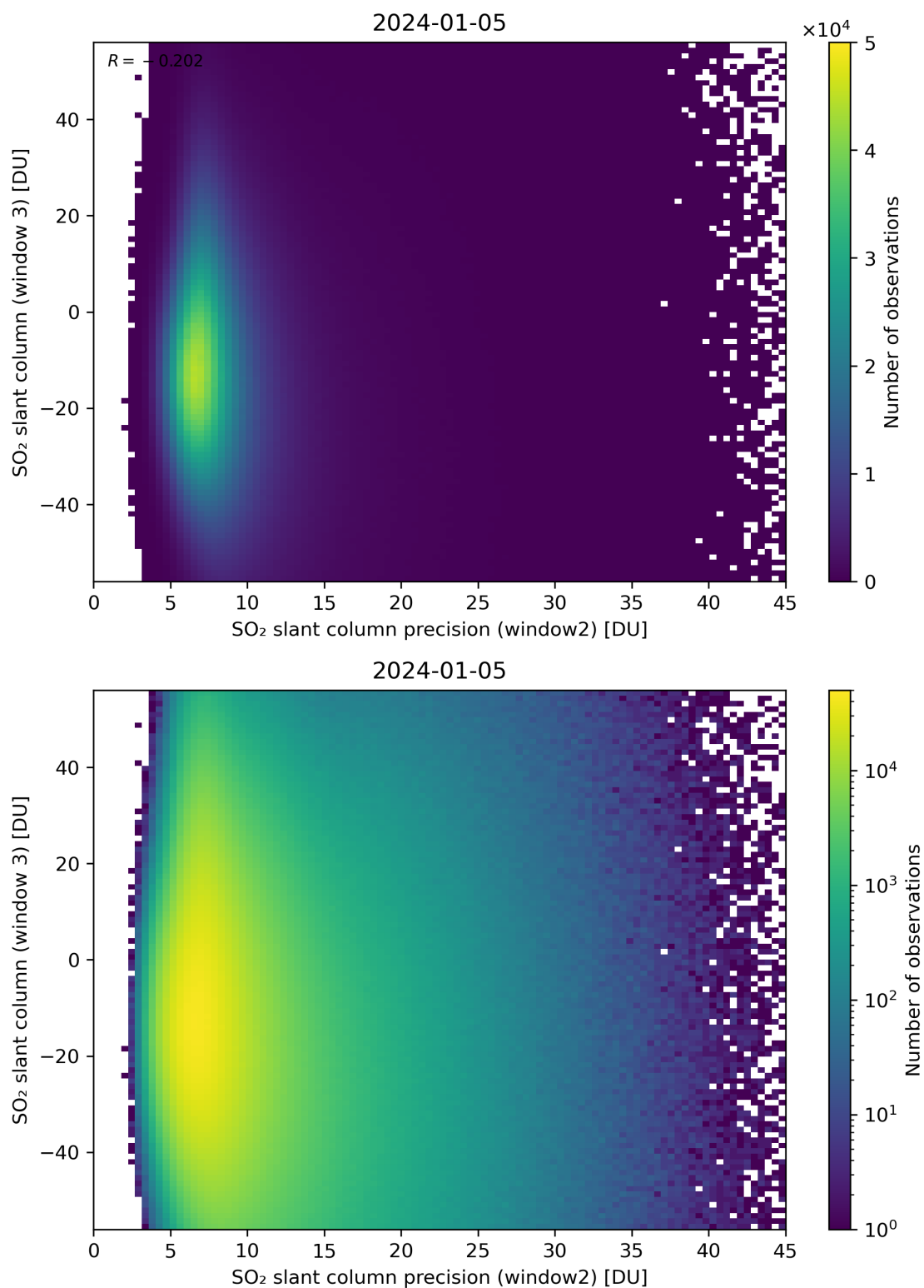
Figure 249: Scatter density plot of “SO 2 slant column precision (window2)” against “SO 2 slant column (window 3)” for 2024-01-05 to 2024-01-06.
