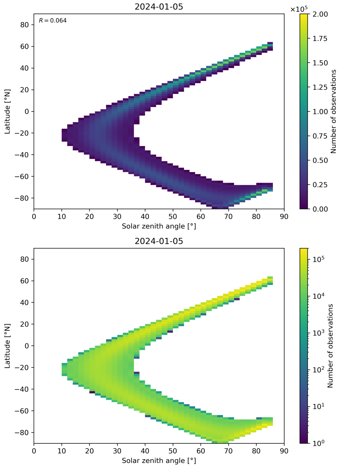
Figure 164: Scatter density plot of “Solar zenith angle” against “Latitude” for 2024-01-05 to 2024-01-06.
