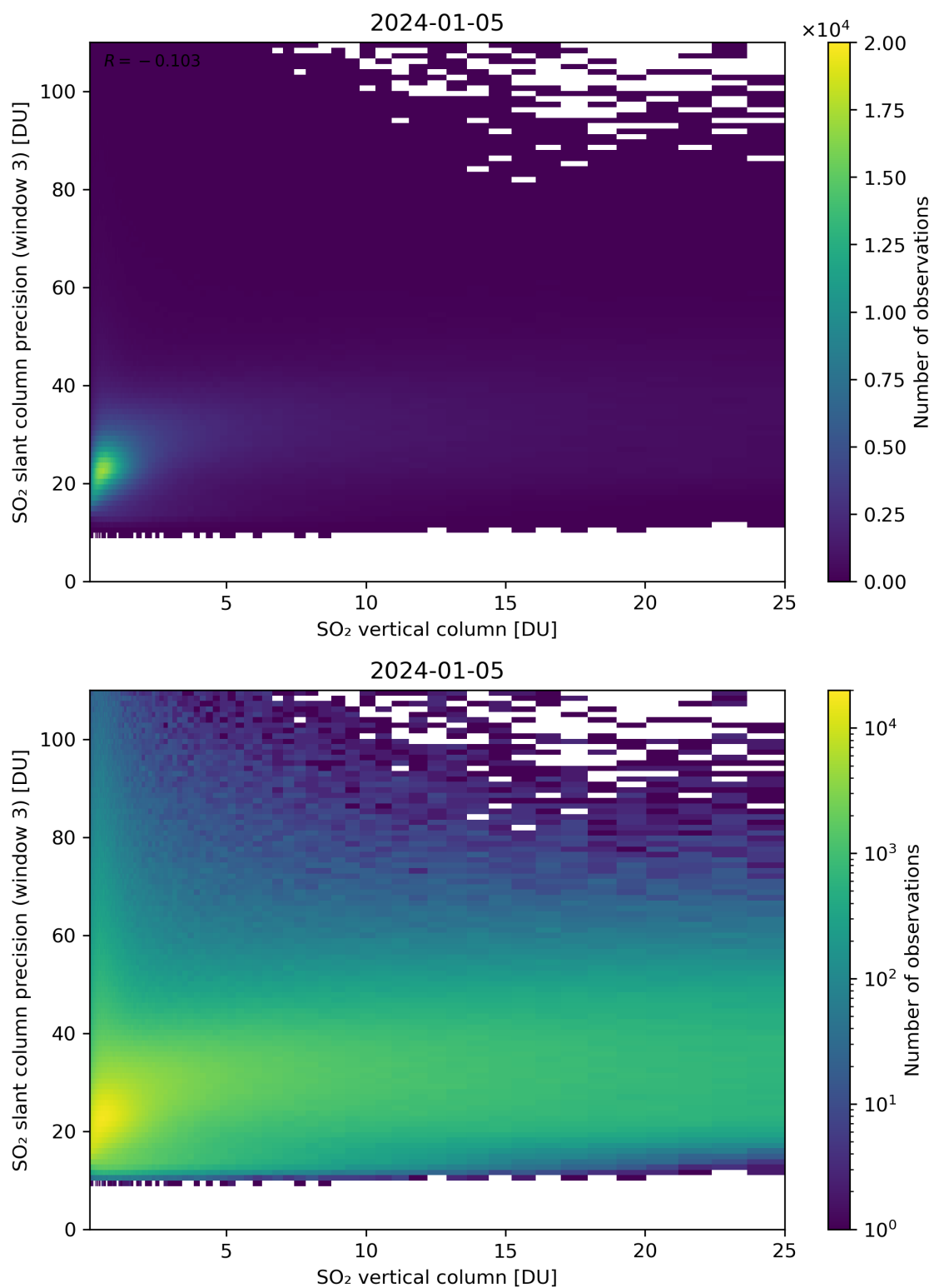
Figure 304: Scatter density plot of “SO 2 vertical column” against “SO 2 slant column precision (window 3)” for 2024-01-05 to 2024-01-06.
