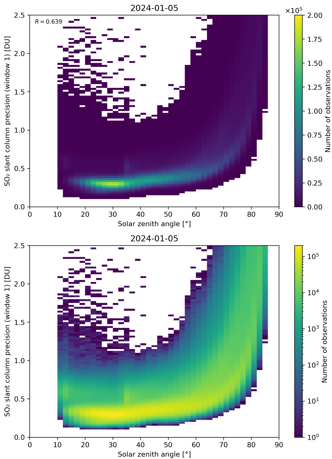
Figure 170: Scatter density plot of “Solar zenith angle” against “SO 2 slant column precision (window 1)” for 2024-01-05 to 2024-01-06.
