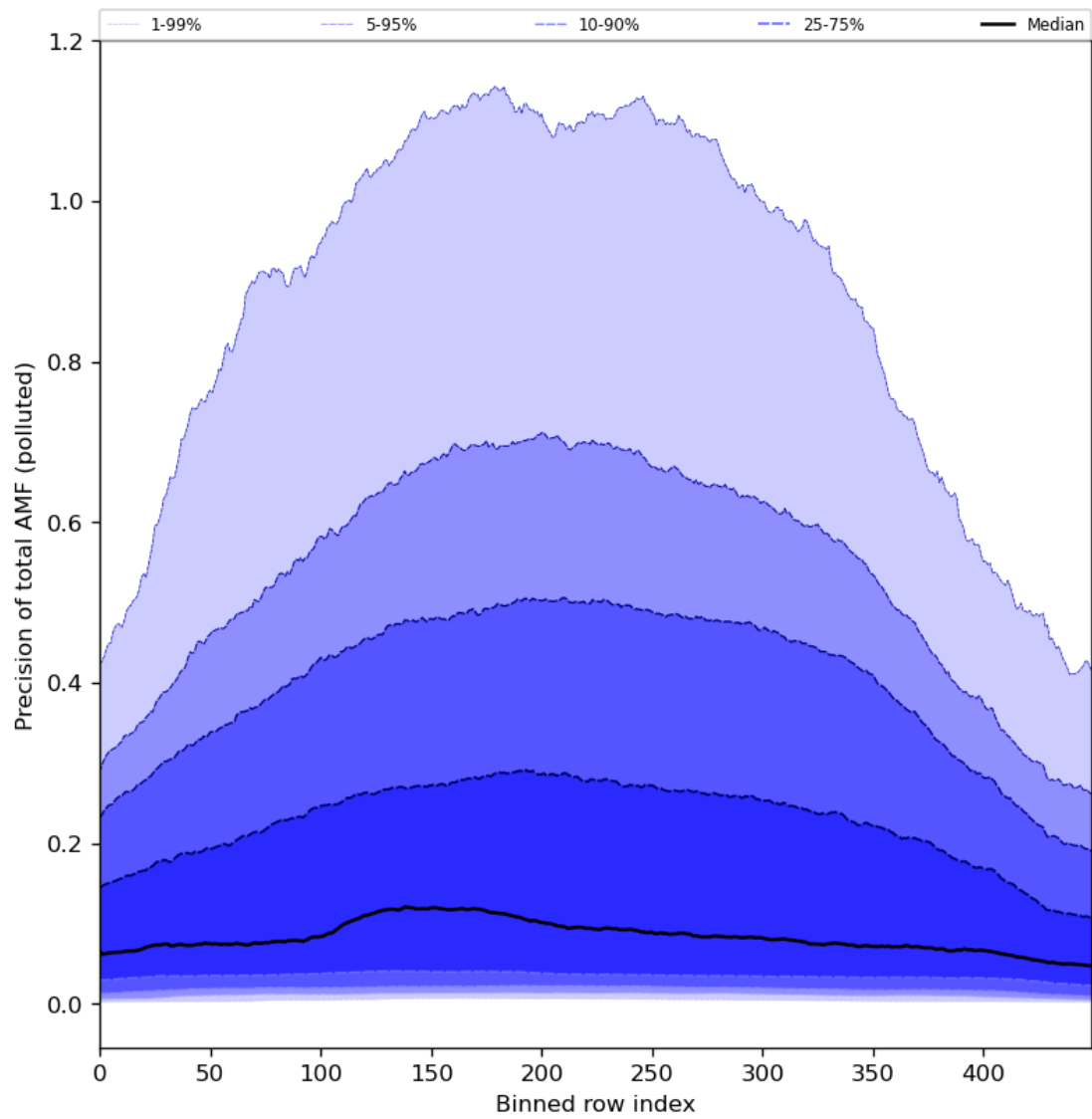
Figure 95: Along track statistics of “Precision of total AMF (polluted)” for 2024-01-05 to 2024-01-06
