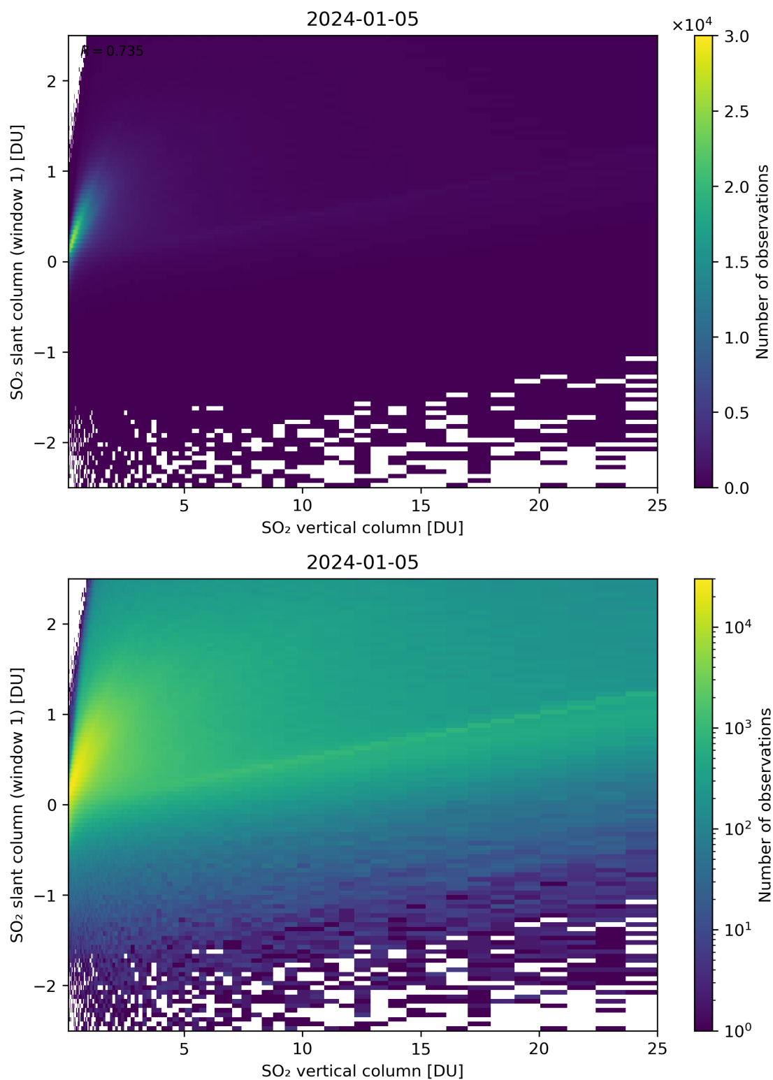
Figure 300: Scatter density plot of “SO 2 vertical column” against “SO 2 slant column (window 1)” for 2024-01-05 to 2024-01-06.
