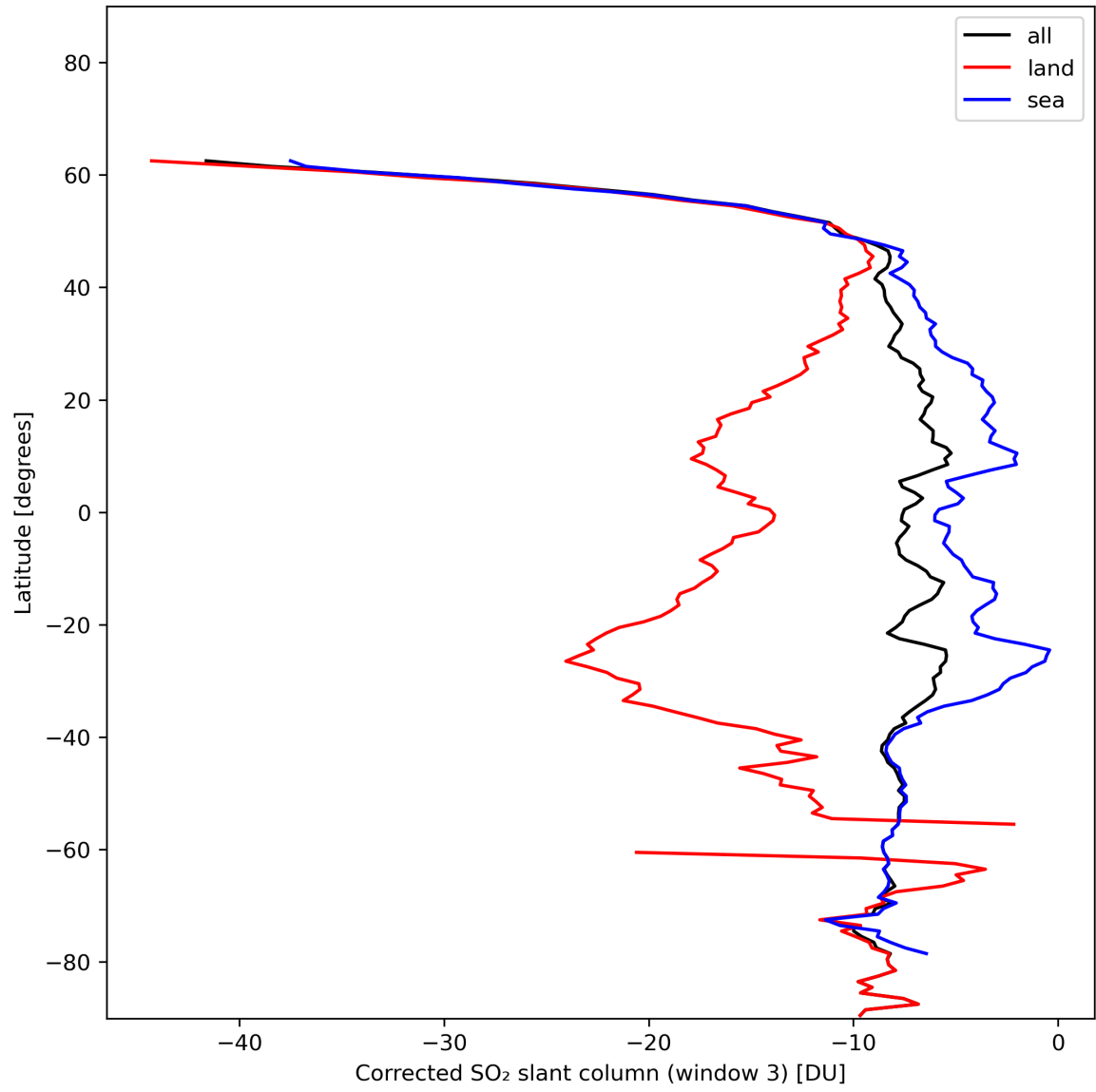
Figure 43: Zonal average of “Corrected SO 2 slant column (window 3)” for 2024-01-05 to 2024-01-06.
