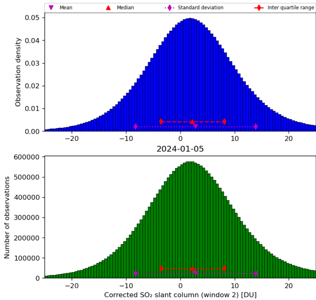
Figure 62: Histogram of “Corrected SO 2 slant column (window 2)” for 2024-01-05 to 2024-01-06
