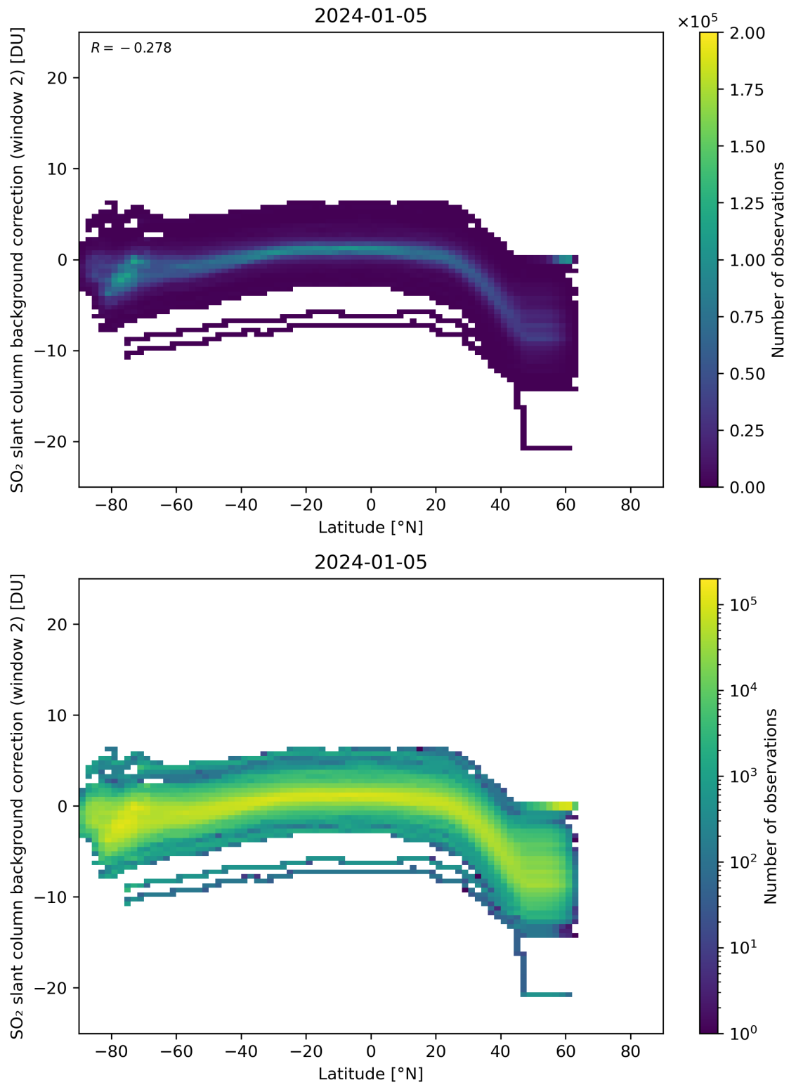
Figure 140: Scatter density plot of “Latitude” against “SO 2 slant column background correction (window 2)” for 2024-01-05 to 2024-01-06.
