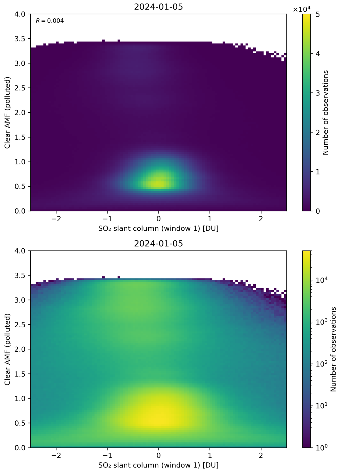
Figure 232: Scatter density plot of “SO 2 slant column (window 1)” against “Clear AMF (polluted)” for 2024-01-05 to 2024-01-06.
