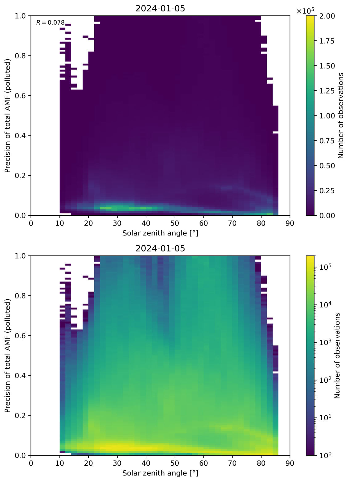
Figure 175: Scatter density plot of “Solar zenith angle” against “Precision of total AMF (polluted)” for 2024-01-05 to 2024-01-06.
