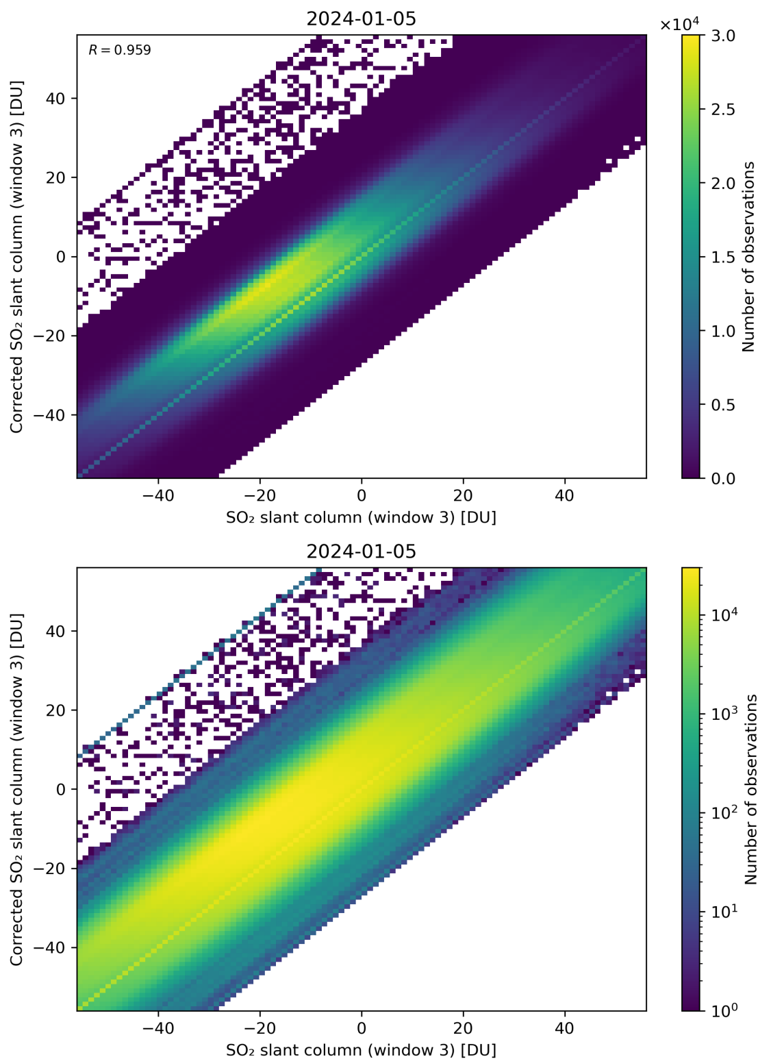
Figure 266: Scatter density plot of “SO 2 slant column (window 3)” against “Corrected SO 2 slant column (window 3)” for 2024-01-05 to 2024-01-06.
