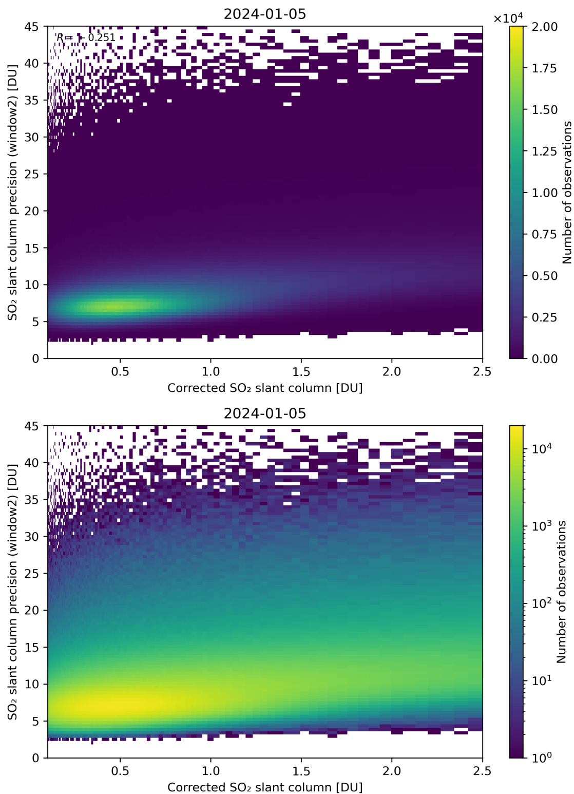
Figure 189: Scatter density plot of “Corrected SO 2 slant column” against “SO 2 slant column precision (window2)” for 2024-01-05 to 2024-01-06.
