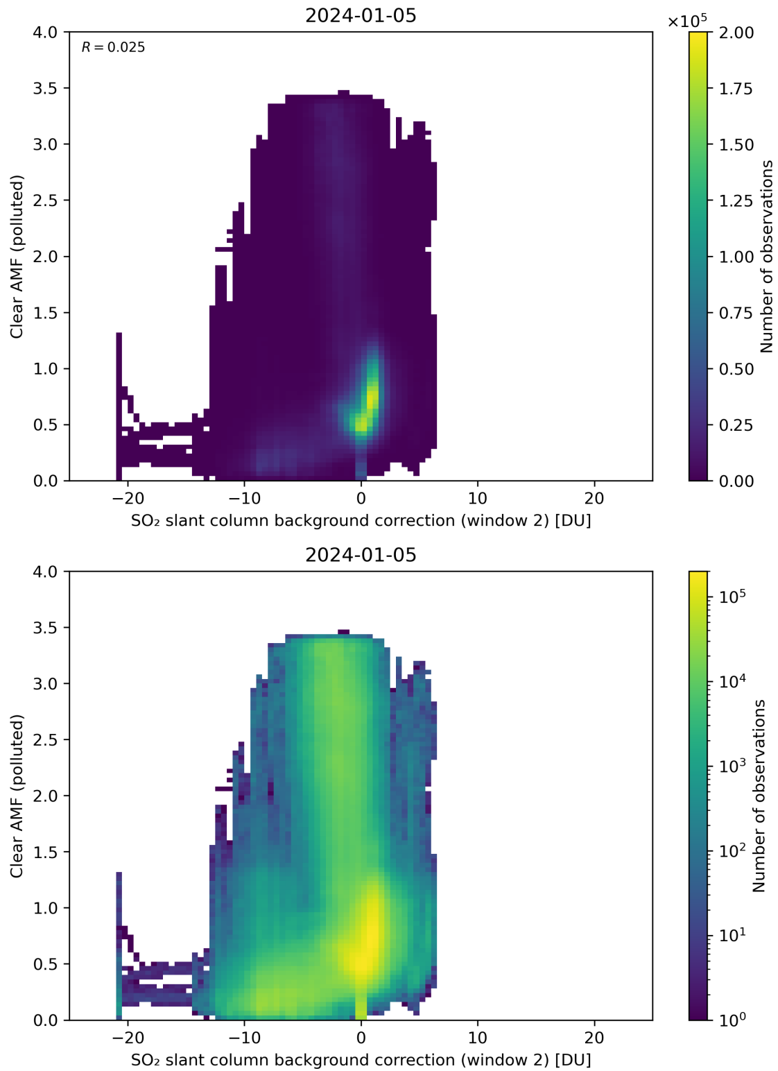
Figure 115: Scatter density plot of “SO 2 slant column background correction (window 2)” against “Clear AMF (polluted)” for 2024-01-05 to 2024-01-06.
