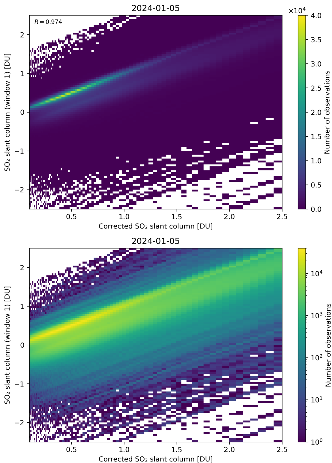
Figure 187: Scatter density plot of “Corrected SO 2 slant column” against “SO 2 slant column (window 1)” for 2024-01-05 to 2024-01-06.
