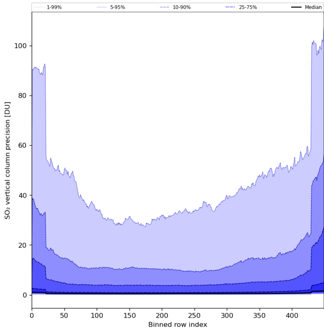
Figure 77: Along track statistics of “SO 2 vertical column precision” for 2024-01-05 to 2024-01-06
