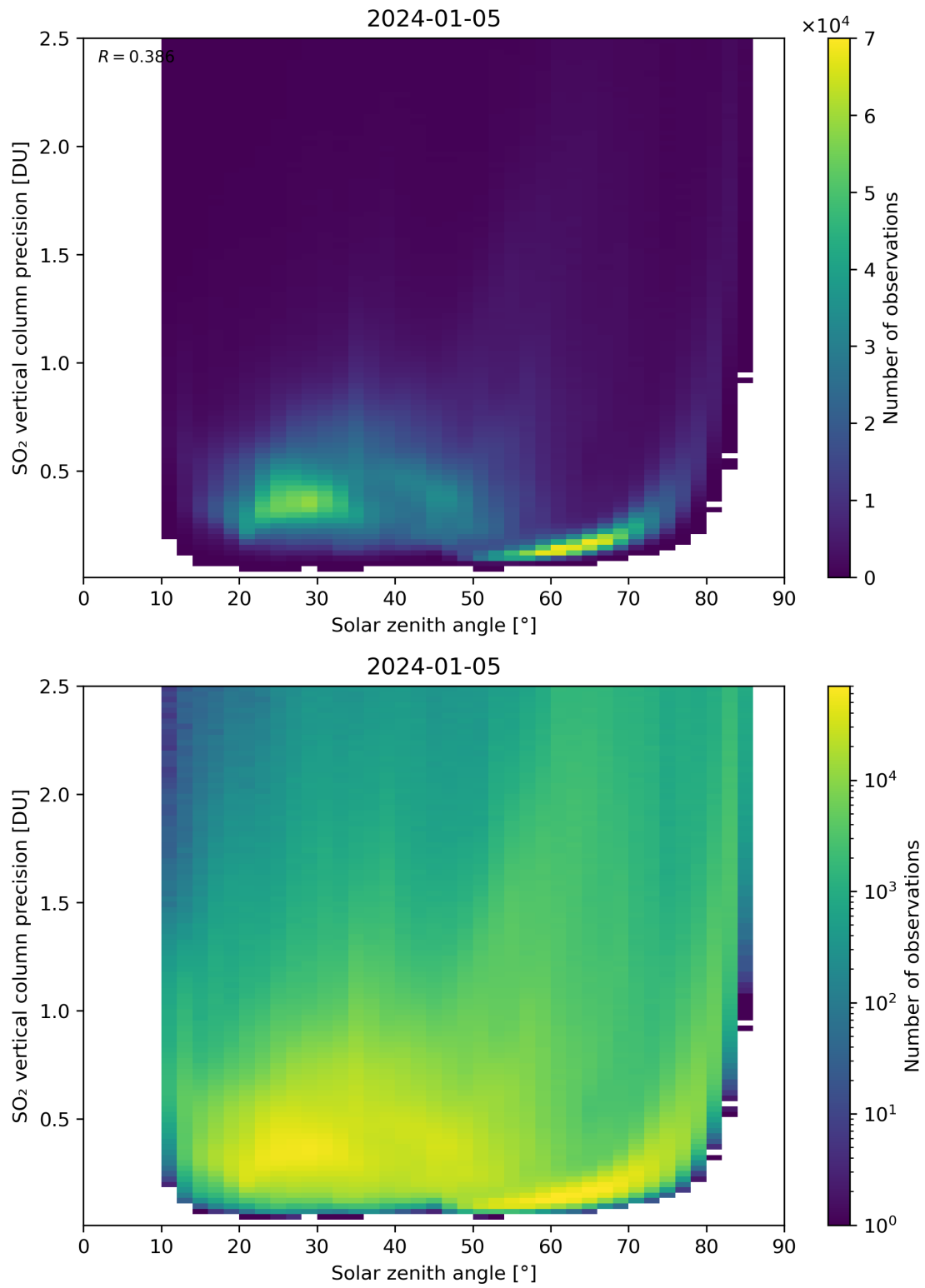
Figure 177: Scatter density plot of “Solar zenith angle” against “SO 2 vertical column precision” for 2024-01-05 to 2024-01-06.
