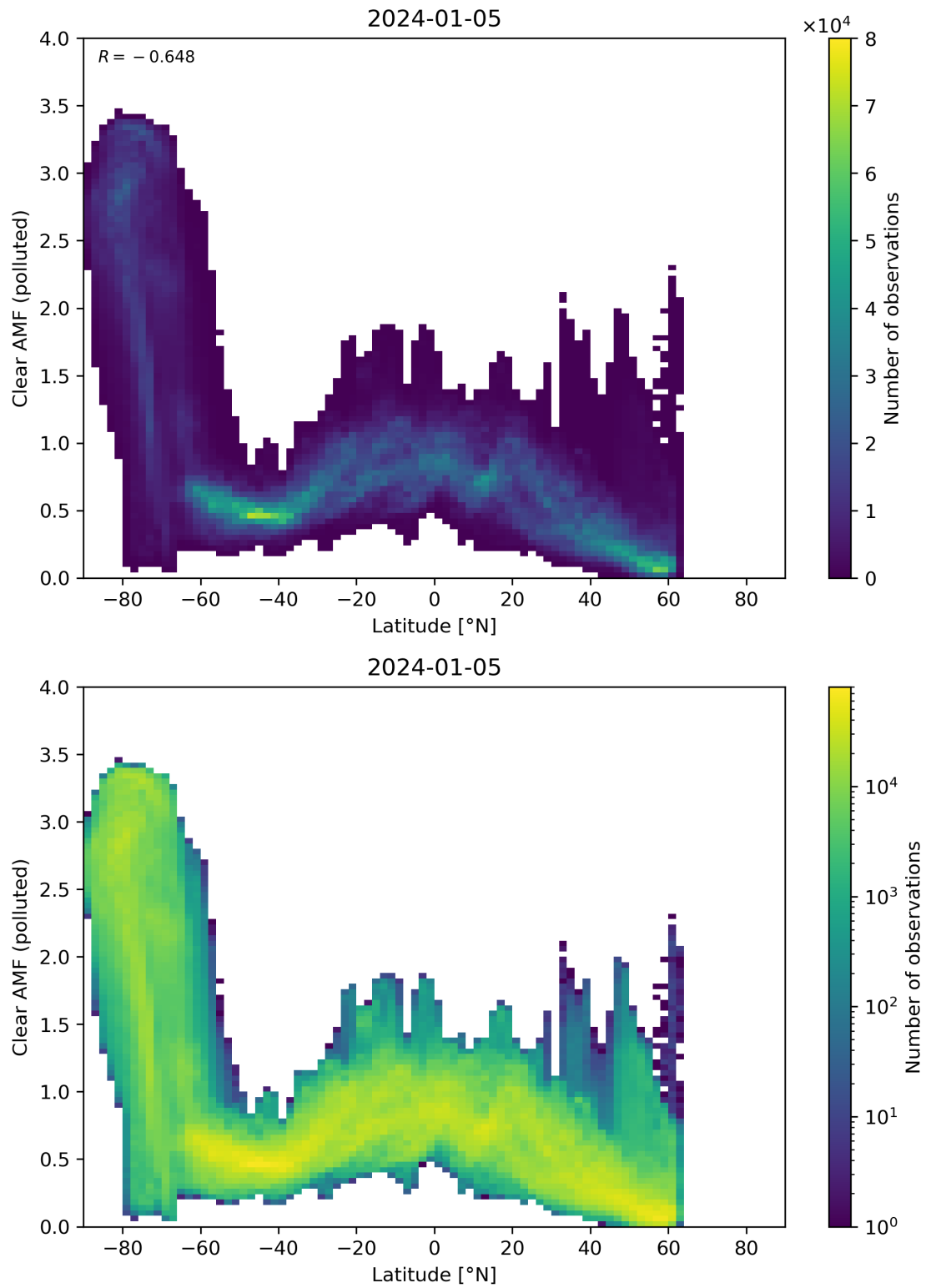
Figure 145: Scatter density plot of “Latitude” against “Clear AMF (polluted)” for 2024-01-05 to 2024-01-06.
