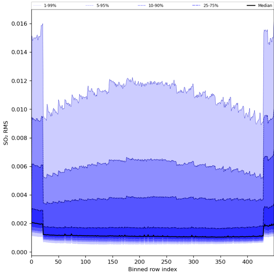
Figure 93: Along track statistics of “SO 2 RMS” for 2024-01-05 to 2024-01-06
