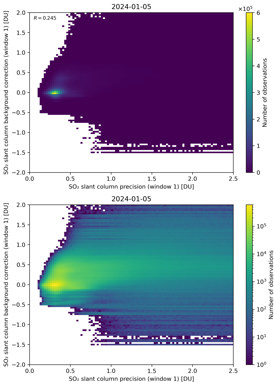
Figure 218: Scatter density plot of “SO 2 slant column precision (window 1)” against “SO 2 slant column background correction (window 1)” for 2024-01-05 to 2024-01-06.
