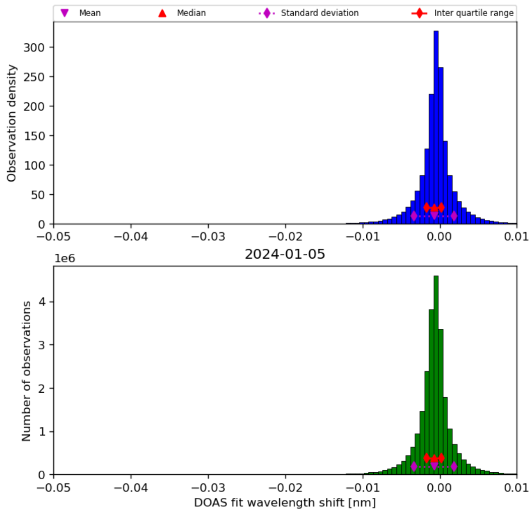
Figure 68: Histogram of “DOAS fit wavelength shift” for 2024-01-05 to 2024-01-06
