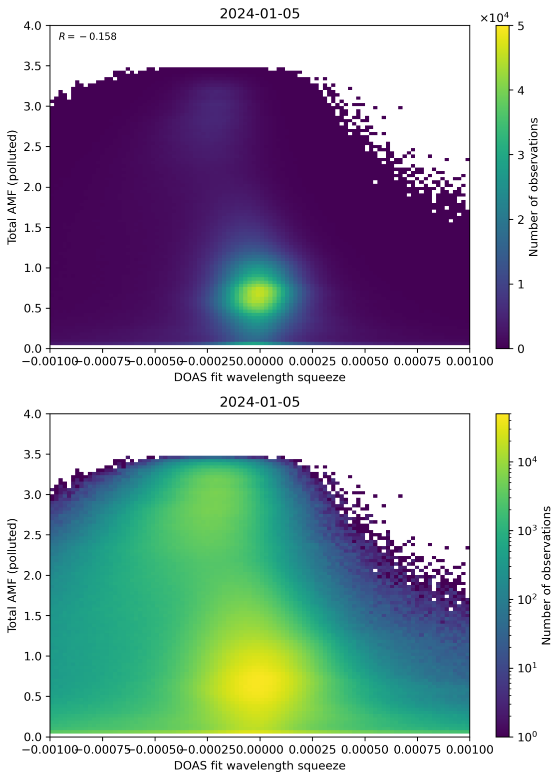
Figure 134: Scatter density plot of “DOAS fit wavelength squeeze” against “Total AMF (polluted)” for 2024-01-05 to 2024-01-06.
