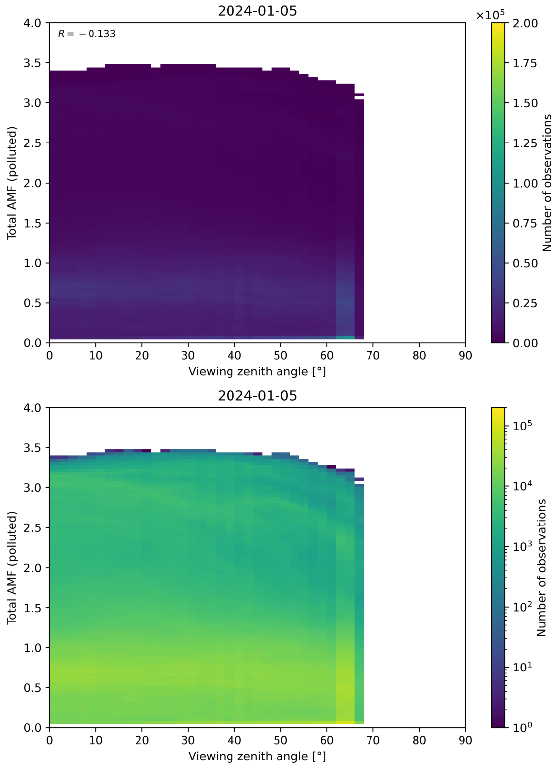
Figure 325: Scatter density plot of “Viewing zenith angle” against “Total AMF (polluted)” for 2024-01-05 to 2024-01-06.
