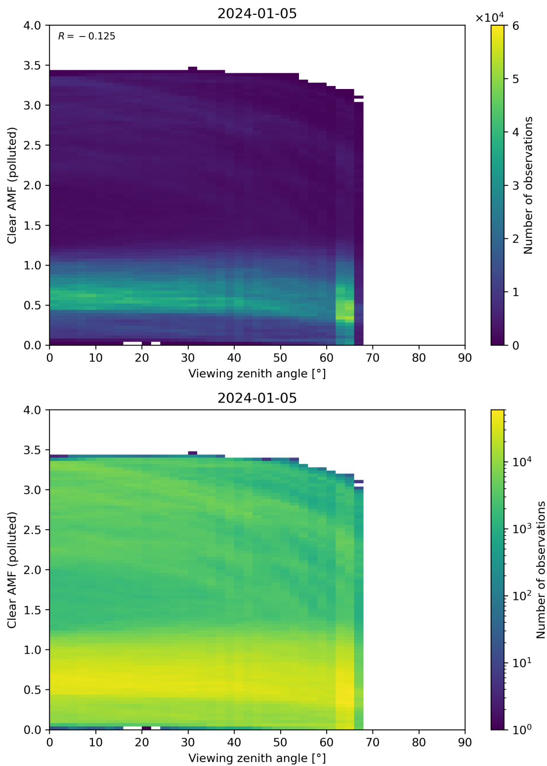
Figure 316: Scatter density plot of “Viewing zenith angle” against “Clear AMF (polluted)” for 2024-01-05 to 2024-01-06.
