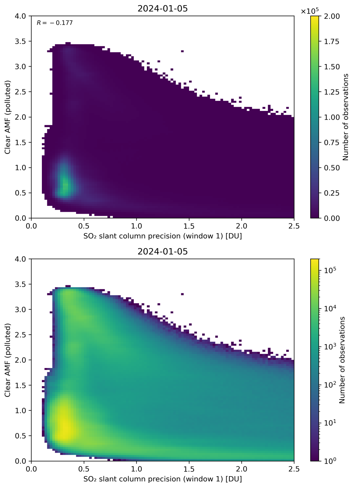
Figure 224: Scatter density plot of “SO 2 slant column precision (window 1)” against “Clear AMF (polluted)” for 2024-01-05 to 2024-01-06.
