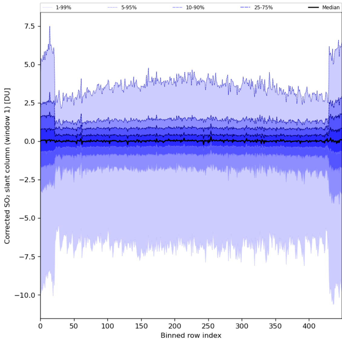
Figure 81: Along track statistics of “Corrected SO 2 slant column (window 1)” for 2024-01-05 to 2024-01-06
