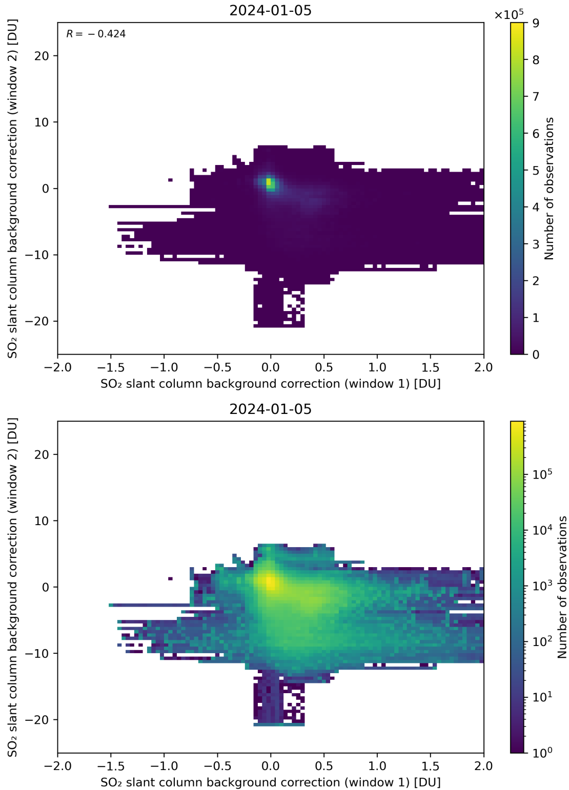
Figure 98: Scatter density plot of “SO 2 slant column background correction (window 1)” against “SO 2 slant column background correction (window 2)” for 2024-01-05 to 2024-01-06.
