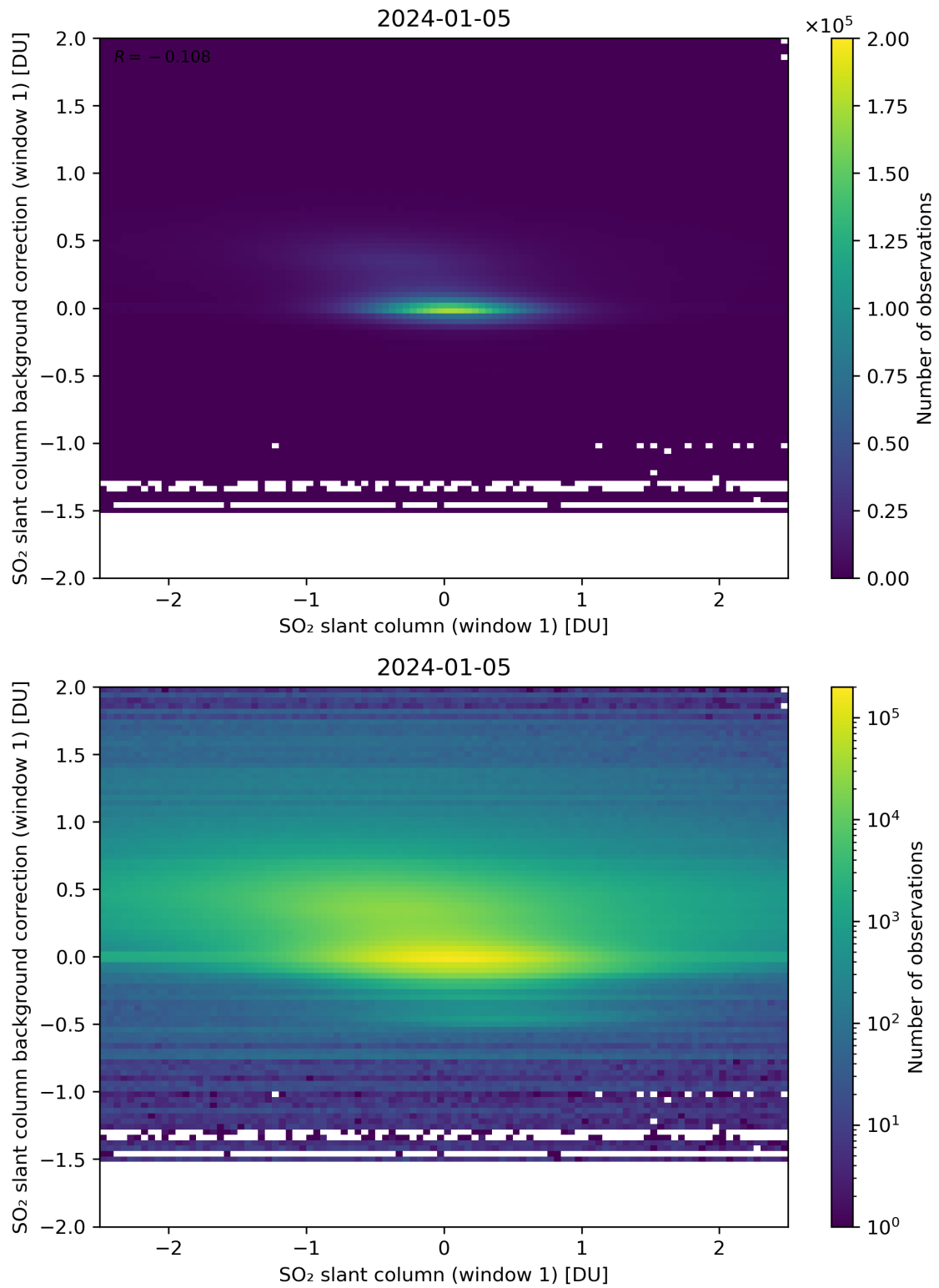
Figure 212: Scatter density plot of “SO 2 slant column (window 1)” against “SO 2 slant column background correction (window 1)” for 2024-01-05 to 2024-01-06.
