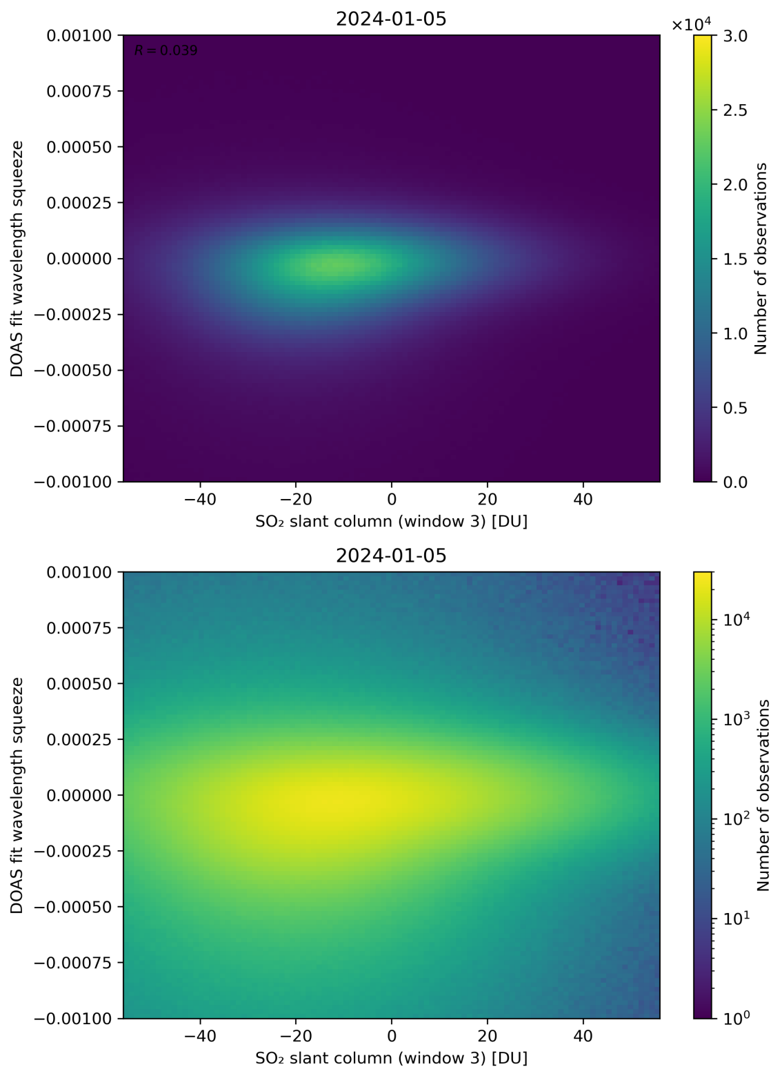
Figure 255: Scatter density plot of “SO 2 slant column (window 3)” against “DOAS fit wavelength squeeze” for 2024-01-05 to 2024-01-06.
