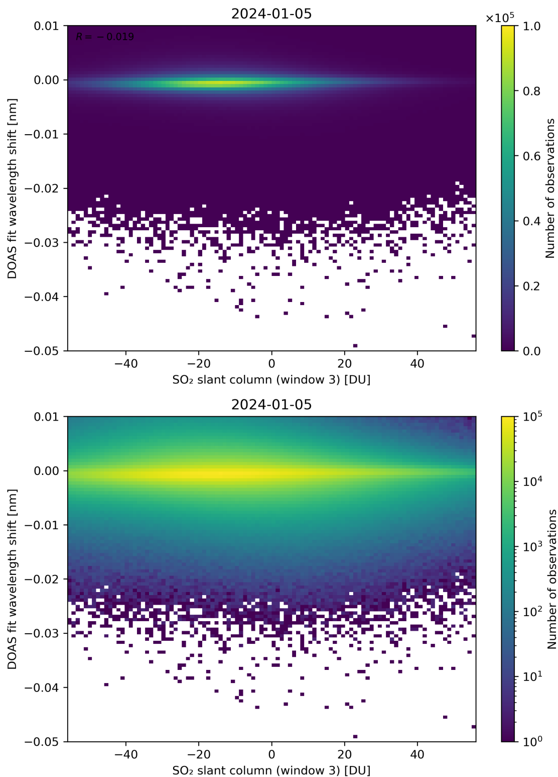
Figure 254: Scatter density plot of “SO 2 slant column (window 3)” against “DOAS fit wavelength shift” for 2024-01-05 to 2024-01-06.
