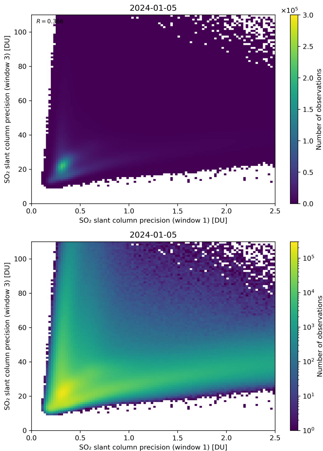
Figure 229: Scatter density plot of “SO 2 slant column precision (window 1)” against “SO 2 slant column precision (window 3)” for 2024-01-05 to 2024-01-06.
