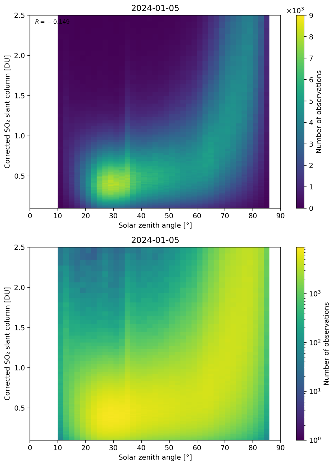
Figure 166: Scatter density plot of “Solar zenith angle” against “Corrected SO 2 slant column” for 2024-01-05 to 2024-01-06.
