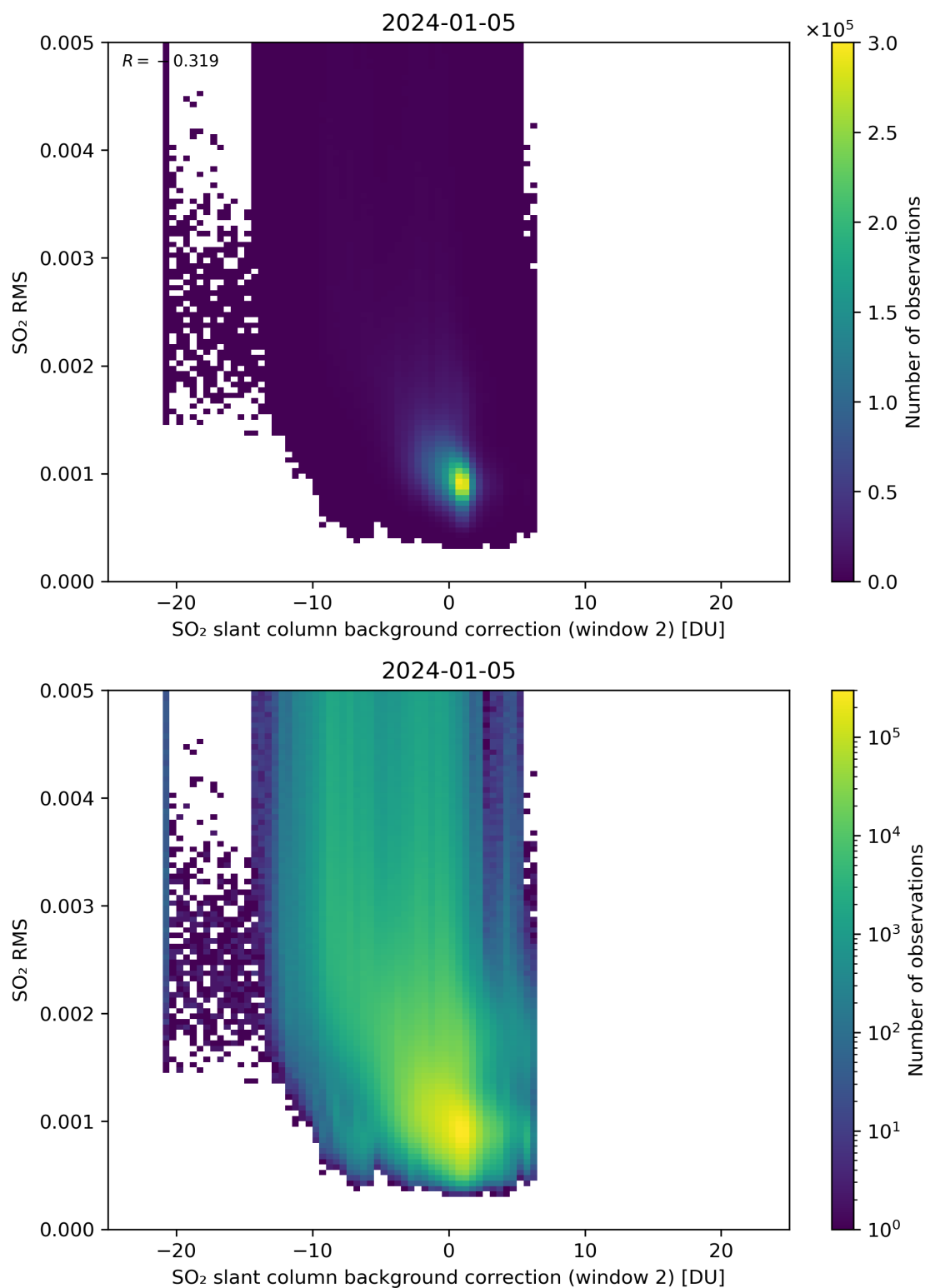
Figure 114: Scatter density plot of “SO 2 slant column background correction (window 2)” against “SO 2 RMS” for 2024-01-05 to 2024-01-06.
