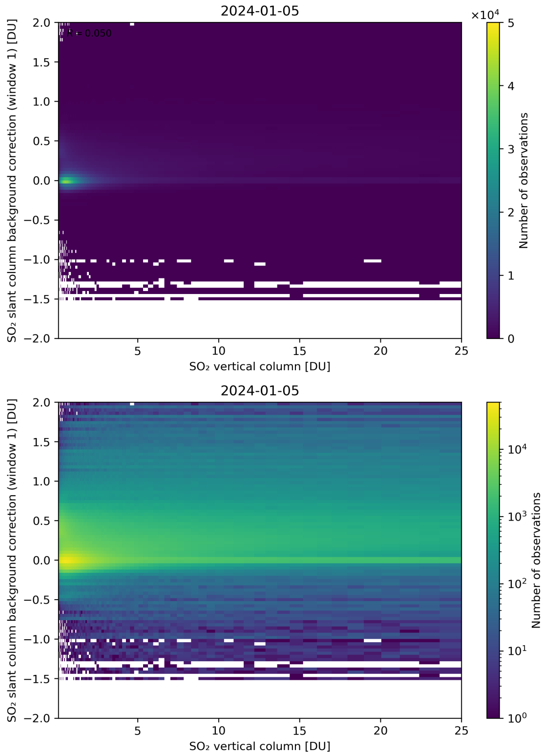
Figure 273: Scatter density plot of “SO 2 vertical column” against “SO 2 slant column background correction (window 1)” for 2024-01-05 to 2024-01-06.
