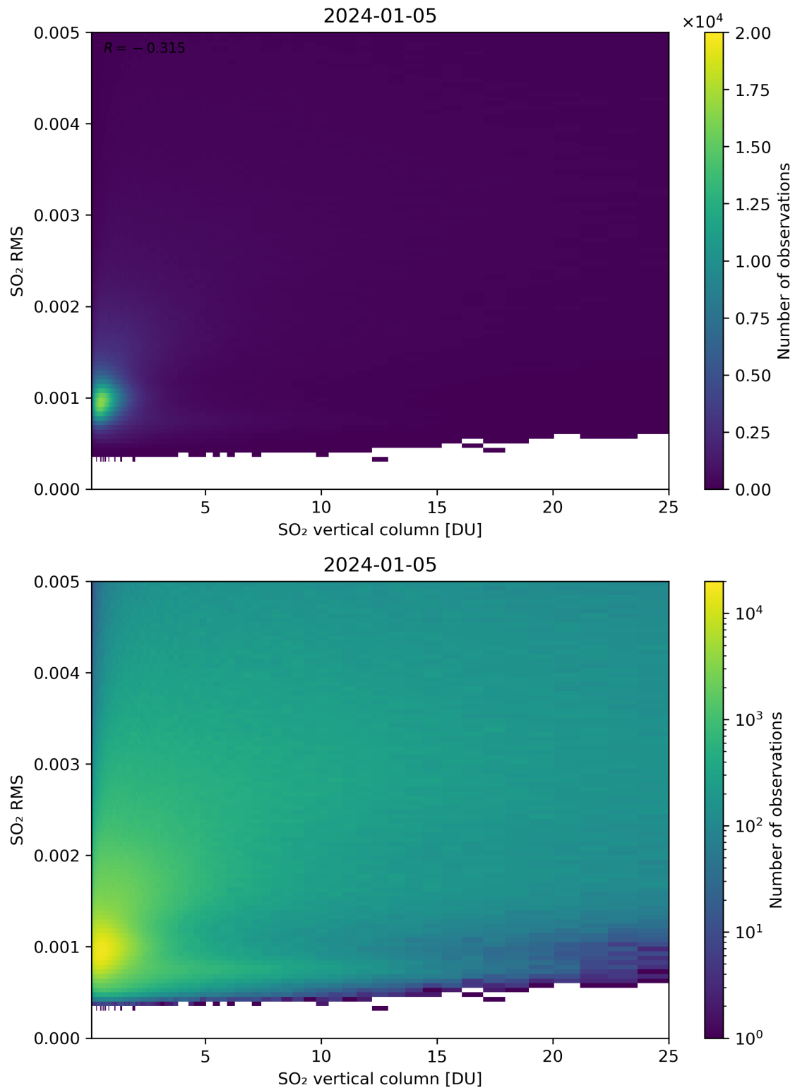
Figure 278: Scatter density plot of “SO 2 vertical column” against “SO 2 RMS” for 2024-01-05 to 2024-01-06.
