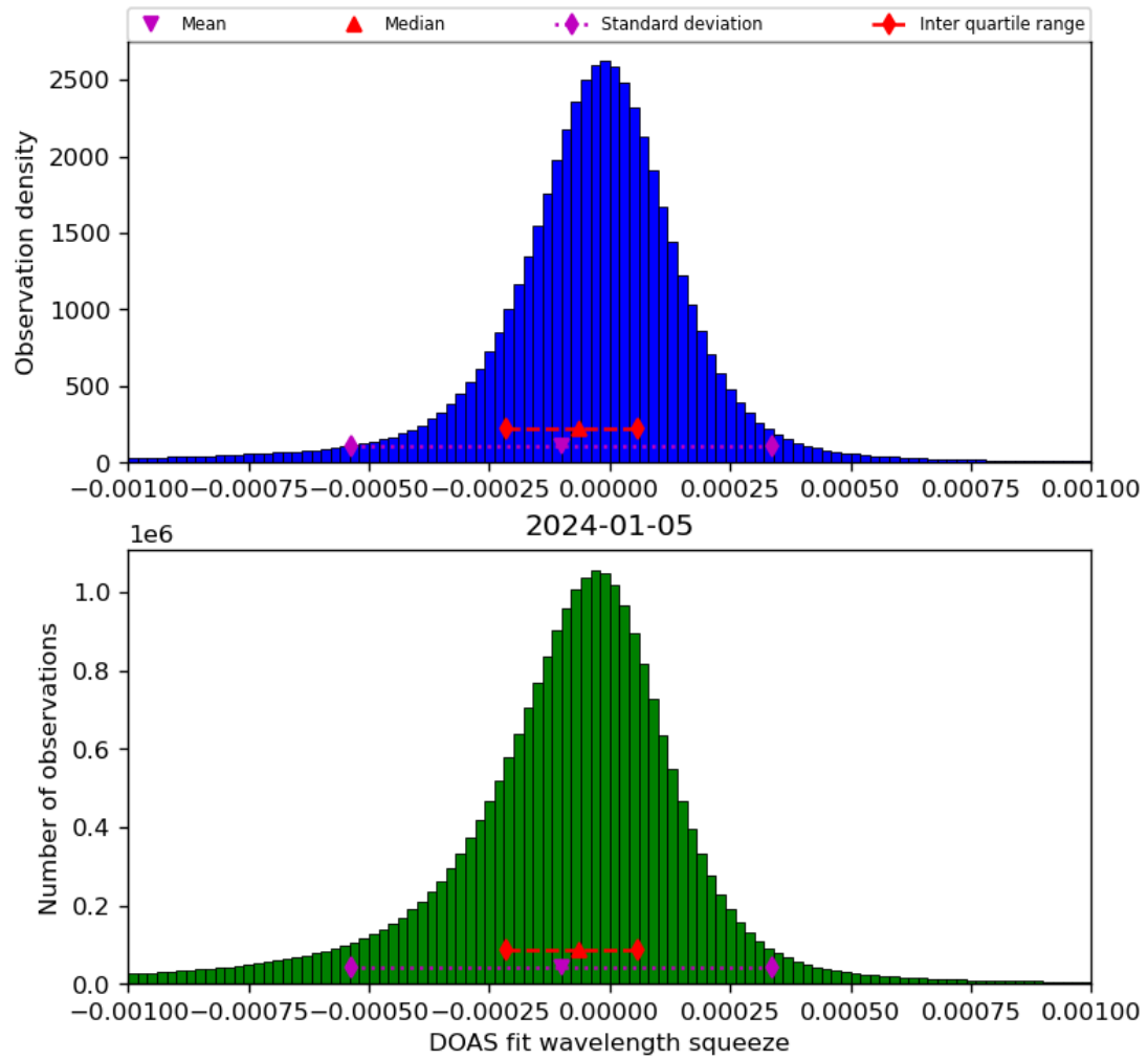
Figure 69: Histogram of “DOAS fit wavelength squeeze” for 2024-01-05 to 2024-01-06
