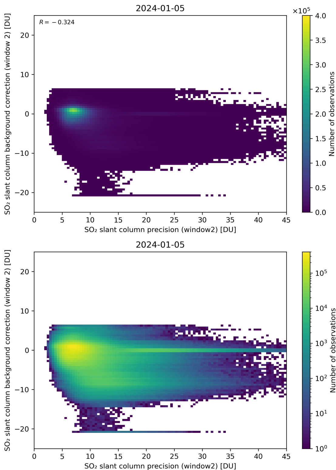
Figure 241: Scatter density plot of “SO 2 slant column precision (window2)” against “SO 2 slant column background correction (window 2)” for 2024-01-05 to 2024-01-06.
