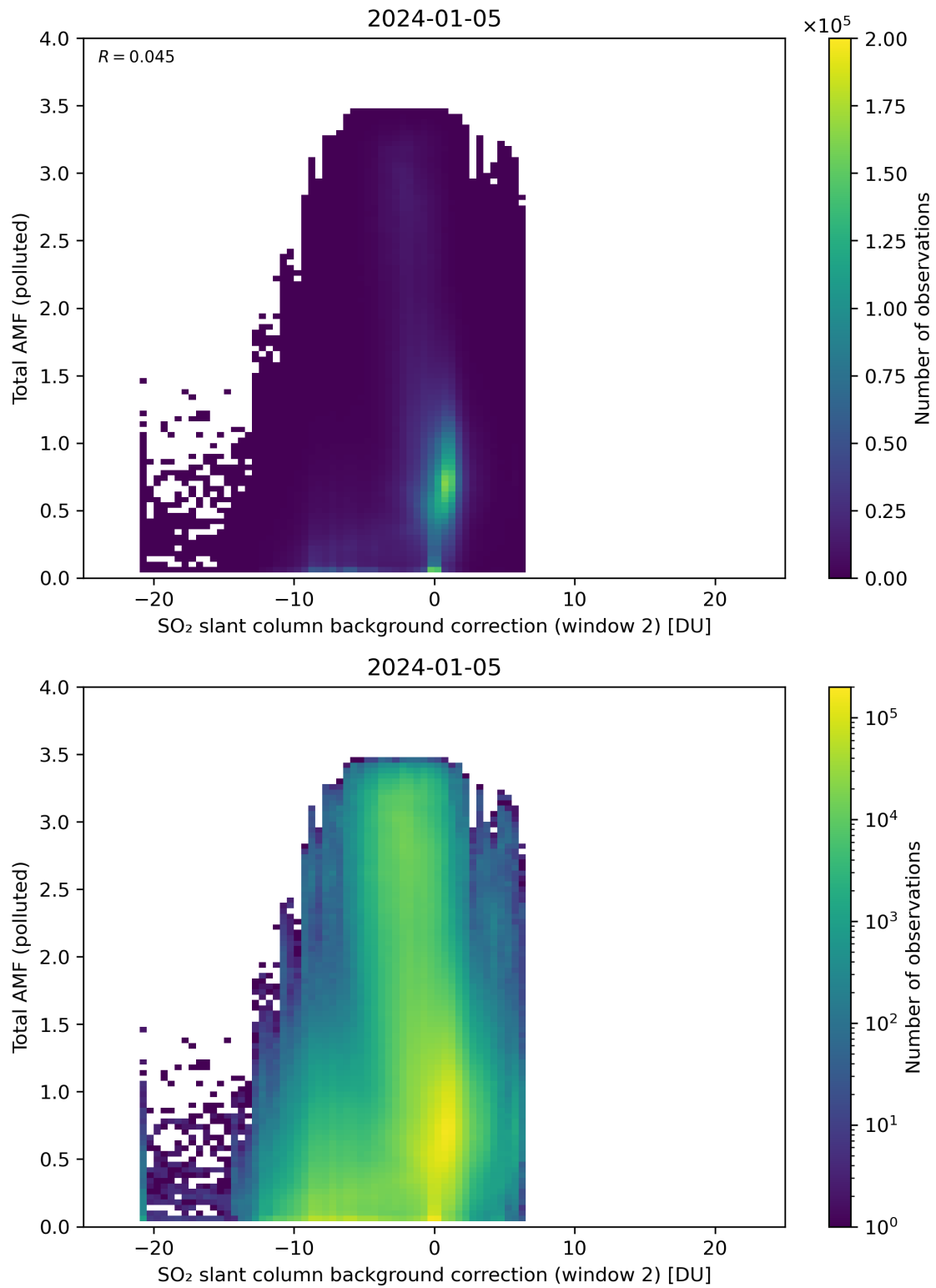
Figure 119: Scatter density plot of “SO 2 slant column background correction (window 2)” against “Total AMF (polluted)” for 2024-01-05 to 2024-01-06.
