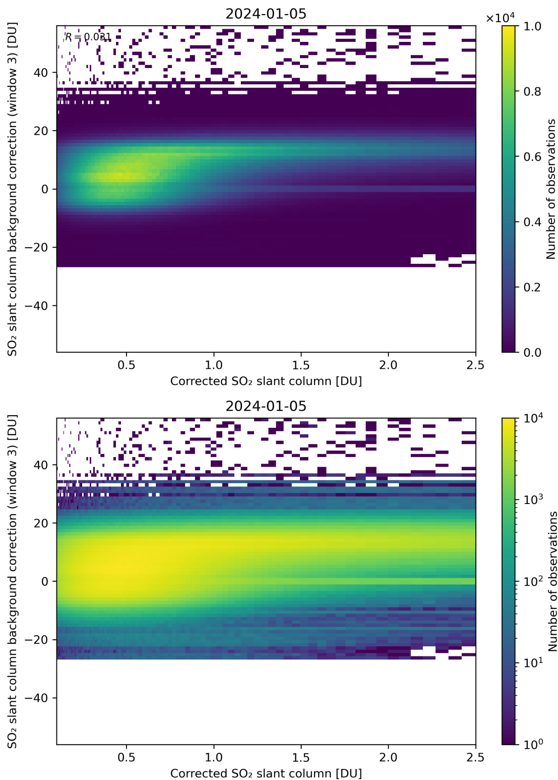
Figure 180: Scatter density plot of “Corrected SO 2 slant column” against “SO 2 slant column background correction (window 3)” for 2024-01-05 to 2024-01-06.
