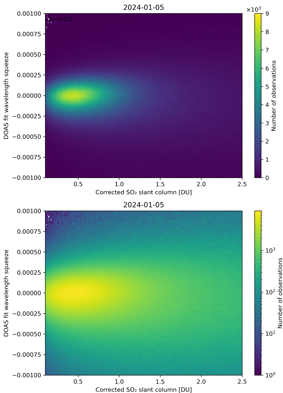
Figure 182: Scatter density plot of “Corrected SO 2 slant column” against “DOAS fit wavelength squeeze” for 2024-01-05 to 2024-01-06.
