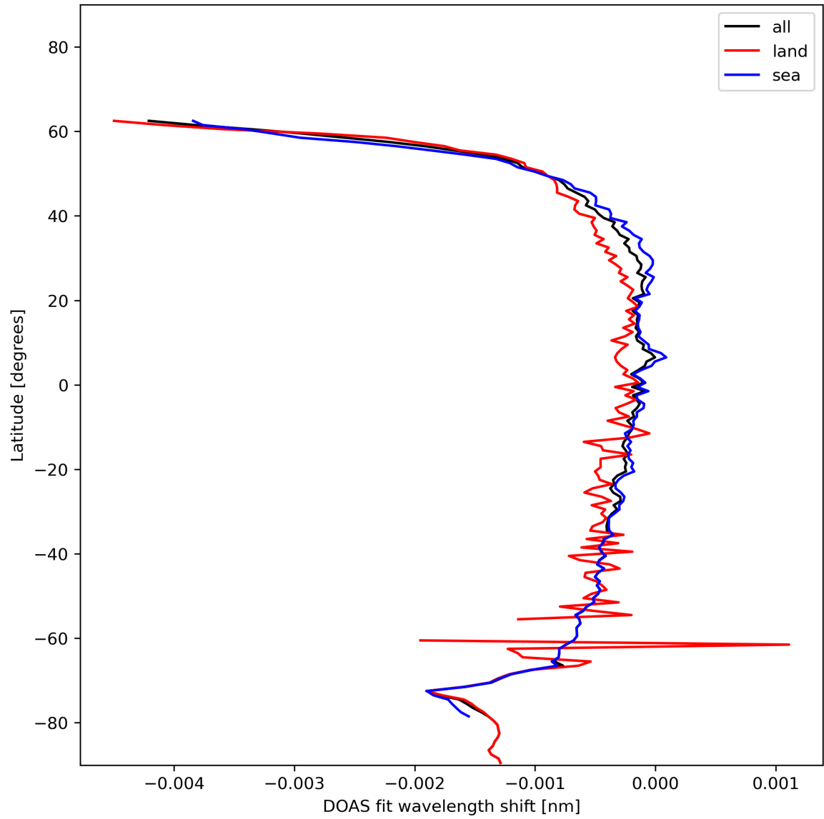
Figure 45: Zonal average of “DOAS fit wavelength shift” for 2024-01-05 to 2024-01-06.
