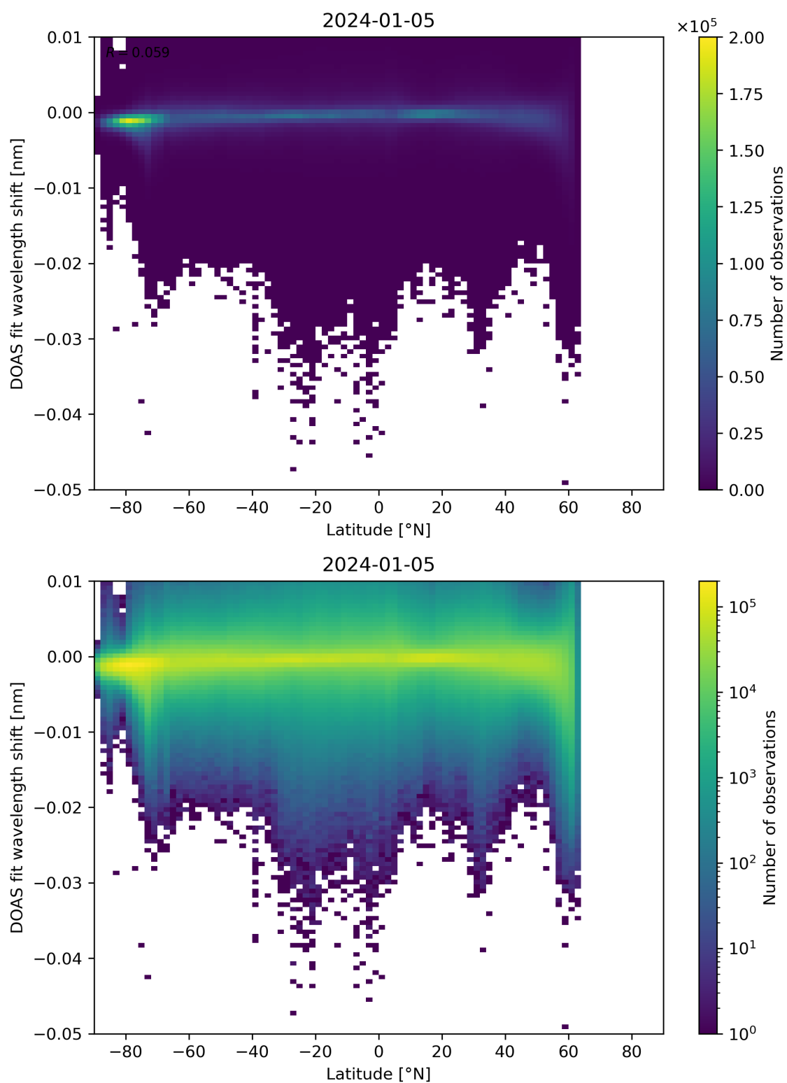
Figure 142: Scatter density plot of “Latitude” against “DOAS fit wavelength shift” for 2024-01-05 to 2024-01-06.
