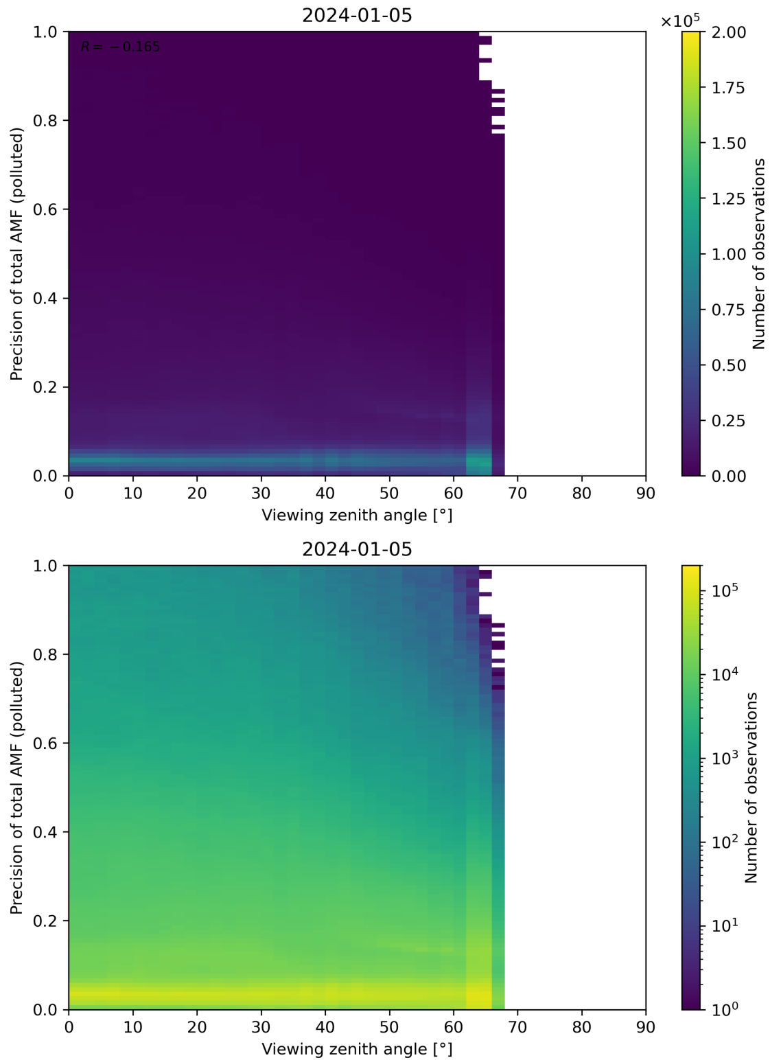
Figure 326: Scatter density plot of “Viewing zenith angle” against “Precision of total AMF (polluted)” for 2024-01-05 to 2024-01-06.
