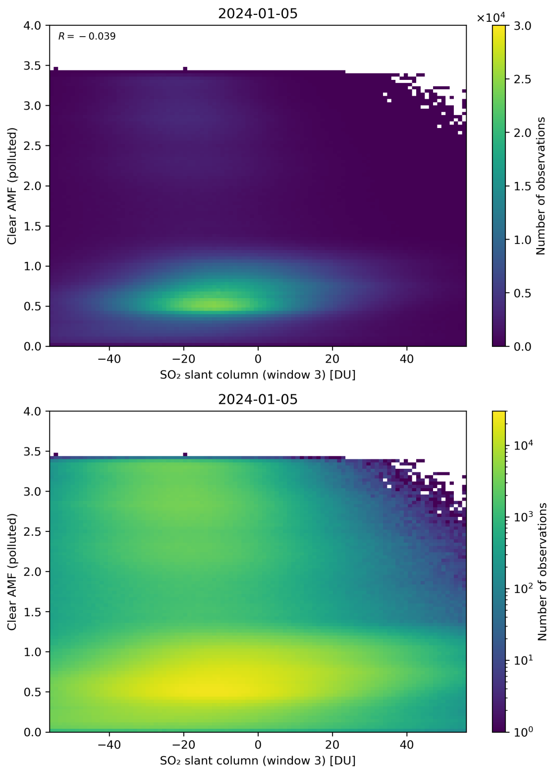
Figure 265: Scatter density plot of “SO 2 slant column (window 3)” against “Clear AMF (polluted)” for 2024-01-05 to 2024-01-06.
