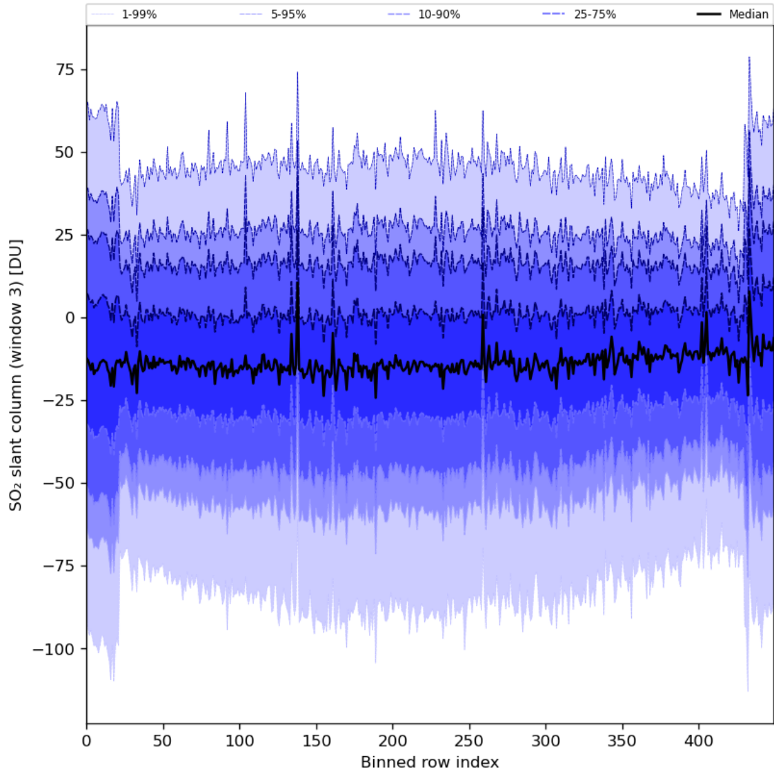
Figure 87: Along track statistics of “SO 2 slant column (window 3)” for 2024-01-05 to 2024-01-06
