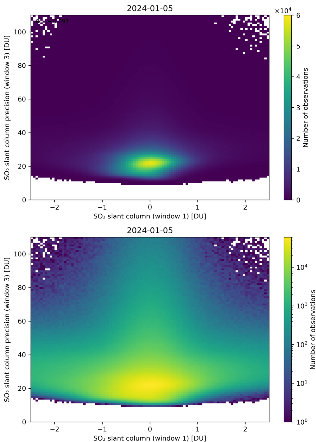
Figure 238: Scatter density plot of “SO 2 slant column (window 1)” against “SO 2 slant column precision (window 3)” for 2024-01-05 to 2024-01-06.
