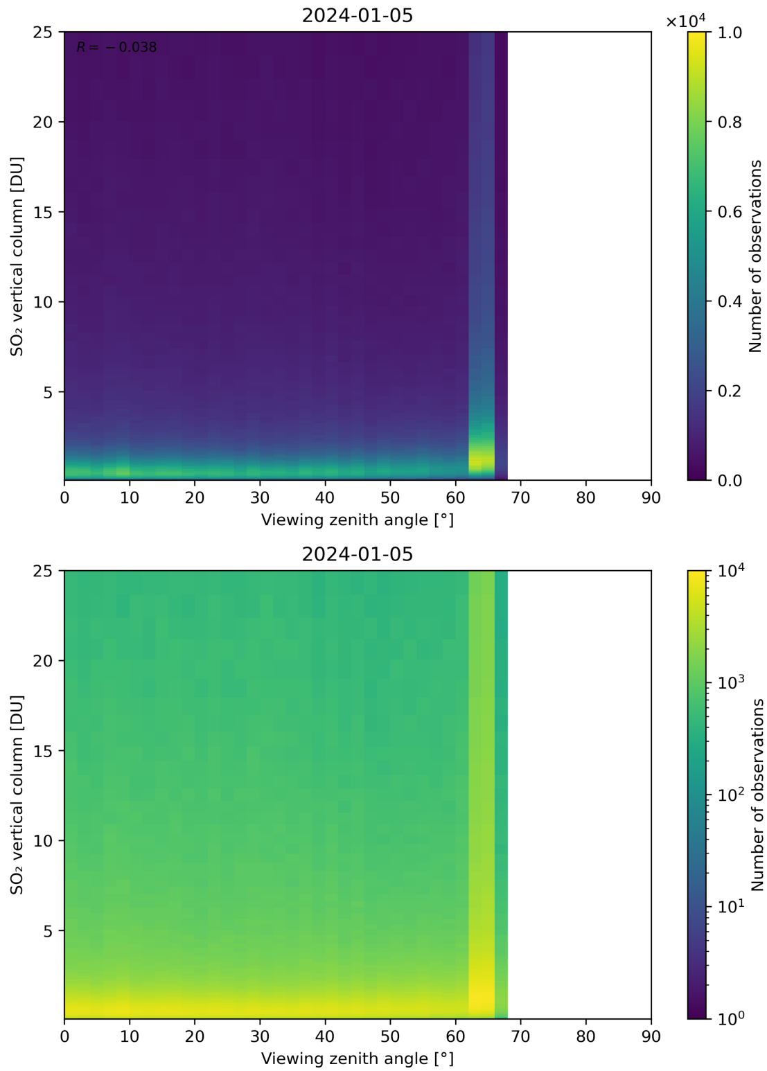
Figure 327: Scatter density plot of “Viewing zenith angle” against “SO 2 vertical column” for 2024-01-05 to 2024-01-06.
