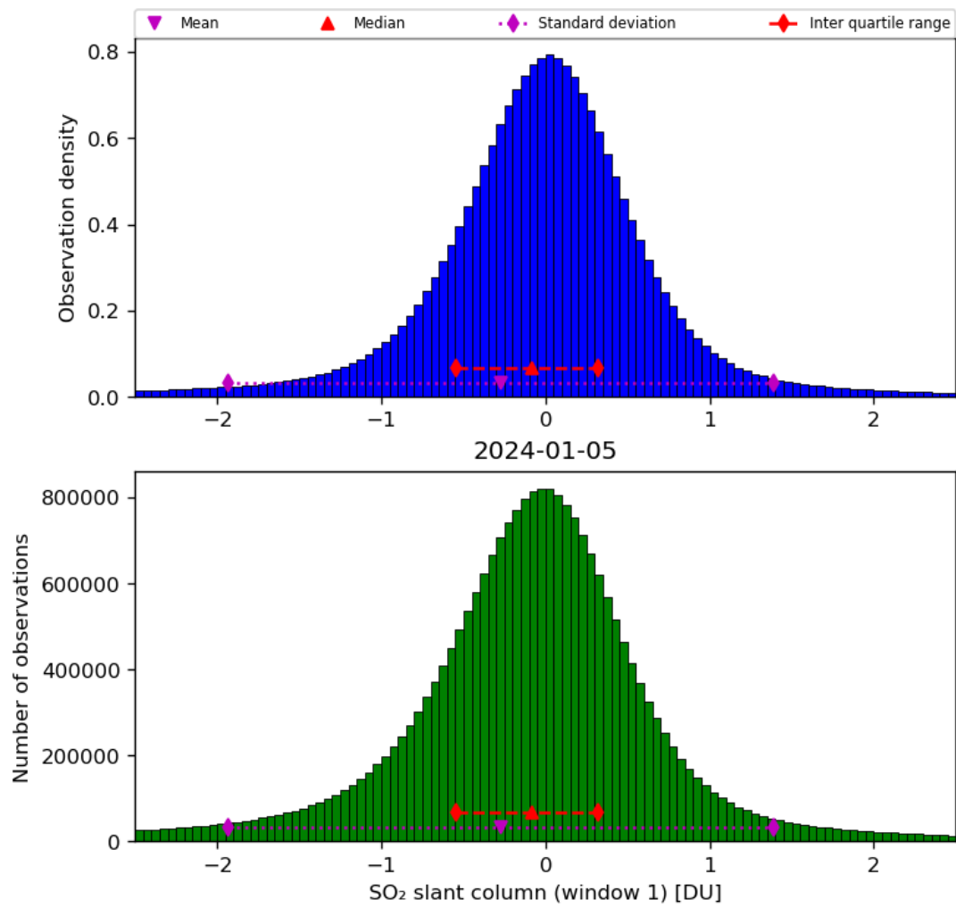
Figure 56: Histogram of “SO 2 slant column (window 1)” for 2024-01-05 to 2024-01-06
