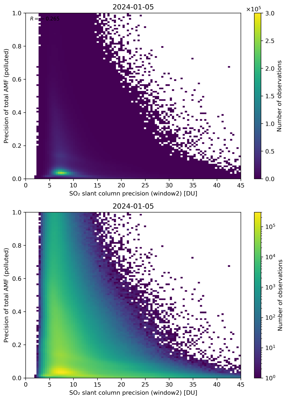
Figure 252: Scatter density plot of “SO 2 slant column precision (window2)” against “Precision of total AMF (polluted)” for 2024-01-05 to 2024-01-06.
