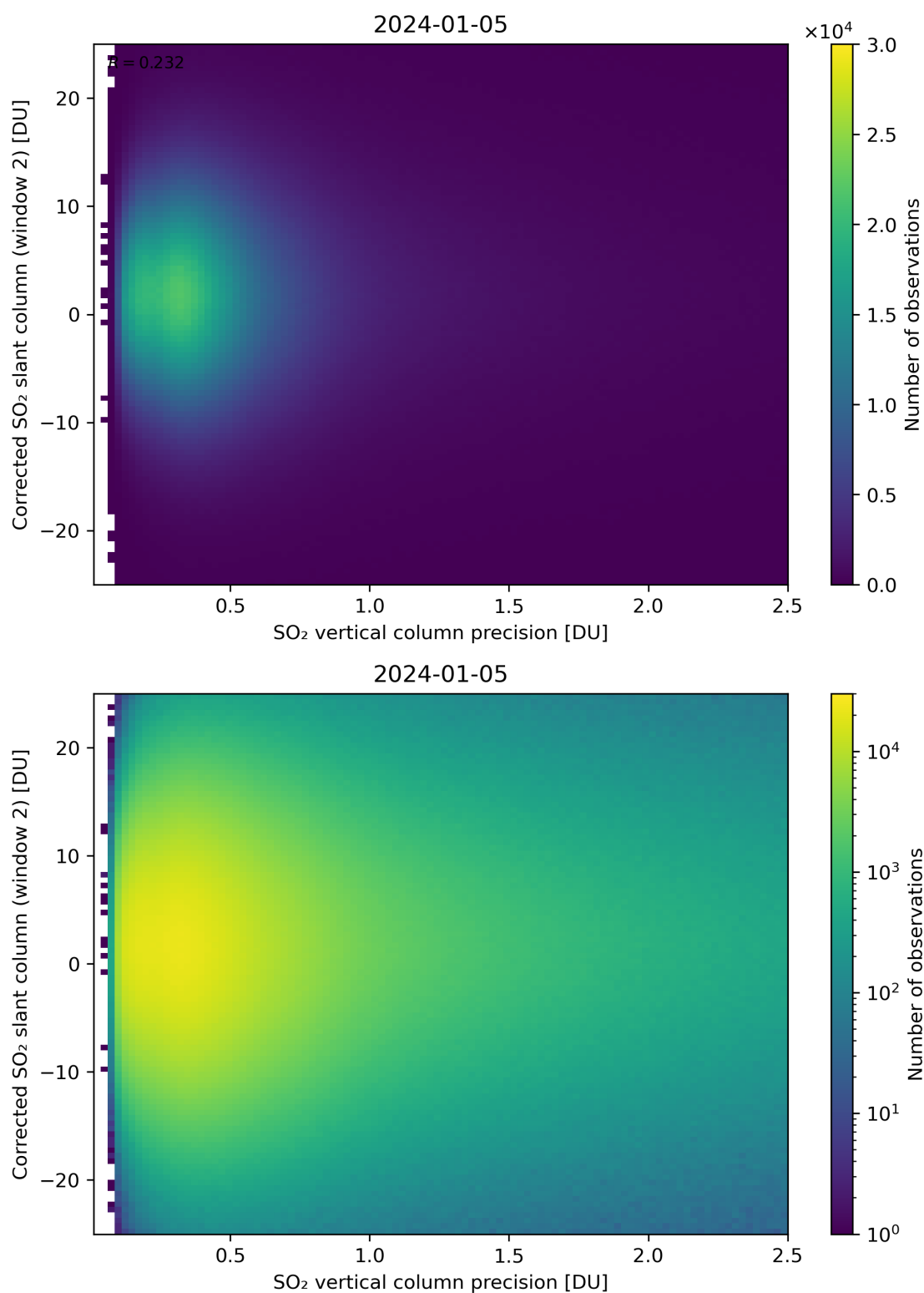
Figure 287: Scatter density plot of “SO 2 vertical column precision” against “Corrected SO 2 slant column (window 2)” for 2024-01-05 to 2024-01-06.
