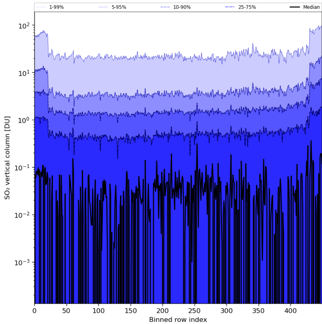
Figure 76: Along track statistics of “SO 2 vertical column” for 2024-01-05 to 2024-01-06
