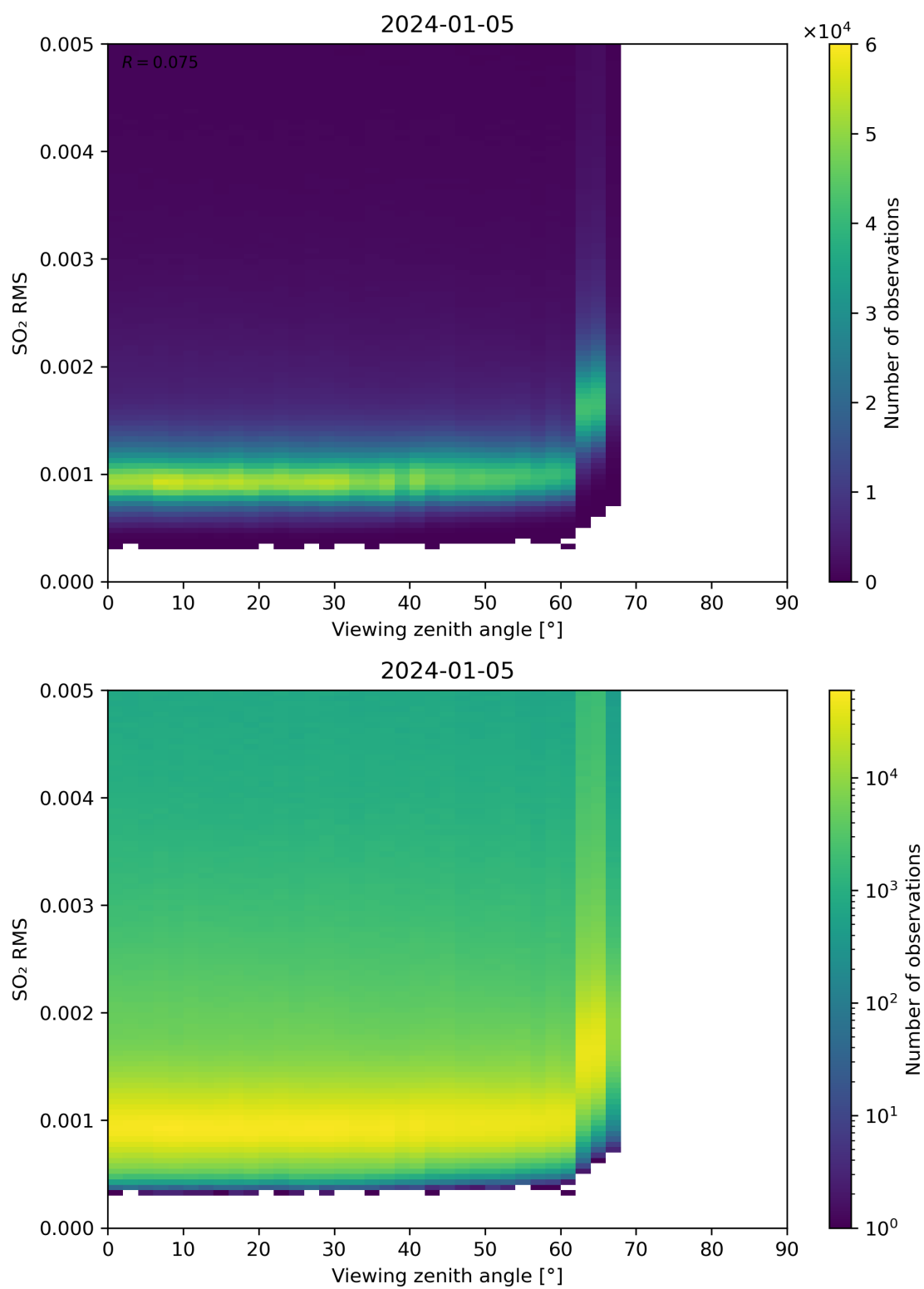
Figure 313: Scatter density plot of “Viewing zenith angle” against “SO 2 RMS” for 2024-01-05 to 2024-01-06.
