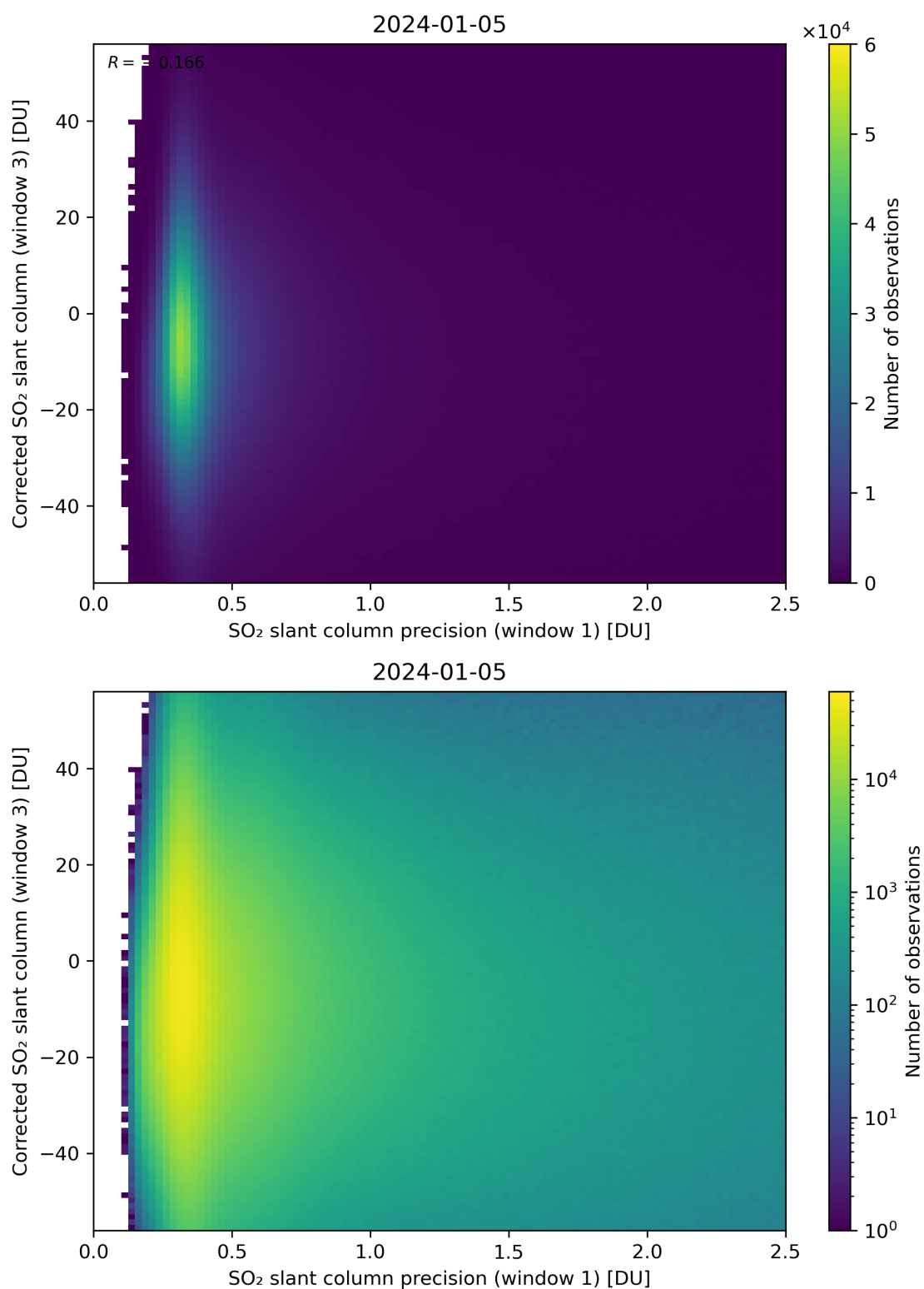
Figure 226: Scatter density plot of “SO 2 slant column precision (window 1)” against “Corrected SO 2 slant column (window 3)” for 2024-01-05 to 2024-01-06.
