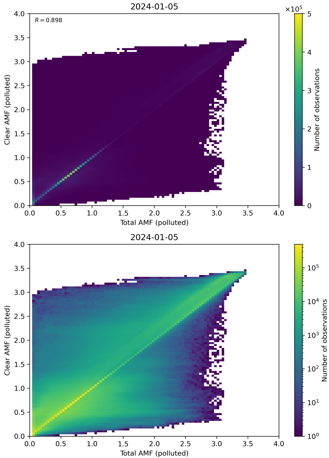
Figure 271: Scatter density plot of “Total AMF (polluted)” against “Clear AMF (polluted)” for 2024-01-05 to 2024-01-06.
