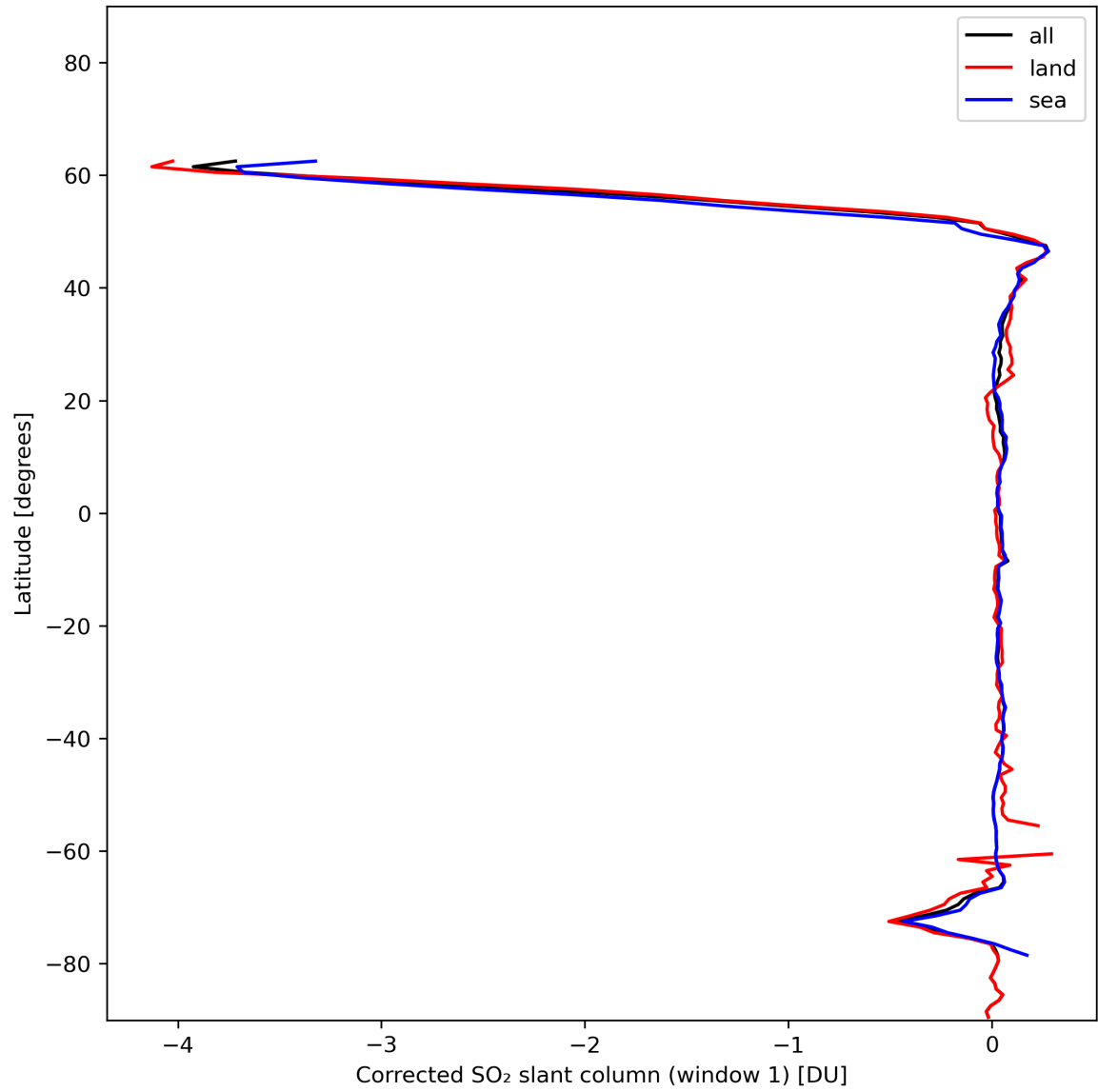
Figure 35: Zonal average of “Corrected SO 2 slant column (window 1)” for 2024-01-05 to 2024-01-06.
