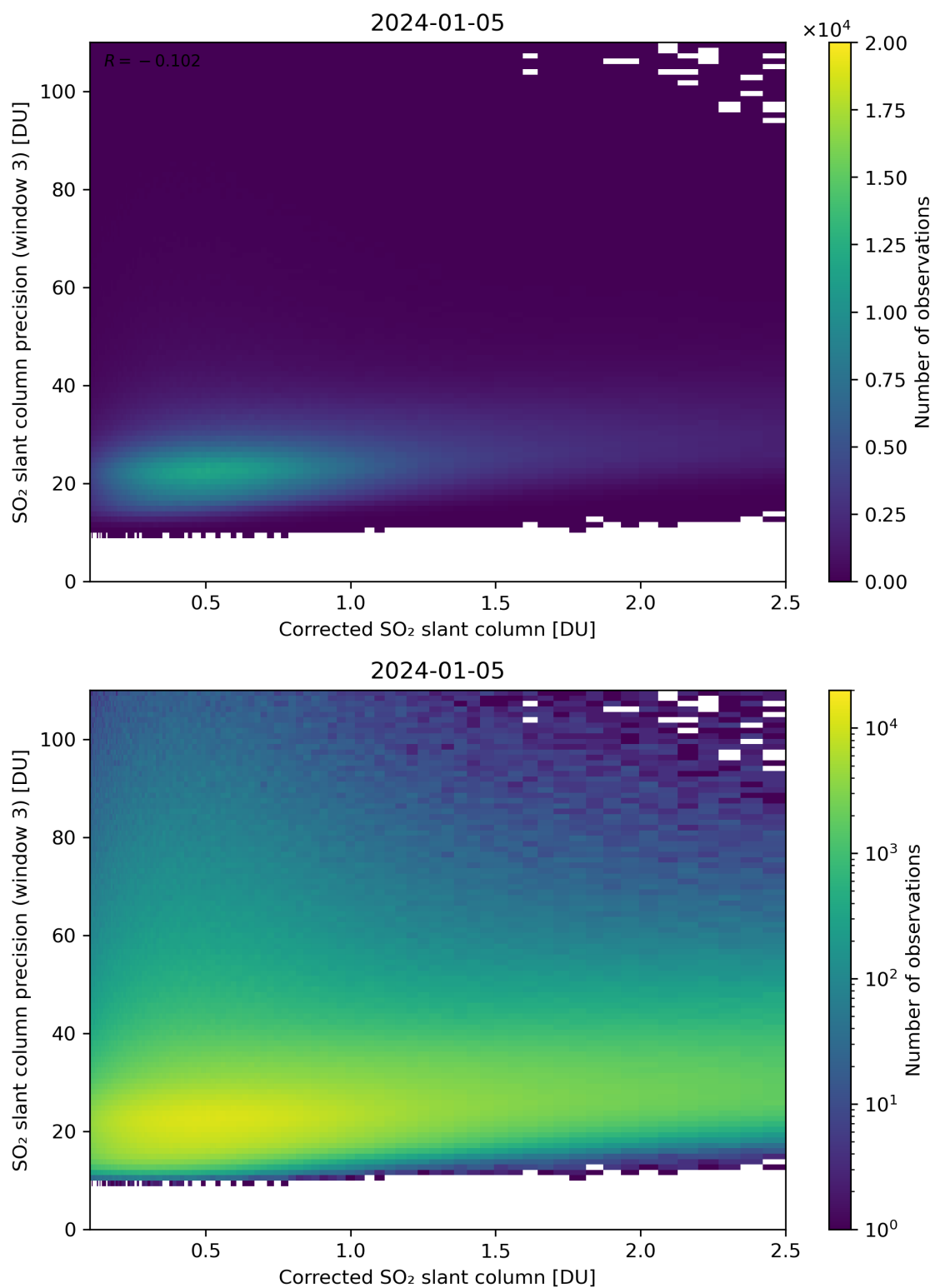
Figure 191: Scatter density plot of “Corrected SO 2 slant column” against “SO 2 slant column precision (window 3)” for 2024-01-05 to 2024-01-06.
