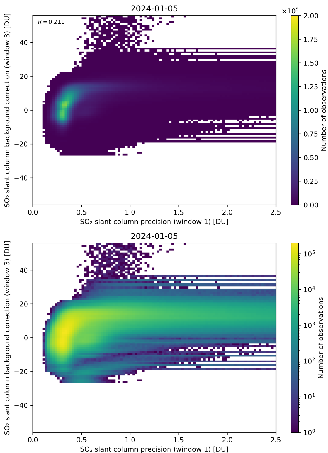
Figure 220: Scatter density plot of “SO 2 slant column precision (window 1)” against “SO 2 slant column background correction (window 3)” for 2024-01-05 to 2024-01-06.
