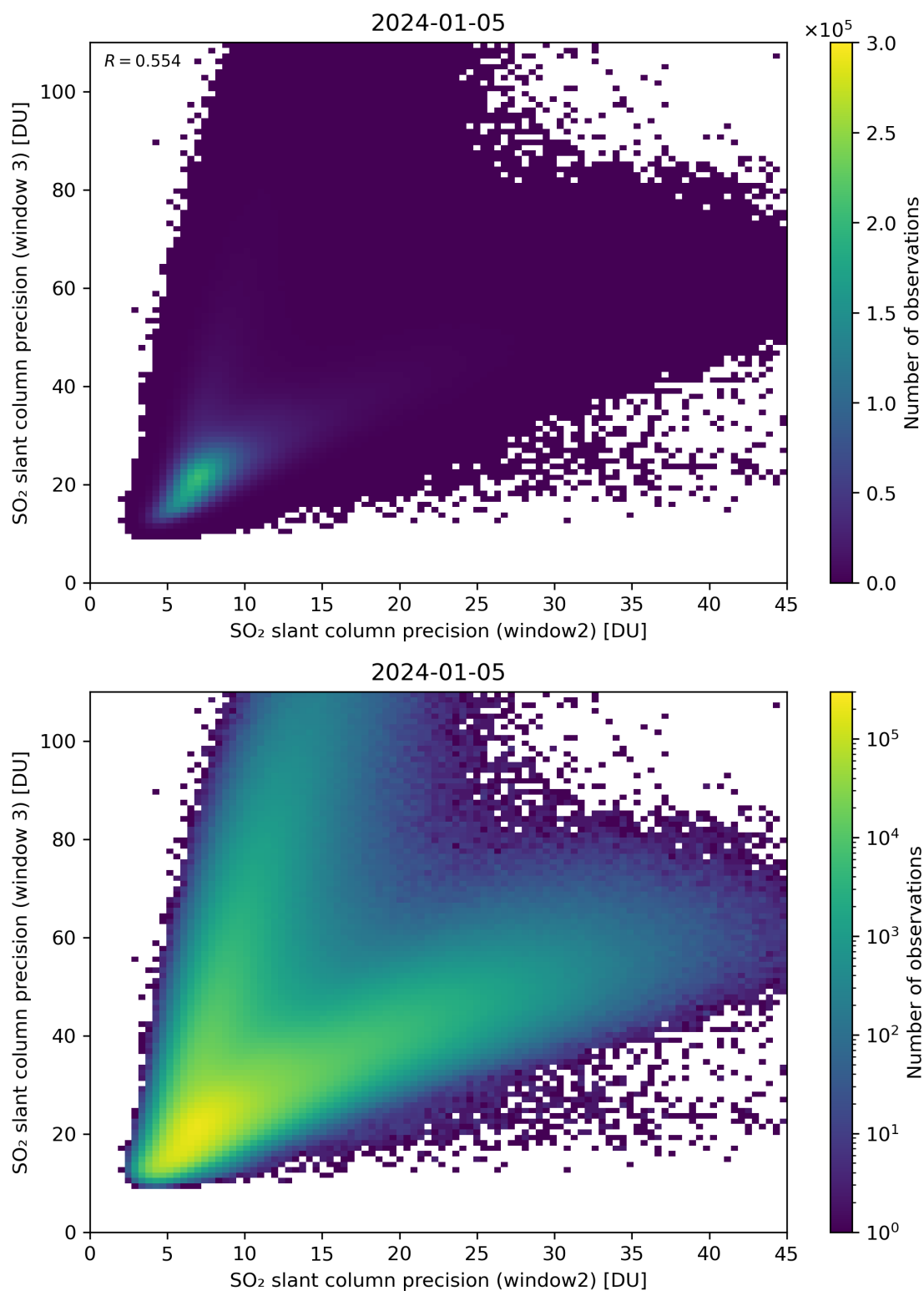
Figure 250: Scatter density plot of “SO 2 slant column precision (window2)” against “SO 2 slant column precision (window 3)” for 2024-01-05 to 2024-01-06.
