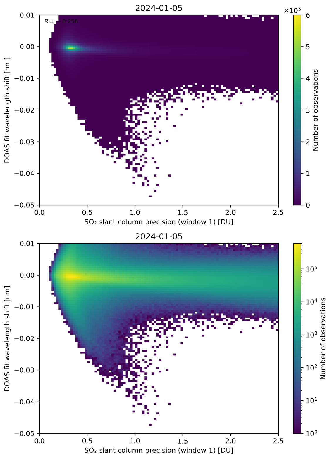
Figure 221: Scatter density plot of “SO 2 slant column precision (window 1)” against “DOAS fit wavelength shift” for 2024-01-05 to 2024-01-06.
