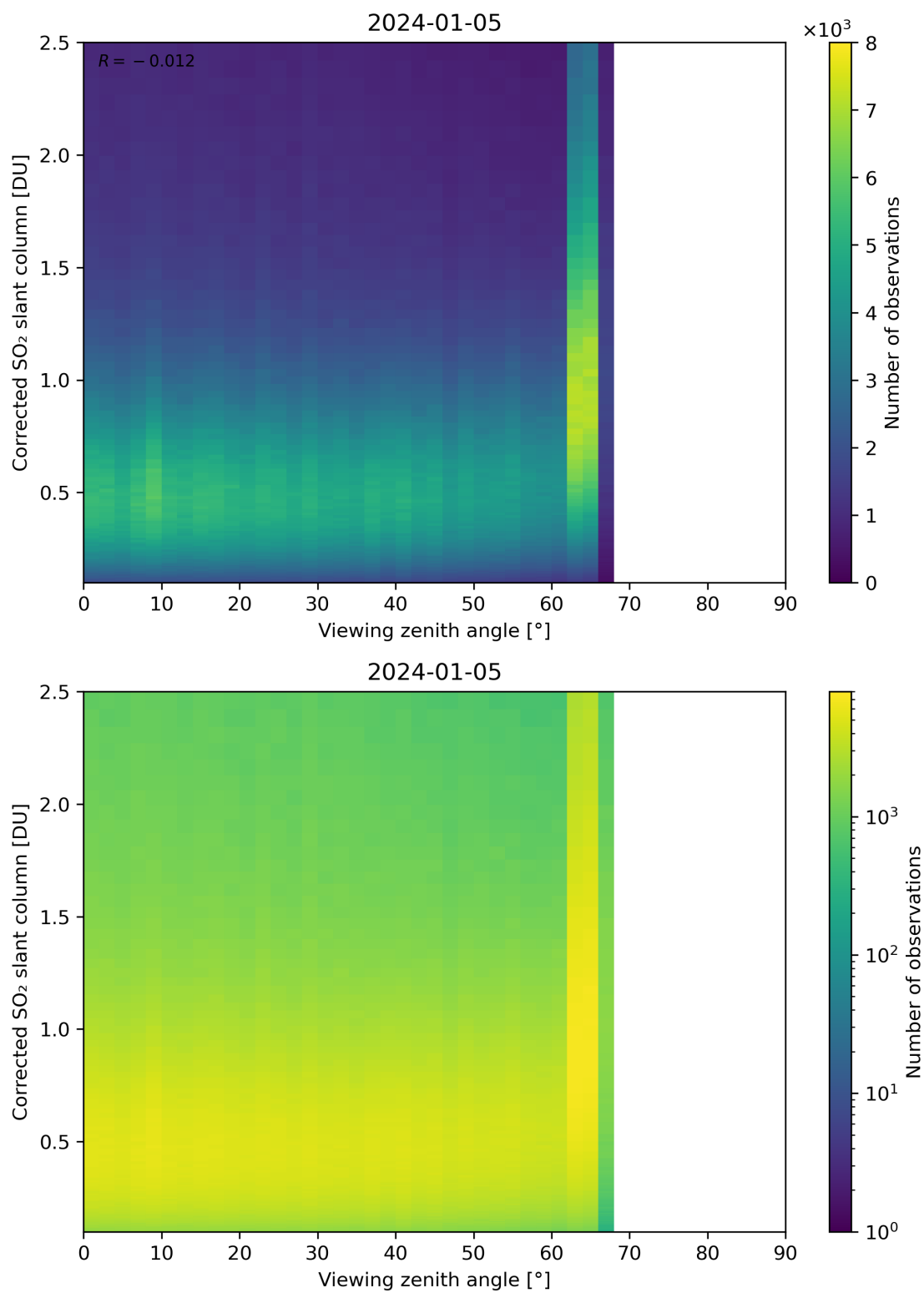
Figure 317: Scatter density plot of “Viewing zenith angle” against “Corrected SO 2 slant column” for 2024-01-05 to 2024-01-06.
