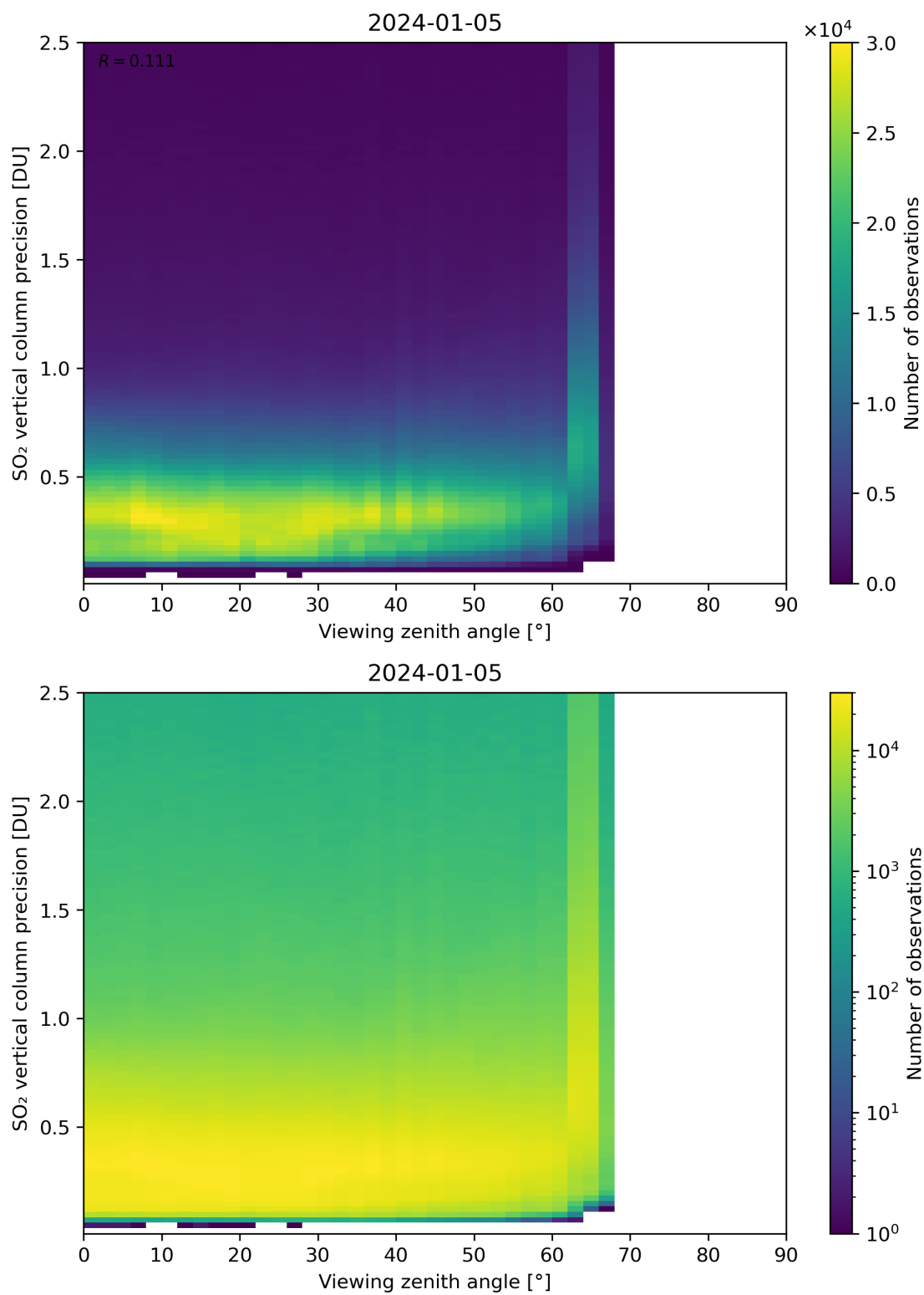
Figure 328: Scatter density plot of “Viewing zenith angle” against “SO 2 vertical column precision” for 2024-01-05 to 2024-01-06.
