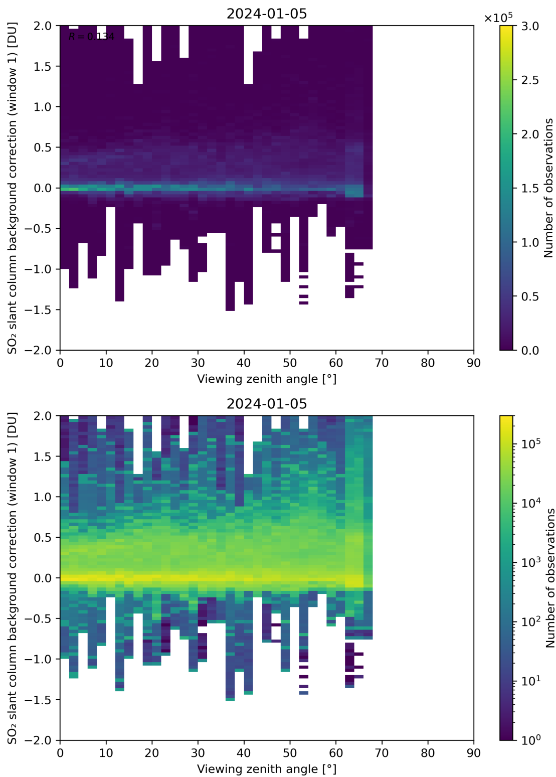
Figure 308: Scatter density plot of “Viewing zenith angle” against “SO 2 slant column background correction (window 1)” for 2024-01-05 to 2024-01-06.
