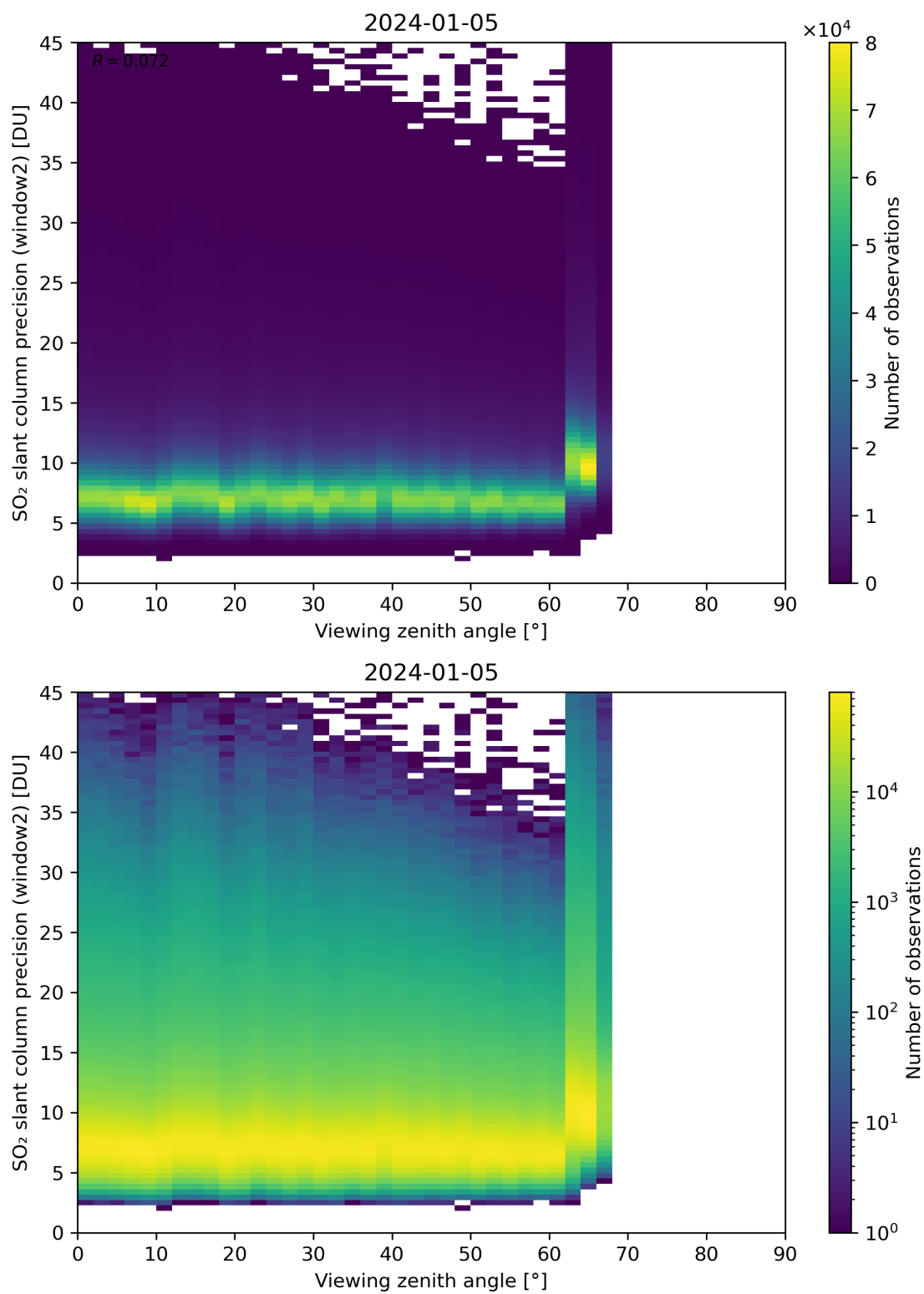
Figure 322: Scatter density plot of “Viewing zenith angle” against “SO 2 slant column precision (window2)” for 2024-01-05 to 2024-01-06.
