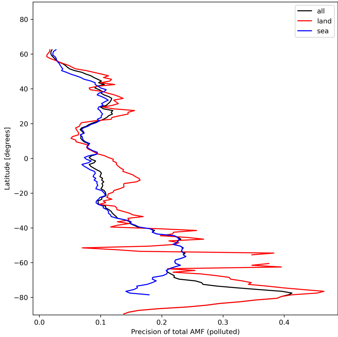
Figure 49: Zonal average of “Precision of total AMF (polluted)” for 2024-01-05 to 2024-01-06.
