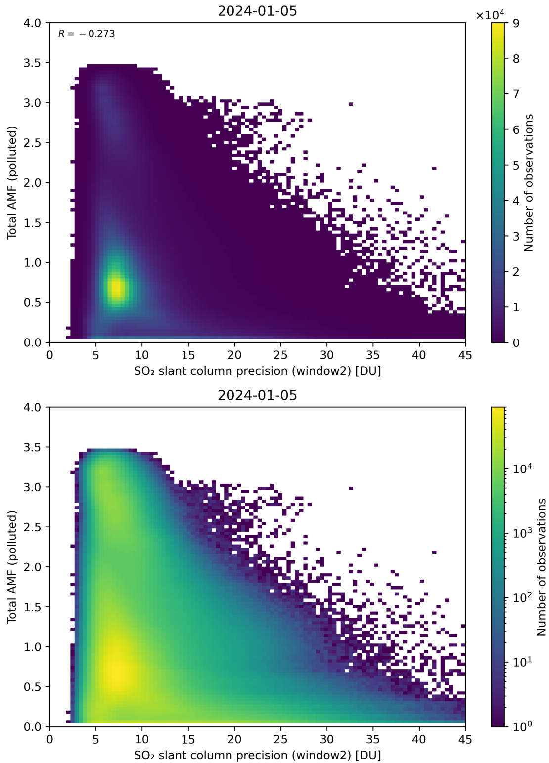
Figure 251: Scatter density plot of “SO 2 slant column precision (window2)” against “Total AMF (polluted)” for 2024-01-05 to 2024-01-06.
