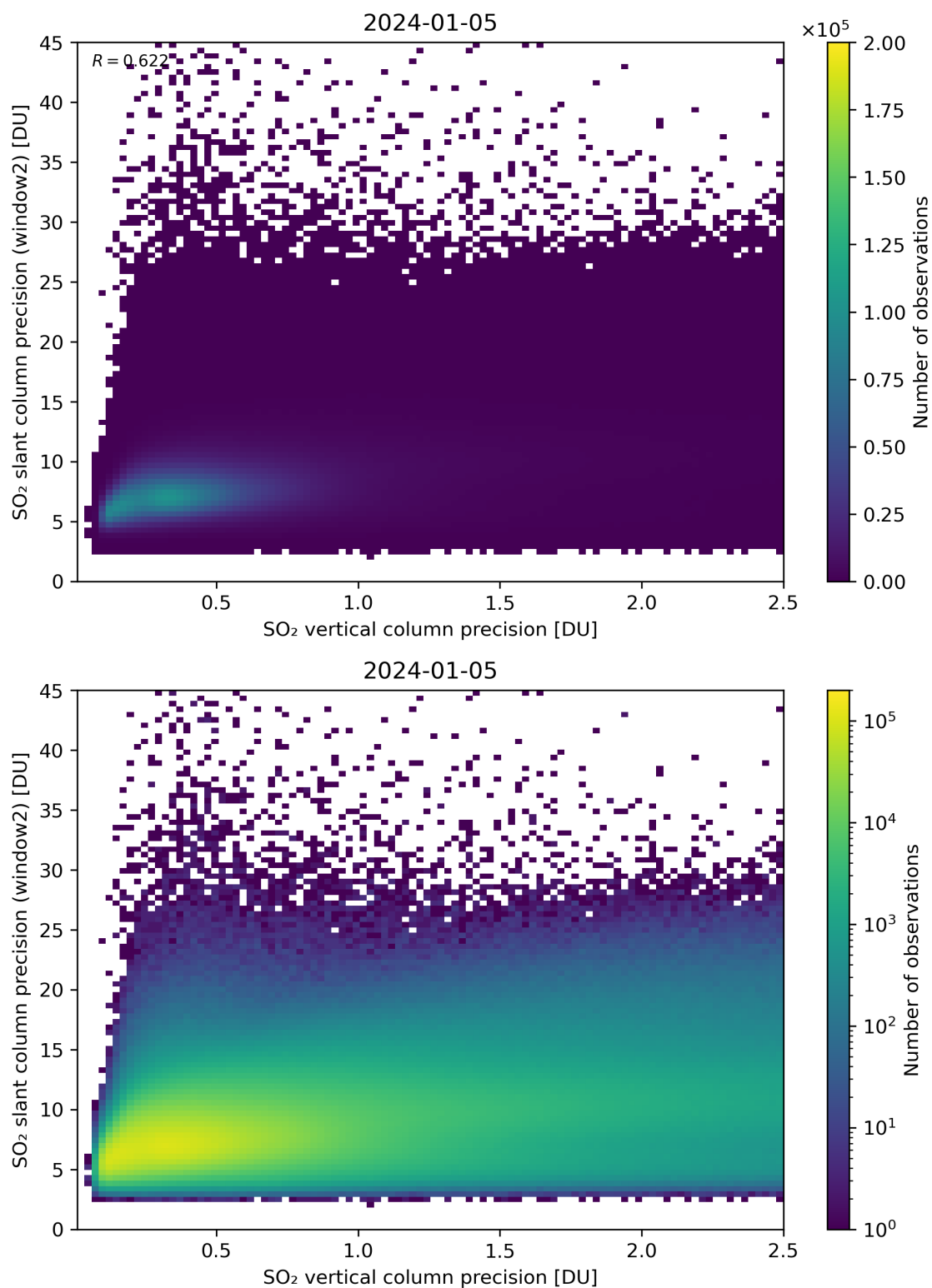
Figure 291: Scatter density plot of “SO 2 vertical column precision” against “SO 2 slant column precision (window2)” for 2024-01-05 to 2024-01-06.
