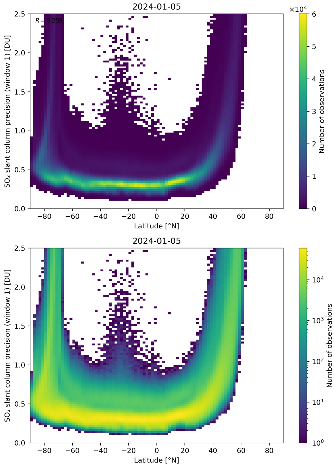
Figure 150: Scatter density plot of “Latitude” against “SO 2 slant column precision (window 1)” for 2024-01-05 to 2024-01-06.
