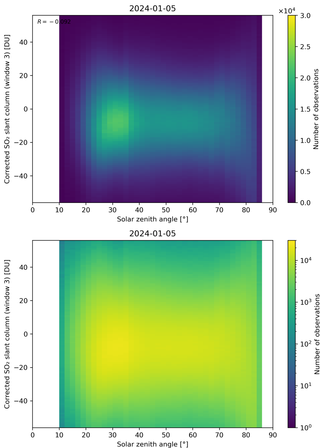
Figure 168: Scatter density plot of “Solar zenith angle” against “Corrected SO 2 slant column (window 3)” for 2024-01-05 to 2024-01-06.
