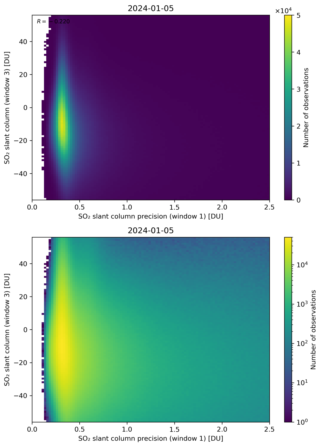
Figure 228: Scatter density plot of “SO 2 slant column precision (window 1)” against “SO 2 slant column (window 3)” for 2024-01-05 to 2024-01-06.
