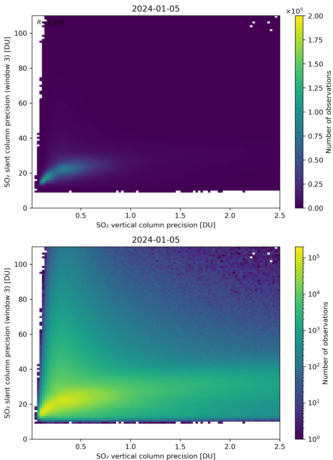
Figure 293: Scatter density plot of “SO 2 vertical column precision” against “SO 2 slant column precision (window 3)” for 2024-01-05 to 2024-01-06.
