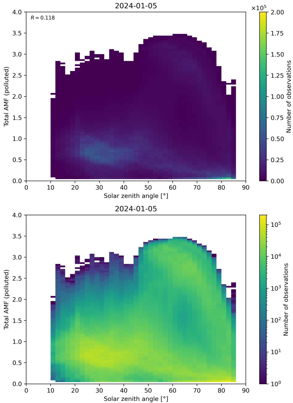
Figure 174: Scatter density plot of “Solar zenith angle” against “Total AMF (polluted)” for 2024-01-05 to 2024-01-06.
