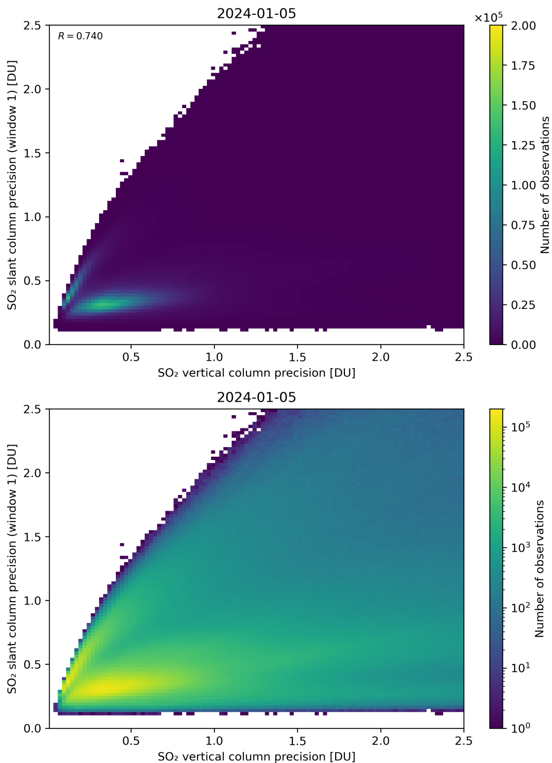
Figure 290: Scatter density plot of “SO 2 vertical column precision” against “SO 2 slant column precision (window 1)” for 2024-01-05 to 2024-01-06.
