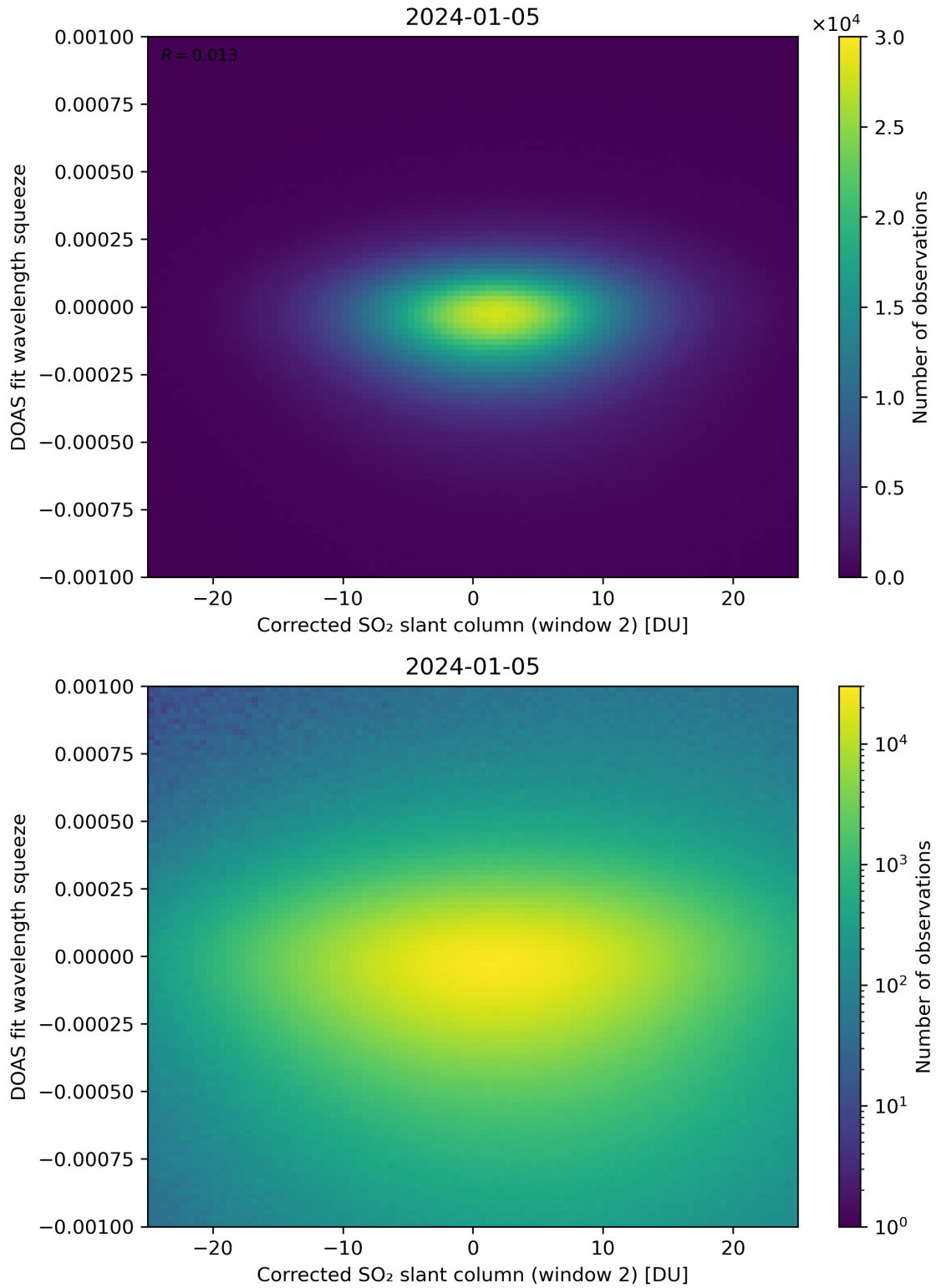
Figure 197: Scatter density plot of “Corrected SO 2 slant column (window 2)” against “DOAS fit wavelength squeeze” for 2024-01-05 to 2024-01-06.
