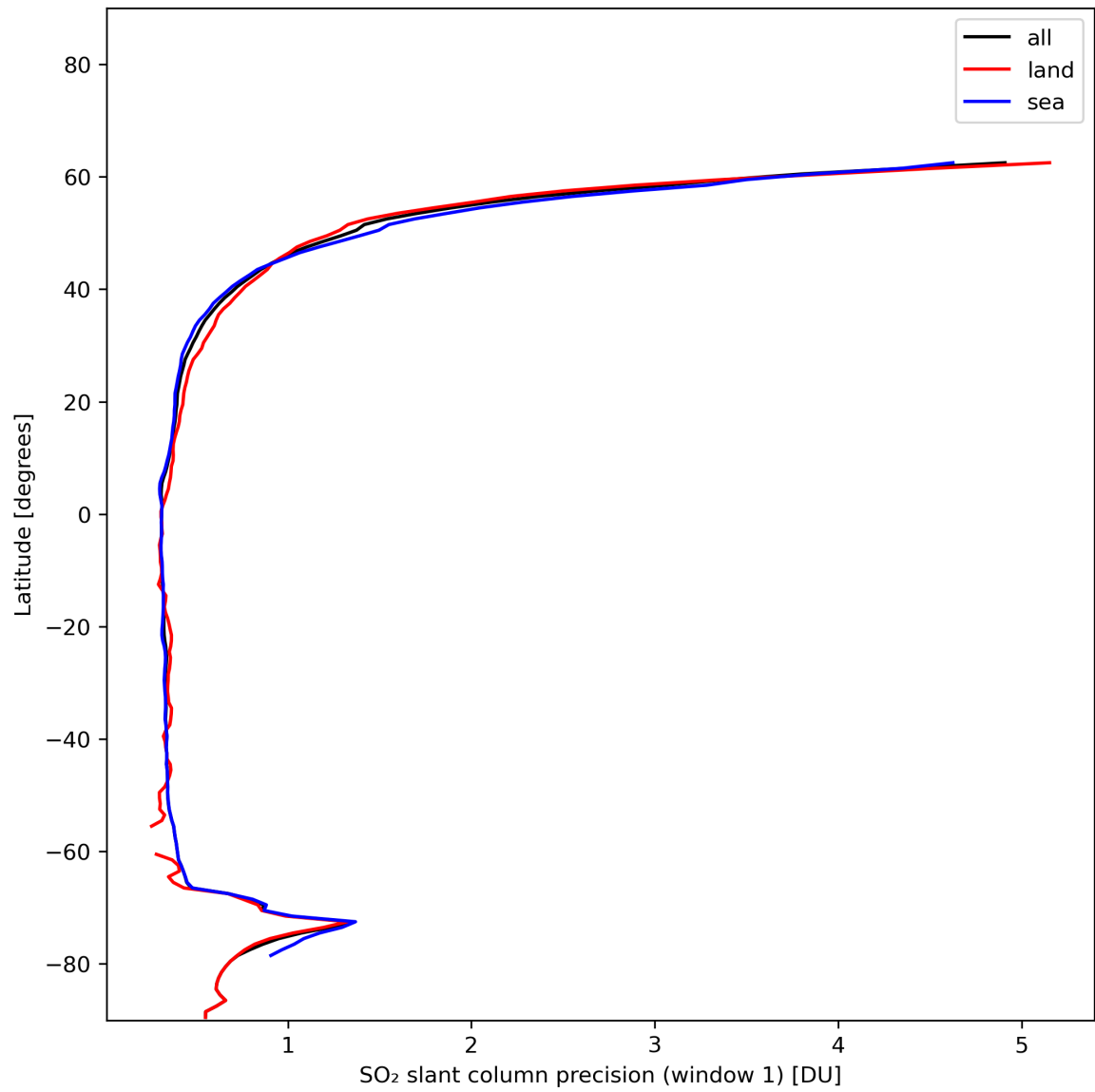
Figure 34: Zonal average of "SO 2 slant column precision (window 1)" for 2024-01-05 to 2024-01-06.
