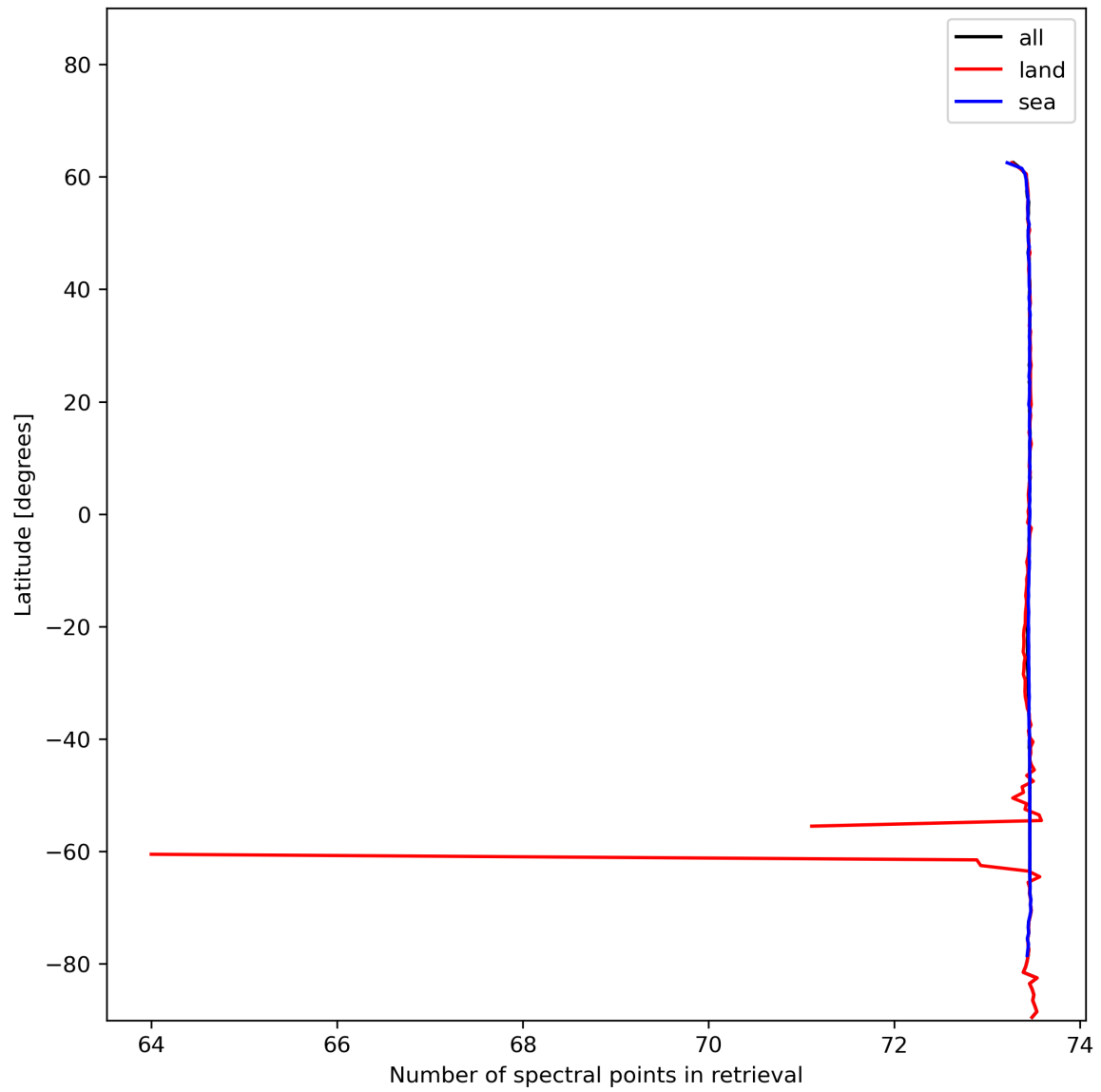
Figure 51: Zonal average of “Number of spectral points in retrieval” for 2024-01-05 to 2024-01-06.
