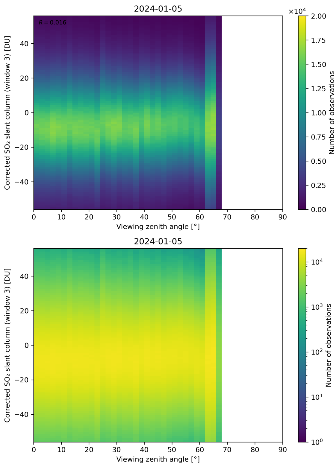
Figure 319: Scatter density plot of “Viewing zenith angle” against “Corrected SO 2 slant column (window 3)” for 2024-01-05 to 2024-01-06.
