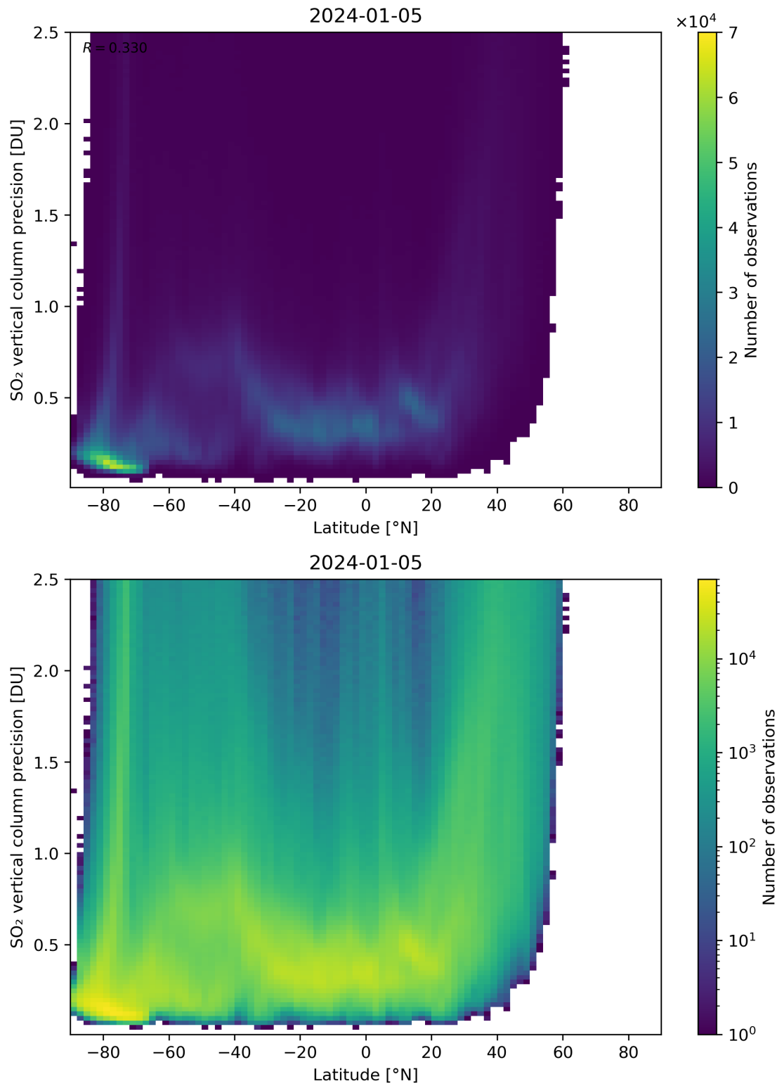
Figure 157: Scatter density plot of “Latitude” against “SO 2 vertical column precision” for 2024-01-05 to 2024-01-06.
