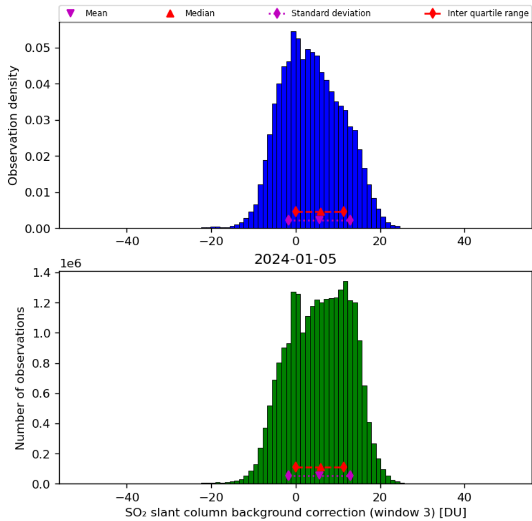
Figure 67: Histogram of “SO 2 slant column background correction (window 3)” for 2024-01-05 to 2024-01-06
