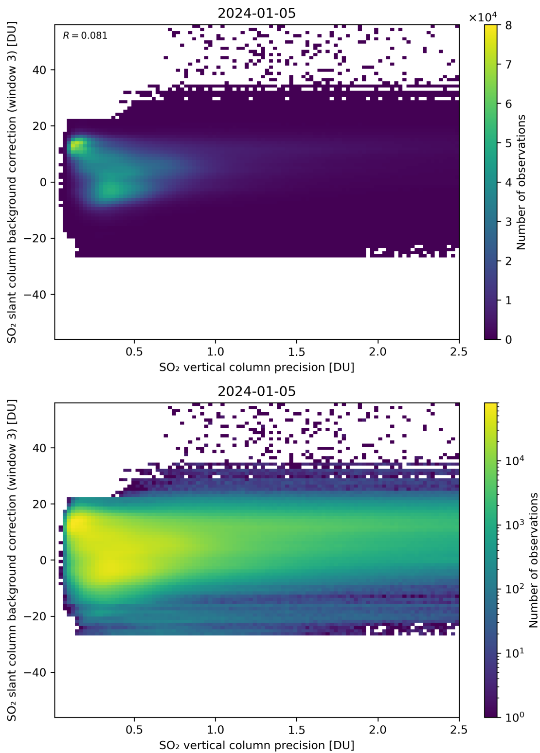
Figure 281: Scatter density plot of “SO 2 vertical column precision” against “SO 2 slant column background correction (window 3)” for 2024-01-05 to 2024-01-06.
