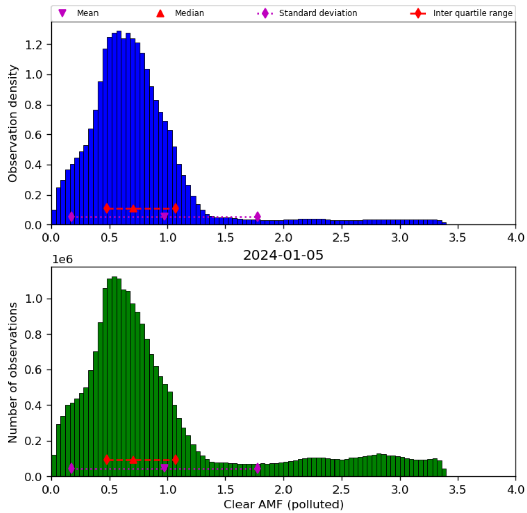
Figure 73: Histogram of “Clear AMF (polluted)” for 2024-01-05 to 2024-01-06
