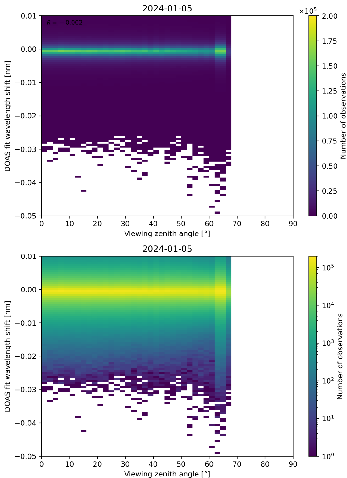
Figure 311: Scatter density plot of “Viewing zenith angle” against “DOAS fit wavelength shift” for 2024-01-05 to 2024-01-06.
