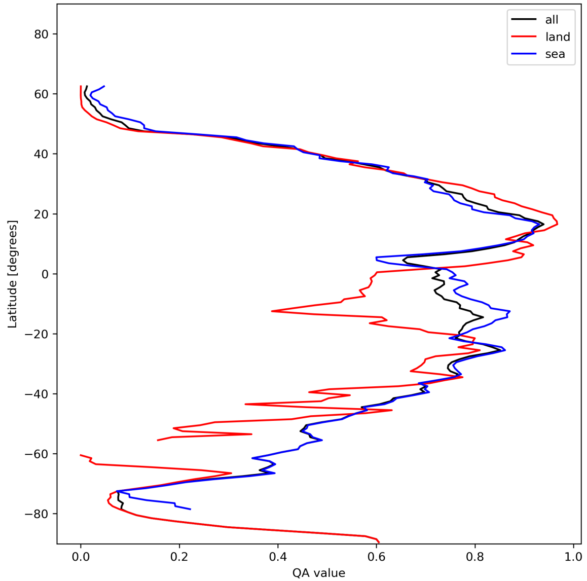
Figure 29: Zonal average of “QA value” for 2024-01-05 to 2024-01-06.
