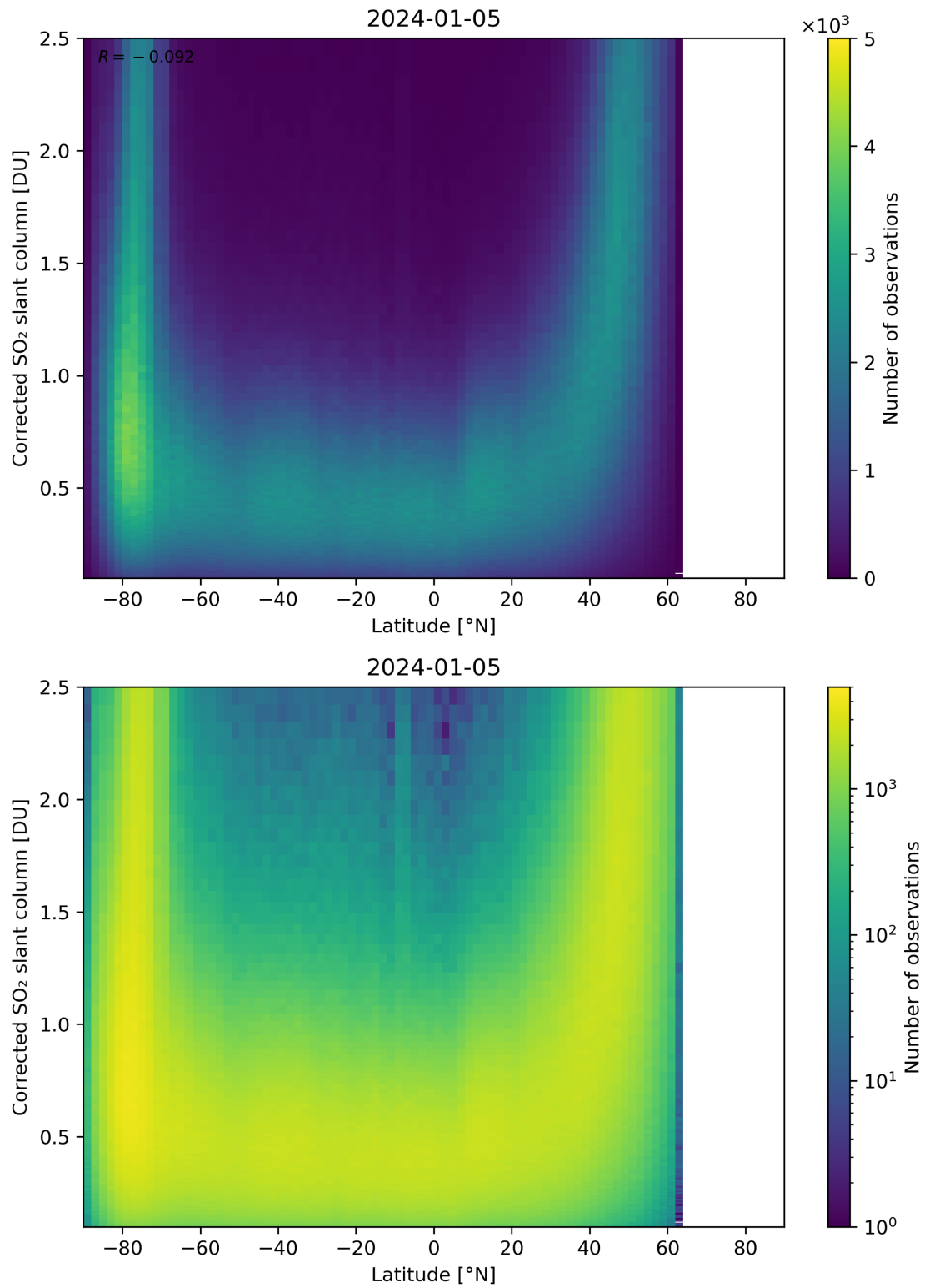
Figure 146: Scatter density plot of “Latitude” against “Corrected SO 2 slant column” for 2024-01-05 to 2024-01-06.
