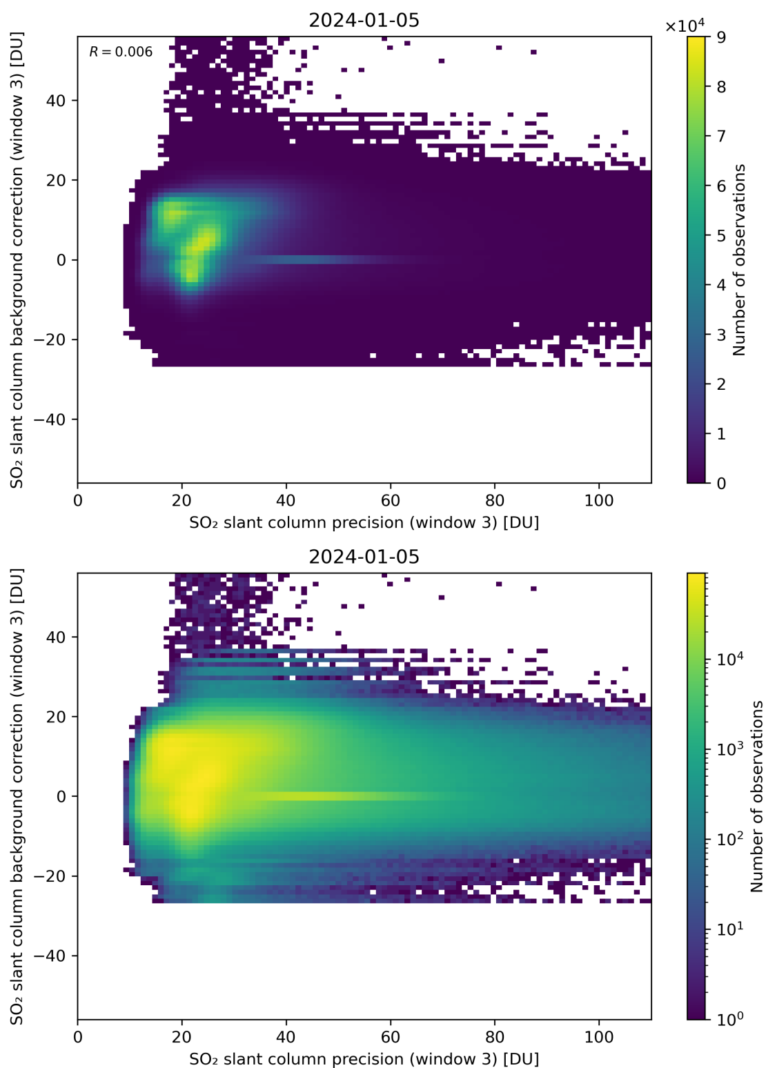
Figure 257: Scatter density plot of “SO 2 slant column precision (window 3)” against “SO 2 slant column background correction (window 3)” for 2024-01-05 to 2024-01-06.
