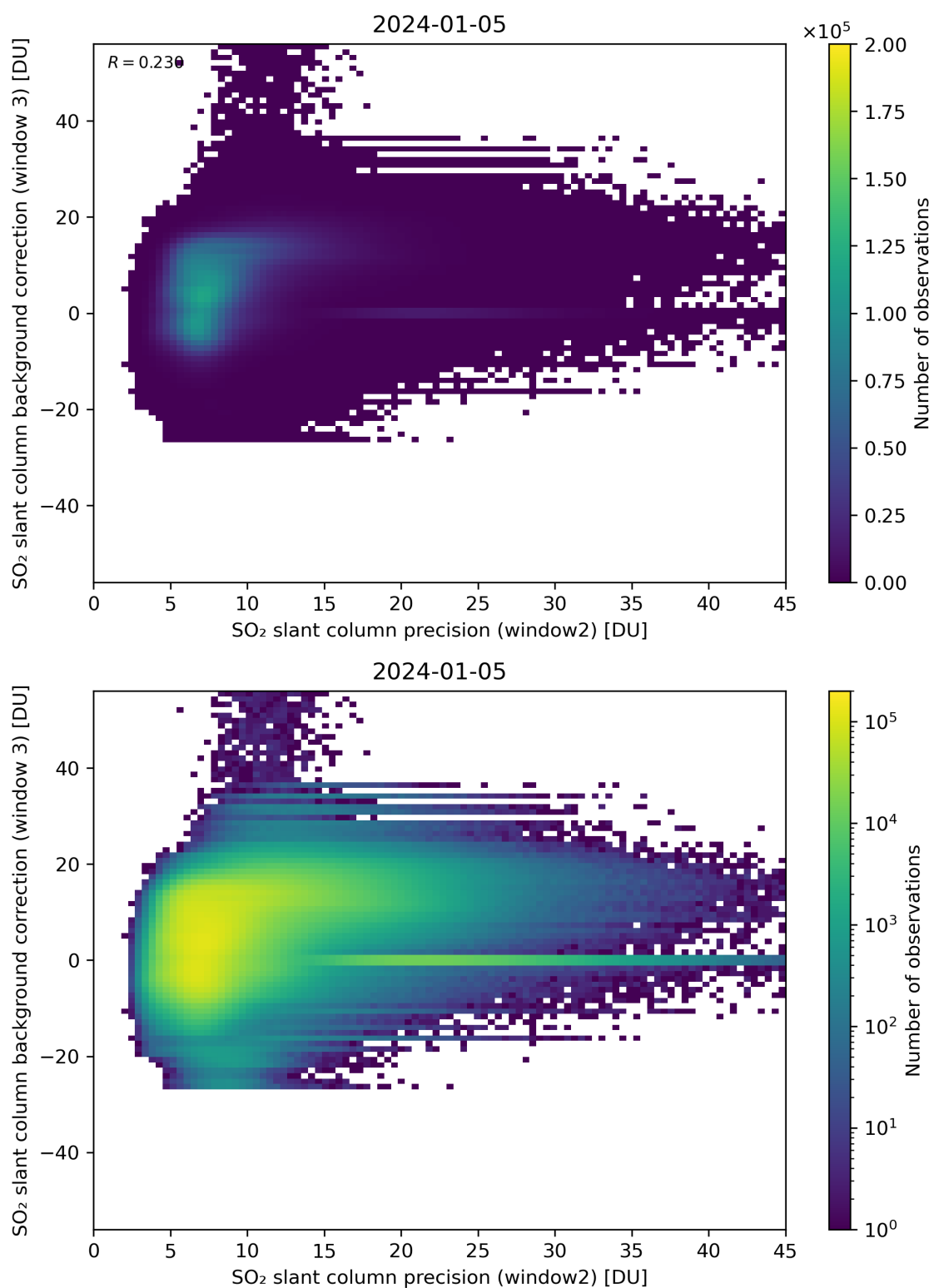
Figure 242: Scatter density plot of “SO 2 slant column precision (window2)” against “SO 2 slant column background correction (window 3)” for 2024-01-05 to 2024-01-06.
