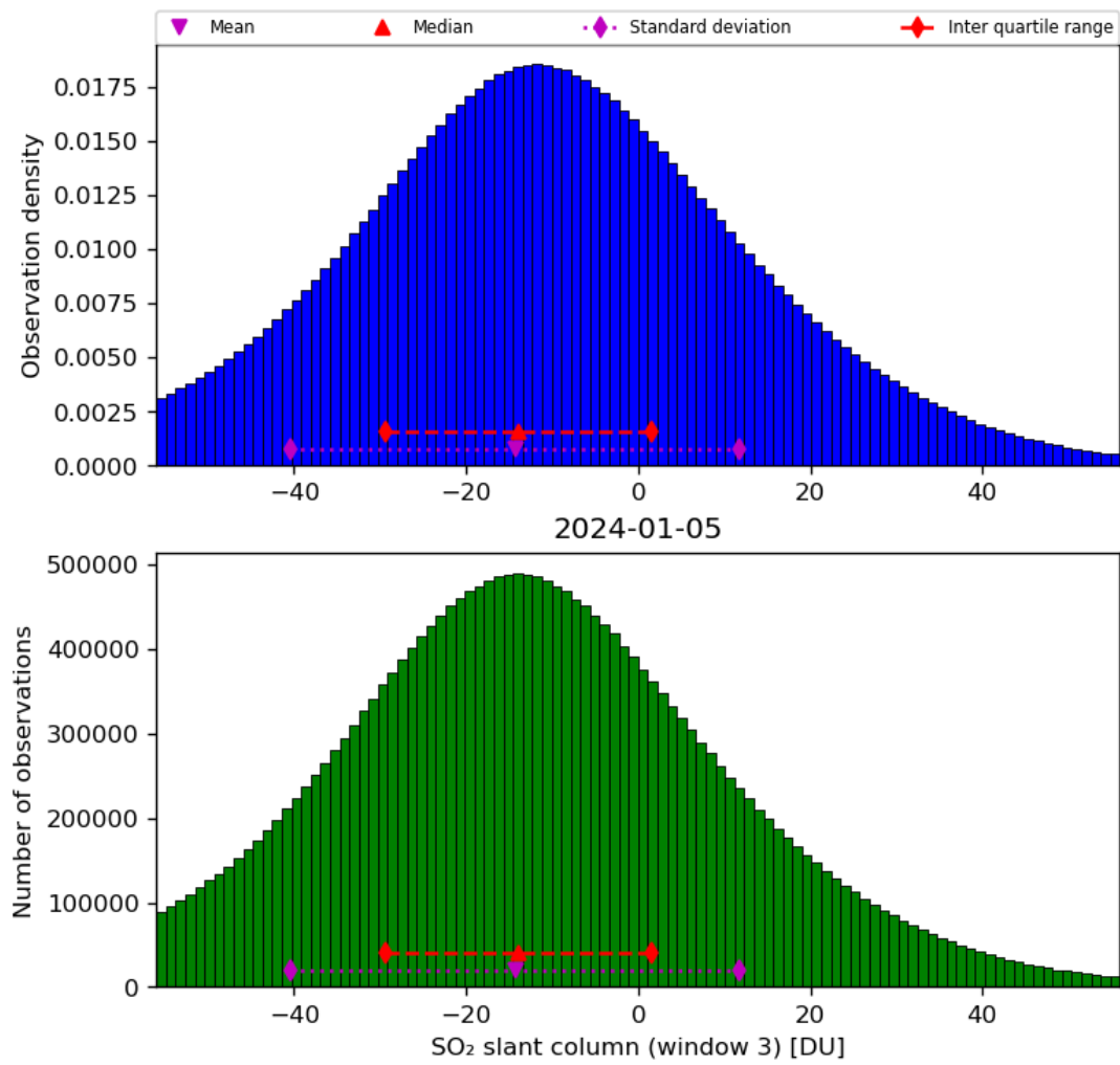
Figure 64: Histogram of “SO 2 slant column (window 3)” for 2024-01-05 to 2024-01-06
