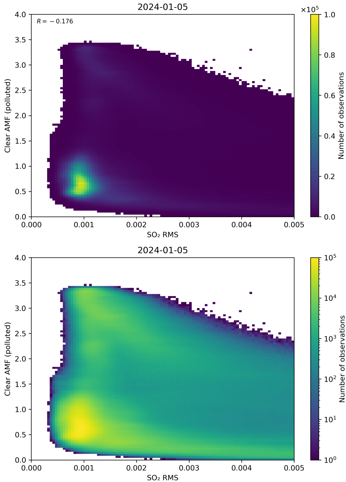
Figure 136: Scatter density plot of “SO 2 RMS” against “Clear AMF (polluted)” for 2024-01-05 to 2024-01-06.
