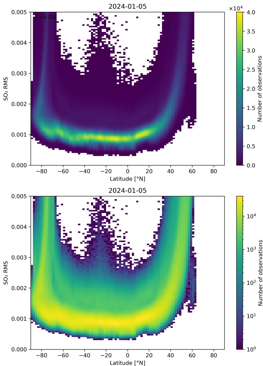
Figure 144: Scatter density plot of “Latitude” against “SO 2 RMS” for 2024-01-05 to 2024-01-06.
