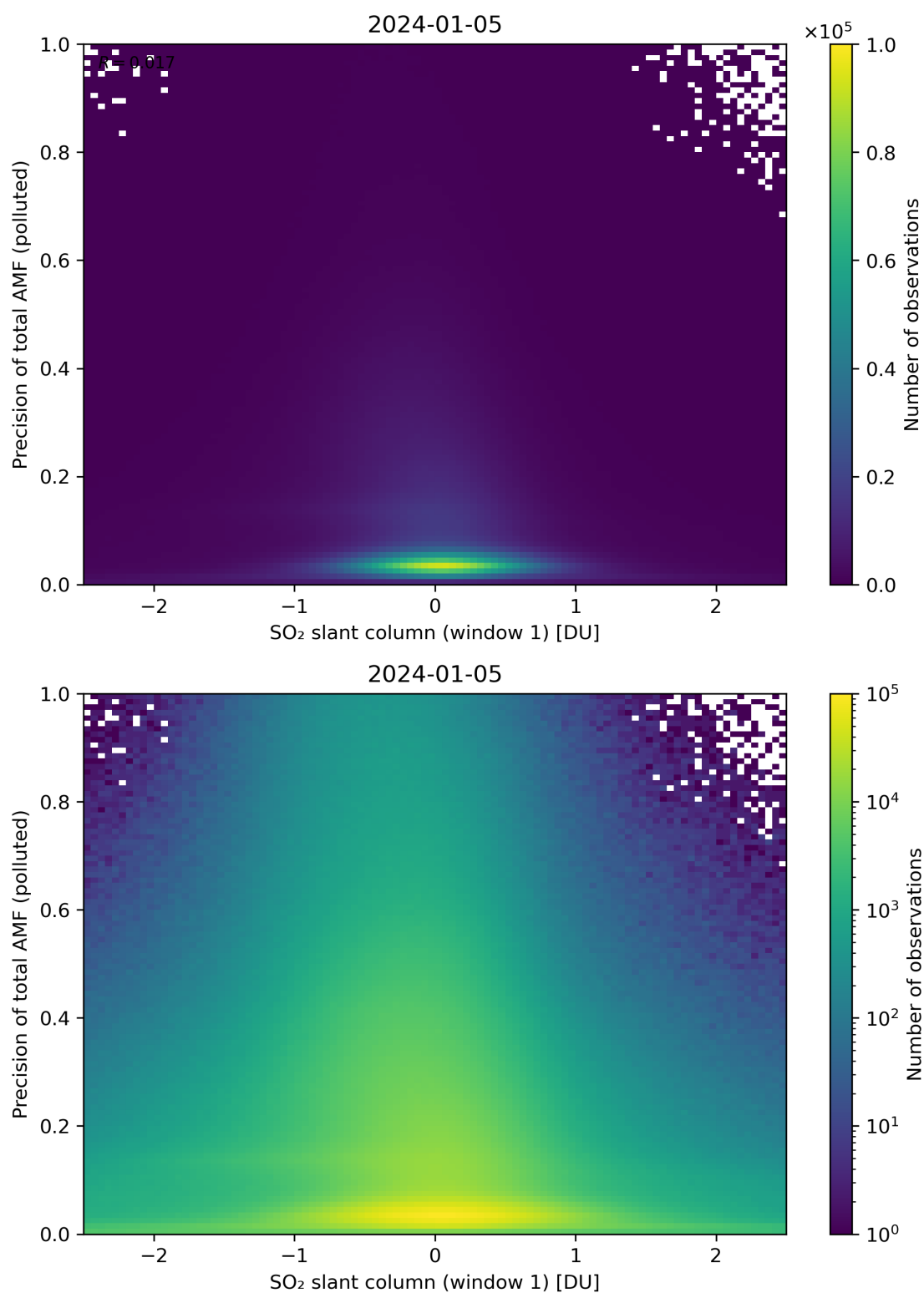
Figure 240: Scatter density plot of “SO 2 slant column (window 1)” against “Precision of total AMF (polluted)” for 2024-01-05 to 2024-01-06.
