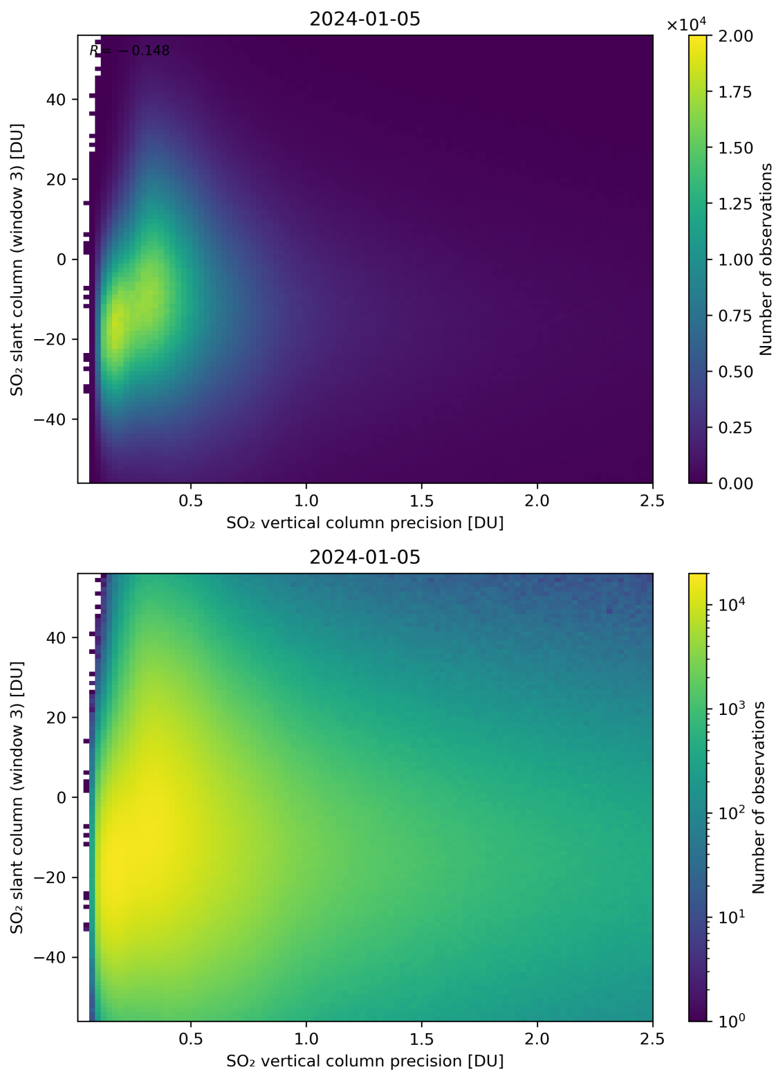
Figure 292: Scatter density plot of “SO 2 vertical column precision” against “SO 2 slant column (window 3)” for 2024-01-05 to 2024-01-06.
