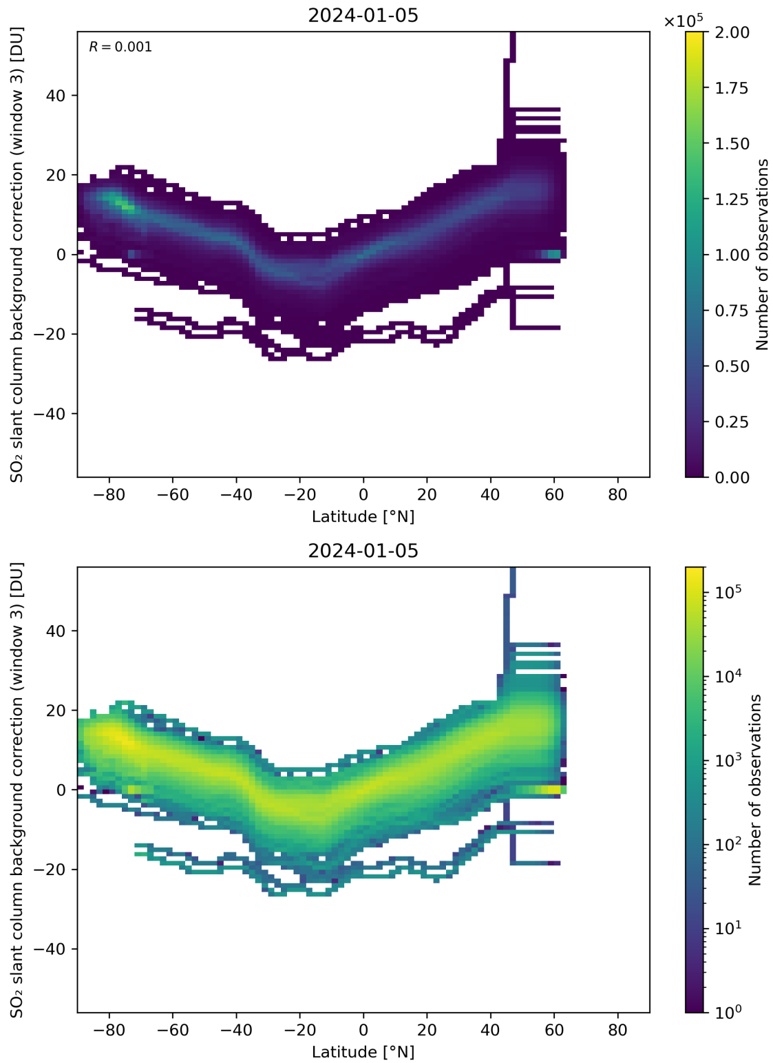
Figure 141: Scatter density plot of “Latitude” against “SO 2 slant column background correction (window 3)” for 2024-01-05 to 2024-01-06.
