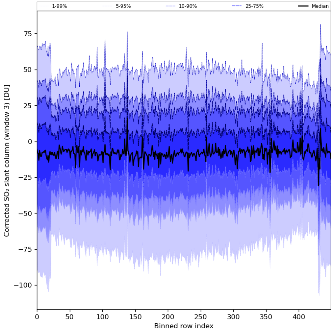
Figure 89: Along track statistics of “Corrected SO 2 slant column (window 3)” for 2024-01-05 to 2024-01-06
