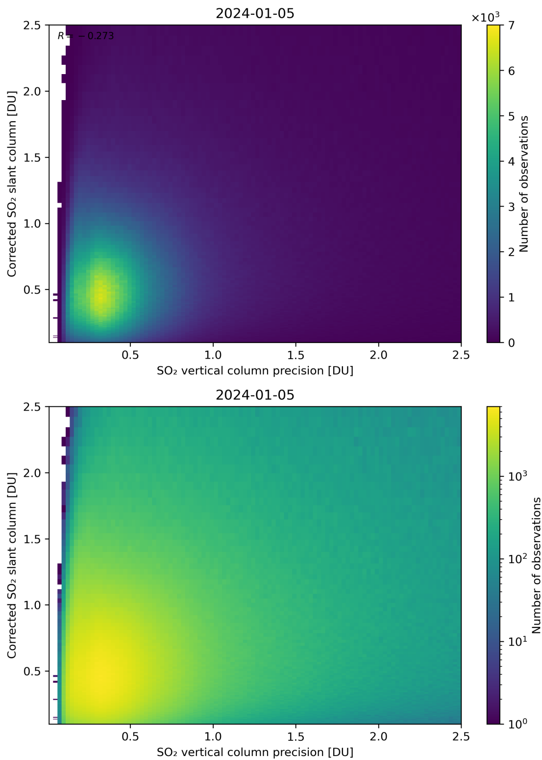
Figure 286: Scatter density plot of “SO 2 vertical column precision” against “Corrected SO 2 slant column” for 2024-01-05 to 2024-01-06.
