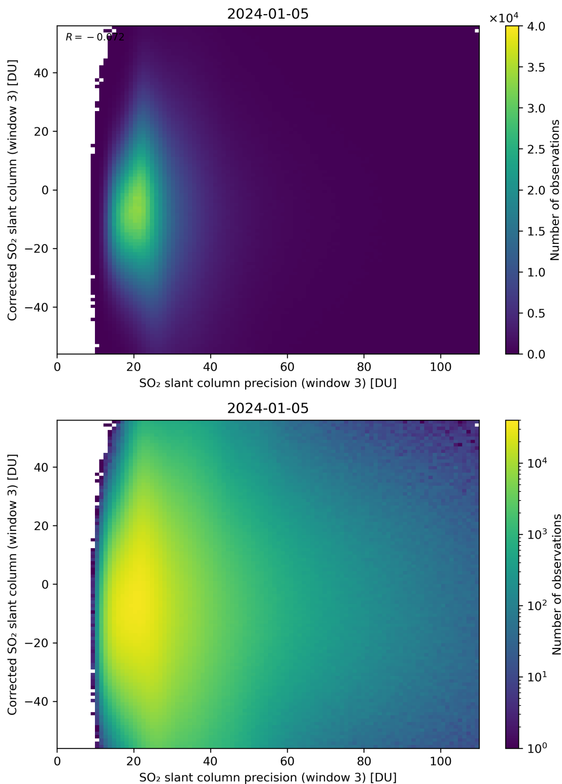
Figure 262: Scatter density plot of “SO 2 slant column precision (window 3)” against “Corrected SO 2 slant column (window 3)” for 2024-01-05 to 2024-01-06.
