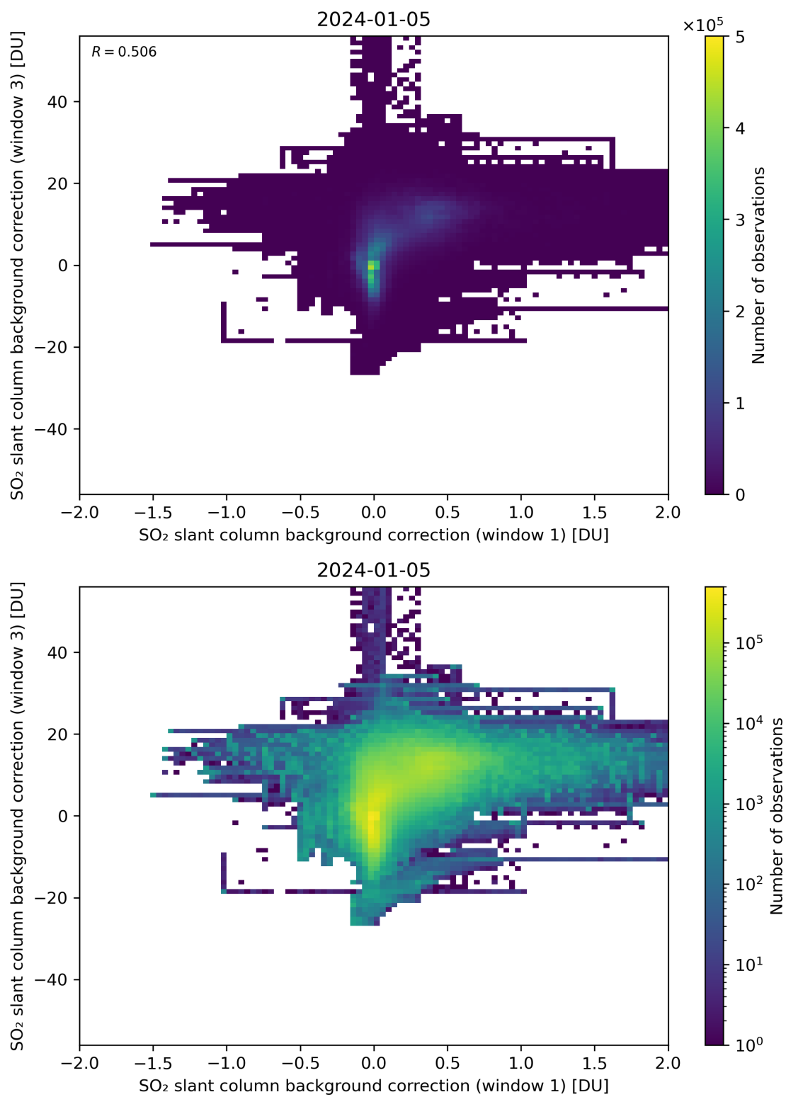
Figure 99: Scatter density plot of “SO 2 slant column background correction (window 1)” against “SO 2 slant column background correction (window 3)” for 2024-01-05 to 2024-01-06.
