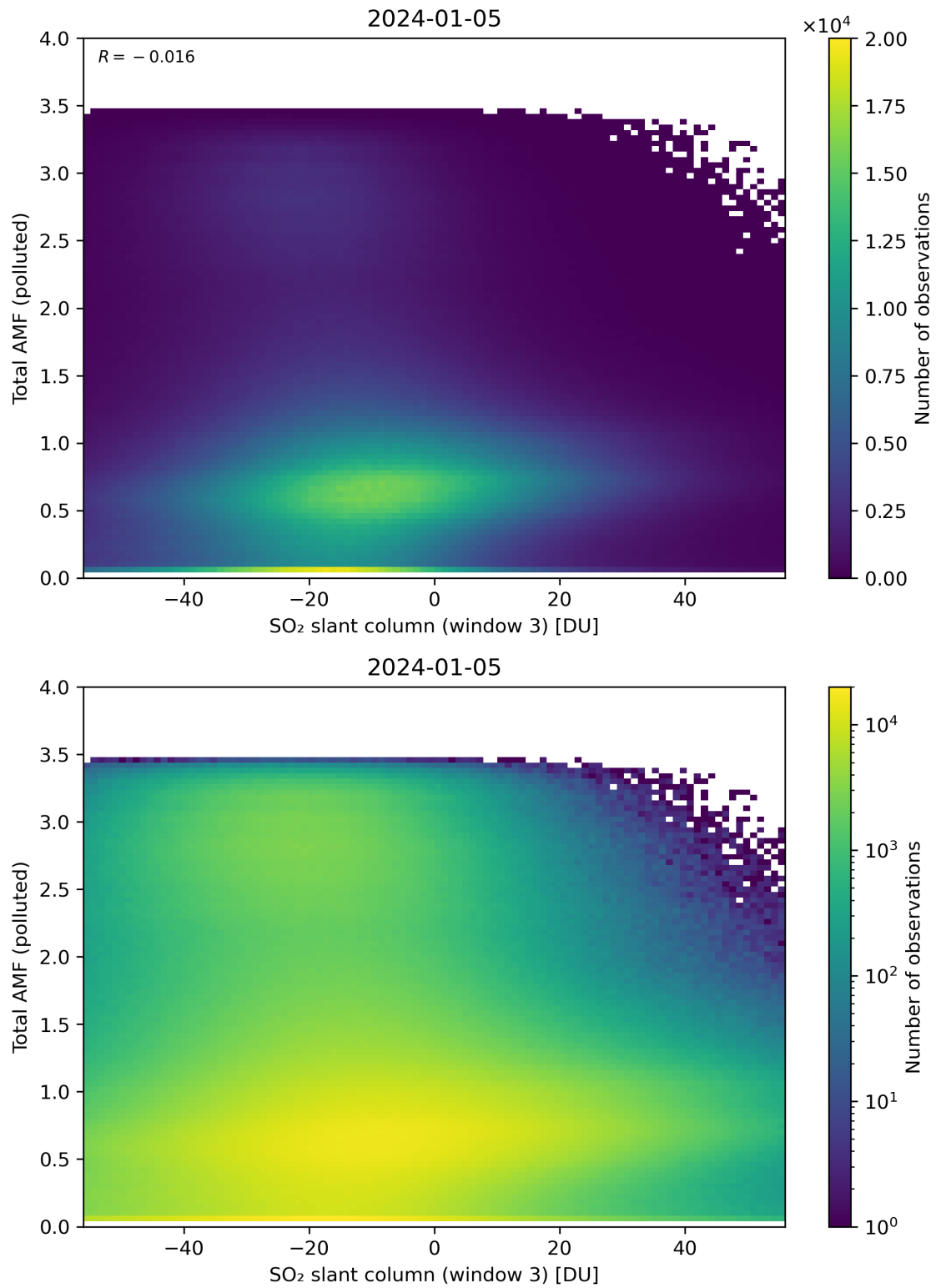
Figure 268: Scatter density plot of “SO 2 slant column (window 3)” against “Total AMF (polluted)” for 2024-01-05 to 2024-01-06.
