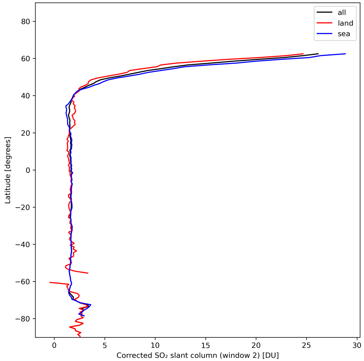
Figure 39: Zonal average of “Corrected SO 2 slant column (window 2)” for 2024-01-05 to 2024-01-06.
