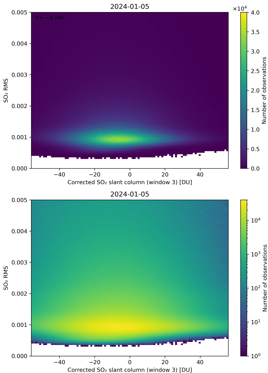
Figure 208: Scatter density plot of “Corrected SO 2 slant column (window 3)” against “SO 2 RMS” for 2024-01-05 to 2024-01-06.
