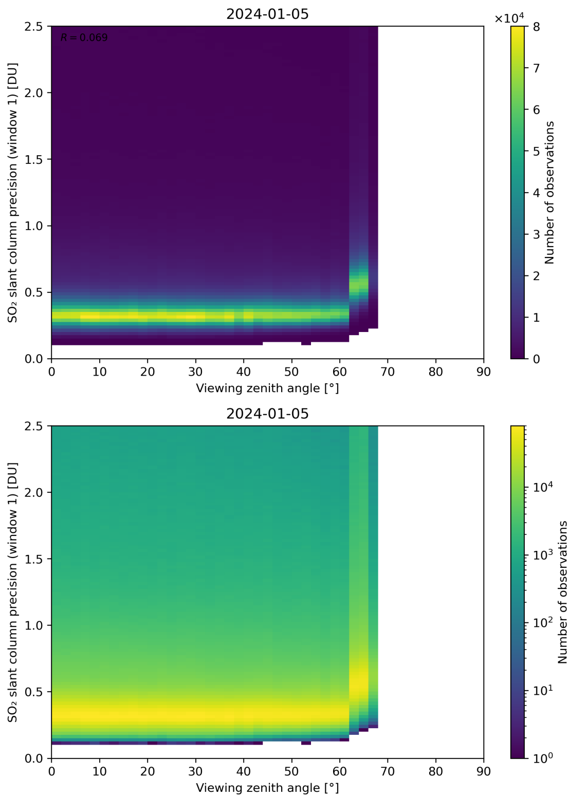
Figure 321: Scatter density plot of “Viewing zenith angle” against “SO 2 slant column precision (window 1)” for 2024-01-05 to 2024-01-06.
