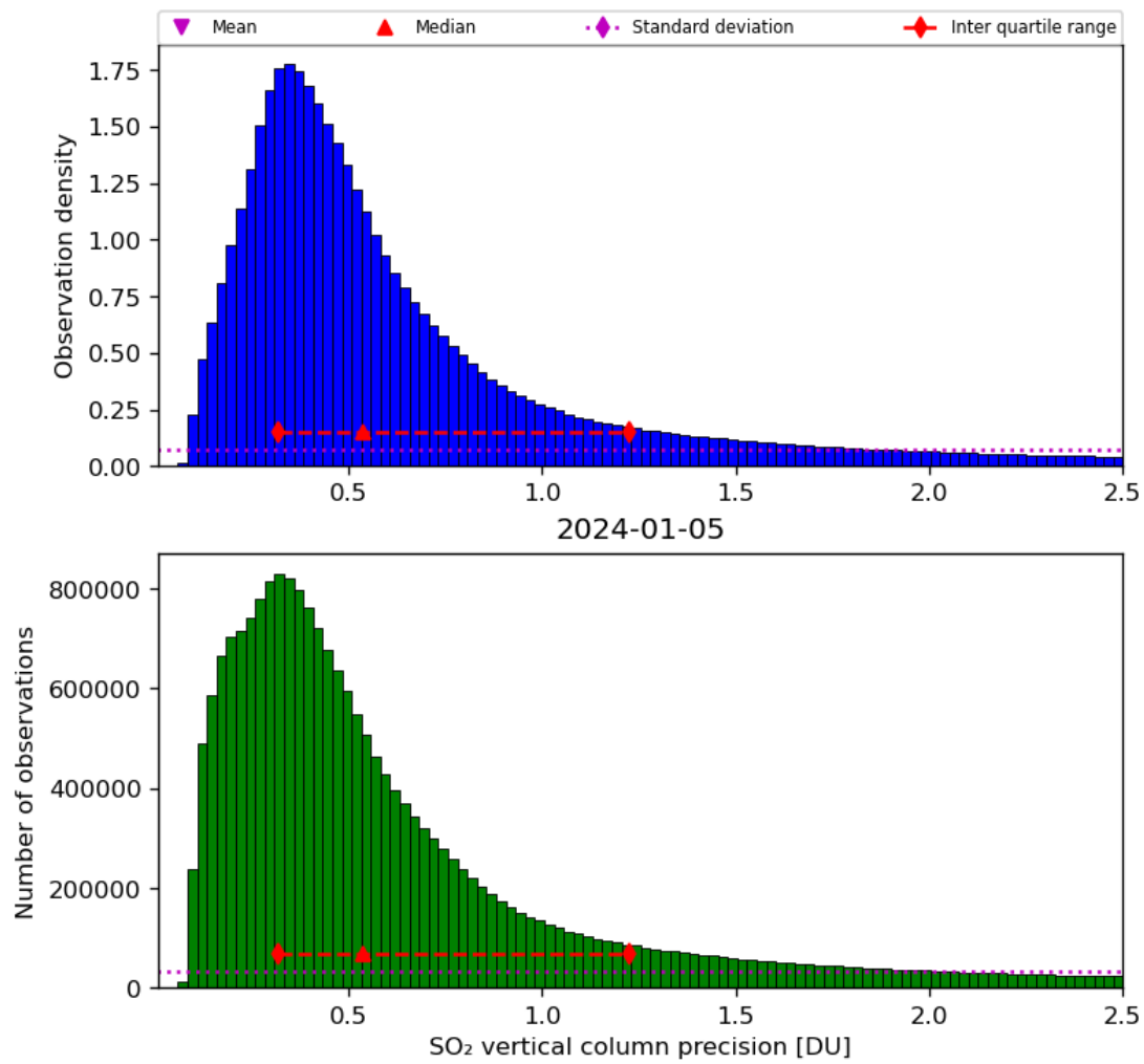
Figure 54: Histogram of “SO 2 vertical column precision” for 2024-01-05 to 2024-01-06
