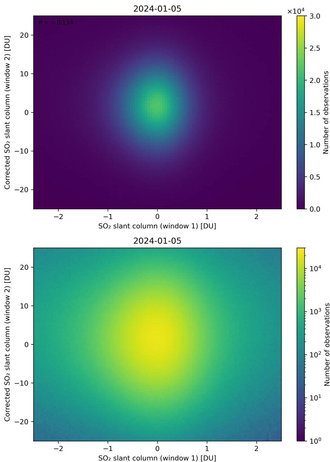
Figure 233: Scatter density plot of “SO 2 slant column (window 1)” against “Corrected SO 2 slant column (window 2)” for 2024-01-05 to 2024-01-06.
