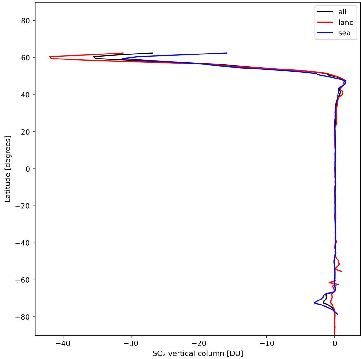
Figure 30: Zonal average of “SO 2 vertical column” for 2024-01-05 to 2024-01-06.
