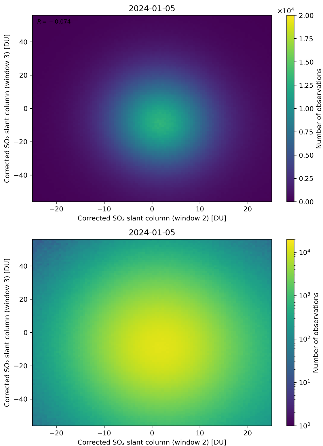
Figure 200: Scatter density plot of “Corrected SO 2 slant column (window 2)” against “Corrected SO 2 slant column (window 3)” for 2024-01-05 to 2024-01-06.
