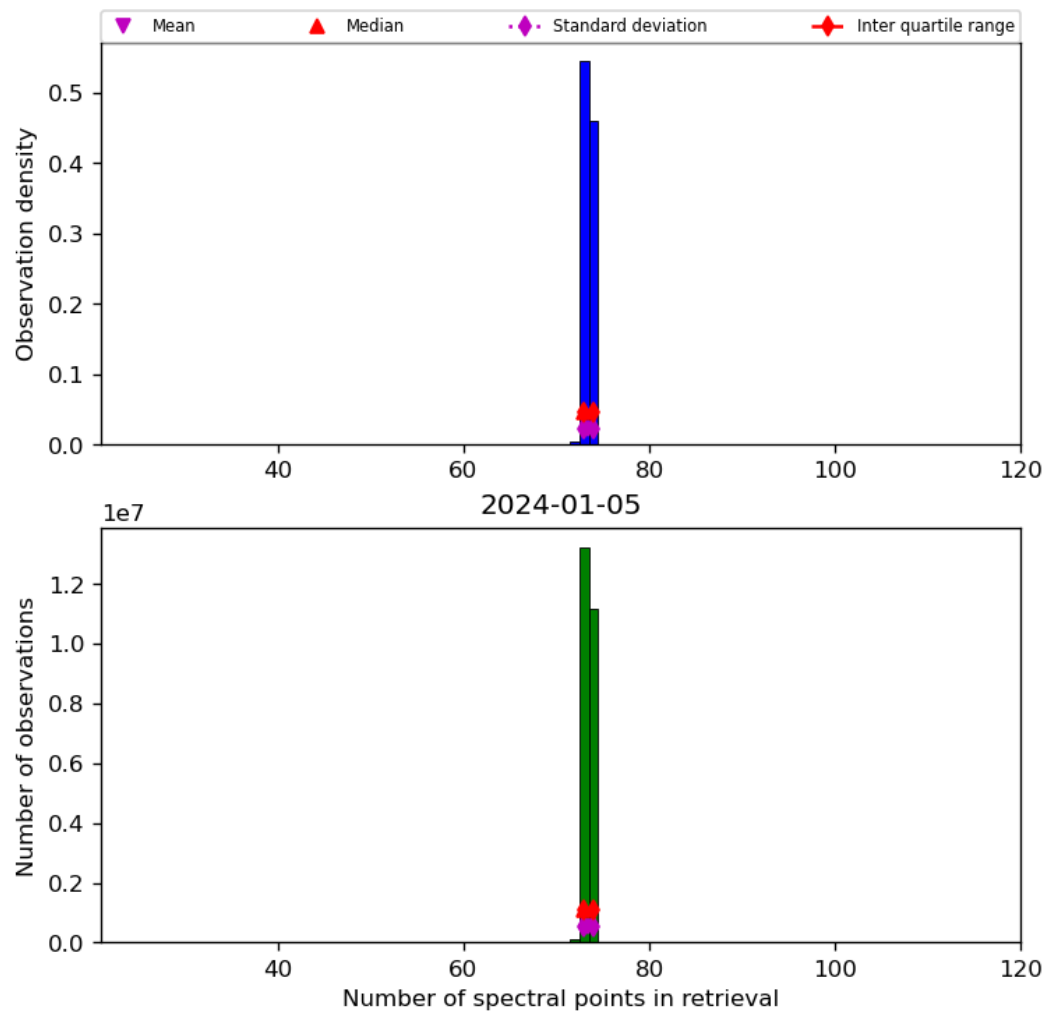
Figure 74: Histogram of “Number of spectral points in retrieval” for 2024-01-05 to 2024-01-06
