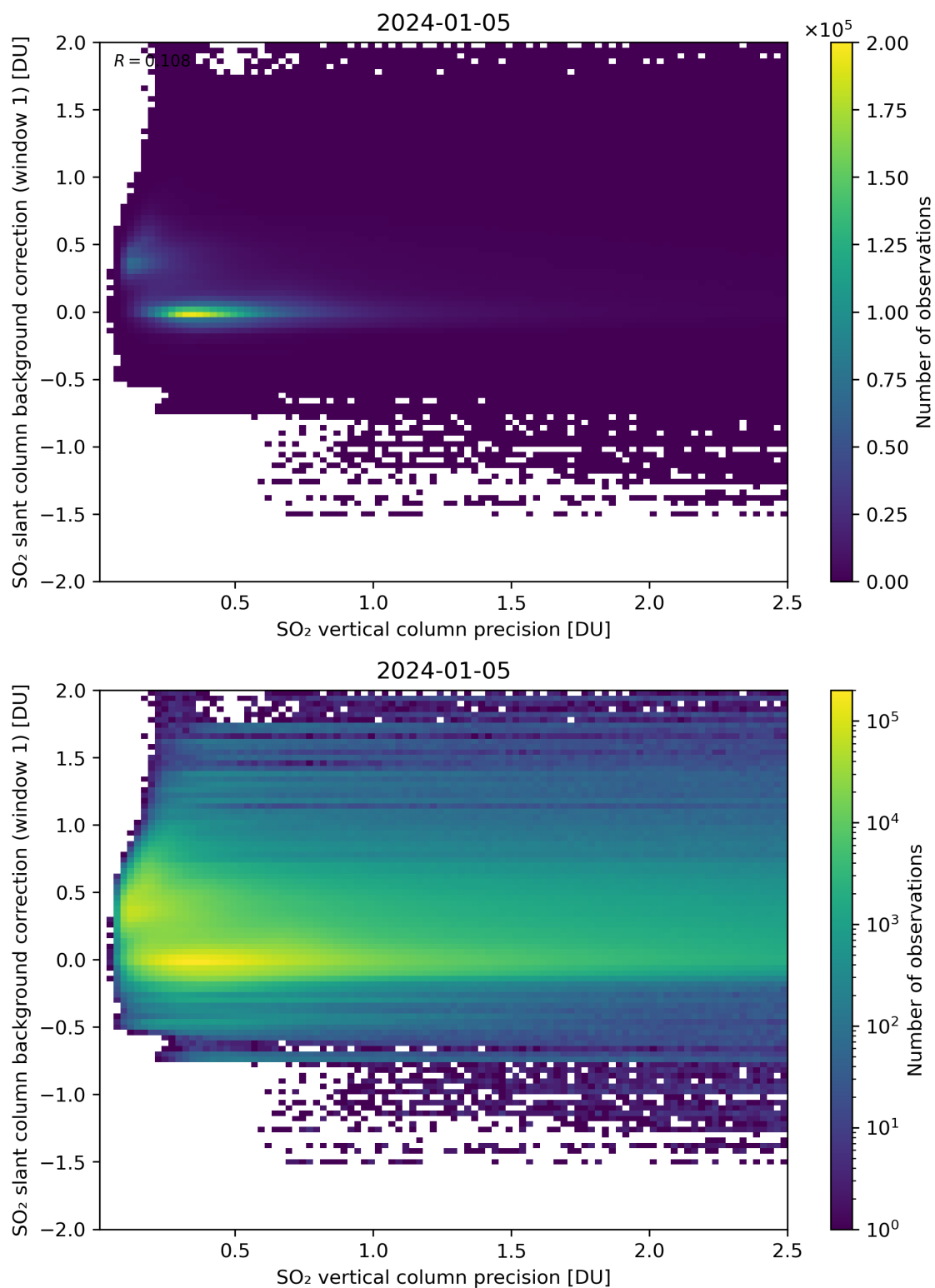
Figure 279: Scatter density plot of “SO 2 vertical column precision” against “SO 2 slant column background correction (window 1)” for 2024-01-05 to 2024-01-06.
