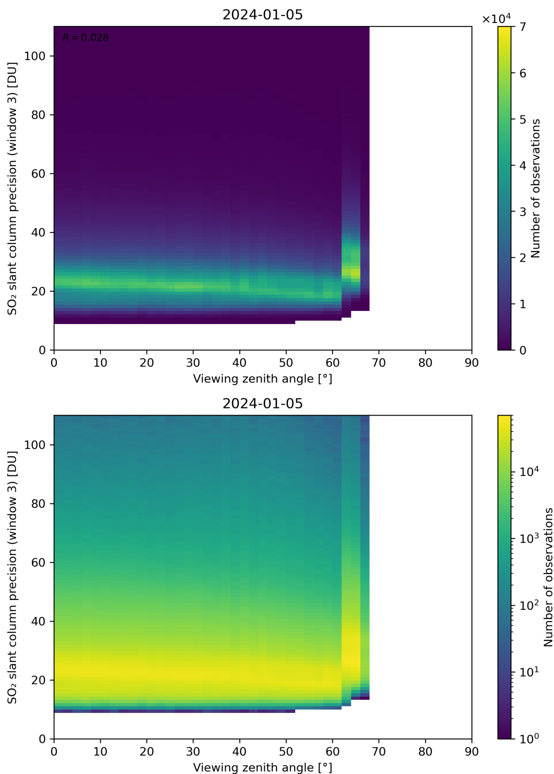
Figure 324: Scatter density plot of “Viewing zenith angle” against “SO 2 slant column precision (window 3)” for 2024-01-05 to 2024-01-06.
