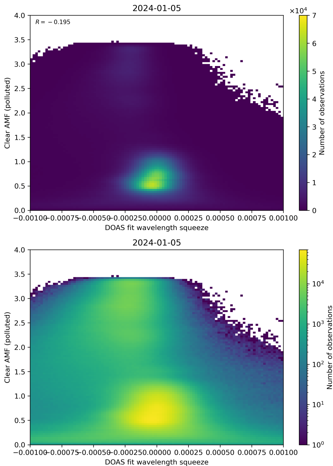
Figure 133: Scatter density plot of “DOAS fit wavelength squeeze” against “Clear AMF (polluted)” for 2024-01-05 to 2024-01-06.
