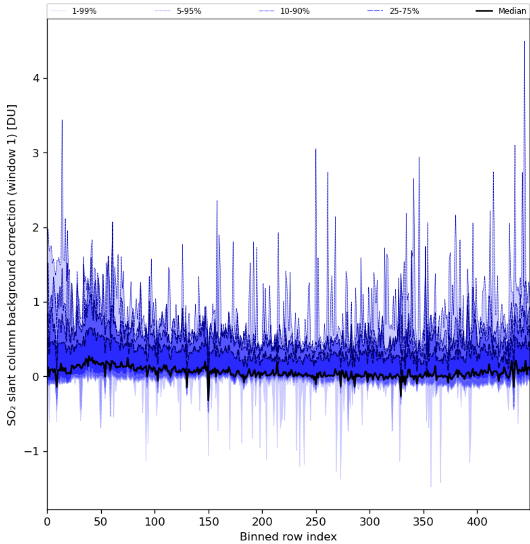
Figure 82: Along track statistics of “SO 2 slant column background correction (window 1)” for 2024-01-05 to 2024-01-06
