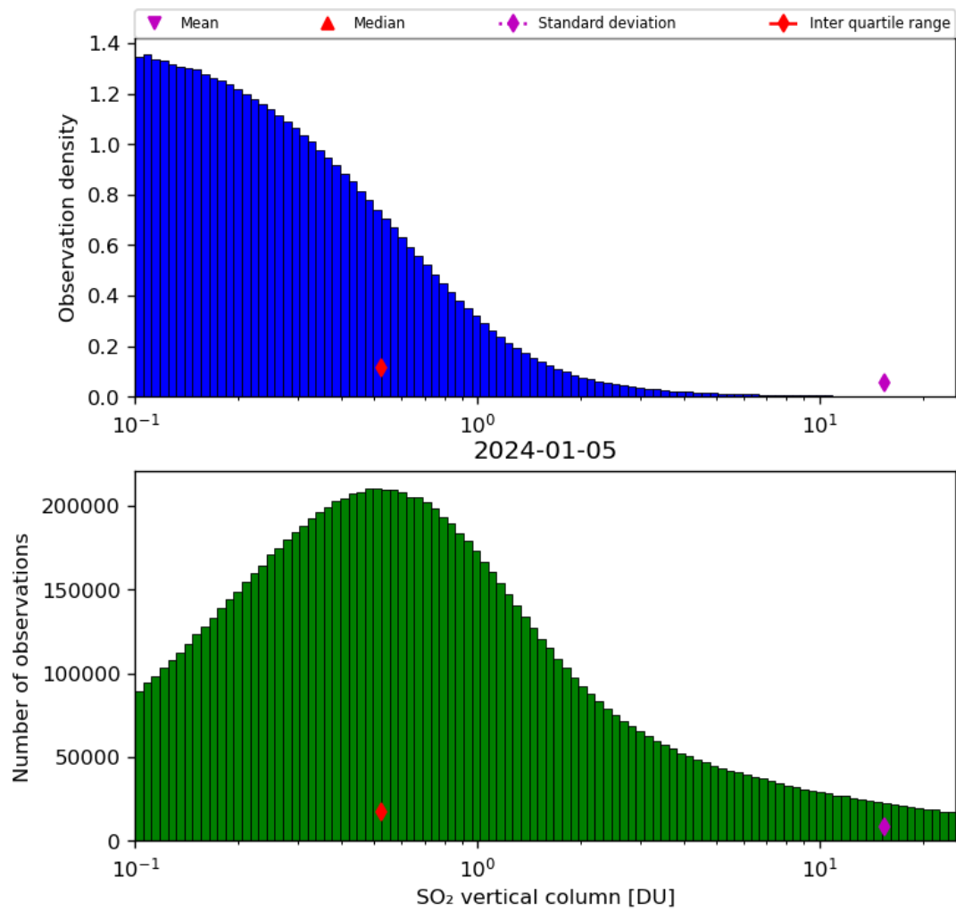
Figure 53: Histogram of “SO 2 vertical column” for 2024-01-05 to 2024-01-06
