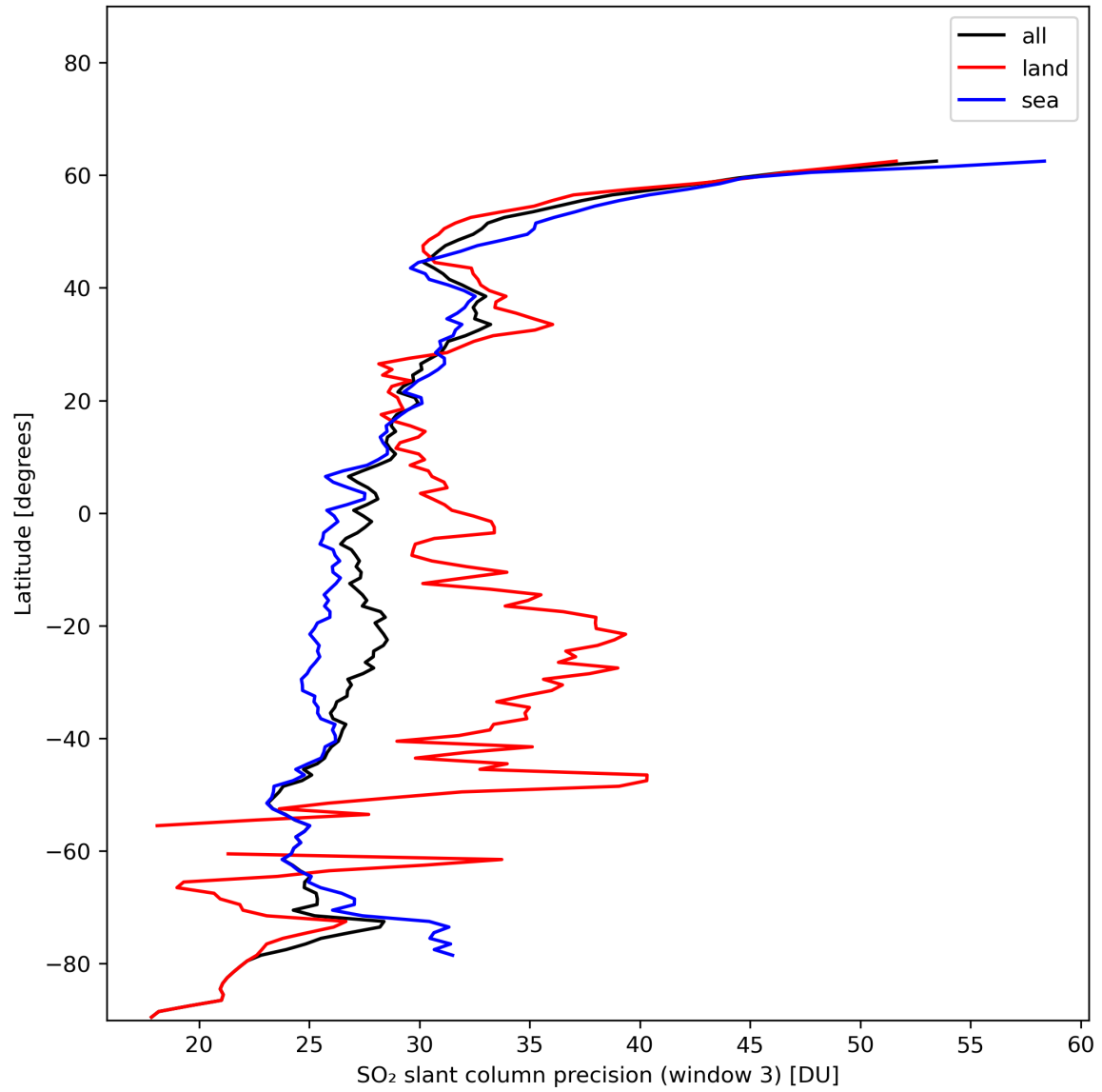
Figure 42: Zonal average of “SO 2 slant column precision (window 3)” for 2024-01-05 to 2024-01-06.
