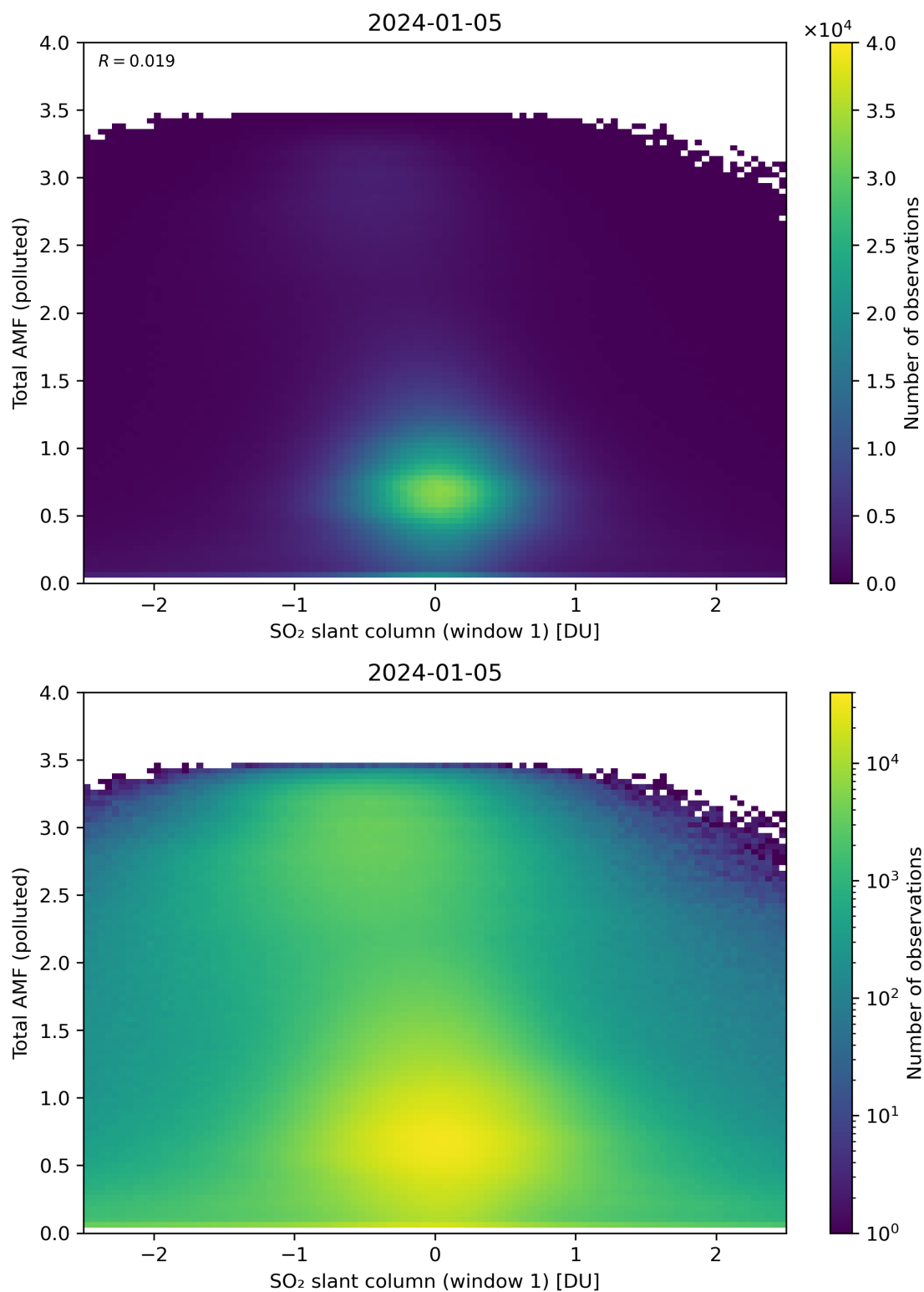
Figure 239: Scatter density plot of “SO 2 slant column (window 1)” against “Total AMF (polluted)” for 2024-01-05 to 2024-01-06.
