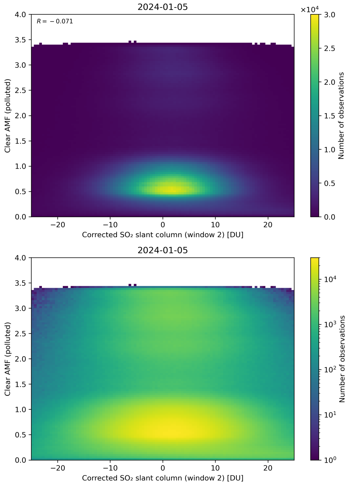
Figure 199: Scatter density plot of “Corrected SO 2 slant column (window 2)” against “Clear AMF (polluted)” for 2024-01-05 to 2024-01-06.
