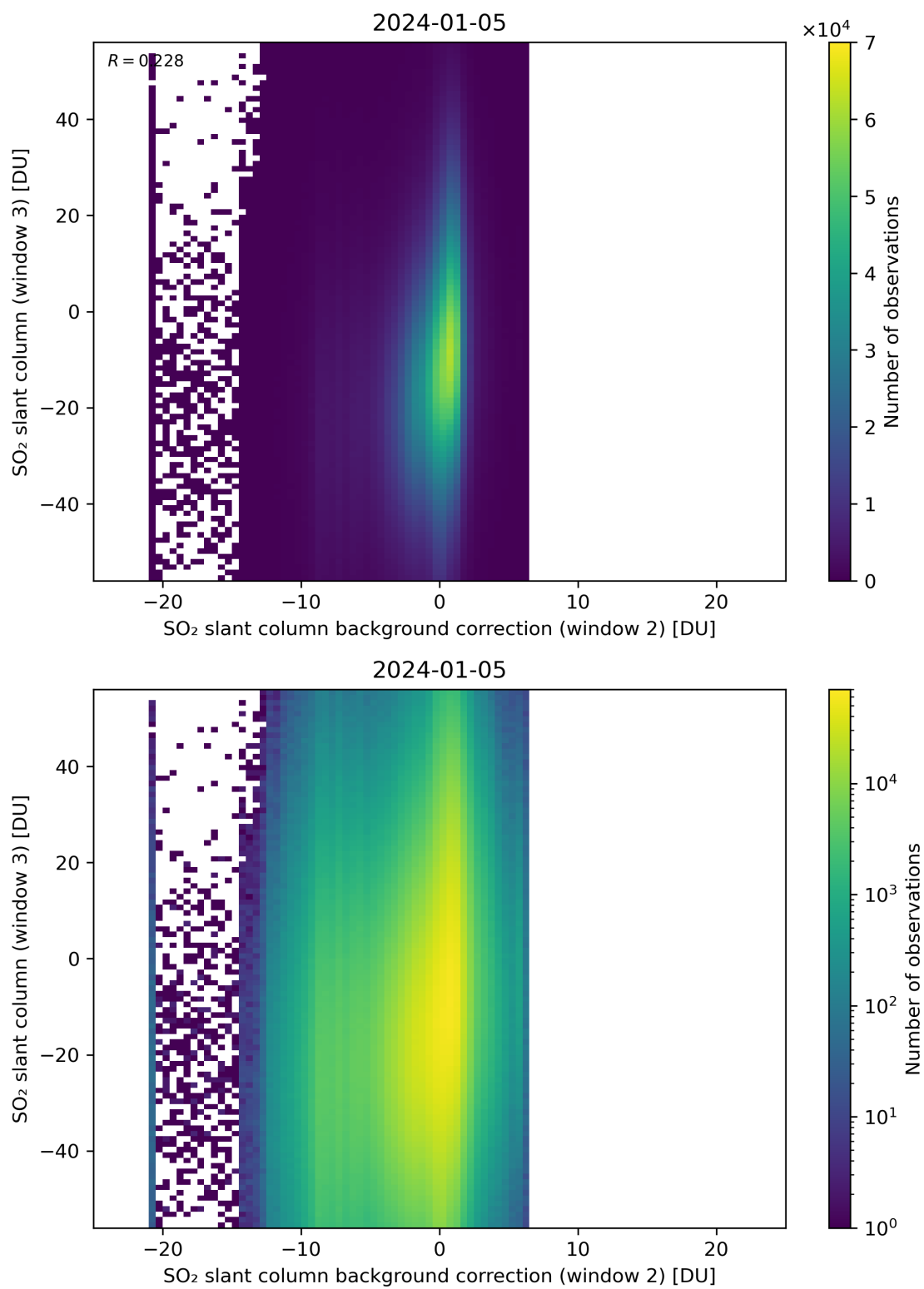
Figure 117: Scatter density plot of “SO 2 slant column background correction (window 2)” against “SO 2 slant column (window 3)” for 2024-01-05 to 2024-01-06.
