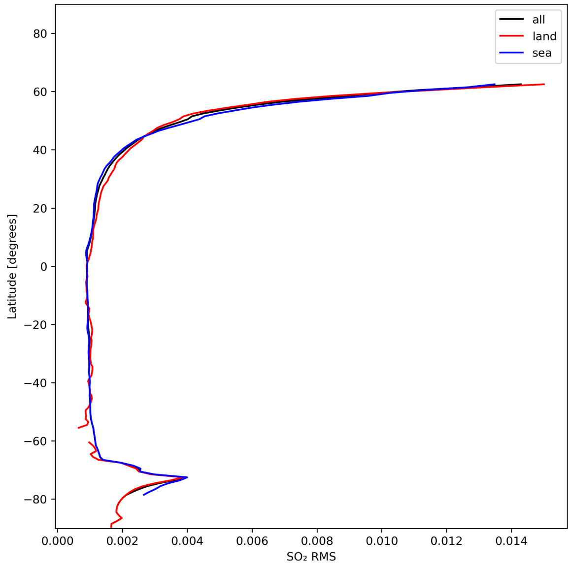
Figure 47: Zonal average of “SO 2 RMS” for 2024-01-05 to 2024-01-06.
