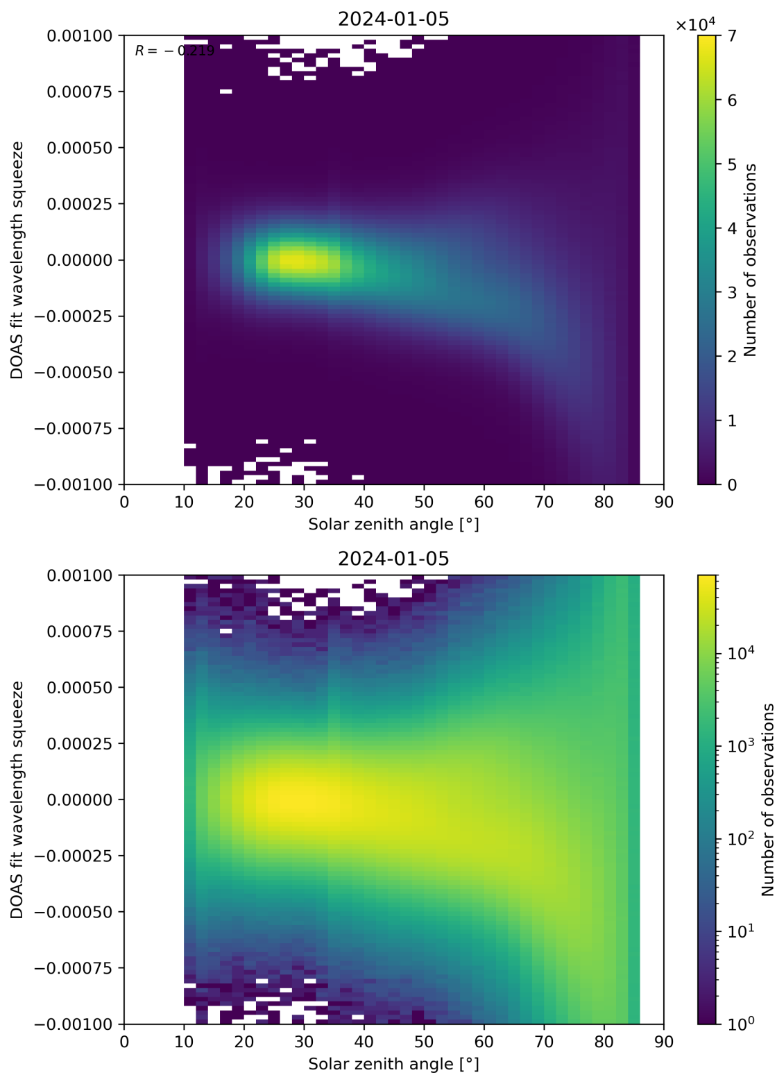
Figure 162: Scatter density plot of “Solar zenith angle” against “DOAS fit wavelength squeeze” for 2024-01-05 to 2024-01-06.
