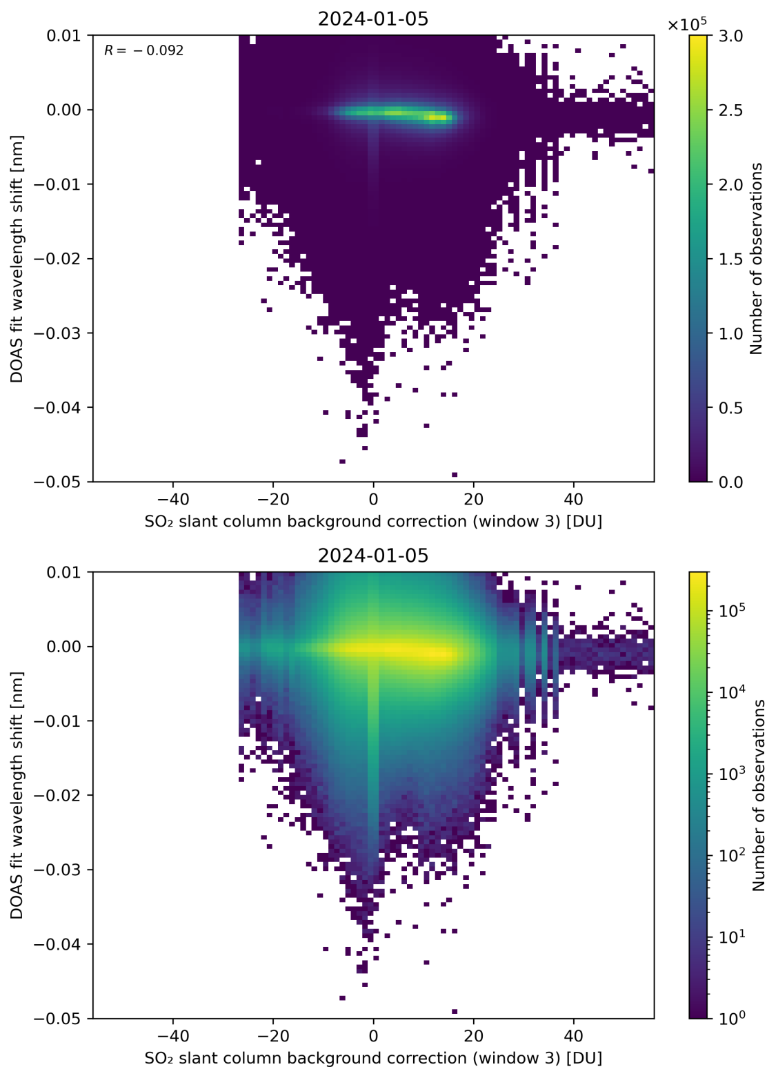
Figure 121: Scatter density plot of “SO 2 slant column background correction (window 3)” against “DOAS fit wavelength shift” for 2024-01-05 to 2024-01-06.
