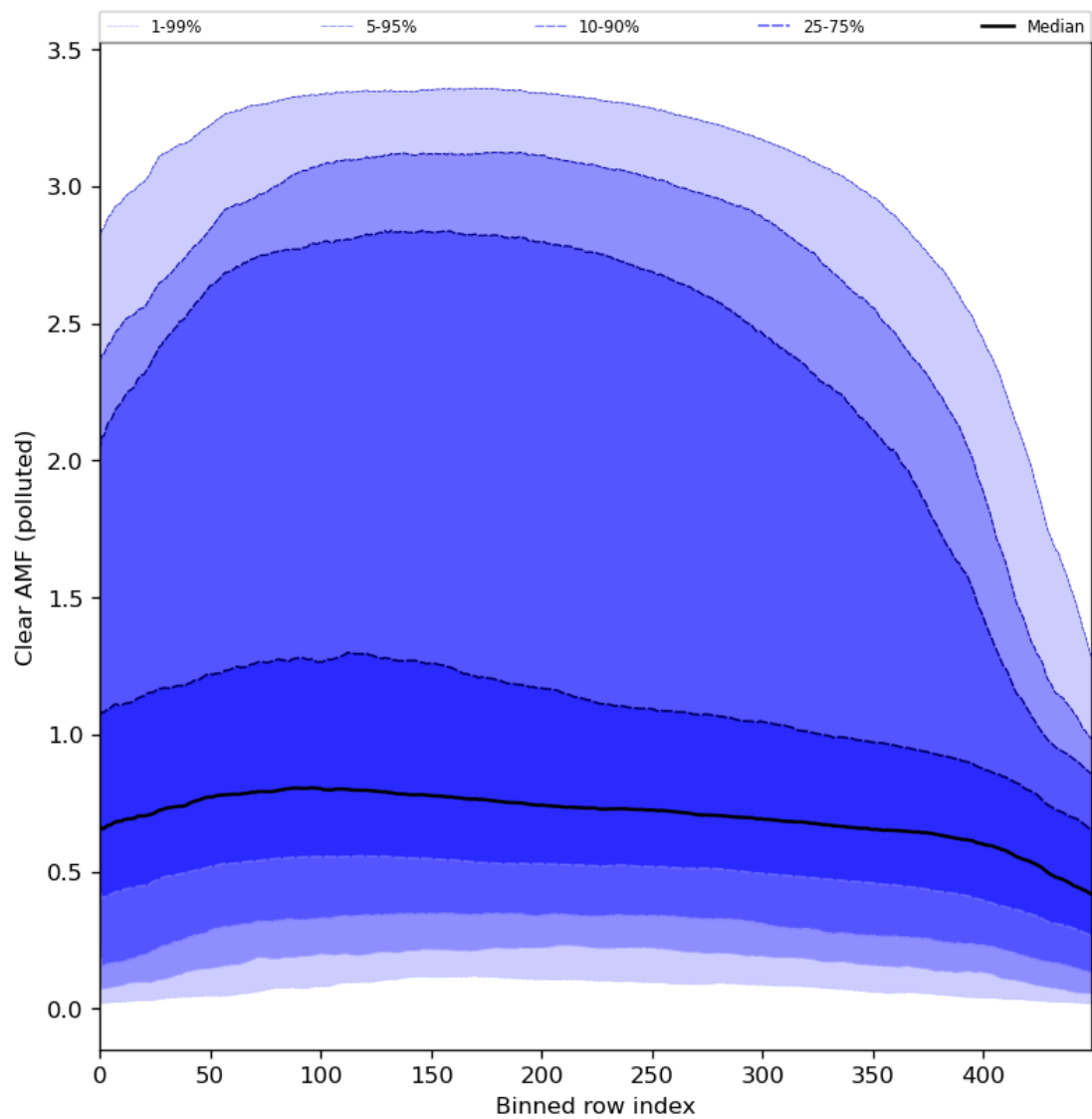
Figure 96: Along track statistics of “Clear AMF (polluted)” for 2024-01-05 to 2024-01-06
