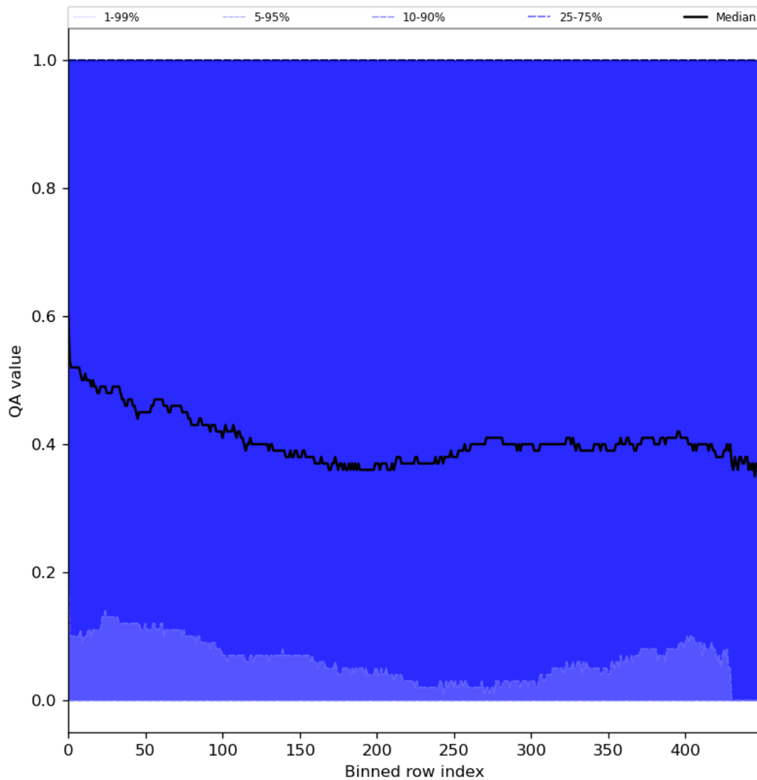
Figure 75: Along track statistics of “QA value” for 2024-01-05 to 2024-01-06
