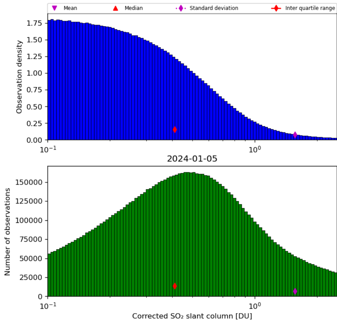
Figure 55: Histogram of “Corrected SO 2 slant column” for 2024-01-05 to 2024-01-06
