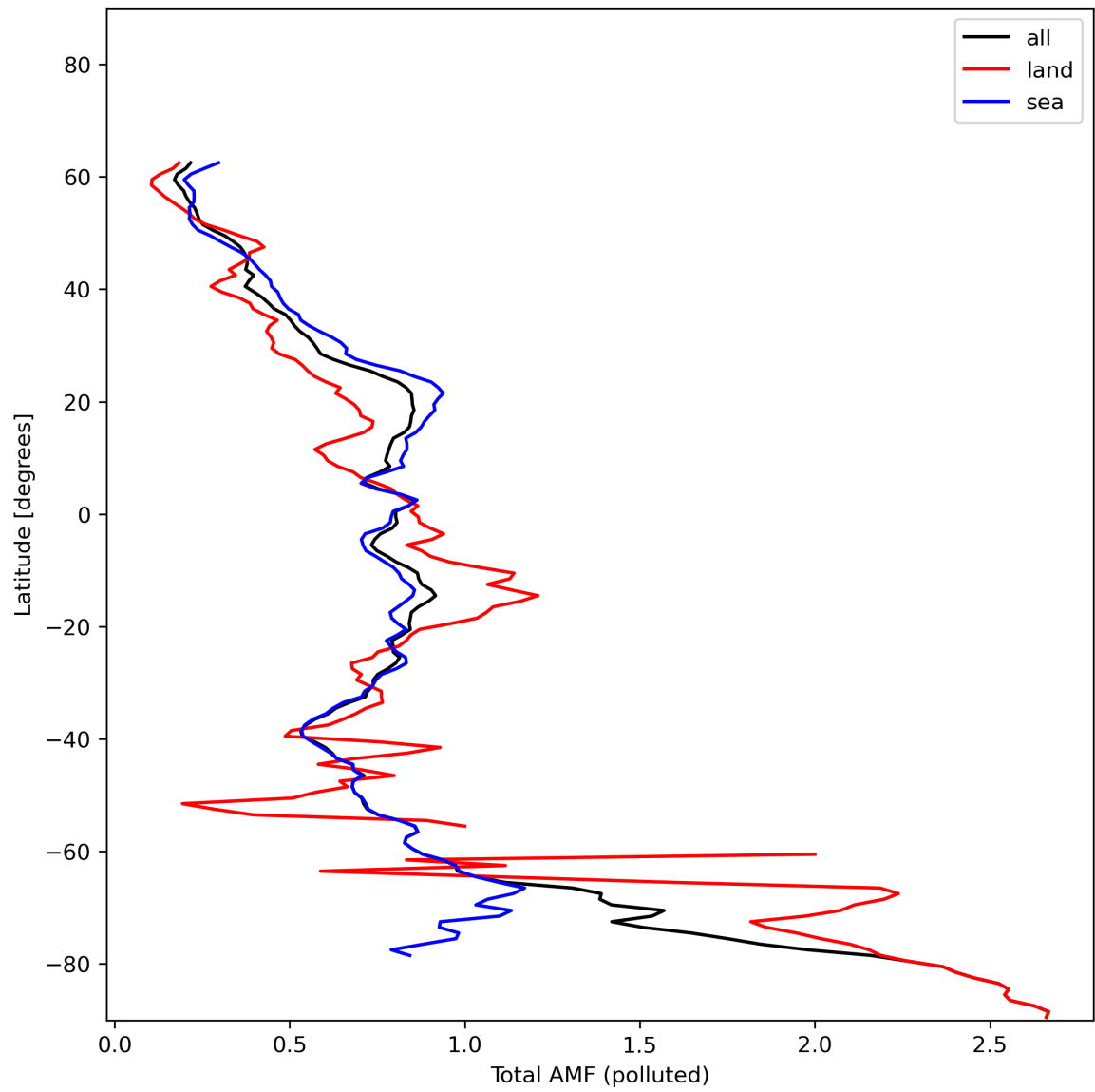
Figure 48: Zonal average of “Total AMF (polluted)” for 2024-01-05 to 2024-01-06.
