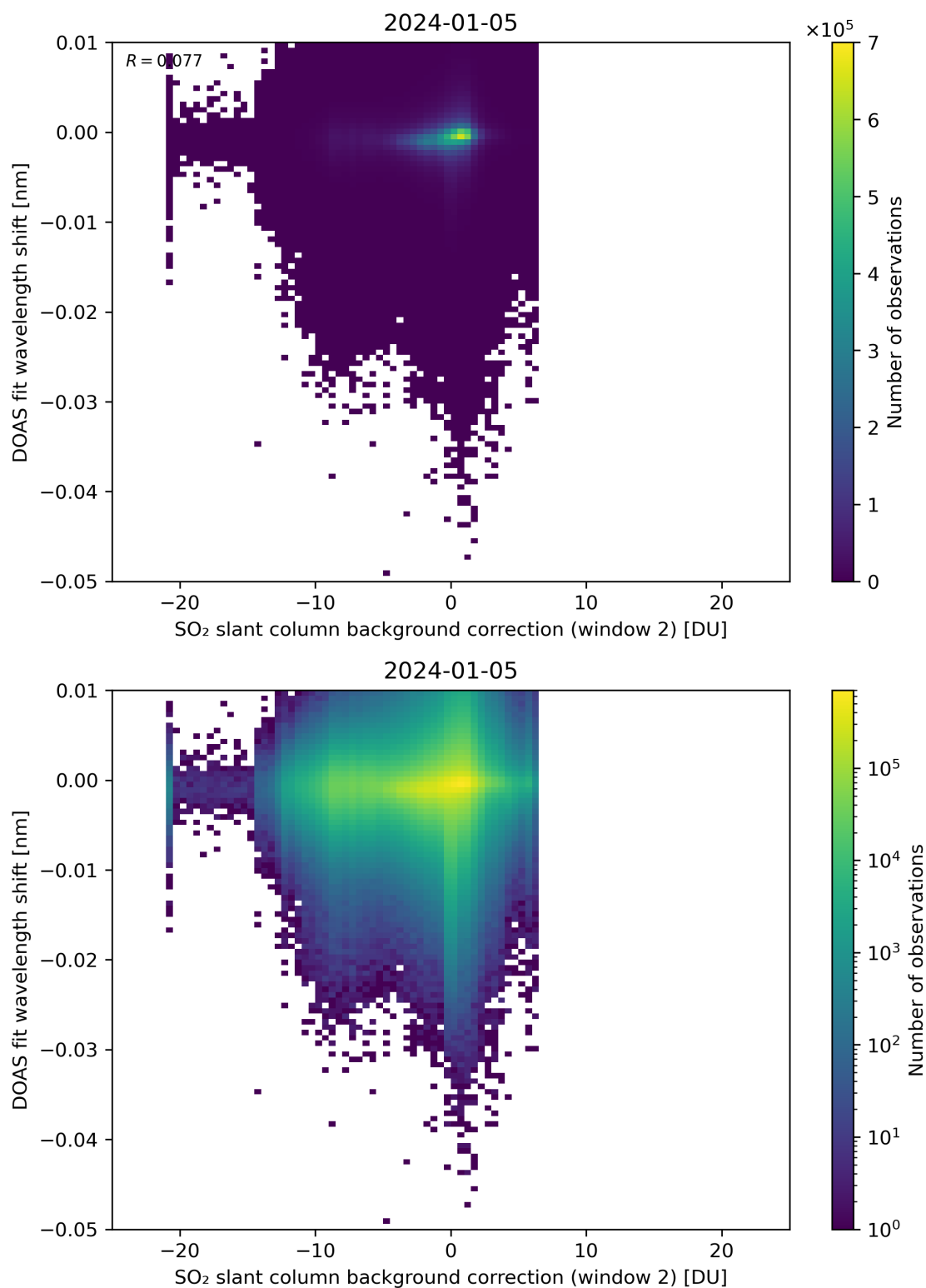
Figure 112: Scatter density plot of “SO 2 slant column background correction (window 2)” against “DOAS fit wavelength shift” for 2024-01-05 to 2024-01-06.
