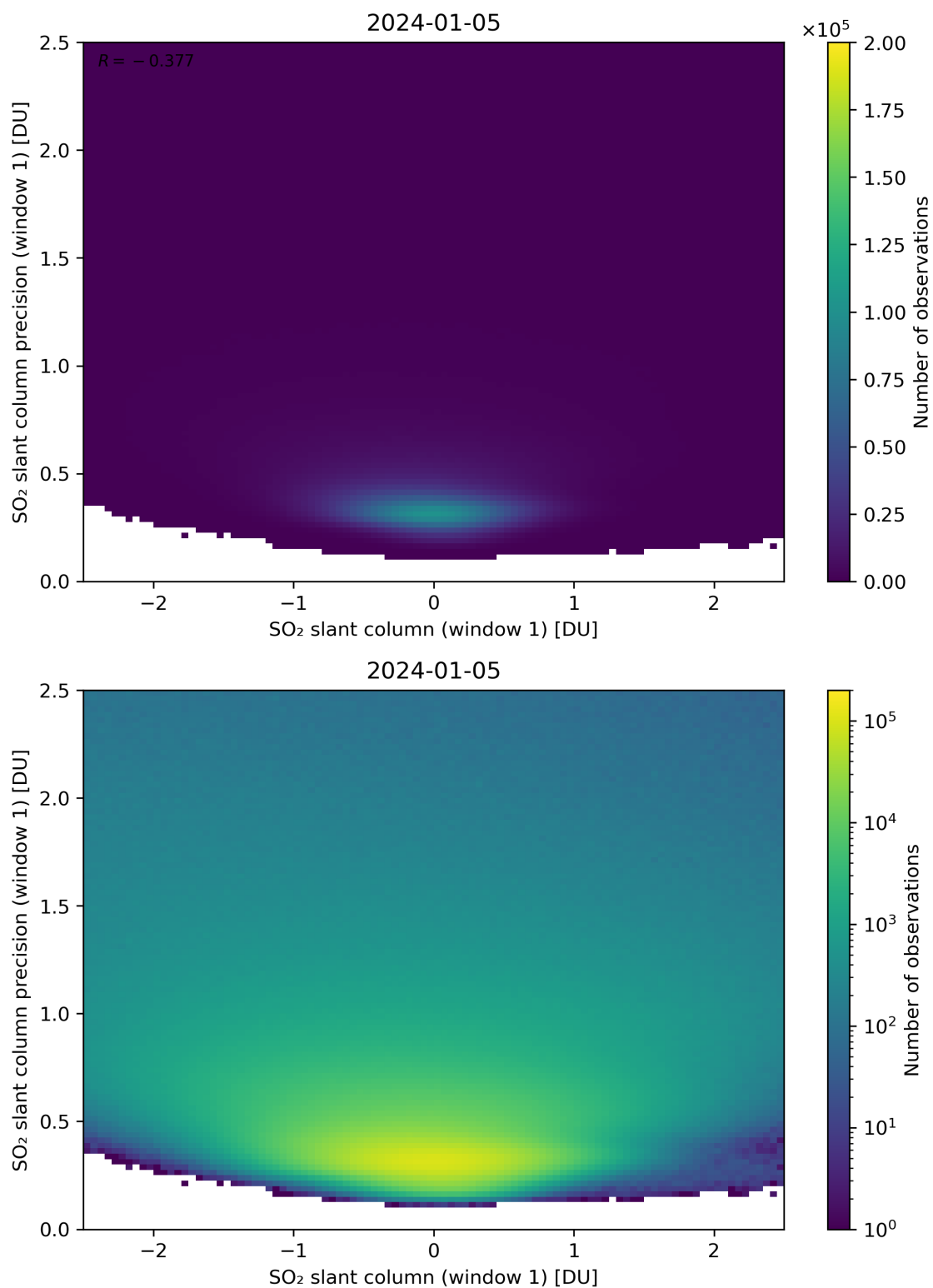
Figure 235: Scatter density plot of “SO 2 slant column (window 1)” against “SO 2 slant column precision (window 1)” for 2024-01-05 to 2024-01-06.
