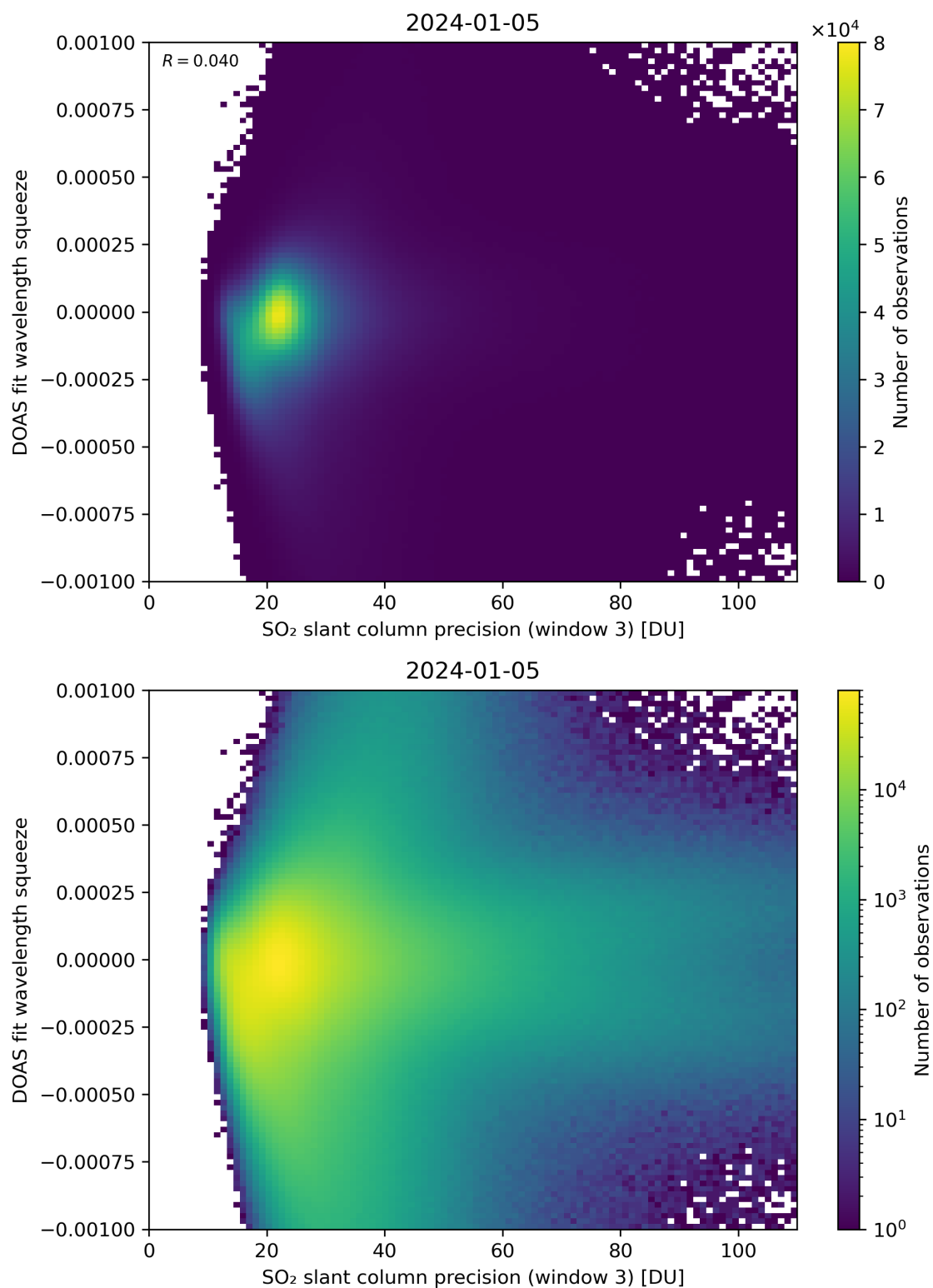
Figure 259: Scatter density plot of “SO 2 slant column precision (window 3)” against “DOAS fit wavelength squeeze” for 2024-01-05 to 2024-01-06.
