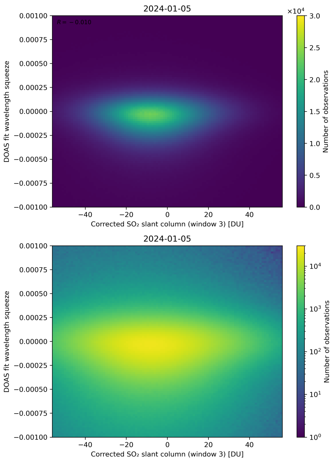
Figure 207: Scatter density plot of “Corrected SO 2 slant column (window 3)” against “DOAS fit wavelength squeeze” for 2024-01-05 to 2024-01-06.
