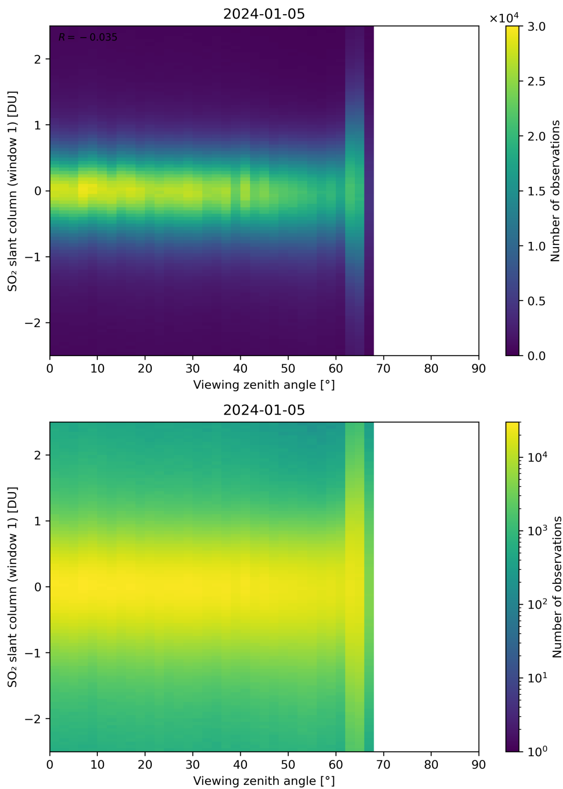
Figure 320: Scatter density plot of “Viewing zenith angle” against “SO 2 slant column (window 1)” for 2024-01-05 to 2024-01-06.
