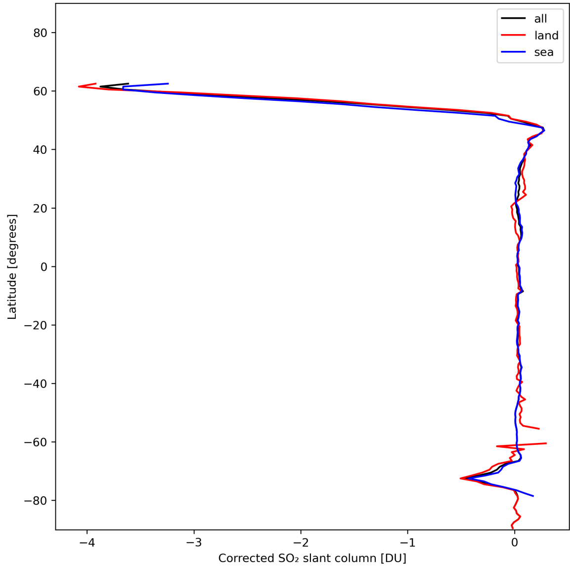
Figure 32: Zonal average of “Corrected SO 2 slant column” for 2024-01-05 to 2024-01-06.
