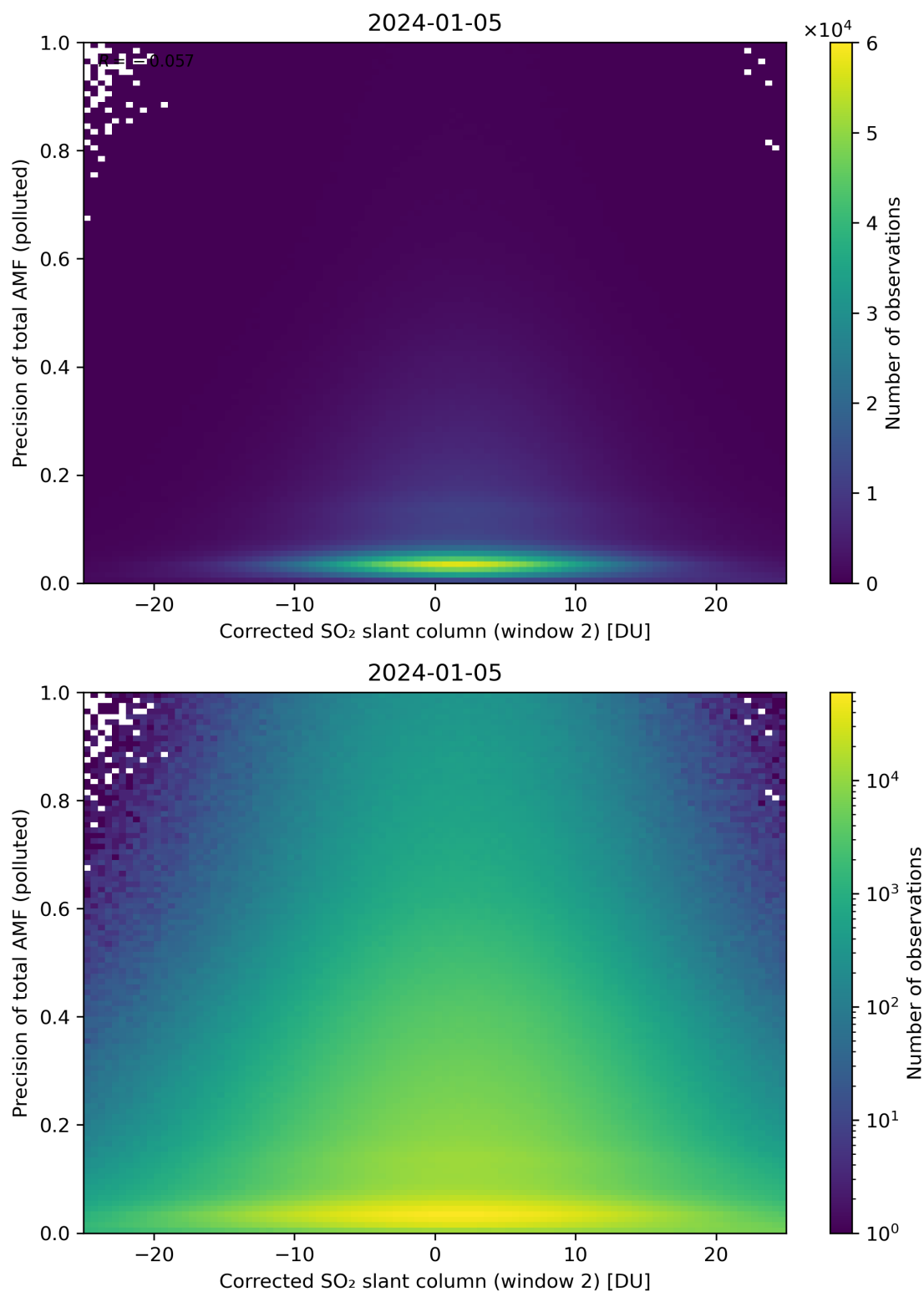
Figure 204: Scatter density plot of “Corrected SO 2 slant column (window 2)” against “Precision of total AMF (polluted)” for 2024-01-05 to 2024-01-06.
