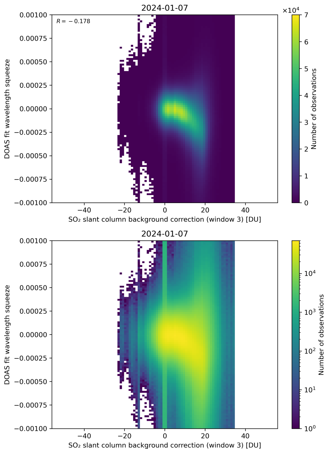
Figure 122: Scatter density plot of “SO 2 slant column background correction (window 3)” against “DOAS fit wavelength squeeze” for 2024-01-06 to 2024-01-08.
