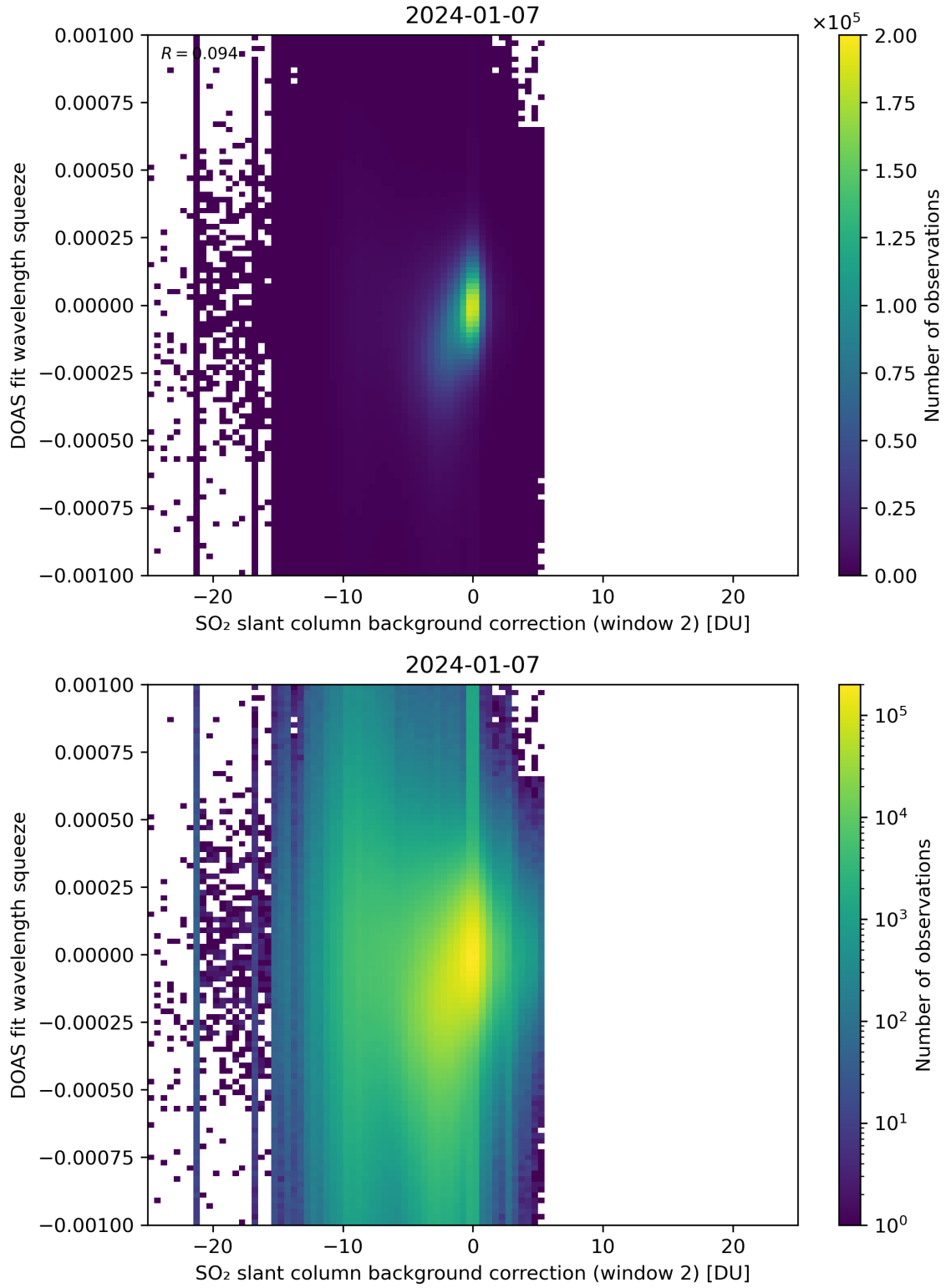
Figure 113: Scatter density plot of “SO 2 slant column background correction (window 2)” against “DOAS fit wavelength squeeze” for 2024-01-06 to 2024-01-08.
