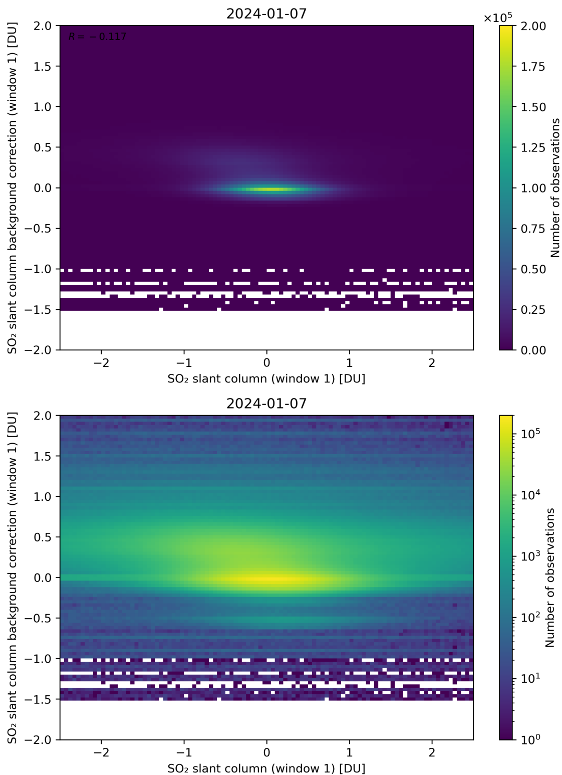
Figure 212: Scatter density plot of “SO 2 slant column (window 1)” against “SO 2 slant column background correction (window 1)” for 2024-01-06 to 2024-01-08.
