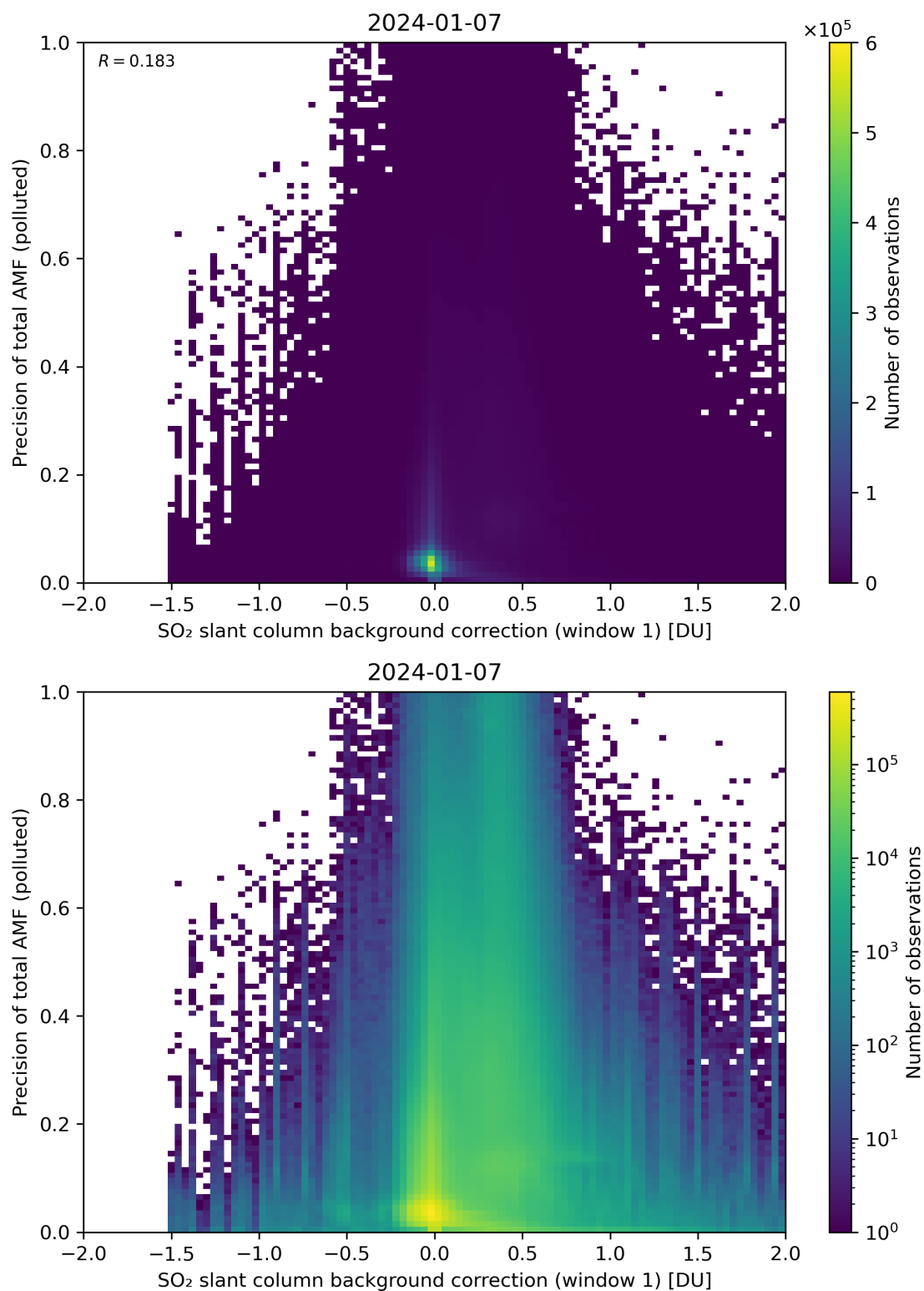
Figure 110: Scatter density plot of “SO 2 slant column background correction (window 1)” against “Precision of total AMF (polluted)” for 2024-01-06 to 2024-01-08.
