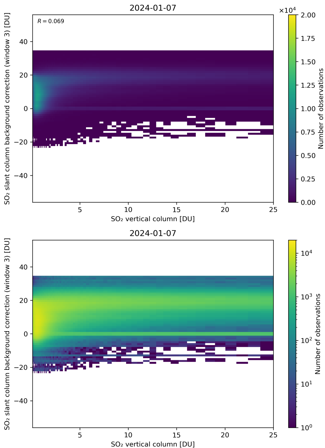
Figure 275: Scatter density plot of “SO 2 vertical column” against “SO 2 slant column background correction (window 3)” for 2024-01-06 to 2024-01-08.
