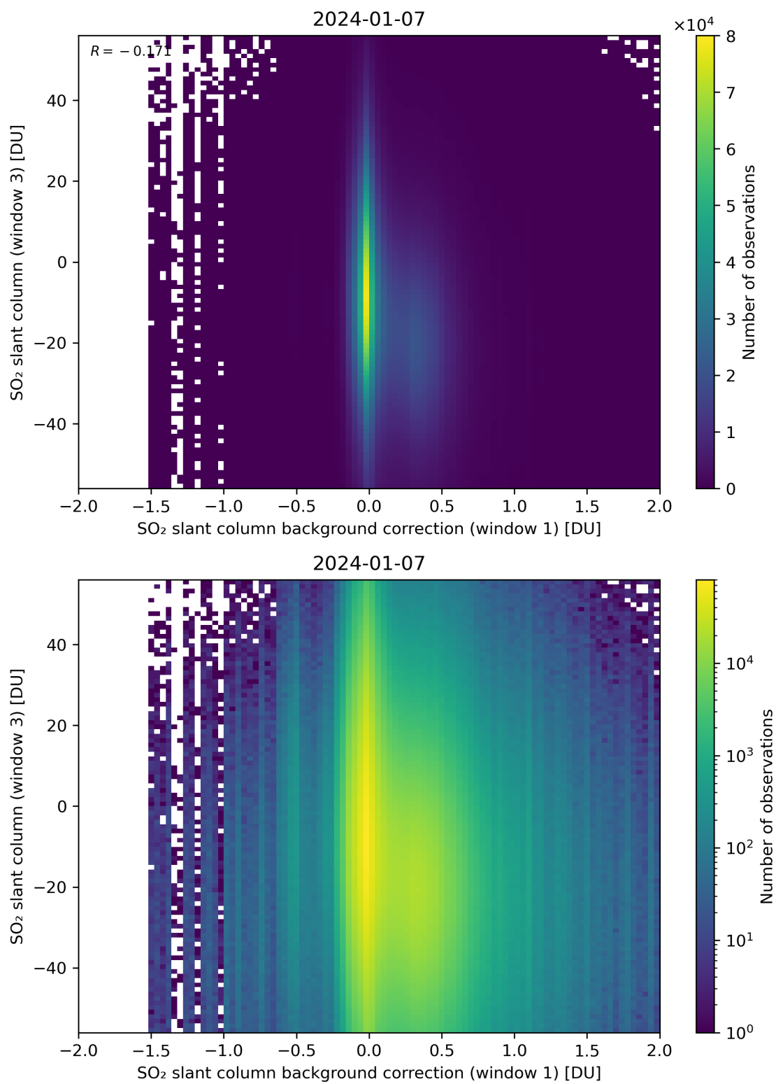
Figure 107: Scatter density plot of “SO 2 slant column background correction (window 1)” against “SO 2 slant column (window 3)” for 2024-01-06 to 2024-01-08.
