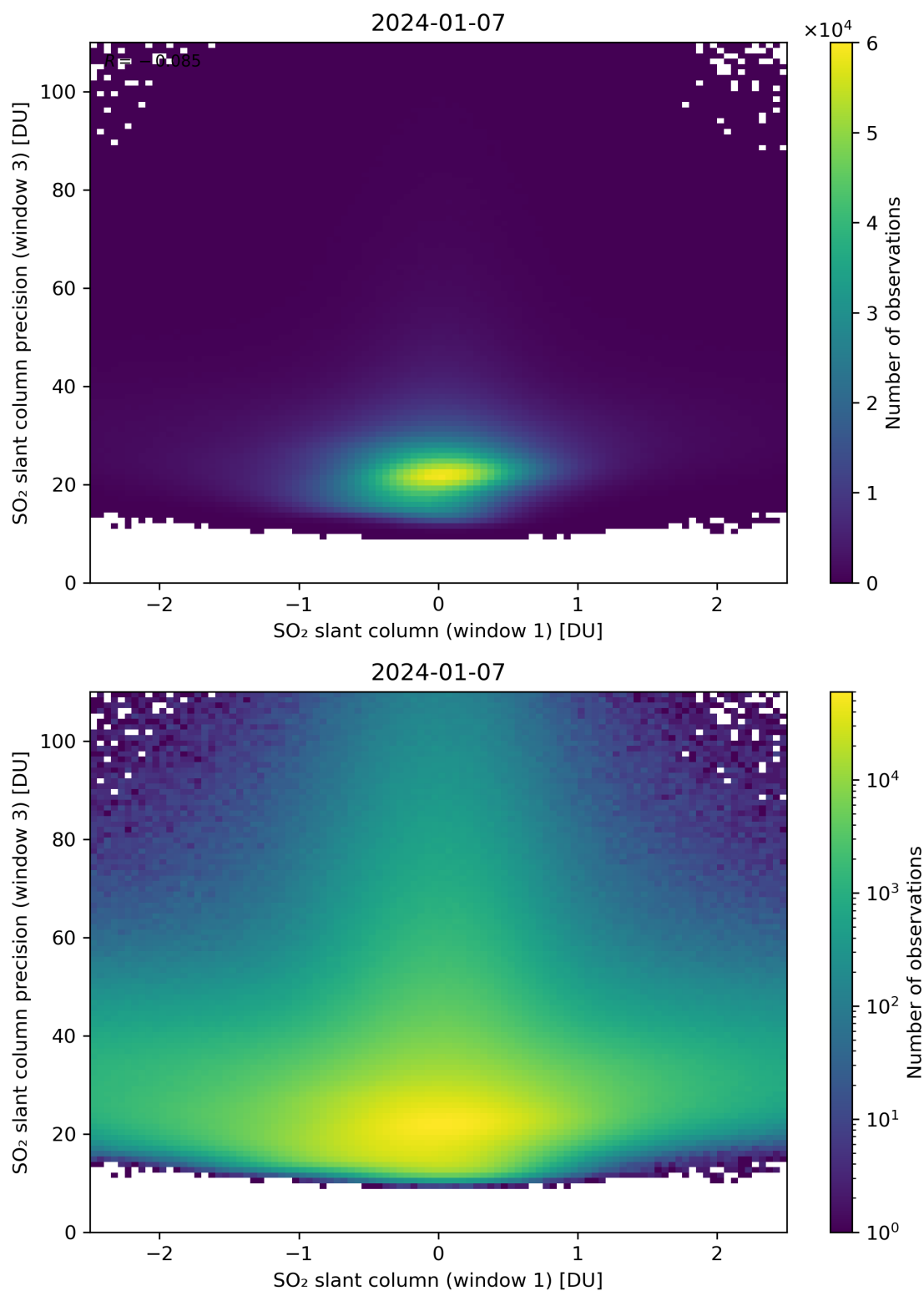
Figure 238: Scatter density plot of “SO 2 slant column (window 1)” against “SO 2 slant column precision (window 3)” for 2024-01-06 to 2024-01-08.
