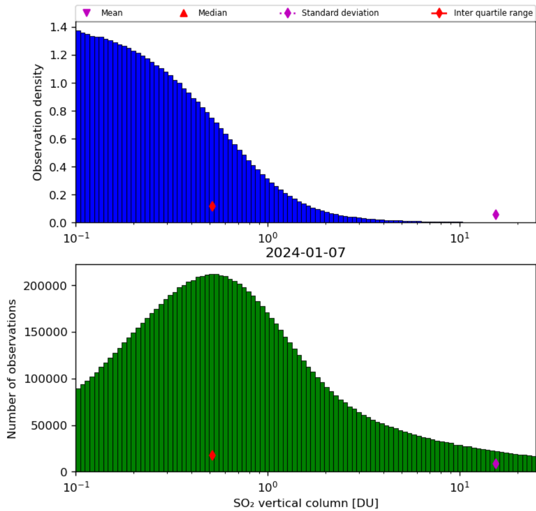
Figure 53: Histogram of “SO 2 vertical column” for 2024-01-06 to 2024-01-08
