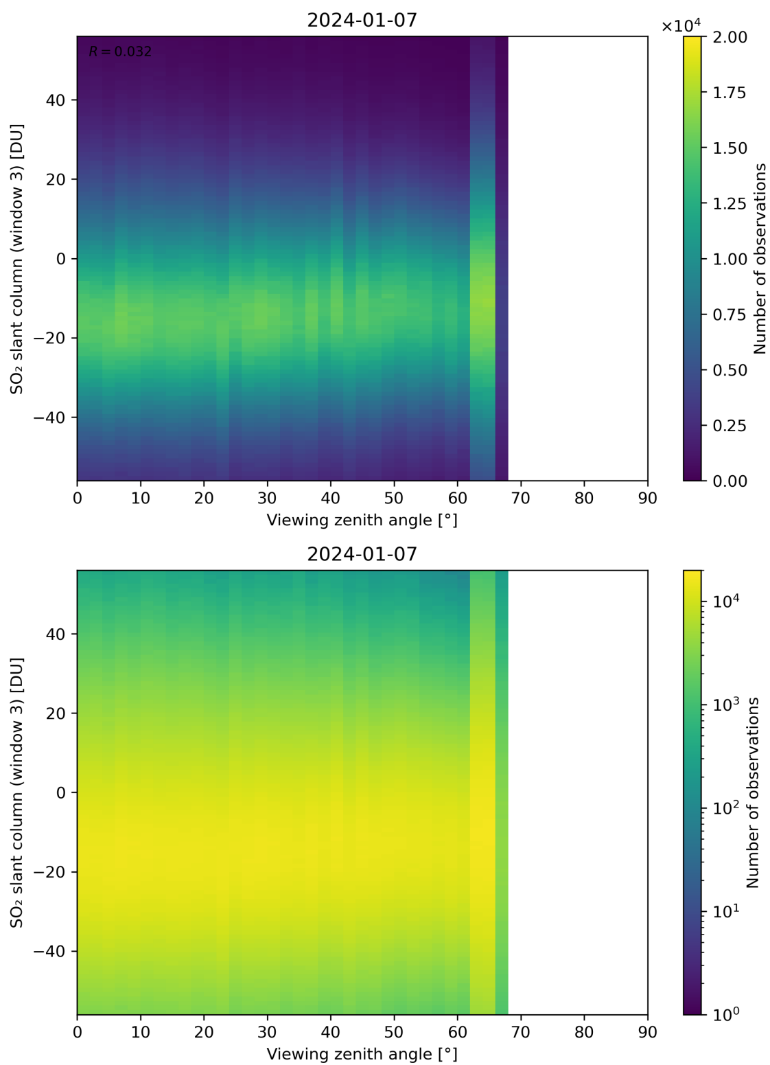
Figure 323: Scatter density plot of “Viewing zenith angle” against “SO 2 slant column (window 3)” for 2024-01-06 to 2024-01-08.
