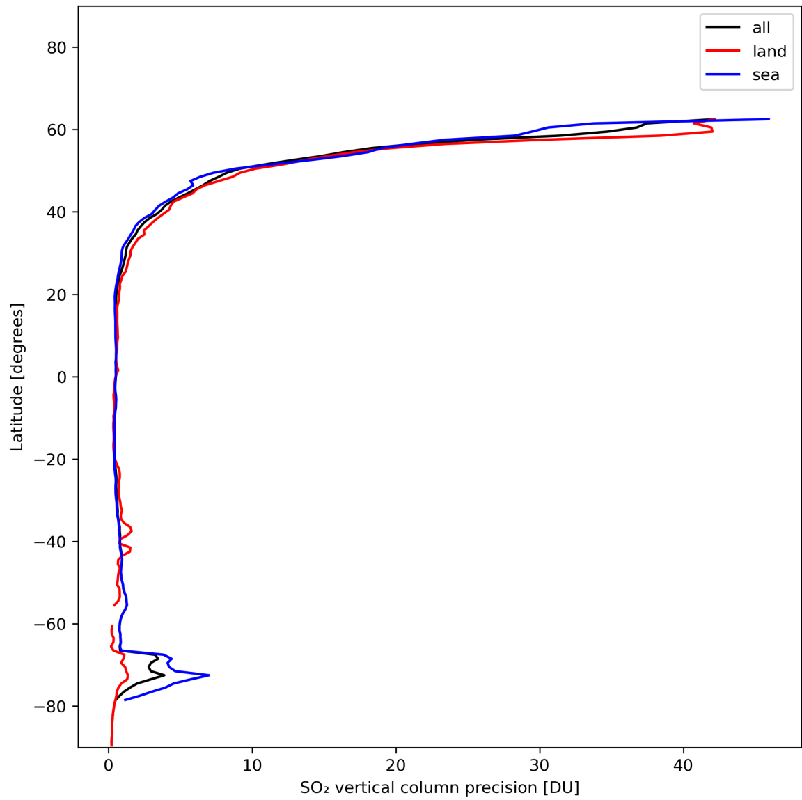
Figure 31: Zonal average of “SO 2 vertical column precision” for 2024-01-06 to 2024-01-08.
