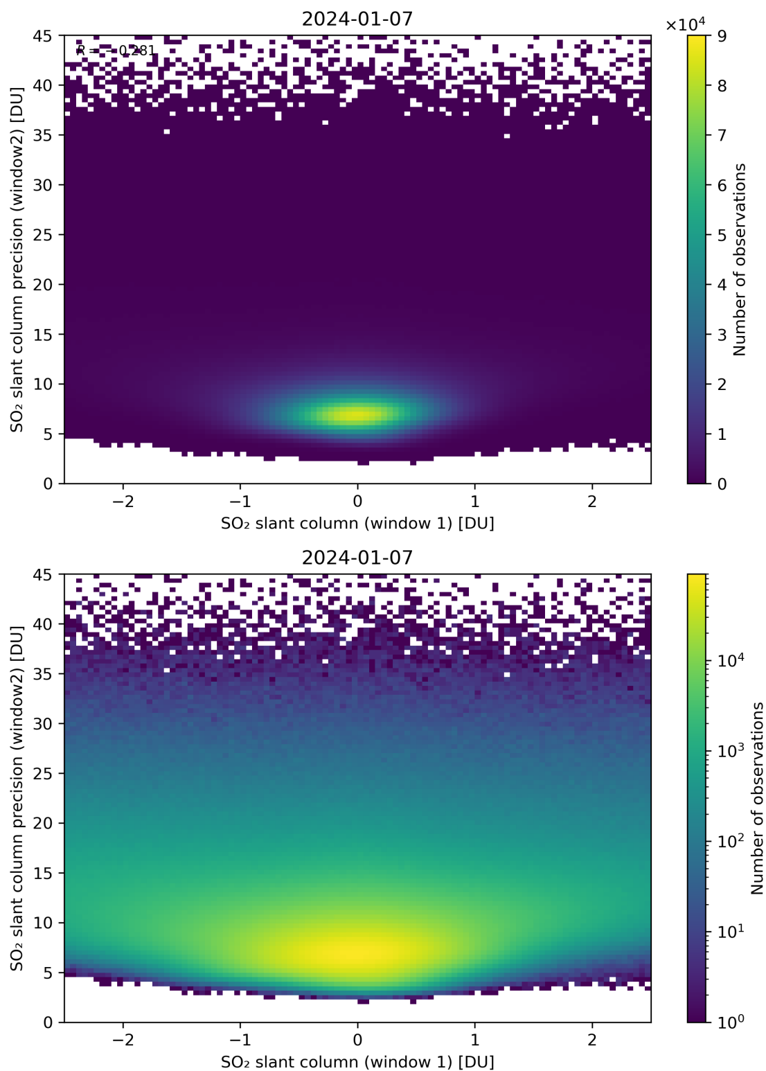
Figure 236: Scatter density plot of “SO 2 slant column (window 1)” against “SO 2 slant column precision (window2)” for 2024-01-06 to 2024-01-08.
