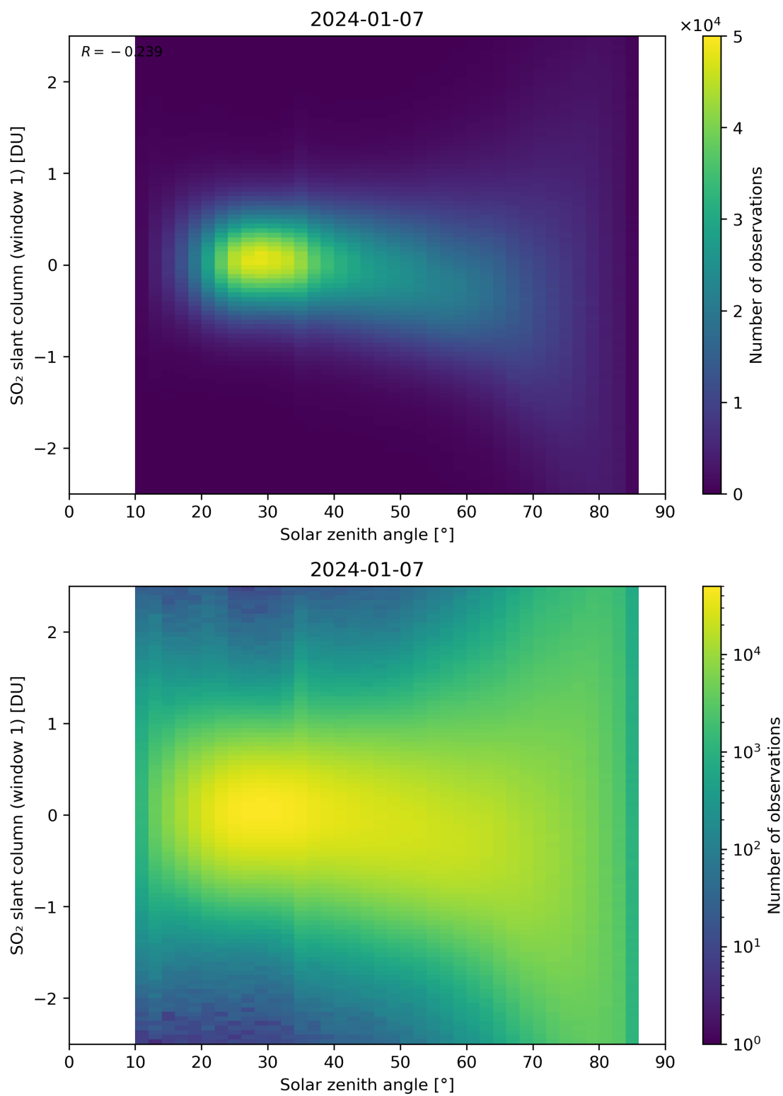
Figure 169: Scatter density plot of “Solar zenith angle” against “SO 2 slant column (window 1)” for 2024-01-06 to 2024-01-08.
