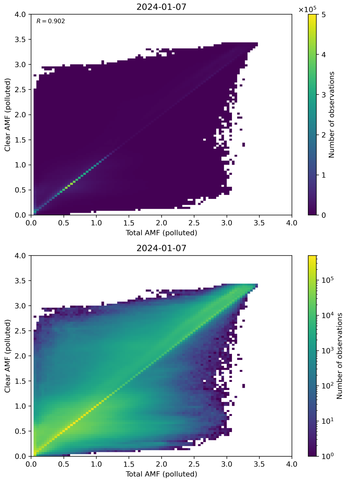
Figure 271: Scatter density plot of “Total AMF (polluted)” against “Clear AMF (polluted)” for 2024-01-06 to 2024-01-08.
