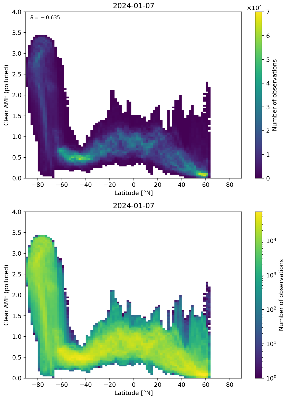
Figure 145: Scatter density plot of “Latitude” against “Clear AMF (polluted)” for 2024-01-06 to 2024-01-08.
