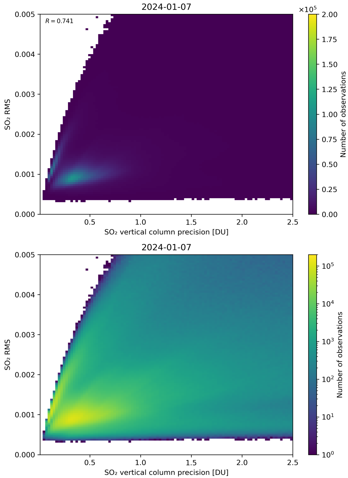
Figure 284: Scatter density plot of “SO 2 vertical column precision” against “SO 2 RMS” for 2024-01-06 to 2024-01-08.
