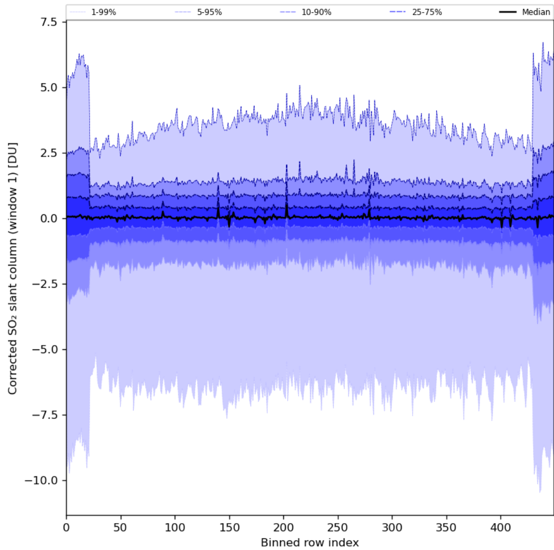
Figure 81: Along track statistics of “Corrected SO 2 slant column (window 1)” for 2024-01-06 to 2024-01-08
