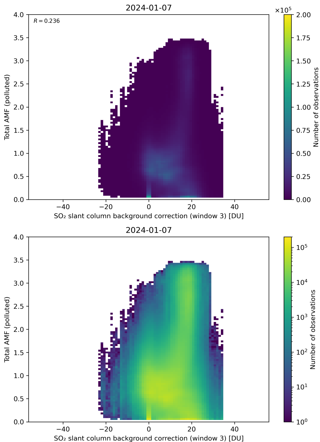
Figure 125: Scatter density plot of “SO 2 slant column background correction (window 3)” against “Total AMF (polluted)” for 2024-01-06 to 2024-01-08.
