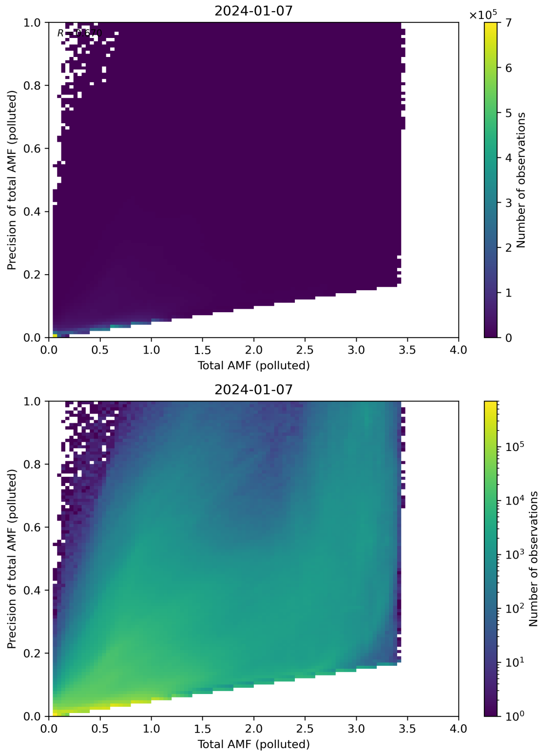
Figure 272: Scatter density plot of “Total AMF (polluted)” against “Precision of total AMF (polluted)” for 2024-01-06 to 2024-01-08.
