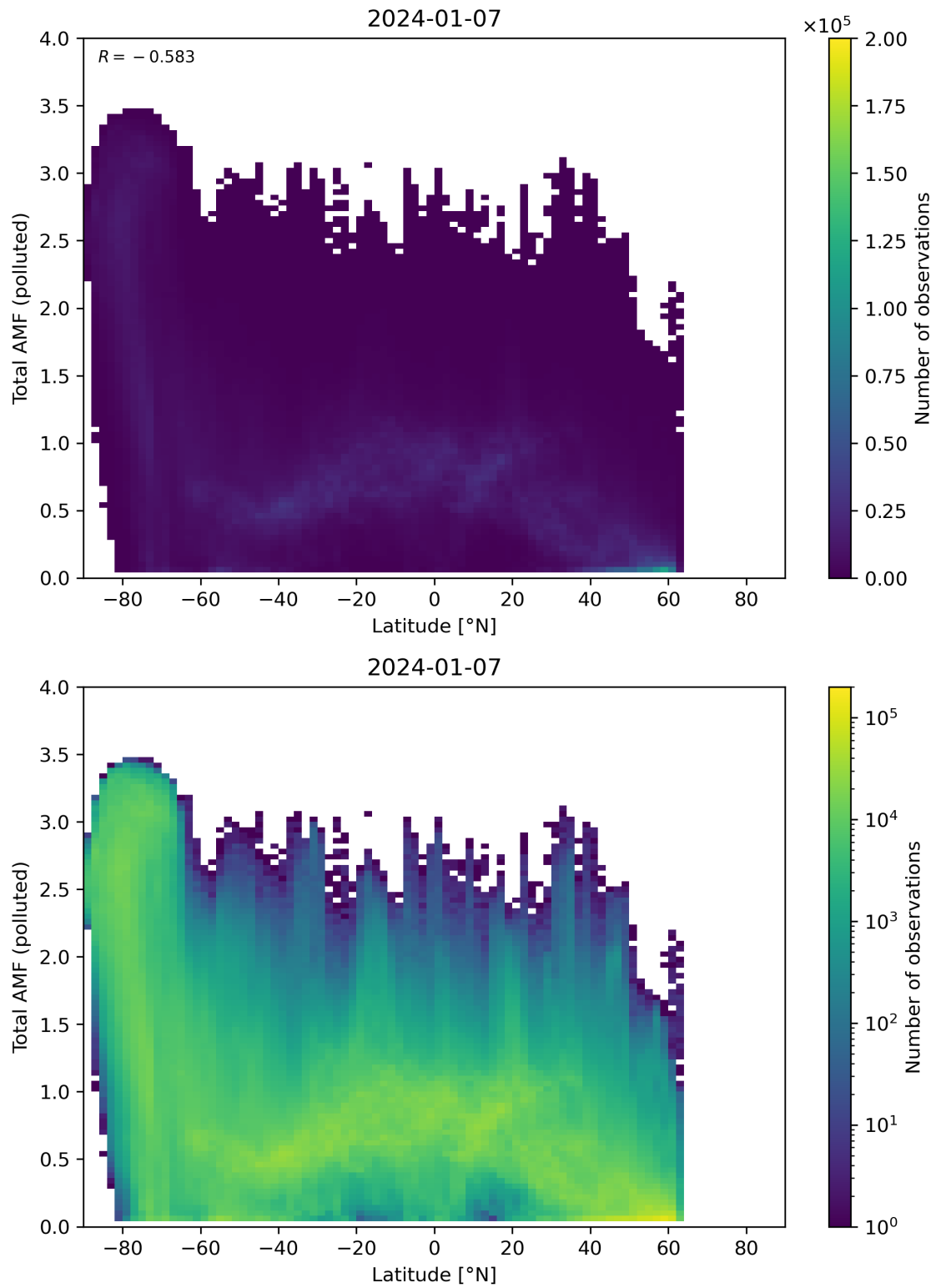
Figure 154: Scatter density plot of “Latitude” against “Total AMF (polluted)” for 2024-01-06 to 2024-01-08.
