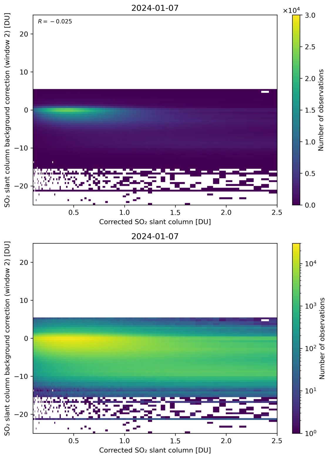
Figure 179: Scatter density plot of “Corrected SO 2 slant column” against “SO 2 slant column background correction (window 2)” for 2024-01-06 to 2024-01-08.
