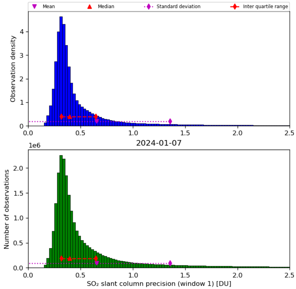
Figure 57: Histogram of “SO 2 slant column precision (window 1)” for 2024-01-06 to 2024-01-08
