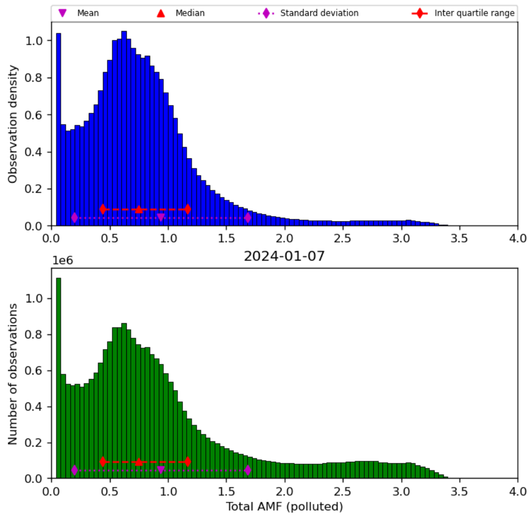
Figure 71: Histogram of “Total AMF (polluted)” for 2024-01-06 to 2024-01-08
