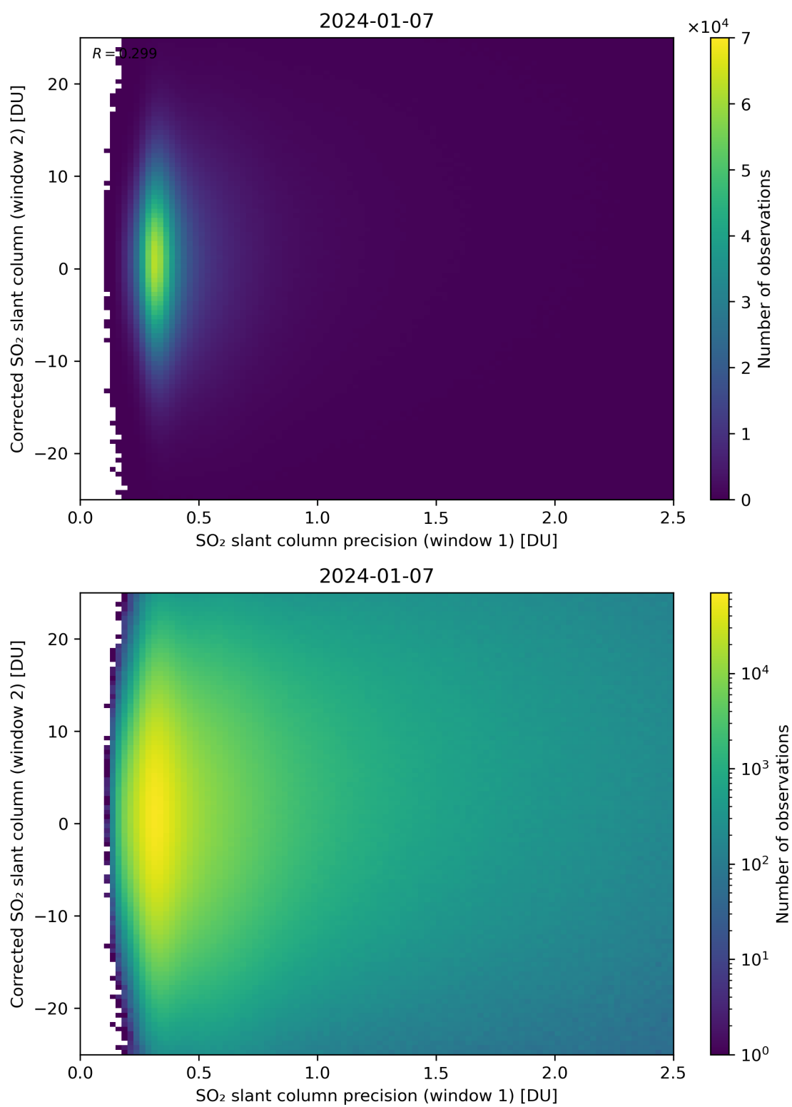
Figure 225: Scatter density plot of “SO 2 slant column precision (window 1)” against “Corrected SO 2 slant column (window 2)” for 2024-01-06 to 2024-01-08.
