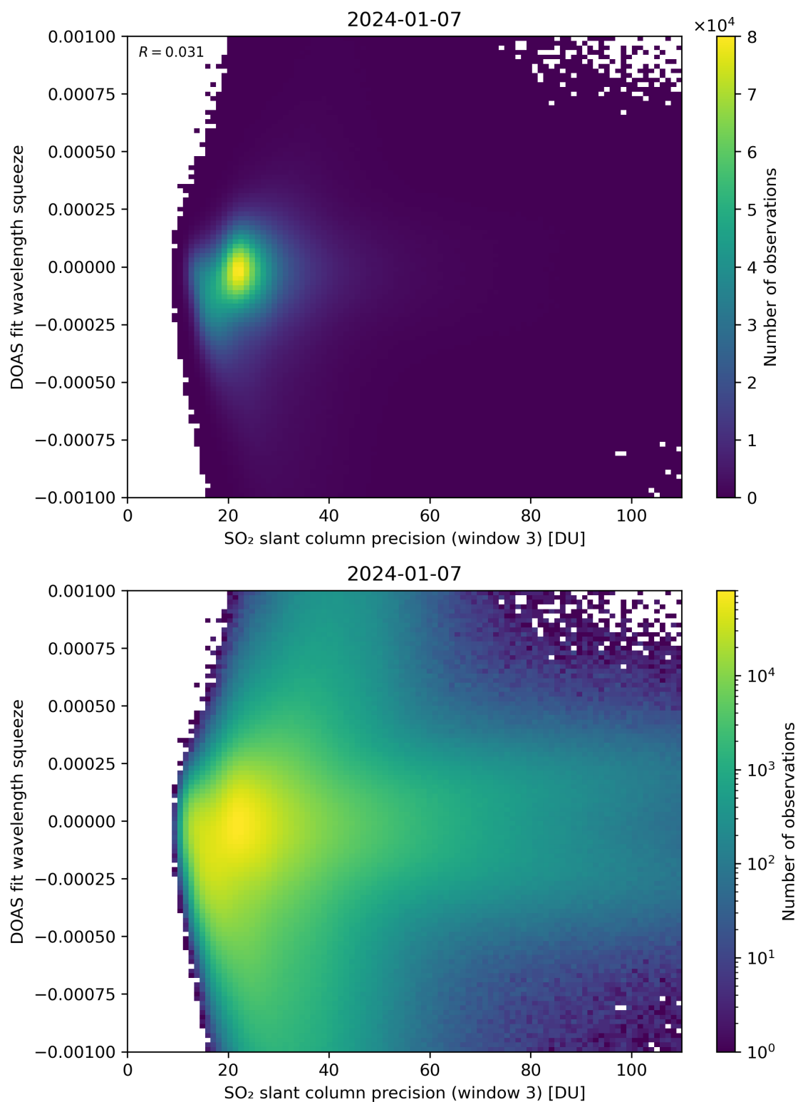
Figure 259: Scatter density plot of “SO 2 slant column precision (window 3)” against “DOAS fit wavelength squeeze” for 2024-01-06 to 2024-01-08.
