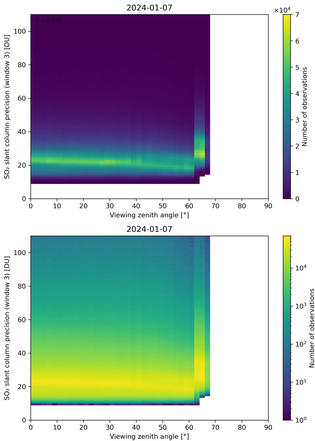
Figure 324: Scatter density plot of “Viewing zenith angle” against “SO 2 slant column precision (window 3)” for 2024-01-06 to 2024-01-08.
