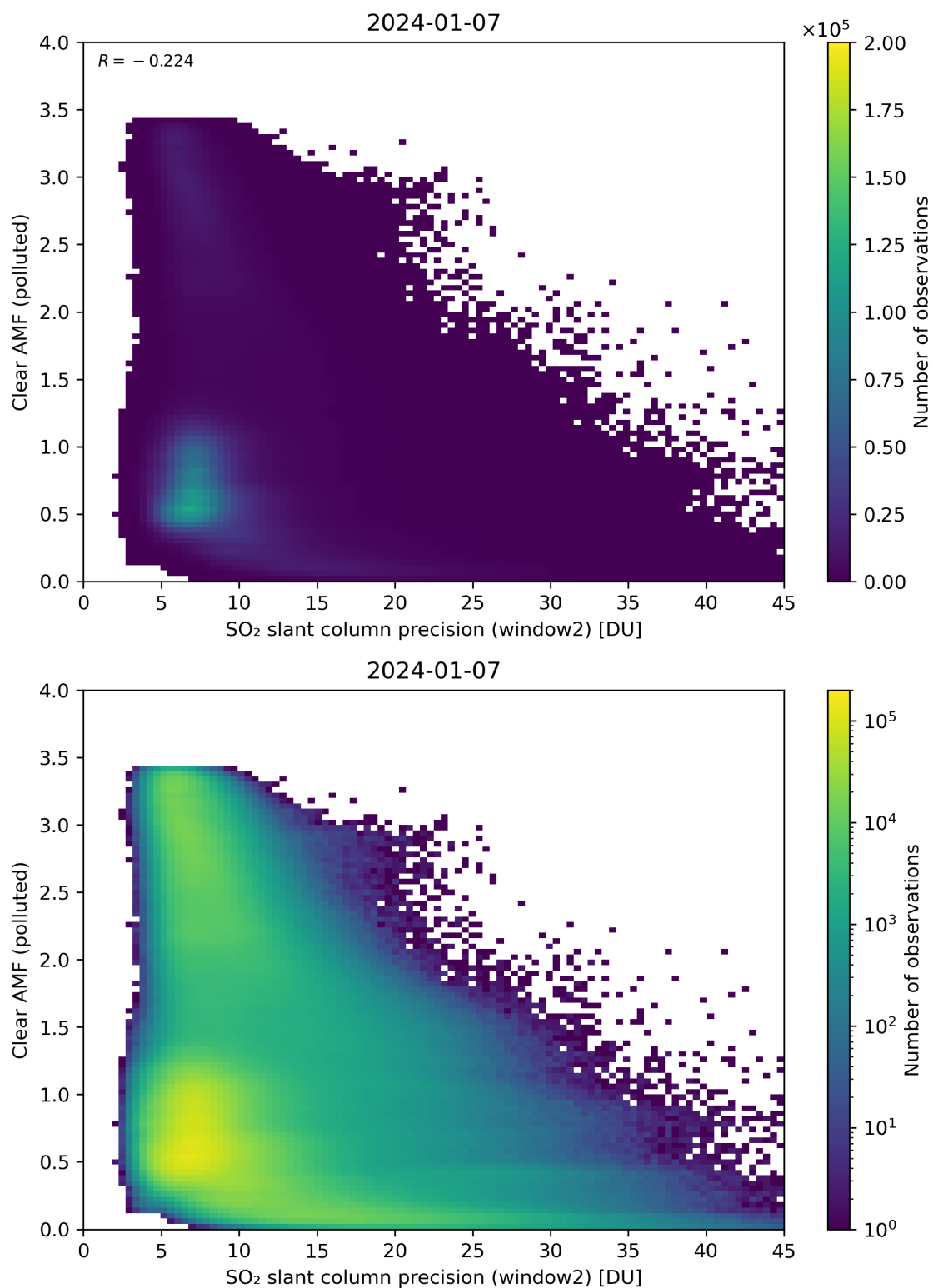
Figure 246: Scatter density plot of “SO 2 slant column precision (window2)” against “Clear AMF (polluted)” for 2024-01-06 to 2024-01-08.
