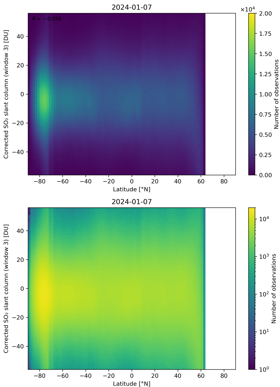
Figure 148: Scatter density plot of “Latitude” against “Corrected SO 2 slant column (window 3)” for 2024-01-06 to 2024-01-08.
