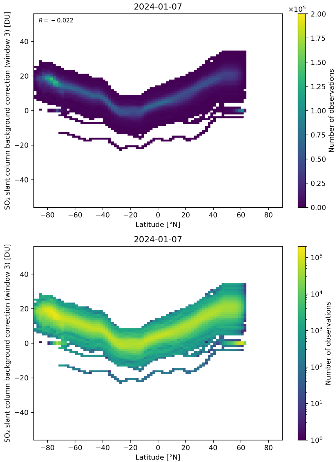
Figure 141: Scatter density plot of “Latitude” against “SO 2 slant column background correction (window 3)” for 2024-01-06 to 2024-01-08.
