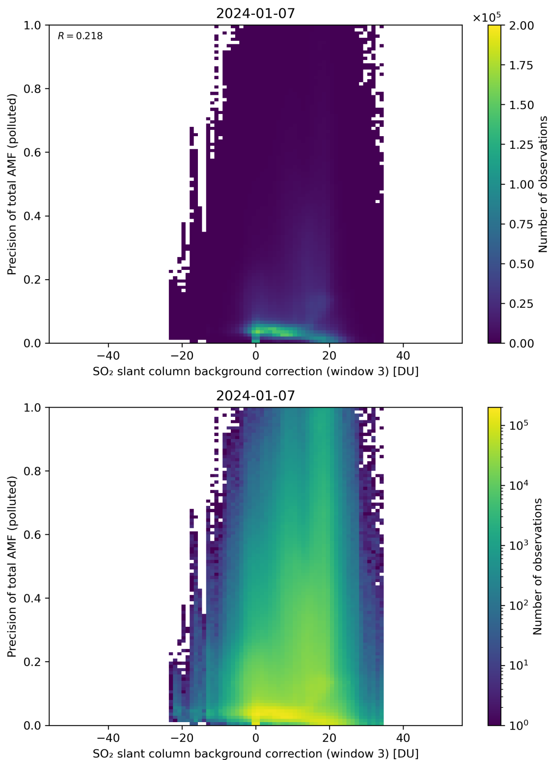
Figure 126: Scatter density plot of “SO 2 slant column background correction (window 3)” against “Precision of total AMF (polluted)” for 2024-01-06 to 2024-01-08.
