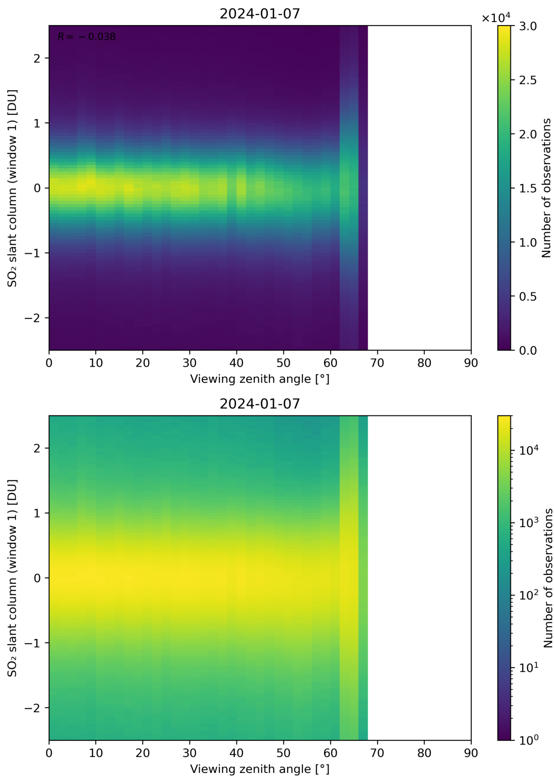
Figure 320: Scatter density plot of “Viewing zenith angle” against “SO 2 slant column (window 1)” for 2024-01-06 to 2024-01-08.
