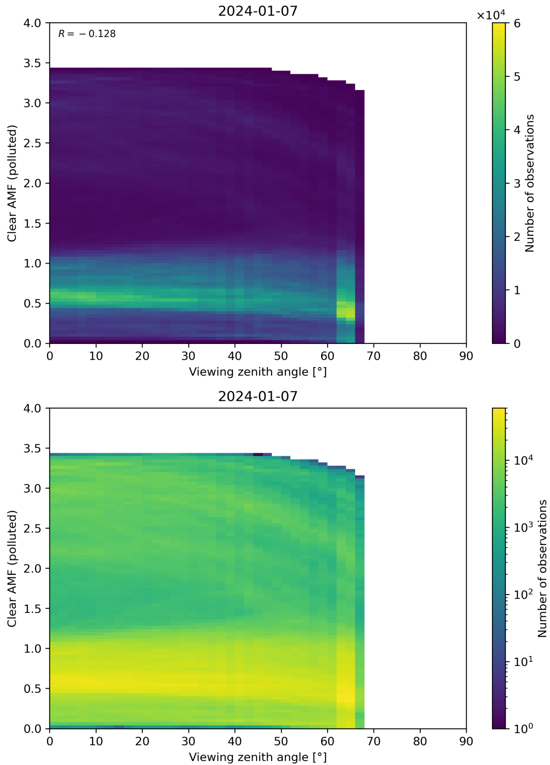
Figure 316: Scatter density plot of “Viewing zenith angle” against “Clear AMF (polluted)” for 2024-01-06 to 2024-01-08.
