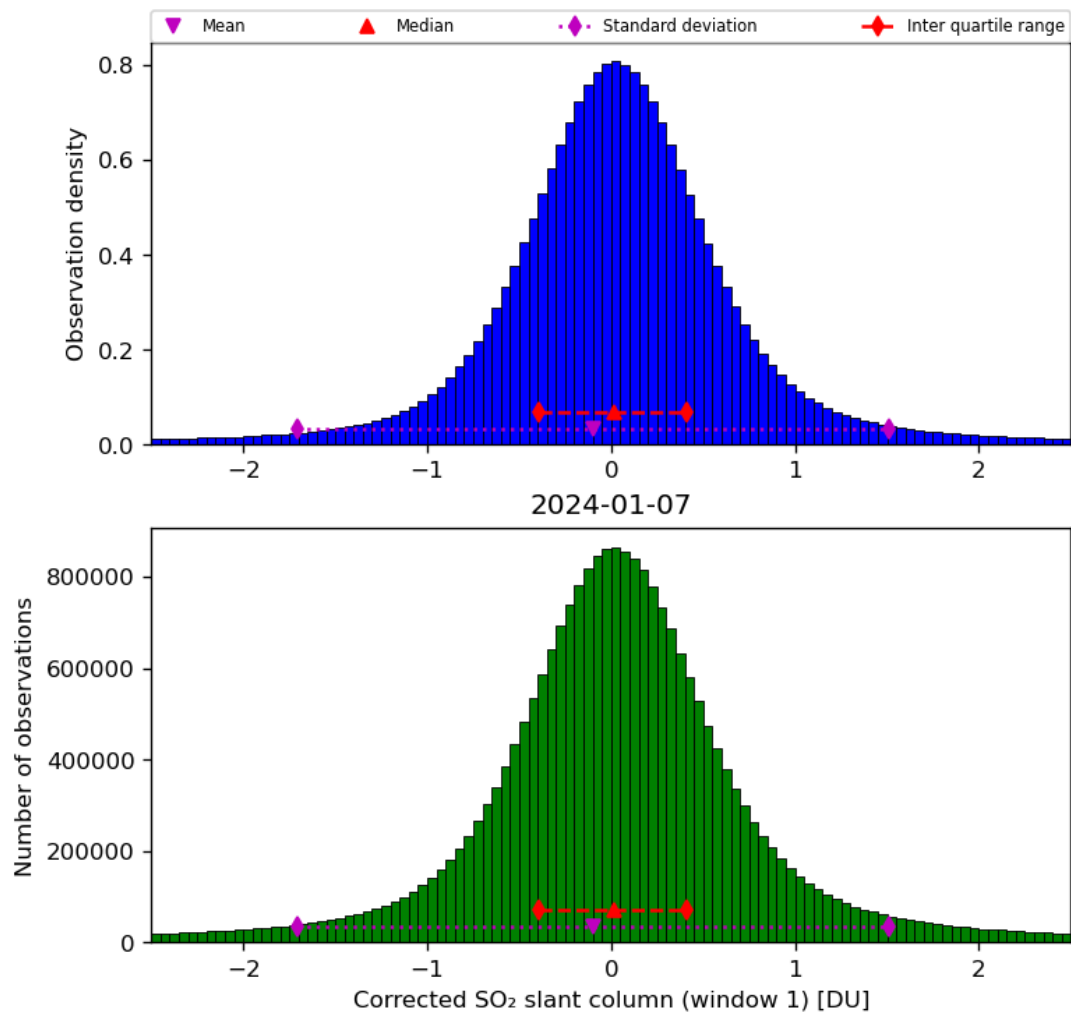
Figure 58: Histogram of “Corrected SO 2 slant column (window 1)” for 2024-01-06 to 2024-01-08
