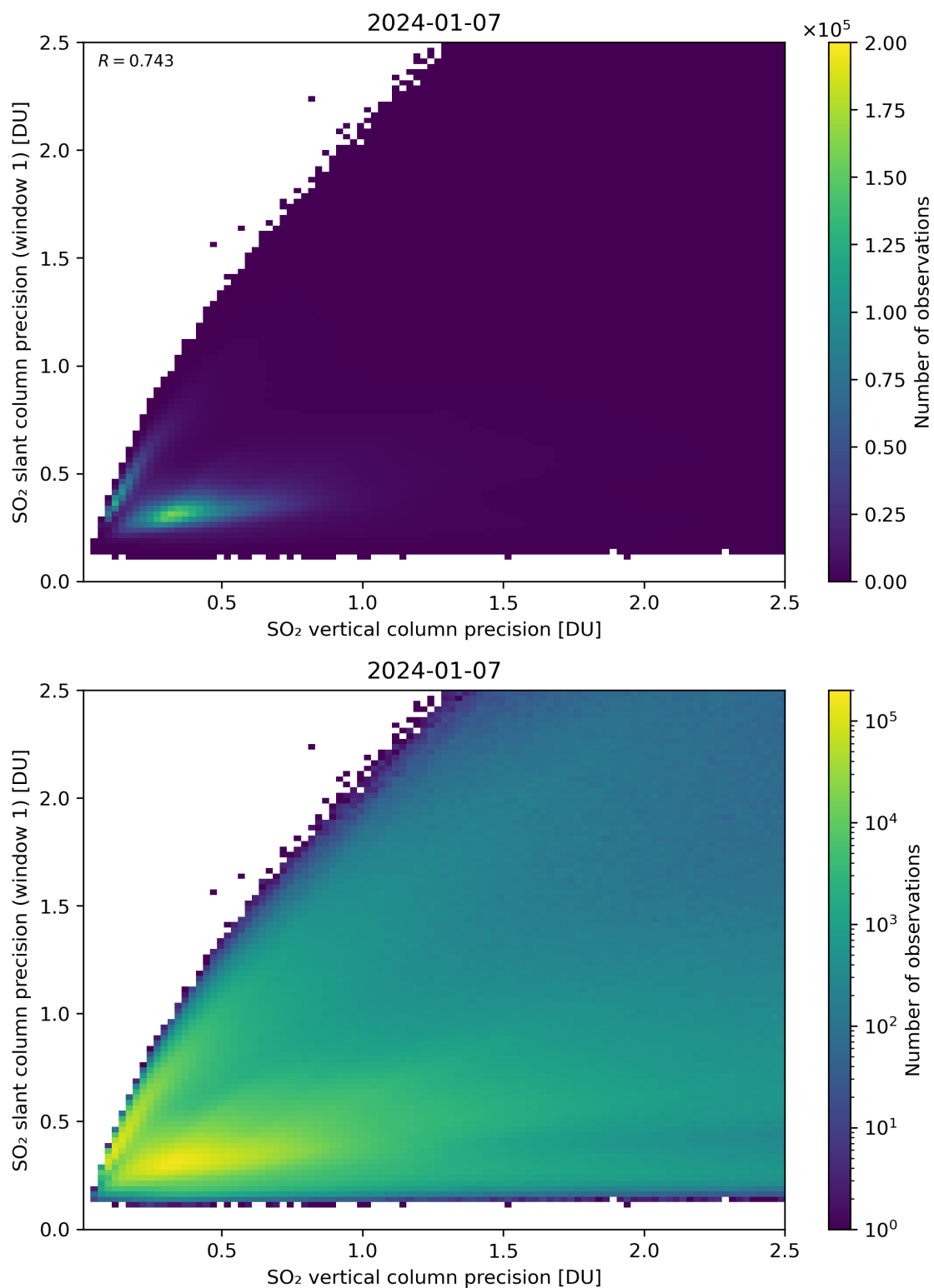
Figure 290: Scatter density plot of “SO 2 vertical column precision” against “SO 2 slant column precision (window 1)” for 2024-01-06 to 2024-01-08.
