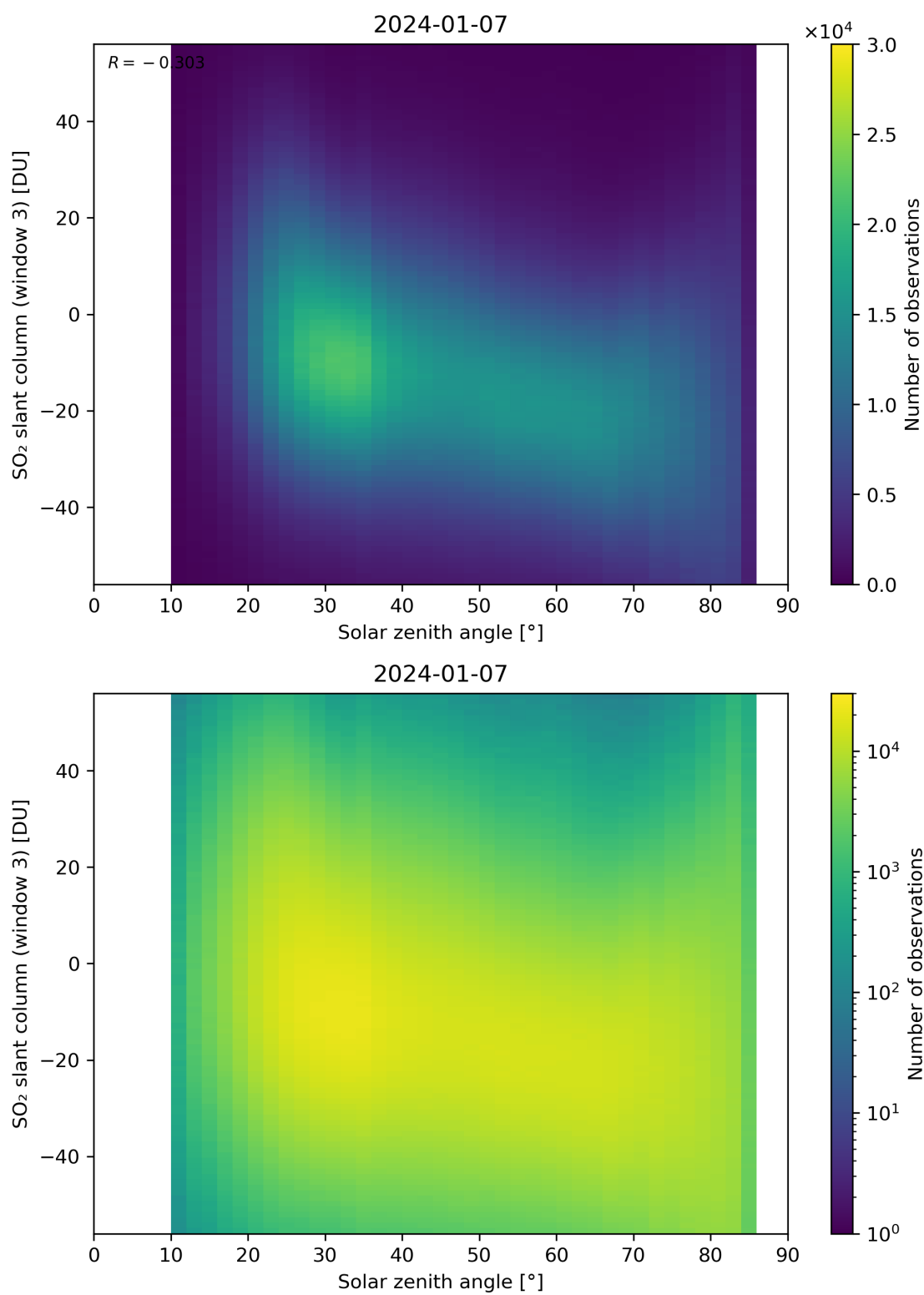
Figure 172: Scatter density plot of “Solar zenith angle” against “SO 2 slant column (window 3)” for 2024-01-06 to 2024-01-08.
