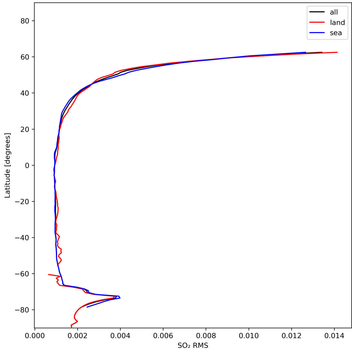
Figure 47: Zonal average of “SO 2 RMS” for 2024-01-06 to 2024-01-08.
