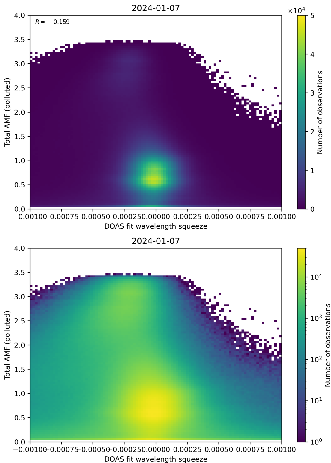
Figure 134: Scatter density plot of “DOAS fit wavelength squeeze” against “Total AMF (polluted)” for 2024-01-06 to 2024-01-08.
