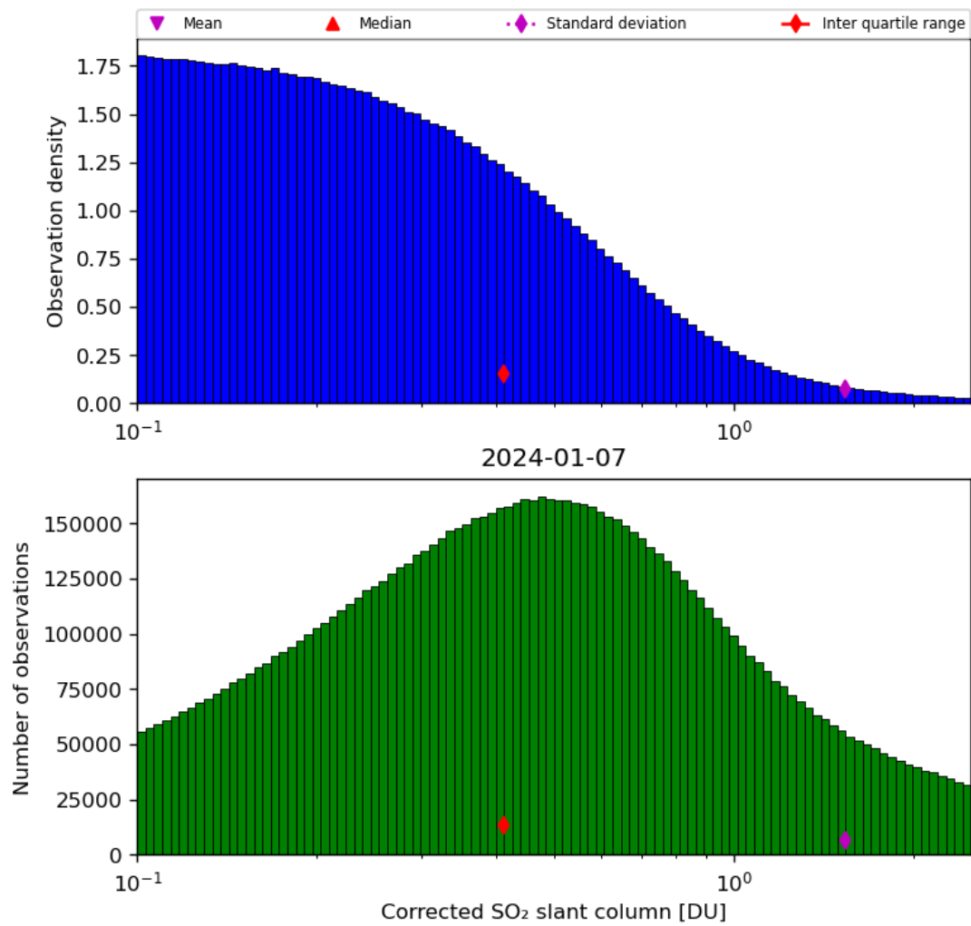
Figure 55: Histogram of “Corrected SO 2 slant column” for 2024-01-06 to 2024-01-08
