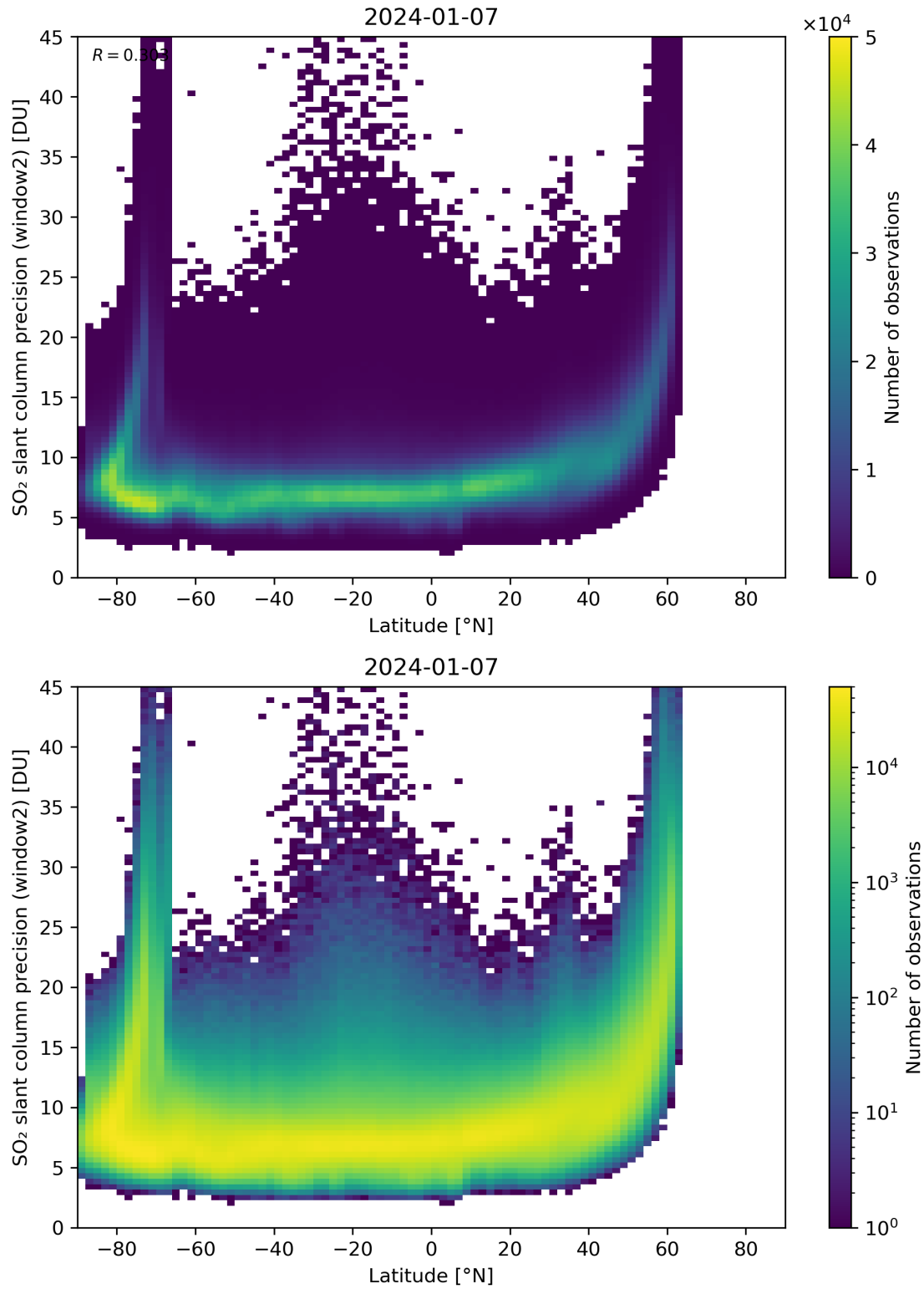
Figure 151: Scatter density plot of “Latitude” against “SO 2 slant column precision (window2)” for 2024-01-06 to 2024-01-08.
