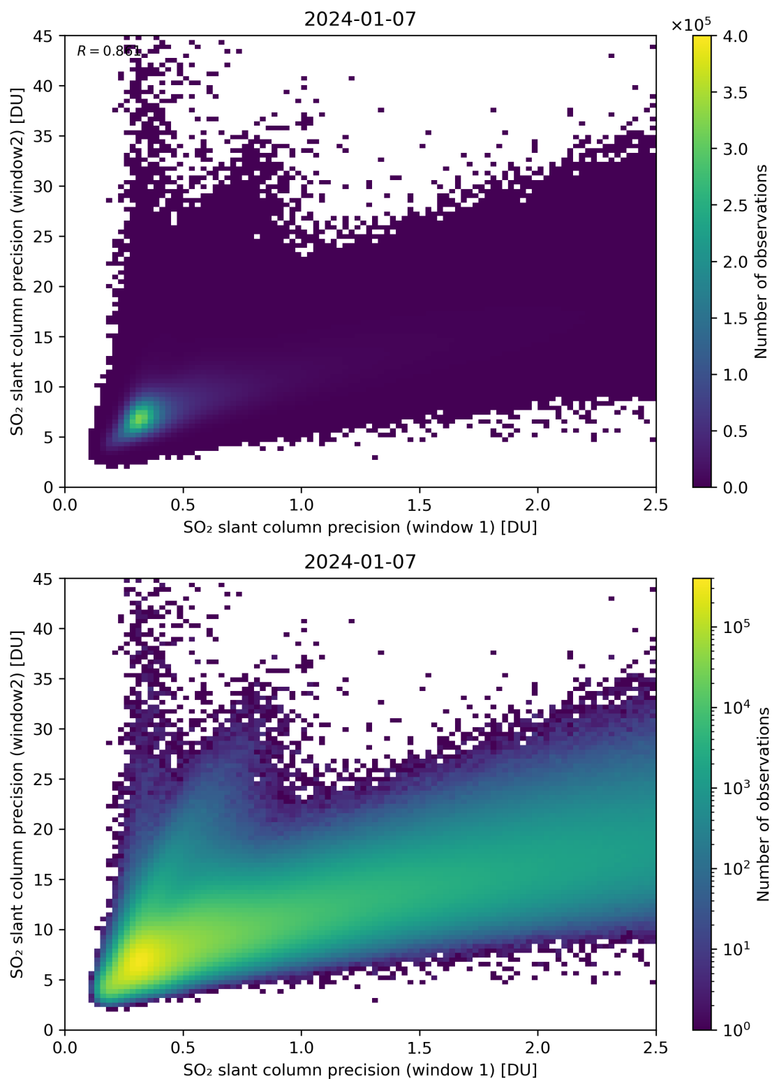
Figure 227: Scatter density plot of “SO 2 slant column precision (window 1)” against “SO 2 slant column precision (window2)” for 2024-01-06 to 2024-01-08.
