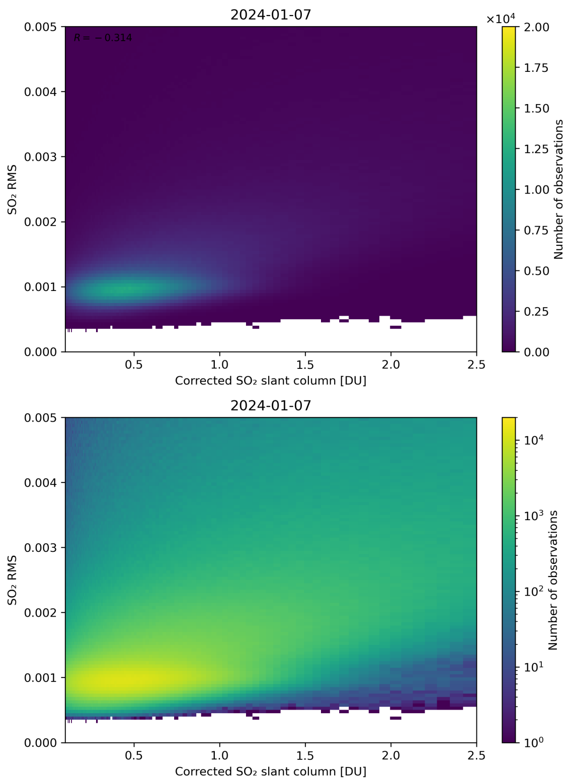
Figure 183: Scatter density plot of “Corrected SO 2 slant column” against “SO 2 RMS” for 2024-01-06 to 2024-01-08.
