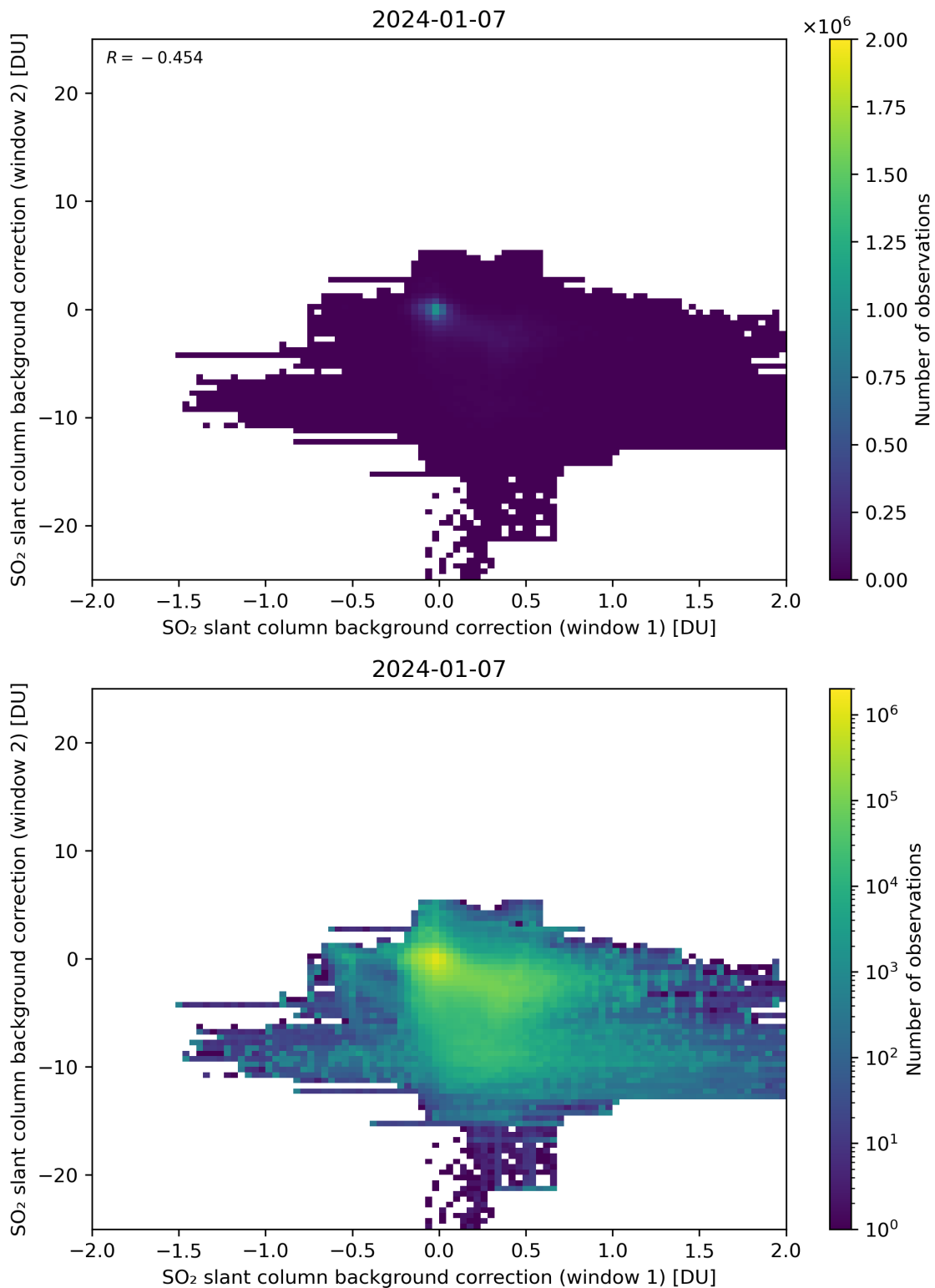
Figure 98: Scatter density plot of “SO 2 slant column background correction (window 1)” against “SO 2 slant column background correction (window 2)” for 2024-01-06 to 2024-01-08.
