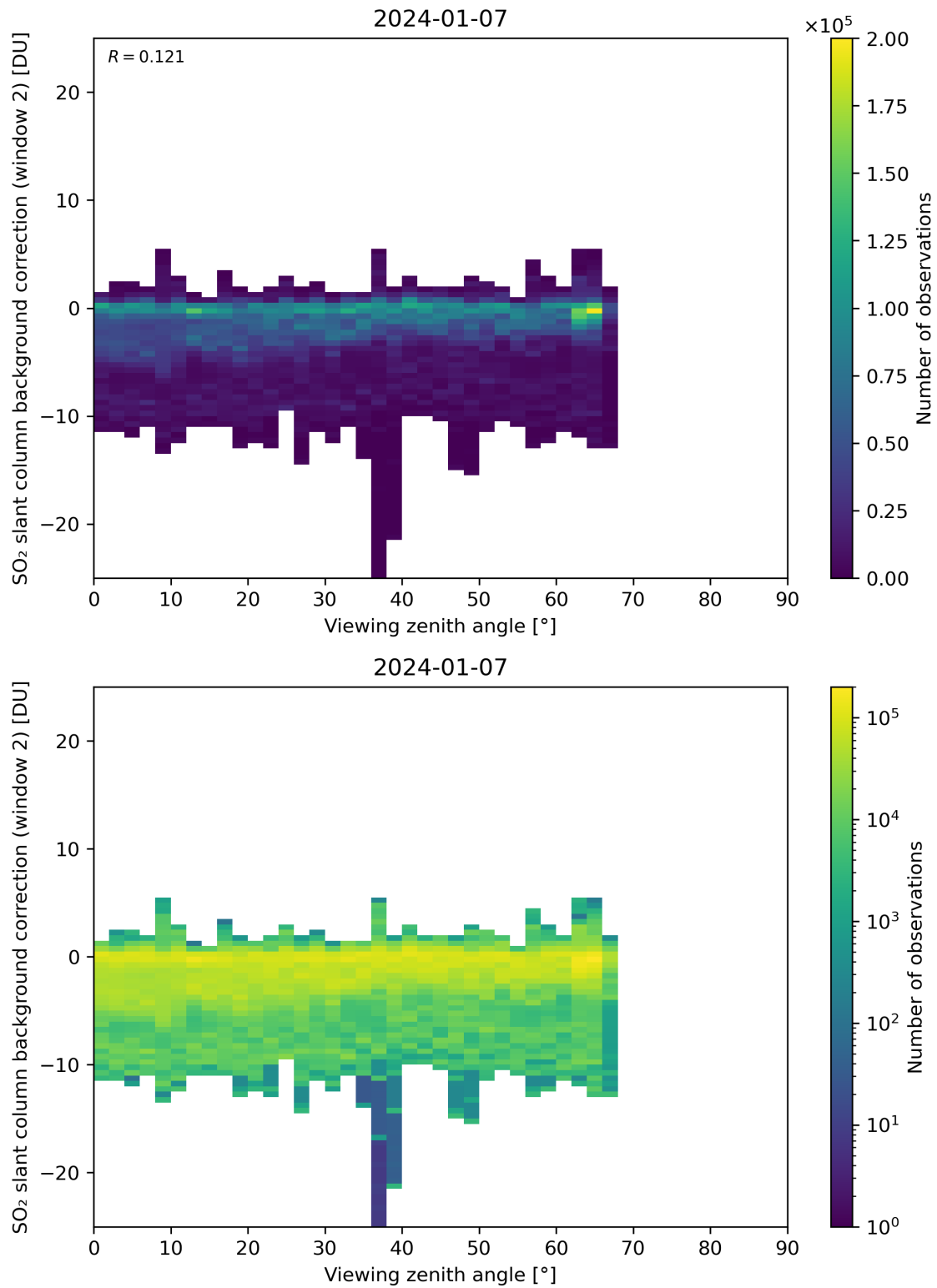
Figure 309: Scatter density plot of “Viewing zenith angle” against “SO 2 slant column background correction (window 2)” for 2024-01-06 to 2024-01-08.
