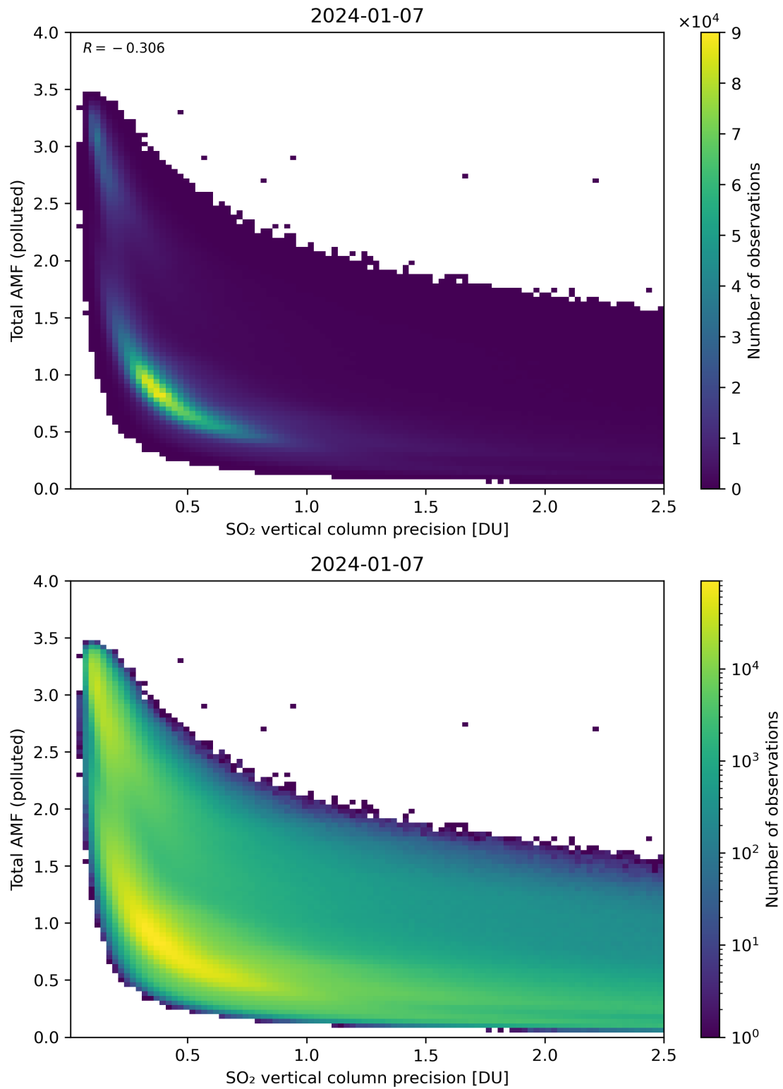
Figure 294: Scatter density plot of “SO 2 vertical column precision” against “Total AMF (polluted)” for 2024-01-06 to 2024-01-08.
