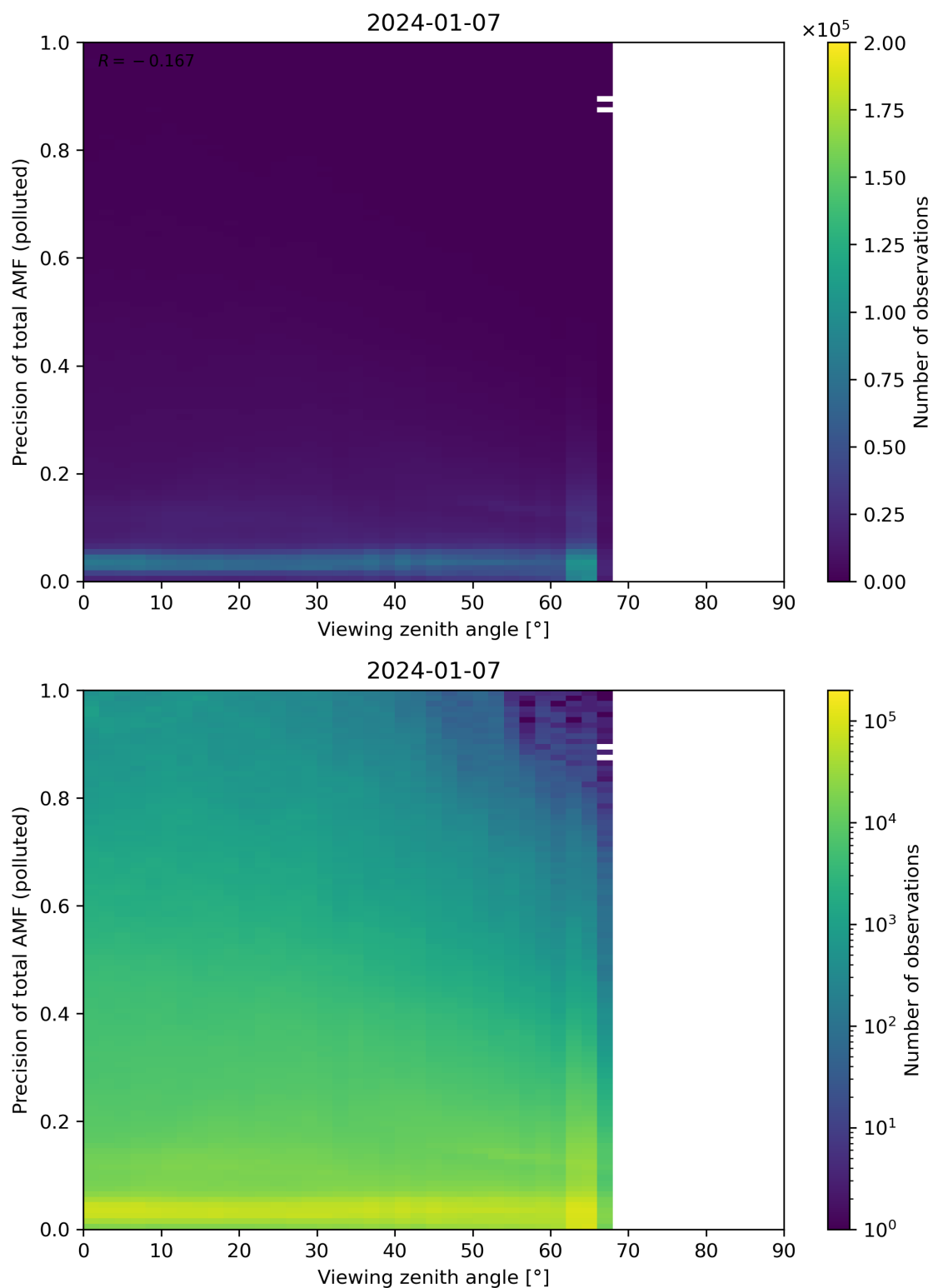
Figure 326: Scatter density plot of “Viewing zenith angle” against “Precision of total AMF (polluted)” for 2024-01-06 to 2024-01-08.
