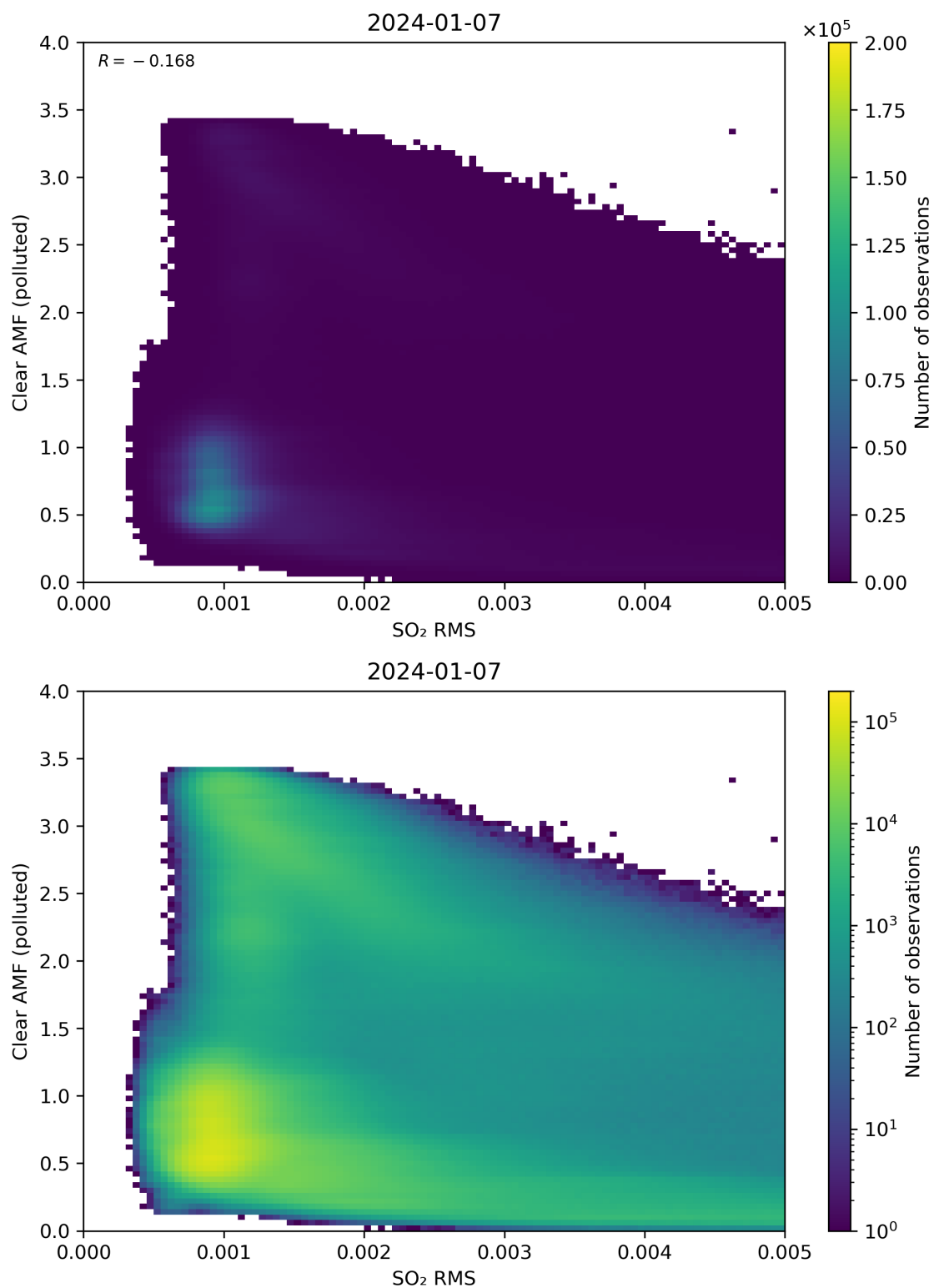
Figure 136: Scatter density plot of “SO 2 RMS” against “Clear AMF (polluted)” for 2024-01-06 to 2024-01-08.
