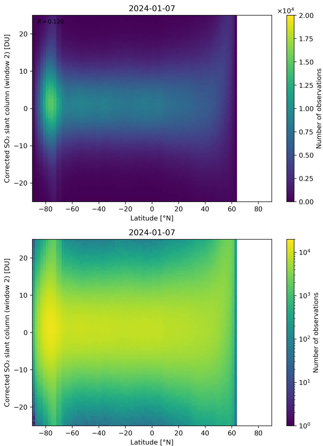
Figure 147: Scatter density plot of “Latitude” against “Corrected SO 2 slant column (window 2)” for 2024-01-06 to 2024-01-08.
