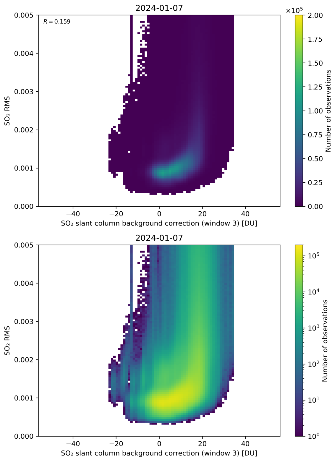
Figure 123: Scatter density plot of “SO 2 slant column background correction (window 3)” against “SO 2 RMS” for 2024-01-06 to 2024-01-08.
