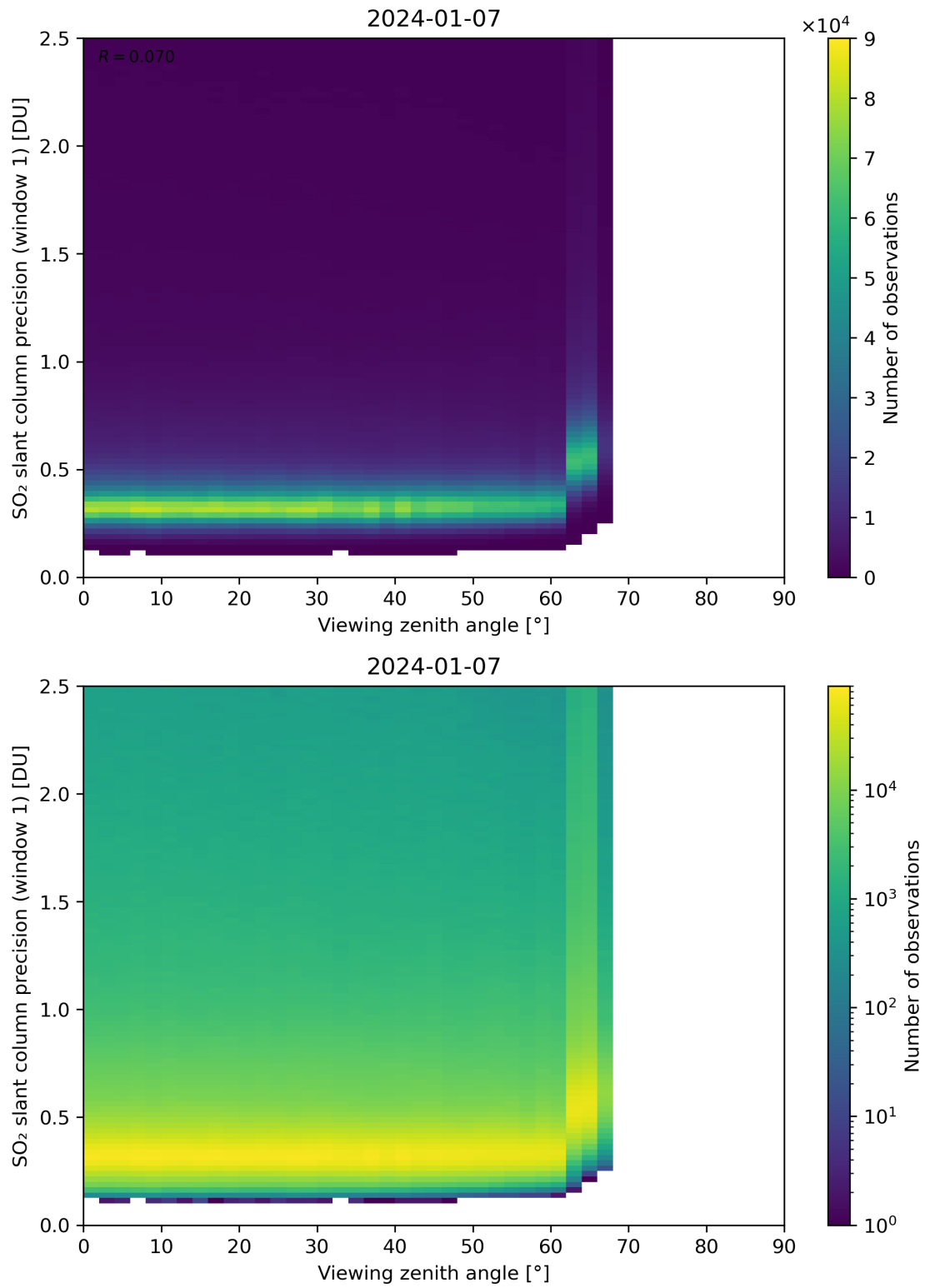
Figure 321: Scatter density plot of “Viewing zenith angle” against “SO 2 slant column precision (window 1)” for 2024-01-06 to 2024-01-08.
