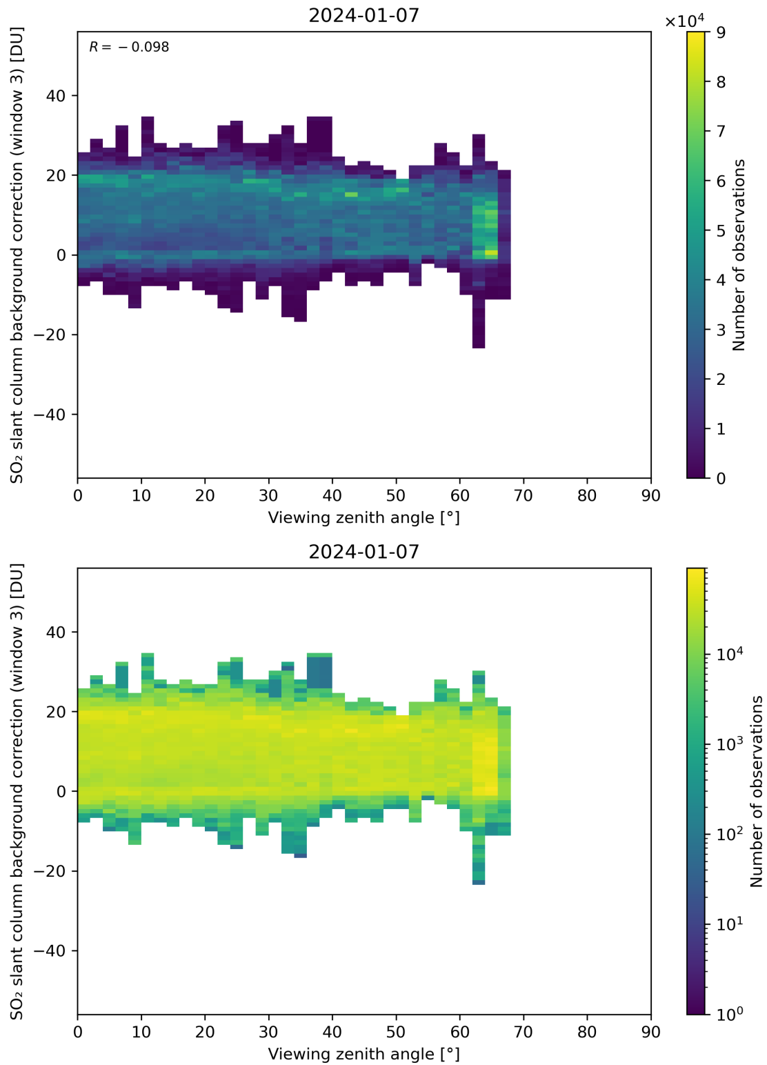
Figure 310: Scatter density plot of “Viewing zenith angle” against “SO 2 slant column background correction (window 3)” for 2024-01-06 to 2024-01-08.
