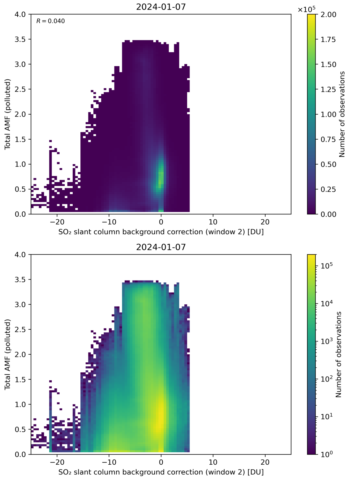
Figure 119: Scatter density plot of “SO 2 slant column background correction (window 2)” against “Total AMF (polluted)” for 2024-01-06 to 2024-01-08.
