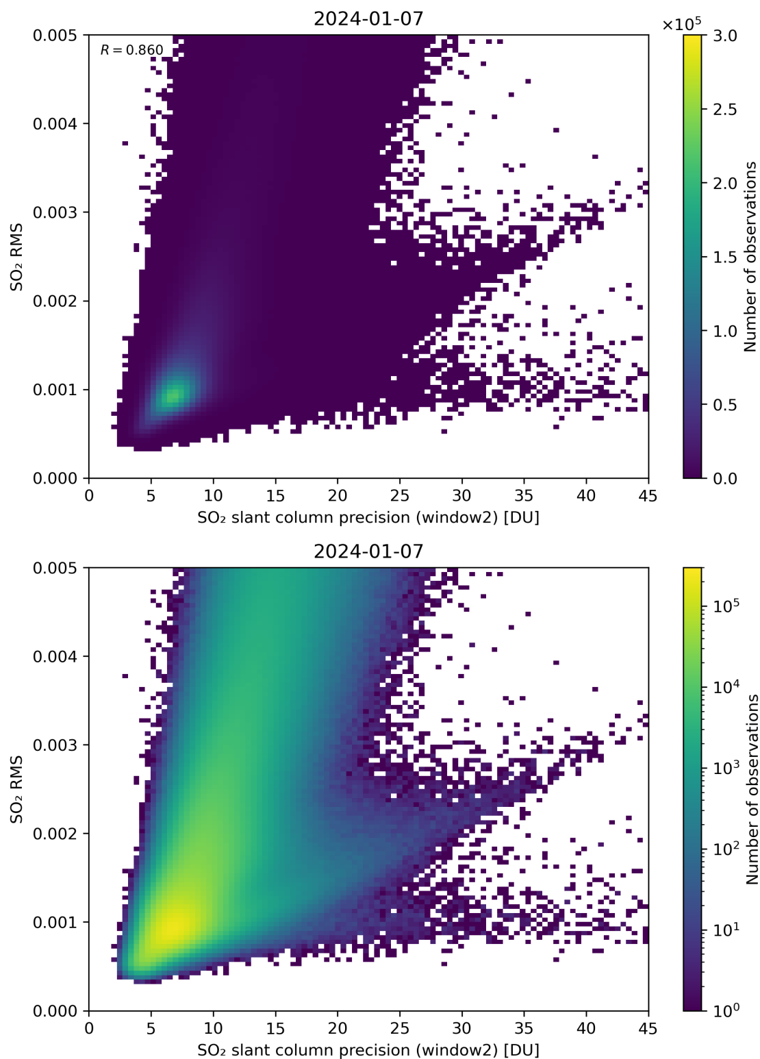
Figure 245: Scatter density plot of “SO 2 slant column precision (window2)” against “SO 2 RMS” for 2024-01-06 to 2024-01-08.
