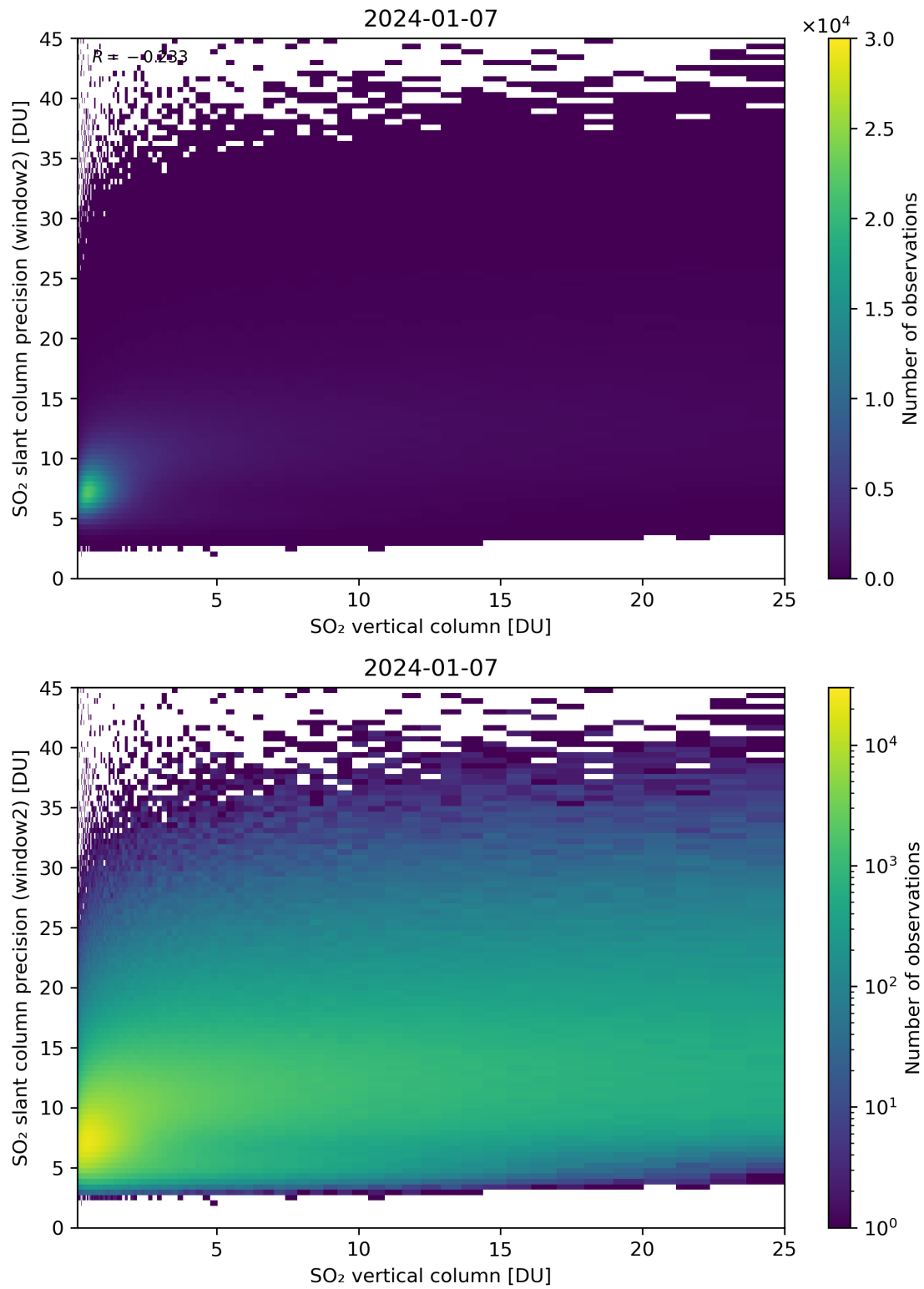
Figure 302: Scatter density plot of “SO 2 vertical column” against “SO 2 slant column precision (window2)” for 2024-01-06 to 2024-01-08.
