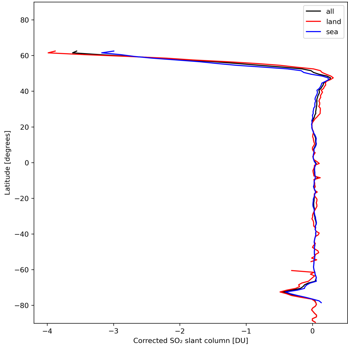
Figure 32: Zonal average of “Corrected SO 2 slant column” for 2024-01-06 to 2024-01-08.
