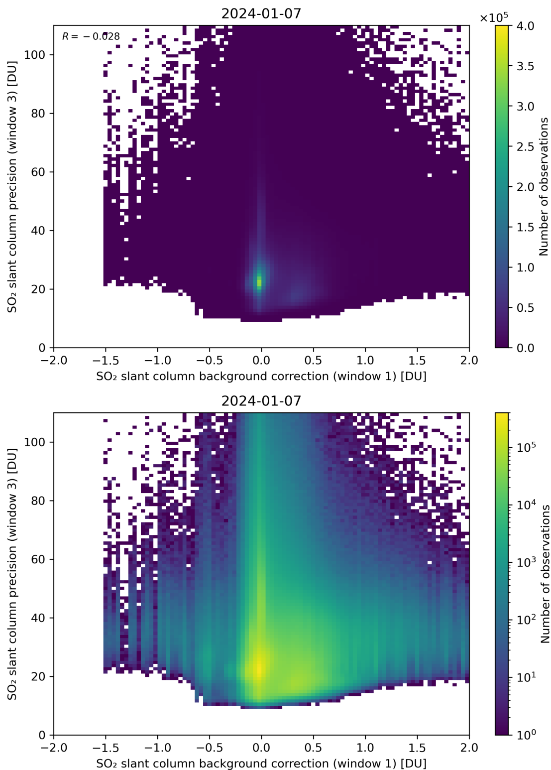
Figure 108: Scatter density plot of “SO 2 slant column background correction (window 1)” against “SO 2 slant column precision (window 3)” for 2024-01-06 to 2024-01-08.
