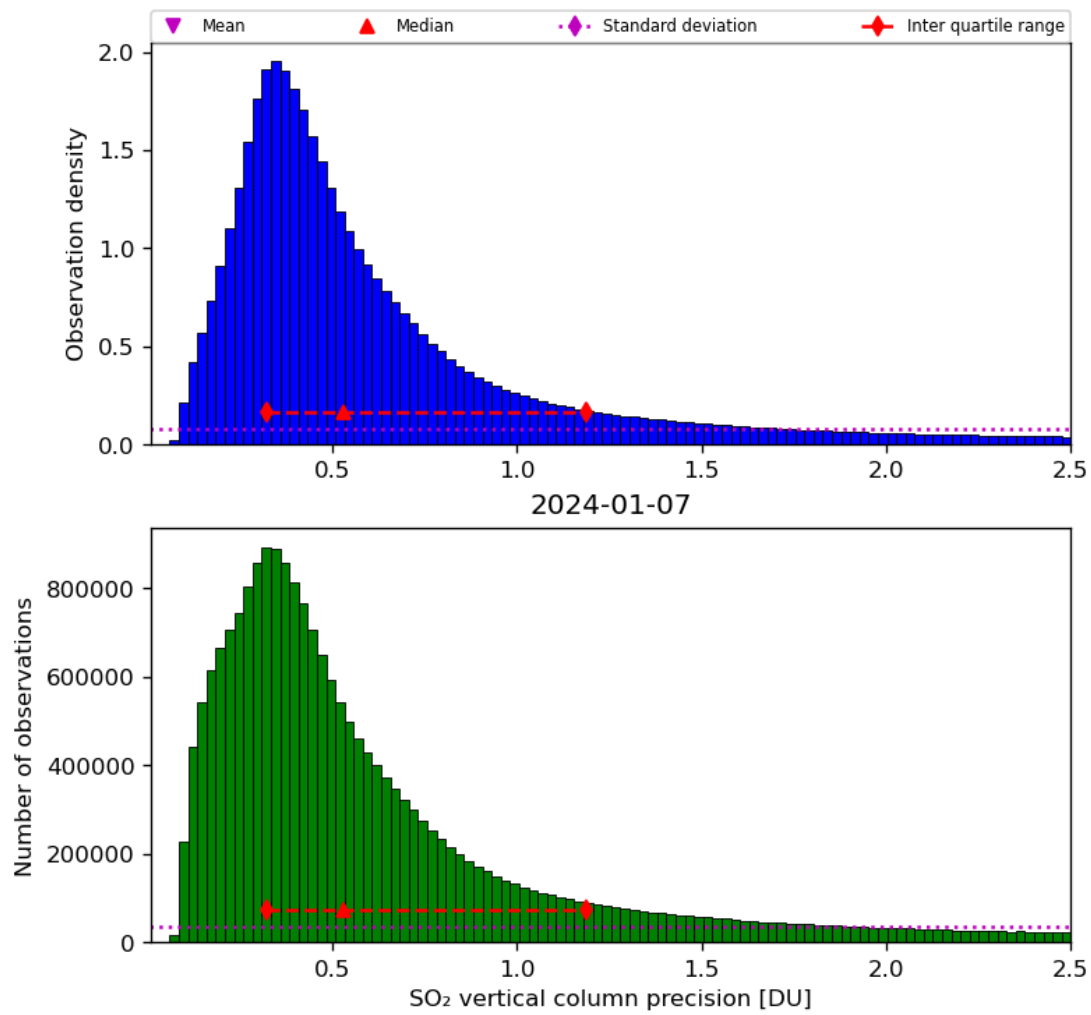
Figure 54: Histogram of “SO 2 vertical column precision” for 2024-01-06 to 2024-01-08
