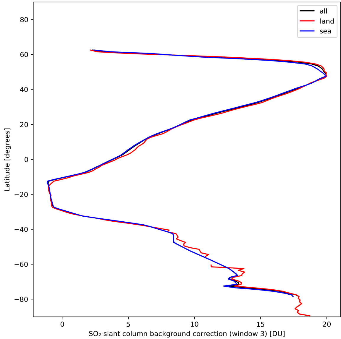
Figure 44: Zonal average of “SO 2 slant column background correction (window 3)” for 2024-01-06 to 2024-01-08.
