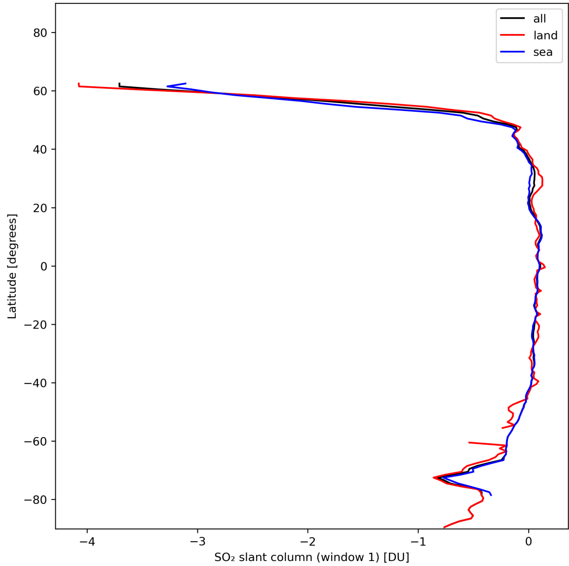
Figure 33: Zonal average of “SO 2 slant column (window 1)” for 2024-01-06 to 2024-01-08.
