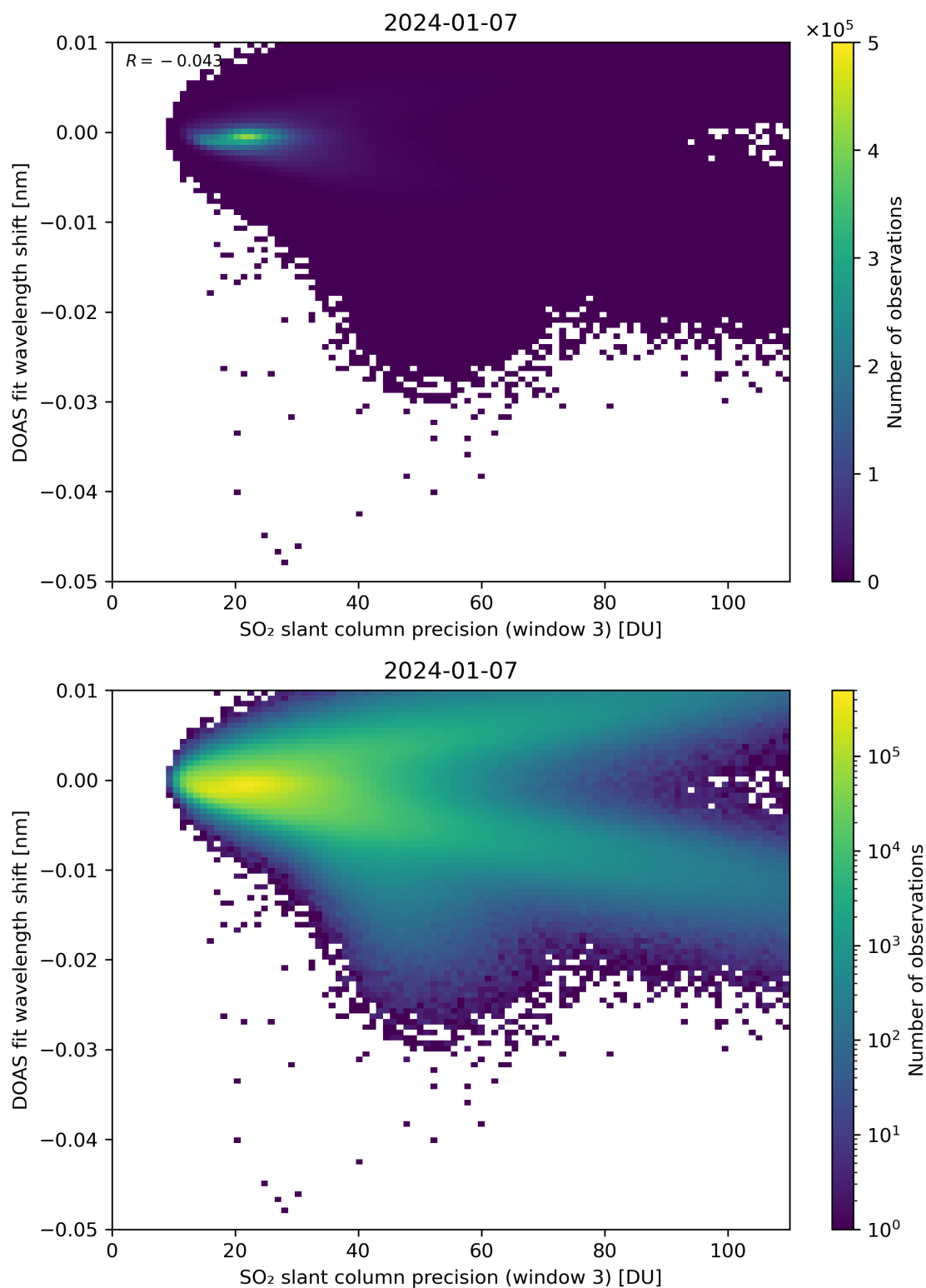
Figure 258: Scatter density plot of “SO 2 slant column precision (window 3)” against “DOAS fit wavelength shift” for 2024-01-06 to 2024-01-08.
