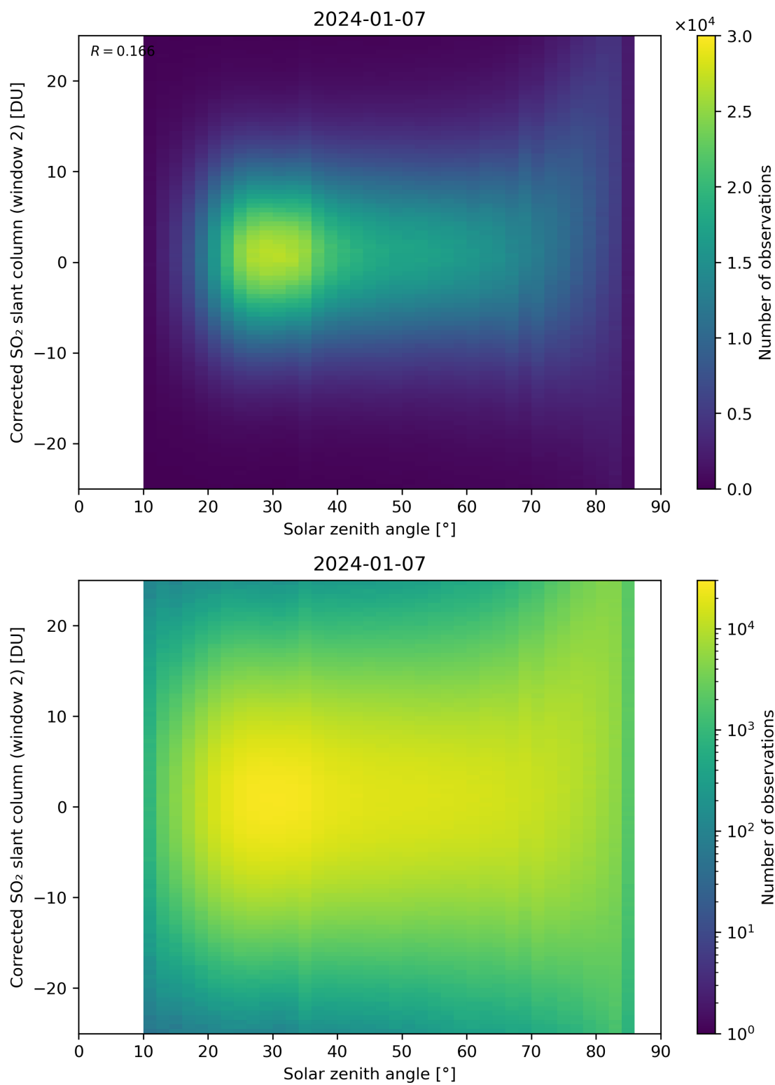
Figure 167: Scatter density plot of “Solar zenith angle” against “Corrected SO 2 slant column (window 2)” for 2024-01-06 to 2024-01-08.
