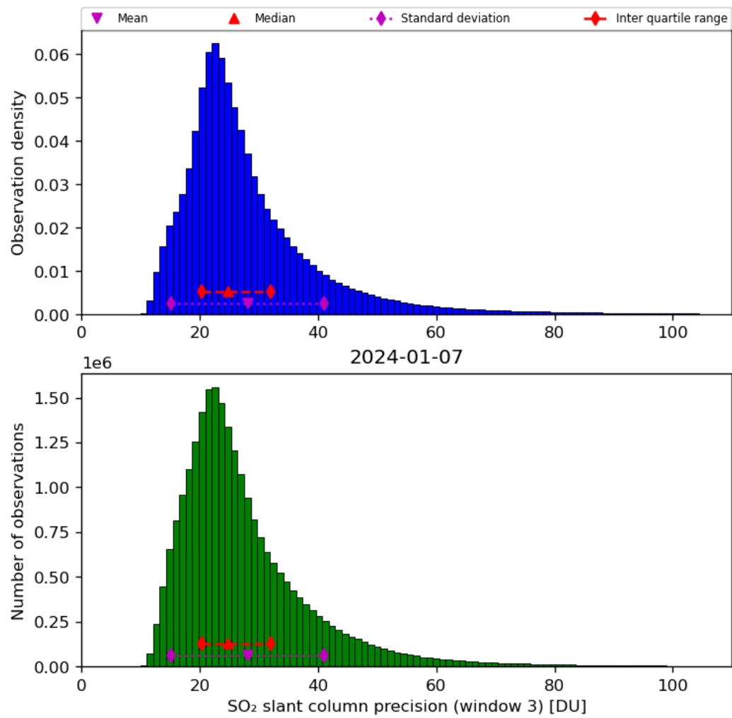
Figure 65: Histogram of “SO 2 slant column precision (window 3)” for 2024-01-06 to 2024-01-08
