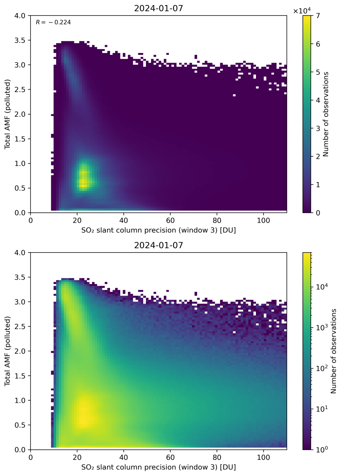
Figure 263: Scatter density plot of “SO 2 slant column precision (window 3)” against “Total AMF (polluted)” for 2024-01-06 to 2024-01-08.
