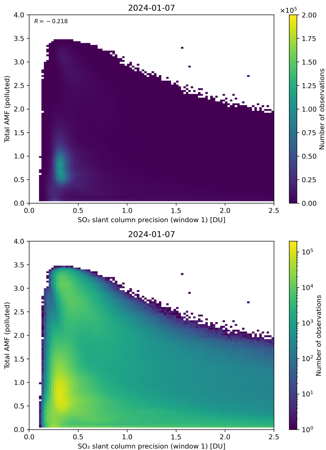
Figure 230: Scatter density plot of “SO 2 slant column precision (window 1)” against “Total AMF (polluted)” for 2024-01-06 to 2024-01-08.
