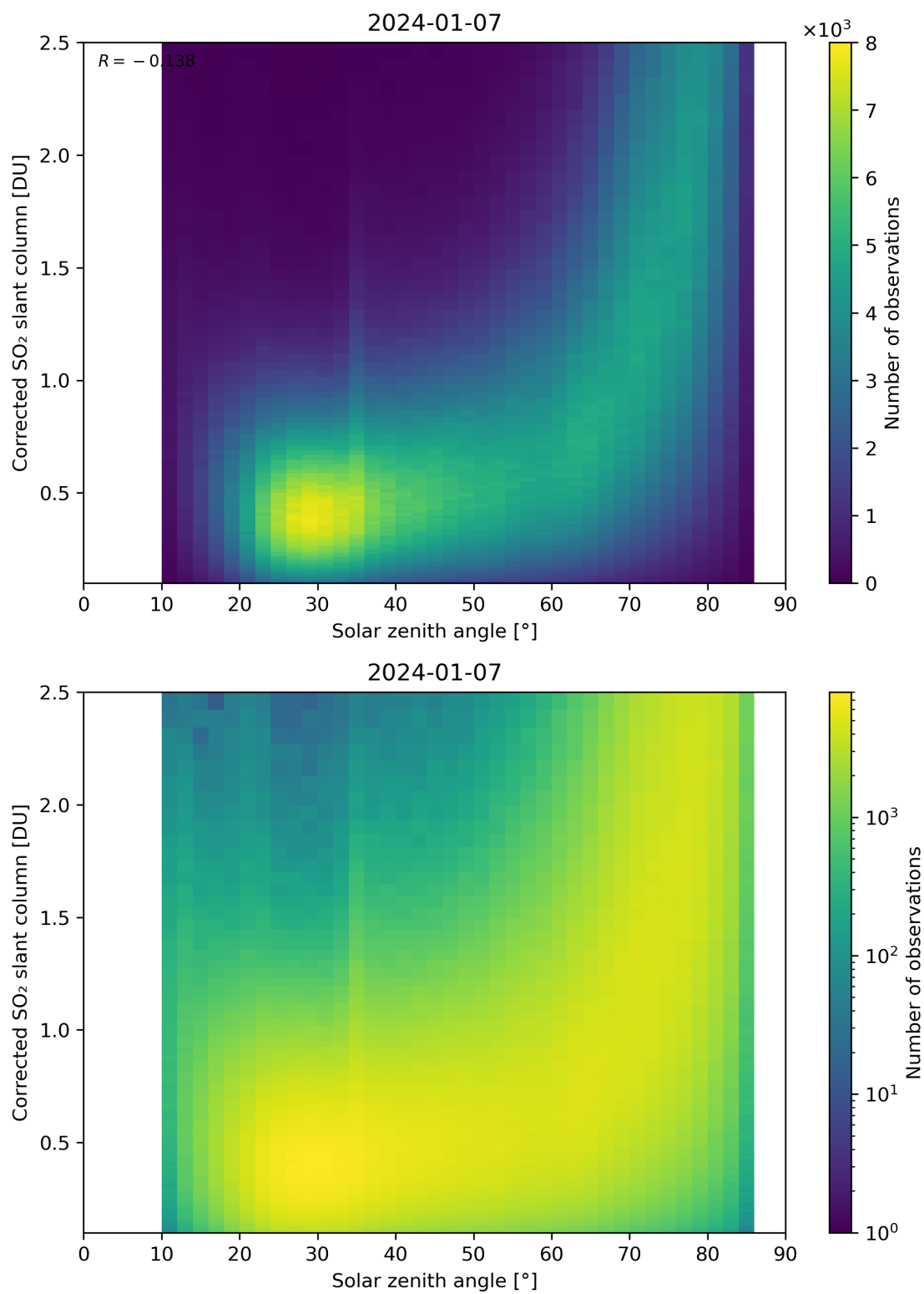
Figure 166: Scatter density plot of “Solar zenith angle” against “Corrected SO 2 slant column” for 2024-01-06 to 2024-01-08.
