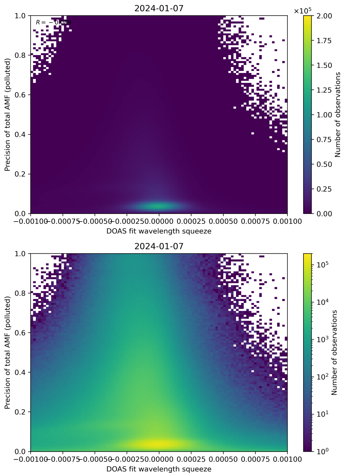
Figure 135: Scatter density plot of “DOAS fit wavelength squeeze” against “Precision of total AMF (polluted)” for 2024-01-06 to 2024-01-08.
