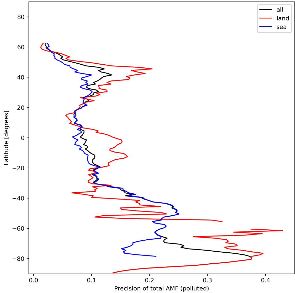
Figure 49: Zonal average of “Precision of total AMF (polluted)” for 2024-01-06 to 2024-01-08.
