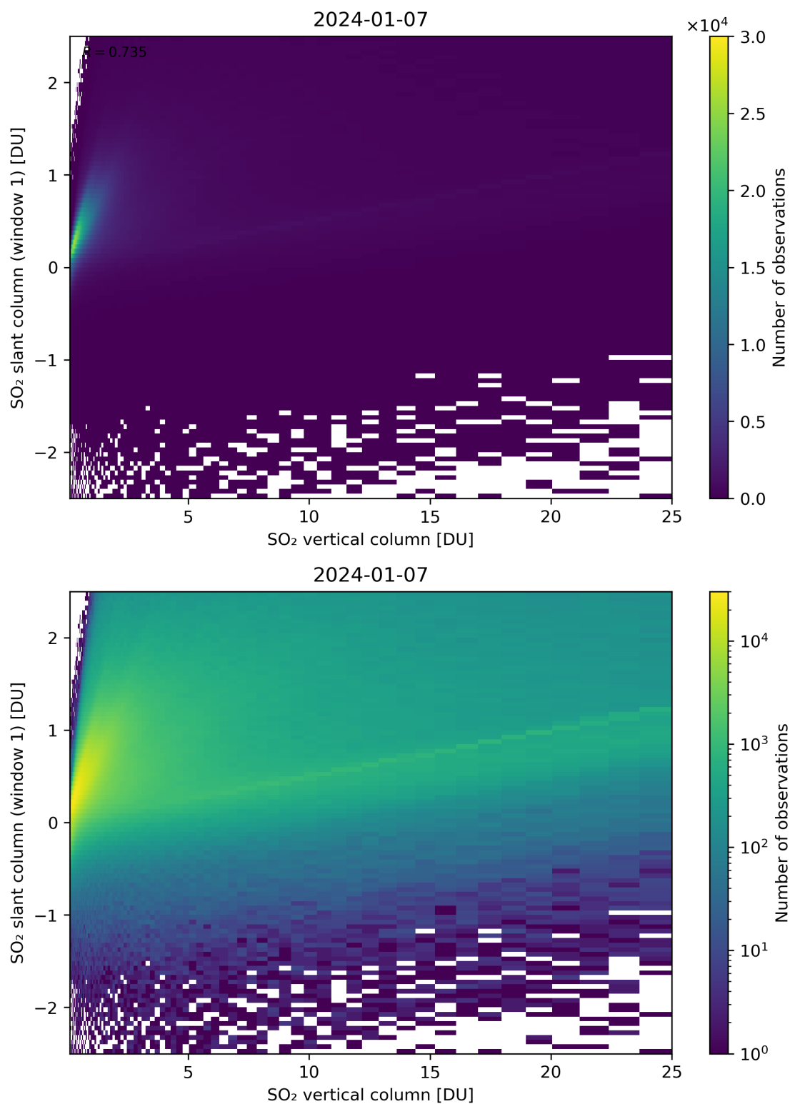
Figure 300: Scatter density plot of “SO 2 vertical column” against “SO 2 slant column (window 1)” for 2024-01-06 to 2024-01-08.
