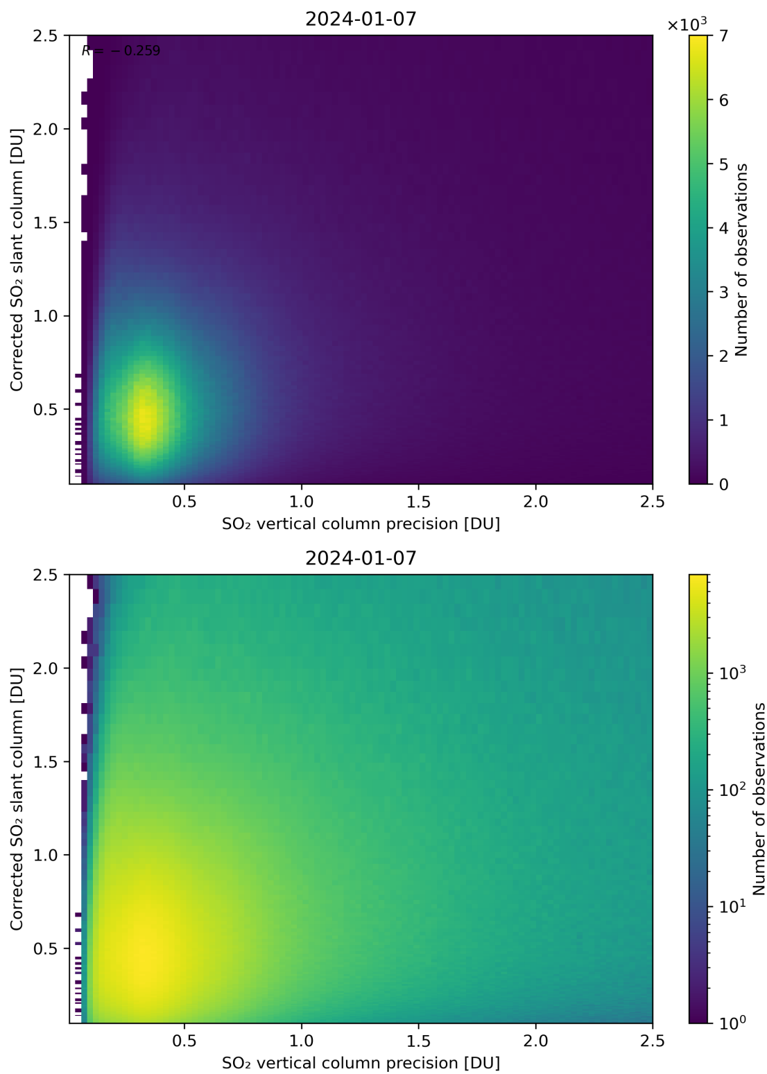
Figure 286: Scatter density plot of “SO 2 vertical column precision” against “Corrected SO 2 slant column” for 2024-01-06 to 2024-01-08.
