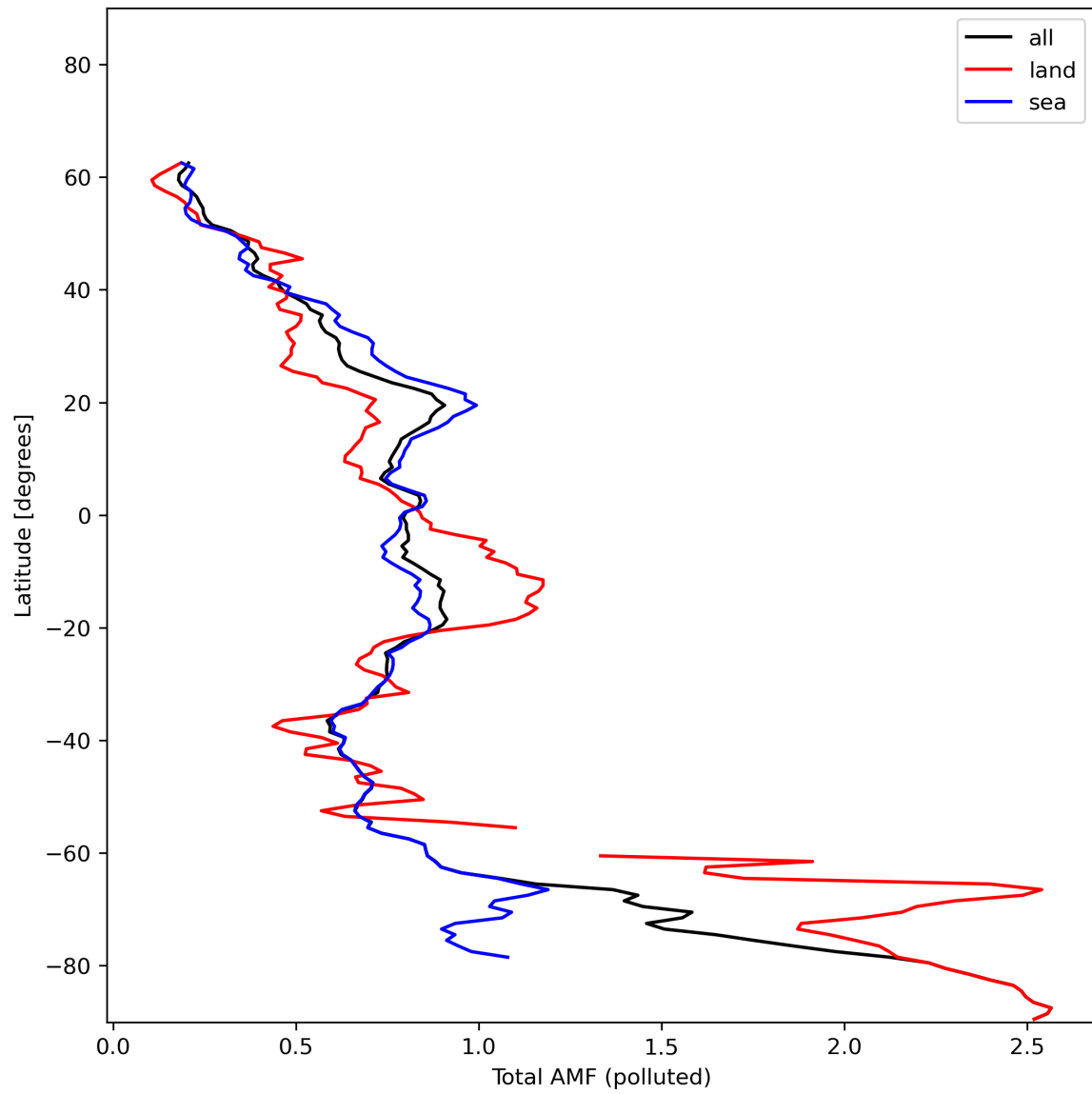
Figure 48: Zonal average of “Total AMF (polluted)” for 2024-01-06 to 2024-01-08.
