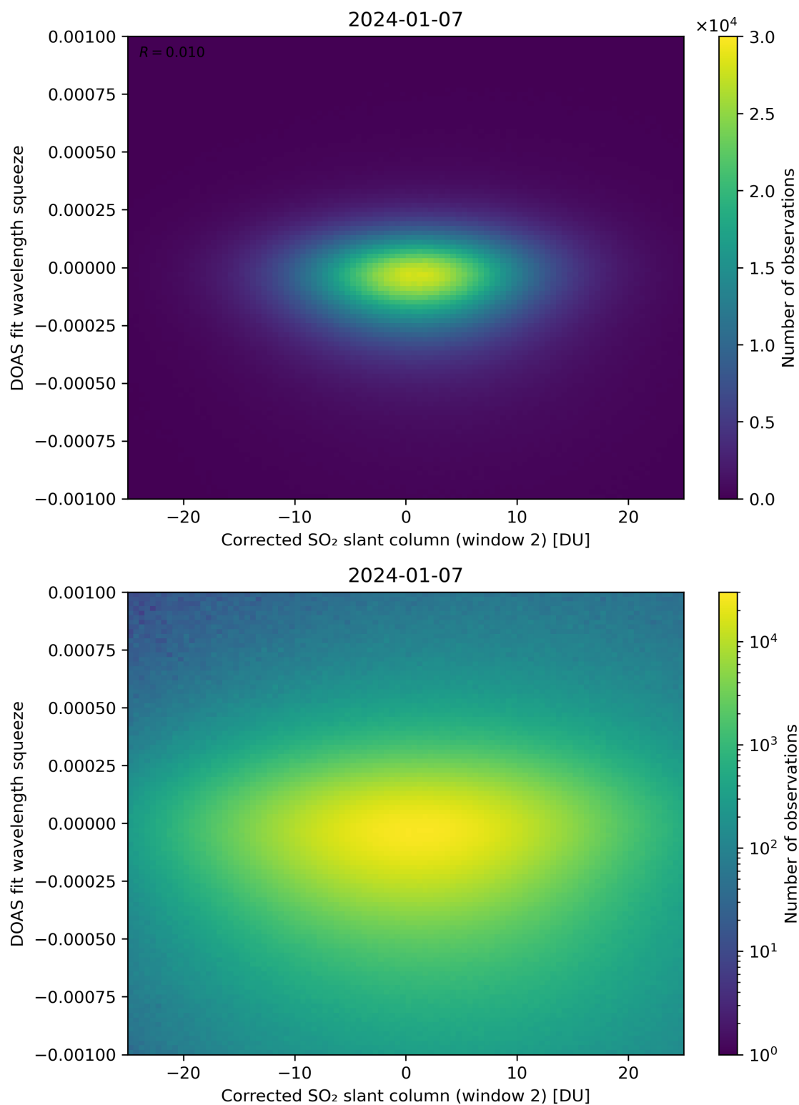
Figure 197: Scatter density plot of “Corrected SO 2 slant column (window 2)” against “DOAS fit wavelength squeeze” for 2024-01-06 to 2024-01-08.
