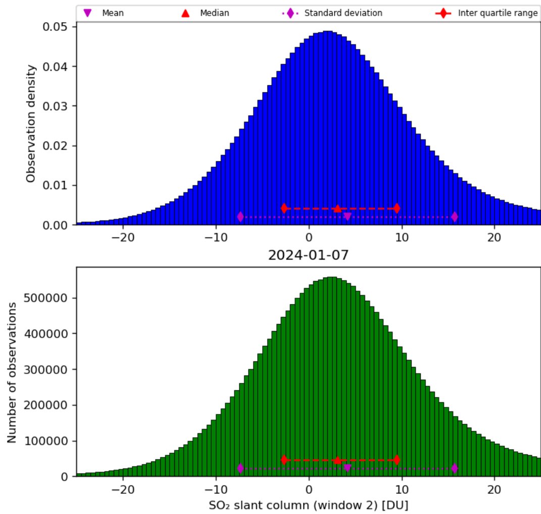
Figure 60: Histogram of “SO 2 slant column (window 2)” for 2024-01-06 to 2024-01-08
