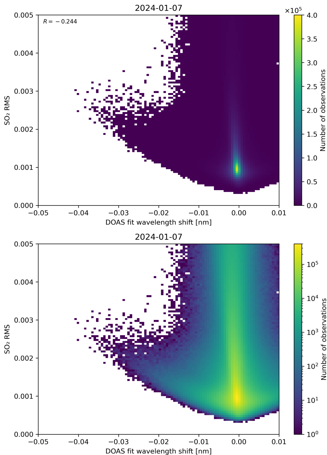
Figure 128: Scatter density plot of “DOAS fit wavelength shift” against “SO 2 RMS” for 2024-01-06 to 2024-01-08.
