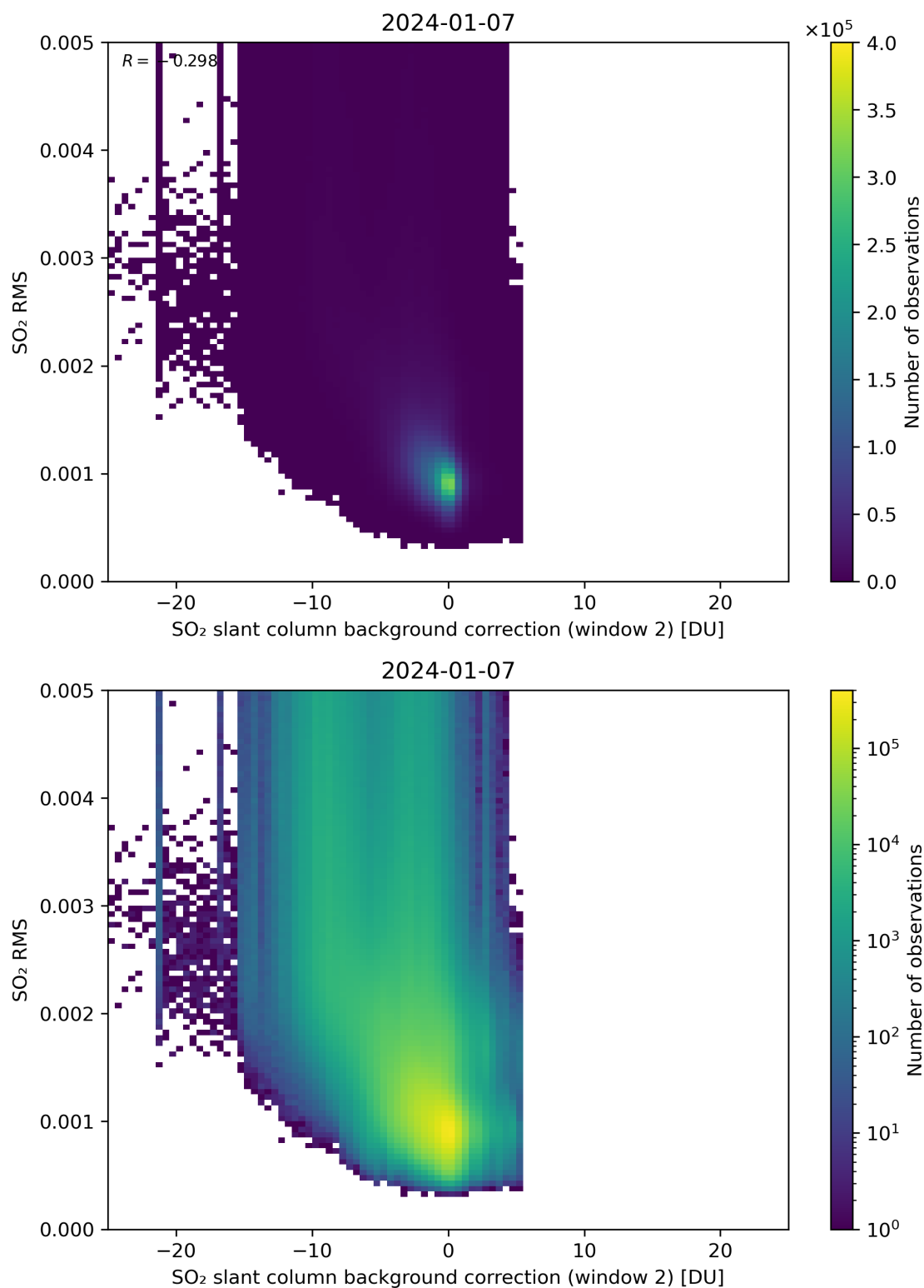
Figure 114: Scatter density plot of “SO 2 slant column background correction (window 2)” against “SO 2 RMS” for 2024-01-06 to 2024-01-08.
