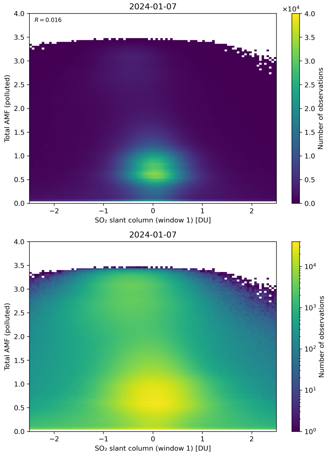
Figure 239: Scatter density plot of “SO 2 slant column (window 1)” against “Total AMF (polluted)” for 2024-01-06 to 2024-01-08.
