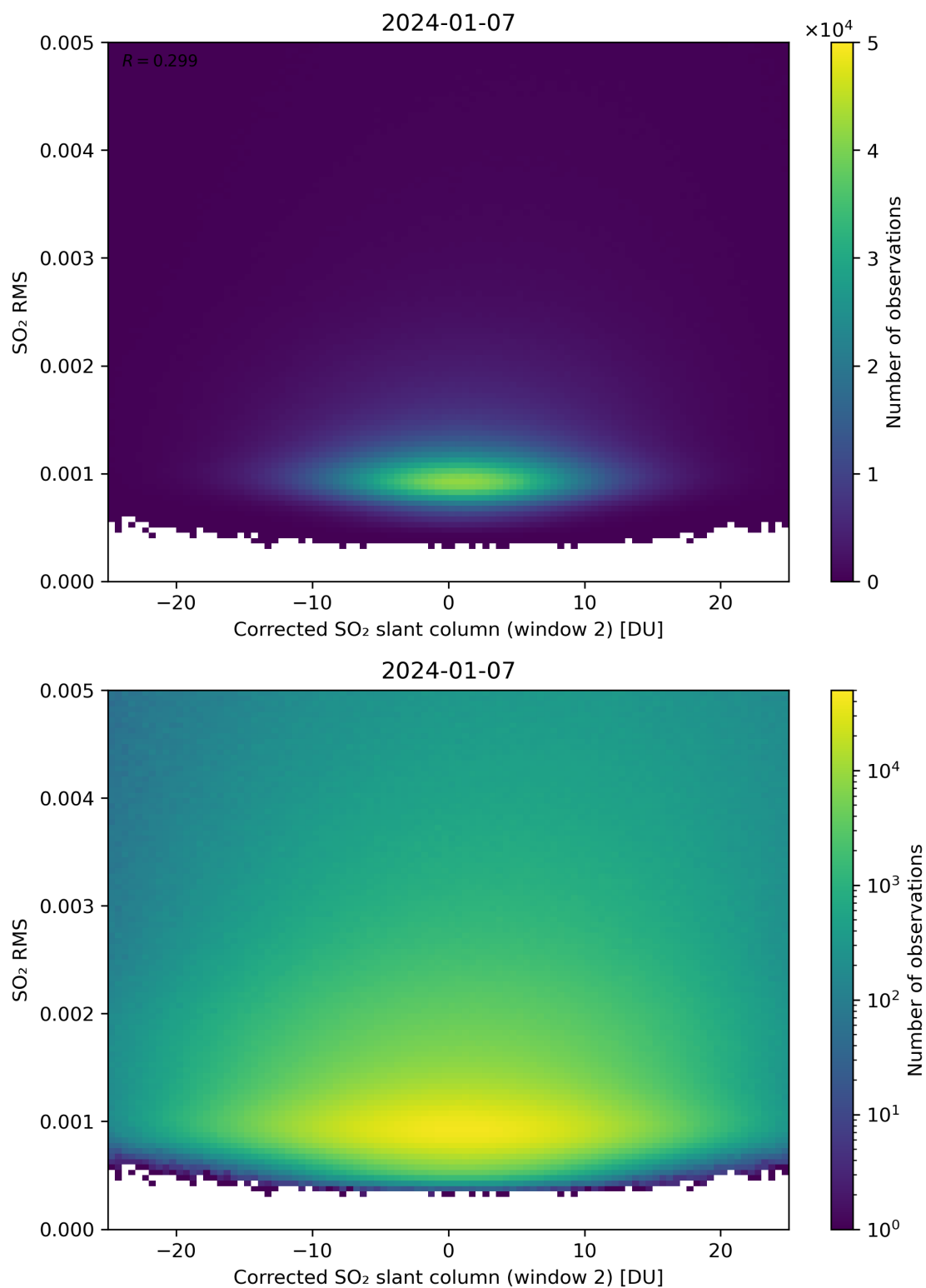
Figure 198: Scatter density plot of “Corrected SO 2 slant column (window 2)” against “SO 2 RMS” for 2024-01-06 to 2024-01-08.
