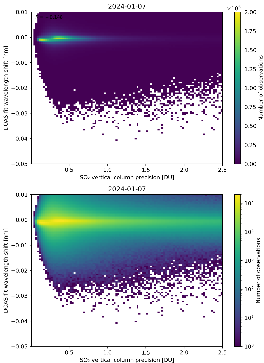
Figure 282: Scatter density plot of “SO 2 vertical column precision” against “DOAS fit wavelength shift” for 2024-01-06 to 2024-01-08.
