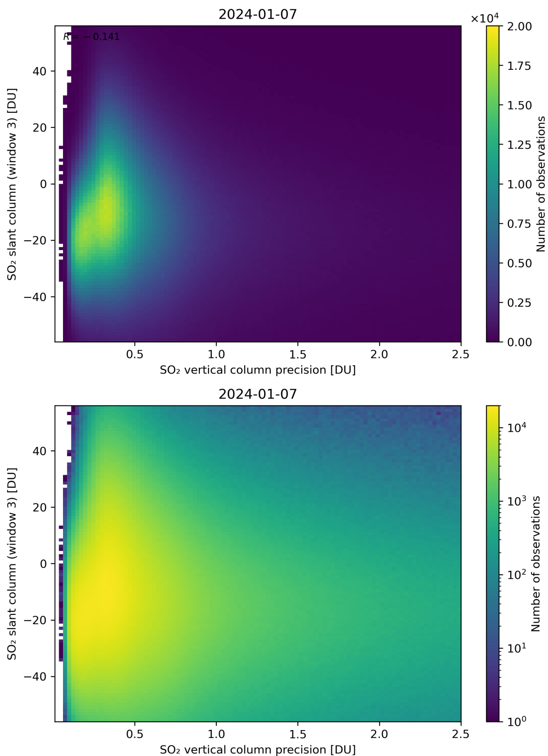
Figure 292: Scatter density plot of “SO 2 vertical column precision” against “SO 2 slant column (window 3)” for 2024-01-06 to 2024-01-08.
