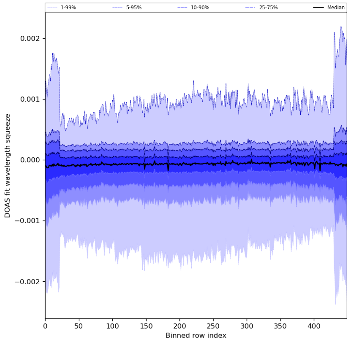
Figure 92: Along track statistics of “DOAS fit wavelength squeeze” for 2024-01-06 to 2024-01-08
