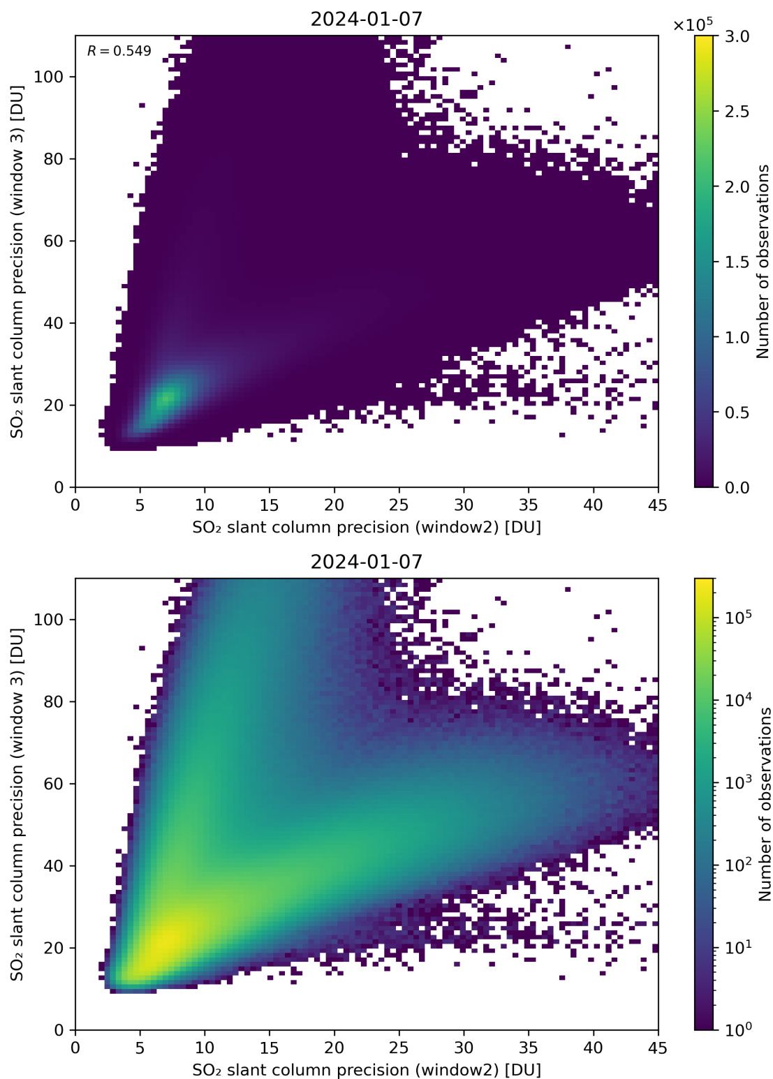
Figure 250: Scatter density plot of “SO 2 slant column precision (window2)” against “SO 2 slant column precision (window 3)” for 2024-01-06 to 2024-01-08.
