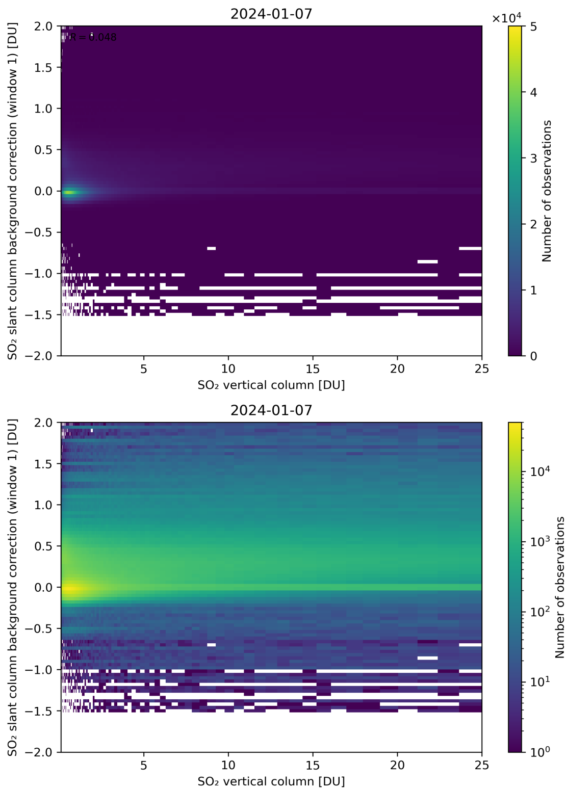
Figure 273: Scatter density plot of “SO 2 vertical column” against “SO 2 slant column background correction (window 1)” for 2024-01-06 to 2024-01-08.
