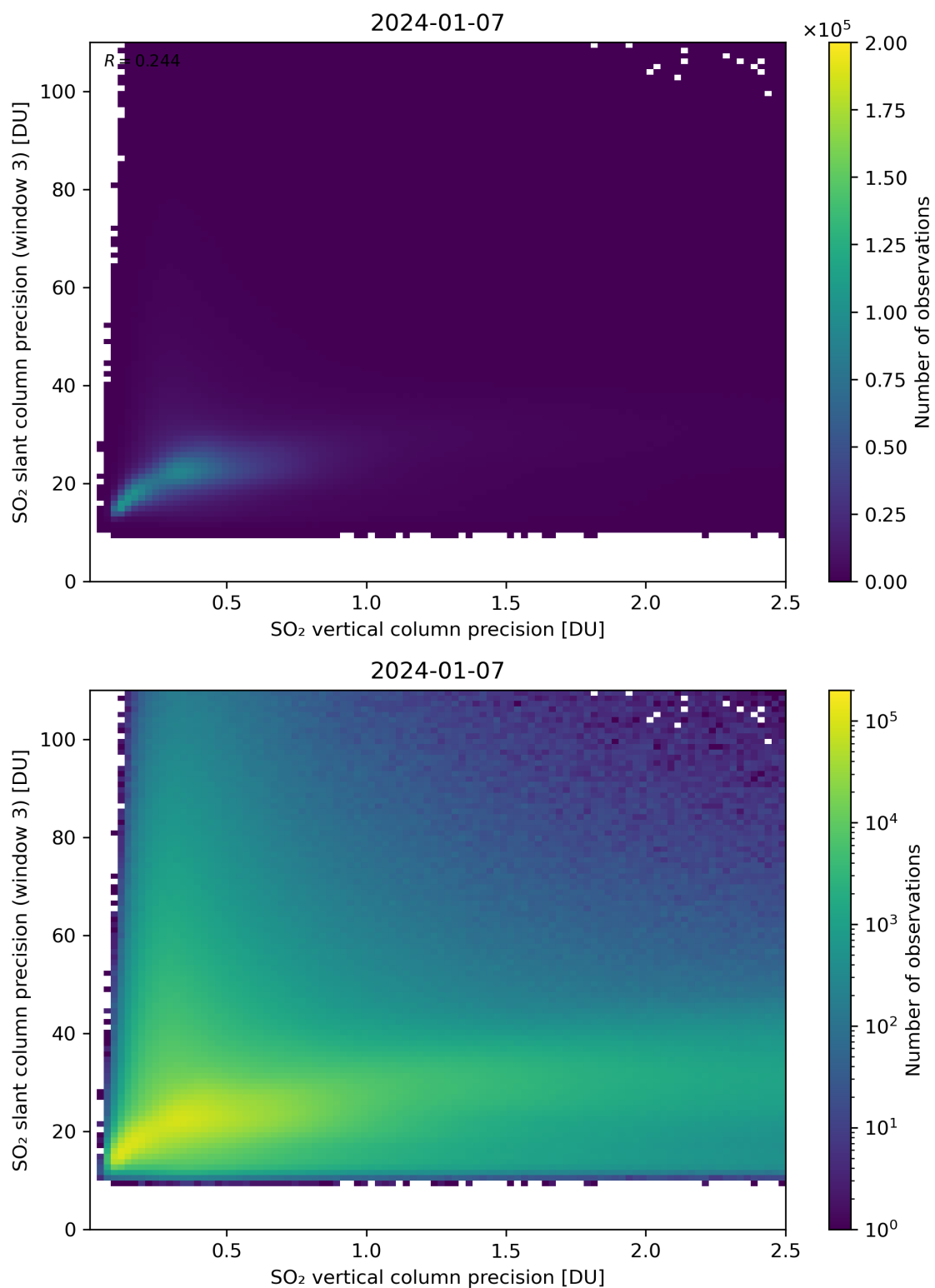
Figure 293: Scatter density plot of “SO 2 vertical column precision” against “SO 2 slant column precision (window 3)” for 2024-01-06 to 2024-01-08.
