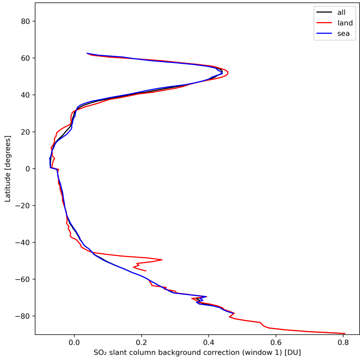
Figure 36: Zonal average of “SO 2 slant column background correction (window 1)” for 2024-01-06 to 2024-01-08.
