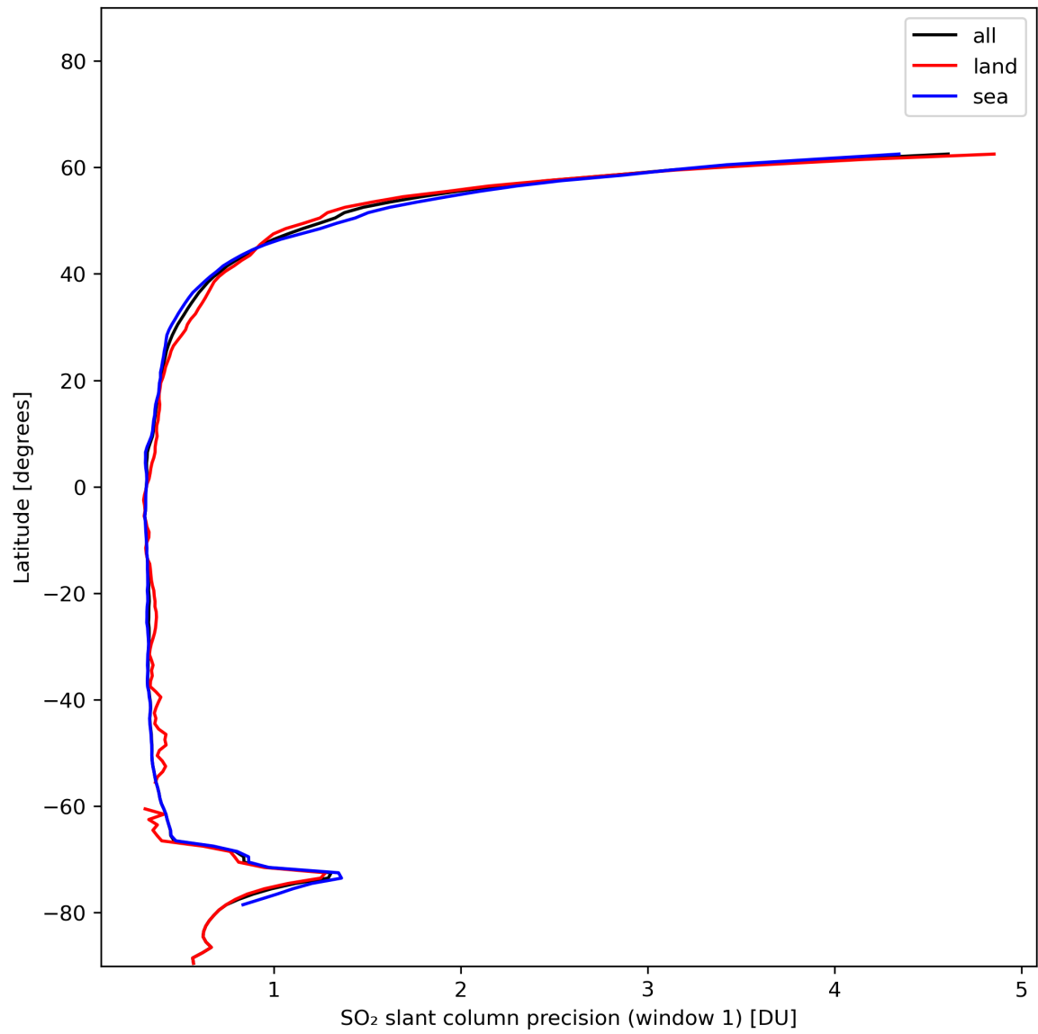
Figure 34: Zonal average of “SO 2 slant column precision (window 1)” for 2024-01-06 to 2024-01-08.
