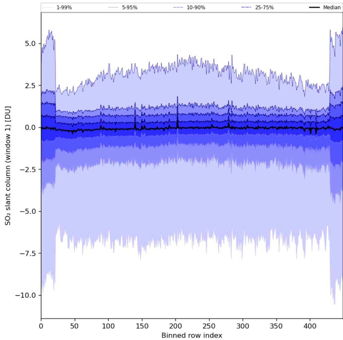
Figure 79: Along track statistics of “SO 2 slant column (window 1)” for 2024-01-06 to 2024-01-08
