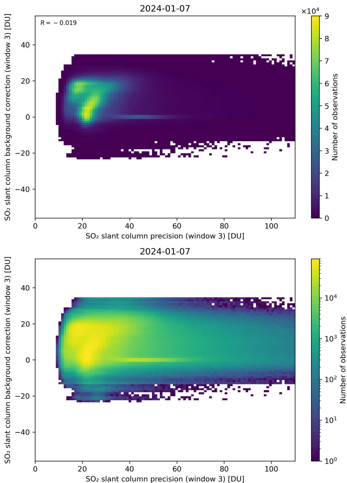
Figure 257: Scatter density plot of “SO 2 slant column precision (window 3)” against “SO 2 slant column background correction (window 3)” for 2024-01-06 to 2024-01-08.
