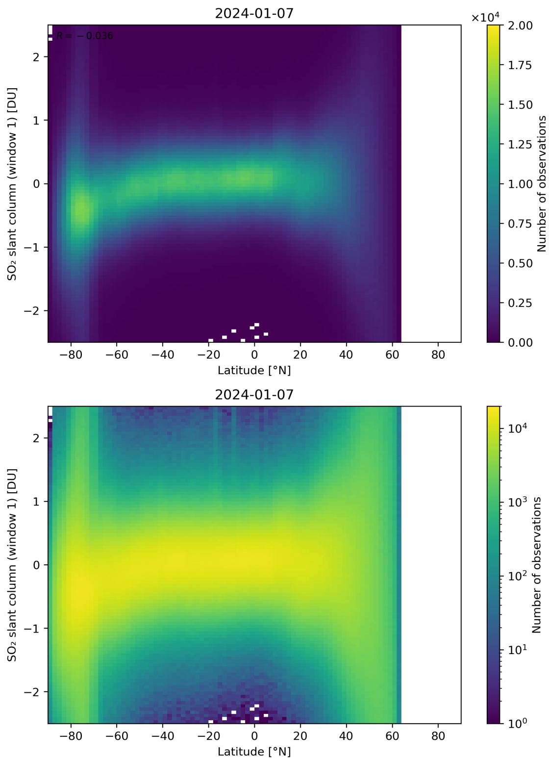
Figure 149: Scatter density plot of “Latitude” against “SO 2 slant column (window 1)” for 2024-01-06 to 2024-01-08.
