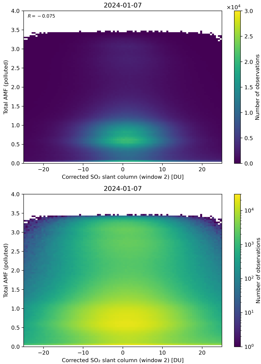
Figure 203: Scatter density plot of “Corrected SO 2 slant column (window 2)” against “Total AMF (polluted)” for 2024-01-06 to 2024-01-08.
