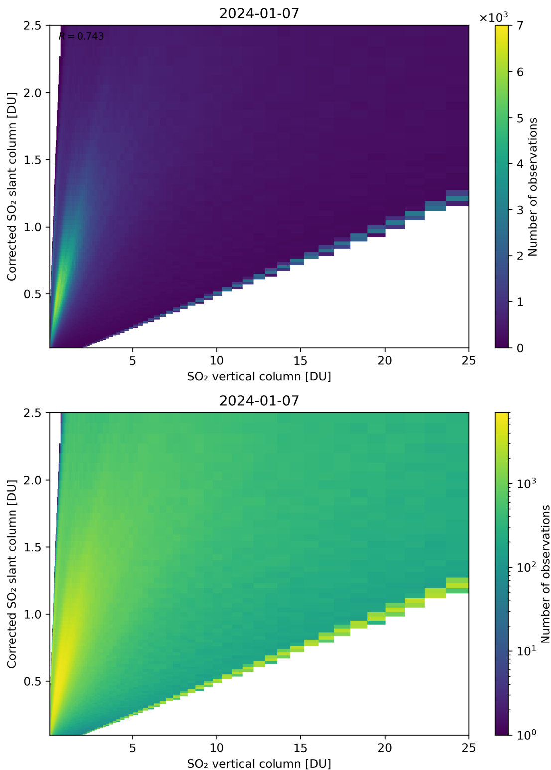
Figure 297: Scatter density plot of “SO 2 vertical column” against “Corrected SO 2 slant column” for 2024-01-06 to 2024-01-08.
