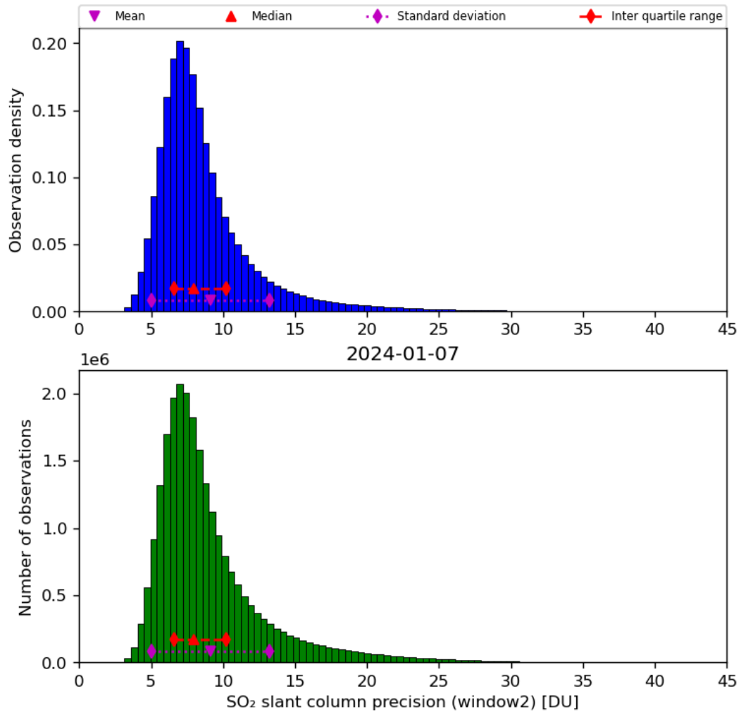
Figure 61: Histogram of “SO 2 slant column precision (window2)” for 2024-01-06 to 2024-01-08
