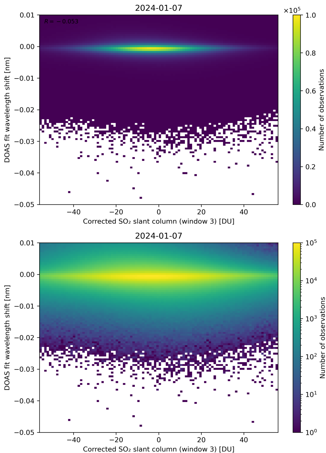
Figure 206: Scatter density plot of “Corrected SO 2 slant column (window 3)” against “DOAS fit wavelength shift” for 2024-01-06 to 2024-01-08.
