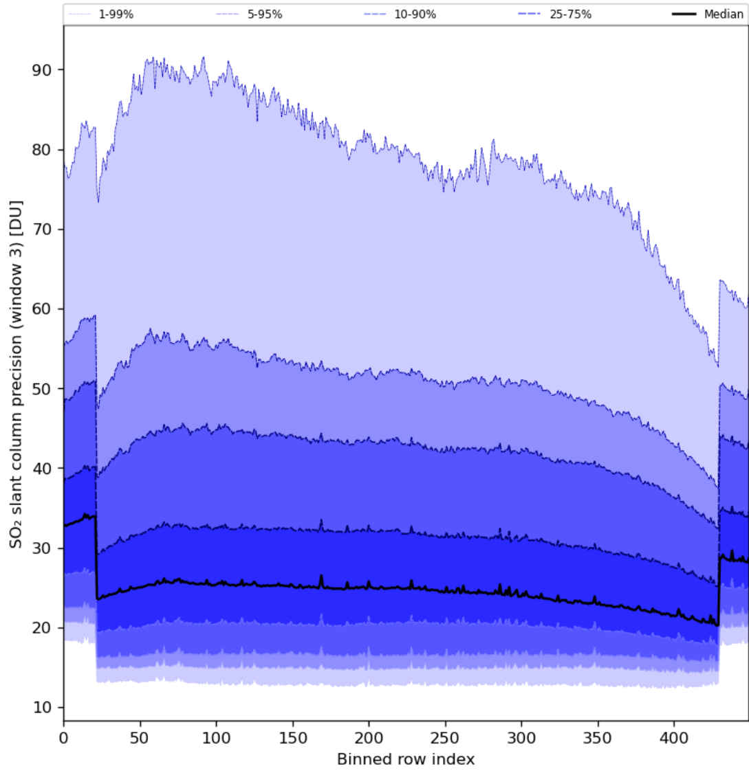
Figure 88: Along track statistics of “SO 2 slant column precision (window 3)” for 2024-01-06 to 2024-01-08
