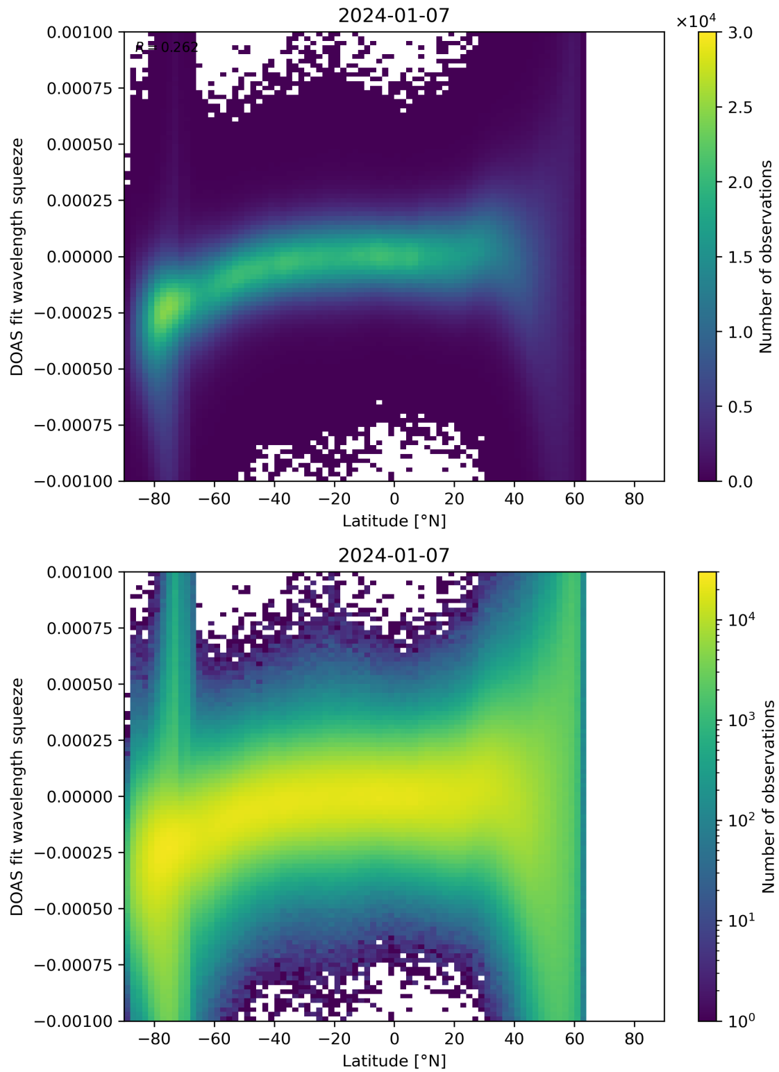
Figure 143: Scatter density plot of “Latitude” against “DOAS fit wavelength squeeze” for 2024-01-06 to 2024-01-08.
