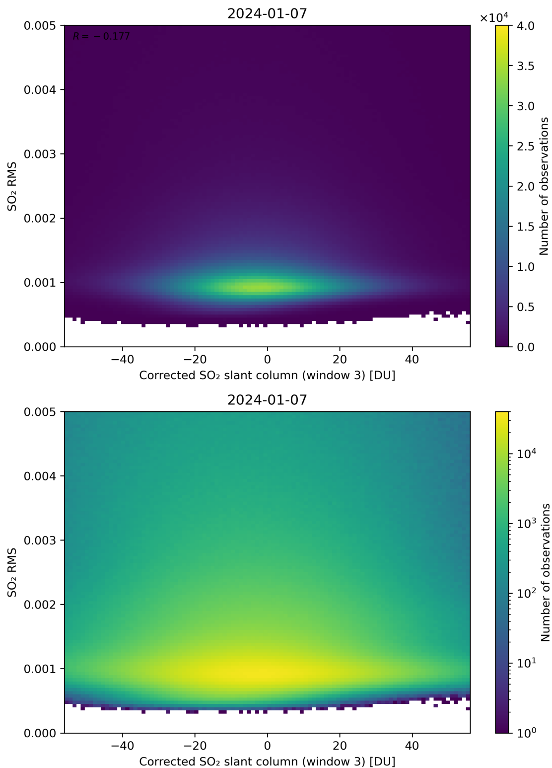
Figure 208: Scatter density plot of “Corrected SO 2 slant column (window 3)” against “SO 2 RMS” for 2024-01-06 to 2024-01-08.
