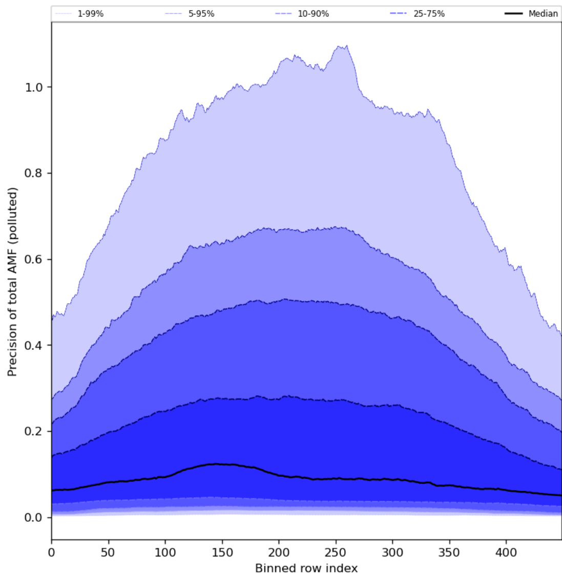
Figure 95: Along track statistics of “Precision of total AMF (polluted)” for 2024-01-06 to 2024-01-08
