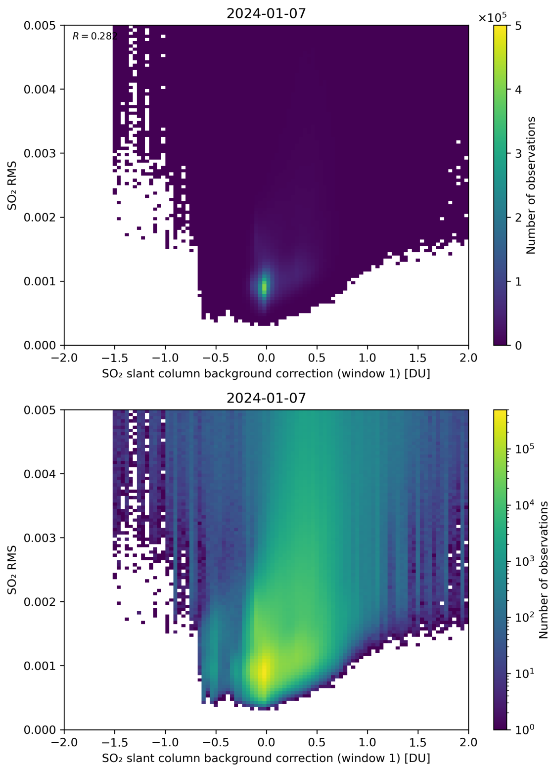
Figure 102: Scatter density plot of “SO 2 slant column background correction (window 1)” against “SO 2 RMS” for 2024-01-06 to 2024-01-08.
