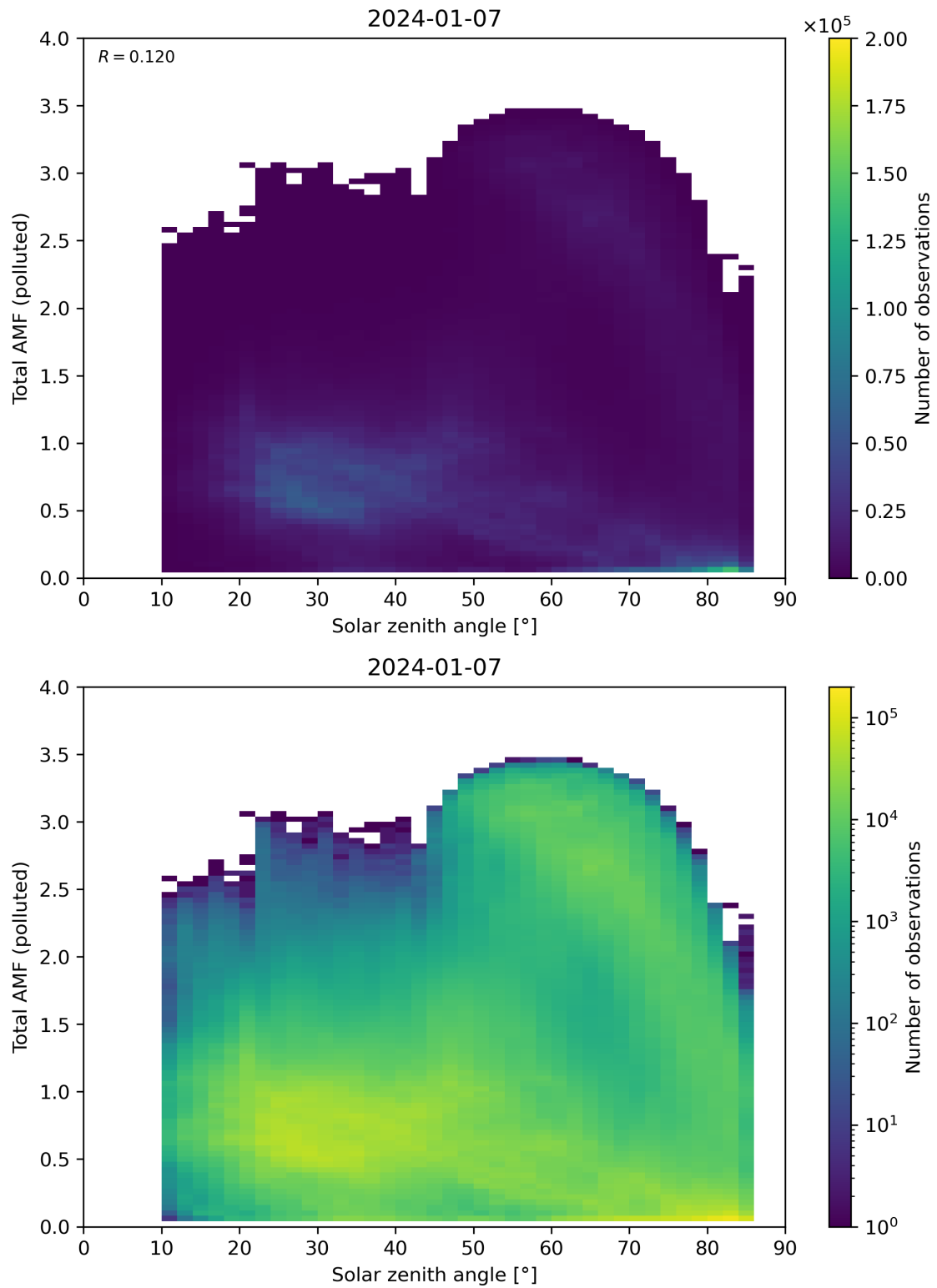
Figure 174: Scatter density plot of “Solar zenith angle” against “Total AMF (polluted)” for 2024-01-06 to 2024-01-08.
