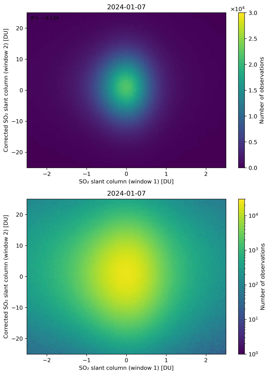
Figure 233: Scatter density plot of “SO 2 slant column (window 1)” against “Corrected SO 2 slant column (window 2)” for 2024-01-06 to 2024-01-08.
