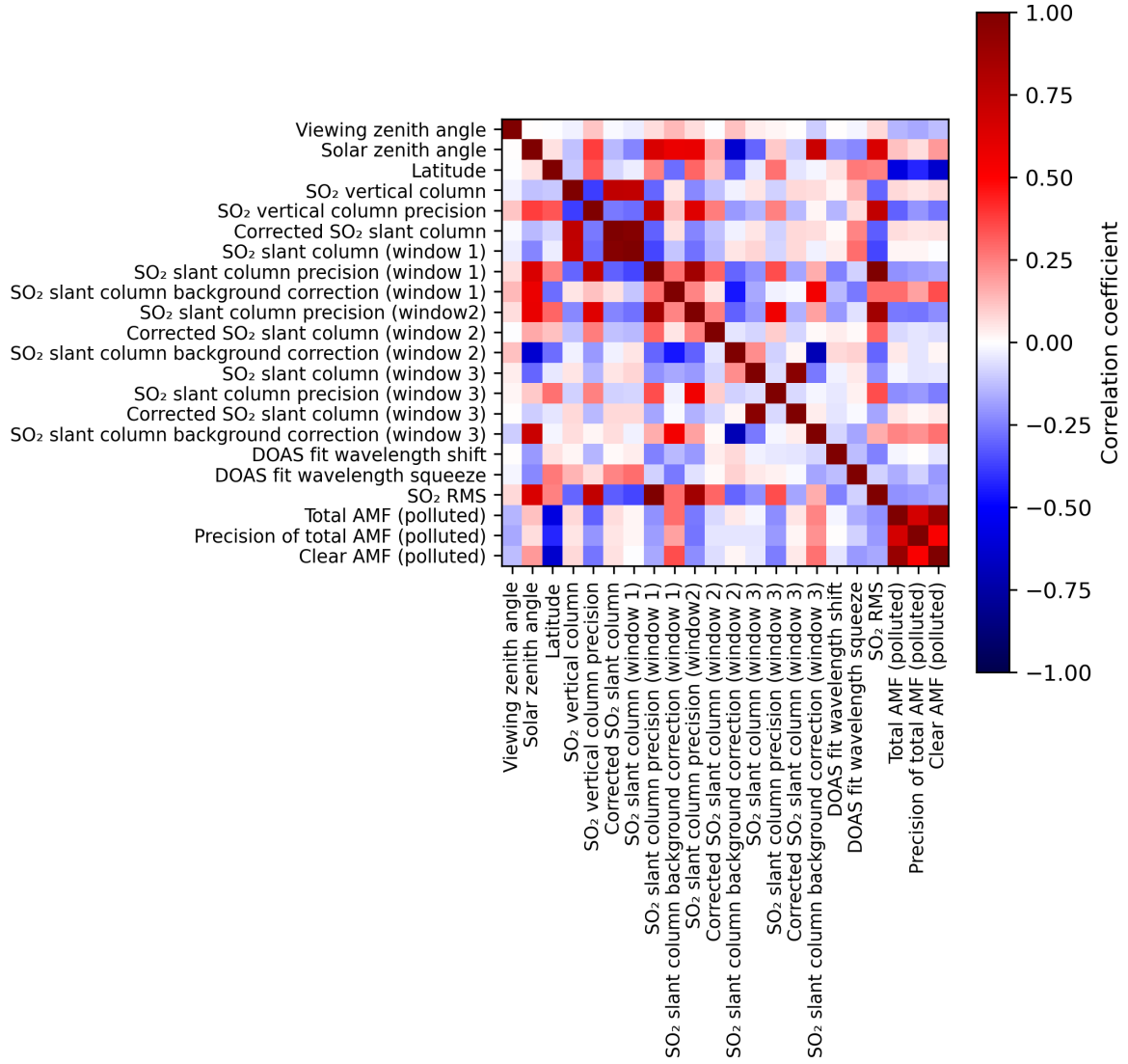
Figure 2: Map of correlation matrix for 2024-01-06 to 2024-01-08.
