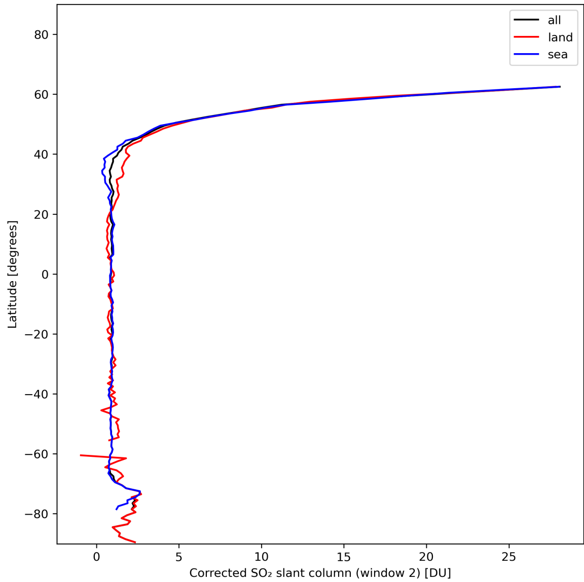
Figure 39: Zonal average of “Corrected SO 2 slant column (window 2)” for 2024-01-06 to 2024-01-08.
