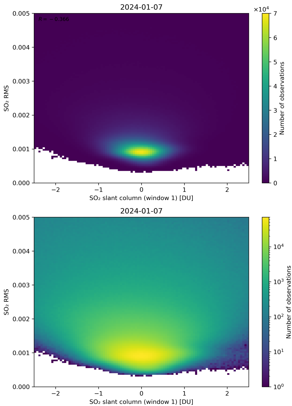
Figure 217: Scatter density plot of “SO 2 slant column (window 1)” against “SO 2 RMS” for 2024-01-06 to 2024-01-08.
