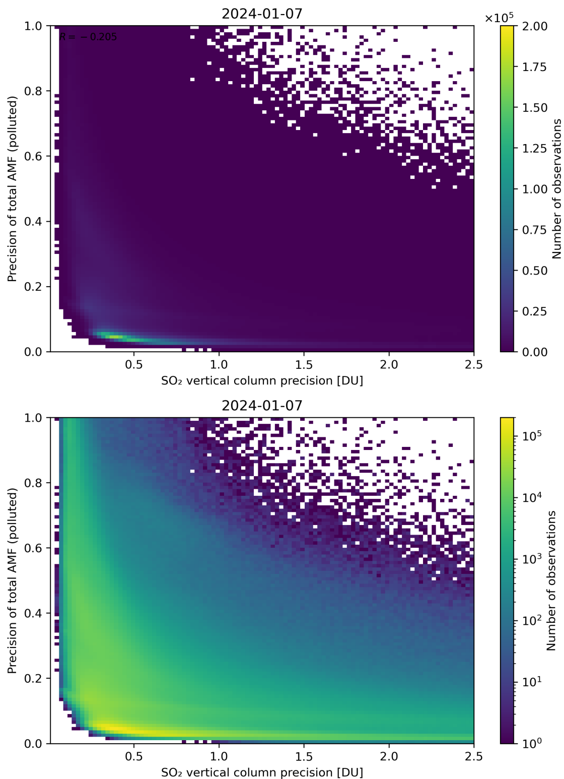
Figure 295: Scatter density plot of “SO 2 vertical column precision” against “Precision of total AMF (polluted)” for 2024-01-06 to 2024-01-08.
