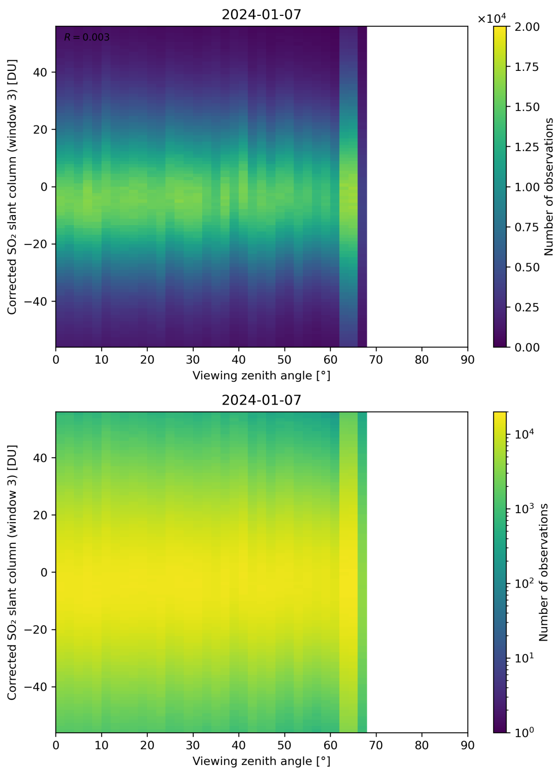
Figure 319: Scatter density plot of “Viewing zenith angle” against “Corrected SO 2 slant column (window 3)” for 2024-01-06 to 2024-01-08.
