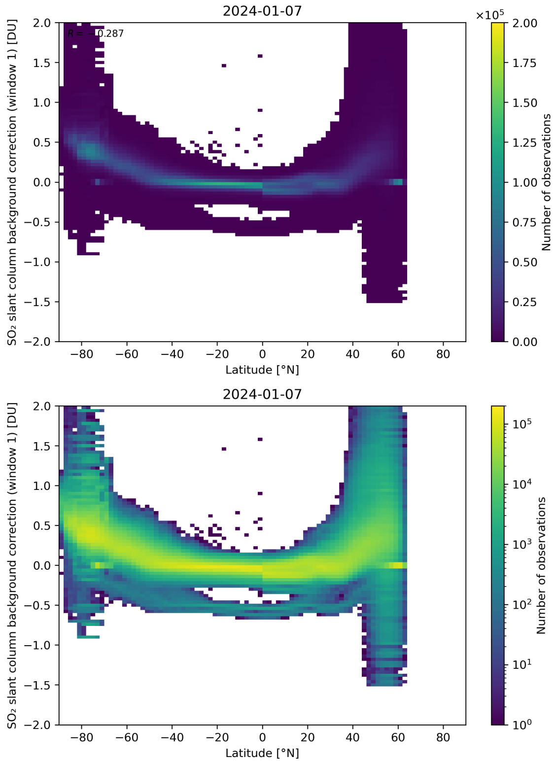
Figure 139: Scatter density plot of “Latitude” against “SO 2 slant column background correction (window 1)” for 2024-01-06 to 2024-01-08.
