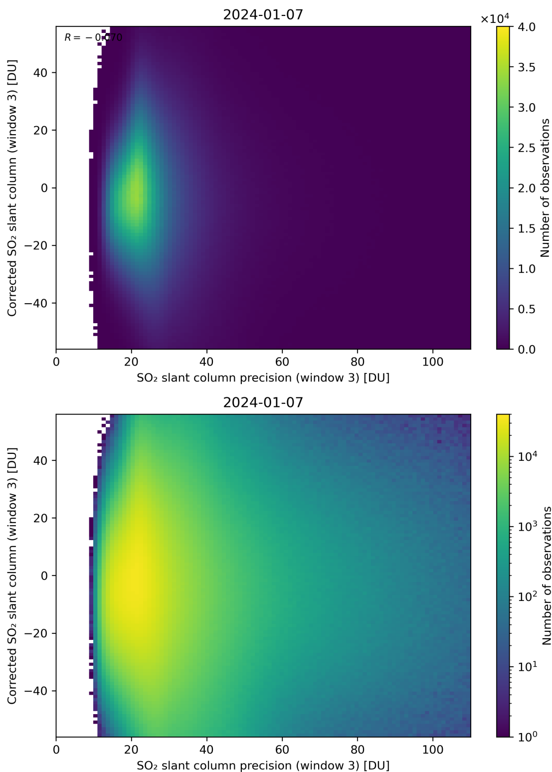
Figure 262: Scatter density plot of “SO 2 slant column precision (window 3)” against “Corrected SO 2 slant column (window 3)” for 2024-01-06 to 2024-01-08.
