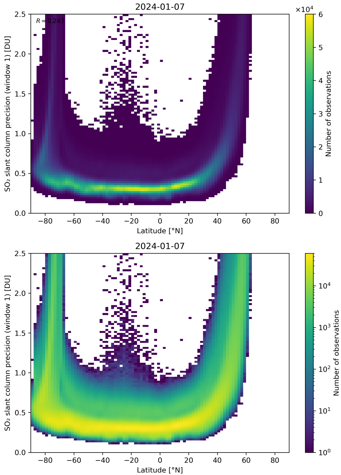
Figure 150: Scatter density plot of “Latitude” against “SO 2 slant column precision (window 1)” for 2024-01-06 to 2024-01-08.
