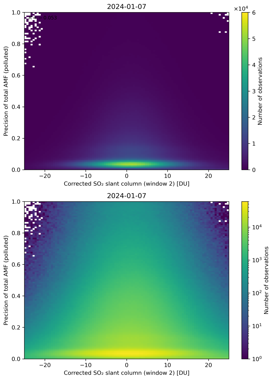
Figure 204: Scatter density plot of “Corrected SO 2 slant column (window 2)” against “Precision of total AMF (polluted)” for 2024-01-06 to 2024-01-08.
