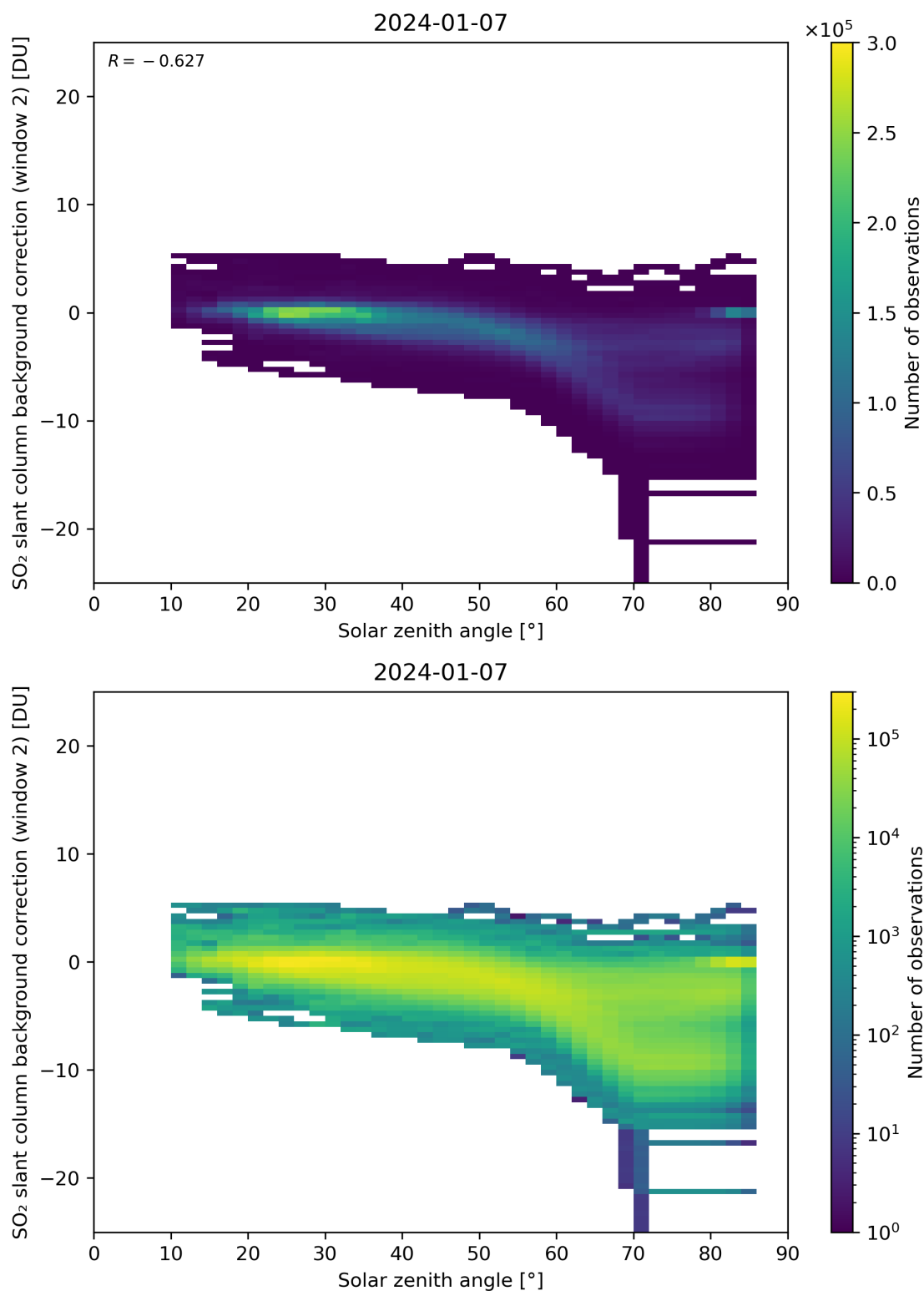
Figure 159: Scatter density plot of “Solar zenith angle” against “SO 2 slant column background correction (window 2)” for 2024-01-06 to 2024-01-08.
