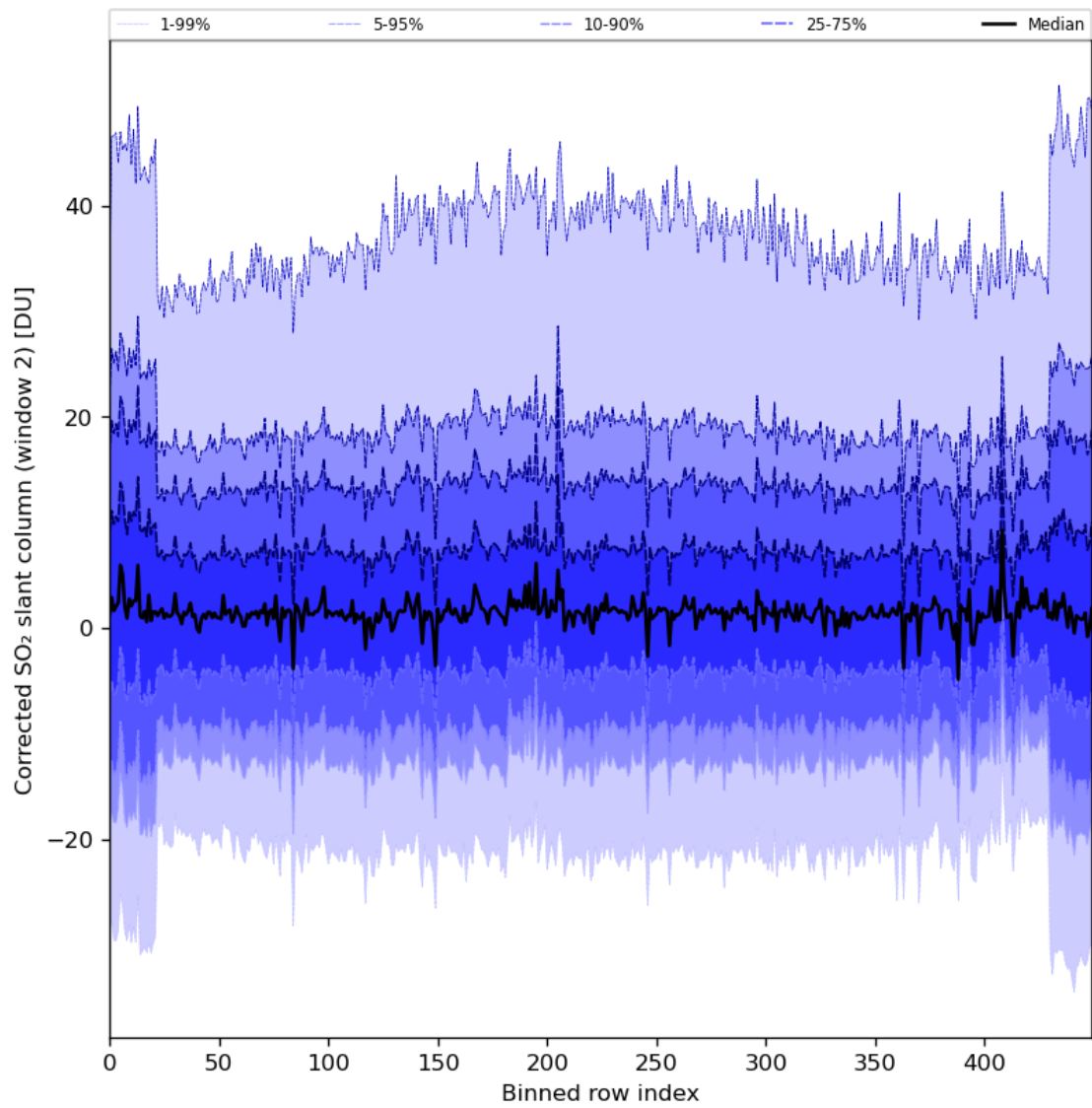
Figure 85: Along track statistics of “Corrected SO 2 slant column (window 2)” for 2024-01-06 to 2024-01-08
