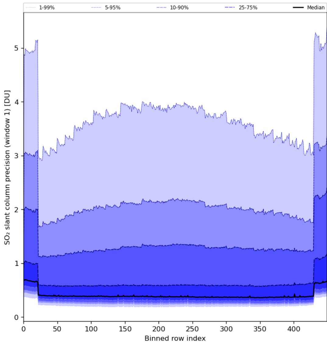
Figure 80: Along track statistics of “SO 2 slant column precision (window 1)” for 2024-01-06 to 2024-01-08
