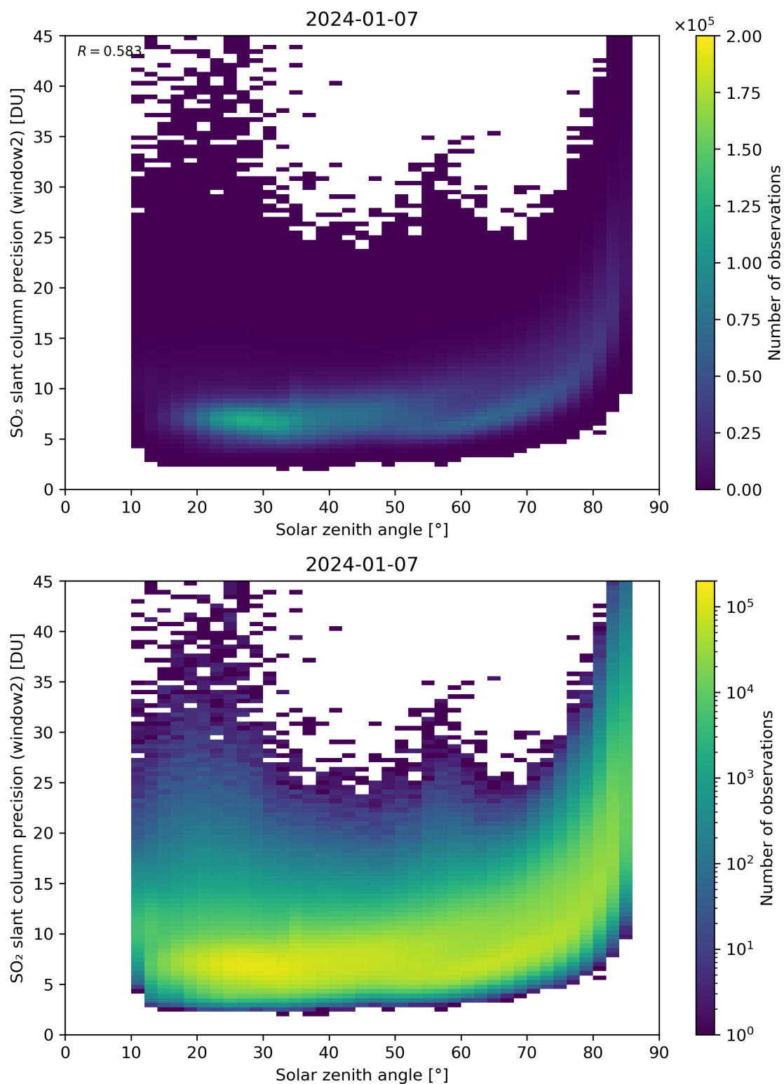
Figure 171: Scatter density plot of “Solar zenith angle” against “SO 2 slant column precision (window2)” for 2024-01-06 to 2024-01-08.
