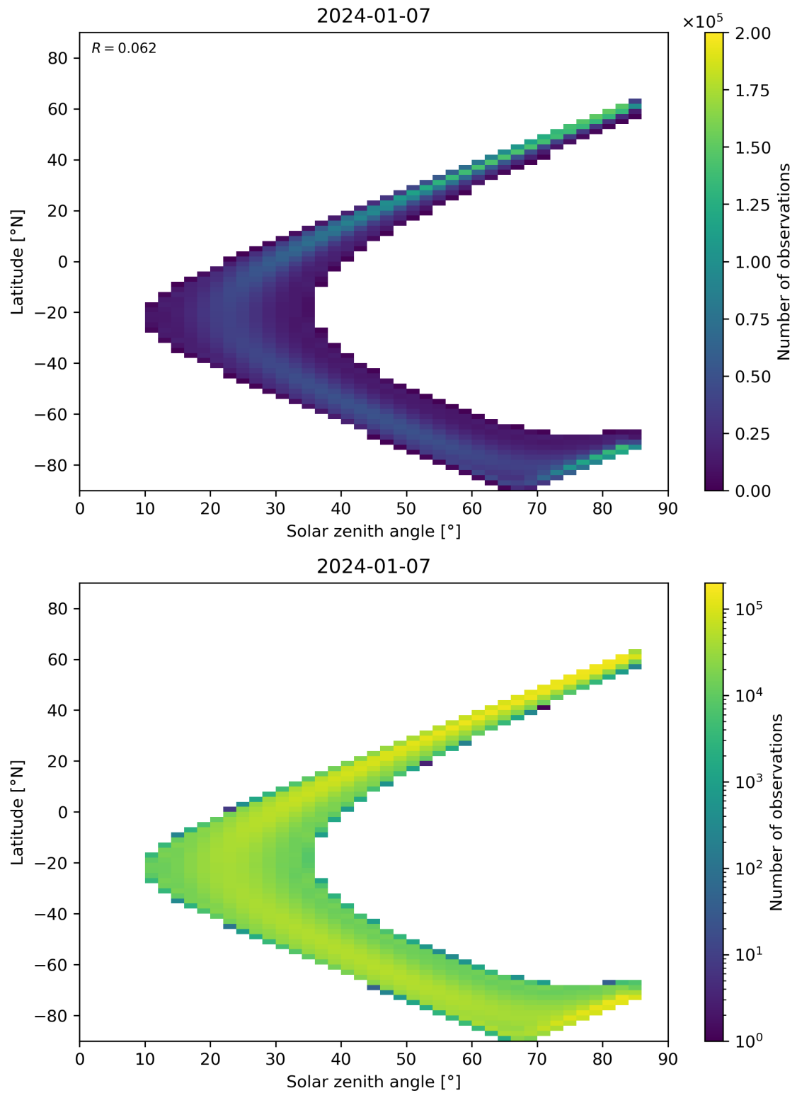
Figure 164: Scatter density plot of “Solar zenith angle” against “Latitude” for 2024-01-06 to 2024-01-08.
