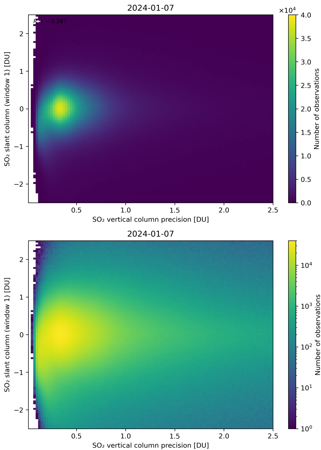
Figure 289: Scatter density plot of “SO 2 vertical column precision” against “SO 2 slant column (window 1)” for 2024-01-06 to 2024-01-08.
