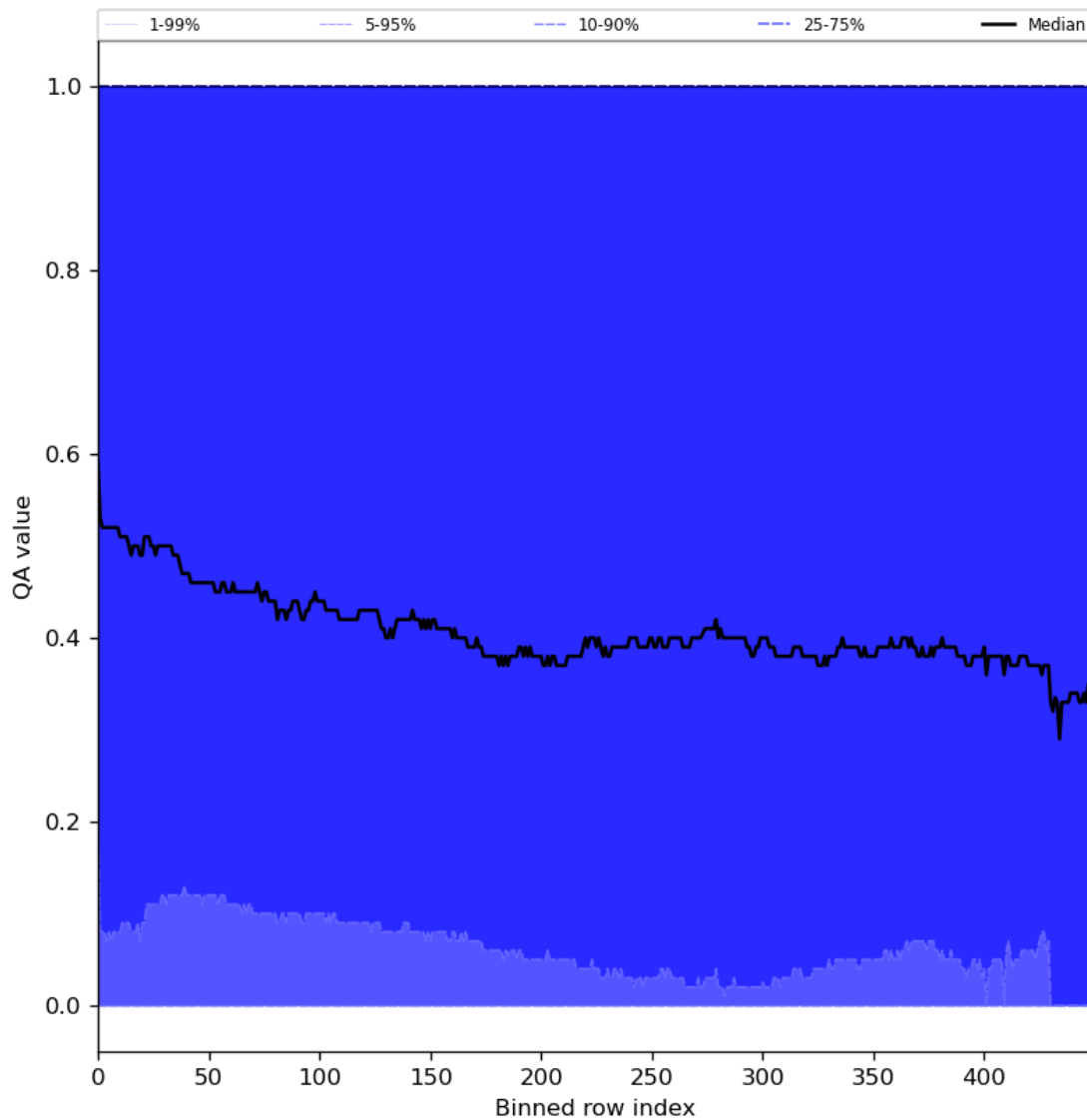
Figure 75: Along track statistics of “QA value” for 2024-01-06 to 2024-01-08
