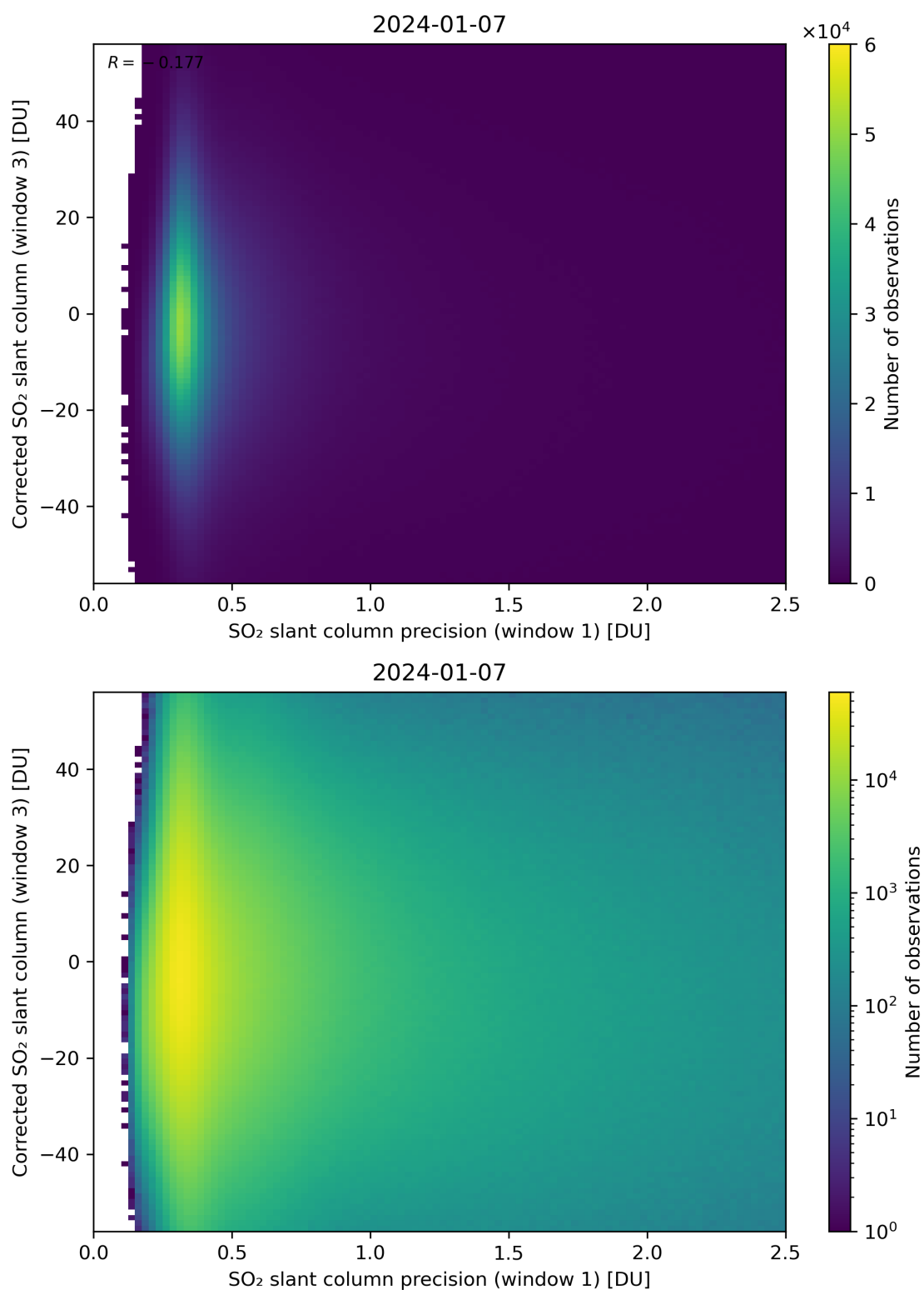
Figure 226: Scatter density plot of “SO 2 slant column precision (window 1)” against “Corrected SO 2 slant column (window 3)” for 2024-01-06 to 2024-01-08.
