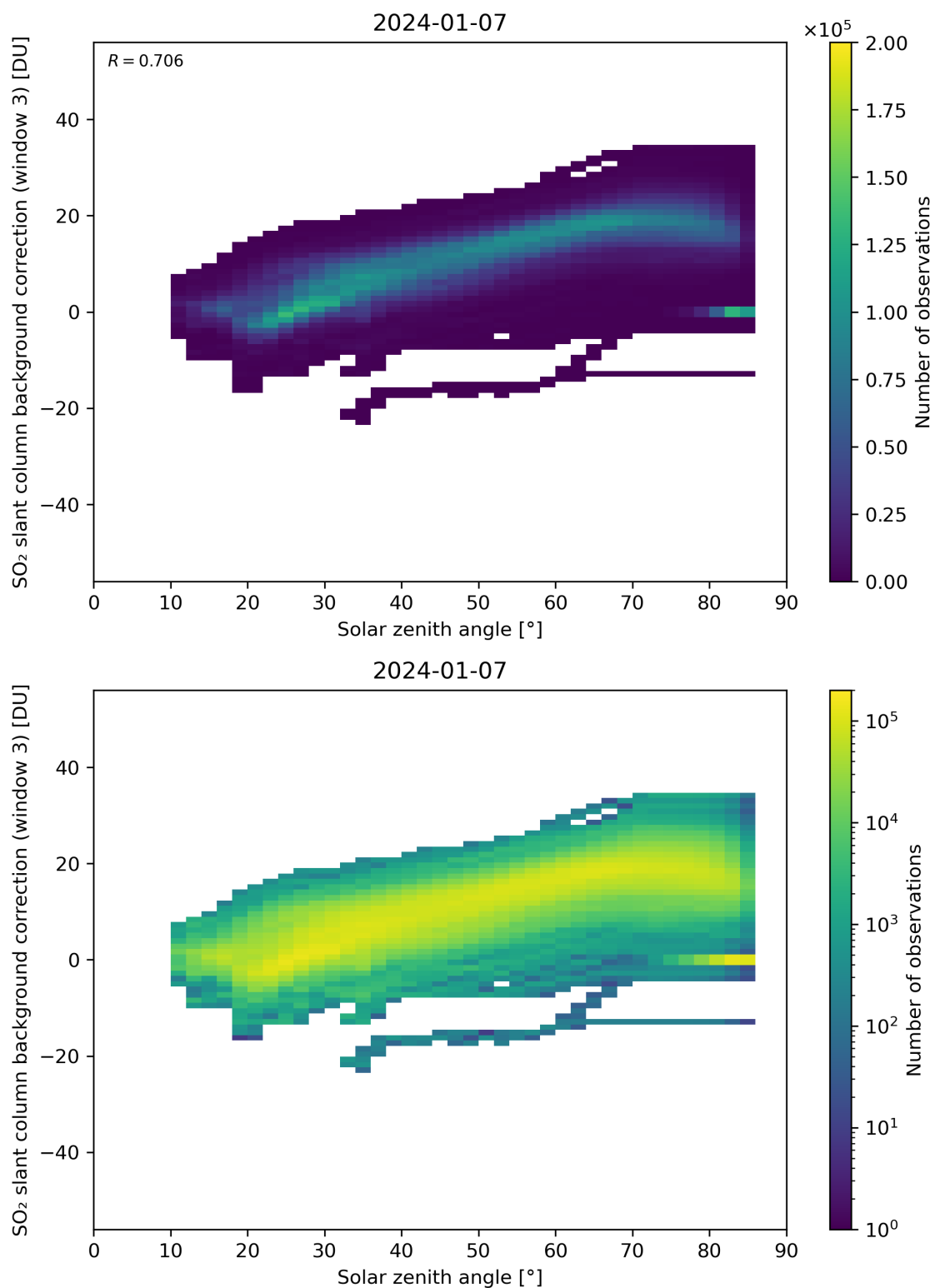
Figure 160: Scatter density plot of “Solar zenith angle” against “SO 2 slant column background correction (window 3)” for 2024-01-06 to 2024-01-08.
