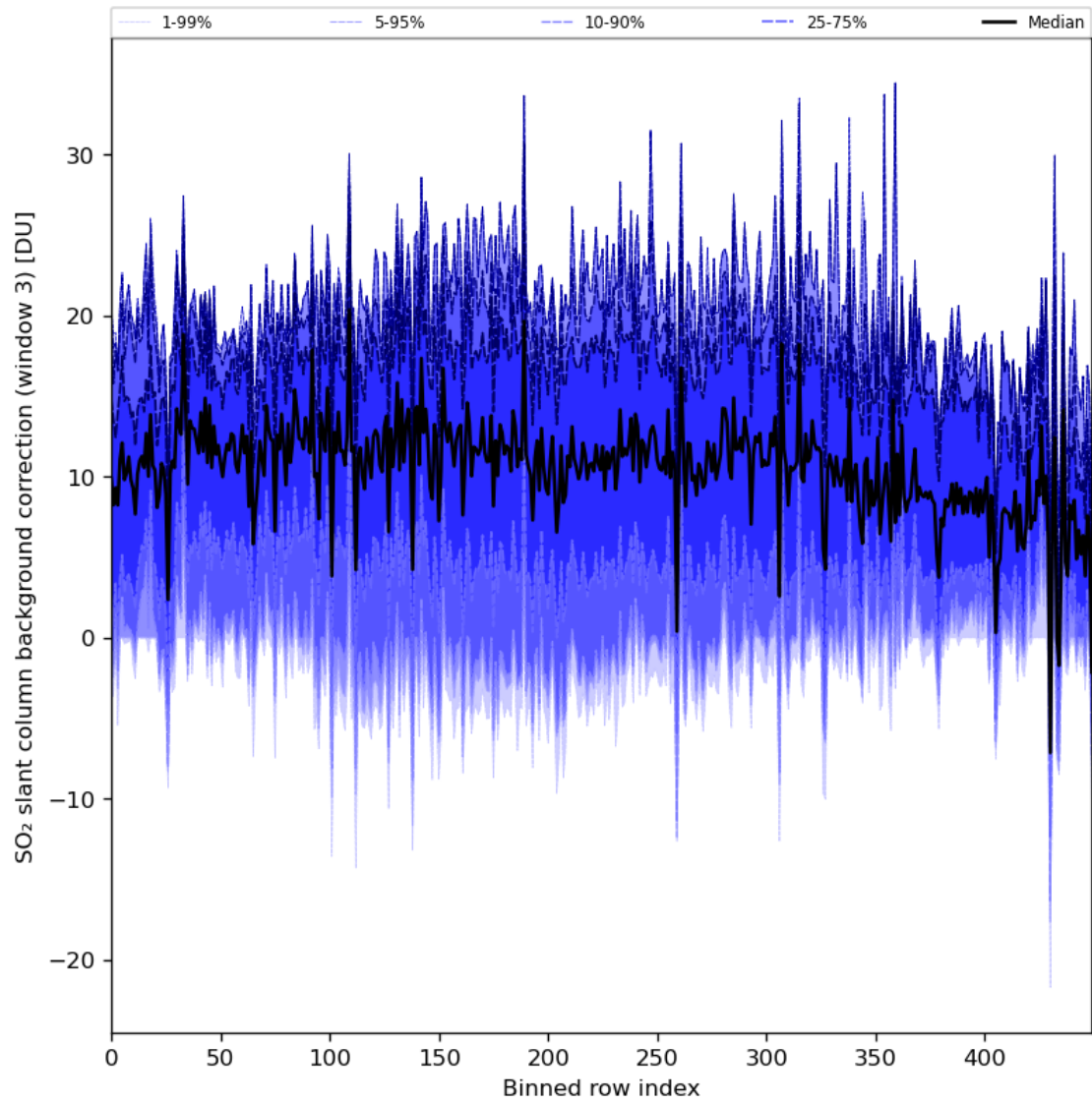
Figure 90: Along track statistics of “SO 2 slant column background correction (window 3)” for 2024-01-06 to 2024-01-08
