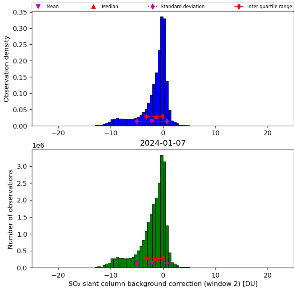
Figure 63: Histogram of “SO 2 slant column background correction (window 2)” for 2024-01-06 to 2024-01-08
