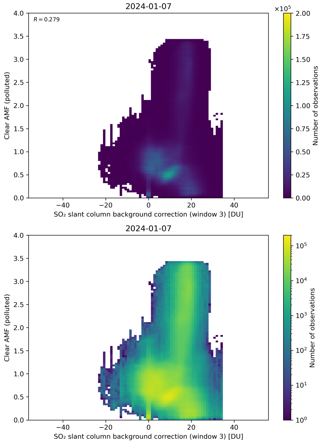
Figure 124: Scatter density plot of “SO 2 slant column background correction (window 3)” against “Clear AMF (polluted)” for 2024-01-06 to 2024-01-08.
