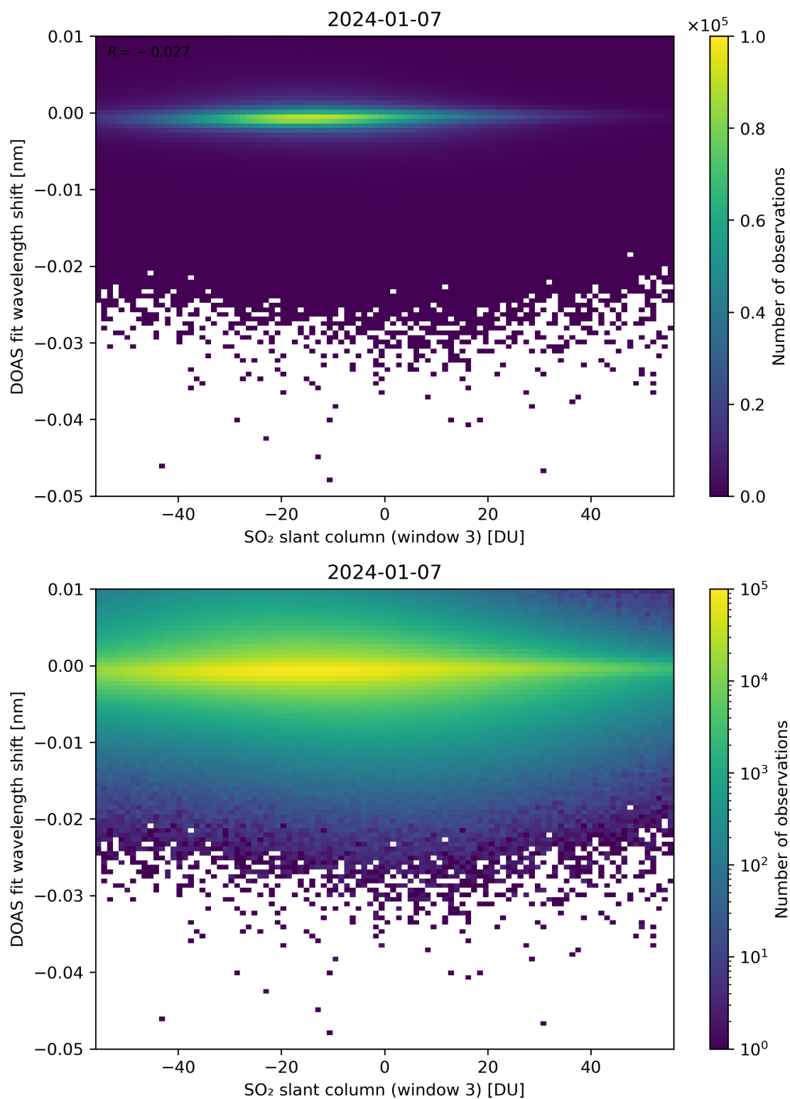
Figure 254: Scatter density plot of “SO 2 slant column (window 3)” against “DOAS fit wavelength shift” for 2024-01-06 to 2024-01-08.
