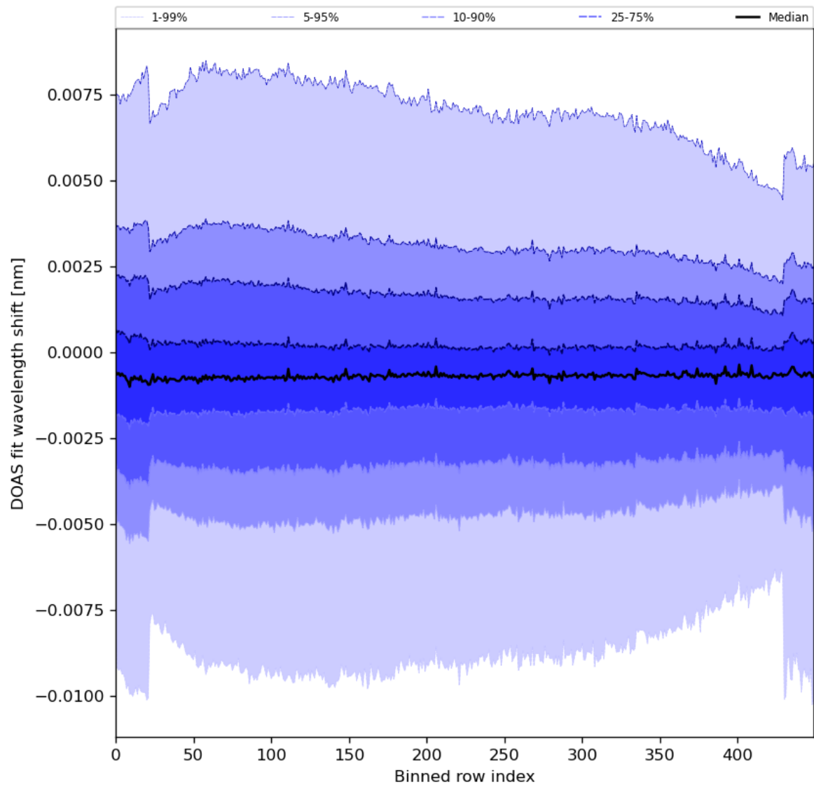
Figure 91: Along track statistics of “DOAS fit wavelength shift” for 2024-01-06 to 2024-01-08
