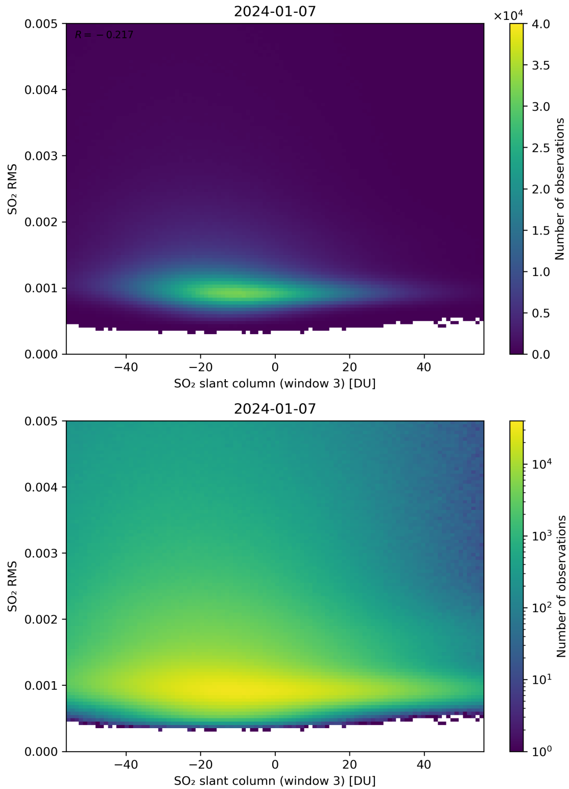
Figure 256: Scatter density plot of “SO 2 slant column (window 3)” against “SO 2 RMS” for 2024-01-06 to 2024-01-08.
