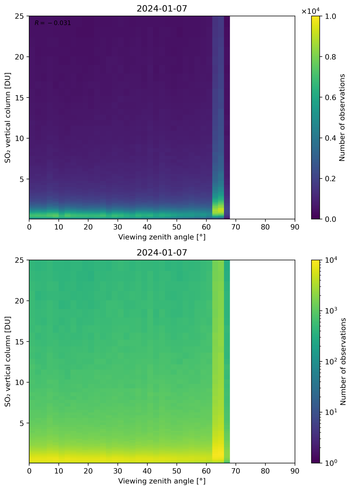
Figure 327: Scatter density plot of “Viewing zenith angle” against “SO 2 vertical column” for 2024-01-06 to 2024-01-08.
