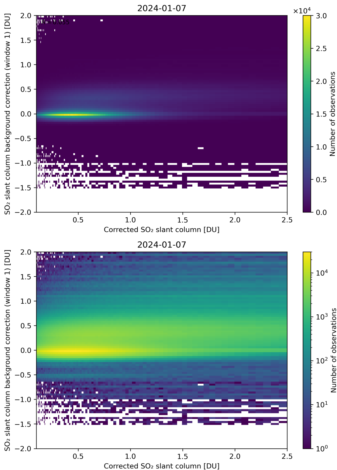
Figure 178: Scatter density plot of “Corrected SO 2 slant column” against “SO 2 slant column background correction (window 1)” for 2024-01-06 to 2024-01-08.
