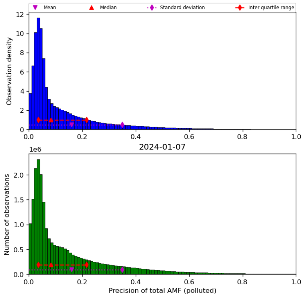
Figure 72: Histogram of “Precision of total AMF (polluted)” for 2024-01-06 to 2024-01-08
