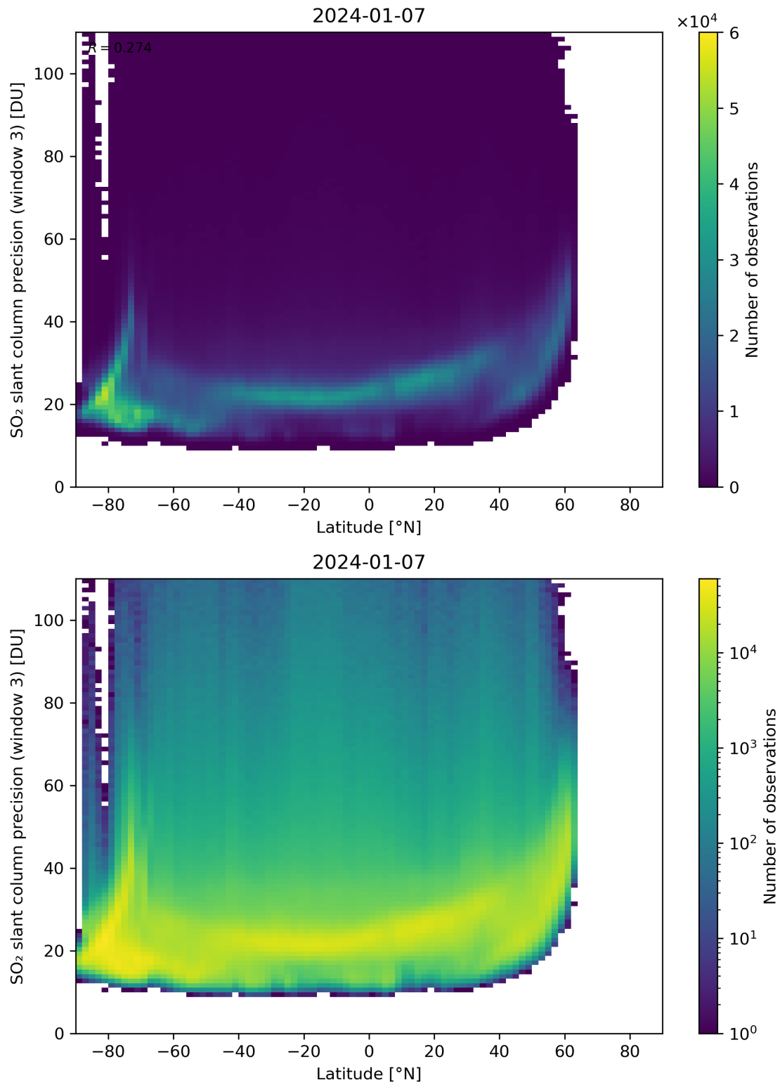
Figure 153: Scatter density plot of “Latitude” against “SO 2 slant column precision (window 3)” for 2024-01-06 to 2024-01-08.
