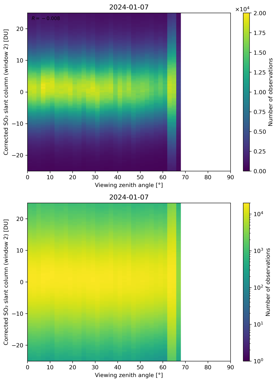
Figure 318: Scatter density plot of “Viewing zenith angle” against “Corrected SO 2 slant column (window 2)” for 2024-01-06 to 2024-01-08.
