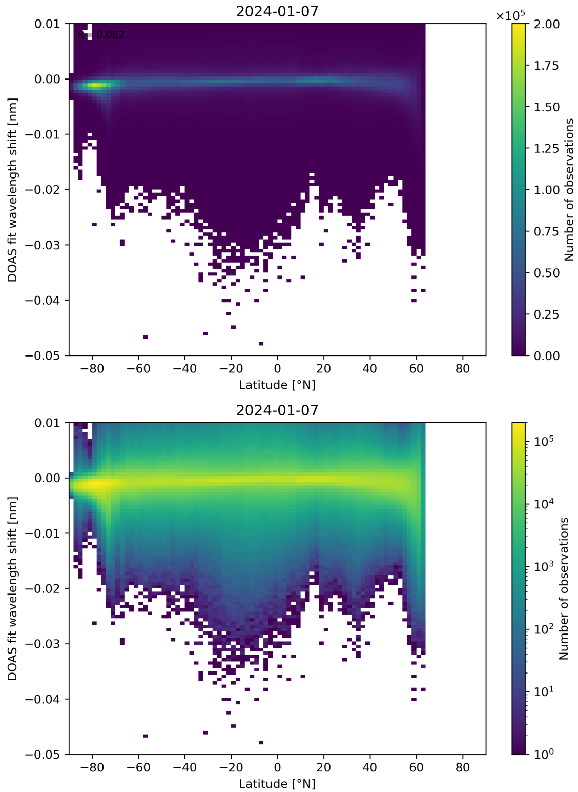
Figure 142: Scatter density plot of “Latitude” against “DOAS fit wavelength shift” for 2024-01-06 to 2024-01-08.
