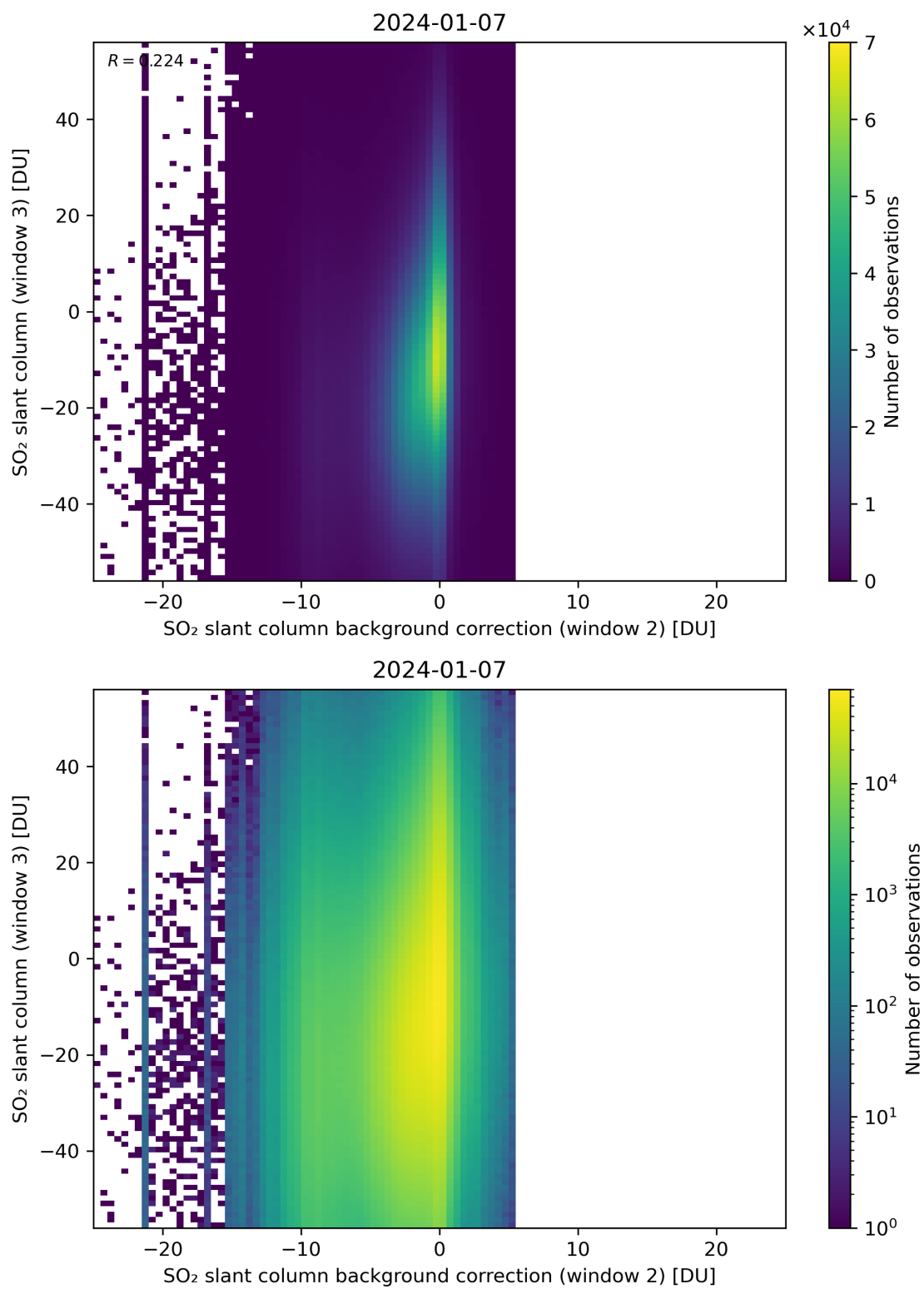
Figure 117: Scatter density plot of “SO 2 slant column background correction (window 2)” against “SO 2 slant column (window 3)” for 2024-01-06 to 2024-01-08.
