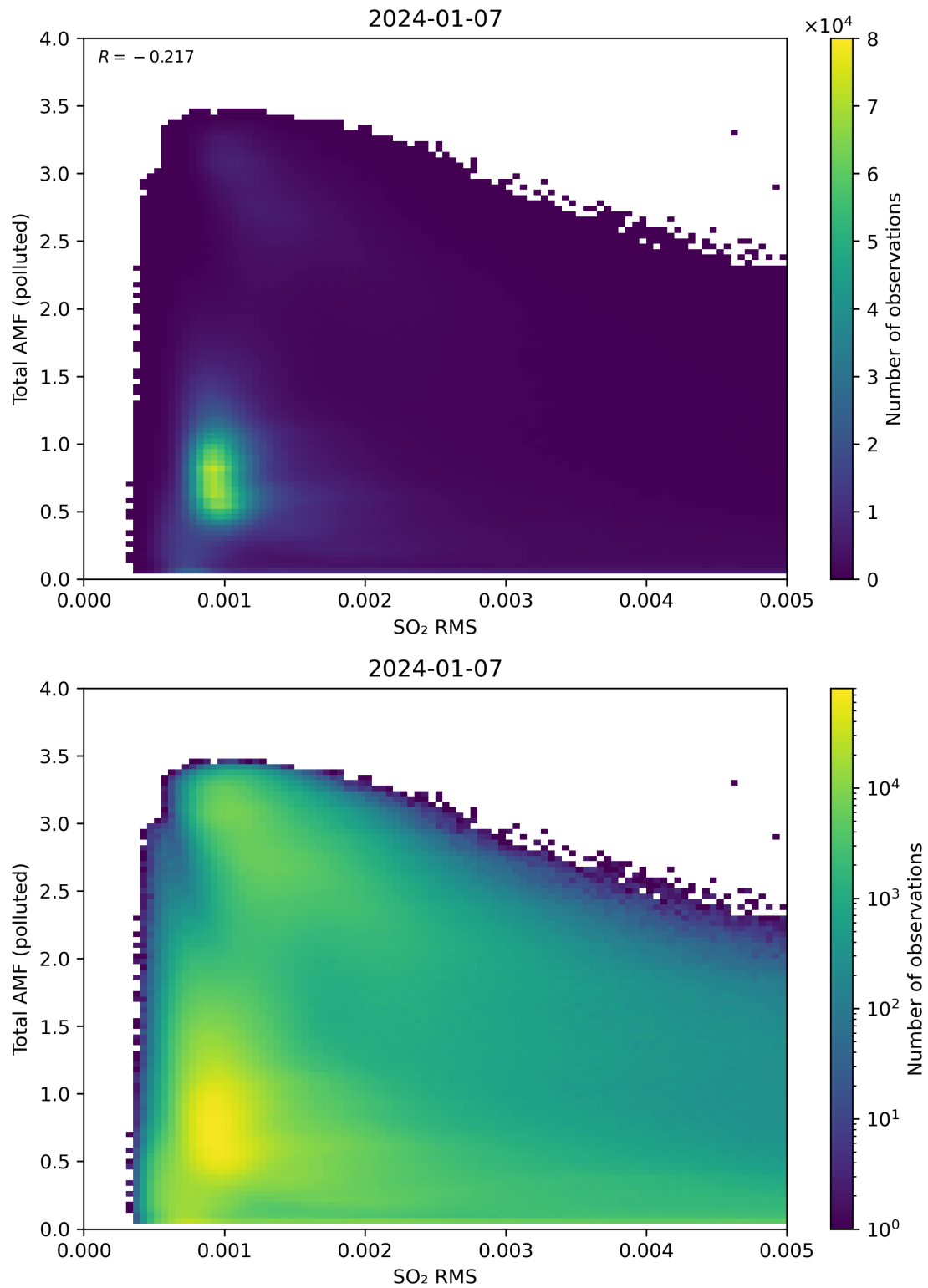
Figure 137: Scatter density plot of “SO 2 RMS” against “Total AMF (polluted)” for 2024-01-06 to 2024-01-08.
