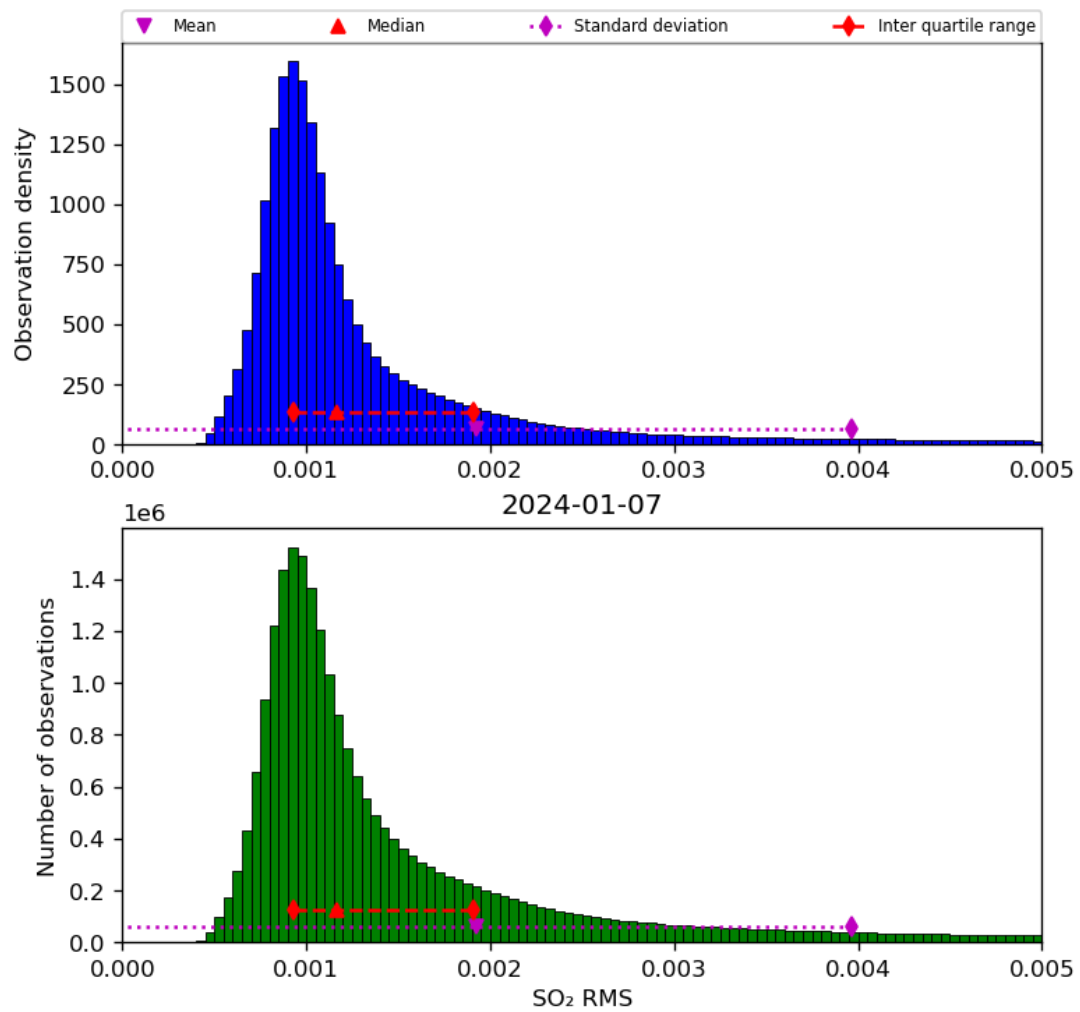
Figure 70: Histogram of “SO 2 RMS” for 2024-01-06 to 2024-01-08
