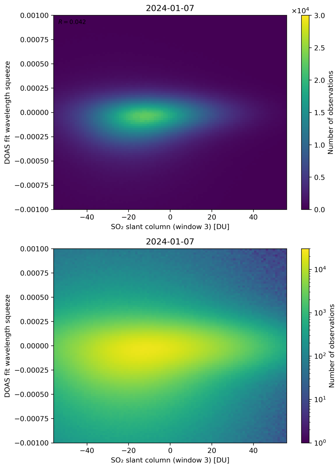
Figure 255: Scatter density plot of “SO 2 slant column (window 3)” against “DOAS fit wavelength squeeze” for 2024-01-06 to 2024-01-08.
