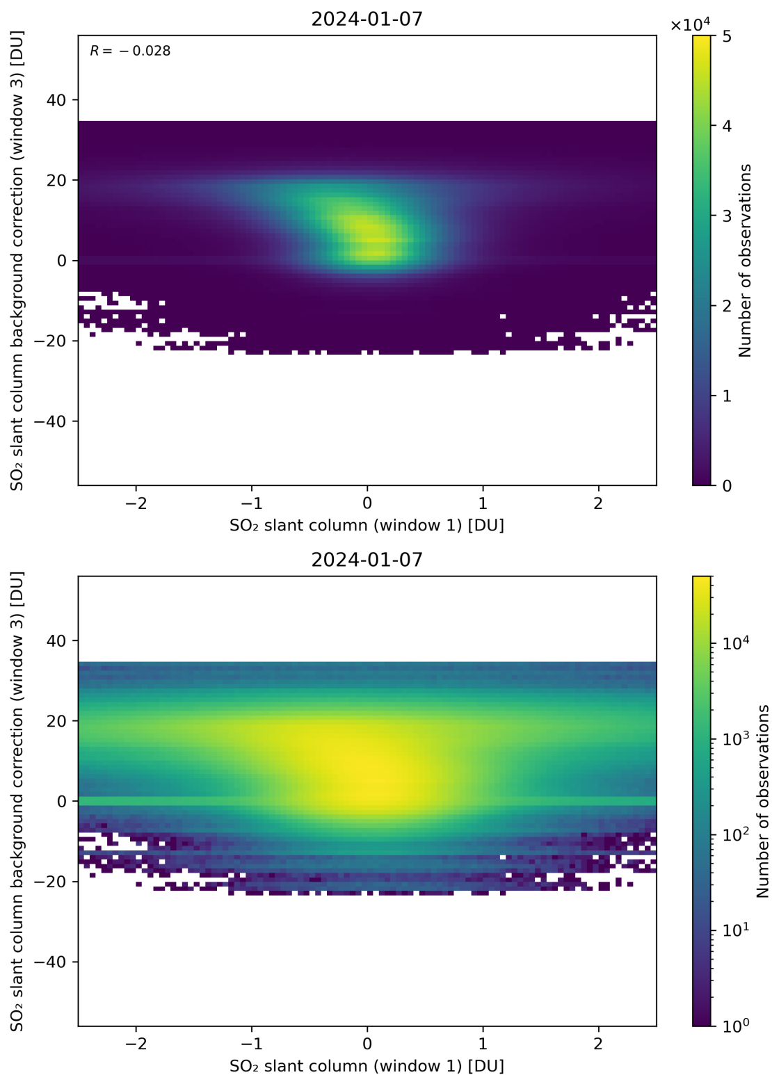
Figure 214: Scatter density plot of “SO 2 slant column (window 1)” against “SO 2 slant column background correction (window 3)” for 2024-01-06 to 2024-01-08.
