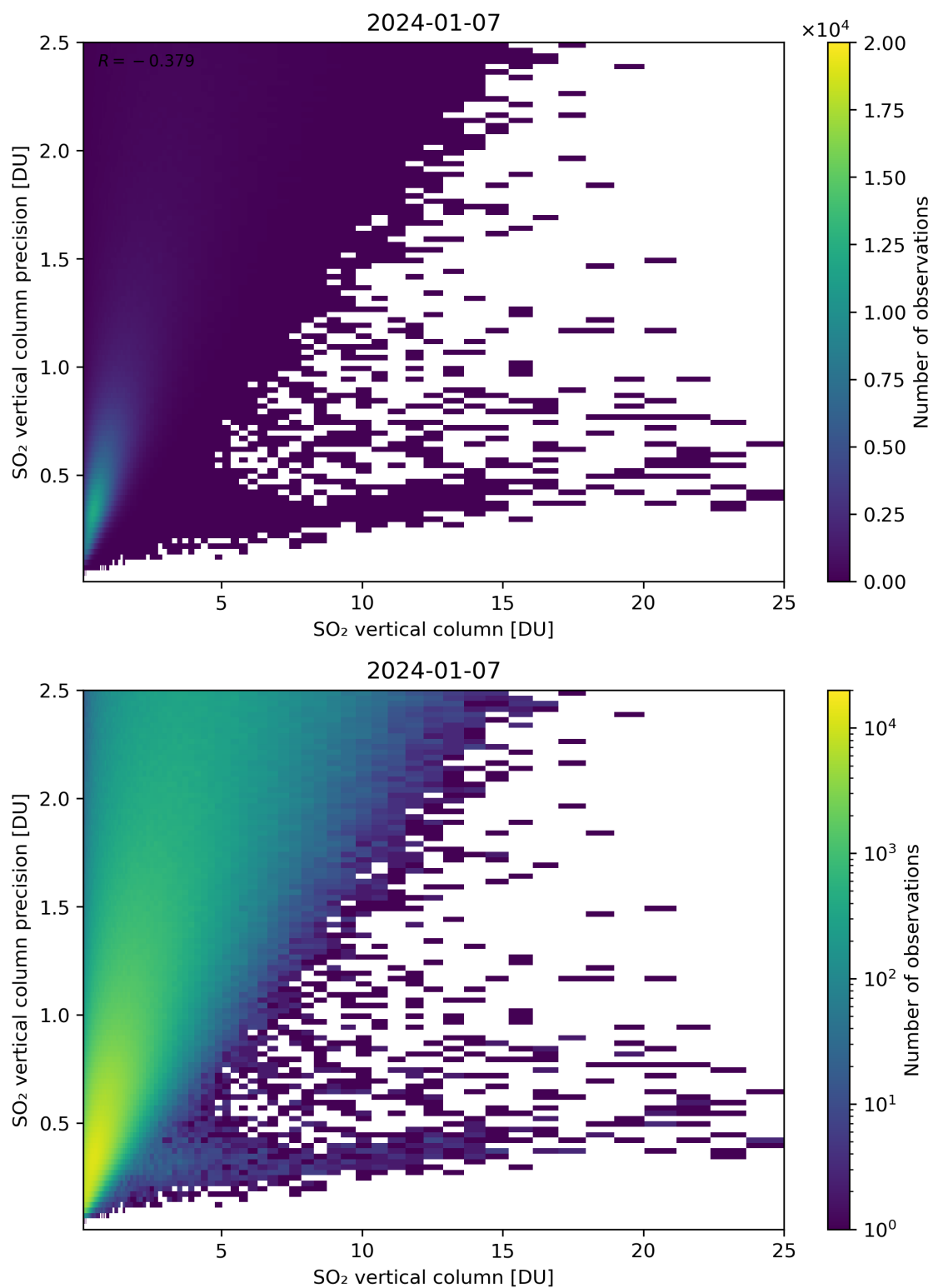
Figure 307: Scatter density plot of “SO 2 vertical column” against “SO 2 vertical column precision” for 2024-01-06 to 2024-01-08.
