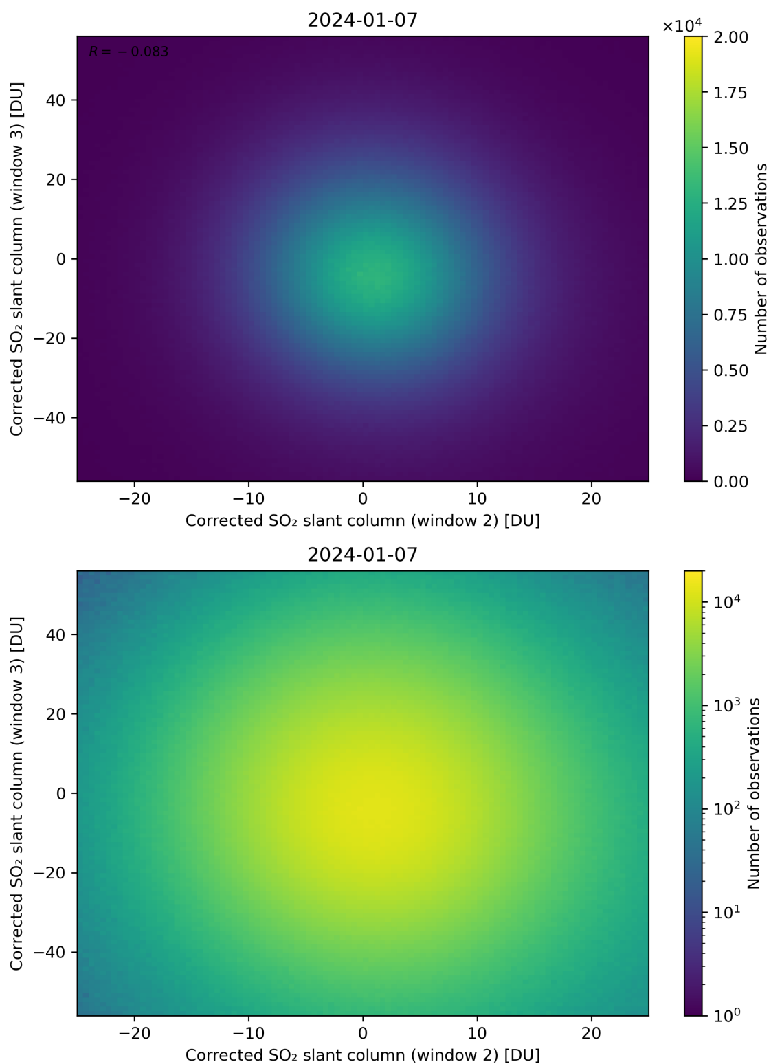
Figure 200: Scatter density plot of “Corrected SO 2 slant column (window 2)” against “Corrected SO 2 slant column (window 3)” for 2024-01-06 to 2024-01-08.
