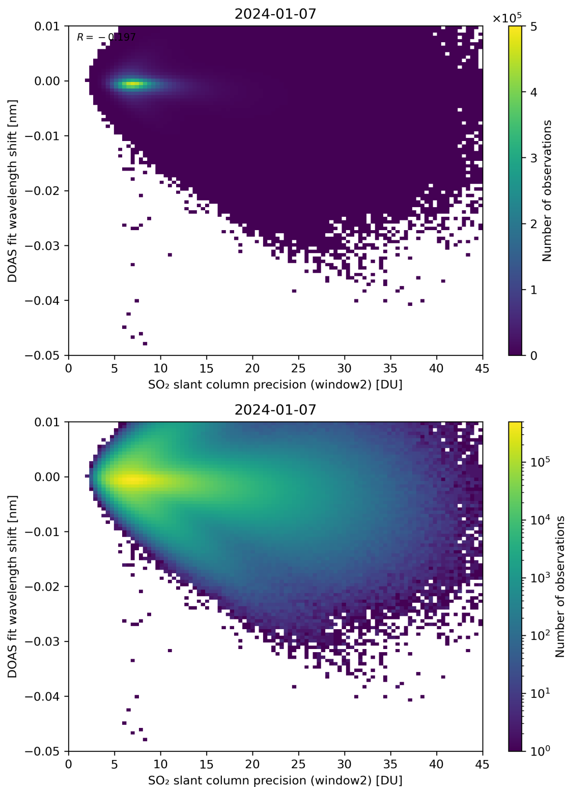
Figure 243: Scatter density plot of “SO 2 slant column precision (window2)” against “DOAS fit wavelength shift” for 2024-01-06 to 2024-01-08.
