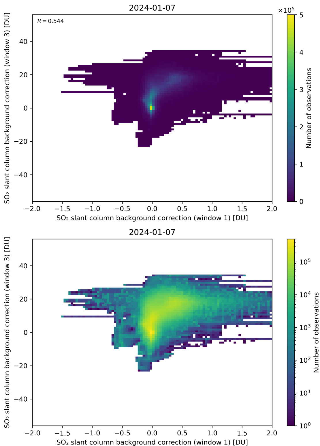
Figure 99: Scatter density plot of “SO 2 slant column background correction (window 1)” against “SO 2 slant column background correction (window 3)” for 2024-01-06 to 2024-01-08.
