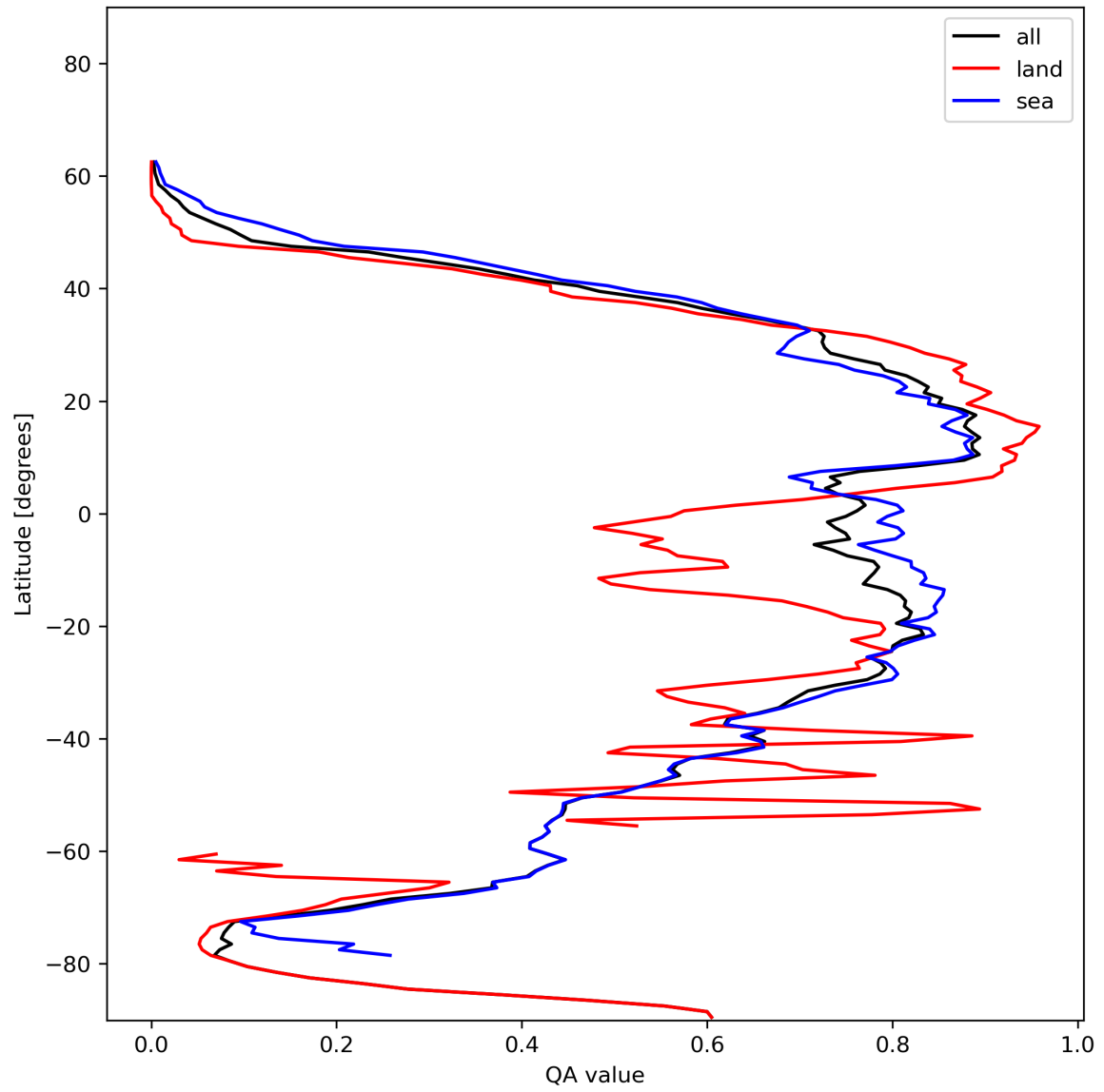
Figure 29: Zonal average of “QA value” for 2024-01-06 to 2024-01-08.
