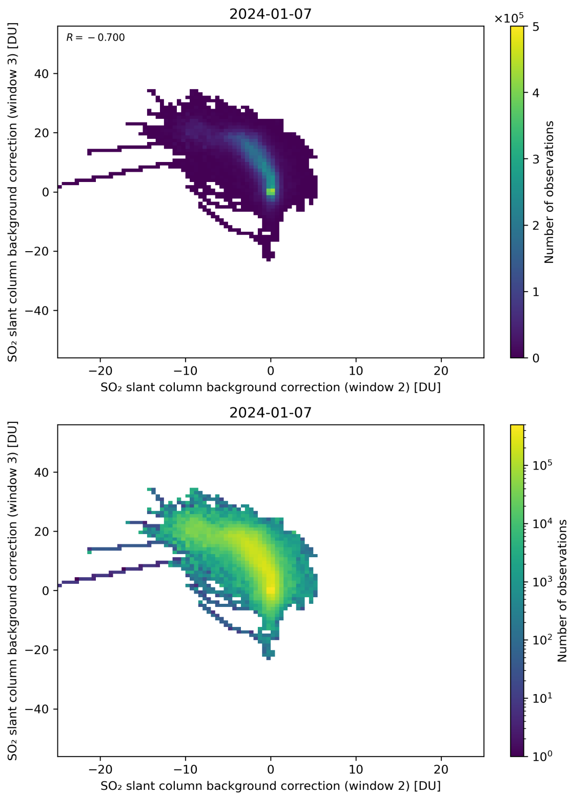
Figure 111: Scatter density plot of “SO 2 slant column background correction (window 2)” against “SO 2 slant column background correction (window 3)” for 2024-01-06 to 2024-01-08.
