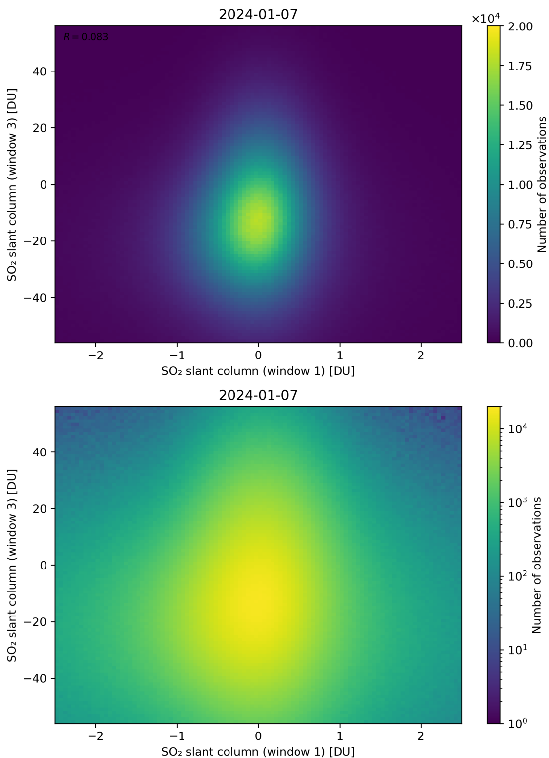
Figure 237: Scatter density plot of “SO 2 slant column (window 1)” against “SO 2 slant column (window 3)” for 2024-01-06 to 2024-01-08.
