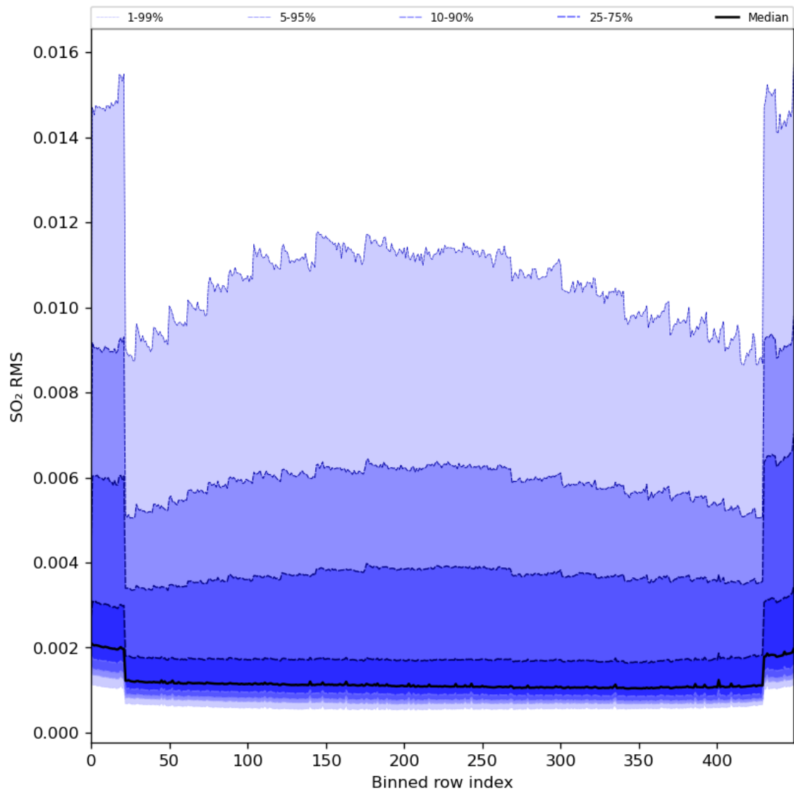
Figure 93: Along track statistics of “SO 2 RMS” for 2024-01-06 to 2024-01-08
