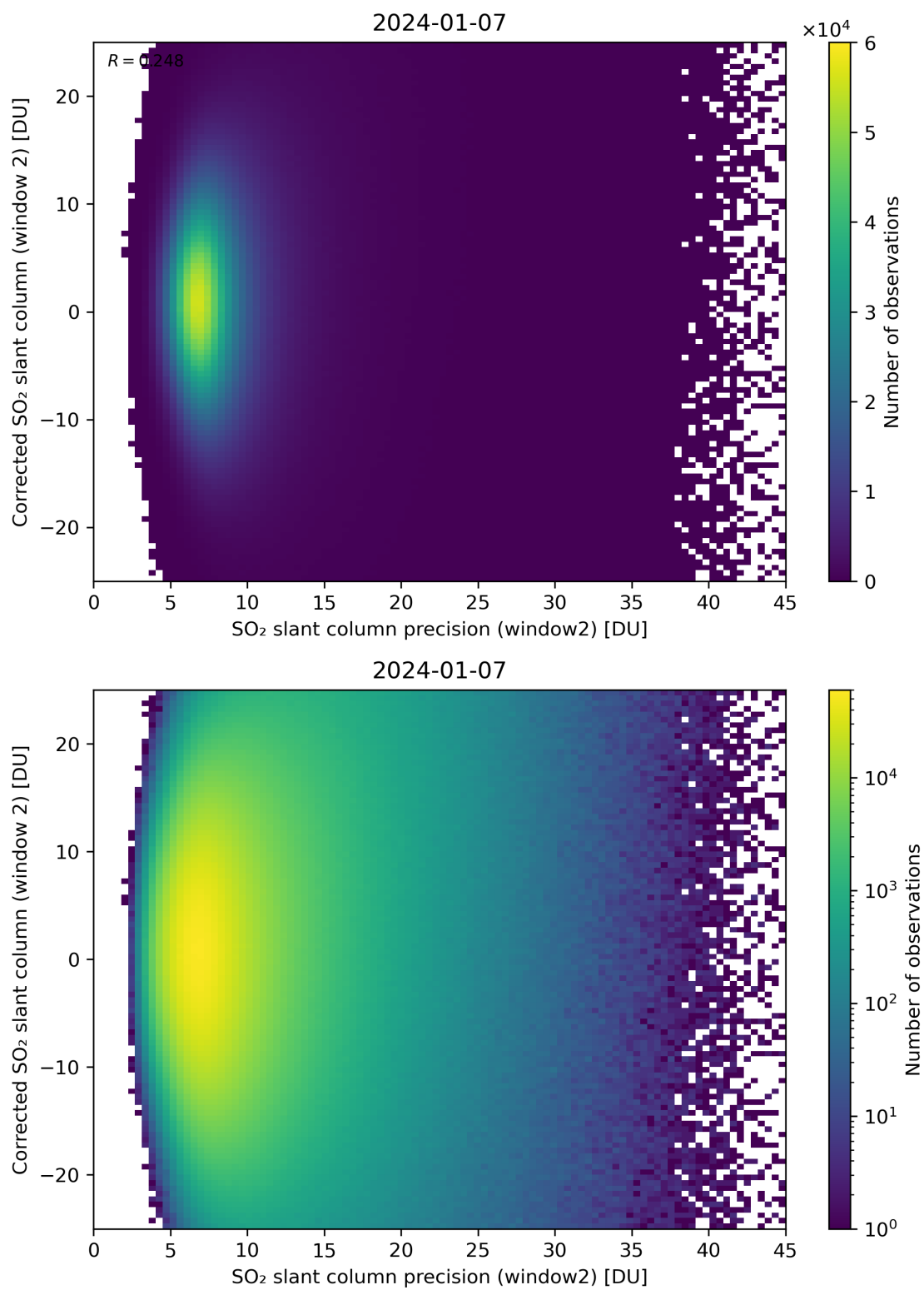
Figure 247: Scatter density plot of “SO 2 slant column precision (window2)” against “Corrected SO 2 slant column (window 2)” for 2024-01-06 to 2024-01-08.
