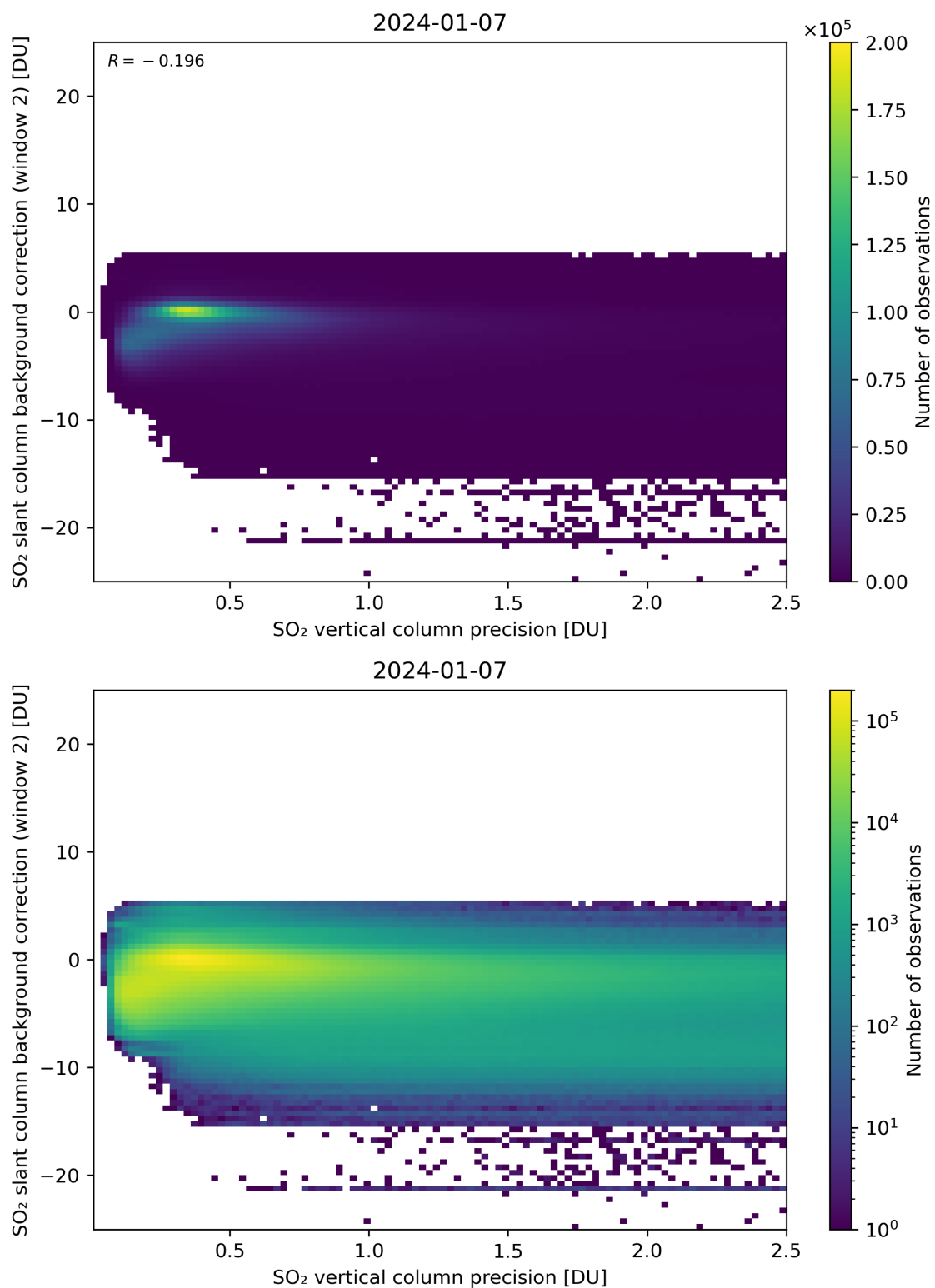
Figure 280: Scatter density plot of “SO 2 vertical column precision” against “SO 2 slant column background correction (window 2)” for 2024-01-06 to 2024-01-08.
