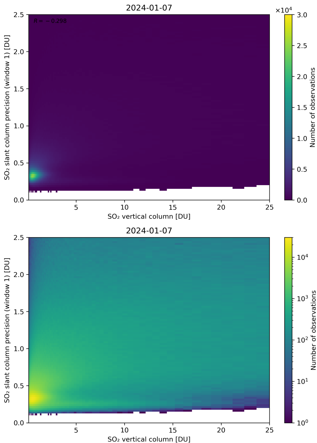
Figure 301: Scatter density plot of “SO 2 vertical column” against “SO 2 slant column precision (window 1)” for 2024-01-06 to 2024-01-08.
