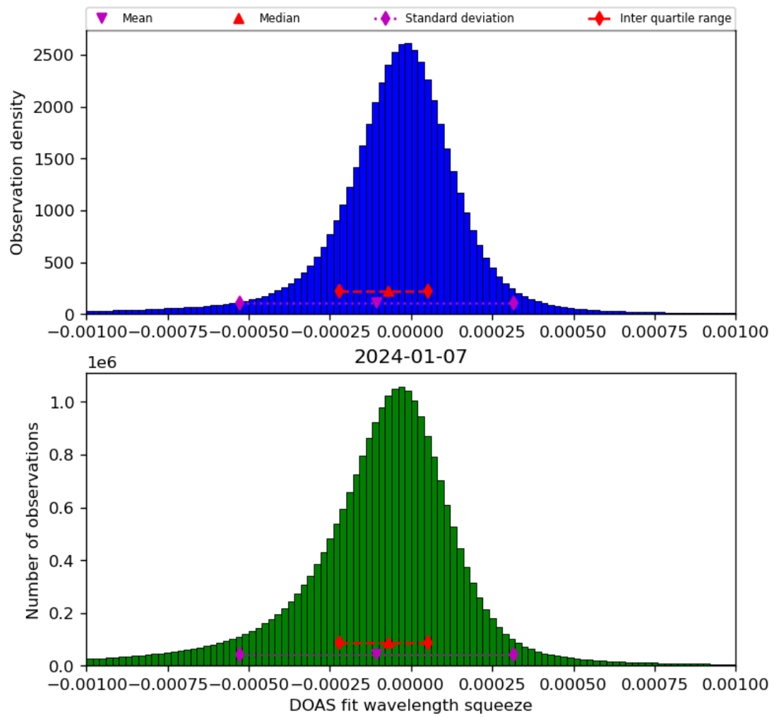
Figure 69: Histogram of “DOAS fit wavelength squeeze” for 2024-01-06 to 2024-01-08
