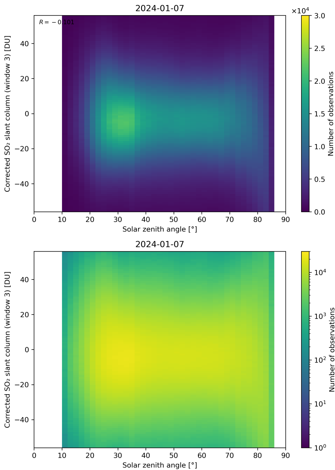
Figure 168: Scatter density plot of “Solar zenith angle” against “Corrected SO 2 slant column (window 3)” for 2024-01-06 to 2024-01-08.
