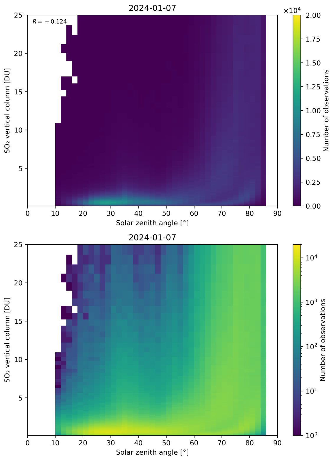
Figure 176: Scatter density plot of “Solar zenith angle” against “SO 2 vertical column” for 2024-01-06 to 2024-01-08.
