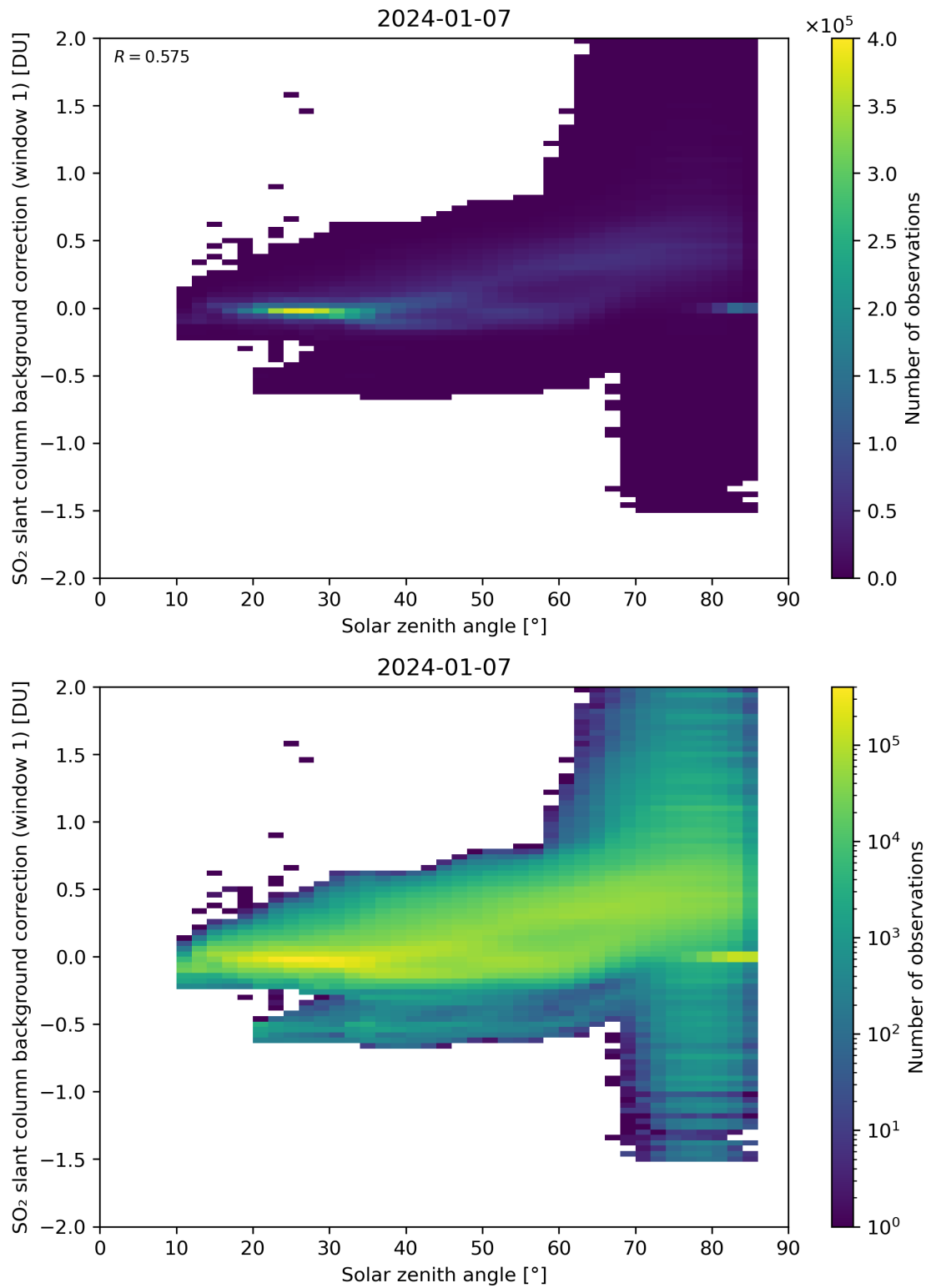
Figure 158: Scatter density plot of “Solar zenith angle” against “SO 2 slant column background correction (window 1)” for 2024-01-06 to 2024-01-08.
