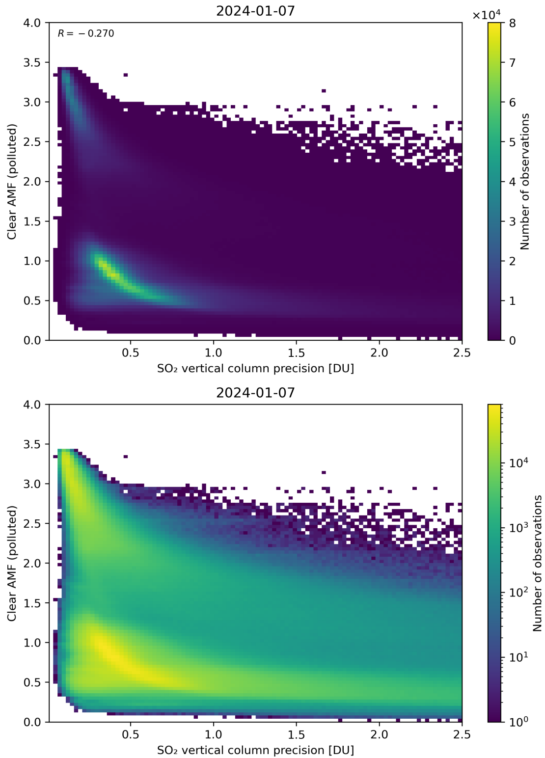
Figure 285: Scatter density plot of “SO 2 vertical column precision” against “Clear AMF (polluted)” for 2024-01-06 to 2024-01-08.
