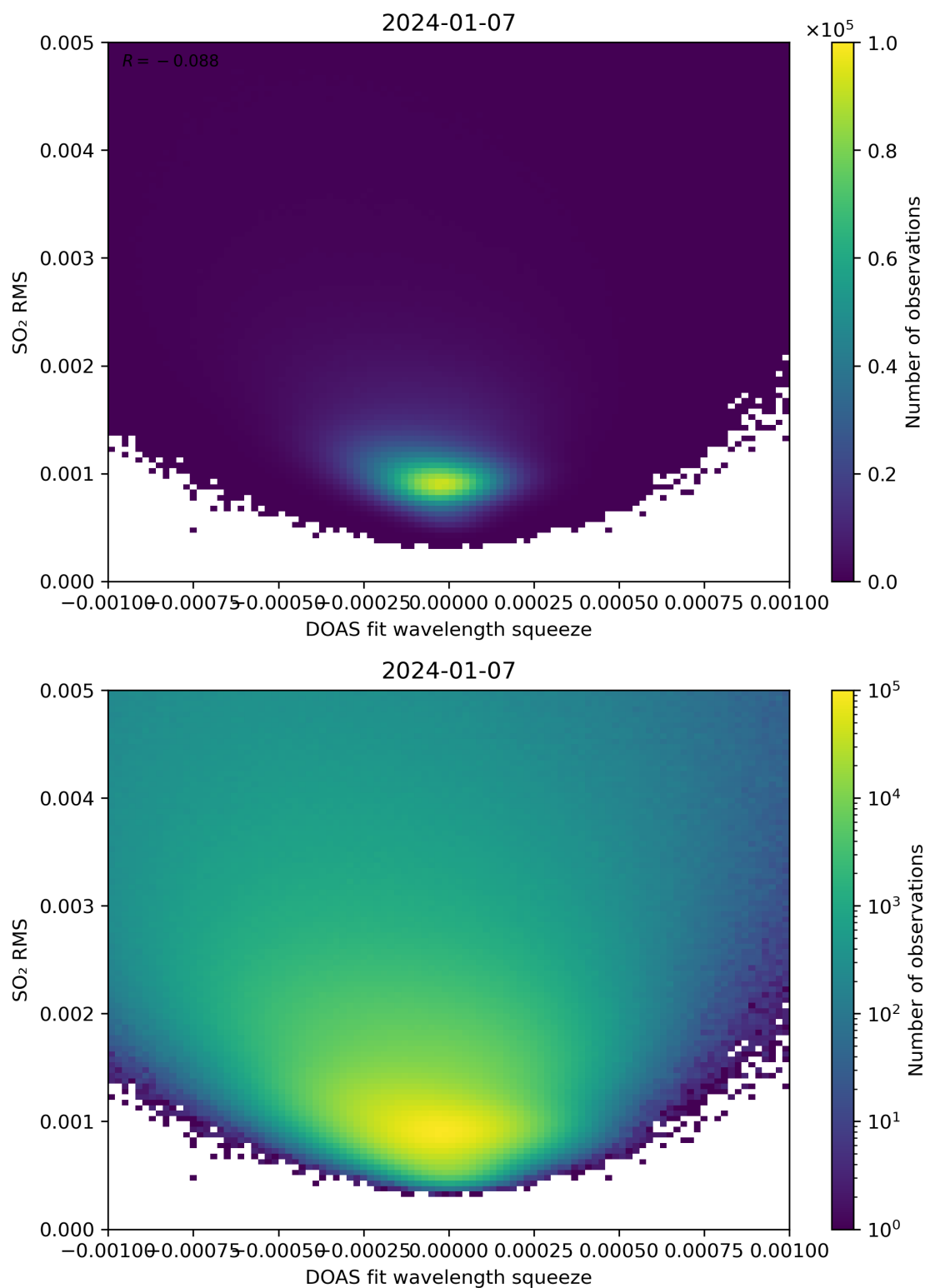
Figure 132: Scatter density plot of “DOAS fit wavelength squeeze” against “SO 2 RMS” for 2024-01-06 to 2024-01-08.
