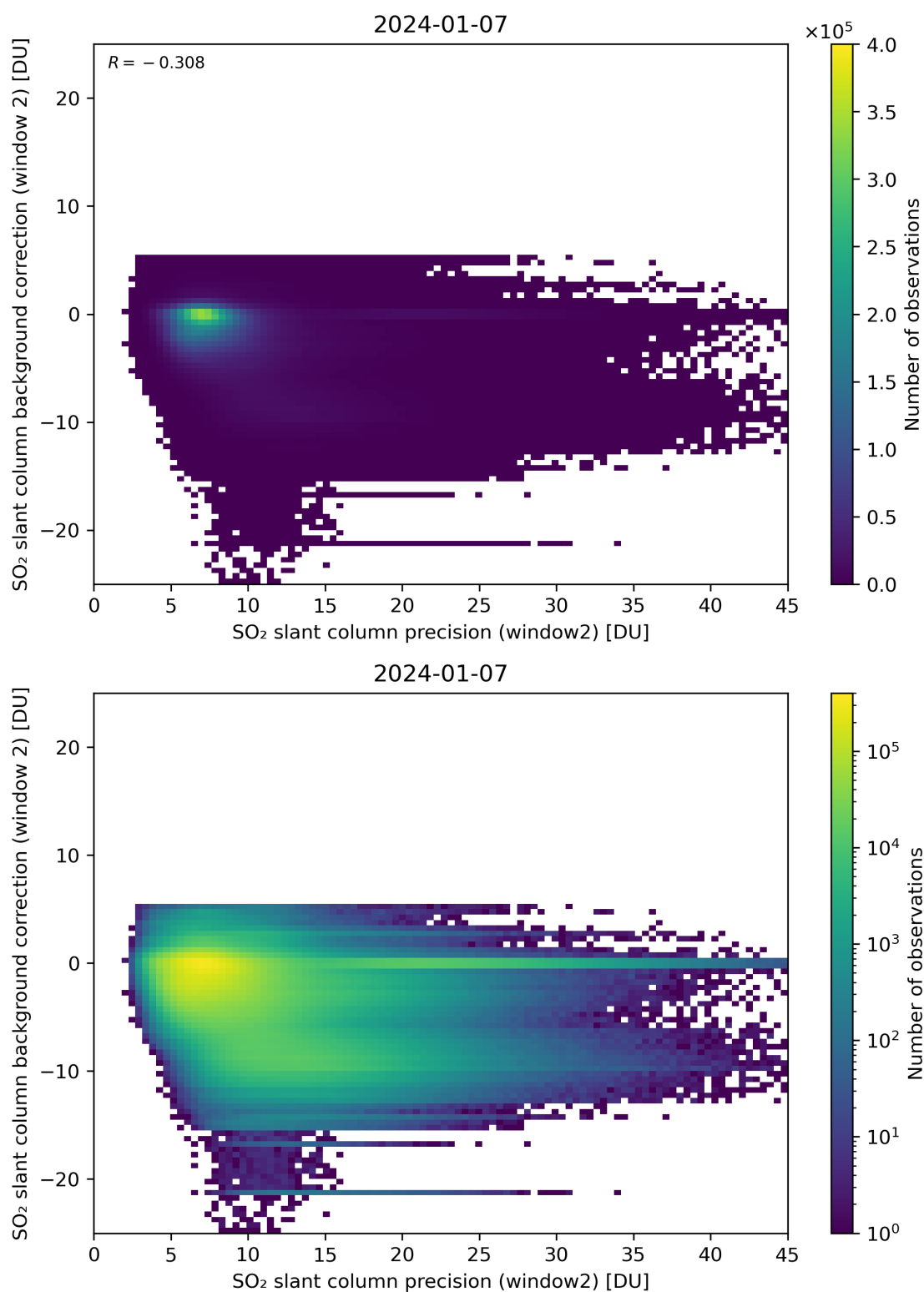
Figure 241: Scatter density plot of “SO 2 slant column precision (window2)” against “SO 2 slant column background correction (window 2)” for 2024-01-06 to 2024-01-08.
