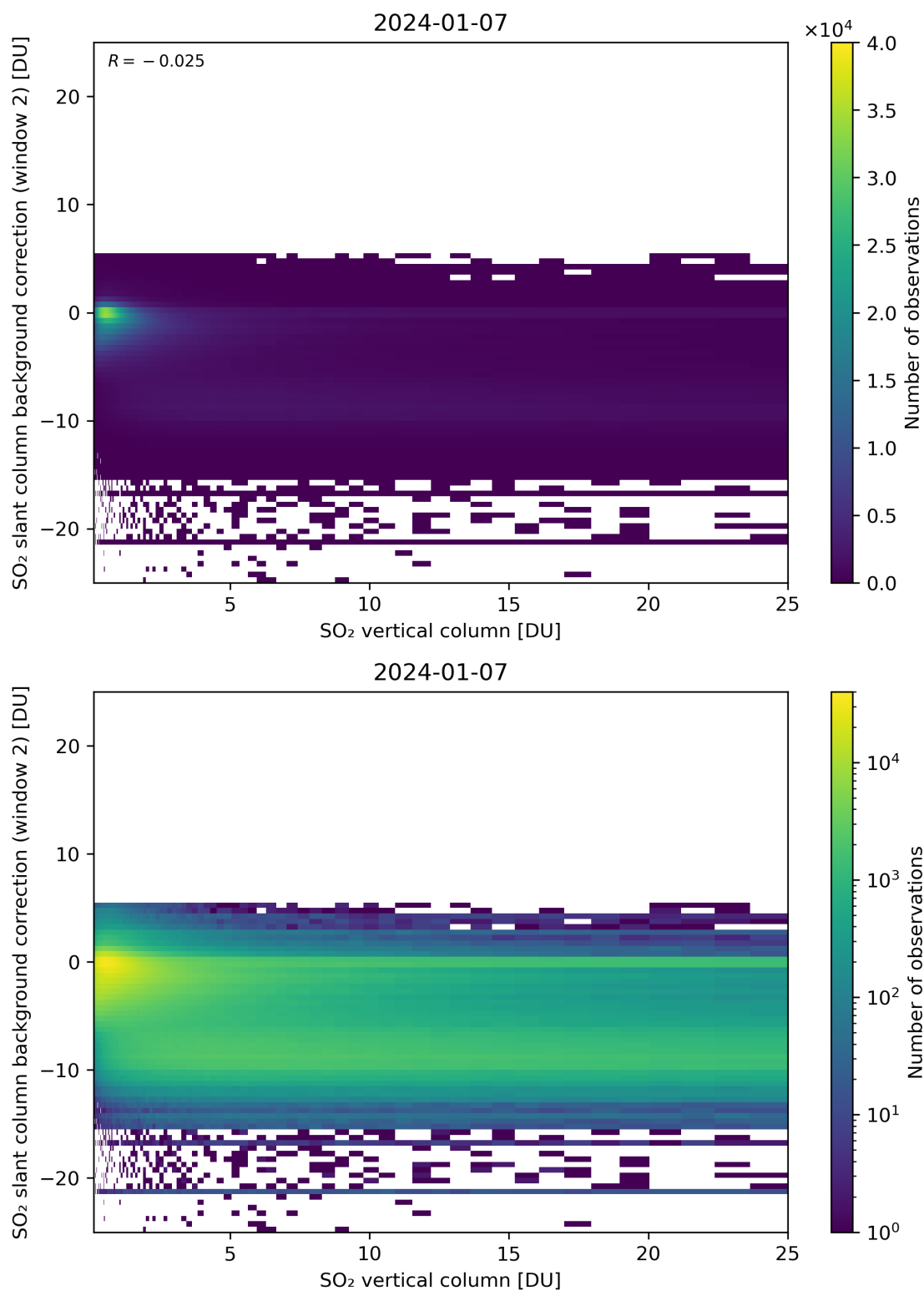
Figure 274: Scatter density plot of “SO 2 vertical column” against “SO 2 slant column background correction (window 2)” for 2024-01-06 to 2024-01-08.
