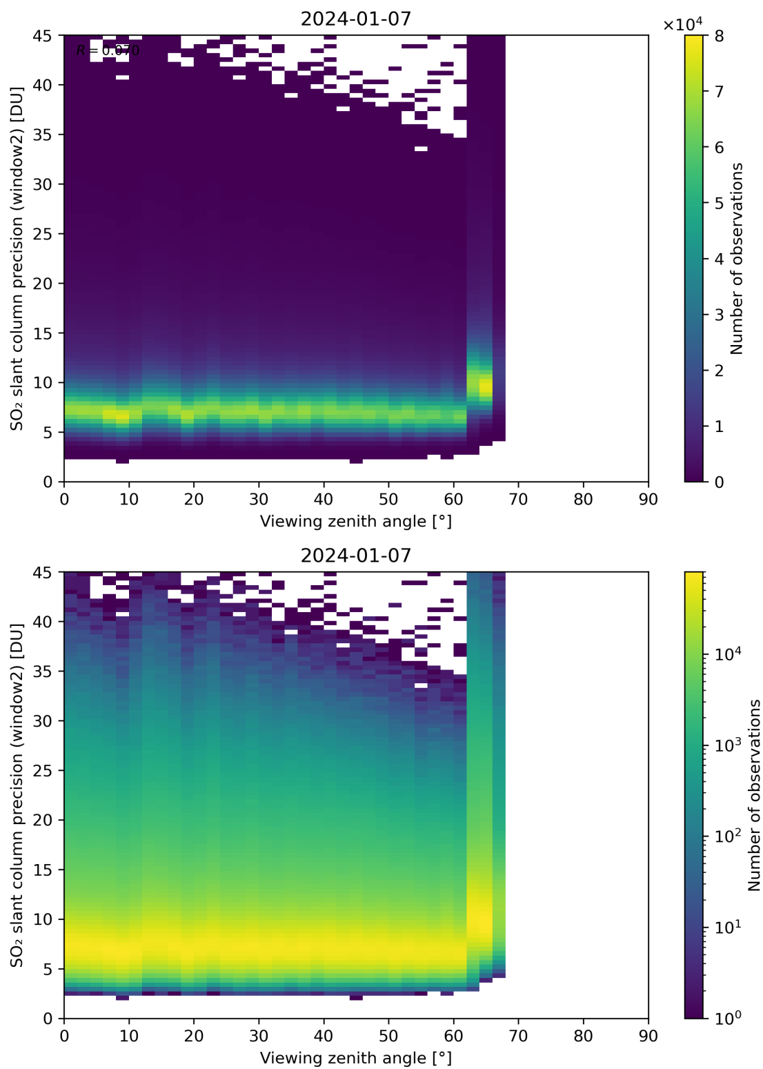
Figure 322: Scatter density plot of “Viewing zenith angle” against “SO 2 slant column precision (window2)” for 2024-01-06 to 2024-01-08.
