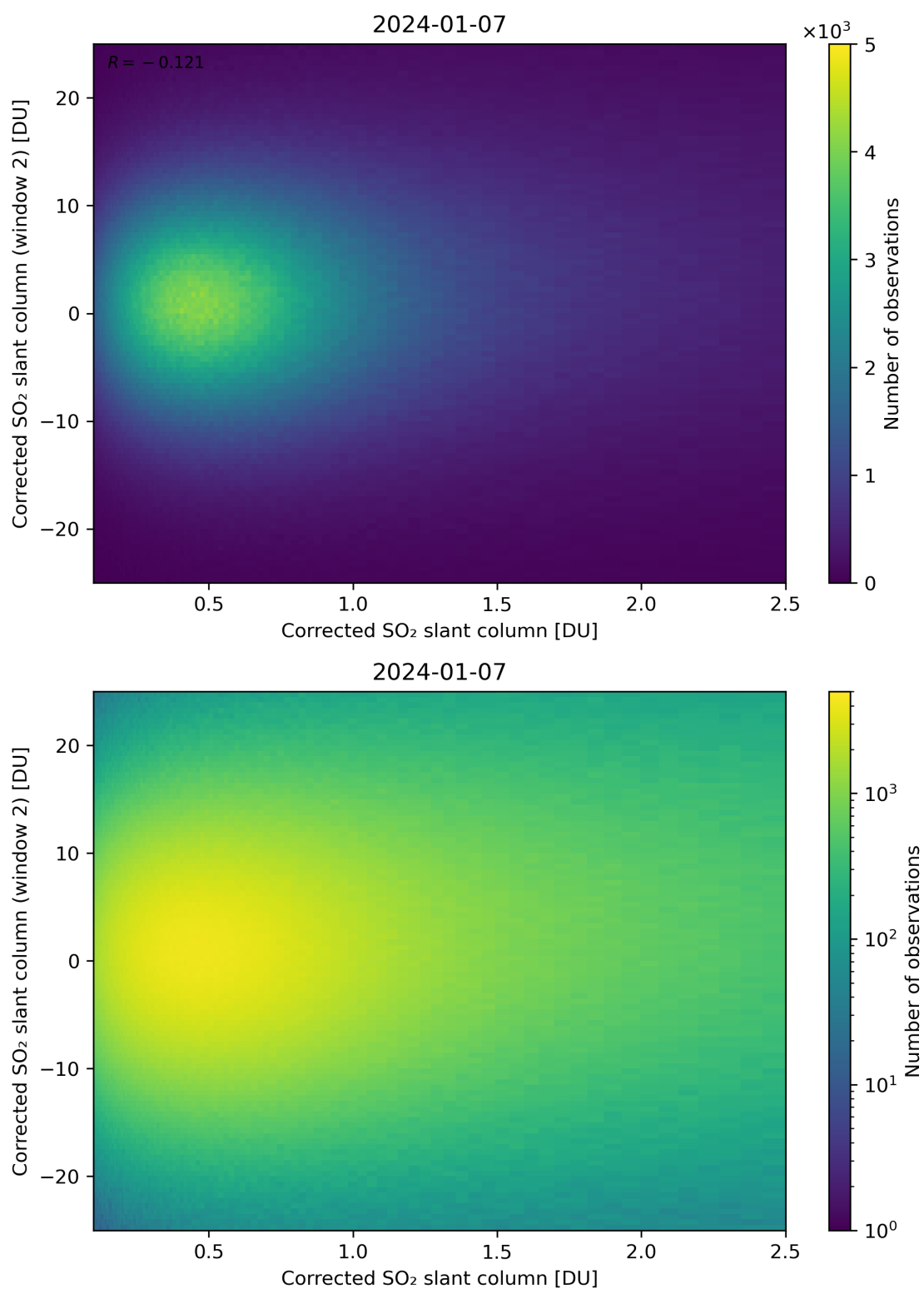
Figure 185: Scatter density plot of “Corrected SO 2 slant column” against “Corrected SO 2 slant column (window 2)” for 2024-01-06 to 2024-01-08.
