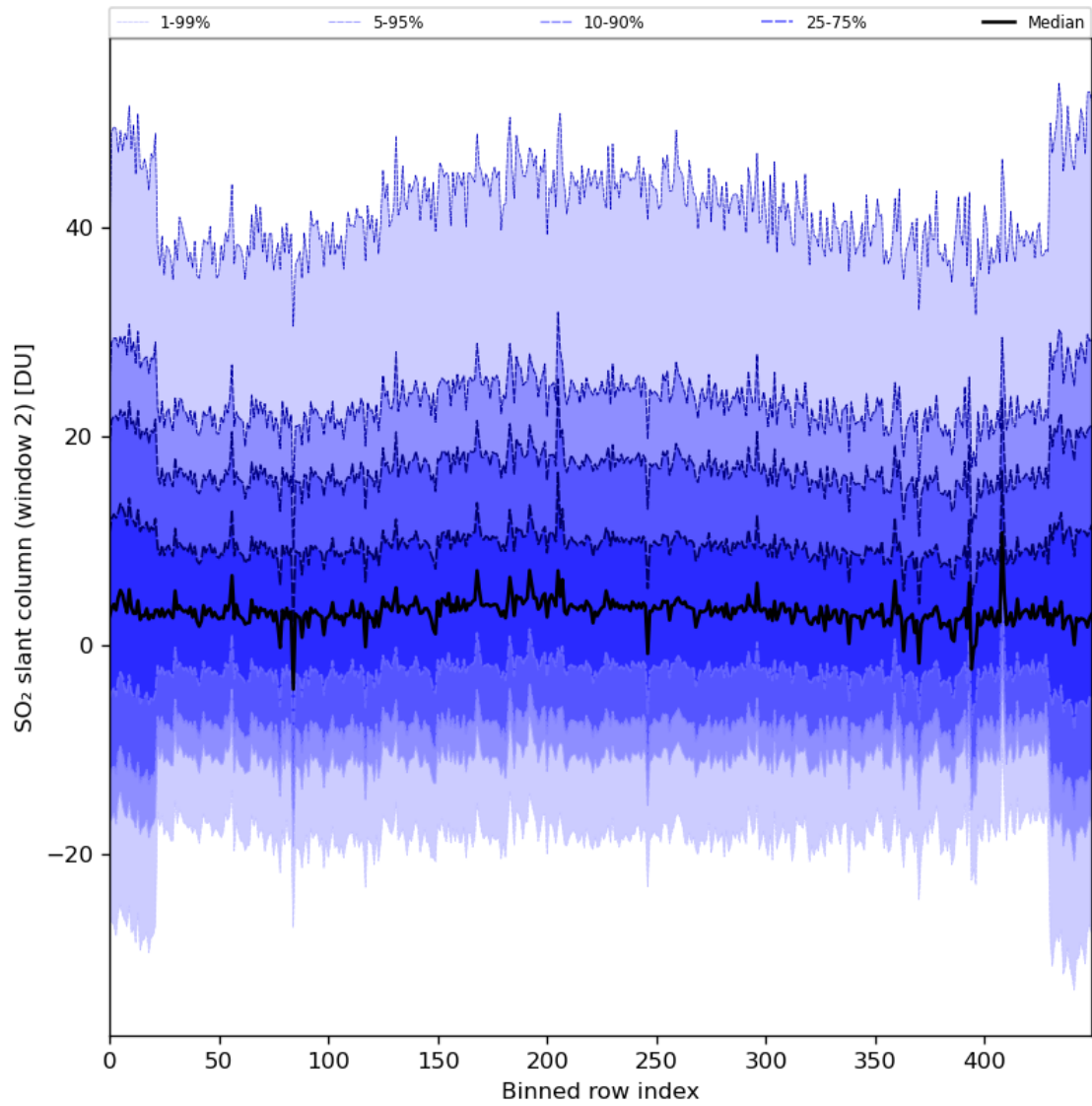
Figure 83: Along track statistics of “SO 2 slant column (window 2)” for 2024-01-06 to 2024-01-08
