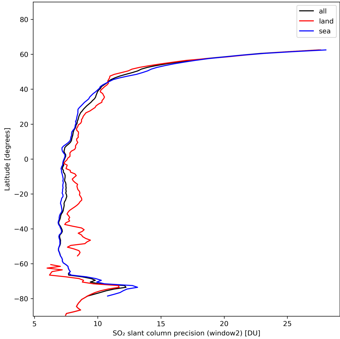
Figure 38: Zonal average of “SO 2 slant column precision (window2)” for 2024-01-06 to 2024-01-08.
