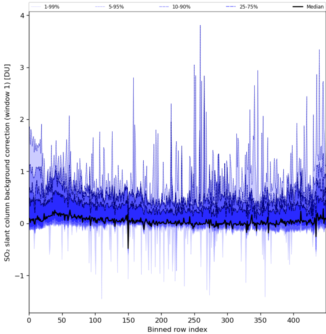
Figure 82: Along track statistics of "SO 2 slant column background correction (window 1)" for 2024-01-06 to 2024-01-08
