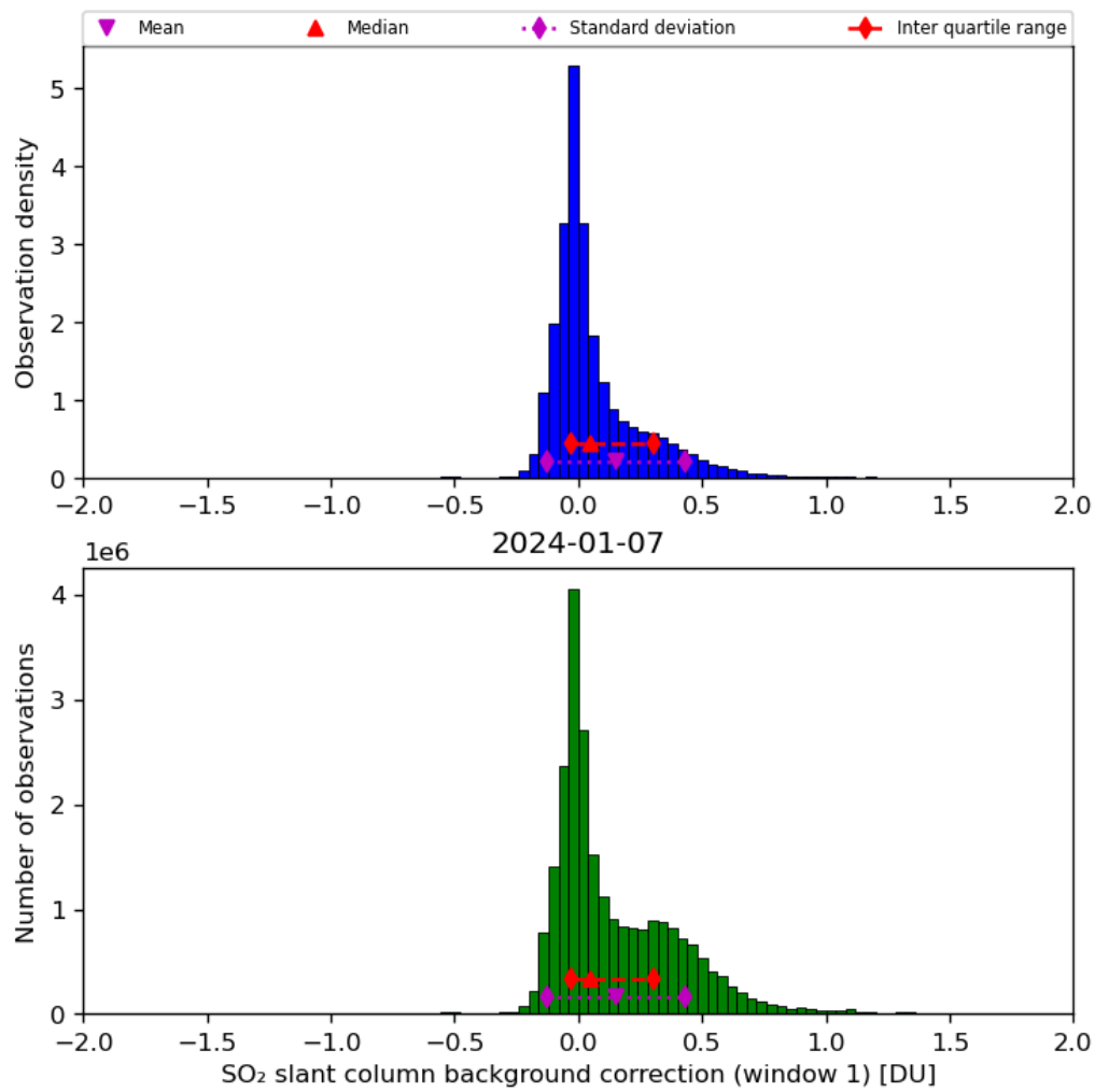
Figure 59: Histogram of “SO 2 slant column background correction (window 1)” for 2024-01-06 to 2024-01-08
