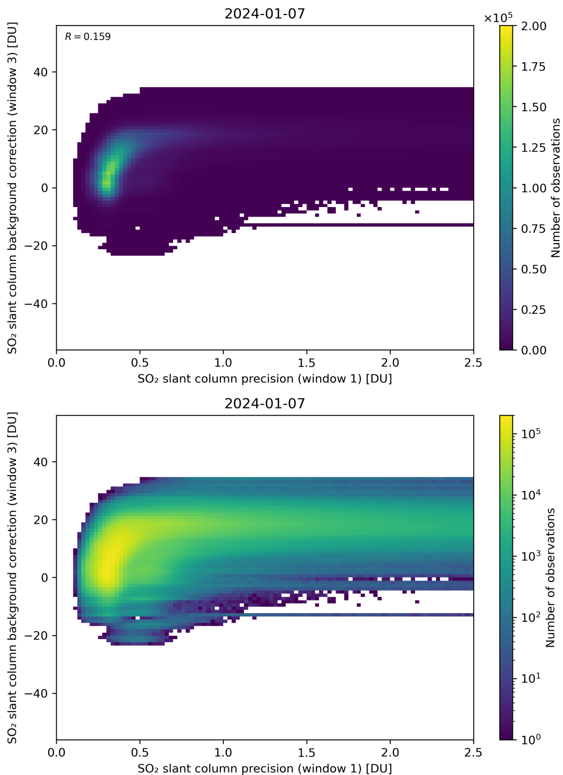
Figure 220: Scatter density plot of “SO 2 slant column precision (window 1)” against “SO 2 slant column background correction (window 3)” for 2024-01-06 to 2024-01-08.
