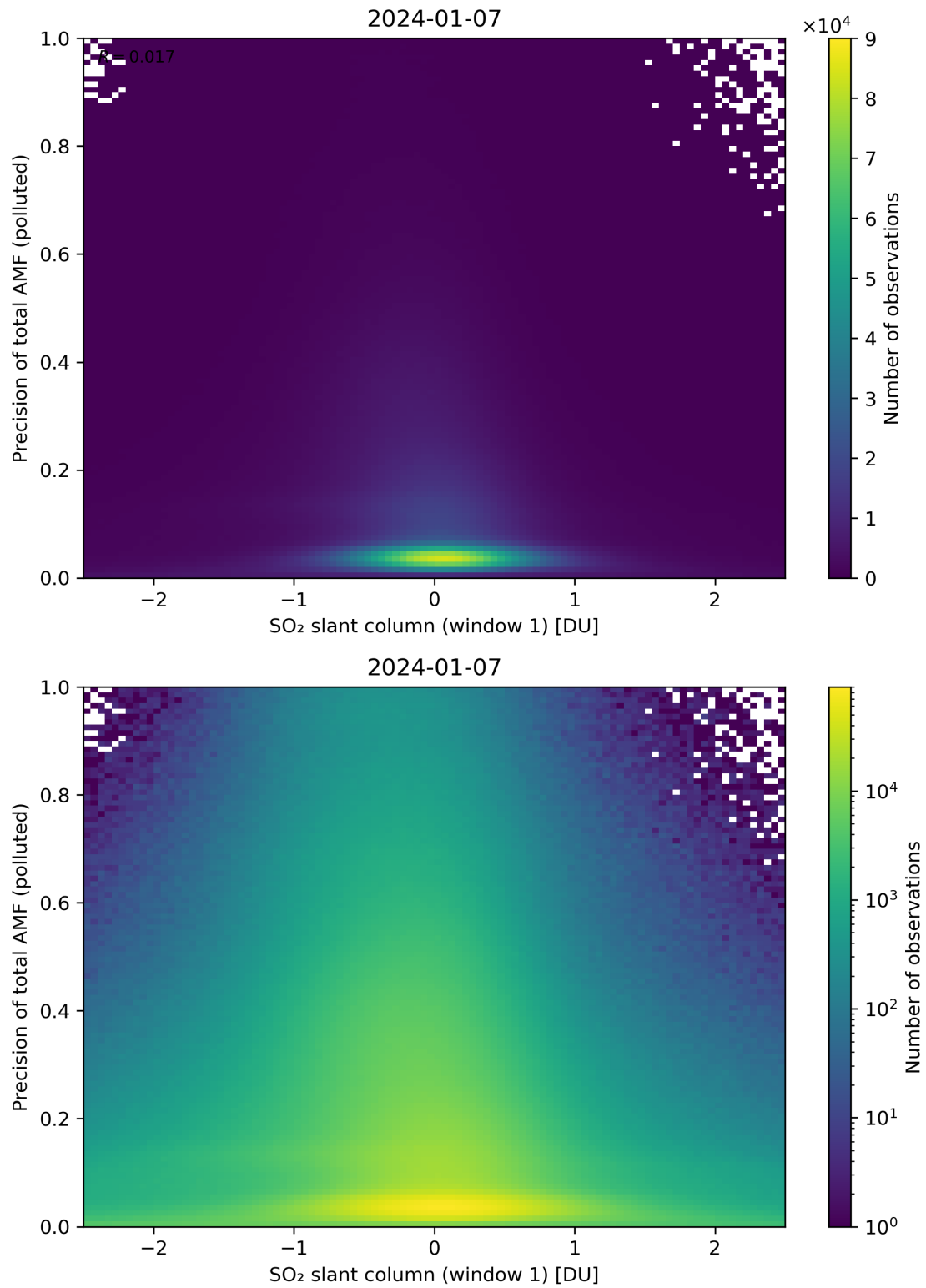
Figure 240: Scatter density plot of “SO 2 slant column (window 1)” against “Precision of total AMF (polluted)” for 2024-01-06 to 2024-01-08.
