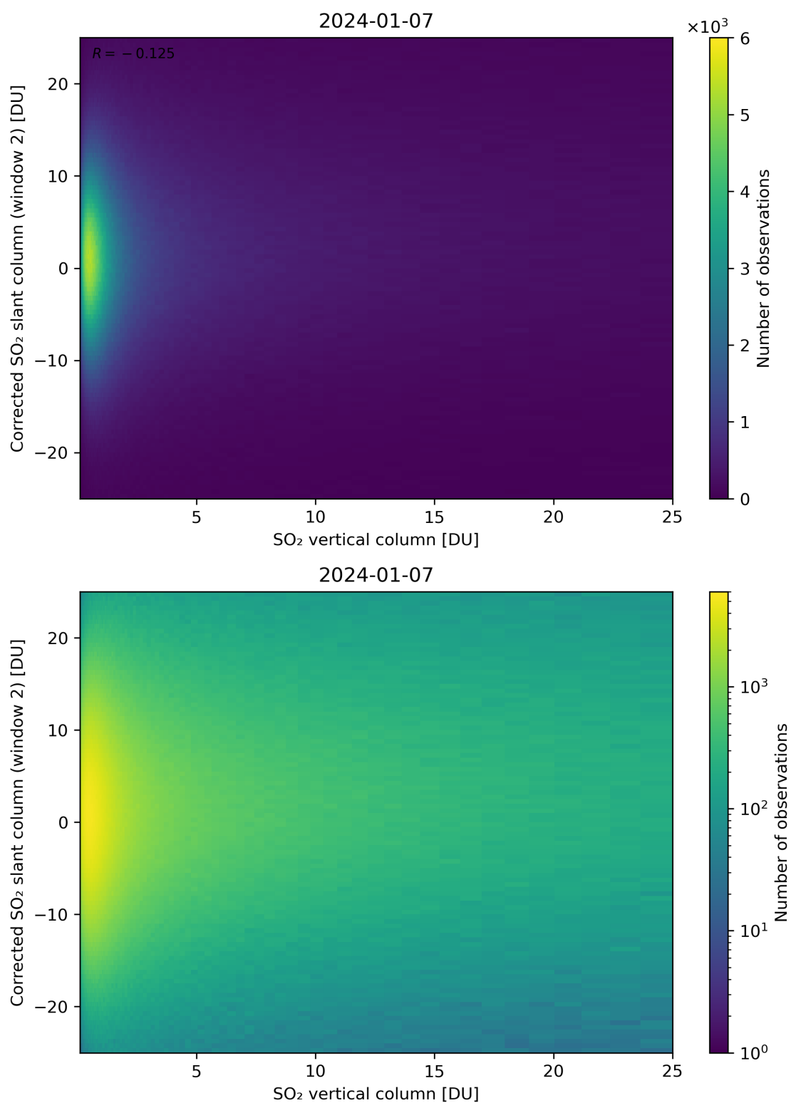
Figure 298: Scatter density plot of “SO 2 vertical column” against “Corrected SO 2 slant column (window 2)” for 2024-01-06 to 2024-01-08.
