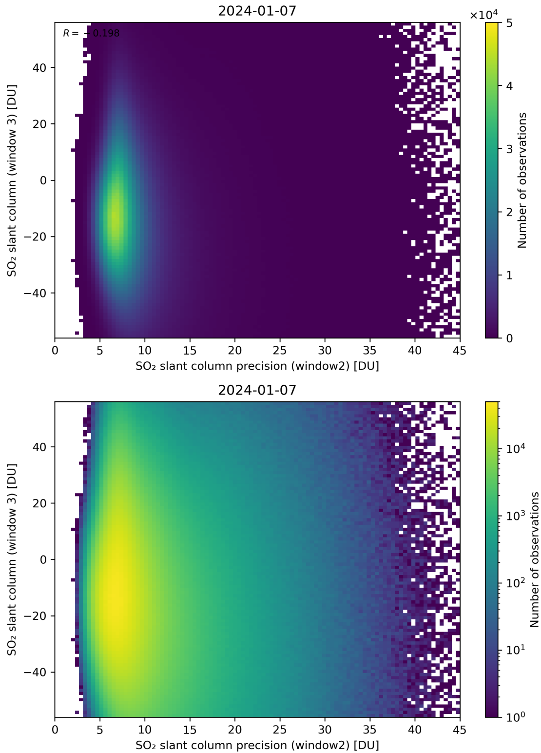
Figure 249: Scatter density plot of “SO 2 slant column precision (window2)” against “SO 2 slant column (window 3)” for 2024-01-06 to 2024-01-08.
