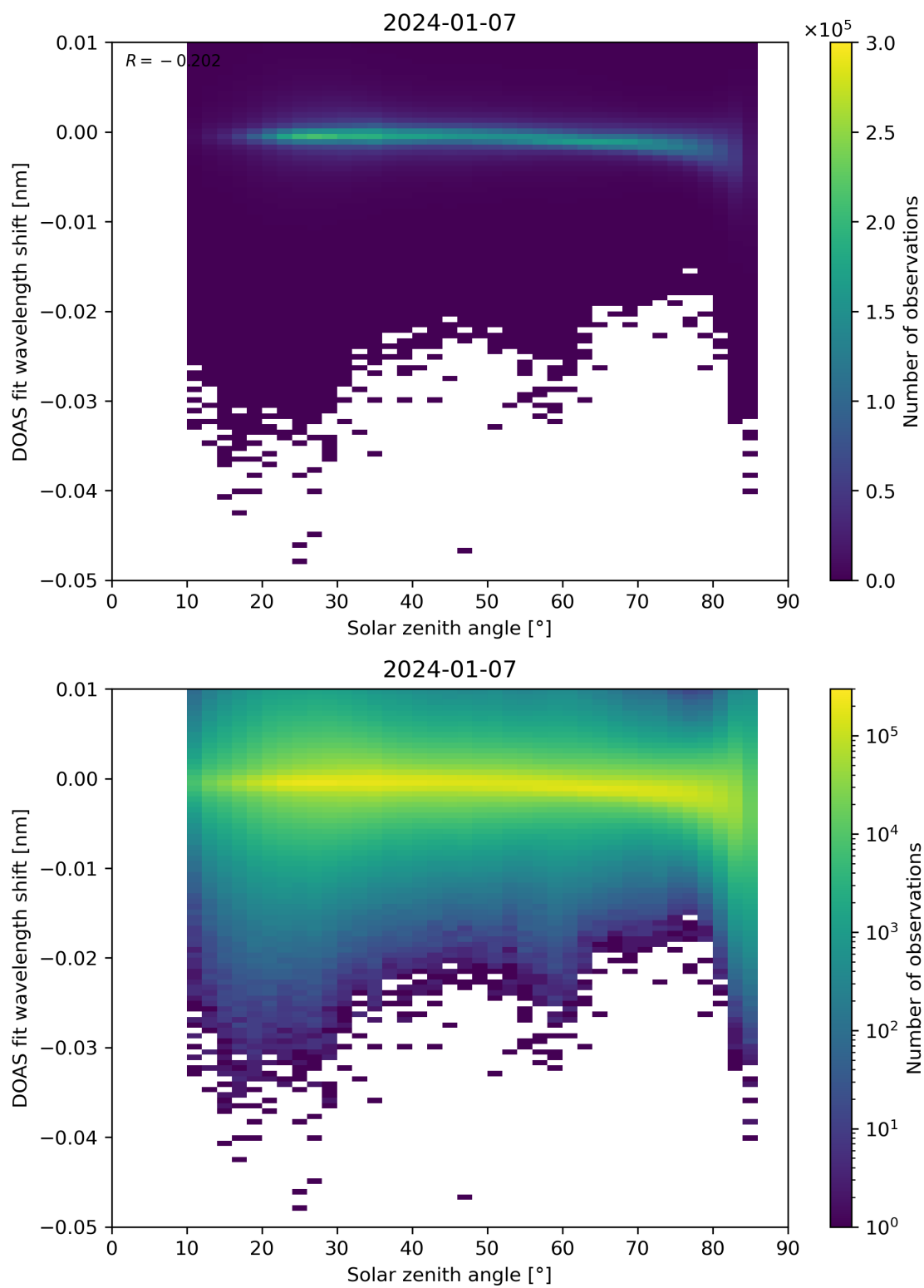
Figure 161: Scatter density plot of “Solar zenith angle” against “DOAS fit wavelength shift” for 2024-01-06 to 2024-01-08.
