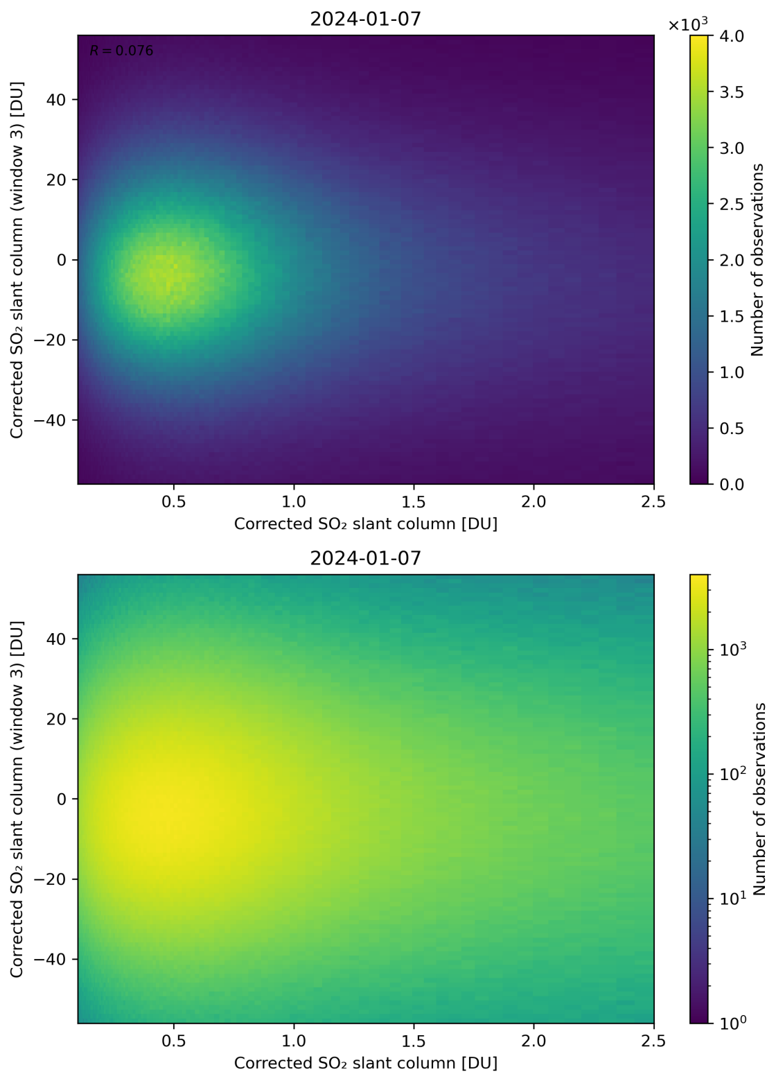
Figure 186: Scatter density plot of “Corrected SO 2 slant column” against “Corrected SO 2 slant column (window 3)” for 2024-01-06 to 2024-01-08.
