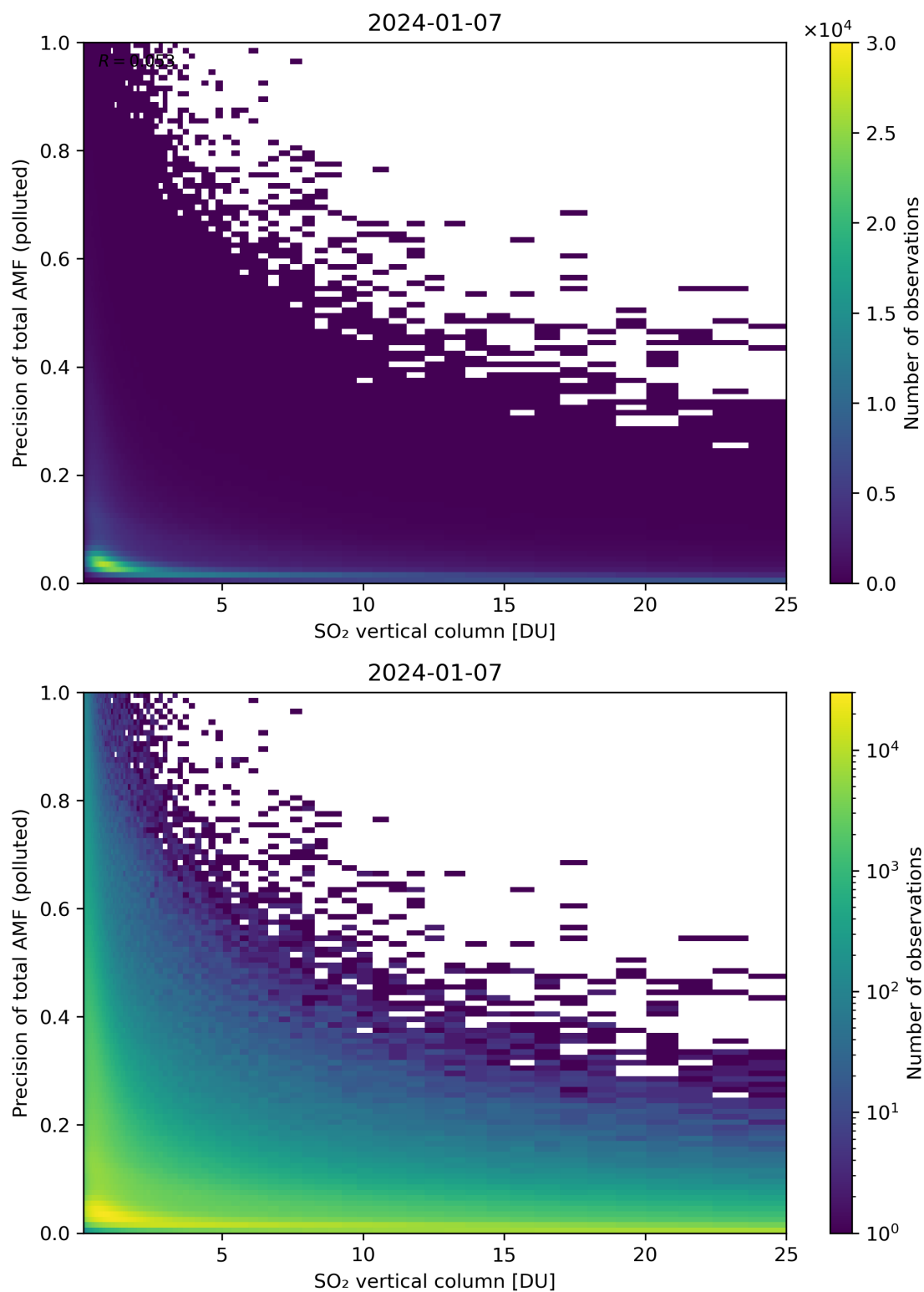
Figure 306: Scatter density plot of “SO 2 vertical column” against “Precision of total AMF (polluted)” for 2024-01-06 to 2024-01-08.
