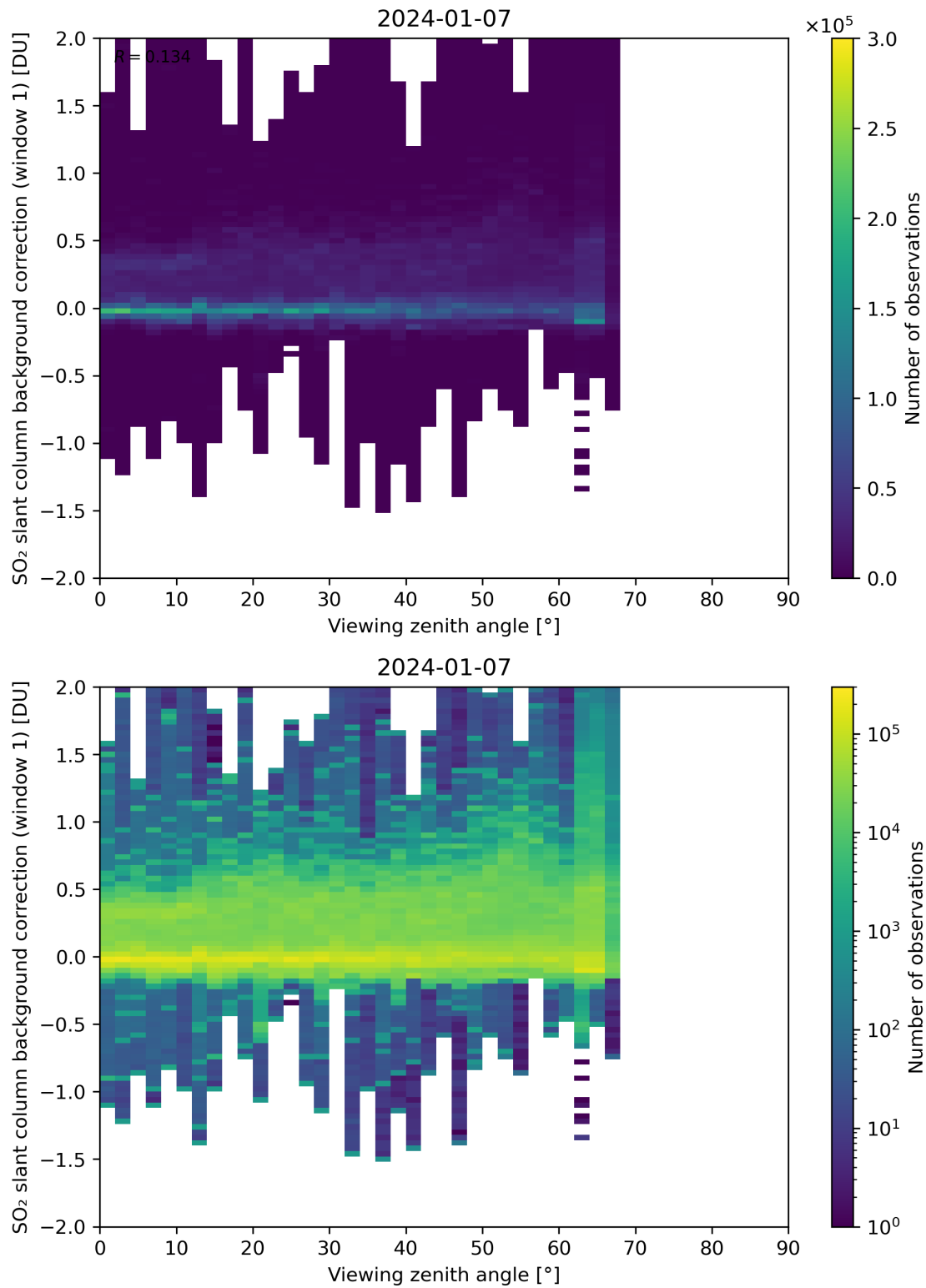
Figure 308: Scatter density plot of “Viewing zenith angle” against “SO 2 slant column background correction (window 1)” for 2024-01-06 to 2024-01-08.
