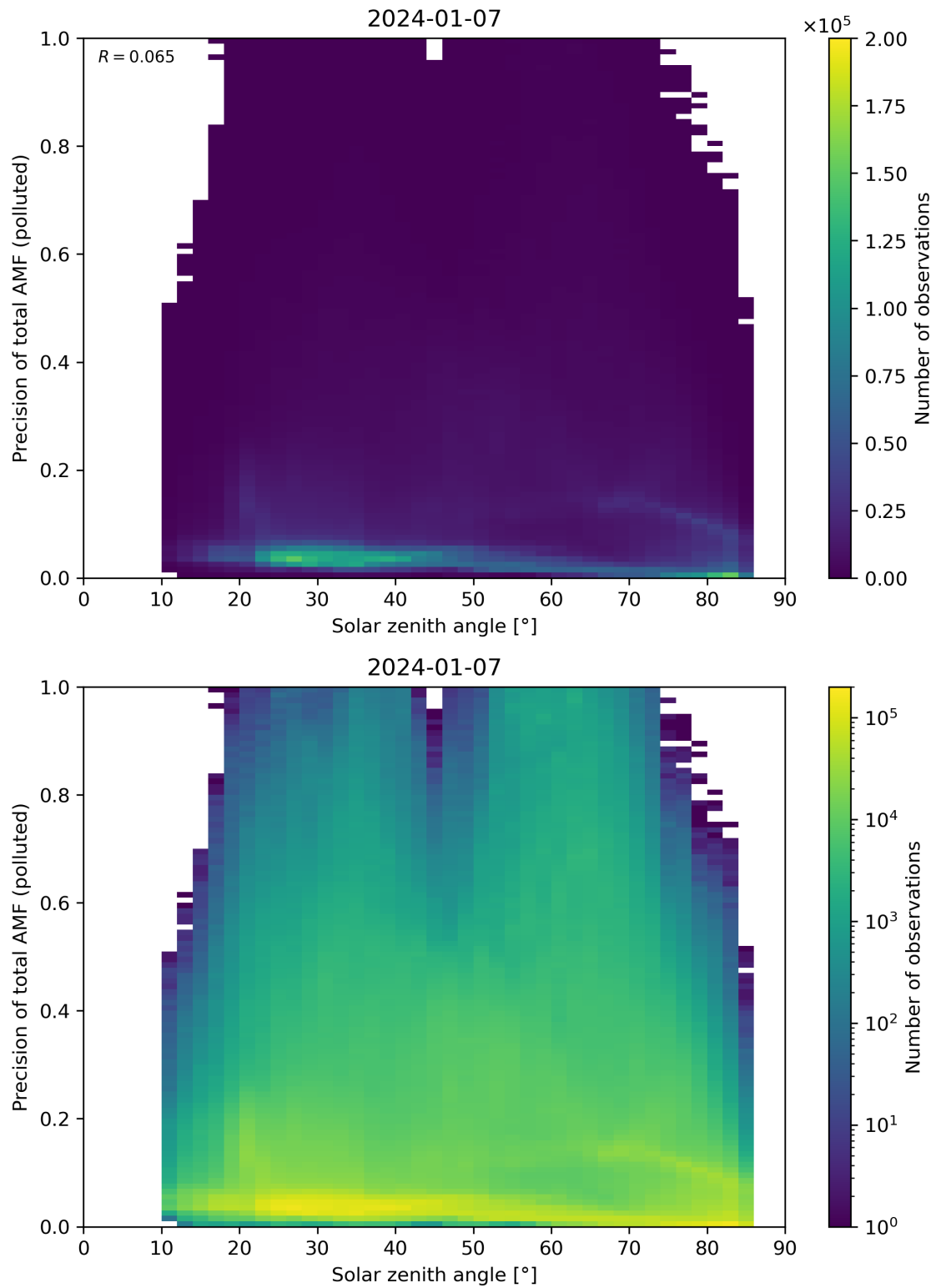
Figure 175: Scatter density plot of “Solar zenith angle” against “Precision of total AMF (polluted)” for 2024-01-06 to 2024-01-08.
