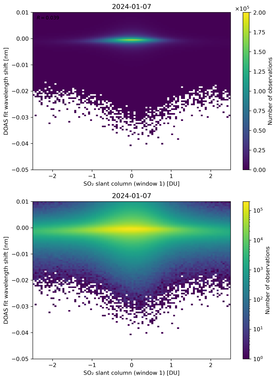
Figure 215: Scatter density plot of “SO 2 slant column (window 1)” against “DOAS fit wavelength shift” for 2024-01-06 to 2024-01-08.
