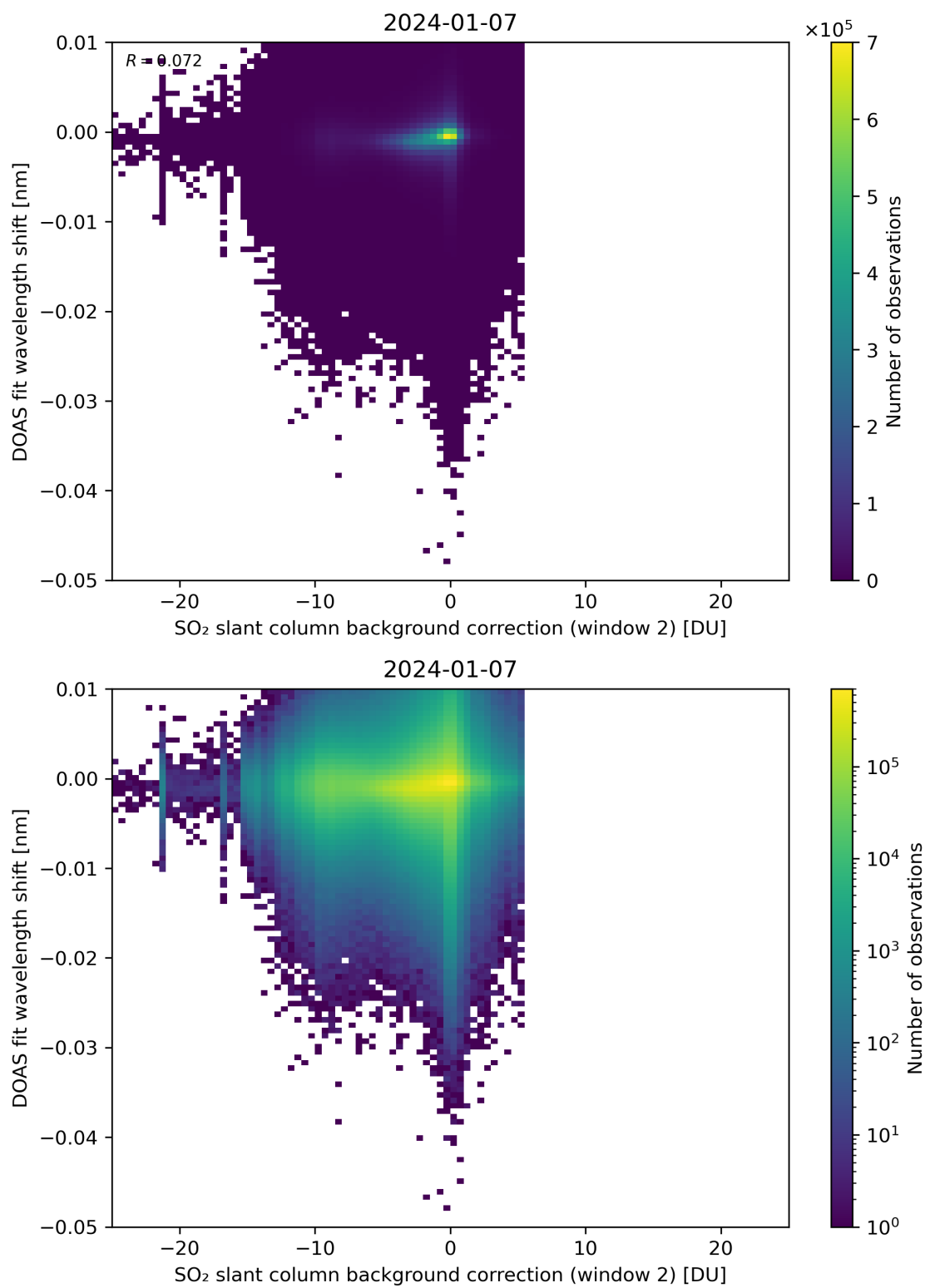
Figure 112: Scatter density plot of “SO 2 slant column background correction (window 2)” against “DOAS fit wavelength shift” for 2024-01-06 to 2024-01-08.
