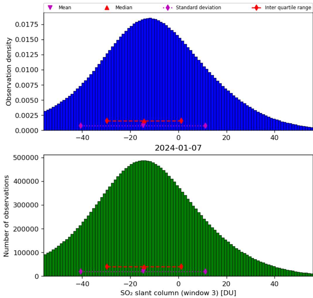
Figure 64: Histogram of “SO 2 slant column (window 3)” for 2024-01-06 to 2024-01-08
