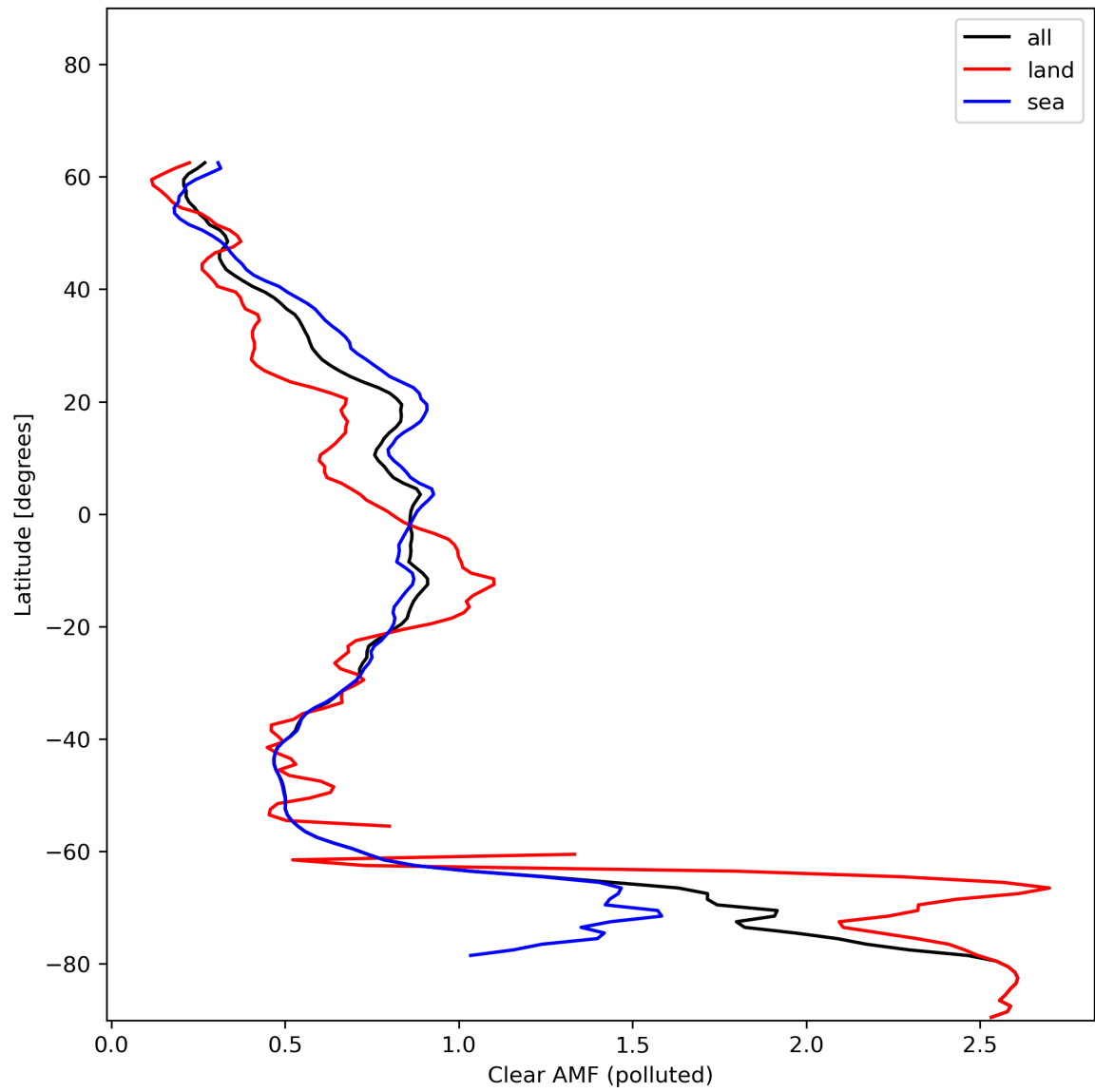
Figure 50: Zonal average of “Clear AMF (polluted)” for 2024-01-06 to 2024-01-08.
