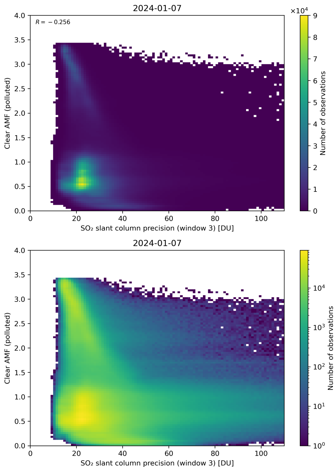
Figure 261: Scatter density plot of “SO 2 slant column precision (window 3)” against “Clear AMF (polluted)” for 2024-01-06 to 2024-01-08.
