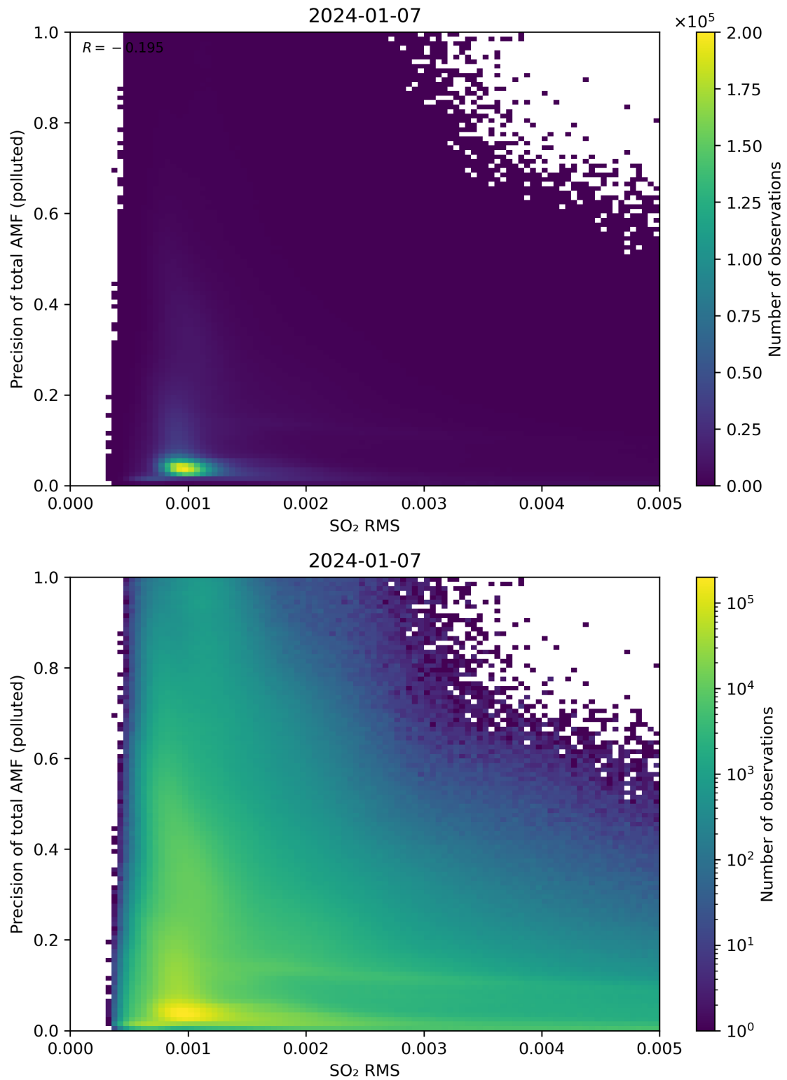
Figure 138: Scatter density plot of “SO 2 RMS” against “Precision of total AMF (polluted)” for 2024-01-06 to 2024-01-08.
