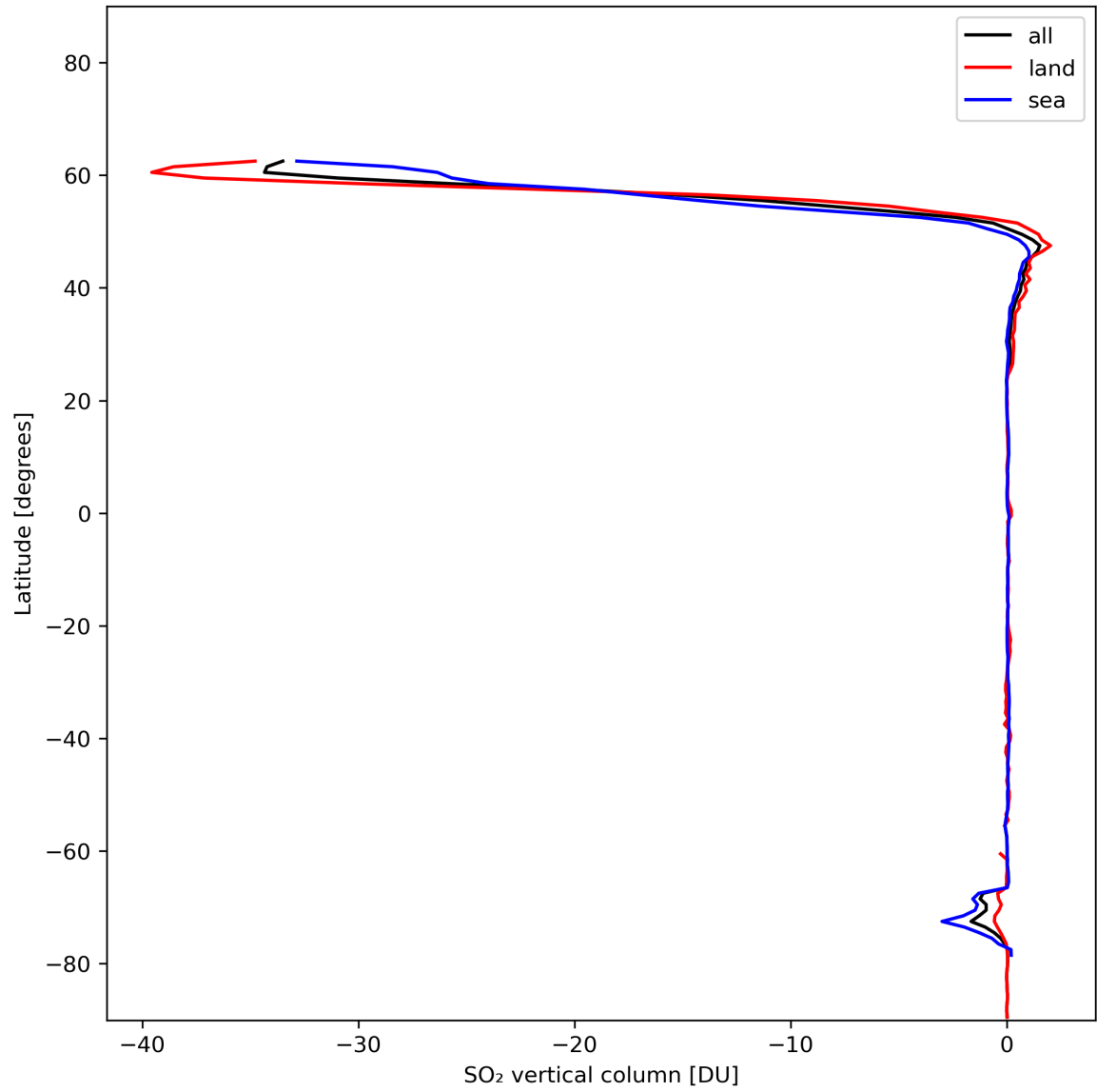
Figure 30: Zonal average of “SO 2 vertical column” for 2024-01-06 to 2024-01-08.
