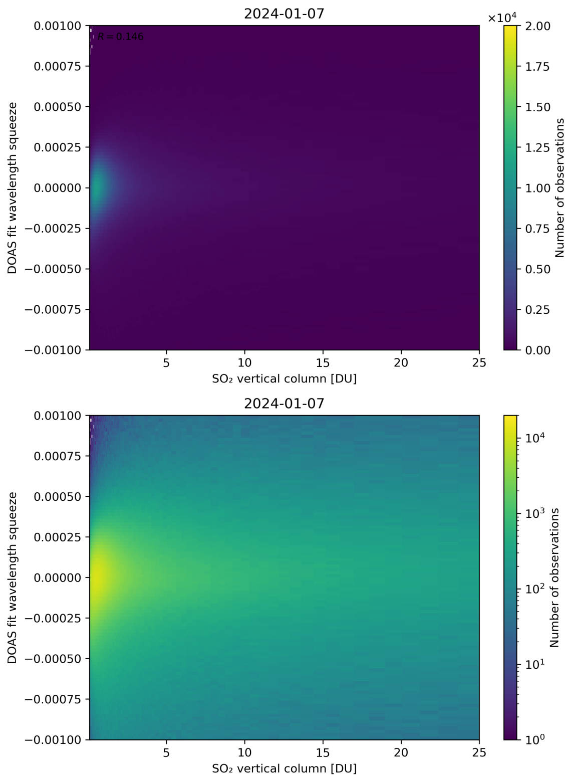
Figure 277: Scatter density plot of “SO 2 vertical column” against “DOAS fit wavelength squeeze” for 2024-01-06 to 2024-01-08.
