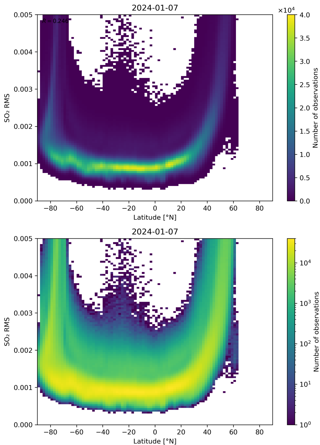
Figure 144: Scatter density plot of “Latitude” against “SO 2 RMS” for 2024-01-06 to 2024-01-08.
