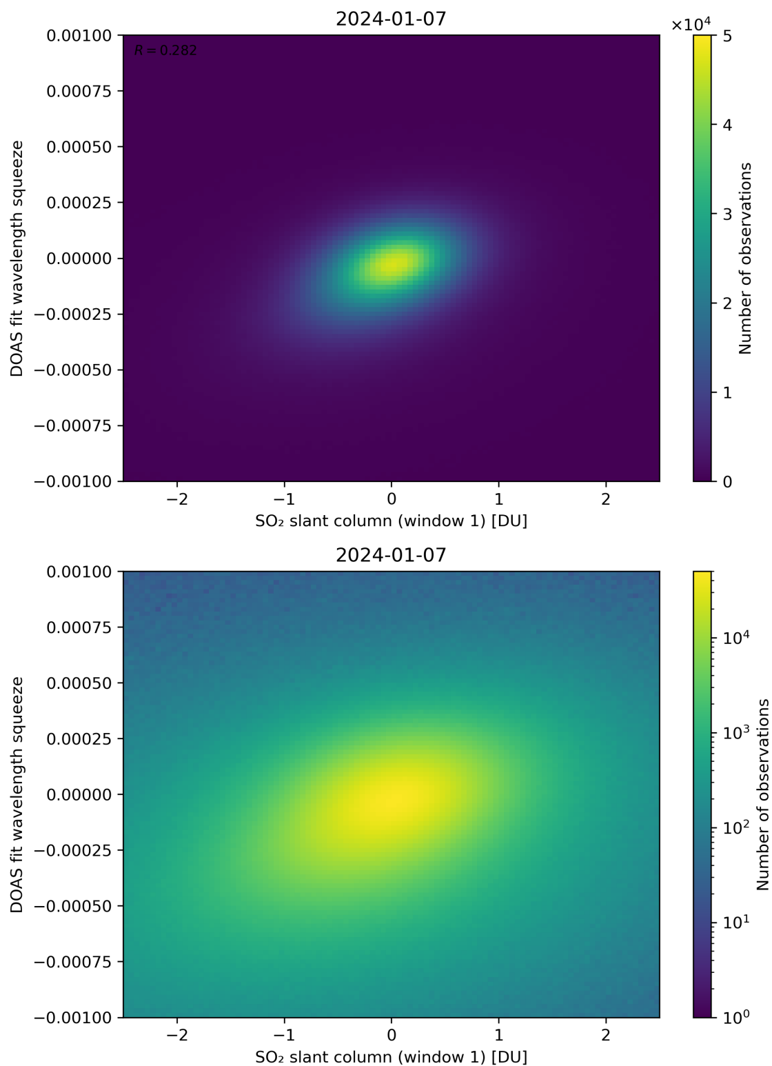
Figure 216: Scatter density plot of “SO 2 slant column (window 1)” against “DOAS fit wavelength squeeze” for 2024-01-06 to 2024-01-08.
