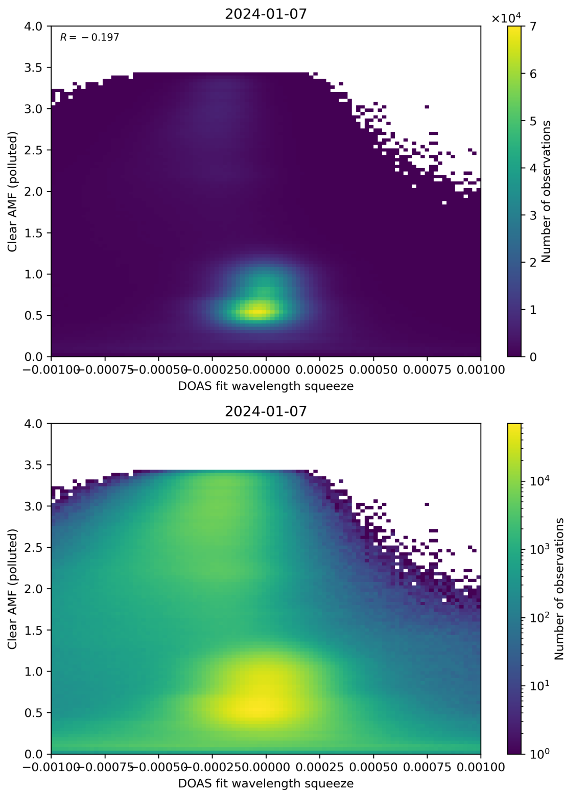
Figure 133: Scatter density plot of “DOAS fit wavelength squeeze” against “Clear AMF (polluted)” for 2024-01-06 to 2024-01-08.
