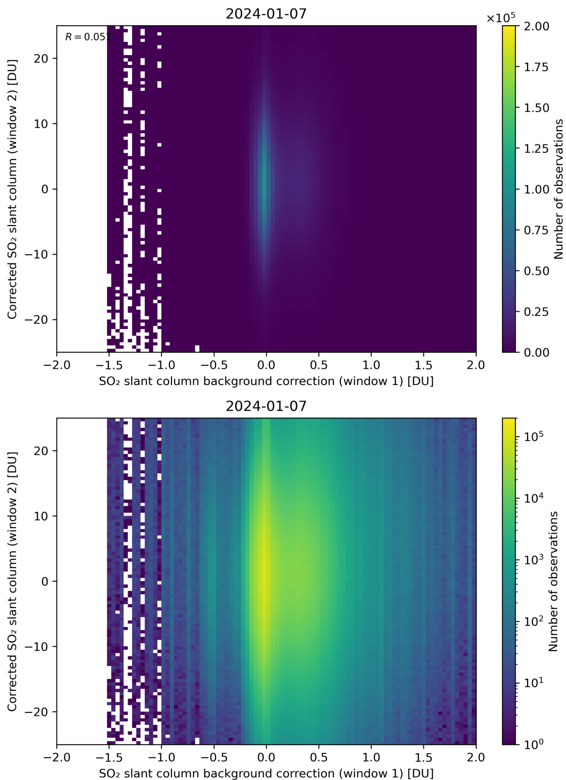
Figure 104: Scatter density plot of “SO 2 slant column background correction (window 1)” against “Corrected SO 2 slant column (window 2)” for 2024-01-06 to 2024-01-08.
