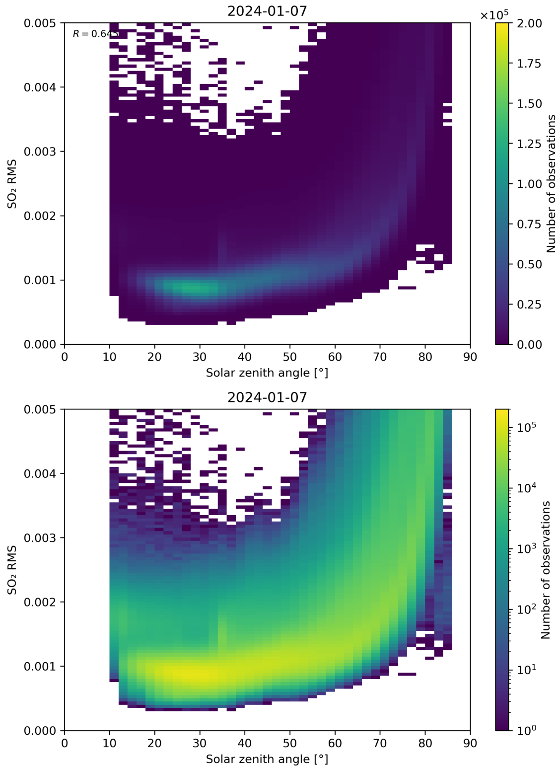
Figure 163: Scatter density plot of “Solar zenith angle” against “SO 2 RMS” for 2024-01-06 to 2024-01-08.
