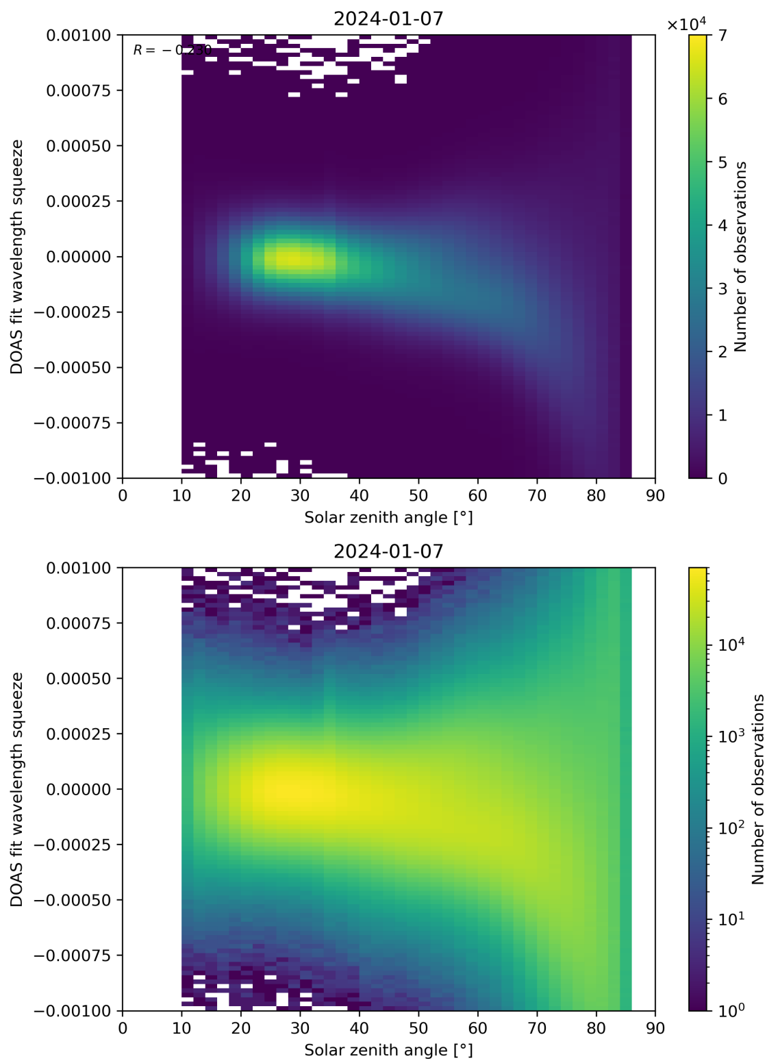
Figure 162: Scatter density plot of “Solar zenith angle” against “DOAS fit wavelength squeeze” for 2024-01-06 to 2024-01-08.
