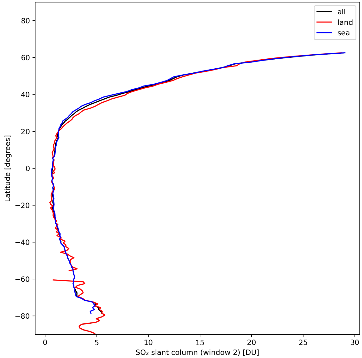
Figure 37: Zonal average of “SO 2 slant column (window 2)” for 2024-01-06 to 2024-01-08.
