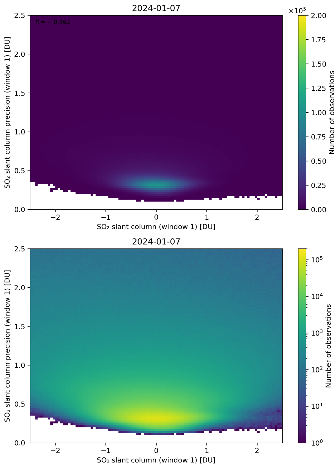
Figure 235: Scatter density plot of “SO 2 slant column (window 1)” against “SO 2 slant column precision (window 1)” for 2024-01-06 to 2024-01-08.
