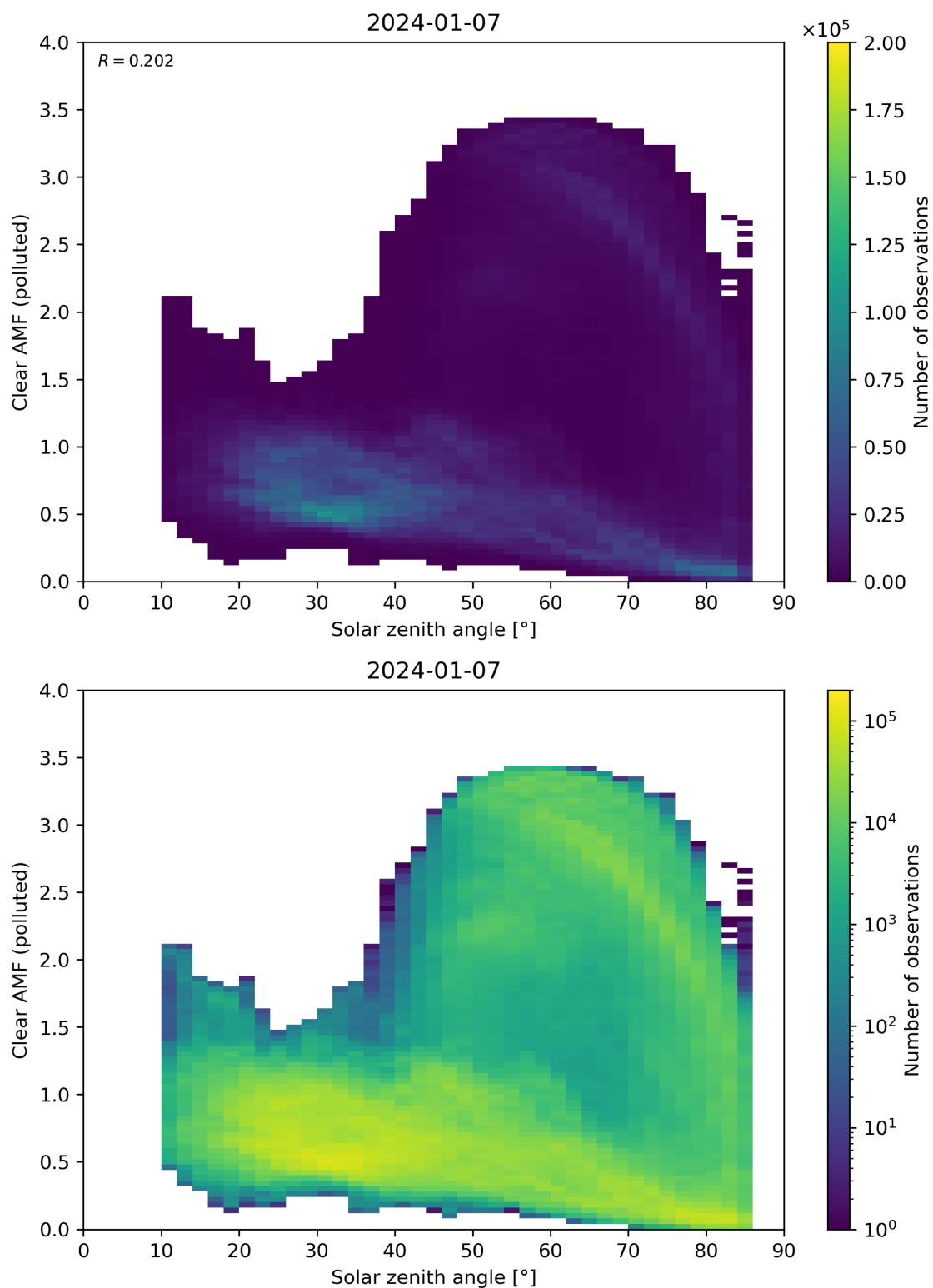
Figure 165: Scatter density plot of “Solar zenith angle” against “Clear AMF (polluted)” for 2024-01-06 to 2024-01-08.
