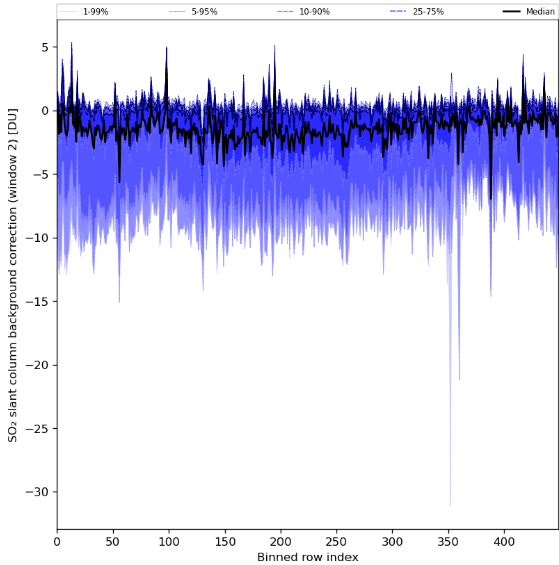
Figure 86: Along track statistics of “SO 2 slant column background correction (window 2)” for 2024-01-06 to 2024-01-08
