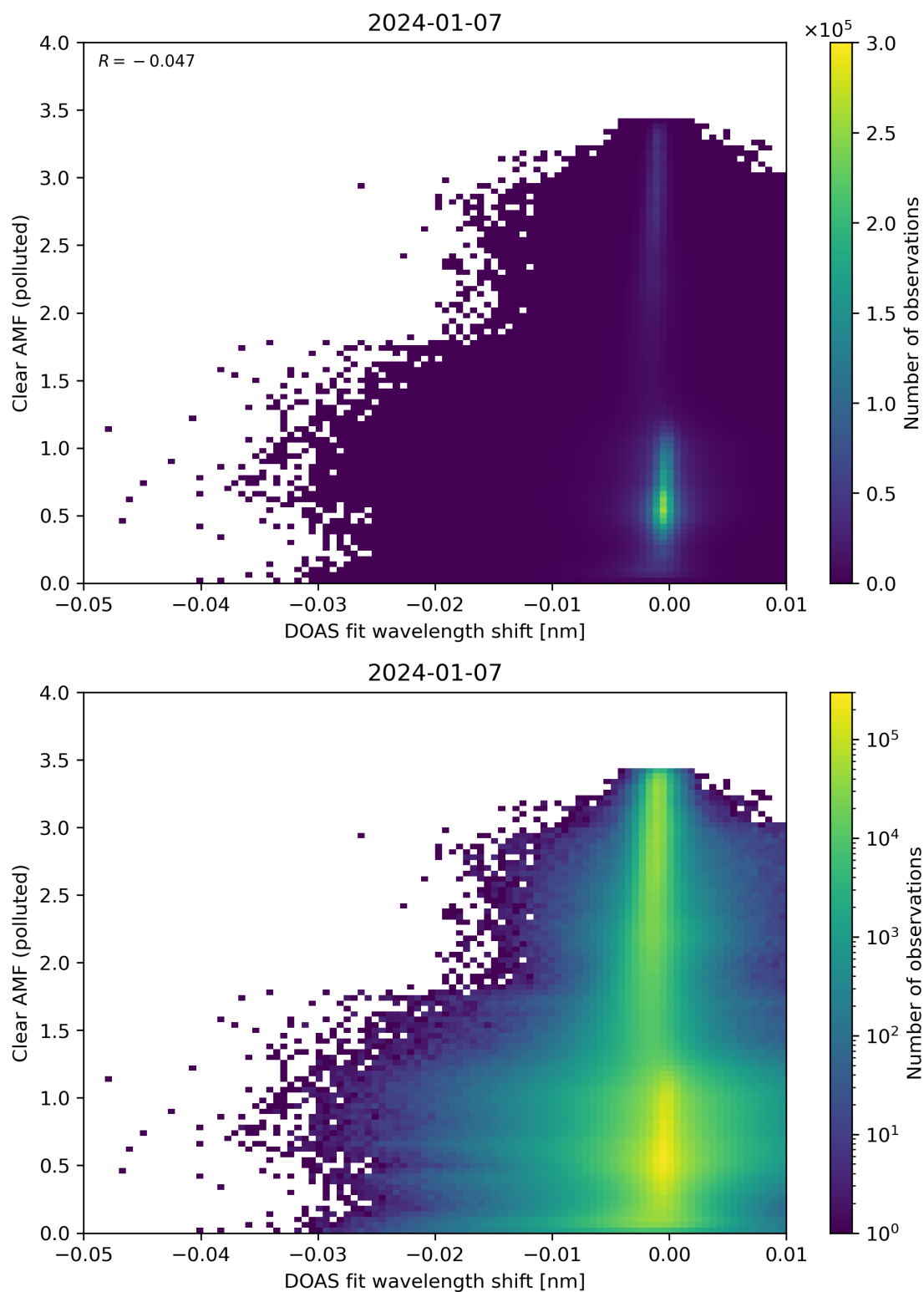
Figure 129: Scatter density plot of “DOAS fit wavelength shift” against “Clear AMF (polluted)” for 2024-01-06 to 2024-01-08.
