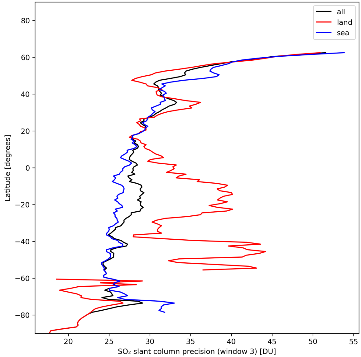
Figure 42: Zonal average of “SO 2 slant column precision (window 3)” for 2024-01-06 to 2024-01-08.
