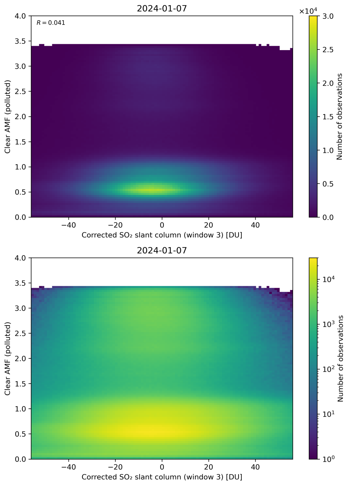
Figure 209: Scatter density plot of “Corrected SO 2 slant column (window 3)” against “Clear AMF (polluted)” for 2024-01-06 to 2024-01-08.
