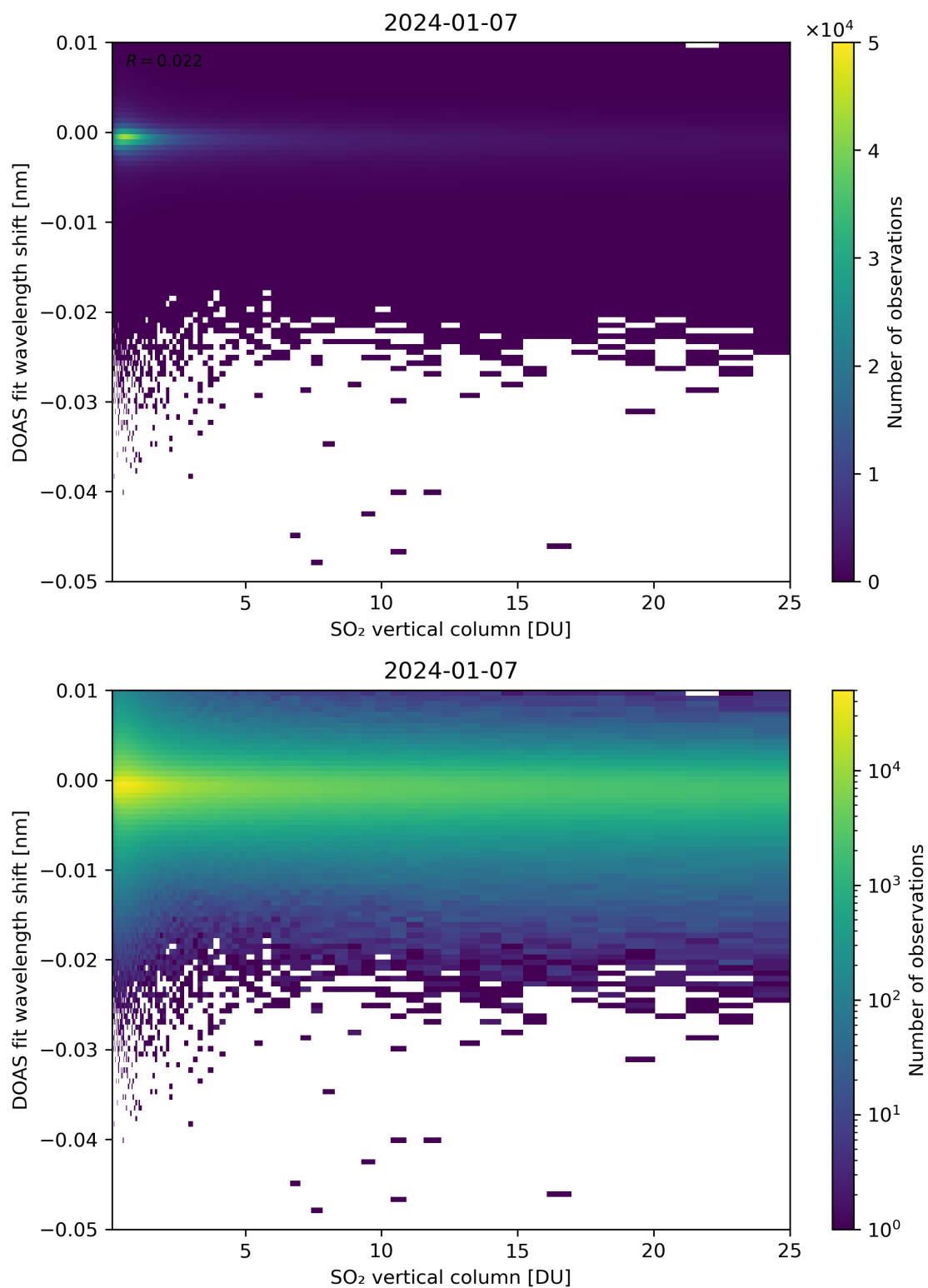
Figure 276: Scatter density plot of “SO 2 vertical column” against “DOAS fit wavelength shift” for 2024-01-06 to 2024-01-08.
