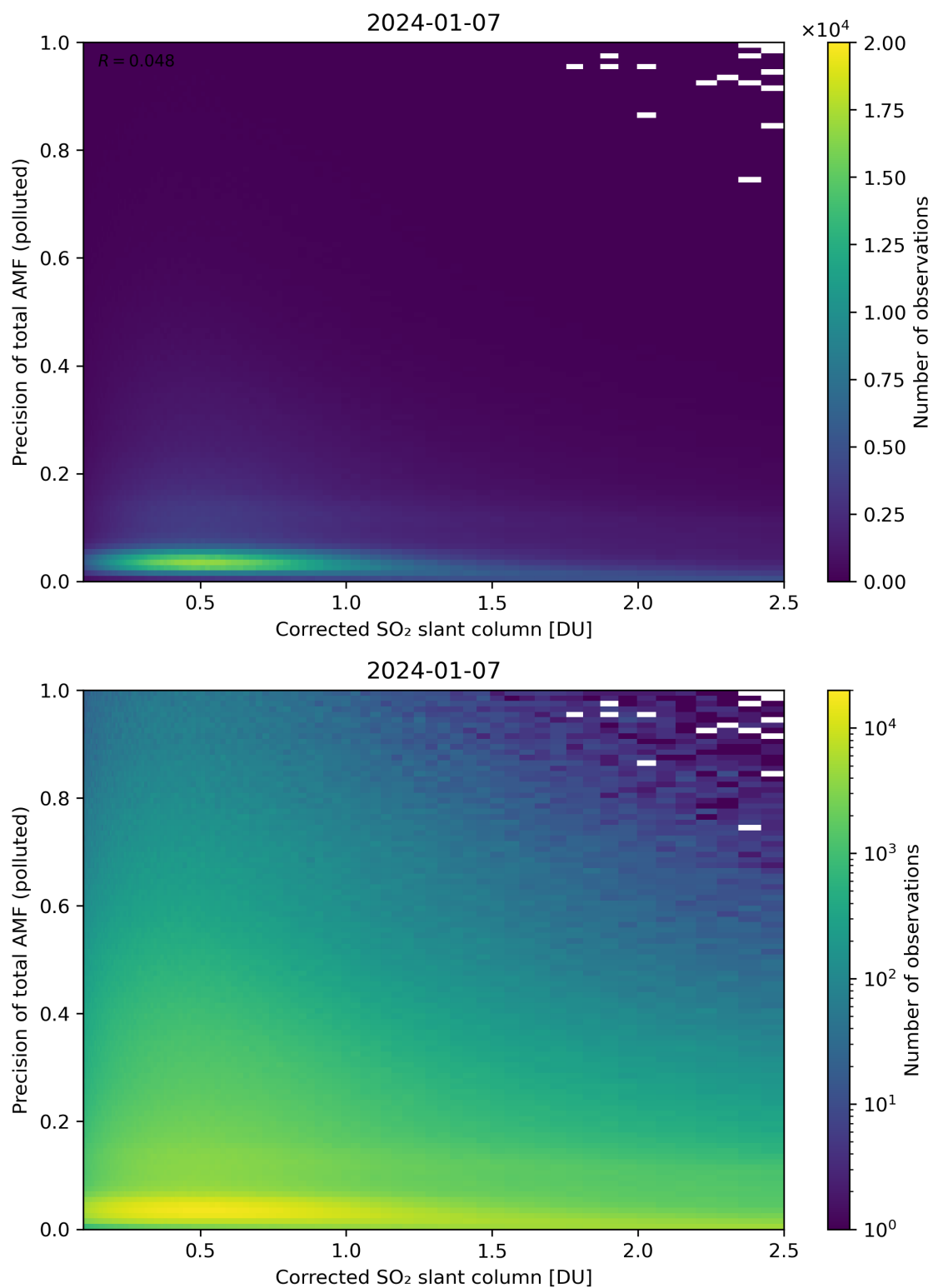
Figure 193: Scatter density plot of “Corrected SO 2 slant column” against “Precision of total AMF (polluted)” for 2024-01-06 to 2024-01-08.
