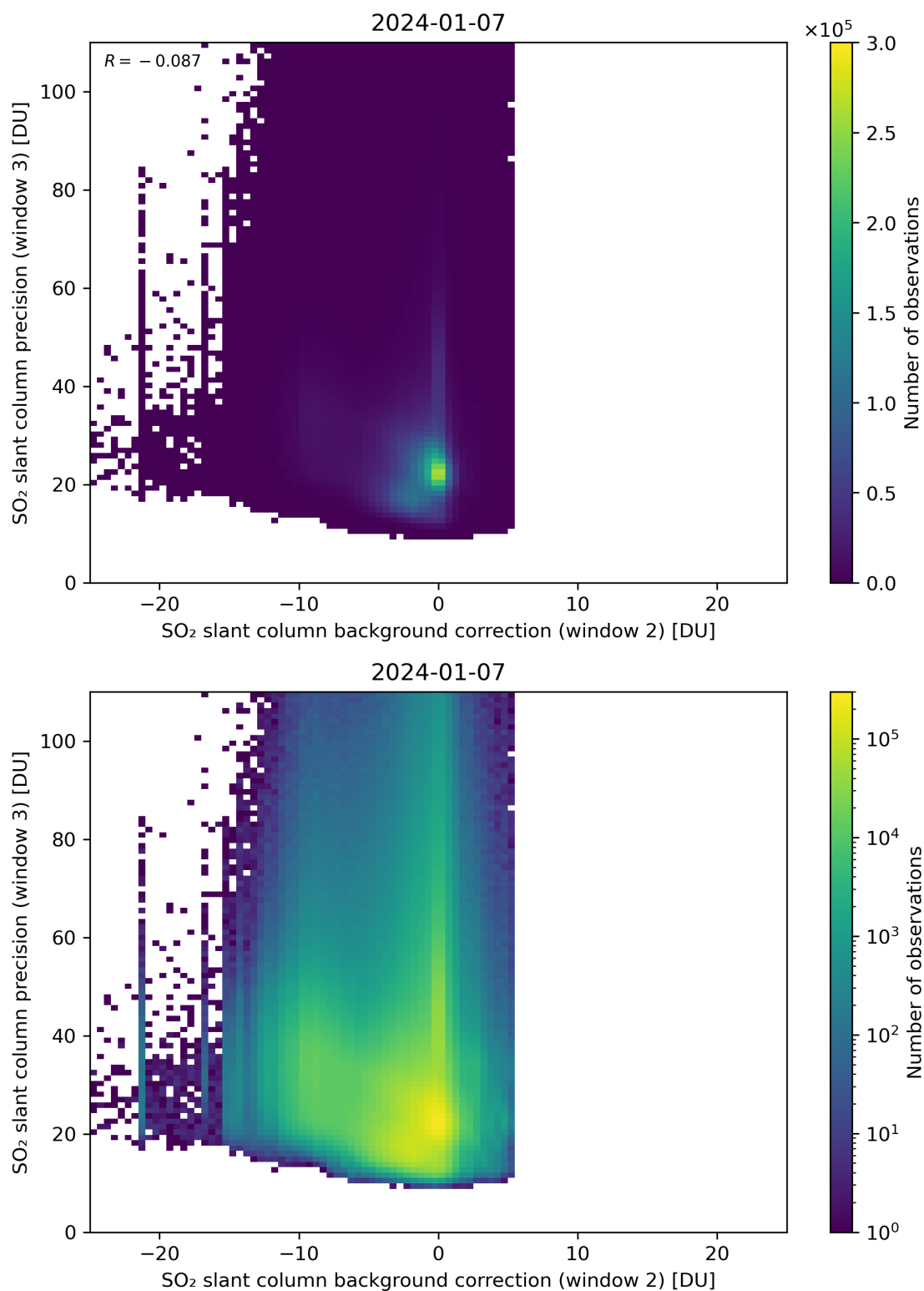
Figure 118: Scatter density plot of “SO 2 slant column background correction (window 2)” against “SO 2 slant column precision (window 3)” for 2024-01-06 to 2024-01-08.
