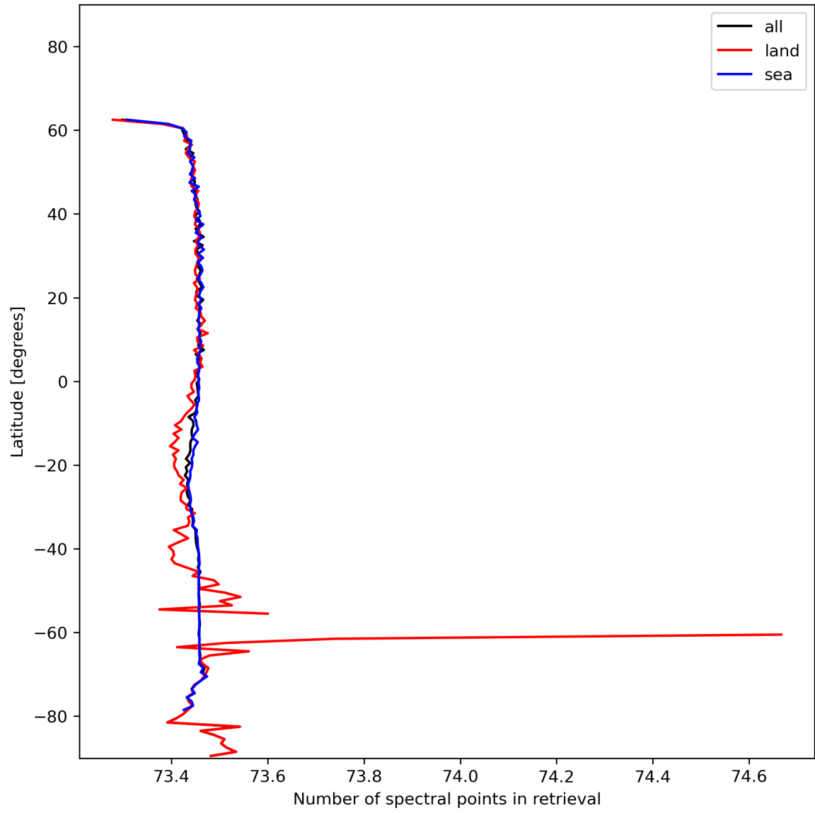
Figure 51: Zonal average of “Number of spectral points in retrieval” for 2024-01-06 to 2024-01-08.
