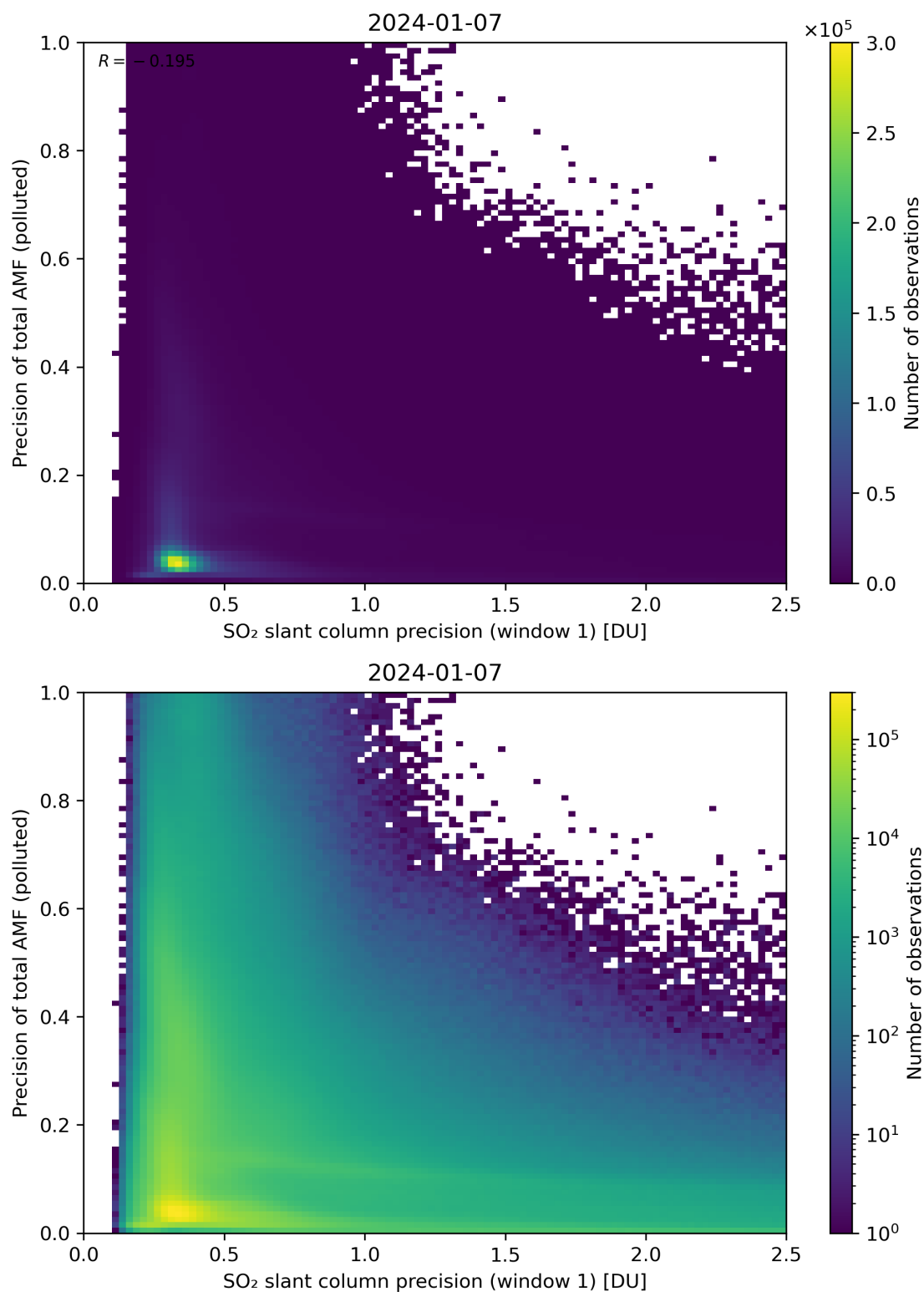
Figure 231: Scatter density plot of “SO 2 slant column precision (window 1)” against “Precision of total AMF (polluted)” for 2024-01-06 to 2024-01-08.
