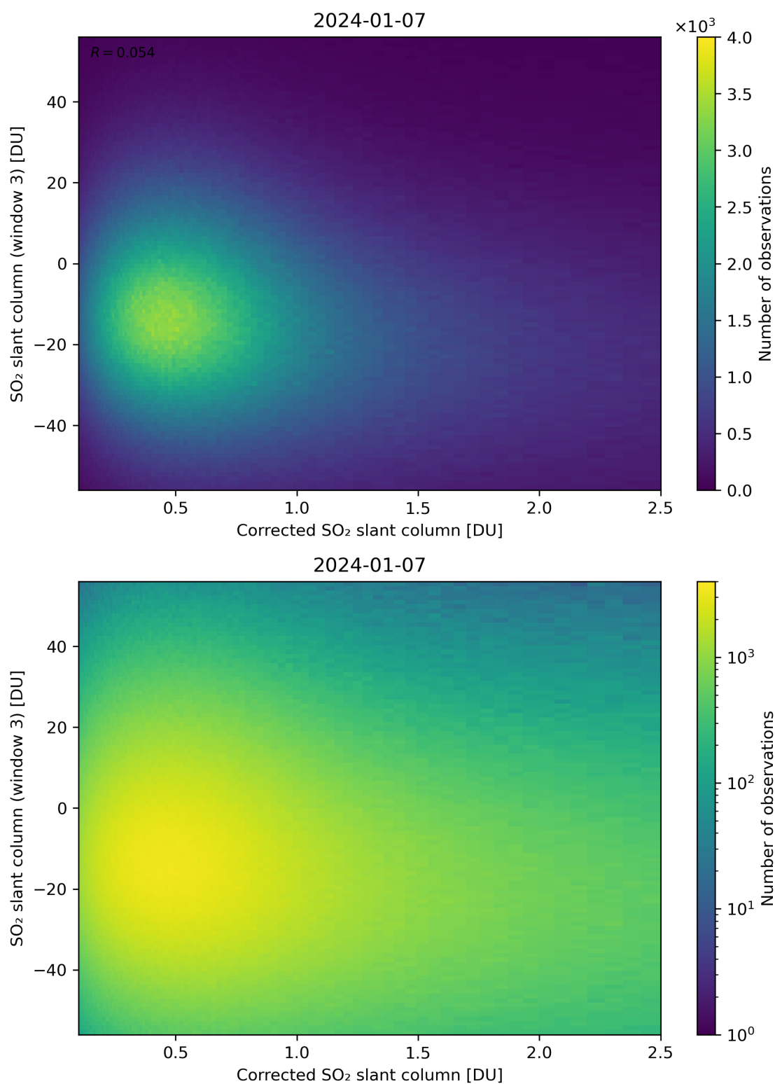
Figure 190: Scatter density plot of “Corrected SO 2 slant column” against “SO 2 slant column (window 3)” for 2024-01-06 to 2024-01-08.
