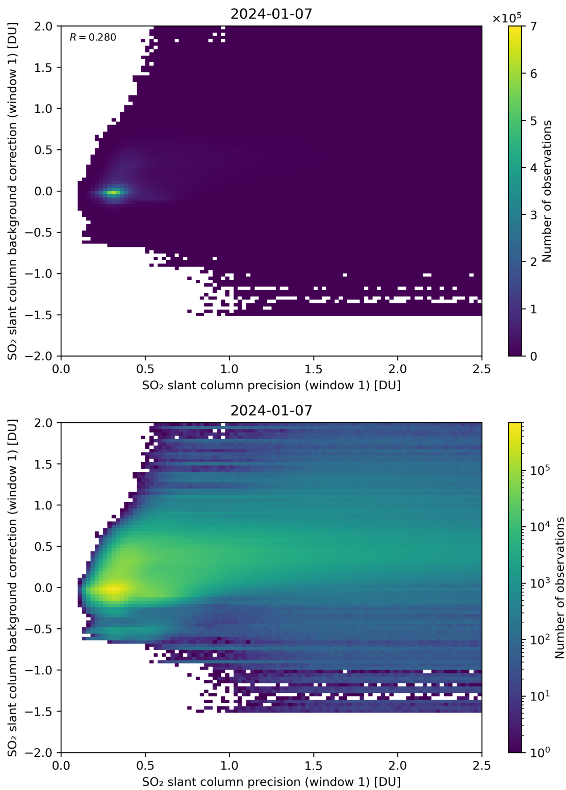
Figure 218: Scatter density plot of “SO 2 slant column precision (window 1)” against “SO 2 slant column background correction (window 1)” for 2024-01-06 to 2024-01-08.
