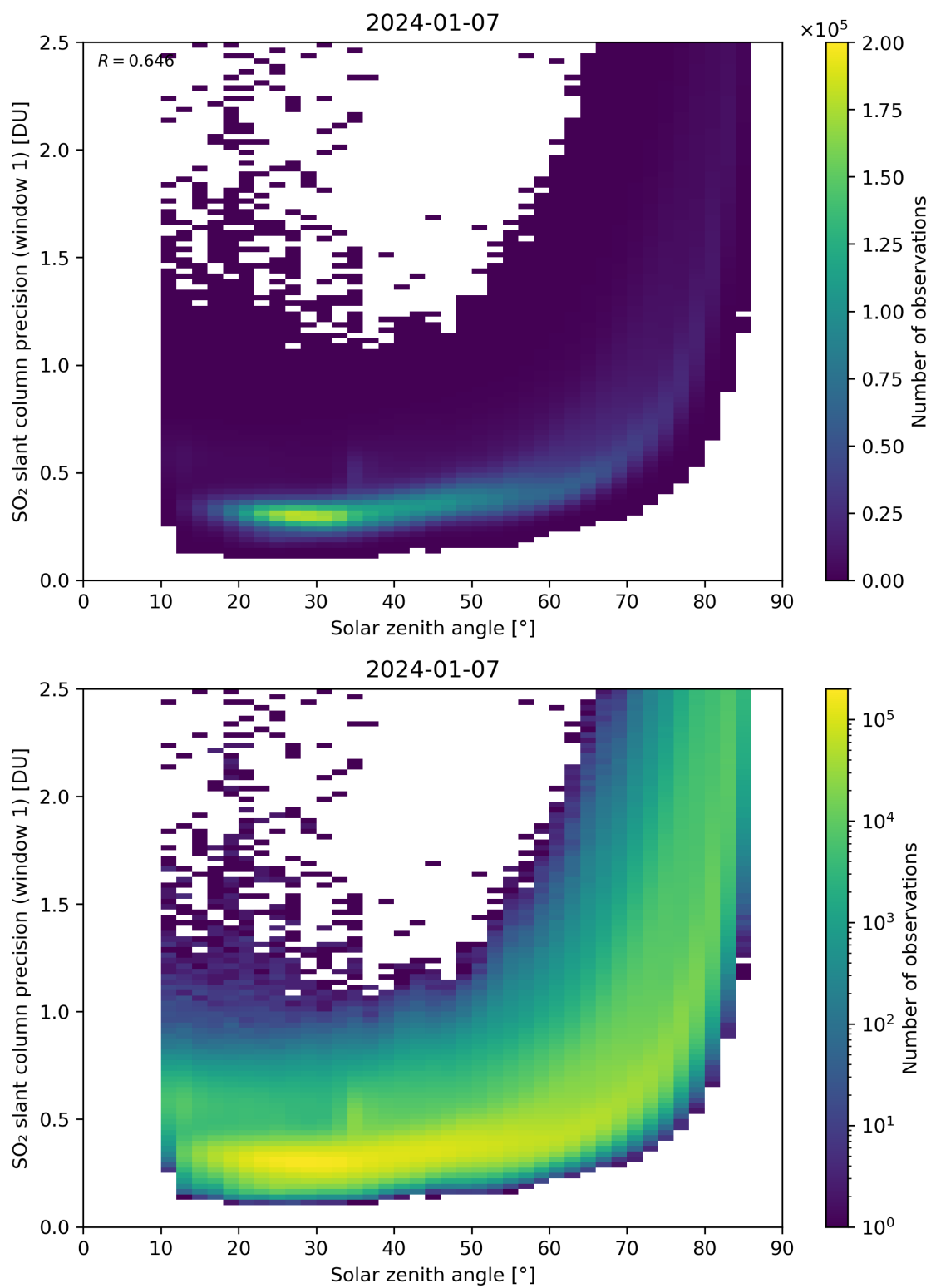
Figure 170: Scatter density plot of “Solar zenith angle” against “SO 2 slant column precision (window 1)” for 2024-01-06 to 2024-01-08.
