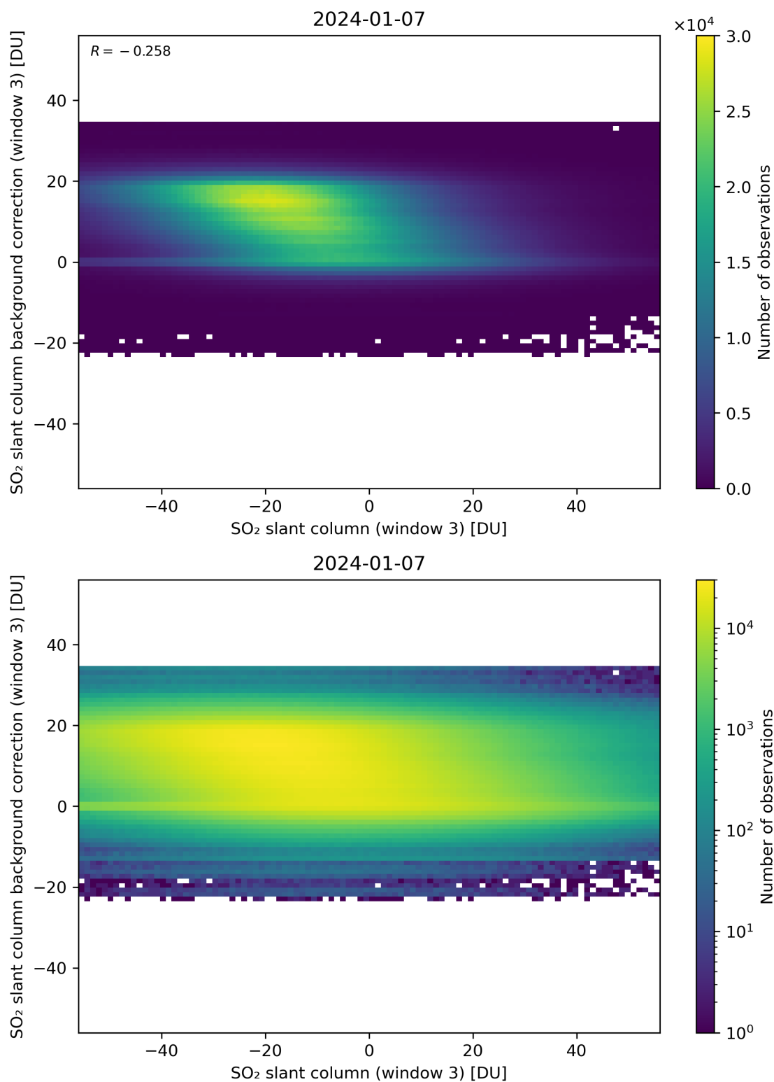
Figure 253: Scatter density plot of “SO 2 slant column (window 3)” against “SO 2 slant column background correction (window 3)” for 2024-01-06 to 2024-01-08.
