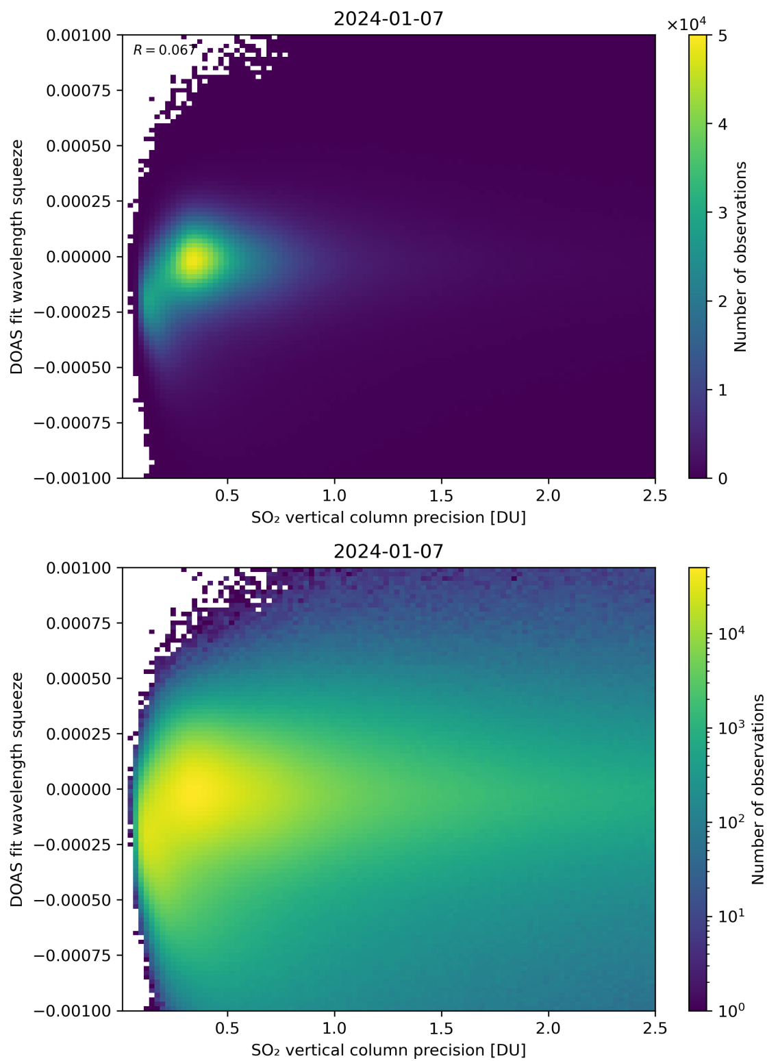
Figure 283: Scatter density plot of “SO 2 vertical column precision” against “DOAS fit wavelength squeeze” for 2024-01-06 to 2024-01-08.
