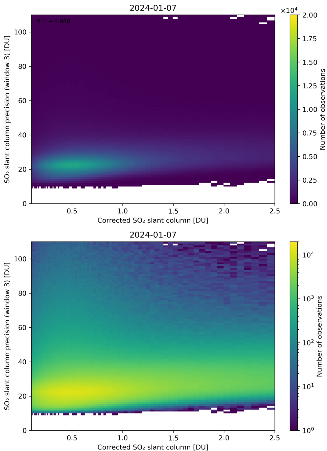
Figure 191: Scatter density plot of “Corrected SO 2 slant column” against “SO 2 slant column precision (window 3)” for 2024-01-06 to 2024-01-08.
