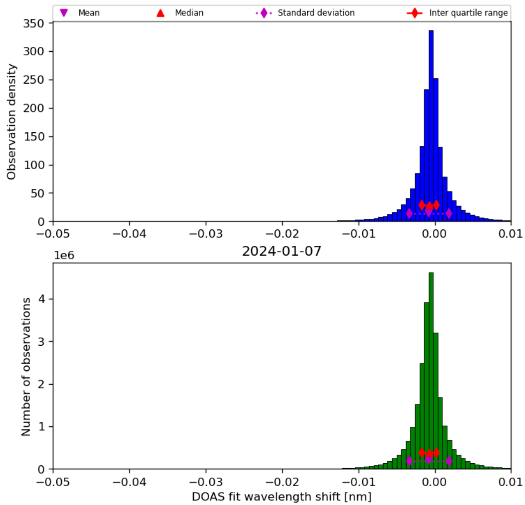
Figure 68: Histogram of “DOAS fit wavelength shift” for 2024-01-06 to 2024-01-08
