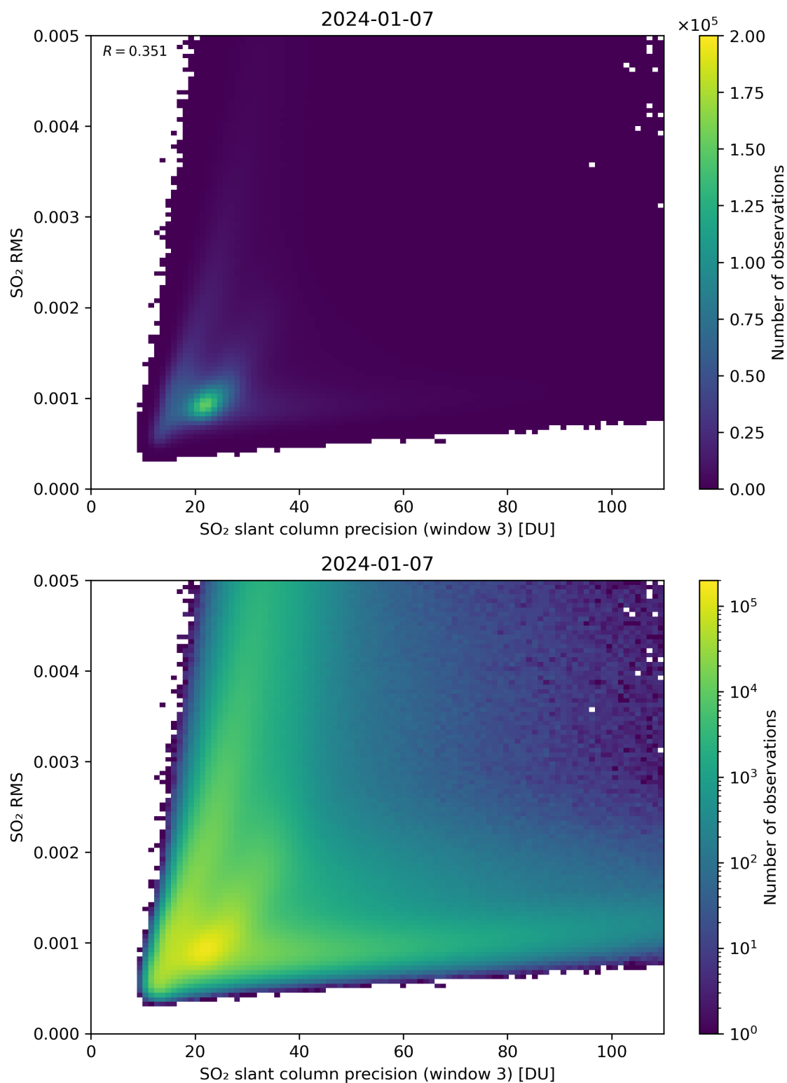
Figure 260: Scatter density plot of “SO 2 slant column precision (window 3)” against “SO 2 RMS” for 2024-01-06 to 2024-01-08.
