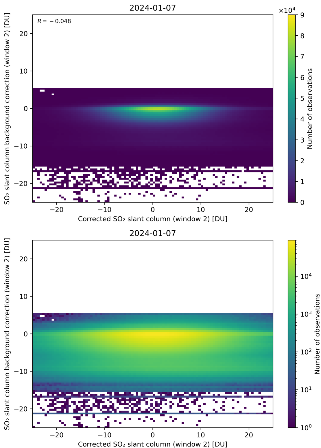
Figure 194: Scatter density plot of “Corrected SO 2 slant column (window 2)” against “SO 2 slant column background correction (window 2)” for 2024-01-06 to 2024-01-08.
