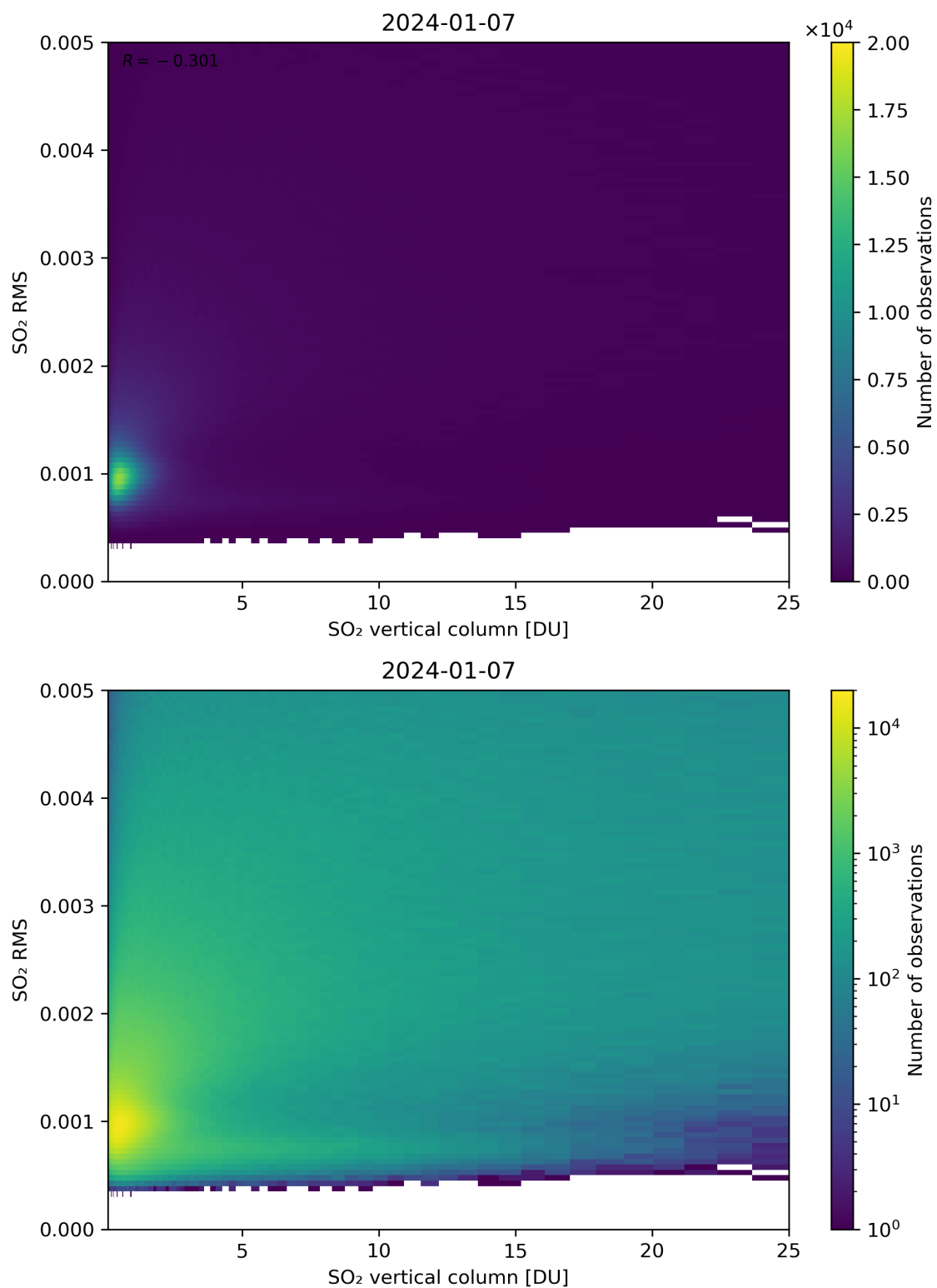
Figure 278: Scatter density plot of “SO 2 vertical column” against “SO 2 RMS” for 2024-01-06 to 2024-01-08.
