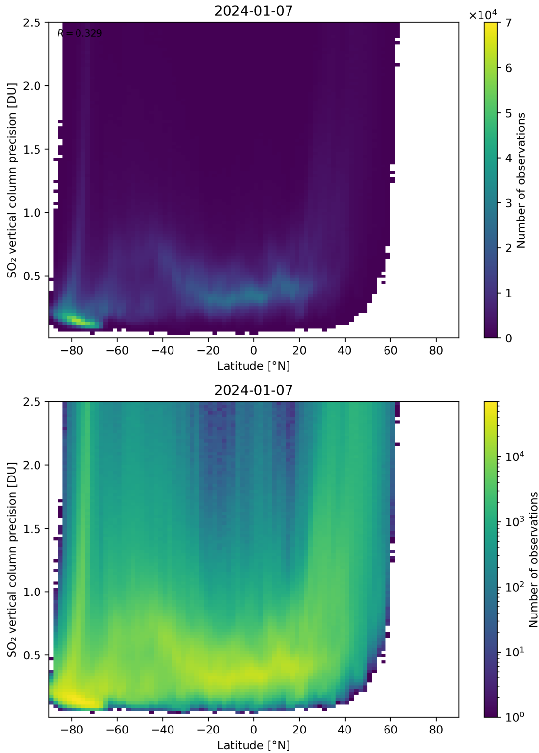
Figure 157: Scatter density plot of “Latitude” against “SO 2 vertical column precision” for 2024-01-06 to 2024-01-08.
