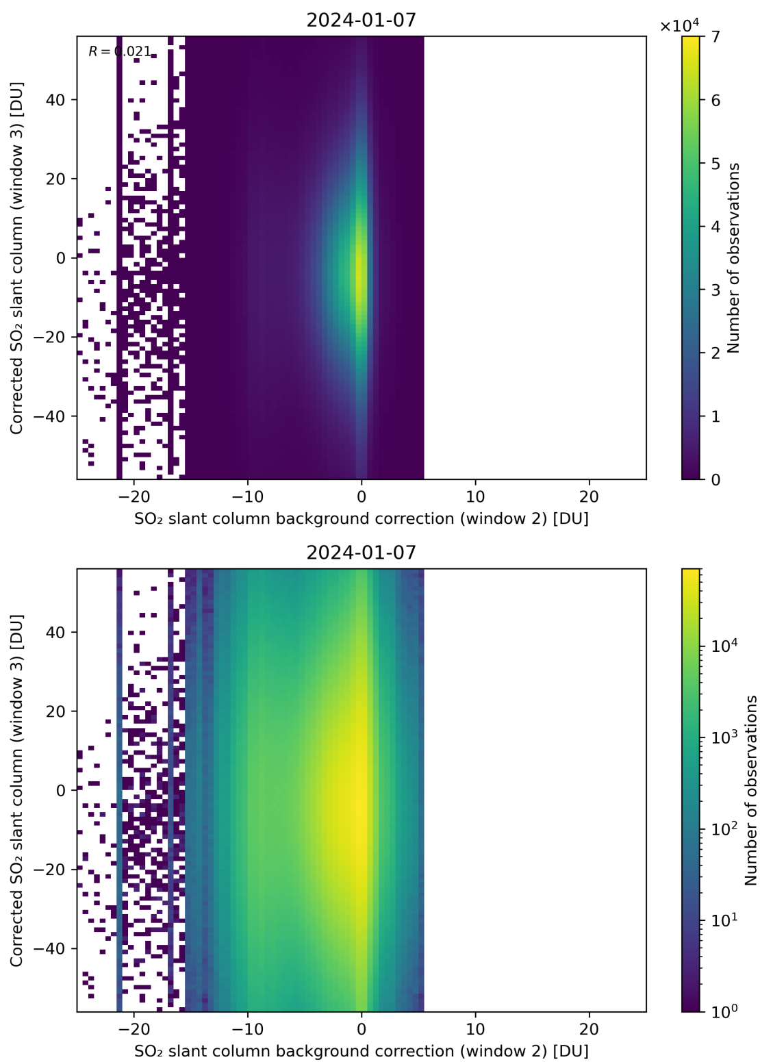
Figure 116: Scatter density plot of “SO 2 slant column background correction (window 2)” against “Corrected SO 2 slant column (window 3)” for 2024-01-06 to 2024-01-08.
