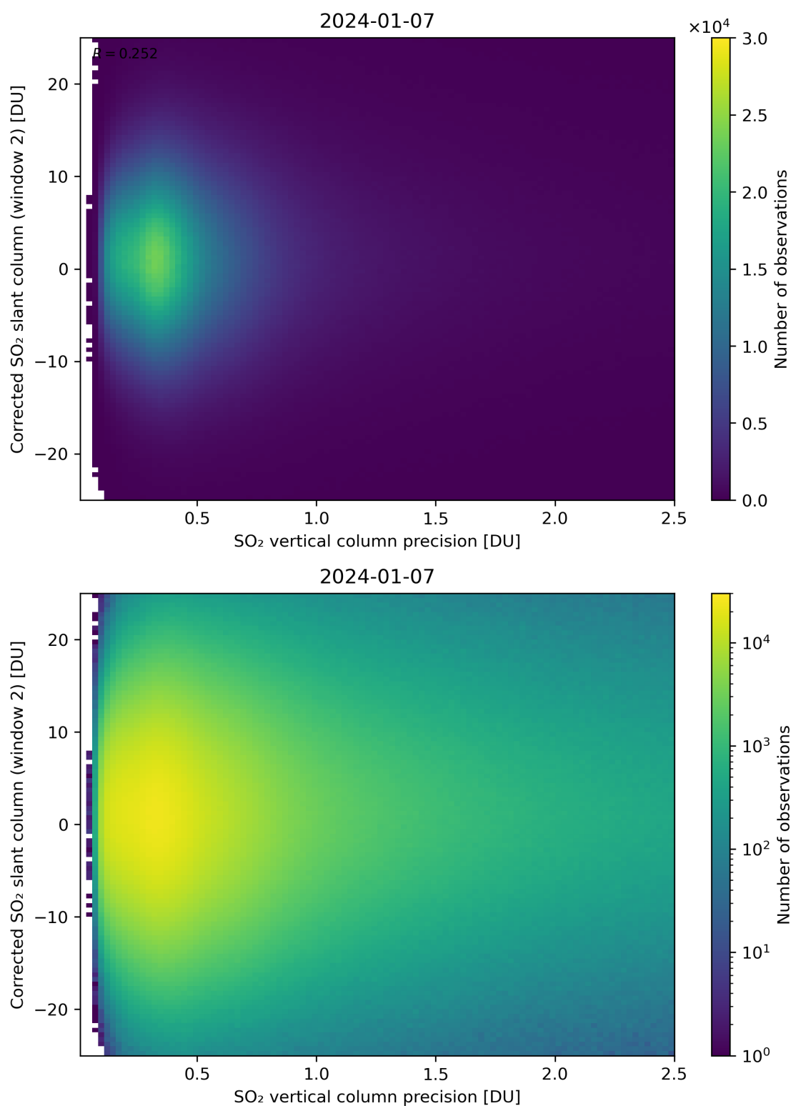
Figure 287: Scatter density plot of “SO 2 vertical column precision” against “Corrected SO 2 slant column (window 2)” for 2024-01-06 to 2024-01-08.
