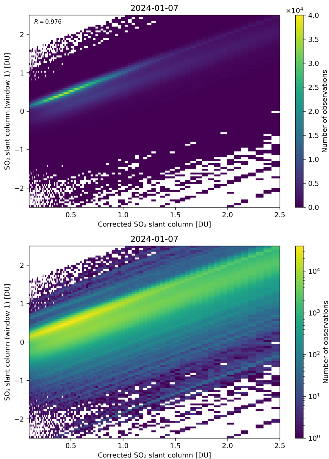
Figure 187: Scatter density plot of “Corrected SO 2 slant column” against “SO 2 slant column (window 1)” for 2024-01-06 to 2024-01-08.
