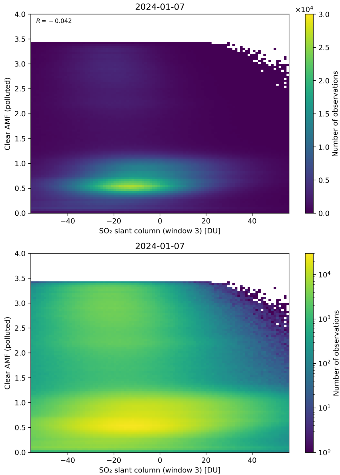
Figure 265: Scatter density plot of “SO 2 slant column (window 3)” against “Clear AMF (polluted)” for 2024-01-06 to 2024-01-08.
