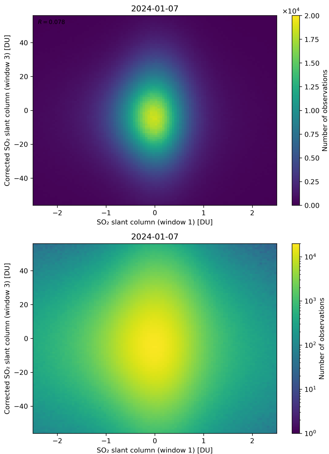
Figure 234: Scatter density plot of “SO 2 slant column (window 1)” against “Corrected SO 2 slant column (window 3)” for 2024-01-06 to 2024-01-08.
