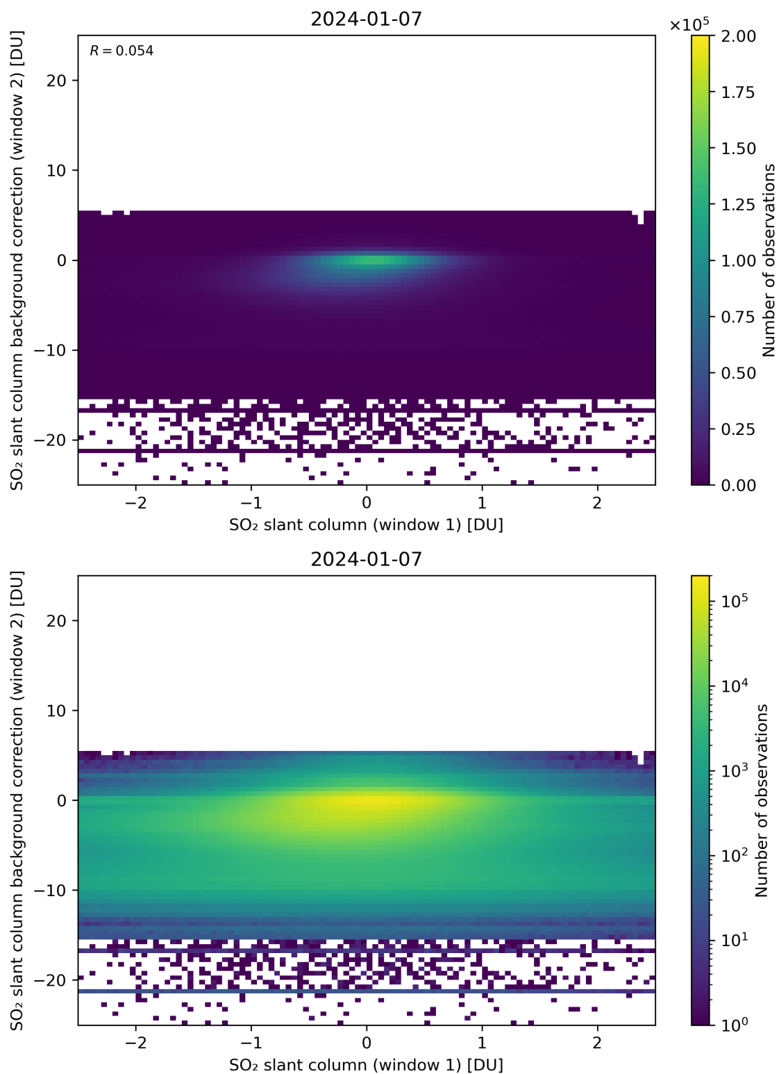
Figure 213: Scatter density plot of “SO 2 slant column (window 1)” against “SO 2 slant column background correction (window 2)” for 2024-01-06 to 2024-01-08.
