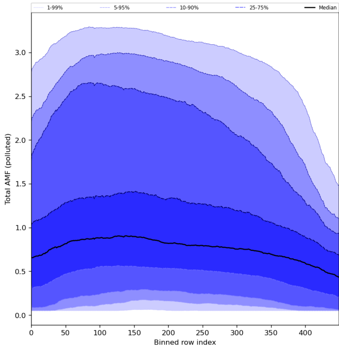
Figure 94: Along track statistics of “Total AMF (polluted)” for 2024-01-06 to 2024-01-08
