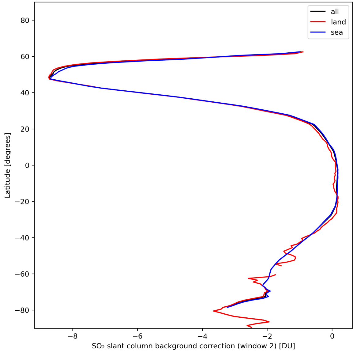
Figure 40: Zonal average of “SO 2 slant column background correction (window 2)” for 2024-01-06 to 2024-01-08.
