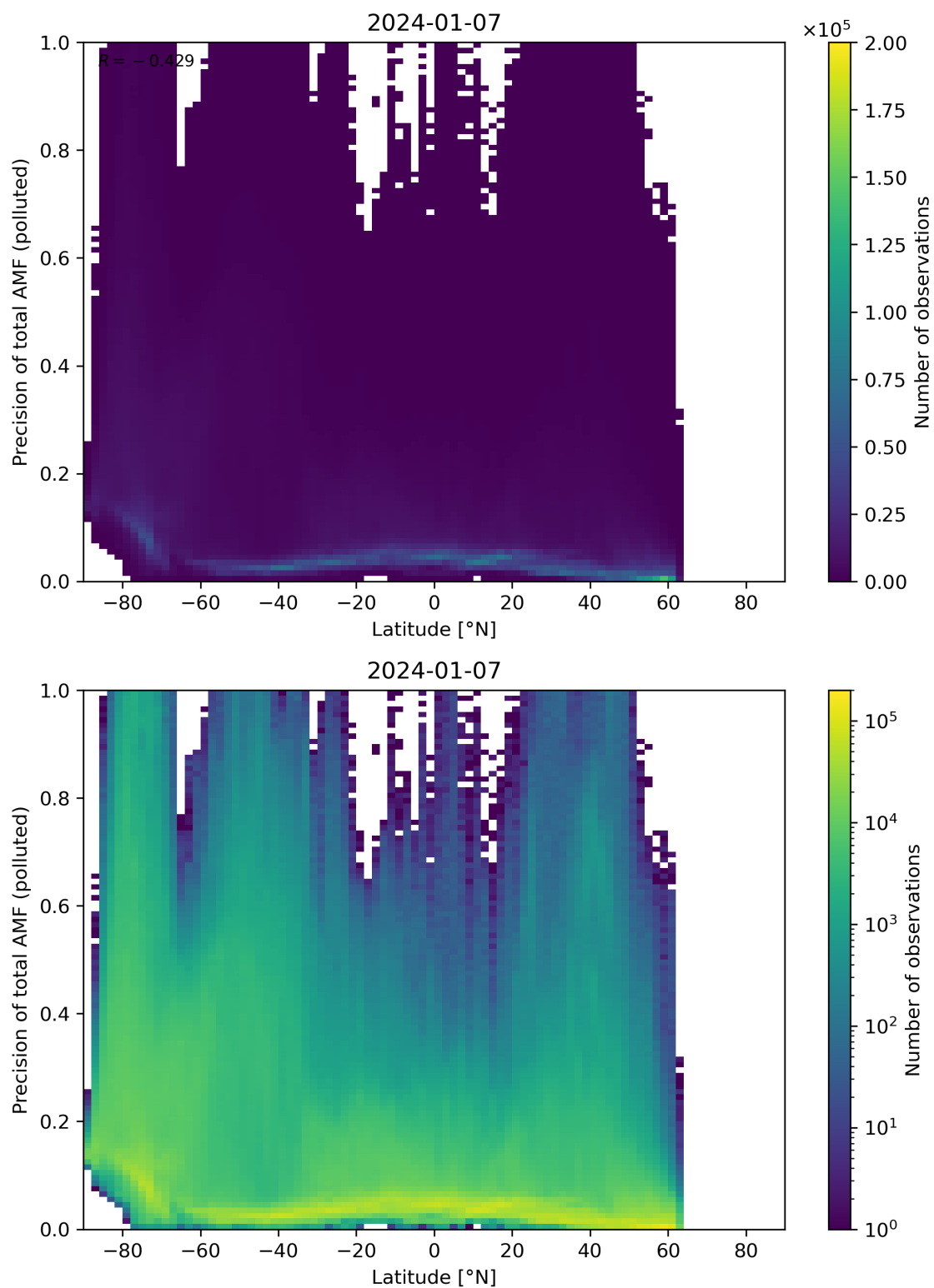
Figure 155: Scatter density plot of “Latitude” against “Precision of total AMF (polluted)” for 2024-01-06 to 2024-01-08.
