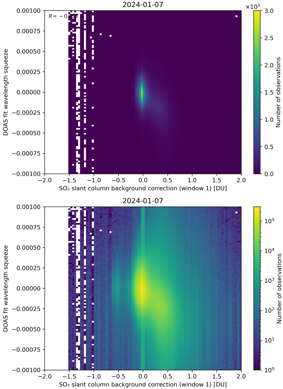
Figure 101: Scatter density plot of “SO 2 slant column background correction (window 1)” against “DOAS fit wavelength squeeze” for 2024-01-06 to 2024-01-08.
