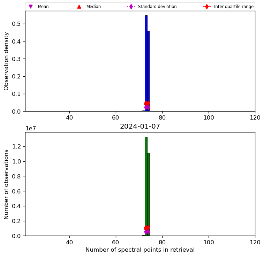
Figure 74: Histogram of “Number of spectral points in retrieval” for 2024-01-06 to 2024-01-08
