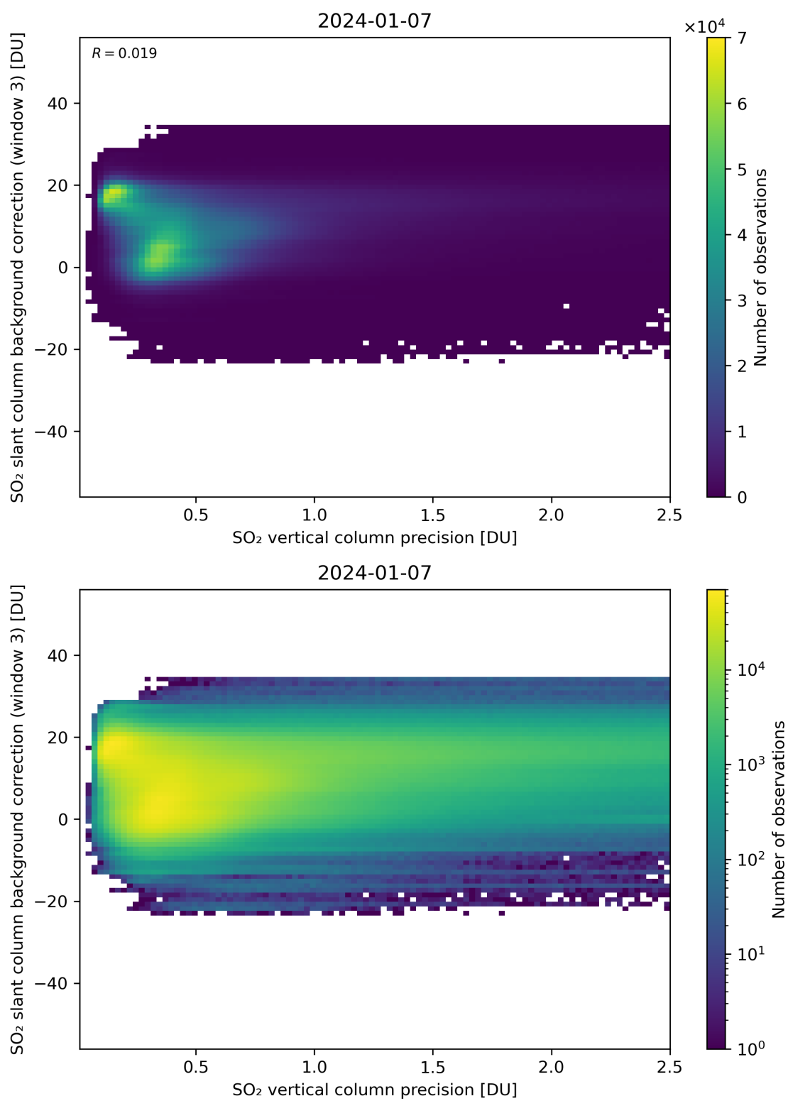
Figure 281: Scatter density plot of “SO 2 vertical column precision” against “SO 2 slant column background correction (window 3)” for 2024-01-06 to 2024-01-08.
