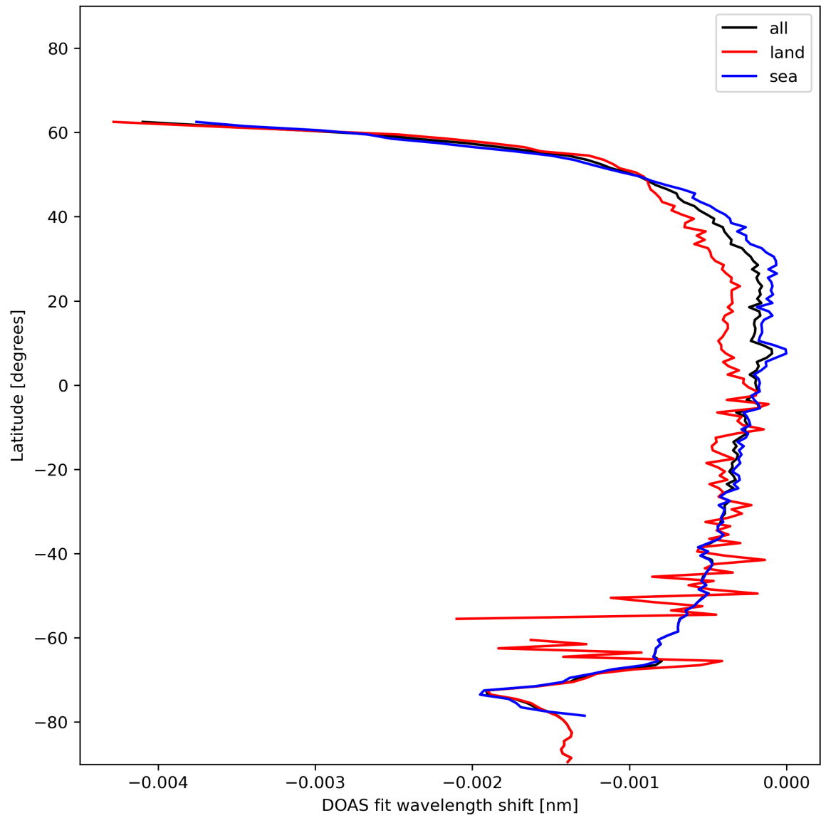
Figure 45: Zonal average of “DOAS fit wavelength shift” for 2024-01-06 to 2024-01-08.
