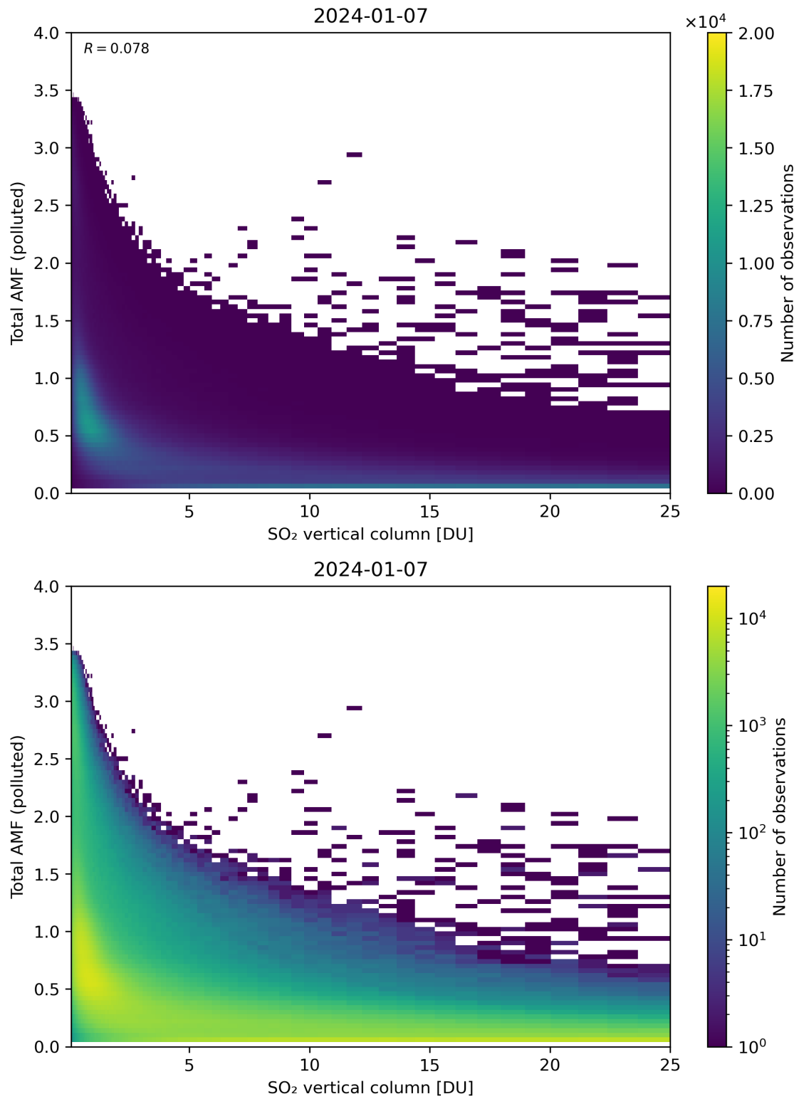
Figure 305: Scatter density plot of “SO 2 vertical column” against “Total AMF (polluted)” for 2024-01-06 to 2024-01-08.
