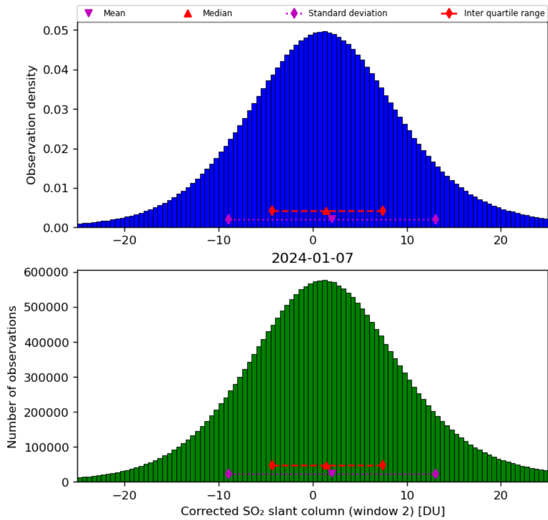
Figure 62: Histogram of “Corrected SO 2 slant column (window 2)” for 2024-01-06 to 2024-01-08
