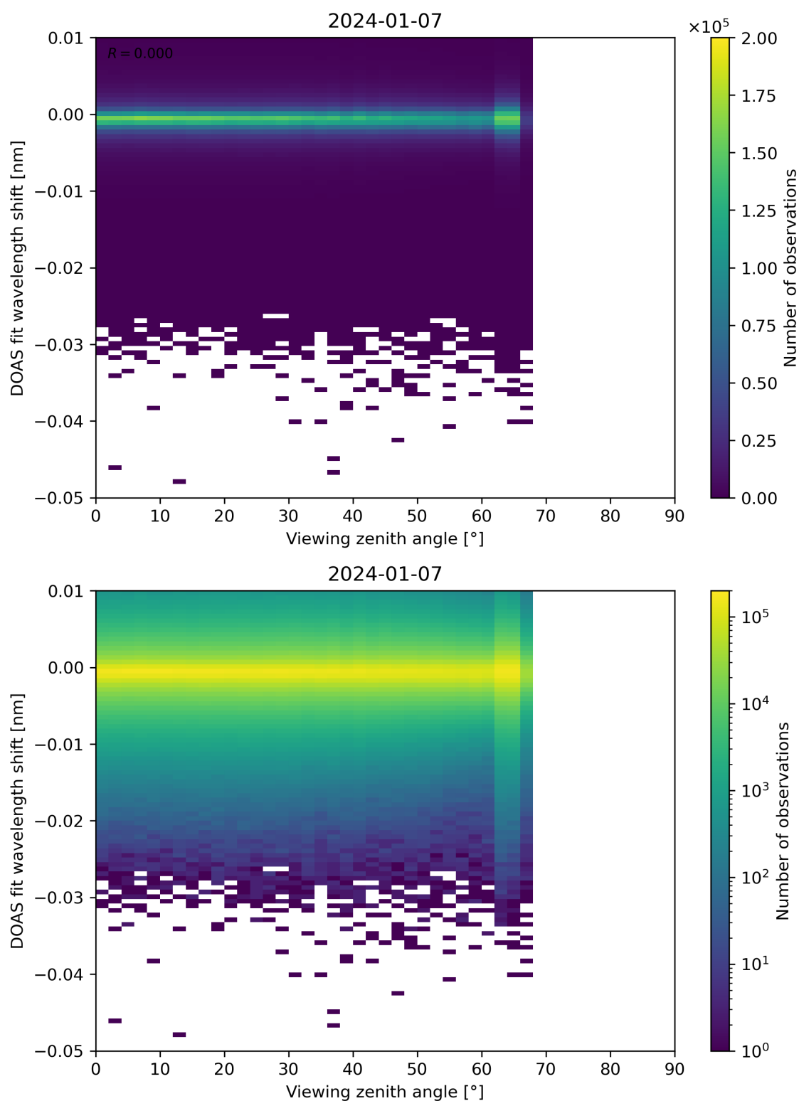
Figure 311: Scatter density plot of “Viewing zenith angle” against “DOAS fit wavelength shift” for 2024-01-06 to 2024-01-08.
