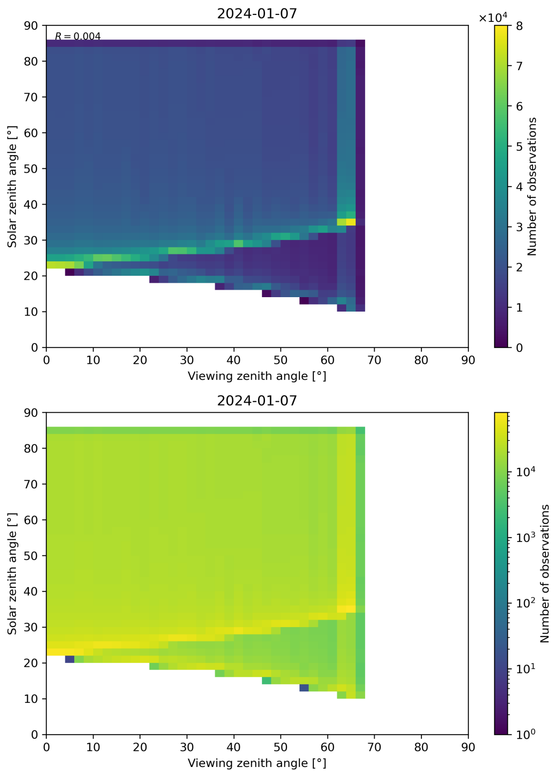
Figure 315: Scatter density plot of “Viewing zenith angle” against “Solar zenith angle” for 2024-01-06 to 2024-01-08.
