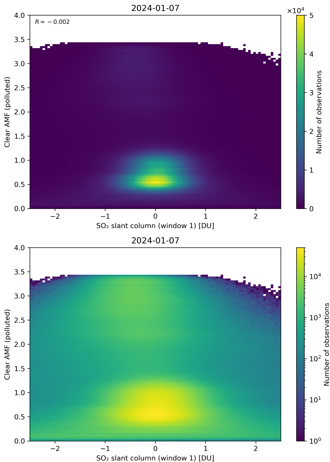
Figure 232: Scatter density plot of “SO 2 slant column (window 1)” against “Clear AMF (polluted)” for 2024-01-06 to 2024-01-08.
