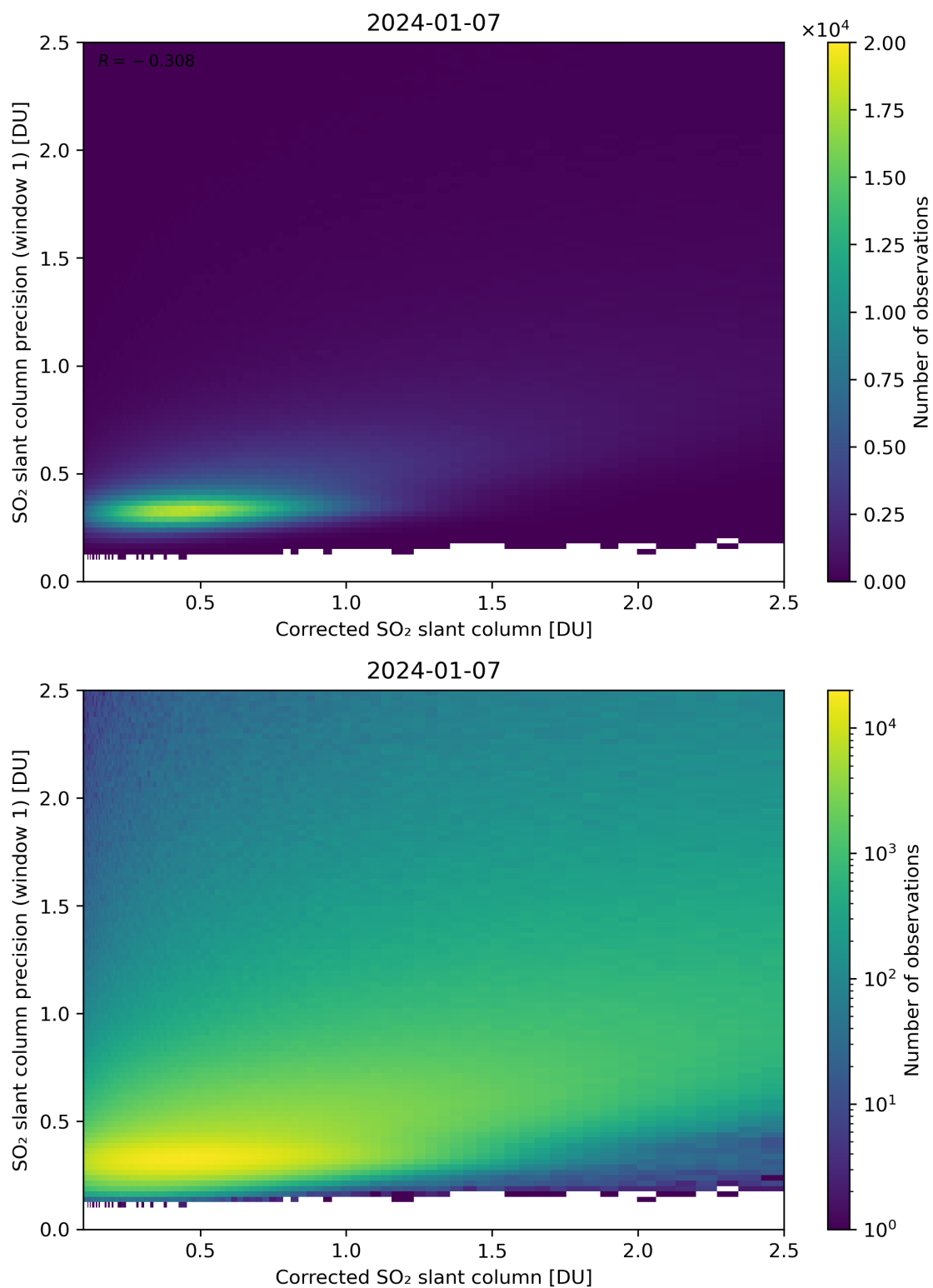
Figure 188: Scatter density plot of “Corrected SO 2 slant column” against “SO 2 slant column precision (window 1)” for 2024-01-06 to 2024-01-08.
