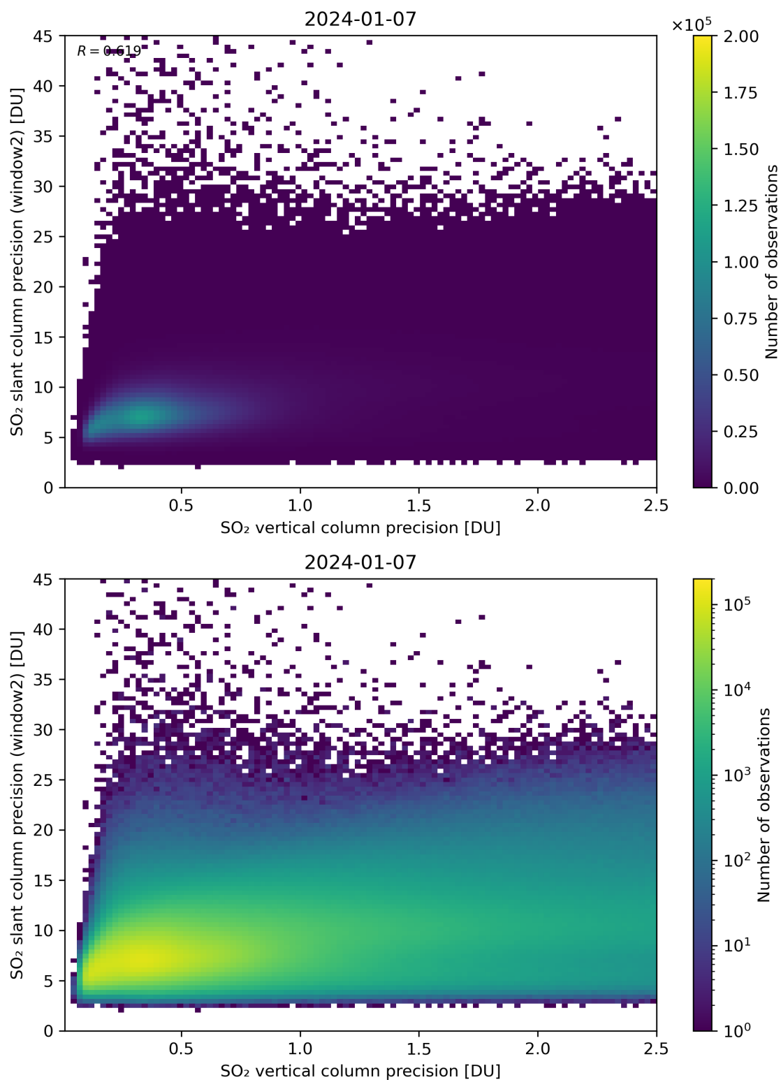
Figure 291: Scatter density plot of “SO 2 vertical column precision” against “SO 2 slant column precision (window2)” for 2024-01-06 to 2024-01-08.
