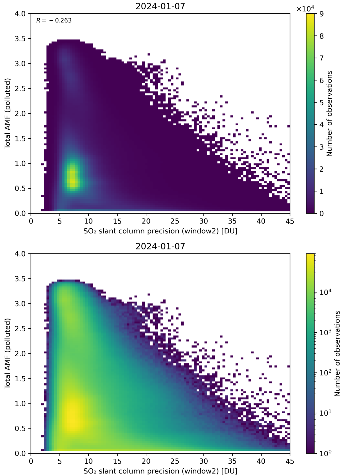
Figure 251: Scatter density plot of “SO 2 slant column precision (window2)” against “Total AMF (polluted)” for 2024-01-06 to 2024-01-08.
