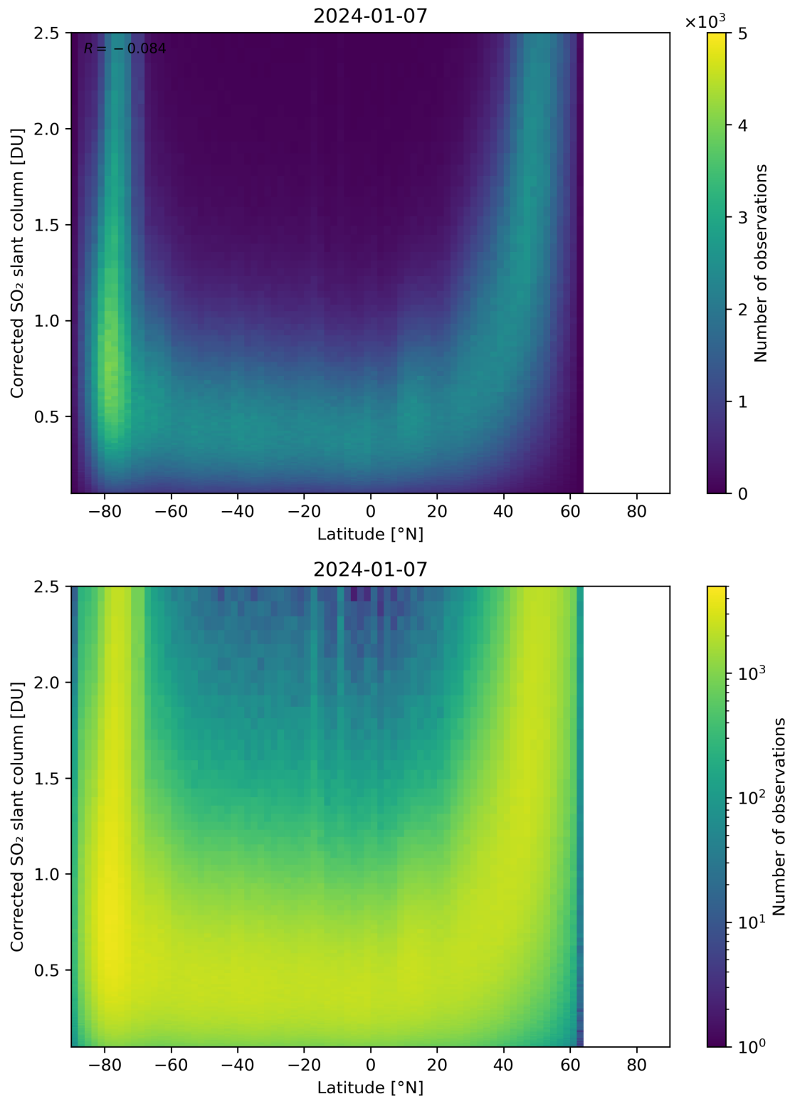
Figure 146: Scatter density plot of “Latitude” against “Corrected SO 2 slant column” for 2024-01-06 to 2024-01-08.
