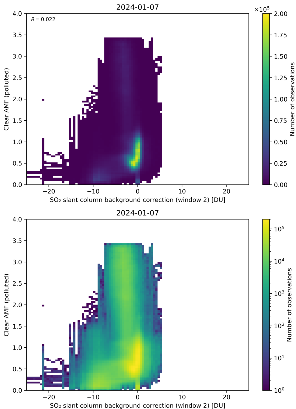
Figure 115: Scatter density plot of “SO 2 slant column background correction (window 2)” against “Clear AMF (polluted)” for 2024-01-06 to 2024-01-08.
