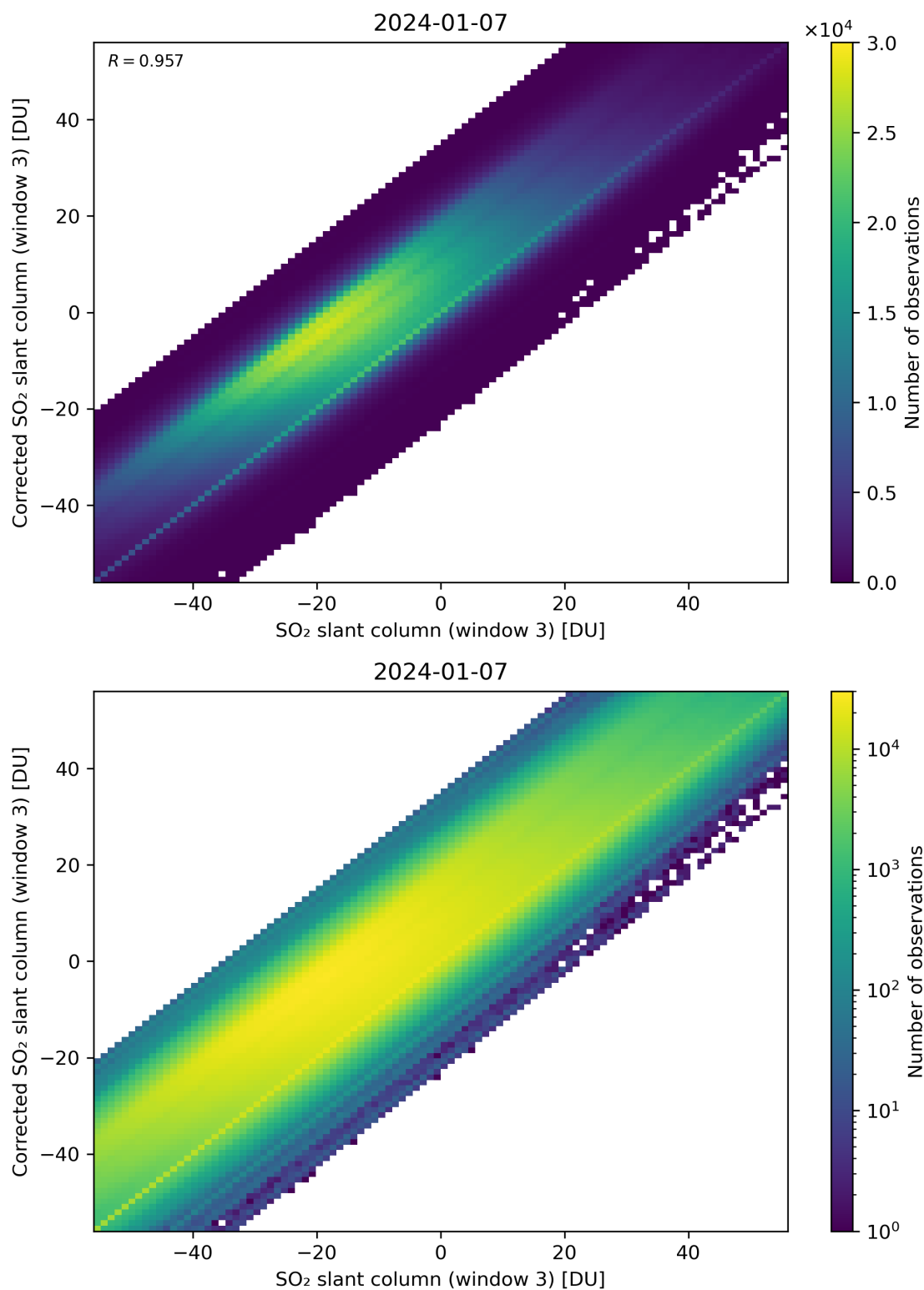
Figure 266: Scatter density plot of “SO 2 slant column (window 3)” against “Corrected SO 2 slant column (window 3)” for 2024-01-06 to 2024-01-08.
