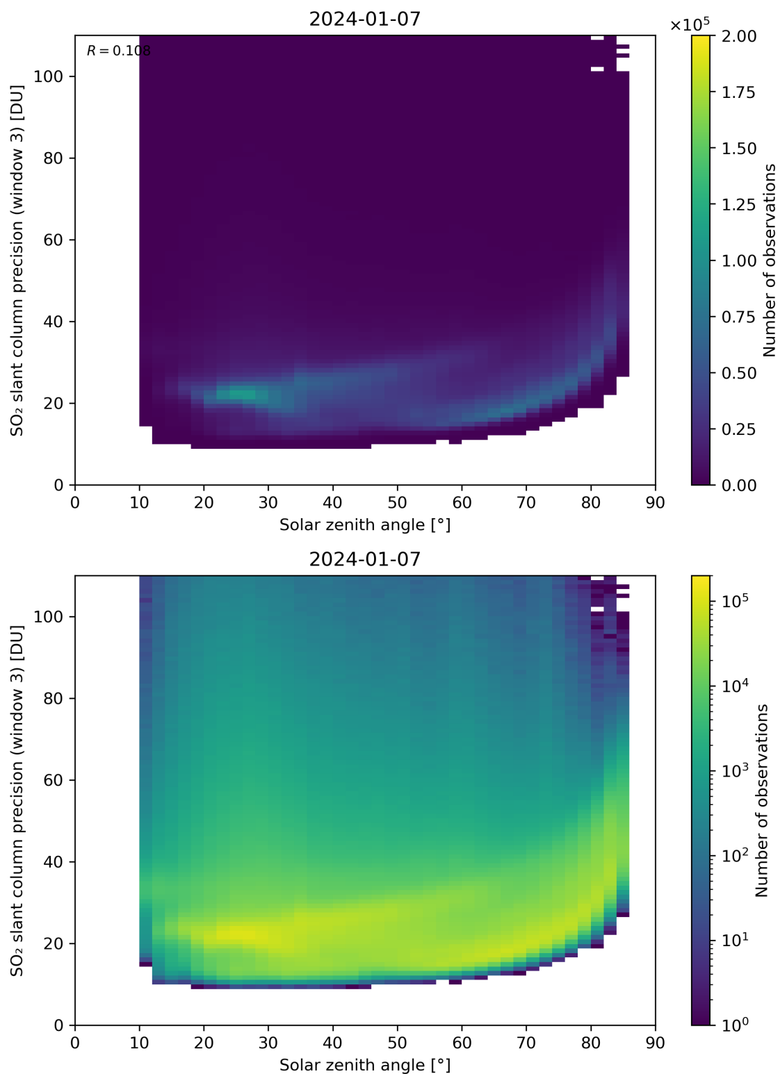
Figure 173: Scatter density plot of “Solar zenith angle” against “SO 2 slant column precision (window 3)” for 2024-01-06 to 2024-01-08.
