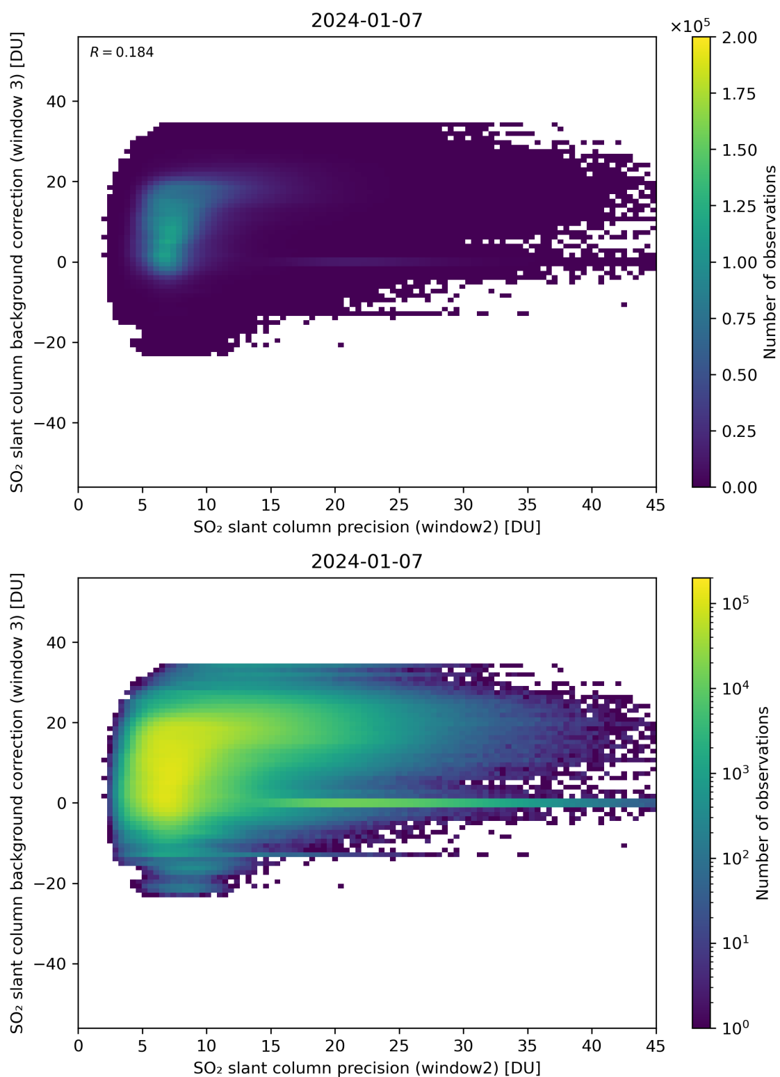
Figure 242: Scatter density plot of “SO 2 slant column precision (window2)” against “SO 2 slant column background correction (window 3)” for 2024-01-06 to 2024-01-08.
