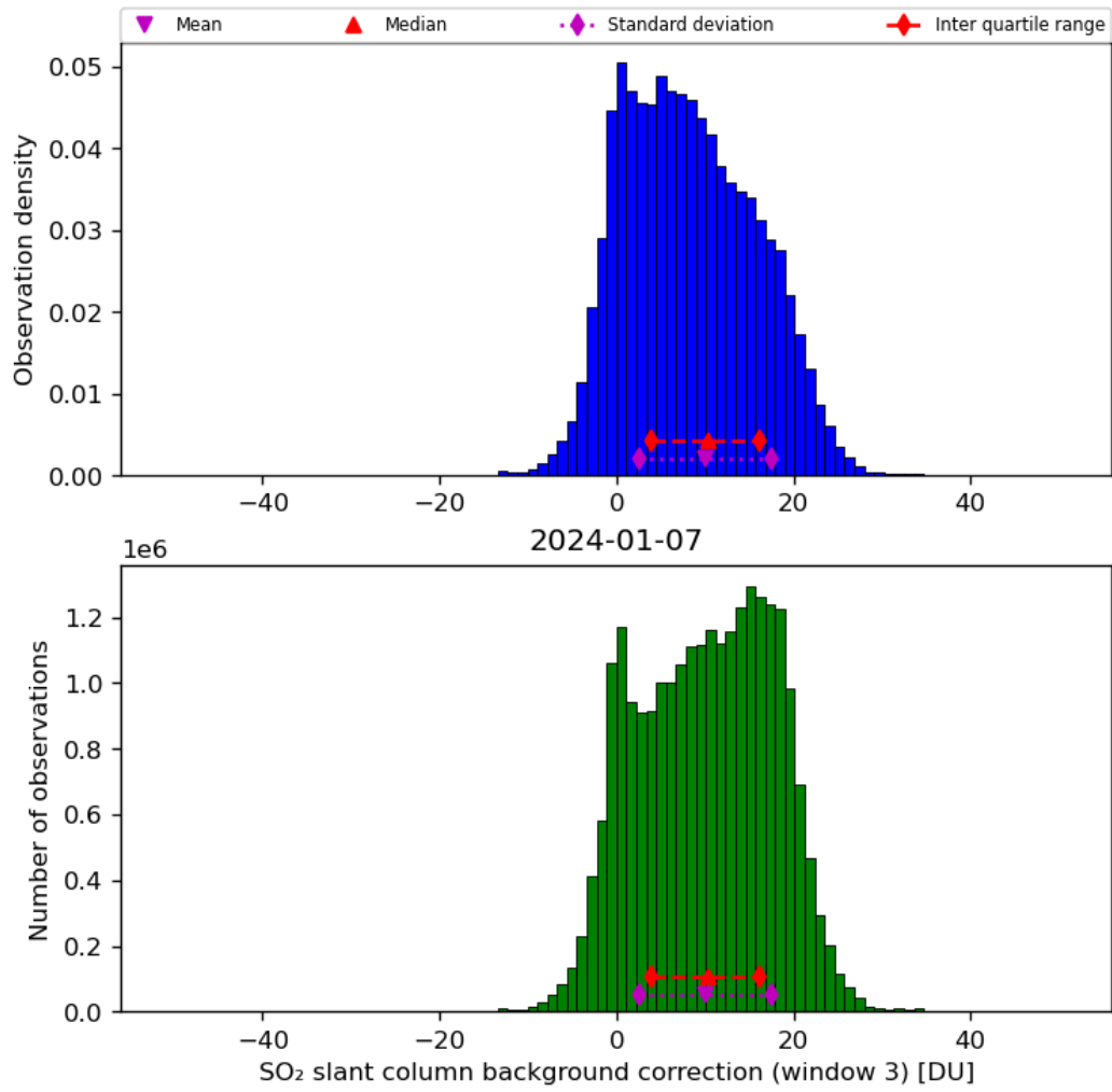
Figure 67: Histogram of “SO 2 slant column background correction (window 3)” for 2024-01-06 to 2024-01-08
