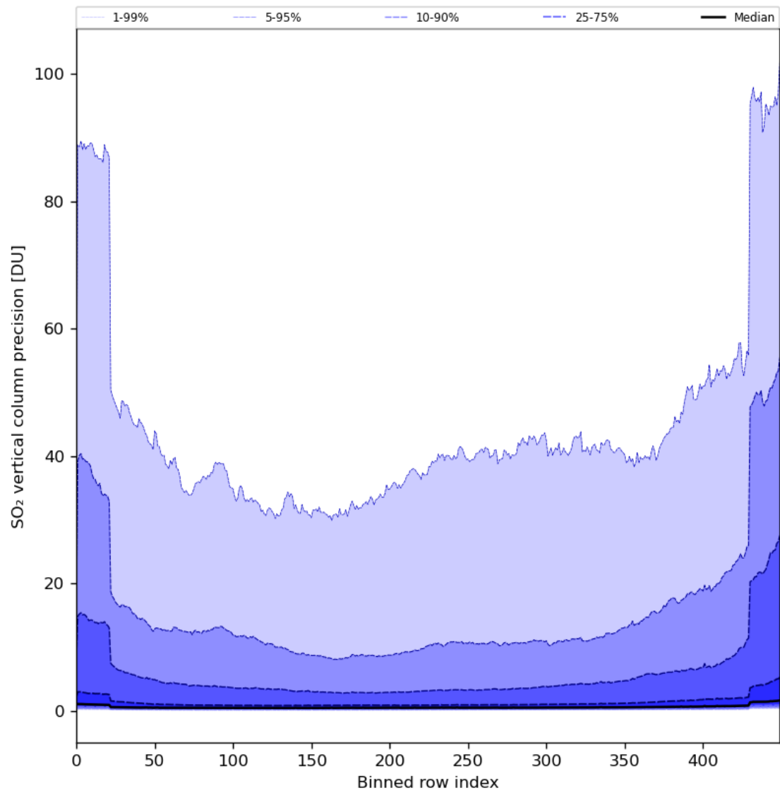
Figure 77: Along track statistics of “SO 2 vertical column precision” for 2024-01-06 to 2024-01-08
