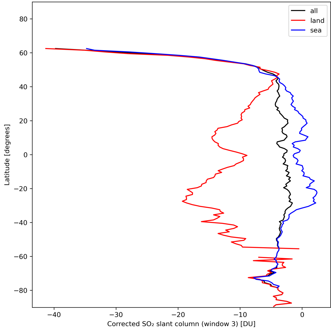
Figure 43: Zonal average of “Corrected SO 2 slant column (window 3)” for 2024-01-06 to 2024-01-08.
