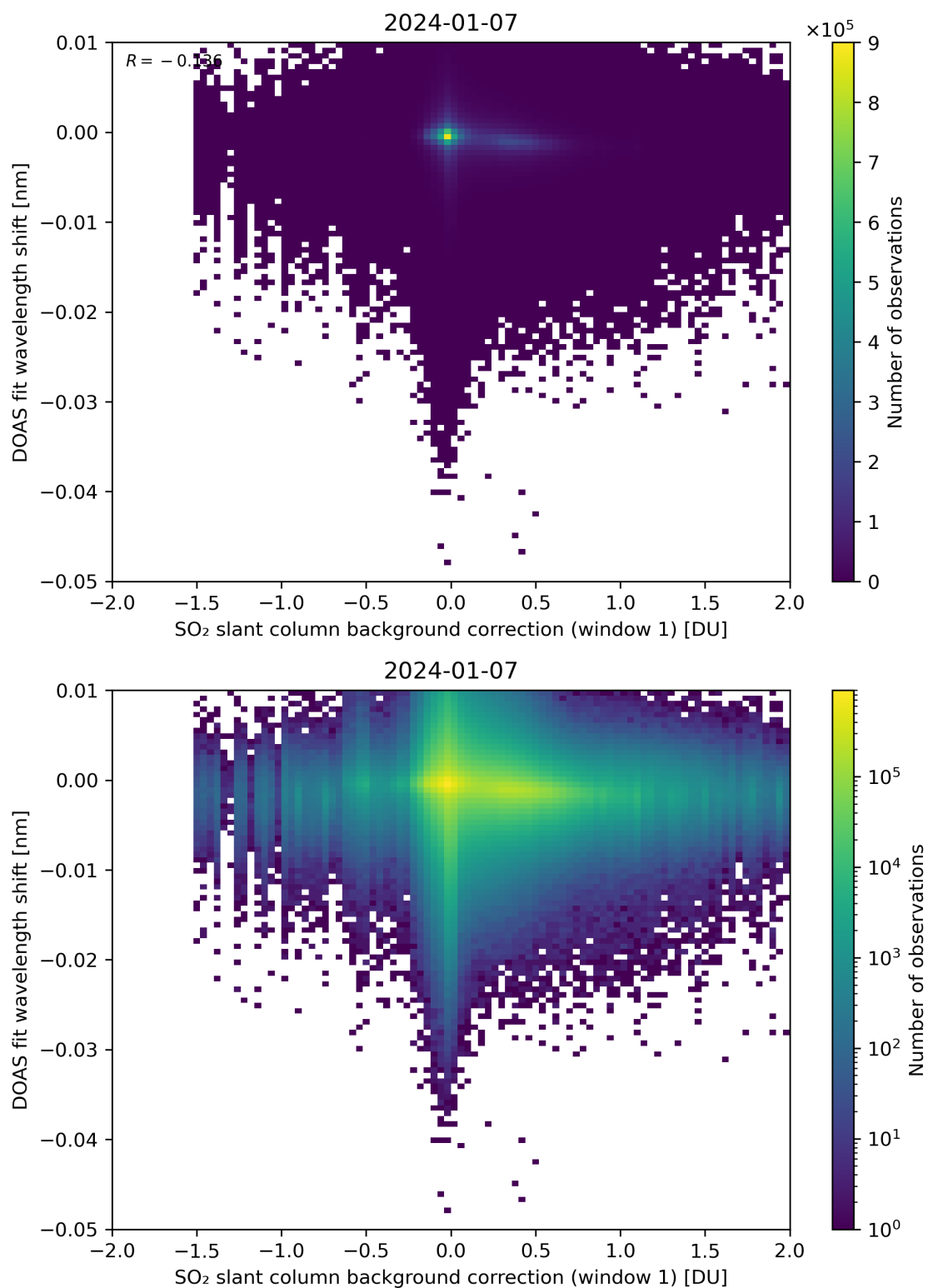
Figure 100: Scatter density plot of “SO 2 slant column background correction (window 1)” against “DOAS fit wavelength shift” for 2024-01-06 to 2024-01-08.
