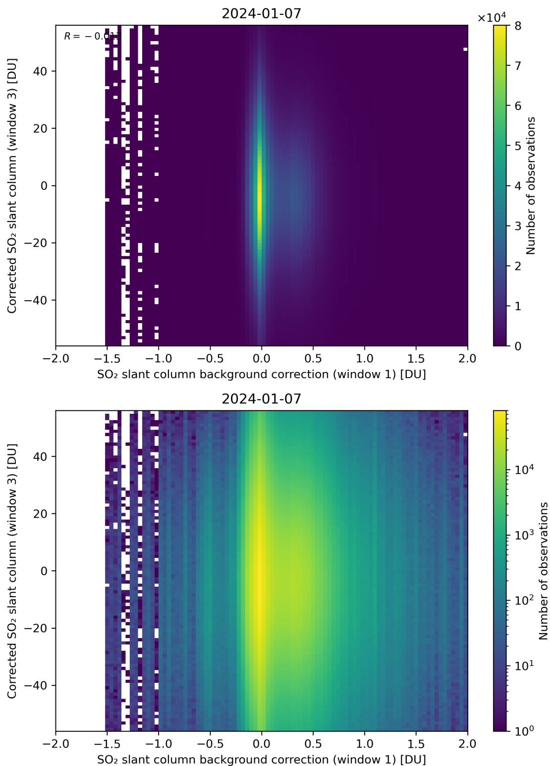
Figure 105: Scatter density plot of “SO 2 slant column background correction (window 1)” against “Corrected SO 2 slant column (window 3)” for 2024-01-06 to 2024-01-08.
