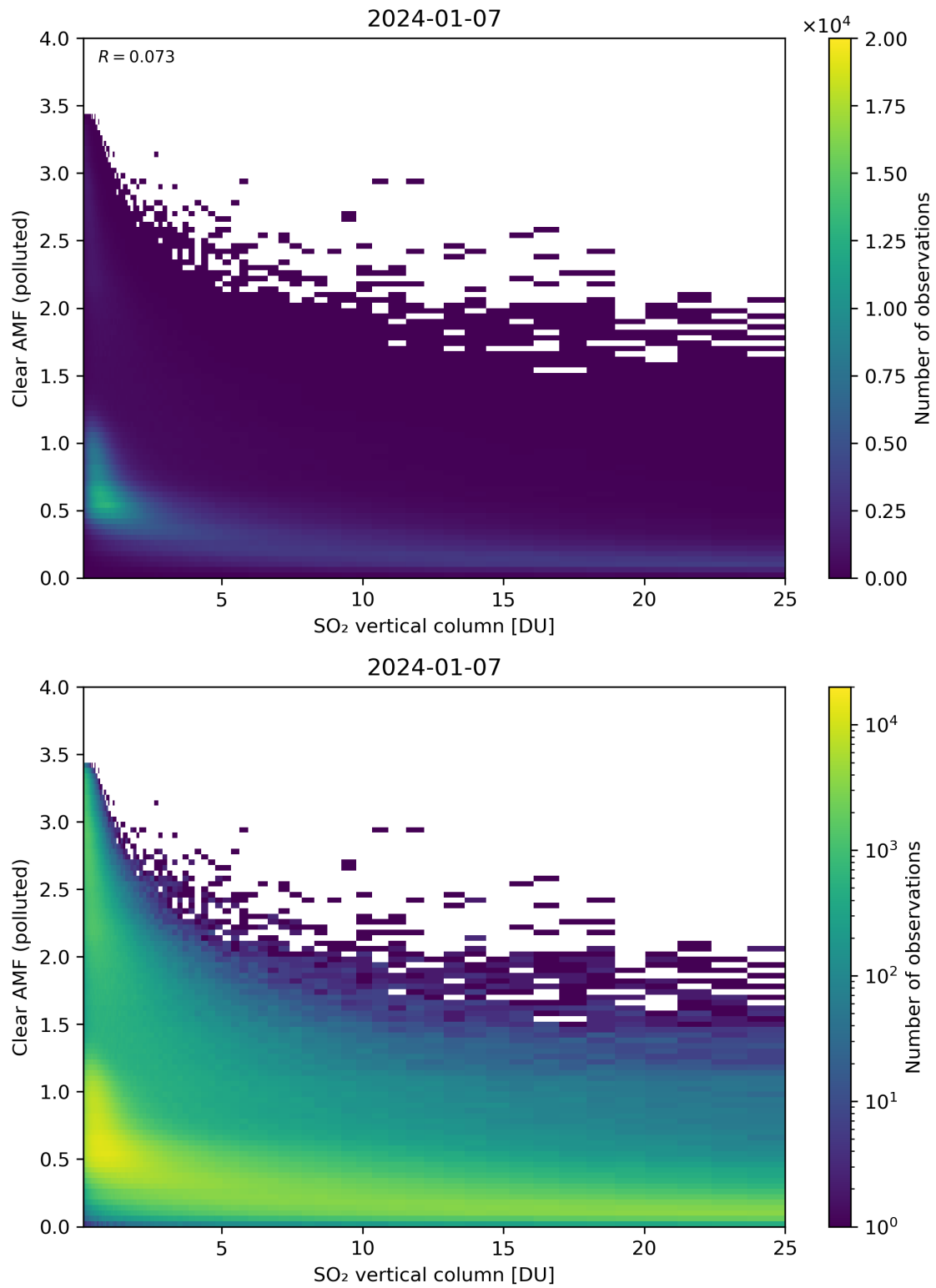
Figure 296: Scatter density plot of “SO 2 vertical column” against “Clear AMF (polluted)” for 2024-01-06 to 2024-01-08.
