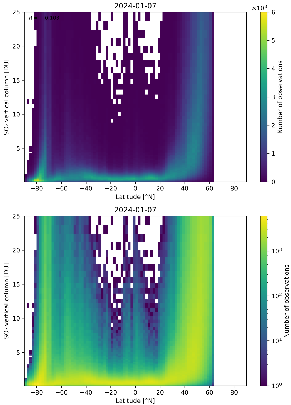
Figure 156: Scatter density plot of “Latitude” against “SO 2 vertical column” for 2024-01-06 to 2024-01-08.
