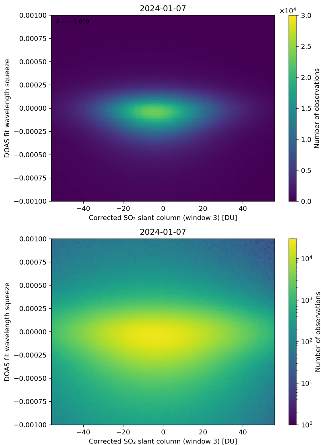
Figure 207: Scatter density plot of “Corrected SO 2 slant column (window 3)” against “DOAS fit wavelength squeeze” for 2024-01-06 to 2024-01-08.
