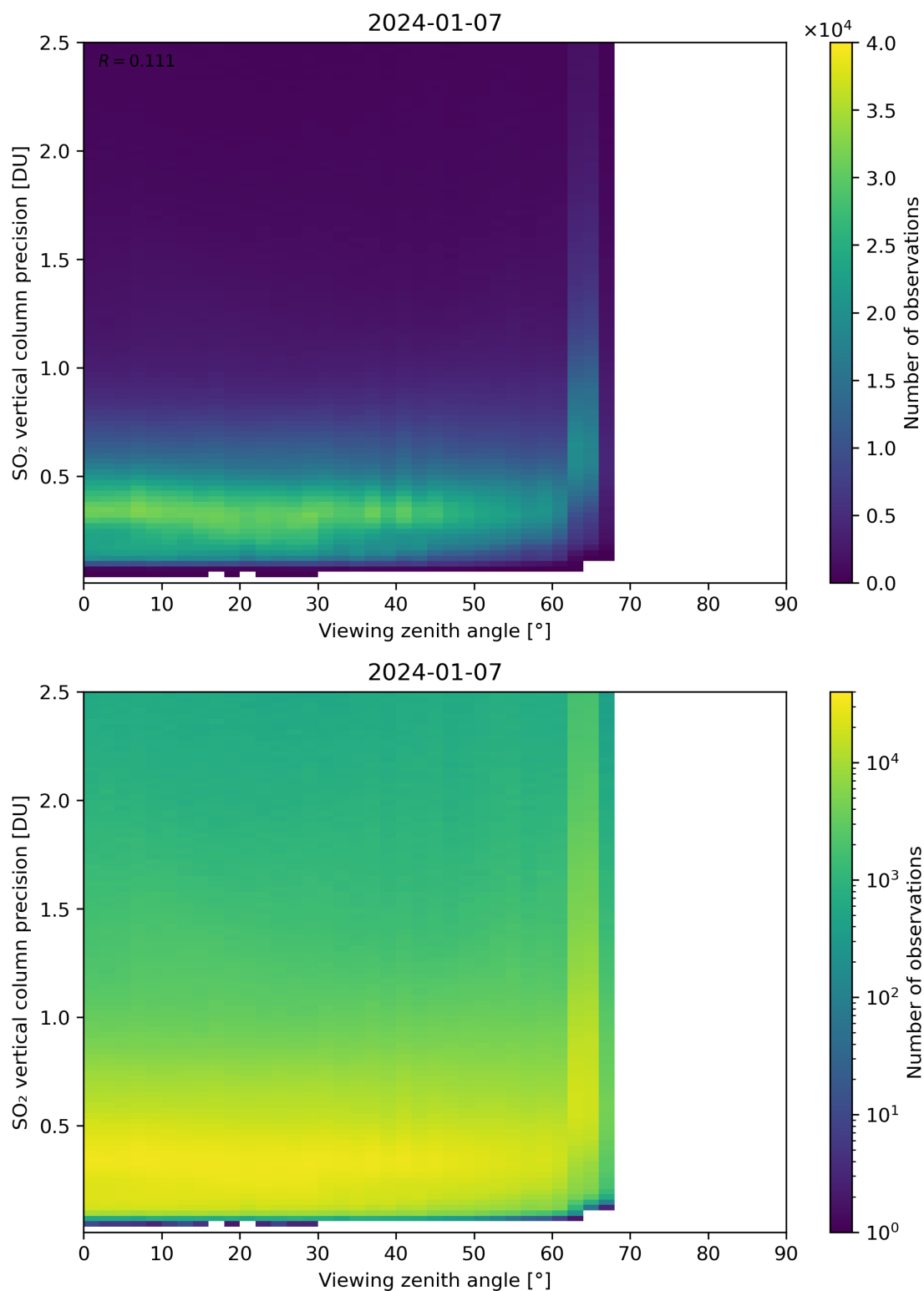
Figure 328: Scatter density plot of “Viewing zenith angle” against “SO 2 vertical column precision” for 2024-01-06 to 2024-01-08.
