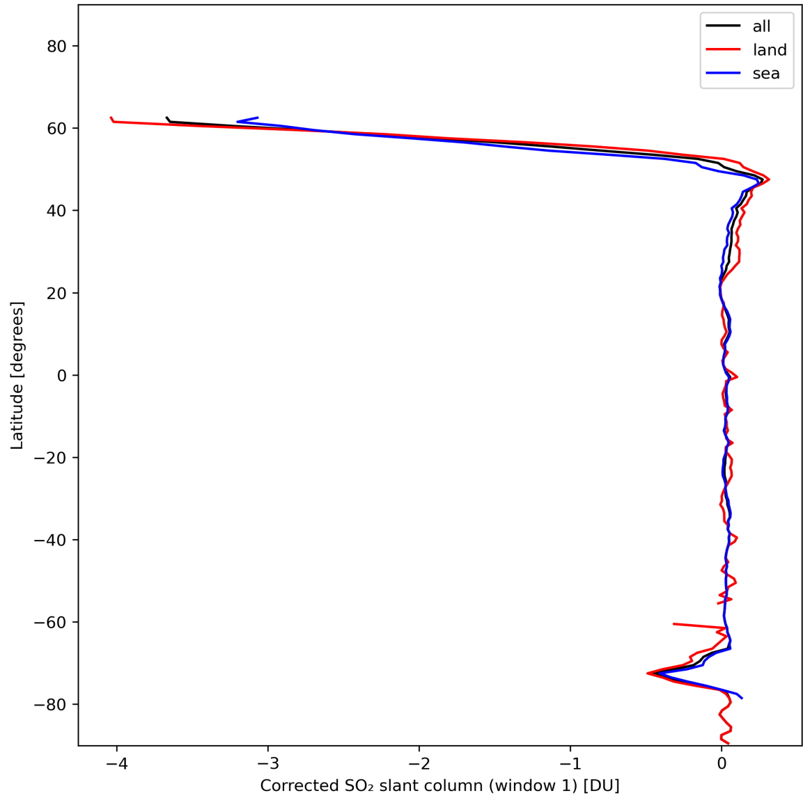
Figure 35: Zonal average of “Corrected SO 2 slant column (window 1)” for 2024-01-06 to 2024-01-08.
