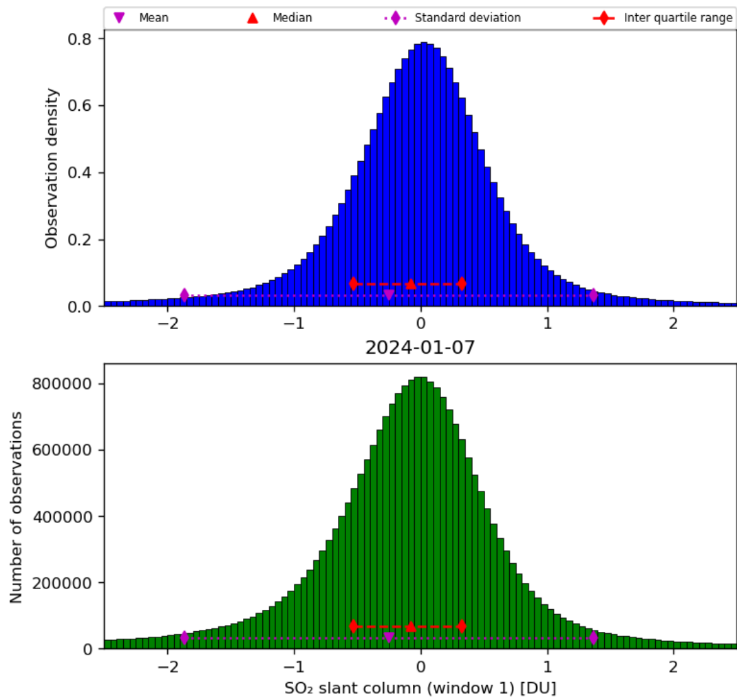
Figure 56: Histogram of “SO 2 slant column (window 1)” for 2024-01-06 to 2024-01-08
