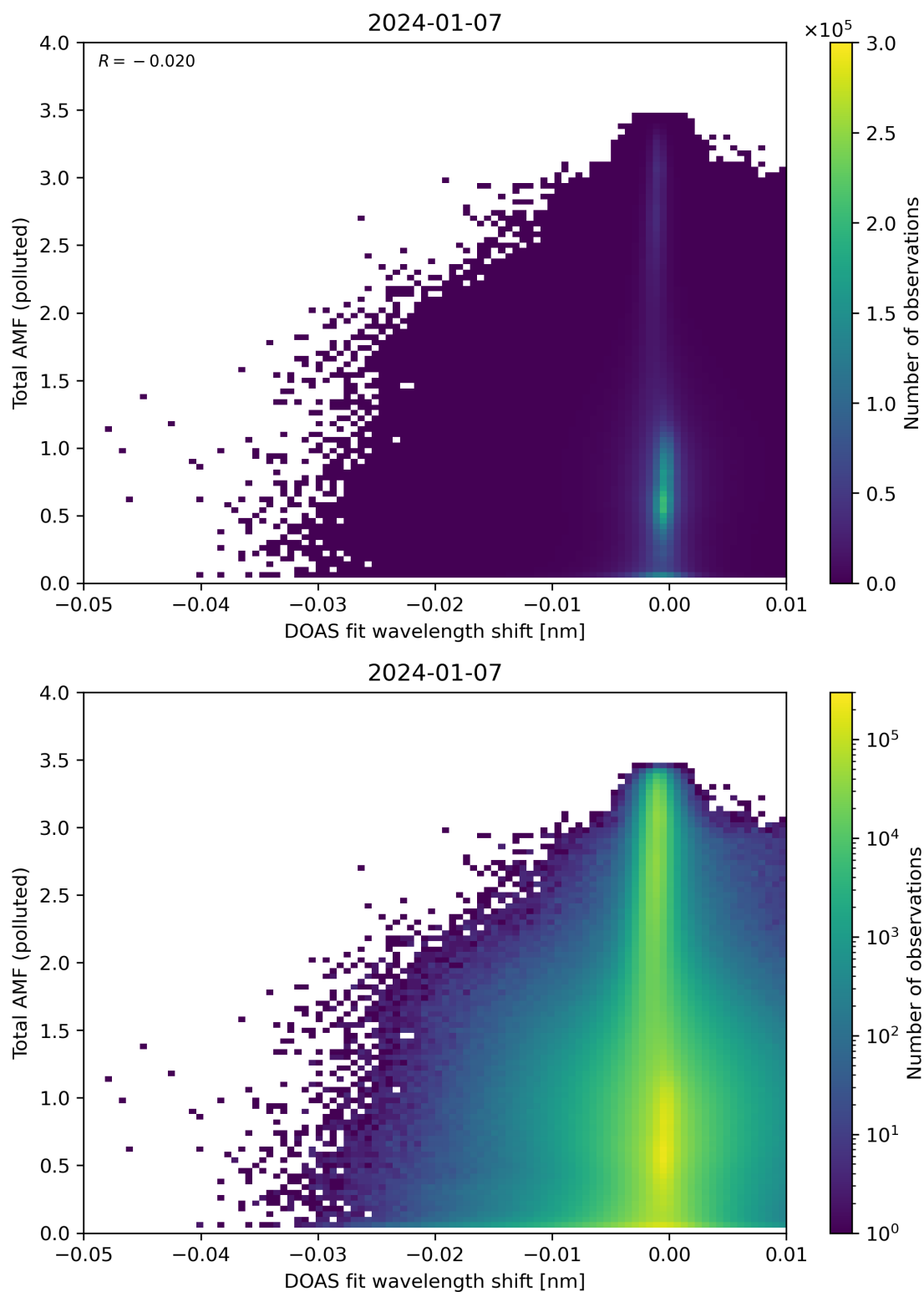
Figure 130: Scatter density plot of “DOAS fit wavelength shift” against “Total AMF (polluted)” for 2024-01-06 to 2024-01-08.
