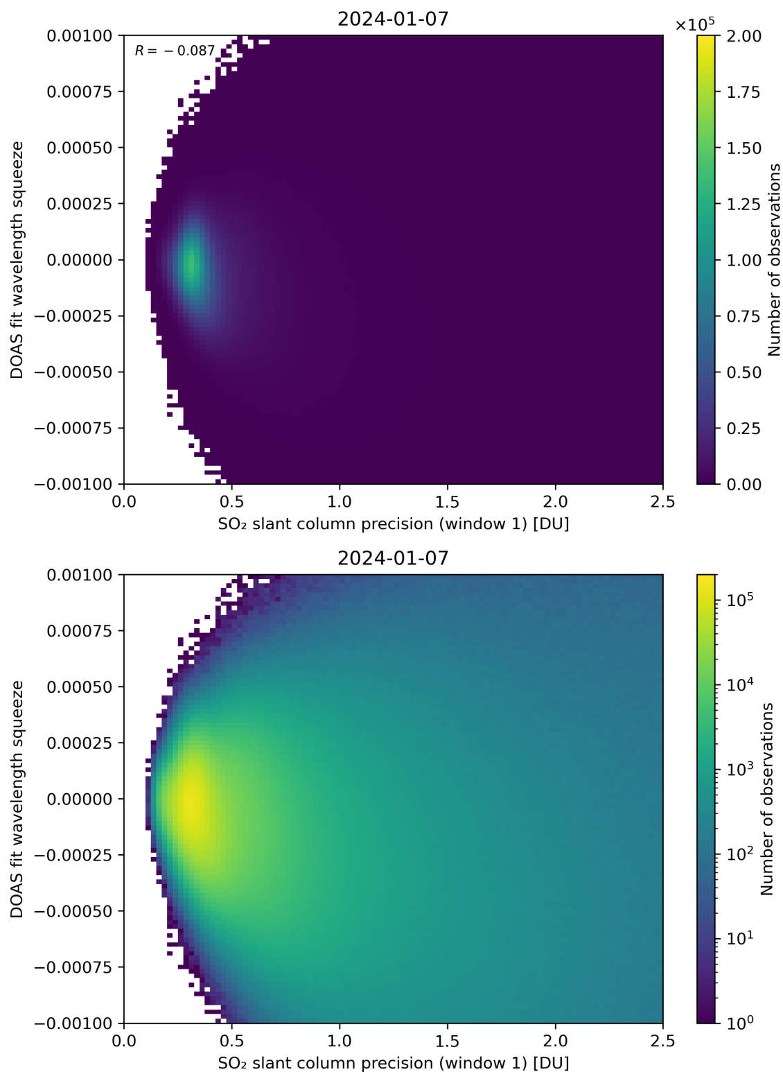
Figure 222: Scatter density plot of “SO 2 slant column precision (window 1)” against “DOAS fit wavelength squeeze” for 2024-01-06 to 2024-01-08.
