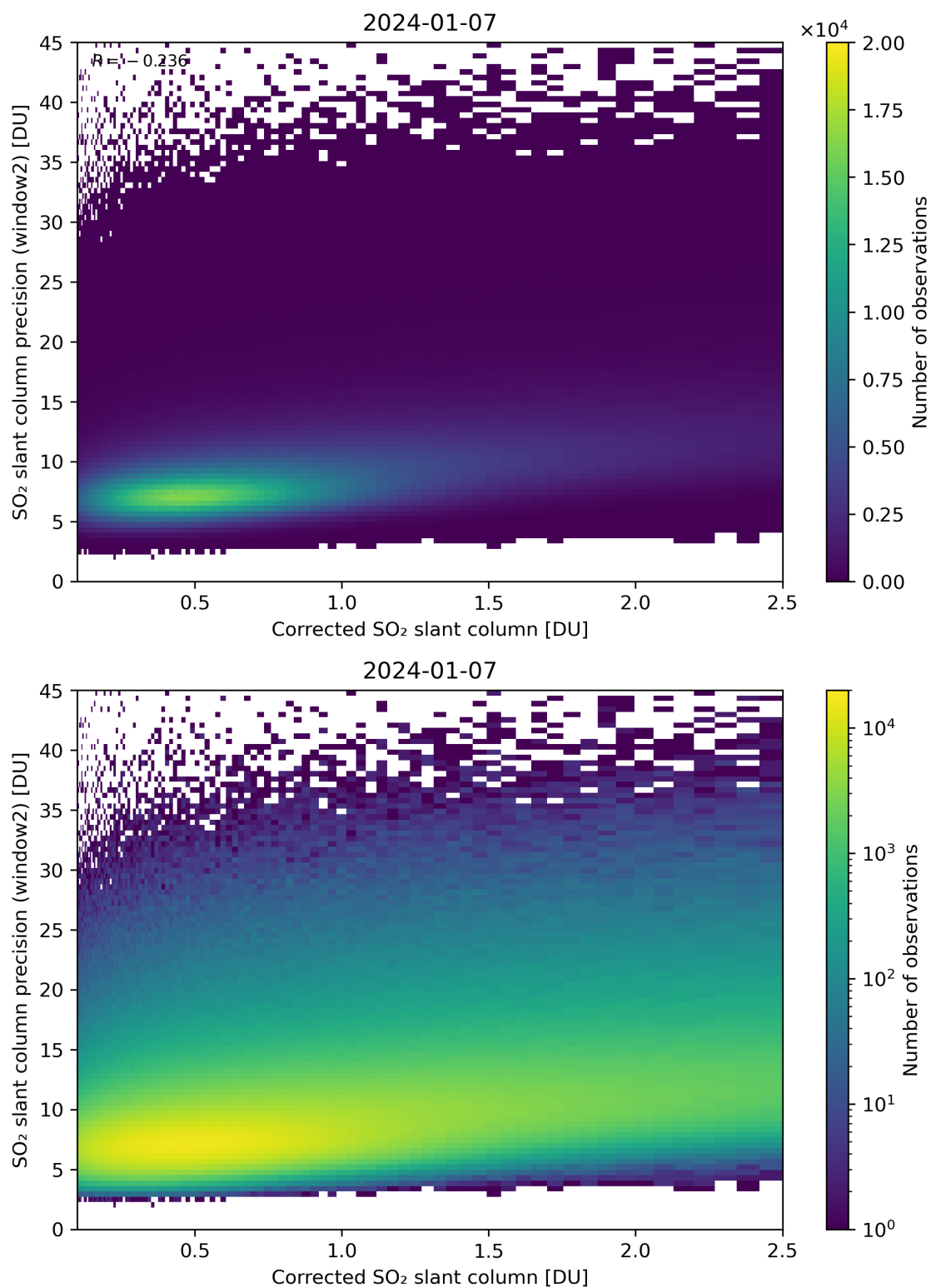
Figure 189: Scatter density plot of “Corrected SO 2 slant column” against “SO 2 slant column precision (window2)” for 2024-01-06 to 2024-01-08.
