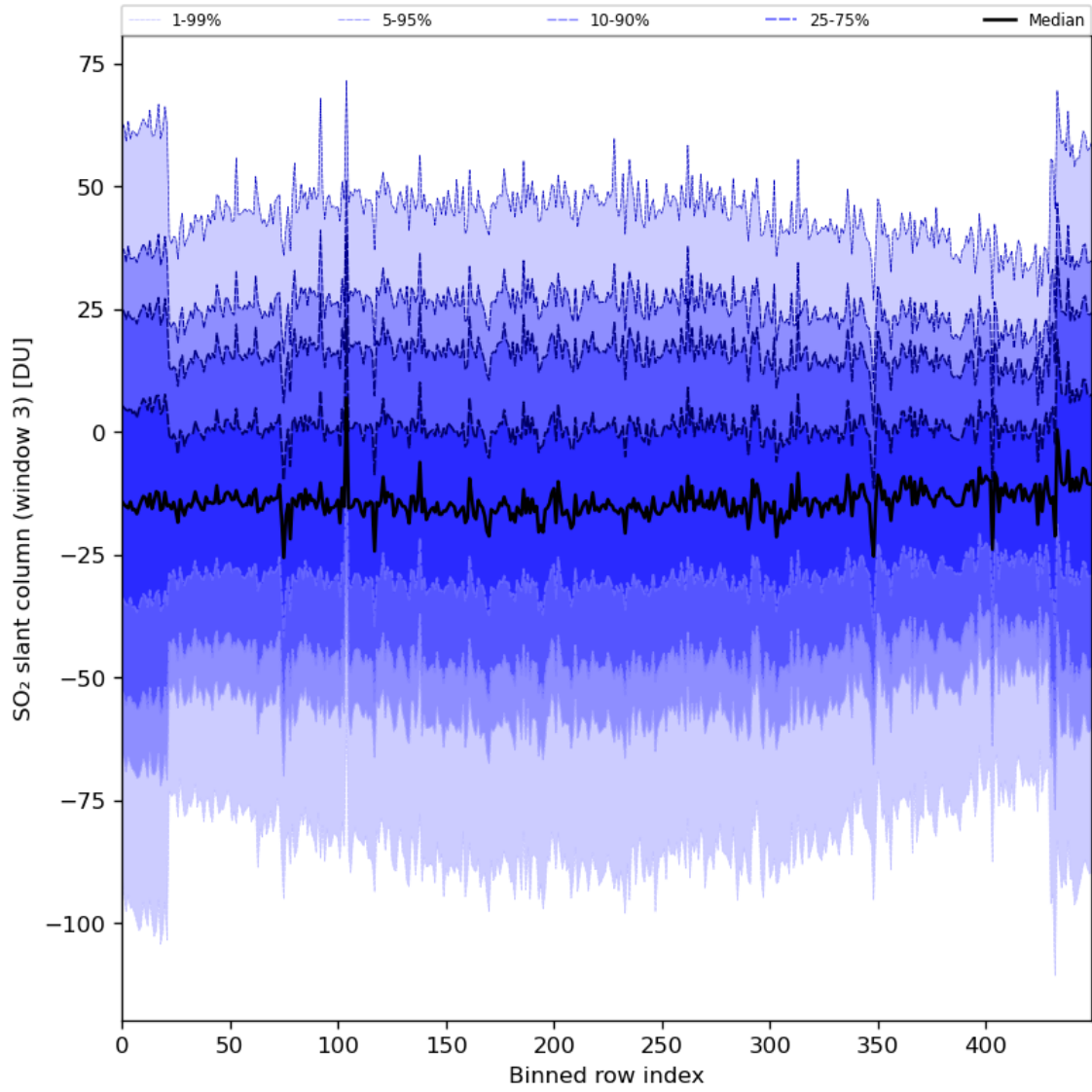
Figure 87: Along track statistics of “SO 2 slant column (window 3)” for 2024-01-06 to 2024-01-08
