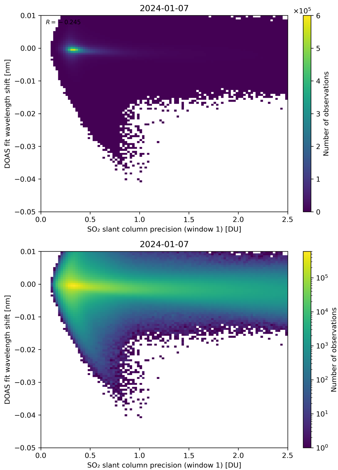
Figure 221: Scatter density plot of “SO 2 slant column precision (window 1)” against “DOAS fit wavelength shift” for 2024-01-06 to 2024-01-08.
