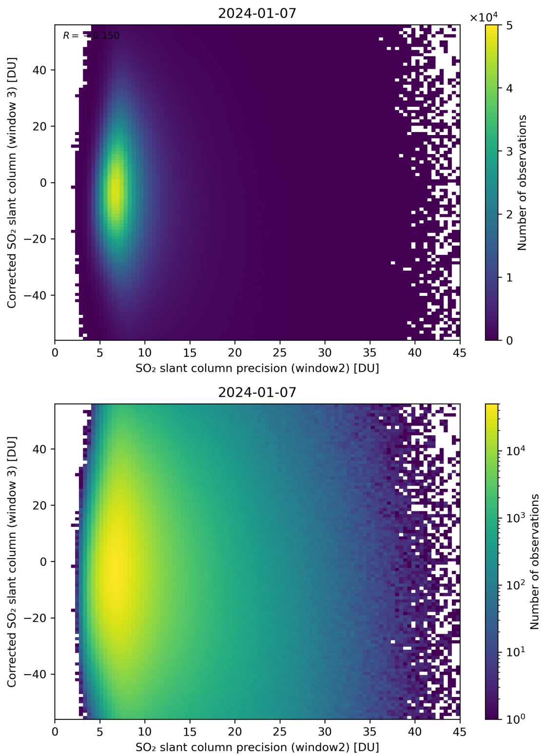
Figure 248: Scatter density plot of “SO 2 slant column precision (window2)” against “Corrected SO 2 slant column (window 3)” for 2024-01-06 to 2024-01-08.
