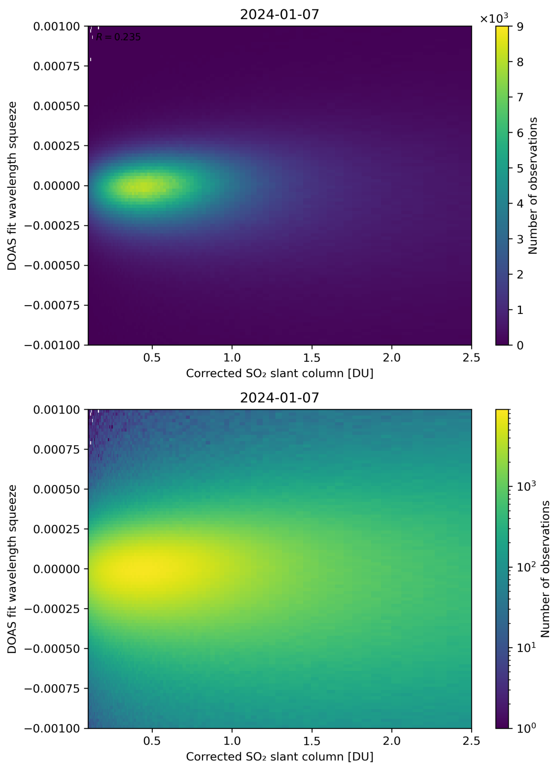
Figure 182: Scatter density plot of “Corrected SO 2 slant column” against “DOAS fit wavelength squeeze” for 2024-01-06 to 2024-01-08.
