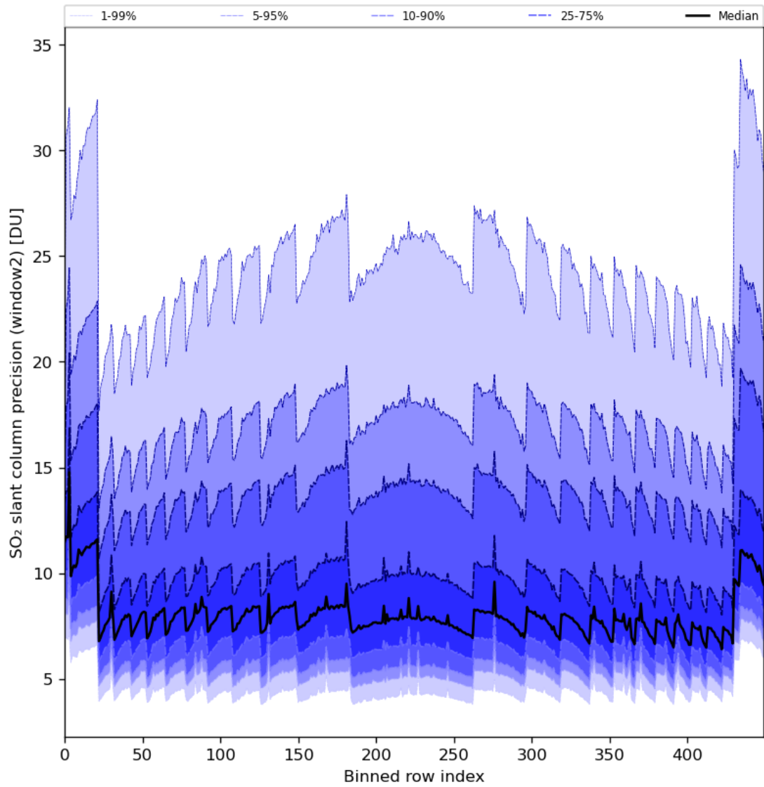
Figure 84: Along track statistics of “SO 2 slant column precision (window2)” for 2024-01-06 to 2024-01-08
