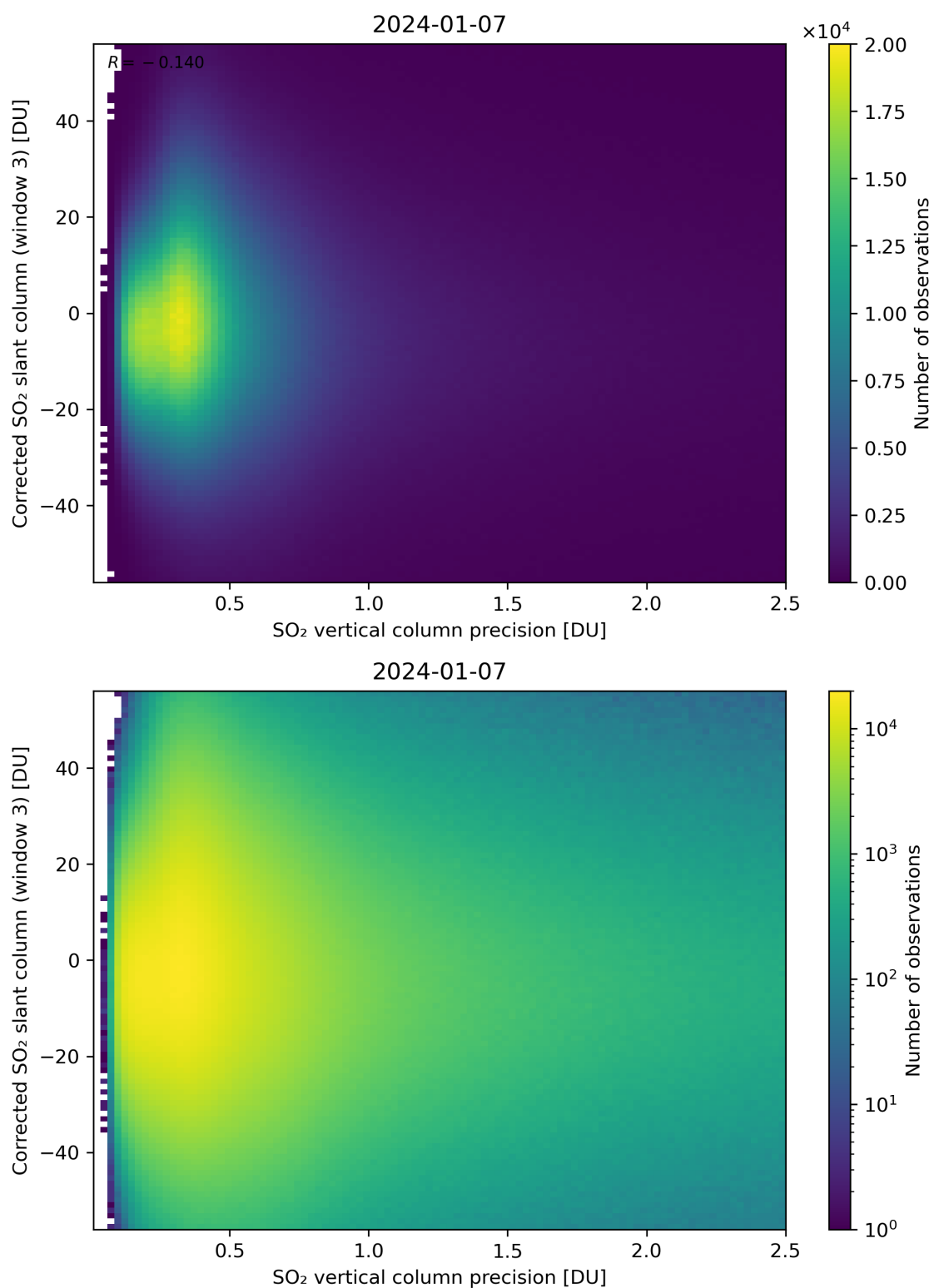
Figure 288: Scatter density plot of “SO 2 vertical column precision” against “Corrected SO 2 slant column (window 3)” for 2024-01-06 to 2024-01-08.
