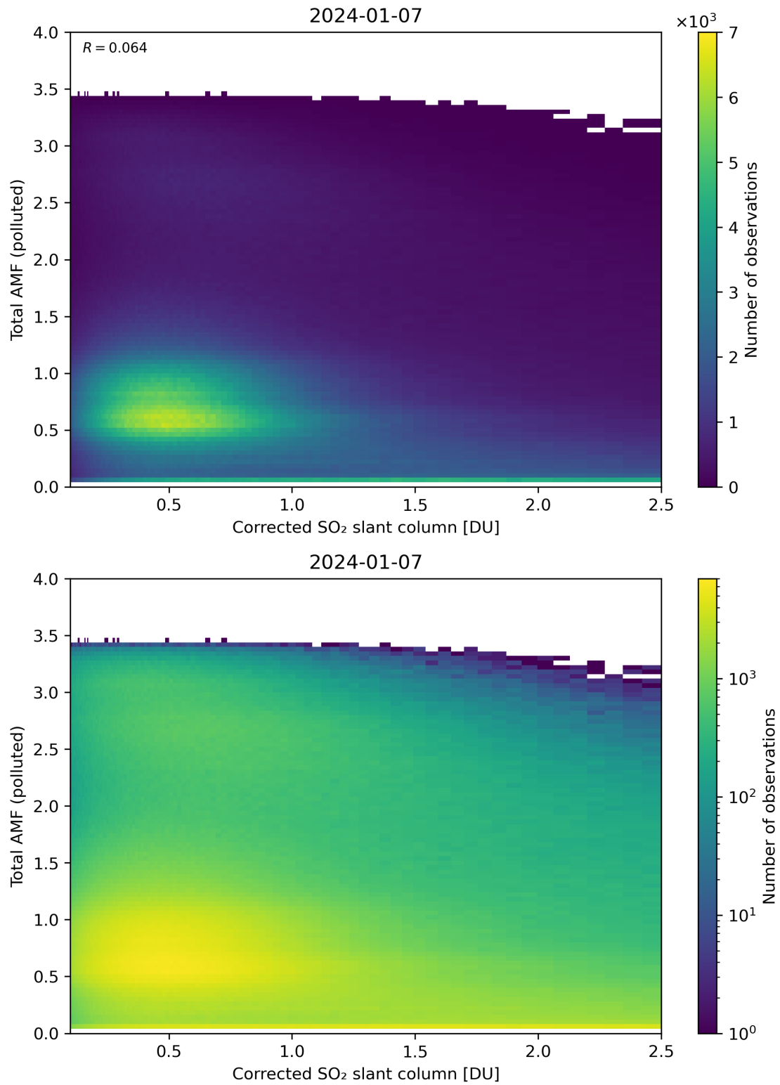
Figure 192: Scatter density plot of “Corrected SO 2 slant column” against “Total AMF (polluted)” for 2024-01-06 to 2024-01-08.
