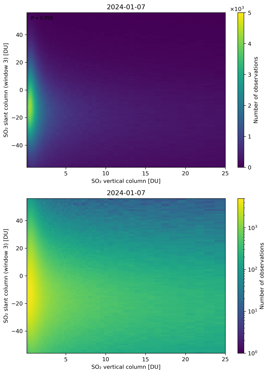
Figure 303: Scatter density plot of “SO 2 vertical column” against “SO 2 slant column (window 3)” for 2024-01-06 to 2024-01-08.
