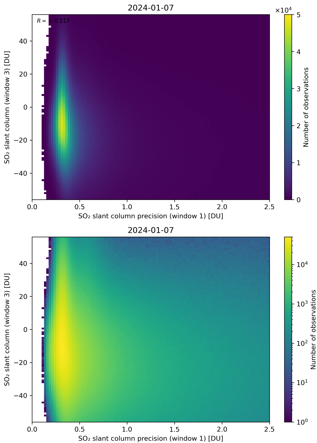
Figure 228: Scatter density plot of “SO 2 slant column precision (window 1)” against “SO 2 slant column (window 3)” for 2024-01-06 to 2024-01-08.
