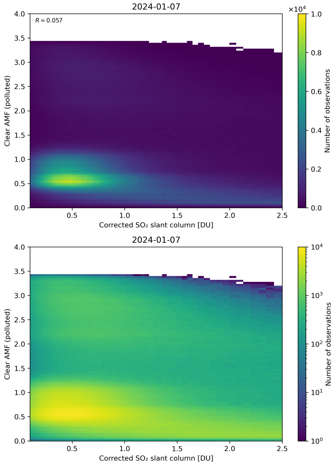
Figure 184: Scatter density plot of “Corrected SO 2 slant column” against “Clear AMF (polluted)” for 2024-01-06 to 2024-01-08.
