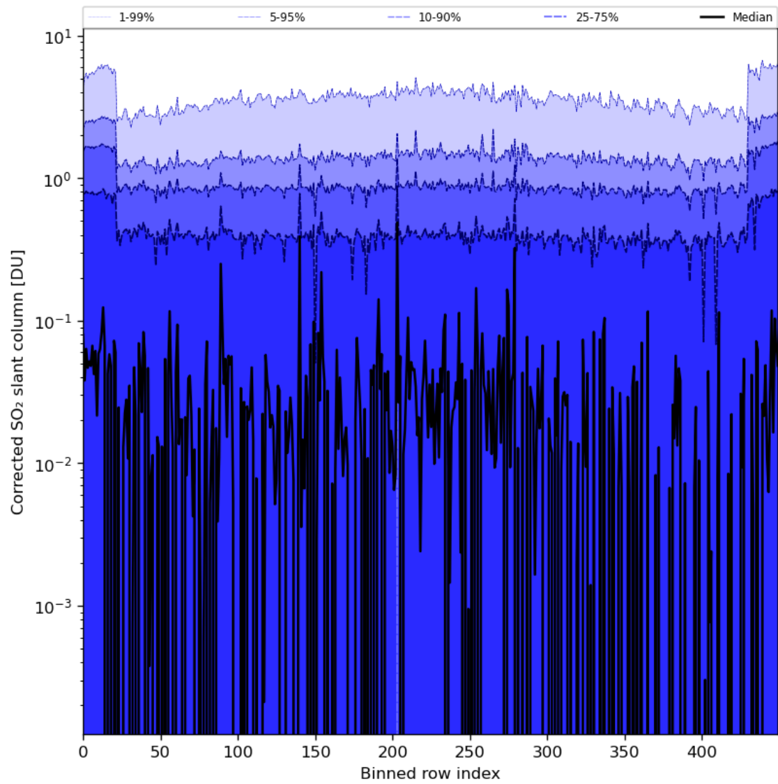
Figure 78: Along track statistics of “Corrected SO 2 slant column” for 2024-01-06 to 2024-01-08
