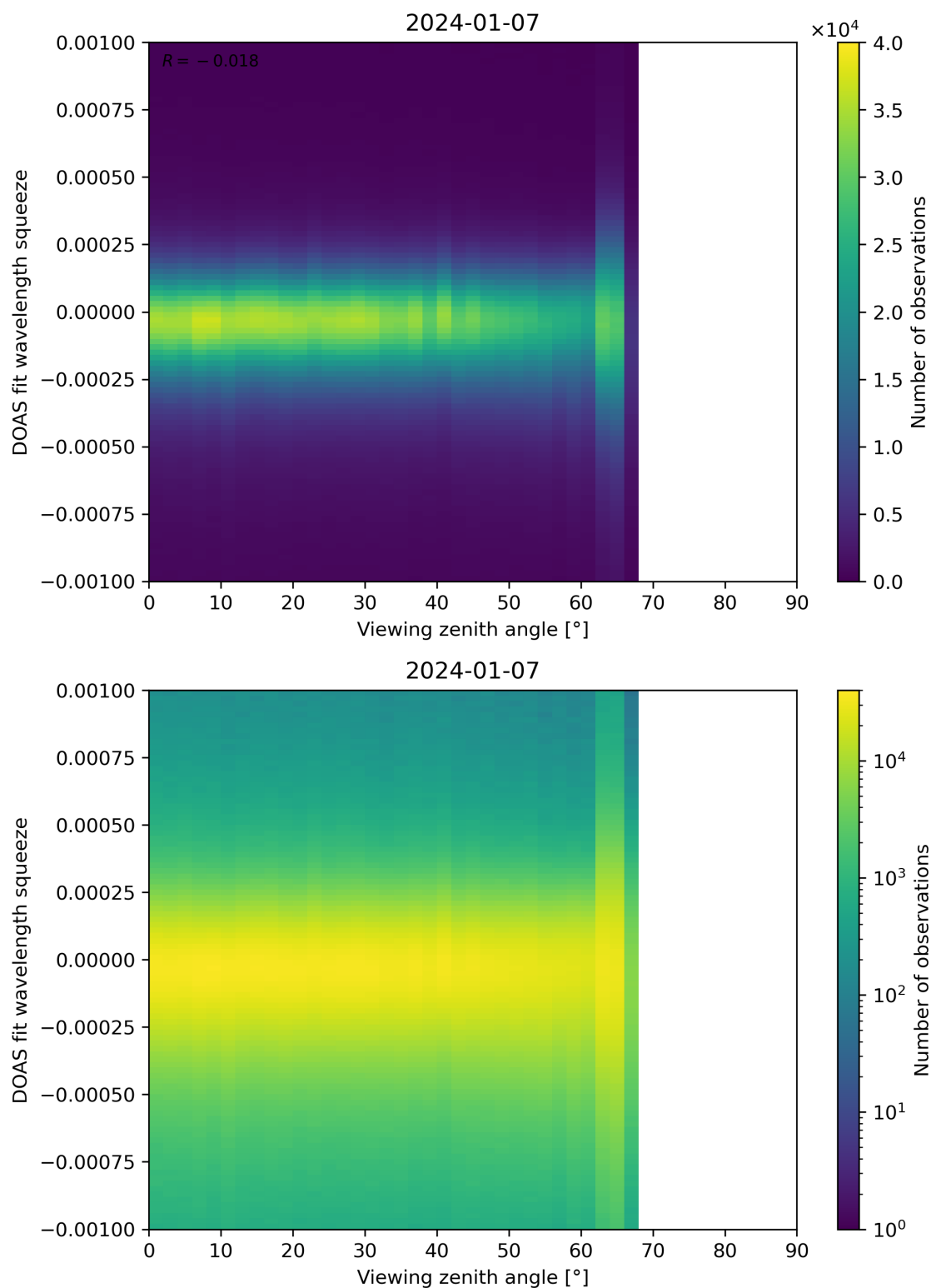
Figure 312: Scatter density plot of “Viewing zenith angle” against “DOAS fit wavelength squeeze” for 2024-01-06 to 2024-01-08.
