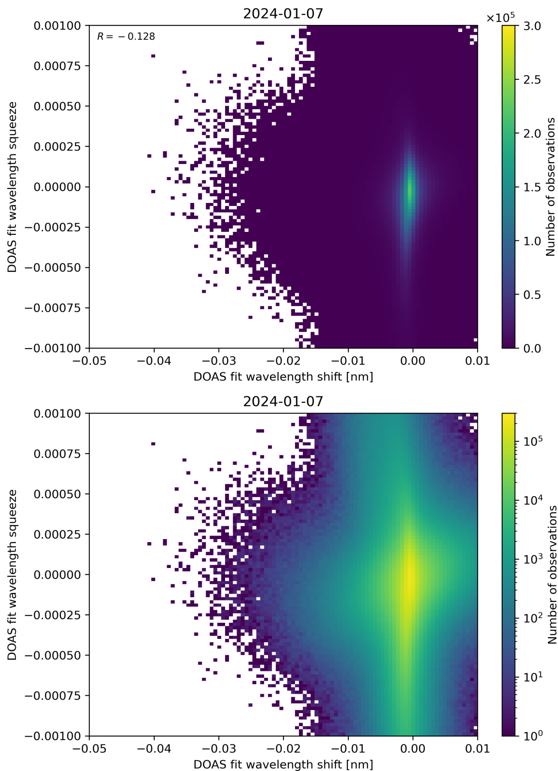
Figure 127: Scatter density plot of “DOAS fit wavelength shift” against “DOAS fit wavelength squeeze” for 2024-01-06 to 2024-01-08.
