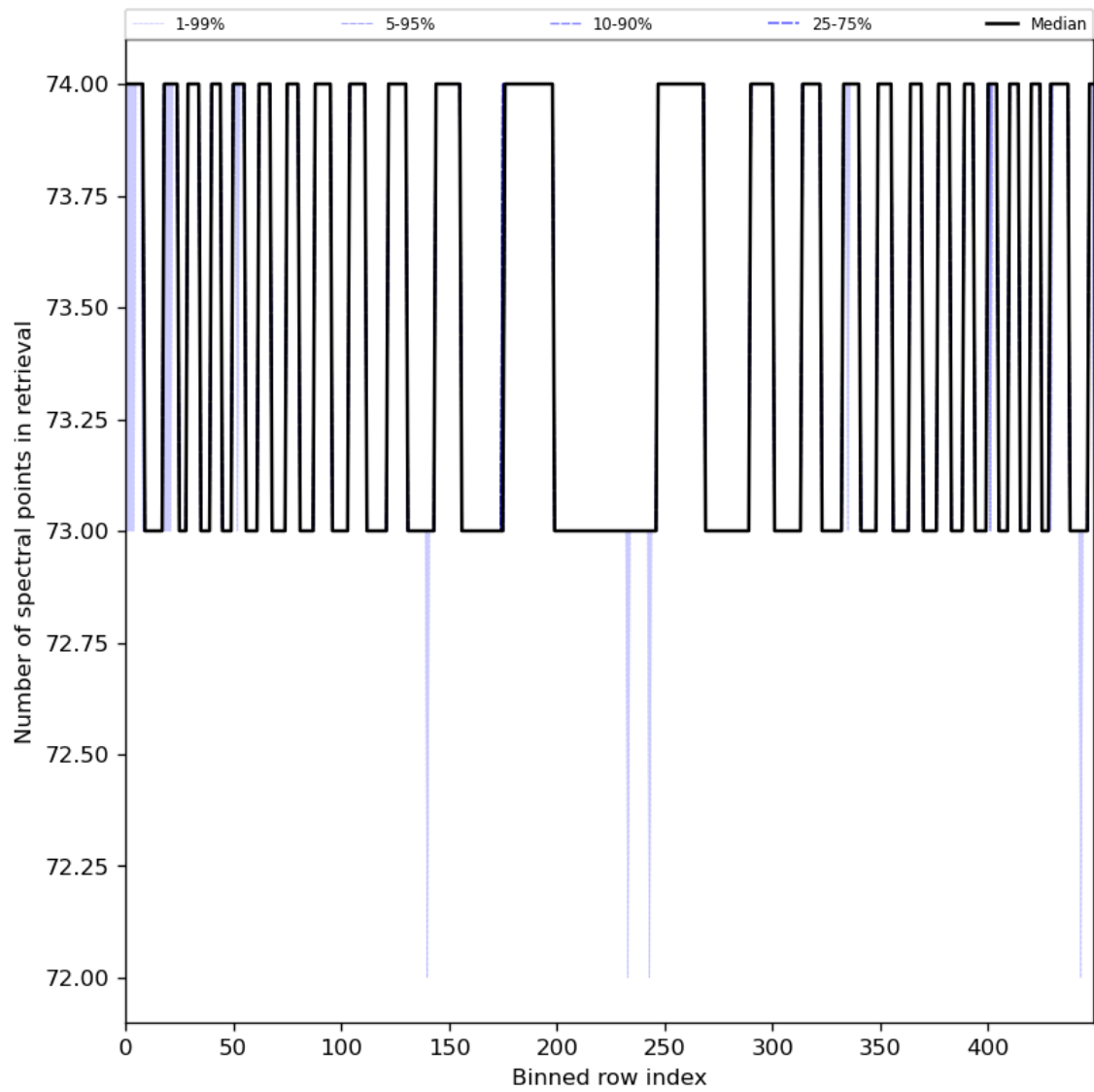
Figure 97: Along track statistics of “Number of spectral points in retrieval” for 2024-01-06 to 2024-01-08
