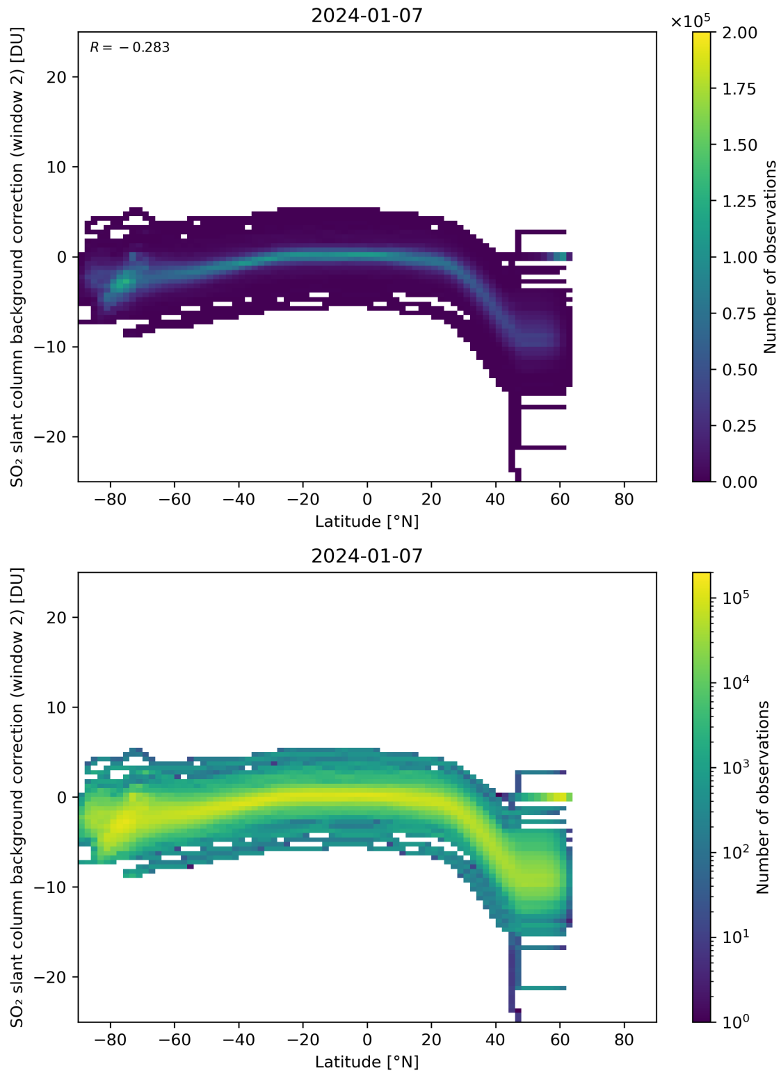
Figure 140: Scatter density plot of “Latitude” against “SO 2 slant column background correction (window 2)” for 2024-01-06 to 2024-01-08.
