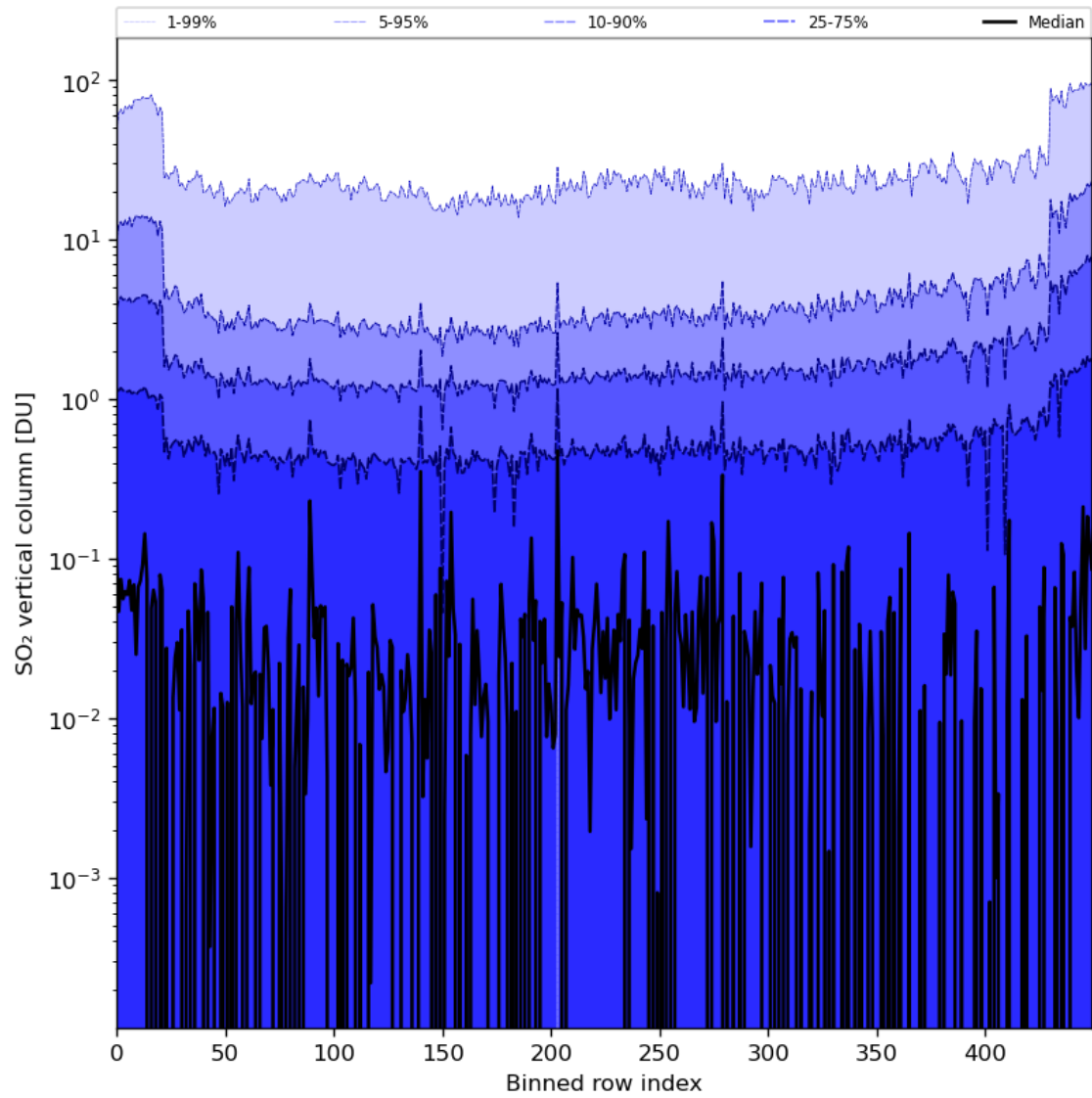
Figure 76: Along track statistics of “SO 2 vertical column” for 2024-01-06 to 2024-01-08
