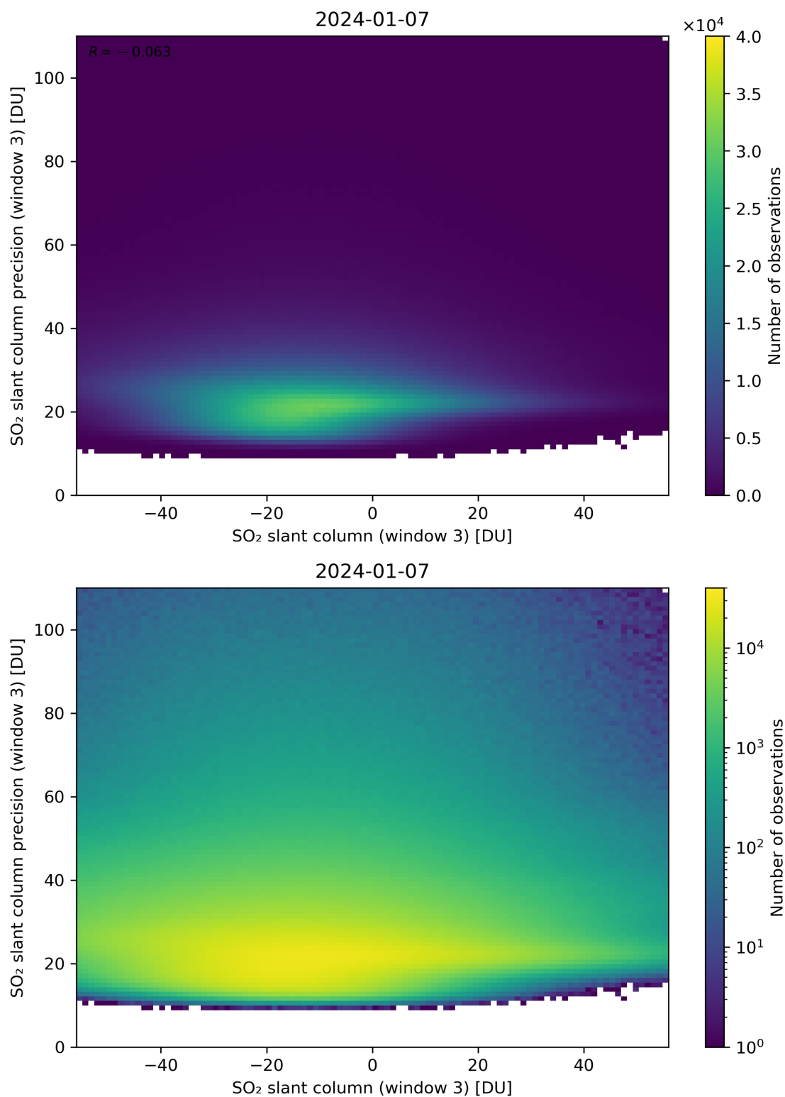
Figure 267: Scatter density plot of “SO 2 slant column (window 3)” against “SO 2 slant column precision (window 3)” for 2024-01-06 to 2024-01-08.
