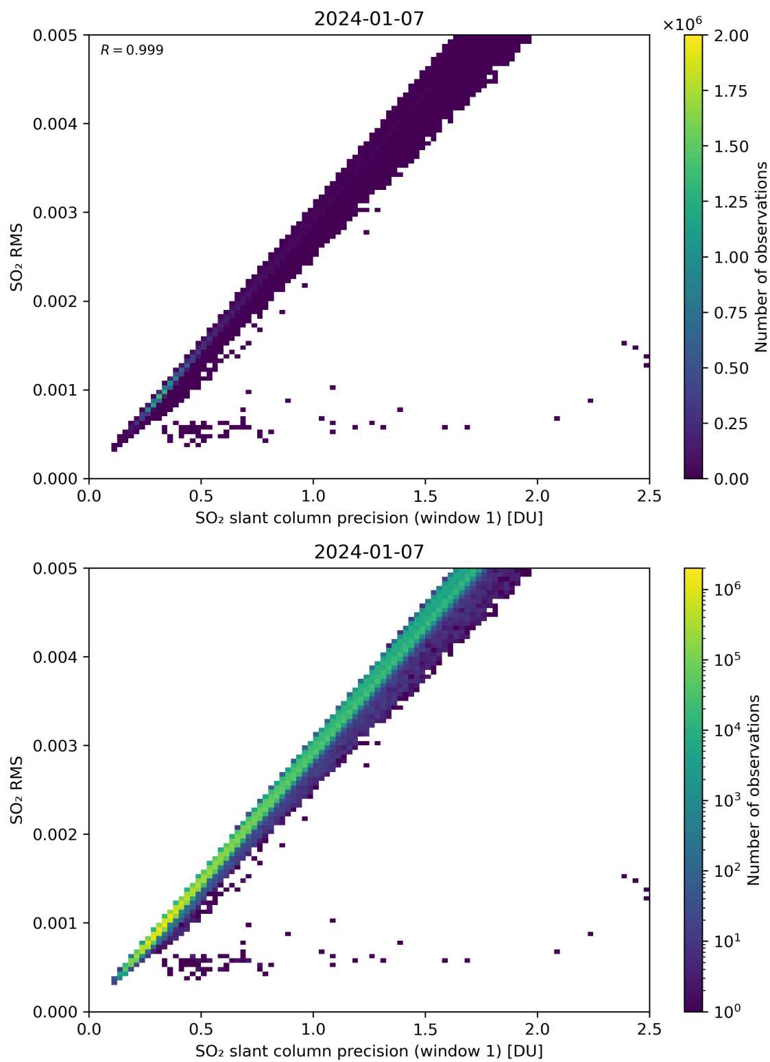
Figure 223: Scatter density plot of “SO 2 slant column precision (window 1)” against “SO 2 RMS” for 2024-01-06 to 2024-01-08.
