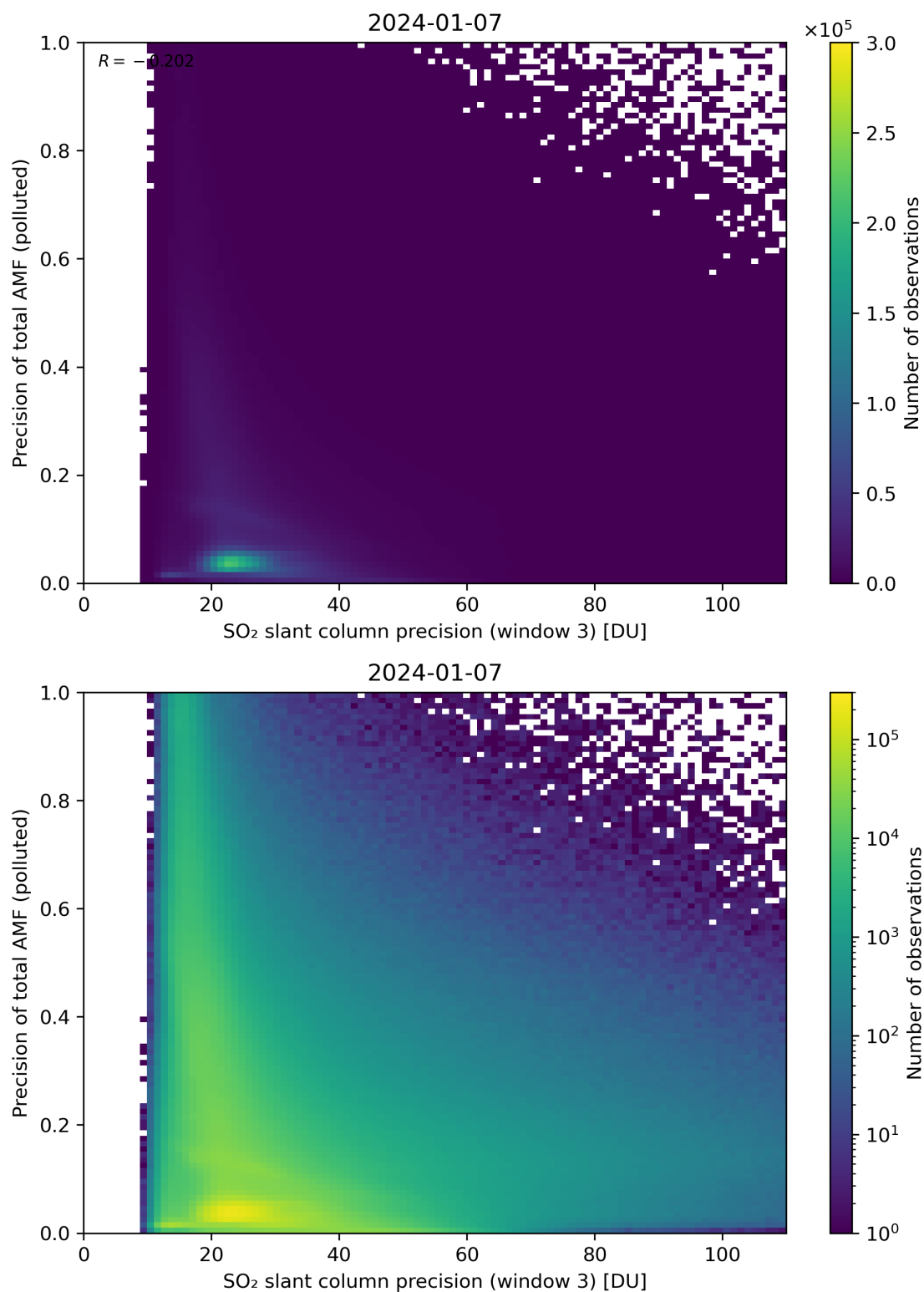
Figure 264: Scatter density plot of “SO 2 slant column precision (window 3)” against “Precision of total AMF (polluted)” for 2024-01-06 to 2024-01-08.
