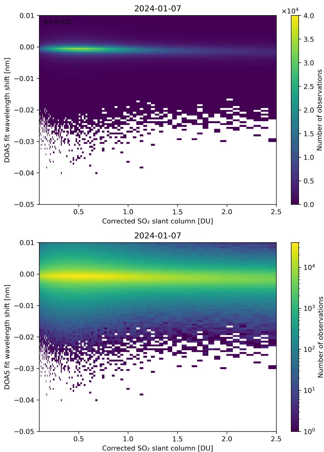
Figure 181: Scatter density plot of “Corrected SO 2 slant column” against “DOAS fit wavelength shift” for 2024-01-06 to 2024-01-08.
