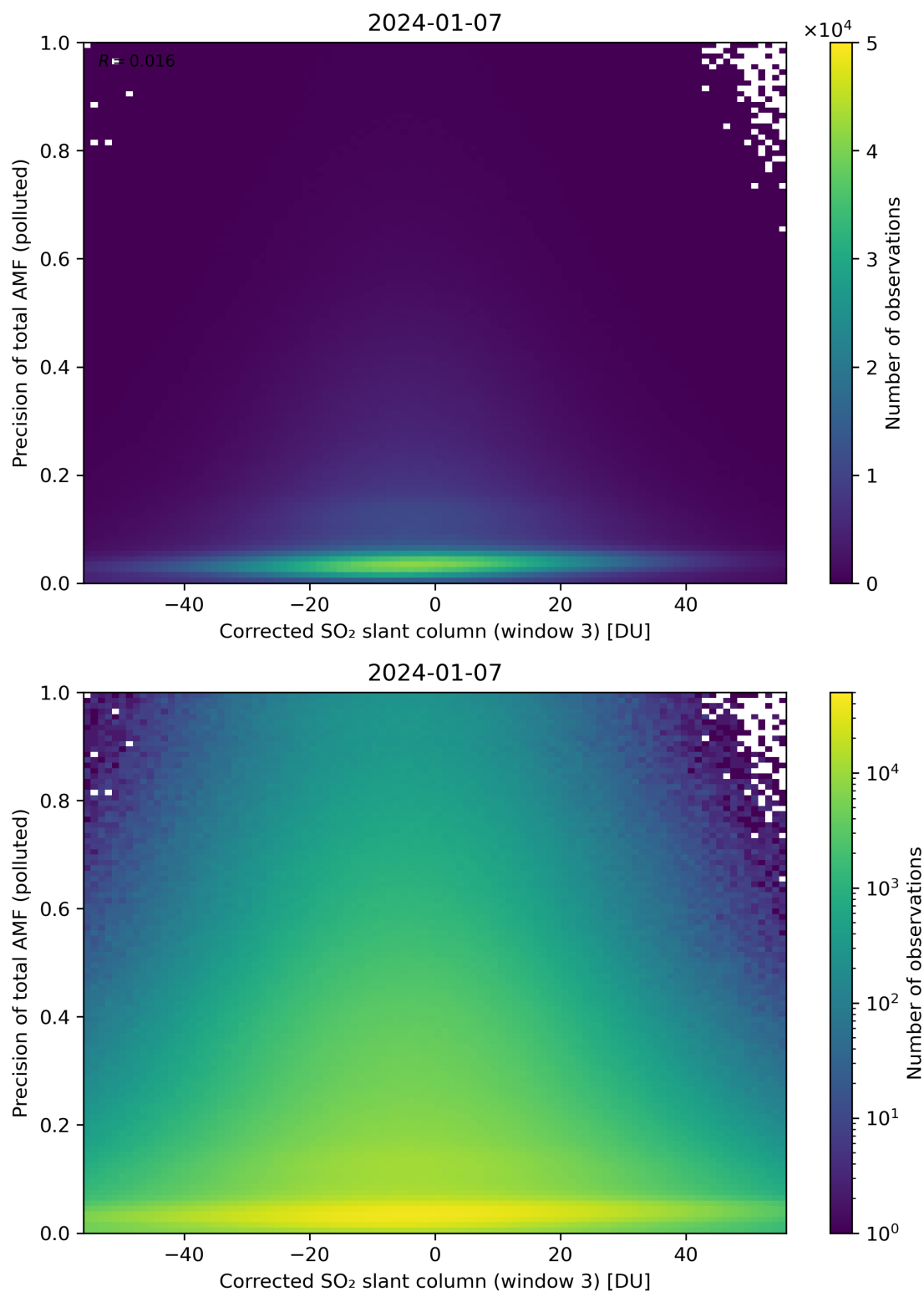
Figure 211: Scatter density plot of “Corrected SO 2 slant column (window 3)” against “Precision of total AMF (polluted)” for 2024-01-06 to 2024-01-08.
