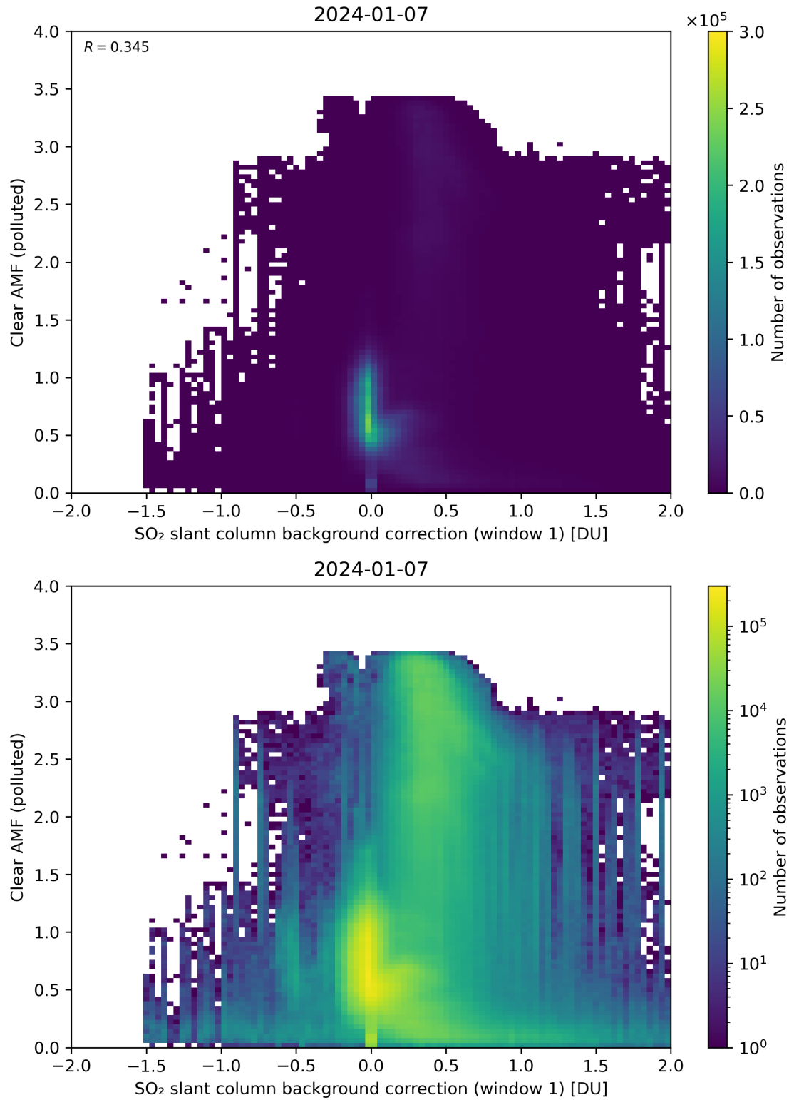
Figure 103: Scatter density plot of “SO 2 slant column background correction (window 1)” against “Clear AMF (polluted)” for 2024-01-06 to 2024-01-08.
