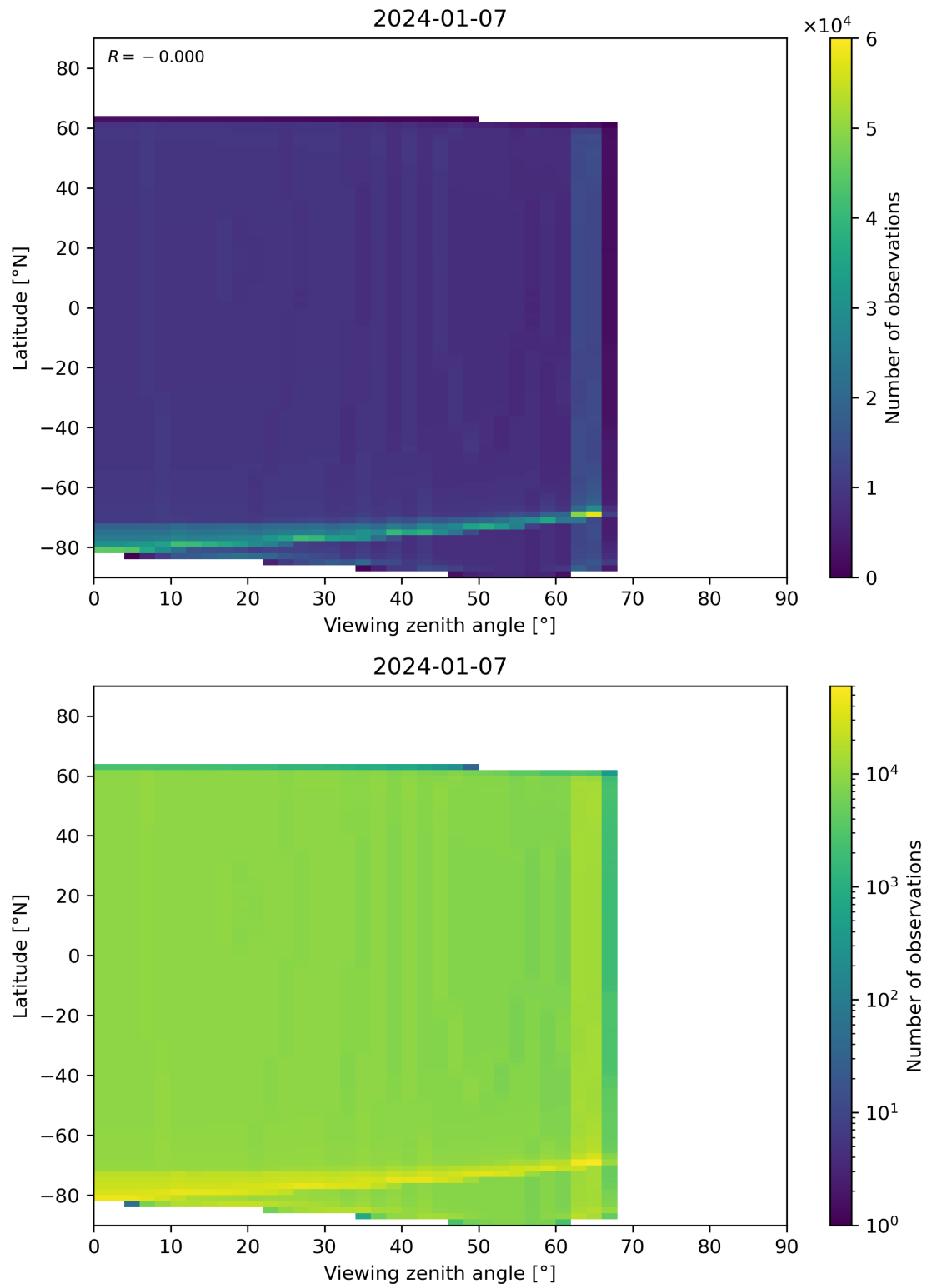
Figure 314: Scatter density plot of “Viewing zenith angle” against “Latitude” for 2024-01-06 to 2024-01-08.
