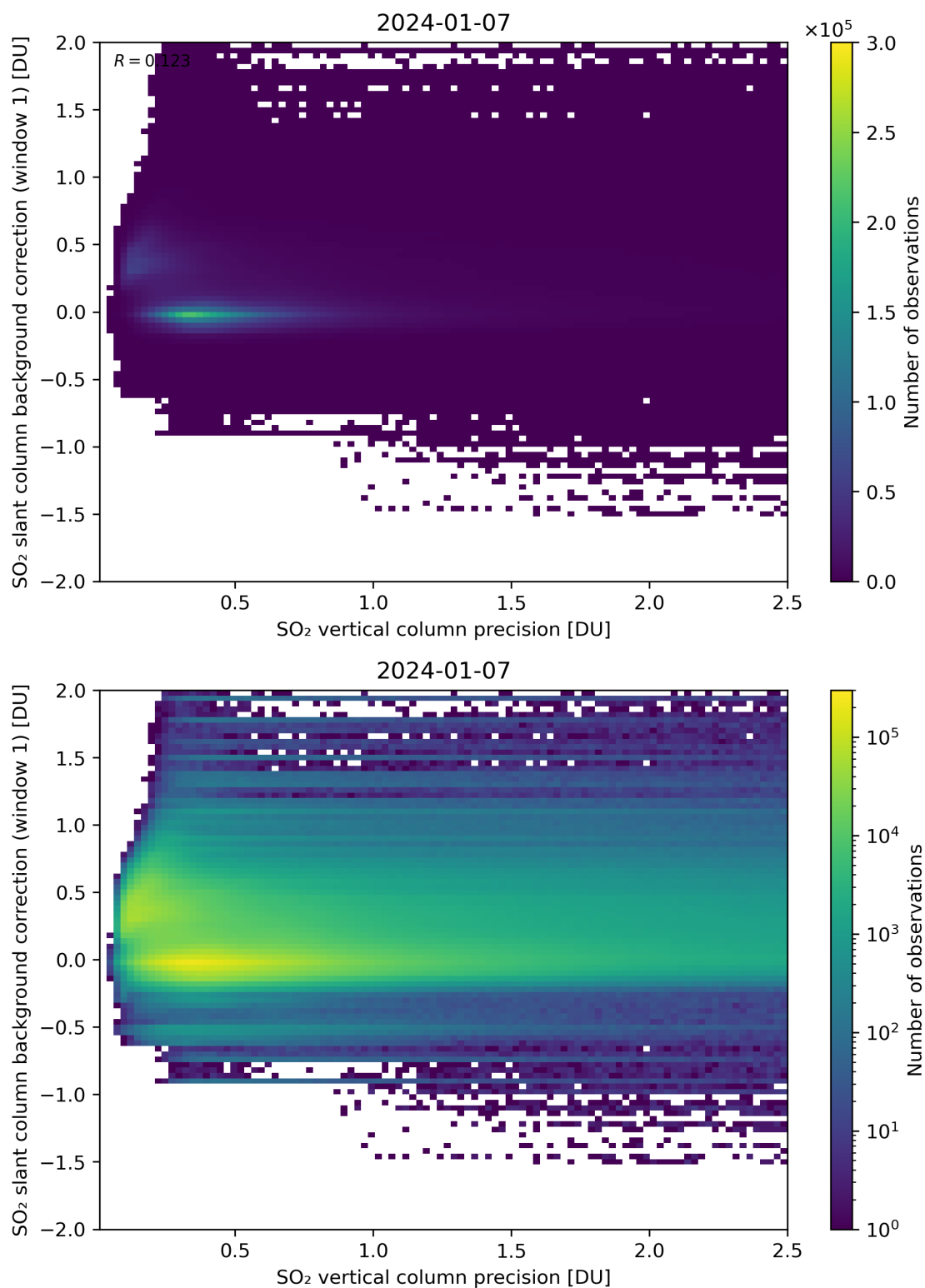
Figure 279: Scatter density plot of “SO 2 vertical column precision” against “SO 2 slant column background correction (window 1)” for 2024-01-06 to 2024-01-08.
