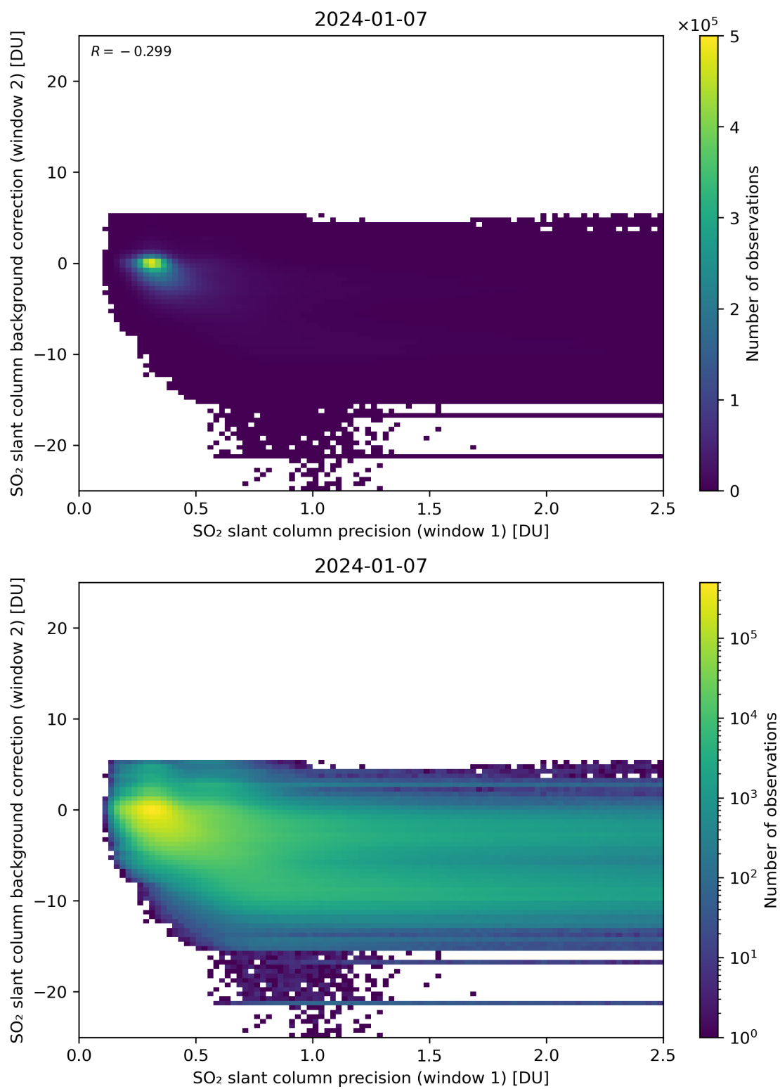
Figure 219: Scatter density plot of “SO 2 slant column precision (window 1)” against “SO 2 slant column background correction (window 2)” for 2024-01-06 to 2024-01-08.
