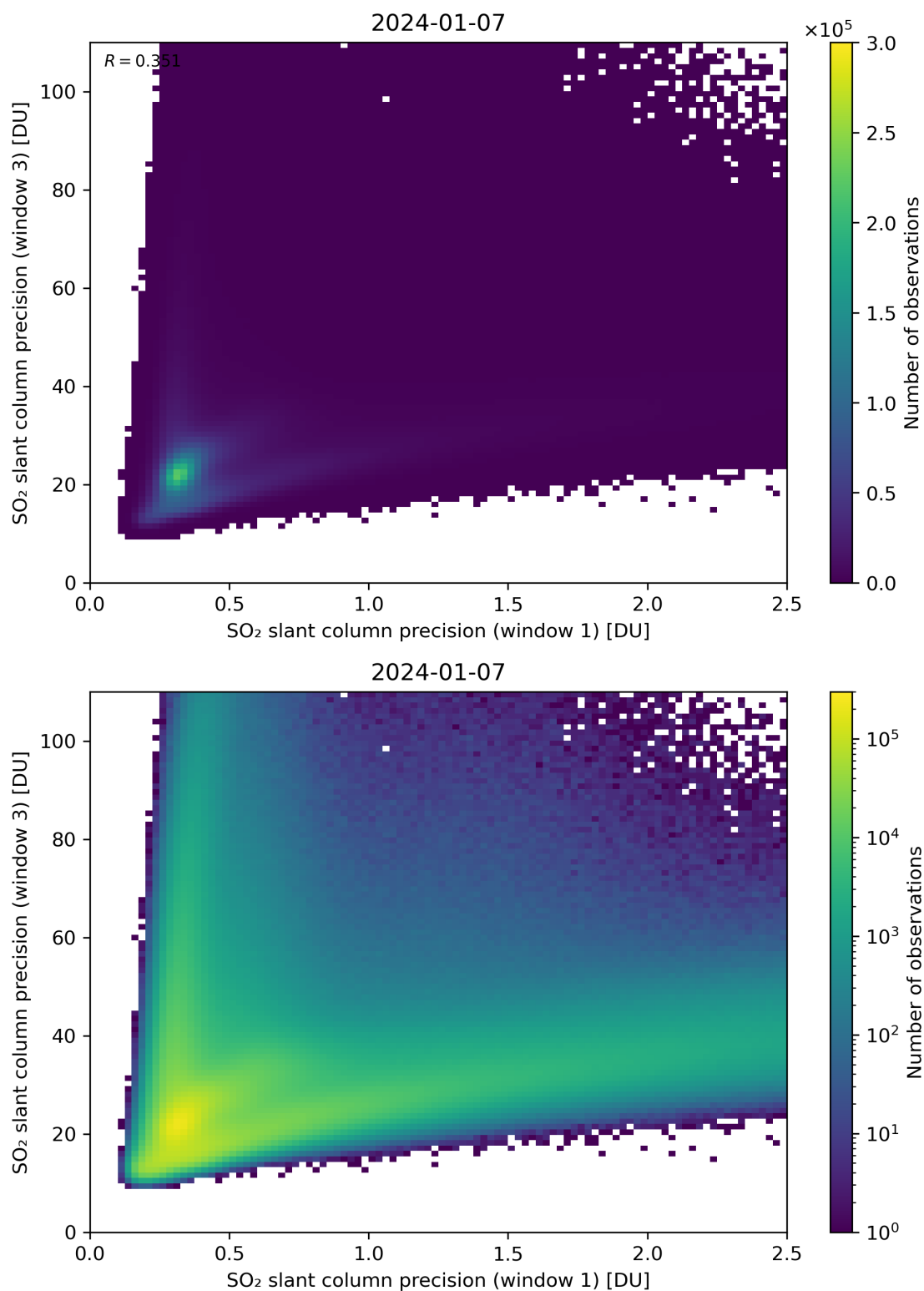
Figure 229: Scatter density plot of “SO 2 slant column precision (window 1)” against “SO 2 slant column precision (window 3)” for 2024-01-06 to 2024-01-08.
