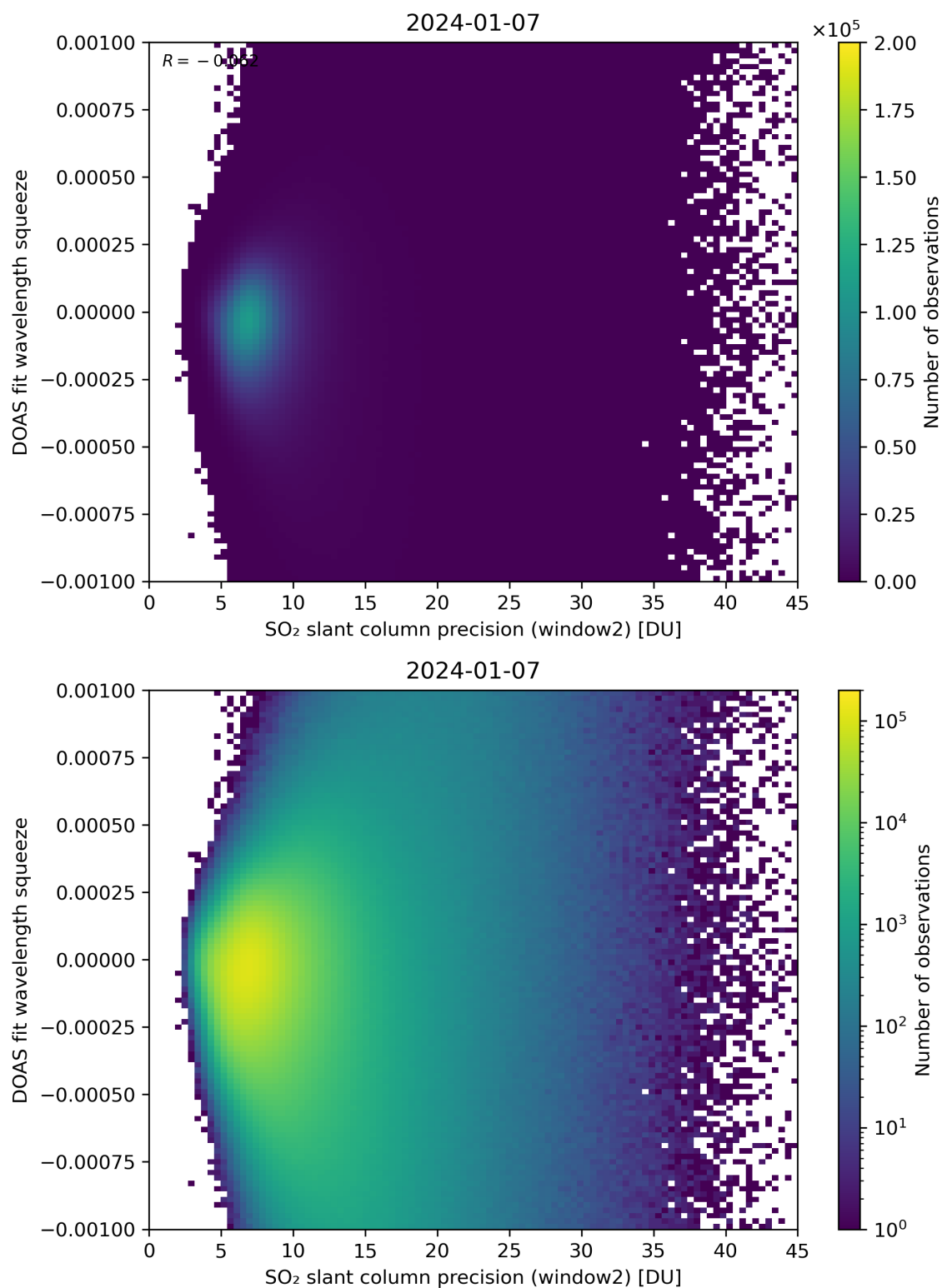
Figure 244: Scatter density plot of “SO 2 slant column precision (window2)” against “DOAS fit wavelength squeeze” for 2024-01-06 to 2024-01-08.
