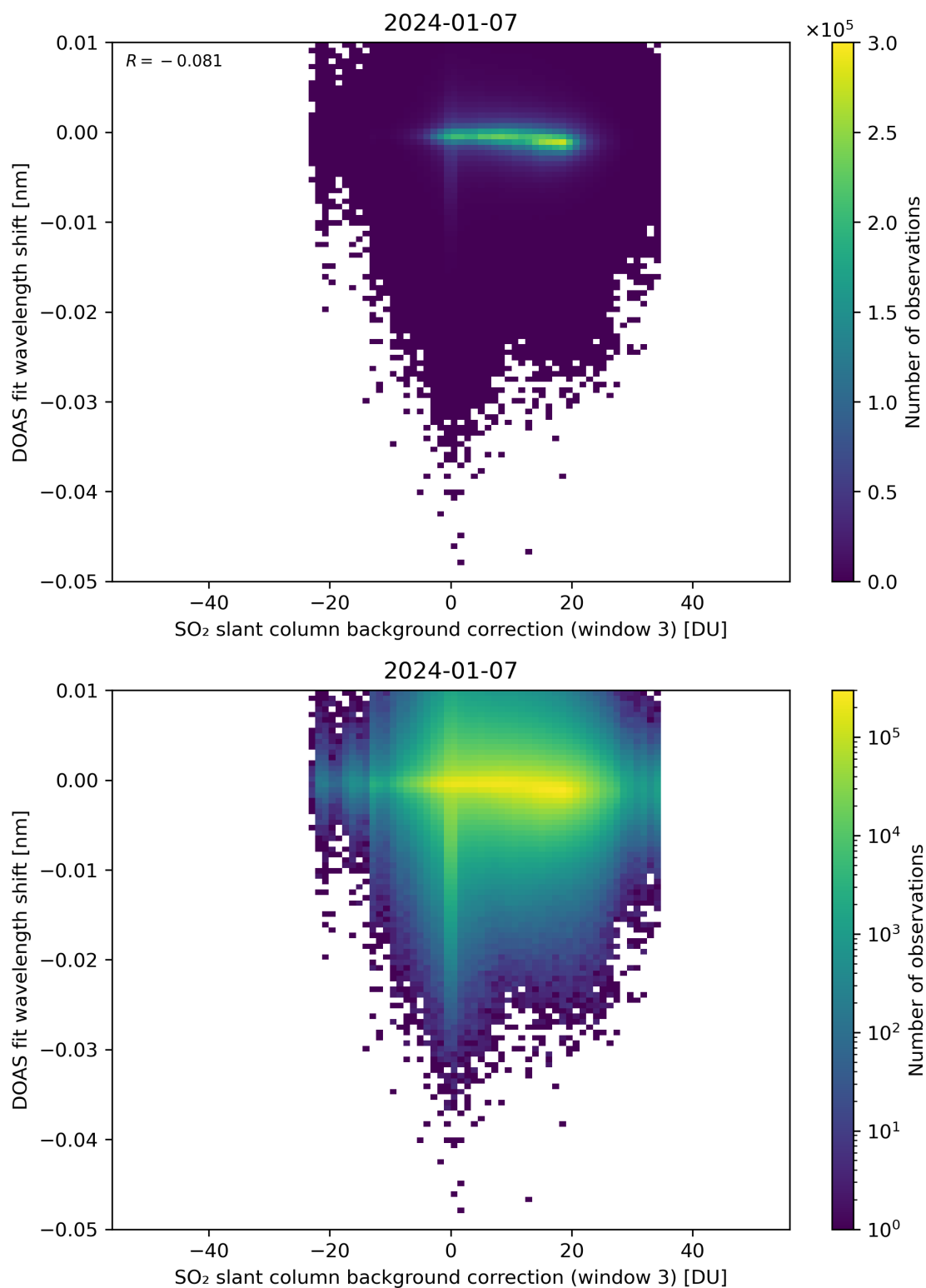
Figure 121: Scatter density plot of “SO 2 slant column background correction (window 3)” against “DOAS fit wavelength shift” for 2024-01-06 to 2024-01-08.
