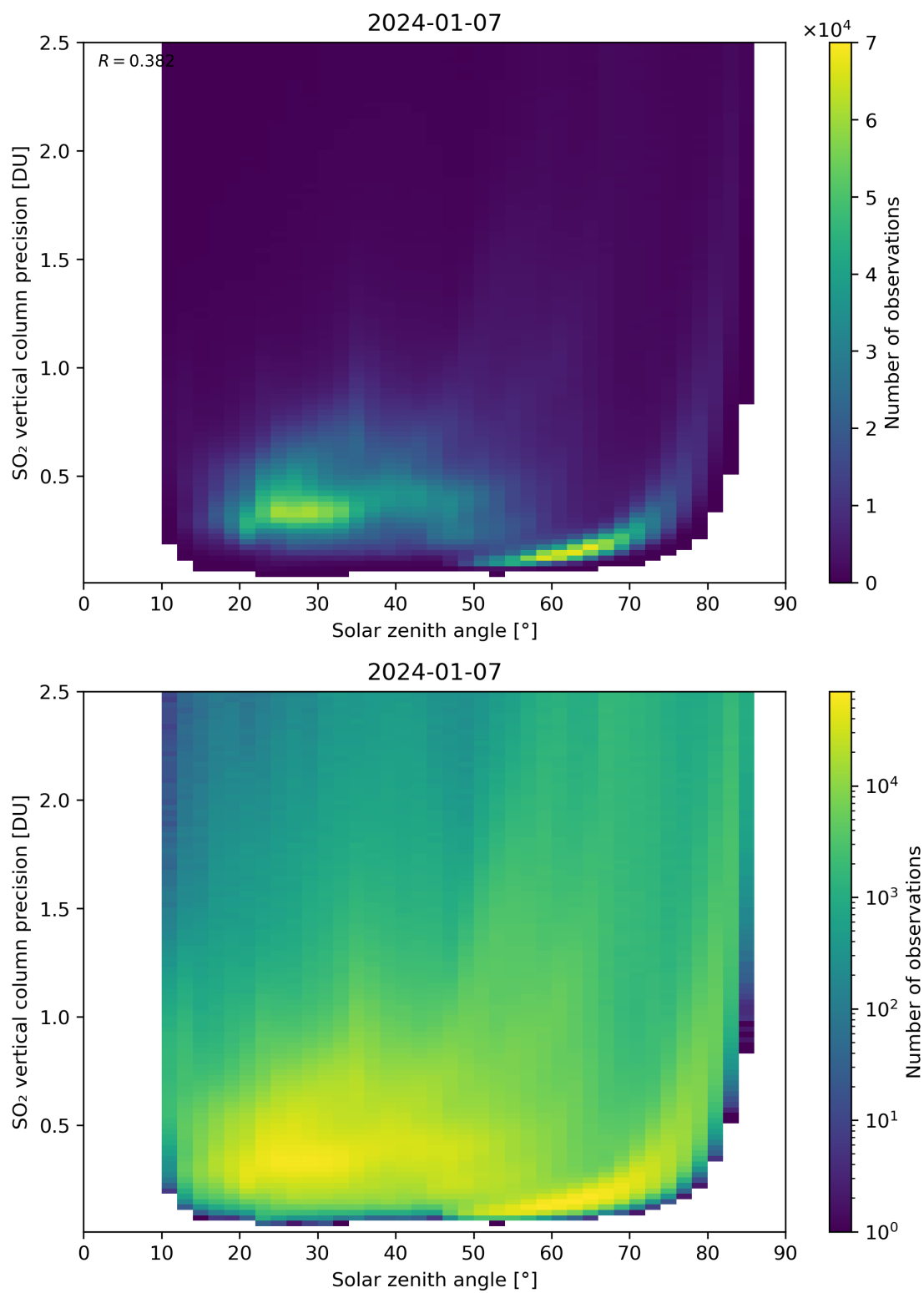
Figure 177: Scatter density plot of “Solar zenith angle” against “SO 2 vertical column precision” for 2024-01-06 to 2024-01-08.
