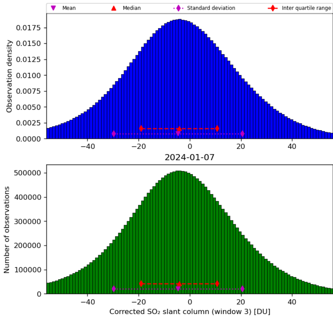
Figure 66: Histogram of “Corrected SO 2 slant column (window 3)” for 2024-01-06 to 2024-01-08
