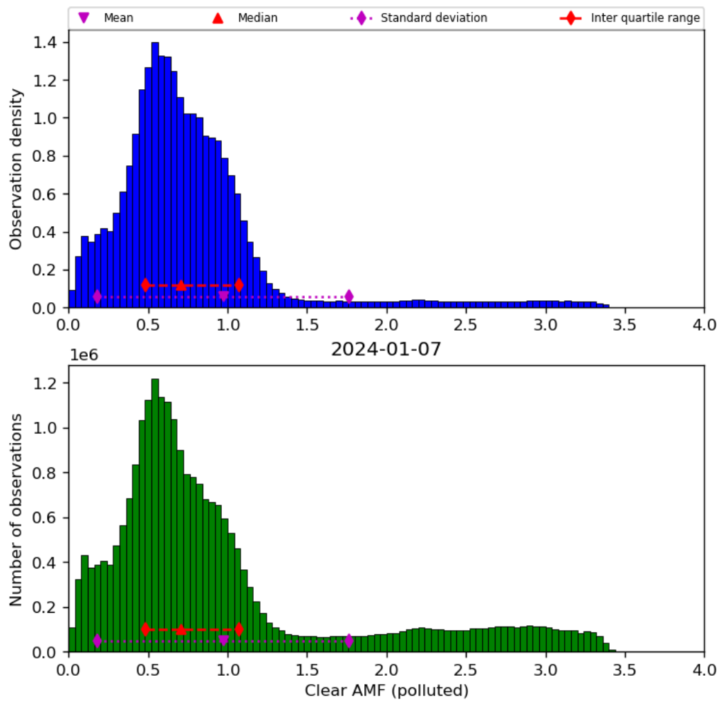
Figure 73: Histogram of “Clear AMF (polluted)” for 2024-01-06 to 2024-01-08
