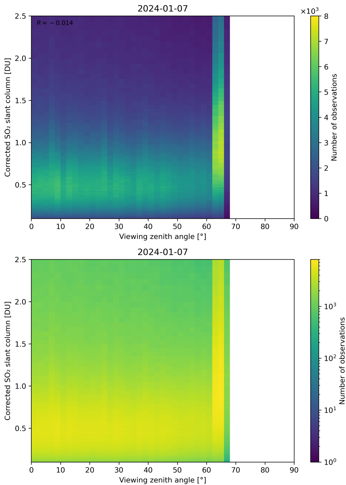
Figure 317: Scatter density plot of “Viewing zenith angle” against “Corrected SO 2 slant column” for 2024-01-06 to 2024-01-08.
