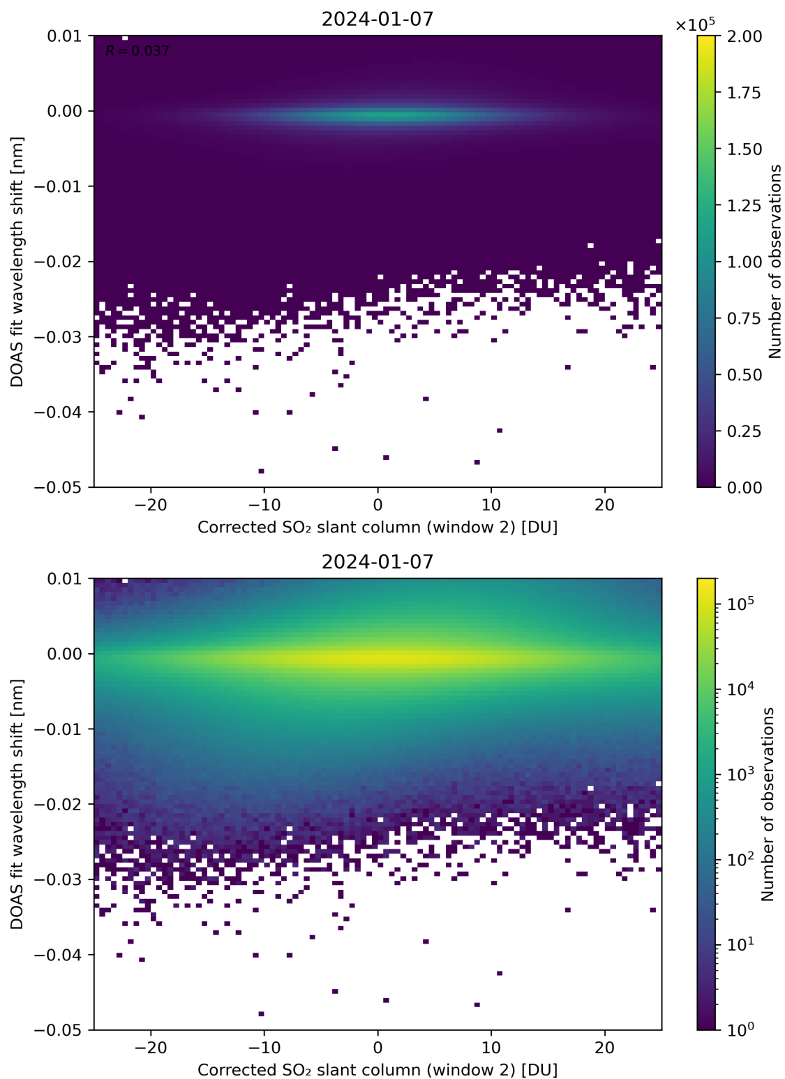
Figure 196: Scatter density plot of “Corrected SO 2 slant column (window 2)” against “DOAS fit wavelength shift” for 2024-01-06 to 2024-01-08.
