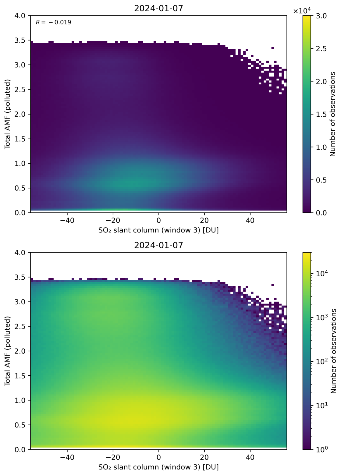
Figure 268: Scatter density plot of “SO 2 slant column (window 3)” against “Total AMF (polluted)” for 2024-01-06 to 2024-01-08.
