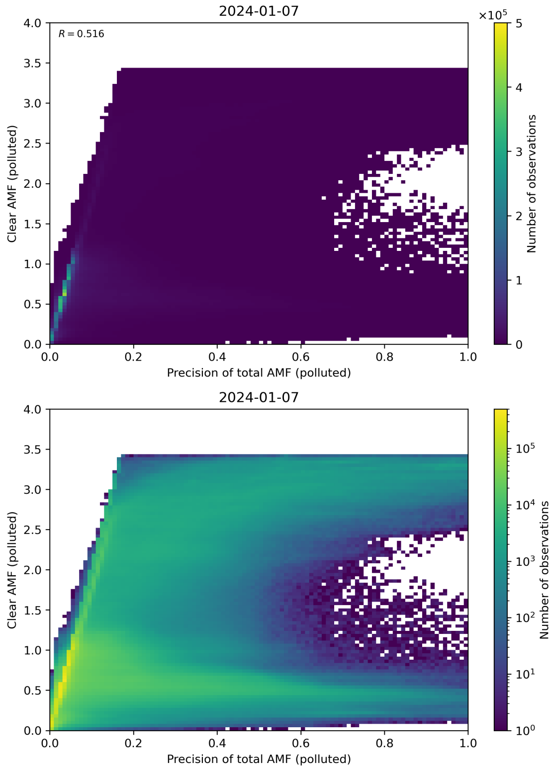
Figure 270: Scatter density plot of “Precision of total AMF (polluted)” against “Clear AMF (polluted)” for 2024-01-06 to 2024-01-08.
