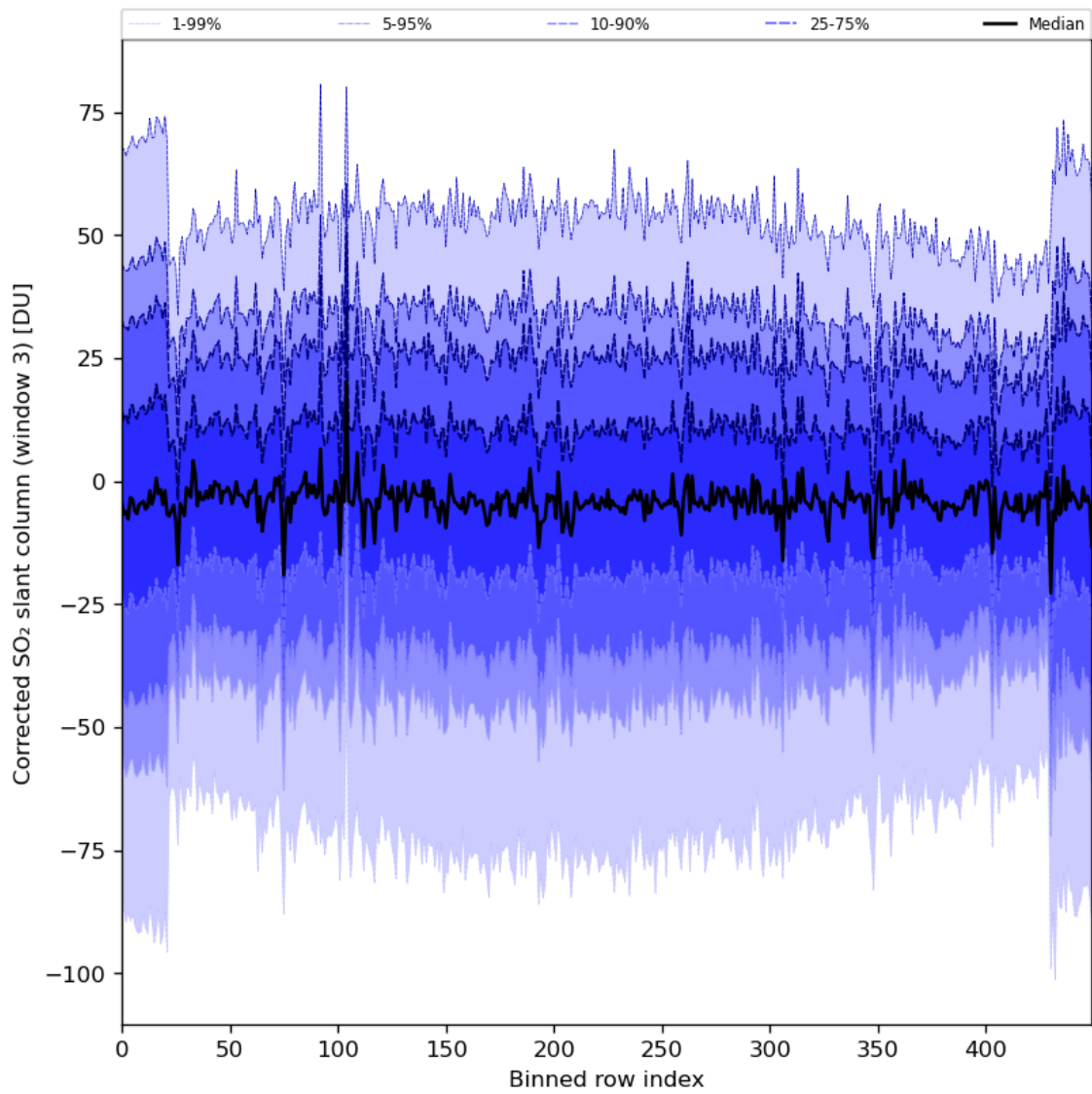
Figure 89: Along track statistics of “Corrected SO 2 slant column (window 3)” for 2024-01-06 to 2024-01-08
