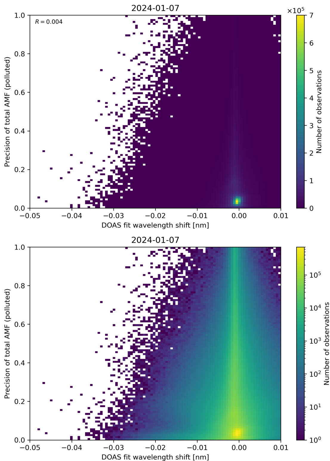
Figure 131: Scatter density plot of “DOAS fit wavelength shift” against “Precision of total AMF (polluted)” for 2024-01-06 to 2024-01-08.
