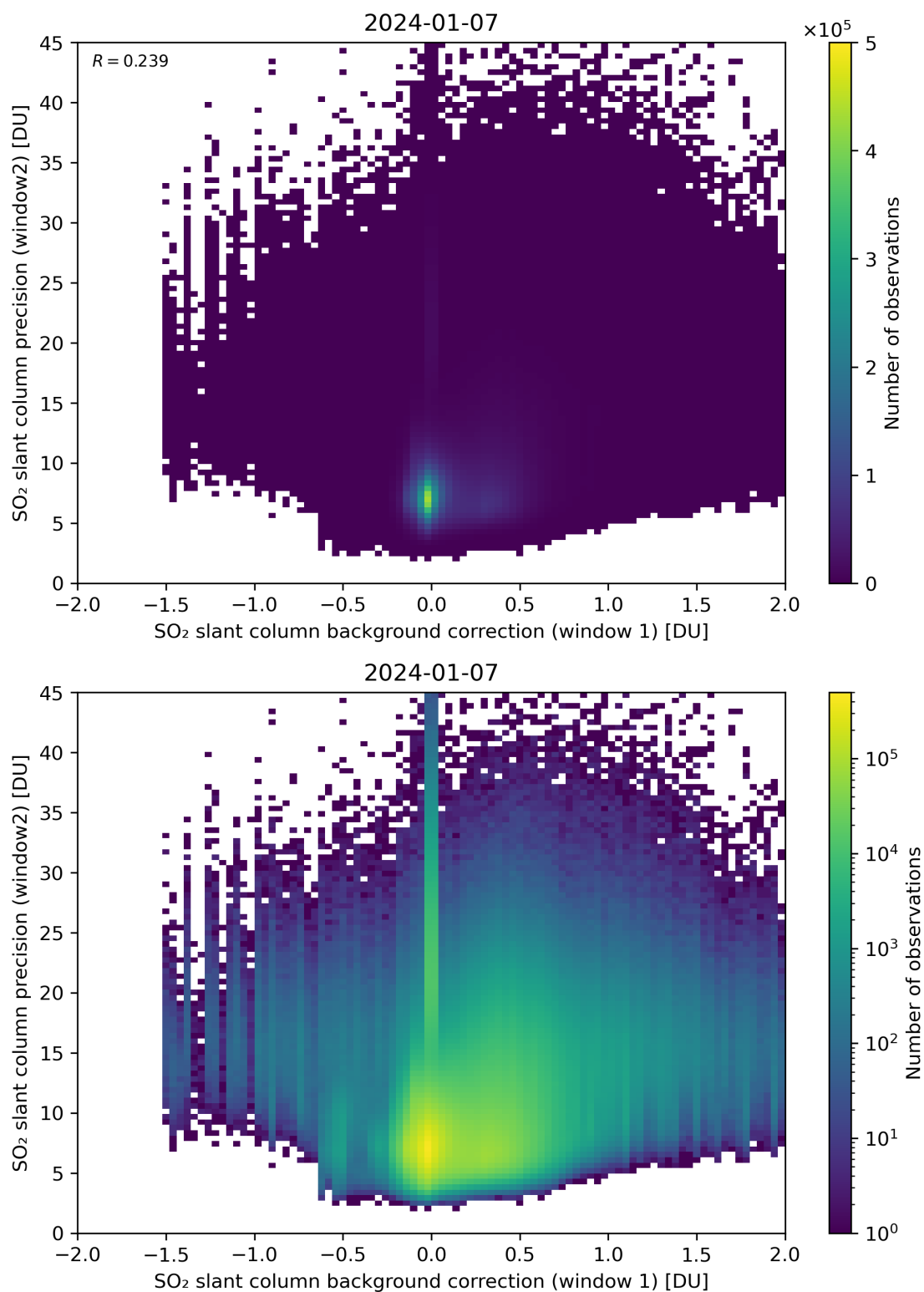
Figure 106: Scatter density plot of “SO 2 slant column background correction (window 1)” against “SO 2 slant column precision (window2)” for 2024-01-06 to 2024-01-08.
