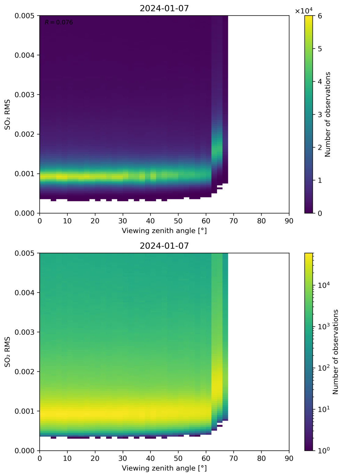
Figure 313: Scatter density plot of “Viewing zenith angle” against “SO 2 RMS” for 2024-01-06 to 2024-01-08.
