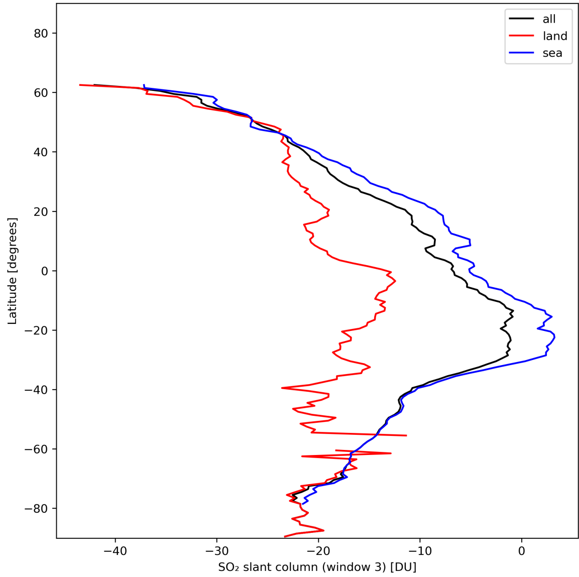
Figure 41: Zonal average of “SO 2 slant column (window 3)” for 2024-01-06 to 2024-01-08.
