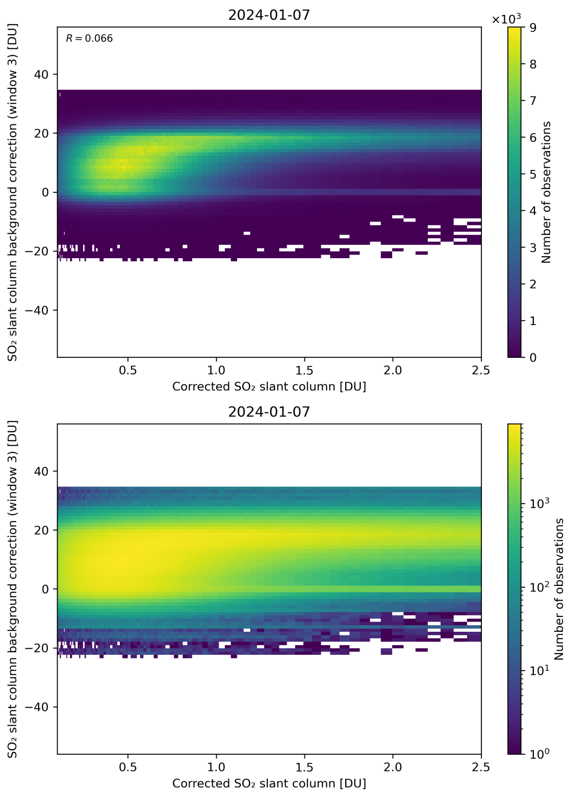
Figure 180: Scatter density plot of “Corrected SO 2 slant column” against “SO 2 slant column background correction (window 3)” for 2024-01-06 to 2024-01-08.
