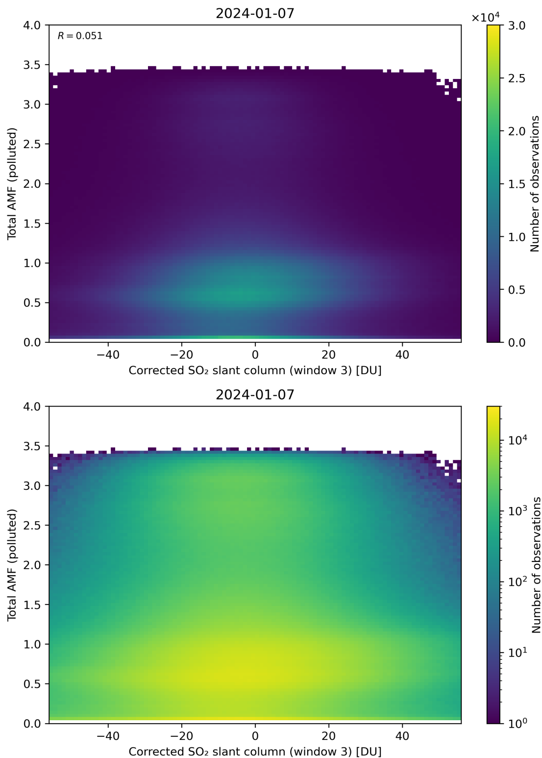
Figure 210: Scatter density plot of “Corrected SO 2 slant column (window 3)” against “Total AMF (polluted)” for 2024-01-06 to 2024-01-08.
