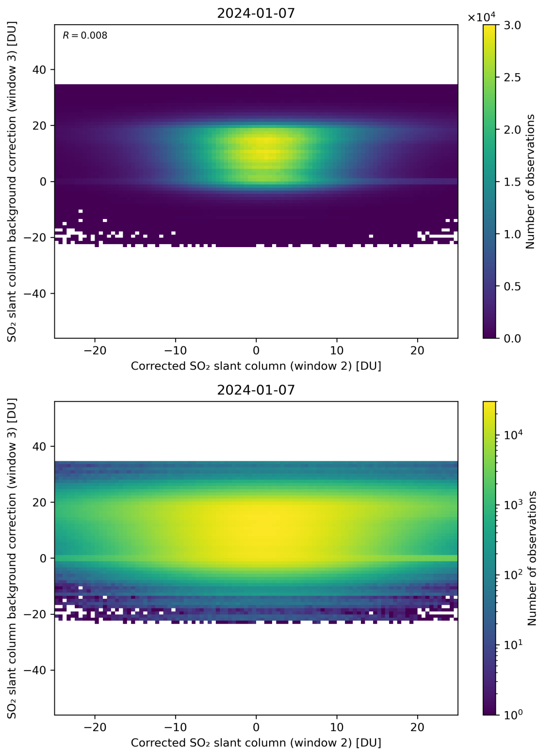
Figure 195: Scatter density plot of “Corrected SO 2 slant column (window 2)” against “SO 2 slant column background correction (window 3)” for 2024-01-06 to 2024-01-08.
