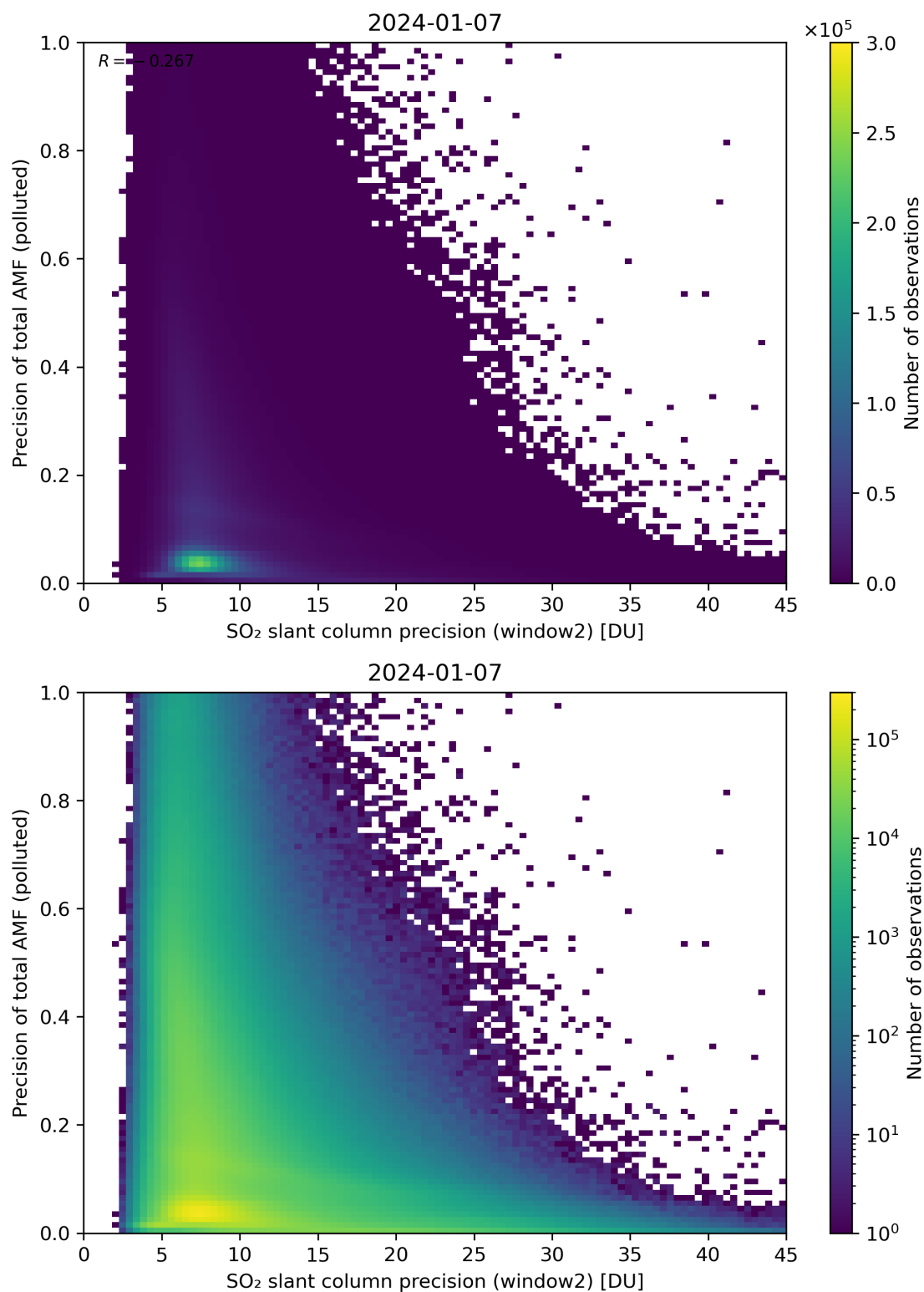
Figure 252: Scatter density plot of “SO 2 slant column precision (window2)” against “Precision of total AMF (polluted)” for 2024-01-06 to 2024-01-08.
