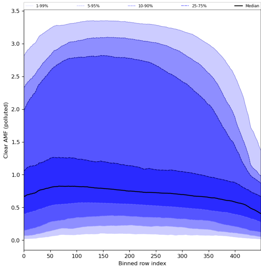
Figure 96: Along track statistics of “Clear AMF (polluted)” for 2024-01-06 to 2024-01-08
