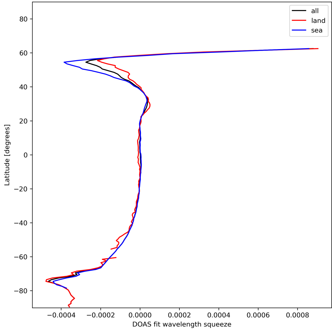
Figure 46: Zonal average of “DOAS fit wavelength squeeze” for 2024-01-06 to 2024-01-08.
