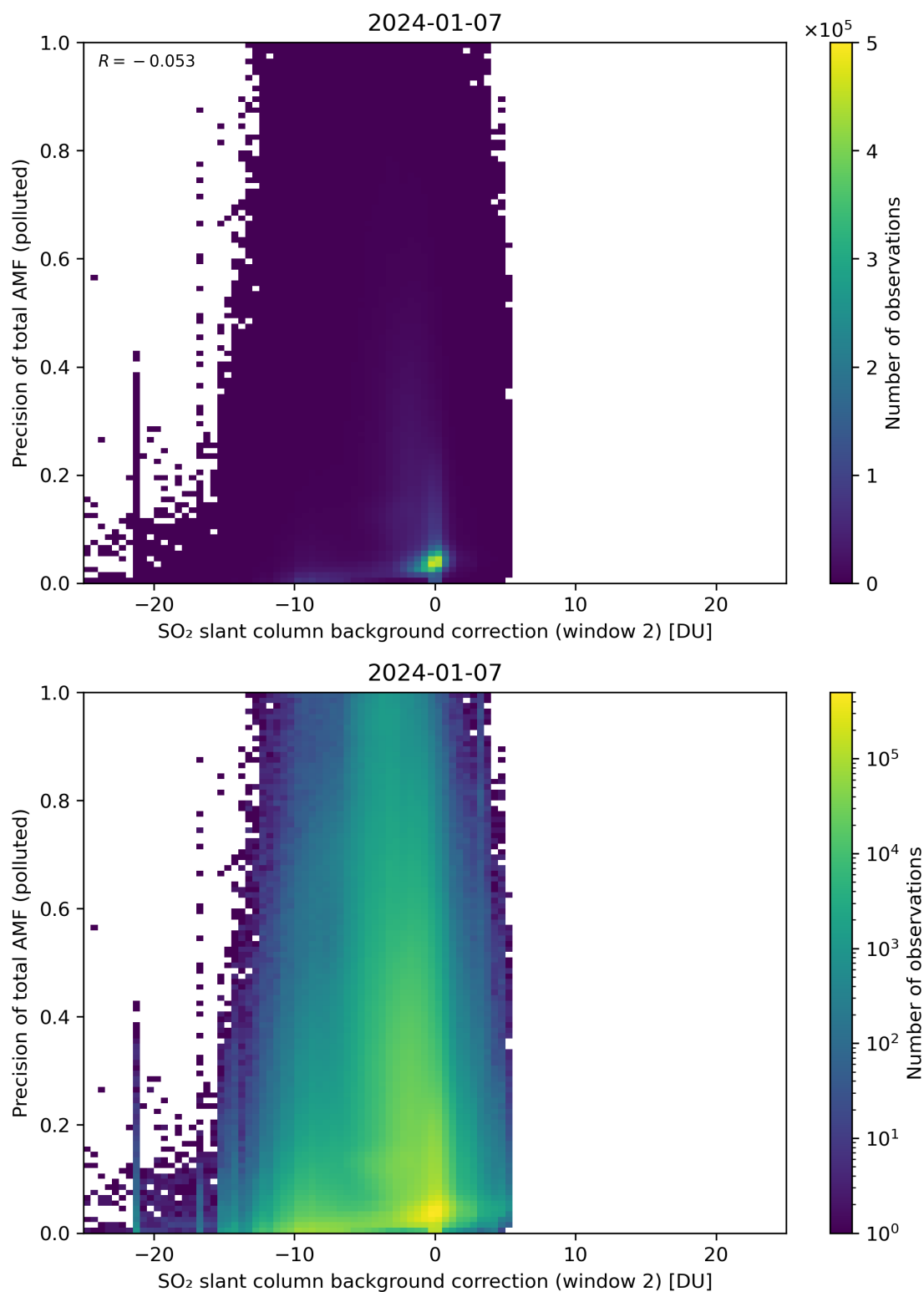
Figure 120: Scatter density plot of “SO 2 slant column background correction (window 2)” against “Precision of total AMF (polluted)” for 2024-01-06 to 2024-01-08.
