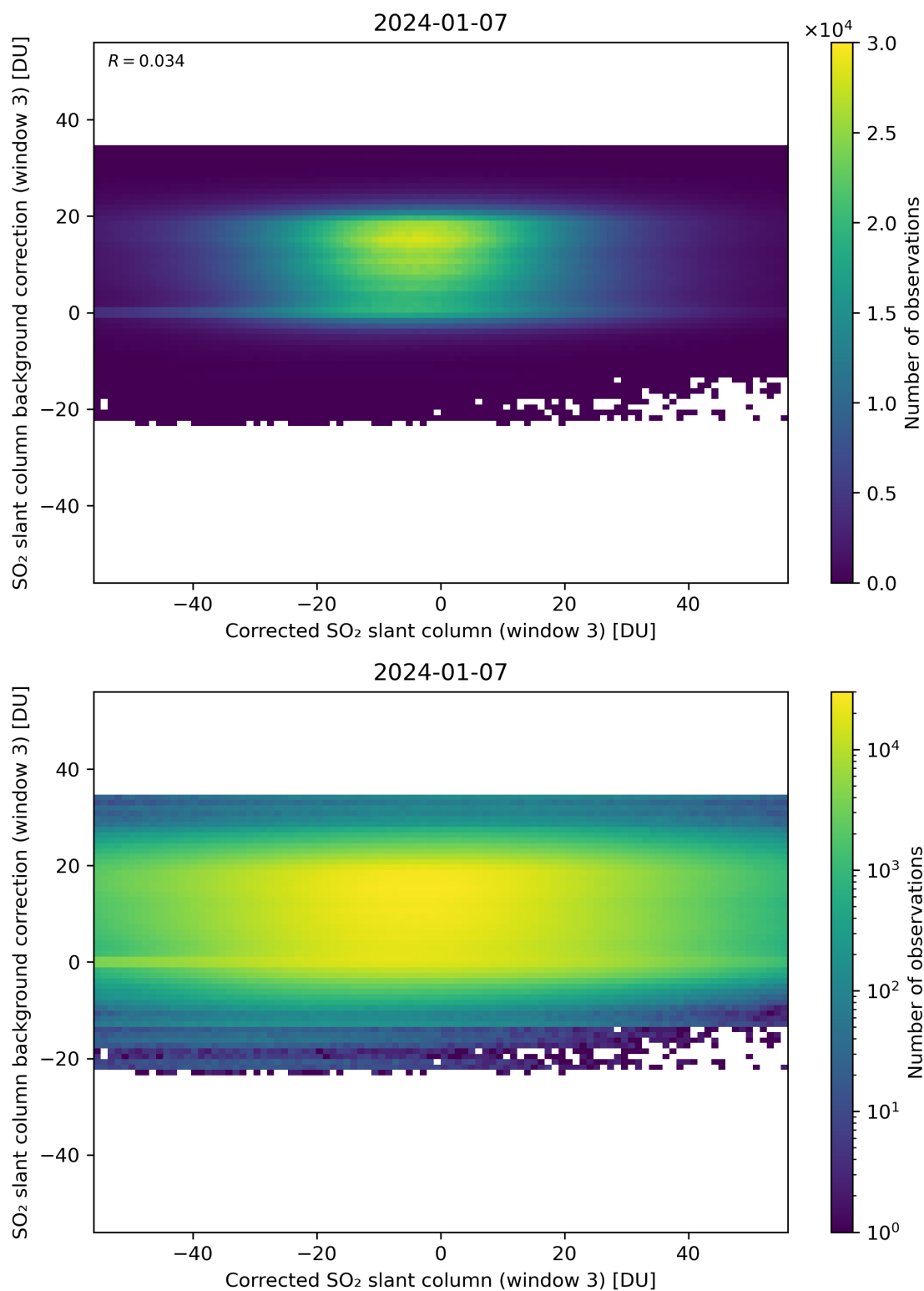
Figure 205: Scatter density plot of “Corrected SO 2 slant column (window 3)” against “SO 2 slant column background correction (window 3)” for 2024-01-06 to 2024-01-08.
