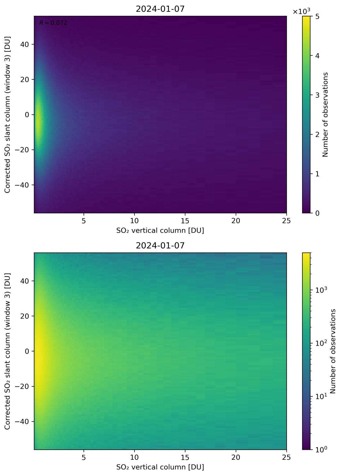
Figure 299: Scatter density plot of “SO 2 vertical column” against “Corrected SO 2 slant column (window 3)” for 2024-01-06 to 2024-01-08.
