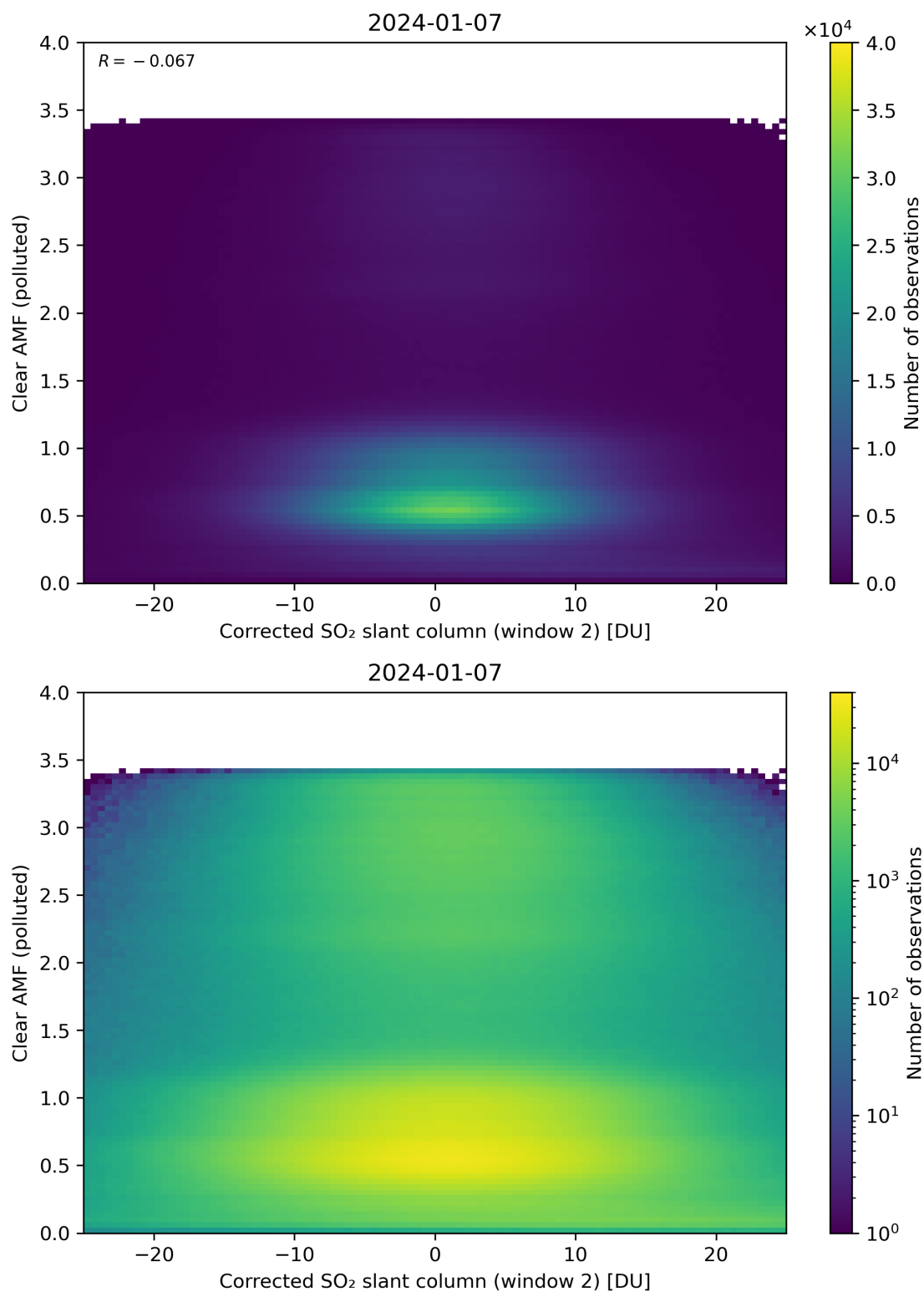
Figure 199: Scatter density plot of “Corrected SO 2 slant column (window 2)” against “Clear AMF (polluted)” for 2024-01-06 to 2024-01-08.
