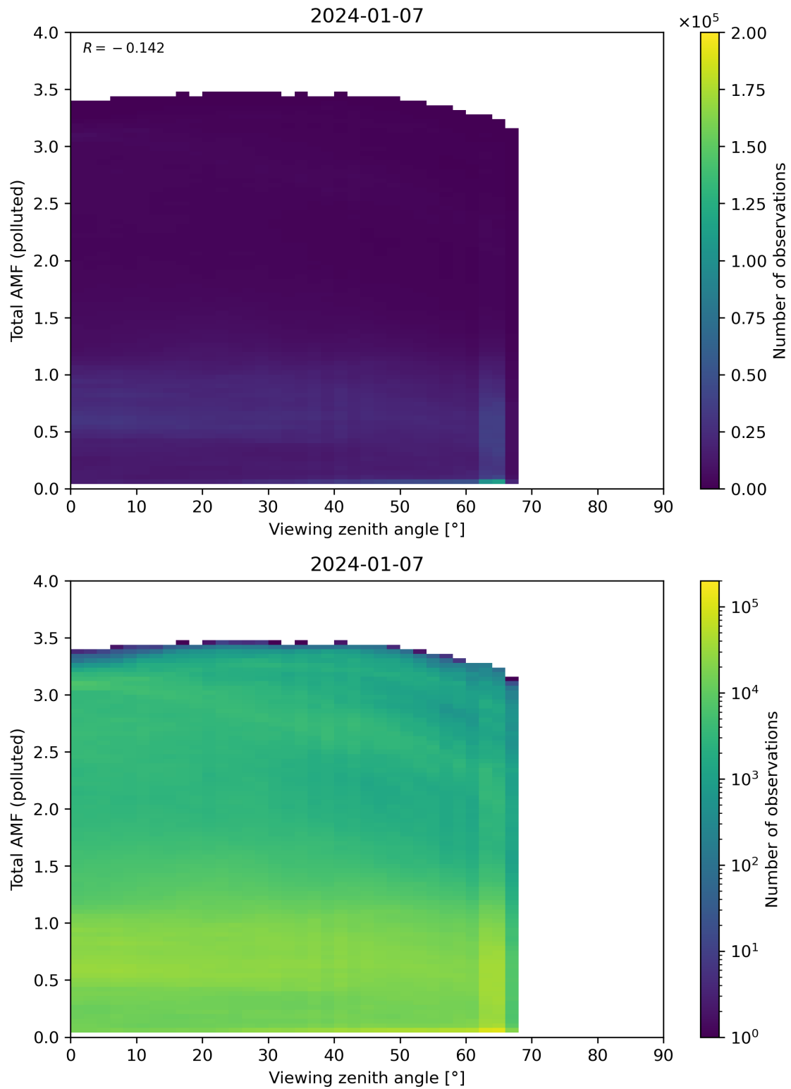
Figure 325: Scatter density plot of “Viewing zenith angle” against “Total AMF (polluted)” for 2024-01-06 to 2024-01-08.
