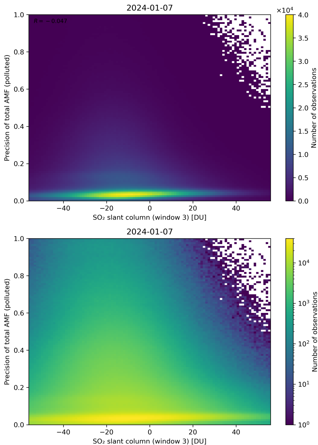
Figure 269: Scatter density plot of “SO 2 slant column (window 3)” against “Precision of total AMF (polluted)” for 2024-01-06 to 2024-01-08.
