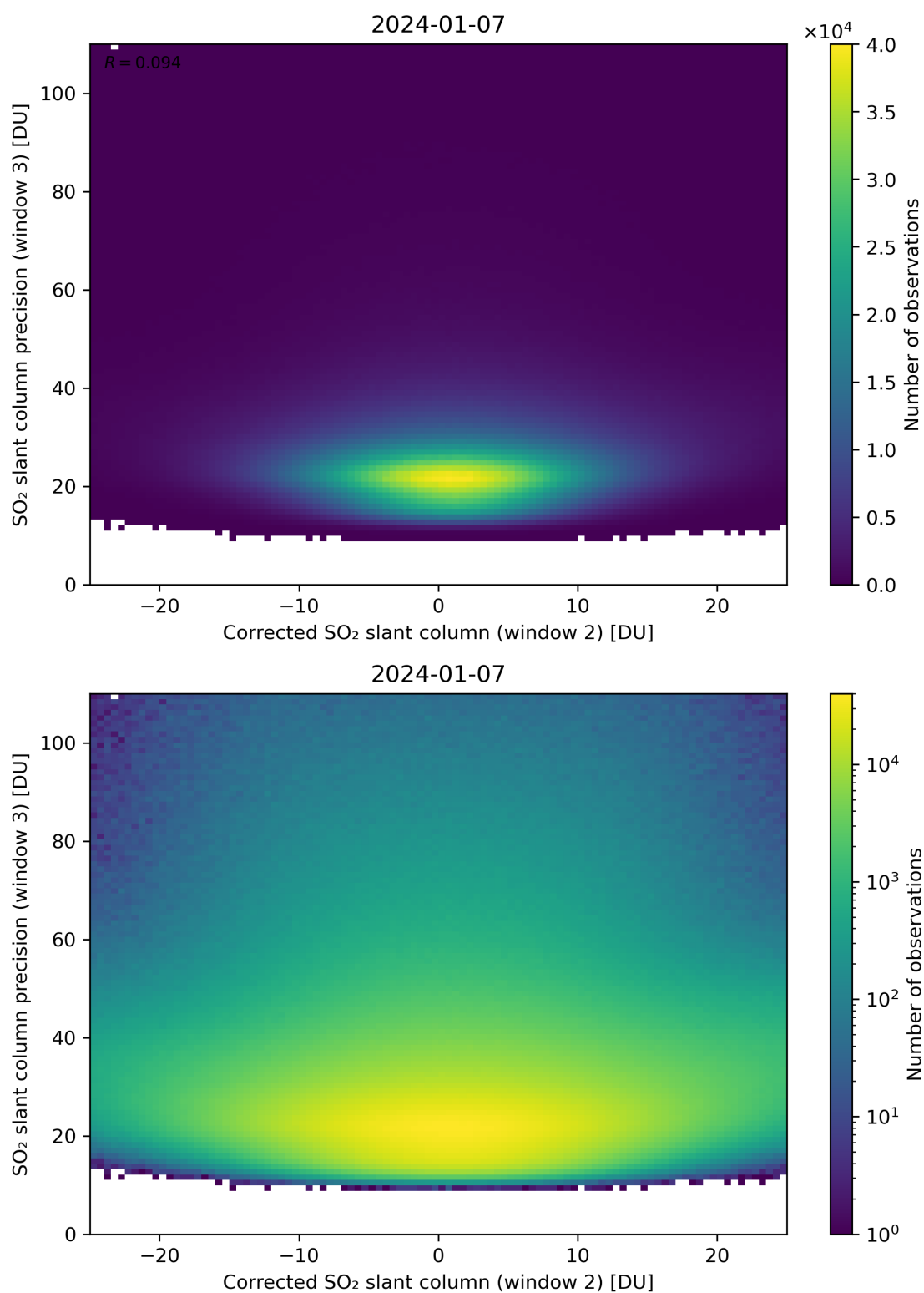
Figure 202: Scatter density plot of “Corrected SO 2 slant column (window 2)” against “SO 2 slant column precision (window 3)” for 2024-01-06 to 2024-01-08.
