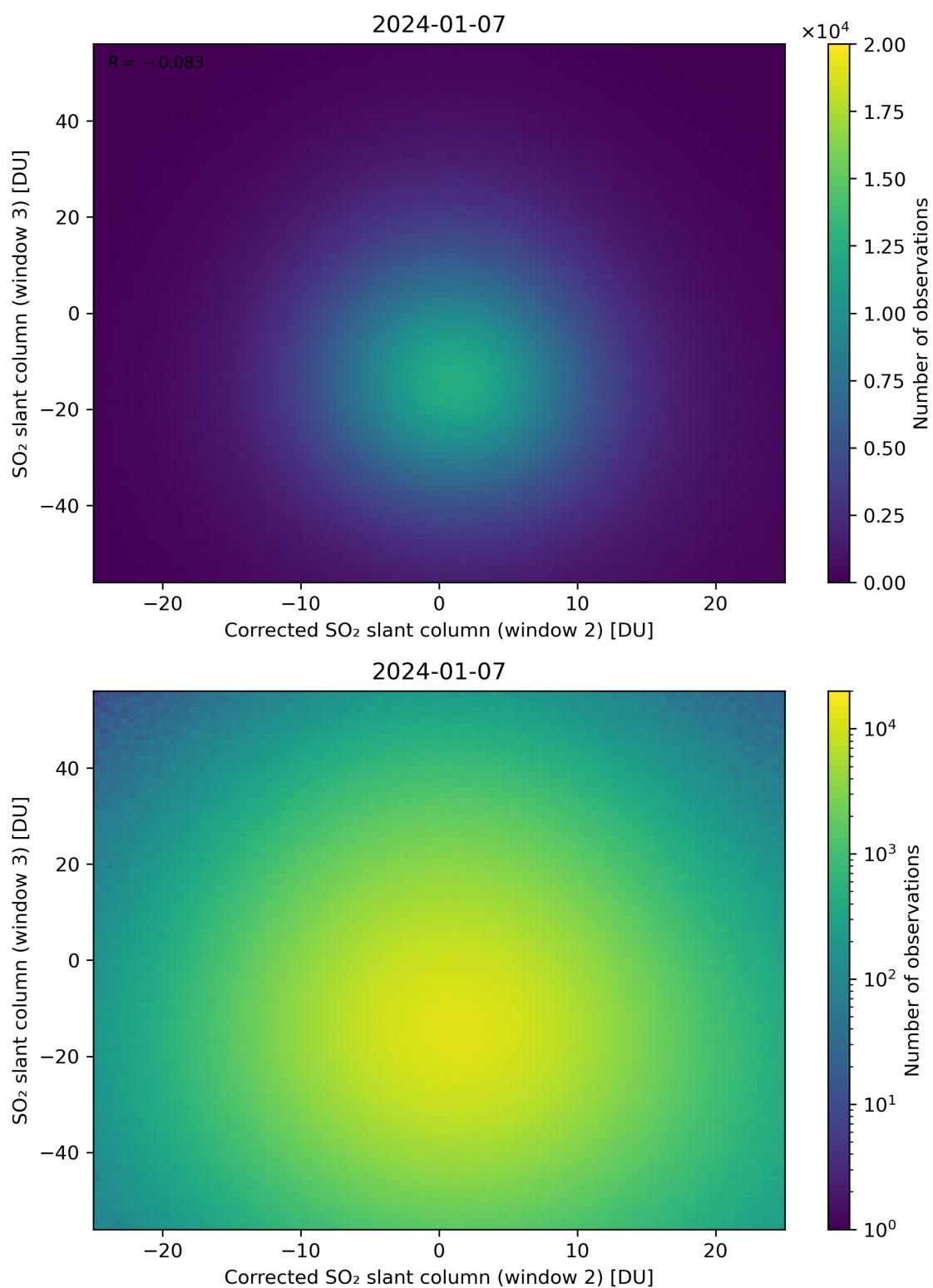
Figure 201: Scatter density plot of “Corrected SO 2 slant column (window 2)” against “SO 2 slant column (window 3)” for 2024-01-06 to 2024-01-08.
