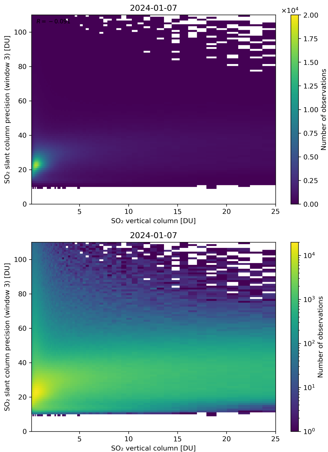
Figure 304: Scatter density plot of “SO 2 vertical column” against “SO 2 slant column precision (window 3)” for 2024-01-06 to 2024-01-08.
