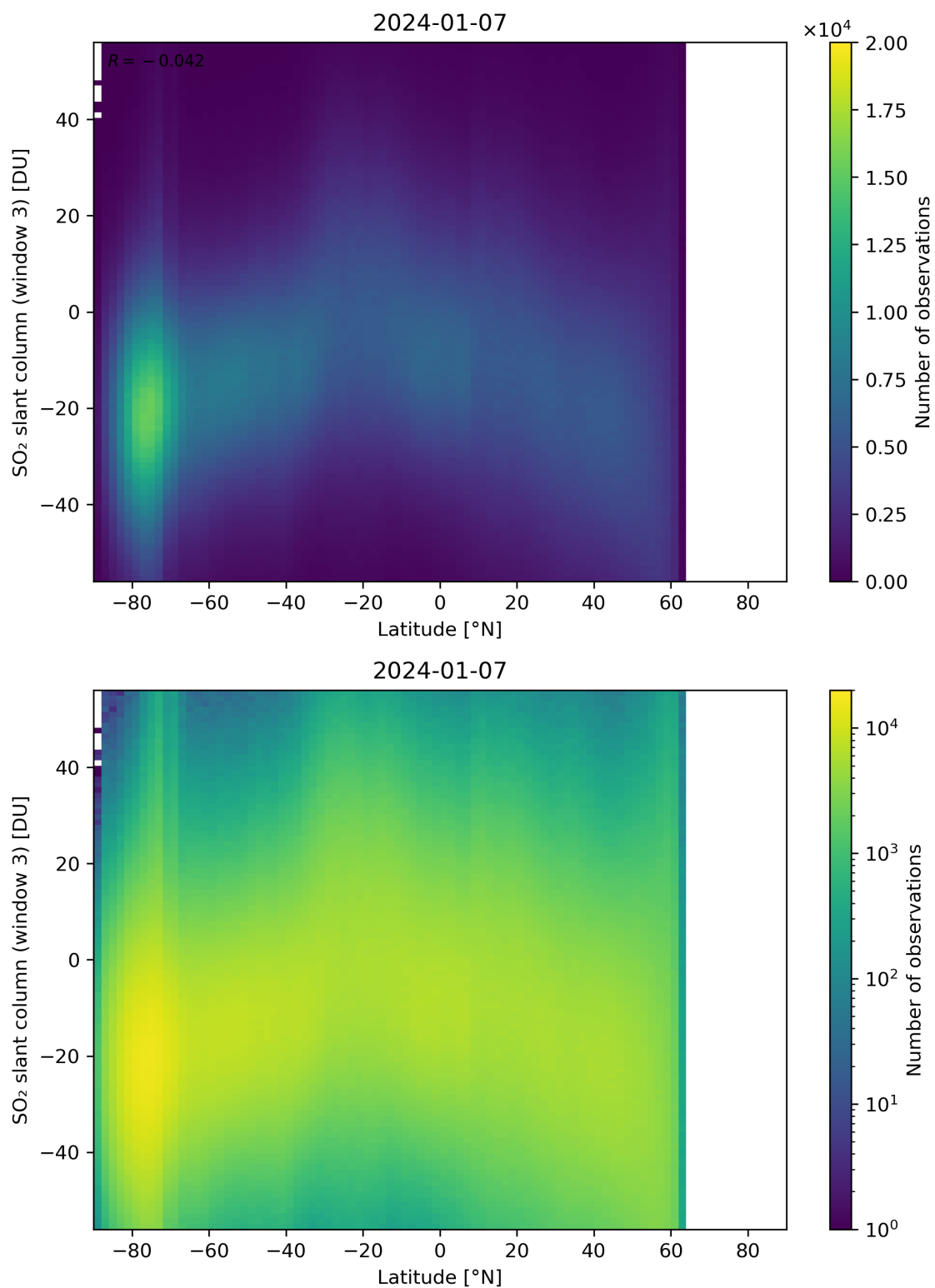
Figure 152: Scatter density plot of “Latitude” against “SO 2 slant column (window 3)” for 2024-01-06 to 2024-01-08.
