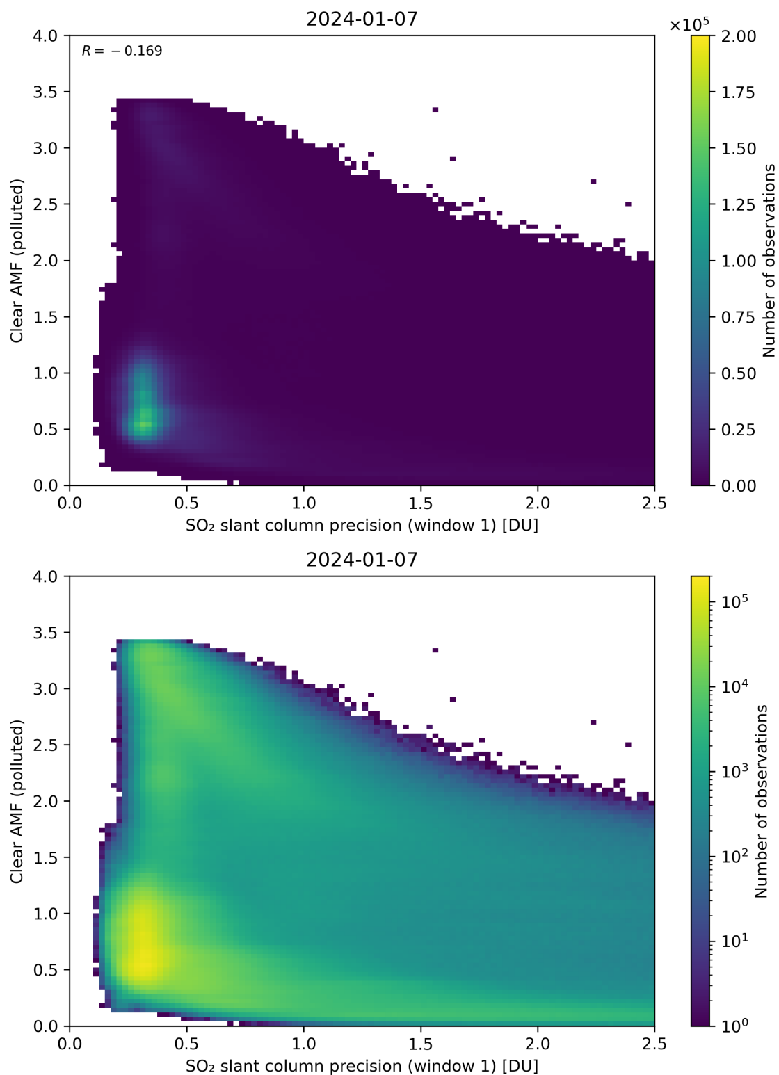
Figure 224: Scatter density plot of “SO 2 slant column precision (window 1)” against “Clear AMF (polluted)” for 2024-01-06 to 2024-01-08.
