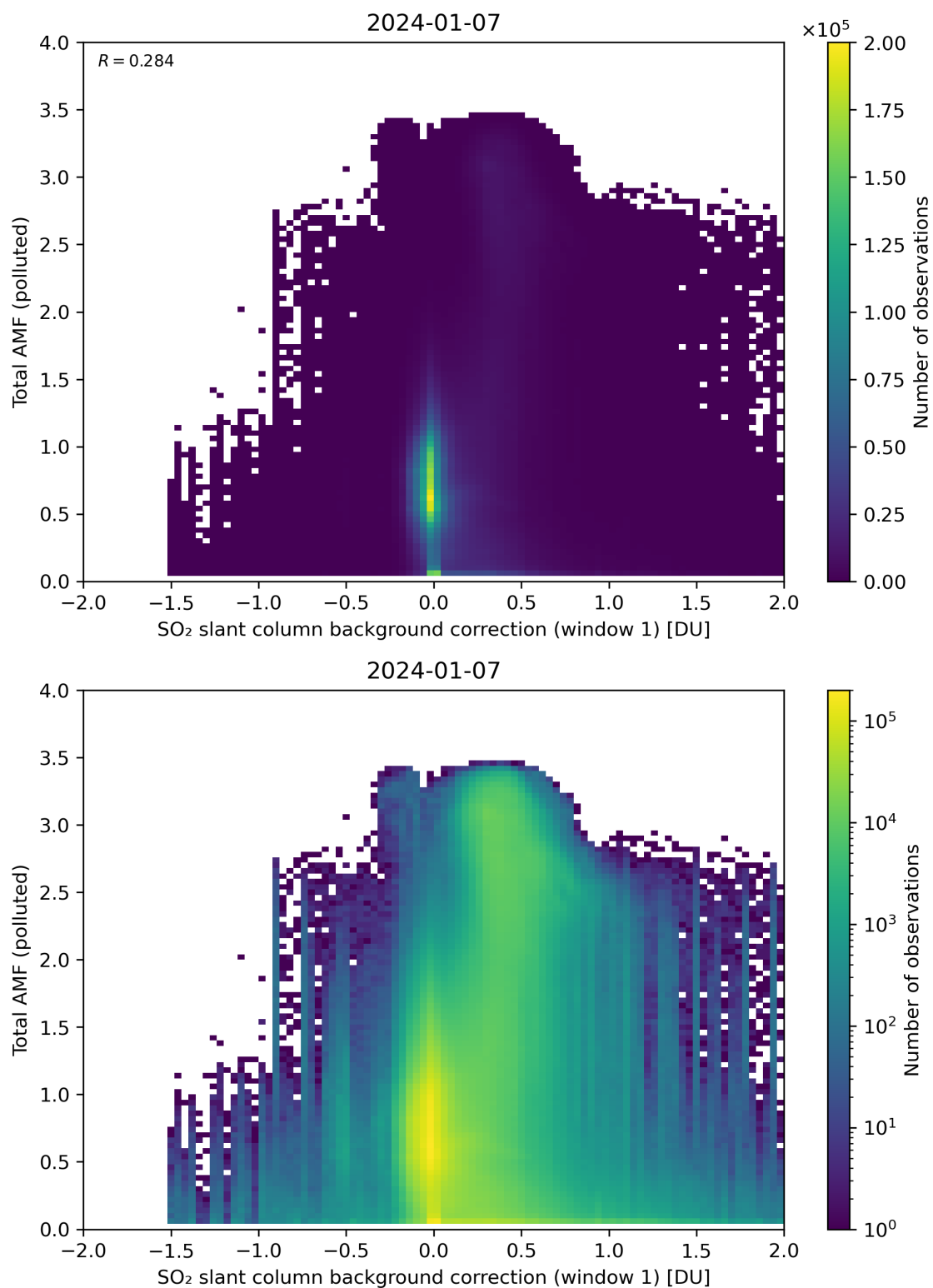
Figure 109: Scatter density plot of “SO 2 slant column background correction (window 1)” against “Total AMF (polluted)” for 2024-01-06 to 2024-01-08.
