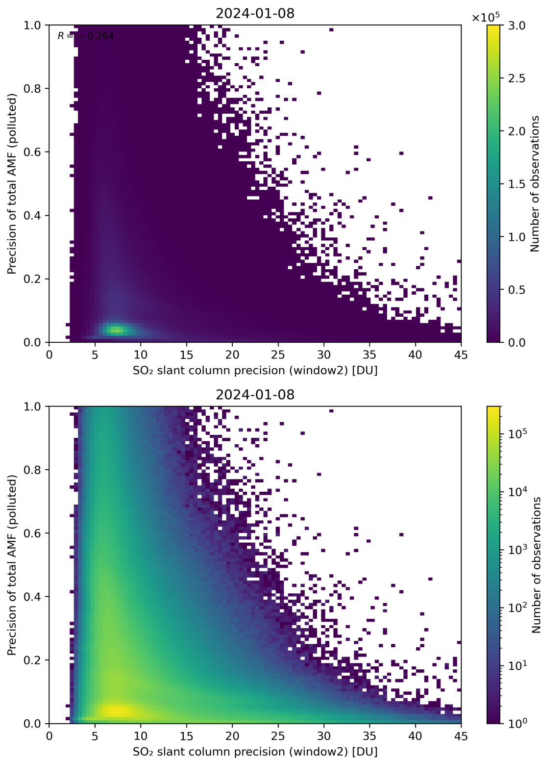
Figure 252: Scatter density plot of “SO 2 slant column precision (window2)” against “Precision of total AMF (polluted)” for 2024-01-07 to 2024-01-09.
