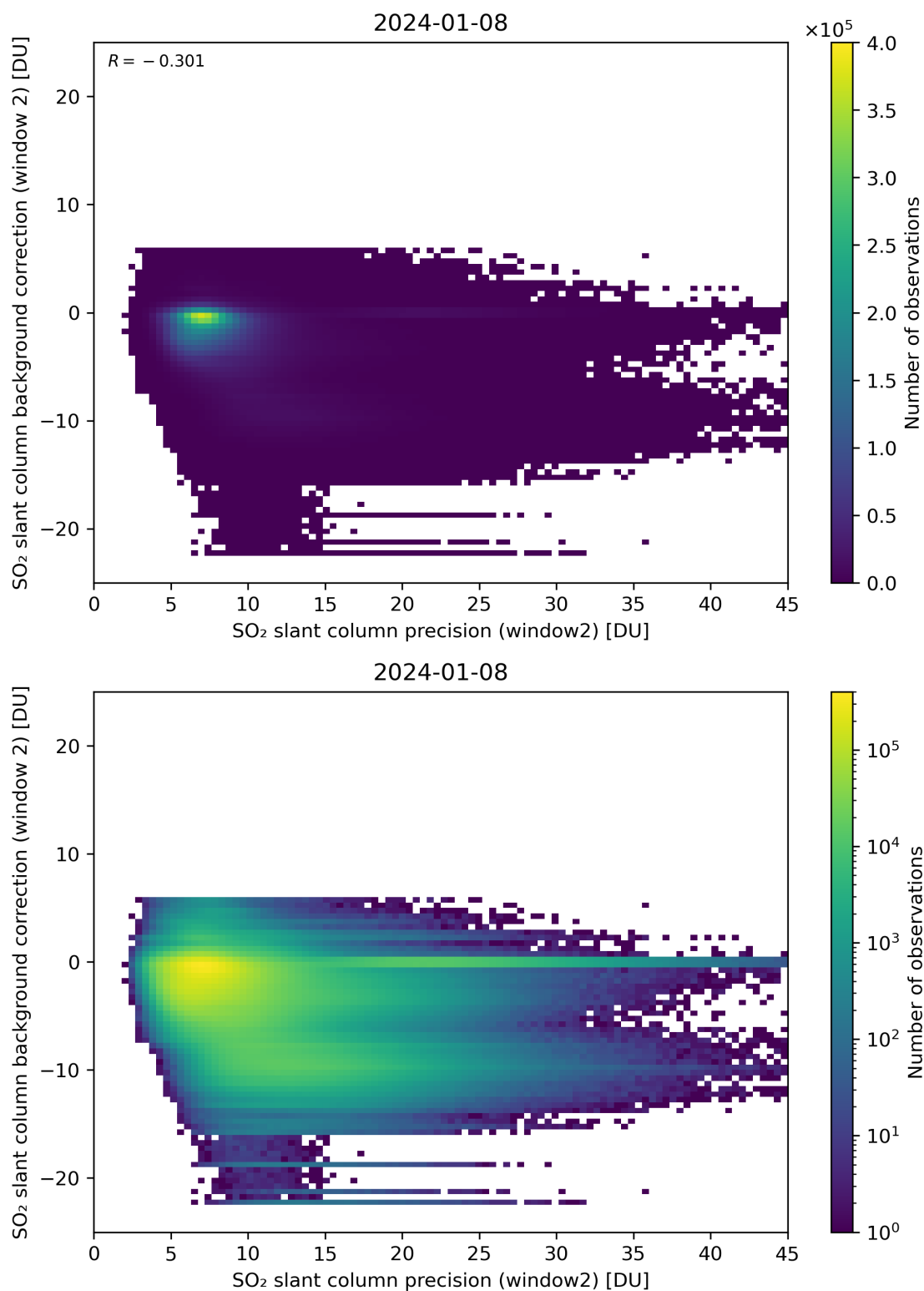
Figure 241: Scatter density plot of “SO 2 slant column precision (window2)” against “SO 2 slant column background correction (window 2)” for 2024-01-07 to 2024-01-09.
