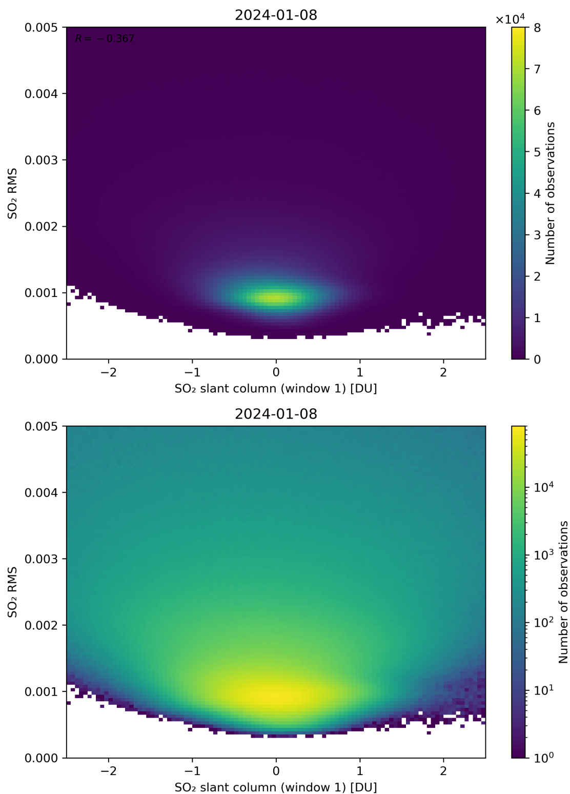
Figure 217: Scatter density plot of “SO 2 slant column (window 1)” against “SO 2 RMS” for 2024-01-07 to 2024-01-09.
