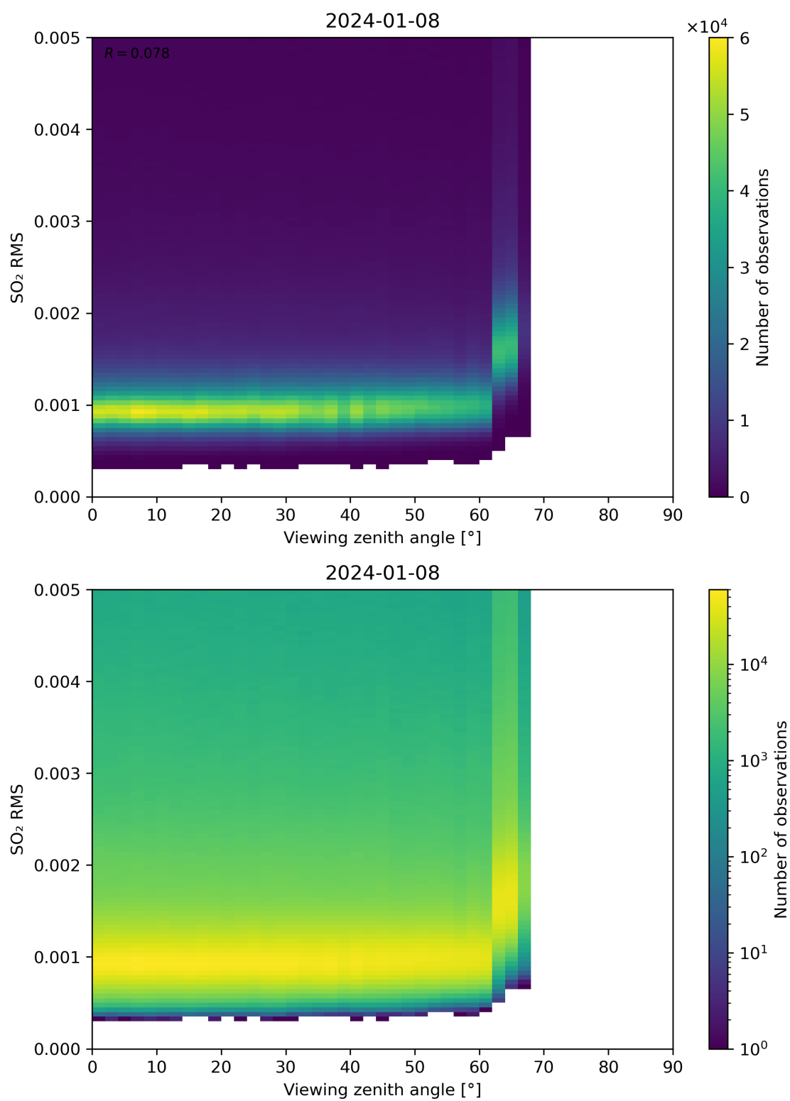
Figure 313: Scatter density plot of “Viewing zenith angle” against “SO 2 RMS” for 2024-01-07 to 2024-01-09.
