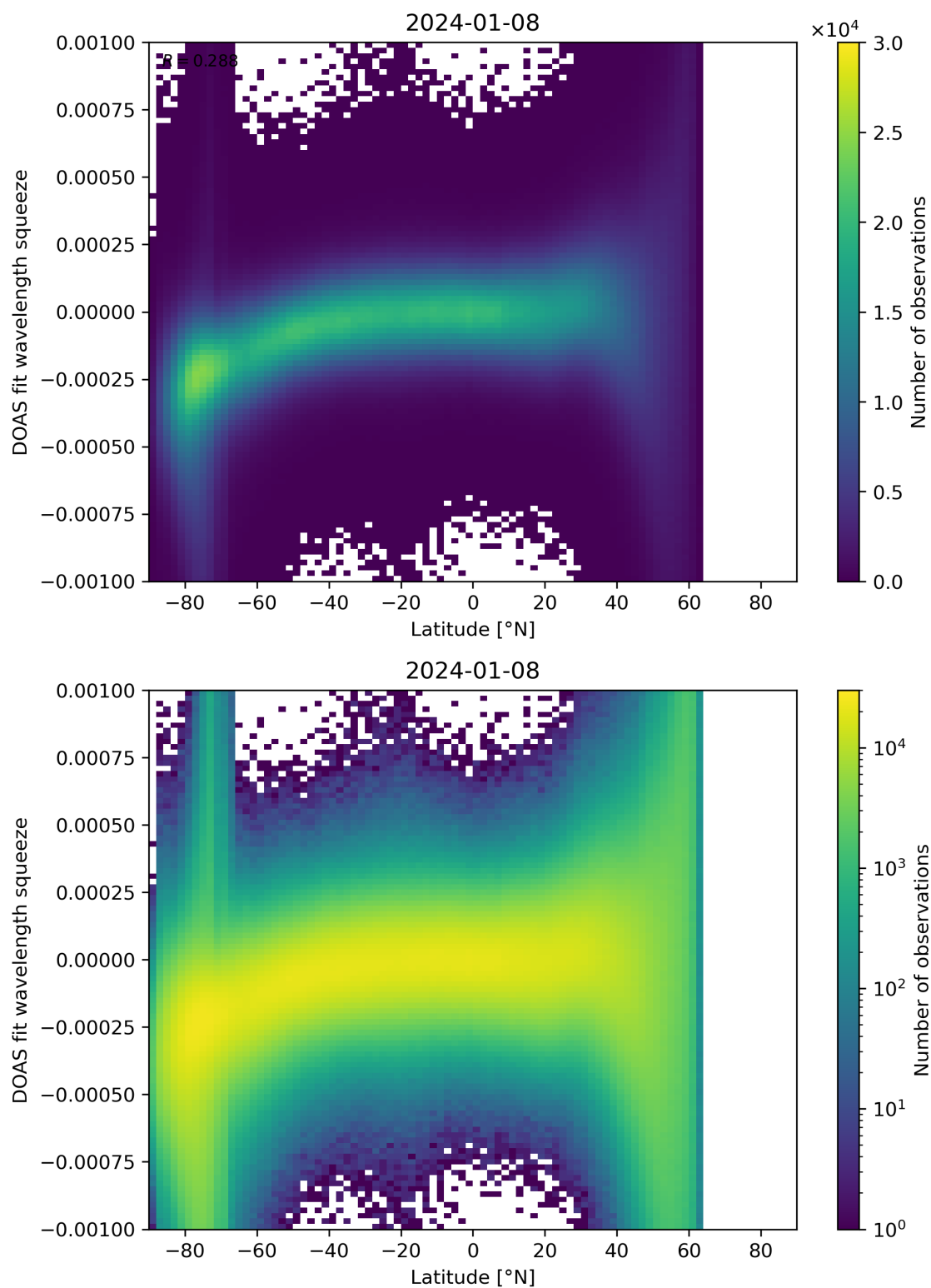
Figure 143: Scatter density plot of “Latitude” against “DOAS fit wavelength squeeze” for 2024-01-07 to 2024-01-09.
