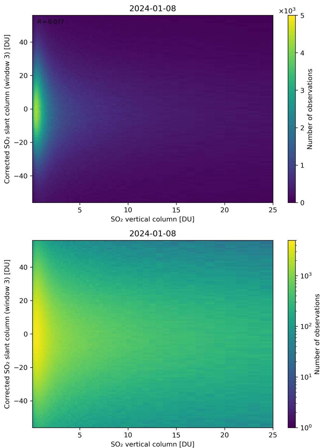
Figure 299: Scatter density plot of “SO 2 vertical column” against “Corrected SO 2 slant column (window 3)” for 2024-01-07 to 2024-01-09.
