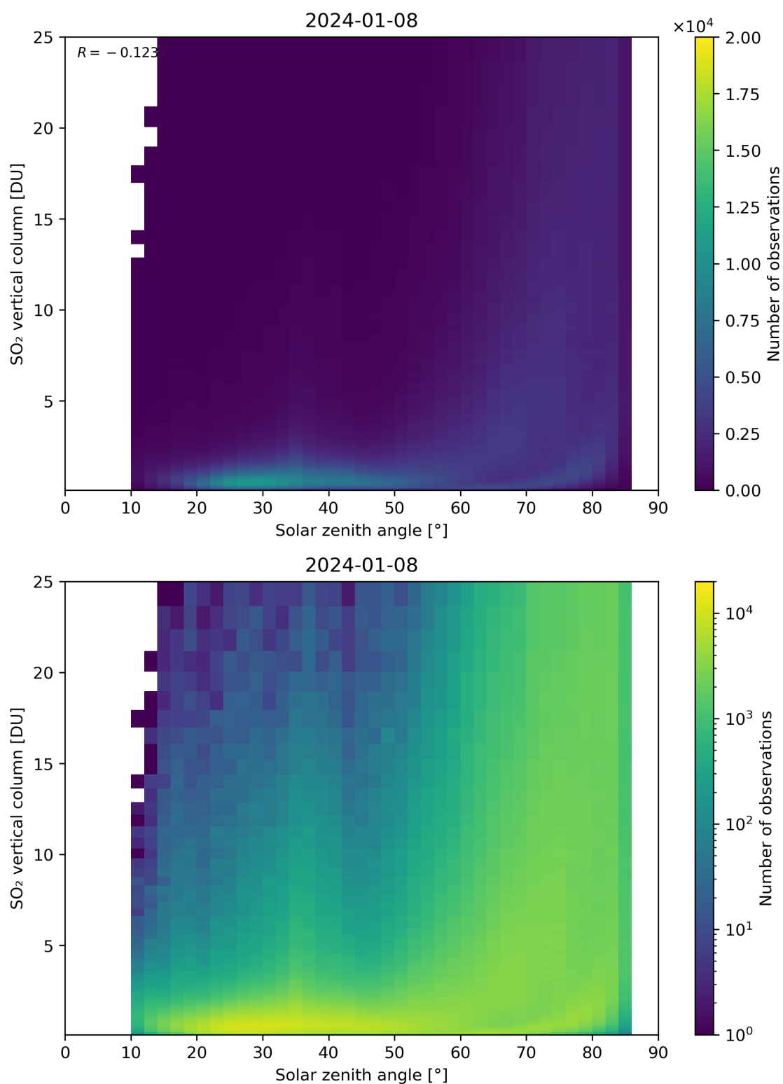
Figure 176: Scatter density plot of “Solar zenith angle” against “SO 2 vertical column” for 2024-01-07 to 2024-01-09.
