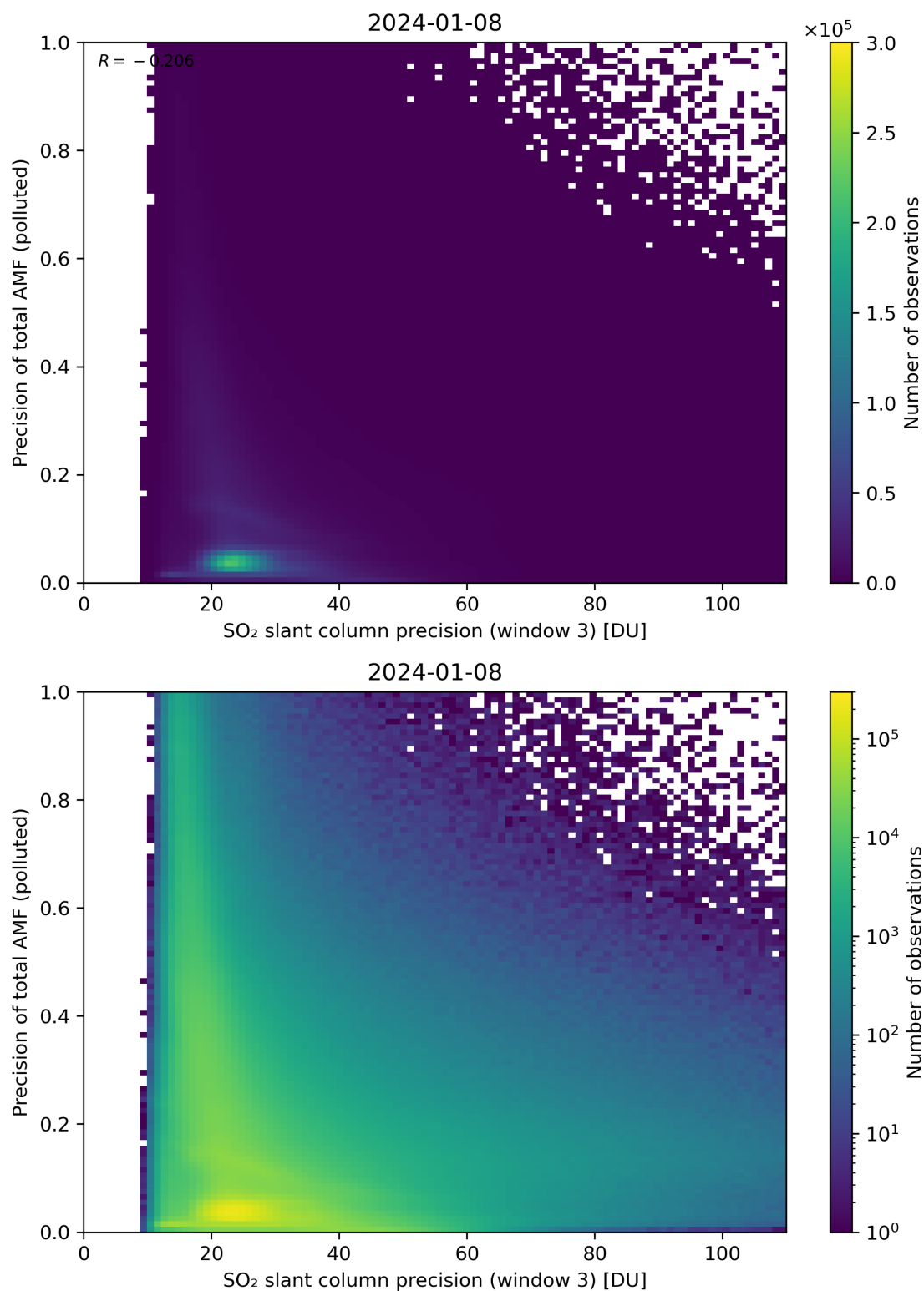
Figure 264: Scatter density plot of “SO 2 slant column precision (window 3)” against “Precision of total AMF (polluted)” for 2024-01-07 to 2024-01-09.
