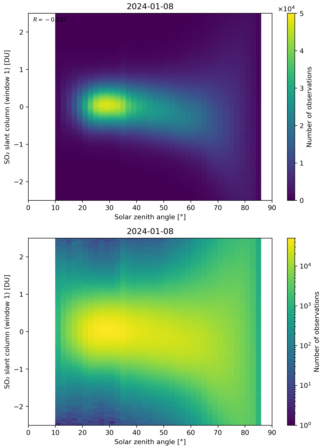
Figure 169: Scatter density plot of “Solar zenith angle” against “SO 2 slant column (window 1)” for 2024-01-07 to 2024-01-09.
