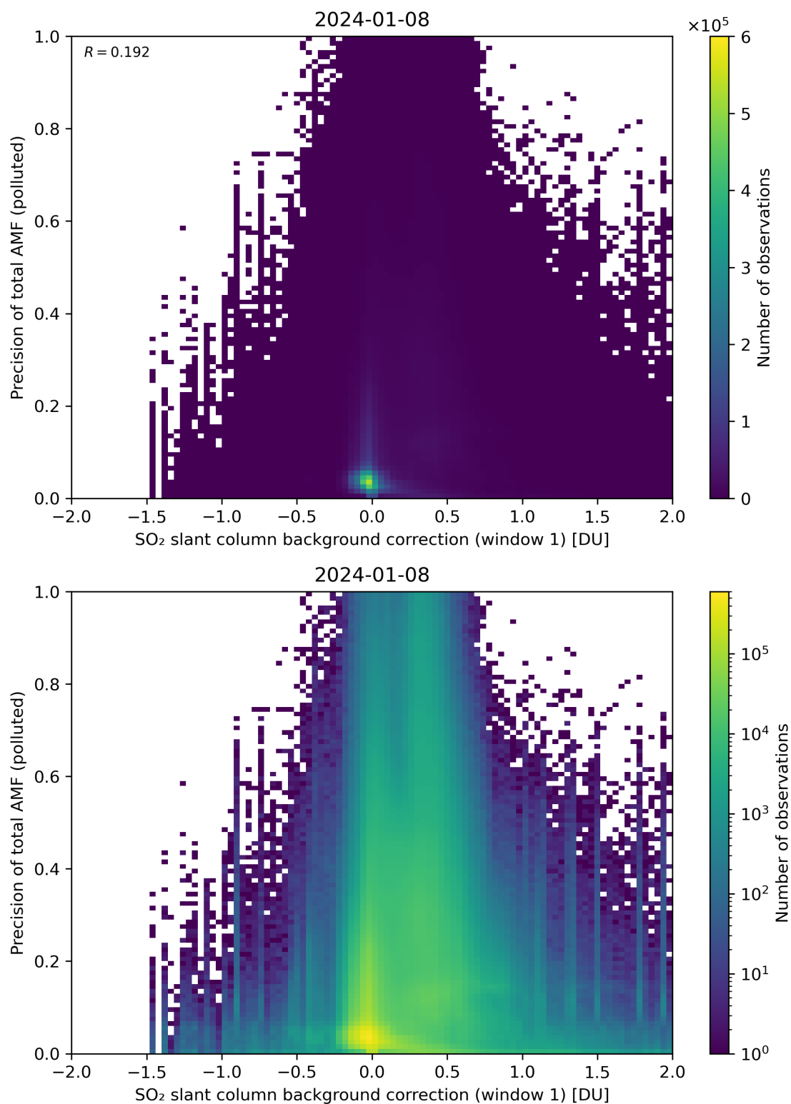
Figure 110: Scatter density plot of “SO 2 slant column background correction (window 1)” against “Precision of total AMF (polluted)” for 2024-01-07 to 2024-01-09.
