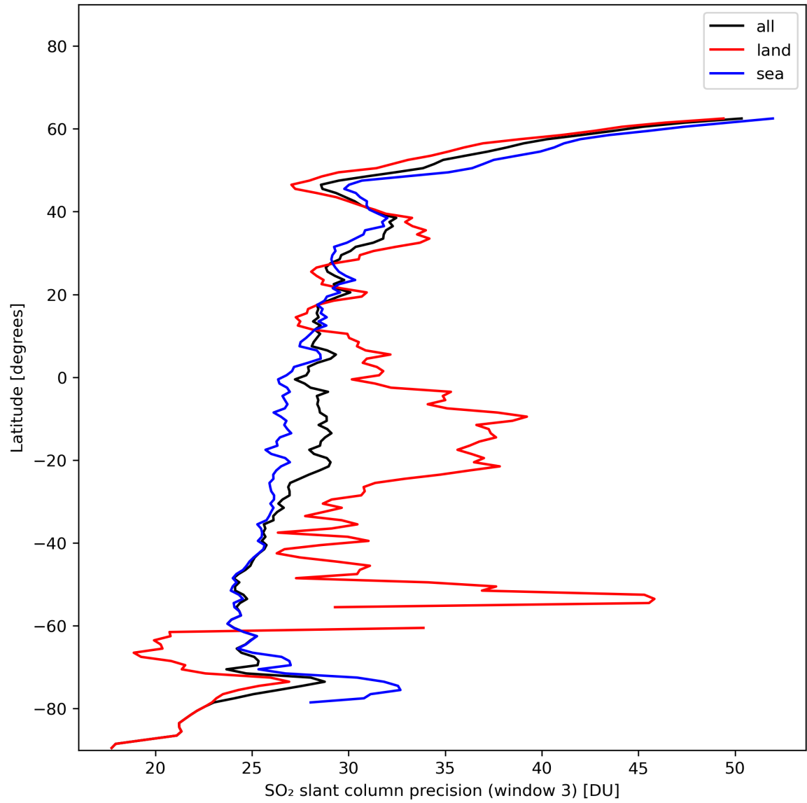
Figure 42: Zonal average of “SO 2 slant column precision (window 3)” for 2024-01-07 to 2024-01-09.
