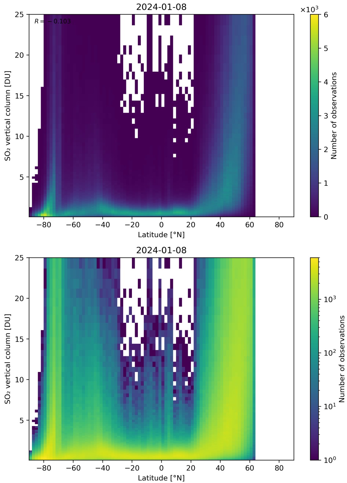
Figure 156: Scatter density plot of “Latitude” against “SO 2 vertical column” for 2024-01-07 to 2024-01-09.
