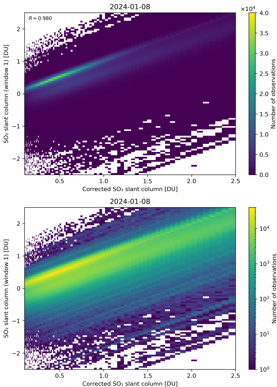
Figure 187: Scatter density plot of “Corrected SO 2 slant column” against “SO 2 slant column (window 1)” for 2024-01-07 to 2024-01-09.
