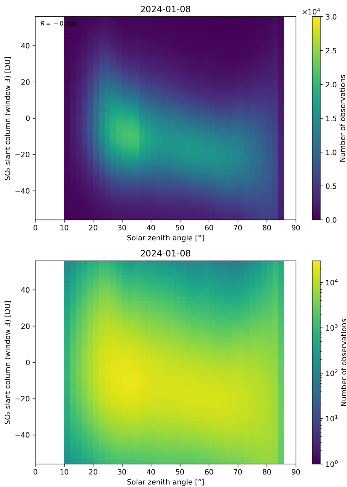
Figure 172: Scatter density plot of “Solar zenith angle” against “SO 2 slant column (window 3)” for 2024-01-07 to 2024-01-09.
