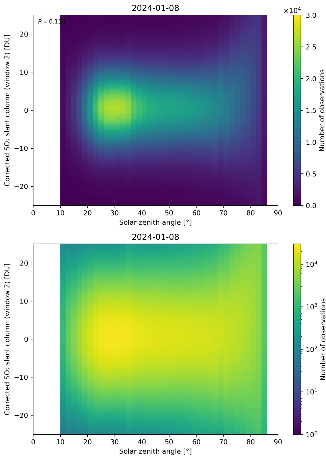
Figure 167: Scatter density plot of “Solar zenith angle” against “Corrected SO 2 slant column (window 2)” for 2024-01-07 to 2024-01-09.
