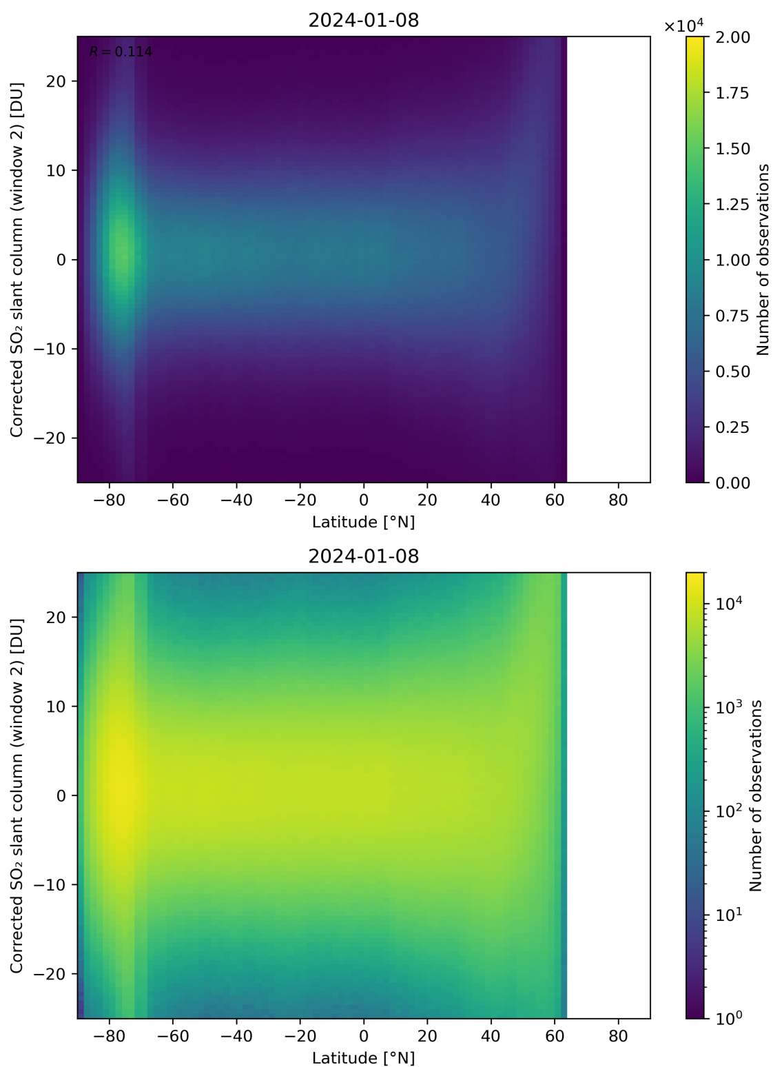
Figure 147: Scatter density plot of “Latitude” against “Corrected SO 2 slant column (window 2)” for 2024-01-07 to 2024-01-09.
