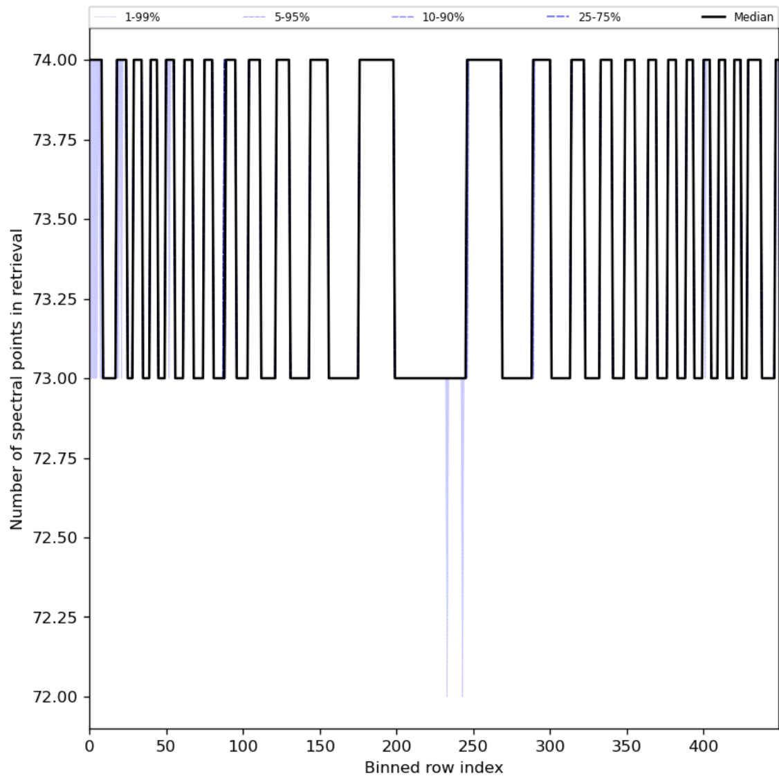
Figure 97: Along track statistics of “Number of spectral points in retrieval” for 2024-01-07 to 2024-01-09
