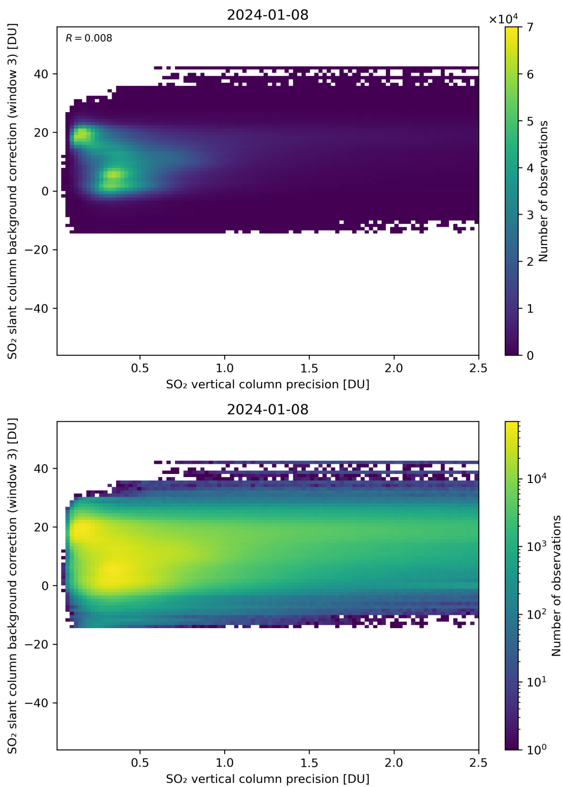
Figure 281: Scatter density plot of “SO 2 vertical column precision” against “SO 2 slant column background correction (window 3)” for 2024-01-07 to 2024-01-09.
