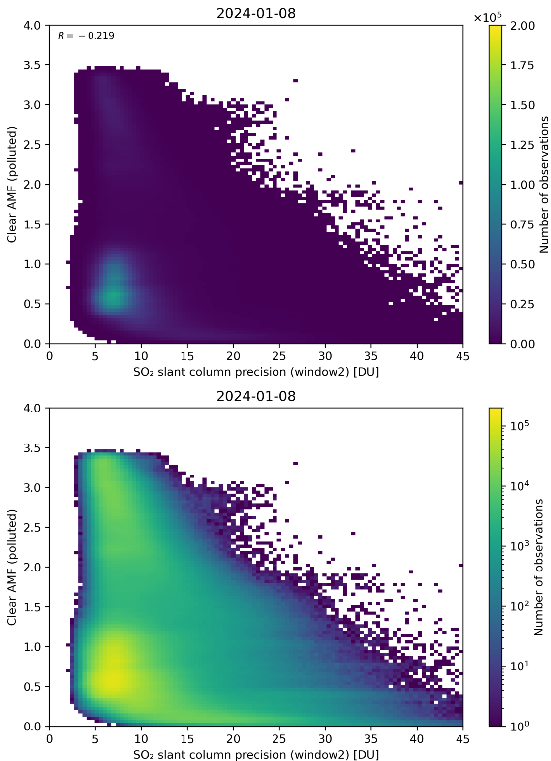
Figure 246: Scatter density plot of “SO 2 slant column precision (window2)” against “Clear AMF (polluted)” for 2024-01-07 to 2024-01-09.
