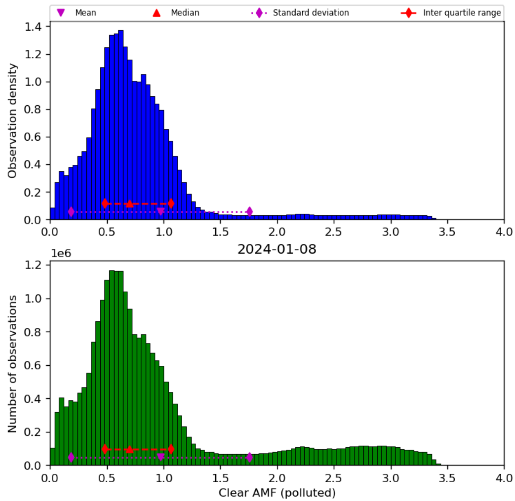
Figure 73: Histogram of “Clear AMF (polluted)” for 2024-01-07 to 2024-01-09
