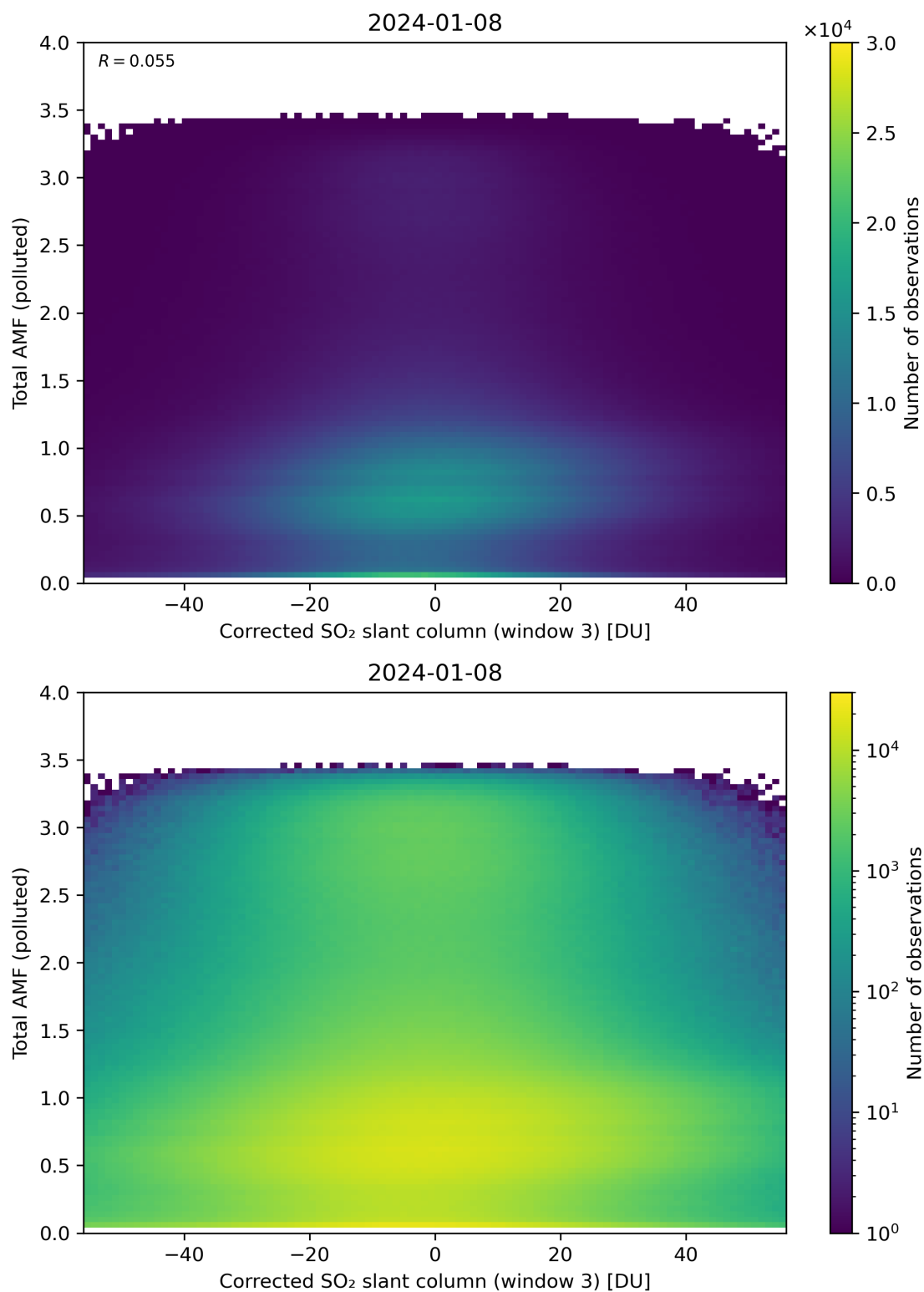
Figure 210: Scatter density plot of “Corrected SO 2 slant column (window 3)” against “Total AMF (polluted)” for 2024-01-07 to 2024-01-09.
