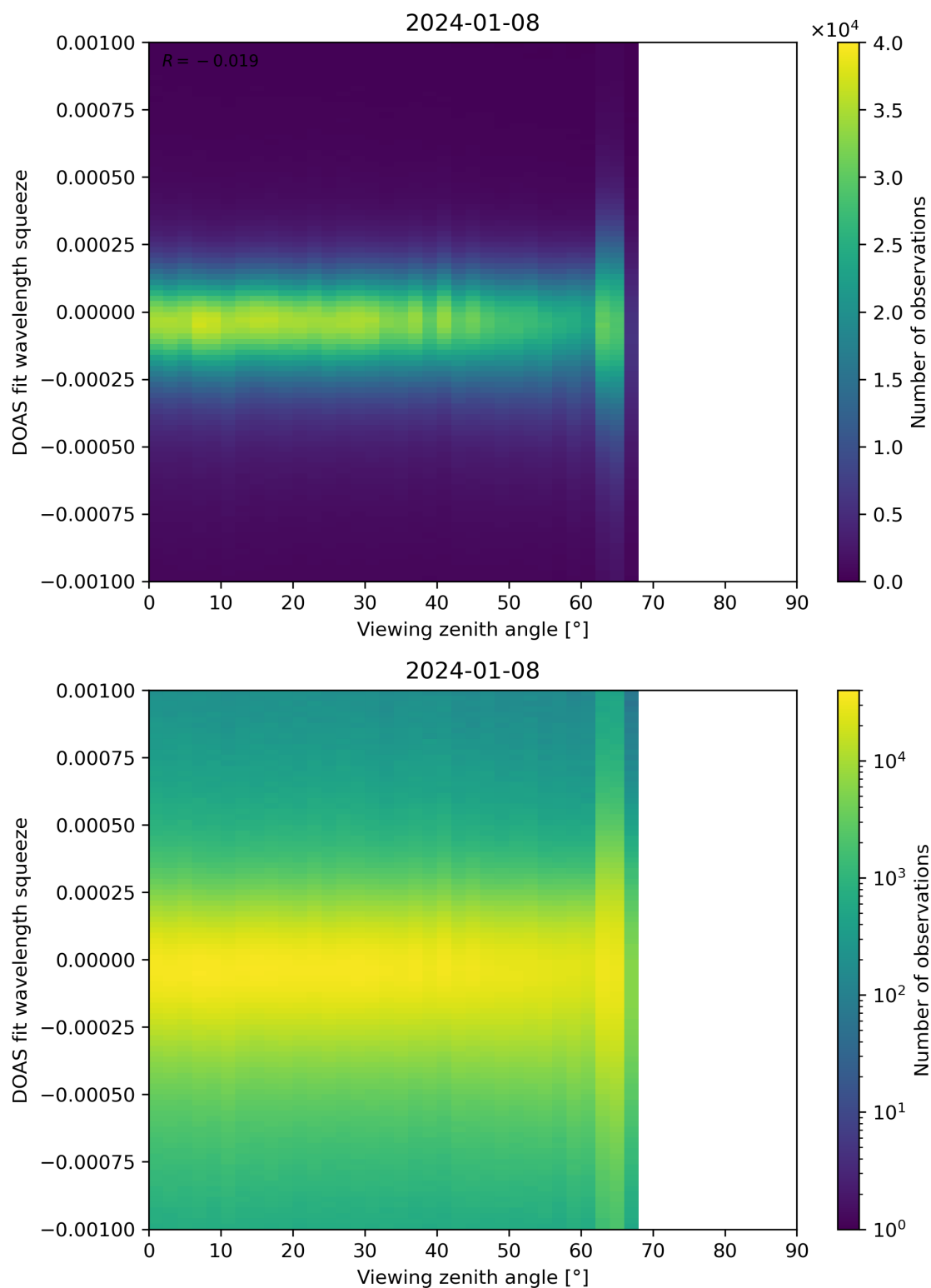
Figure 312: Scatter density plot of “Viewing zenith angle” against “DOAS fit wavelength squeeze” for 2024-01-07 to 2024-01-09.
