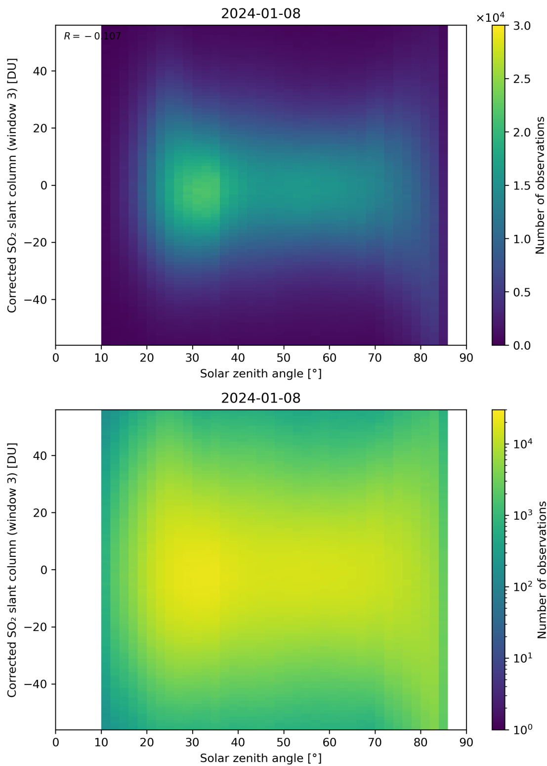
Figure 168: Scatter density plot of “Solar zenith angle” against “Corrected SO 2 slant column (window 3)” for 2024-01-07 to 2024-01-09.
