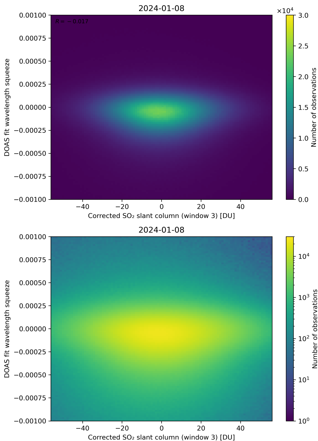
Figure 207: Scatter density plot of “Corrected SO 2 slant column (window 3)” against “DOAS fit wavelength squeeze” for 2024-01-07 to 2024-01-09.
