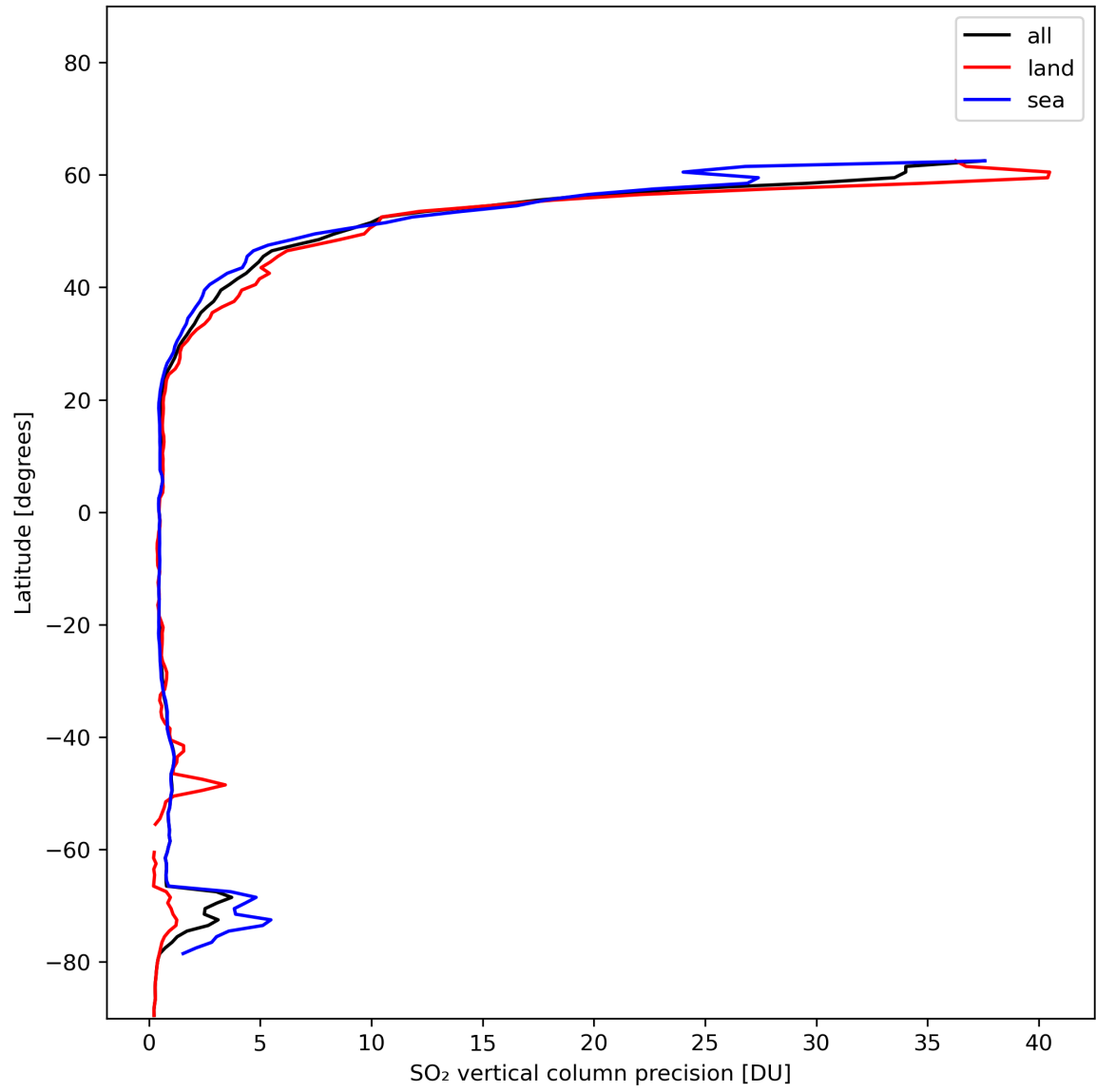
Figure 31: Zonal average of “SO 2 vertical column precision” for 2024-01-07 to 2024-01-09.
