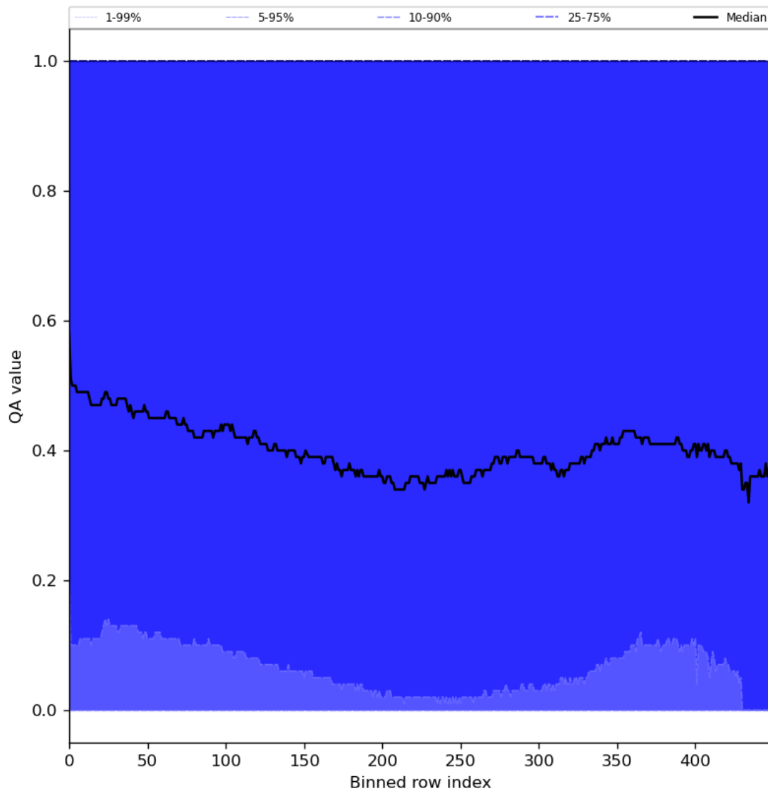
Figure 75: Along track statistics of “QA value” for 2024-01-07 to 2024-01-09
