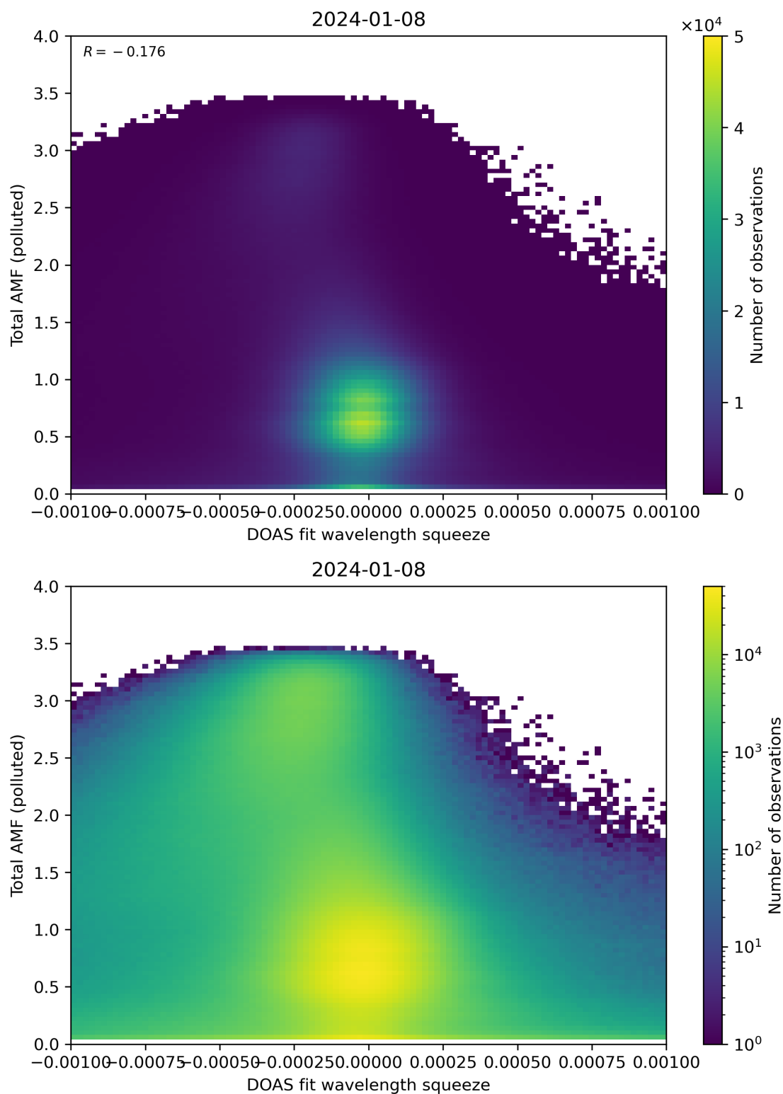
Figure 134: Scatter density plot of “DOAS fit wavelength squeeze” against “Total AMF (polluted)” for 2024-01-07 to 2024-01-09.
