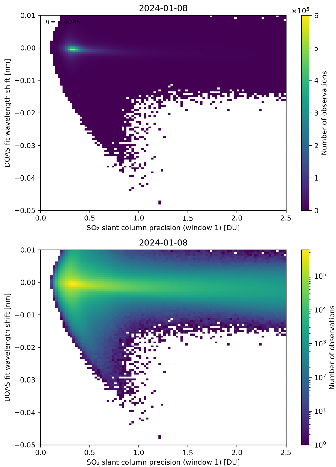
Figure 221: Scatter density plot of “SO 2 slant column precision (window 1)” against “DOAS fit wavelength shift” for 2024-01-07 to 2024-01-09.
