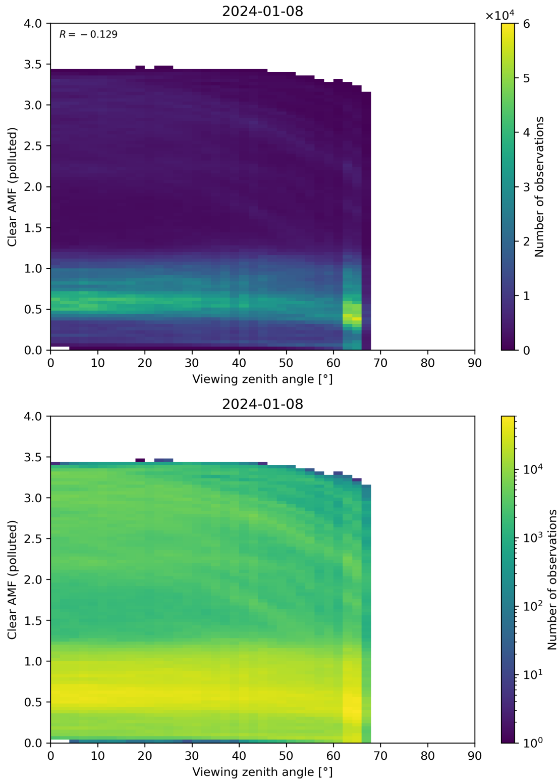
Figure 316: Scatter density plot of “Viewing zenith angle” against “Clear AMF (polluted)” for 2024-01-07 to 2024-01-09.
