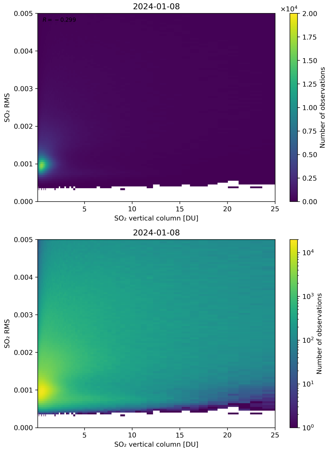
Figure 278: Scatter density plot of “SO 2 vertical column” against “SO 2 RMS” for 2024-01-07 to 2024-01-09.
