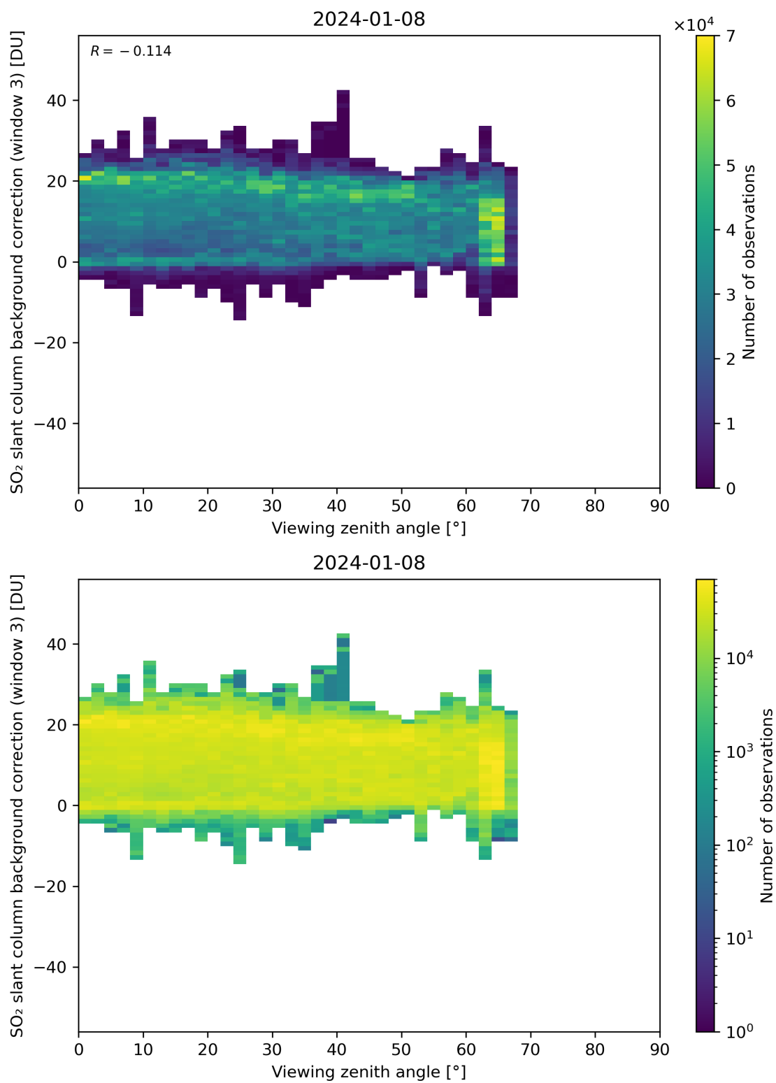
Figure 310: Scatter density plot of “Viewing zenith angle” against “SO 2 slant column background correction (window 3)” for 2024-01-07 to 2024-01-09.
