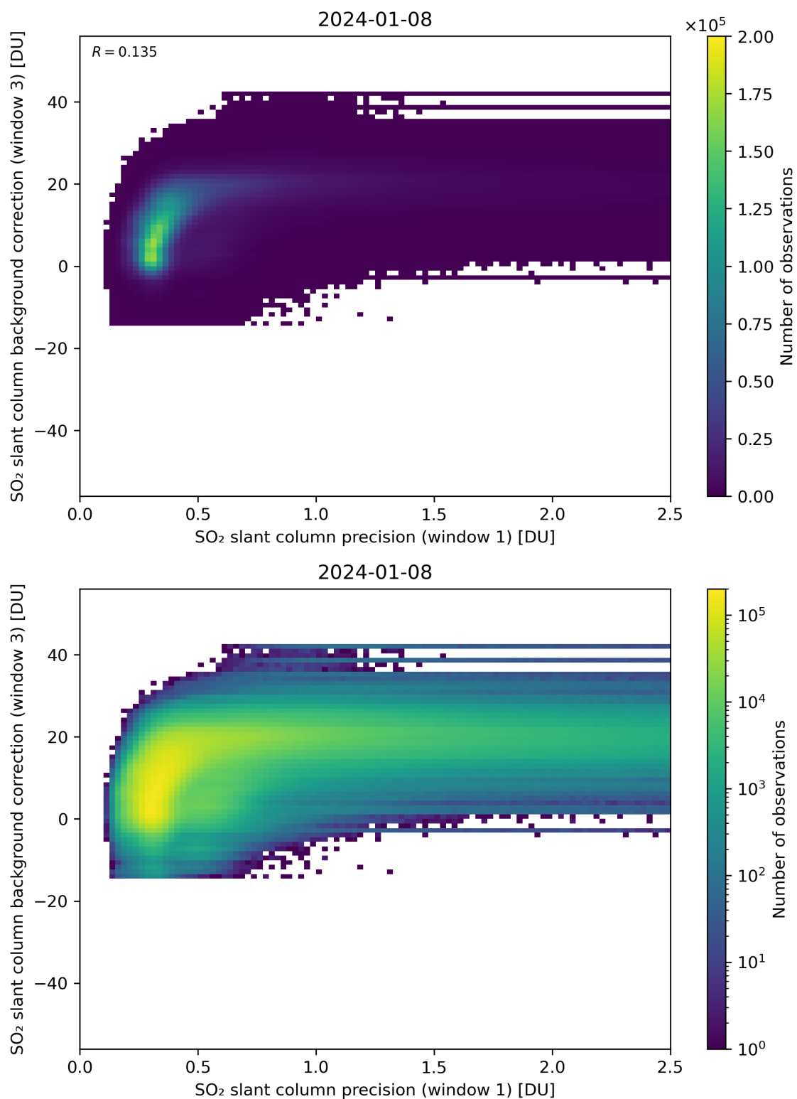
Figure 220: Scatter density plot of “SO 2 slant column precision (window 1)” against “SO 2 slant column background correction (window 3)” for 2024-01-07 to 2024-01-09.
