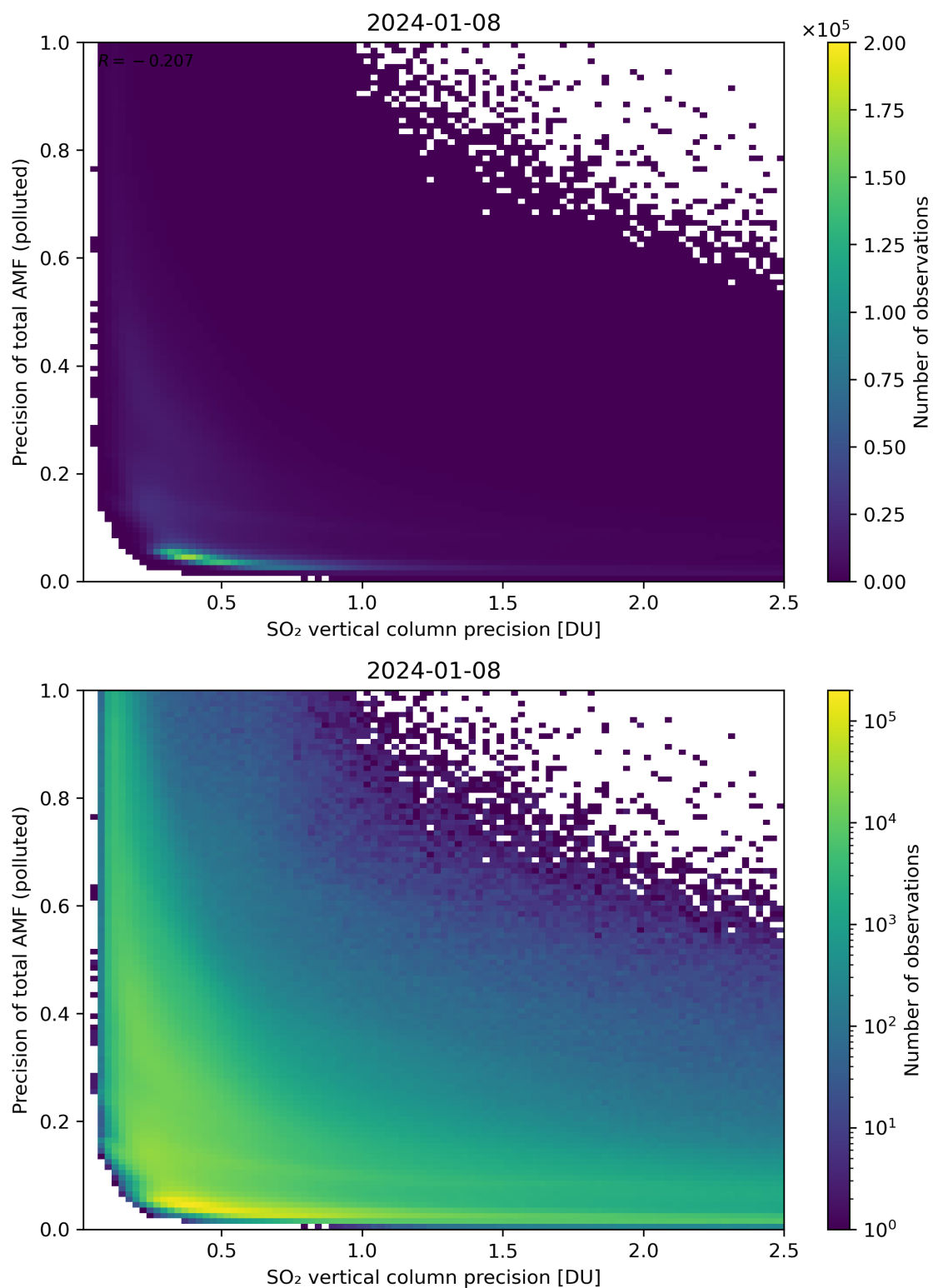
Figure 295: Scatter density plot of “SO 2 vertical column precision” against “Precision of total AMF (polluted)” for 2024-01-07 to 2024-01-09.
