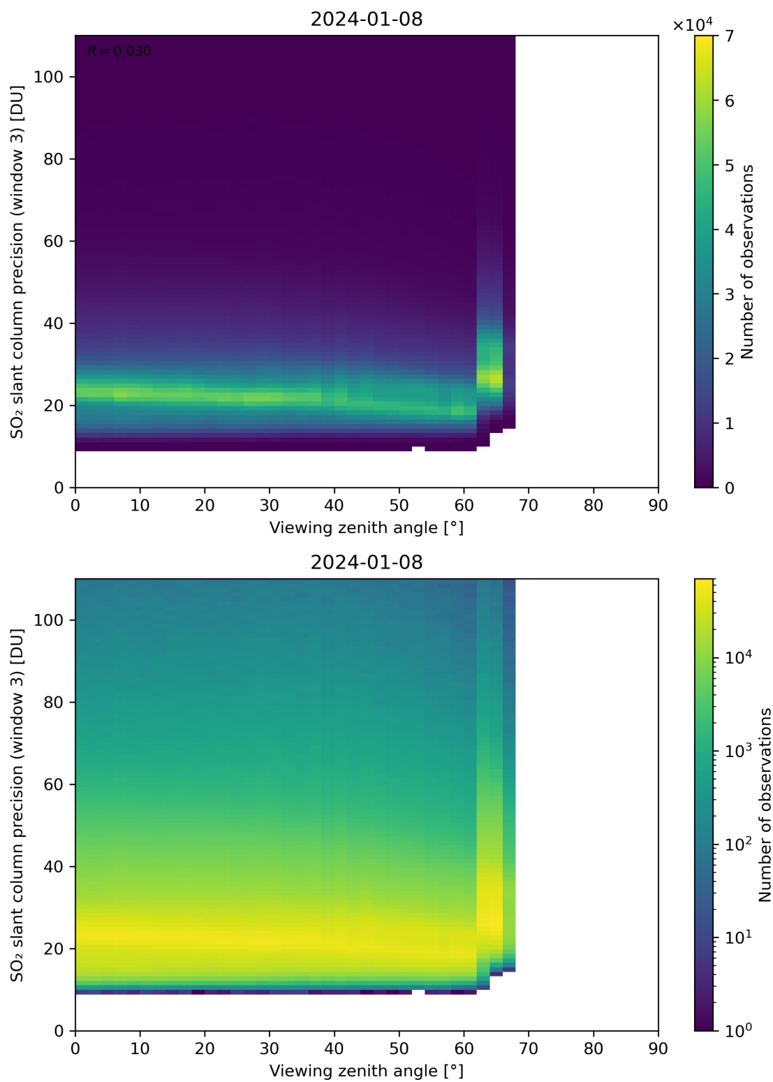
Figure 324: Scatter density plot of “Viewing zenith angle” against “SO 2 slant column precision (window 3)” for 2024-01-07 to 2024-01-09.
