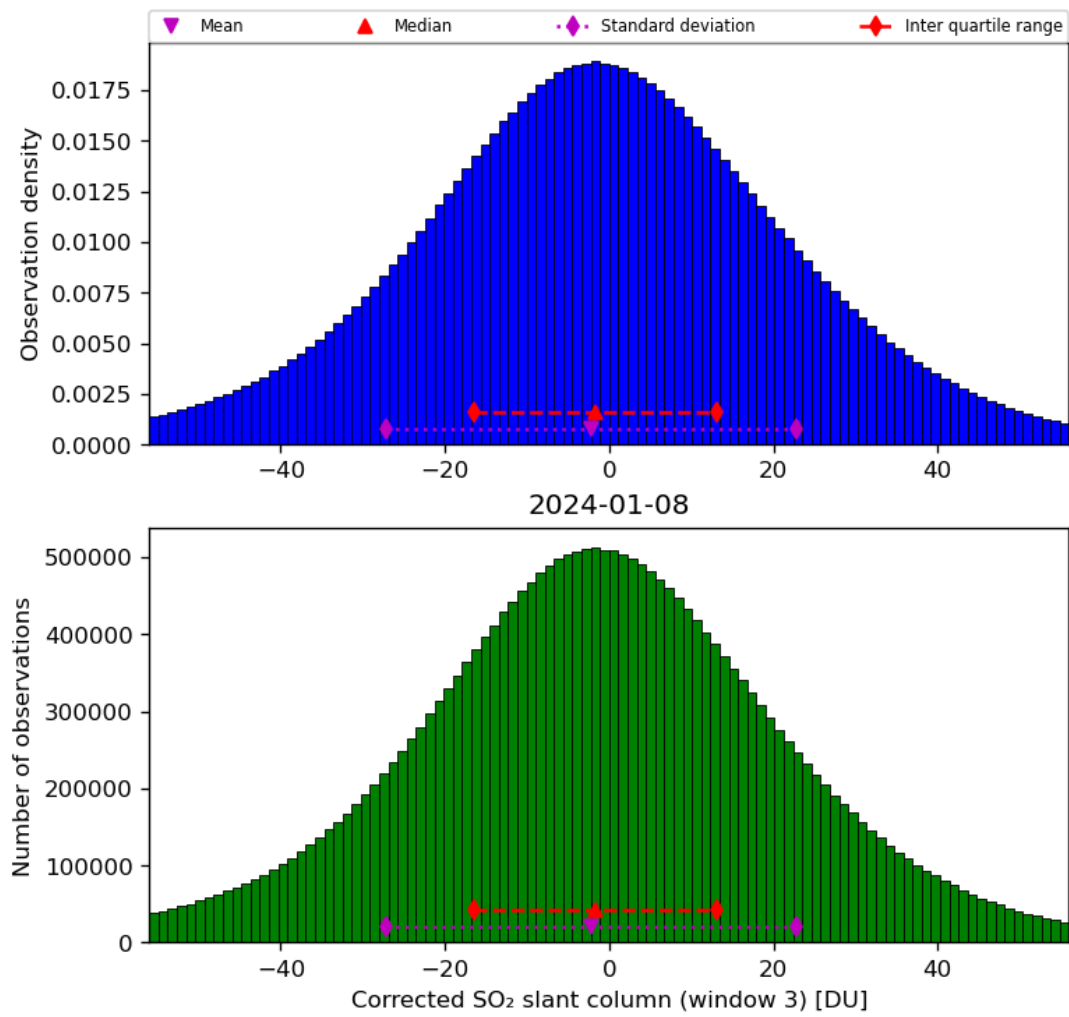
Figure 66: Histogram of “Corrected SO 2 slant column (window 3)” for 2024-01-07 to 2024-01-09
