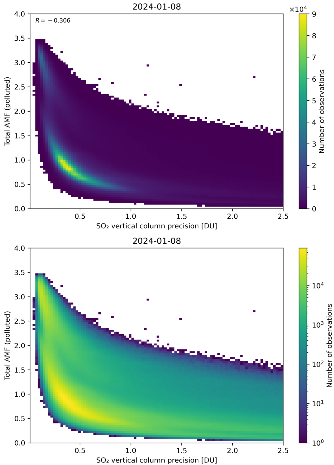
Figure 294: Scatter density plot of “SO 2 vertical column precision” against “Total AMF (polluted)” for 2024-01-07 to 2024-01-09.
