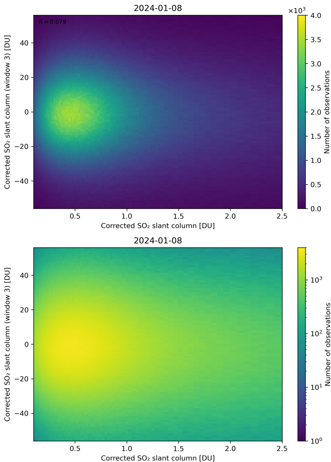
Figure 186: Scatter density plot of “Corrected SO 2 slant column” against “Corrected SO 2 slant column (window 3)” for 2024-01-07 to 2024-01-09.
