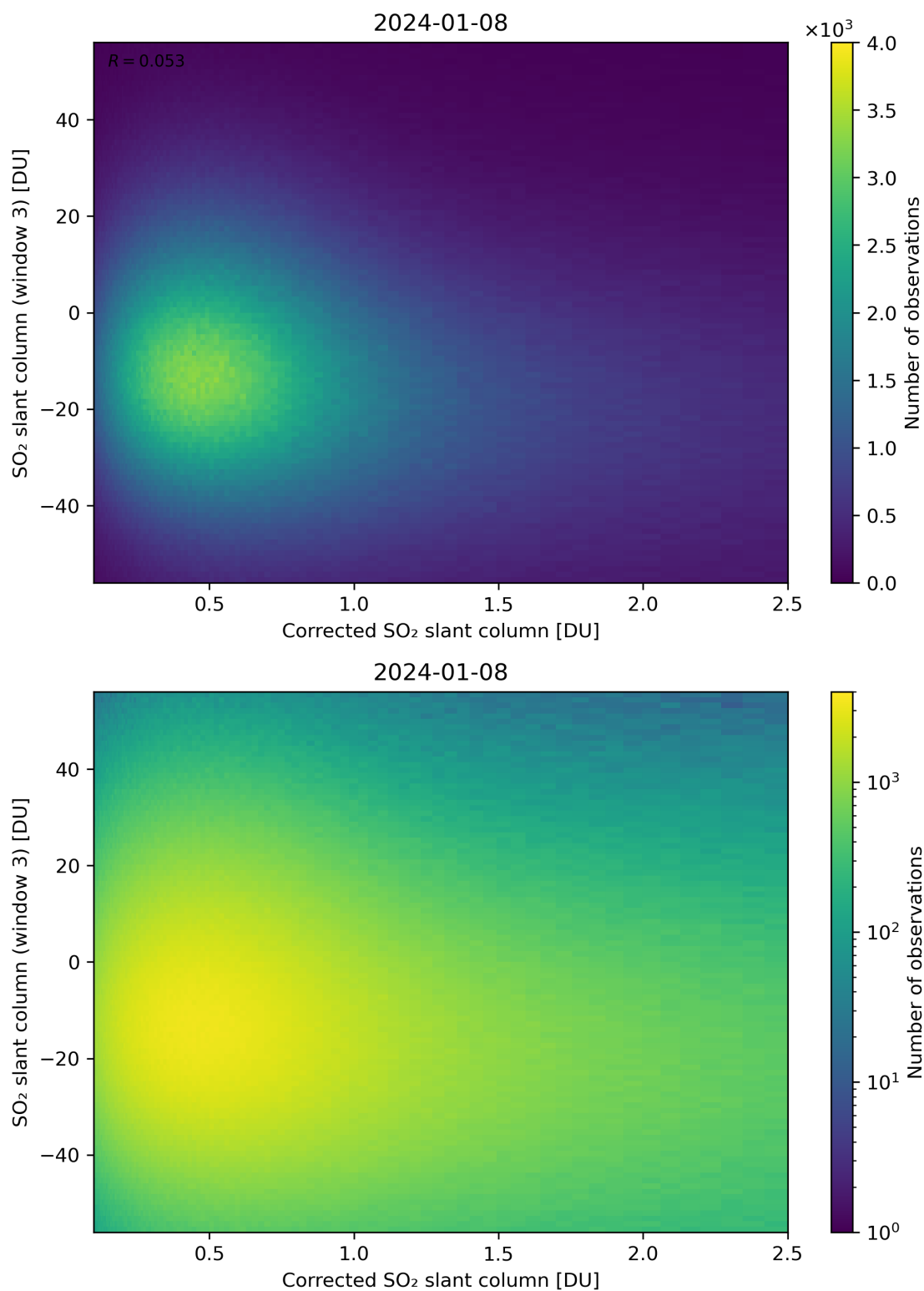
Figure 190: Scatter density plot of “Corrected SO 2 slant column” against “SO 2 slant column (window 3)” for 2024-01-07 to 2024-01-09.
