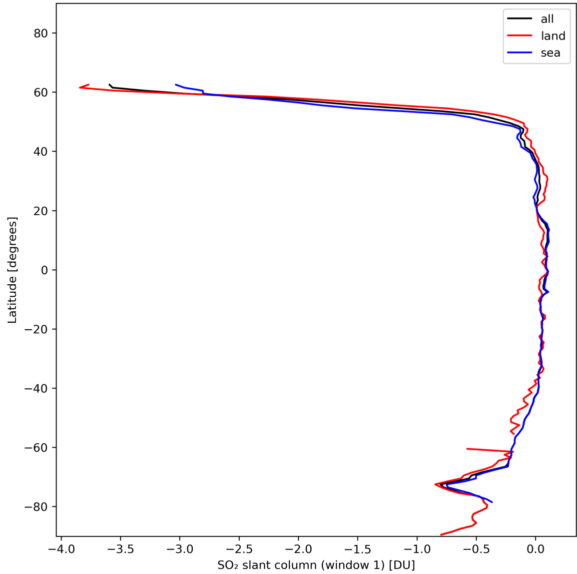
Figure 33: Zonal average of “SO 2 slant column (window 1)” for 2024-01-07 to 2024-01-09.
