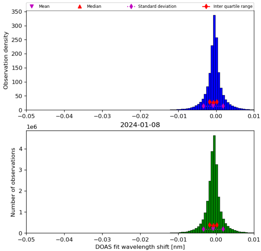
Figure 68: Histogram of “DOAS fit wavelength shift” for 2024-01-07 to 2024-01-09
