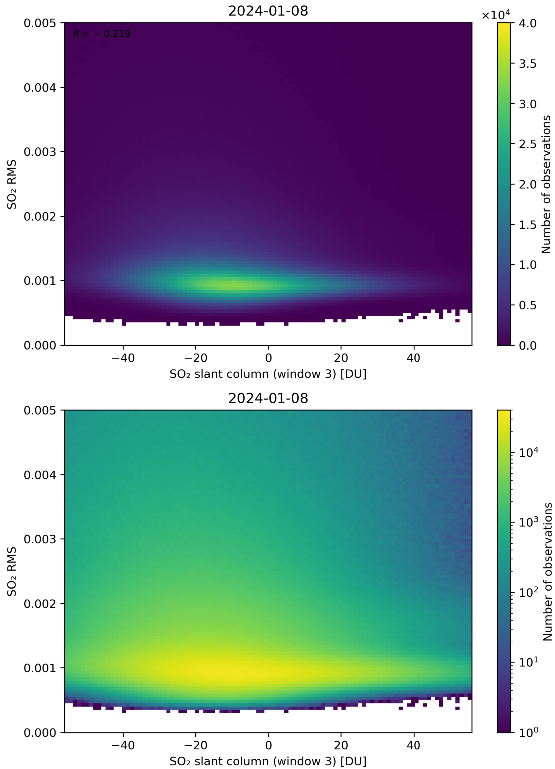
Figure 256: Scatter density plot of “SO 2 slant column (window 3)” against “SO 2 RMS” for 2024-01-07 to 2024-01-09.
