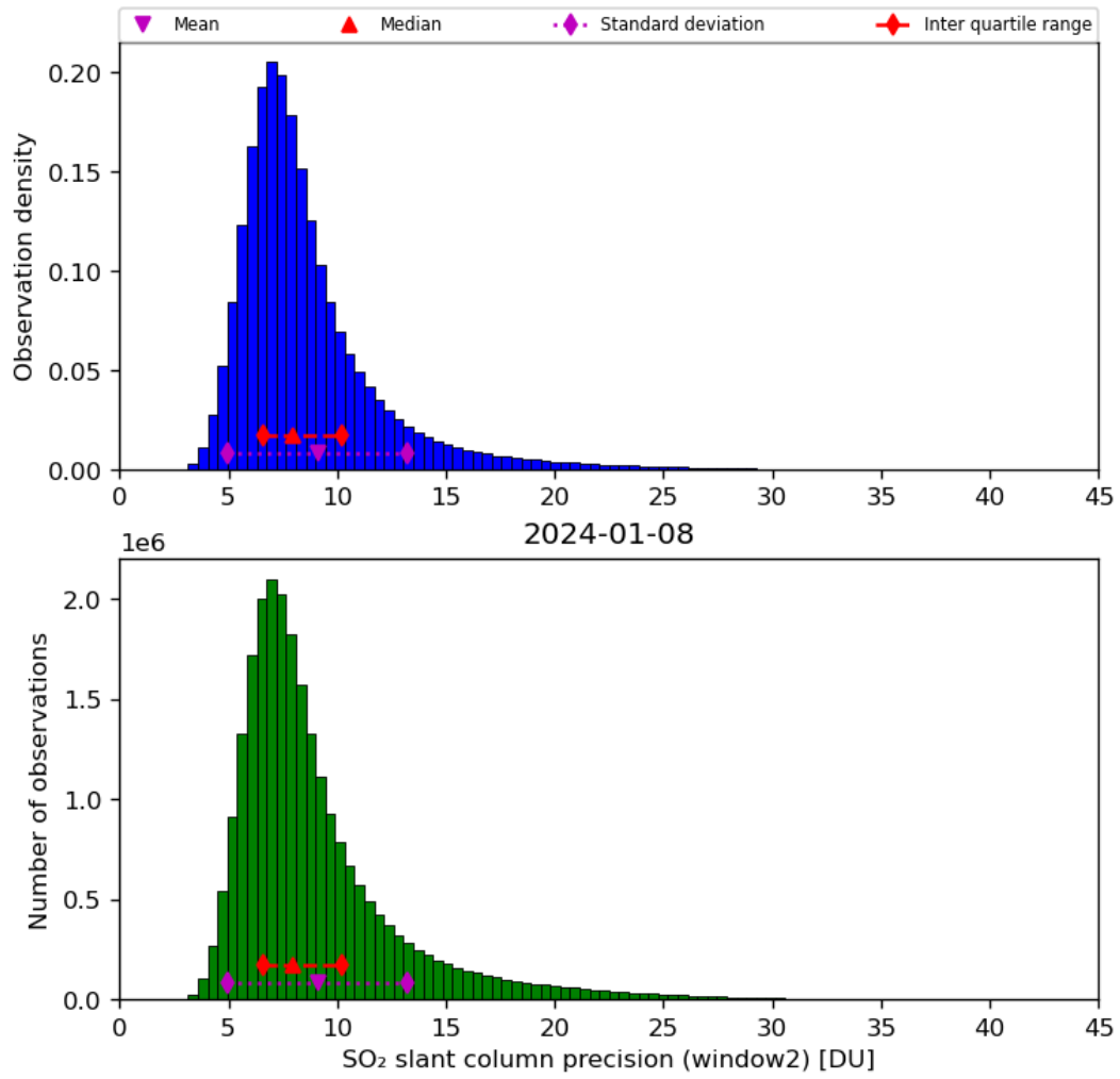
Figure 61: Histogram of “SO 2 slant column precision (window2)” for 2024-01-07 to 2024-01-09
