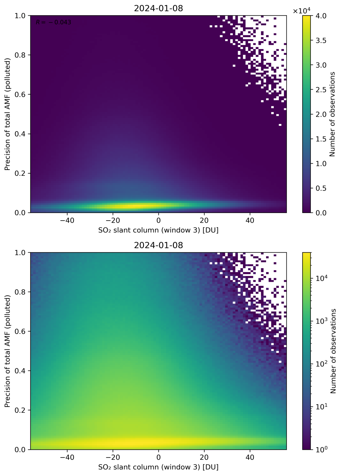
Figure 269: Scatter density plot of “SO 2 slant column (window 3)” against “Precision of total AMF (polluted)” for 2024-01-07 to 2024-01-09.
