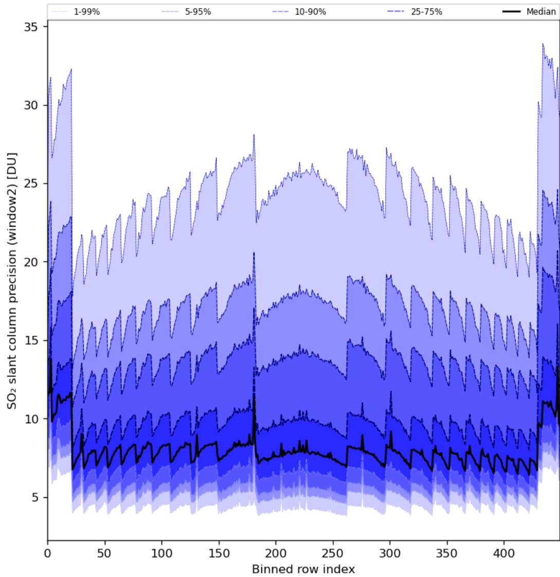
Figure 84: Along track statistics of “SO 2 slant column precision (window2)” for 2024-01-07 to 2024-01-09
