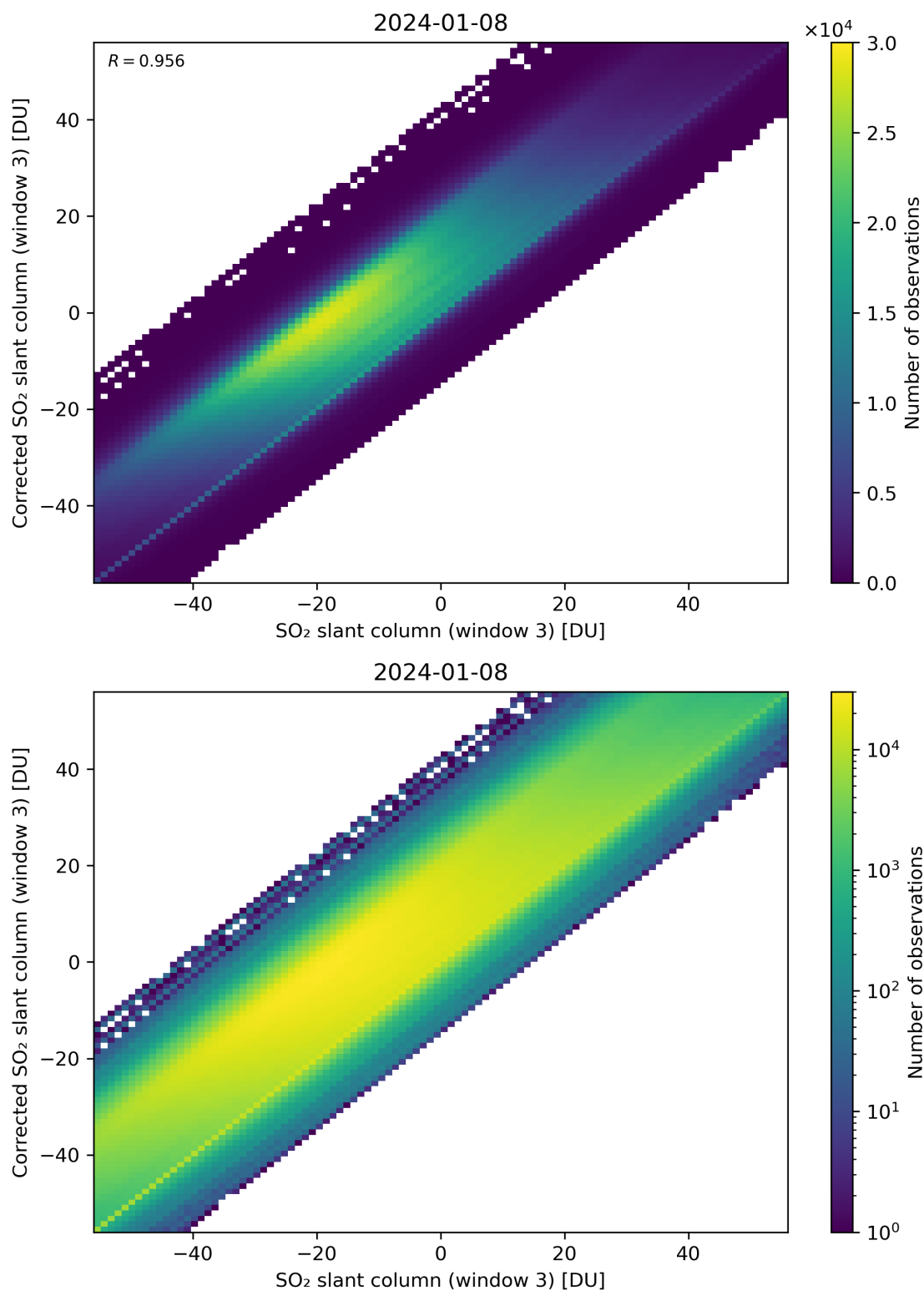
Figure 266: Scatter density plot of “SO 2 slant column (window 3)” against “Corrected SO 2 slant column (window 3)” for 2024-01-07 to 2024-01-09.
