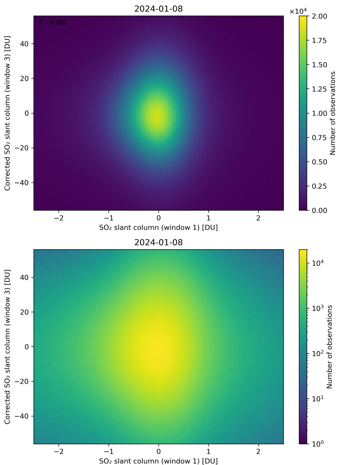
Figure 234: Scatter density plot of “SO 2 slant column (window 1)” against “Corrected SO 2 slant column (window 3)” for 2024-01-07 to 2024-01-09.
