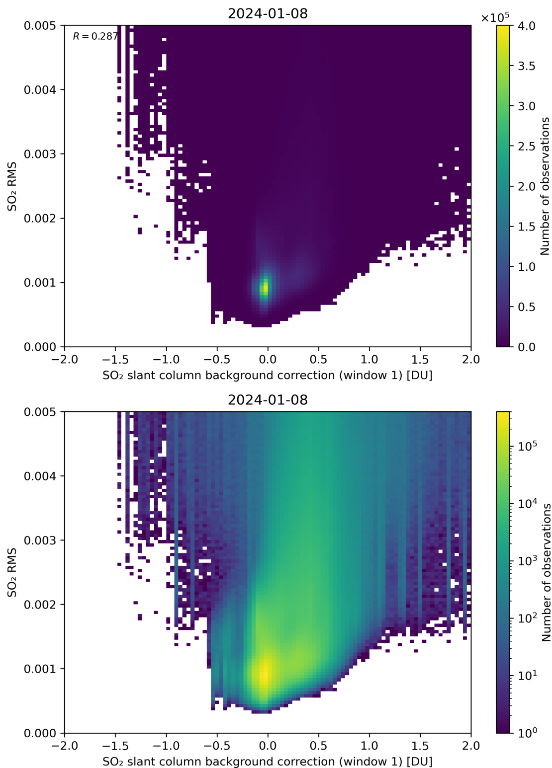
Figure 102: Scatter density plot of “SO 2 slant column background correction (window 1)” against “SO 2 RMS” for 2024-01-07 to 2024-01-09.
