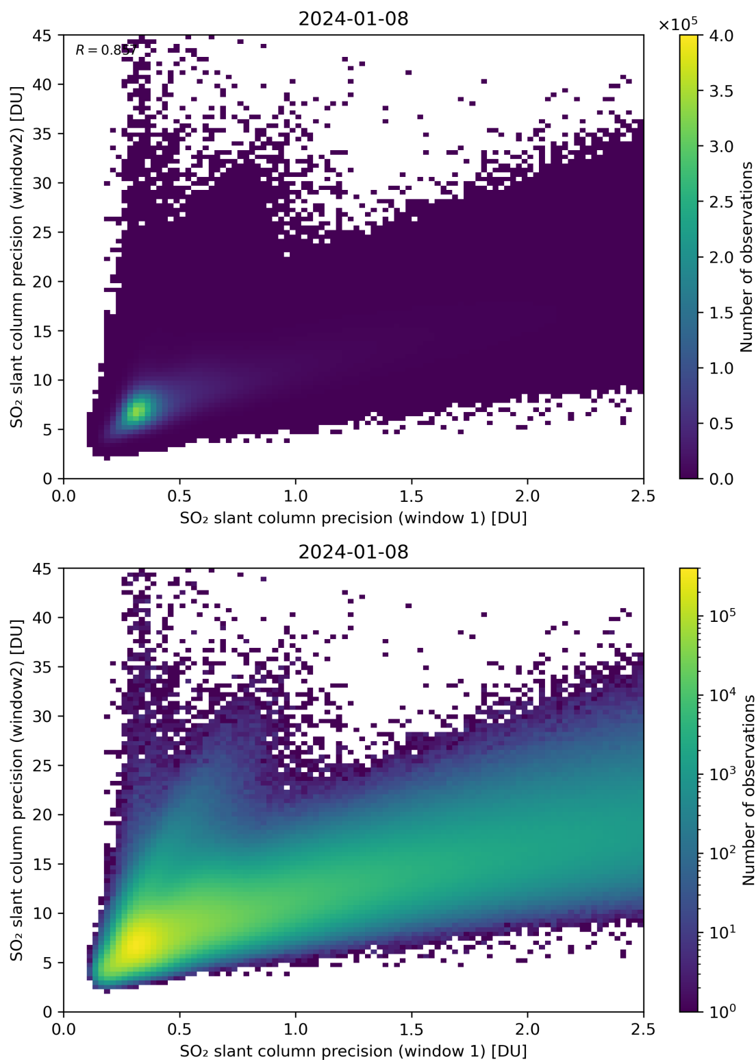
Figure 227: Scatter density plot of “SO 2 slant column precision (window 1)” against “SO 2 slant column precision (window2)” for 2024-01-07 to 2024-01-09.
