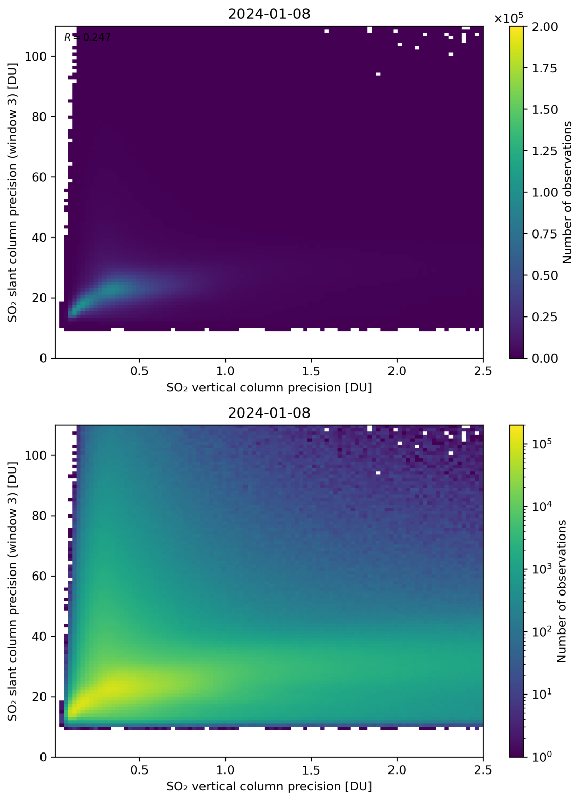
Figure 293: Scatter density plot of “SO 2 vertical column precision” against “SO 2 slant column precision (window 3)” for 2024-01-07 to 2024-01-09.
