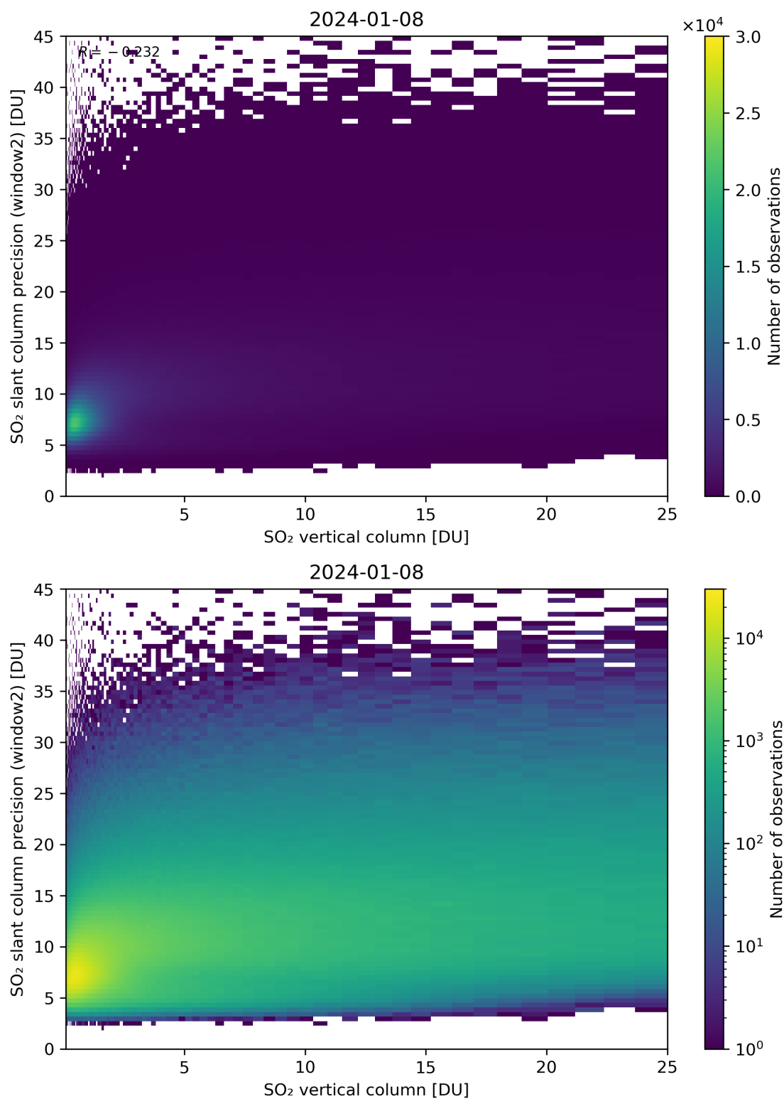
Figure 302: Scatter density plot of “SO 2 vertical column” against “SO 2 slant column precision (window2)” for 2024-01-07 to 2024-01-09.
