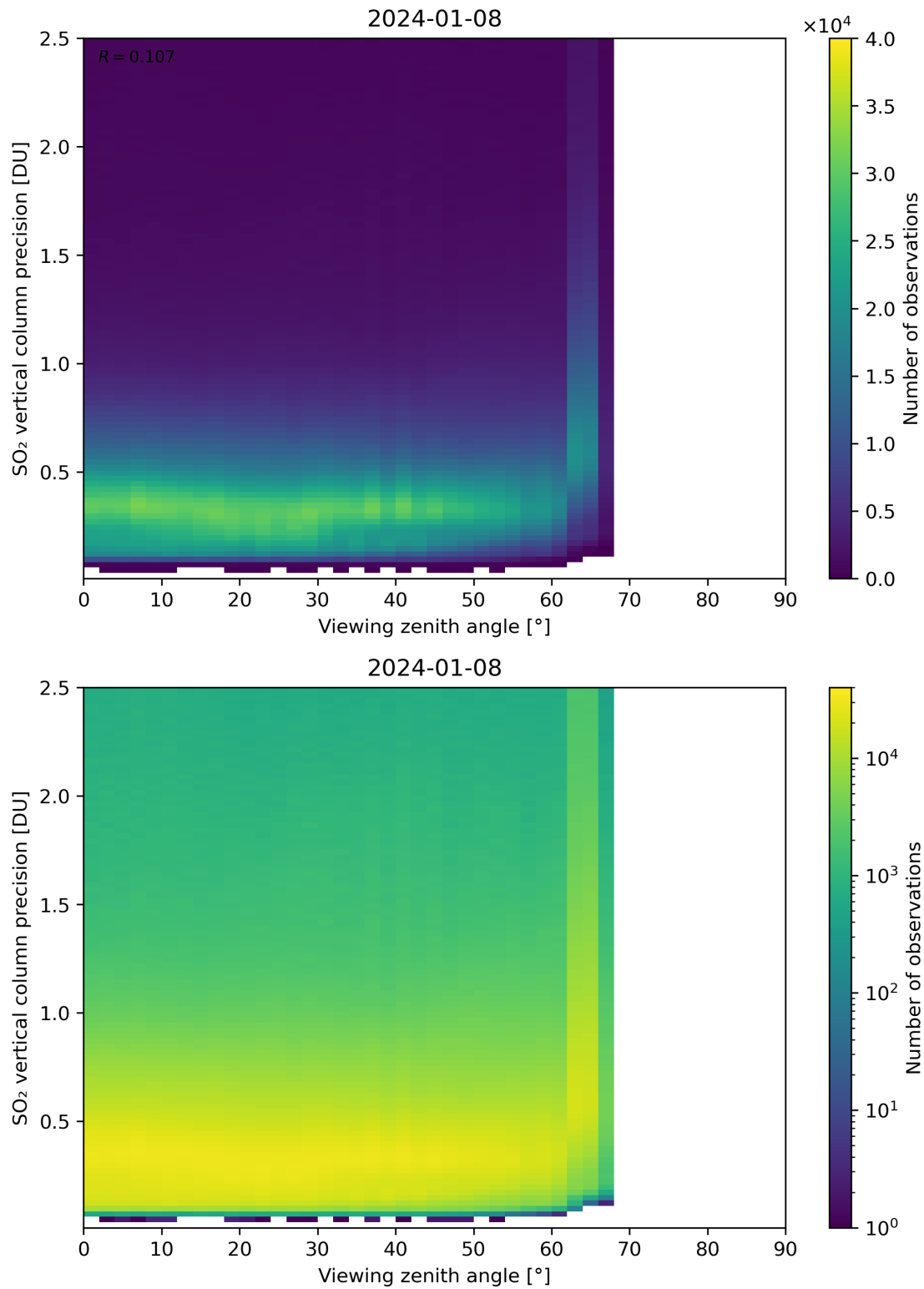
Figure 328: Scatter density plot of “Viewing zenith angle” against “SO 2 vertical column precision” for 2024-01-07 to 2024-01-09.
