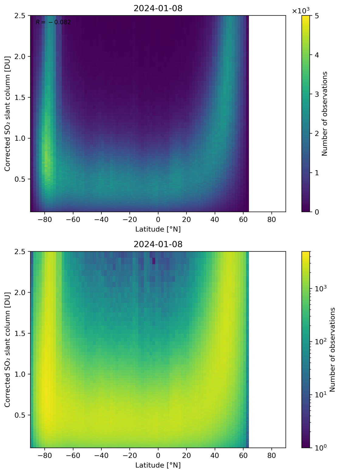
Figure 146: Scatter density plot of “Latitude” against “Corrected SO 2 slant column” for 2024-01-07 to 2024-01-09.
