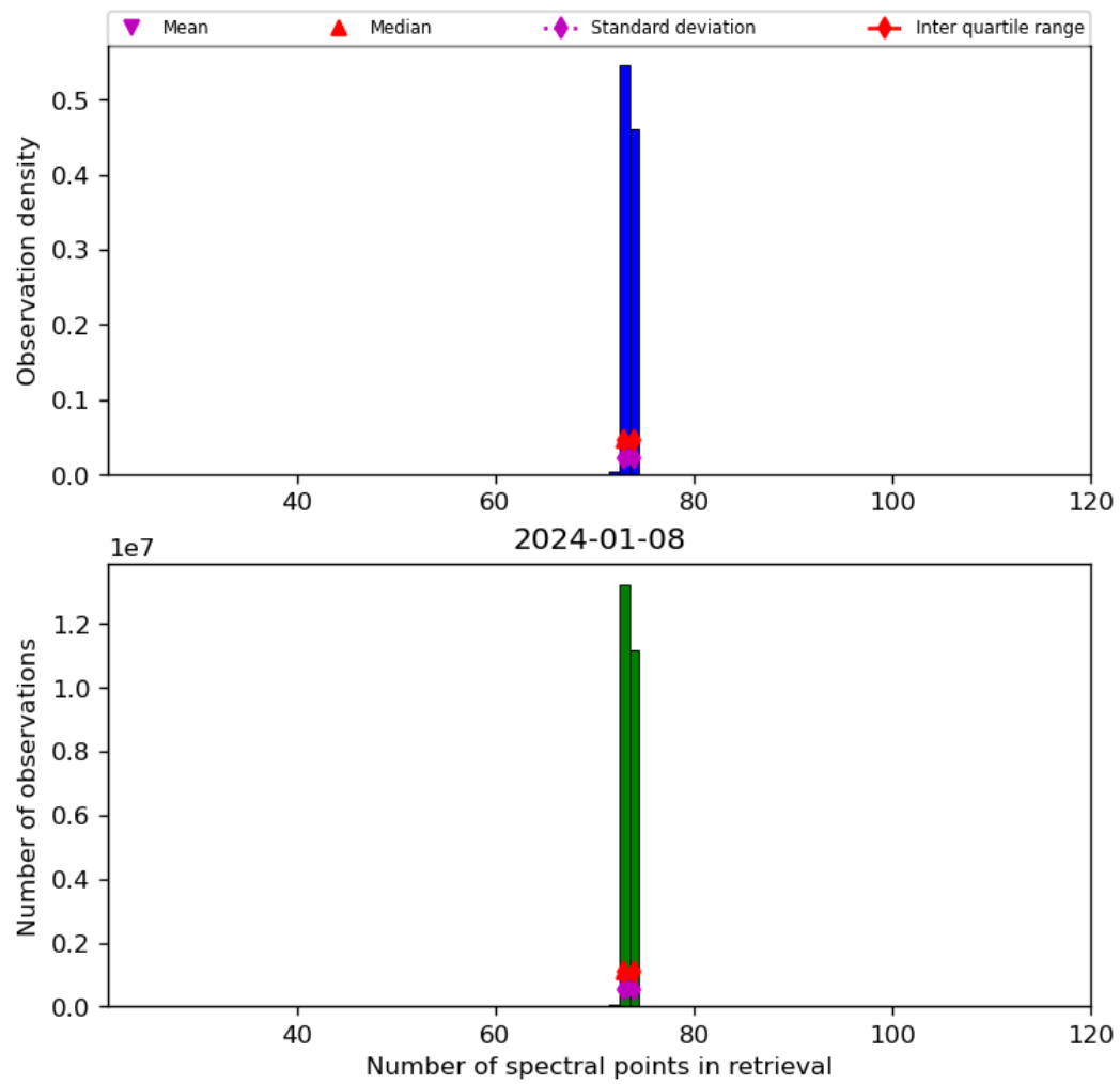
Figure 74: Histogram of “Number of spectral points in retrieval” for 2024-01-07 to 2024-01-09
