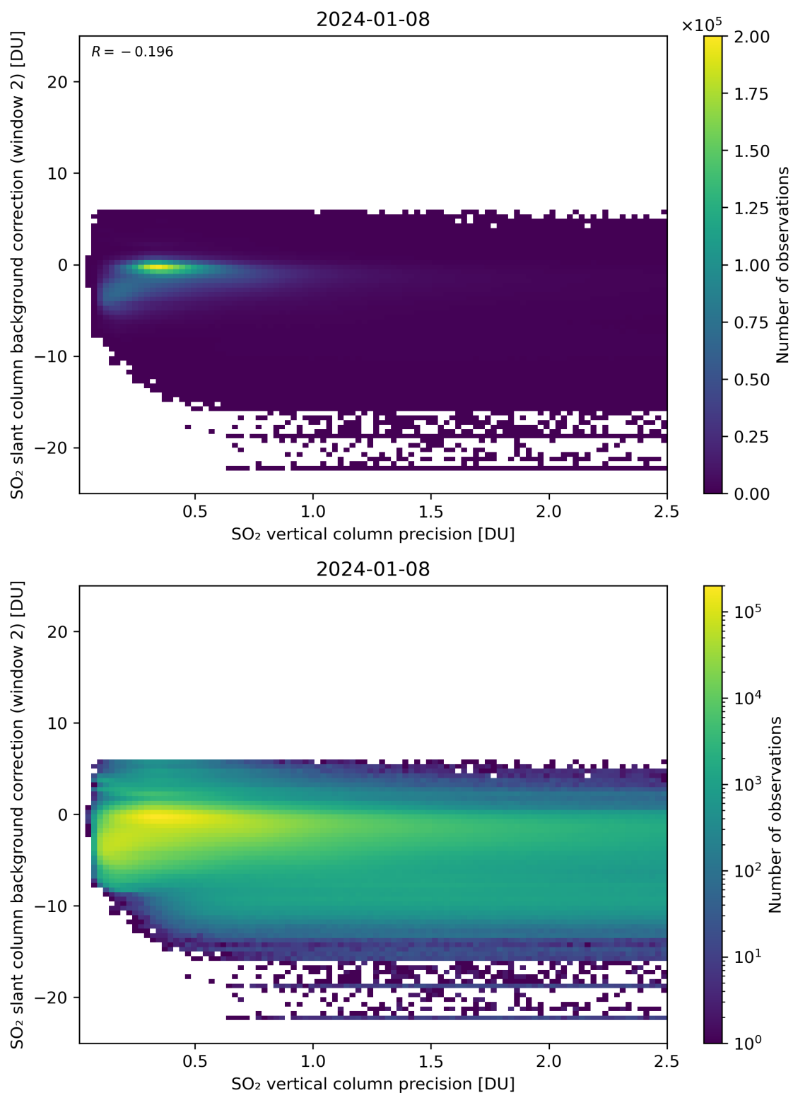
Figure 280: Scatter density plot of “SO 2 vertical column precision” against “SO 2 slant column background correction (window 2)” for 2024-01-07 to 2024-01-09.
