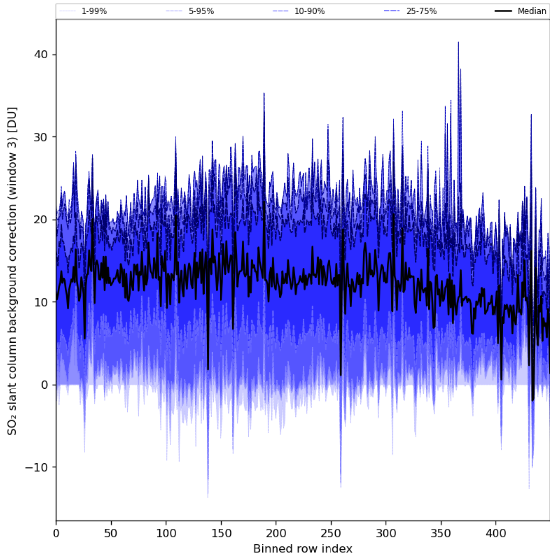
Figure 90: Along track statistics of “SO 2 slant column background correction (window 3)” for 2024-01-07 to 2024-01-09
