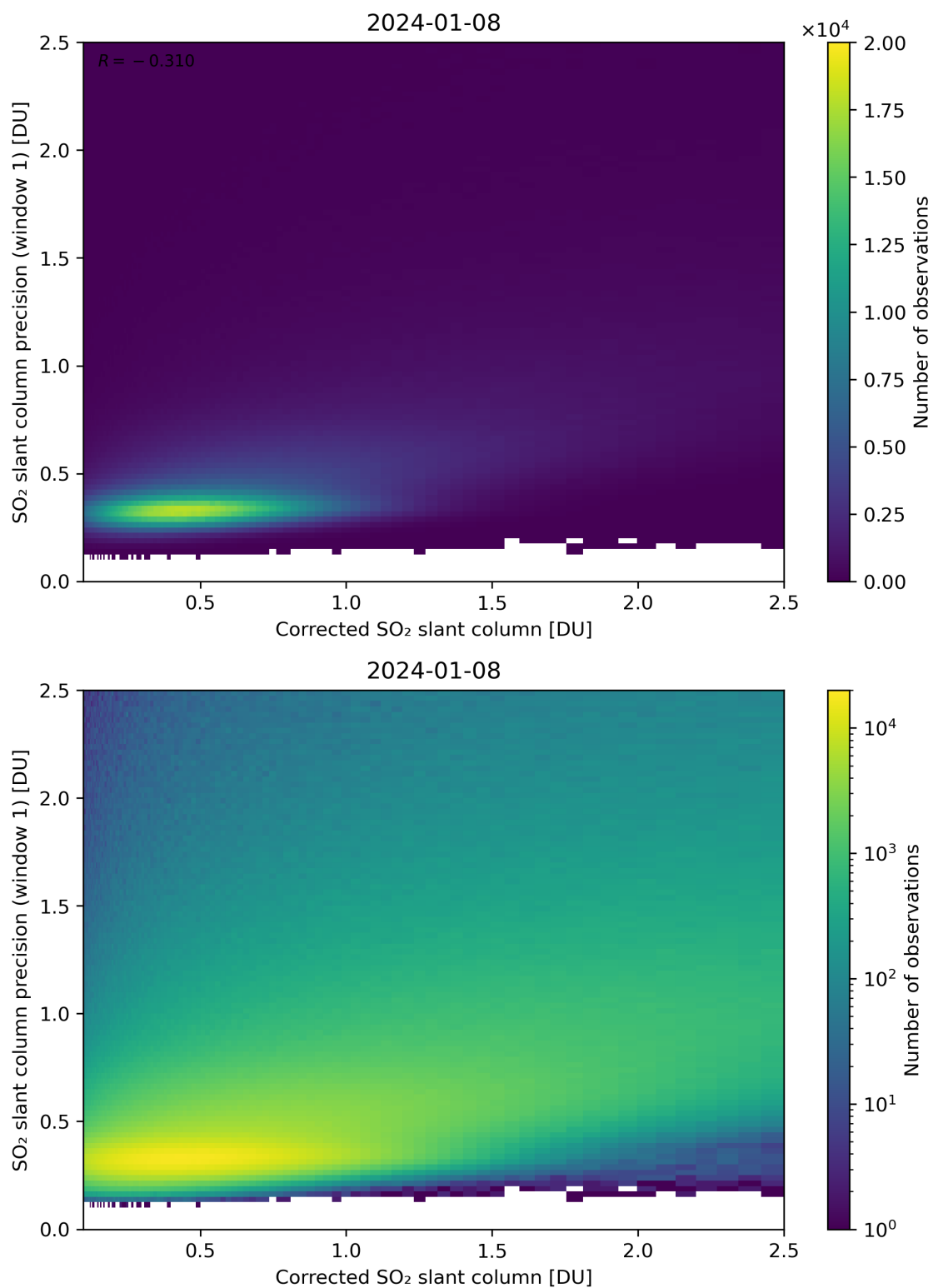
Figure 188: Scatter density plot of “Corrected SO 2 slant column” against “SO 2 slant column precision (window 1)” for 2024-01-07 to 2024-01-09.
