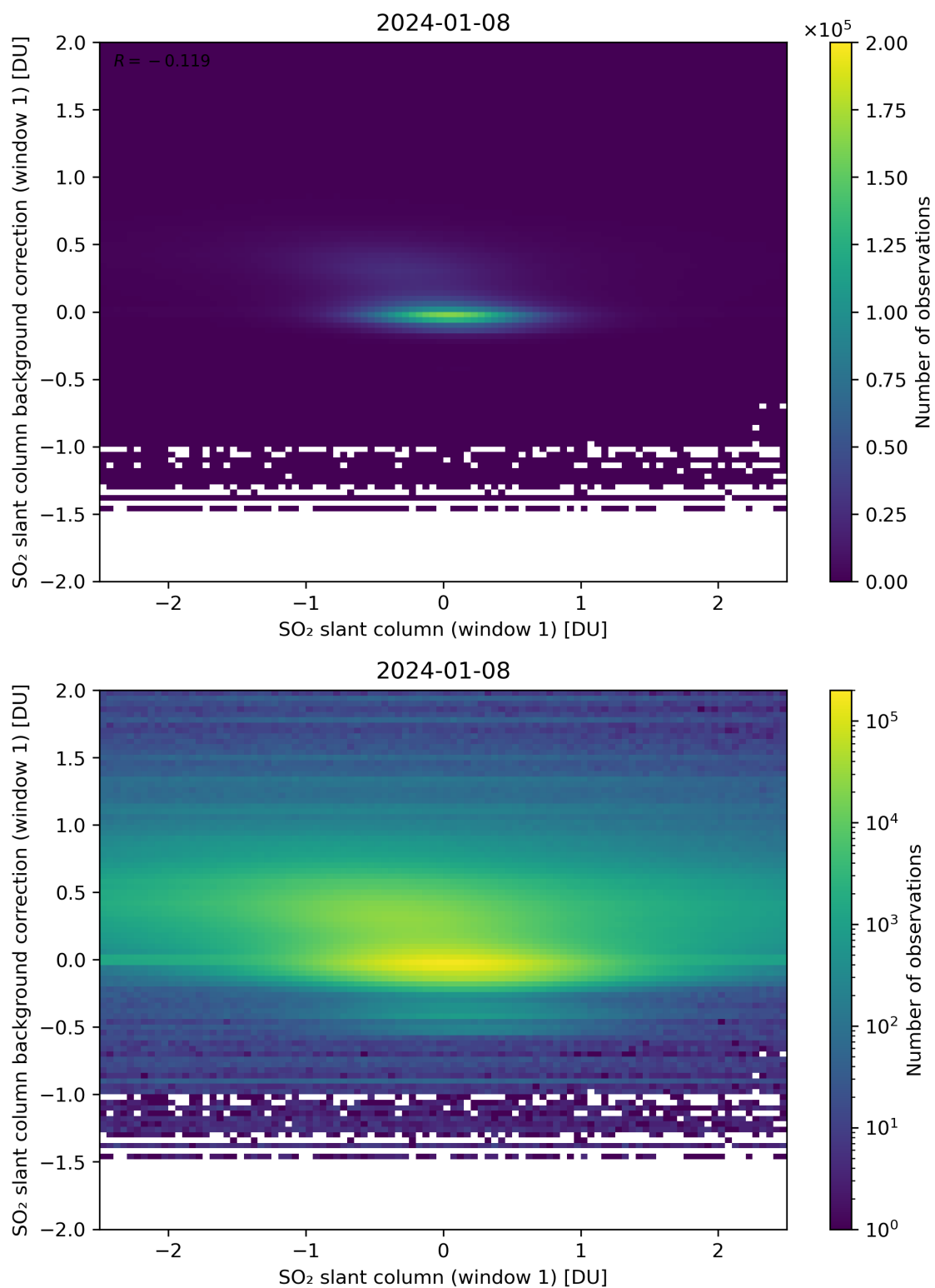
Figure 212: Scatter density plot of “SO 2 slant column (window 1)” against “SO 2 slant column background correction (window 1)” for 2024-01-07 to 2024-01-09.
