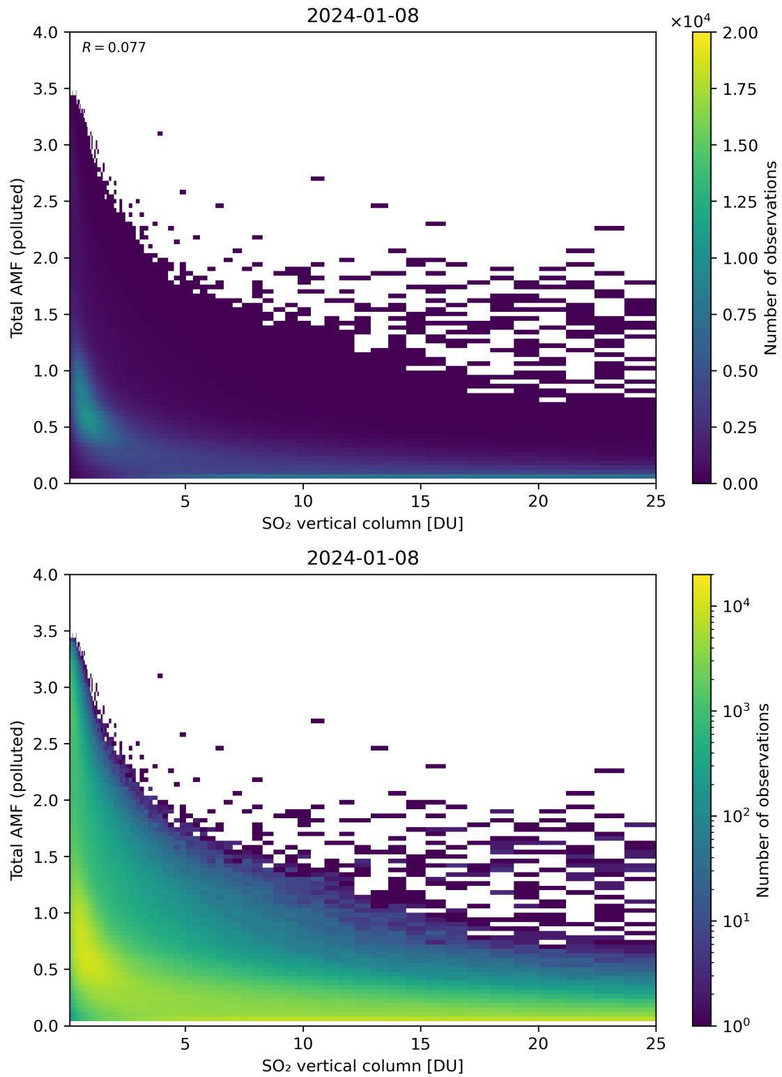
Figure 305: Scatter density plot of “SO 2 vertical column” against “Total AMF (polluted)” for 2024-01-07 to 2024-01-09.
