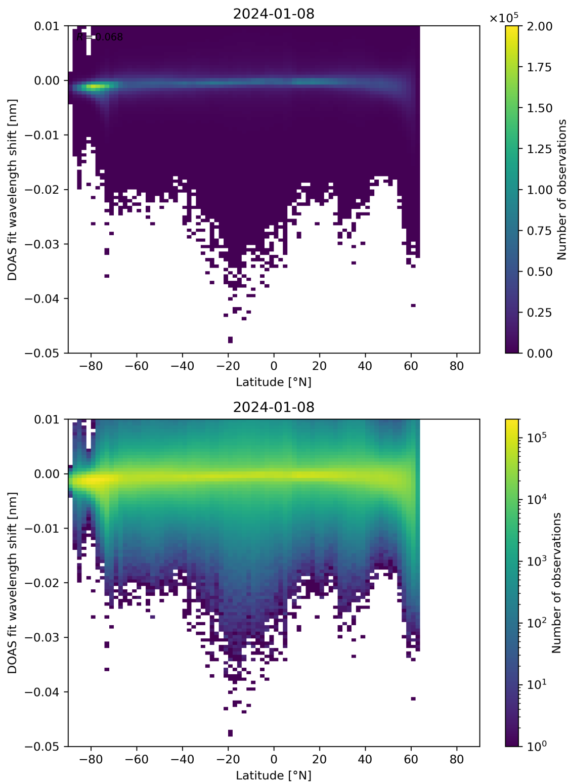
Figure 142: Scatter density plot of “Latitude” against “DOAS fit wavelength shift” for 2024-01-07 to 2024-01-09.
