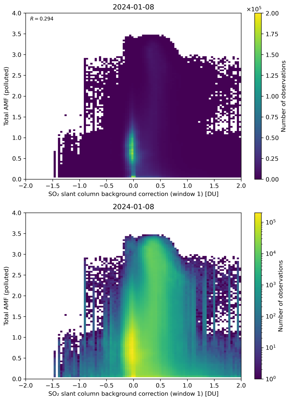
Figure 109: Scatter density plot of “SO 2 slant column background correction (window 1)” against “Total AMF (polluted)” for 2024-01-07 to 2024-01-09.
