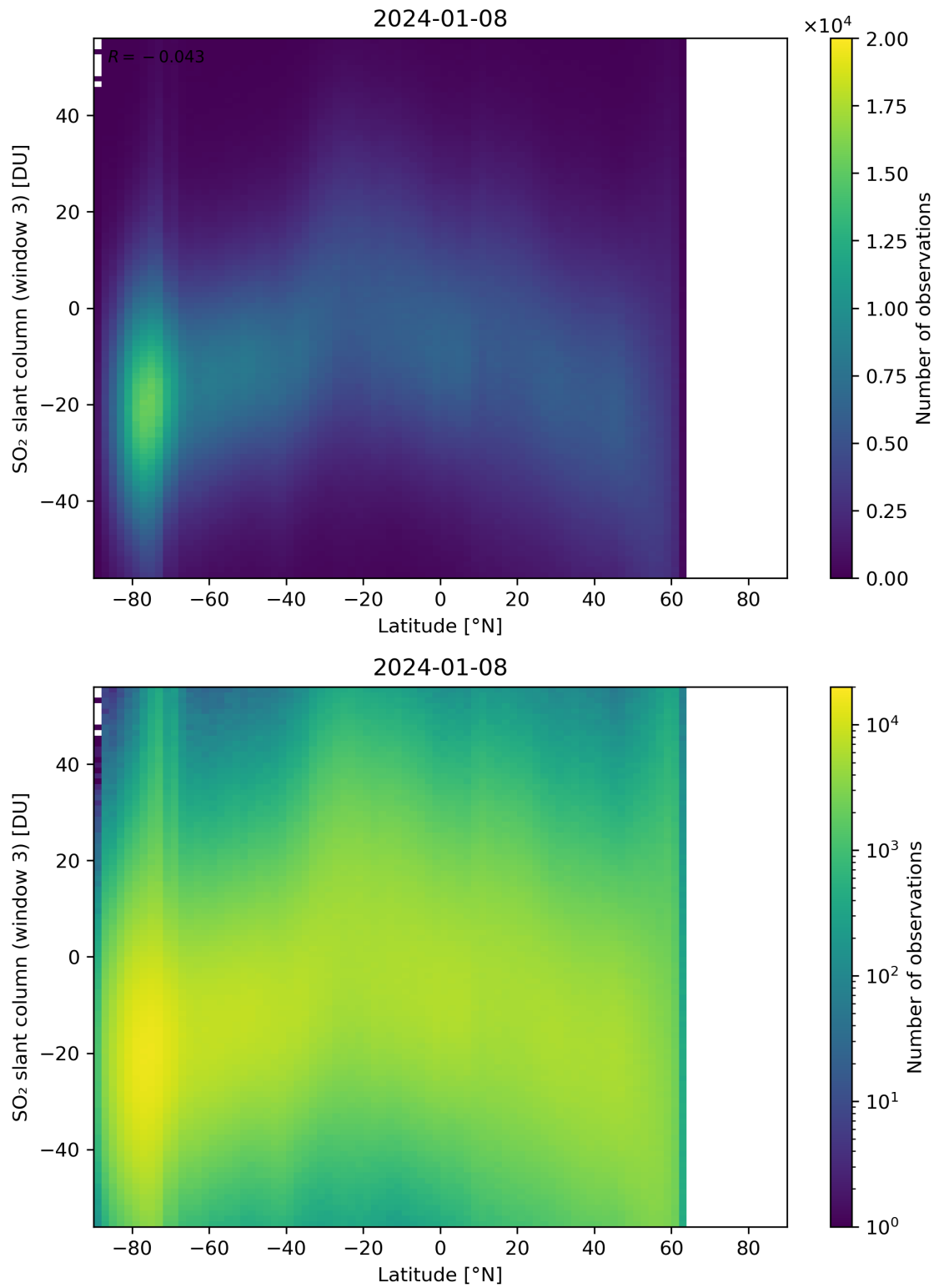
Figure 152: Scatter density plot of “Latitude” against “SO 2 slant column (window 3)” for 2024-01-07 to 2024-01-09.
