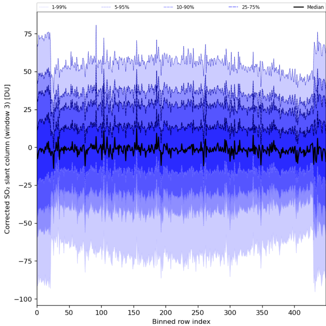
Figure 89: Along track statistics of “Corrected SO 2 slant column (window 3)” for 2024-01-07 to 2024-01-09
