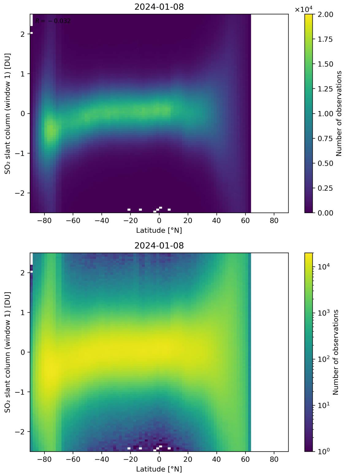
Figure 149: Scatter density plot of “Latitude” against “SO 2 slant column (window 1)” for 2024-01-07 to 2024-01-09.
