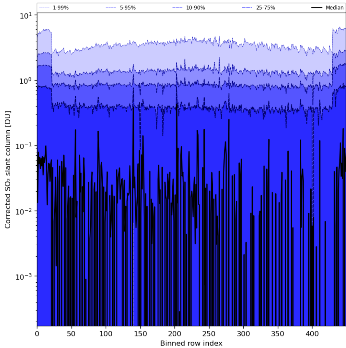
Figure 78: Along track statistics of “Corrected SO 2 slant column” for 2024-01-07 to 2024-01-09
