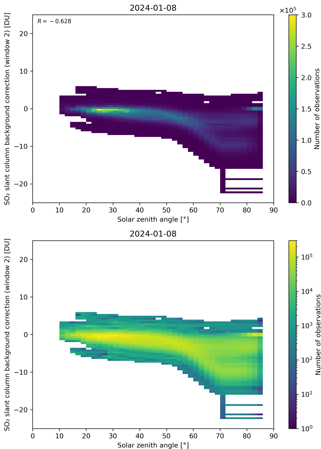
Figure 159: Scatter density plot of “Solar zenith angle” against “SO 2 slant column background correction (window 2)” for 2024-01-07 to 2024-01-09.
