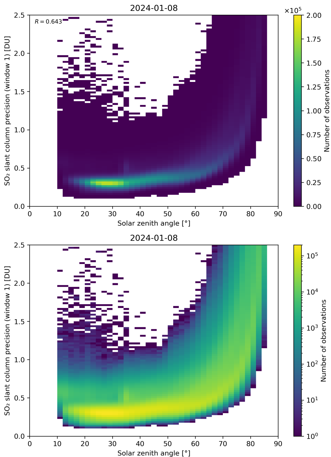
Figure 170: Scatter density plot of “Solar zenith angle” against “SO 2 slant column precision (window 1)” for 2024-01-07 to 2024-01-09.
