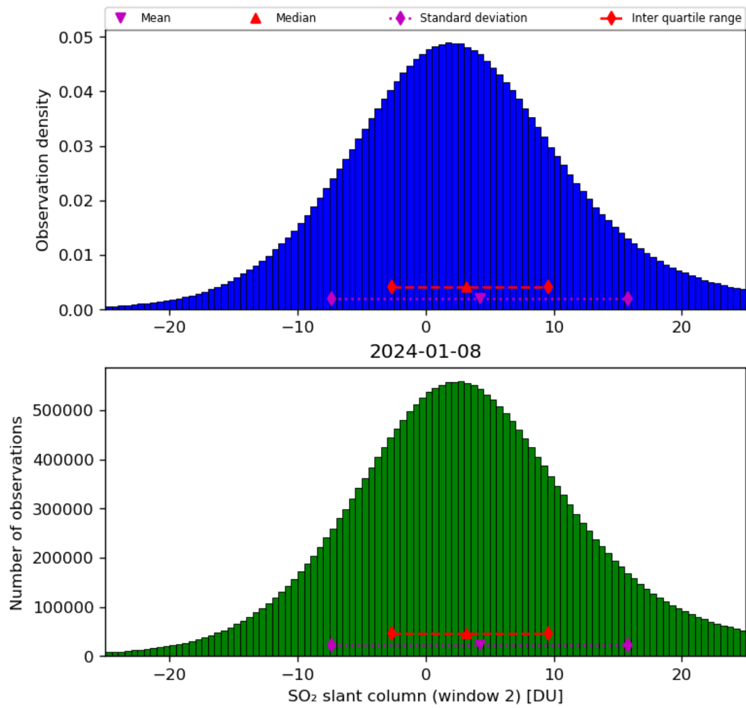
Figure 60: Histogram of “SO 2 slant column (window 2)” for 2024-01-07 to 2024-01-09
