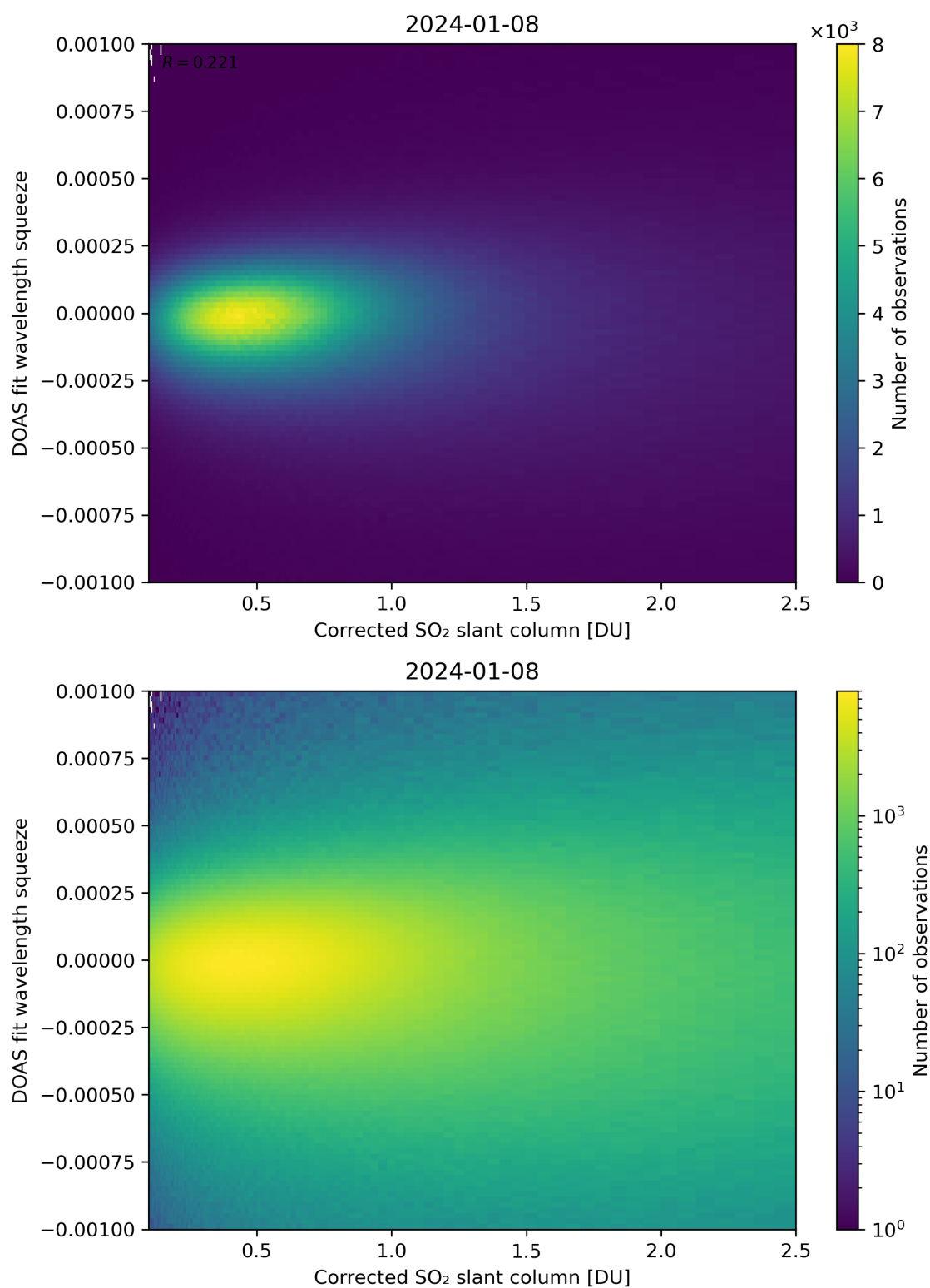
Figure 182: Scatter density plot of “Corrected SO 2 slant column” against “DOAS fit wavelength squeeze” for 2024-01-07 to 2024-01-09.
