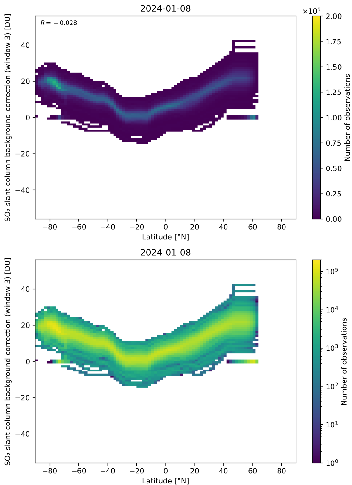
Figure 141: Scatter density plot of “Latitude” against “SO 2 slant column background correction (window 3)” for 2024-01-07 to 2024-01-09.
