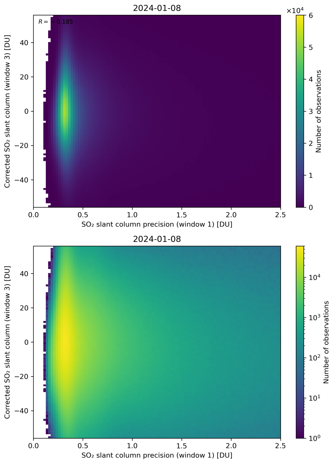
Figure 226: Scatter density plot of “SO 2 slant column precision (window 1)” against “Corrected SO 2 slant column (window 3)” for 2024-01-07 to 2024-01-09.
