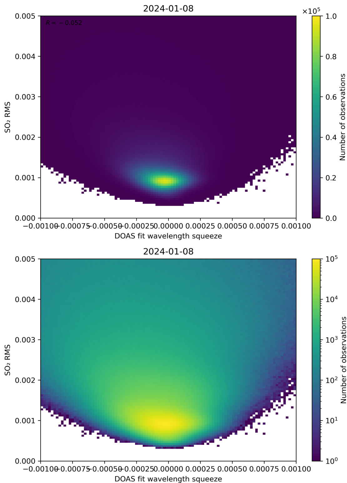
Figure 132: Scatter density plot of “DOAS fit wavelength squeeze” against “SO 2 RMS” for 2024-01-07 to 2024-01-09.
