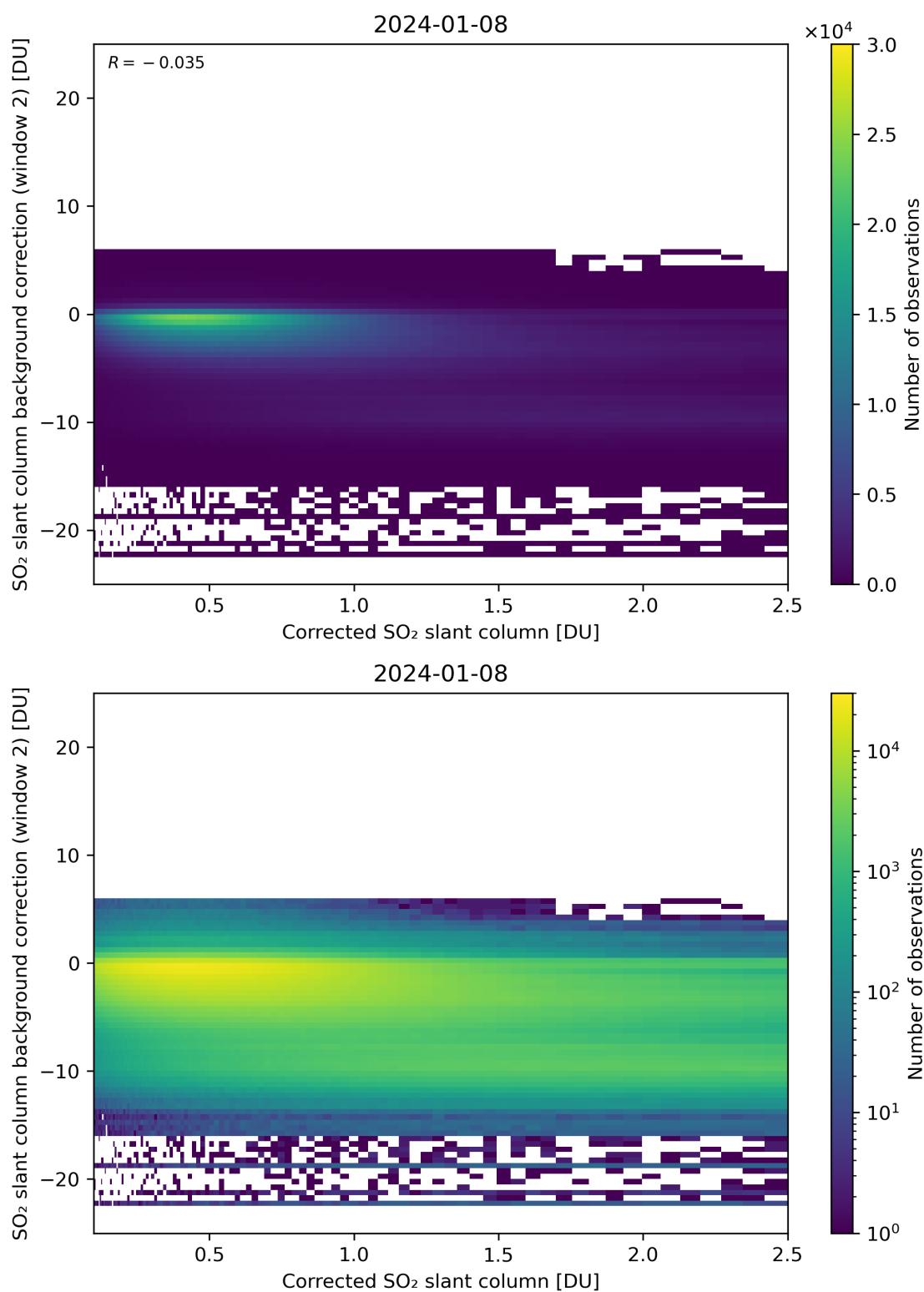
Figure 179: Scatter density plot of “Corrected SO 2 slant column” against “SO 2 slant column background correction (window 2)” for 2024-01-07 to 2024-01-09.
