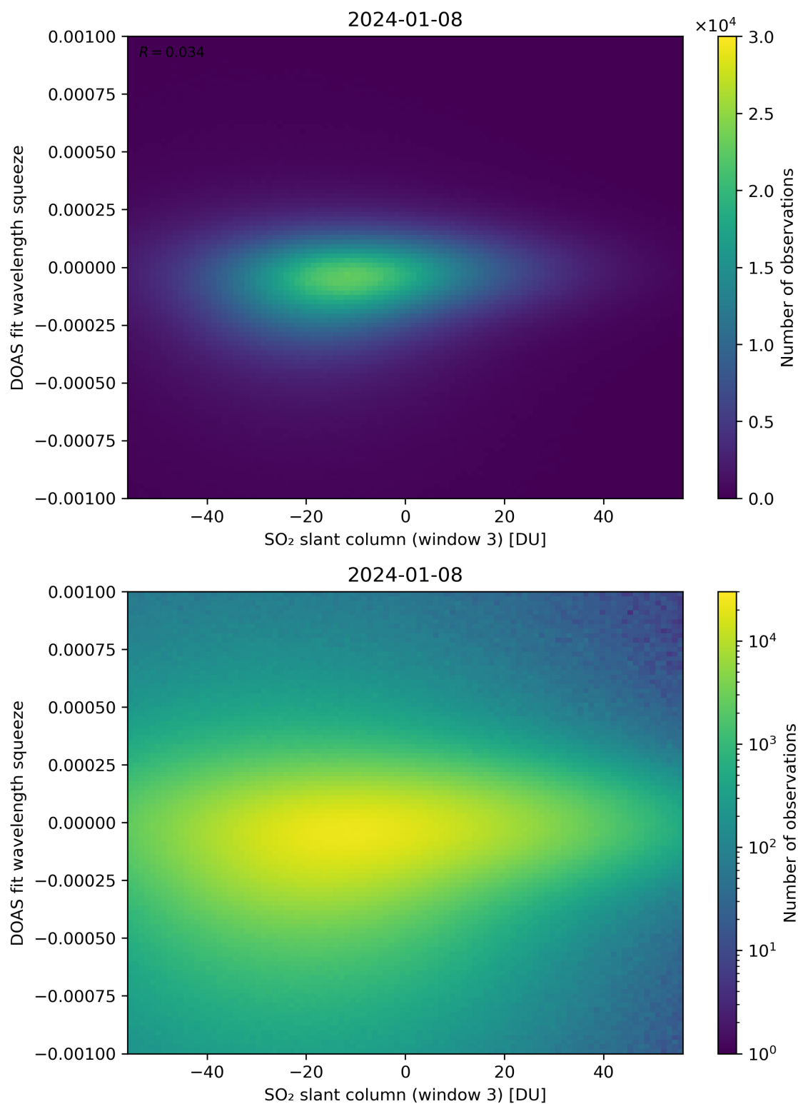
Figure 255: Scatter density plot of “SO 2 slant column (window 3)” against “DOAS fit wavelength squeeze” for 2024-01-07 to 2024-01-09.
