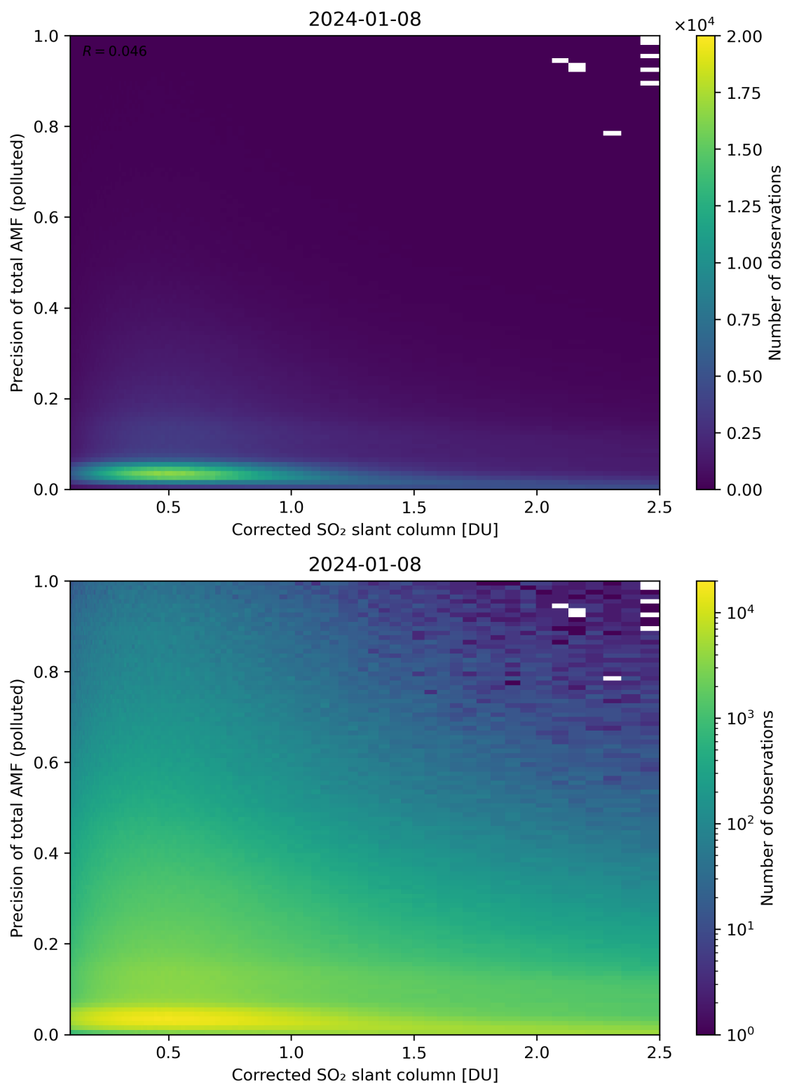
Figure 193: Scatter density plot of “Corrected SO 2 slant column” against “Precision of total AMF (polluted)” for 2024-01-07 to 2024-01-09.
