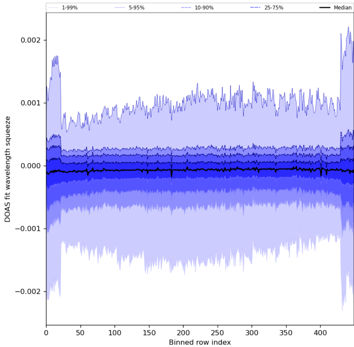
Figure 92: Along track statistics of “DOAS fit wavelength squeeze” for 2024-01-07 to 2024-01-09
