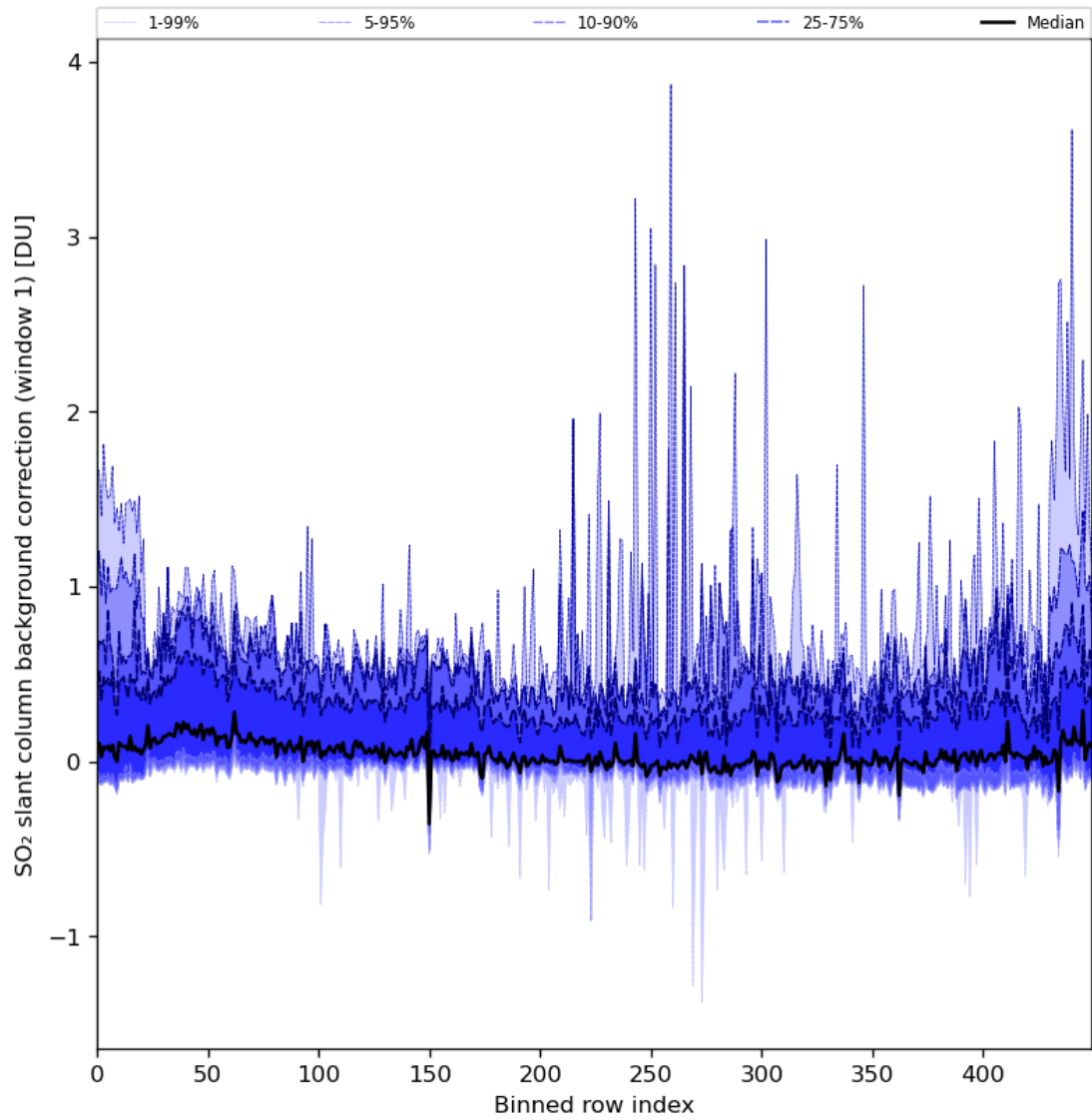
Figure 82: Along track statistics of “SO 2 slant column background correction (window 1)” for 2024-01-07 to 2024-01-09
