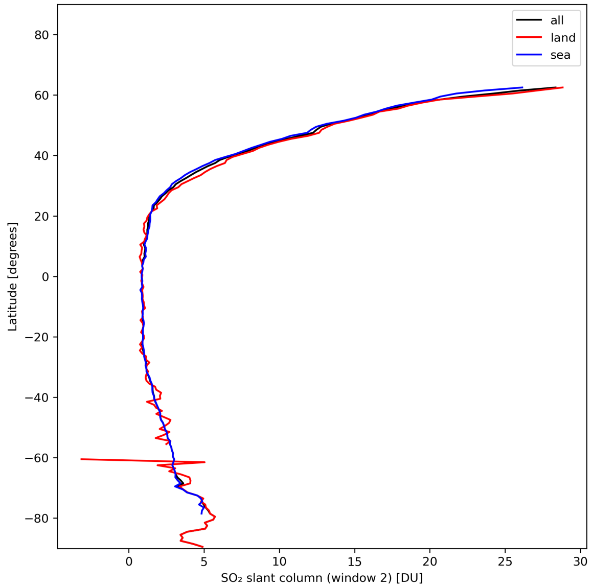
Figure 37: Zonal average of “SO 2 slant column (window 2)” for 2024-01-07 to 2024-01-09.
