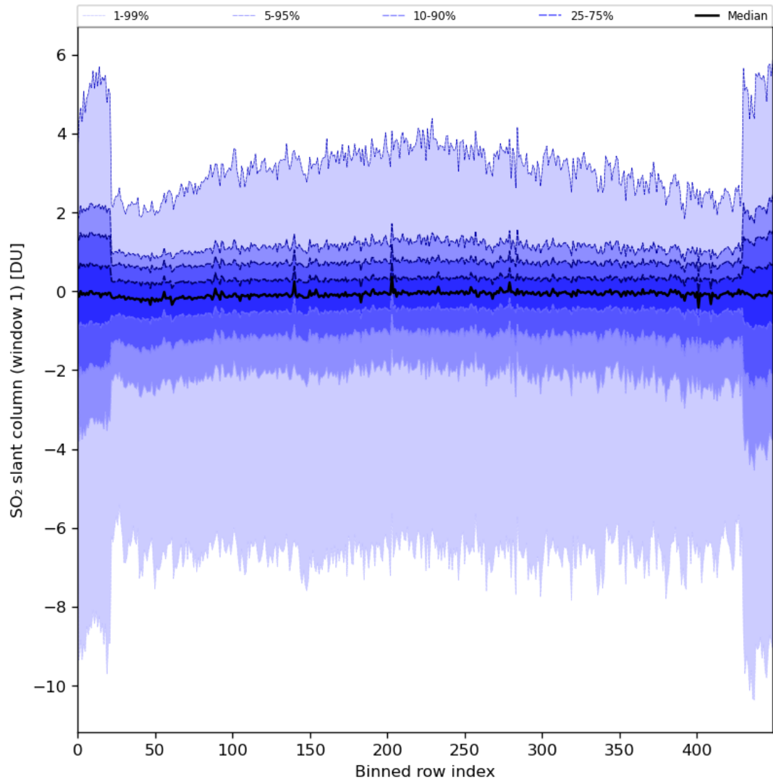
Figure 79: Along track statistics of “SO 2 slant column (window 1)” for 2024-01-07 to 2024-01-09
