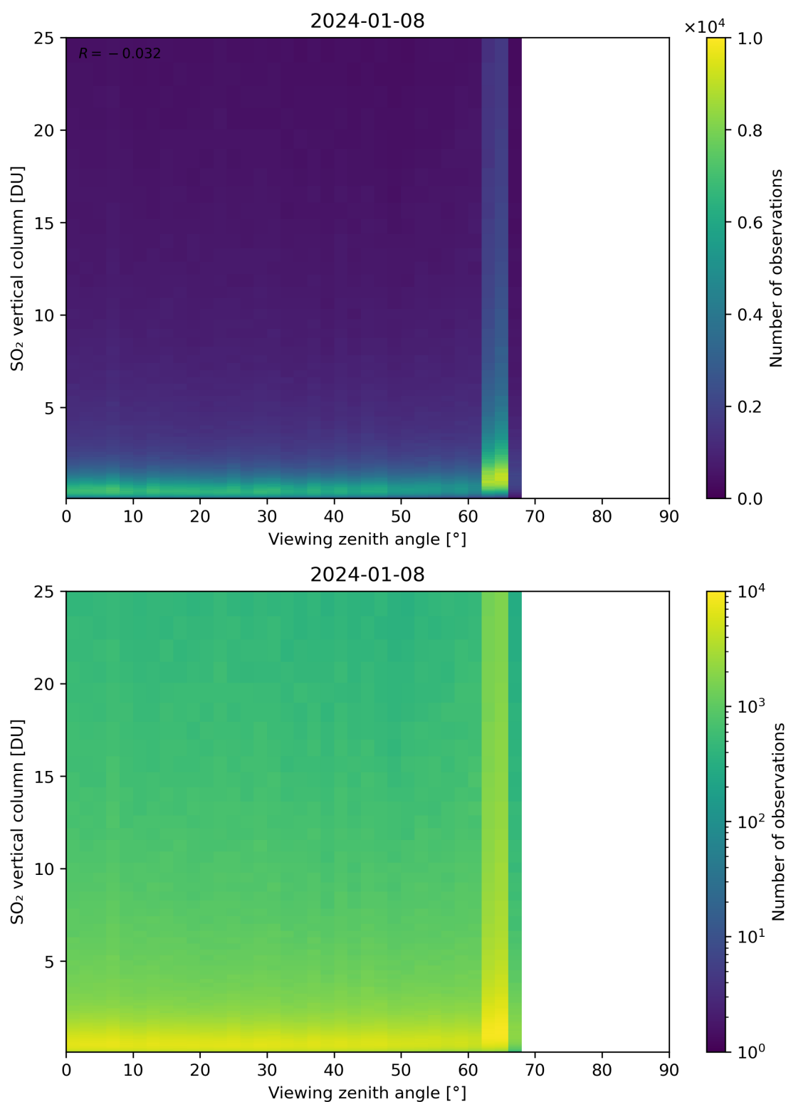
Figure 327: Scatter density plot of “Viewing zenith angle” against “SO 2 vertical column” for 2024-01-07 to 2024-01-09.
