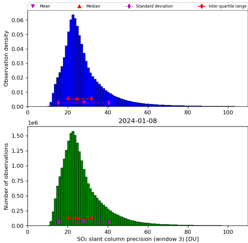
Figure 65: Histogram of “SO 2 slant column precision (window 3)” for 2024-01-07 to 2024-01-09
