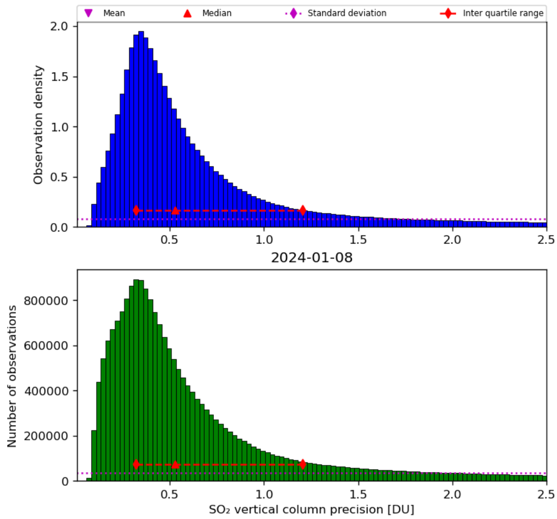
Figure 54: Histogram of “SO 2 vertical column precision” for 2024-01-07 to 2024-01-09
