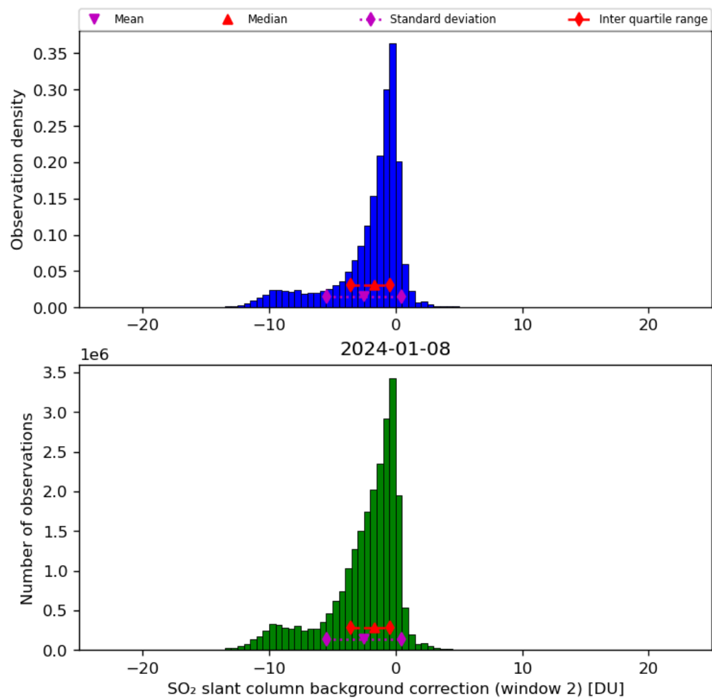
Figure 63: Histogram of “SO 2 slant column background correction (window 2)” for 2024-01-07 to 2024-01-09
