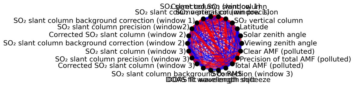
Figure 1: Map of correlation graph for 2024-01-07 to 2024-01-09.
