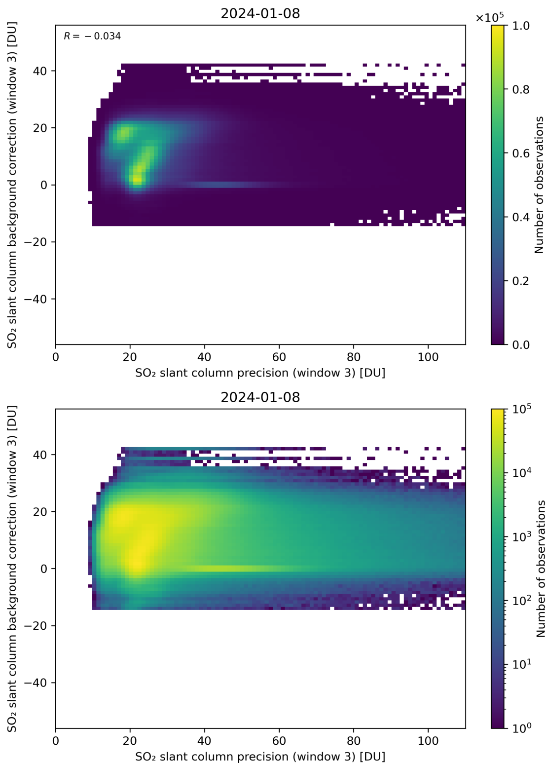
Figure 257: Scatter density plot of “SO 2 slant column precision (window 3)” against “SO 2 slant column background correction (window 3)” for 2024-01-07 to 2024-01-09.
