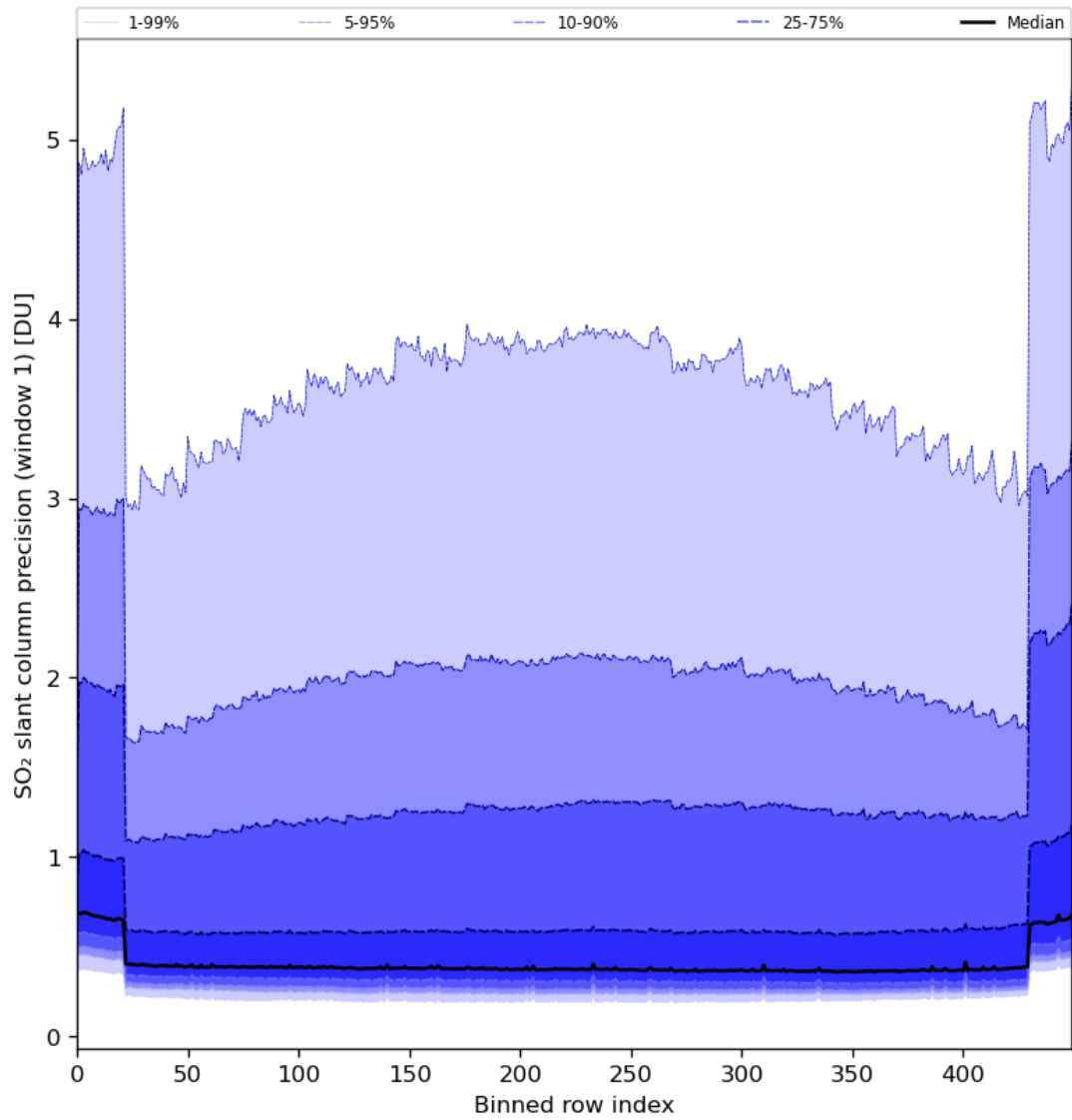
Figure 80: Along track statistics of “SO 2 slant column precision (window 1)” for 2024-01-07 to 2024-01-09
