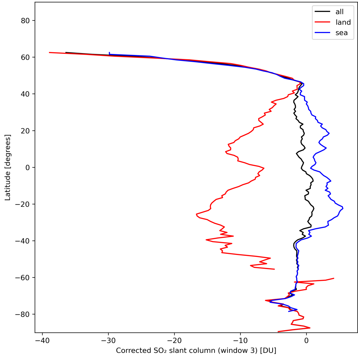
Figure 43: Zonal average of “Corrected SO 2 slant column (window 3)” for 2024-01-07 to 2024-01-09.
