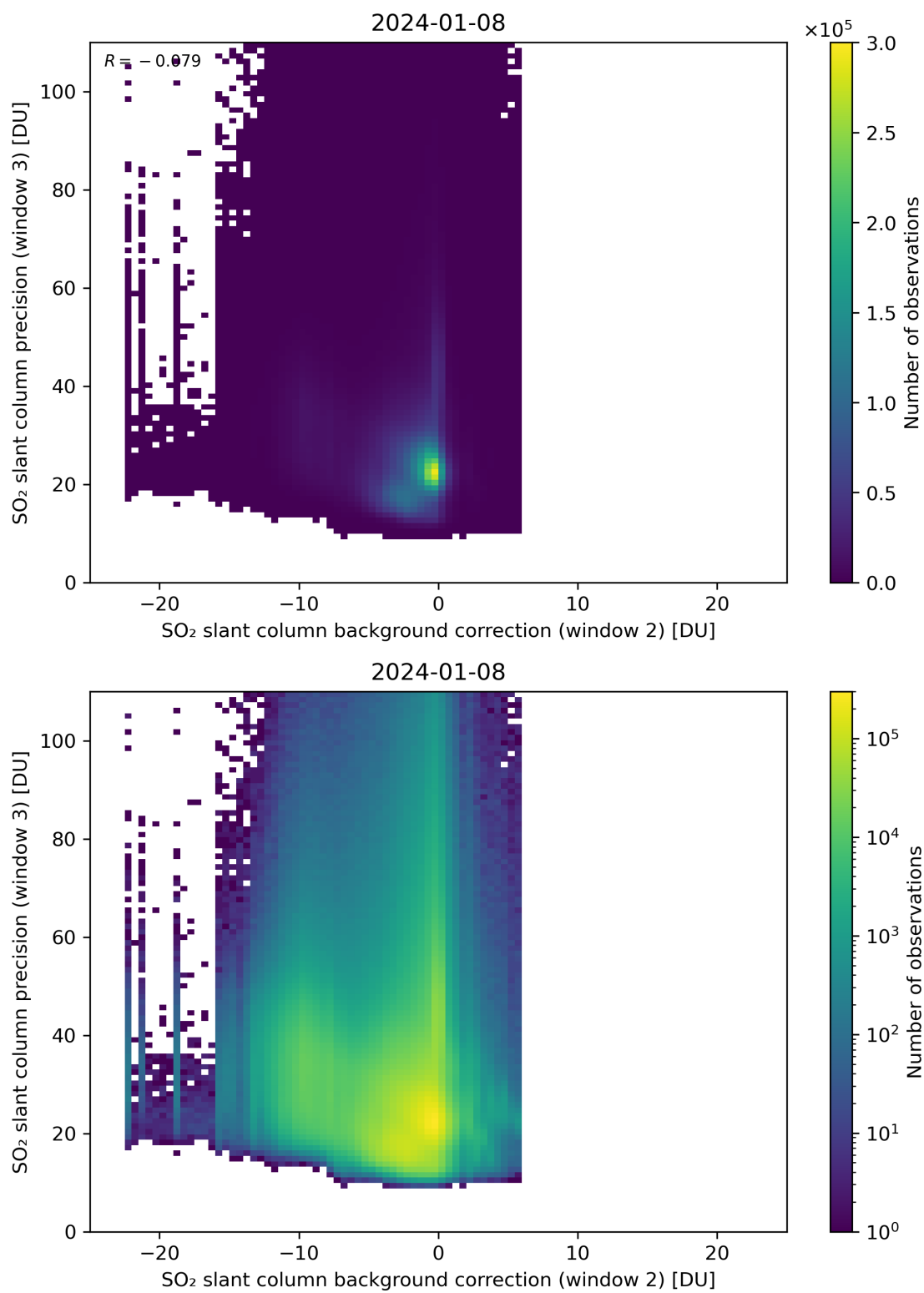
Figure 118: Scatter density plot of “SO 2 slant column background correction (window 2)” against “SO 2 slant column precision (window 3)” for 2024-01-07 to 2024-01-09.
