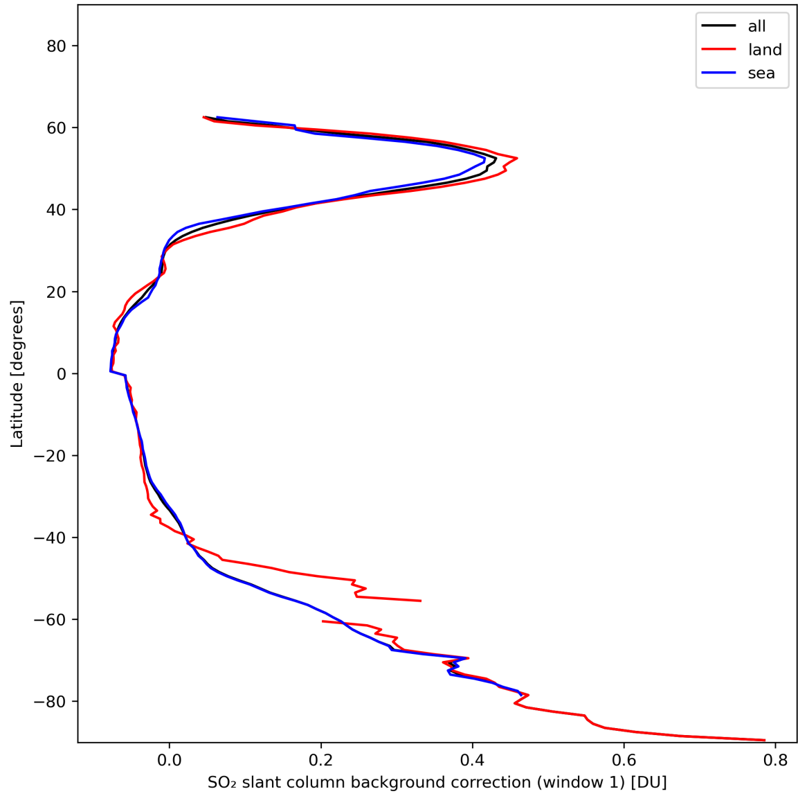
Figure 36: Zonal average of “SO 2 slant column background correction (window 1)” for 2024-01-07 to 2024-01-09.
