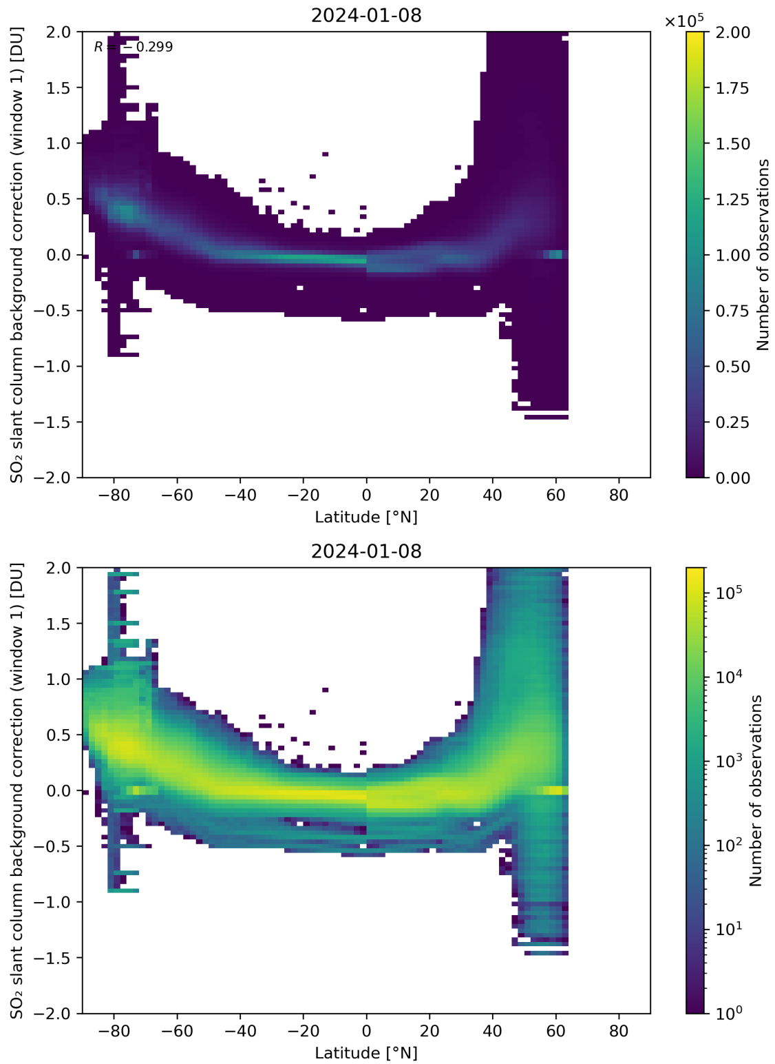
Figure 139: Scatter density plot of “Latitude” against “SO 2 slant column background correction (window 1)” for 2024-01-07 to 2024-01-09.
