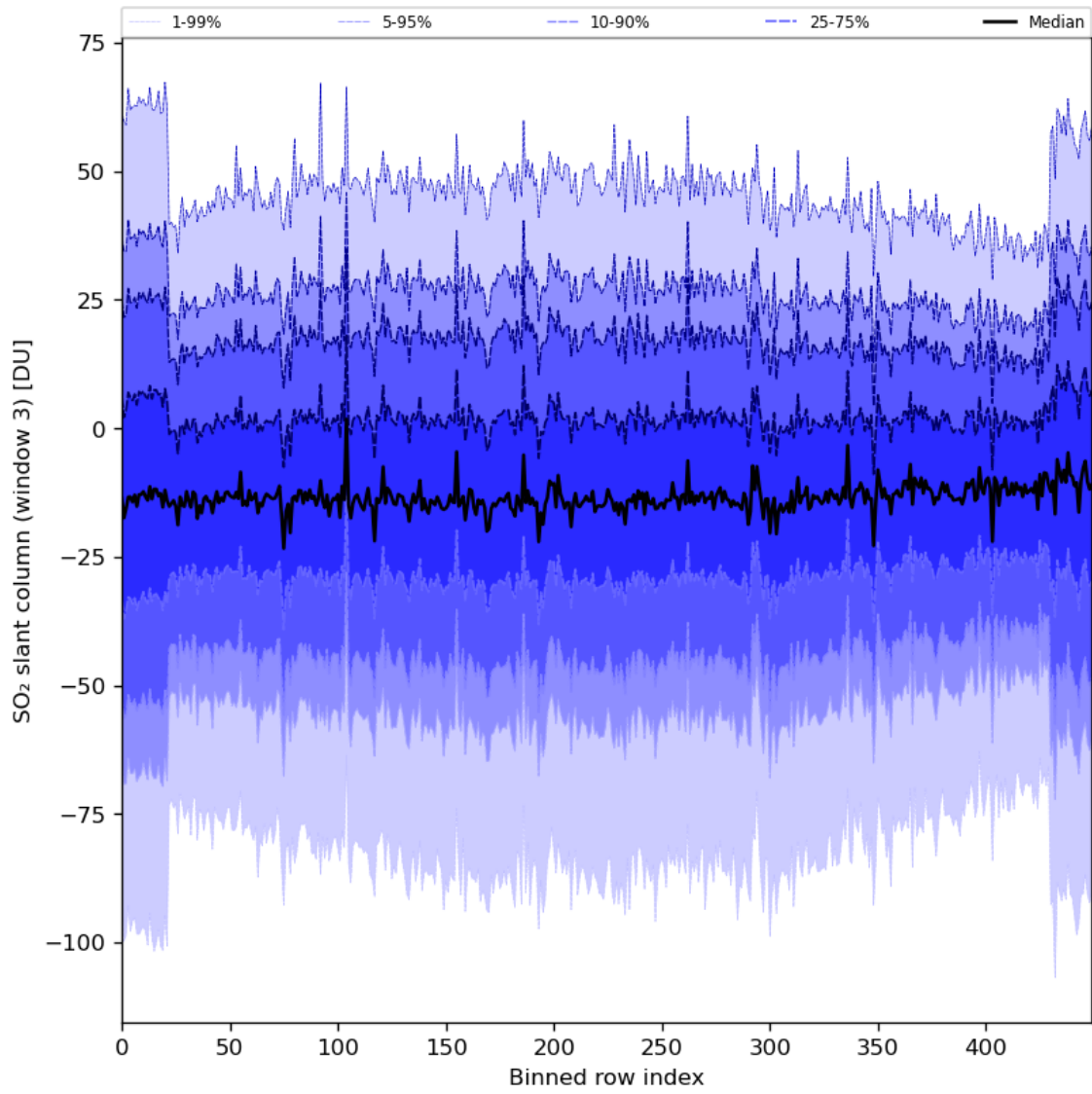
Figure 87: Along track statistics of “SO 2 slant column (window 3)” for 2024-01-07 to 2024-01-09
