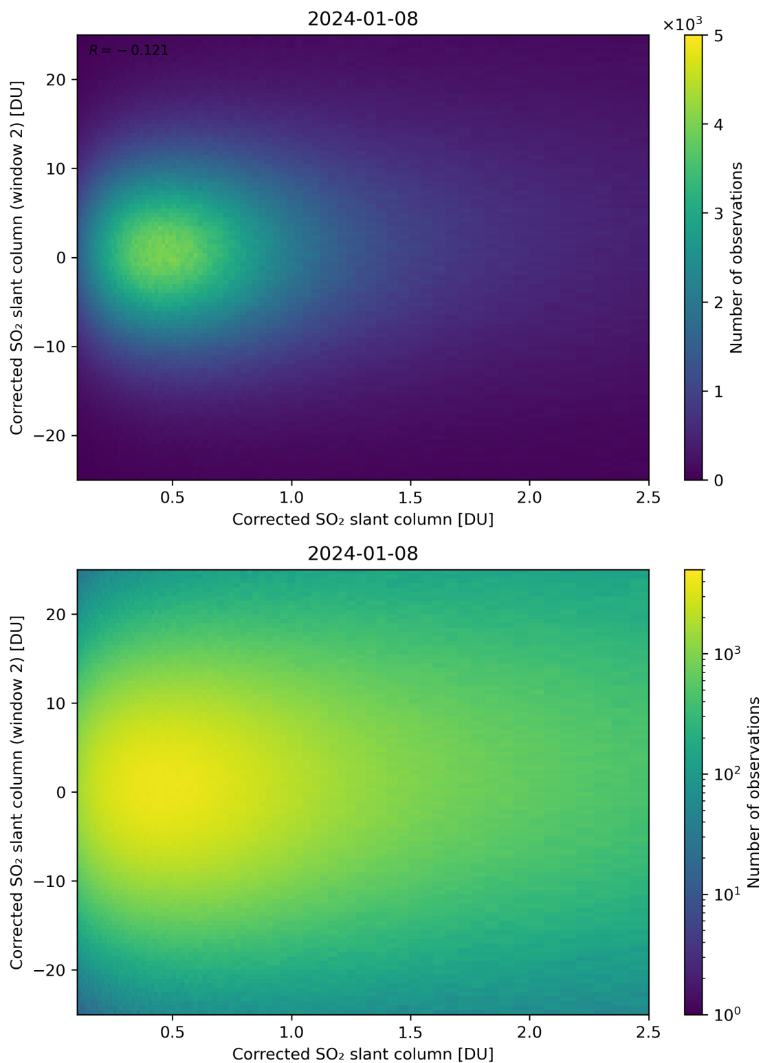
Figure 185: Scatter density plot of “Corrected SO 2 slant column” against “Corrected SO 2 slant column (window 2)” for 2024-01-07 to 2024-01-09.
