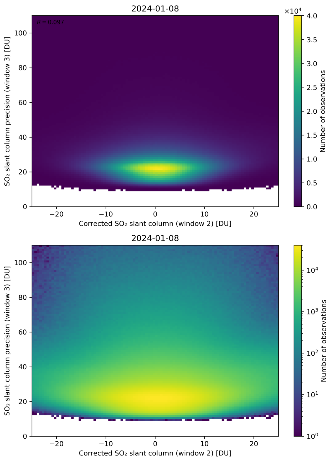
Figure 202: Scatter density plot of “Corrected SO 2 slant column (window 2)” against “SO 2 slant column precision (window 3)” for 2024-01-07 to 2024-01-09.
