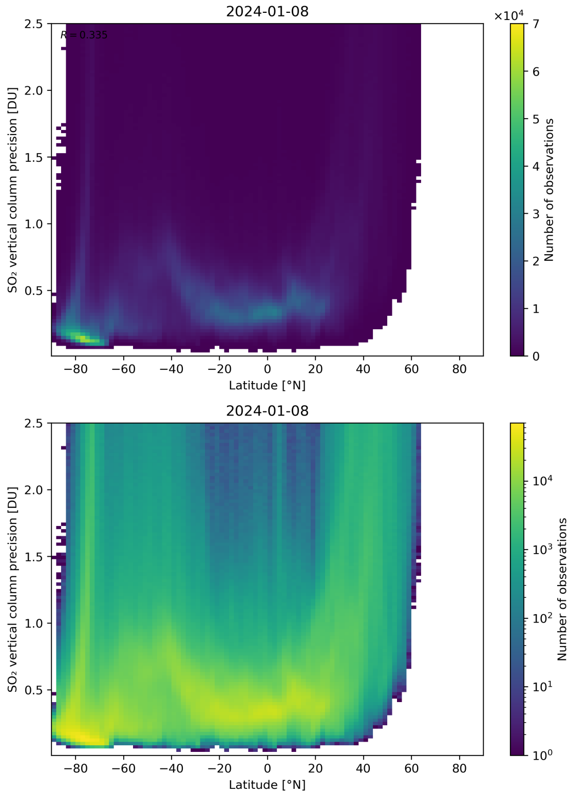
Figure 157: Scatter density plot of “Latitude” against “SO 2 vertical column precision” for 2024-01-07 to 2024-01-09.
