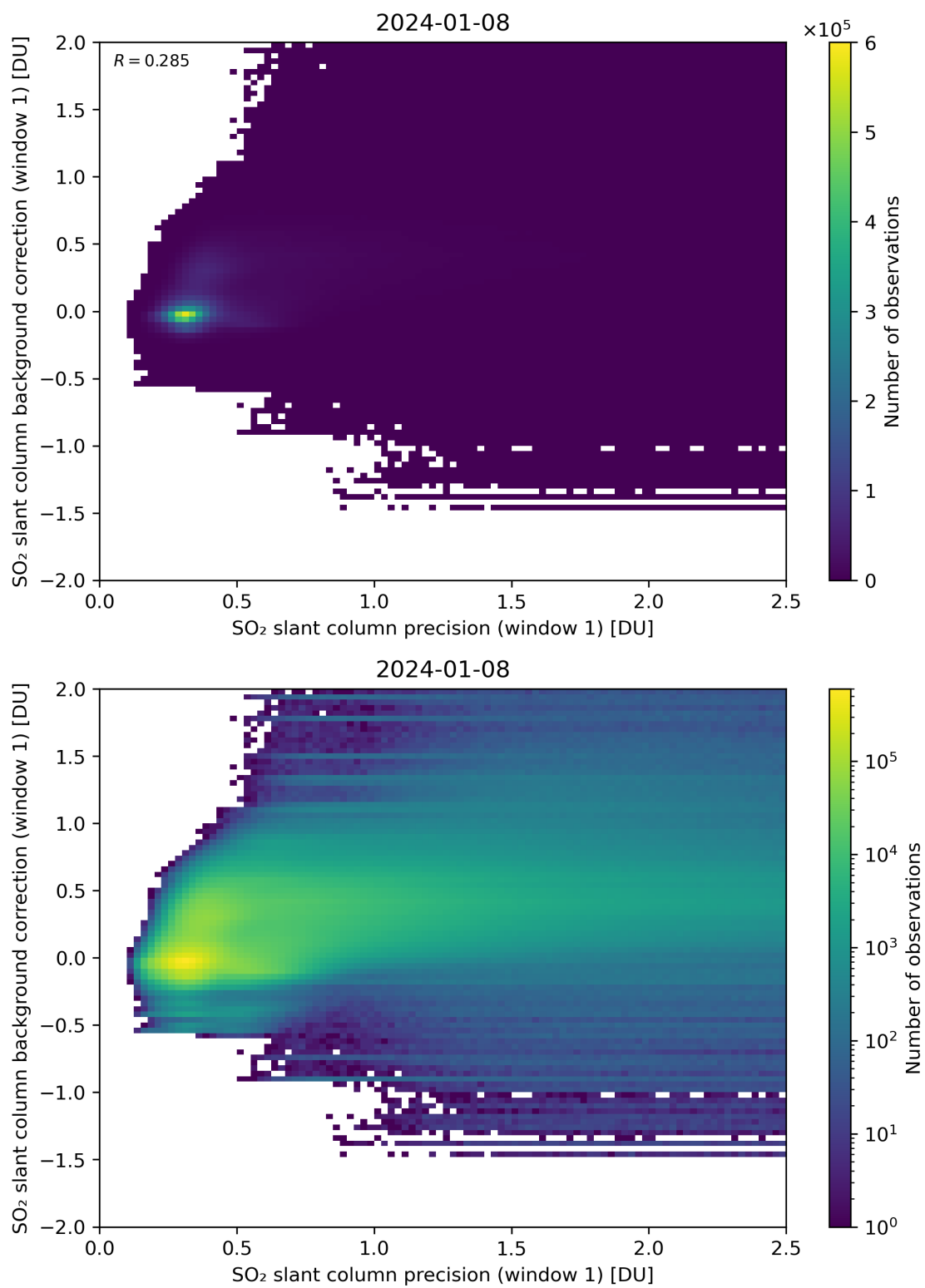
Figure 218: Scatter density plot of “SO 2 slant column precision (window 1)” against “SO 2 slant column background correction (window 1)” for 2024-01-07 to 2024-01-09.
