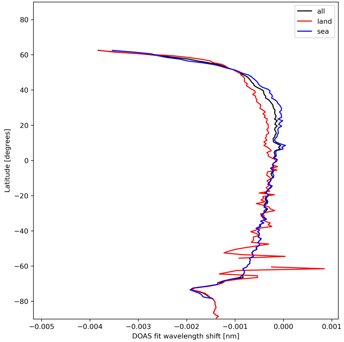
Figure 45: Zonal average of “DOAS fit wavelength shift” for 2024-01-07 to 2024-01-09.
