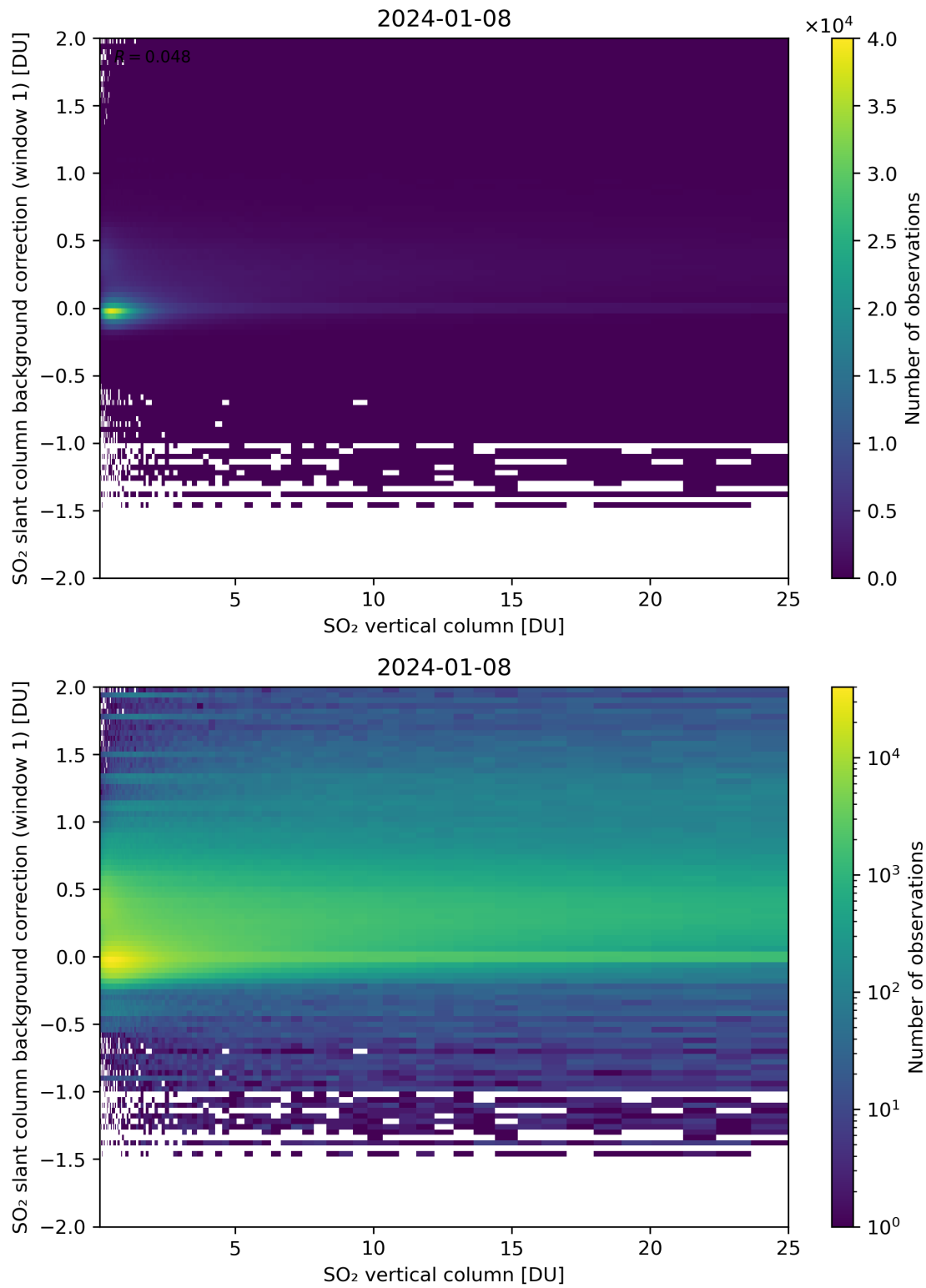
Figure 273: Scatter density plot of “SO 2 vertical column” against “SO 2 slant column background correction (window 1)” for 2024-01-07 to 2024-01-09.
