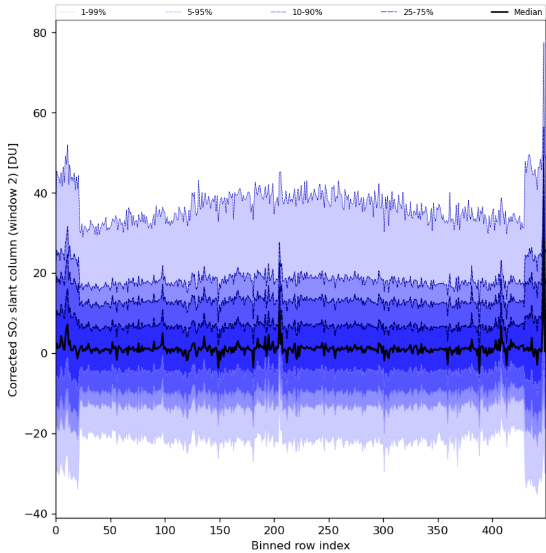
Figure 85: Along track statistics of “Corrected SO 2 slant column (window 2)” for 2024-01-07 to 2024-01-09
