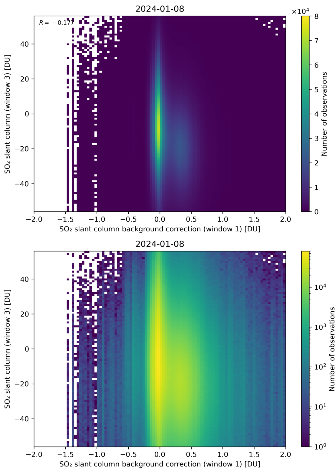
Figure 107: Scatter density plot of “SO 2 slant column background correction (window 1)” against “SO 2 slant column (window 3)” for 2024-01-07 to 2024-01-09.
