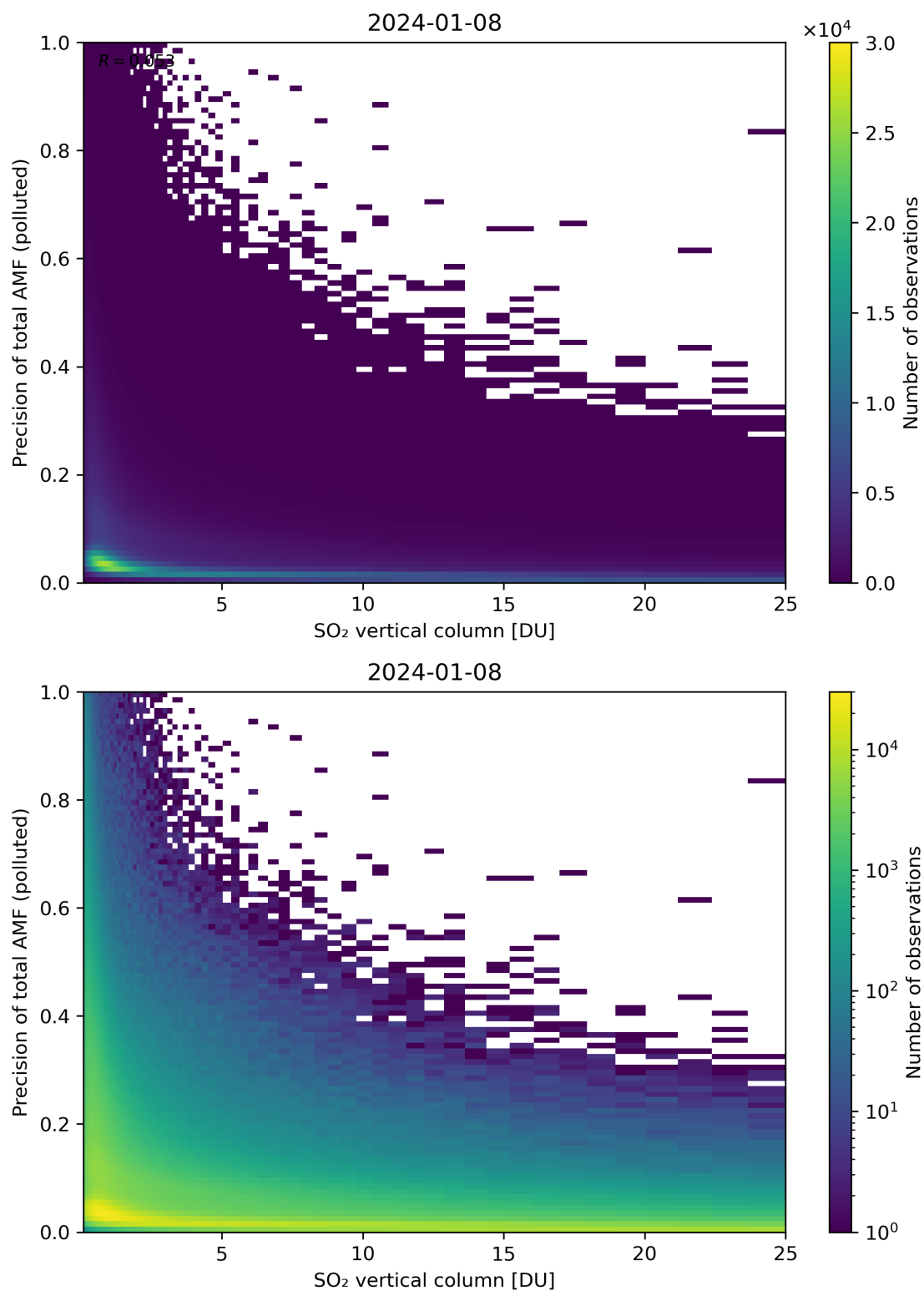
Figure 306: Scatter density plot of “SO 2 vertical column” against “Precision of total AMF (polluted)” for 2024-01-07 to 2024-01-09.
