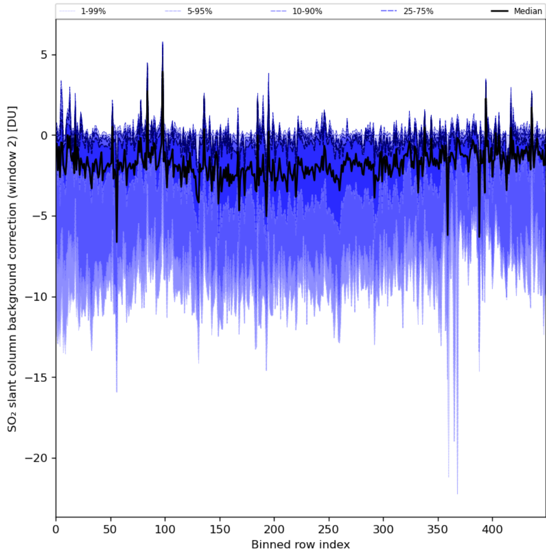
Figure 86: Along track statistics of “SO 2 slant column background correction (window 2)” for 2024-01-07 to 2024-01-09
