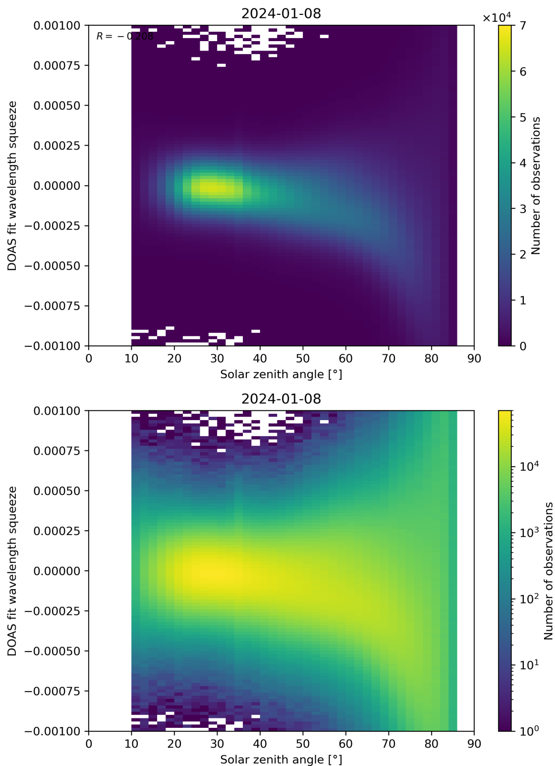
Figure 162: Scatter density plot of “Solar zenith angle” against “DOAS fit wavelength squeeze” for 2024-01-07 to 2024-01-09.
