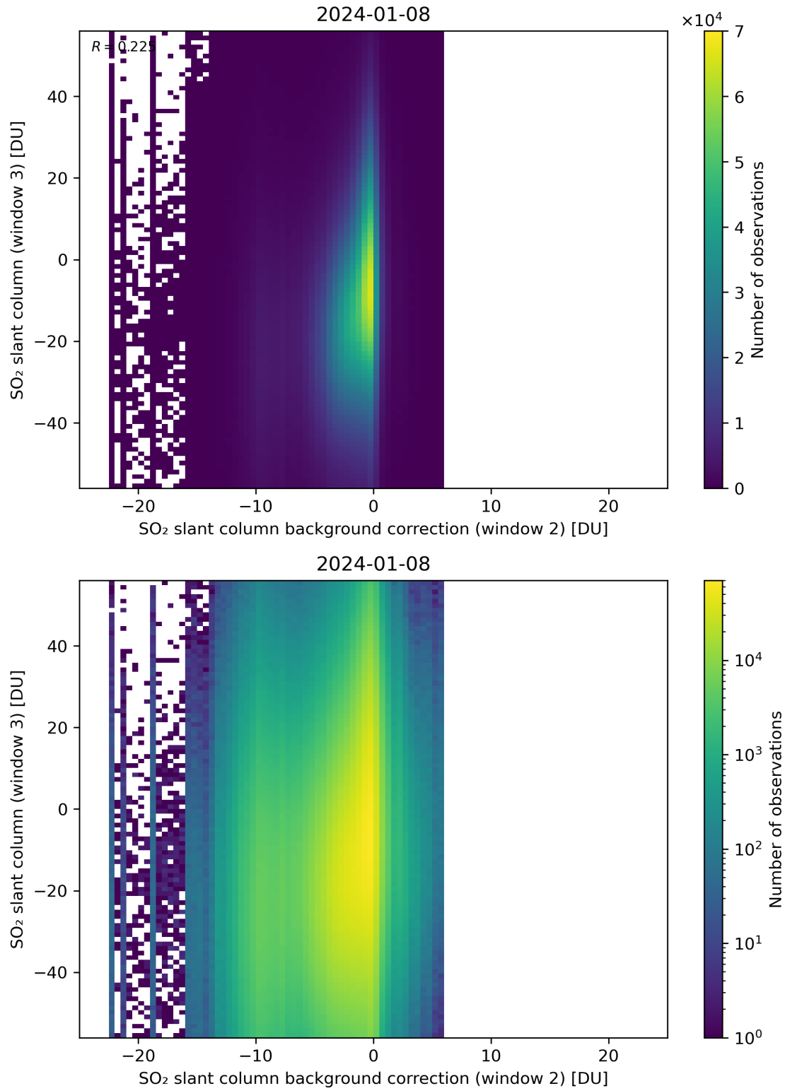
Figure 117: Scatter density plot of “SO 2 slant column background correction (window 2)” against “SO 2 slant column (window 3)” for 2024-01-07 to 2024-01-09.
