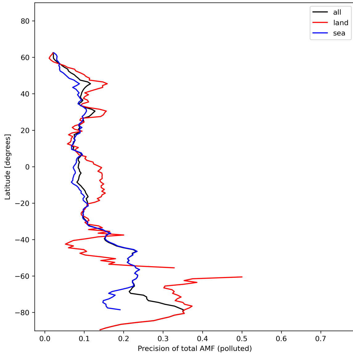
Figure 49: Zonal average of “Precision of total AMF (polluted)” for 2024-01-07 to 2024-01-09.
