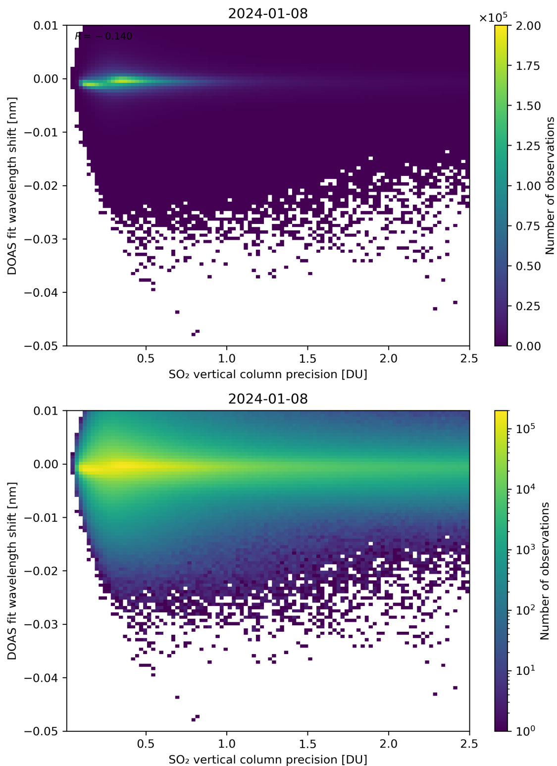
Figure 282: Scatter density plot of “SO 2 vertical column precision” against “DOAS fit wavelength shift” for 2024-01-07 to 2024-01-09.
