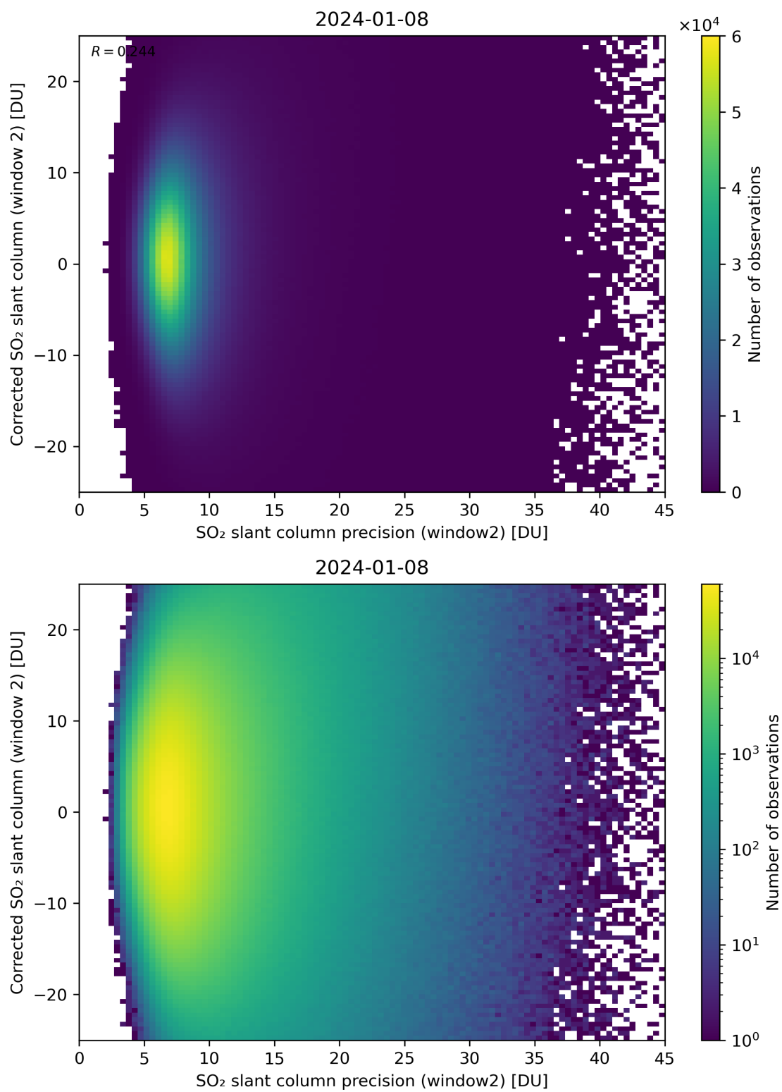
Figure 247: Scatter density plot of “SO 2 slant column precision (window2)” against “Corrected SO 2 slant column (window 2)” for 2024-01-07 to 2024-01-09.
