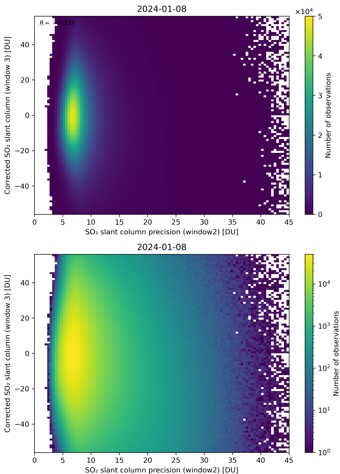
Figure 248: Scatter density plot of “SO 2 slant column precision (window2)” against “Corrected SO 2 slant column (window 3)” for 2024-01-07 to 2024-01-09.
