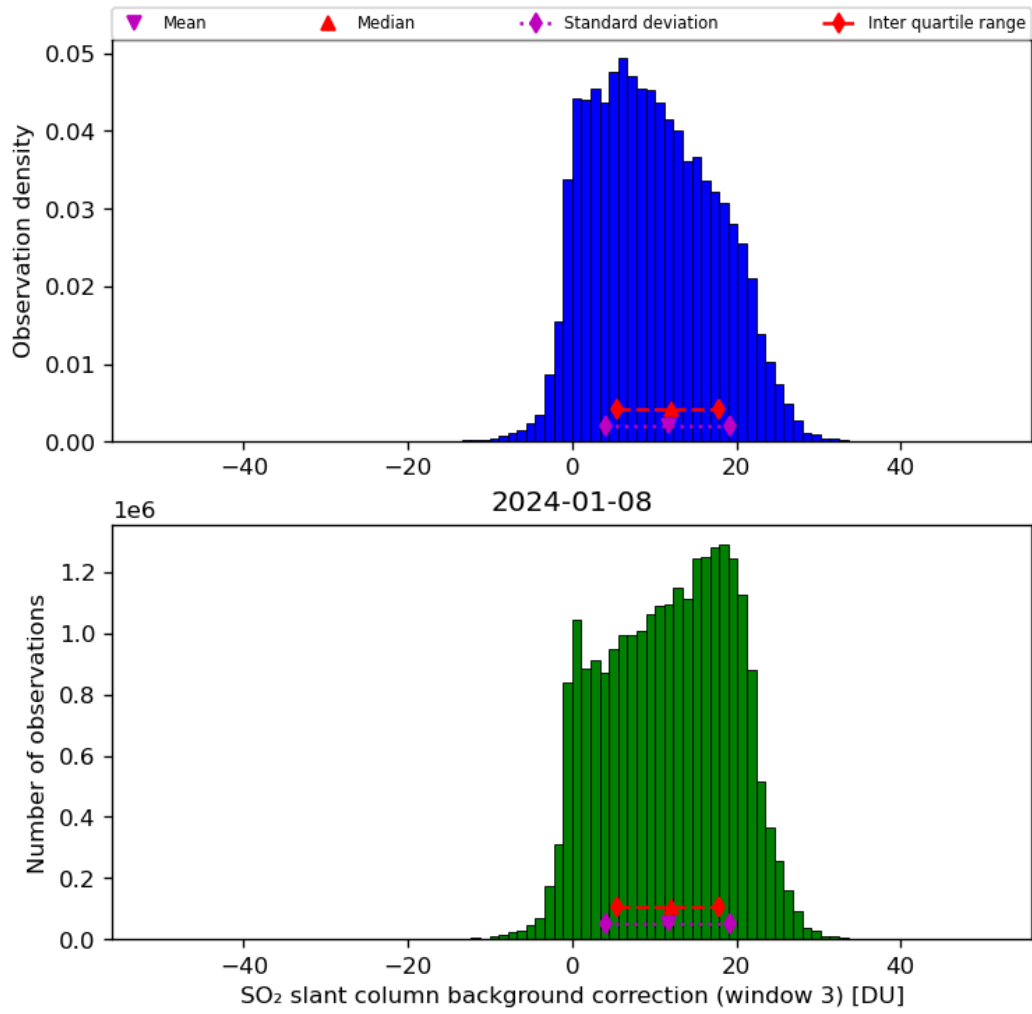
Figure 67: Histogram of “SO 2 slant column background correction (window 3)” for 2024-01-07 to 2024-01-09
