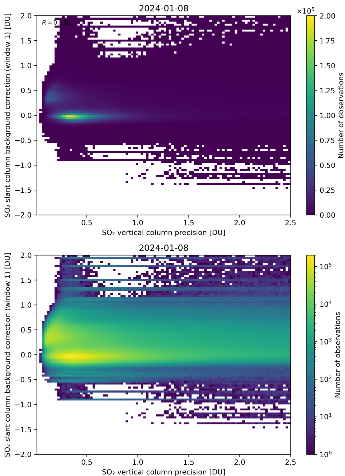
Figure 279: Scatter density plot of “SO 2 vertical column precision” against “SO 2 slant column background correction (window 1)” for 2024-01-07 to 2024-01-09.
