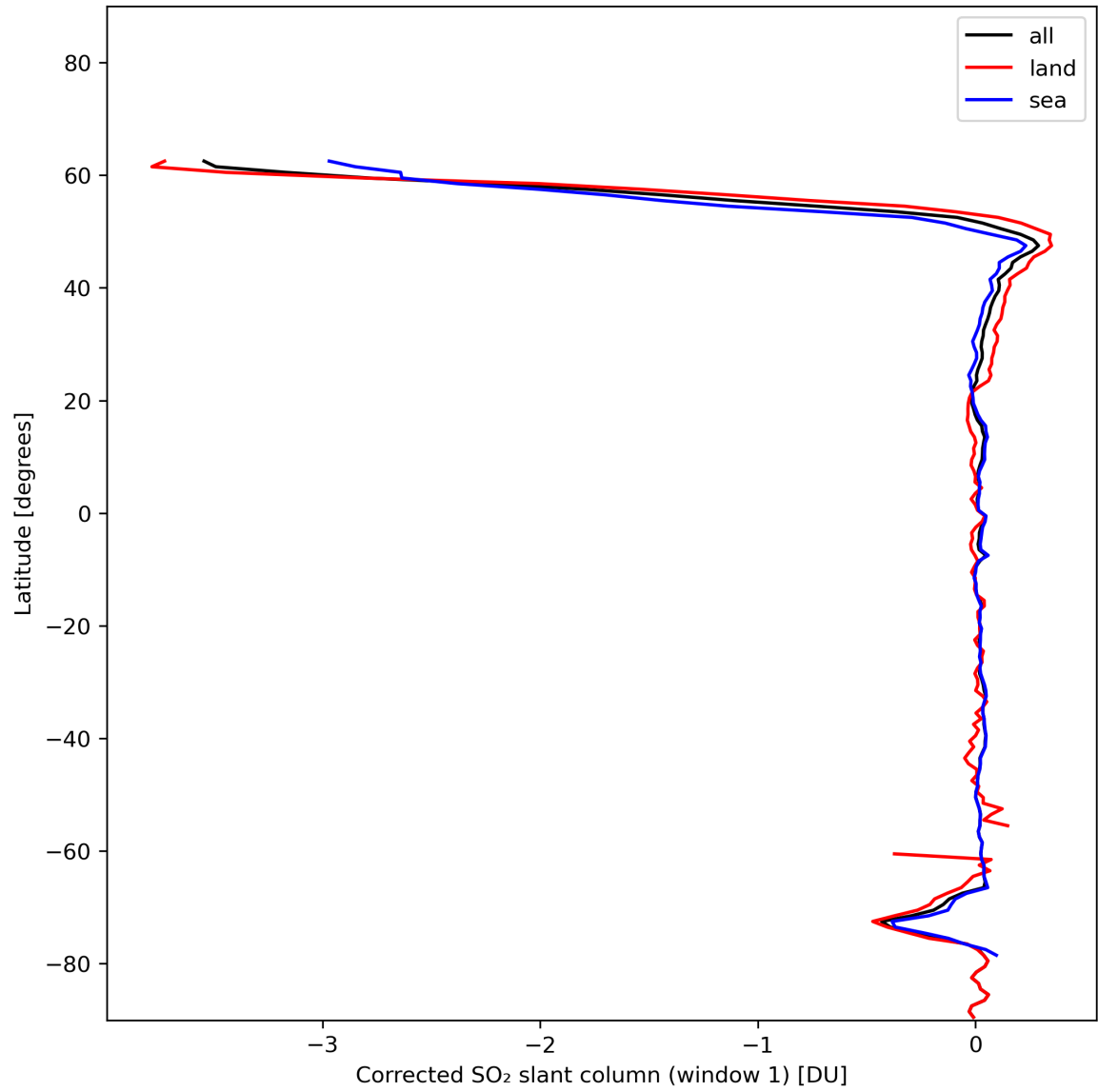
Figure 35: Zonal average of “Corrected SO 2 slant column (window 1)” for 2024-01-07 to 2024-01-09.
