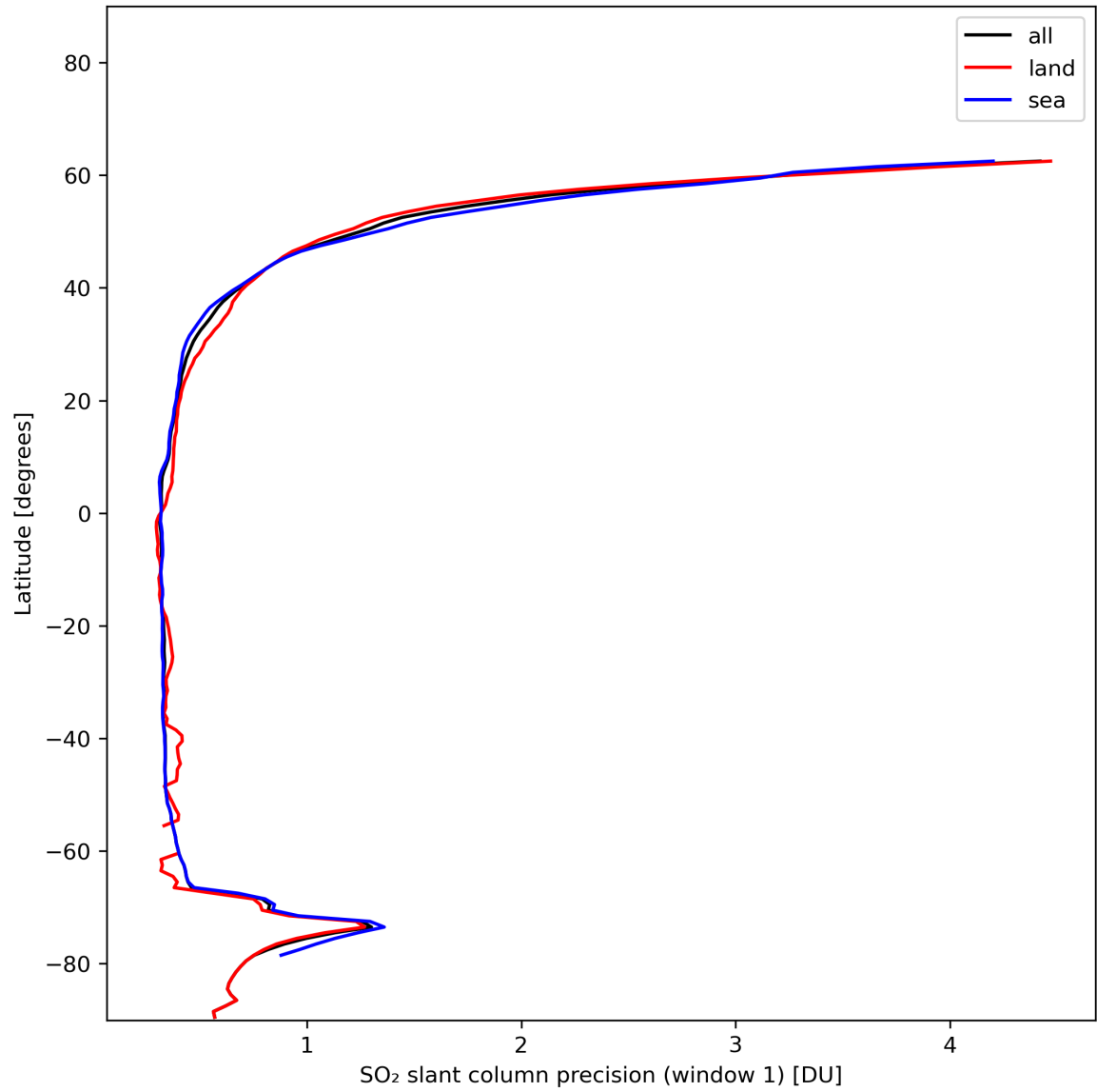
Figure 34: Zonal average of “SO 2 slant column precision (window 1)” for 2024-01-07 to 2024-01-09.
