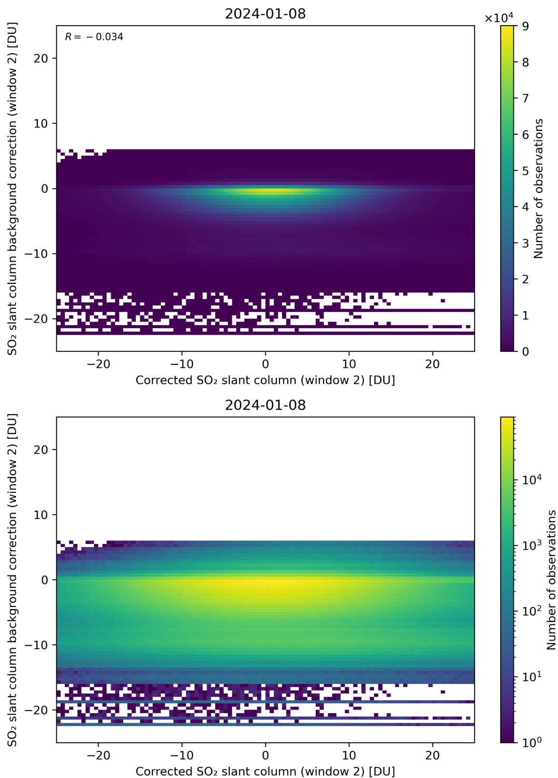
Figure 194: Scatter density plot of “Corrected SO 2 slant column (window 2)” against “SO 2 slant column background correction (window 2)” for 2024-01-07 to 2024-01-09.
