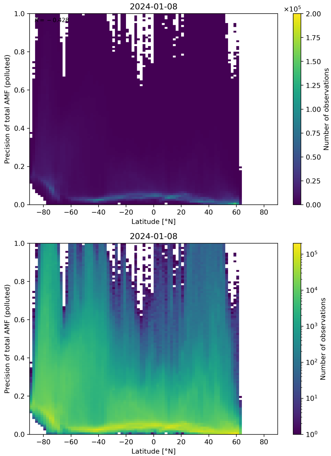
Figure 155: Scatter density plot of “Latitude” against “Precision of total AMF (polluted)” for 2024-01-07 to 2024-01-09.
