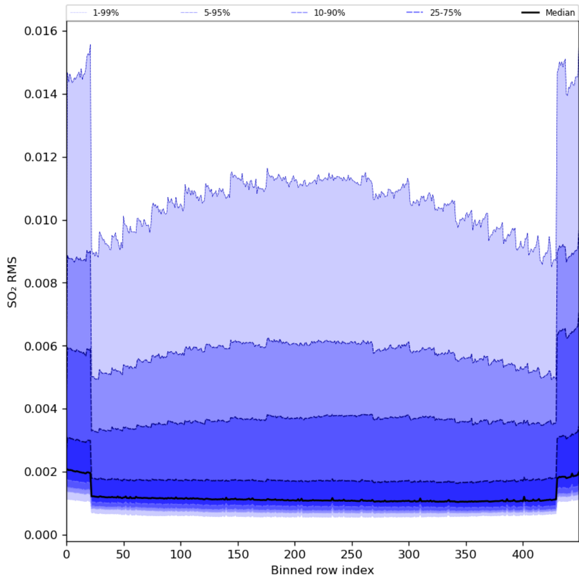
Figure 93: Along track statistics of “SO 2 RMS” for 2024-01-07 to 2024-01-09
