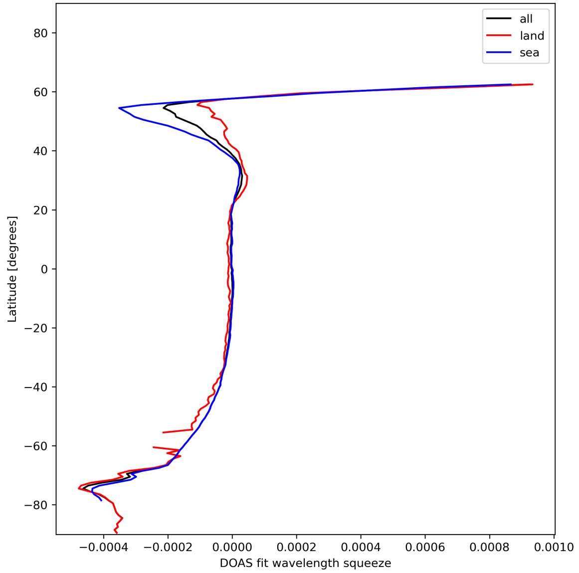
Figure 46: Zonal average of “DOAS fit wavelength squeeze” for 2024-01-07 to 2024-01-09.
