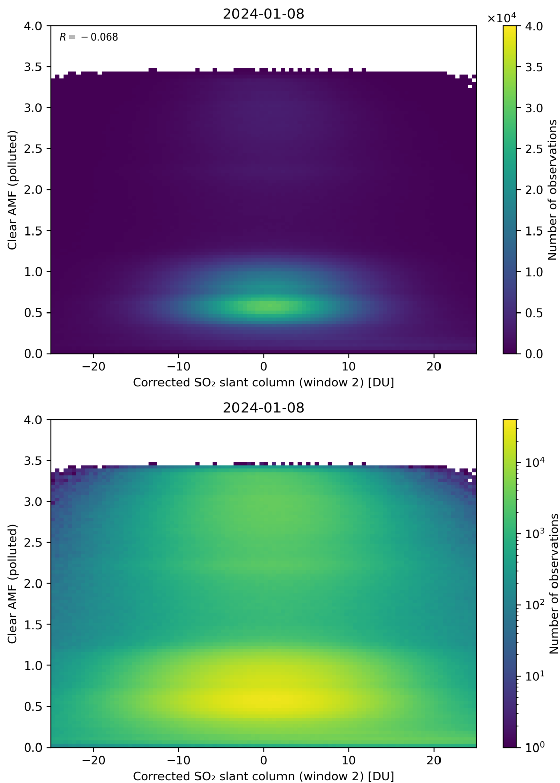
Figure 199: Scatter density plot of “Corrected SO 2 slant column (window 2)” against “Clear AMF (polluted)” for 2024-01-07 to 2024-01-09.
