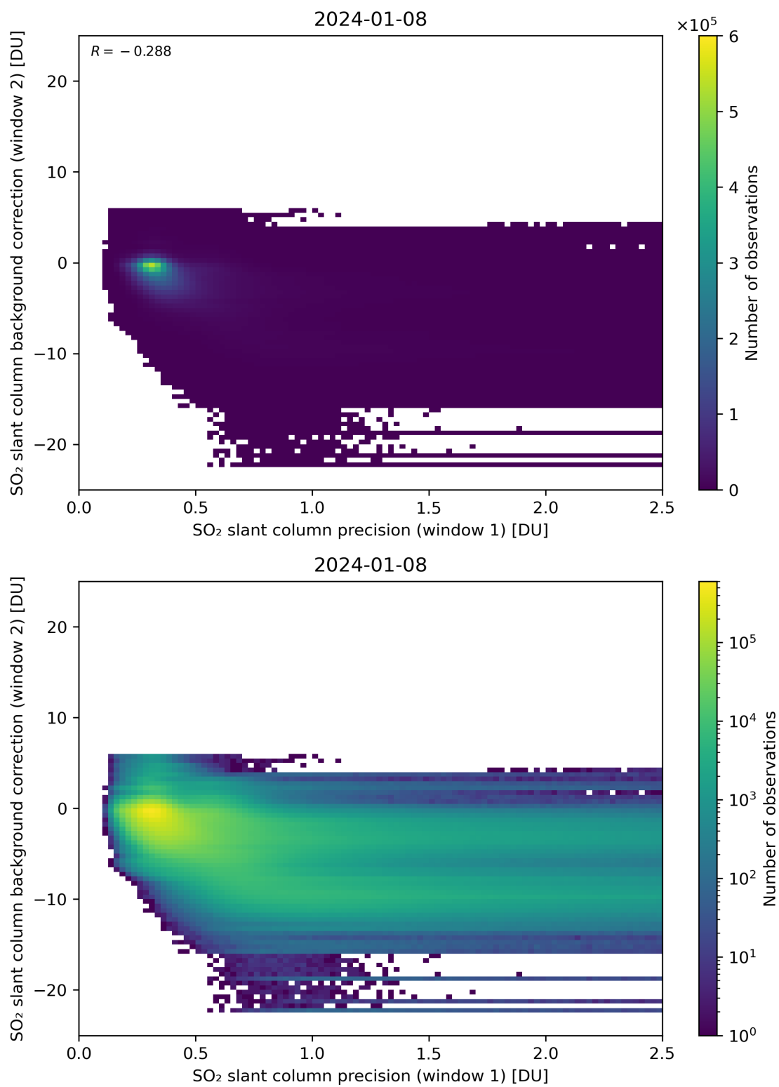
Figure 219: Scatter density plot of “SO 2 slant column precision (window 1)” against “SO 2 slant column background correction (window 2)” for 2024-01-07 to 2024-01-09.
