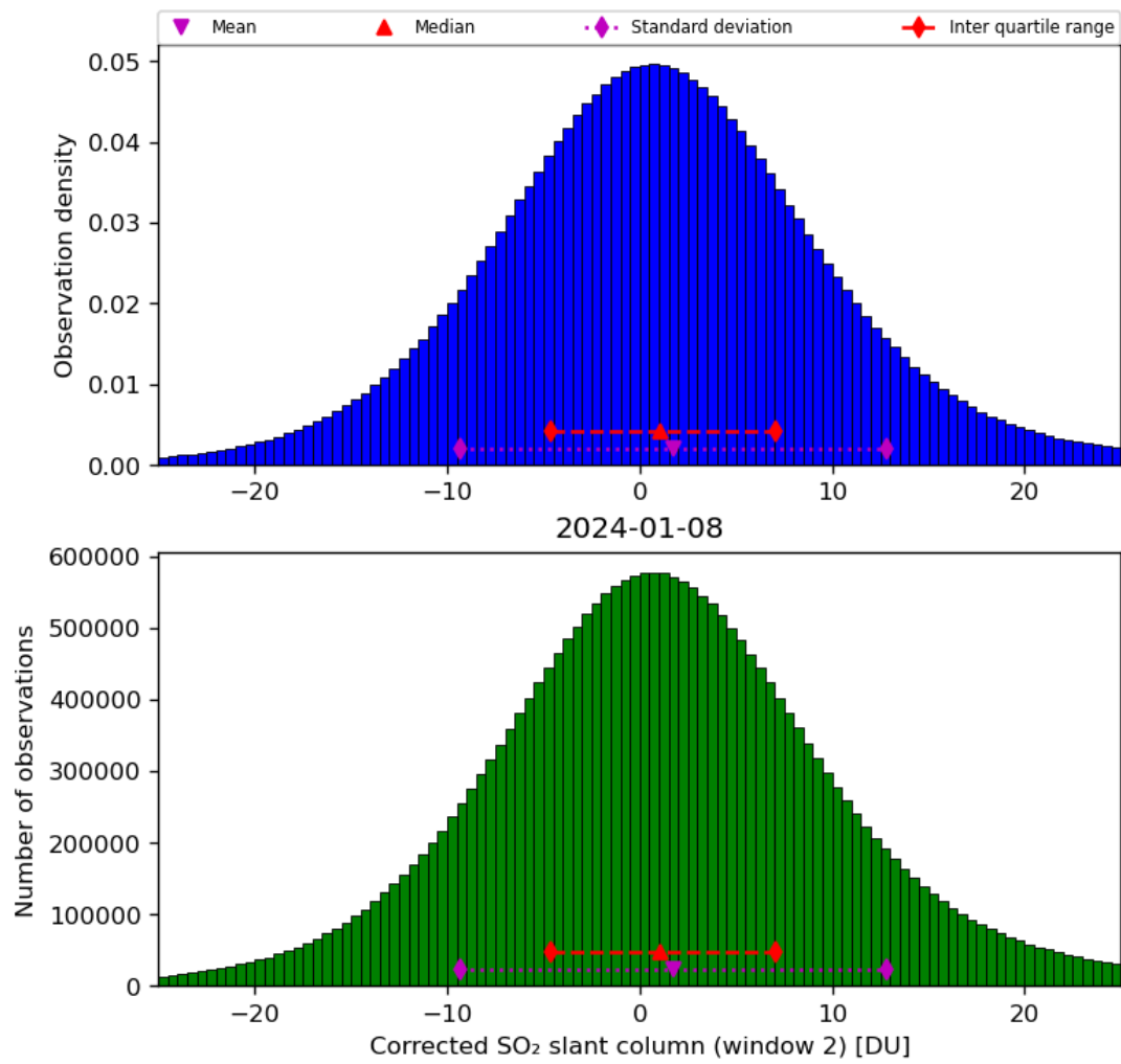
Figure 62: Histogram of “Corrected SO 2 slant column (window 2)” for 2024-01-07 to 2024-01-09
