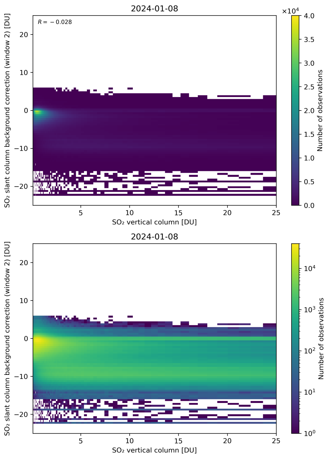
Figure 274: Scatter density plot of “SO 2 vertical column” against “SO 2 slant column background correction (window 2)” for 2024-01-07 to 2024-01-09.
