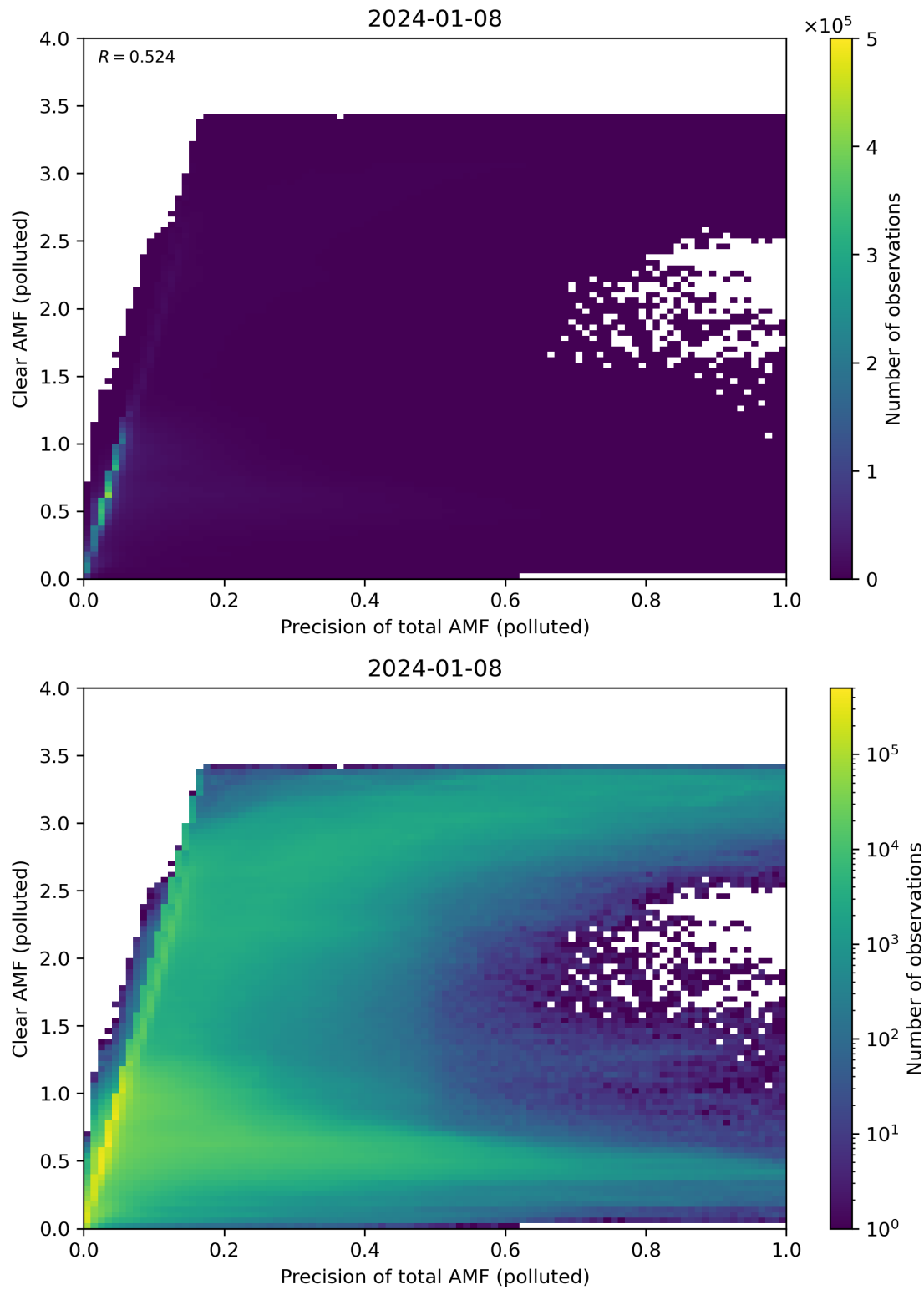
Figure 270: Scatter density plot of “Precision of total AMF (polluted)” against “Clear AMF (polluted)” for 2024-01-07 to 2024-01-09.
