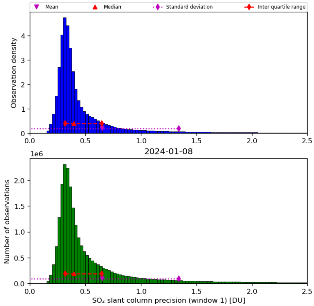
Figure 57: Histogram of “SO 2 slant column precision (window 1)” for 2024-01-07 to 2024-01-09
