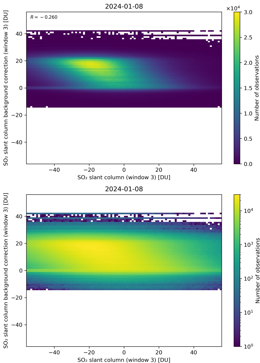
Figure 253: Scatter density plot of “SO 2 slant column (window 3)” against “SO 2 slant column background correction (window 3)” for 2024-01-07 to 2024-01-09.
