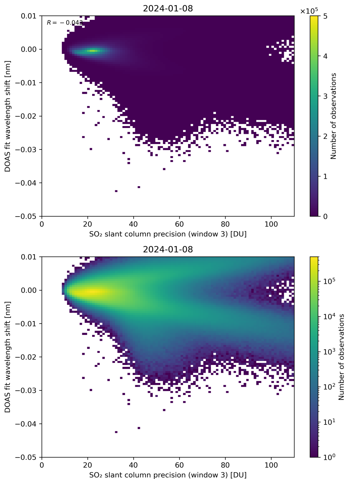
Figure 258: Scatter density plot of “SO 2 slant column precision (window 3)” against “DOAS fit wavelength shift” for 2024-01-07 to 2024-01-09.
