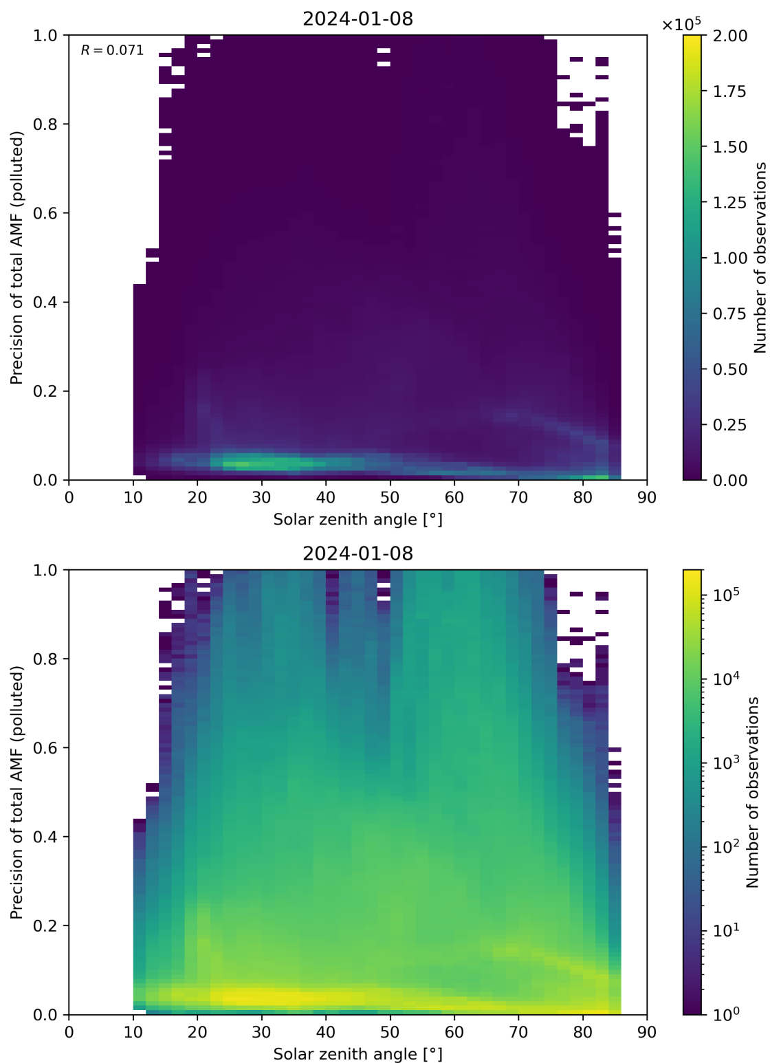
Figure 175: Scatter density plot of “Solar zenith angle” against “Precision of total AMF (polluted)” for 2024-01-07 to 2024-01-09.
