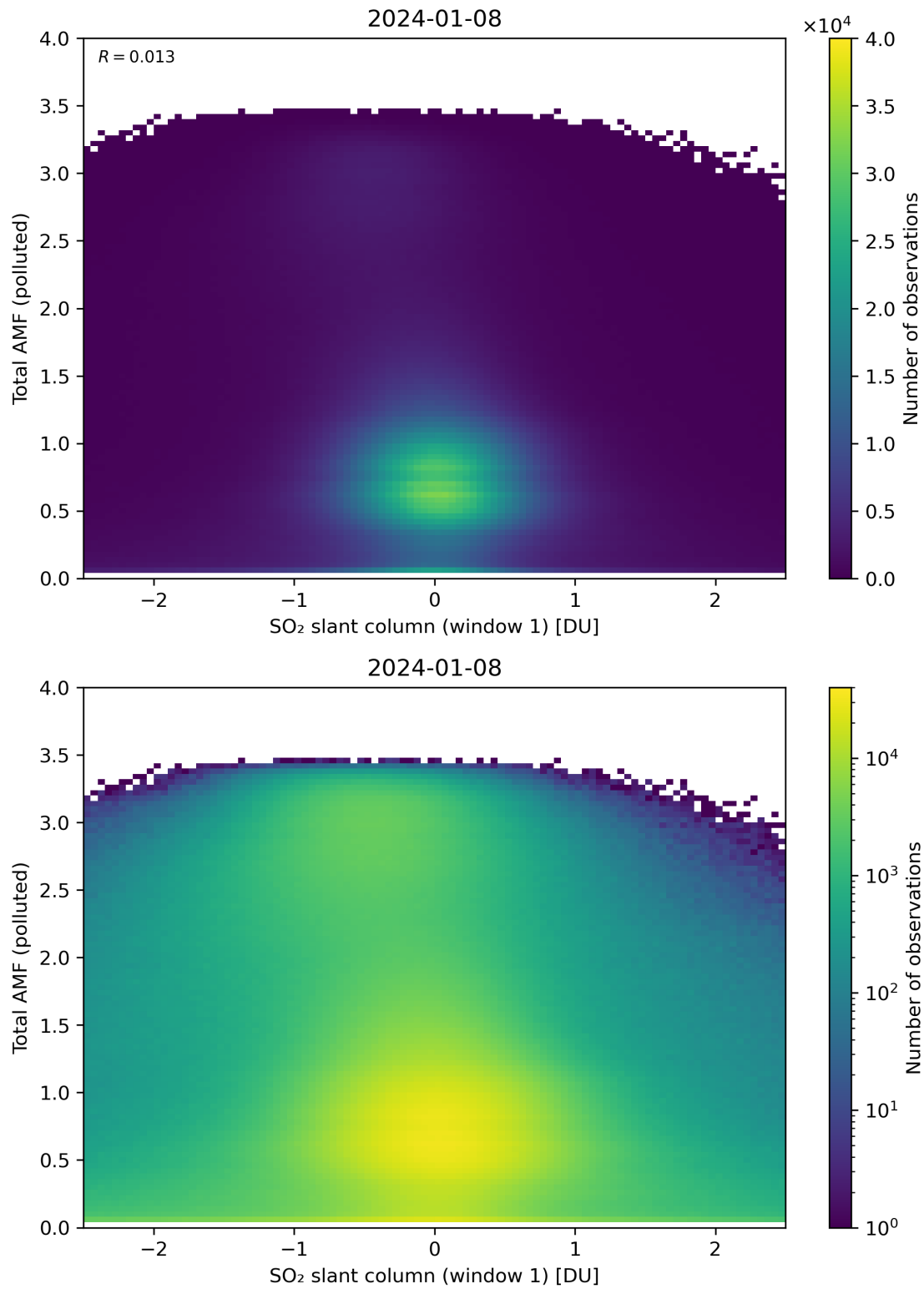
Figure 239: Scatter density plot of “SO 2 slant column (window 1)” against “Total AMF (polluted)” for 2024-01-07 to 2024-01-09.
