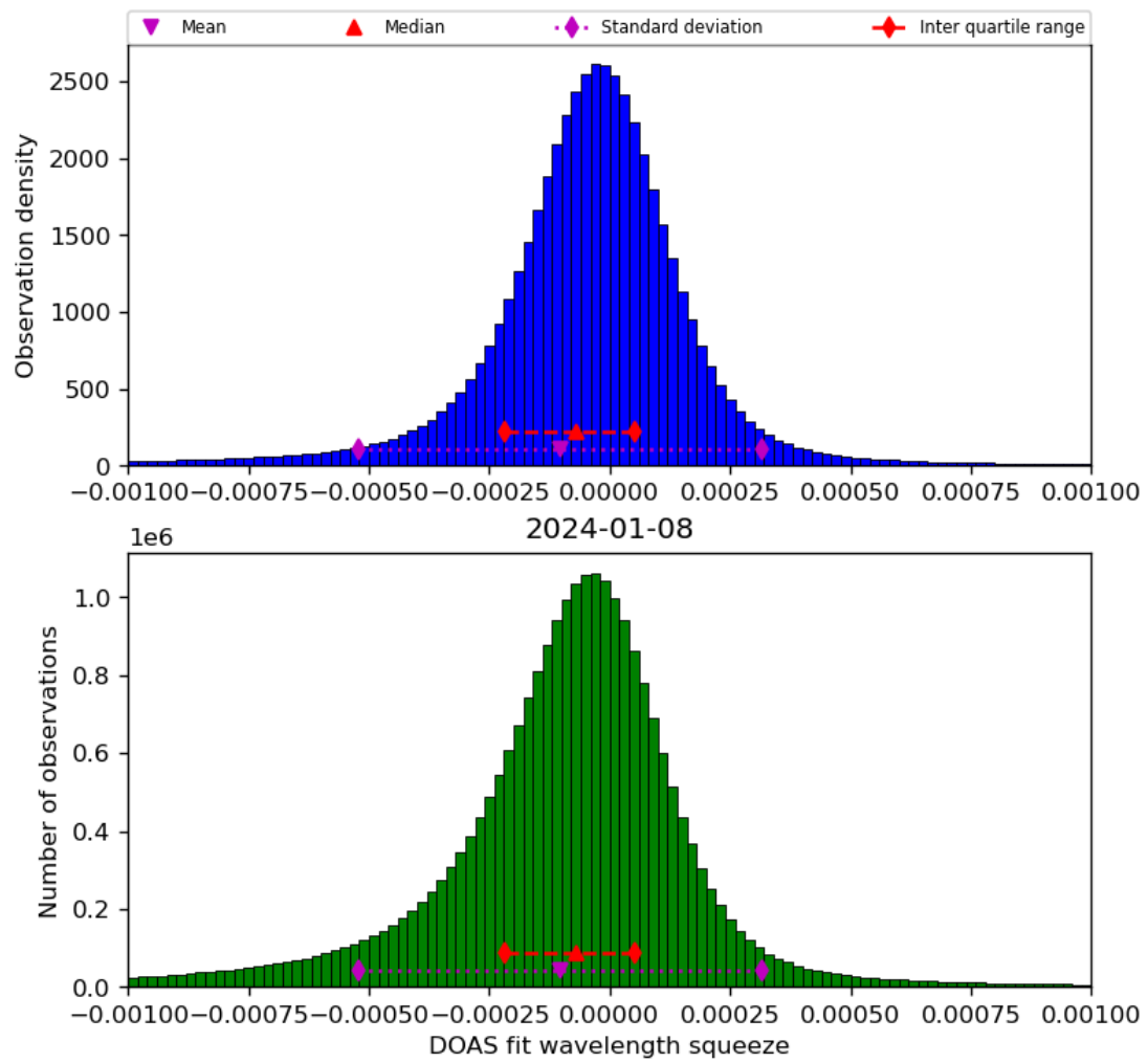
Figure 69: Histogram of “DOAS fit wavelength squeeze” for 2024-01-07 to 2024-01-09
