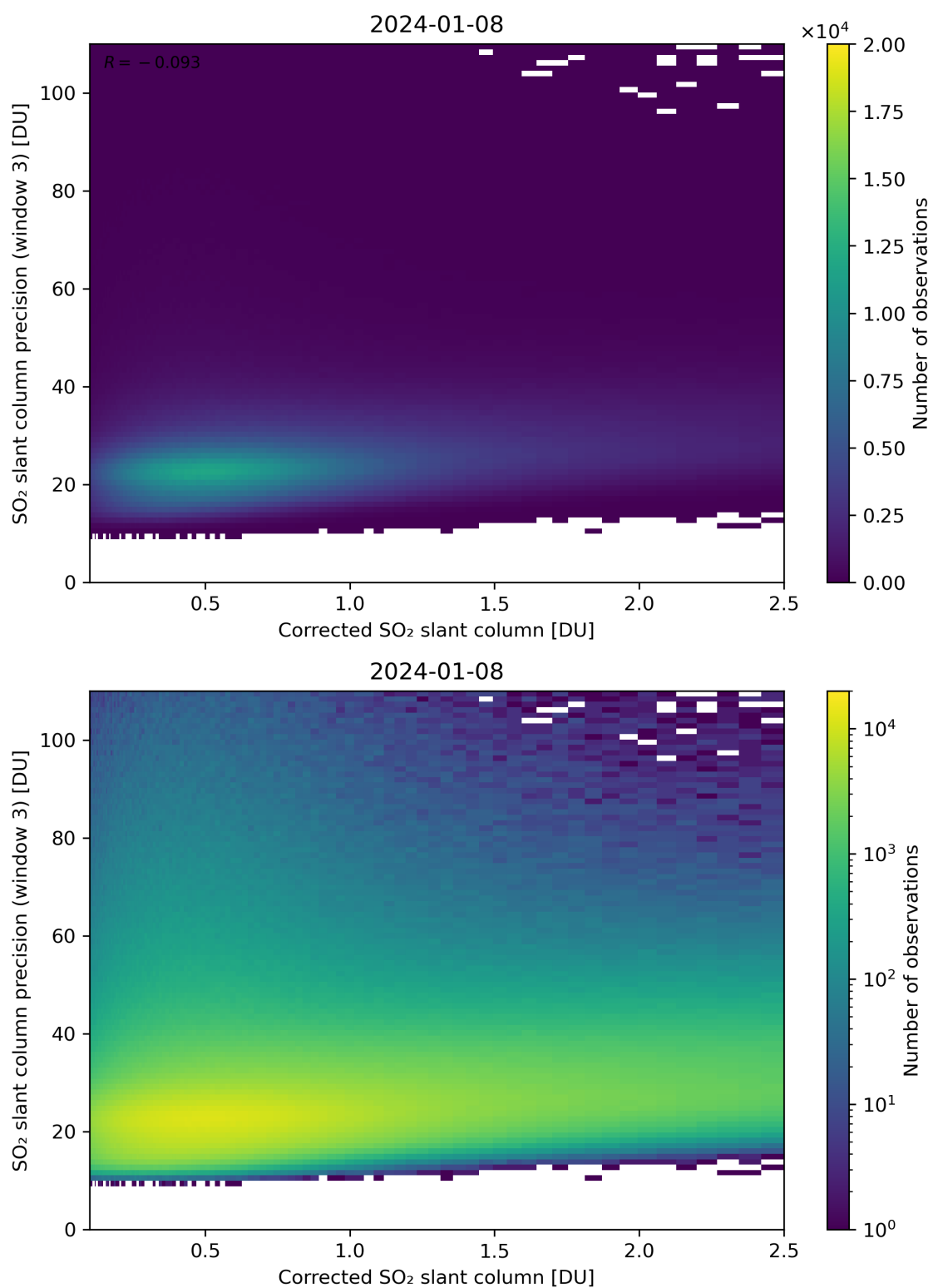
Figure 191: Scatter density plot of “Corrected SO 2 slant column” against “SO 2 slant column precision (window 3)” for 2024-01-07 to 2024-01-09.
