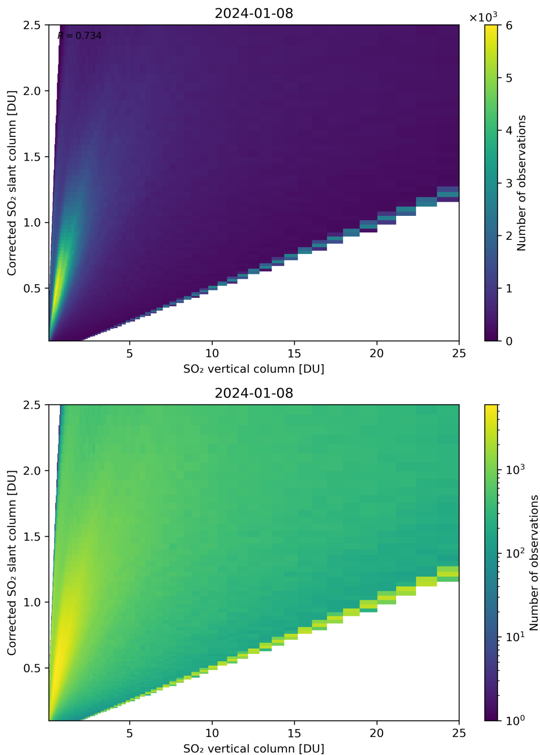
Figure 297: Scatter density plot of “SO 2 vertical column” against “Corrected SO 2 slant column” for 2024-01-07 to 2024-01-09.
