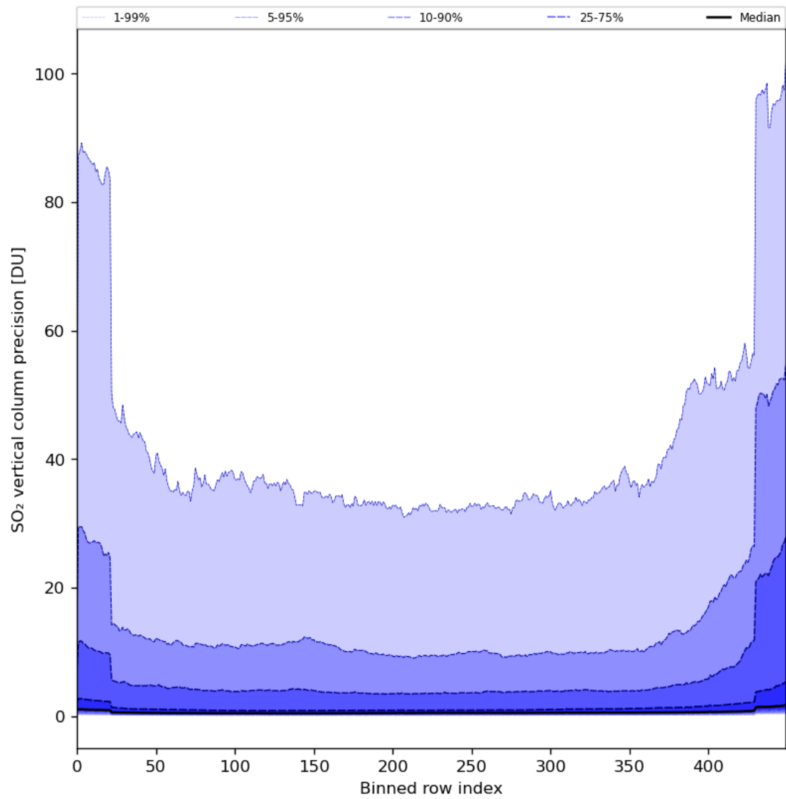
Figure 77: Along track statistics of “SO 2 vertical column precision” for 2024-01-07 to 2024-01-09
