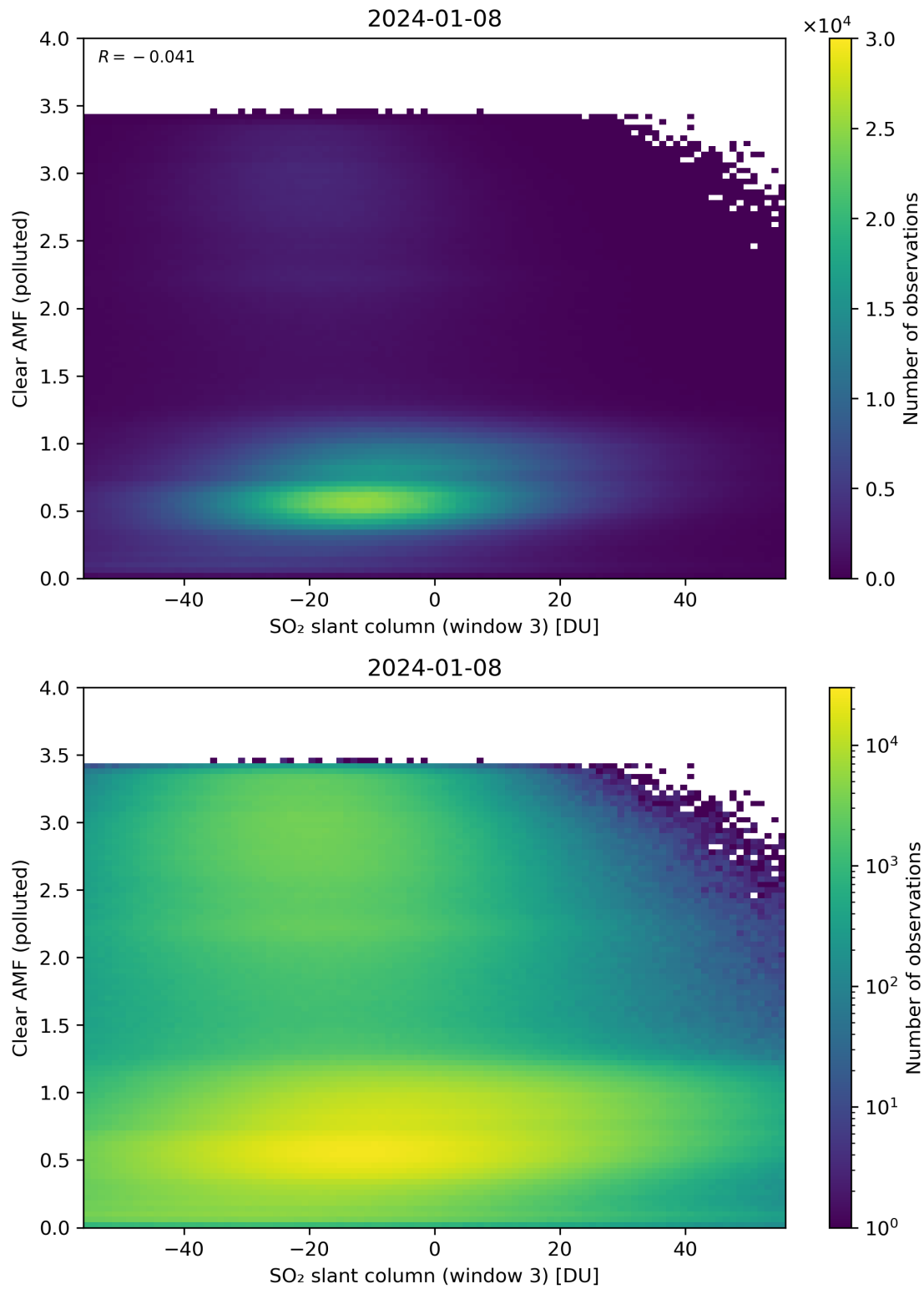
Figure 265: Scatter density plot of “SO 2 slant column (window 3)” against “Clear AMF (polluted)” for 2024-01-07 to 2024-01-09.
