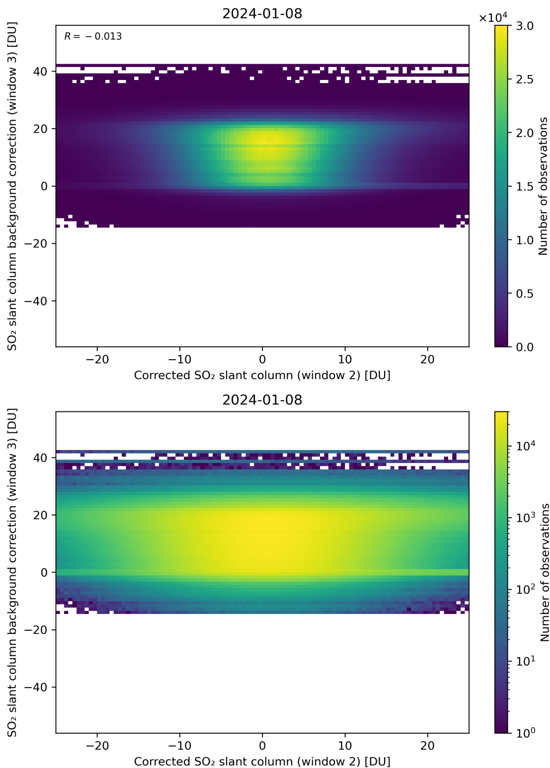
Figure 195: Scatter density plot of “Corrected SO 2 slant column (window 2)” against “SO 2 slant column background correction (window 3)” for 2024-01-07 to 2024-01-09.
