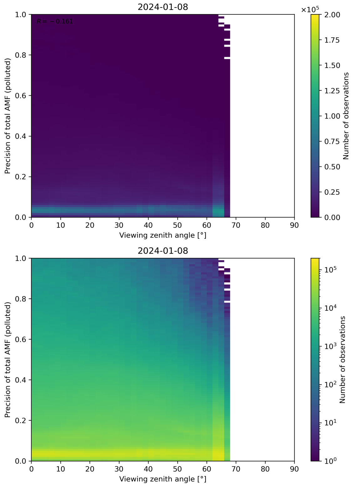
Figure 326: Scatter density plot of “Viewing zenith angle” against “Precision of total AMF (polluted)” for 2024-01-07 to 2024-01-09.
