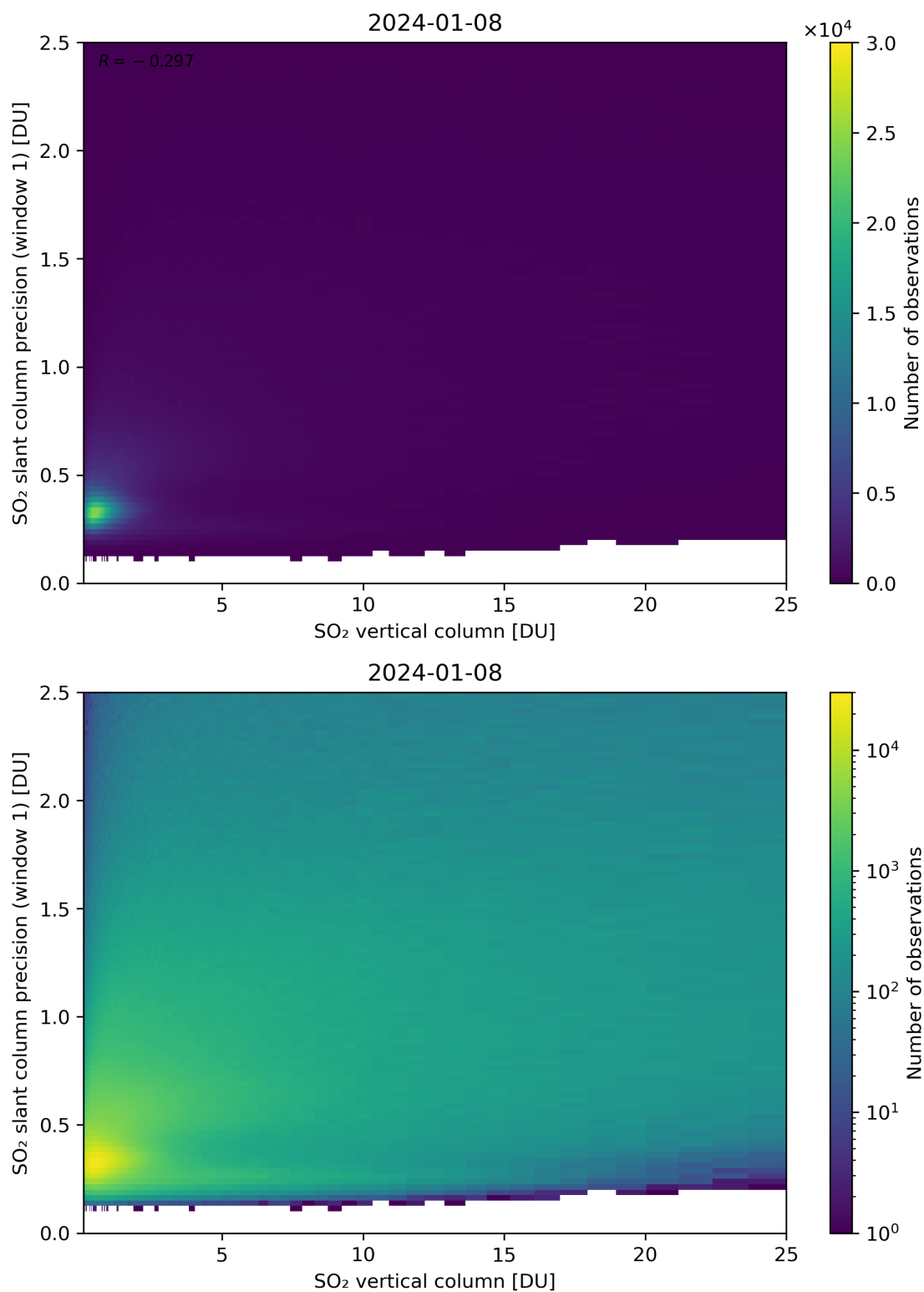
Figure 301: Scatter density plot of “SO 2 vertical column” against “SO 2 slant column precision (window 1)” for 2024-01-07 to 2024-01-09.
