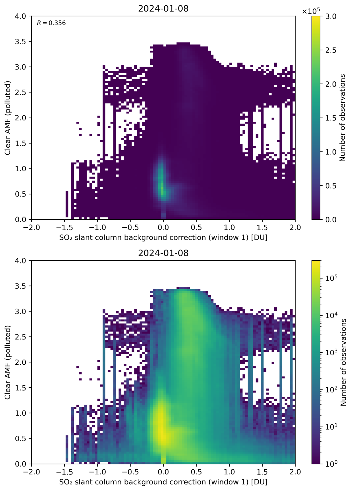
Figure 103: Scatter density plot of “SO 2 slant column background correction (window 1)” against “Clear AMF (polluted)” for 2024-01-07 to 2024-01-09.
