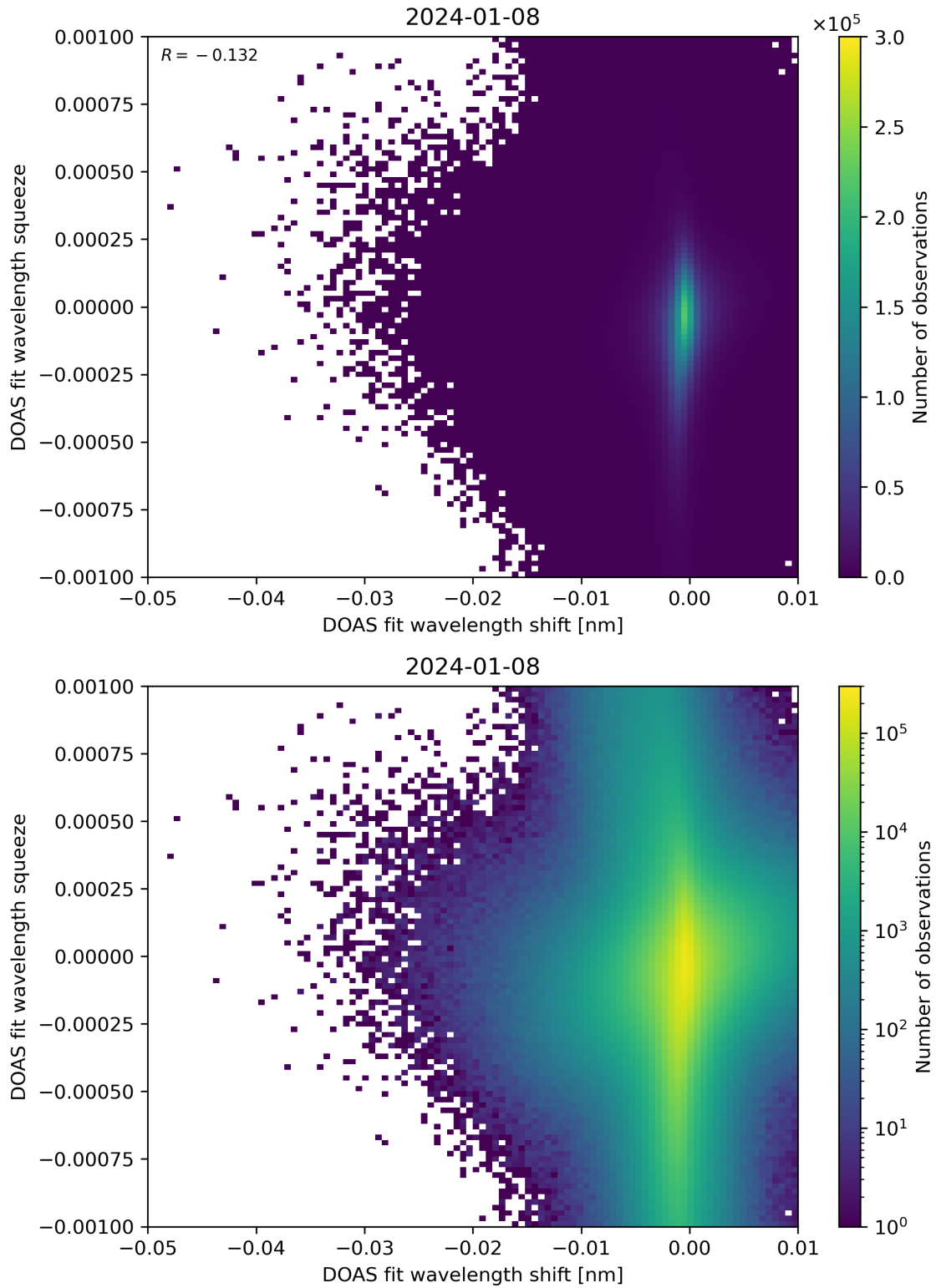
Figure 127: Scatter density plot of “DOAS fit wavelength shift” against “DOAS fit wavelength squeeze” for 2024-01-07 to 2024-01-09.
