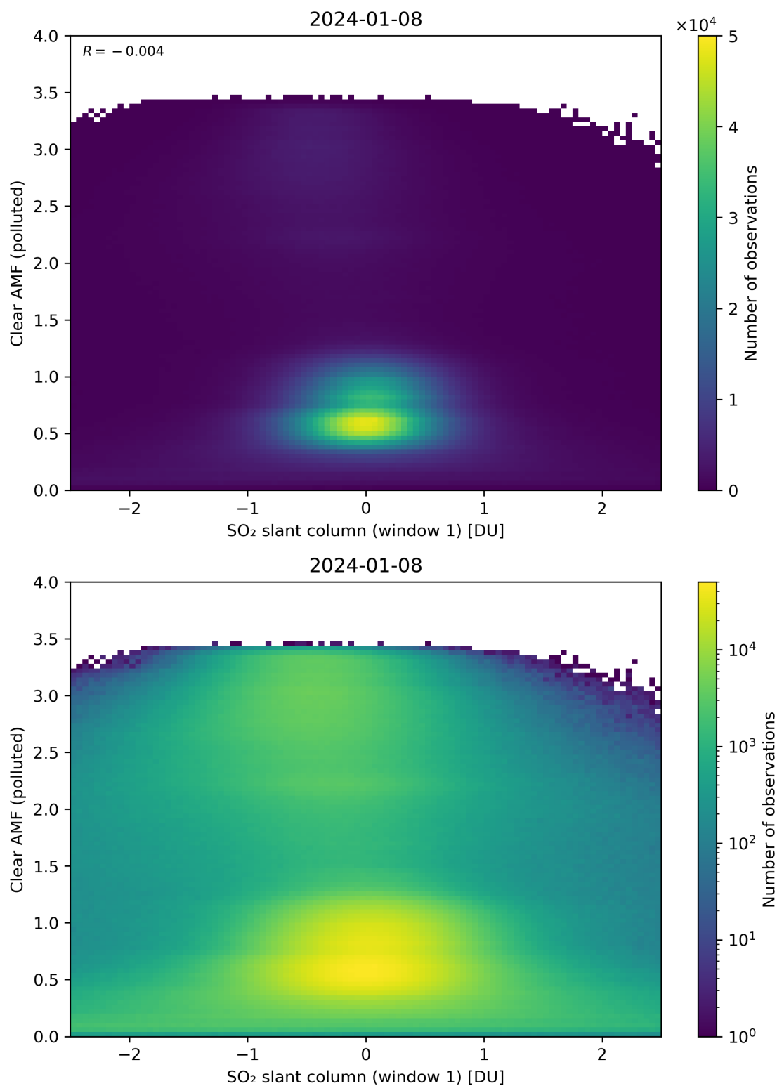
Figure 232: Scatter density plot of “SO 2 slant column (window 1)” against “Clear AMF (polluted)” for 2024-01-07 to 2024-01-09.
