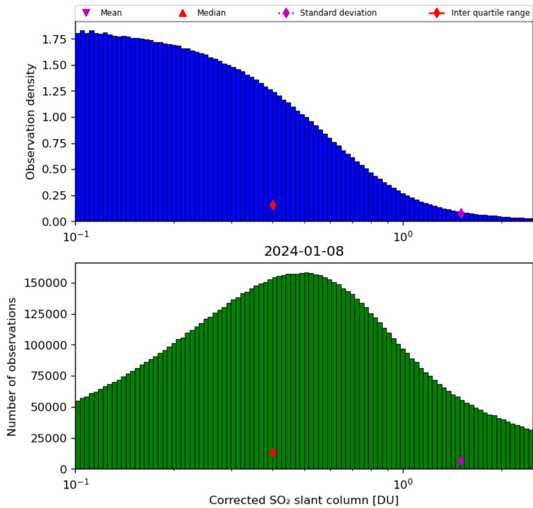
Figure 55: Histogram of “Corrected SO 2 slant column” for 2024-01-07 to 2024-01-09
