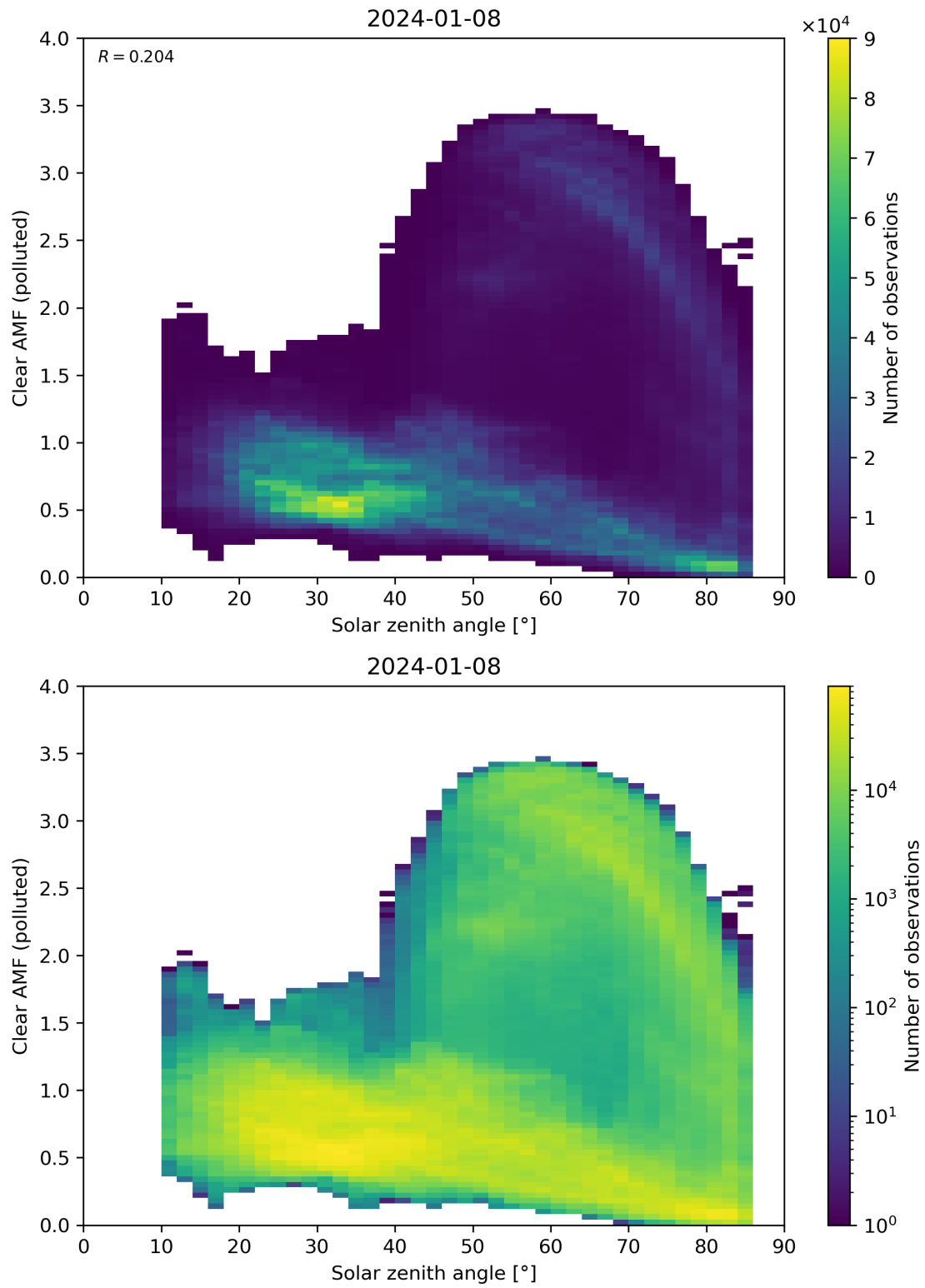
Figure 165: Scatter density plot of “Solar zenith angle” against “Clear AMF (polluted)” for 2024-01-07 to 2024-01-09.
