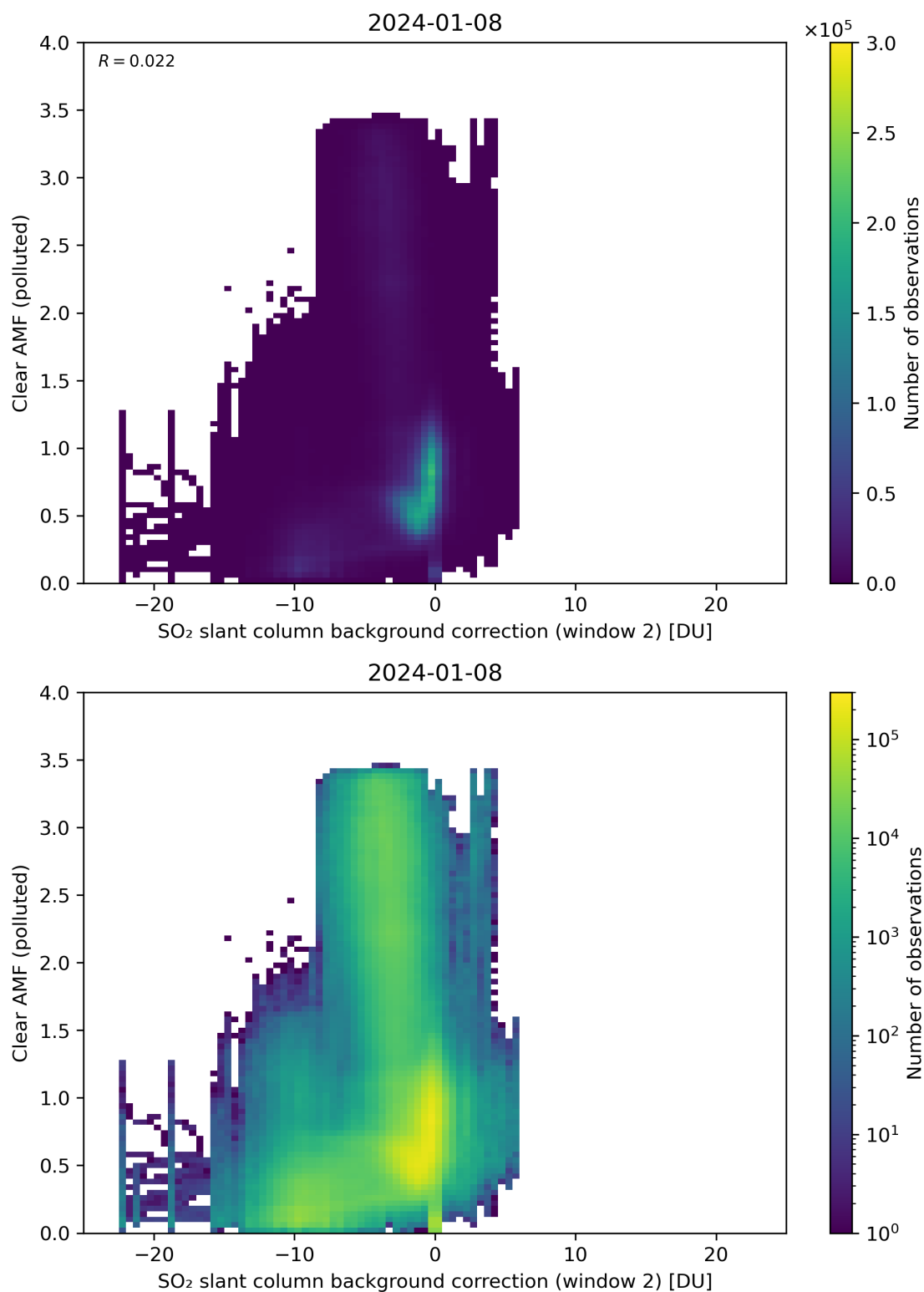
Figure 115: Scatter density plot of “SO 2 slant column background correction (window 2)” against “Clear AMF (polluted)” for 2024-01-07 to 2024-01-09.
