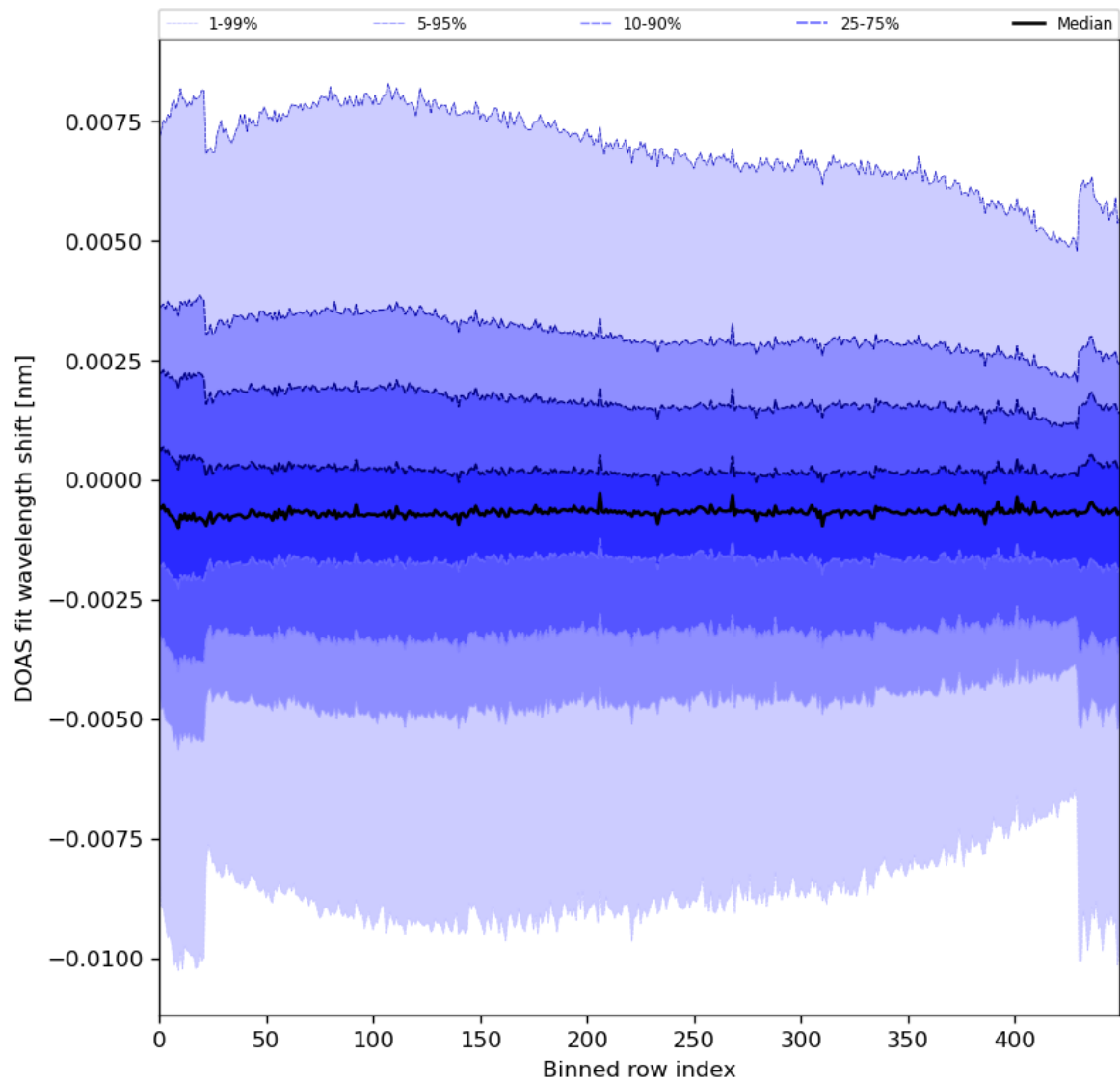
Figure 91: Along track statistics of “DOAS fit wavelength shift” for 2024-01-07 to 2024-01-09
