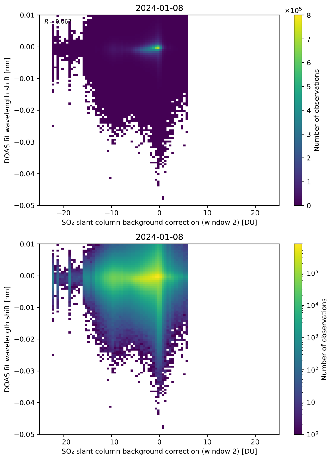
Figure 112: Scatter density plot of “SO 2 slant column background correction (window 2)” against “DOAS fit wavelength shift” for 2024-01-07 to 2024-01-09.
