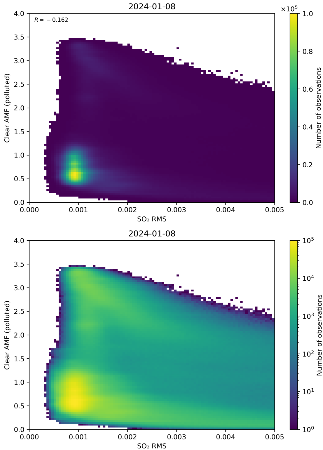
Figure 136: Scatter density plot of “SO 2 RMS” against “Clear AMF (polluted)” for 2024-01-07 to 2024-01-09.
