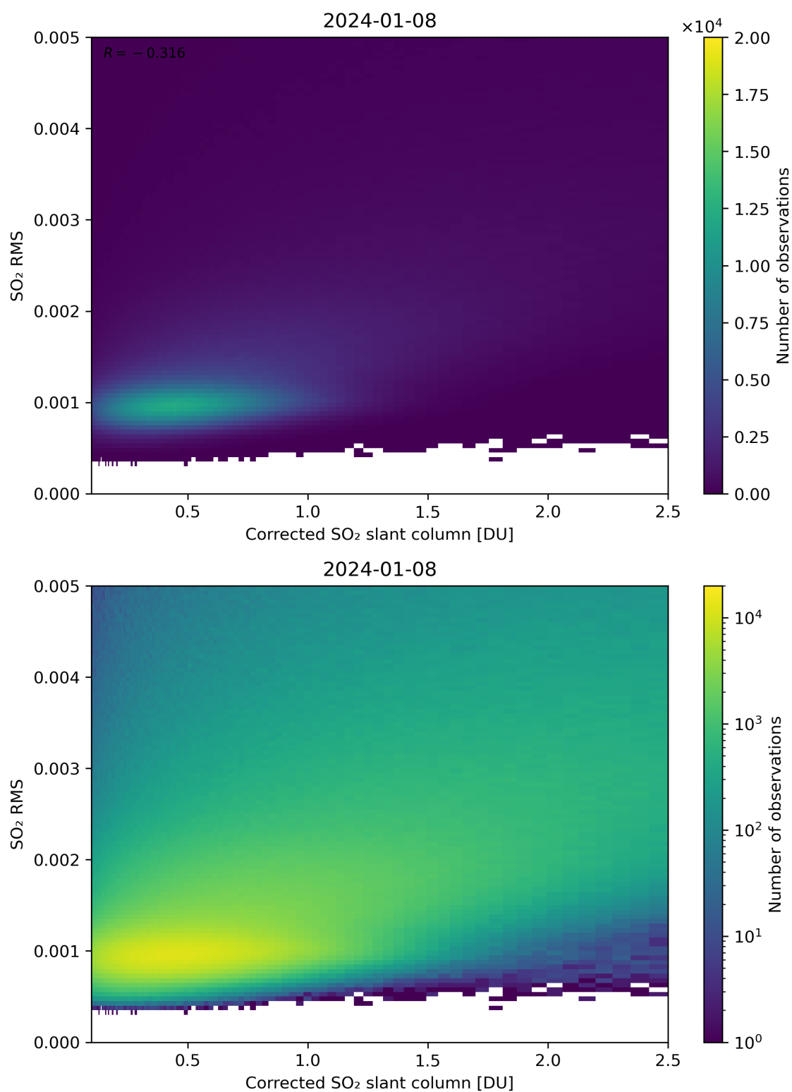
Figure 183: Scatter density plot of “Corrected SO 2 slant column” against “SO 2 RMS” for 2024-01-07 to 2024-01-09.
