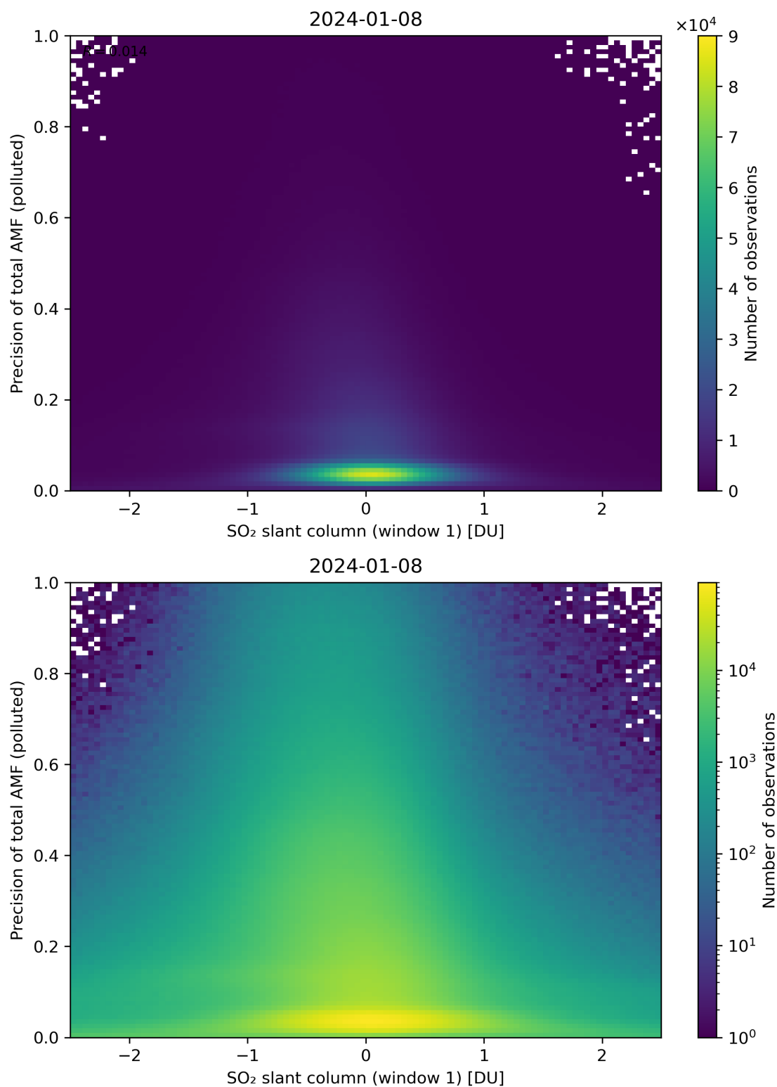
Figure 240: Scatter density plot of “SO 2 slant column (window 1)” against “Precision of total AMF (polluted)” for 2024-01-07 to 2024-01-09.
