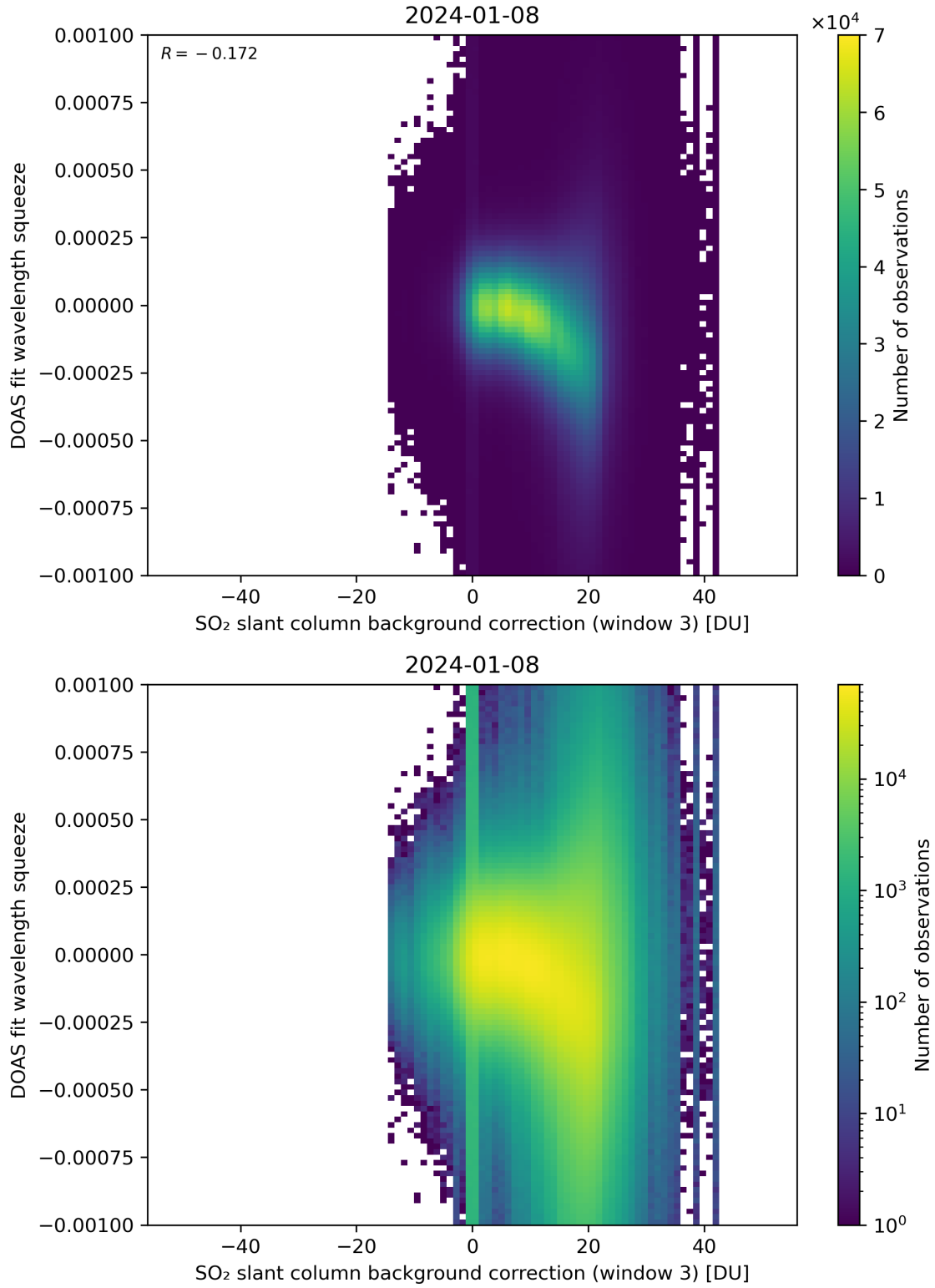
Figure 122: Scatter density plot of “SO 2 slant column background correction (window 3)” against “DOAS fit wavelength squeeze” for 2024-01-07 to 2024-01-09.
