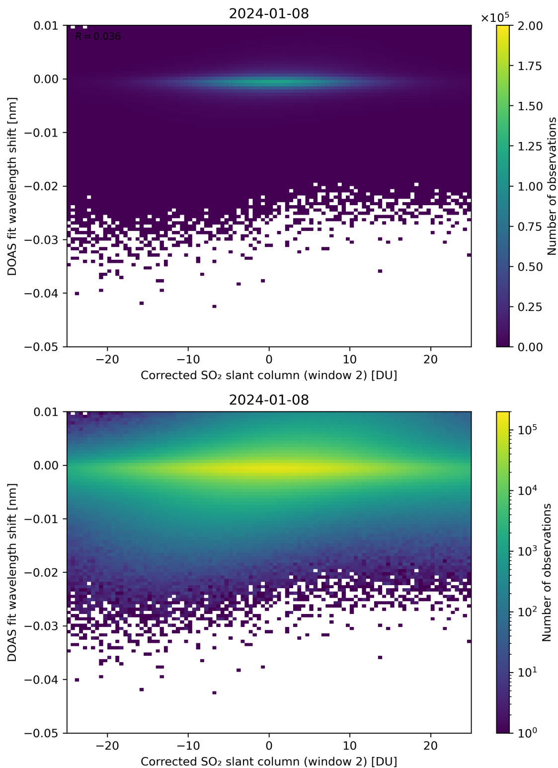
Figure 196: Scatter density plot of “Corrected SO 2 slant column (window 2)” against “DOAS fit wavelength shift” for 2024-01-07 to 2024-01-09.
