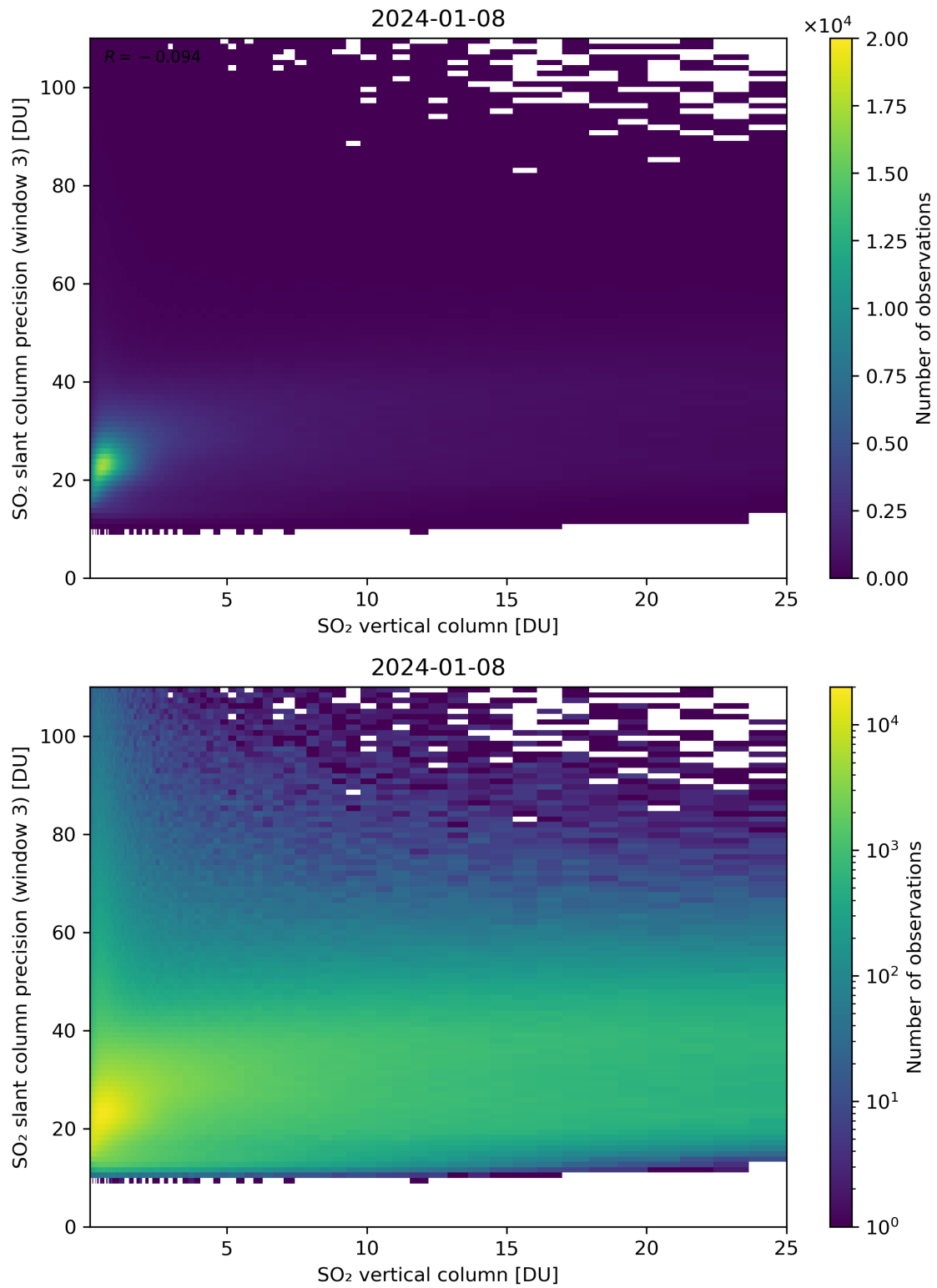
Figure 304: Scatter density plot of “SO 2 vertical column” against “SO 2 slant column precision (window 3)” for 2024-01-07 to 2024-01-09.
