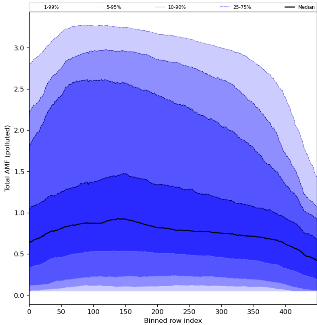
Figure 94: Along track statistics of “Total AMF (polluted)” for 2024-01-07 to 2024-01-09
