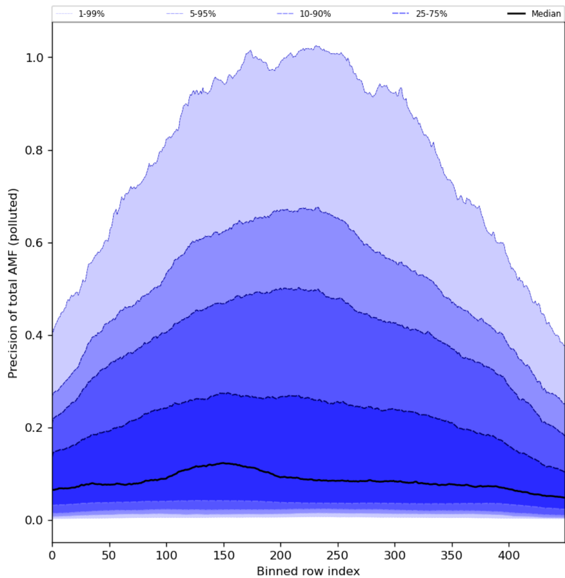
Figure 95: Along track statistics of “Precision of total AMF (polluted)” for 2024-01-07 to 2024-01-09
