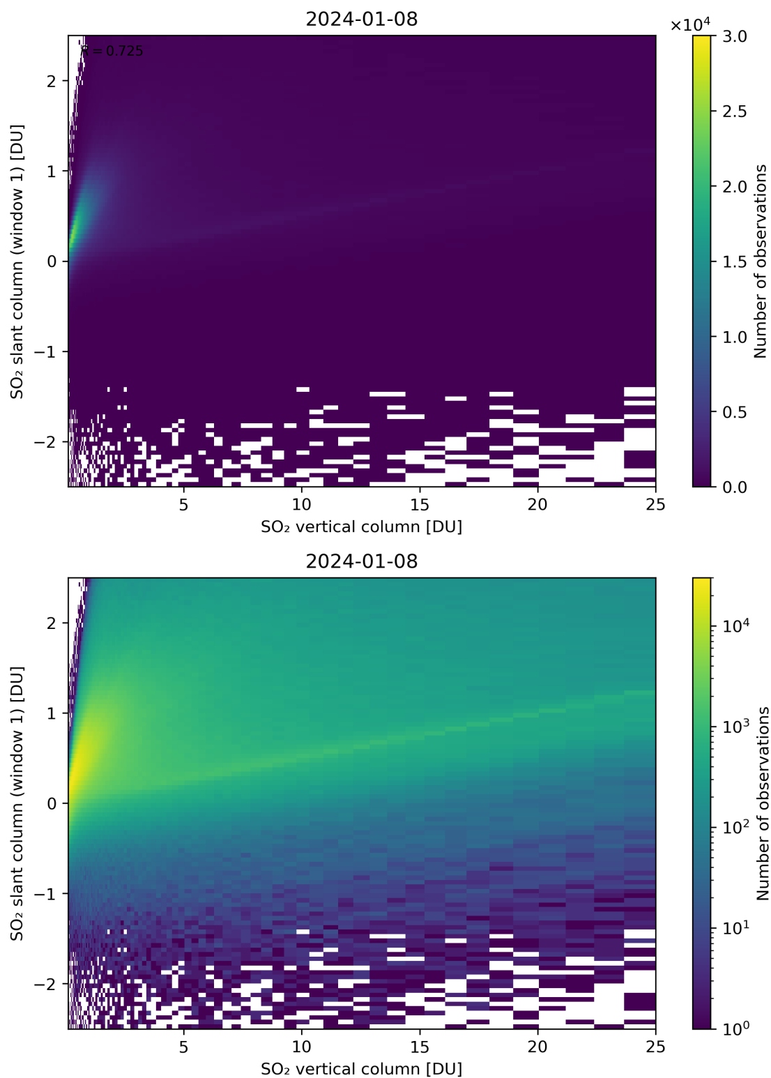
Figure 300: Scatter density plot of “SO 2 vertical column” against “SO 2 slant column (window 1)” for 2024-01-07 to 2024-01-09.
