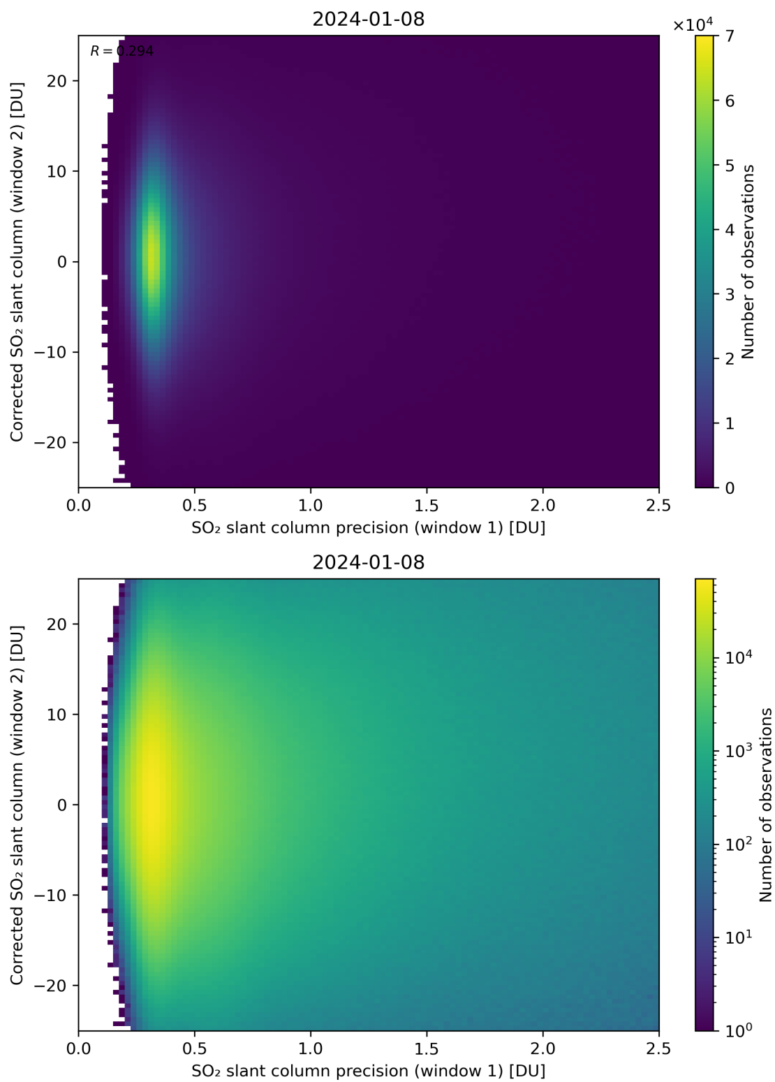
Figure 225: Scatter density plot of “SO 2 slant column precision (window 1)” against “Corrected SO 2 slant column (window 2)” for 2024-01-07 to 2024-01-09.
