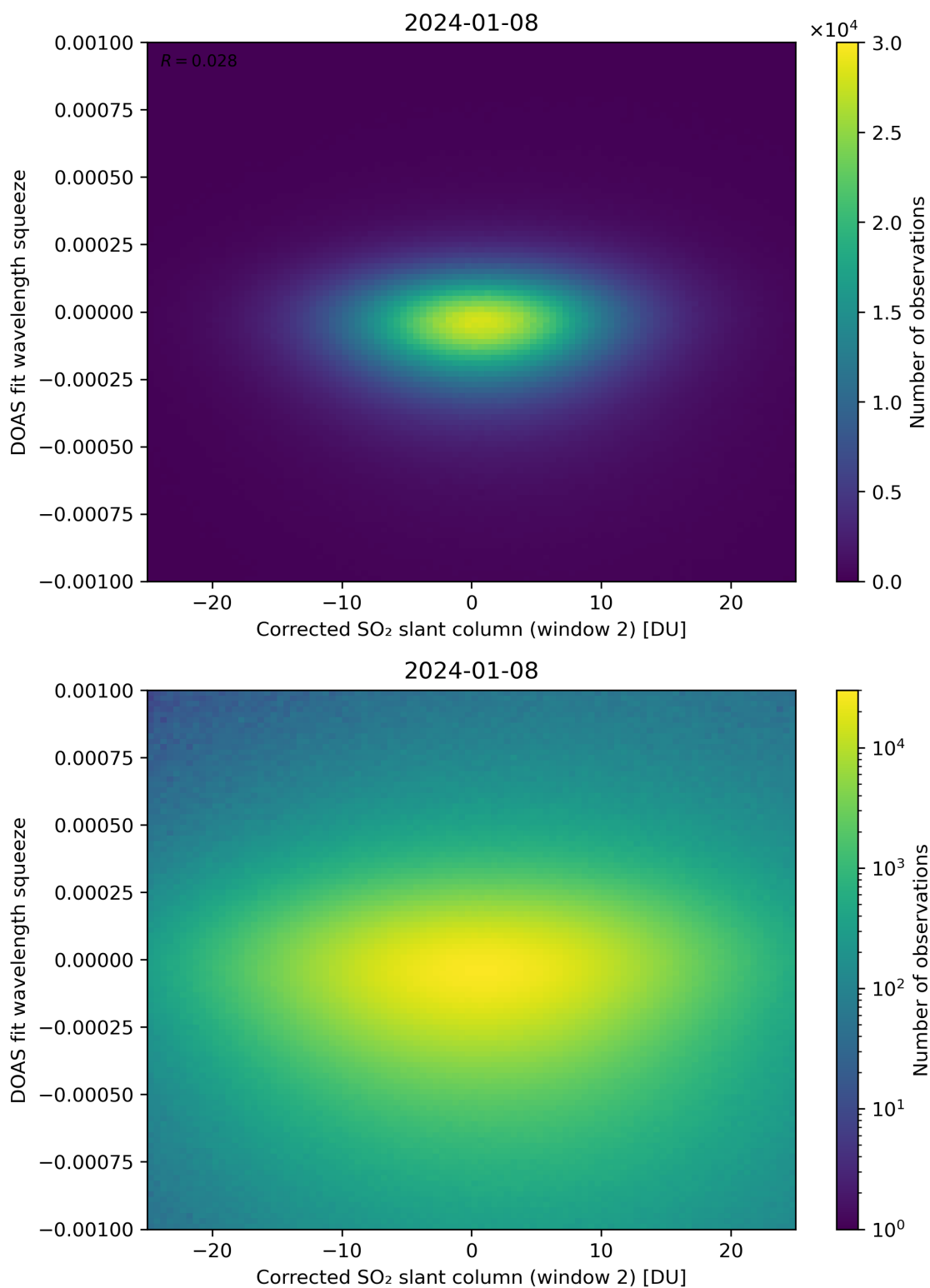
Figure 197: Scatter density plot of “Corrected SO 2 slant column (window 2)” against “DOAS fit wavelength squeeze” for 2024-01-07 to 2024-01-09.
