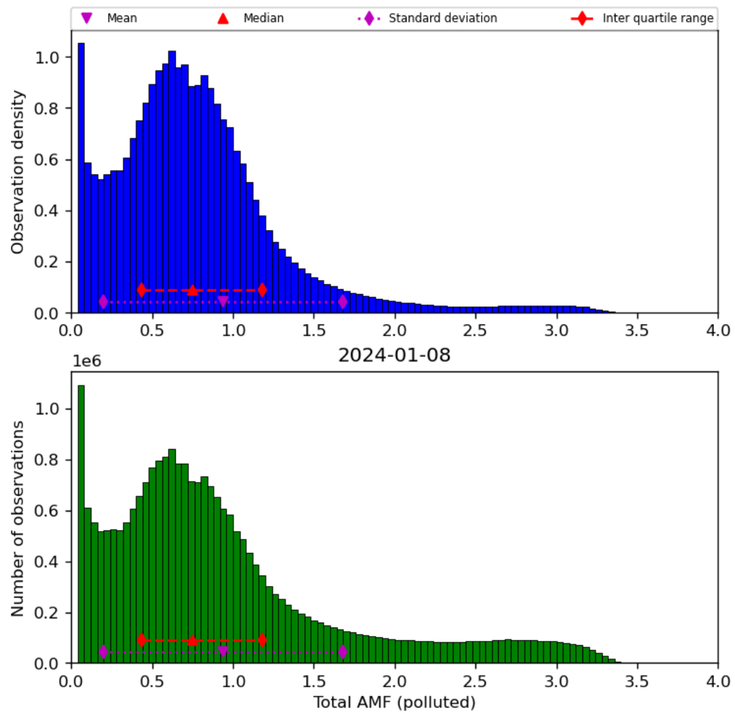
Figure 71: Histogram of “Total AMF (polluted)” for 2024-01-07 to 2024-01-09
