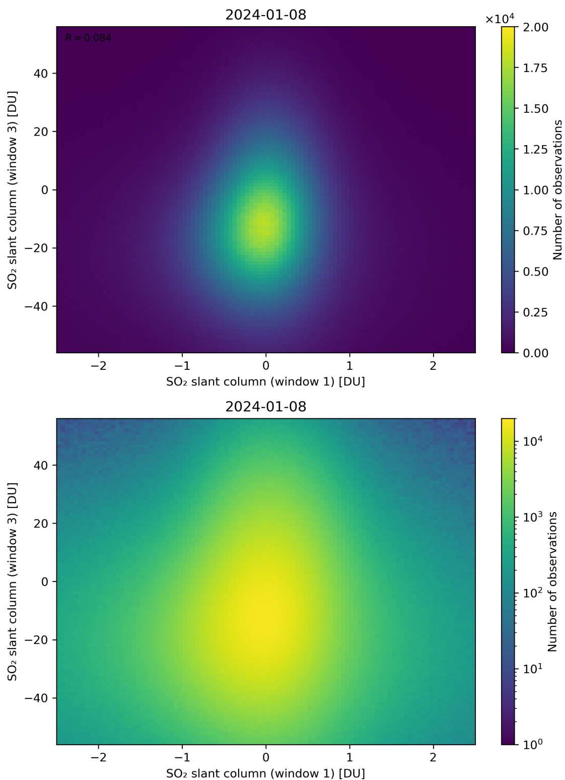
Figure 237: Scatter density plot of “SO 2 slant column (window 1)” against “SO 2 slant column (window 3)” for 2024-01-07 to 2024-01-09.
