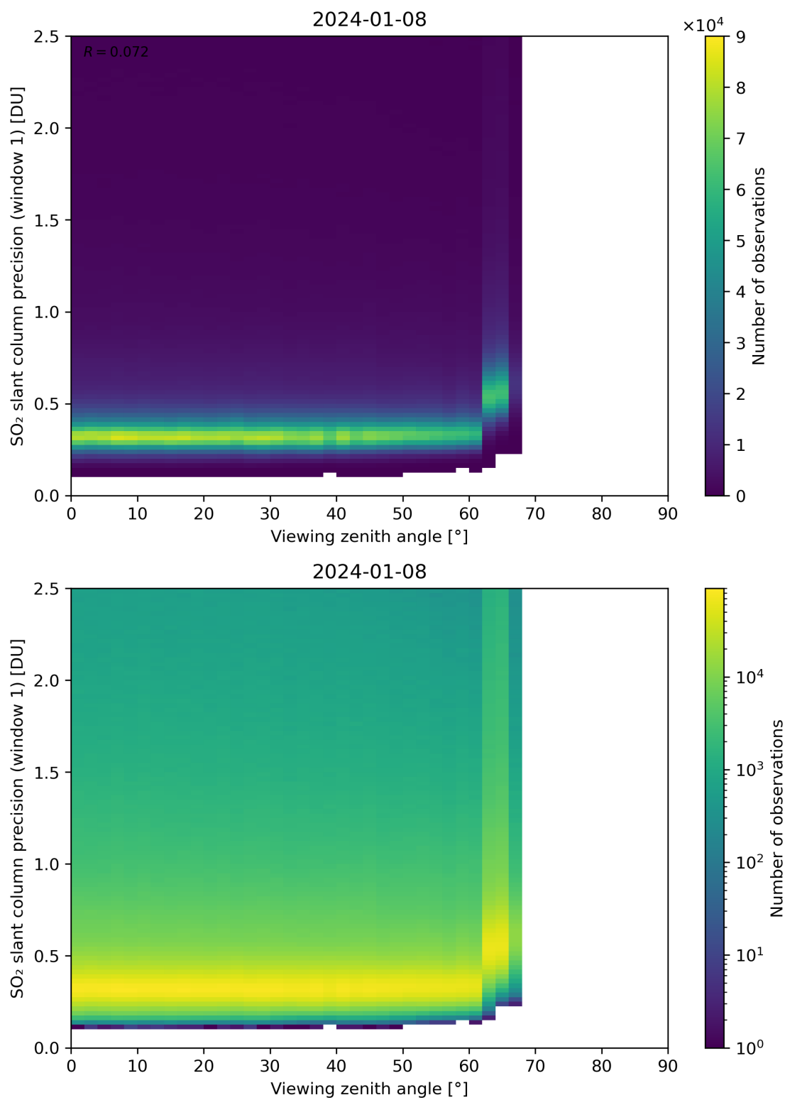
Figure 321: Scatter density plot of “Viewing zenith angle” against “SO 2 slant column precision (window 1)” for 2024-01-07 to 2024-01-09.
