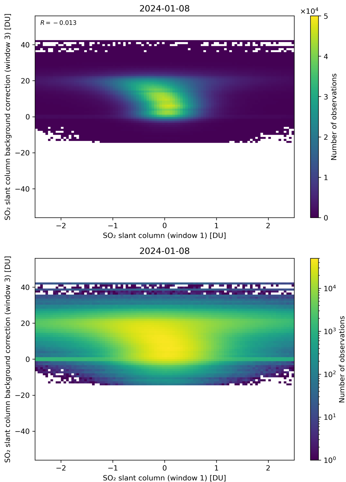
Figure 214: Scatter density plot of “SO 2 slant column (window 1)” against “SO 2 slant column background correction (window 3)” for 2024-01-07 to 2024-01-09.
