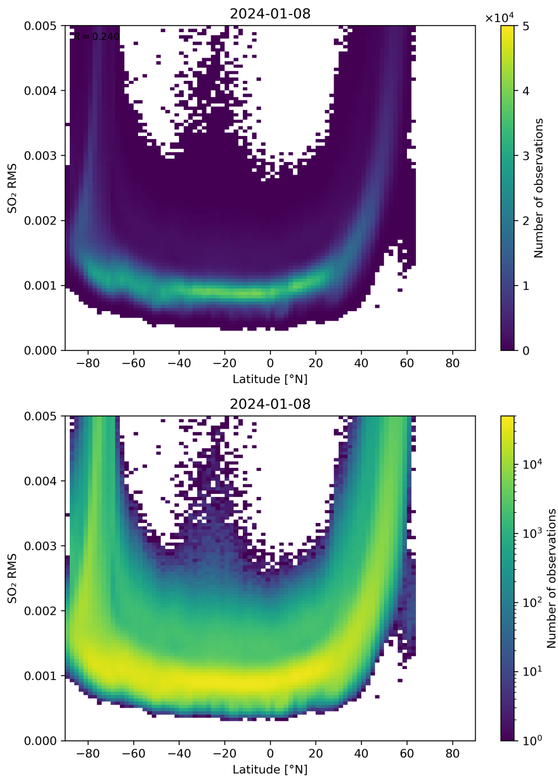
Figure 144: Scatter density plot of “Latitude” against “SO 2 RMS” for 2024-01-07 to 2024-01-09.
