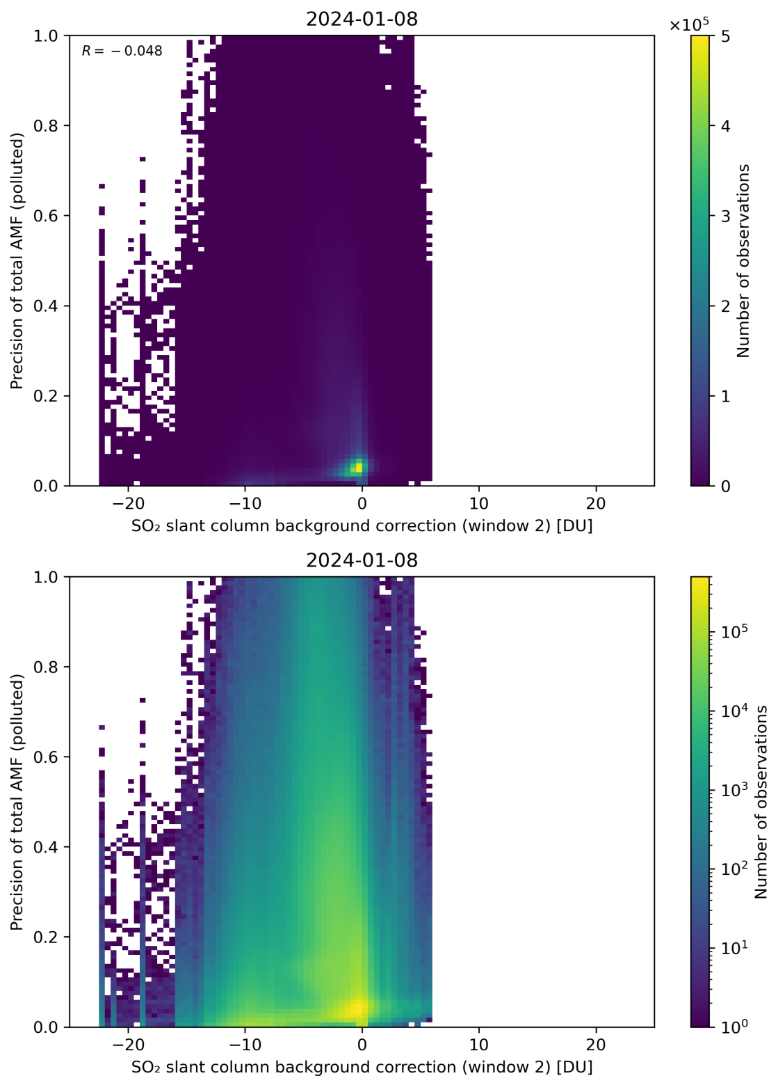
Figure 120: Scatter density plot of “SO 2 slant column background correction (window 2)” against “Precision of total AMF (polluted)” for 2024-01-07 to 2024-01-09.
