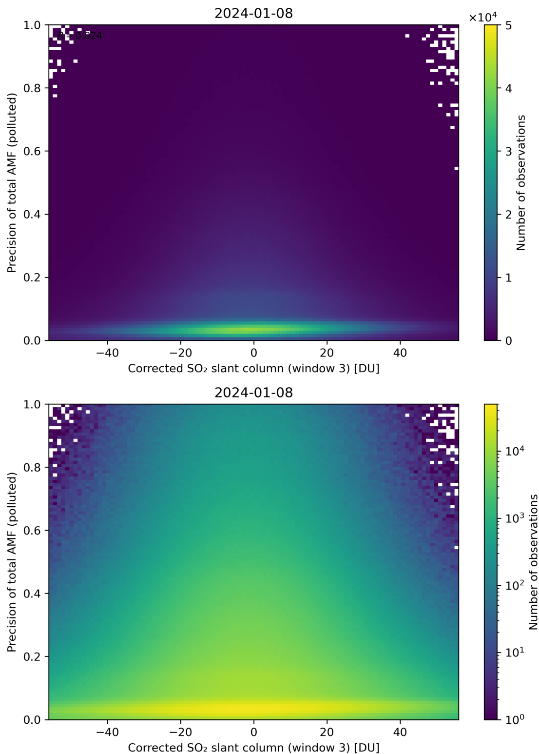
Figure 211: Scatter density plot of “Corrected SO 2 slant column (window 3)” against “Precision of total AMF (polluted)” for 2024-01-07 to 2024-01-09.
