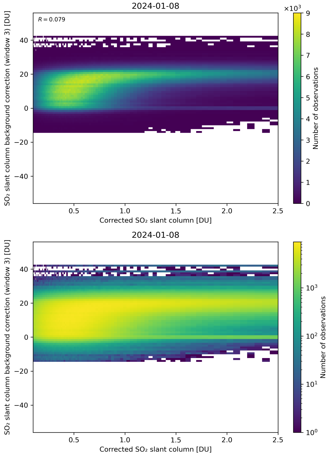
Figure 180: Scatter density plot of “Corrected SO 2 slant column” against “SO 2 slant column background correction (window 3)” for 2024-01-07 to 2024-01-09.
