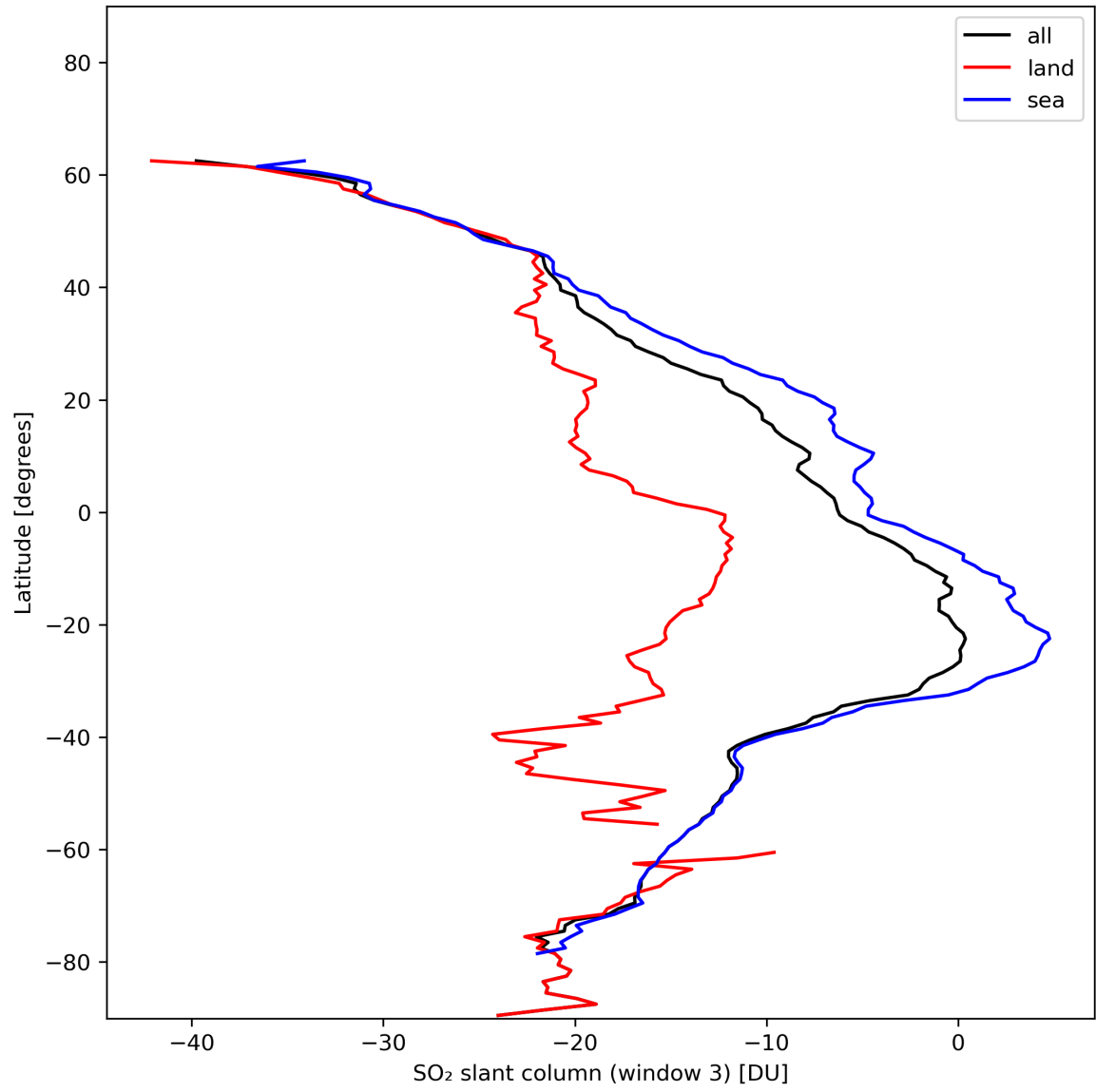
Figure 41: Zonal average of “SO 2 slant column (window 3)” for 2024-01-07 to 2024-01-09.
