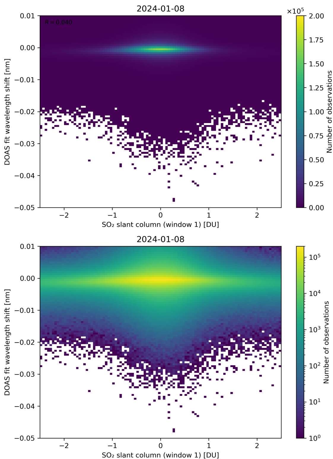
Figure 215: Scatter density plot of “SO 2 slant column (window 1)” against “DOAS fit wavelength shift” for 2024-01-07 to 2024-01-09.
