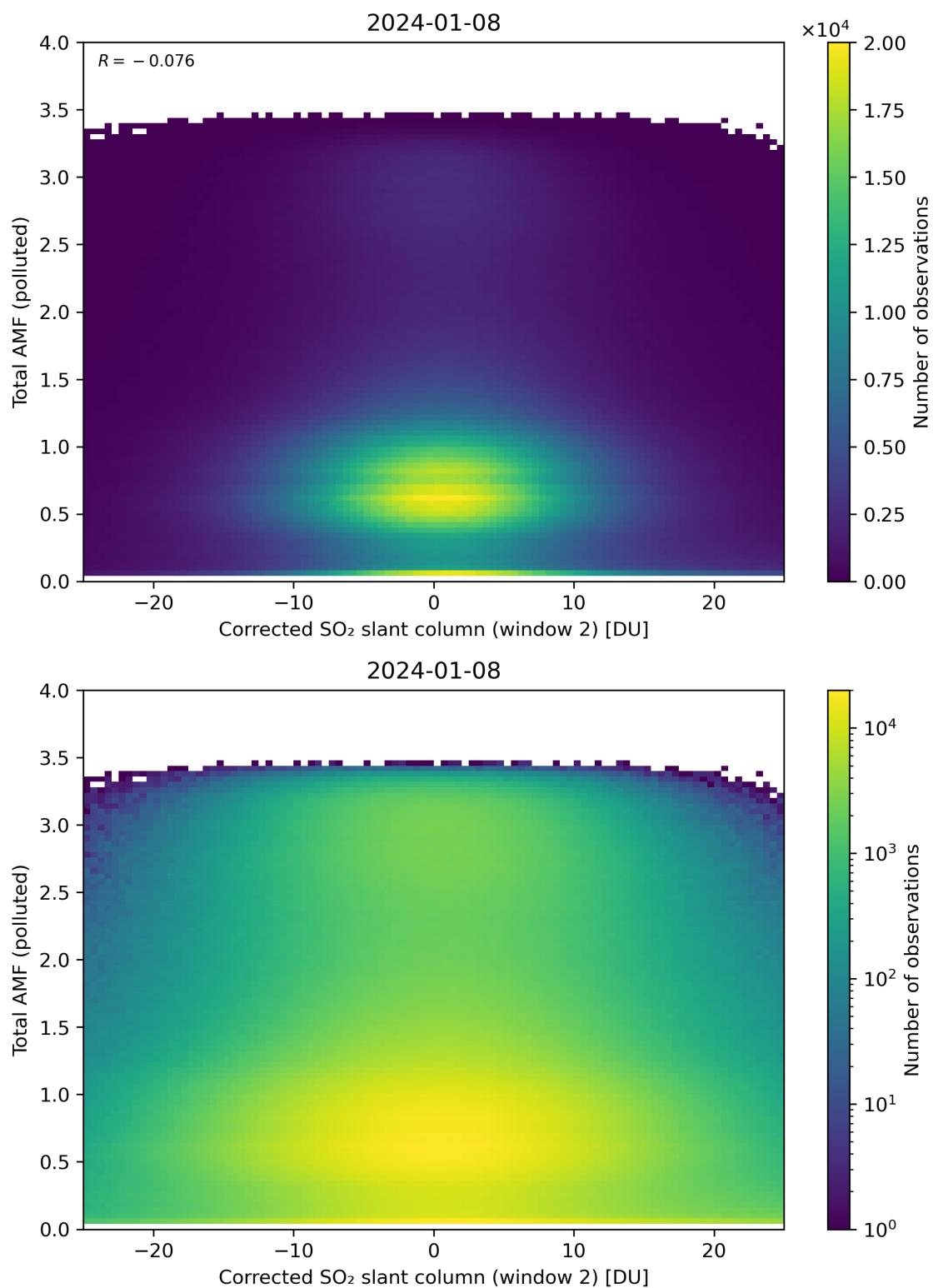
Figure 203: Scatter density plot of “Corrected SO 2 slant column (window 2)” against “Total AMF (polluted)” for 2024-01-07 to 2024-01-09.
