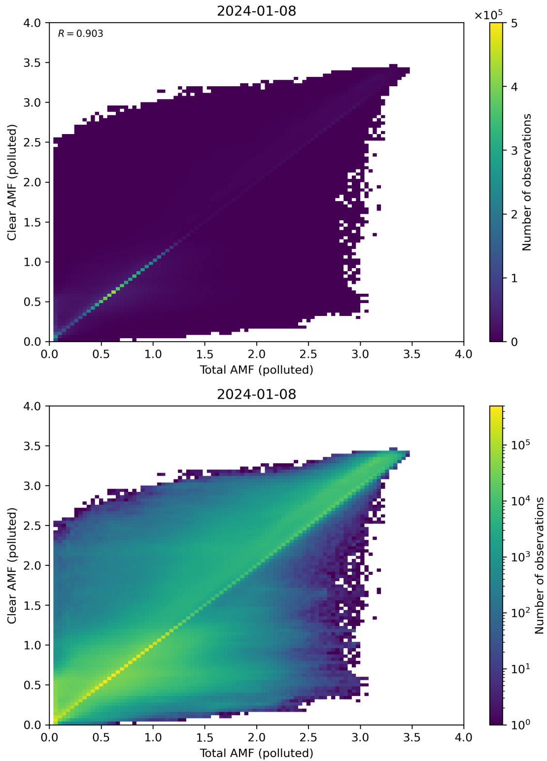
Figure 271: Scatter density plot of “Total AMF (polluted)” against “Clear AMF (polluted)” for 2024-01-07 to 2024-01-09.
