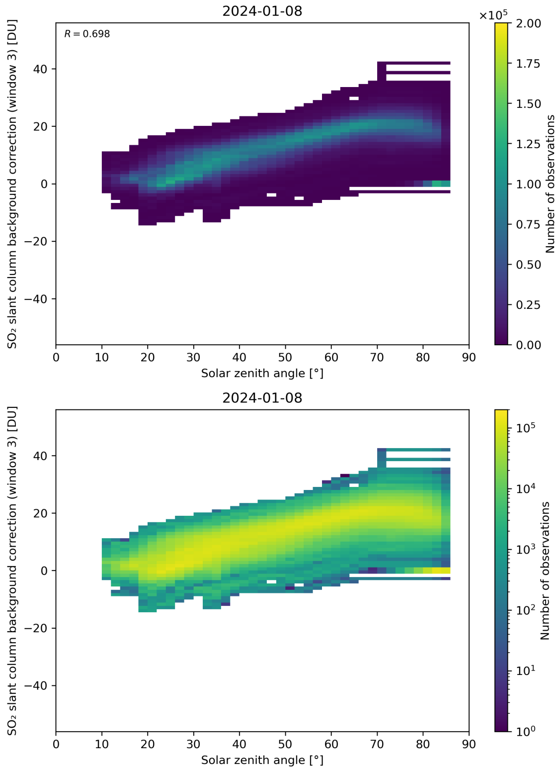
Figure 160: Scatter density plot of “Solar zenith angle” against “SO 2 slant column background correction (window 3)” for 2024-01-07 to 2024-01-09.
