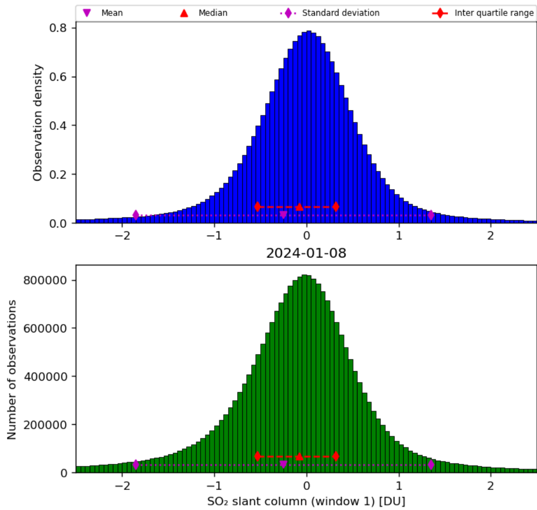
Figure 56: Histogram of “SO 2 slant column (window 1)” for 2024-01-07 to 2024-01-09
