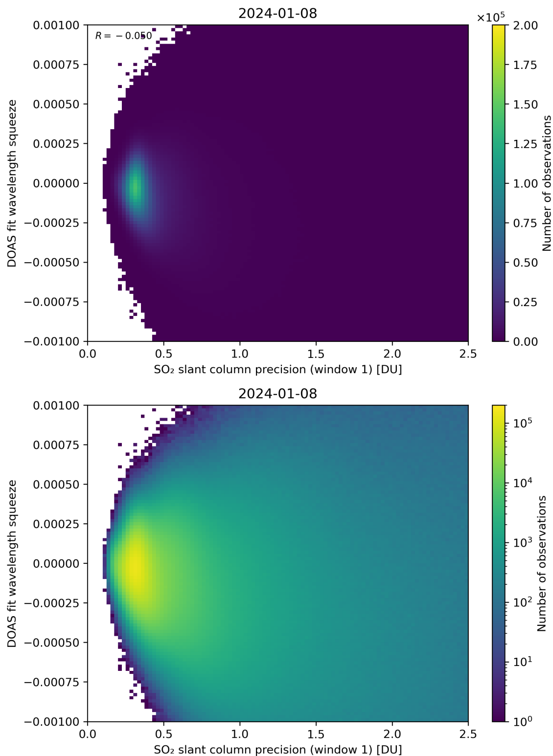
Figure 222: Scatter density plot of “SO 2 slant column precision (window 1)” against “DOAS fit wavelength squeeze” for 2024-01-07 to 2024-01-09.
