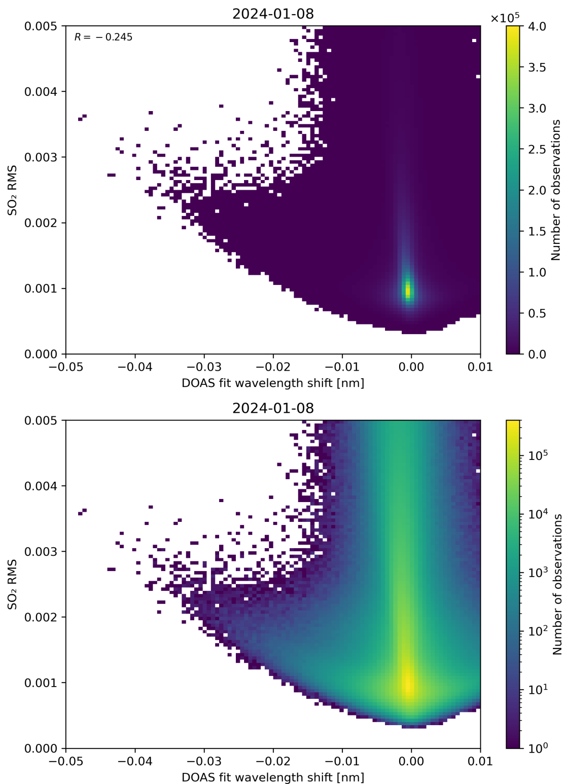
Figure 128: Scatter density plot of “DOAS fit wavelength shift” against “SO 2 RMS” for 2024-01-07 to 2024-01-09.
