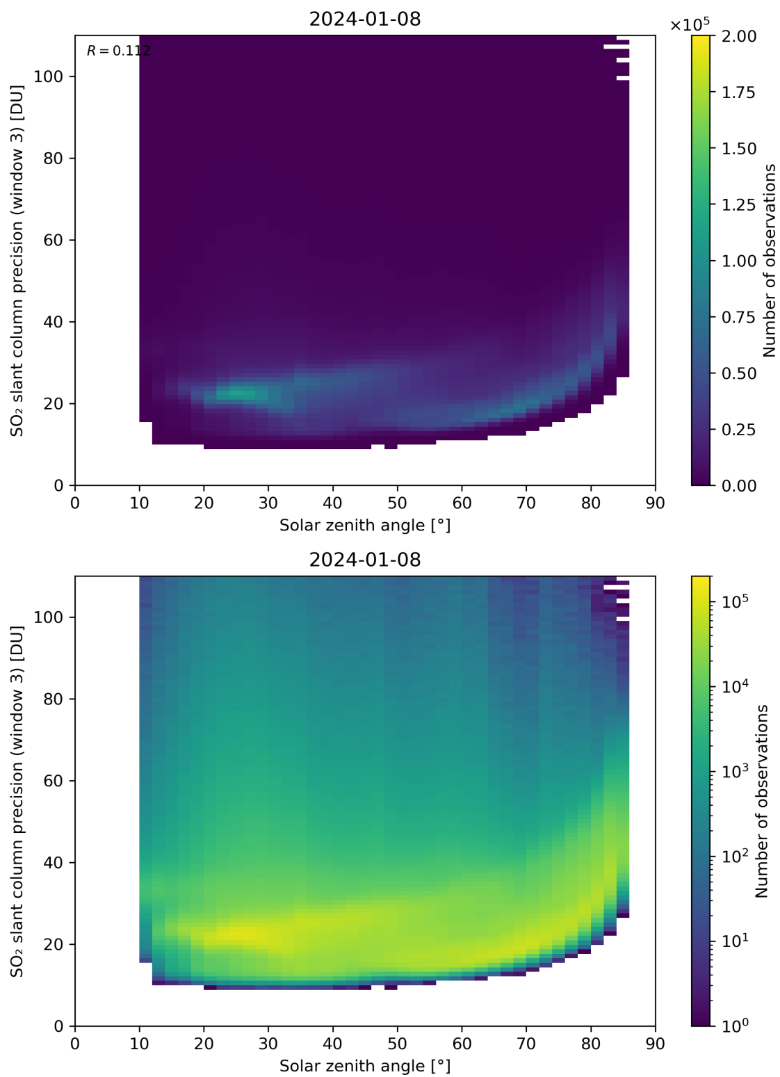
Figure 173: Scatter density plot of “Solar zenith angle” against “SO 2 slant column precision (window 3)” for 2024-01-07 to 2024-01-09.
