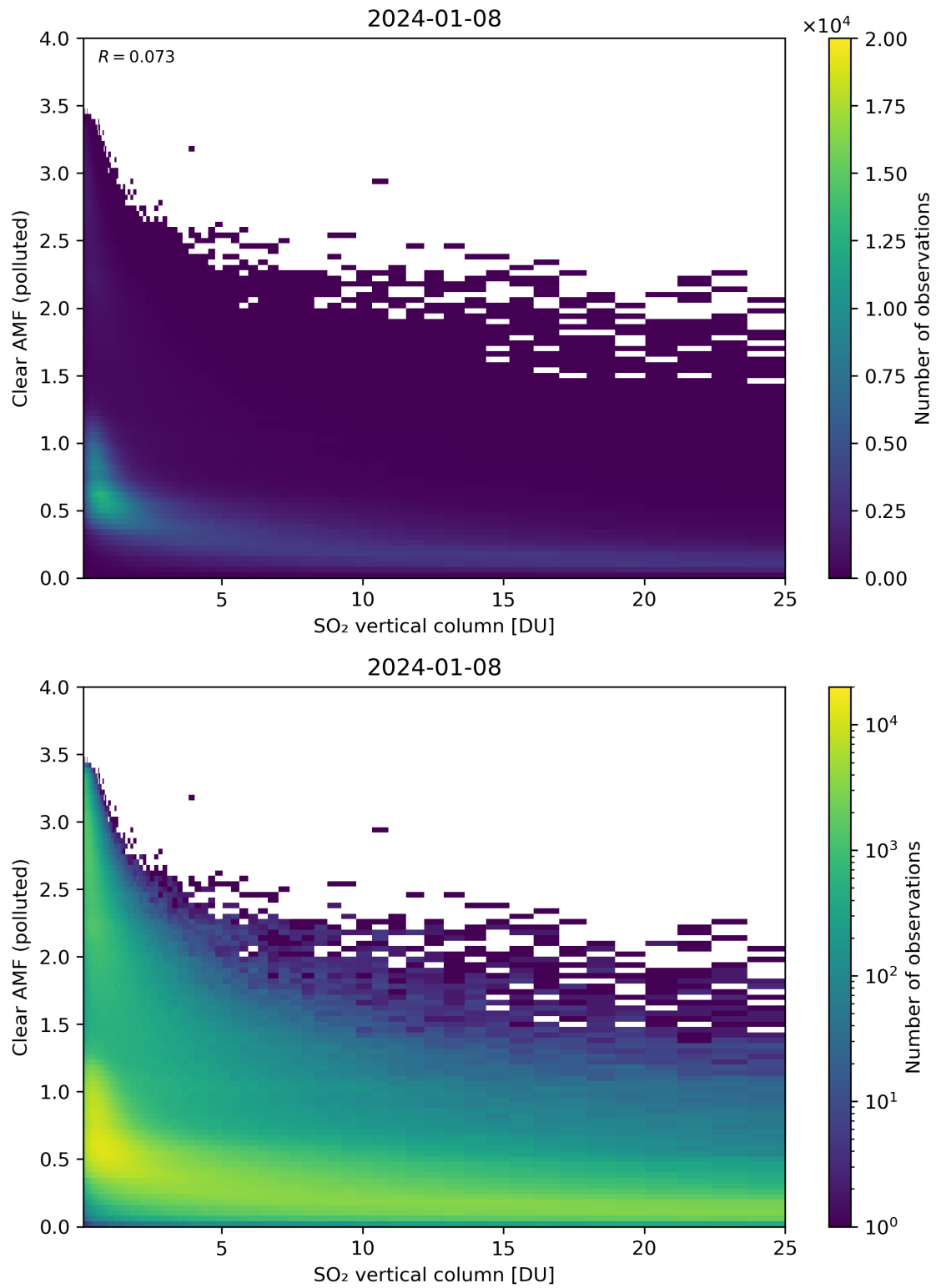
Figure 296: Scatter density plot of “SO 2 vertical column” against “Clear AMF (polluted)” for 2024-01-07 to 2024-01-09.
