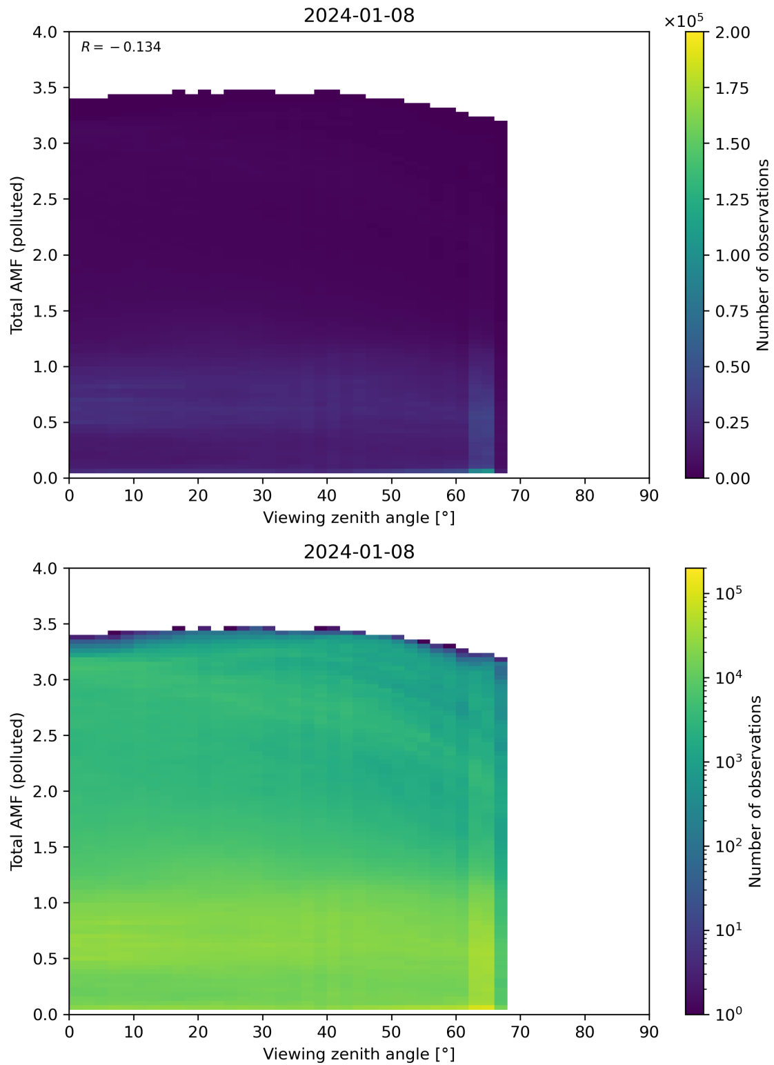
Figure 325: Scatter density plot of “Viewing zenith angle” against “Total AMF (polluted)” for 2024-01-07 to 2024-01-09.
