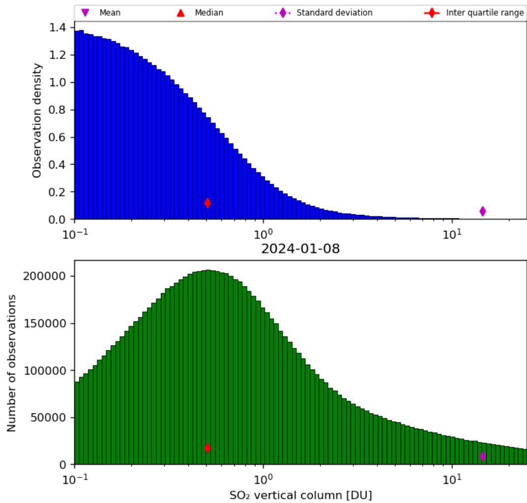
Figure 53: Histogram of “SO 2 vertical column” for 2024-01-07 to 2024-01-09
