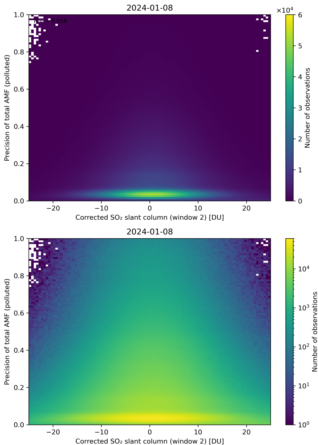
Figure 204: Scatter density plot of “Corrected SO 2 slant column (window 2)” against “Precision of total AMF (polluted)” for 2024-01-07 to 2024-01-09.
