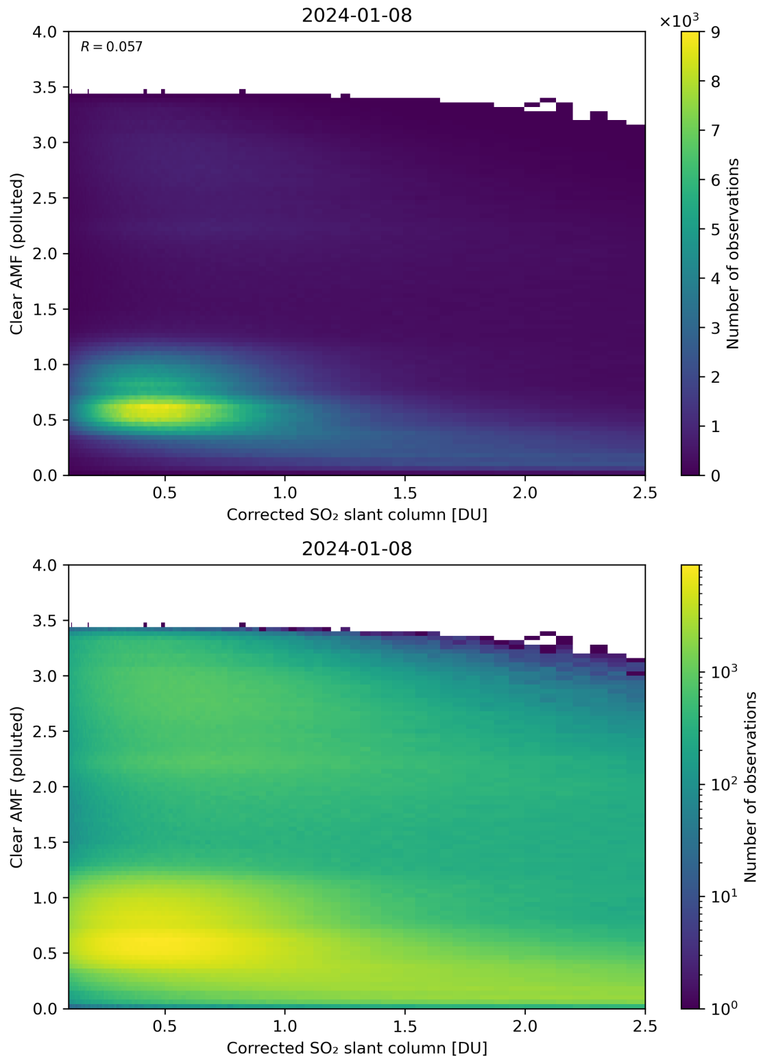
Figure 184: Scatter density plot of “Corrected SO 2 slant column” against “Clear AMF (polluted)” for 2024-01-07 to 2024-01-09.
