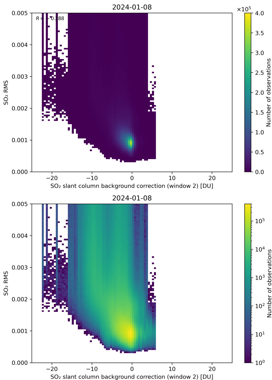
Figure 114: Scatter density plot of “SO 2 slant column background correction (window 2)” against “SO 2 RMS” for 2024-01-07 to 2024-01-09.
