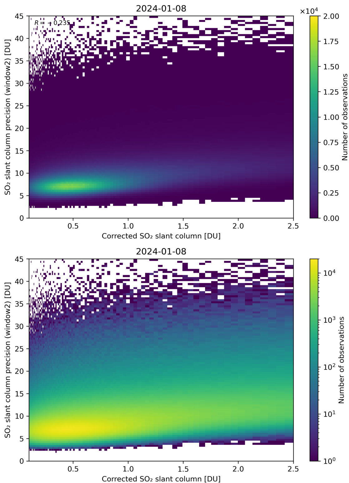
Figure 189: Scatter density plot of “Corrected SO 2 slant column” against “SO 2 slant column precision (window2)” for 2024-01-07 to 2024-01-09.
