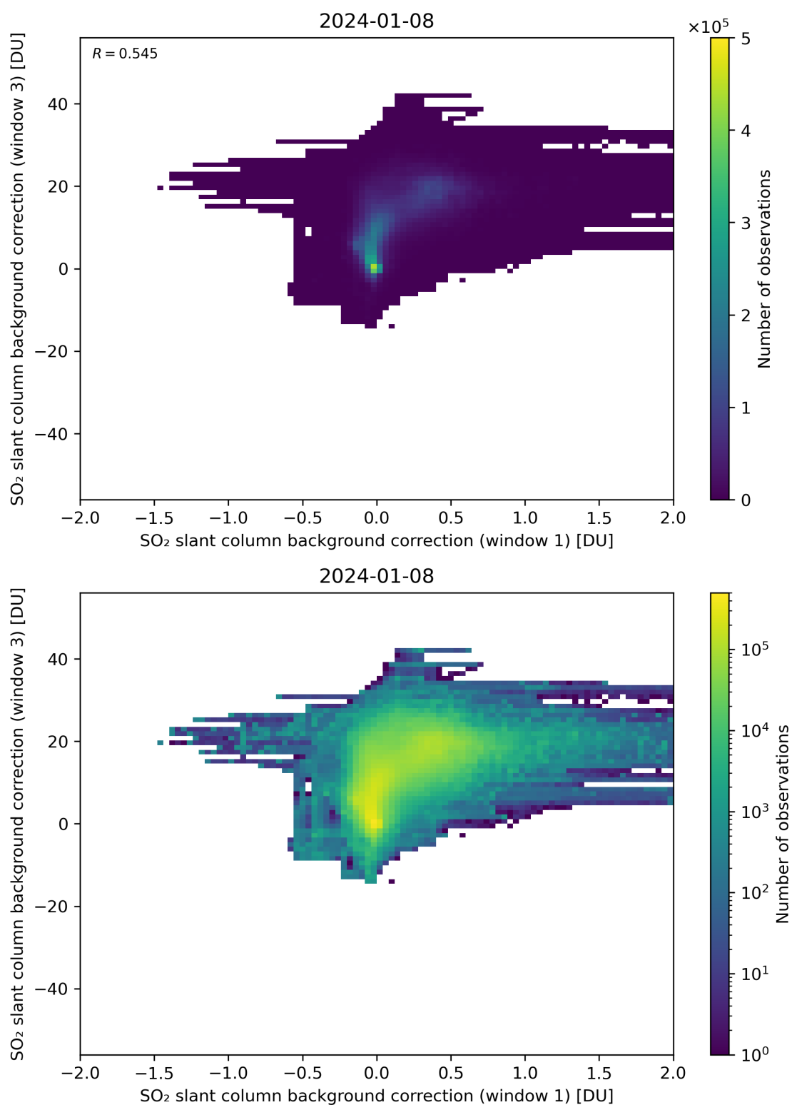
Figure 99: Scatter density plot of “SO 2 slant column background correction (window 1)” against “SO 2 slant column background correction (window 3)” for 2024-01-07 to 2024-01-09.
