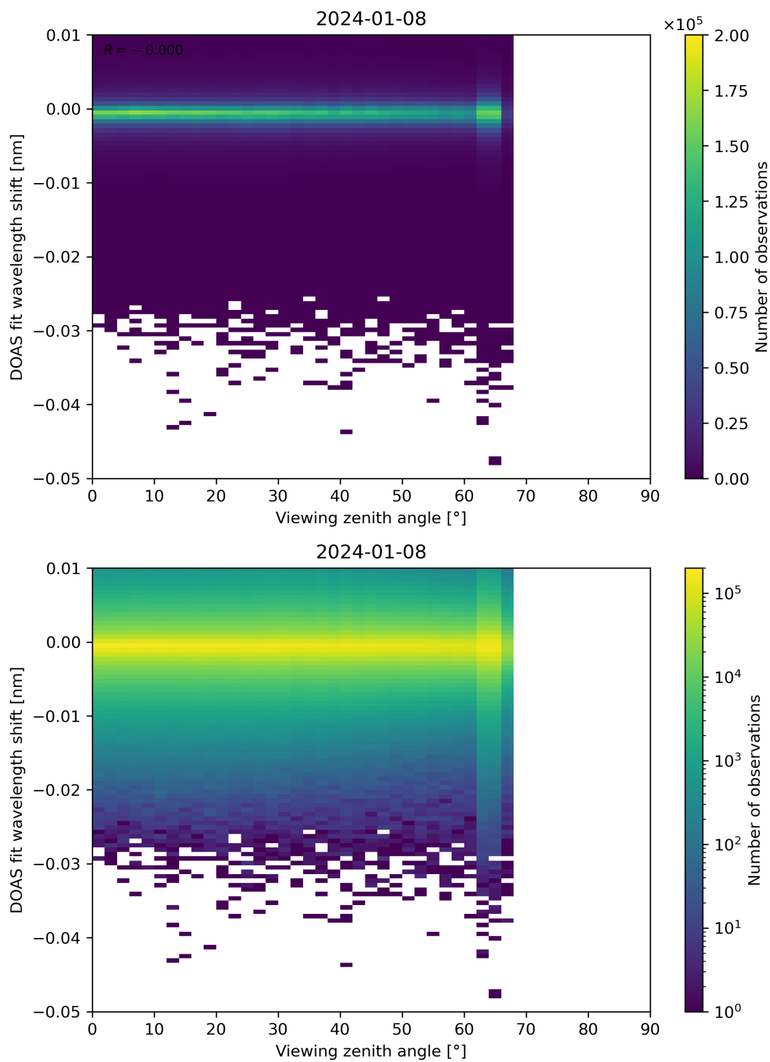
Figure 311: Scatter density plot of “Viewing zenith angle” against “DOAS fit wavelength shift” for 2024-01-07 to 2024-01-09.
