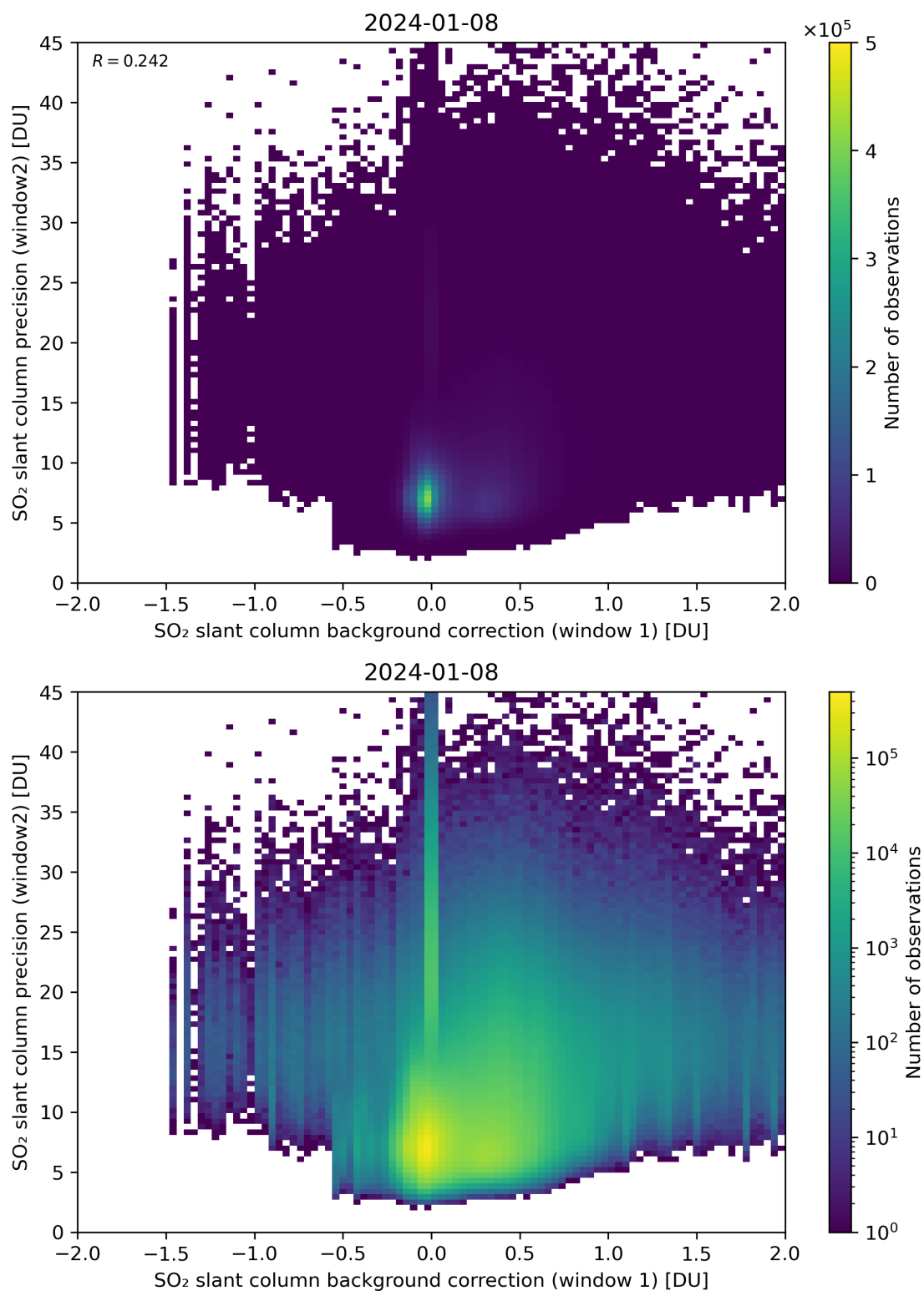
Figure 106: Scatter density plot of “SO 2 slant column background correction (window 1)” against “SO 2 slant column precision (window2)” for 2024-01-07 to 2024-01-09.
