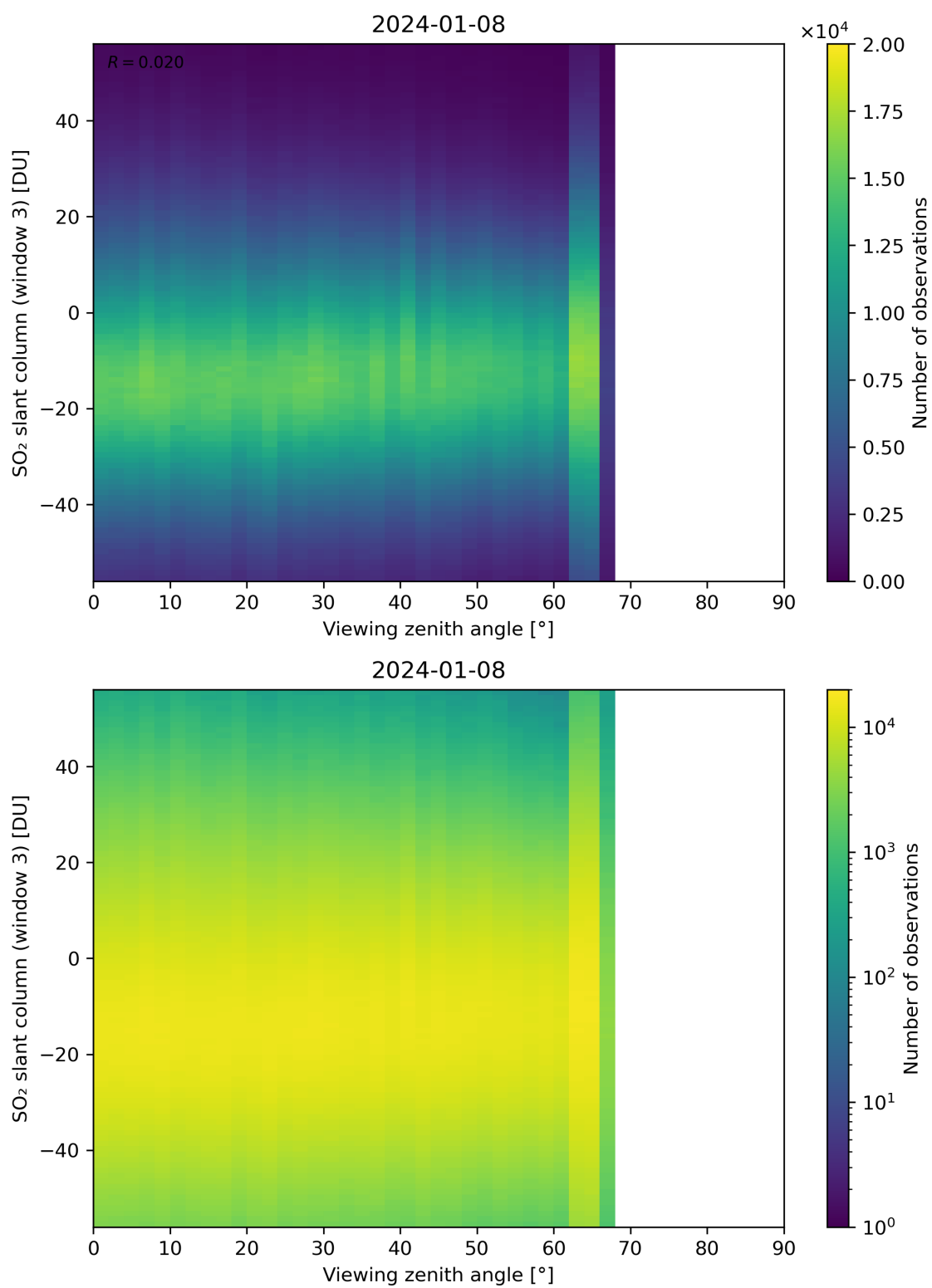
Figure 323: Scatter density plot of “Viewing zenith angle” against “SO 2 slant column (window 3)” for 2024-01-07 to 2024-01-09.
