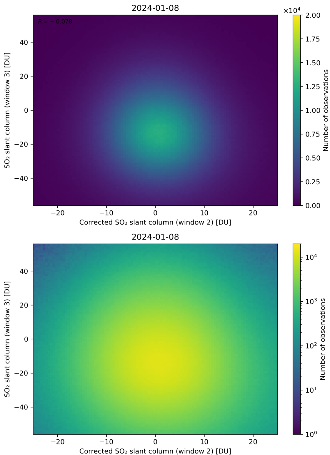
Figure 201: Scatter density plot of “Corrected SO 2 slant column (window 2)” against “SO 2 slant column (window 3)” for 2024-01-07 to 2024-01-09.
