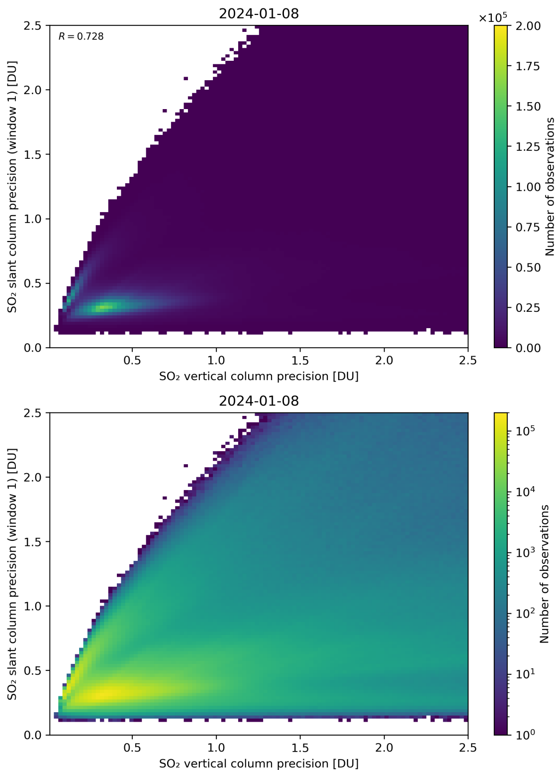
Figure 290: Scatter density plot of “SO 2 vertical column precision” against “SO 2 slant column precision (window 1)” for 2024-01-07 to 2024-01-09.
