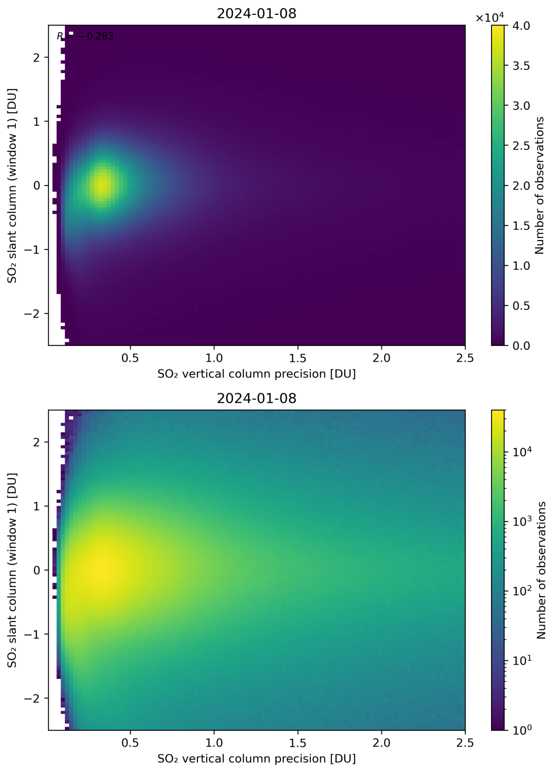
Figure 289: Scatter density plot of “SO 2 vertical column precision” against “SO 2 slant column (window 1)” for 2024-01-07 to 2024-01-09.
