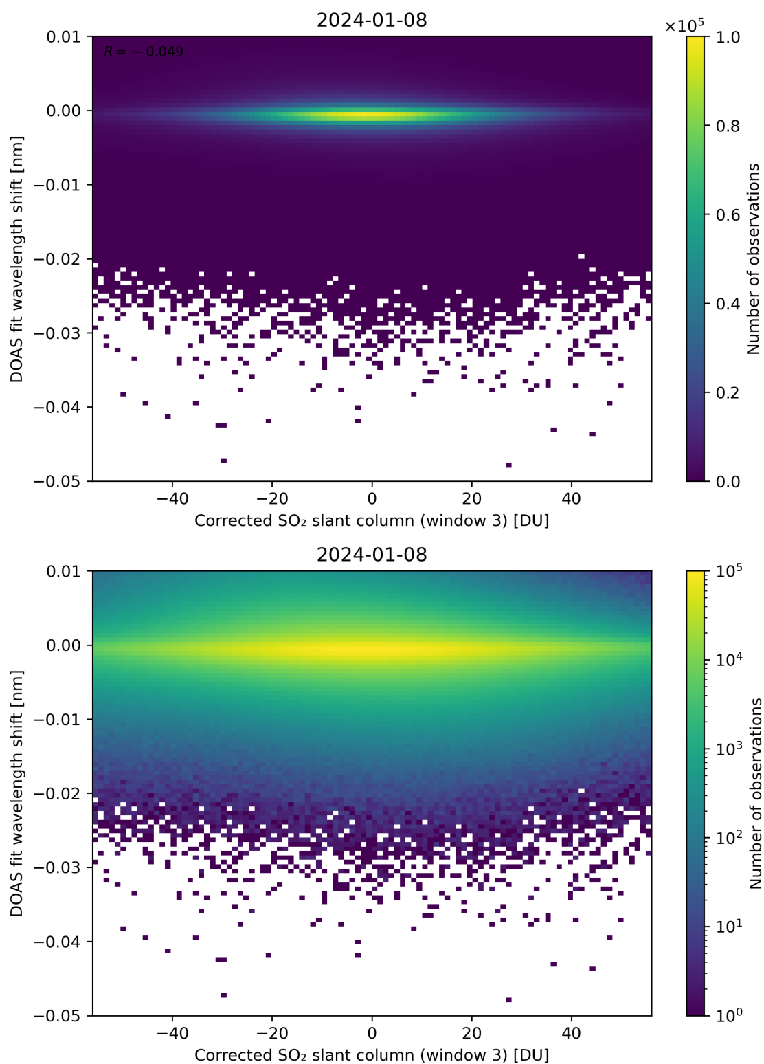
Figure 206: Scatter density plot of “Corrected SO 2 slant column (window 3)” against “DOAS fit wavelength shift” for 2024-01-07 to 2024-01-09.
