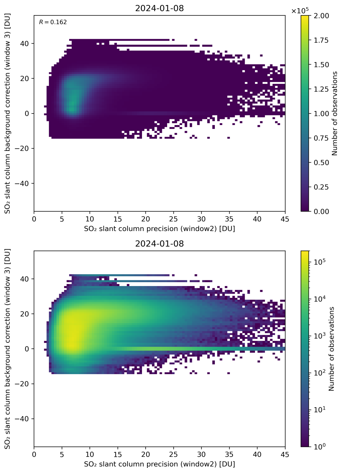
Figure 242: Scatter density plot of “SO 2 slant column precision (window2)” against “SO 2 slant column background correction (window 3)” for 2024-01-07 to 2024-01-09.
