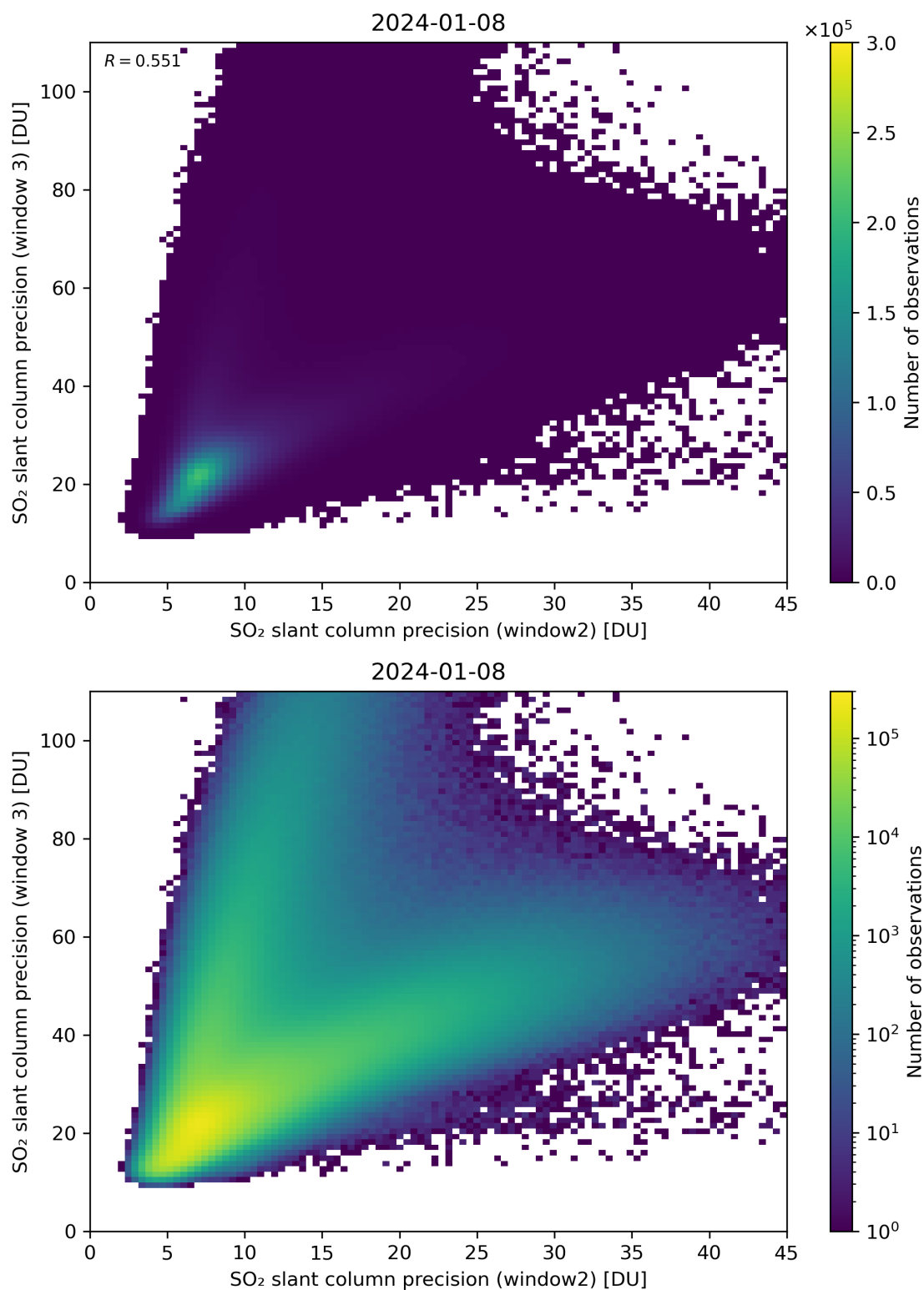
Figure 250: Scatter density plot of “SO 2 slant column precision (window2)” against “SO 2 slant column precision (window 3)” for 2024-01-07 to 2024-01-09.
