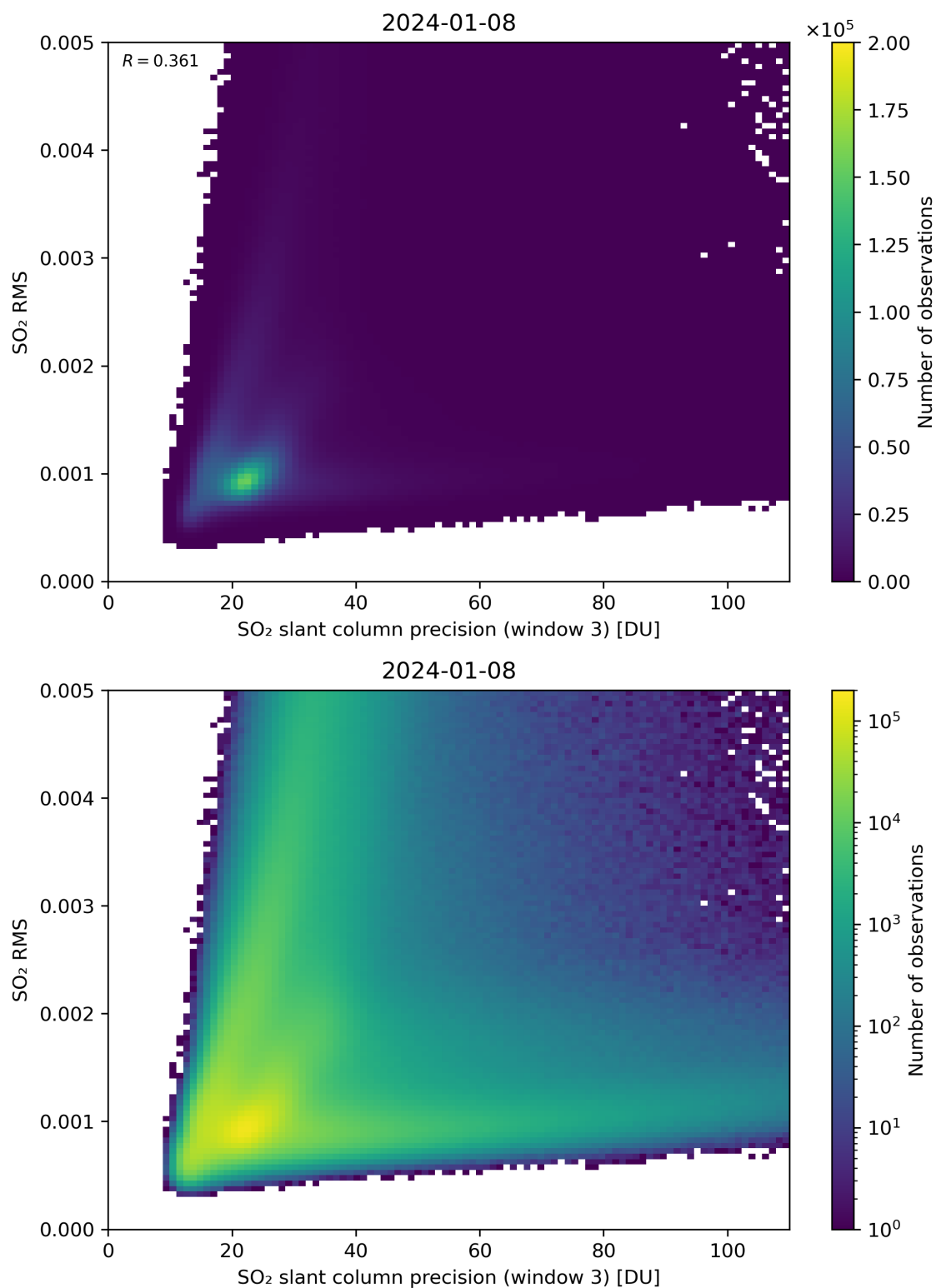
Figure 260: Scatter density plot of “SO 2 slant column precision (window 3)” against “SO 2 RMS” for 2024-01-07 to 2024-01-09.
