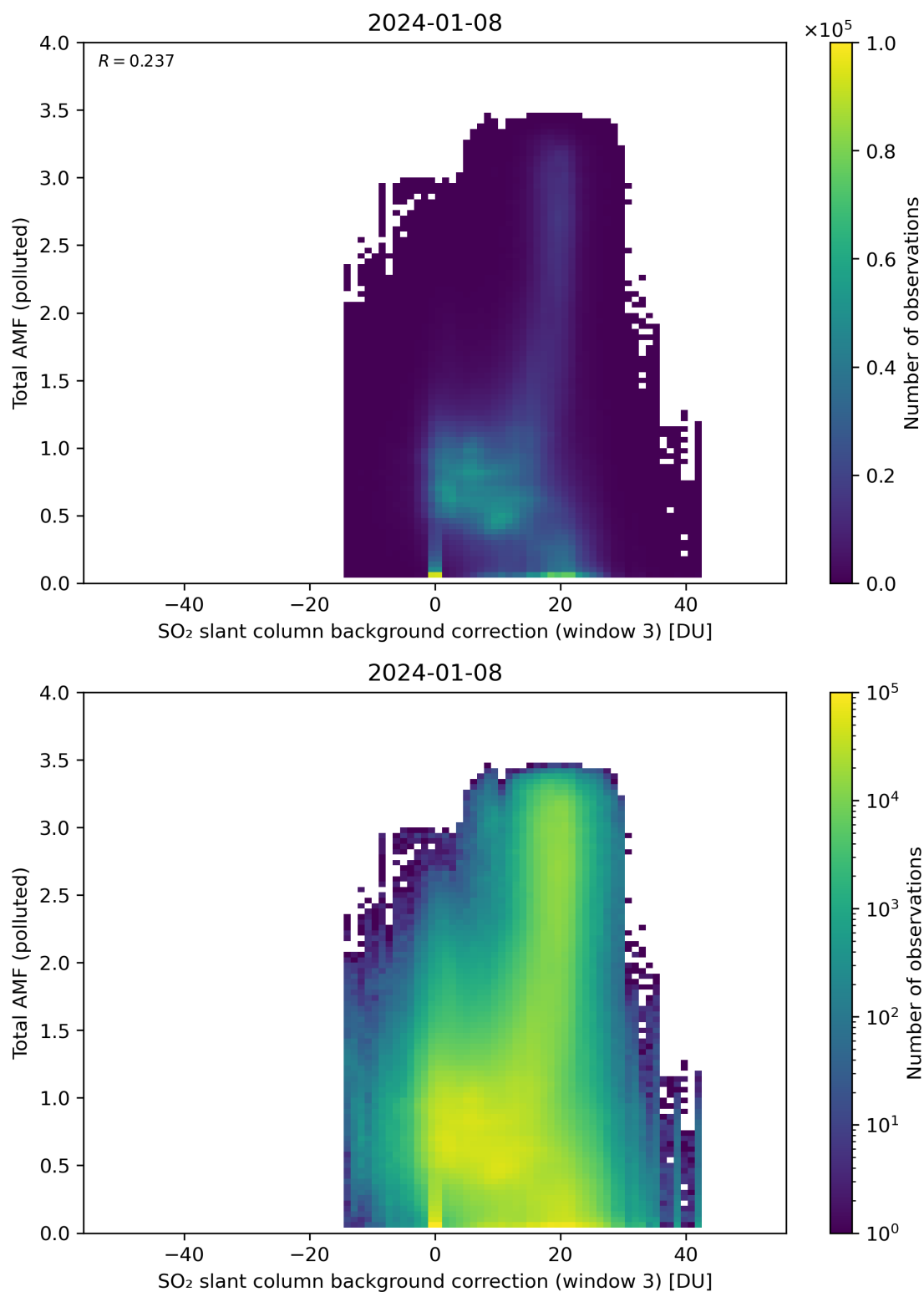
Figure 125: Scatter density plot of “SO 2 slant column background correction (window 3)” against “Total AMF (polluted)” for 2024-01-07 to 2024-01-09.
