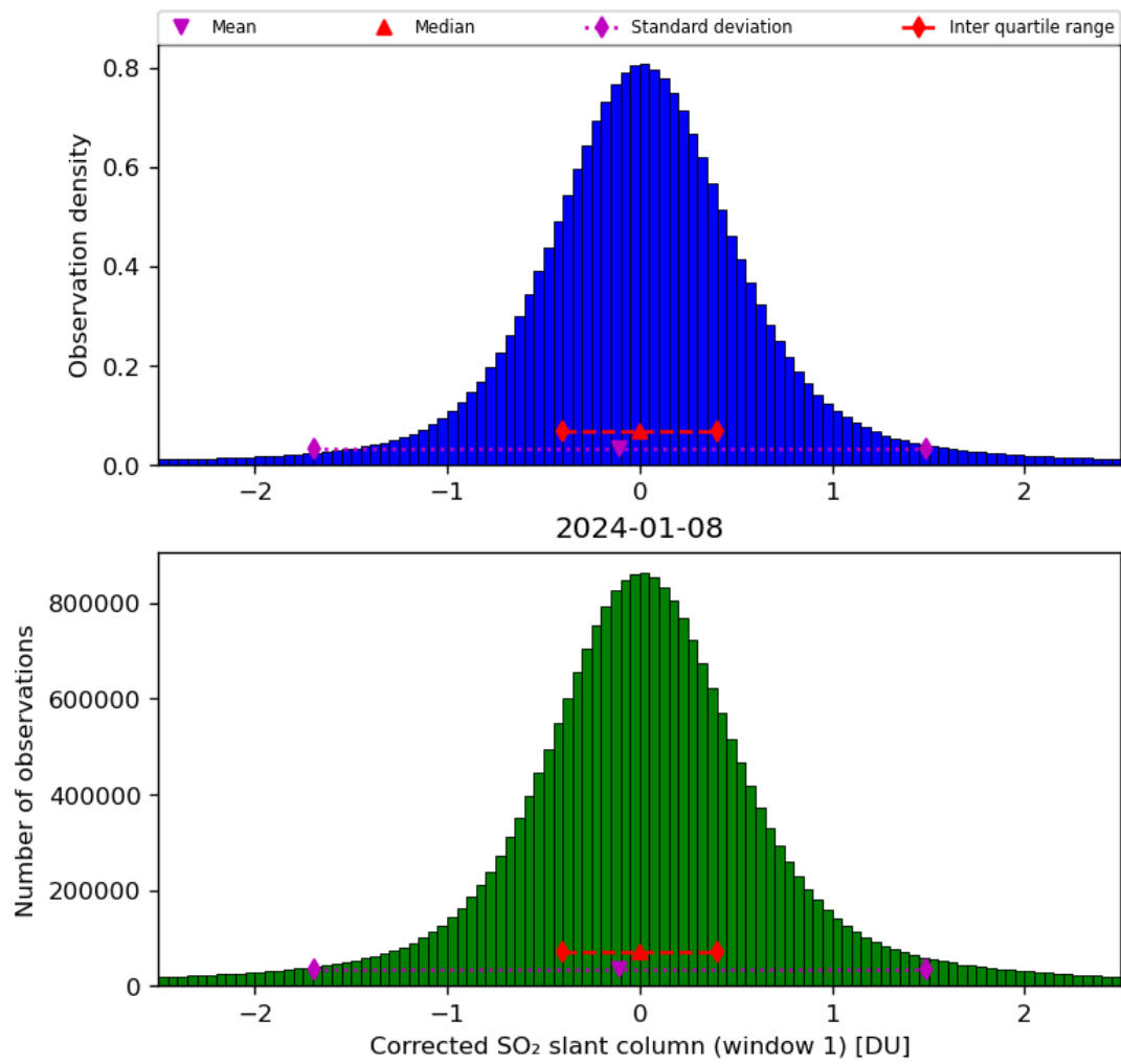
Figure 58: Histogram of “Corrected SO 2 slant column (window 1)” for 2024-01-07 to 2024-01-09
