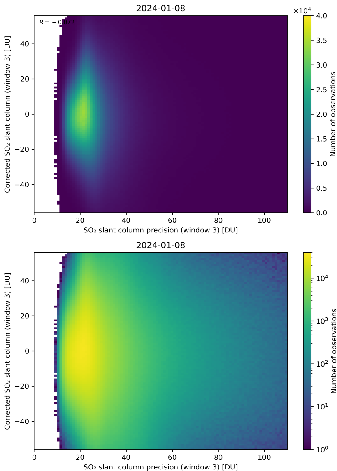
Figure 262: Scatter density plot of “SO 2 slant column precision (window 3)” against “Corrected SO 2 slant column (window 3)” for 2024-01-07 to 2024-01-09.
