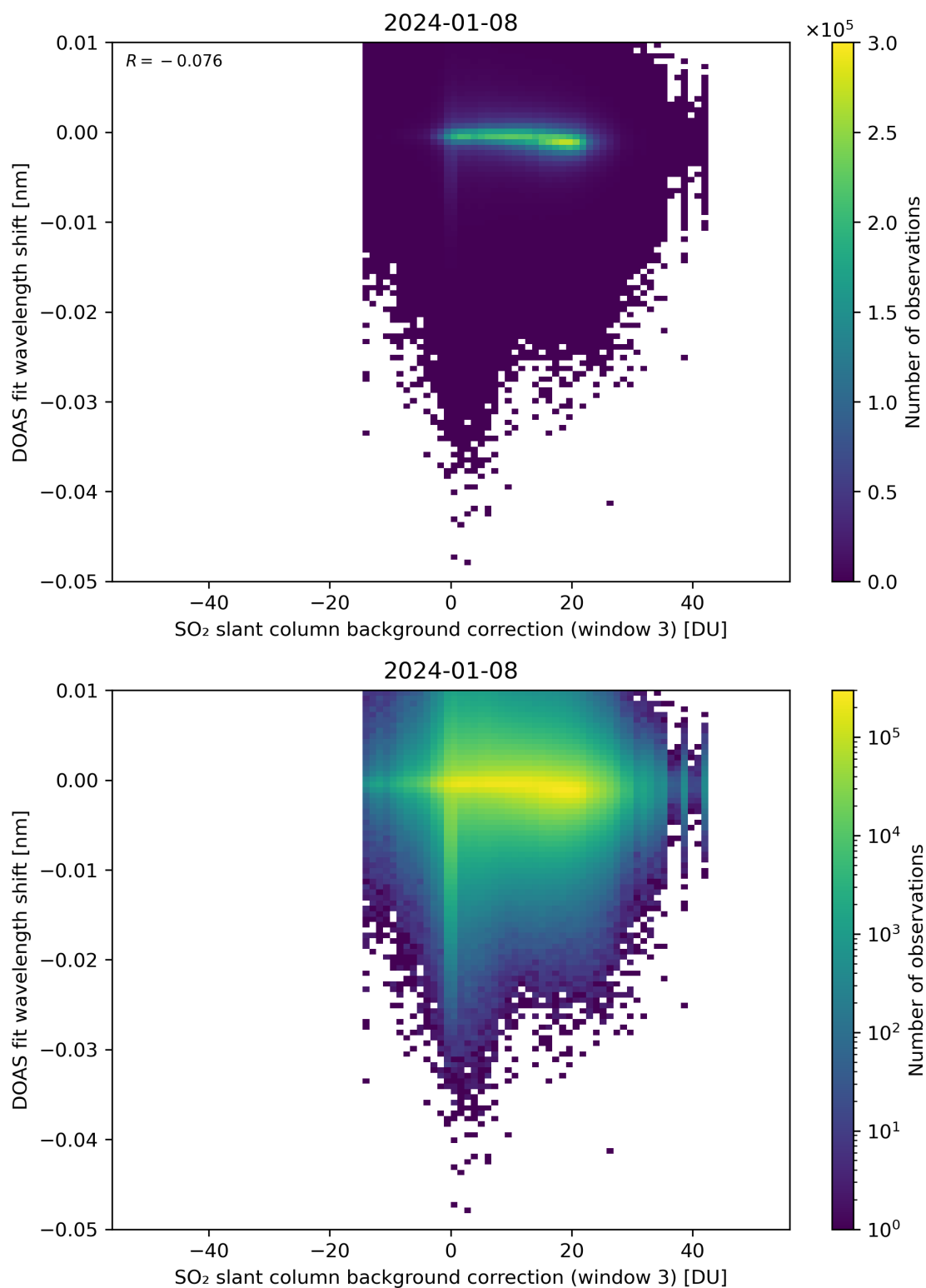
Figure 121: Scatter density plot of “SO 2 slant column background correction (window 3)” against “DOAS fit wavelength shift” for 2024-01-07 to 2024-01-09.
