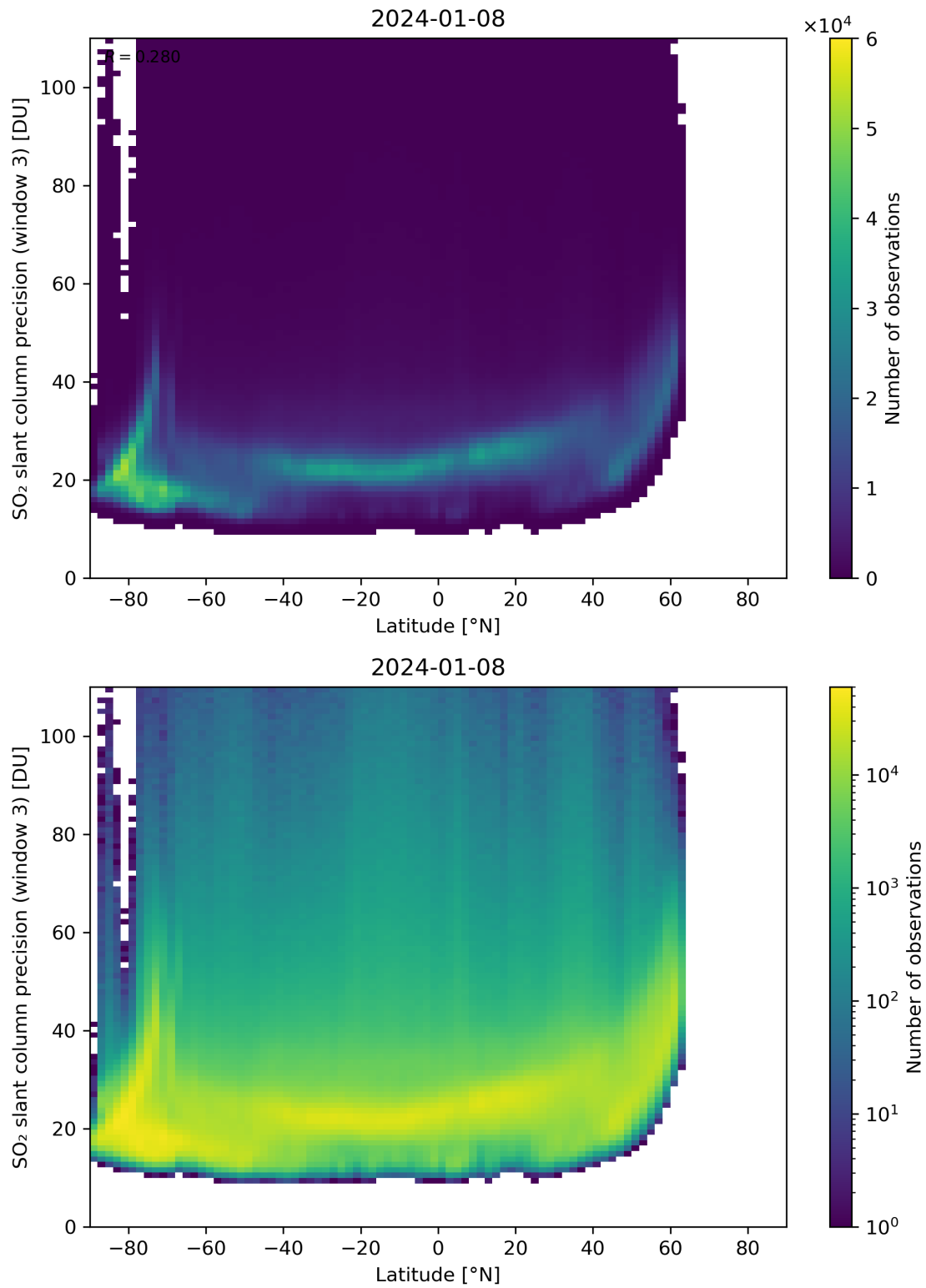
Figure 153: Scatter density plot of “Latitude” against “SO 2 slant column precision (window 3)” for 2024-01-07 to 2024-01-09.
