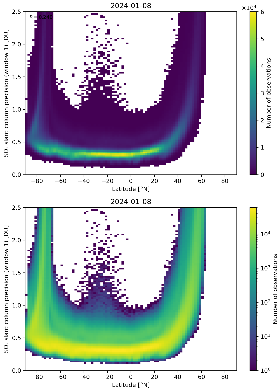
Figure 150: Scatter density plot of “Latitude” against “SO 2 slant column precision (window 1)” for 2024-01-07 to 2024-01-09.
