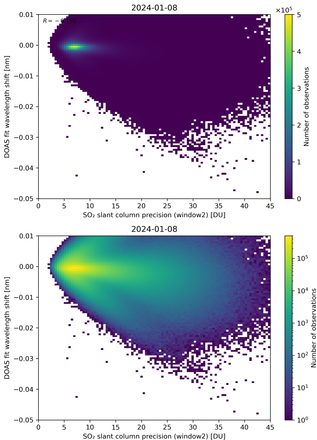
Figure 243: Scatter density plot of “SO 2 slant column precision (window2)” against “DOAS fit wavelength shift” for 2024-01-07 to 2024-01-09.
