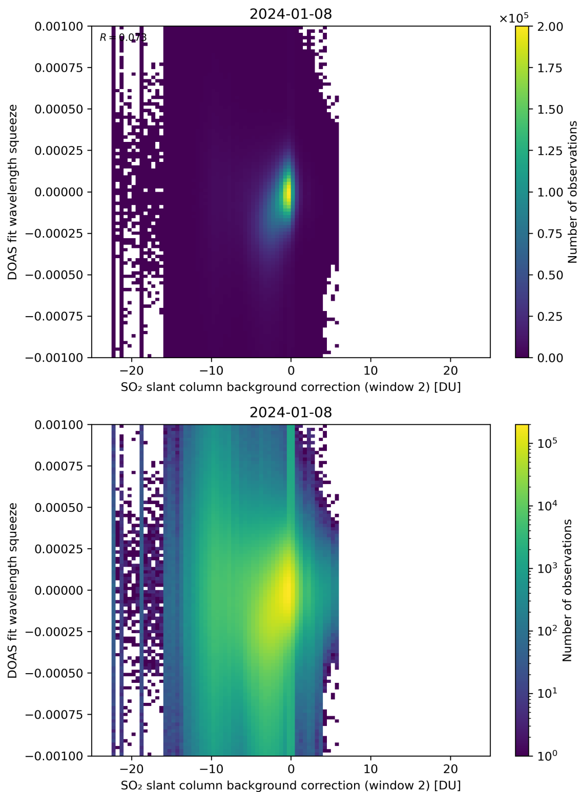
Figure 113: Scatter density plot of “SO 2 slant column background correction (window 2)” against “DOAS fit wavelength squeeze” for 2024-01-07 to 2024-01-09.
