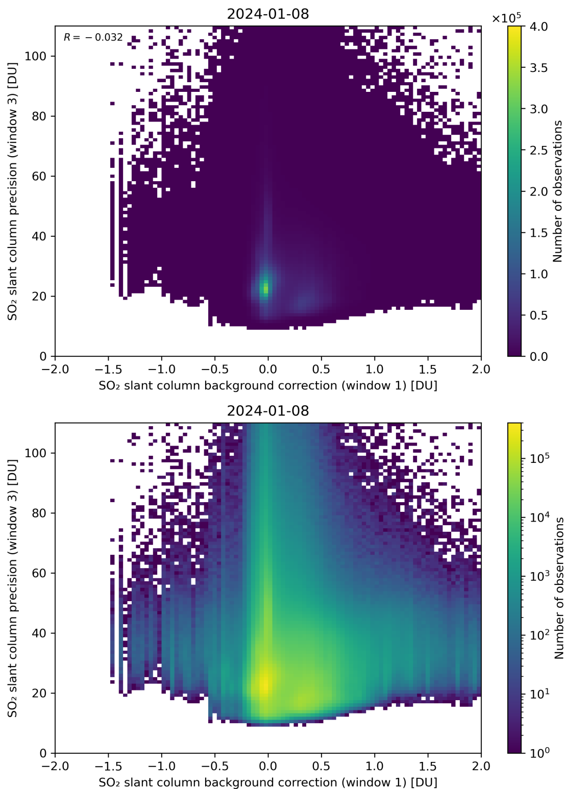
Figure 108: Scatter density plot of “SO 2 slant column background correction (window 1)” against “SO 2 slant column precision (window 3)” for 2024-01-07 to 2024-01-09.
