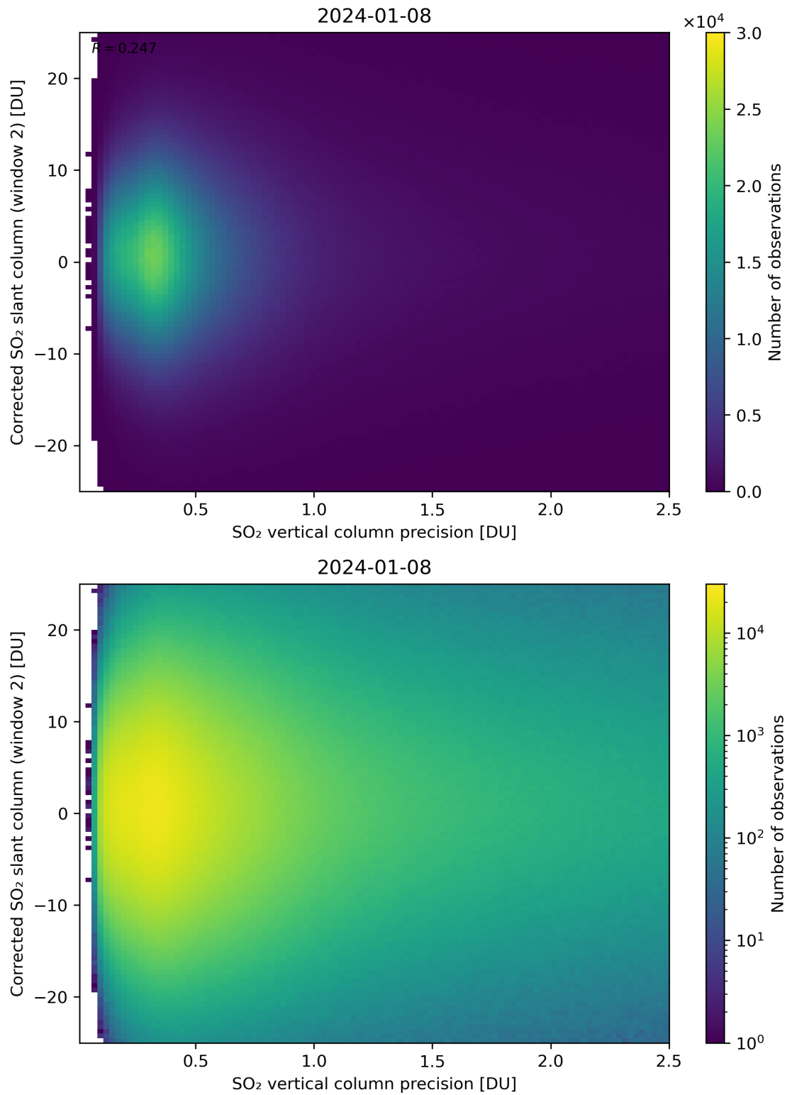
Figure 287: Scatter density plot of “SO 2 vertical column precision” against “Corrected SO 2 slant column (window 2)” for 2024-01-07 to 2024-01-09.
