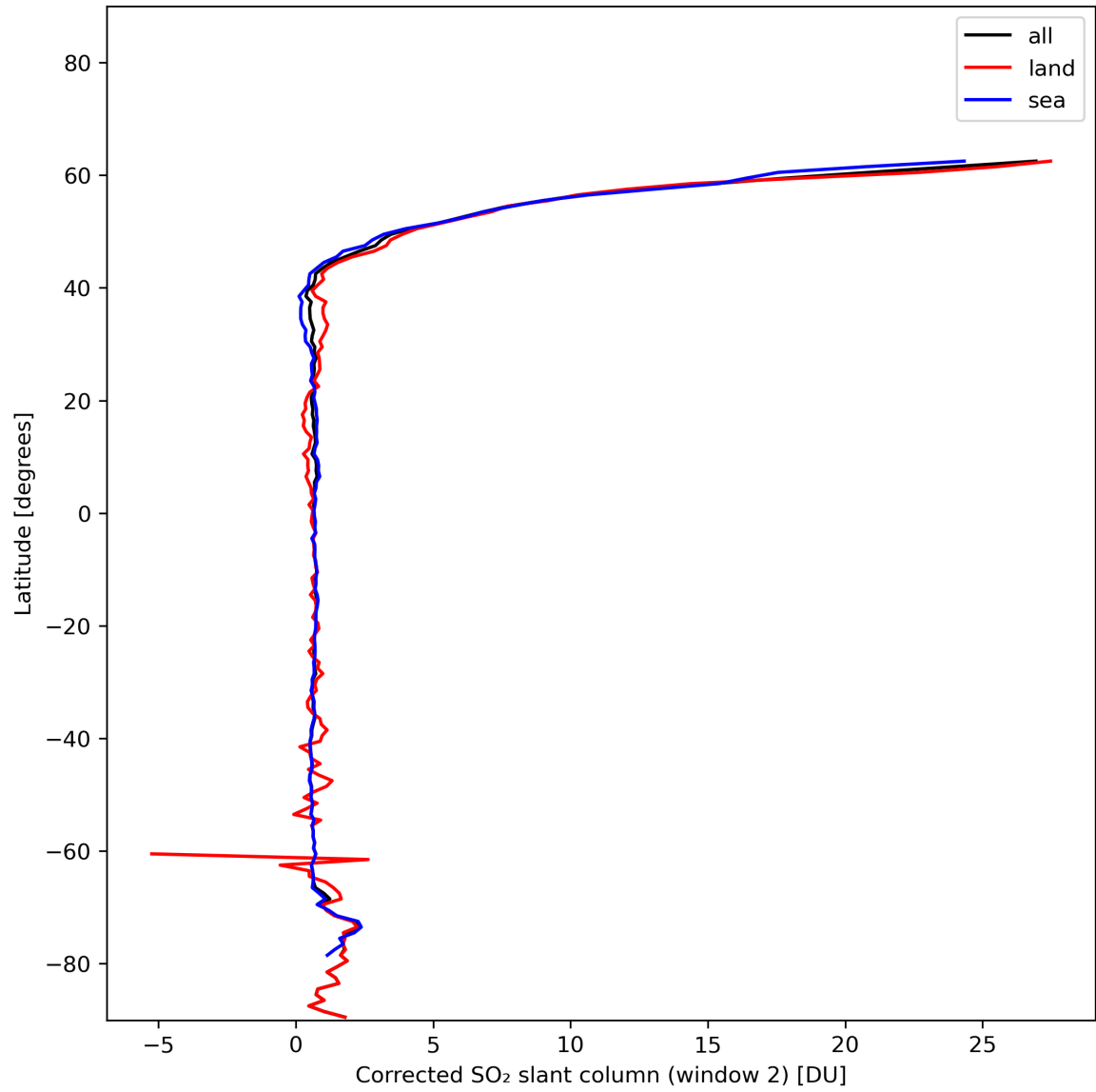
Figure 39: Zonal average of “Corrected SO 2 slant column (window 2)” for 2024-01-07 to 2024-01-09.
