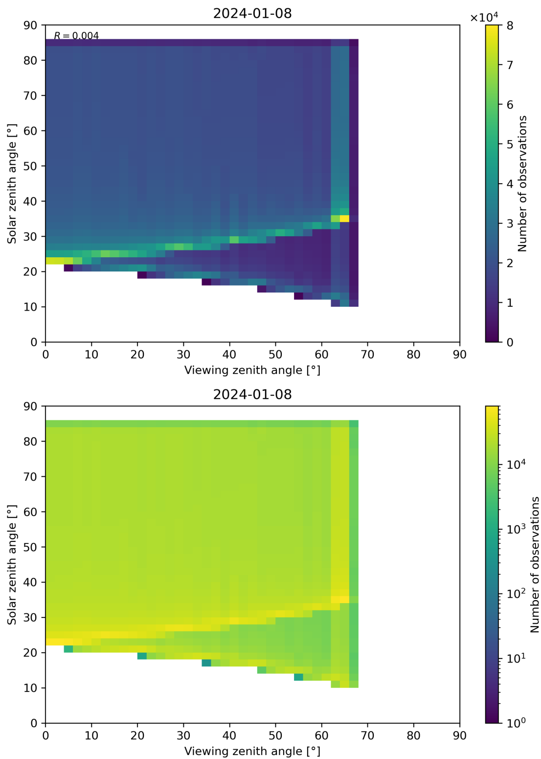
Figure 315: Scatter density plot of “Viewing zenith angle” against “Solar zenith angle” for 2024-01-07 to 2024-01-09.
