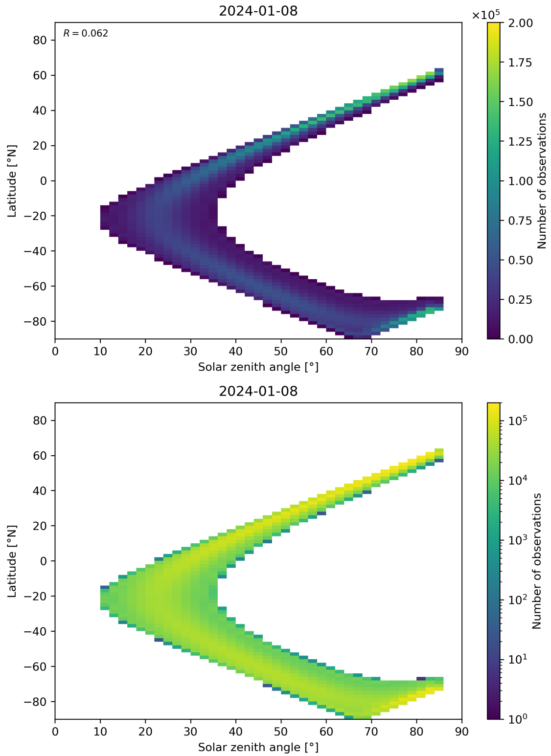
Figure 164: Scatter density plot of “Solar zenith angle” against “Latitude” for 2024-01-07 to 2024-01-09.
