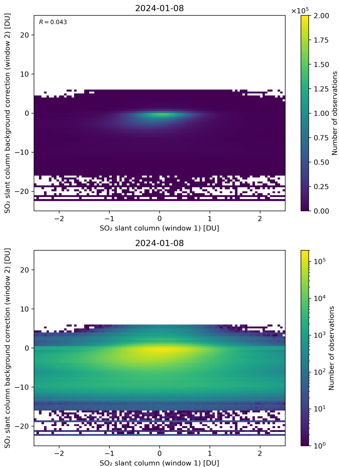
Figure 213: Scatter density plot of “SO 2 slant column (window 1)” against “SO 2 slant column background correction (window 2)” for 2024-01-07 to 2024-01-09.
