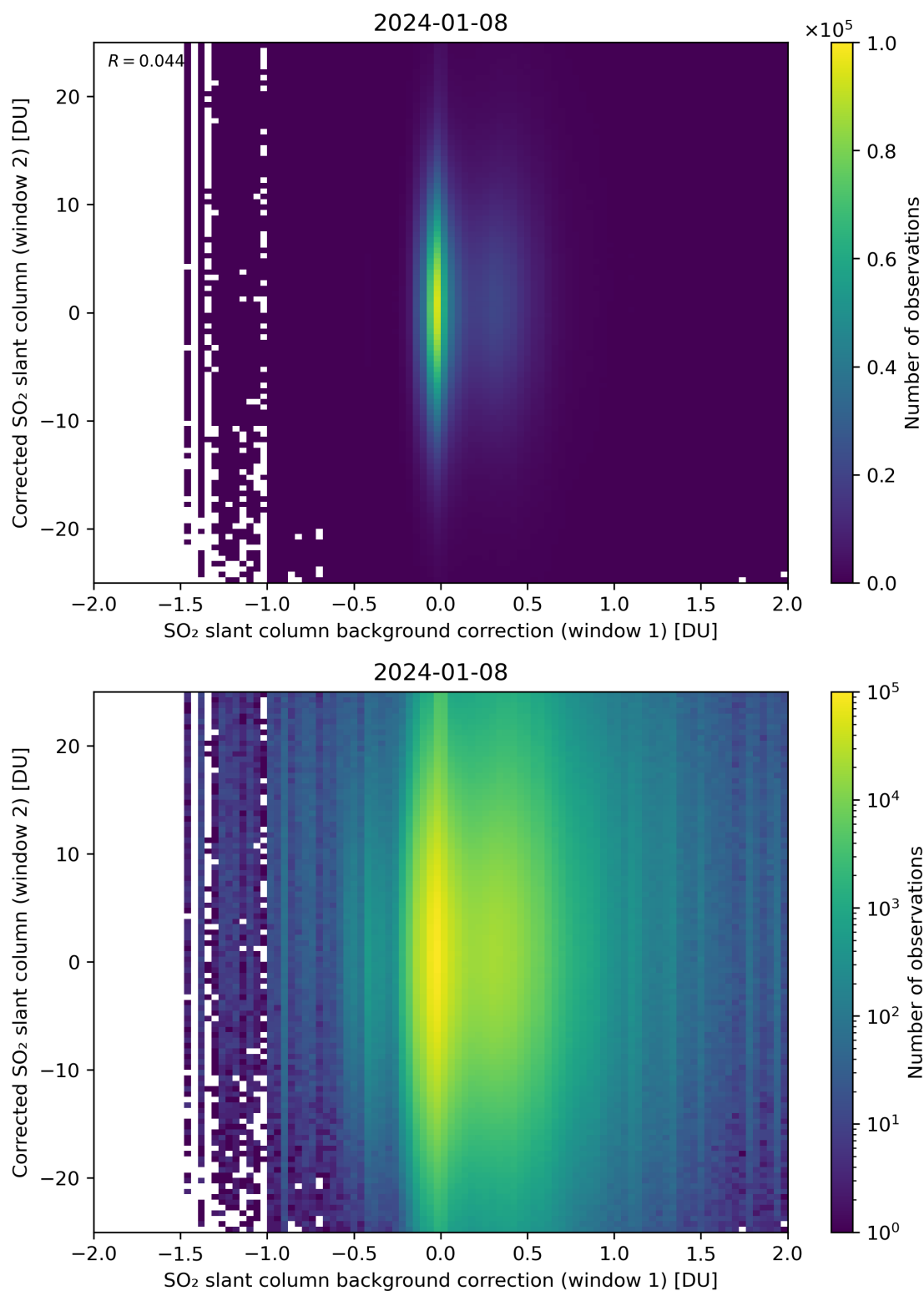
Figure 104: Scatter density plot of “SO 2 slant column background correction (window 1)” against “Corrected SO 2 slant column (window 2)” for 2024-01-07 to 2024-01-09.
