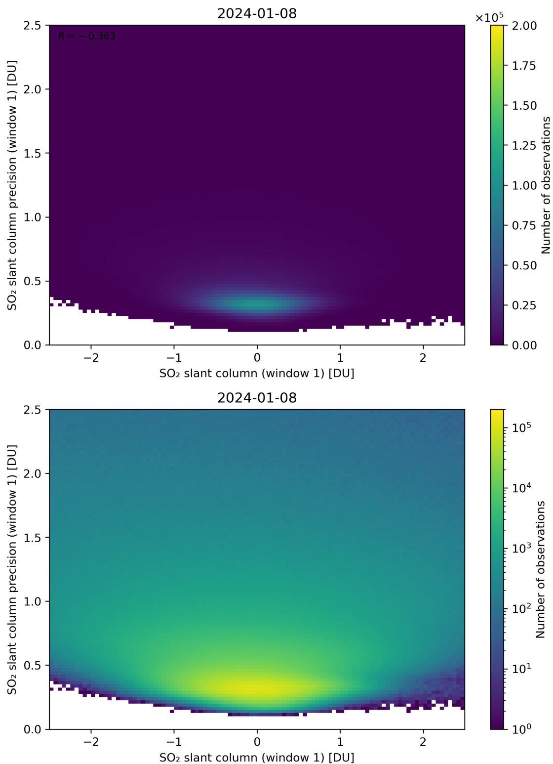
Figure 235: Scatter density plot of “SO 2 slant column (window 1)” against “SO 2 slant column precision (window 1)” for 2024-01-07 to 2024-01-09.
