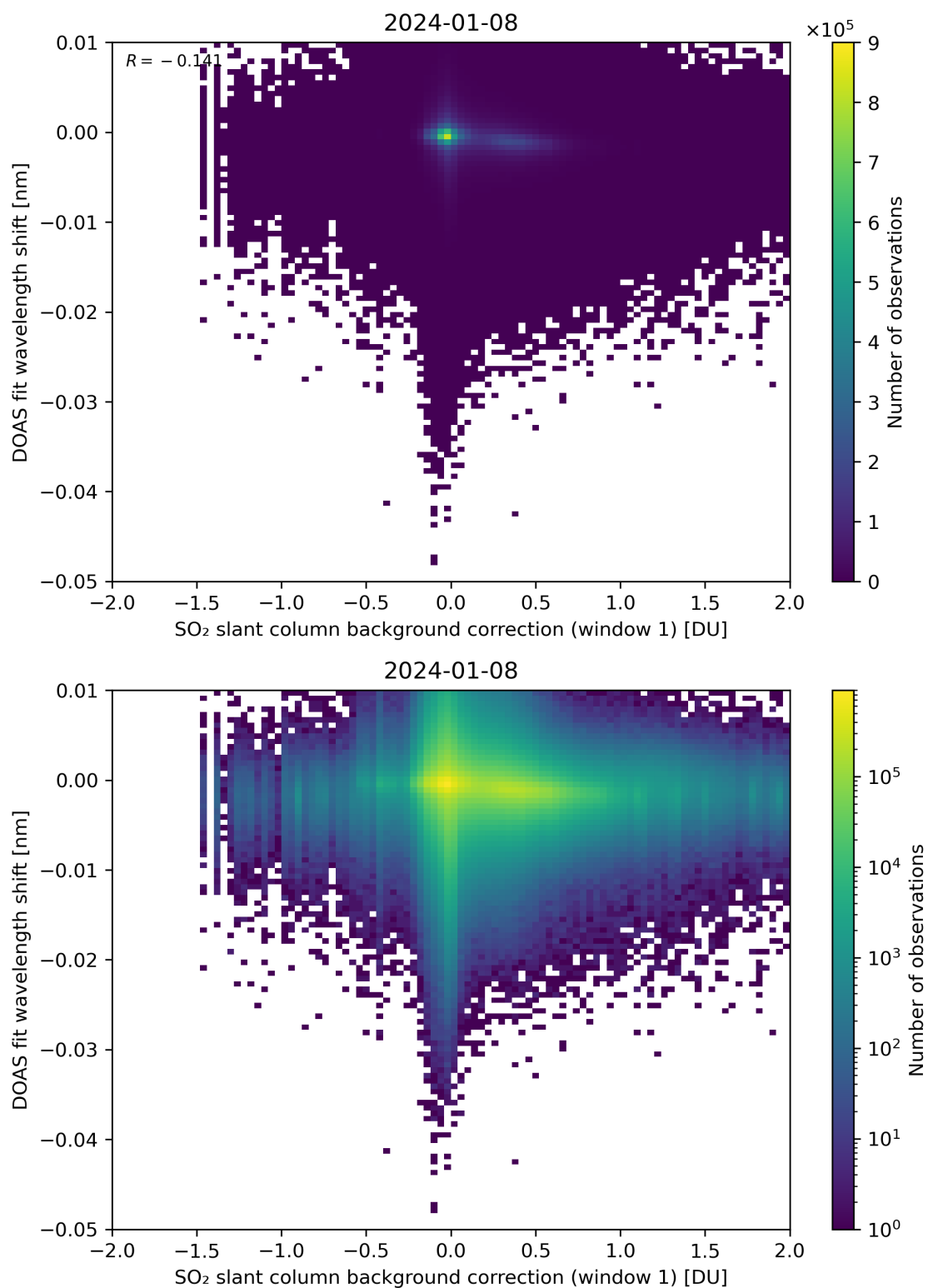
Figure 100: Scatter density plot of “SO 2 slant column background correction (window 1)” against “DOAS fit wavelength shift” for 2024-01-07 to 2024-01-09.
