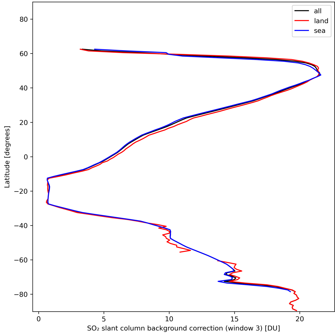
Figure 44: Zonal average of “SO 2 slant column background correction (window 3)” for 2024-01-07 to 2024-01-09.
