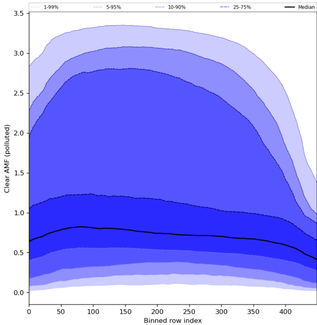
Figure 96: Along track statistics of “Clear AMF (polluted)” for 2024-01-07 to 2024-01-09
