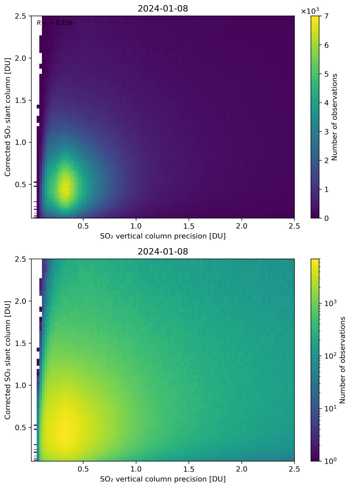
Figure 286: Scatter density plot of “SO 2 vertical column precision” against “Corrected SO 2 slant column” for 2024-01-07 to 2024-01-09.
