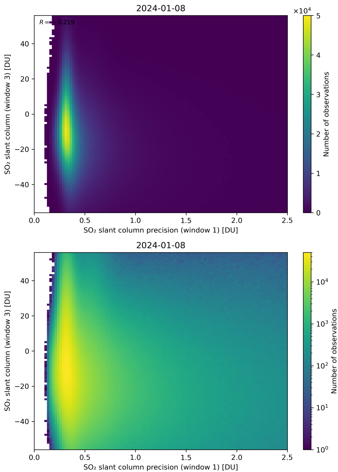
Figure 228: Scatter density plot of “SO 2 slant column precision (window 1)” against “SO 2 slant column (window 3)” for 2024-01-07 to 2024-01-09.
