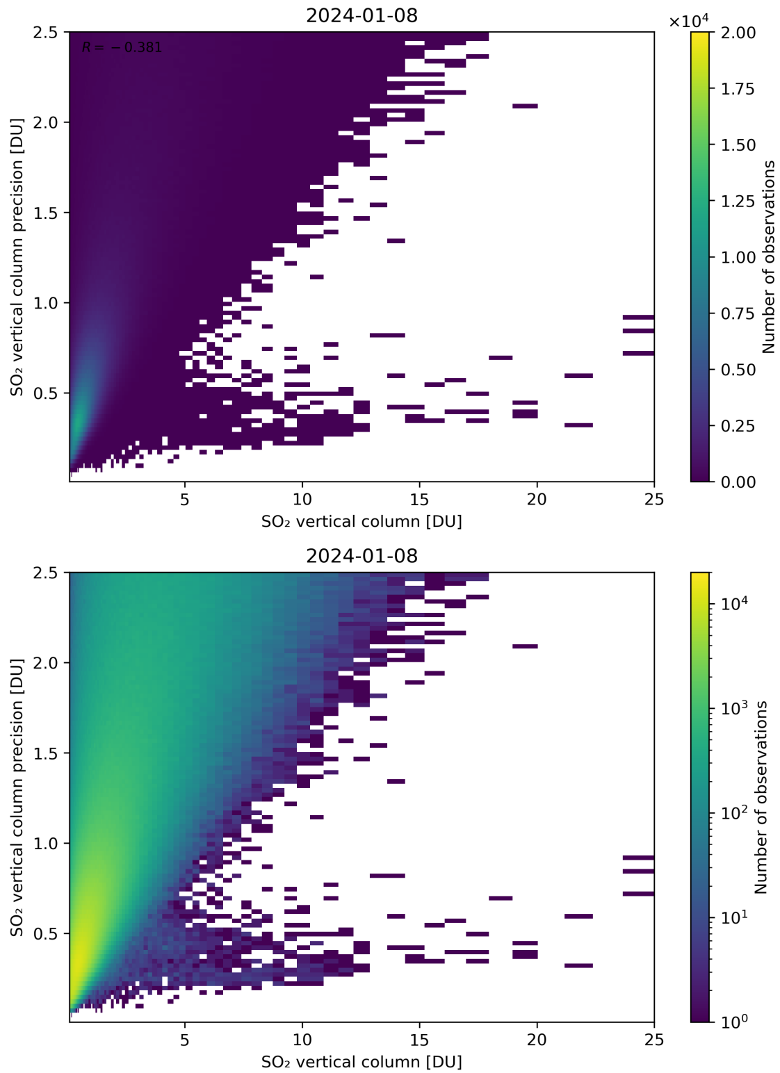
Figure 307: Scatter density plot of “SO 2 vertical column” against “SO 2 vertical column precision” for 2024-01-07 to 2024-01-09.
