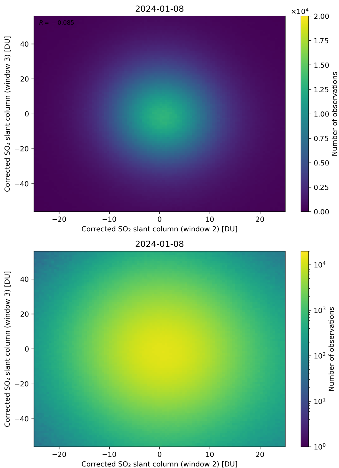
Figure 200: Scatter density plot of “Corrected SO 2 slant column (window 2)” against “Corrected SO 2 slant column (window 3)” for 2024-01-07 to 2024-01-09.
