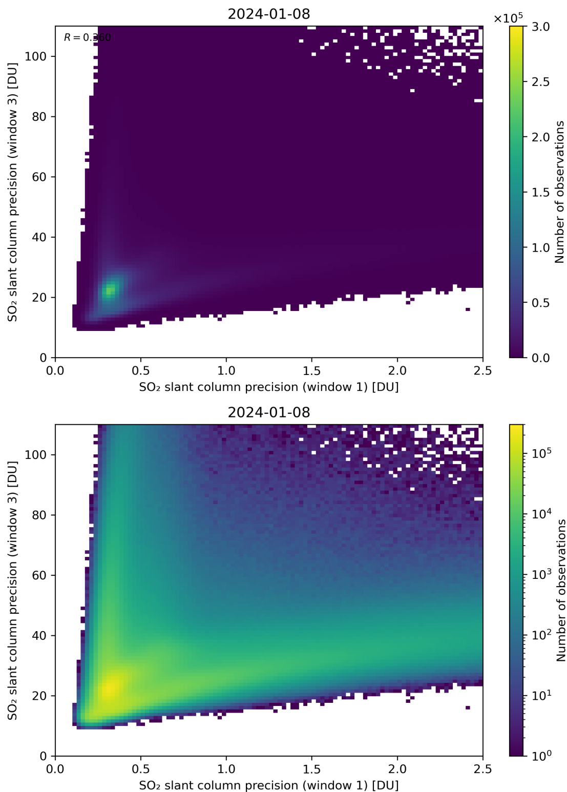
Figure 229: Scatter density plot of “SO 2 slant column precision (window 1)” against “SO 2 slant column precision (window 3)” for 2024-01-07 to 2024-01-09.
