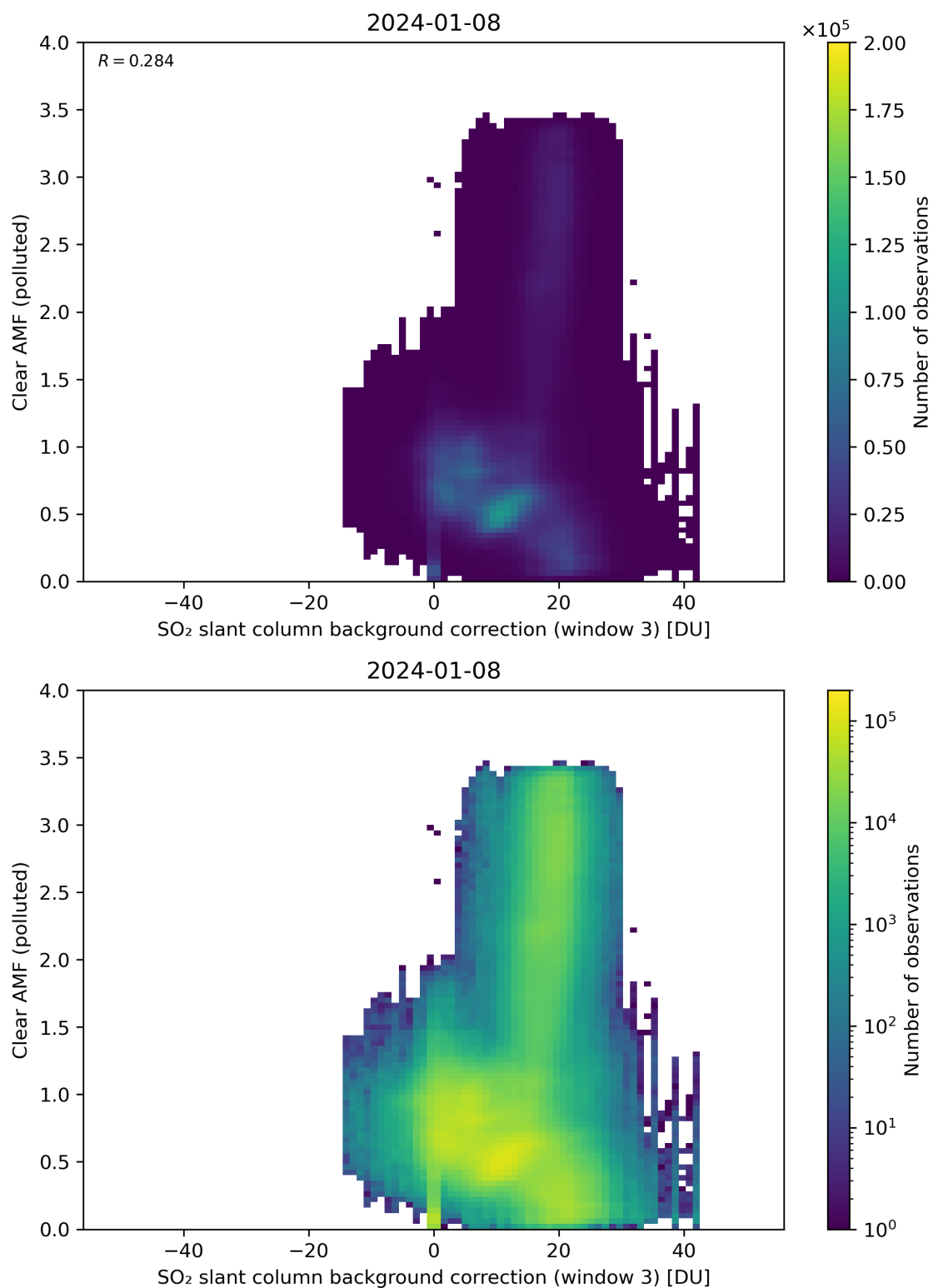
Figure 124: Scatter density plot of “SO 2 slant column background correction (window 3)” against “Clear AMF (polluted)” for 2024-01-07 to 2024-01-09.
