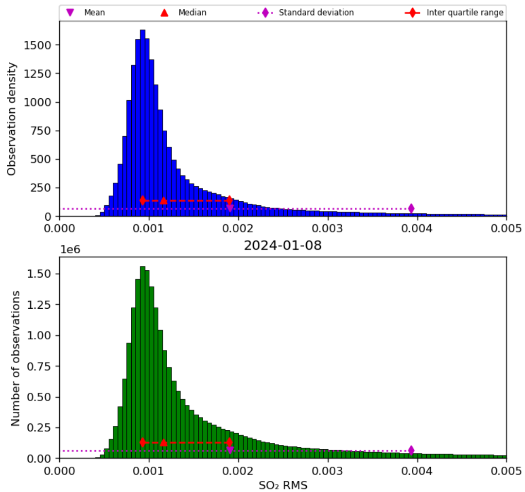
Figure 70: Histogram of “SO 2 RMS” for 2024-01-07 to 2024-01-09
