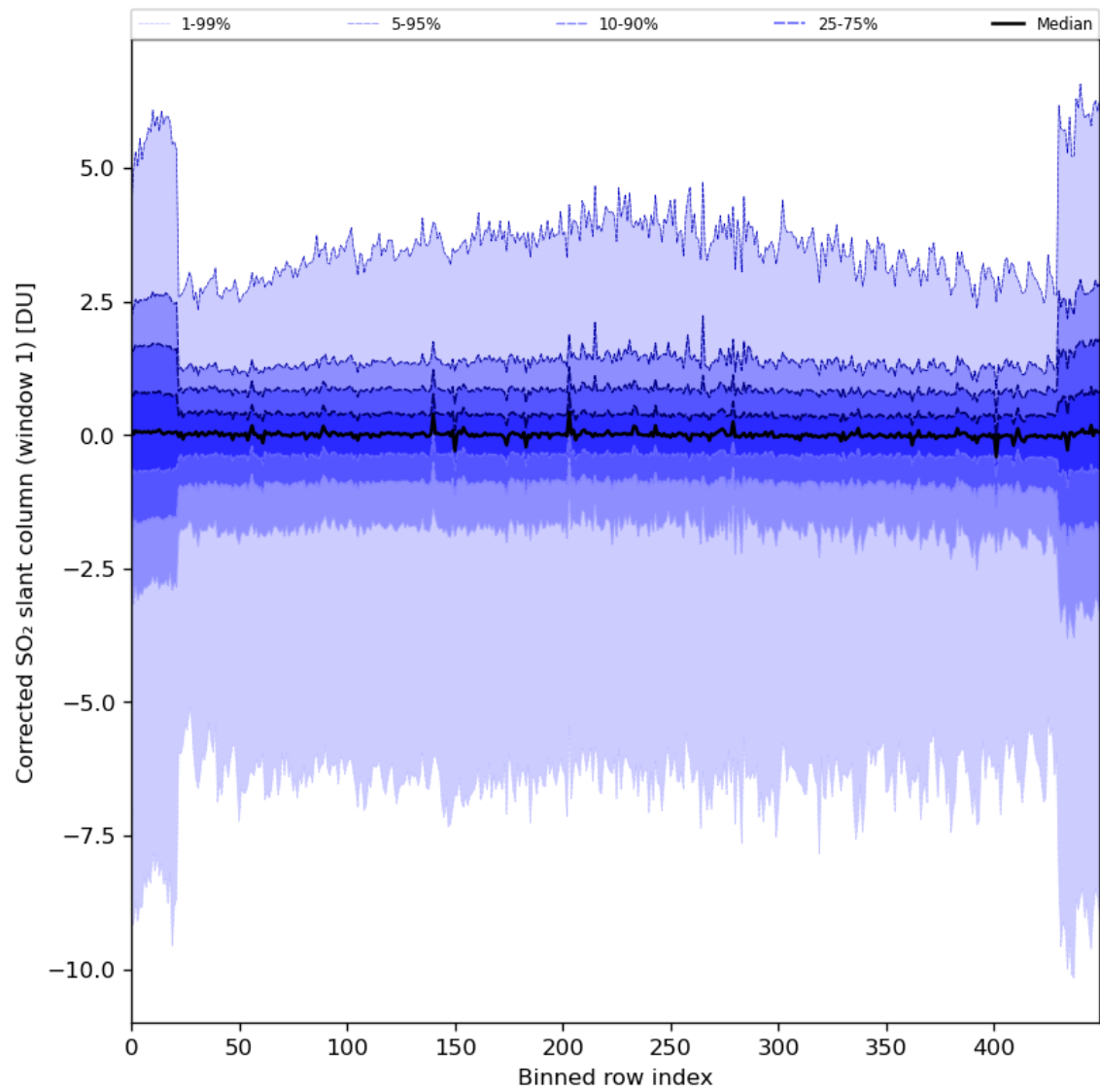
Figure 81: Along track statistics of “Corrected SO 2 slant column (window 1)” for 2024-01-07 to 2024-01-09
