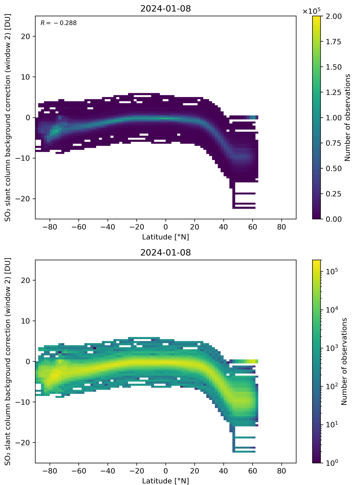
Figure 140: Scatter density plot of “Latitude” against “SO 2 slant column background correction (window 2)” for 2024-01-07 to 2024-01-09.
