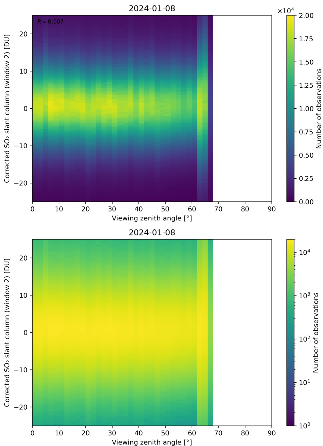
Figure 318: Scatter density plot of “Viewing zenith angle” against “Corrected SO 2 slant column (window 2)” for 2024-01-07 to 2024-01-09.
