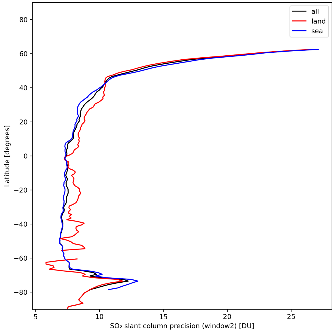
Figure 38: Zonal average of “SO 2 slant column precision (window2)” for 2024-01-07 to 2024-01-09.
