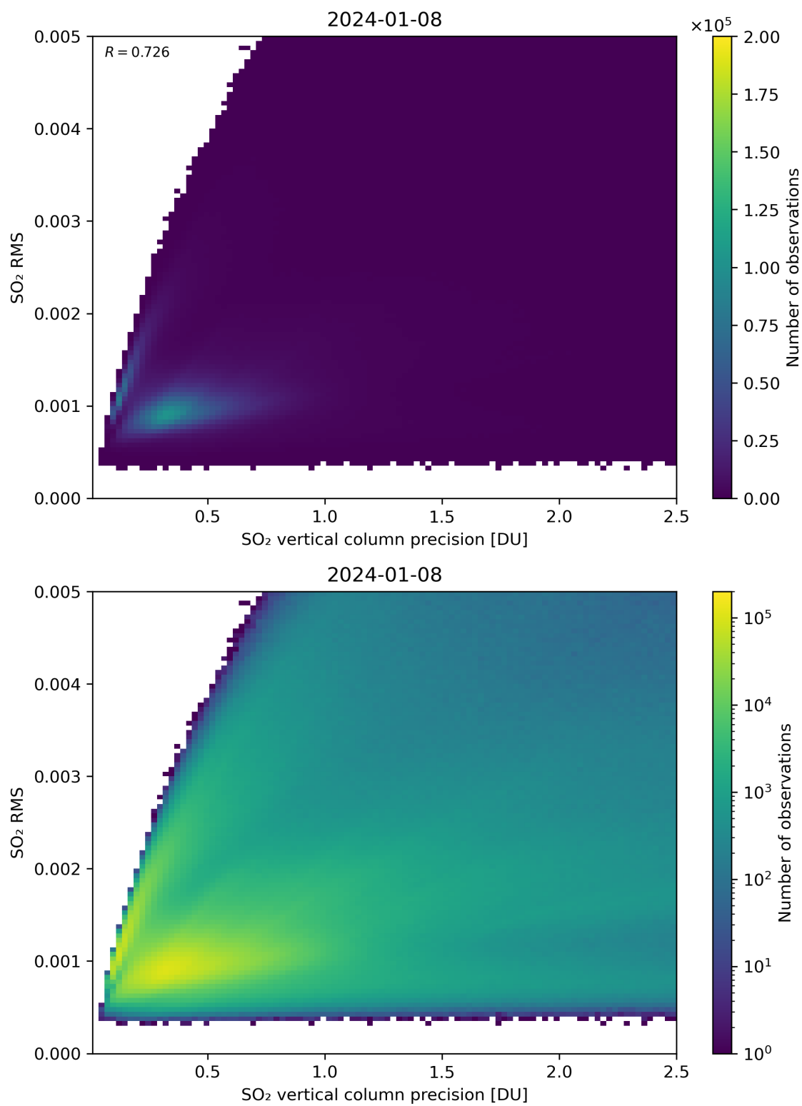
Figure 284: Scatter density plot of “SO 2 vertical column precision” against “SO 2 RMS” for 2024-01-07 to 2024-01-09.
