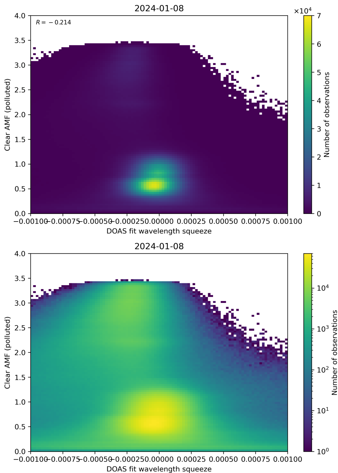
Figure 133: Scatter density plot of “DOAS fit wavelength squeeze” against “Clear AMF (polluted)” for 2024-01-07 to 2024-01-09.
