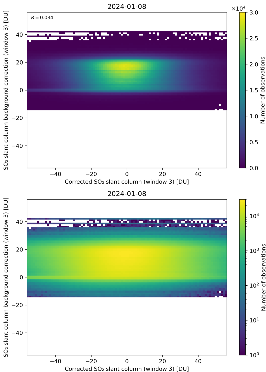
Figure 205: Scatter density plot of “Corrected SO 2 slant column (window 3)” against “SO 2 slant column background correction (window 3)” for 2024-01-07 to 2024-01-09.
