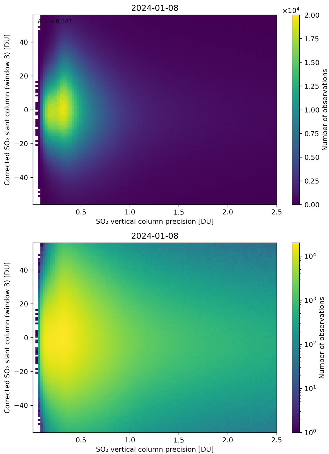
Figure 288: Scatter density plot of “SO 2 vertical column precision” against “Corrected SO 2 slant column (window 3)” for 2024-01-07 to 2024-01-09.
