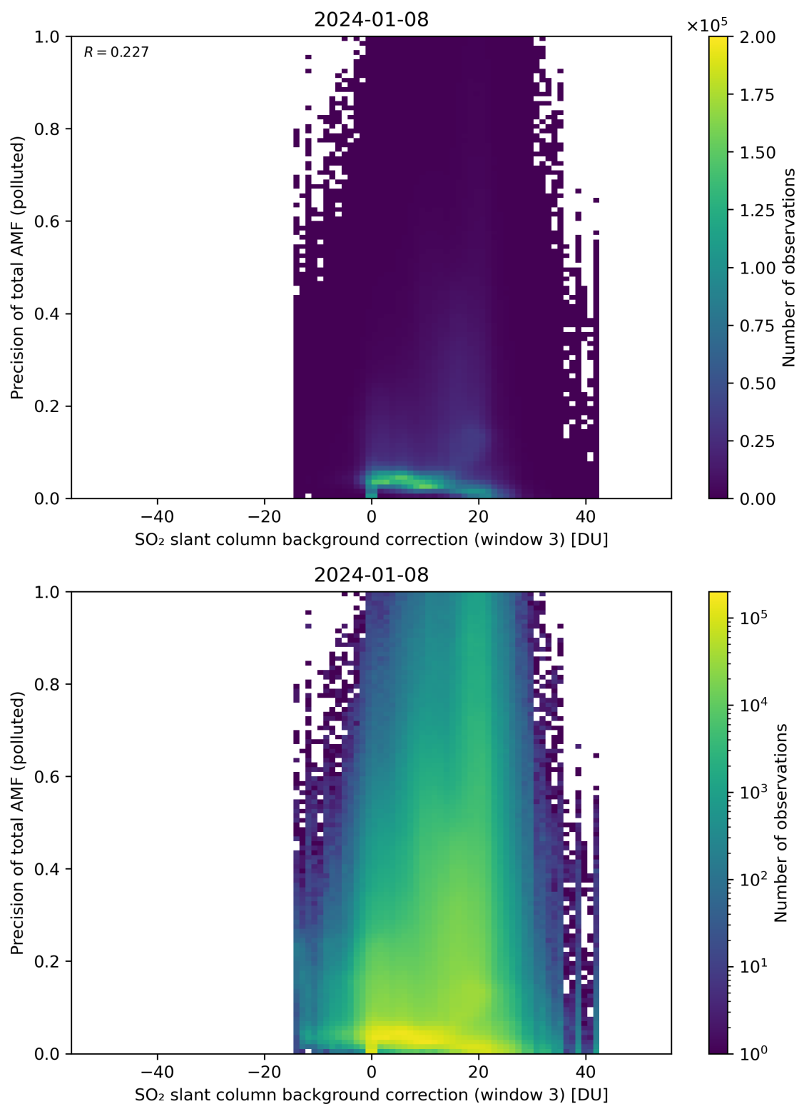
Figure 126: Scatter density plot of “SO 2 slant column background correction (window 3)” against “Precision of total AMF (polluted)” for 2024-01-07 to 2024-01-09.
