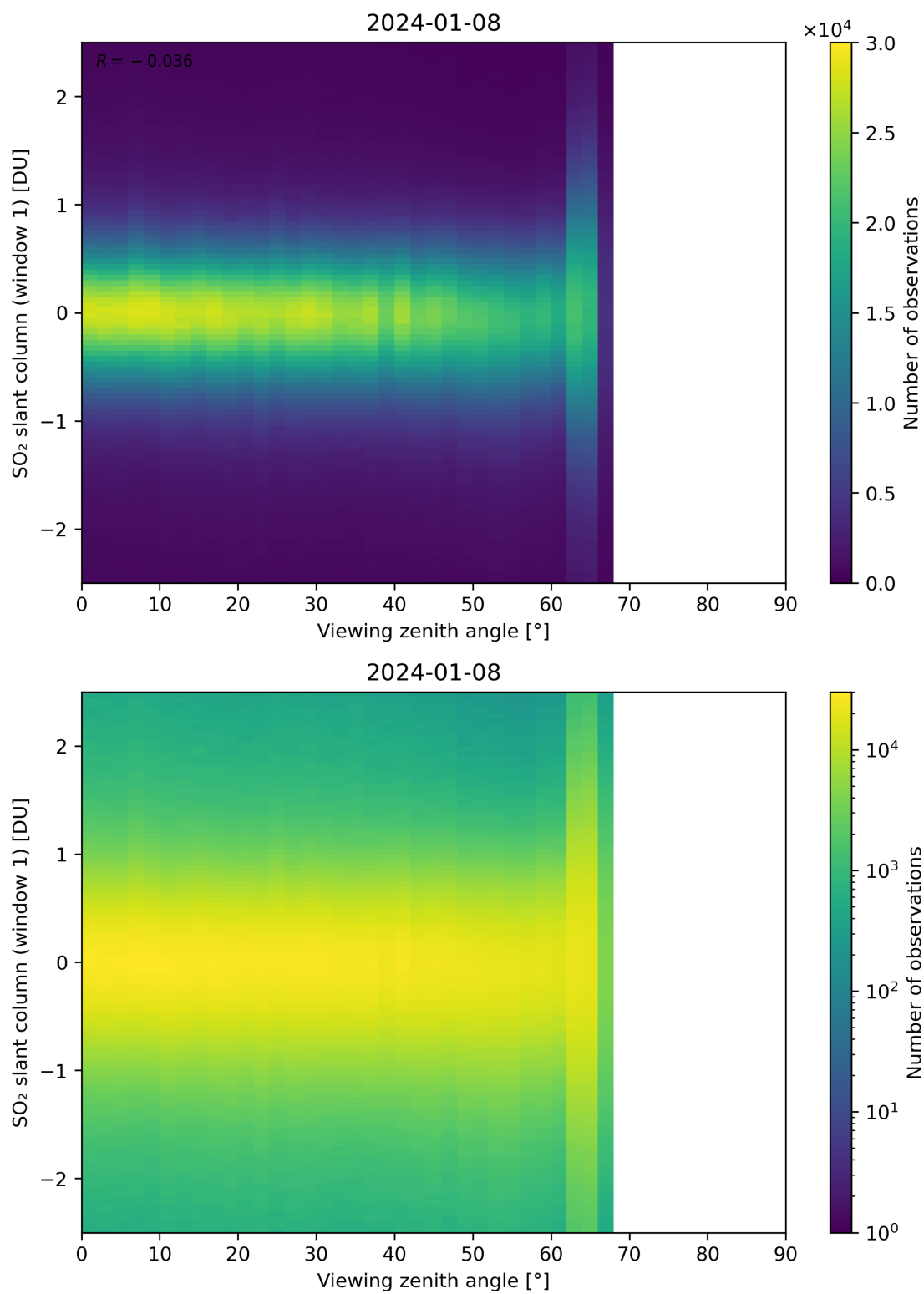
Figure 320: Scatter density plot of “Viewing zenith angle” against “SO 2 slant column (window 1)” for 2024-01-07 to 2024-01-09.
