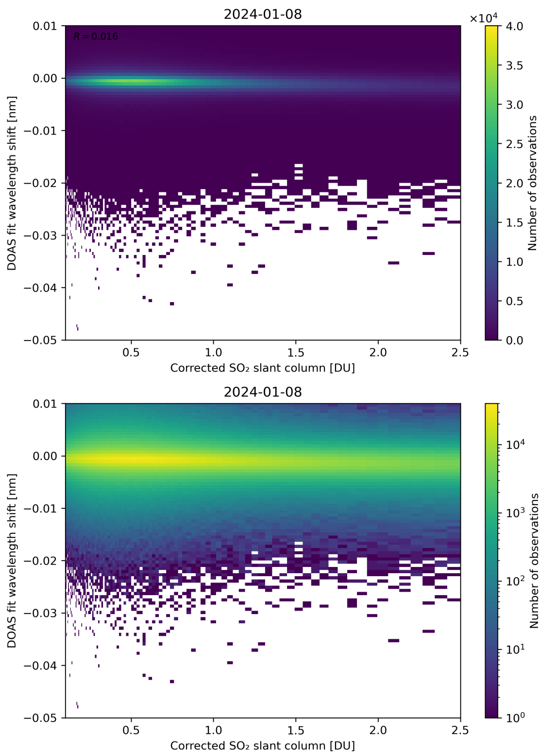
Figure 181: Scatter density plot of “Corrected SO 2 slant column” against “DOAS fit wavelength shift” for 2024-01-07 to 2024-01-09.
