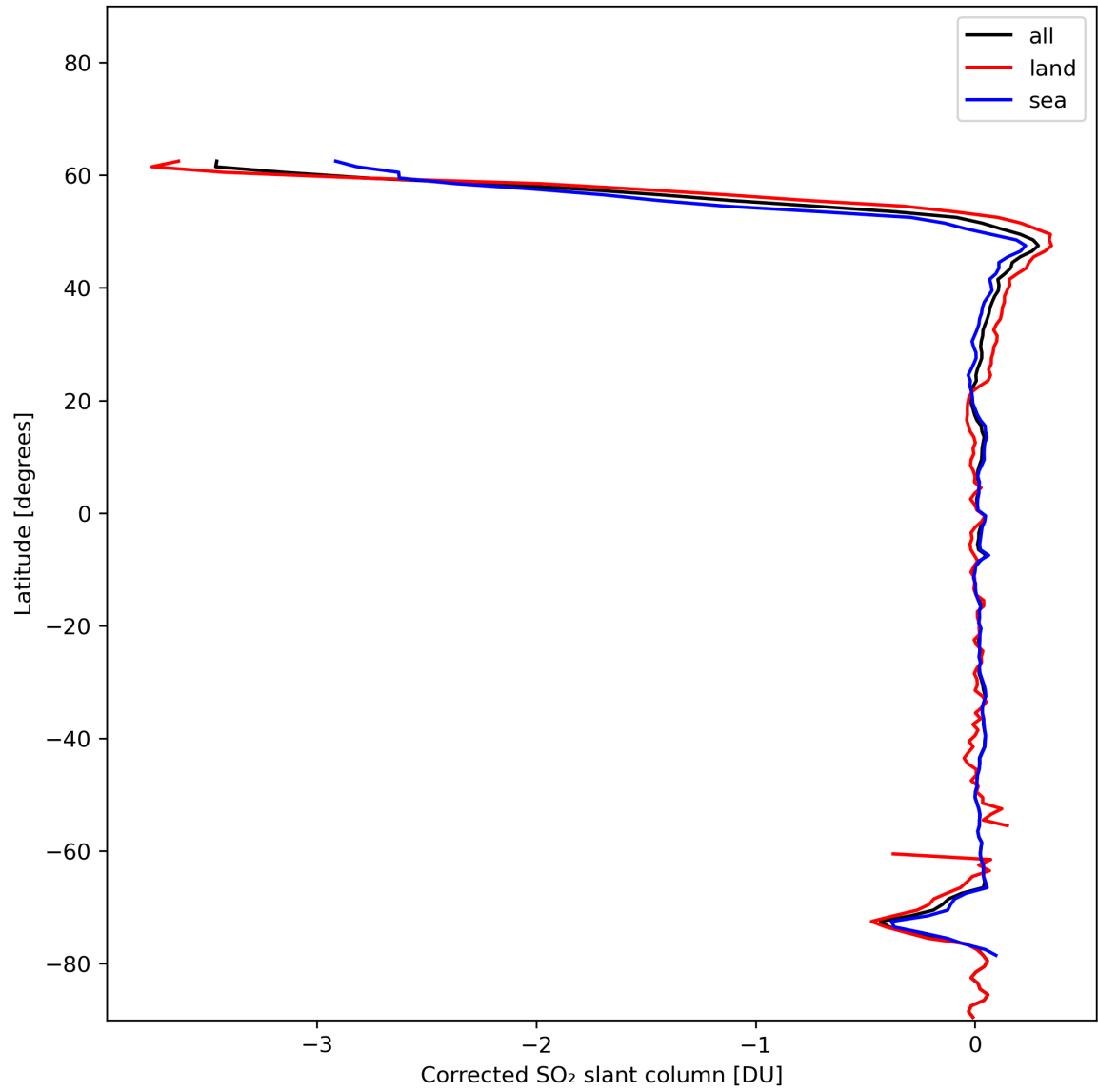
Figure 32: Zonal average of “Corrected SO 2 slant column” for 2024-01-07 to 2024-01-09.
