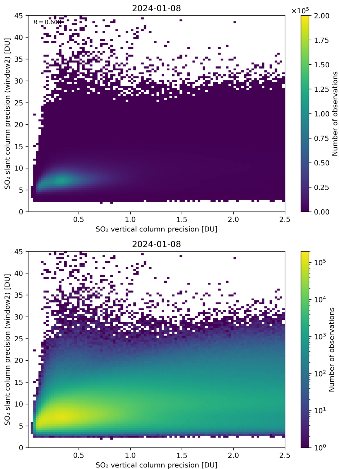
Figure 291: Scatter density plot of “SO 2 vertical column precision” against “SO 2 slant column precision (window2)” for 2024-01-07 to 2024-01-09.
