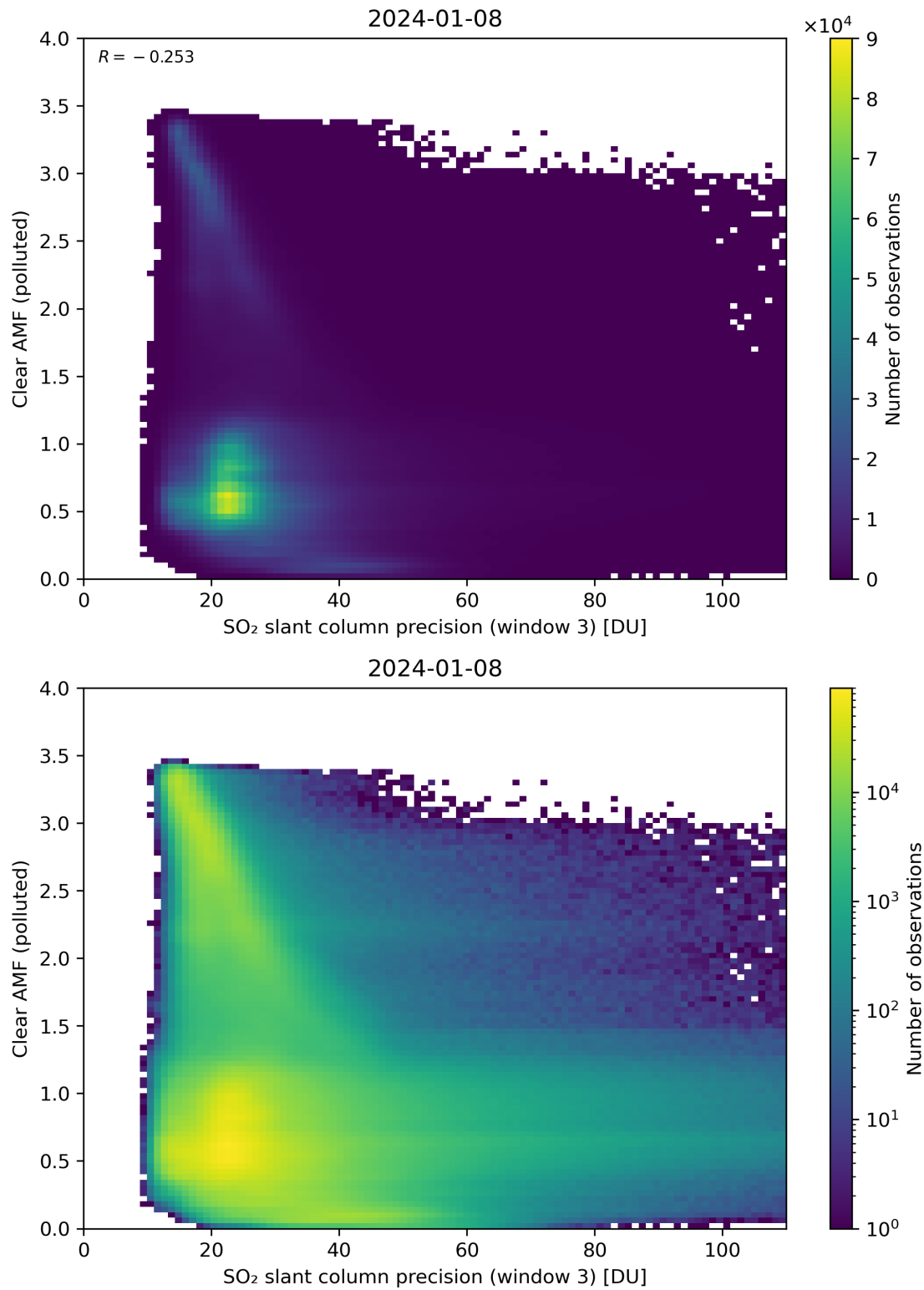
Figure 261: Scatter density plot of “SO 2 slant column precision (window 3)” against “Clear AMF (polluted)” for 2024-01-07 to 2024-01-09.
