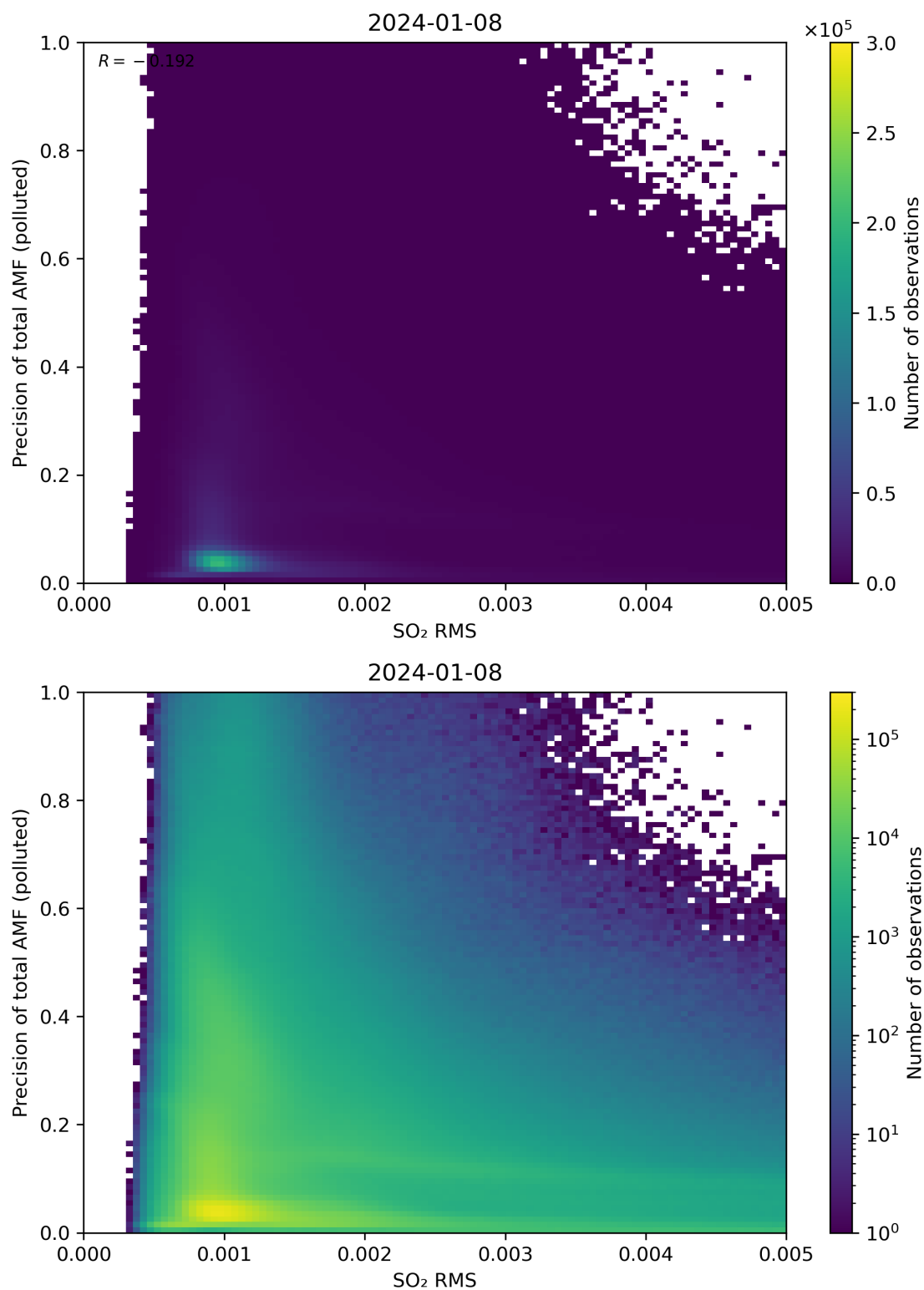
Figure 138: Scatter density plot of “SO 2 RMS” against “Precision of total AMF (polluted)” for 2024-01-07 to 2024-01-09.
