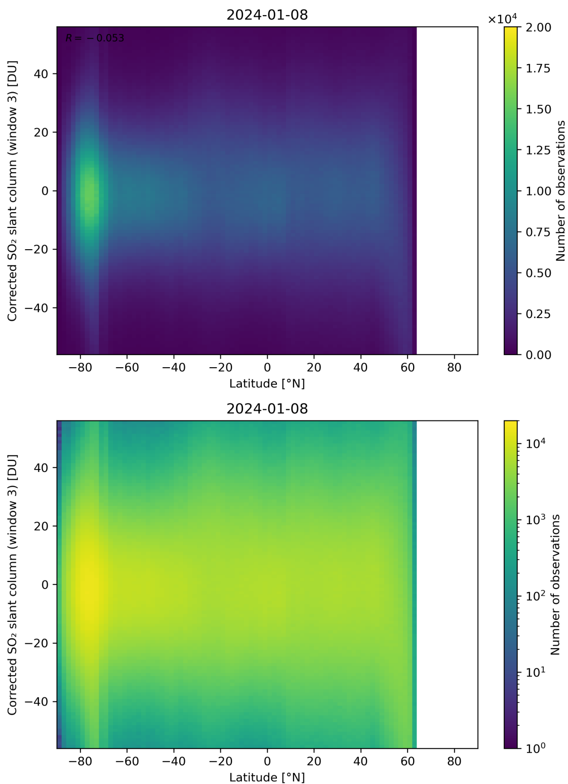
Figure 148: Scatter density plot of “Latitude” against “Corrected SO 2 slant column (window 3)” for 2024-01-07 to 2024-01-09.
