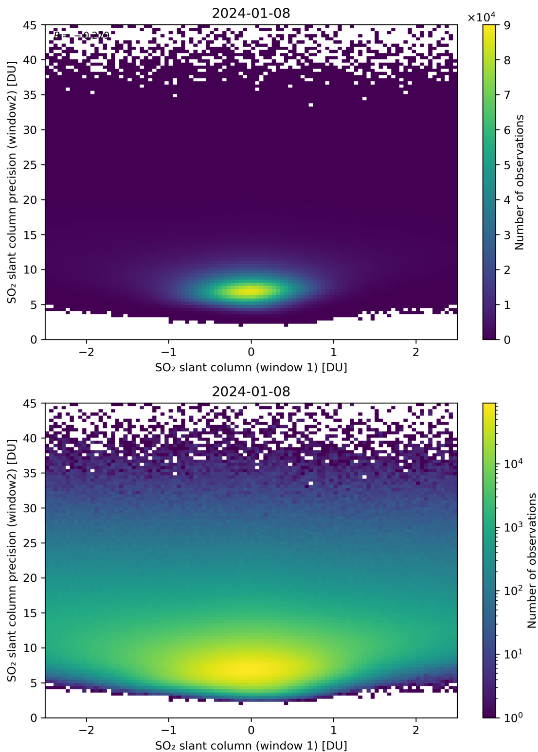
Figure 236: Scatter density plot of “SO 2 slant column (window 1)” against “SO 2 slant column precision (window2)” for 2024-01-07 to 2024-01-09.
