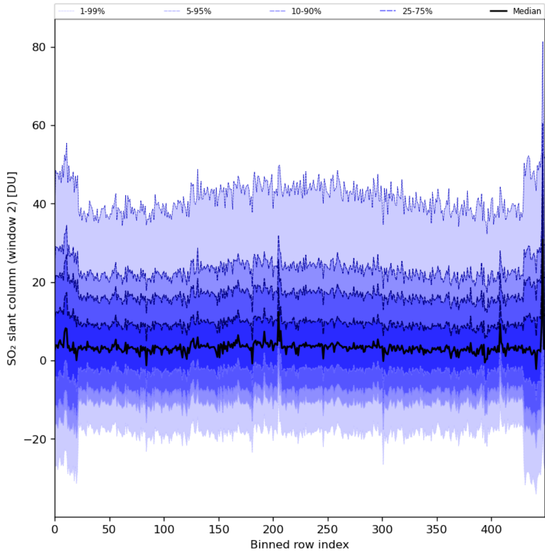
Figure 83: Along track statistics of “SO 2 slant column (window 2)” for 2024-01-07 to 2024-01-09
