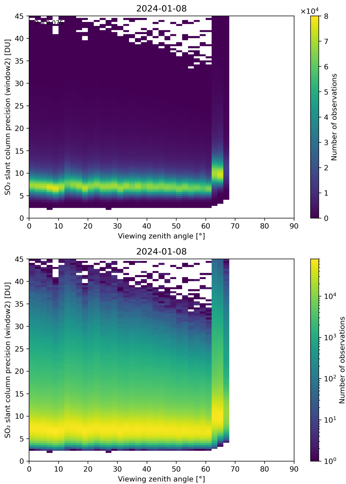
Figure 322: Scatter density plot of “Viewing zenith angle” against “SO 2 slant column precision (window2)” for 2024-01-07 to 2024-01-09.
