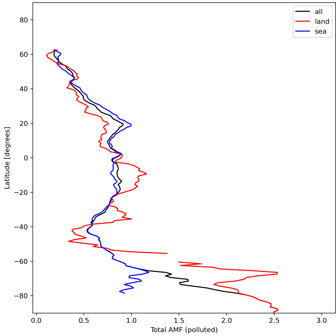
Figure 48: Zonal average of “Total AMF (polluted)” for 2024-01-07 to 2024-01-09.
