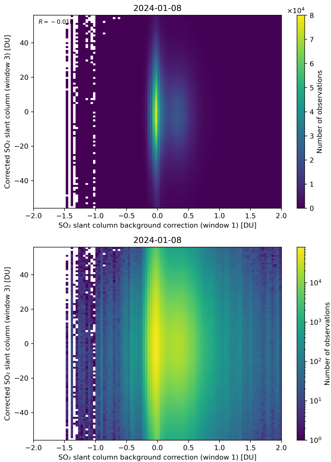
Figure 105: Scatter density plot of “SO 2 slant column background correction (window 1)” against “Corrected SO 2 slant column (window 3)” for 2024-01-07 to 2024-01-09.
