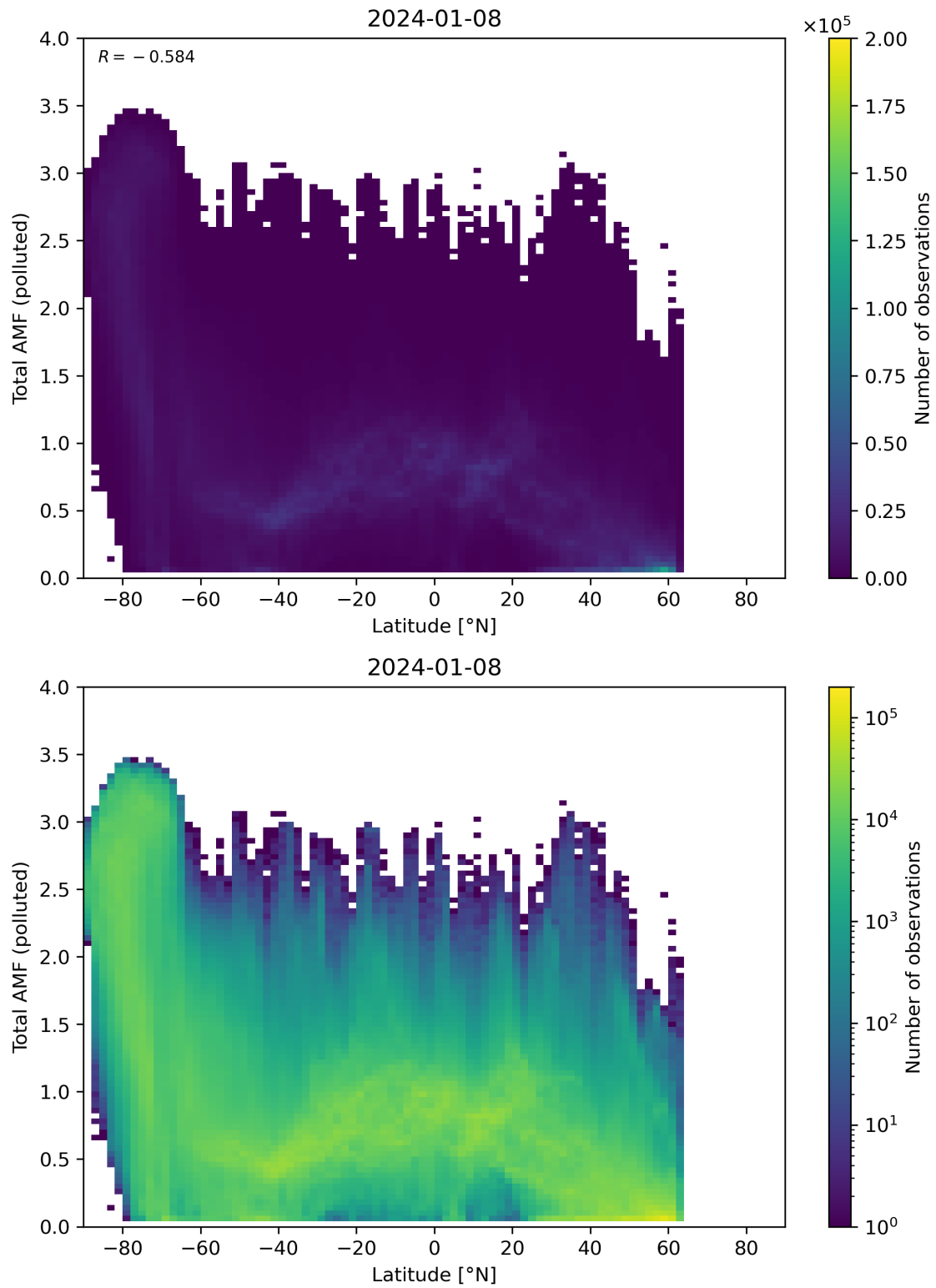
Figure 154: Scatter density plot of “Latitude” against “Total AMF (polluted)” for 2024-01-07 to 2024-01-09.
