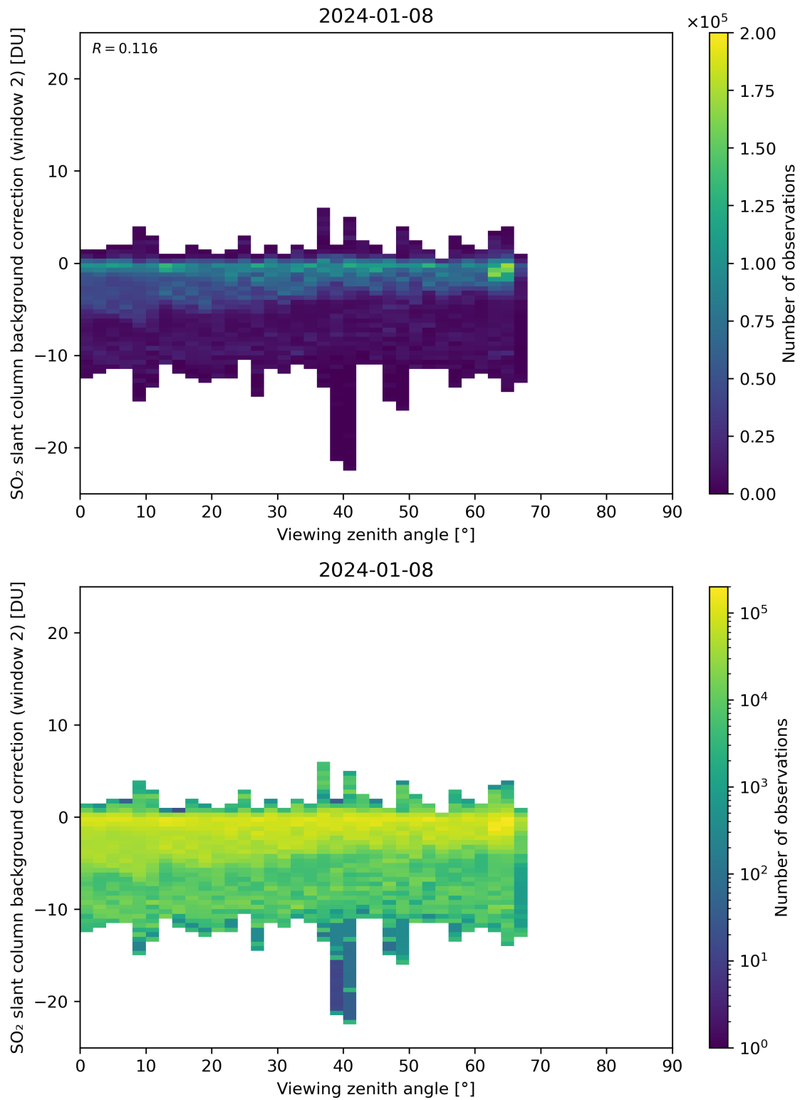
Figure 309: Scatter density plot of “Viewing zenith angle” against “SO 2 slant column background correction (window 2)” for 2024-01-07 to 2024-01-09.
