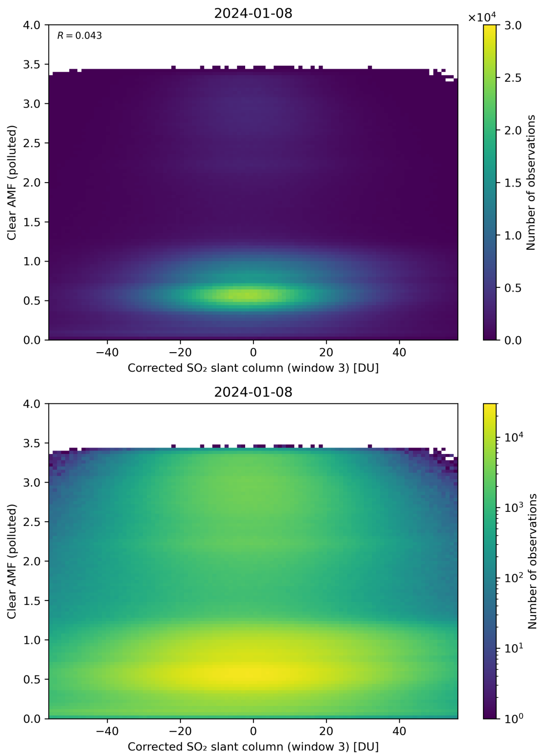
Figure 209: Scatter density plot of “Corrected SO 2 slant column (window 3)” against “Clear AMF (polluted)” for 2024-01-07 to 2024-01-09.
