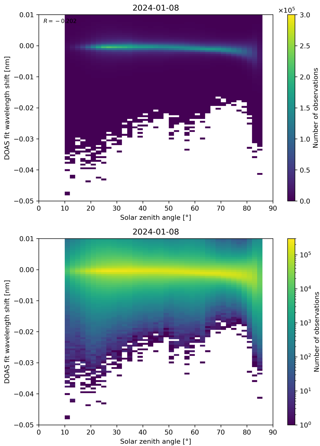
Figure 161: Scatter density plot of “Solar zenith angle” against “DOAS fit wavelength shift” for 2024-01-07 to 2024-01-09.
