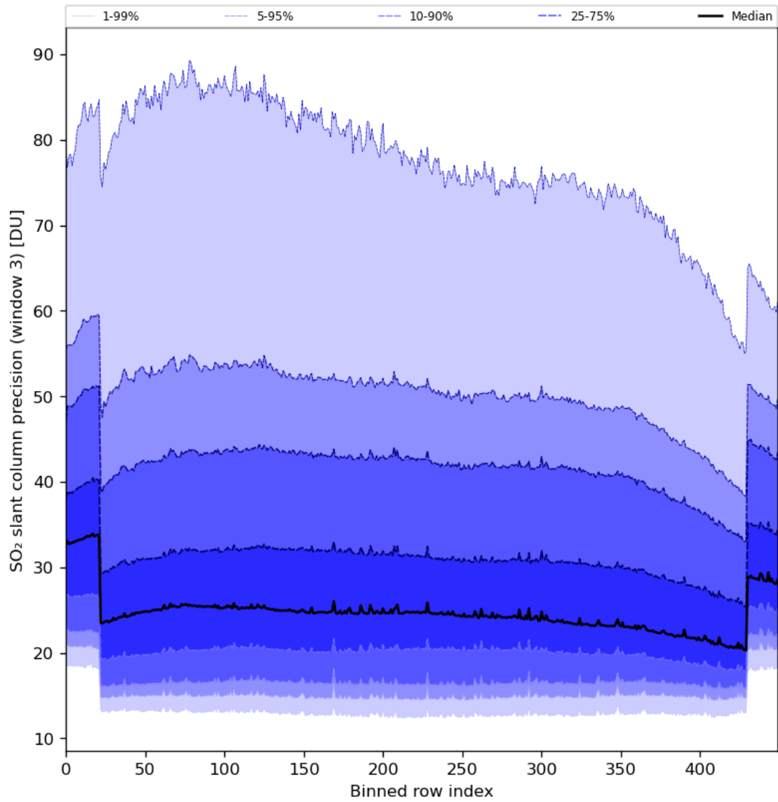
Figure 88: Along track statistics of “SO 2 slant column precision (window 3)” for 2024-01-07 to 2024-01-09
