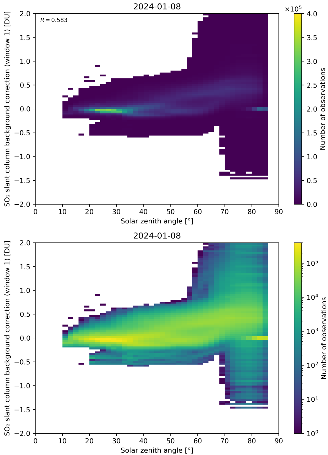
Figure 158: Scatter density plot of “Solar zenith angle” against “SO 2 slant column background correction (window 1)” for 2024-01-07 to 2024-01-09.
