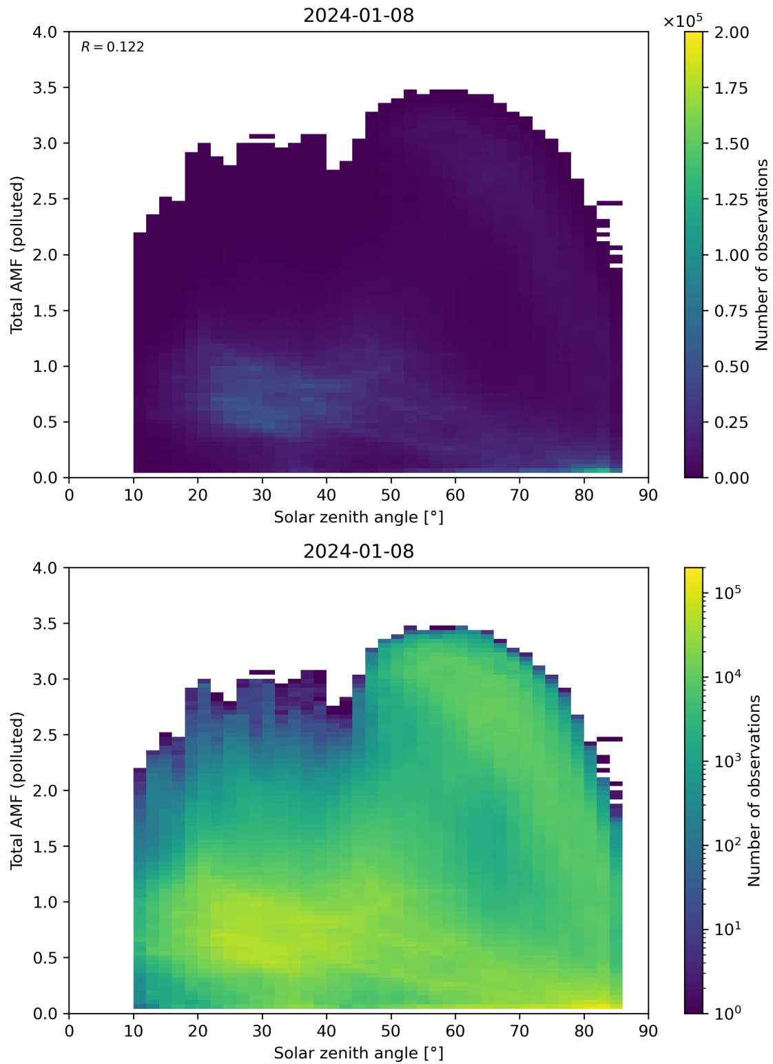
Figure 174: Scatter density plot of “Solar zenith angle” against “Total AMF (polluted)” for 2024-01-07 to 2024-01-09.
