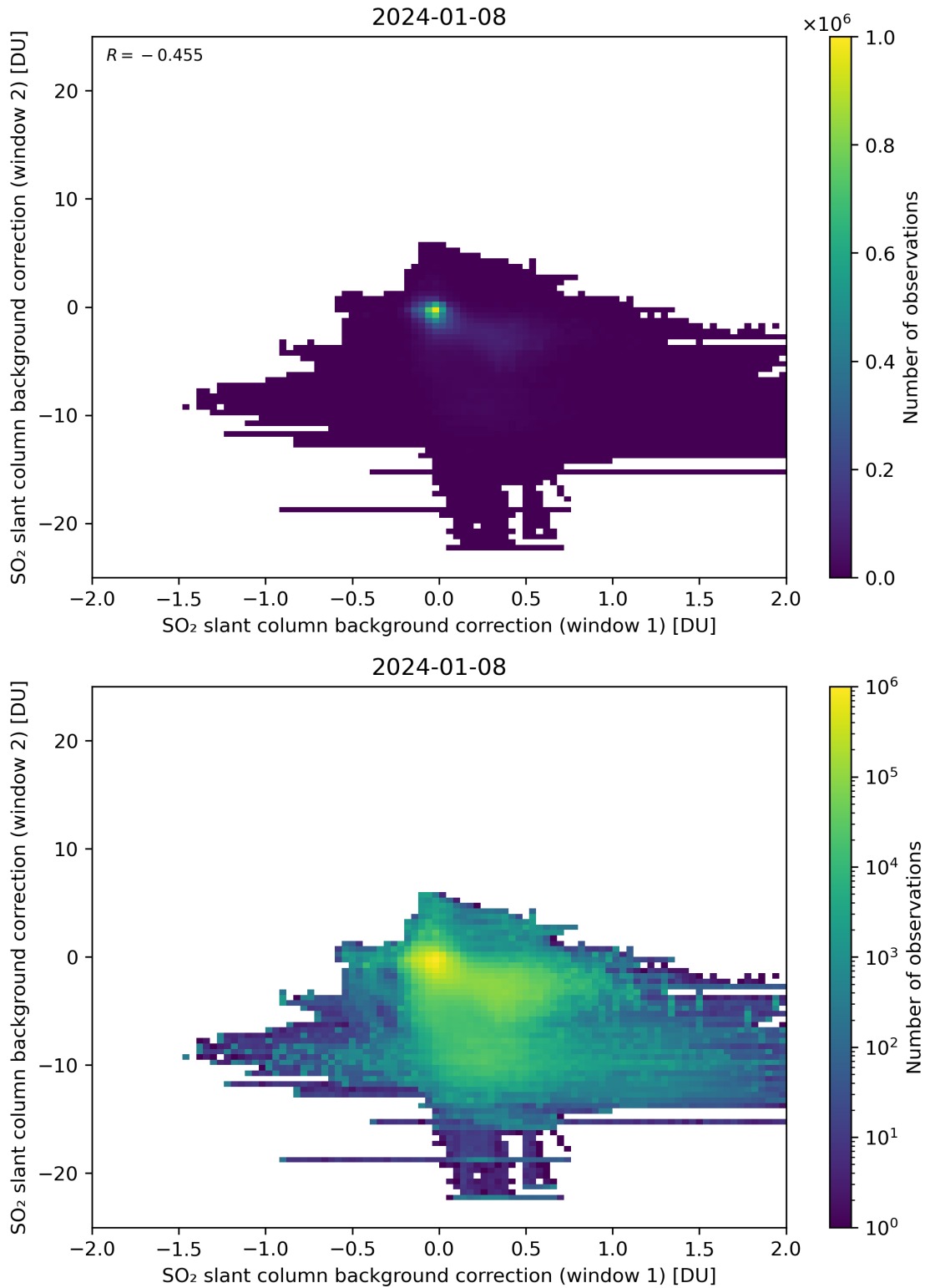
Figure 98: Scatter density plot of “SO 2 slant column background correction (window 1)” against “SO 2 slant column background correction (window 2)” for 2024-01-07 to 2024-01-09.
