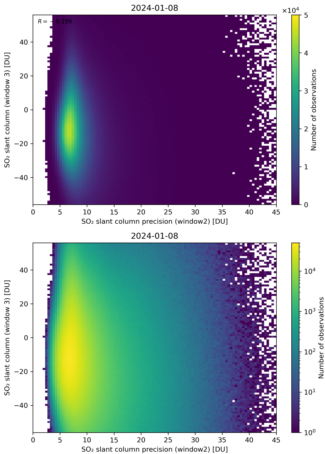
Figure 249: Scatter density plot of “SO 2 slant column precision (window2)” against “SO 2 slant column (window 3)” for 2024-01-07 to 2024-01-09.
