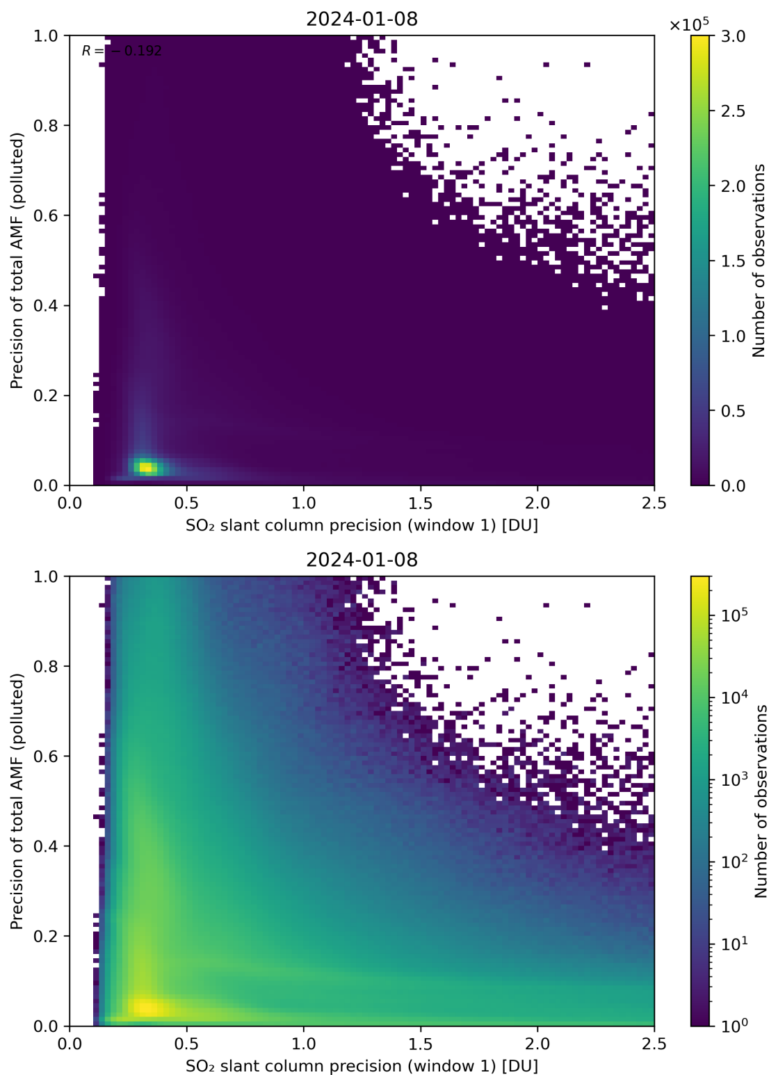
Figure 231: Scatter density plot of “SO 2 slant column precision (window 1)” against “Precision of total AMF (polluted)” for 2024-01-07 to 2024-01-09.
