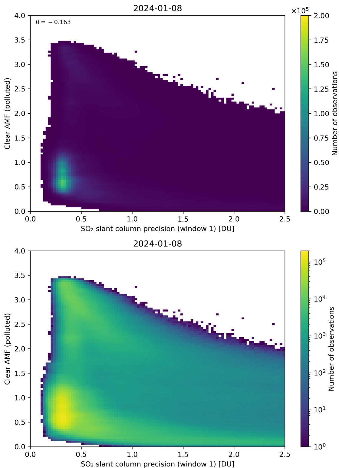
Figure 224: Scatter density plot of “SO 2 slant column precision (window 1)” against “Clear AMF (polluted)” for 2024-01-07 to 2024-01-09.
