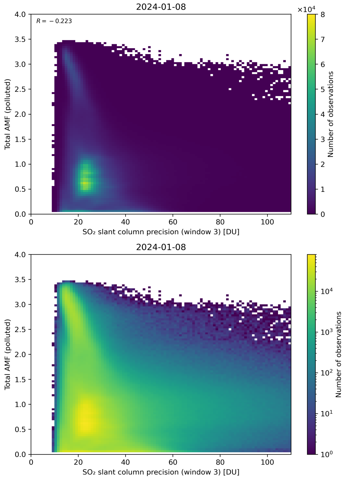
Figure 263: Scatter density plot of “SO 2 slant column precision (window 3)” against “Total AMF (polluted)” for 2024-01-07 to 2024-01-09.
