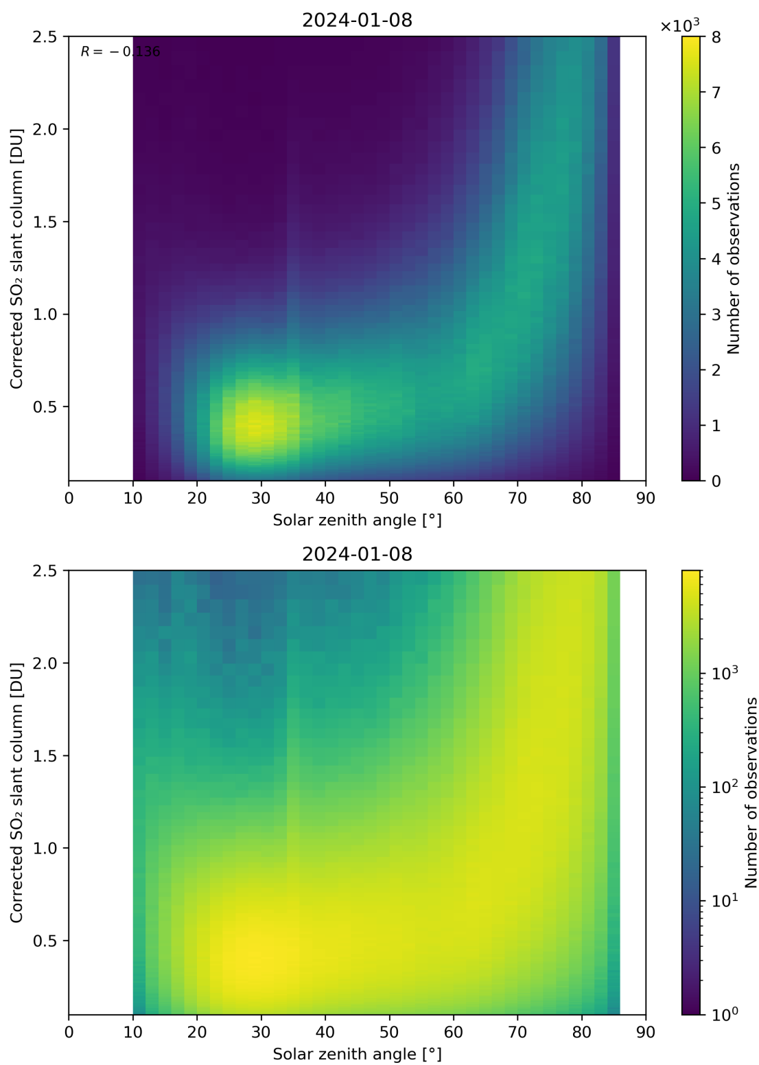
Figure 166: Scatter density plot of “Solar zenith angle” against “Corrected SO 2 slant column” for 2024-01-07 to 2024-01-09.
