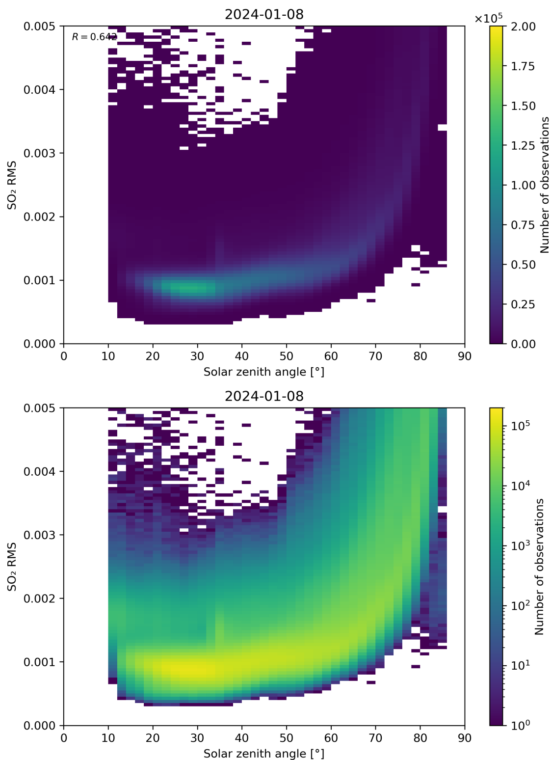
Figure 163: Scatter density plot of “Solar zenith angle” against “SO 2 RMS” for 2024-01-07 to 2024-01-09.
