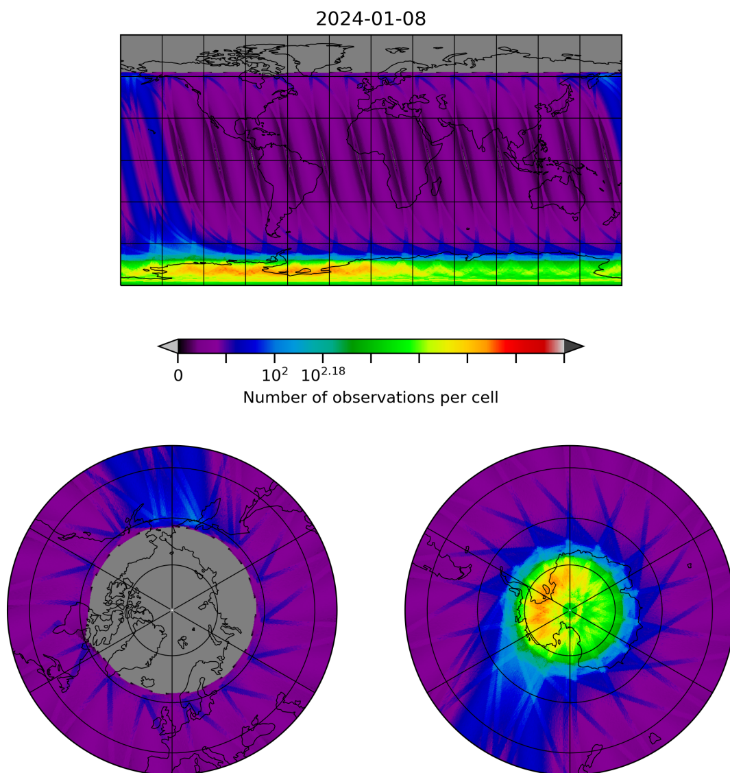
Figure 28: Map of the number of observations for 2024-01-07 to 2024-01-09
