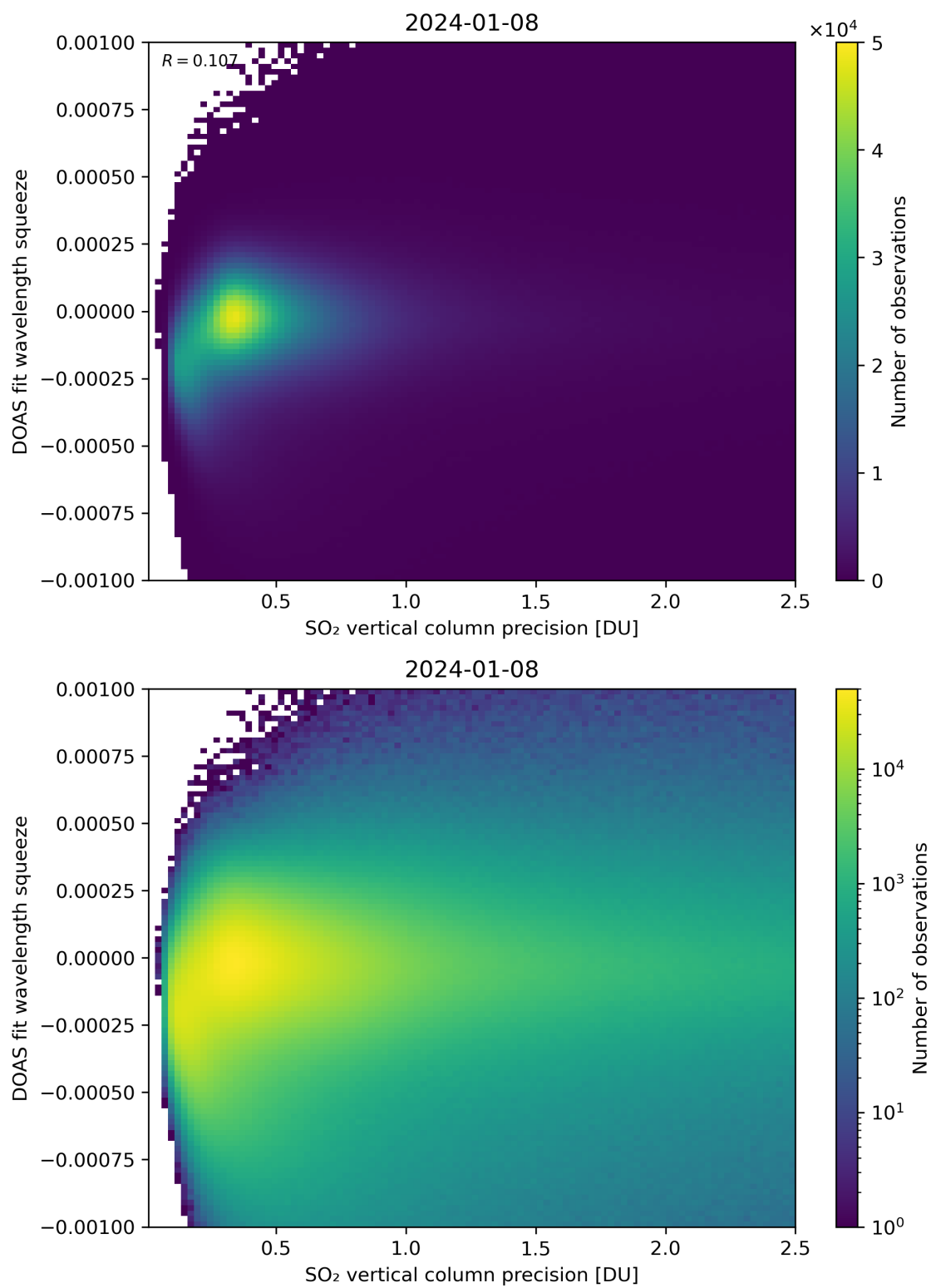
Figure 283: Scatter density plot of “SO 2 vertical column precision” against “DOAS fit wavelength squeeze” for 2024-01-07 to 2024-01-09.
