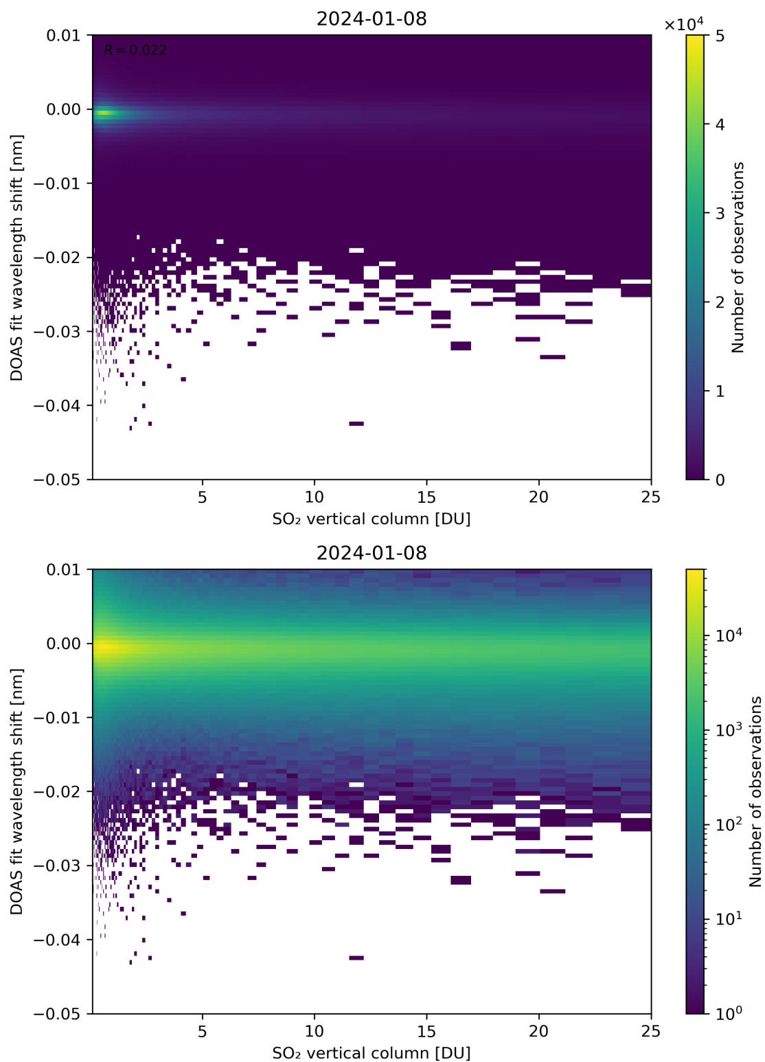
Figure 276: Scatter density plot of “SO 2 vertical column” against “DOAS fit wavelength shift” for 2024-01-07 to 2024-01-09.
