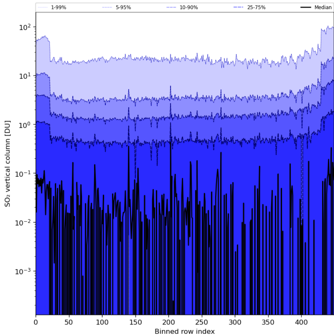
Figure 76: Along track statistics of “SO 2 vertical column” for 2024-01-07 to 2024-01-09
