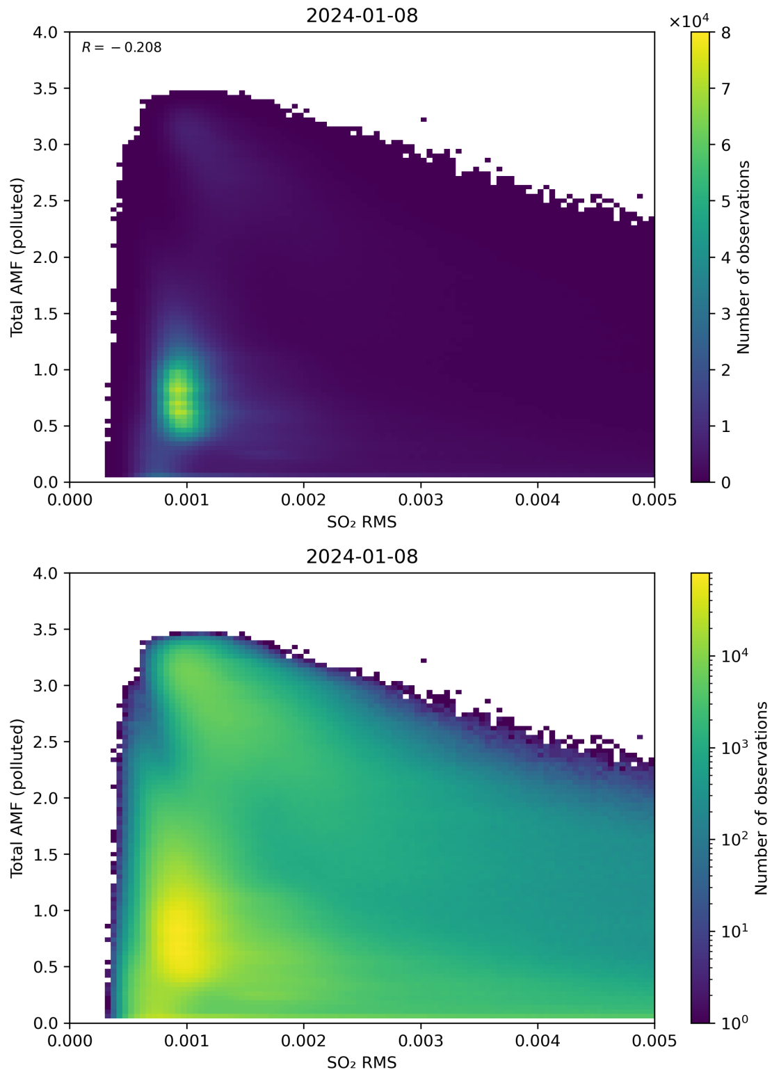
Figure 137: Scatter density plot of “SO 2 RMS” against “Total AMF (polluted)” for 2024-01-07 to 2024-01-09.
