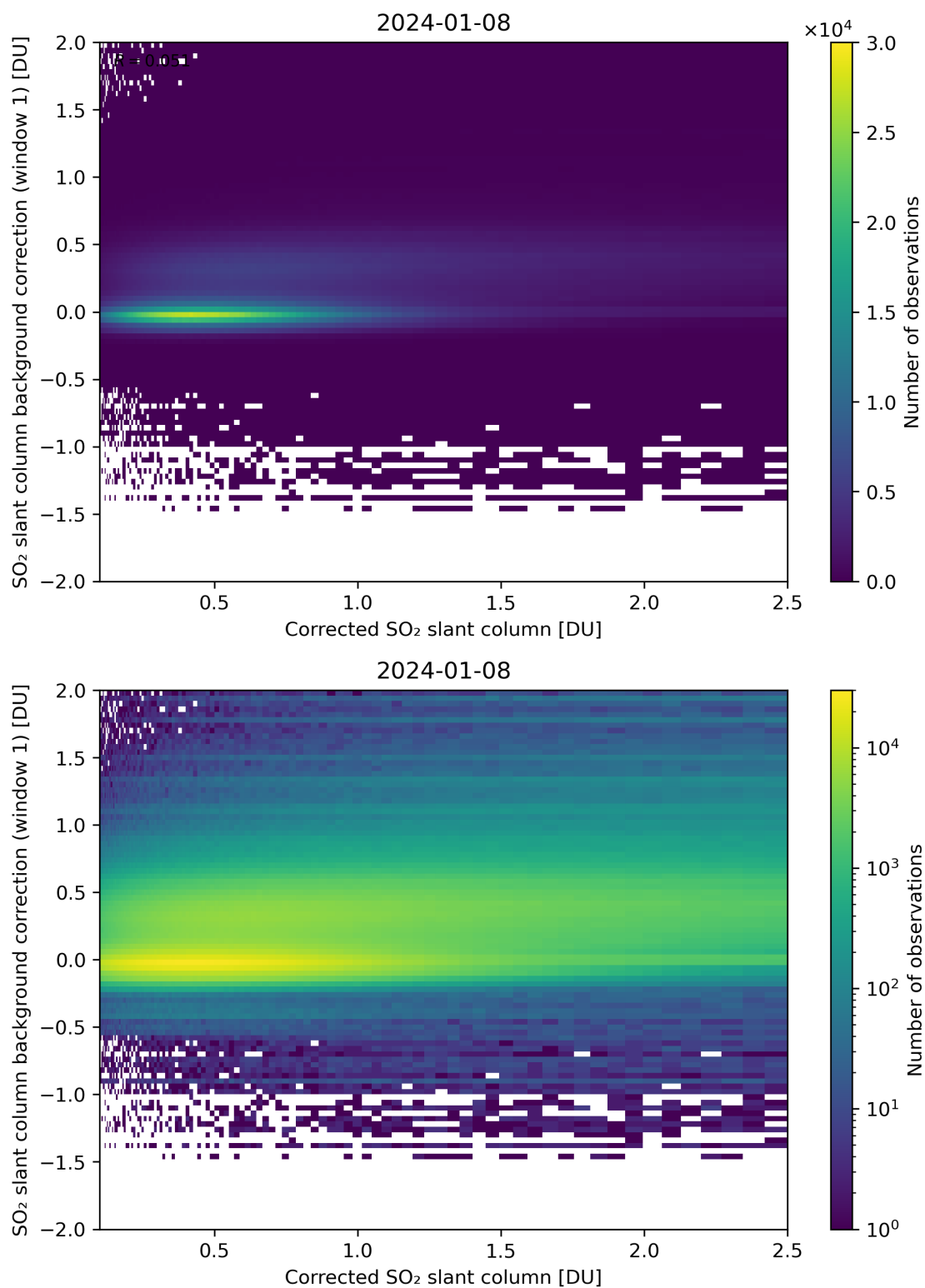
Figure 178: Scatter density plot of “Corrected SO 2 slant column” against “SO 2 slant column background correction (window 1)” for 2024-01-07 to 2024-01-09.
