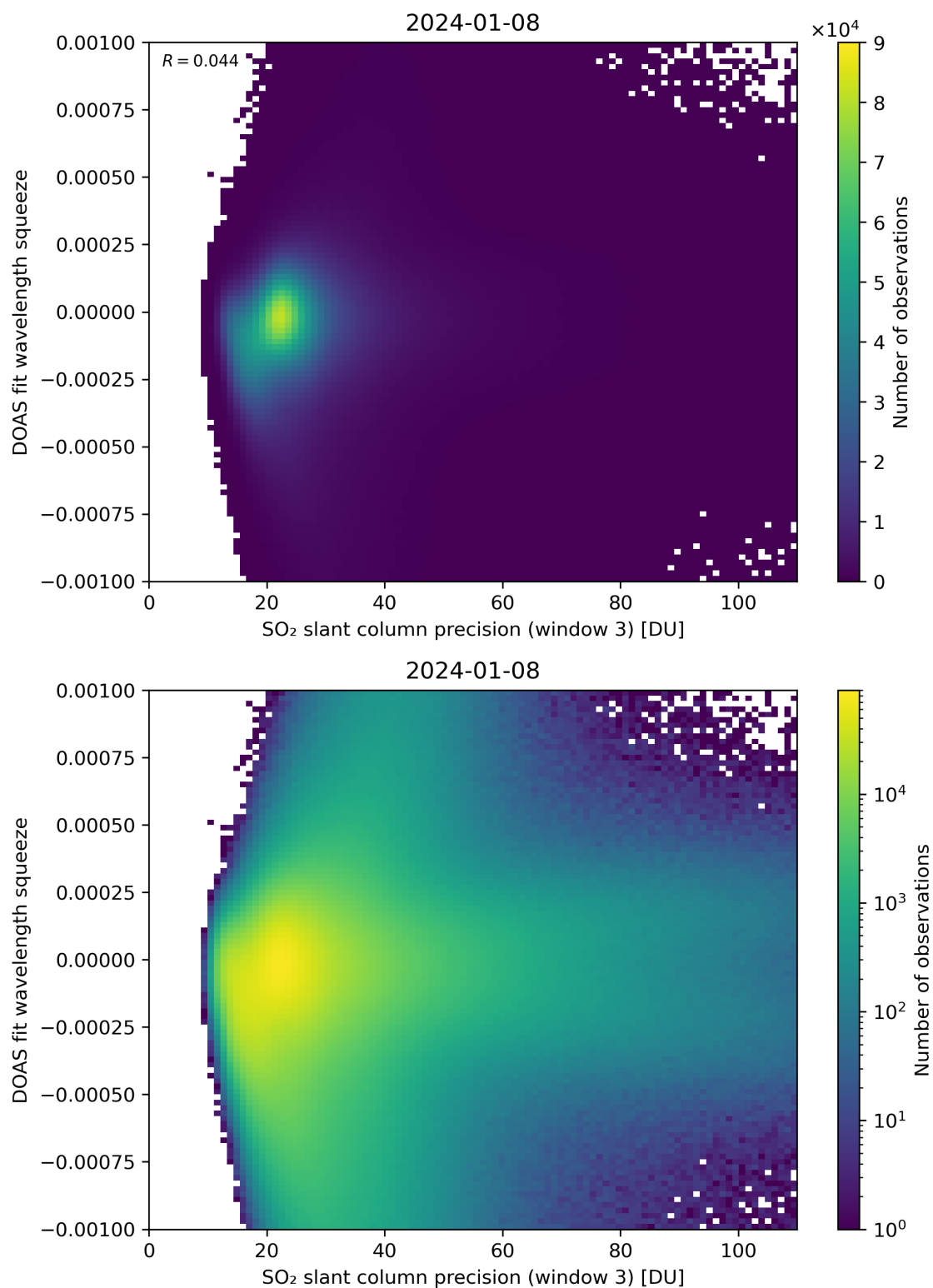
Figure 259: Scatter density plot of “SO 2 slant column precision (window 3)” against “DOAS fit wavelength squeeze” for 2024-01-07 to 2024-01-09.
