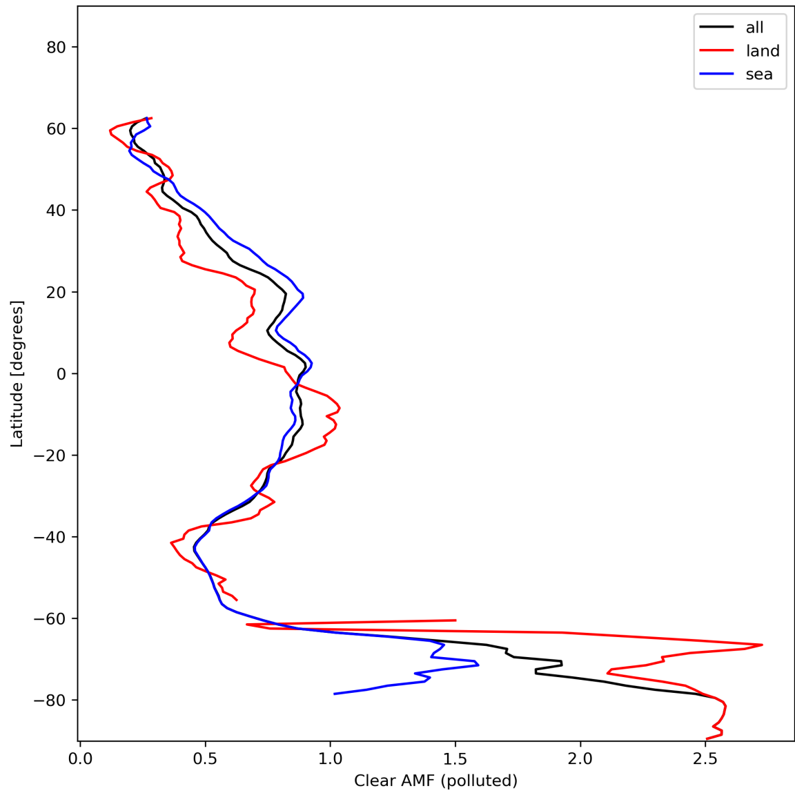
Figure 50: Zonal average of “Clear AMF (polluted)” for 2024-01-07 to 2024-01-09.
