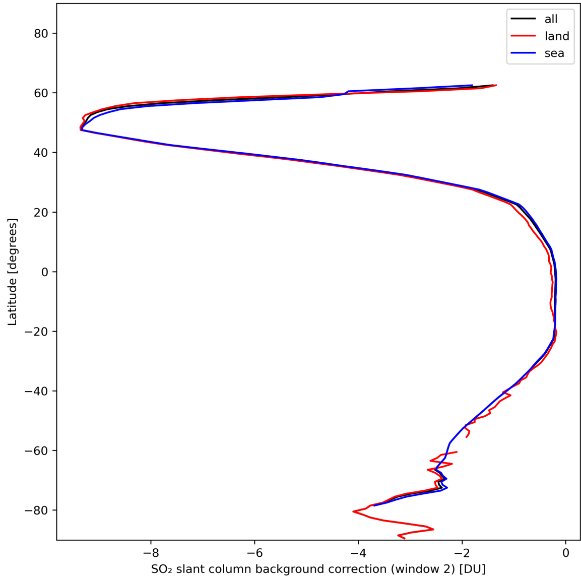
Figure 40: Zonal average of “SO 2 slant column background correction (window 2)” for 2024-01-07 to 2024-01-09.
