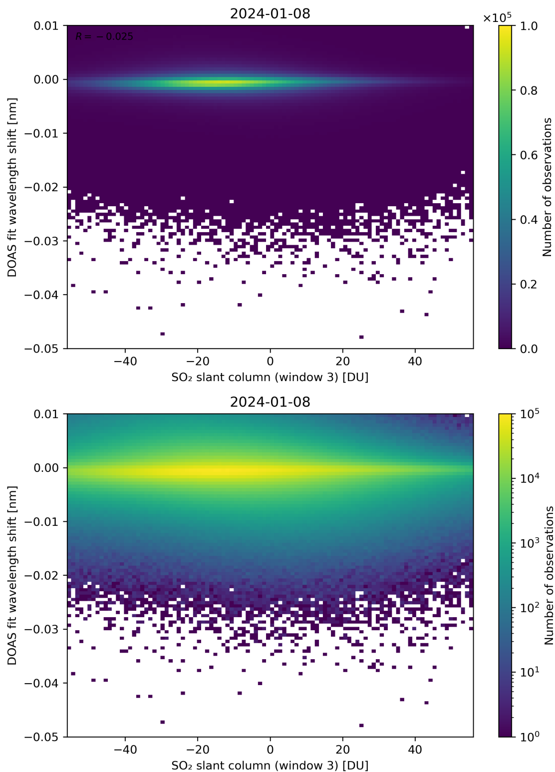
Figure 254: Scatter density plot of “SO 2 slant column (window 3)” against “DOAS fit wavelength shift” for 2024-01-07 to 2024-01-09.
