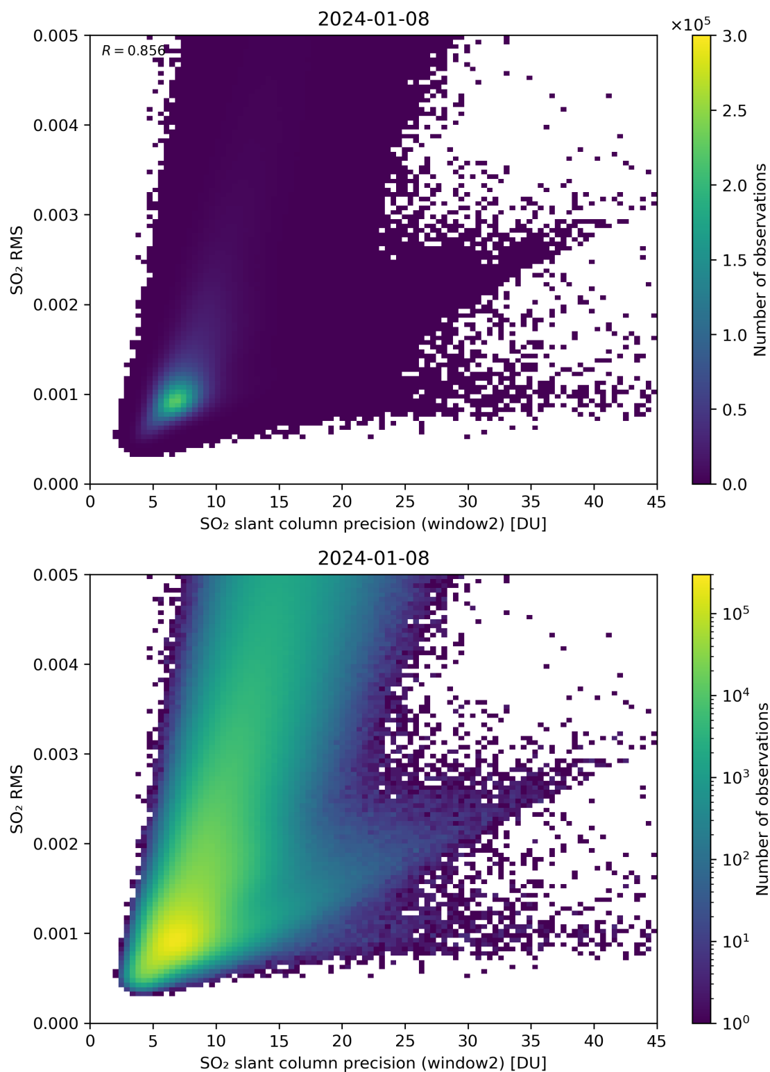
Figure 245: Scatter density plot of “SO 2 slant column precision (window2)” against “SO 2 RMS” for 2024-01-07 to 2024-01-09.
