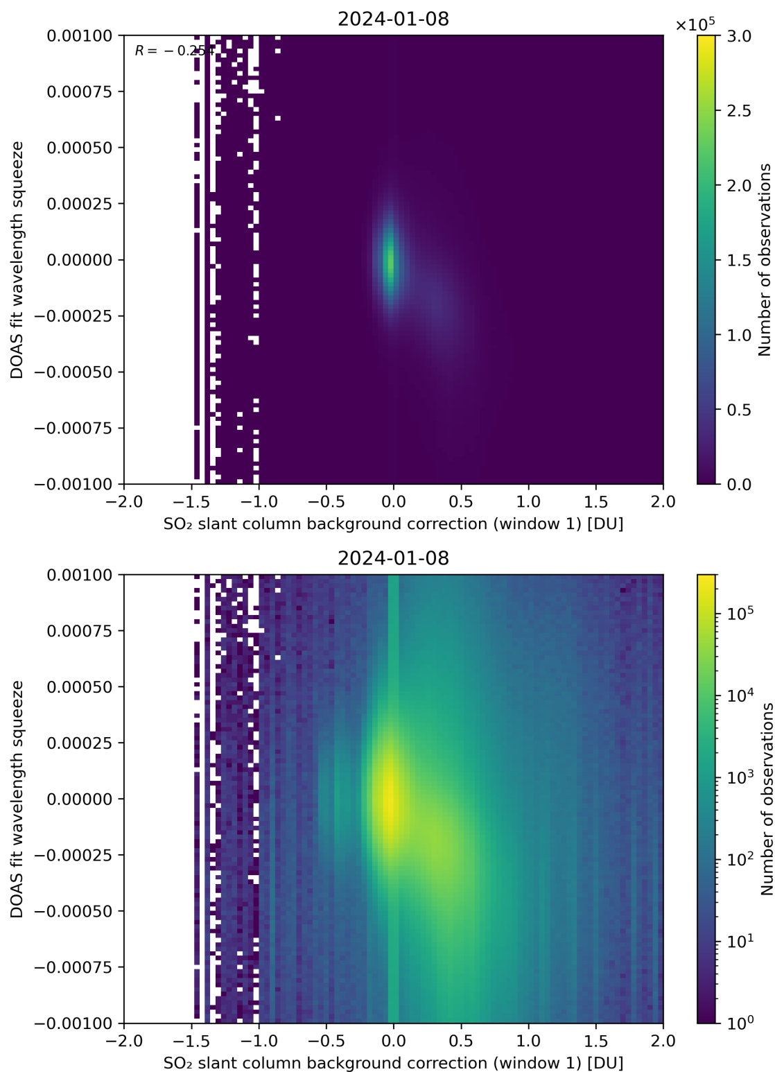
Figure 101: Scatter density plot of “SO 2 slant column background correction (window 1)” against “DOAS fit wavelength squeeze” for 2024-01-07 to 2024-01-09.
