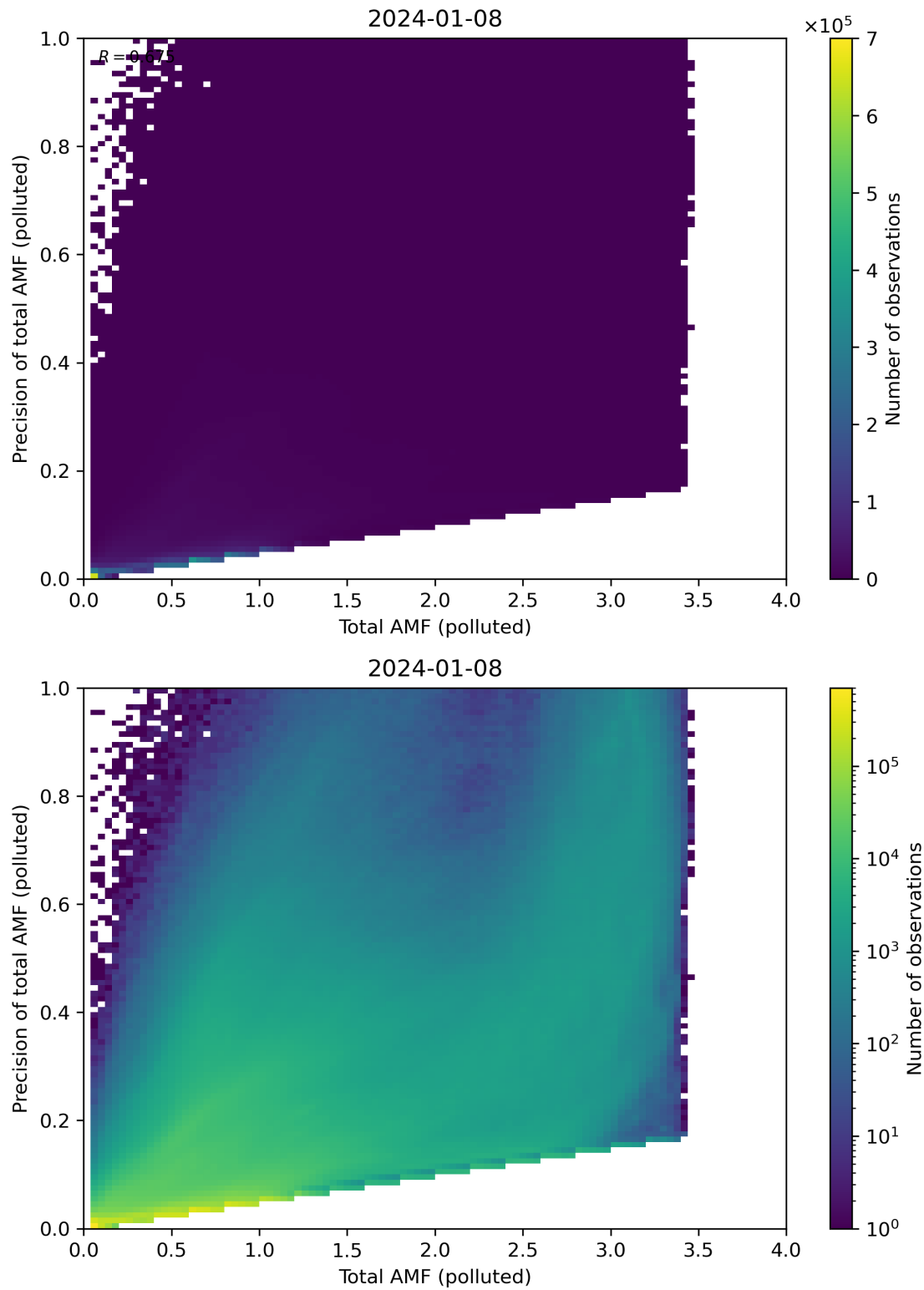
Figure 272: Scatter density plot of “Total AMF (polluted)” against “Precision of total AMF (polluted)” for 2024-01-07 to 2024-01-09.
