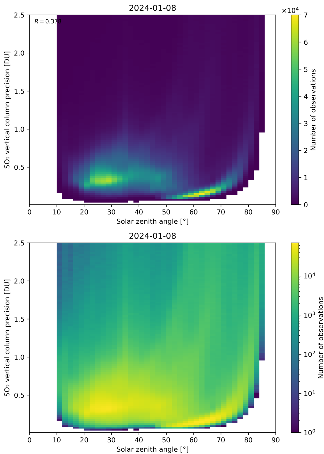
Figure 177: Scatter density plot of “Solar zenith angle” against “SO 2 vertical column precision” for 2024-01-07 to 2024-01-09.
