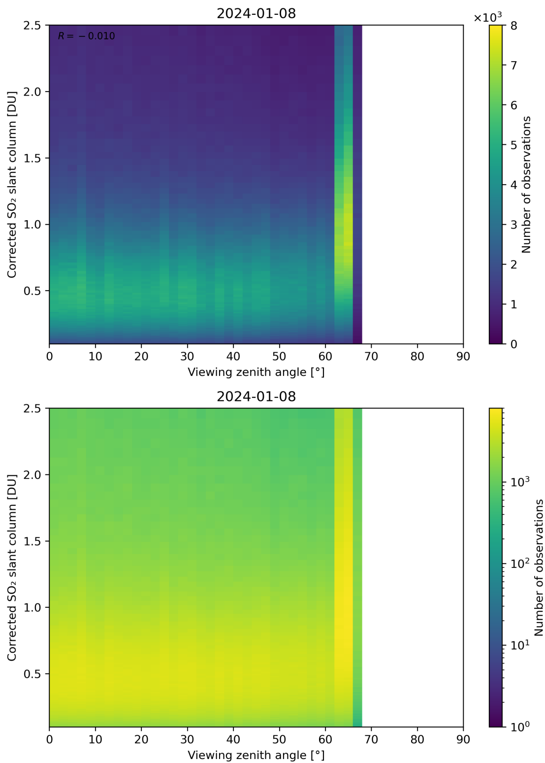
Figure 317: Scatter density plot of “Viewing zenith angle” against “Corrected SO 2 slant column” for 2024-01-07 to 2024-01-09.
