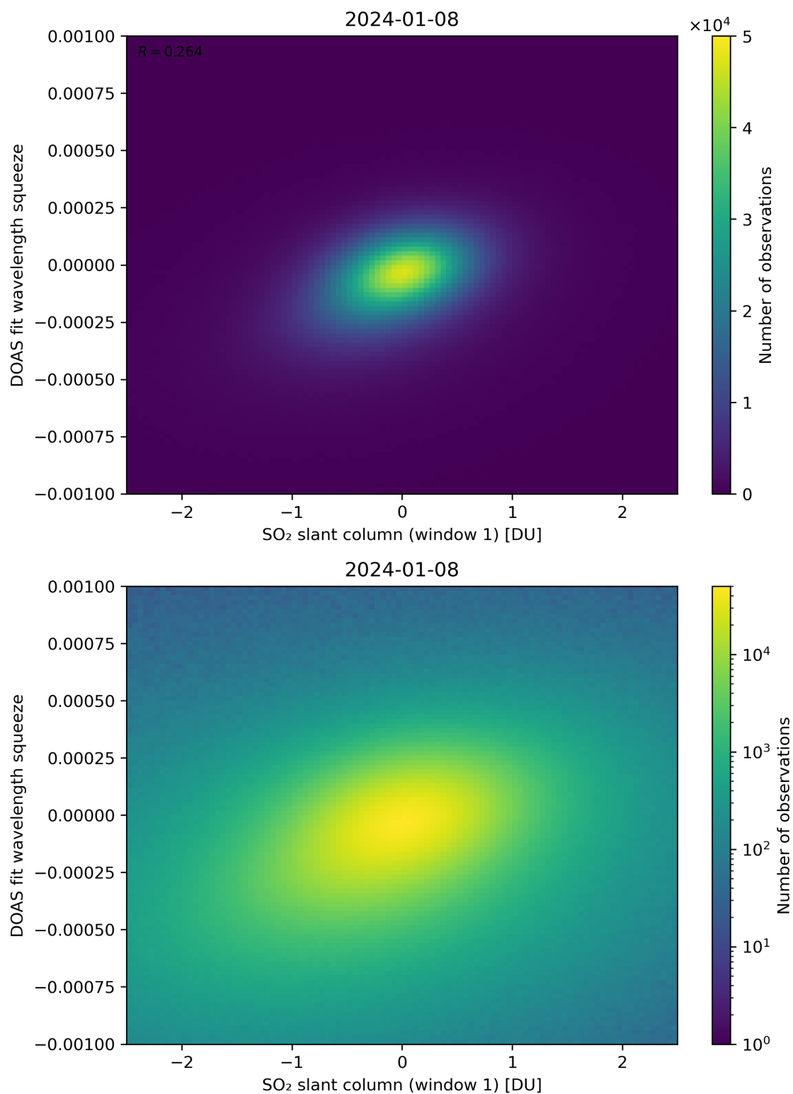
Figure 216: Scatter density plot of “SO 2 slant column (window 1)” against “DOAS fit wavelength squeeze” for 2024-01-07 to 2024-01-09.
