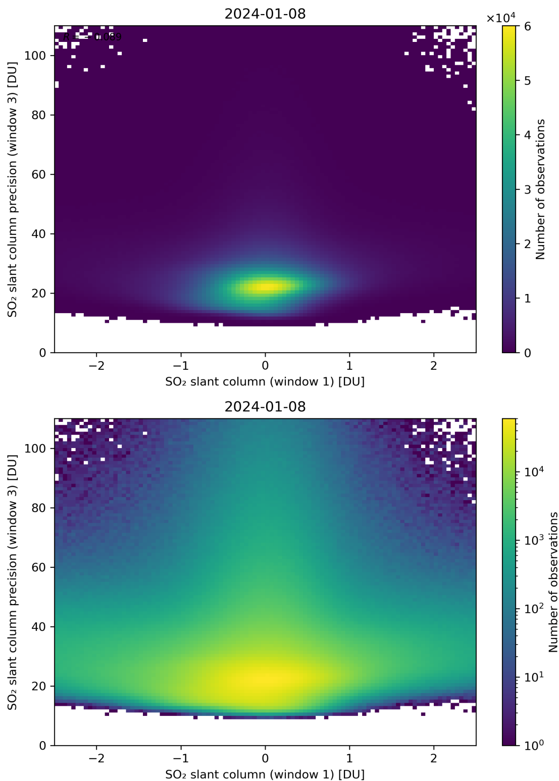
Figure 238: Scatter density plot of “SO 2 slant column (window 1)” against “SO 2 slant column precision (window 3)” for 2024-01-07 to 2024-01-09.
