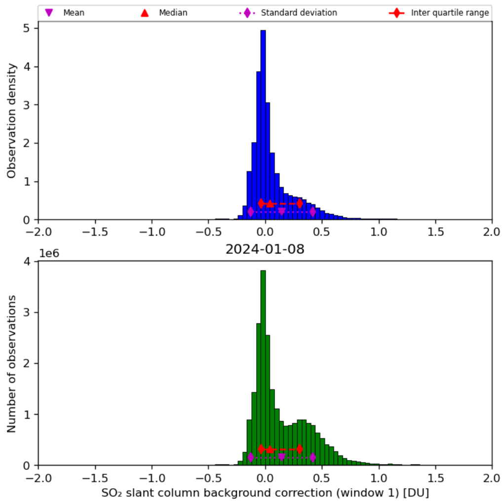
Figure 59: Histogram of “SO 2 slant column background correction (window 1)” for 2024-01-07 to 2024-01-09
