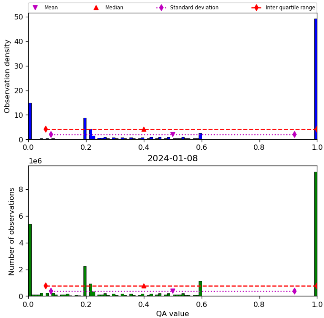
Figure 52: Histogram of “QA value” for 2024-01-07 to 2024-01-09
