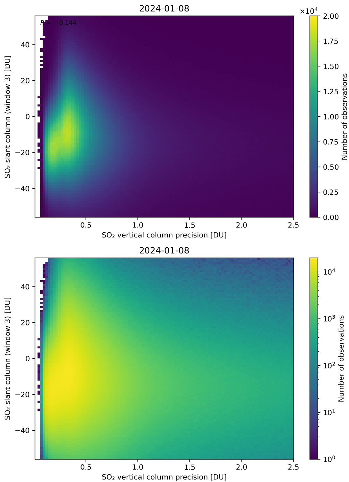
Figure 292: Scatter density plot of “SO 2 vertical column precision” against “SO 2 slant column (window 3)” for 2024-01-07 to 2024-01-09.
