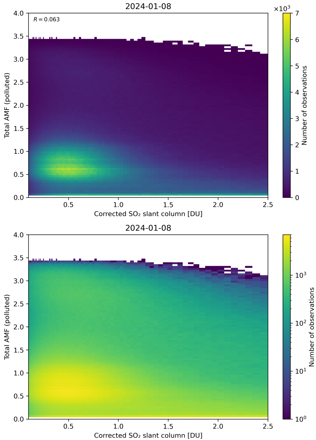
Figure 192: Scatter density plot of “Corrected SO 2 slant column” against “Total AMF (polluted)” for 2024-01-07 to 2024-01-09.
