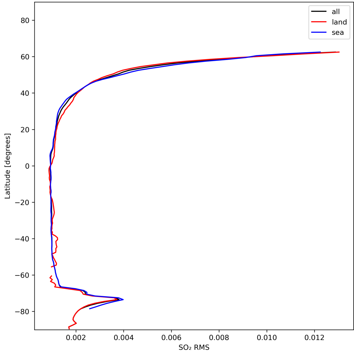
Figure 47: Zonal average of “SO 2 RMS” for 2024-01-07 to 2024-01-09.
