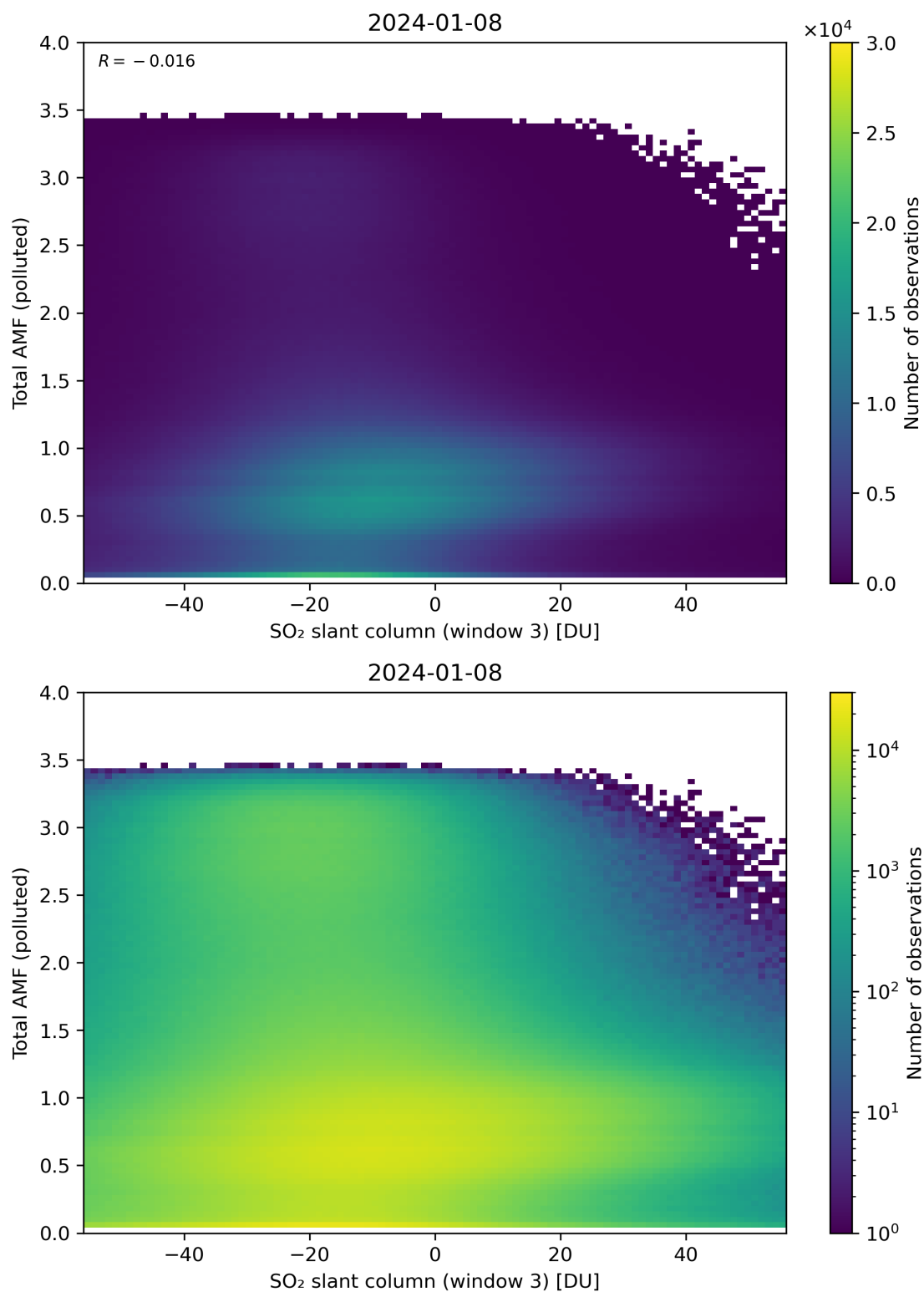
Figure 268: Scatter density plot of “SO 2 slant column (window 3)” against “Total AMF (polluted)” for 2024-01-07 to 2024-01-09.
