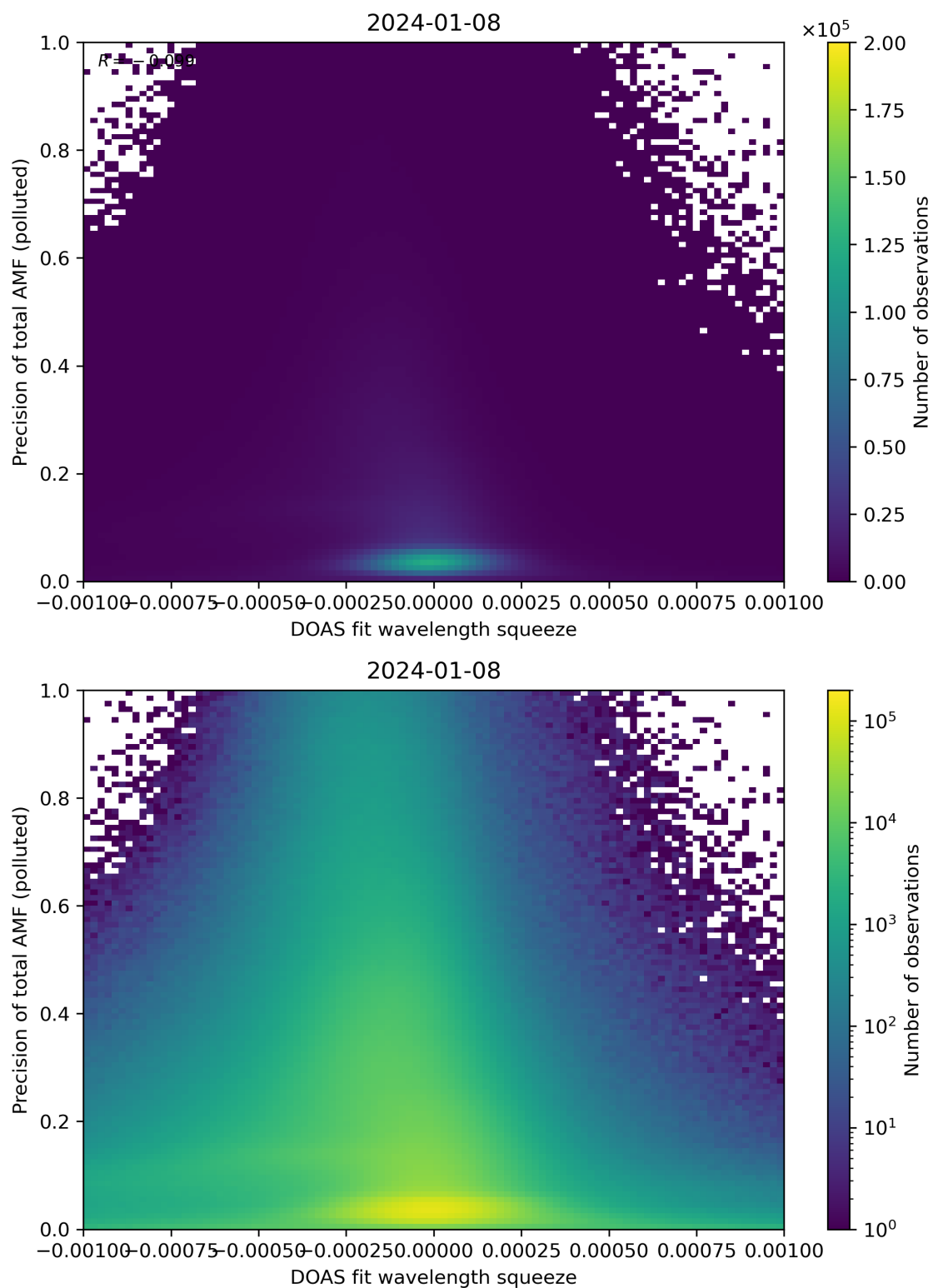
Figure 135: Scatter density plot of “DOAS fit wavelength squeeze” against “Precision of total AMF (polluted)” for 2024-01-07 to 2024-01-09.
