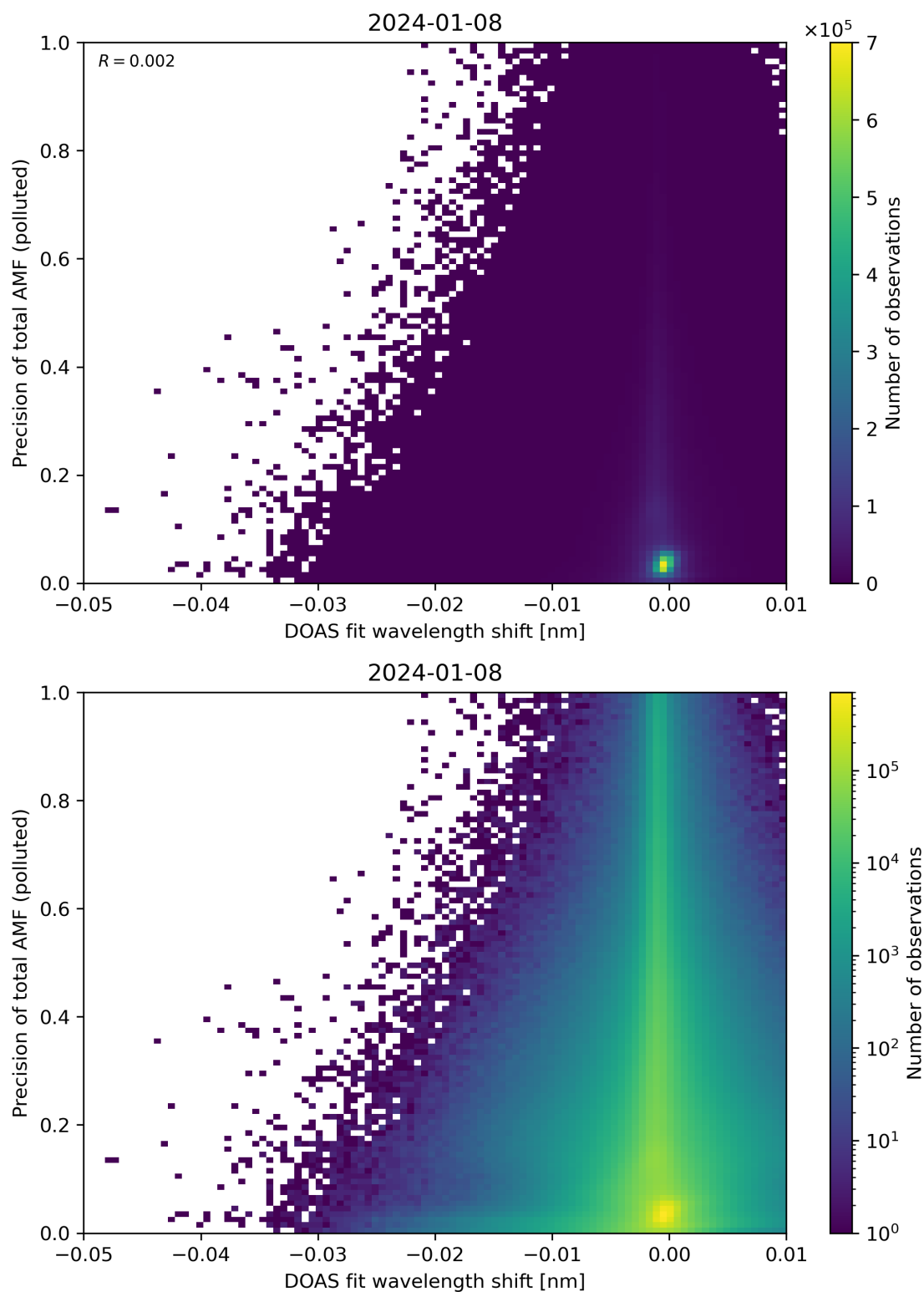
Figure 131: Scatter density plot of “DOAS fit wavelength shift” against “Precision of total AMF (polluted)” for 2024-01-07 to 2024-01-09.
