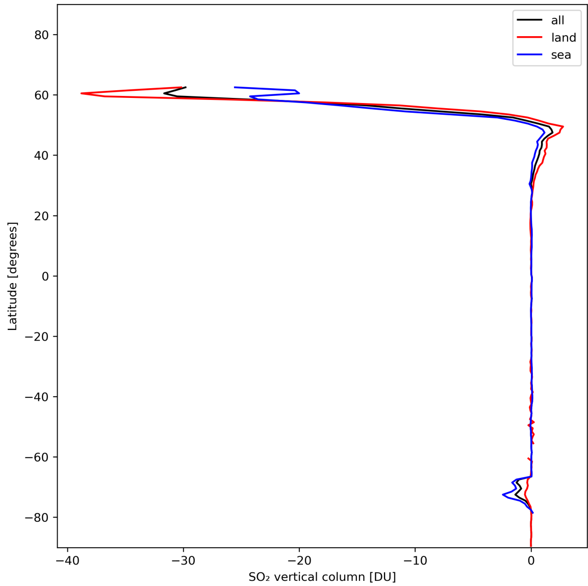
Figure 30: Zonal average of “SO 2 vertical column” for 2024-01-07 to 2024-01-09.
