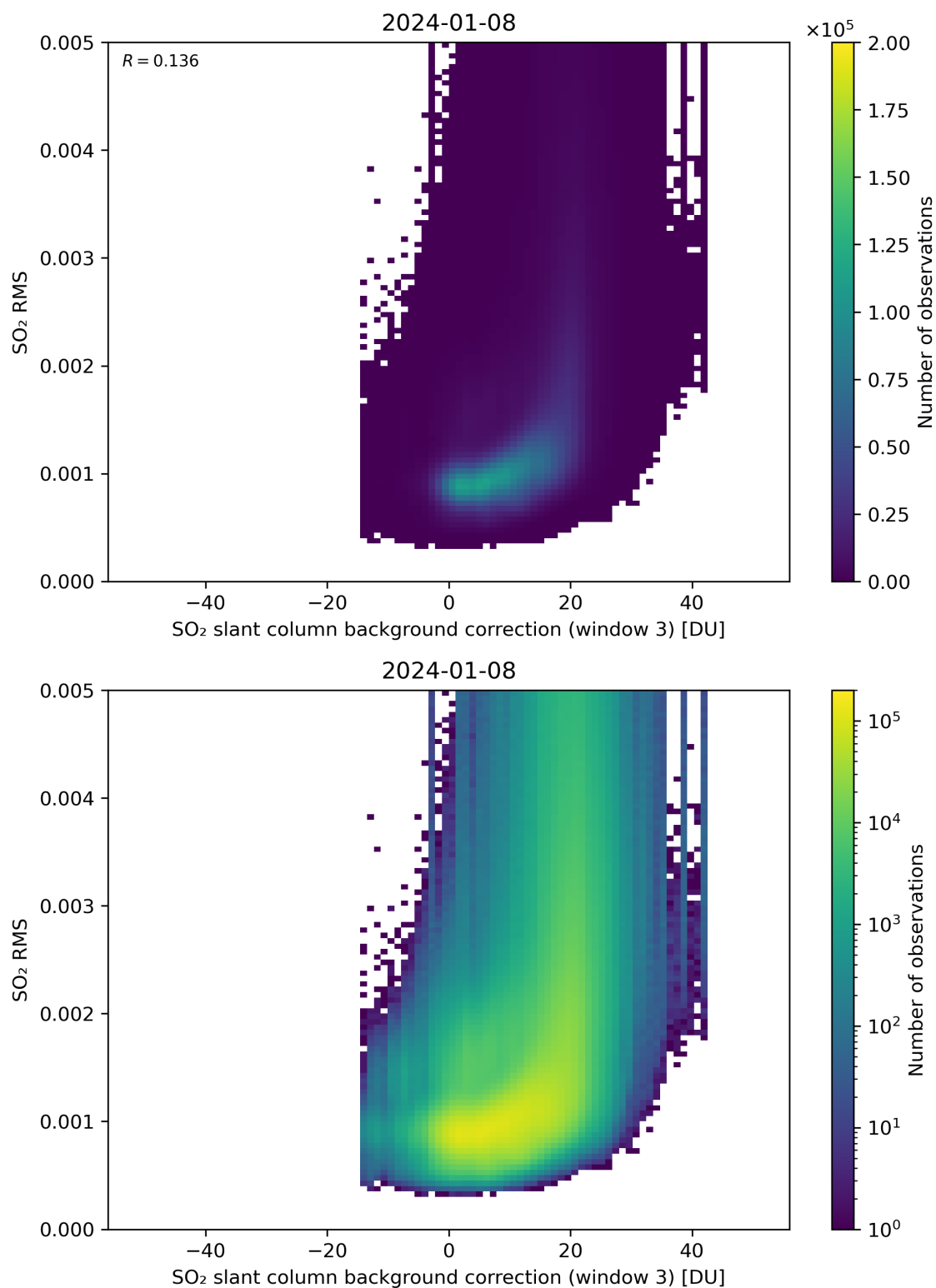
Figure 123: Scatter density plot of “SO 2 slant column background correction (window 3)” against “SO 2 RMS” for 2024-01-07 to 2024-01-09.
