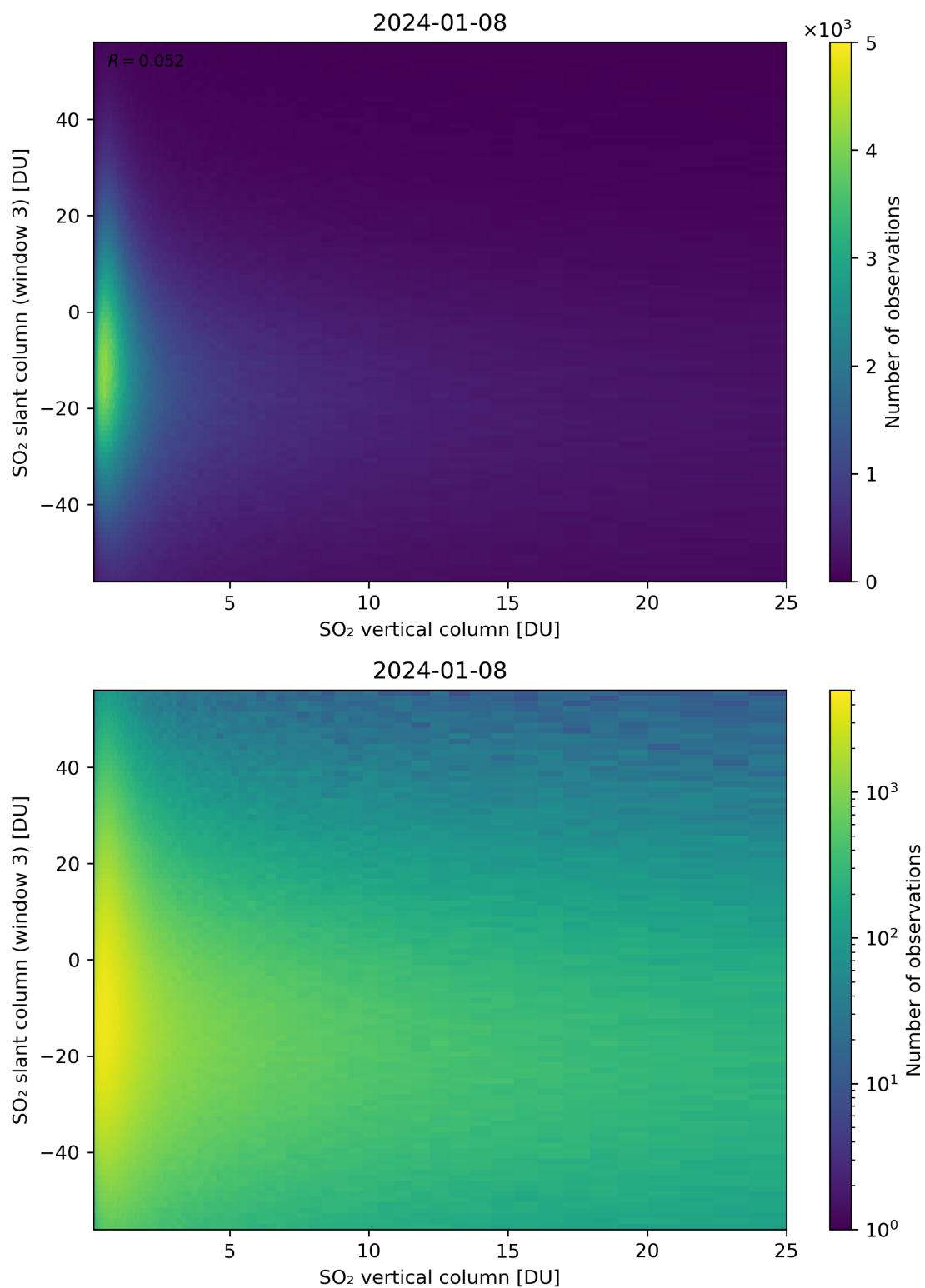
Figure 303: Scatter density plot of “SO 2 vertical column” against “SO 2 slant column (window 3)” for 2024-01-07 to 2024-01-09.
