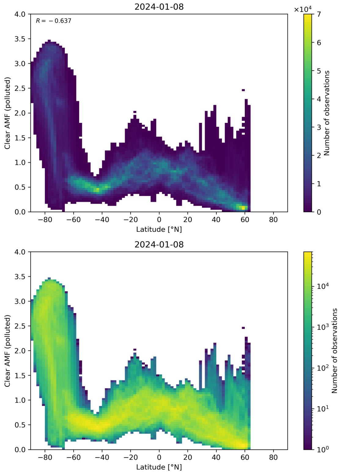
Figure 145: Scatter density plot of “Latitude” against “Clear AMF (polluted)” for 2024-01-07 to 2024-01-09.
