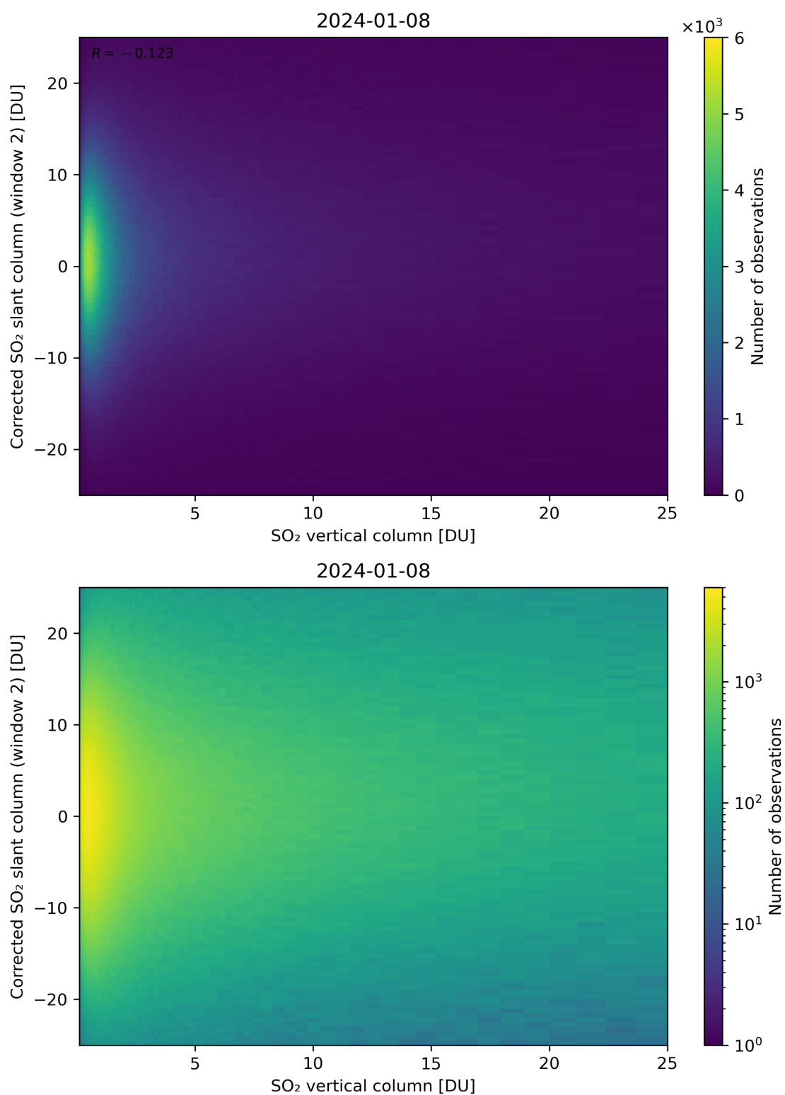
Figure 298: Scatter density plot of “SO 2 vertical column” against “Corrected SO 2 slant column (window 2)” for 2024-01-07 to 2024-01-09.
