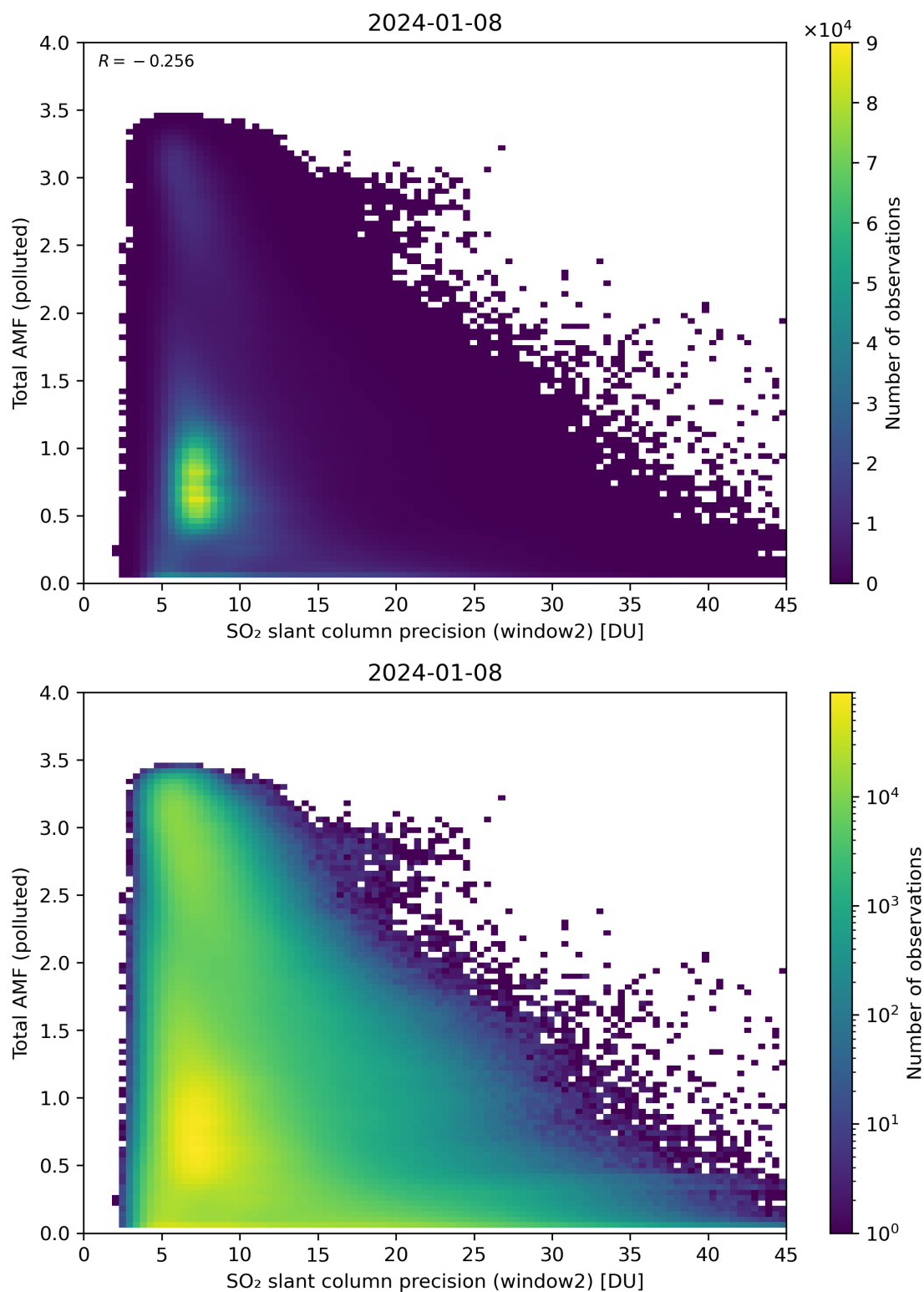
Figure 251: Scatter density plot of “SO 2 slant column precision (window2)” against “Total AMF (polluted)” for 2024-01-07 to 2024-01-09.
