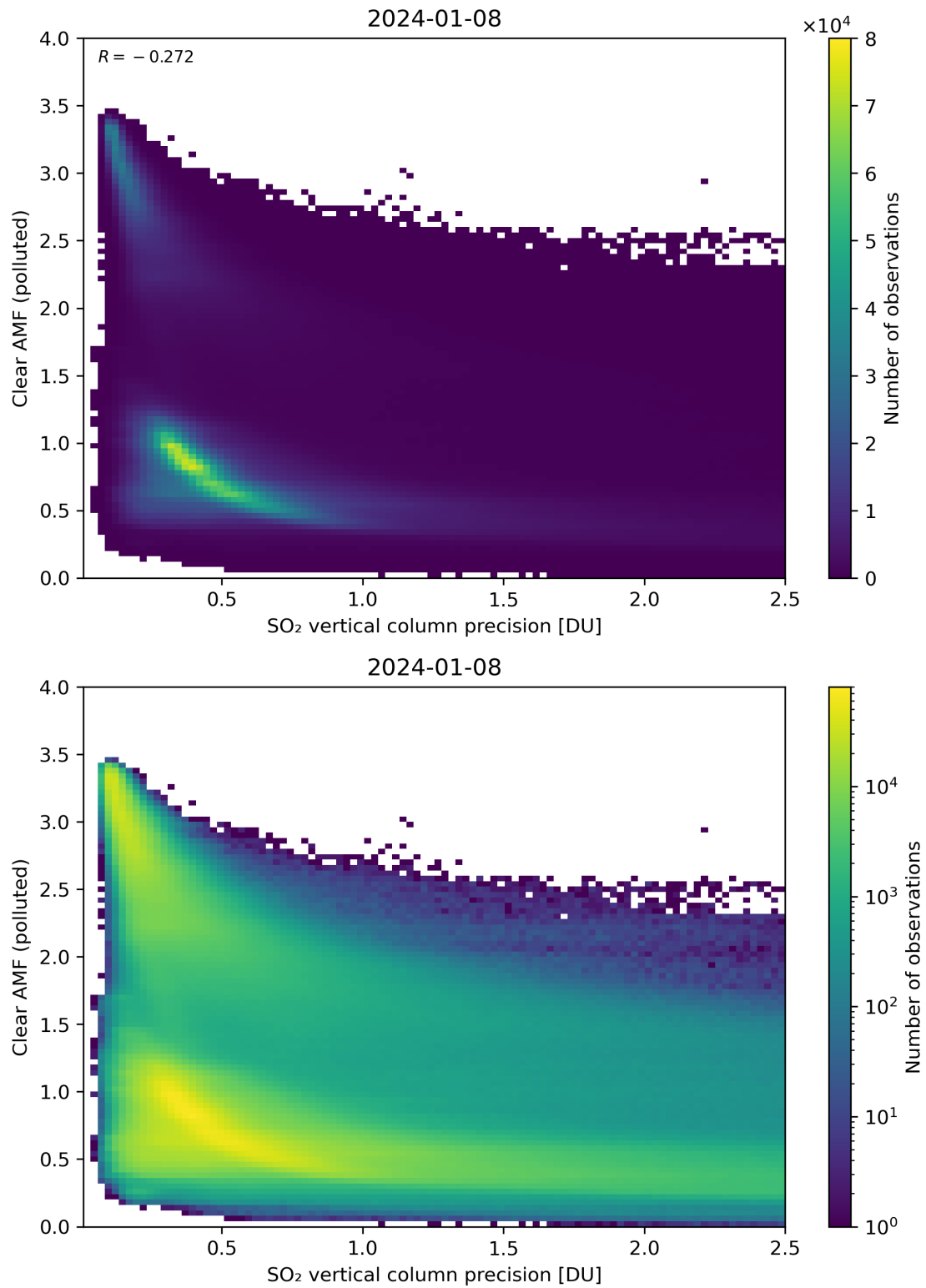
Figure 285: Scatter density plot of “SO 2 vertical column precision” against “Clear AMF (polluted)” for 2024-01-07 to 2024-01-09.
