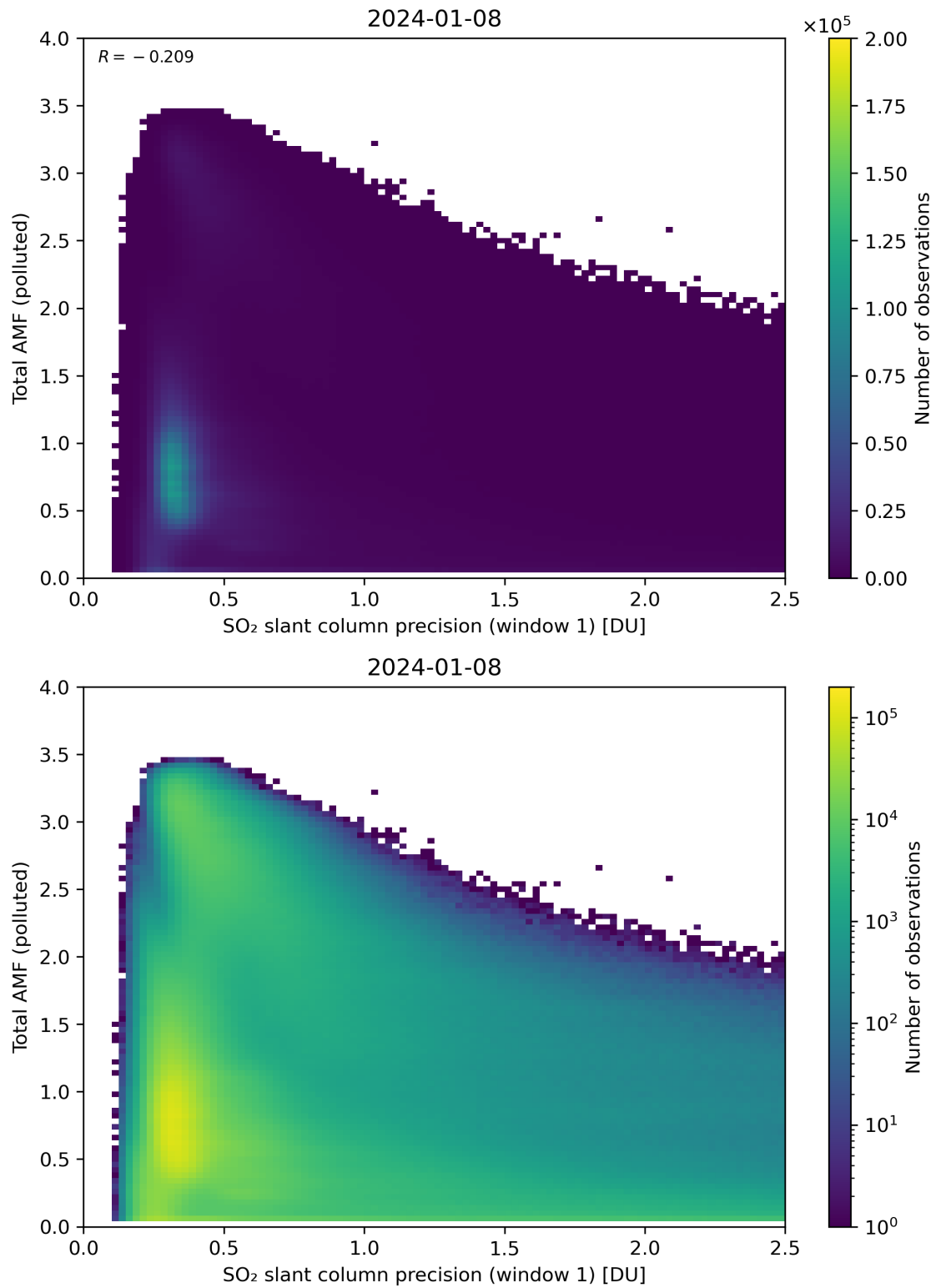
Figure 230: Scatter density plot of “SO 2 slant column precision (window 1)” against “Total AMF (polluted)” for 2024-01-07 to 2024-01-09.
