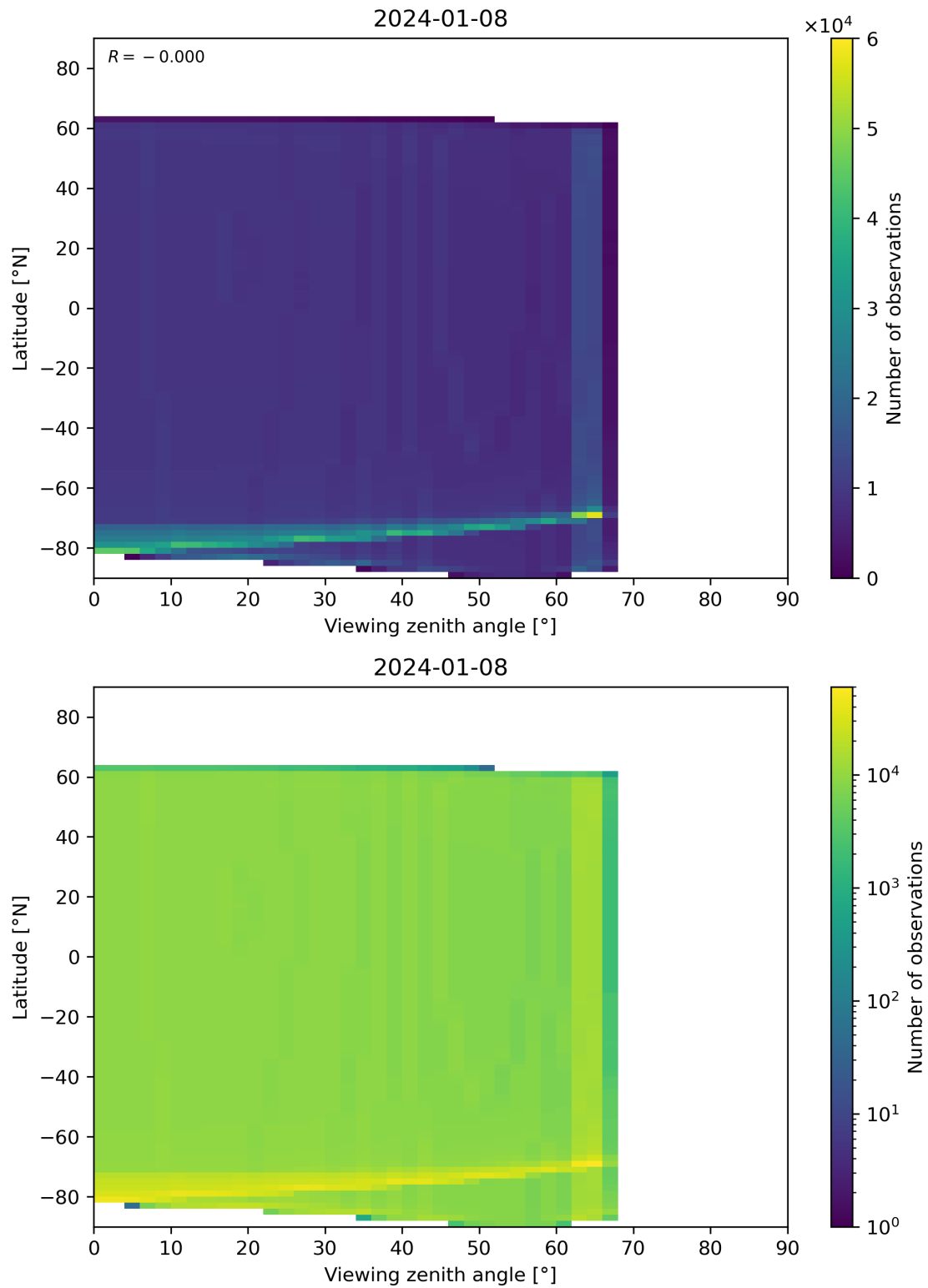
Figure 314: Scatter density plot of “Viewing zenith angle” against “Latitude” for 2024-01-07 to 2024-01-09.
