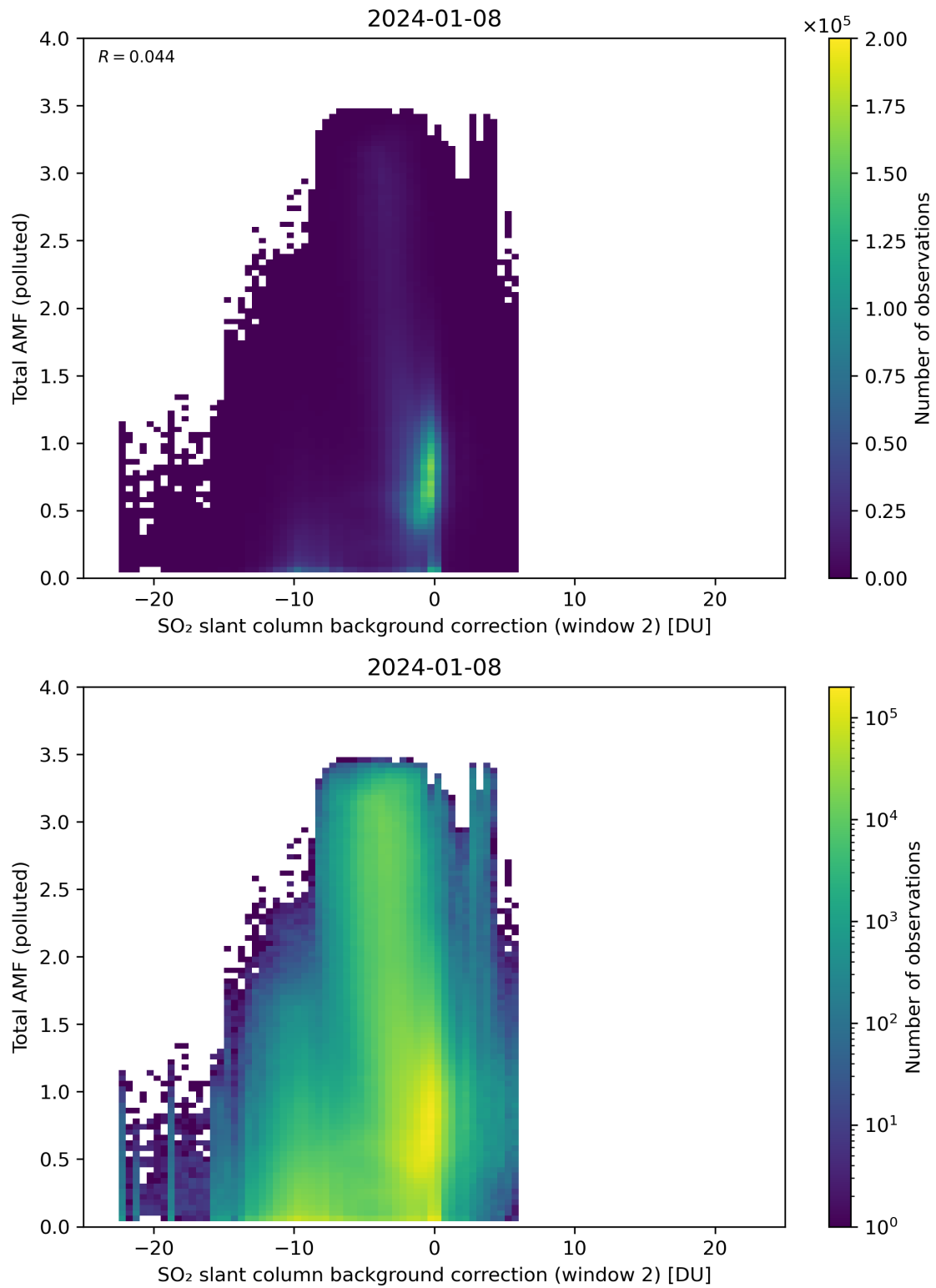
Figure 119: Scatter density plot of “SO 2 slant column background correction (window 2)” against “Total AMF (polluted)” for 2024-01-07 to 2024-01-09.
