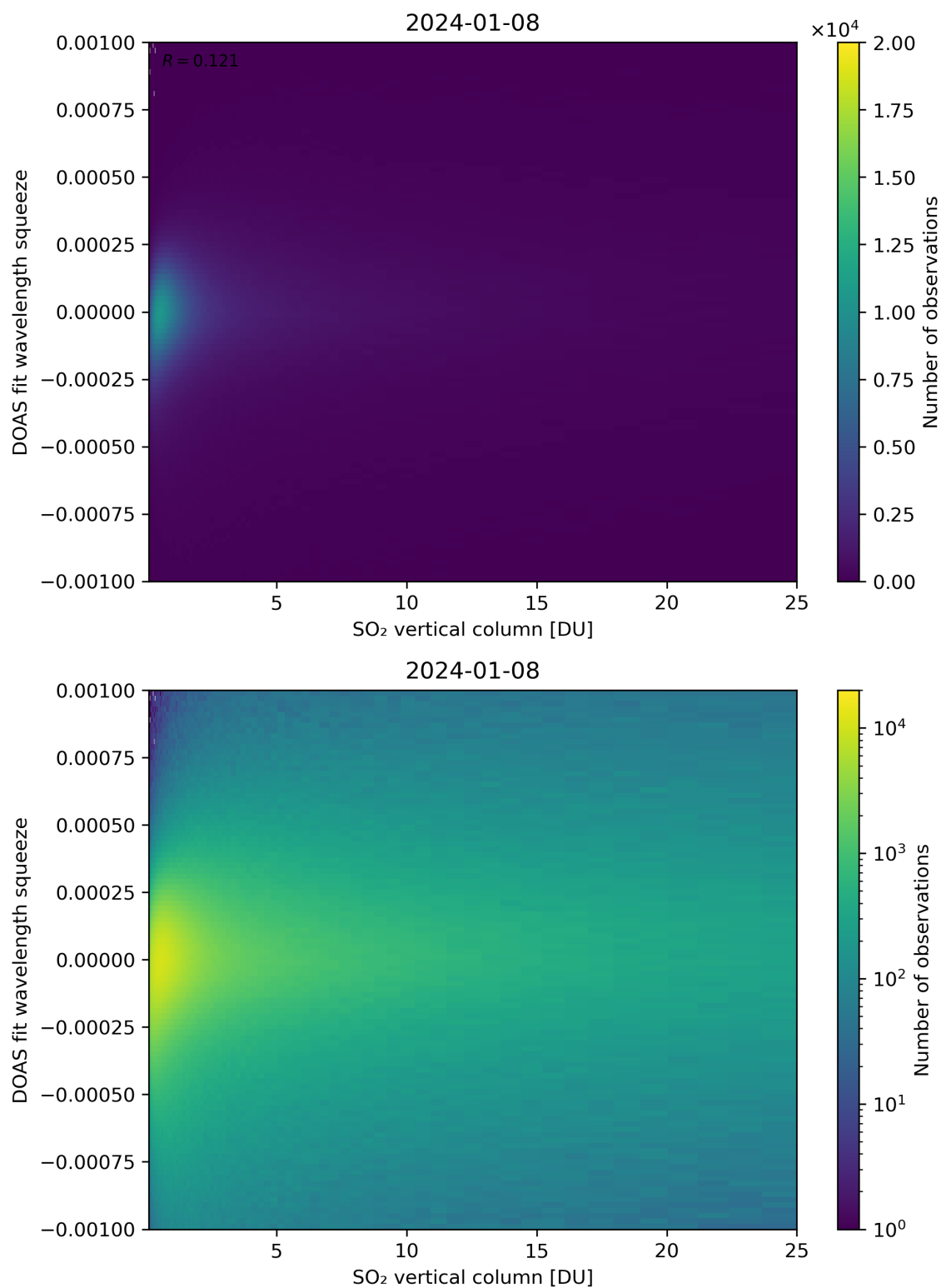
Figure 277: Scatter density plot of “SO 2 vertical column” against “DOAS fit wavelength squeeze” for 2024-01-07 to 2024-01-09.
