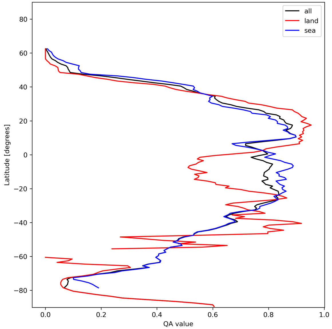
Figure 29: Zonal average of “QA value” for 2024-01-07 to 2024-01-09.
