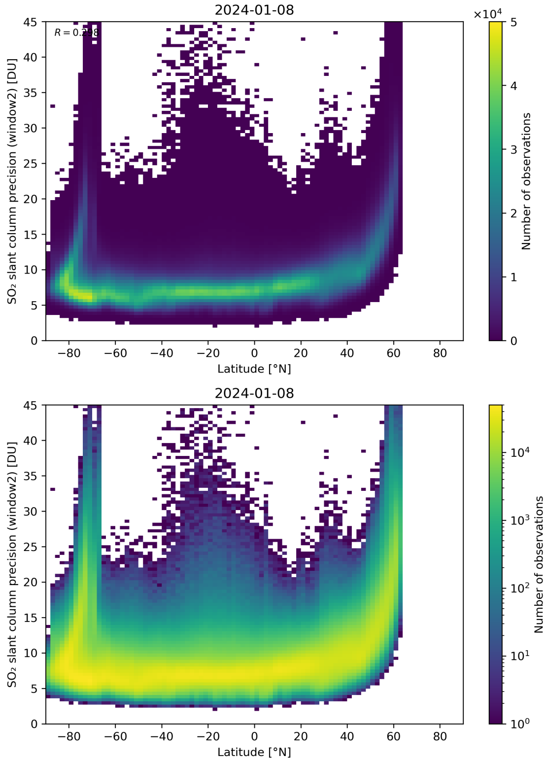
Figure 151: Scatter density plot of “Latitude” against “SO 2 slant column precision (window2)” for 2024-01-07 to 2024-01-09.
