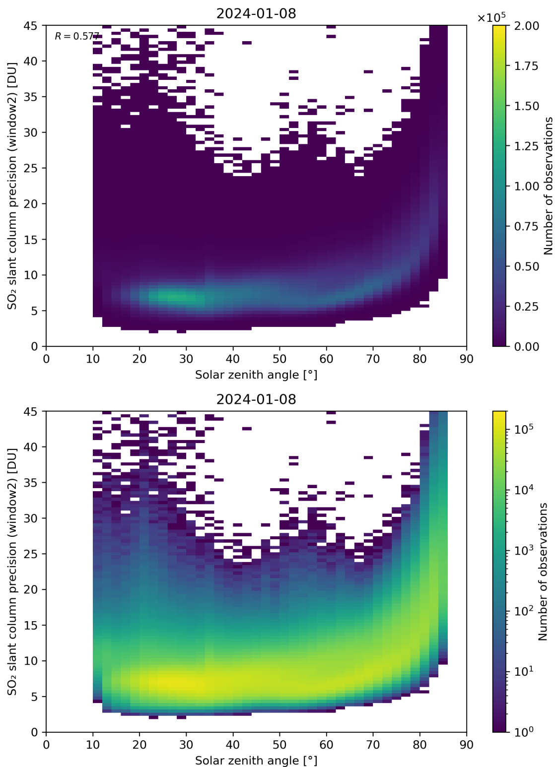
Figure 171: Scatter density plot of “Solar zenith angle” against “SO 2 slant column precision (window2)” for 2024-01-07 to 2024-01-09.
