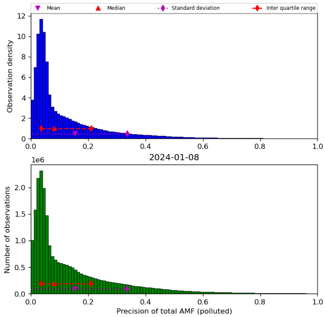
Figure 72: Histogram of “Precision of total AMF (polluted)” for 2024-01-07 to 2024-01-09
